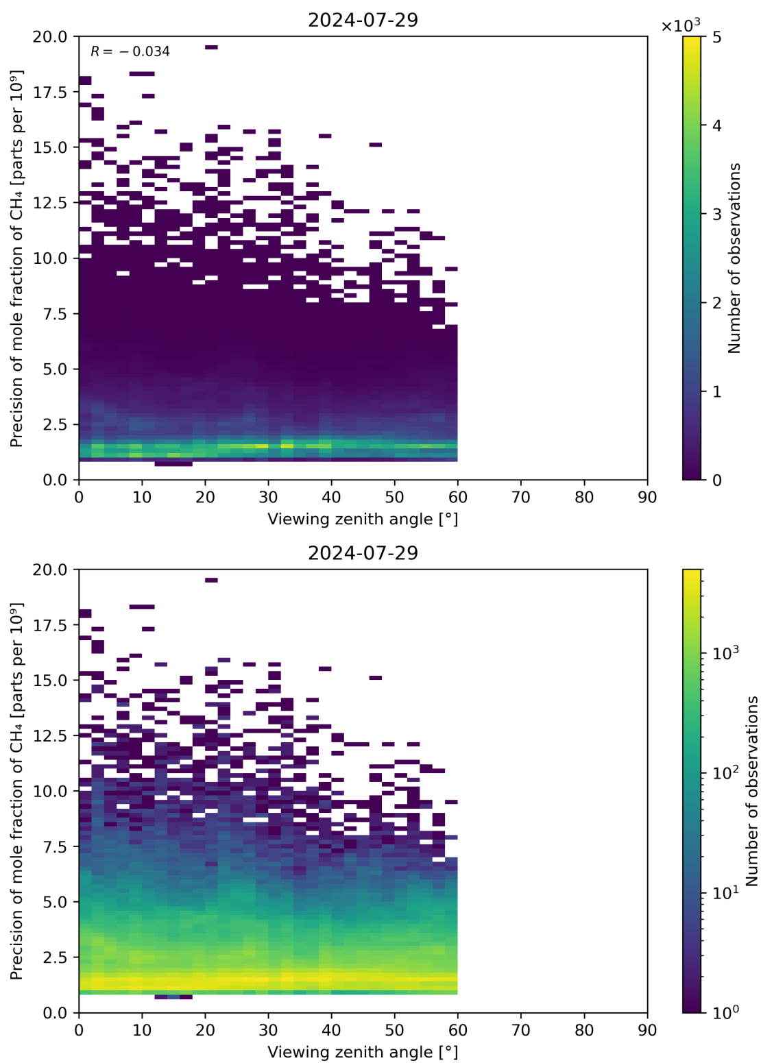
Figure 112: Scatter density plot of “Viewing zenith angle” against “Precision of mole fraction of CH 4 ” for 2024-07-28 to 2024-07-30.
