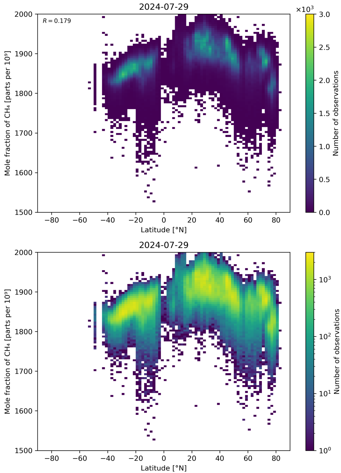
Figure 57: Scatter density plot of “Latitude” against “Mole fraction of \text{CH}_4 ” for 2024-07-28 to 2024-07-30.
