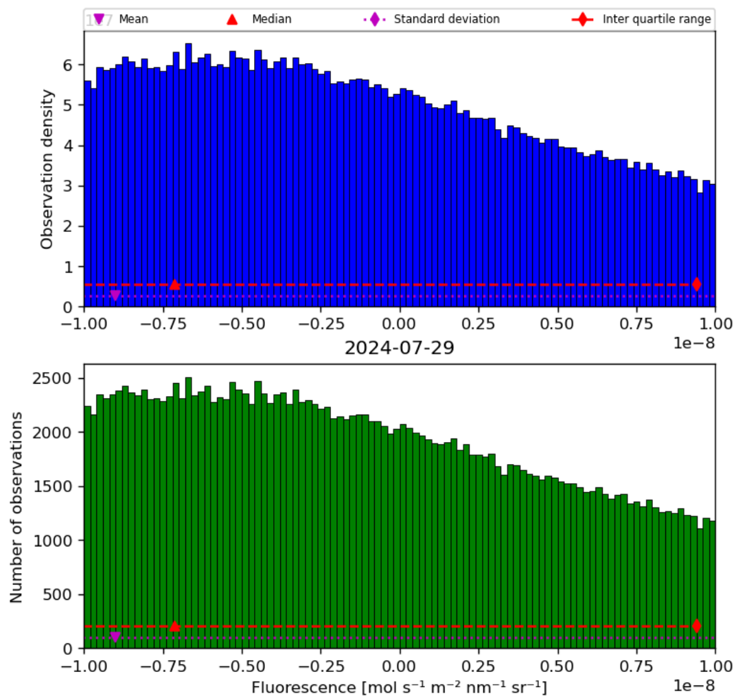
Figure 32: Histogram of “Fluorescence” for 2024-07-28 to 2024-07-30
