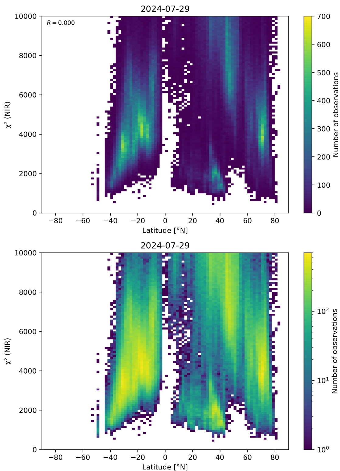
Figure 53: Scatter density plot of “Latitude” against “ \chi^2 (NIR)” for 2024-07-28 to 2024-07-30.
