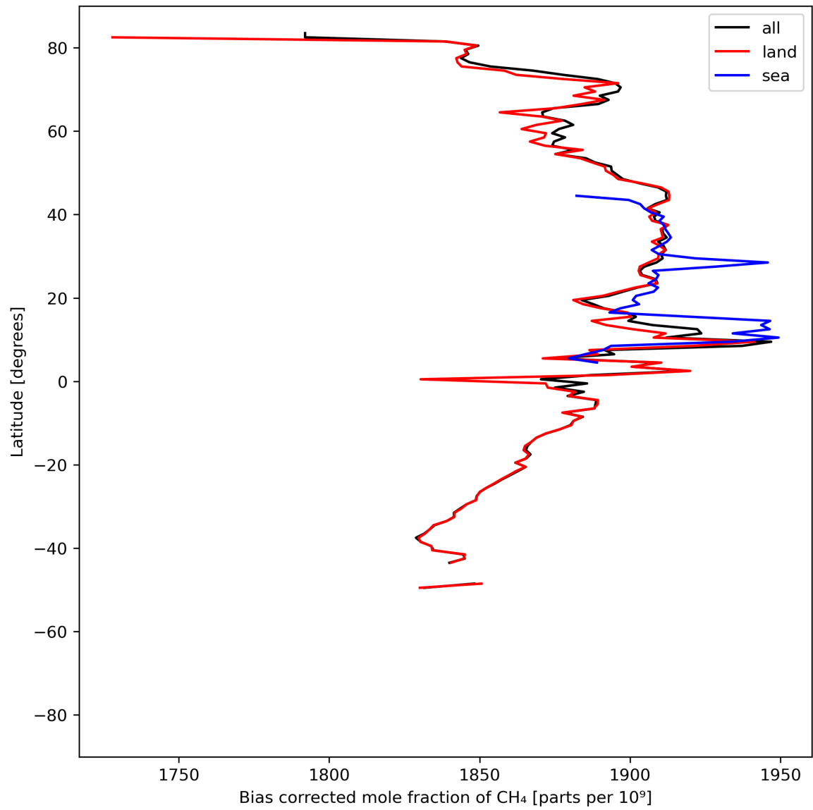
Figure 14: Zonal average of “Bias corrected mole fraction of CH 4 ” for 2024-07-28 to 2024-07-30.
