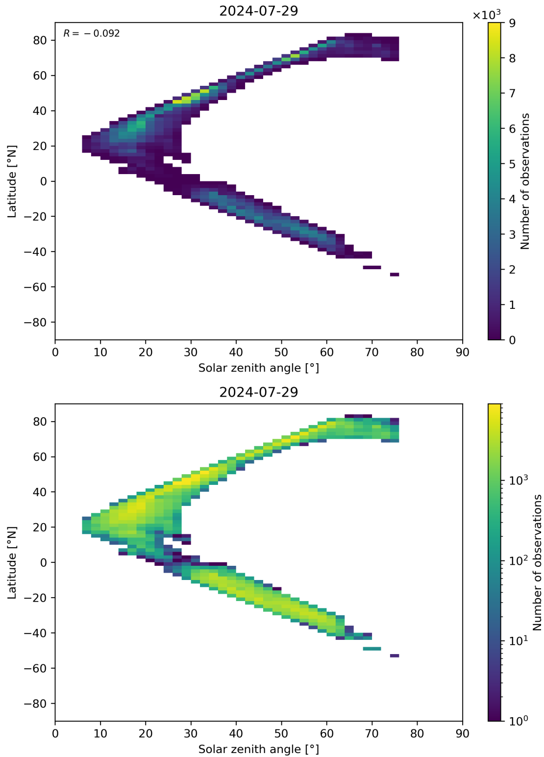
Figure 98: Scatter density plot of “Solar zenith angle” against “Latitude” for 2024-07-28 to 2024-07-30.
