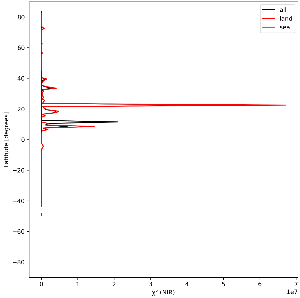
Figure 18: Zonal average of “ \chi^2 (NIR)” for 2024-07-28 to 2024-07-30.
