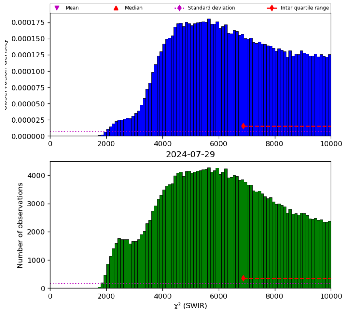
Figure 28: Histogram of “ \chi^2 (SWIR)” for 2024-07-28 to 2024-07-30
