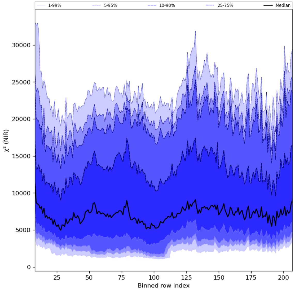
Figure 40: Along track statistics of “ \chi^2 (NIR)” for 2024-07-28 to 2024-07-30
