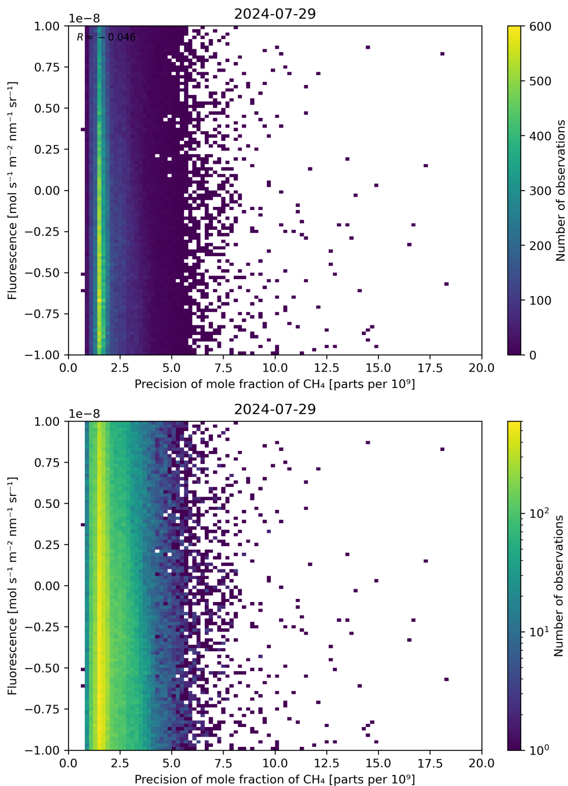
Figure 81: Scatter density plot of “Precision of mole fraction of \text{CH}_4 ” against “Fluorescence” for 2024-07-28 to 2024-07-30.
