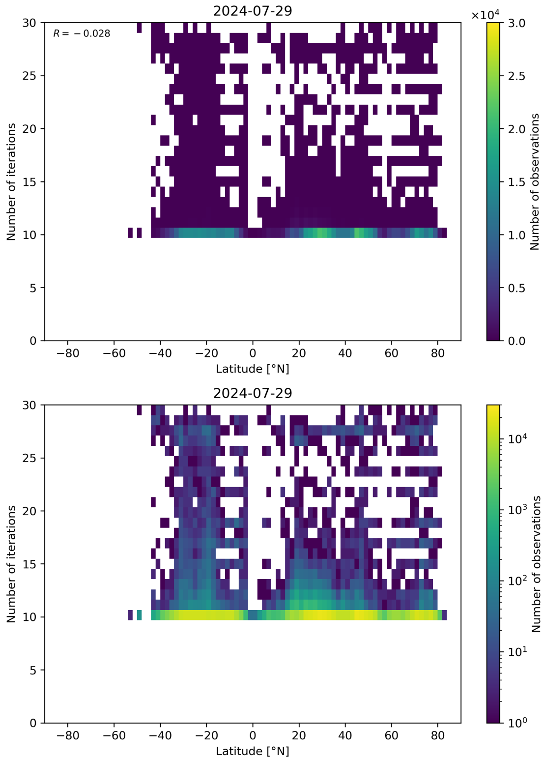
Figure 60: Scatter density plot of “Latitude” against “Number of iterations” for 2024-07-28 to 2024-07-30.
