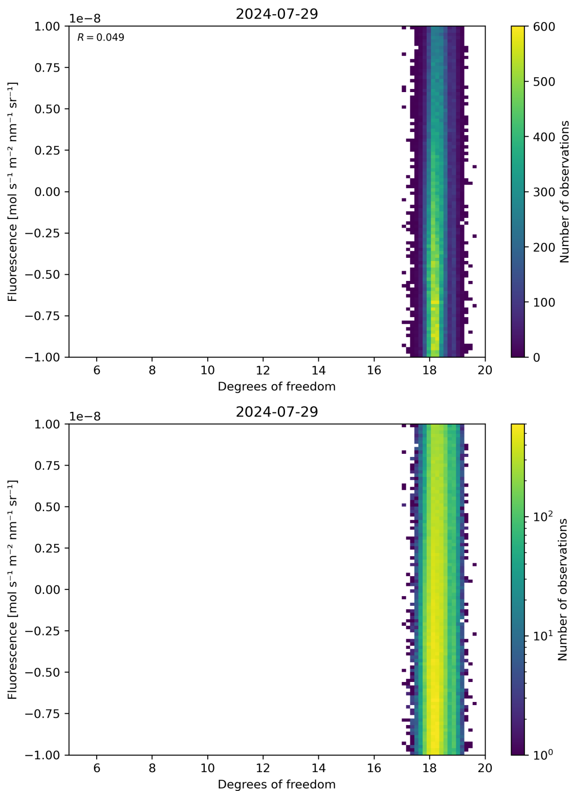
Figure 51: Scatter density plot of “Degrees of freedom” against “Fluorescence” for 2024-07-28 to 2024-07-30.
