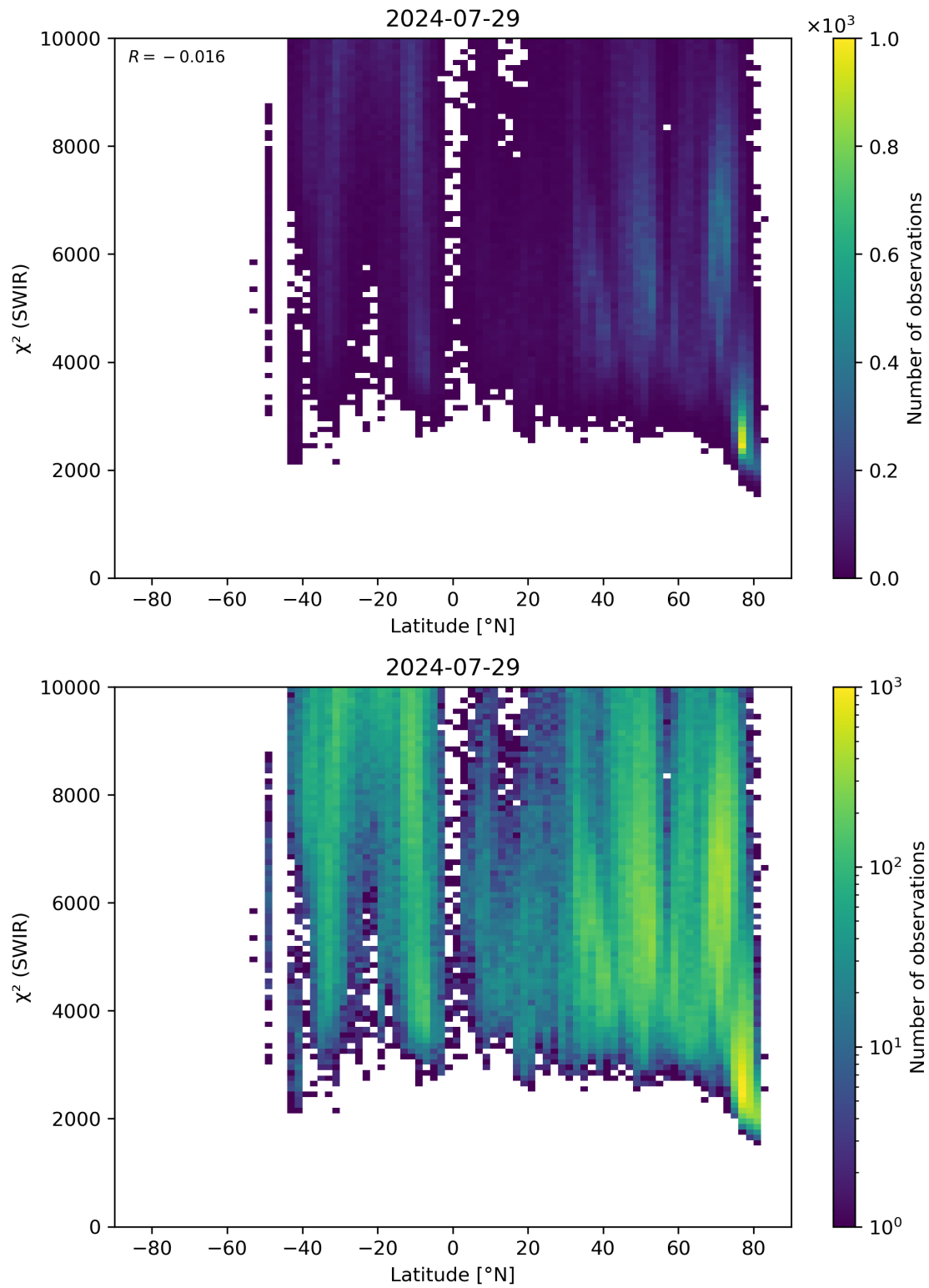
Figure 54: Scatter density plot of “Latitude” against “ \chi^2 (SWIR)” for 2024-07-28 to 2024-07-30.
