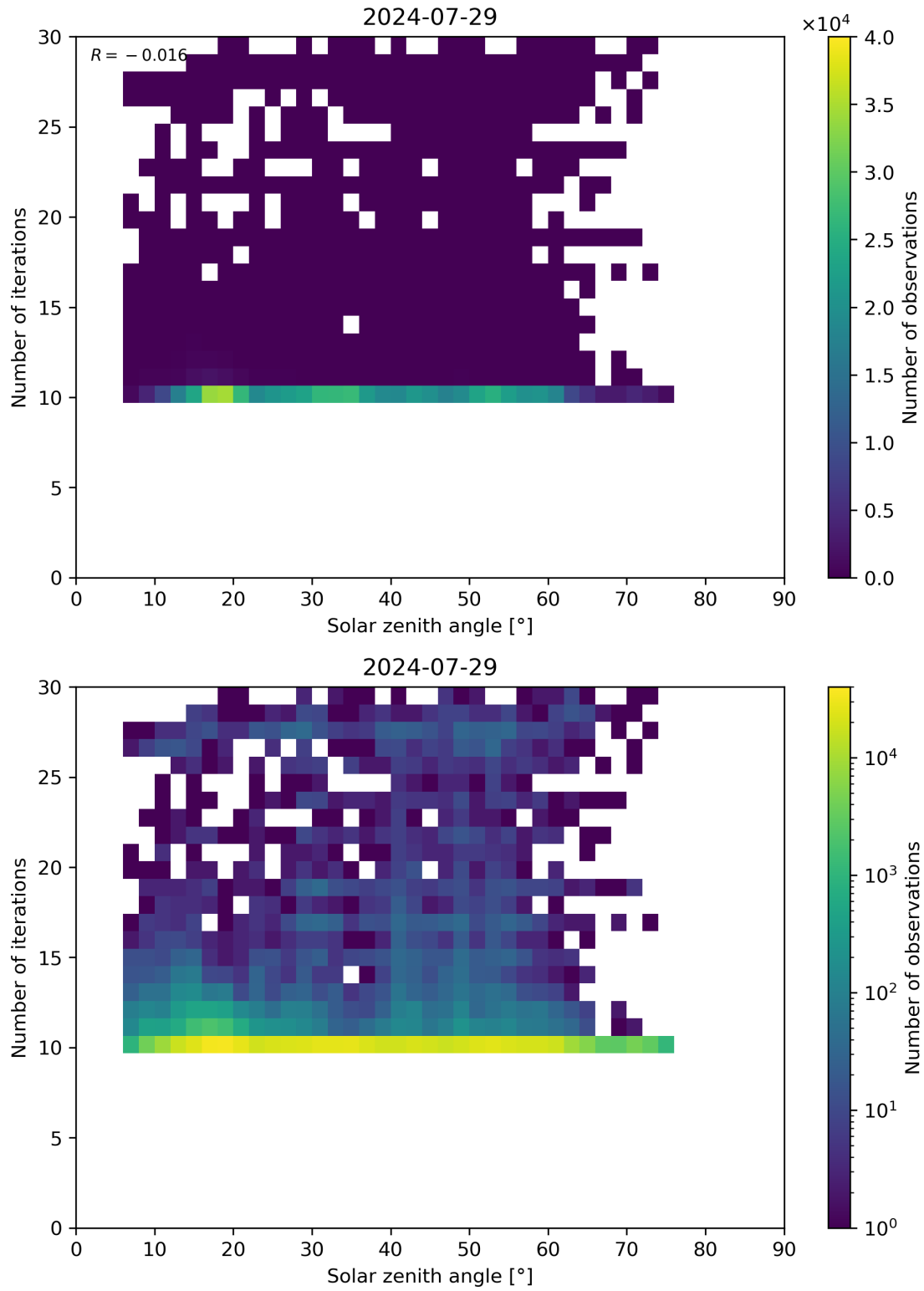
Figure 102: Scatter density plot of “Solar zenith angle” against “Number of iterations” for 2024-07-28 to 2024-07-30.
