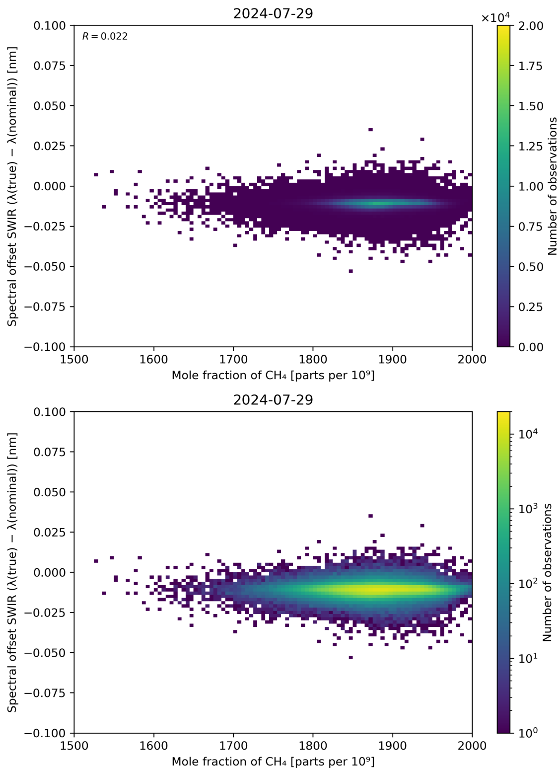
Figure 86: Scatter density plot of “Mole fraction of CH 4 ” against “Spectral offset SWIR ( \lambda(\text{true}) - \lambda(\text{nominal}) )” for 2024-07-28 to 2024-07-30.
