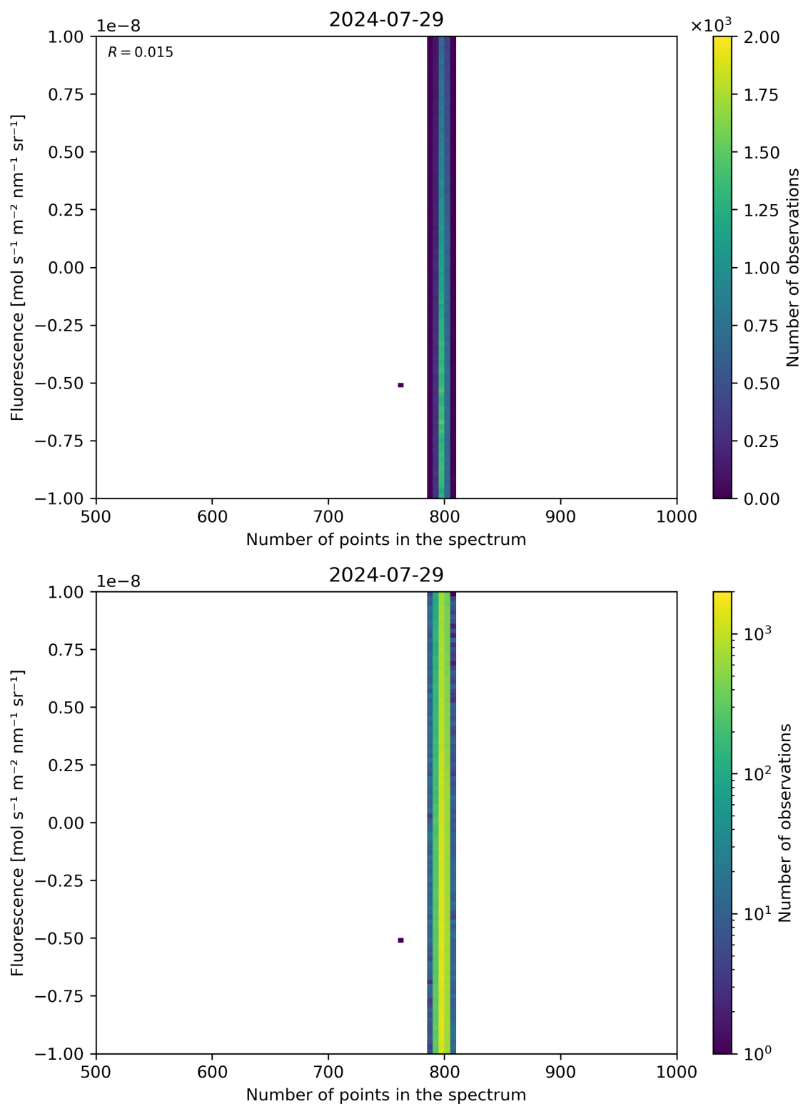
Figure 91: Scatter density plot of “Number of points in the spectrum” against “Fluorescence” for 2024-07-28 to 2024-07-30.
