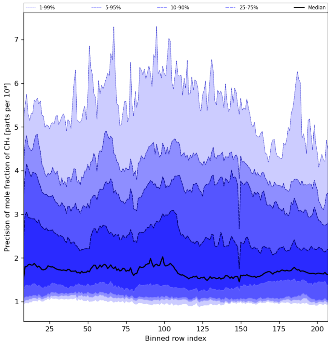
Figure 35: Along track statistics of “Precision of mole fraction of CH 4 ” for 2024-07-28 to 2024-07-30
