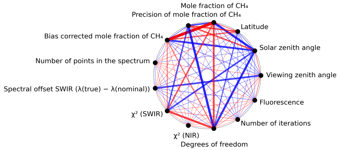
Figure 1: Map of correlation graph for 2024-07-28 to 2024-07-30.
