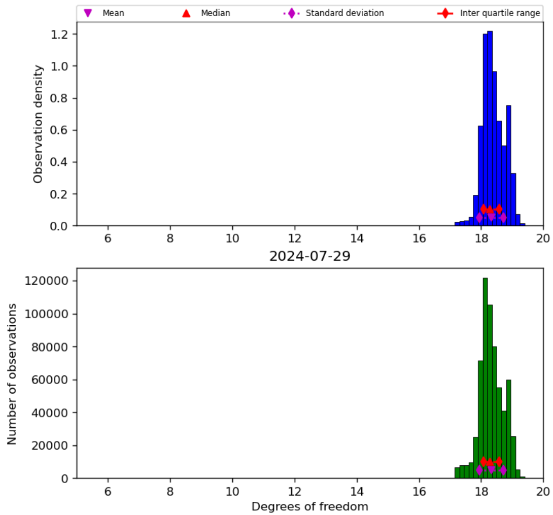
Figure 30: Histogram of “Degrees of freedom” for 2024-07-28 to 2024-07-30
