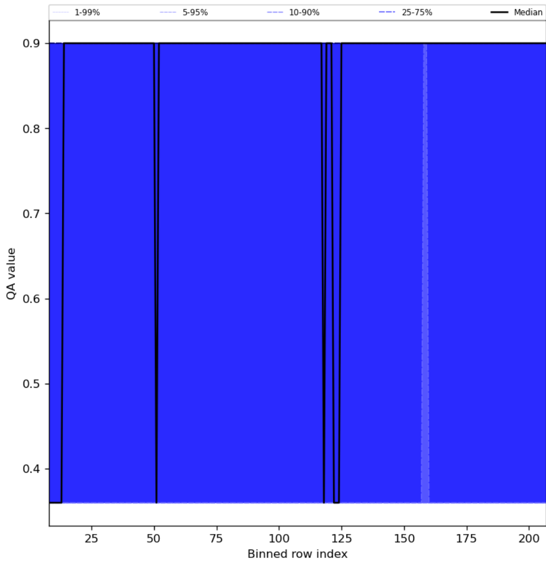
Figure 33: Along track statistics of “QA value” for 2024-07-28 to 2024-07-30
