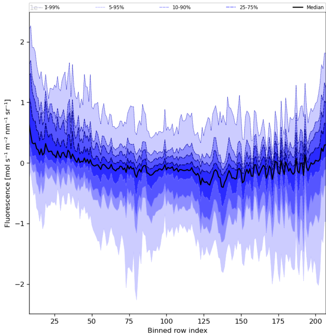
Figure 43: Along track statistics of “Fluorescence” for 2024-07-28 to 2024-07-30
