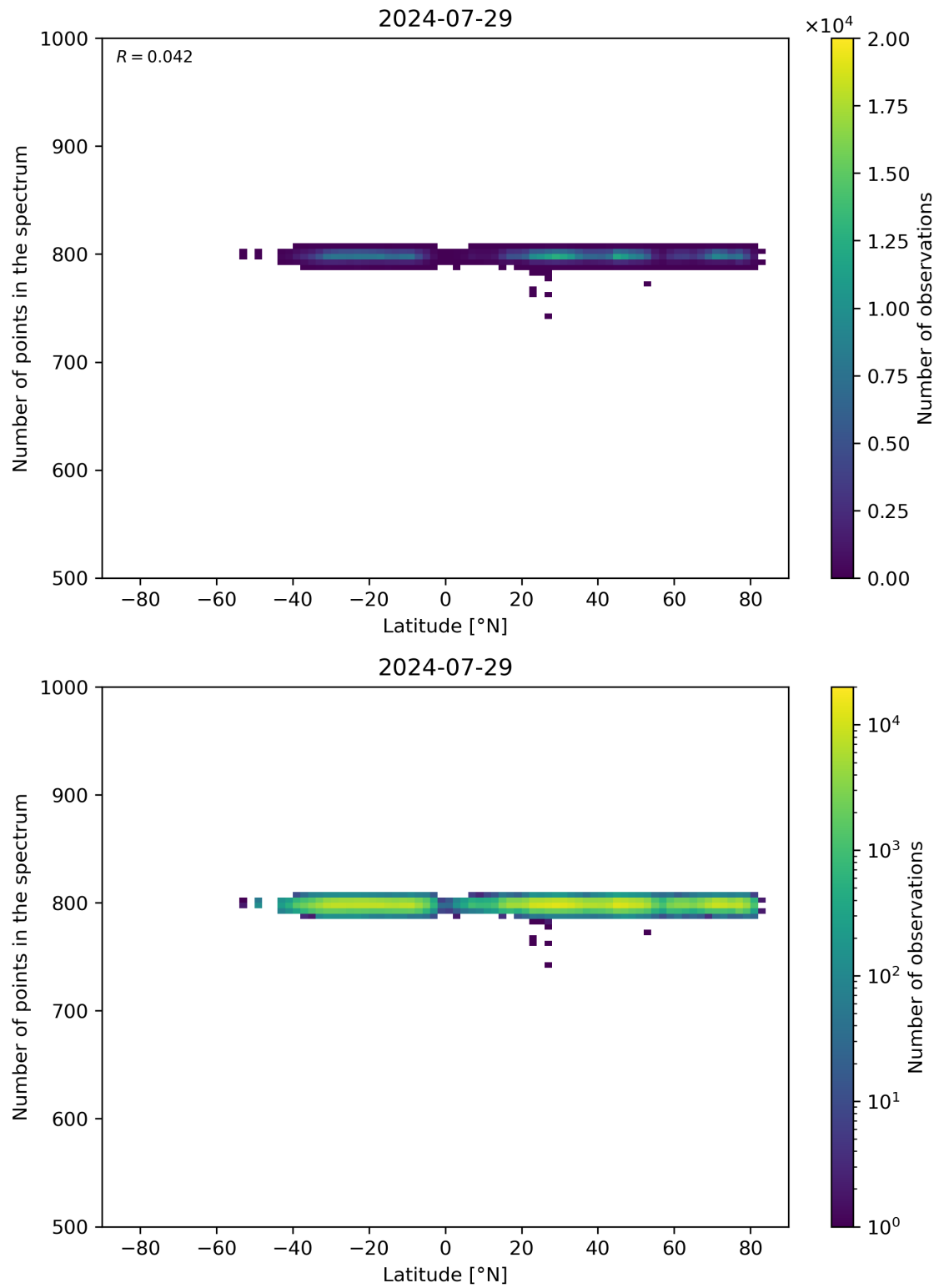
Figure 61: Scatter density plot of “Latitude” against “Number of points in the spectrum” for 2024-07-28 to 2024-07-30.
