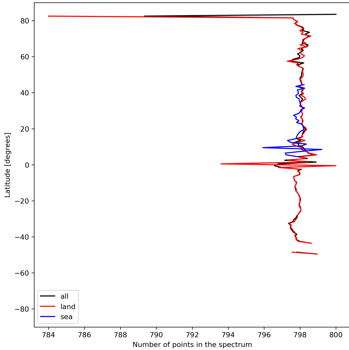
Figure 15: Zonal average of “Number of points in the spectrum” for 2024-07-28 to 2024-07-30.
