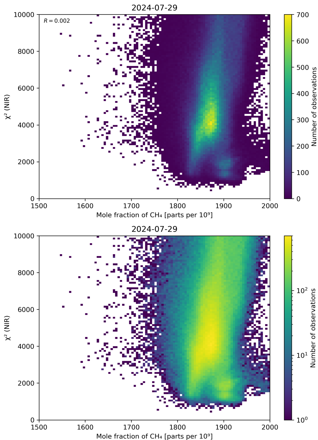
Figure 70: Scatter density plot of “Mole fraction of CH 4 ” against “ \chi^2 (NIR)” for 2024-07-28 to 2024-07-30.
