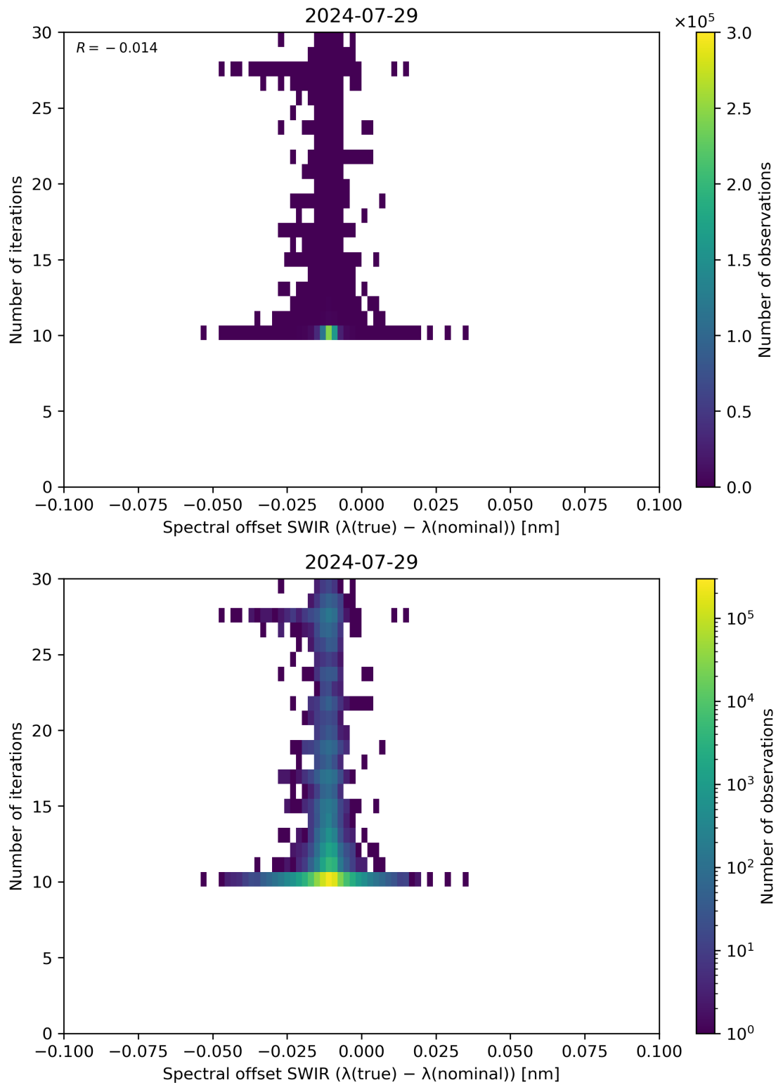
Figure 121: Scatter density plot of “Spectral offset SWIR ( \lambda(\text{true}) - \lambda(\text{nominal}) )” against “Number of iterations” for 2024-07-28 to 2024-07-30.
