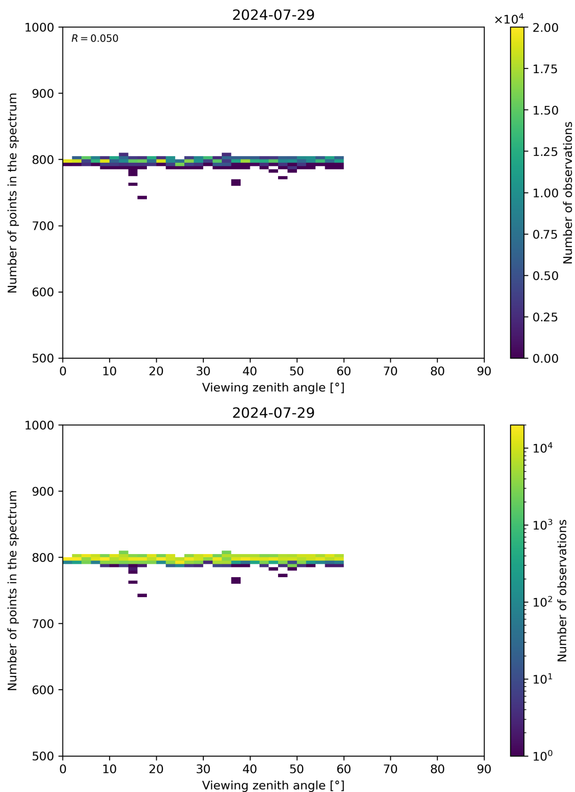
Figure 114: Scatter density plot of “Viewing zenith angle” against “Number of points in the spectrum” for 2024-07-28 to 2024-07-30.
