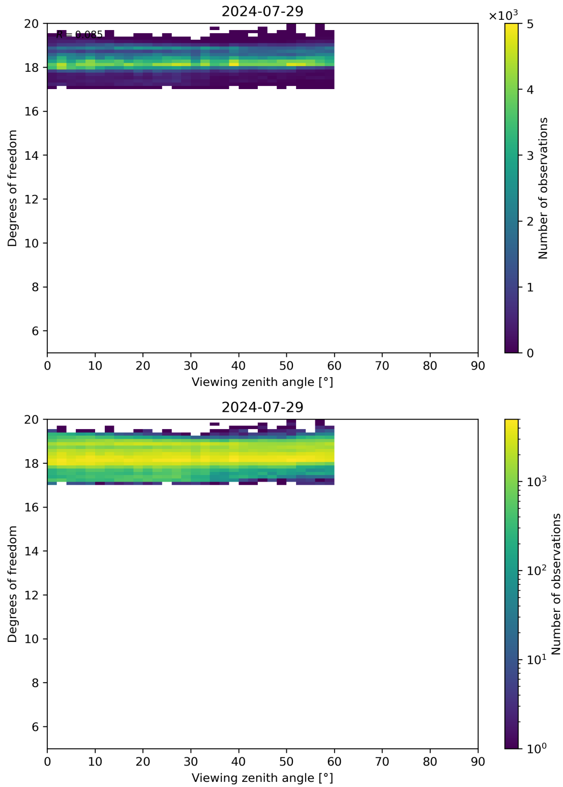
Figure 107: Scatter density plot of “Viewing zenith angle” against “Degrees of freedom” for 2024-07-28 to 2024-07-30.
