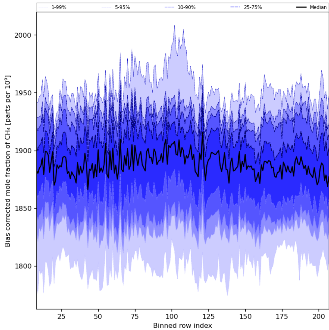
Figure 36: Along track statistics of “Bias corrected mole fraction of CH 4 ” for 2024-07-28 to 2024-07-30
