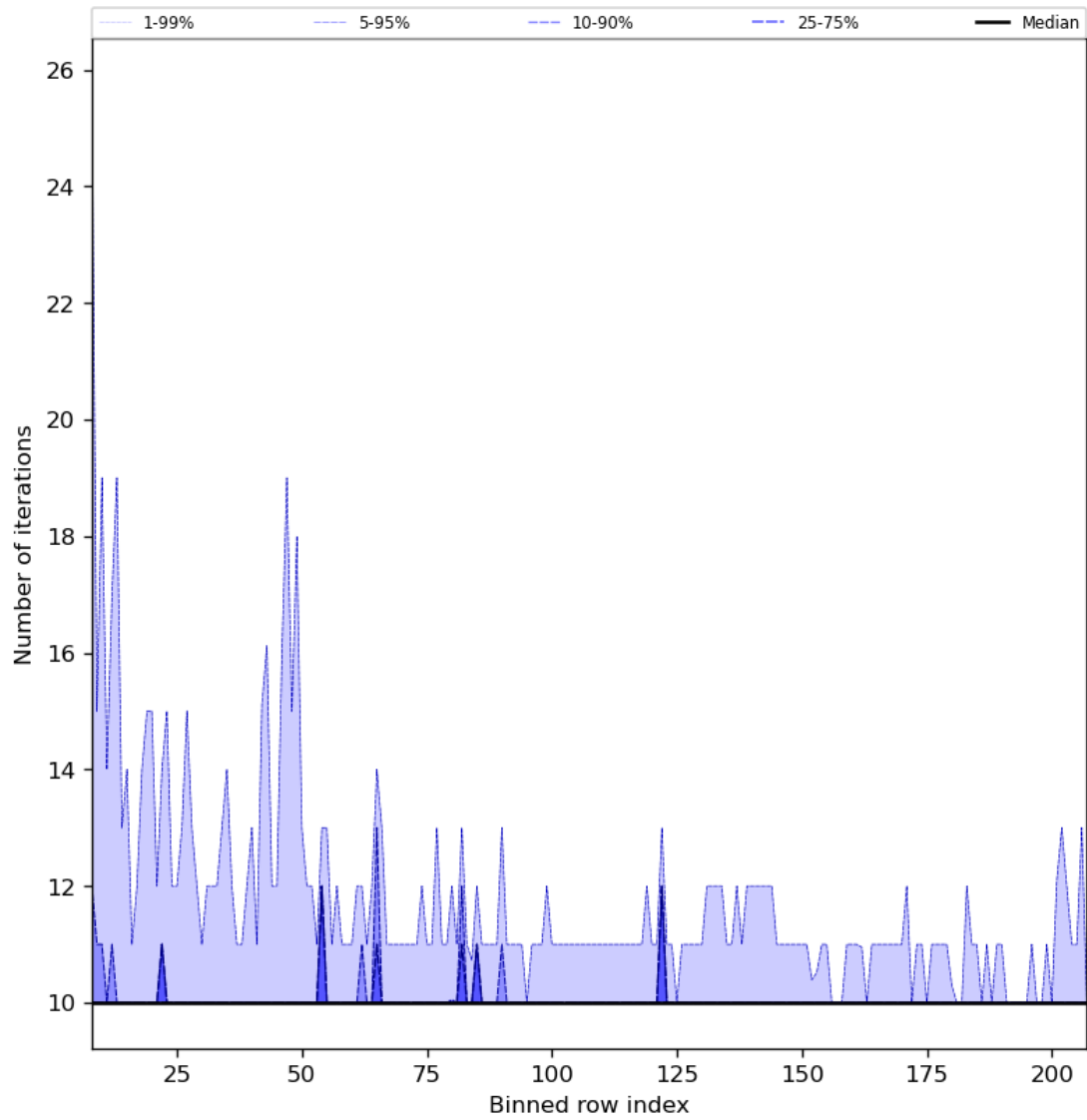
Figure 42: Along track statistics of “Number of iterations” for 2024-07-28 to 2024-07-30
