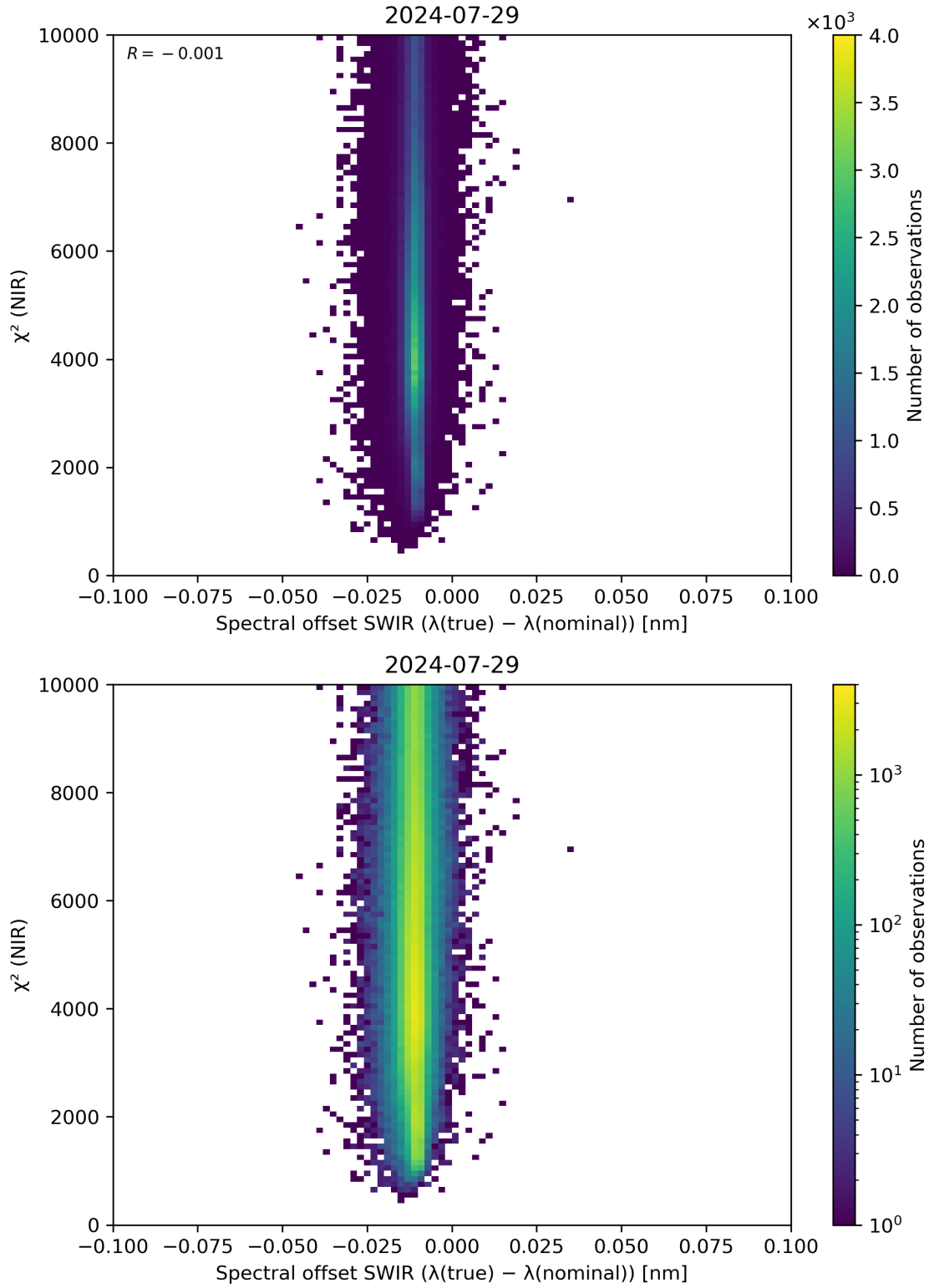
Figure 117: Scatter density plot of “Spectral offset SWIR ( \lambda(\text{true}) - \lambda(\text{nominal}) )” against “ \chi^2 (NIR)” for 2024-07-28 to 2024-07-30.
