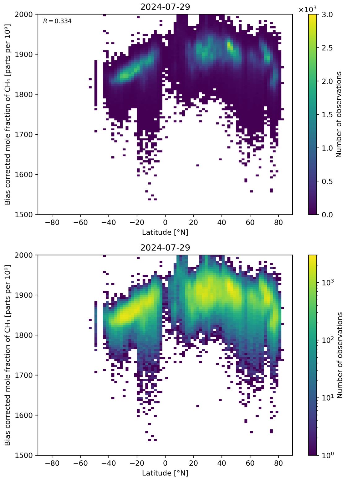
Figure 58: Scatter density plot of “Latitude” against “Bias corrected mole fraction of CH 4 ” for 2024-07-28 to 2024-07-30.
