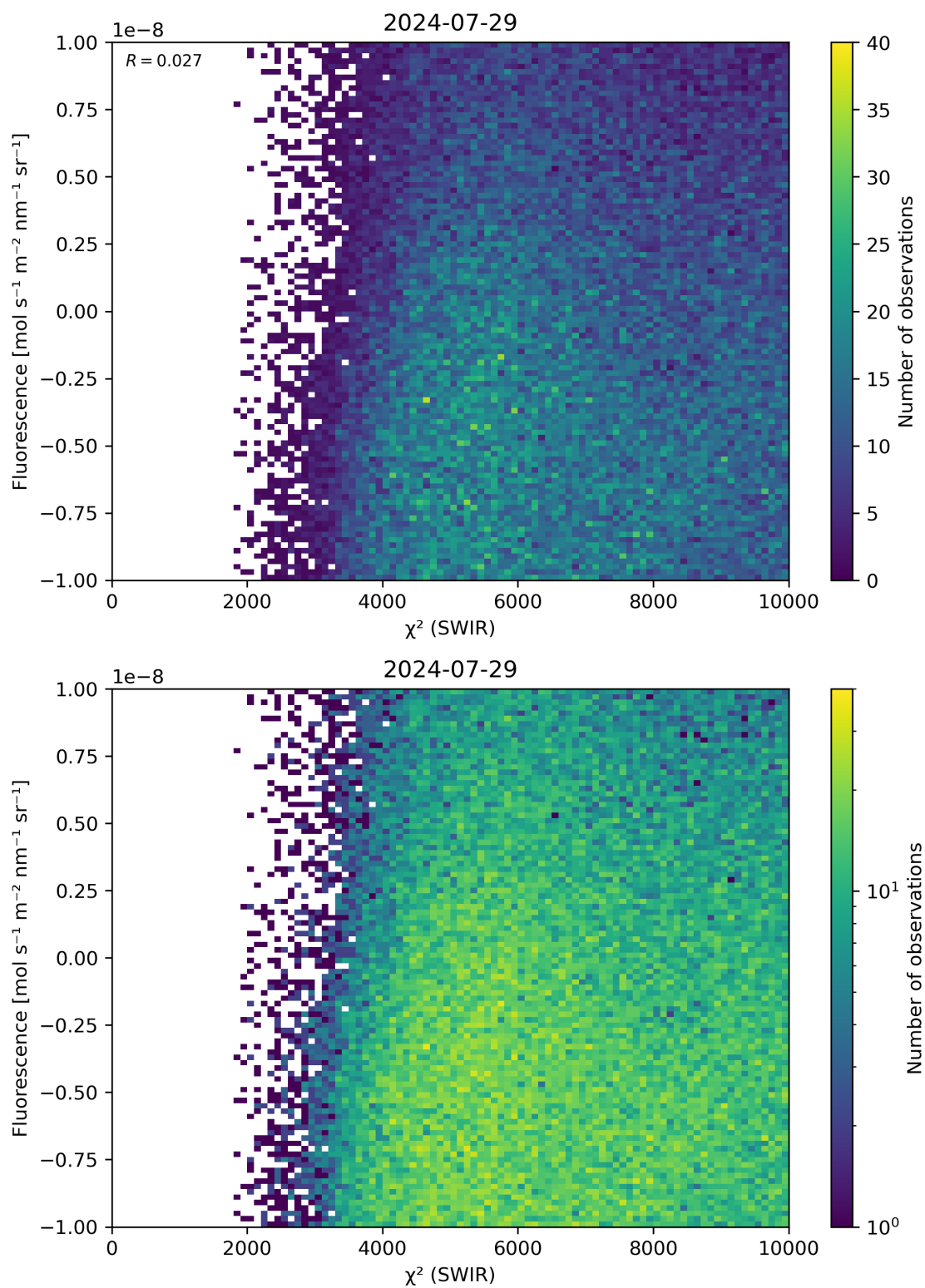
Figure 49: Scatter density plot of “ \chi^2 (SWIR)” against “Fluorescence” for 2024-07-28 to 2024-07-30.
