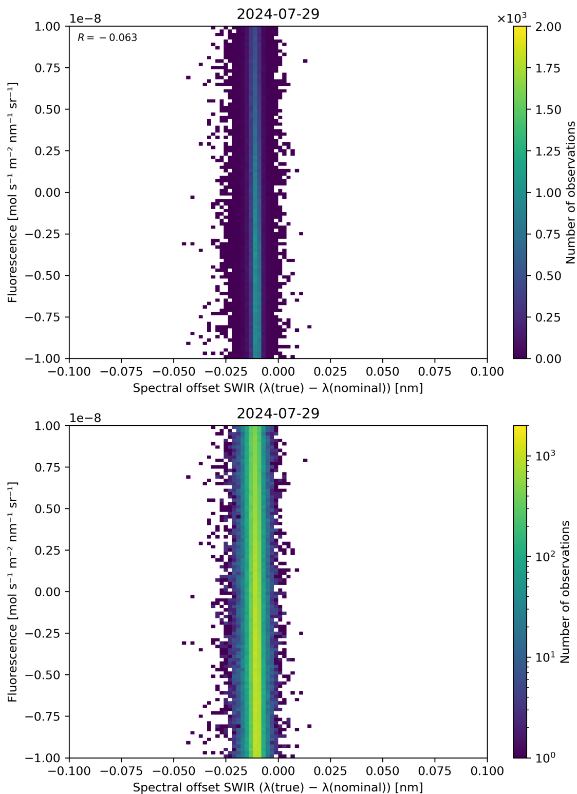
Figure 120: Scatter density plot of “Spectral offset SWIR ( \lambda(\text{true}) - \lambda(\text{nominal}) )” against “Fluorescence” for 2024-07-28 to 2024-07-30.
