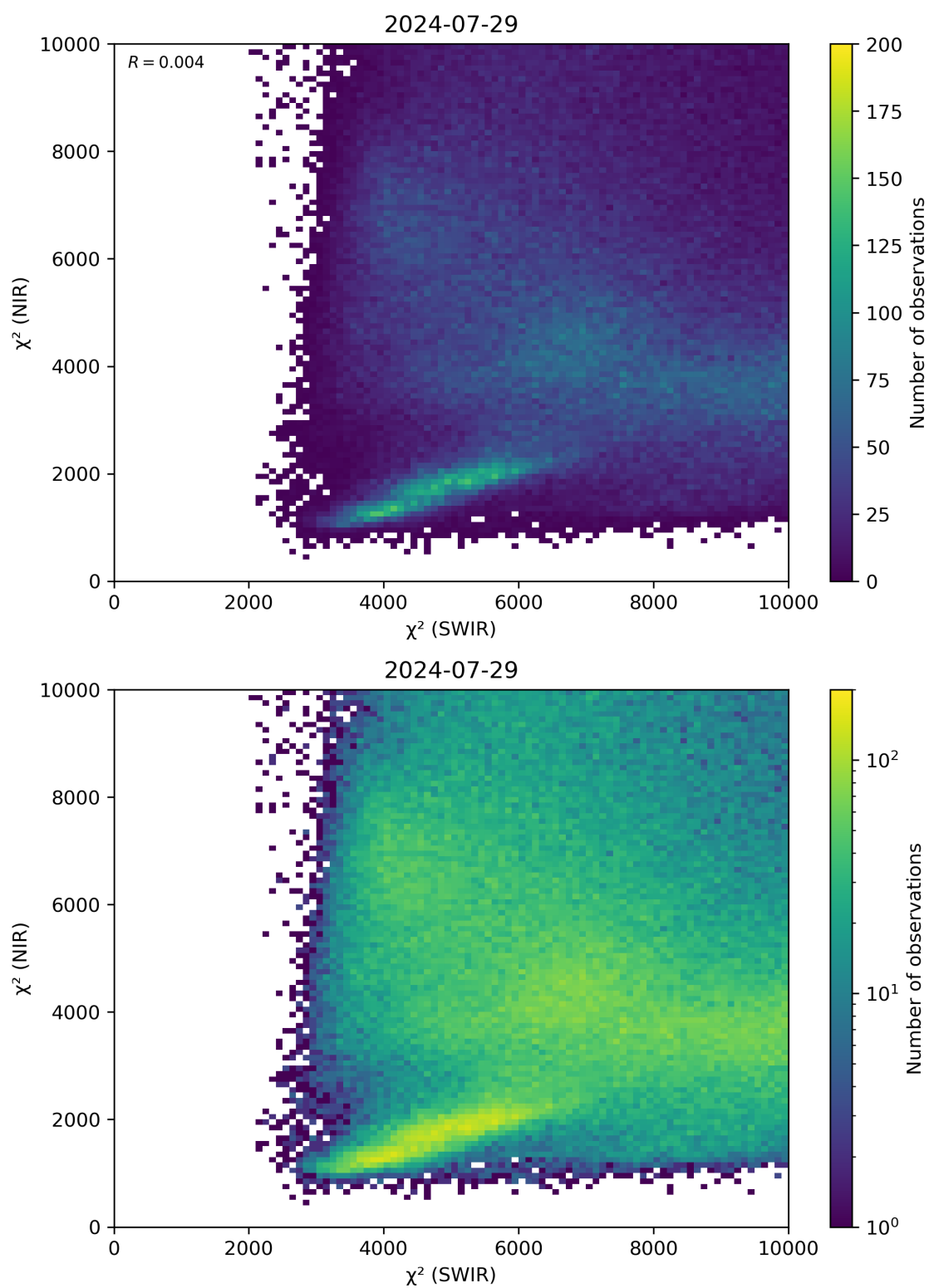
Figure 47: Scatter density plot of “ \chi^2 (SWIR)” against “ \chi^2 (NIR)” for 2024-07-28 to 2024-07-30.
