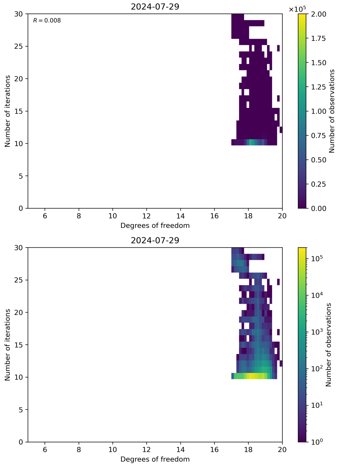
Figure 52: Scatter density plot of “Degrees of freedom” against “Number of iterations” for 2024-07-28 to 2024-07-30.
