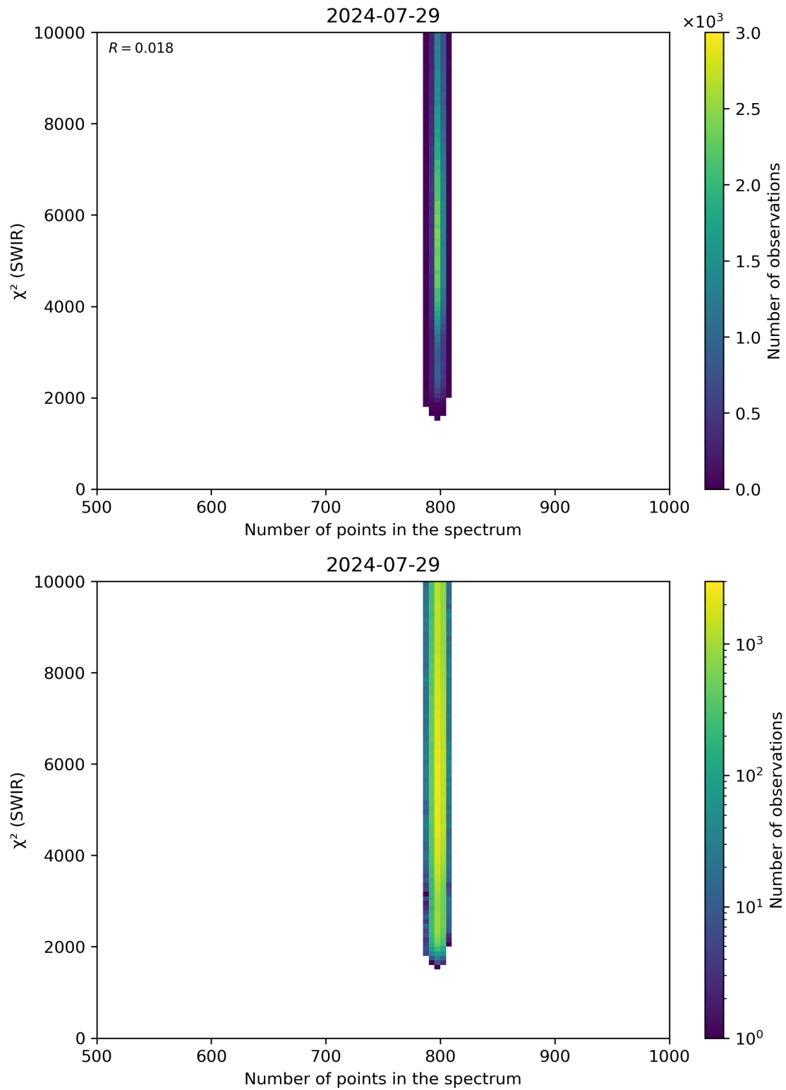
Figure 89: Scatter density plot of “Number of points in the spectrum” against “ \chi^2 (SWIR)” for 2024-07-28 to 2024-07-30.
