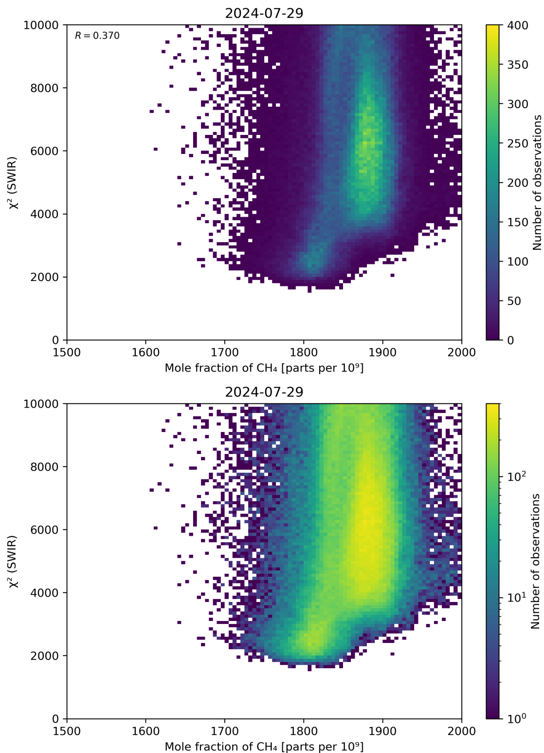
Figure 71: Scatter density plot of “Mole fraction of \text{CH}_4 ” against “ \chi^2 (SWIR)” for 2024-07-28 to 2024-07-30.
