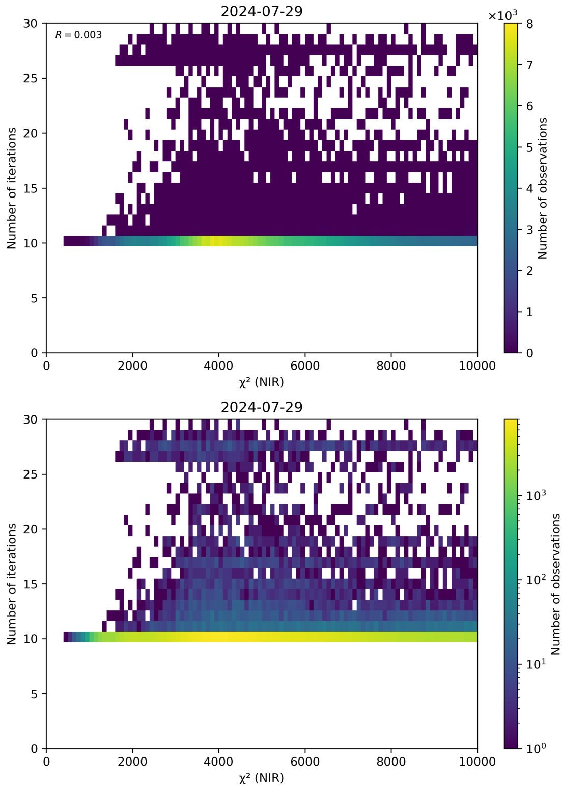
Figure 46: Scatter density plot of “ \chi^2 (NIR)” against “Number of iterations” for 2024-07-28 to 2024-07-30.
