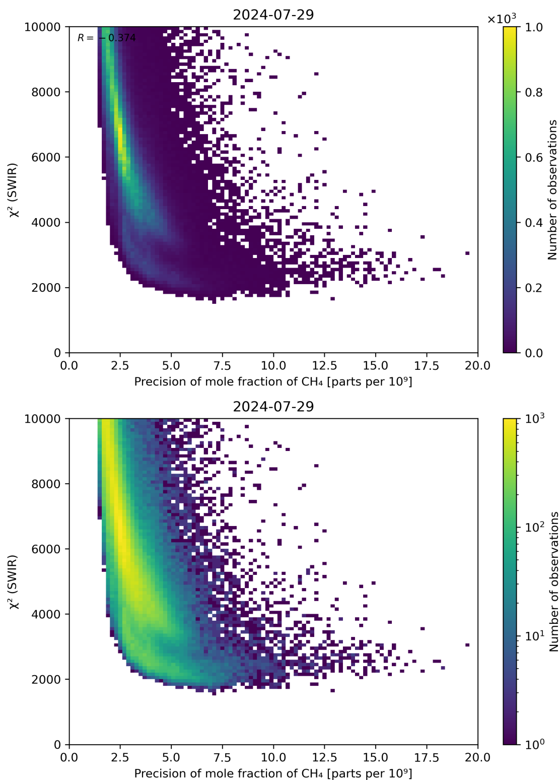
Figure 79: Scatter density plot of “Precision of mole fraction of \text{CH}_4 ” against “ \chi^2 (SWIR)” for 2024-07-28 to 2024-07-30.
