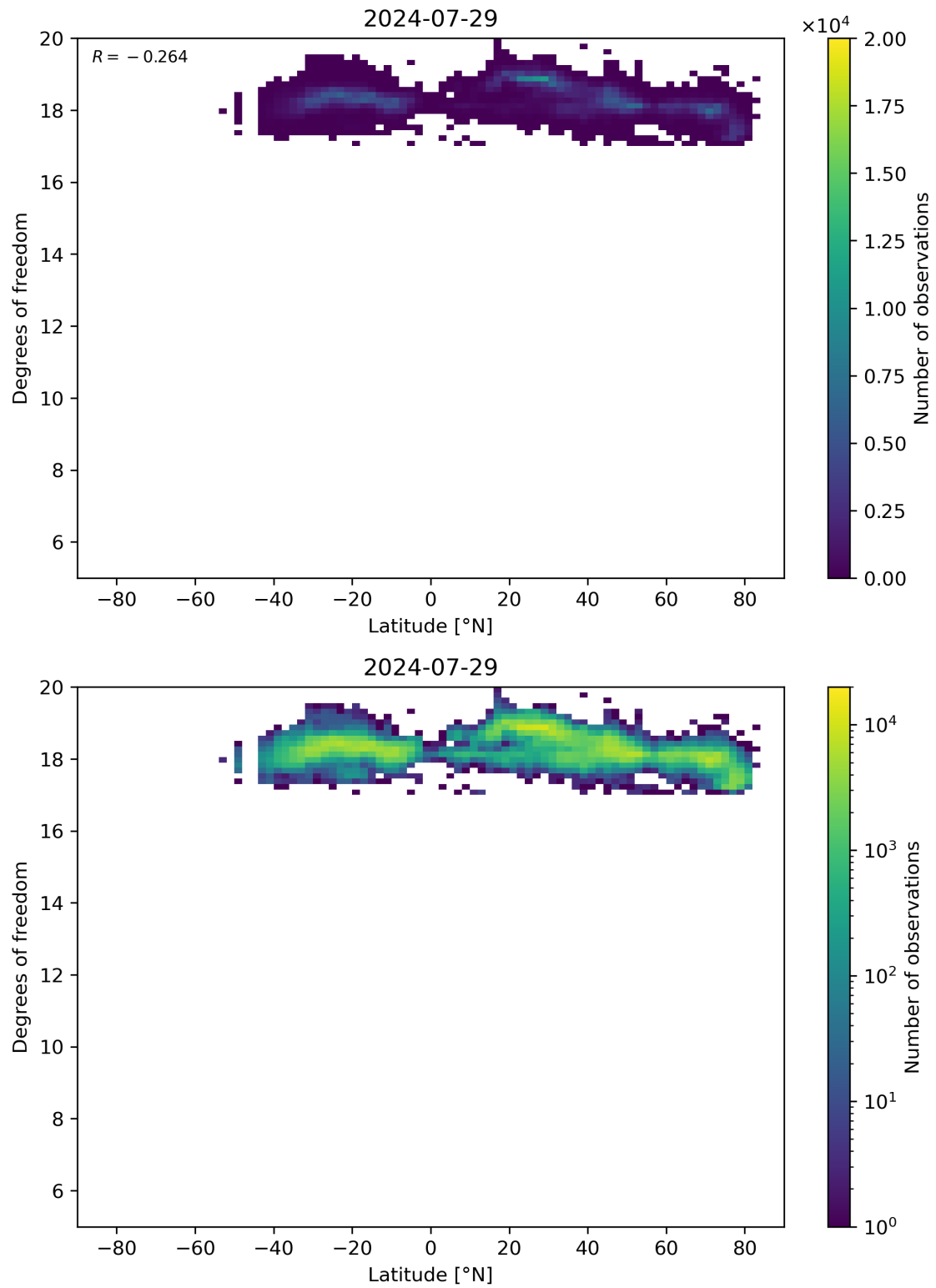
Figure 55: Scatter density plot of “Latitude” against “Degrees of freedom” for 2024-07-28 to 2024-07-30.
