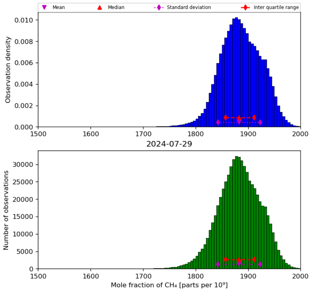
Figure 23: Histogram of "Mole fraction of CH 4 " for 2024-07-28 to 2024-07-30
