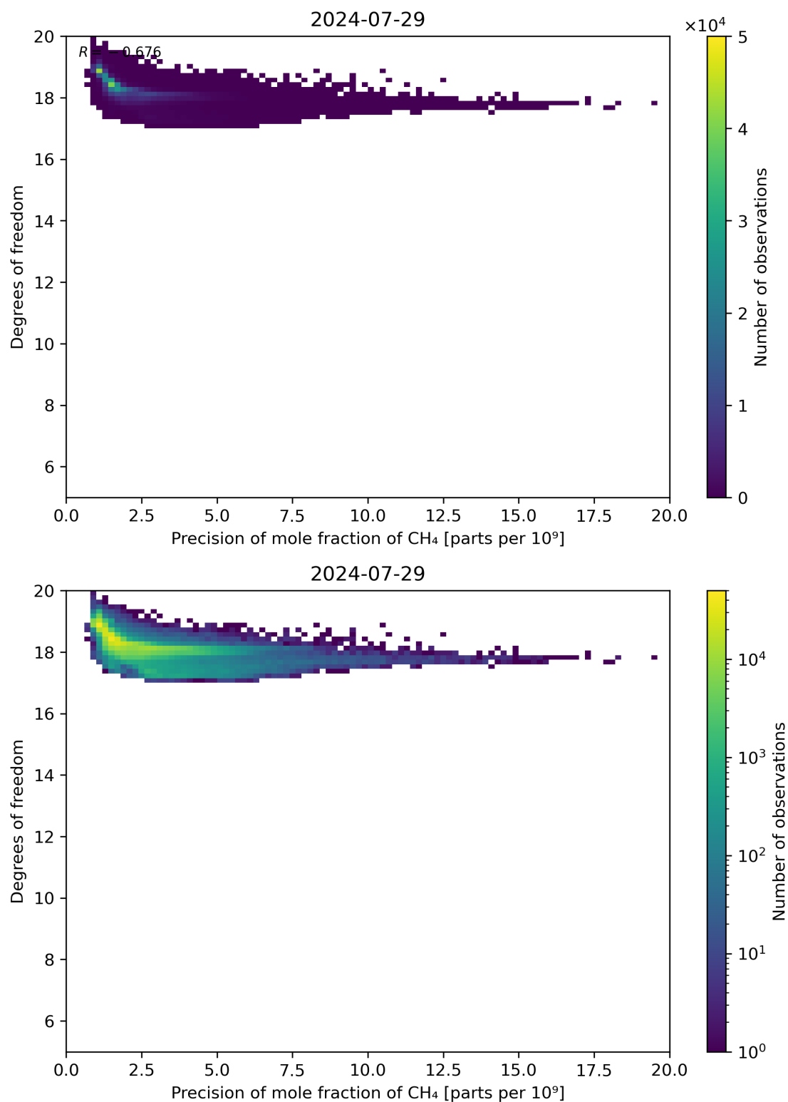
Figure 80: Scatter density plot of “Precision of mole fraction of CH 4 ” against “Degrees of freedom” for 2024-07-28 to 2024-07-30.
