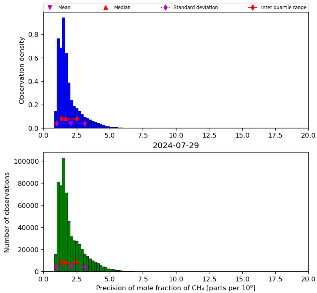
Figure 24: Histogram of “Precision of mole fraction of CH 4 ” for 2024-07-28 to 2024-07-30
