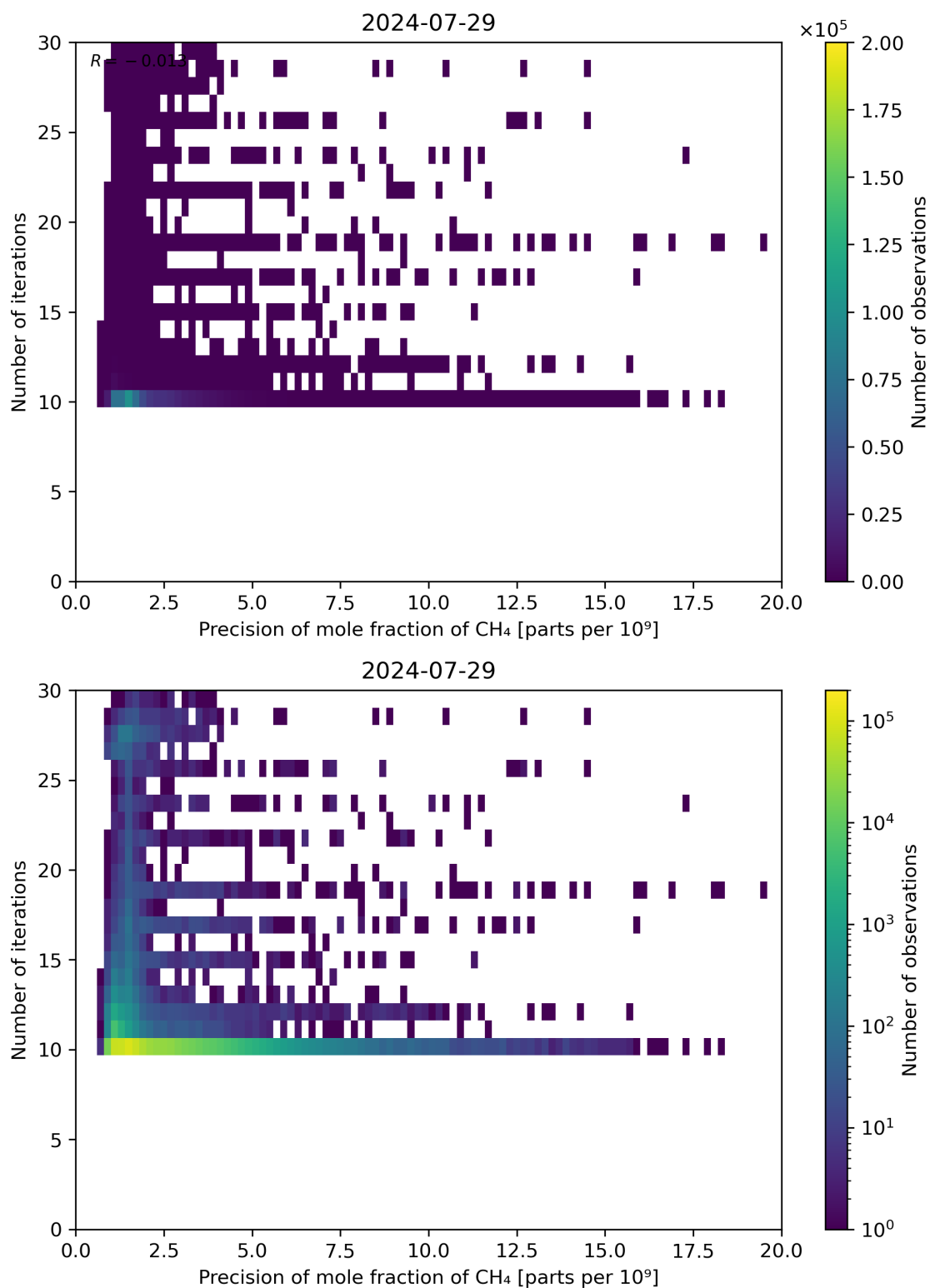
Figure 83: Scatter density plot of “Precision of mole fraction of CH 4 ” against “Number of iterations” for 2024-07-28 to 2024-07-30.
