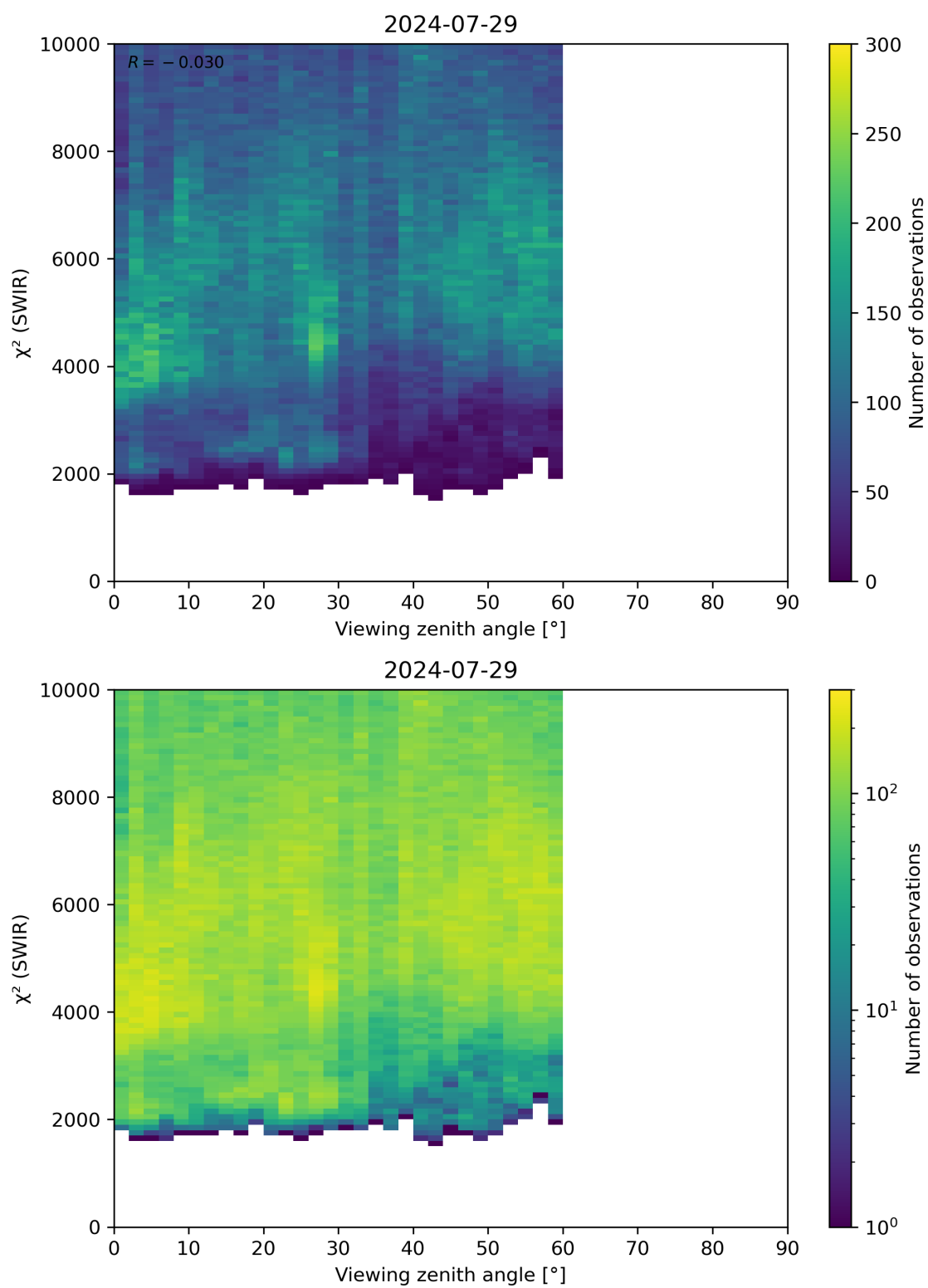
Figure 106: Scatter density plot of “Viewing zenith angle” against “ \chi^2 (SWIR)” for 2024-07-28 to 2024-07-30.
