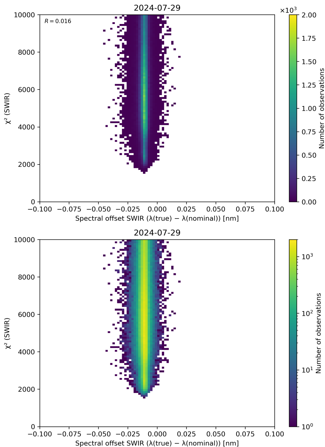
Figure 118: Scatter density plot of “Spectral offset SWIR ( \lambda(\text{true}) - \lambda(\text{nominal}) )” against “ \chi^2 (SWIR)” for 2024-07-28 to 2024-07-30.
