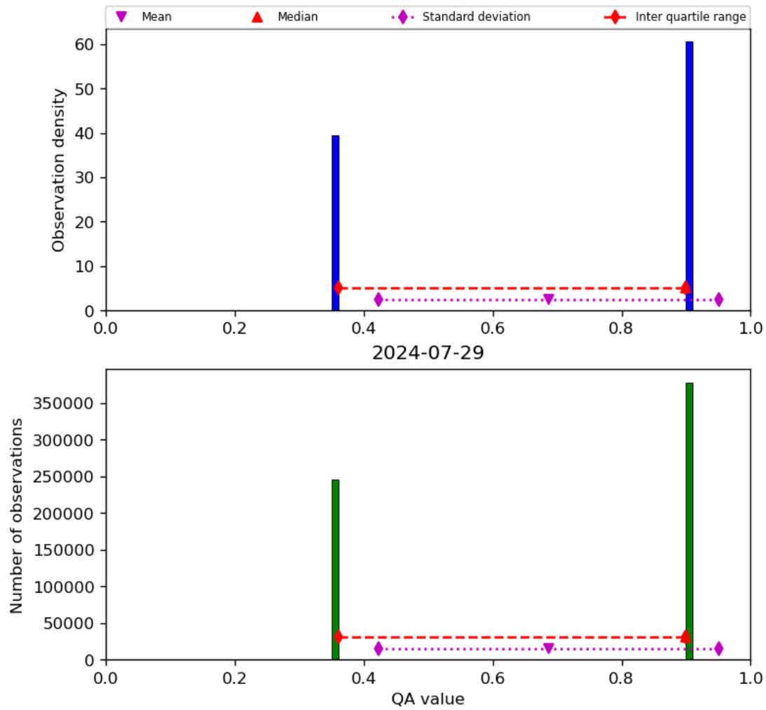
Figure 22: Histogram of “QA value” for 2024-07-28 to 2024-07-30
