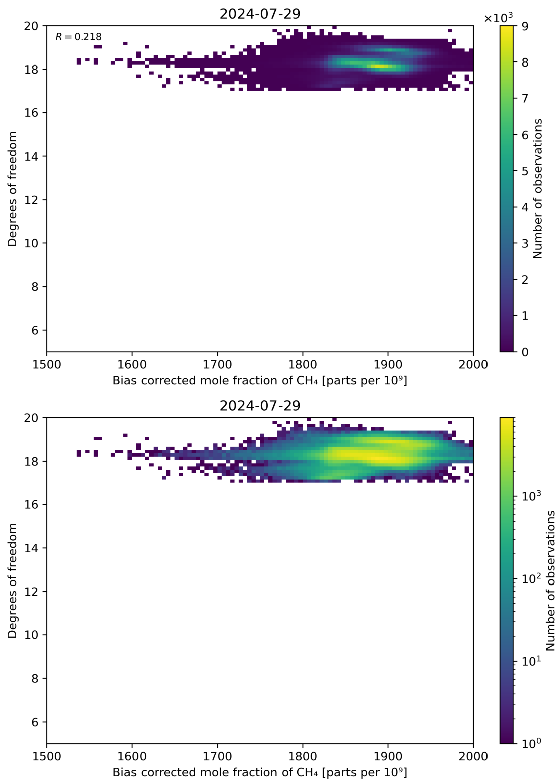
Figure 65: Scatter density plot of “Bias corrected mole fraction of CH 4 ” against “Degrees of freedom” for 2024-07-28 to 2024-07-30.
