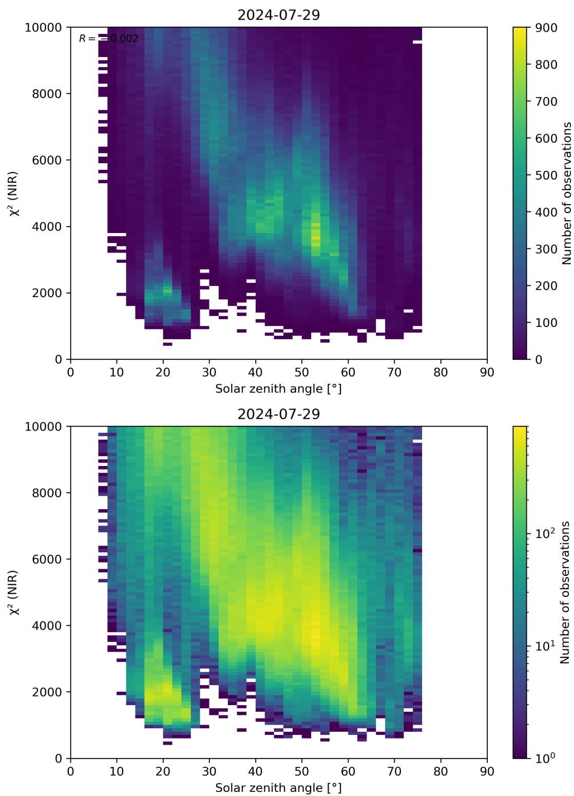
Figure 94: Scatter density plot of “Solar zenith angle” against “ \chi^2 (NIR)” for 2024-07-28 to 2024-07-30.
