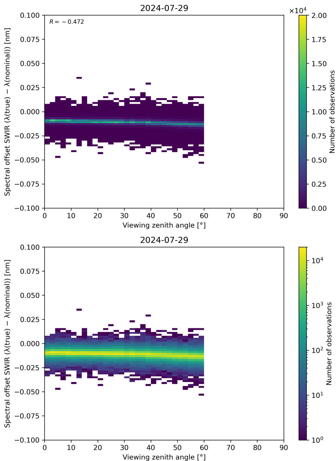
Figure 116: Scatter density plot of “Viewing zenith angle” against “Spectral offset SWIR ( \lambda(\text{true}) - \lambda(\text{nominal}) )” for 2024-07-28 to 2024-07-30.
