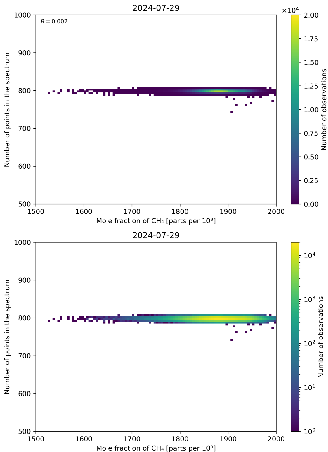
Figure 77: Scatter density plot of “Mole fraction of CH 4 ” against “Number of points in the spectrum” for 2024-07-28 to 2024-07-30.
