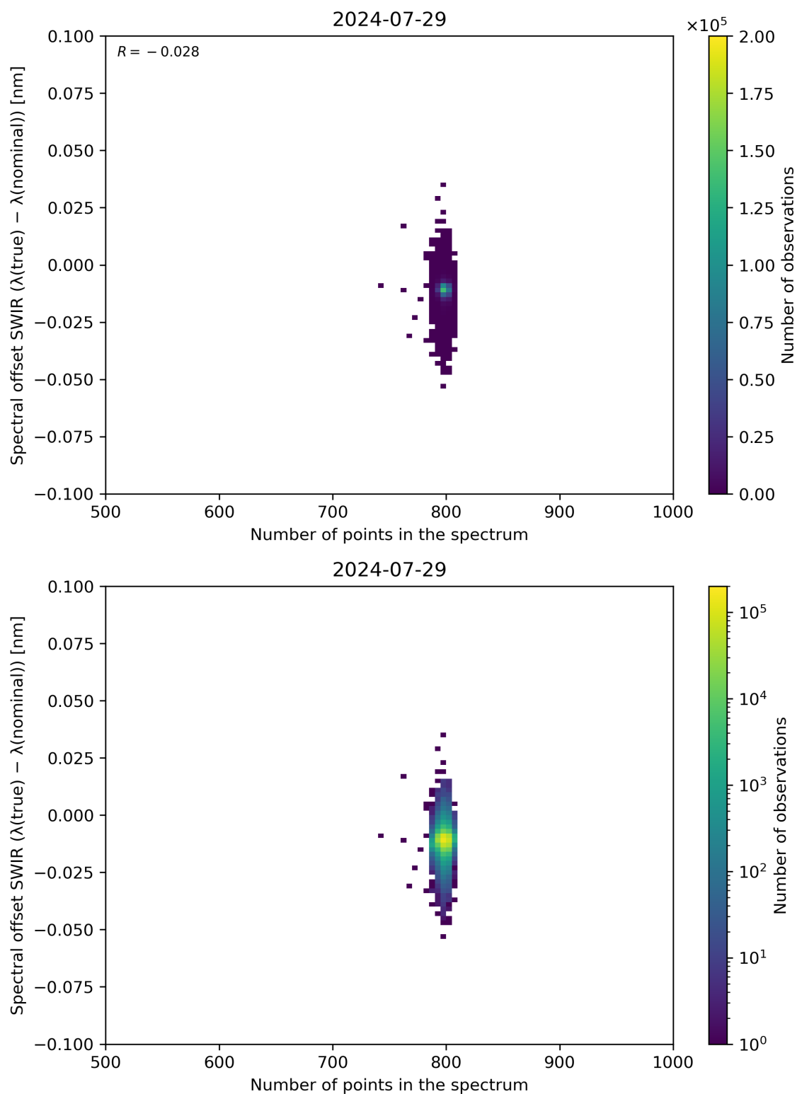
Figure 93: Scatter density plot of “Number of points in the spectrum” against “Spectral offset SWIR ( \lambda(\text{true}) - \lambda(\text{nominal}) )” for 2024-07-28 to 2024-07-30.
