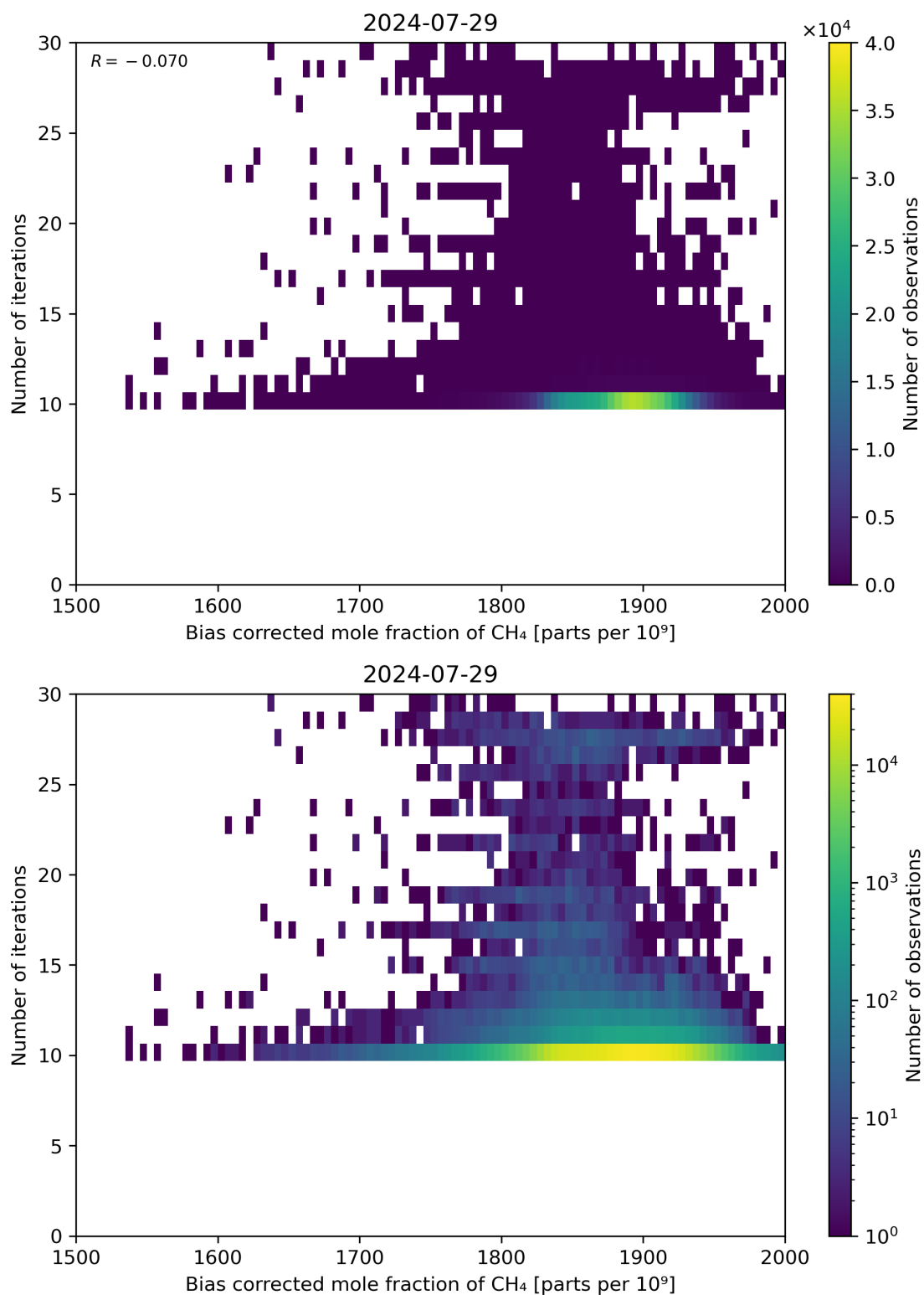
Figure 67: Scatter density plot of “Bias corrected mole fraction of \text{CH}_4 ” against “Number of iterations” for 2024-07-28 to 2024-07-30.
