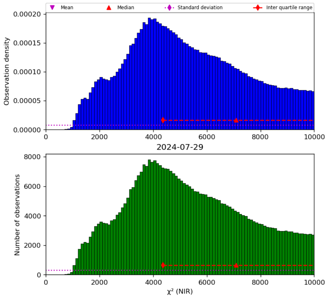
Figure 29: Histogram of “ \chi^2 (NIR)” for 2024-07-28 to 2024-07-30
