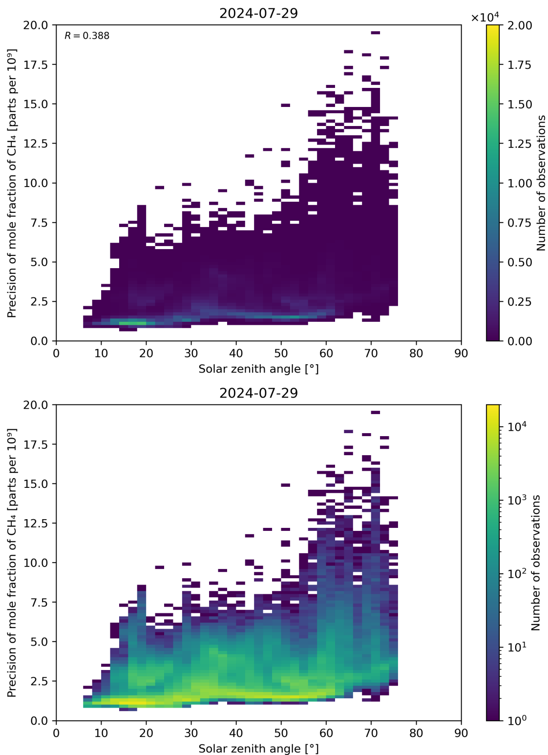
Figure 101: Scatter density plot of “Solar zenith angle” against “Precision of mole fraction of CH 4 ” for 2024-07-28 to 2024-07-30.
