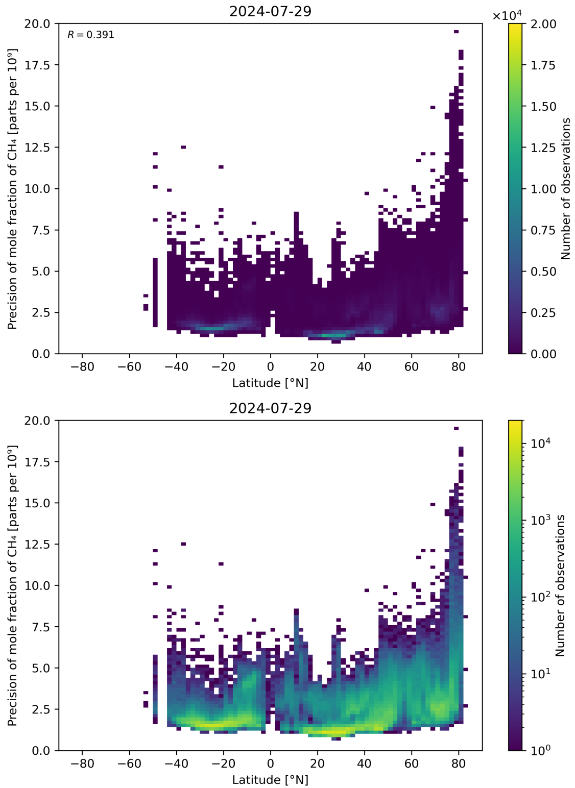
Figure 59: Scatter density plot of “Latitude” against “Precision of mole fraction of \text{CH}_4 ” for 2024-07-28 to 2024-07-30.
