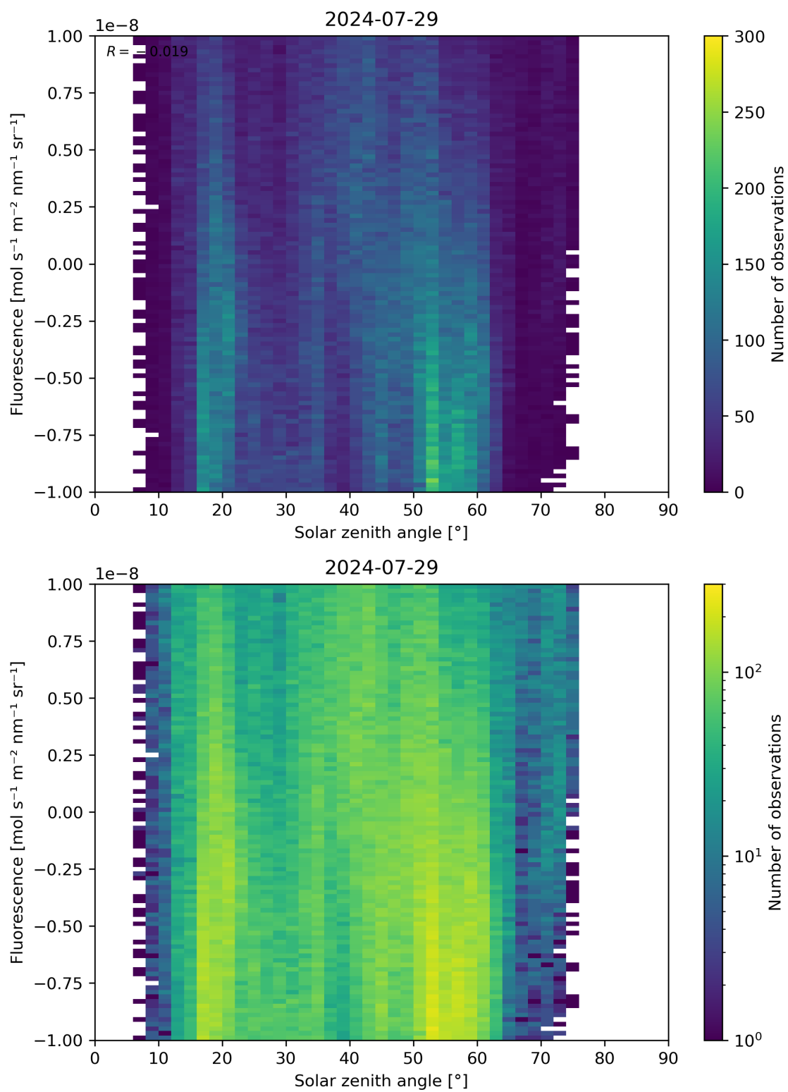
Figure 97: Scatter density plot of “Solar zenith angle” against “Fluorescence” for 2024-07-28 to 2024-07-30.
