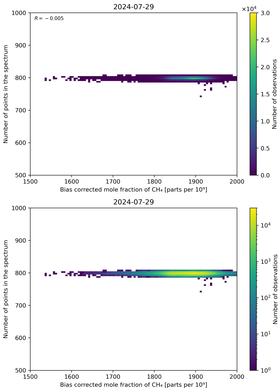
Figure 68: Scatter density plot of “Bias corrected mole fraction of CH 4 ” against “Number of points in the spectrum” for 2024-07-28 to 2024-07-30.
