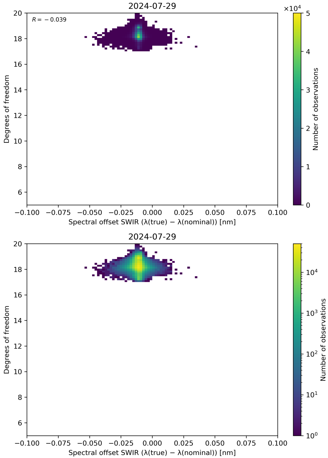
Figure 119: Scatter density plot of “Spectral offset SWIR ( \lambda(\text{true}) - \lambda(\text{nominal}) )” against “Degrees of freedom” for 2024-07-28 to 2024-07-30.
