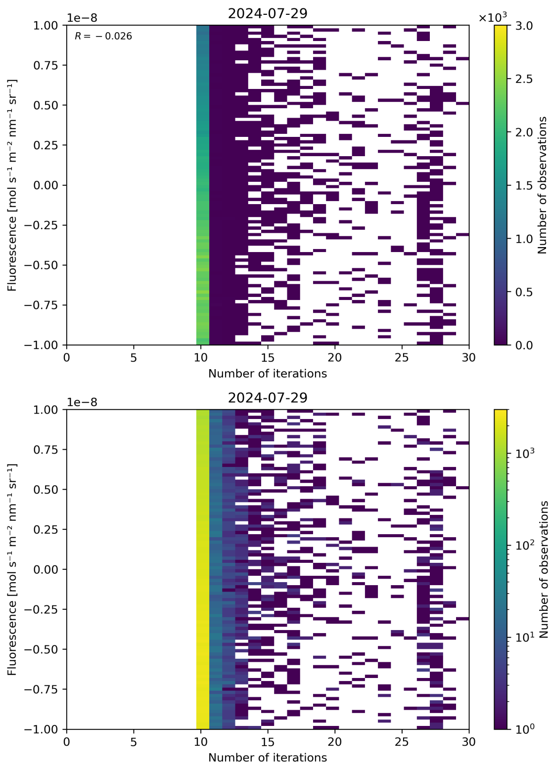
Figure 87: Scatter density plot of “Number of iterations” against “Fluorescence” for 2024-07-28 to 2024-07-30.
