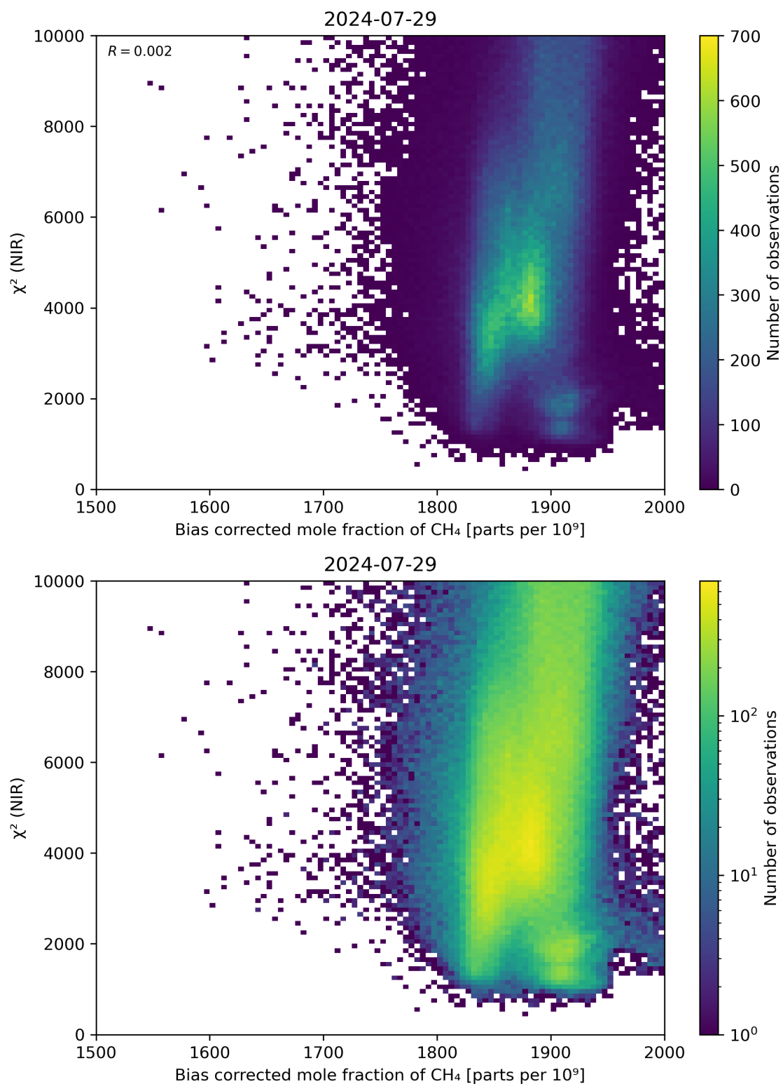
Figure 63: Scatter density plot of “Bias corrected mole fraction of CH 4 ” against “ \chi^2 (NIR)” for 2024-07-28 to 2024-07-30.
