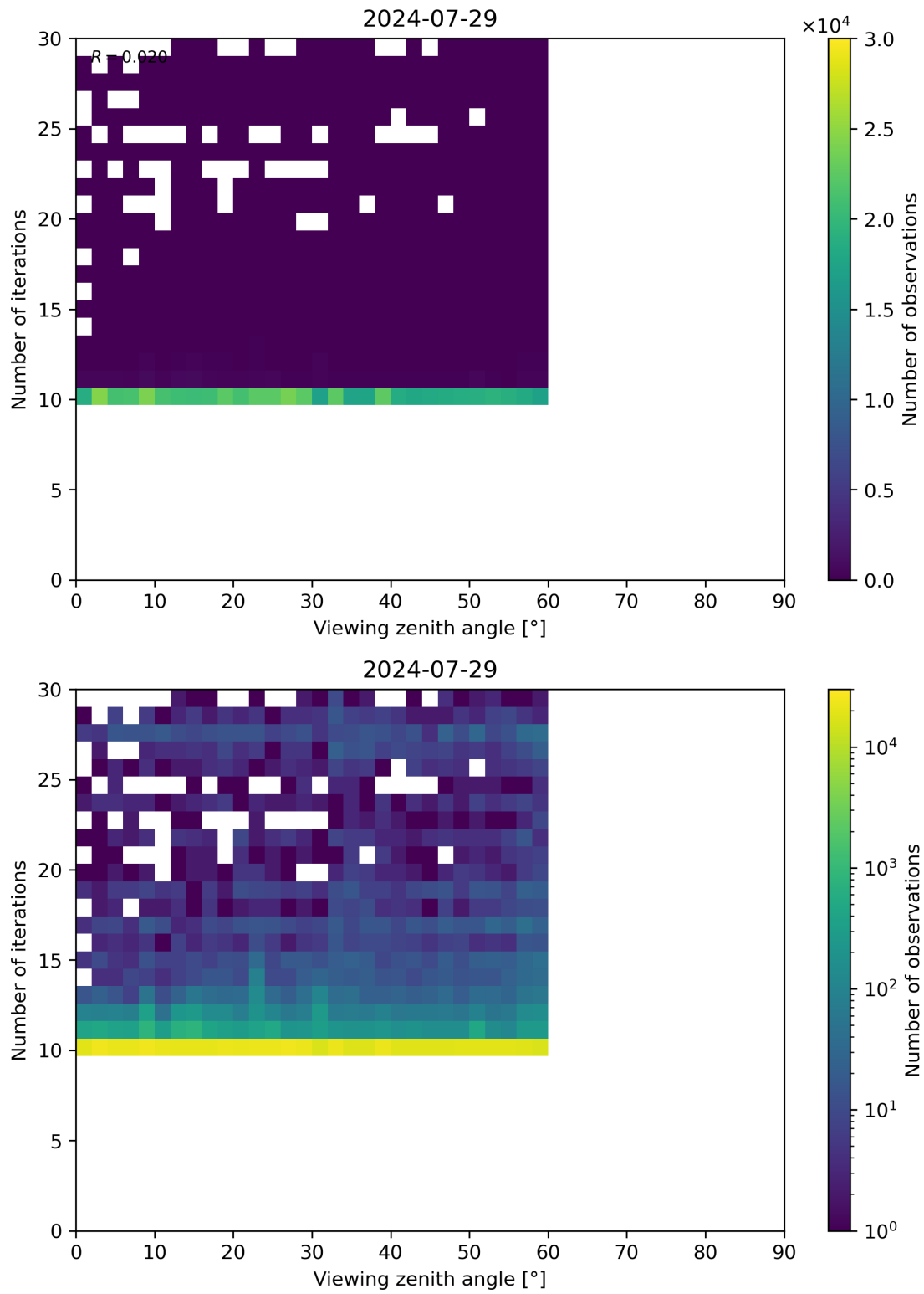
Figure 113: Scatter density plot of “Viewing zenith angle” against “Number of iterations” for 2024-07-28 to 2024-07-30.
