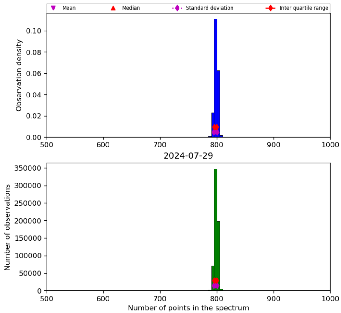
Figure 26: Histogram of “Number of points in the spectrum” for 2024-07-28 to 2024-07-30
