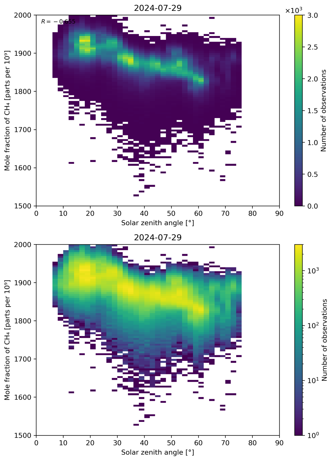
Figure 99: Scatter density plot of “Solar zenith angle” against “Mole fraction of CH 4 ” for 2024-07-28 to 2024-07-30.
