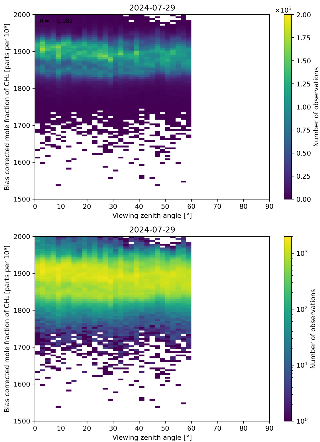
Figure 111: Scatter density plot of “Viewing zenith angle” against “Bias corrected mole fraction of CH 4 ” for 2024-07-28 to 2024-07-30.
