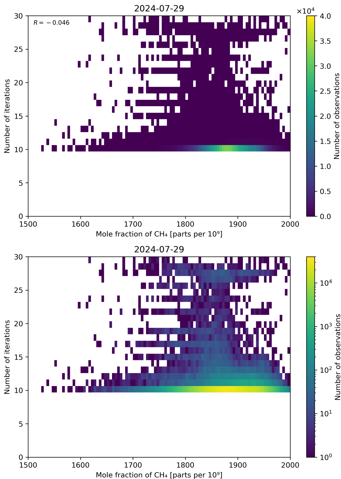
Figure 76: Scatter density plot of “Mole fraction of CH 4 ” against “Number of iterations” for 2024-07-28 to 2024-07-30.
