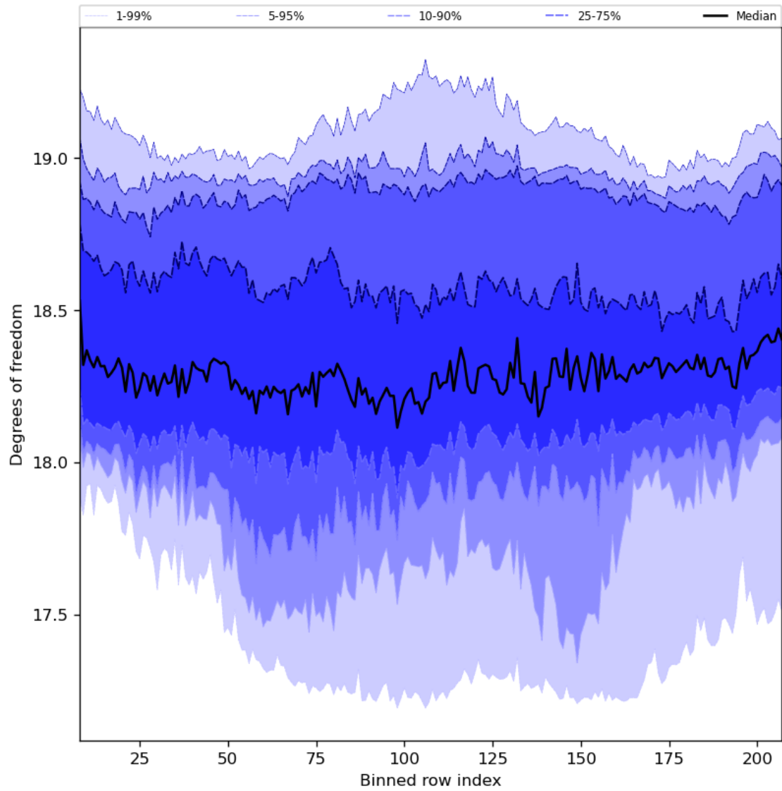
Figure 41: Along track statistics of “Degrees of freedom” for 2024-07-28 to 2024-07-30
