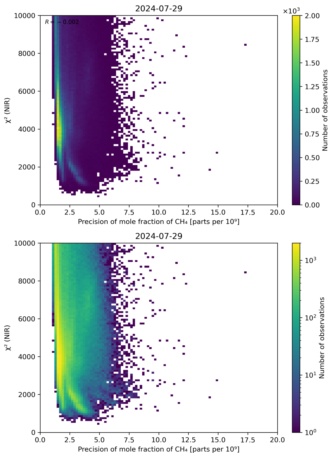
Figure 78: Scatter density plot of “Precision of mole fraction of \text{CH}_4 ” against “ \chi^2 (NIR)” for 2024-07-28 to 2024-07-30.
