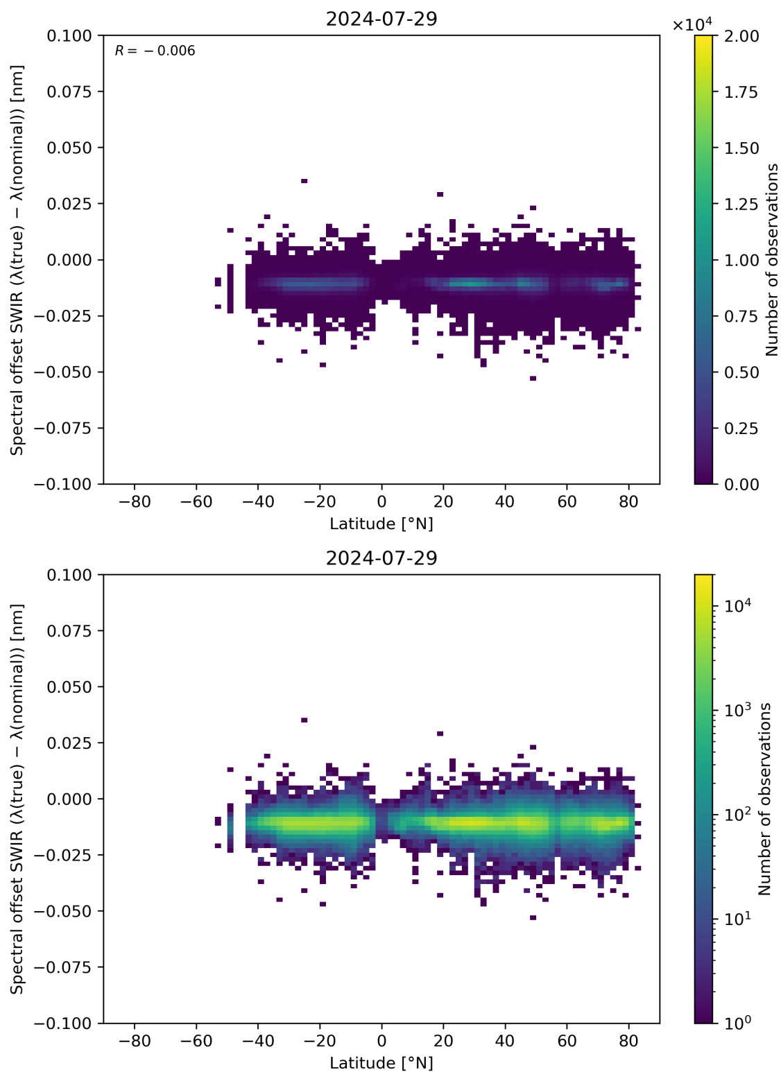
Figure 62: Scatter density plot of “Latitude” against “Spectral offset SWIR ( \lambda(\text{true}) - \lambda(\text{nominal}) )” for 2024-07-28 to 2024-07-30.
