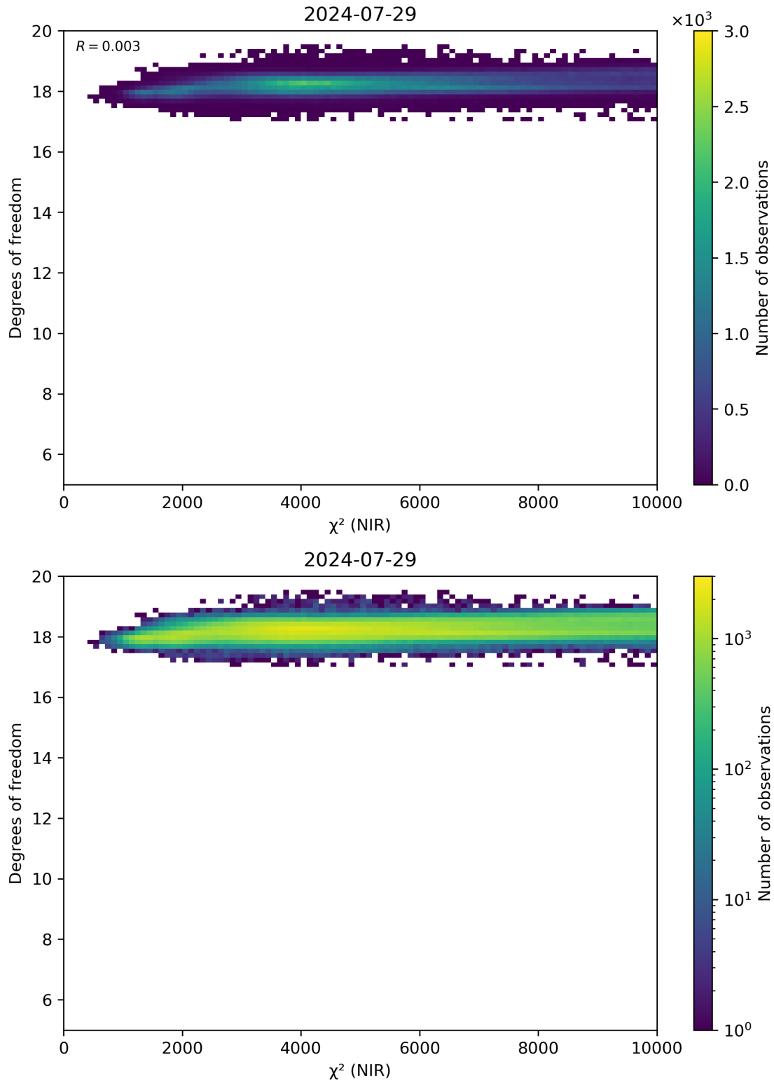
Figure 44: Scatter density plot of “ \chi^2 (NIR)” against “Degrees of freedom” for 2024-07-28 to 2024-07-30.
