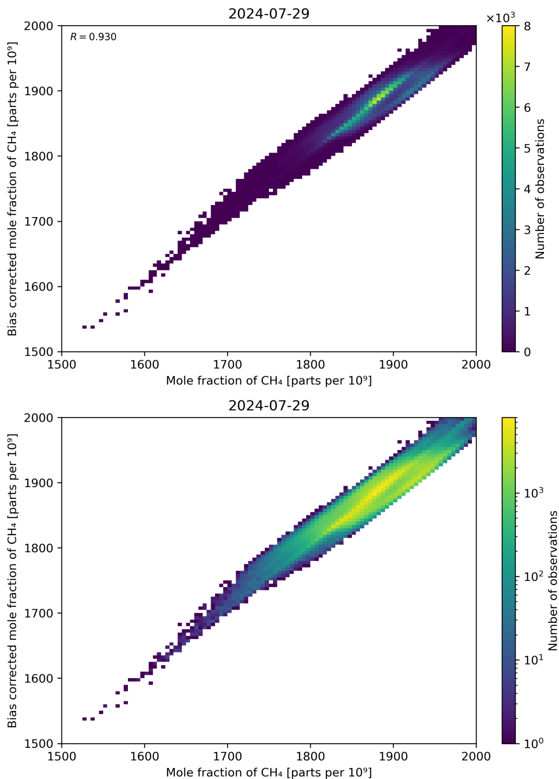
Figure 74: Scatter density plot of “Mole fraction of CH 4 ” against “Bias corrected mole fraction of CH 4 ” for 2024-07-28 to 2024-07-30.
