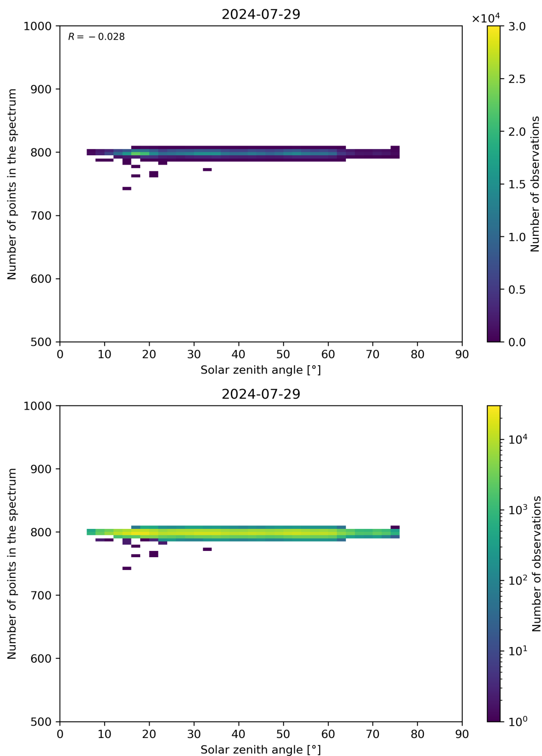
Figure 103: Scatter density plot of “Solar zenith angle” against “Number of points in the spectrum” for 2024-07-28 to 2024-07-30.
