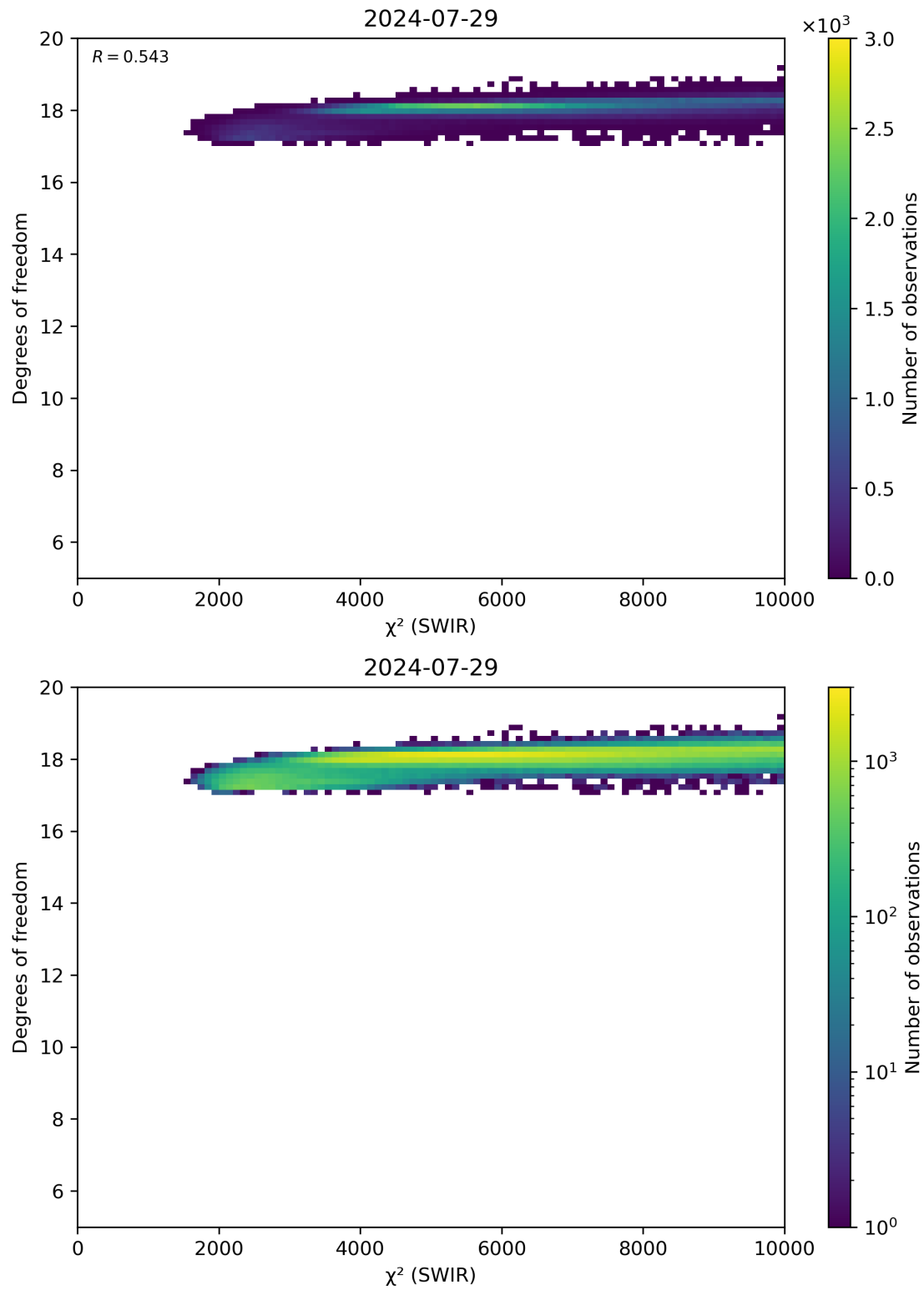
Figure 48: Scatter density plot of “ \chi^2 (SWIR)” against “Degrees of freedom” for 2024-07-28 to 2024-07-30.
