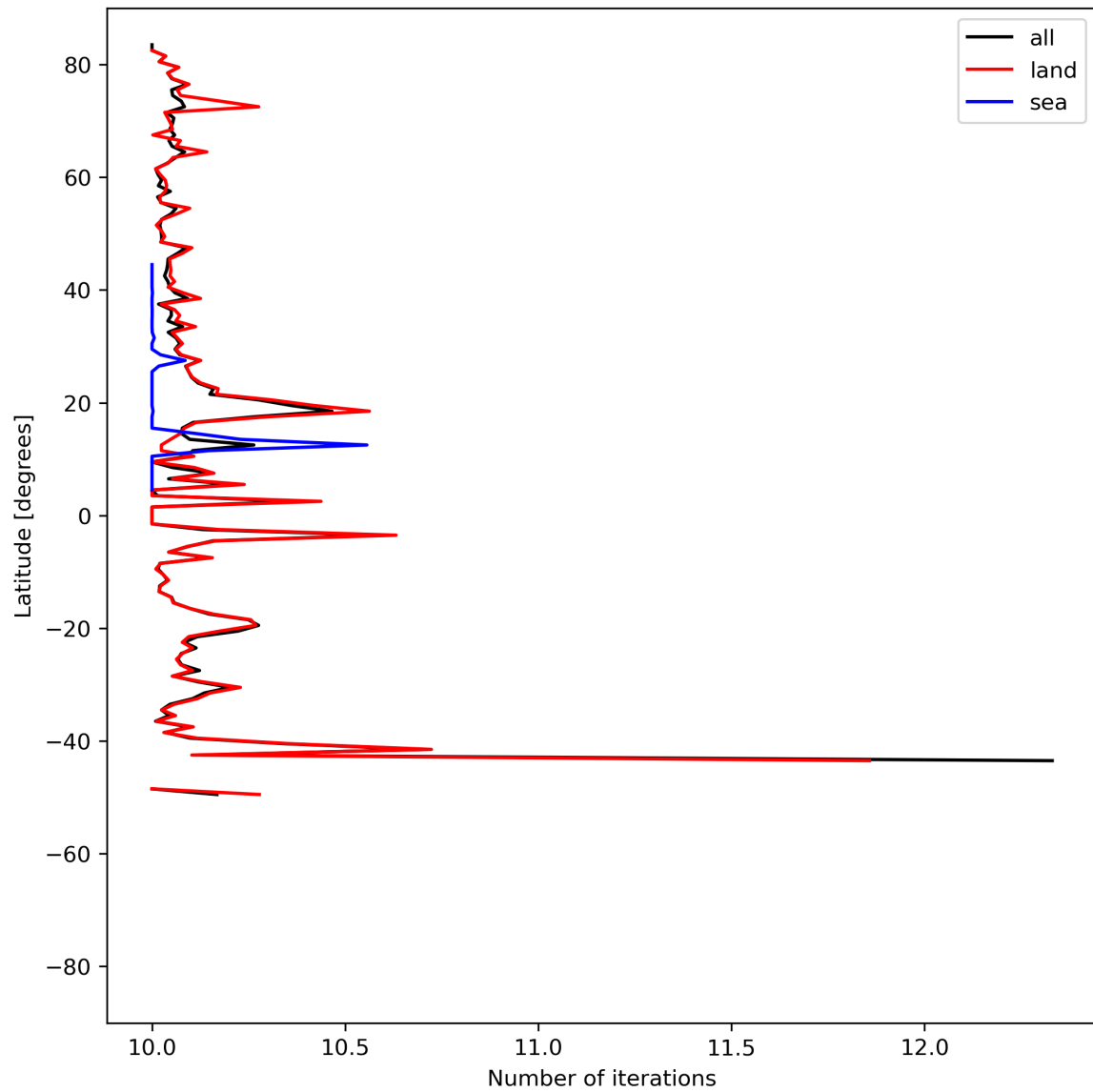
Figure 20: Zonal average of “Number of iterations” for 2024-07-28 to 2024-07-30.
