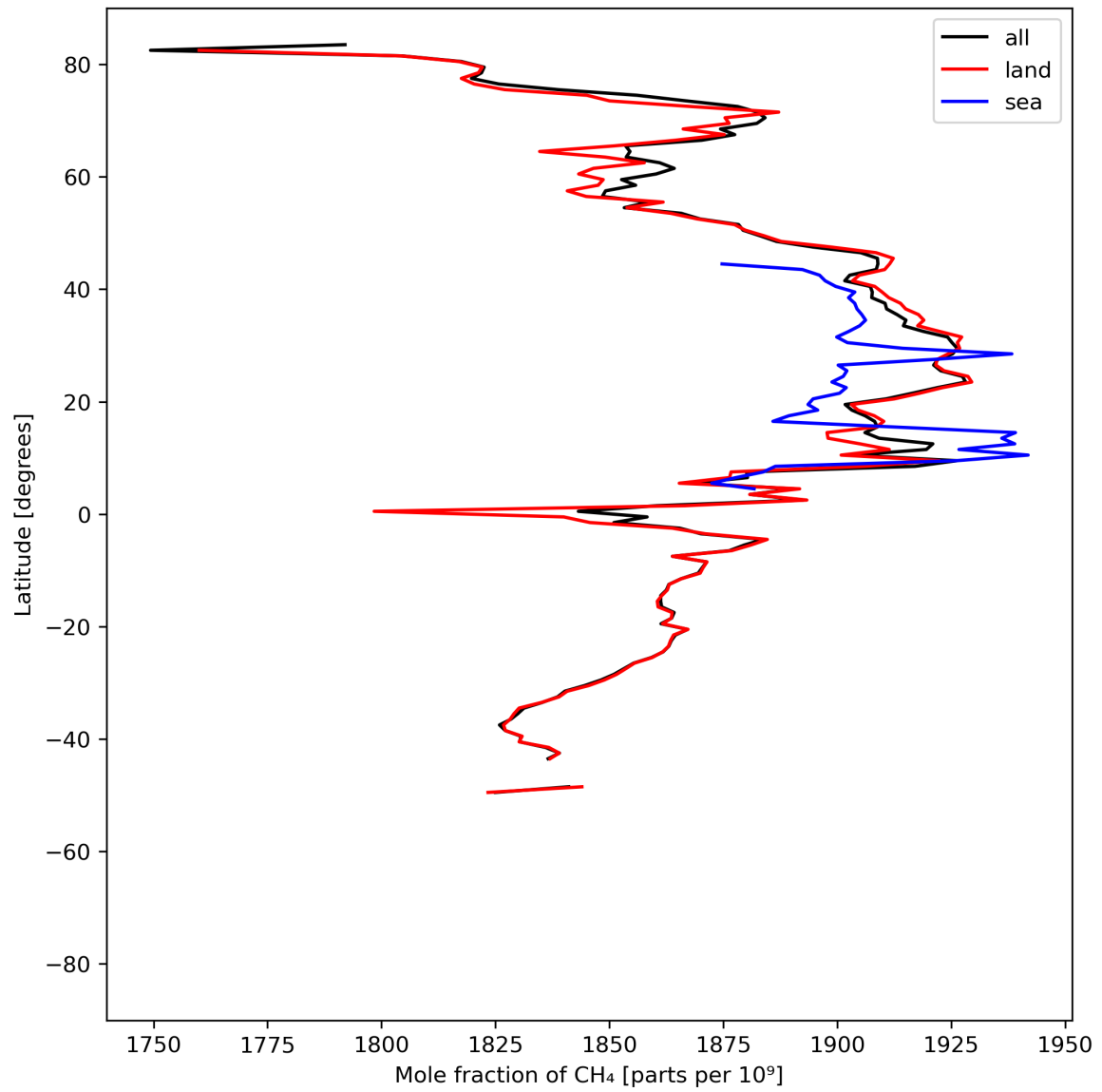
Figure 12: Zonal average of “Mole fraction of \text{CH}_4 ” for 2024-07-28 to 2024-07-30.
