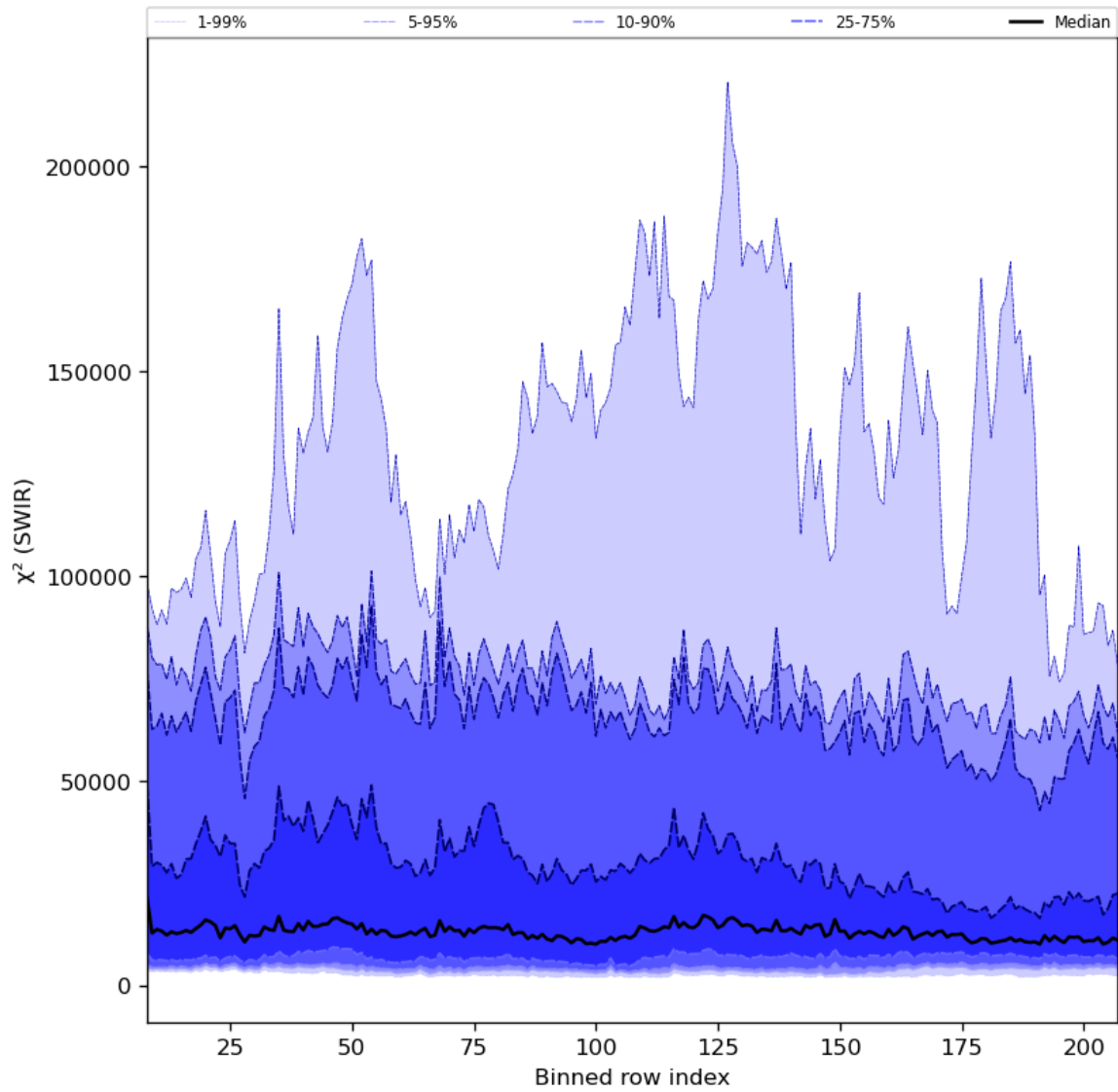
Figure 39: Along track statistics of “ \chi^2 (SWIR)” for 2024-07-28 to 2024-07-30
