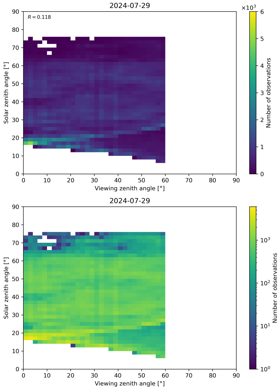
Figure 115: Scatter density plot of “Viewing zenith angle” against “Solar zenith angle” for 2024-07-28 to 2024-07-30.
