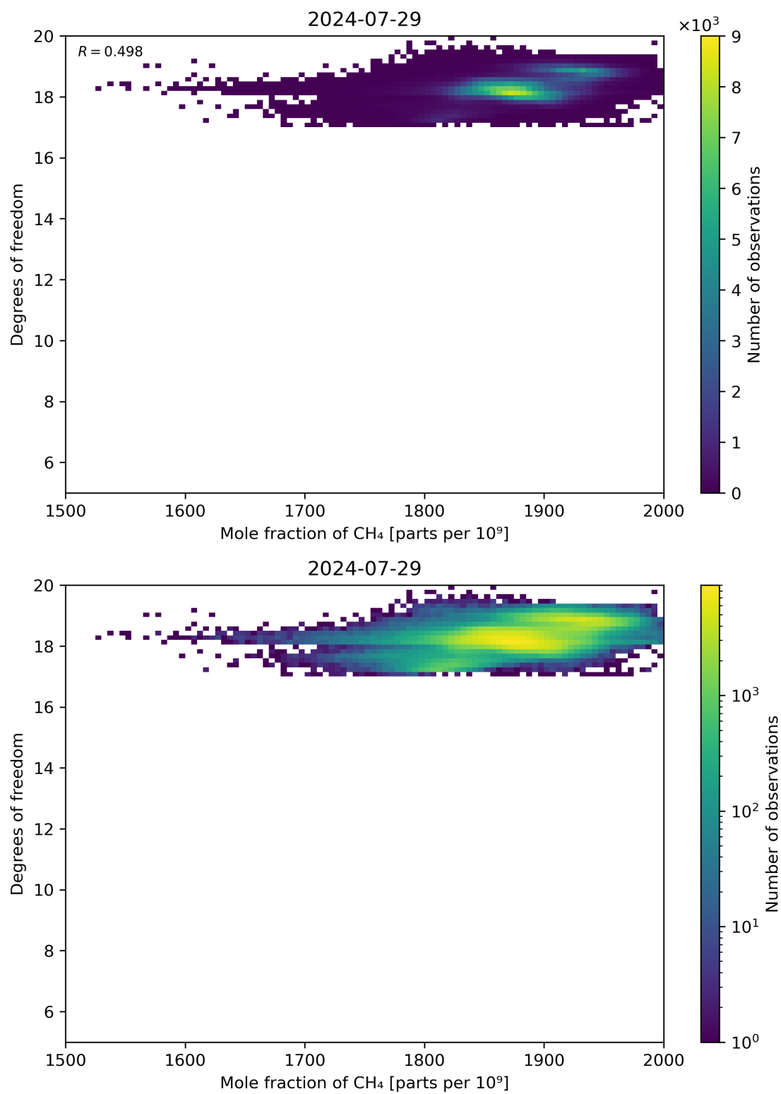
Figure 72: Scatter density plot of “Mole fraction of CH 4 ” against “Degrees of freedom” for 2024-07-28 to 2024-07-30.
