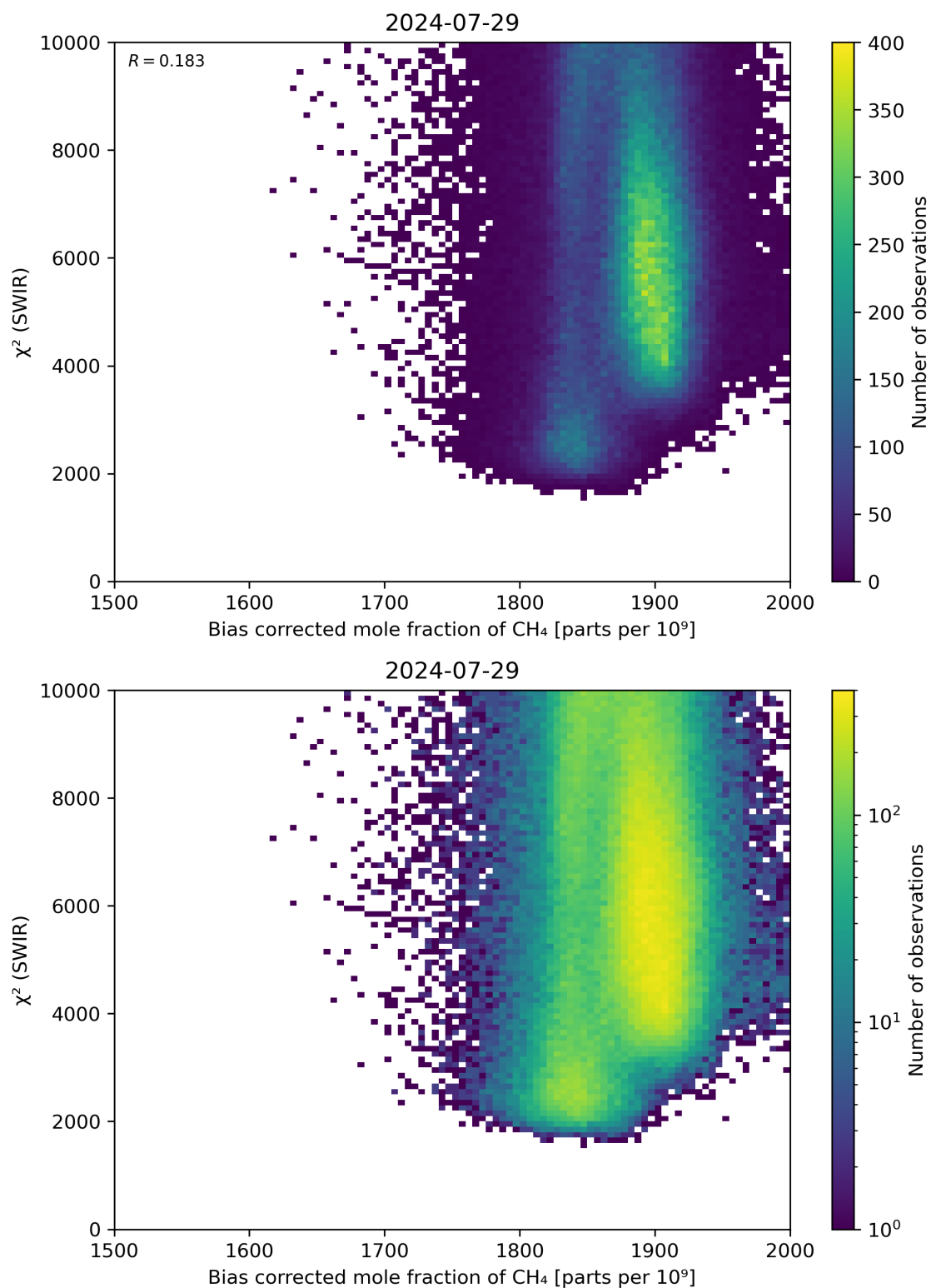
Figure 64: Scatter density plot of “Bias corrected mole fraction of \text{CH}_4 ” against “ \chi^2 (SWIR)” for 2024-07-28 to 2024-07-30.
