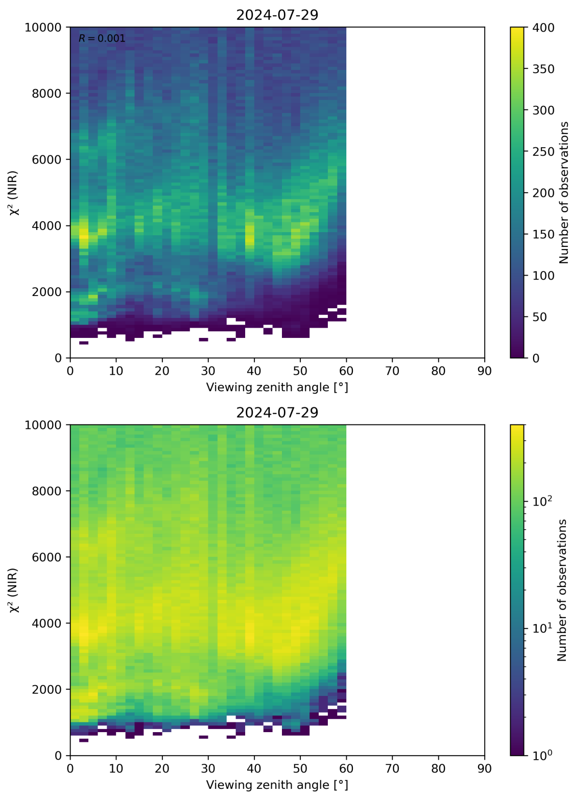
Figure 105: Scatter density plot of “Viewing zenith angle” against “ \chi^2 (NIR)” for 2024-07-28 to 2024-07-30.
