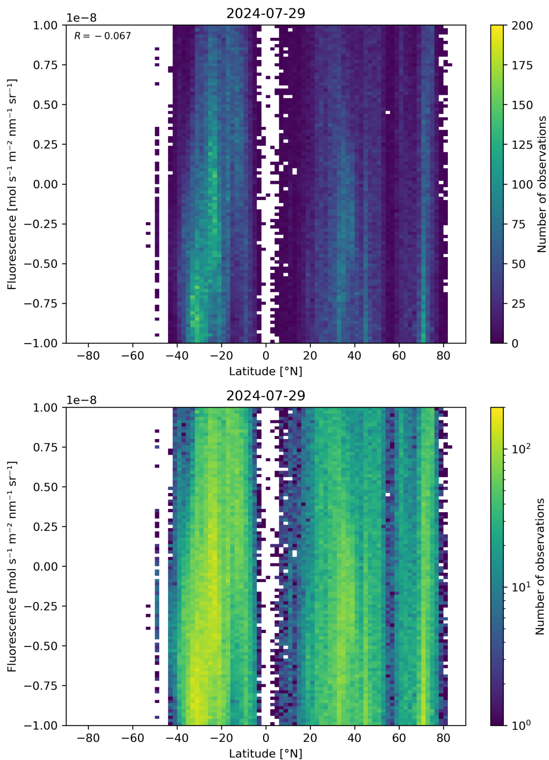
Figure 56: Scatter density plot of “Latitude” against “Fluorescence” for 2024-07-28 to 2024-07-30.
