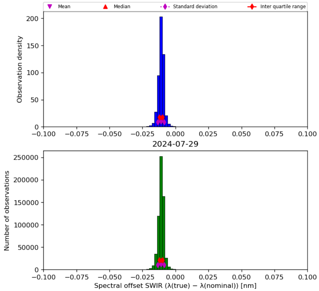
Figure 27: Histogram of “Spectral offset SWIR ( \lambda(\text{true}) - \lambda(\text{nominal}) )” for 2024-07-28 to 2024-07-30
