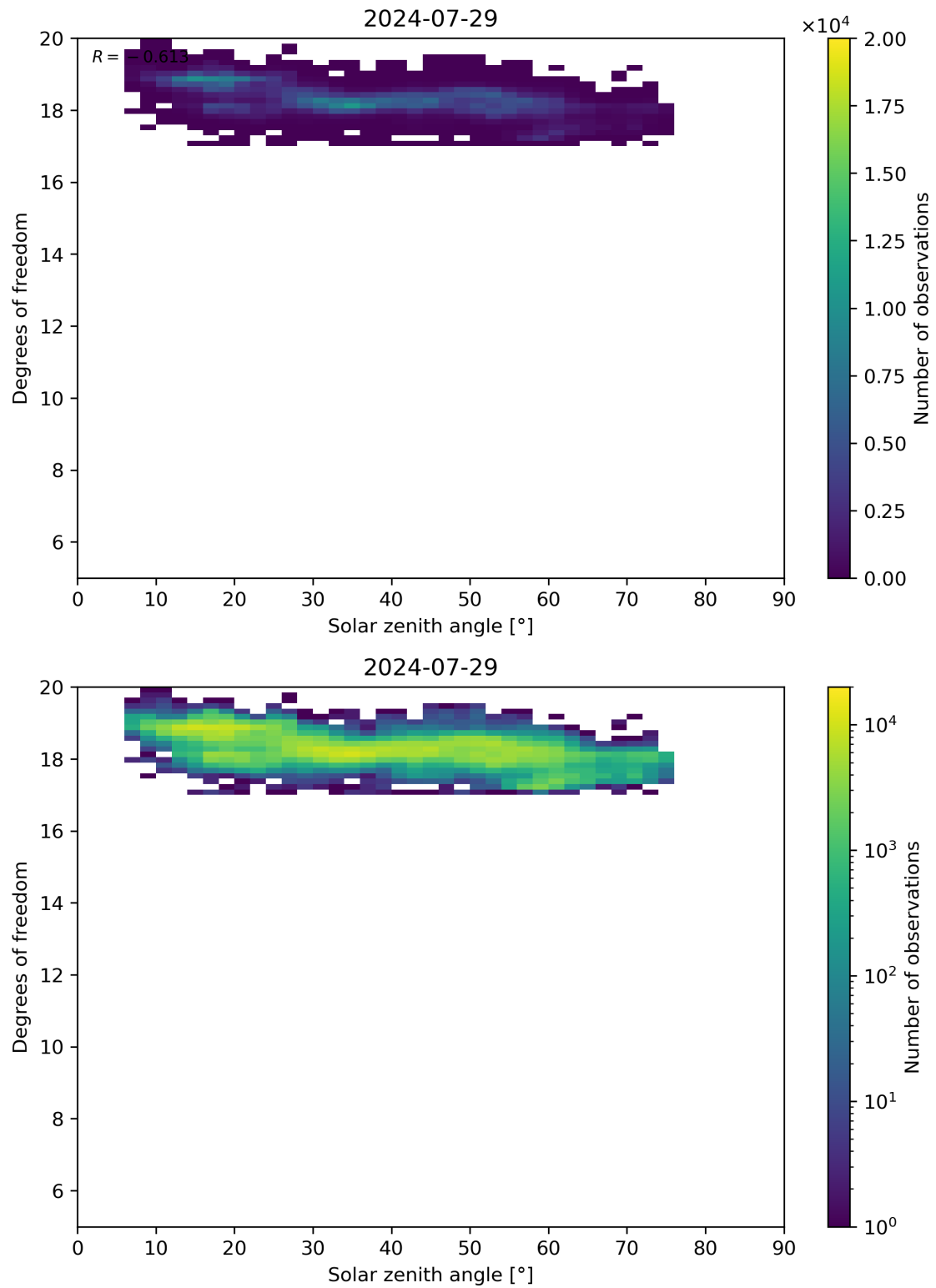
Figure 96: Scatter density plot of “Solar zenith angle” against “Degrees of freedom” for 2024-07-28 to 2024-07-30.
