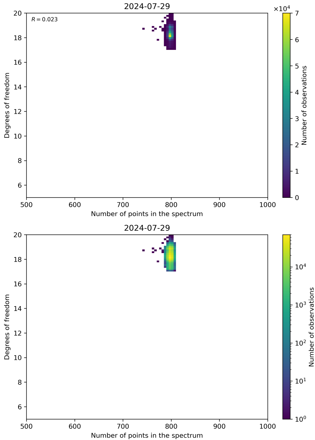
Figure 90: Scatter density plot of “Number of points in the spectrum” against “Degrees of freedom” for 2024-07-28 to 2024-07-30.
