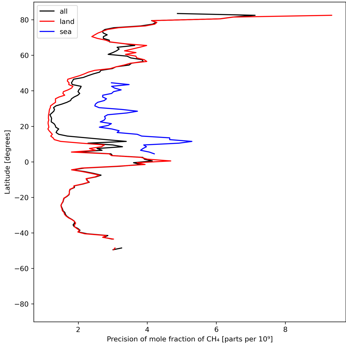
Figure 13: Zonal average of “Precision of mole fraction of CH 4 ” for 2024-07-28 to 2024-07-30.
