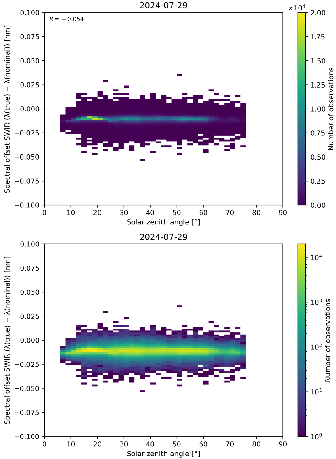
Figure 104: Scatter density plot of “Solar zenith angle” against “Spectral offset SWIR ( \lambda(\text{true}) - \lambda(\text{nominal}) )” for 2024-07-28 to 2024-07-30.
