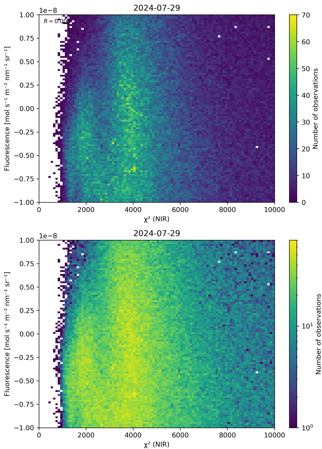
Figure 45: Scatter density plot of “ \chi^2 (NIR)” against “Fluorescence” for 2024-07-28 to 2024-07-30.
