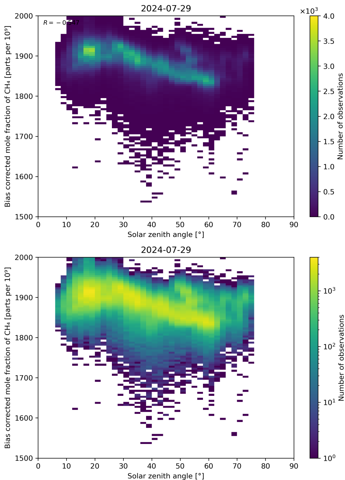
Figure 100: Scatter density plot of “Solar zenith angle” against “Bias corrected mole fraction of \text{CH}_4 ” for 2024-07-28 to 2024-07-30.
