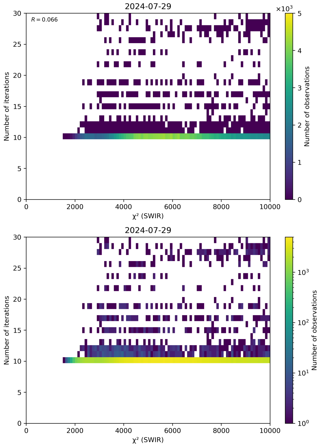
Figure 50: Scatter density plot of “ \chi^2 (SWIR)” against “Number of iterations” for 2024-07-28 to 2024-07-30.
