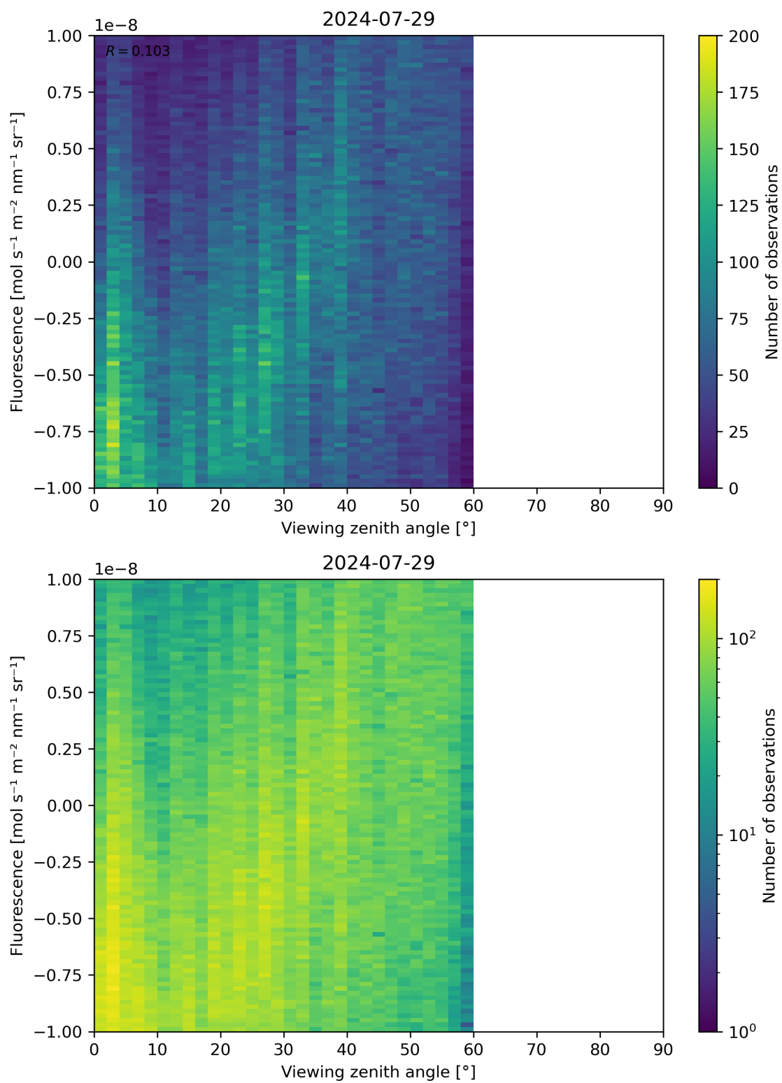
Figure 108: Scatter density plot of “Viewing zenith angle” against “Fluorescence” for 2024-07-28 to 2024-07-30.
