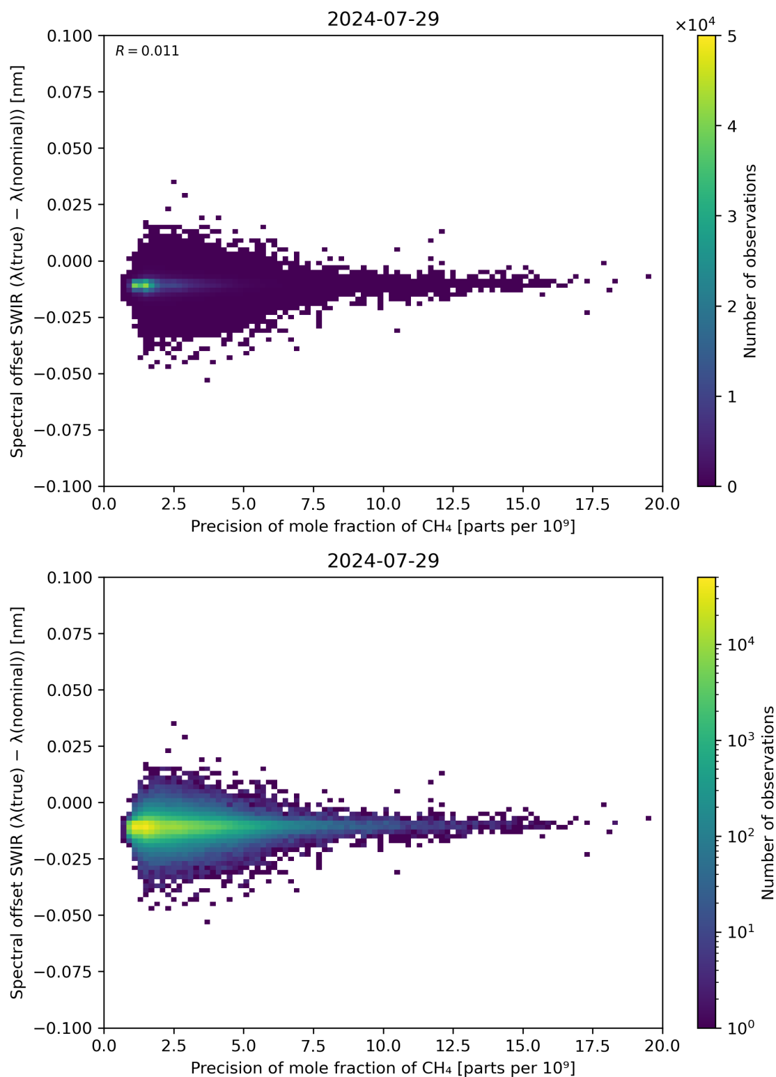
Figure 85: Scatter density plot of “Precision of mole fraction of CH 4 ” against “Spectral offset SWIR ( \lambda(\text{true}) - \lambda(\text{nominal}) )” for 2024-07-28 to 2024-07-30.
