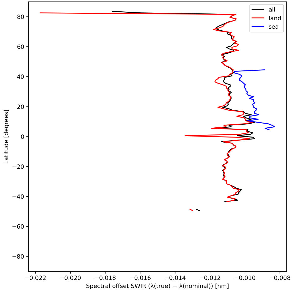
Figure 16: Zonal average of “Spectral offset SWIR ( \lambda(\text{true}) - \lambda(\text{nominal}) )” for 2024-07-28 to 2024-07-30.
