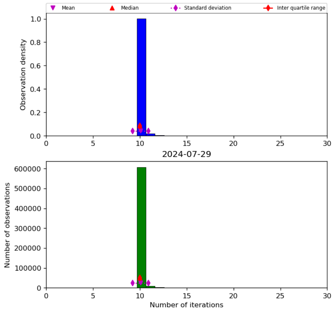
Figure 31: Histogram of “Number of iterations” for 2024-07-28 to 2024-07-30
