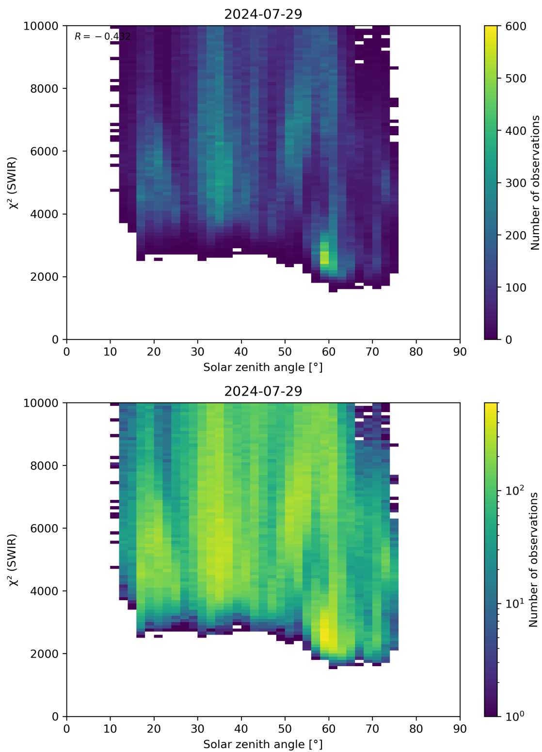
Figure 95: Scatter density plot of “Solar zenith angle” against “ \chi^2 (SWIR)” for 2024-07-28 to 2024-07-30.
