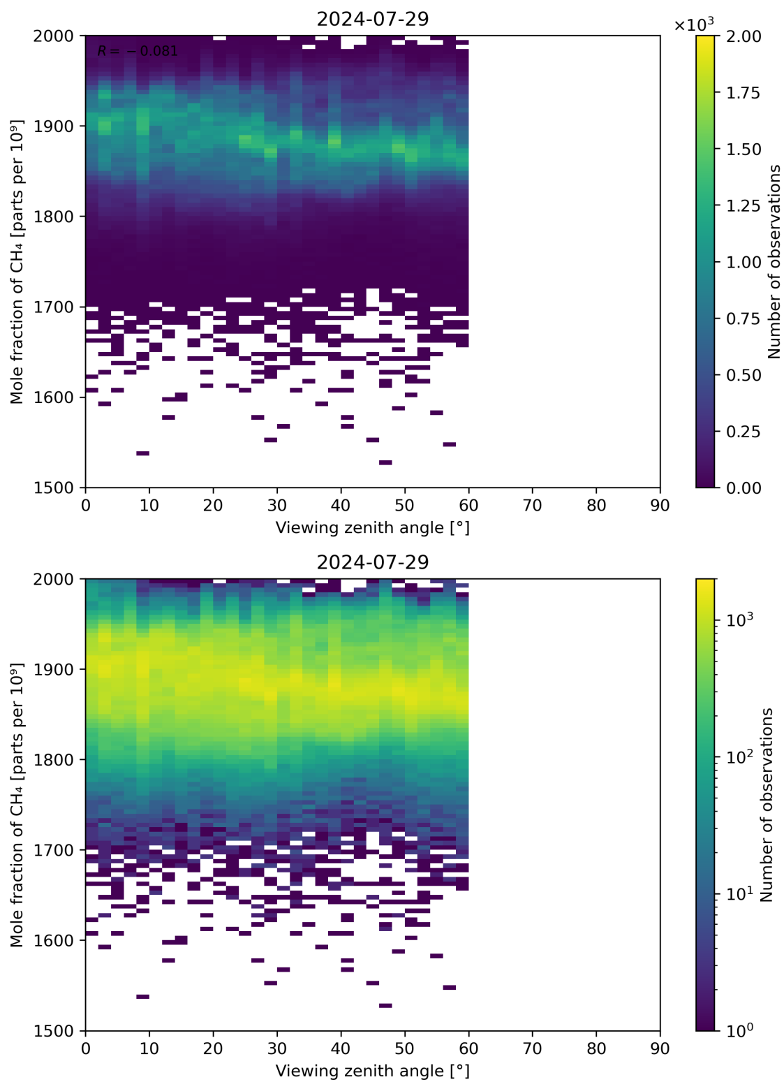
Figure 110: Scatter density plot of “Viewing zenith angle” against “Mole fraction of \text{CH}_4 ” for 2024-07-28 to 2024-07-30.
