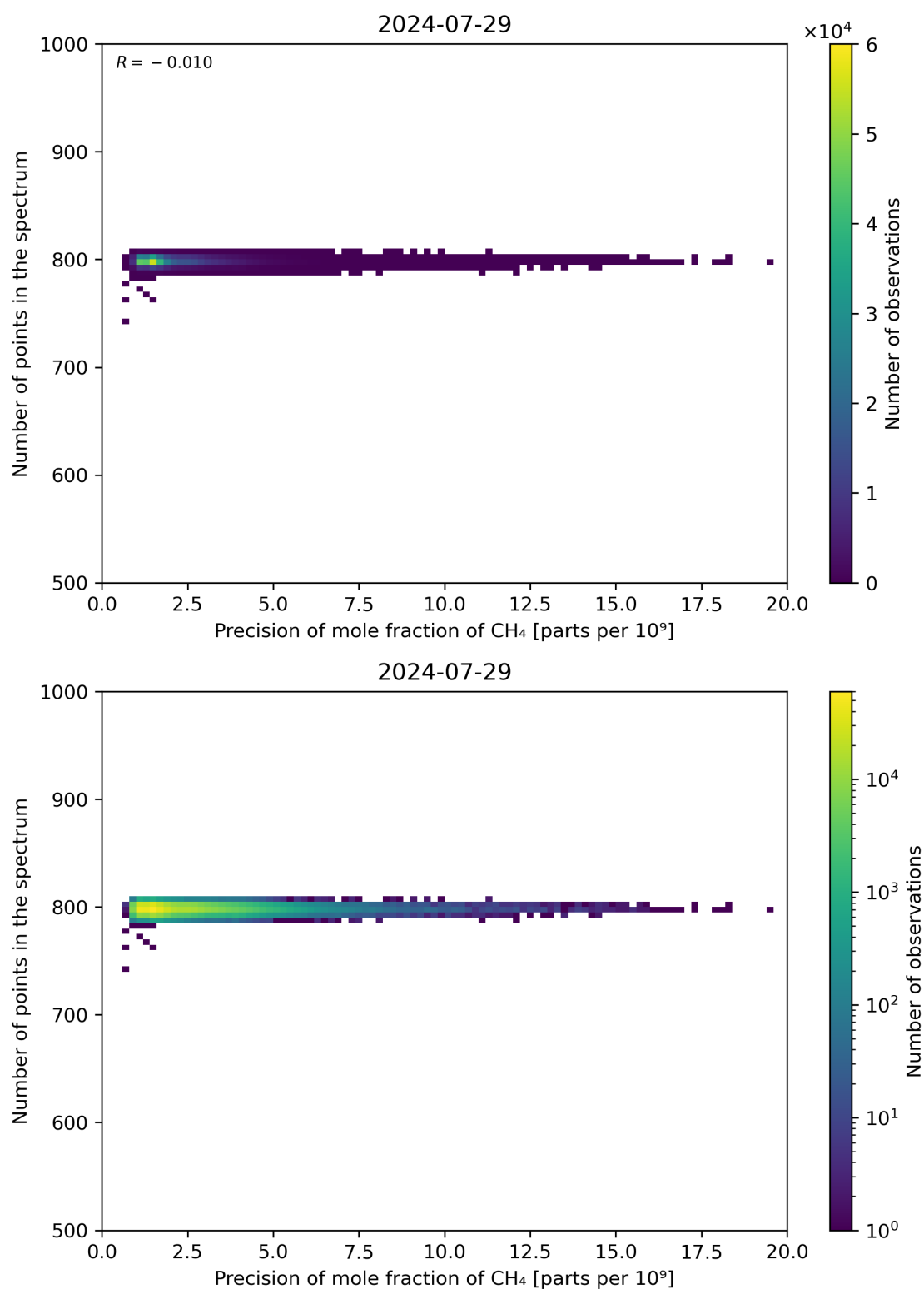
Figure 84: Scatter density plot of “Precision of mole fraction of CH 4 ” against “Number of points in the spectrum” for 2024-07-28 to 2024-07-30.
