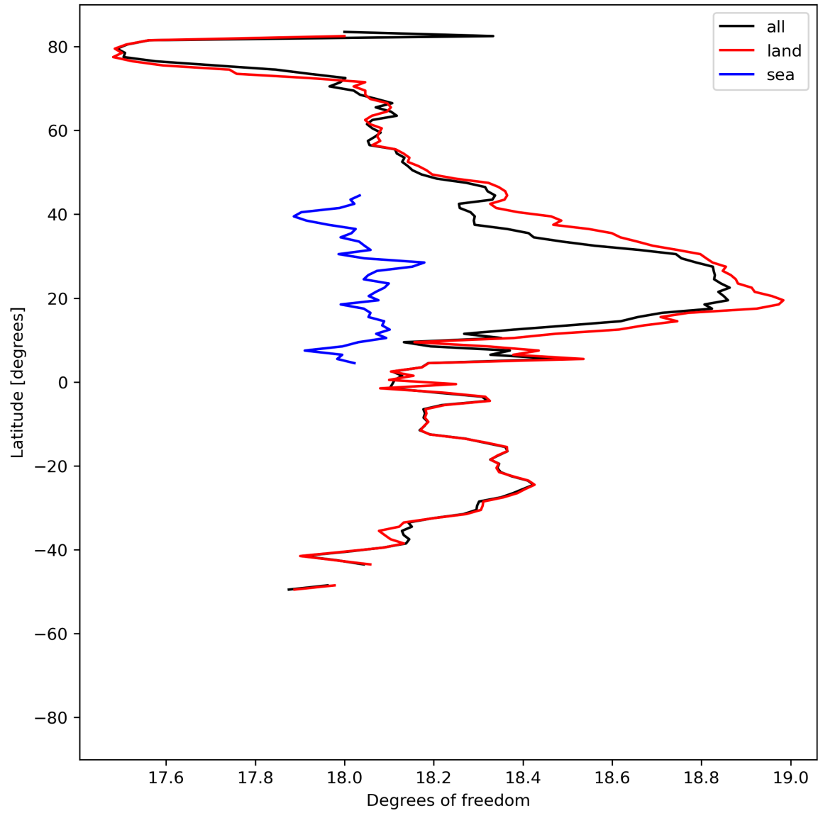
Figure 19: Zonal average of “Degrees of freedom” for 2024-07-28 to 2024-07-30.
