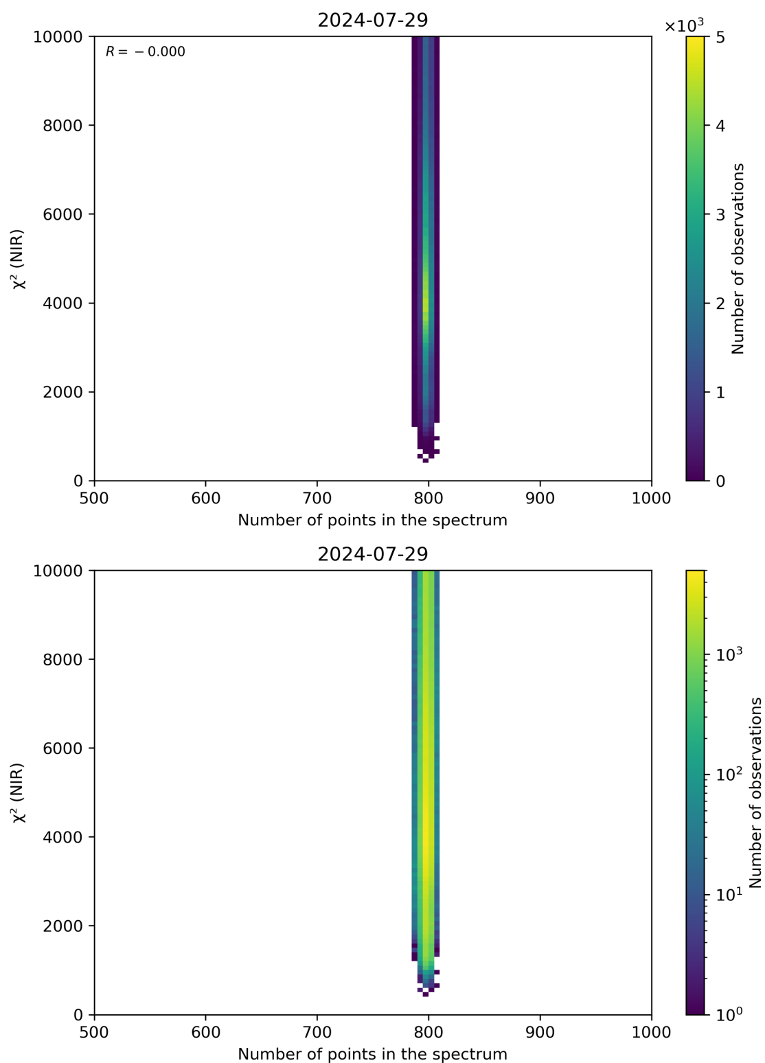
Figure 88: Scatter density plot of “Number of points in the spectrum” against “ \chi^2 (NIR)” for 2024-07-28 to 2024-07-30.
