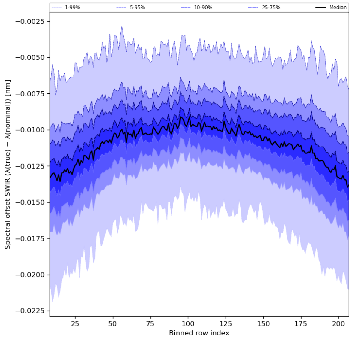
Figure 38: Along track statistics of “Spectral offset SWIR ( \lambda(\text{true}) - \lambda(\text{nominal}) )” for 2024-07-28 to 2024-07-30
