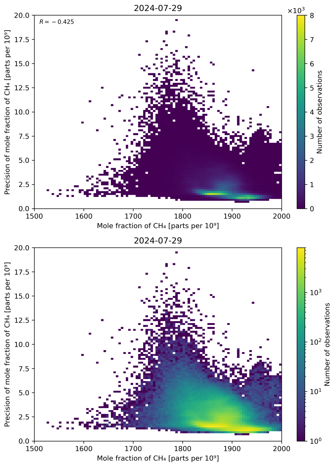
Figure 75: Scatter density plot of “Mole fraction of CH 4 ” against “Precision of mole fraction of CH 4 ” for 2024-07-28 to 2024-07-30.
