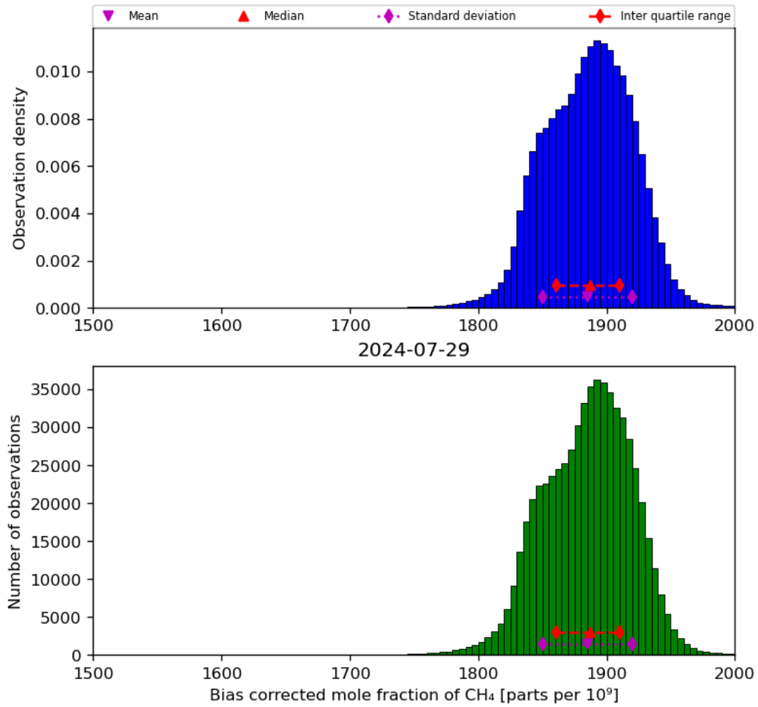
Figure 25: Histogram of “Bias corrected mole fraction of CH 4 ” for 2024-07-28 to 2024-07-30
