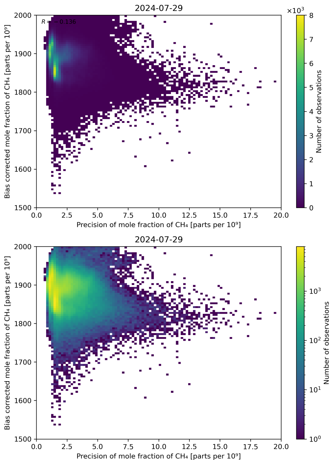
Figure 82: Scatter density plot of “Precision of mole fraction of \text{CH}_4 ” against “Bias corrected mole fraction of \text{CH}_4 ” for 2024-07-28 to 2024-07-30.
