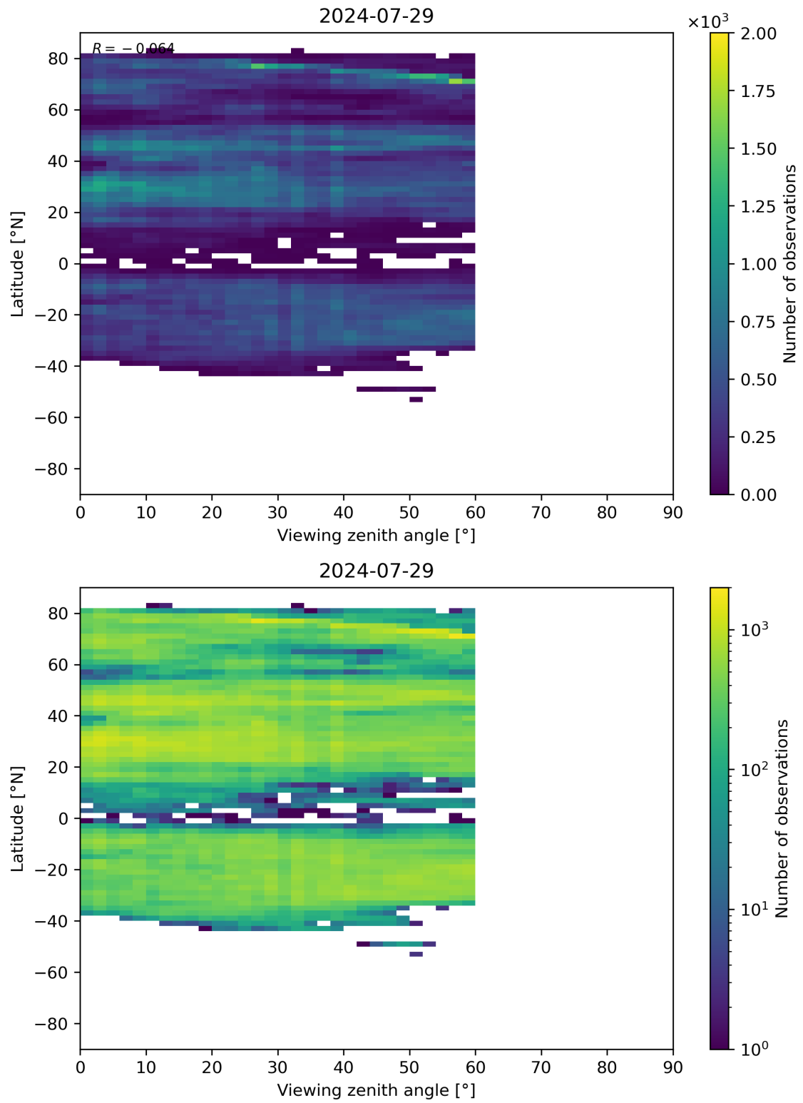
Figure 109: Scatter density plot of “Viewing zenith angle” against “Latitude” for 2024-07-28 to 2024-07-30.
