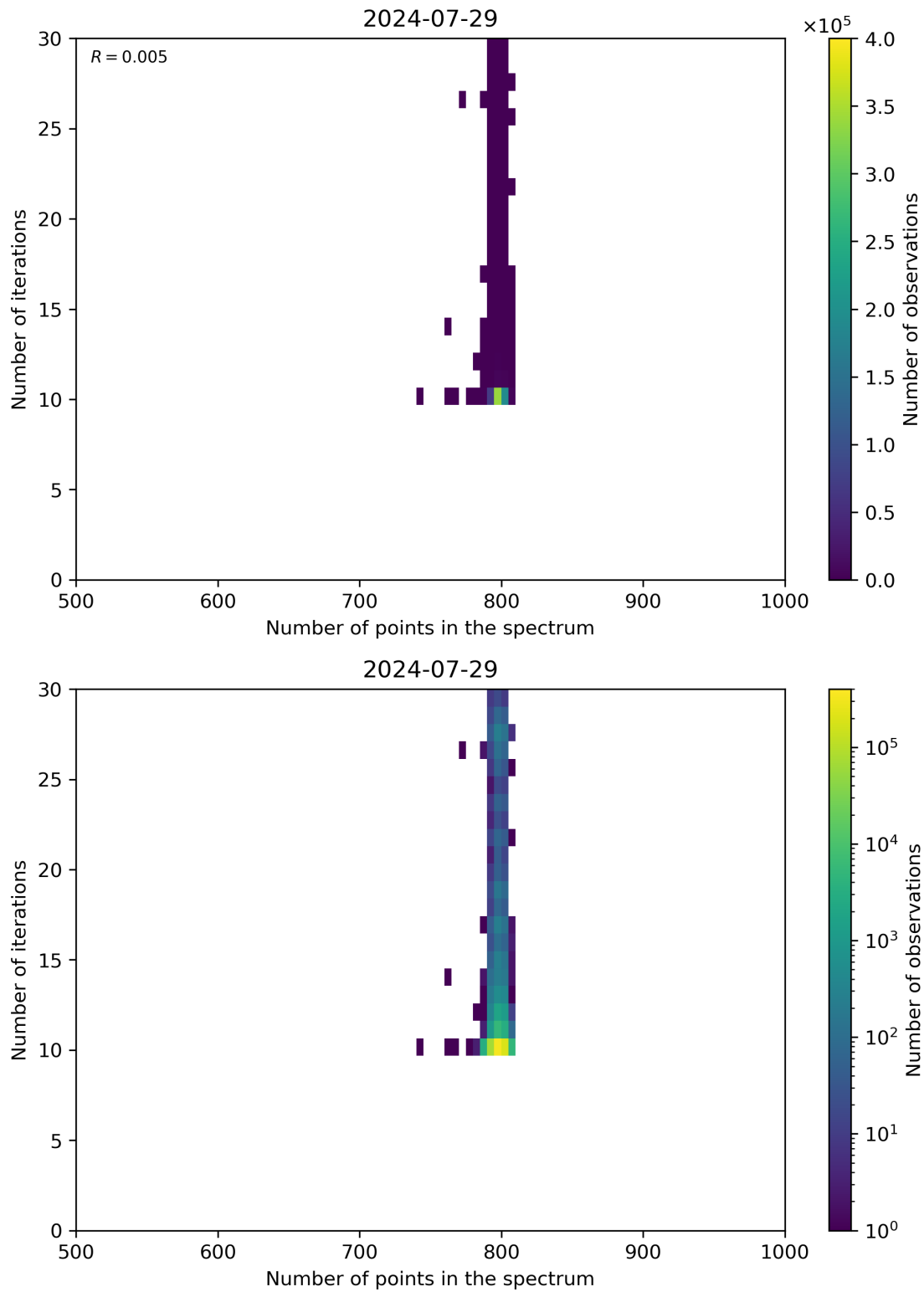
Figure 92: Scatter density plot of “Number of points in the spectrum” against “Number of iterations” for 2024-07-28 to 2024-07-30.
