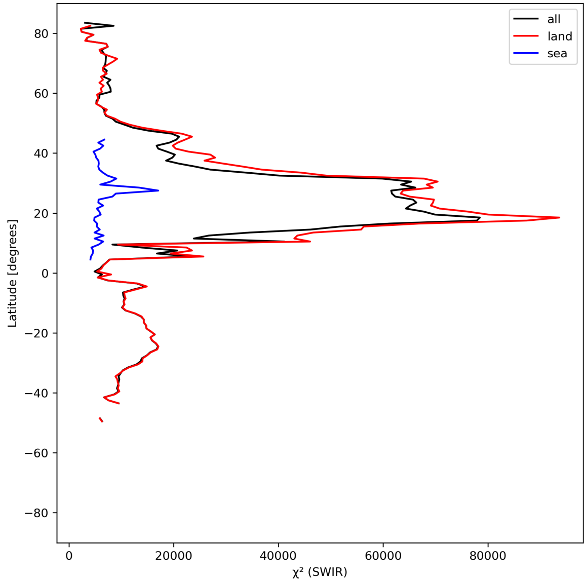
Figure 17: Zonal average of “ \chi^2 (SWIR)” for 2024-07-28 to 2024-07-30.
