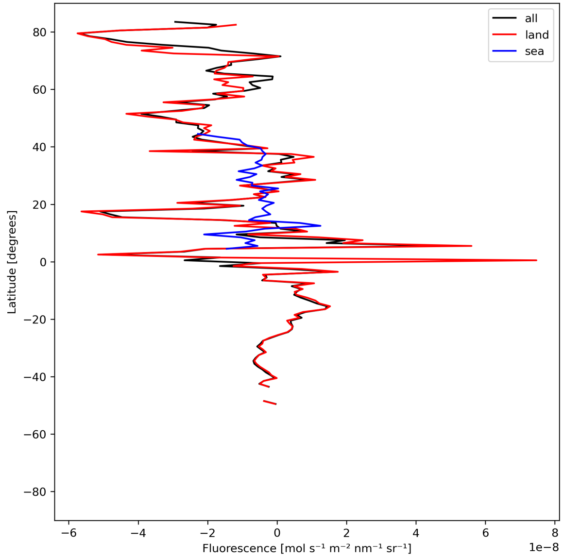
Figure 21: Zonal average of “Fluorescence” for 2024-07-28 to 2024-07-30.
