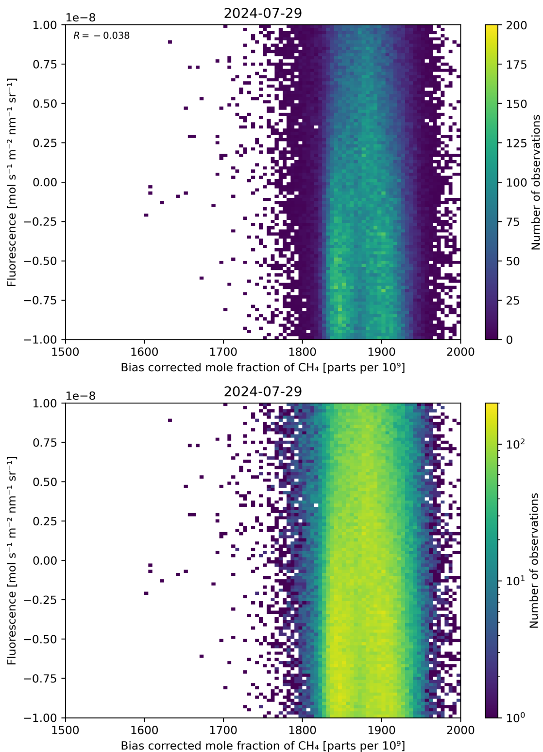
Figure 66: Scatter density plot of “Bias corrected mole fraction of \text{CH}_4 ” against “Fluorescence” for 2024-07-28 to 2024-07-30.
