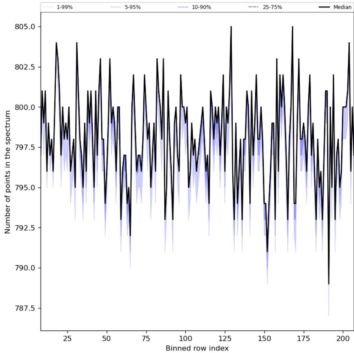
Figure 37: Along track statistics of “Number of points in the spectrum” for 2024-07-28 to 2024-07-30
