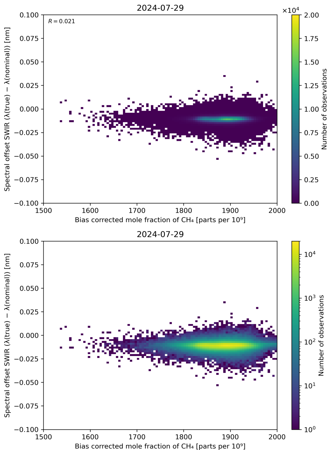
Figure 69: Scatter density plot of “Bias corrected mole fraction of \text{CH}_4 ” against “Spectral offset SWIR ( \lambda(\text{true}) - \lambda(\text{nominal}) )” for 2024-07-28 to 2024-07-30.
