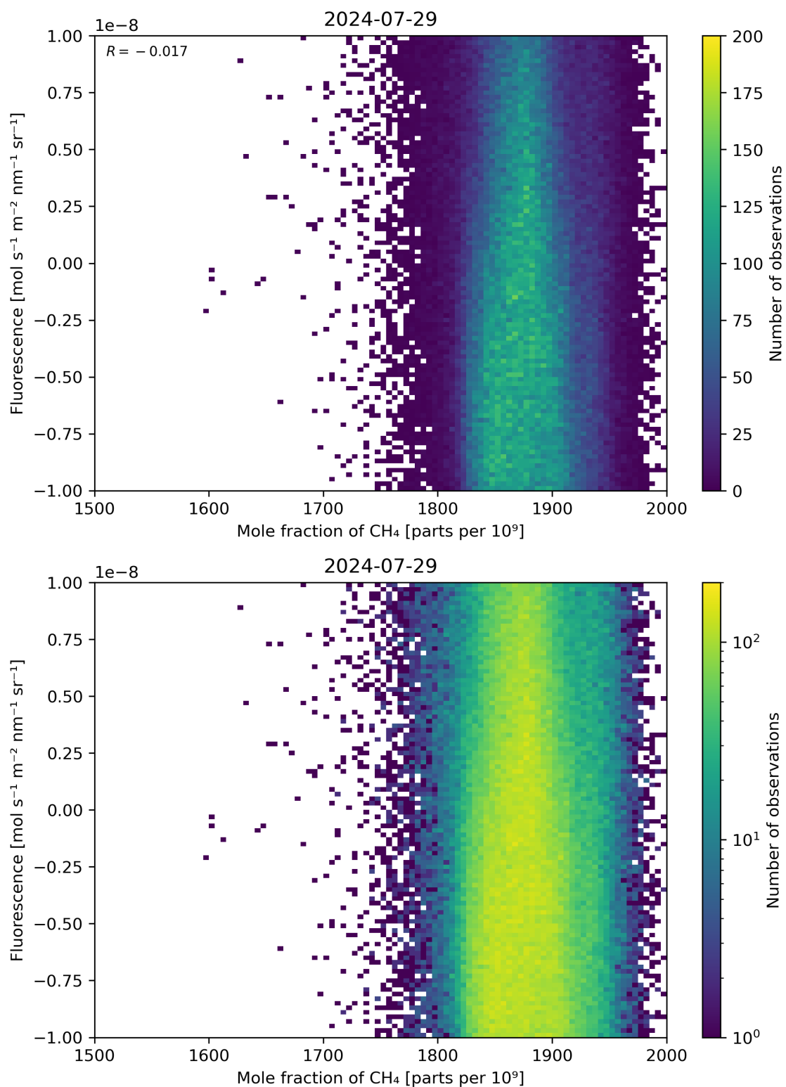
Figure 73: Scatter density plot of “Mole fraction of \text{CH}_4 ” against “Fluorescence” for 2024-07-28 to 2024-07-30.
