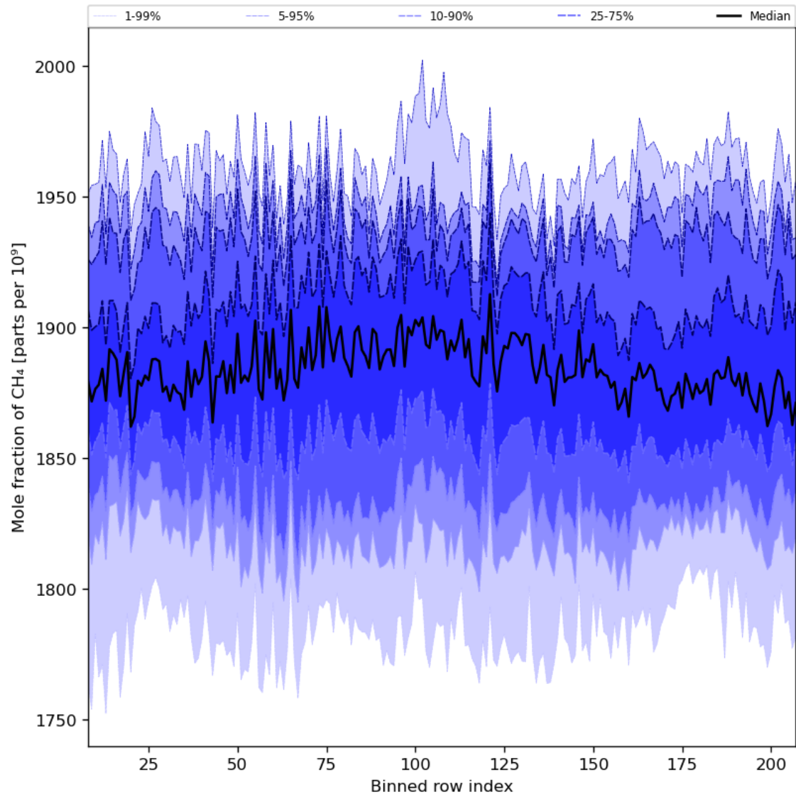
Figure 34: Along track statistics of “Mole fraction of CH 4 ” for 2024-07-28 to 2024-07-30
