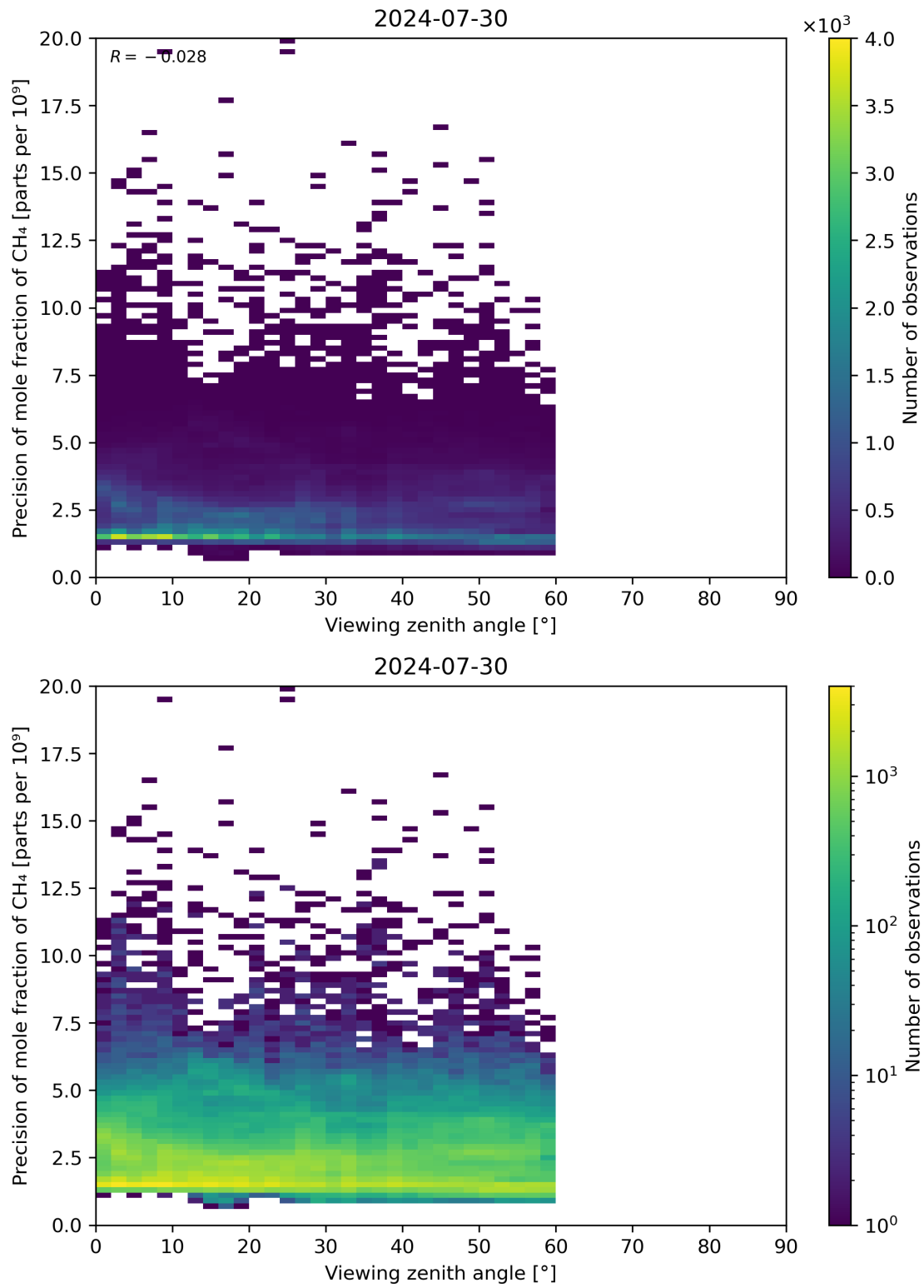
Figure 112: Scatter density plot of “Viewing zenith angle” against “Precision of mole fraction of CH 4 ” for 2024-07-29 to 2024-07-31.
