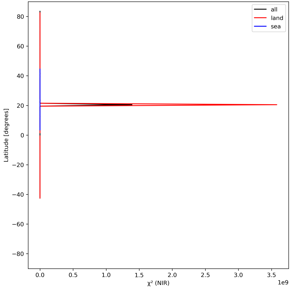
Figure 18: Zonal average of “ \chi^2 (NIR)” for 2024-07-29 to 2024-07-31.
