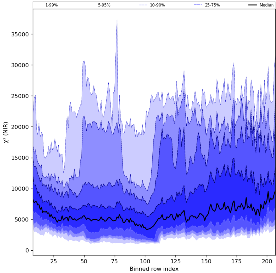
Figure 40: Along track statistics of “ \chi^2 (NIR)” for 2024-07-29 to 2024-07-31
