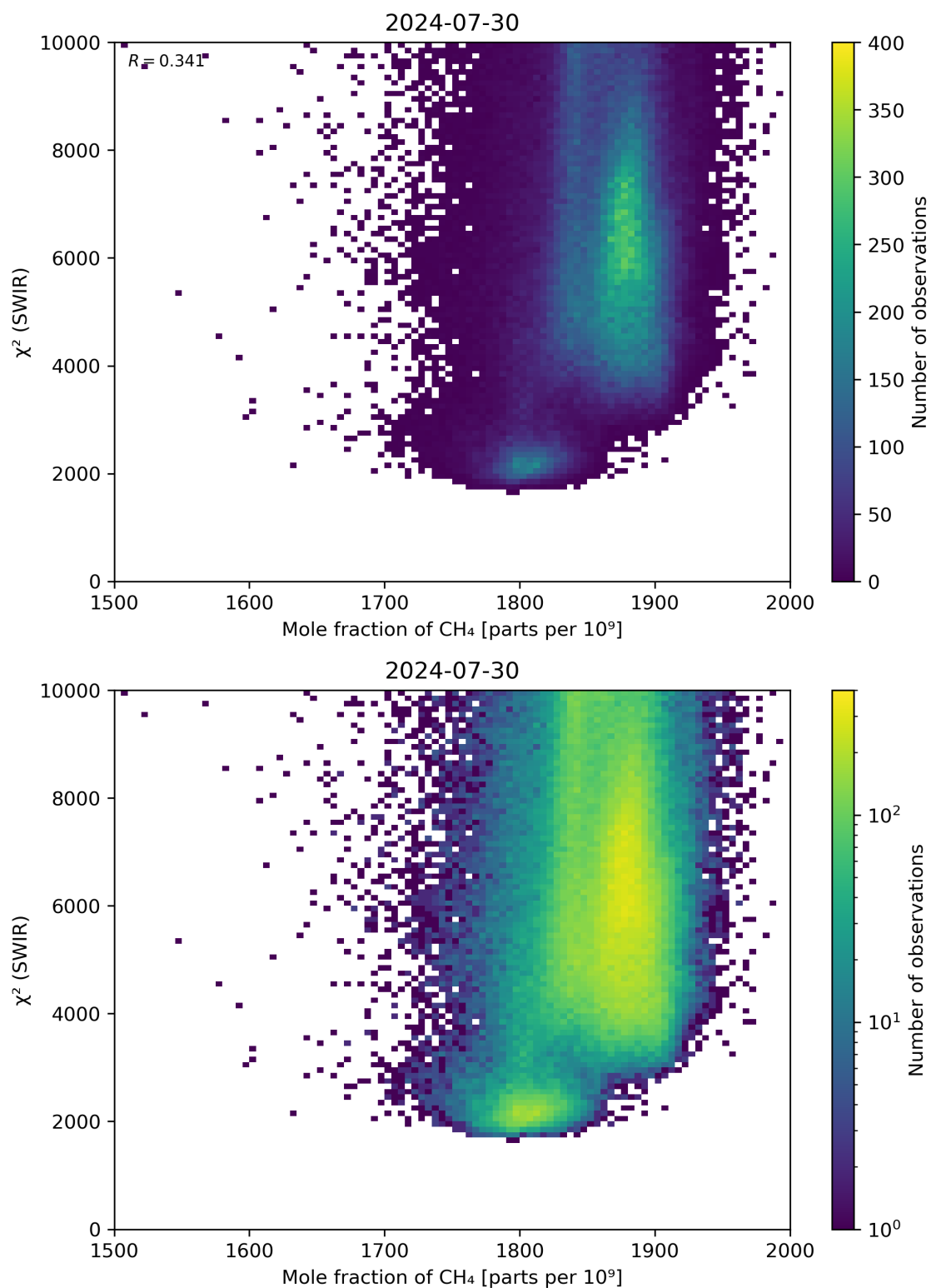
Figure 71: Scatter density plot of “Mole fraction of \text{CH}_4 ” against “ \chi^2 (SWIR)” for 2024-07-29 to 2024-07-31.
