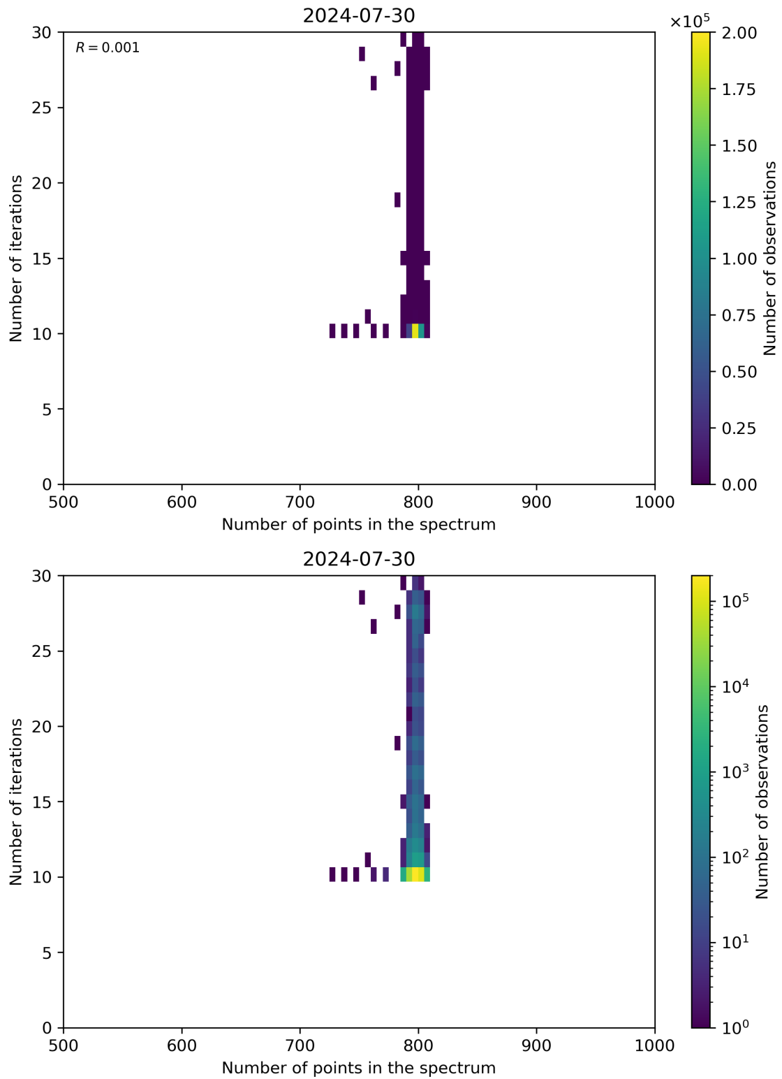
Figure 92: Scatter density plot of “Number of points in the spectrum” against “Number of iterations” for 2024-07-29 to 2024-07-31.
