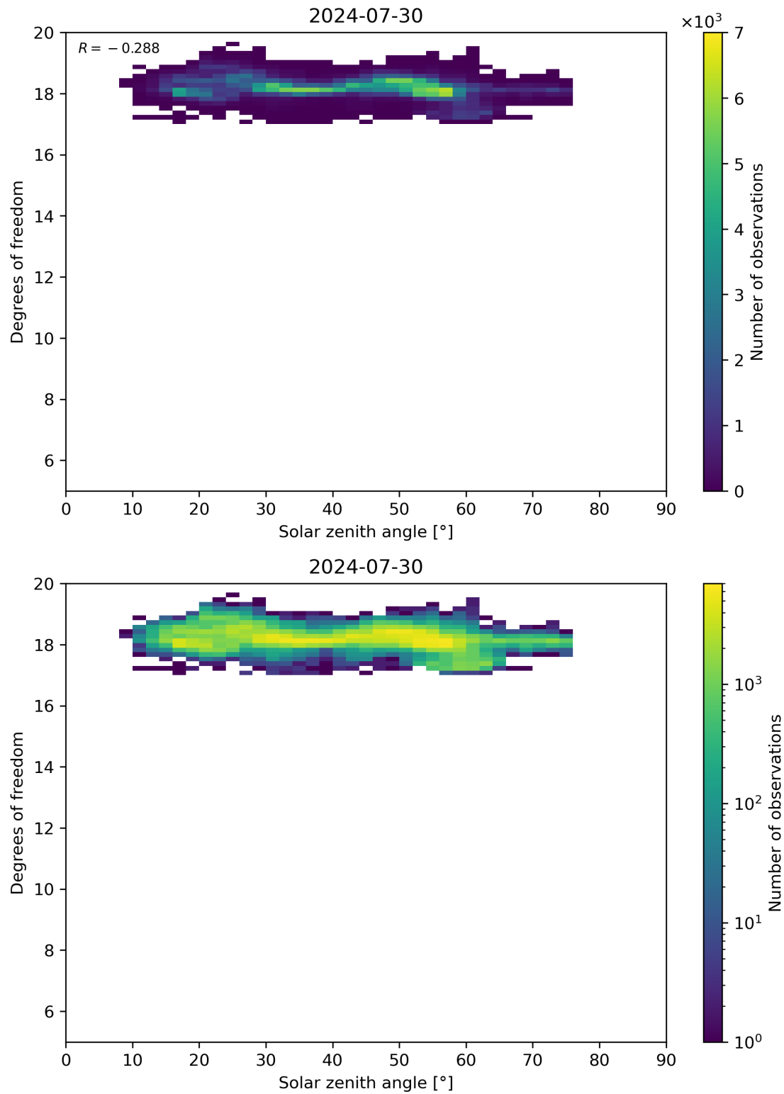
Figure 96: Scatter density plot of “Solar zenith angle” against “Degrees of freedom” for 2024-07-29 to 2024-07-31.
