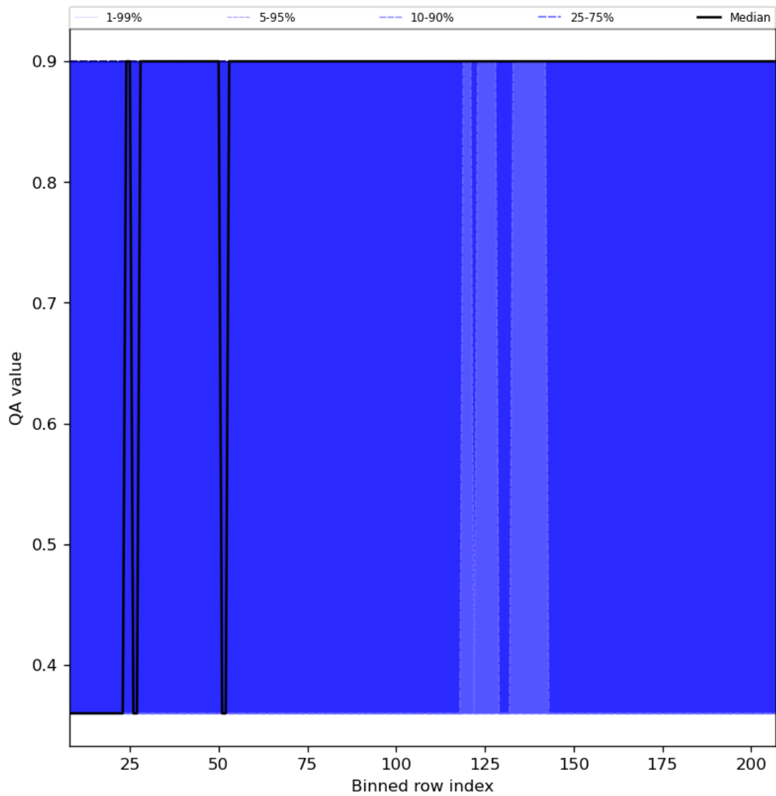
Figure 33: Along track statistics of “QA value” for 2024-07-29 to 2024-07-31
