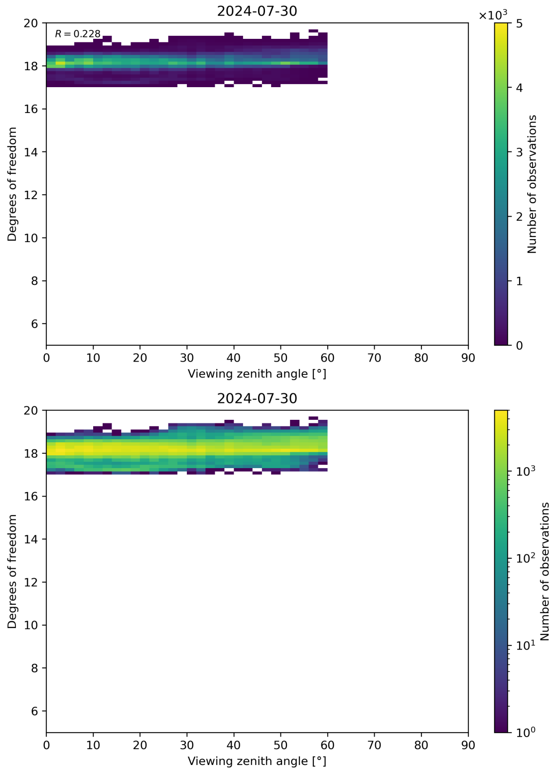
Figure 107: Scatter density plot of “Viewing zenith angle” against “Degrees of freedom” for 2024-07-29 to 2024-07-31.
