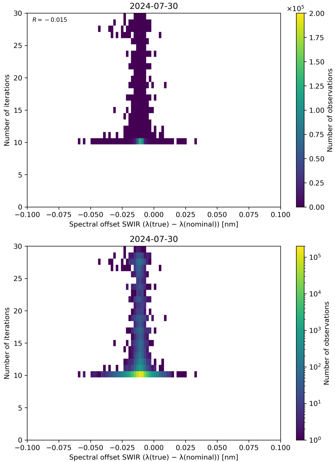
Figure 121: Scatter density plot of “Spectral offset SWIR ( \lambda(\text{true}) - \lambda(\text{nominal}) )” against “Number of iterations” for 2024-07-29 to 2024-07-31.
