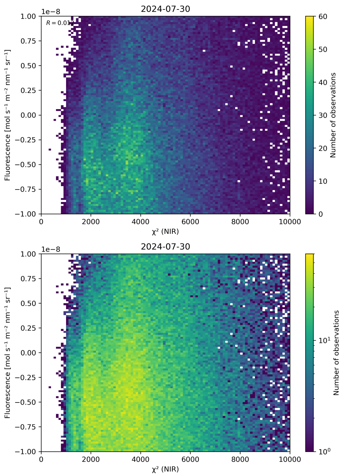
Figure 45: Scatter density plot of “ \chi^2 (NIR)” against “Fluorescence” for 2024-07-29 to 2024-07-31.
