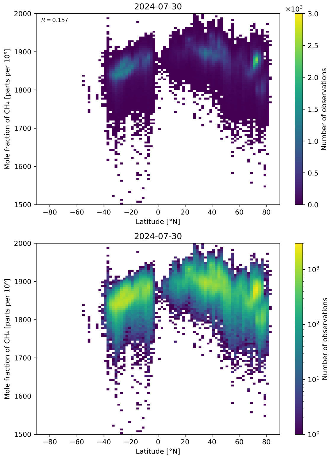
Figure 57: Scatter density plot of “Latitude” against “Mole fraction of CH 4 ” for 2024-07-29 to 2024-07-31.
