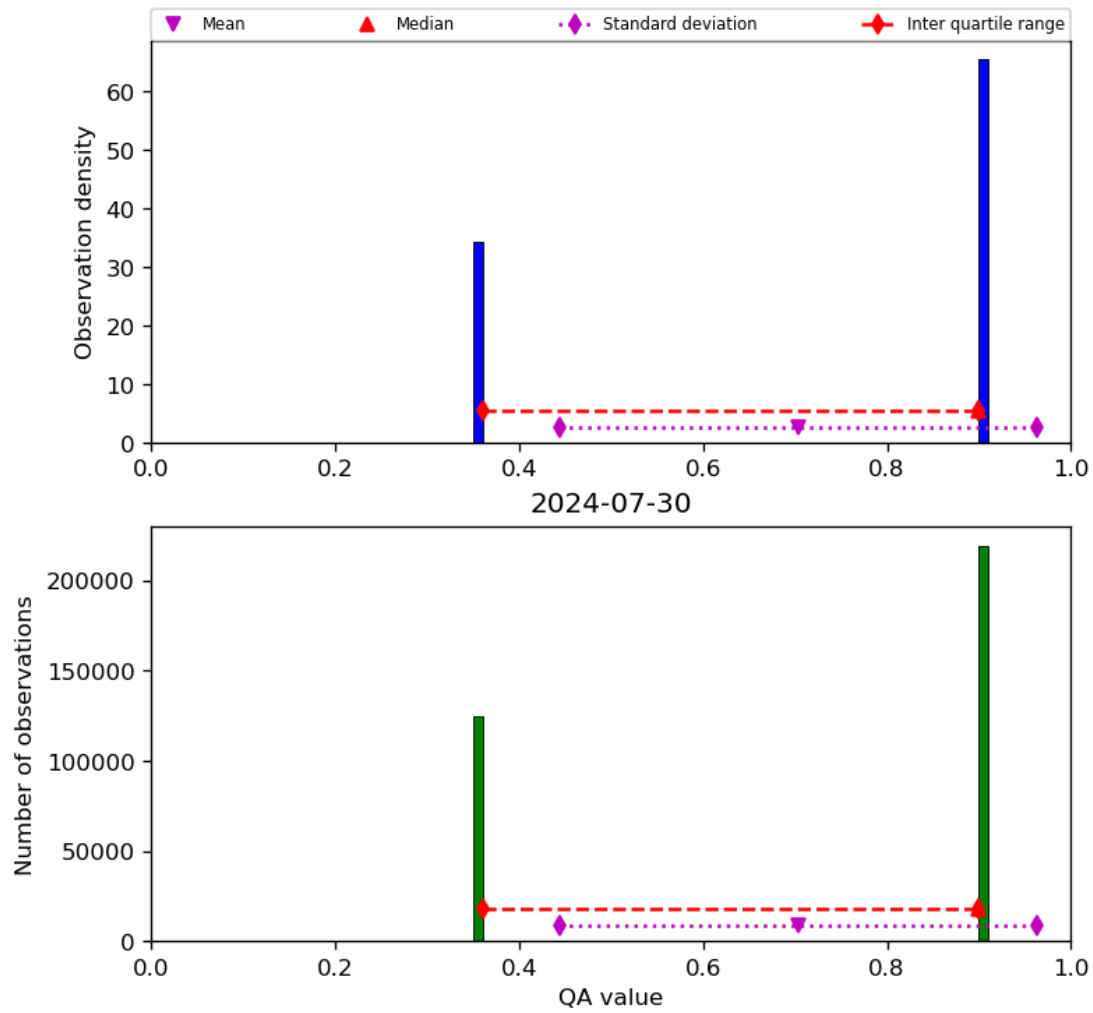
Figure 22: Histogram of “QA value” for 2024-07-29 to 2024-07-31
