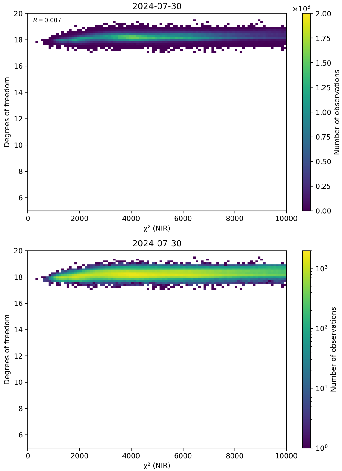
Figure 44: Scatter density plot of “ \chi^2 (NIR)” against “Degrees of freedom” for 2024-07-29 to 2024-07-31.
