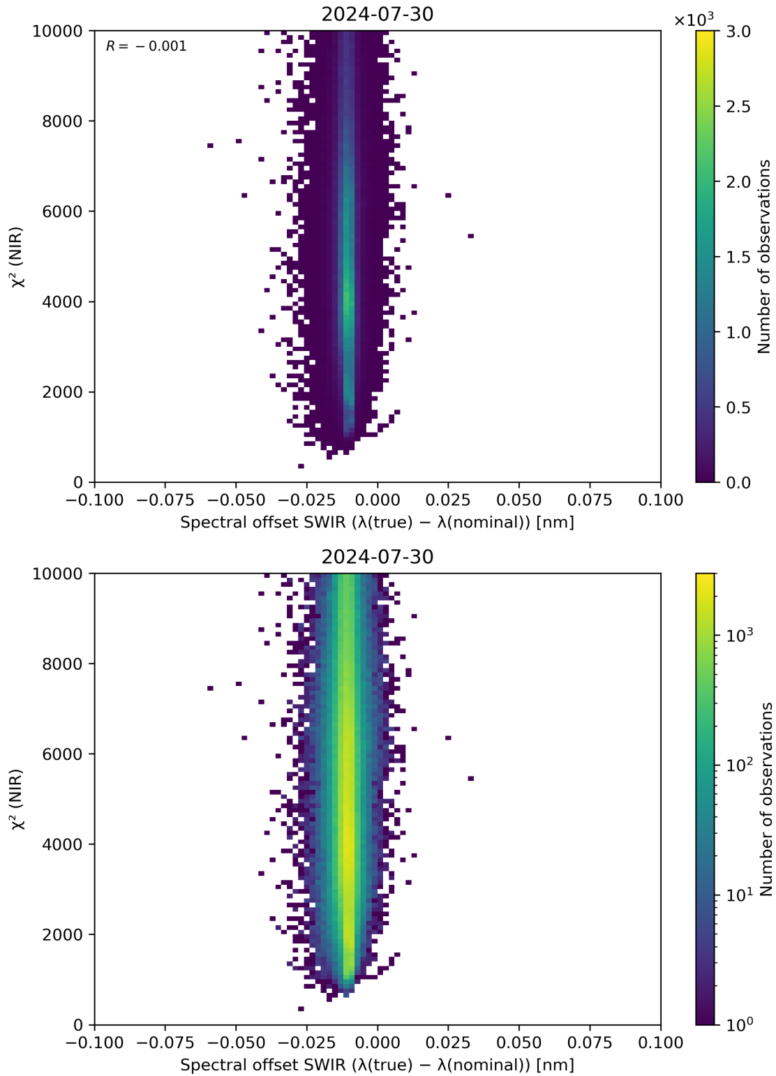
Figure 117: Scatter density plot of “Spectral offset SWIR ( \lambda(\text{true}) - \lambda(\text{nominal}) )” against “ \chi^2 (NIR)” for 2024-07-29 to 2024-07-31.
