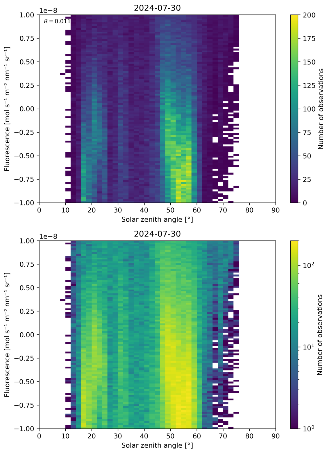
Figure 97: Scatter density plot of “Solar zenith angle” against “Fluorescence” for 2024-07-29 to 2024-07-31.
