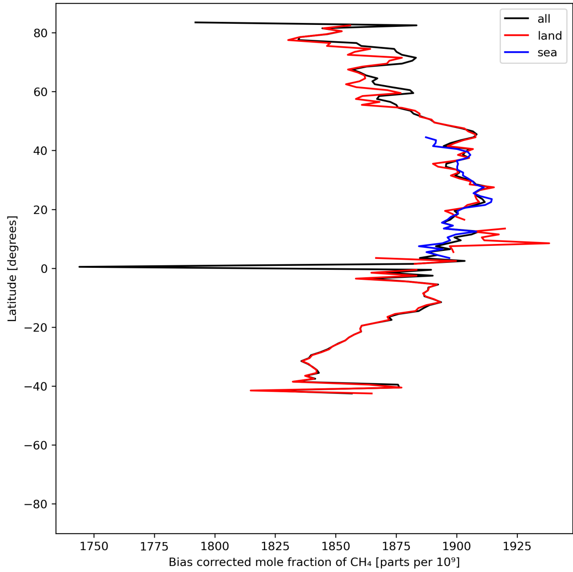
Figure 14: Zonal average of “Bias corrected mole fraction of CH 4 ” for 2024-07-29 to 2024-07-31.
