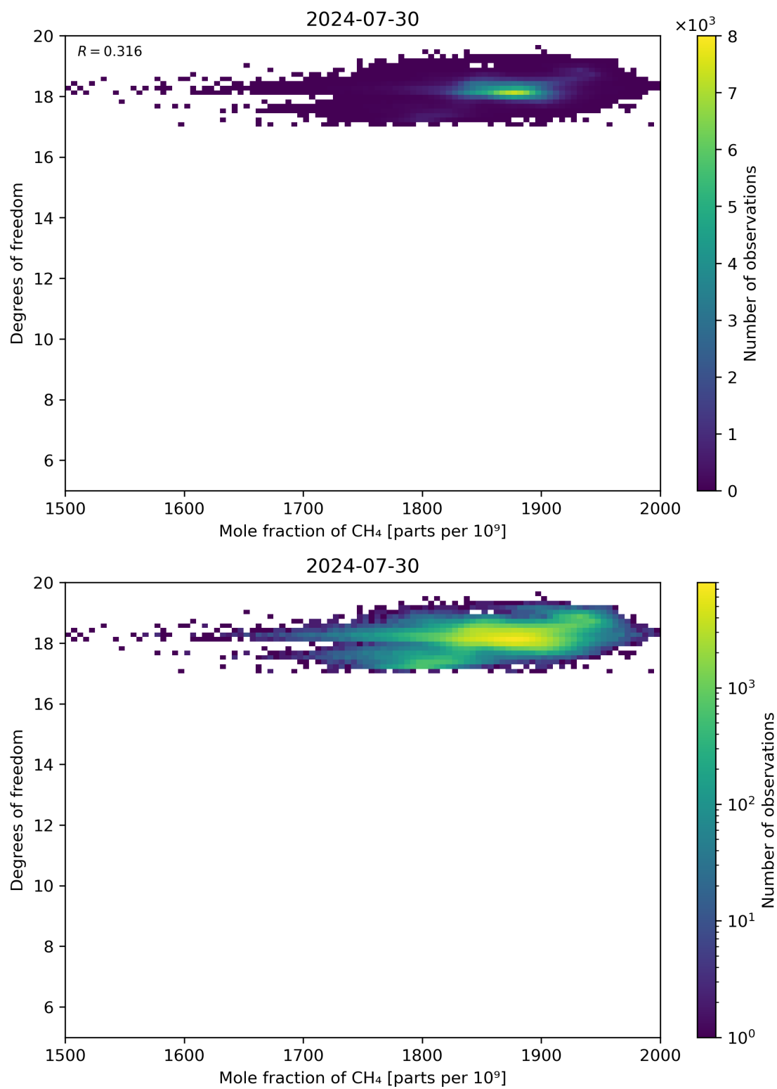
Figure 72: Scatter density plot of “Mole fraction of CH 4 ” against “Degrees of freedom” for 2024-07-29 to 2024-07-31.
