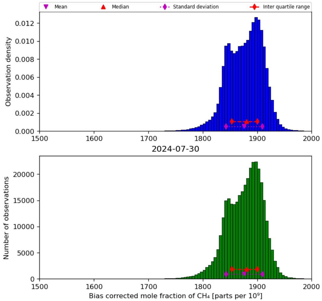
Figure 25: Histogram of “Bias corrected mole fraction of CH 4 ” for 2024-07-29 to 2024-07-31
