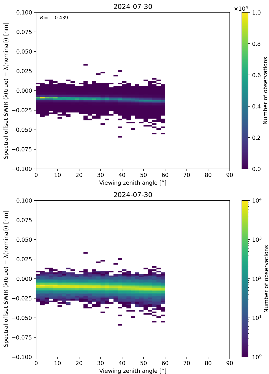
Figure 116: Scatter density plot of “Viewing zenith angle” against “Spectral offset SWIR ( \lambda(\text{true}) - \lambda(\text{nominal}) )” for 2024-07-29 to 2024-07-31.
