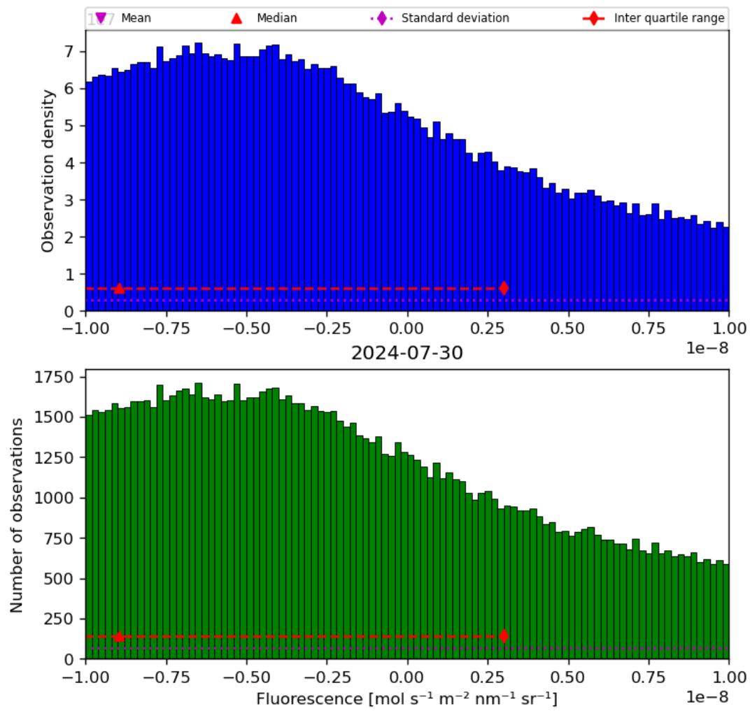
Figure 32: Histogram of “Fluorescence” for 2024-07-29 to 2024-07-31
