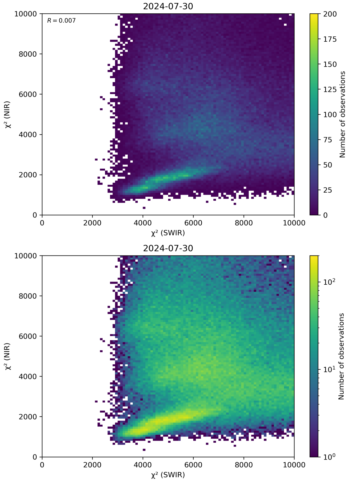
Figure 47: Scatter density plot of “ \chi^2 (SWIR)” against “ \chi^2 (NIR)” for 2024-07-29 to 2024-07-31.
