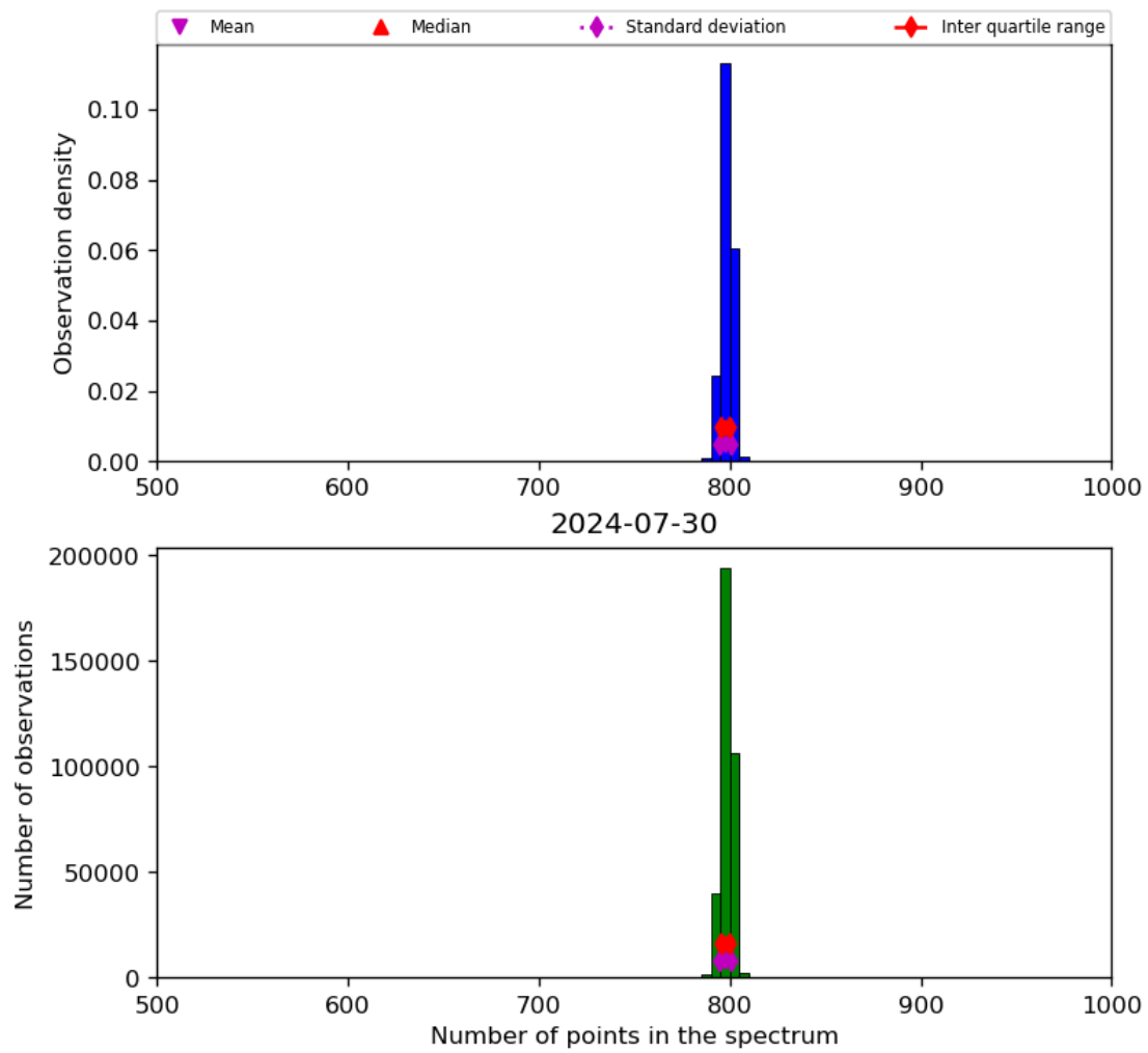
Figure 26: Histogram of “Number of points in the spectrum” for 2024-07-29 to 2024-07-31
