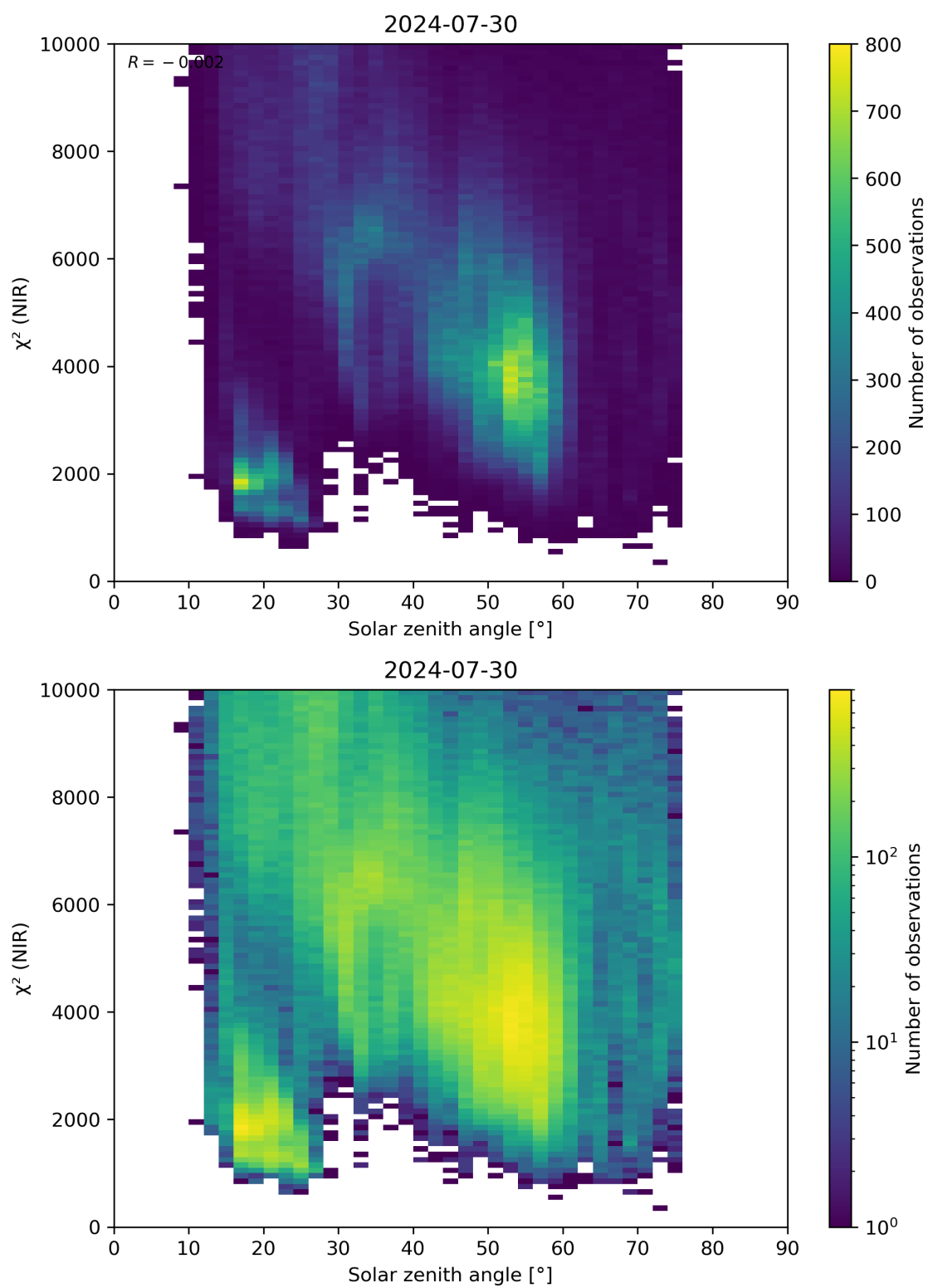
Figure 94: Scatter density plot of “Solar zenith angle” against “ \chi^2 (NIR)” for 2024-07-29 to 2024-07-31.
