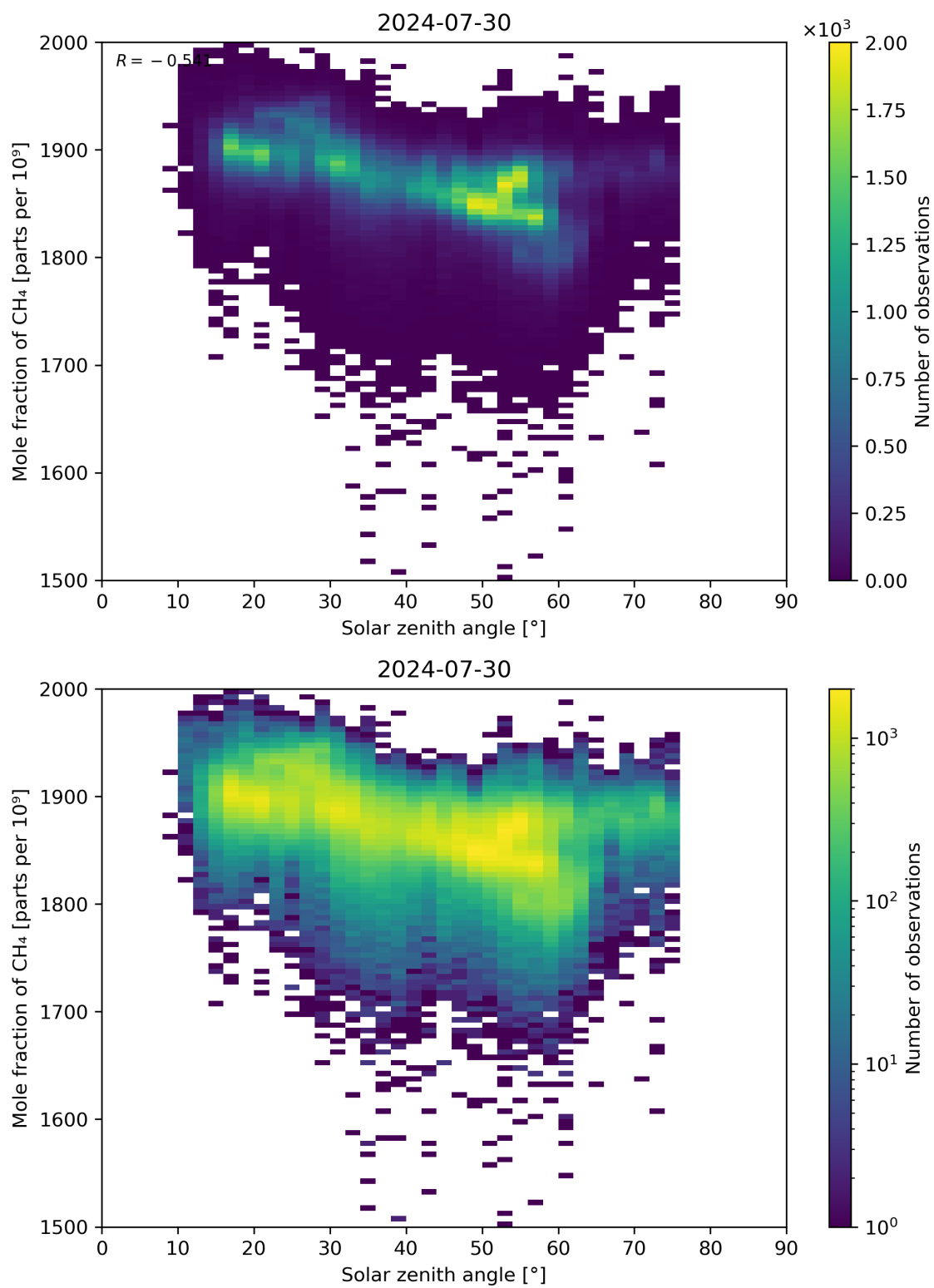
Figure 99: Scatter density plot of “Solar zenith angle” against “Mole fraction of CH 4 ” for 2024-07-29 to 2024-07-31.
