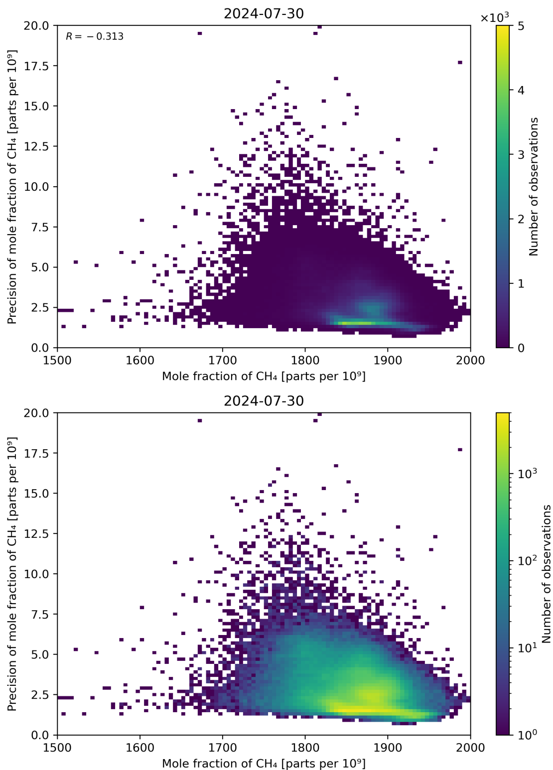
Figure 75: Scatter density plot of “Mole fraction of CH 4 ” against “Precision of mole fraction of CH 4 ” for 2024-07-29 to 2024-07-31.
