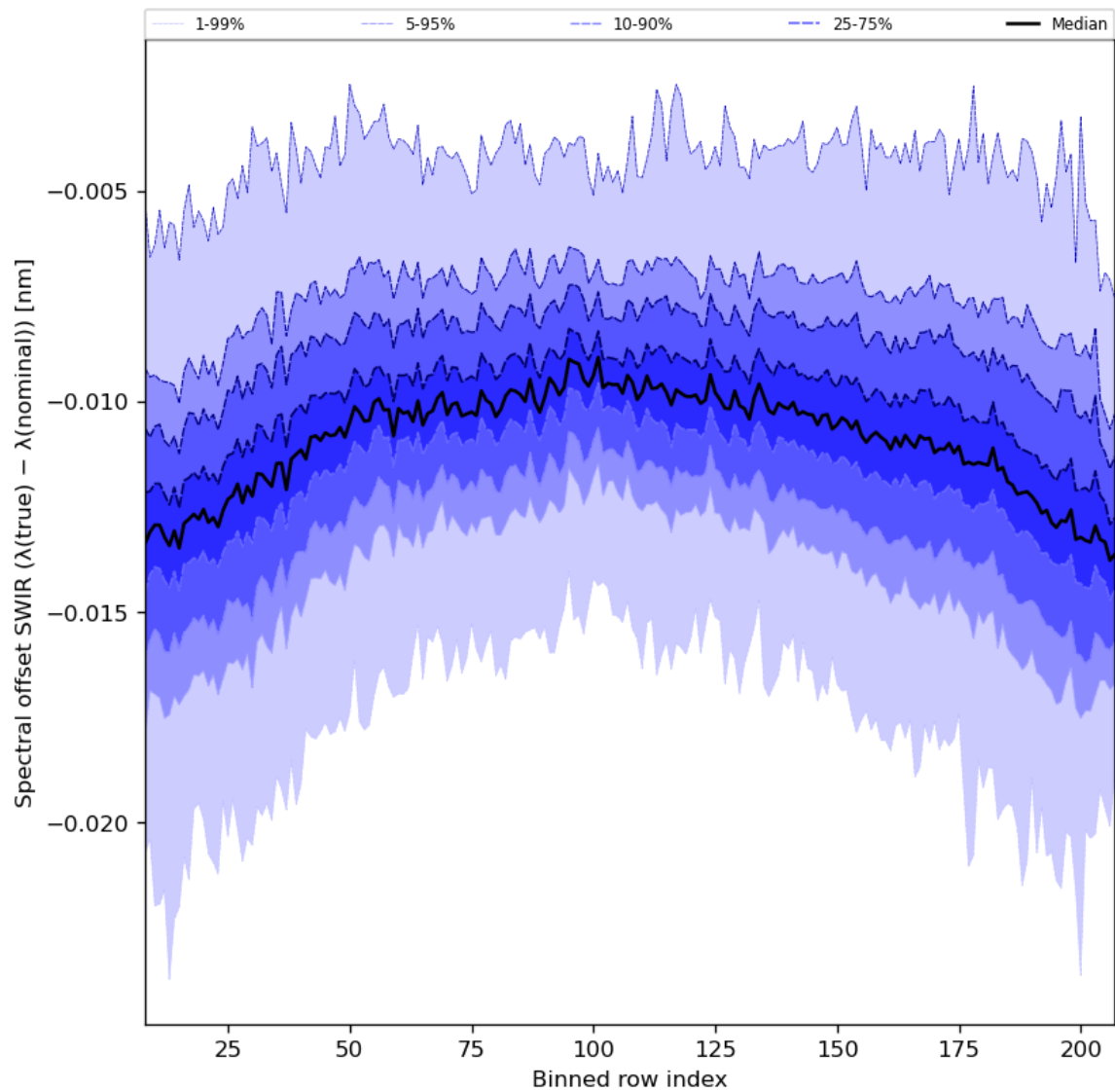
Figure 38: Along track statistics of “Spectral offset SWIR ( \lambda(\text{true}) - \lambda(\text{nominal}) )” for 2024-07-29 to 2024-07-31
