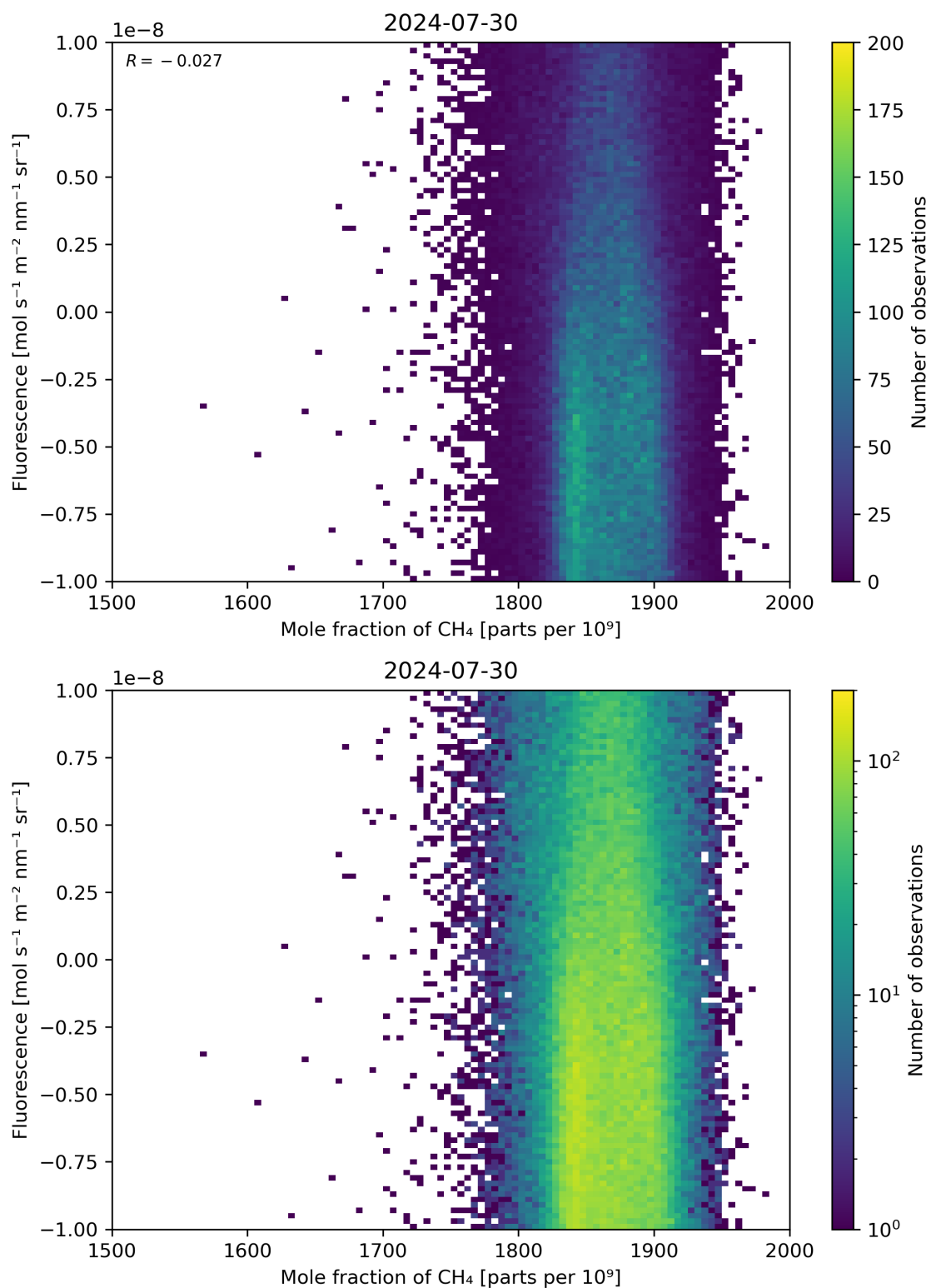
Figure 73: Scatter density plot of “Mole fraction of \text{CH}_4 ” against “Fluorescence” for 2024-07-29 to 2024-07-31.
