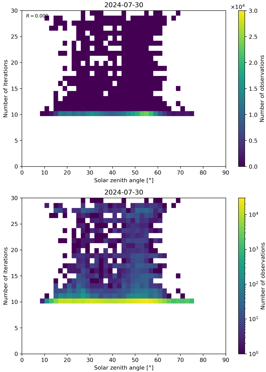
Figure 102: Scatter density plot of “Solar zenith angle” against “Number of iterations” for 2024-07-29 to 2024-07-31.
