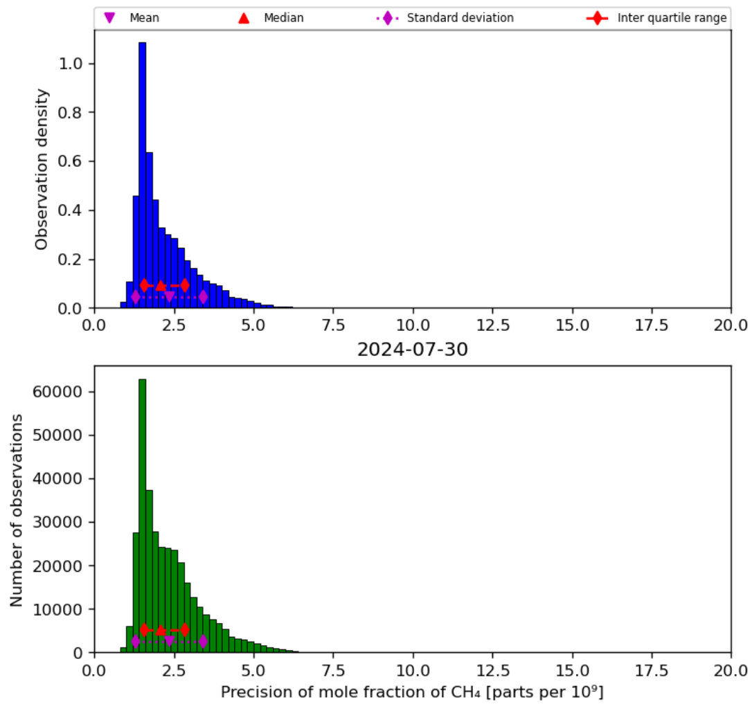
Figure 24: Histogram of “Precision of mole fraction of CH 4 ” for 2024-07-29 to 2024-07-31
