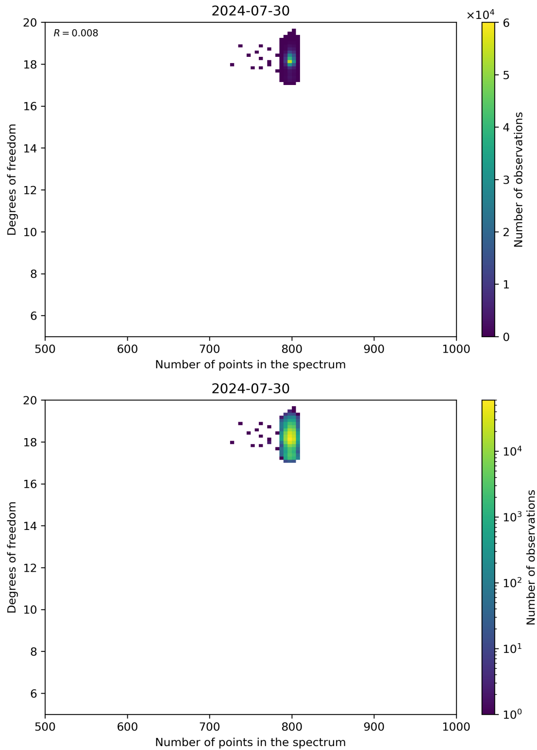
Figure 90: Scatter density plot of “Number of points in the spectrum” against “Degrees of freedom” for 2024-07-29 to 2024-07-31.
