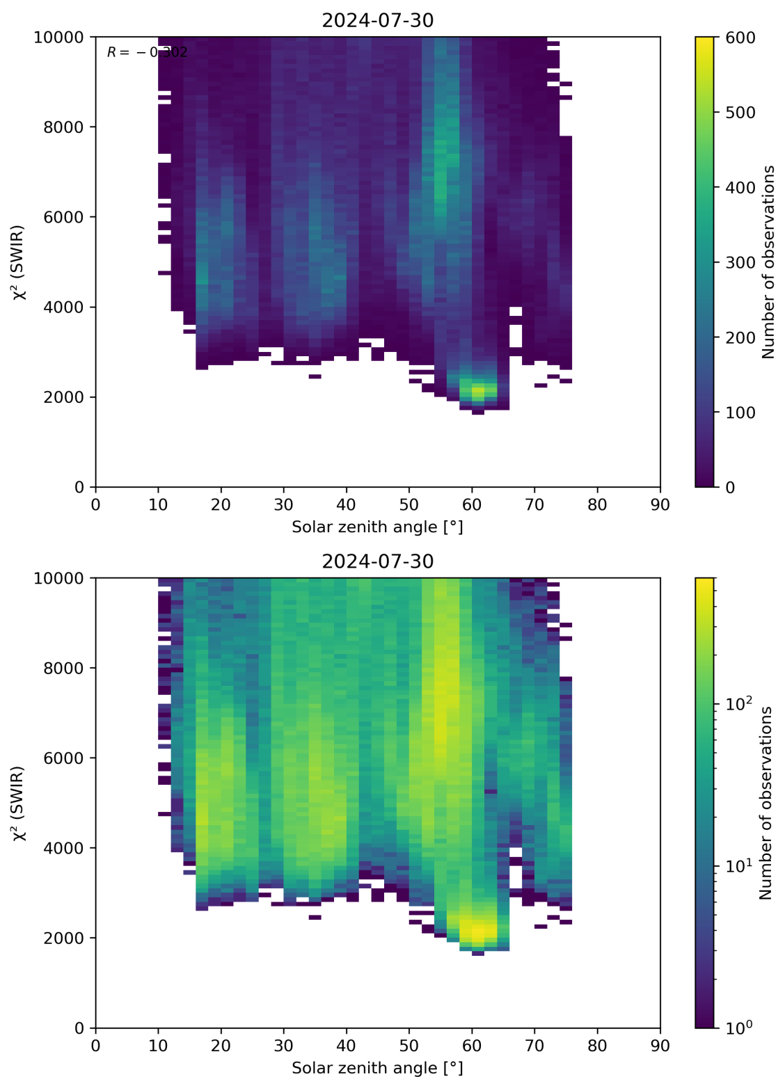
Figure 95: Scatter density plot of “Solar zenith angle” against “ \chi^2 (SWIR)” for 2024-07-29 to 2024-07-31.
