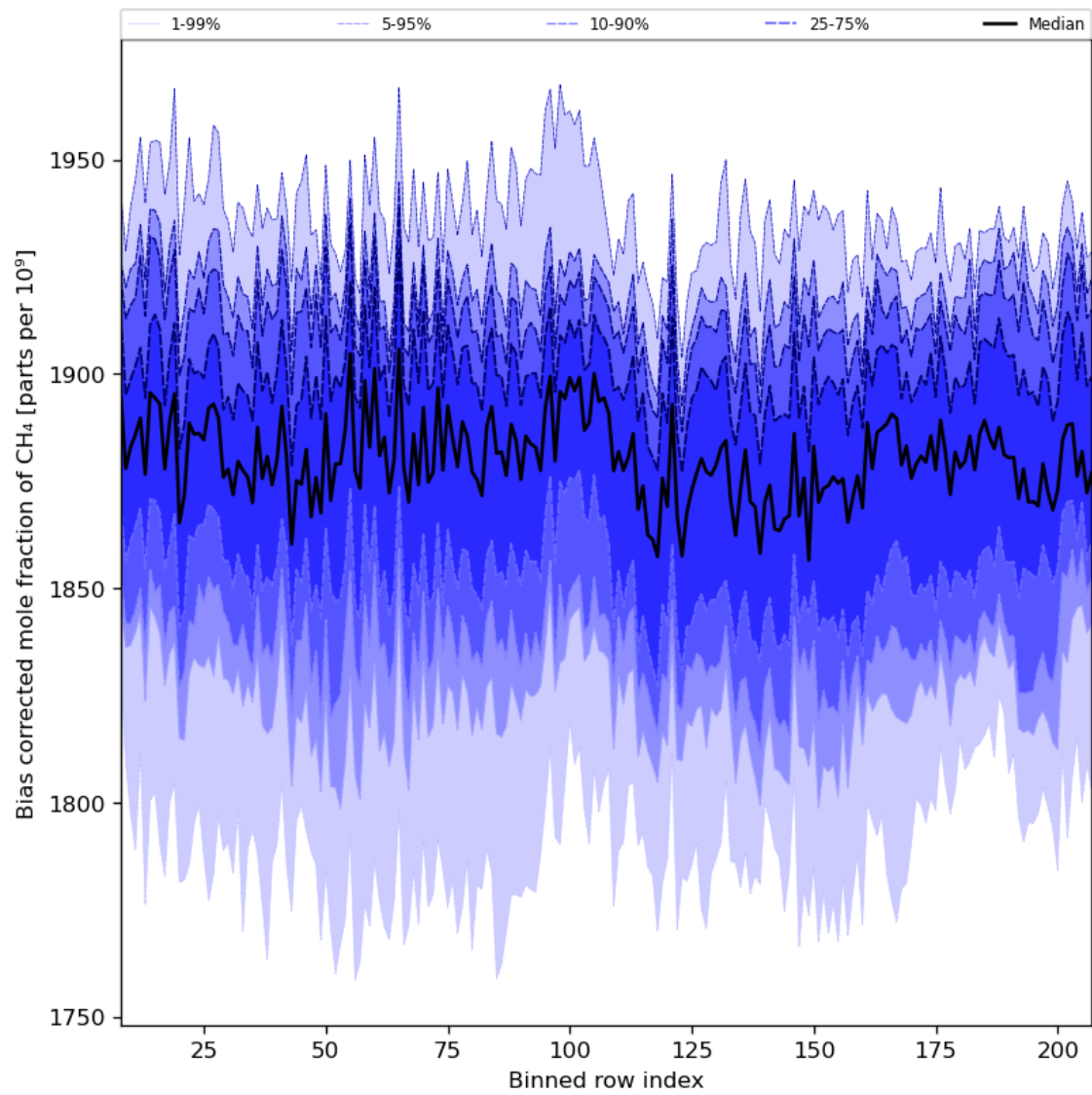
Figure 36: Along track statistics of “Bias corrected mole fraction of CH 4 ” for 2024-07-29 to 2024-07-31
