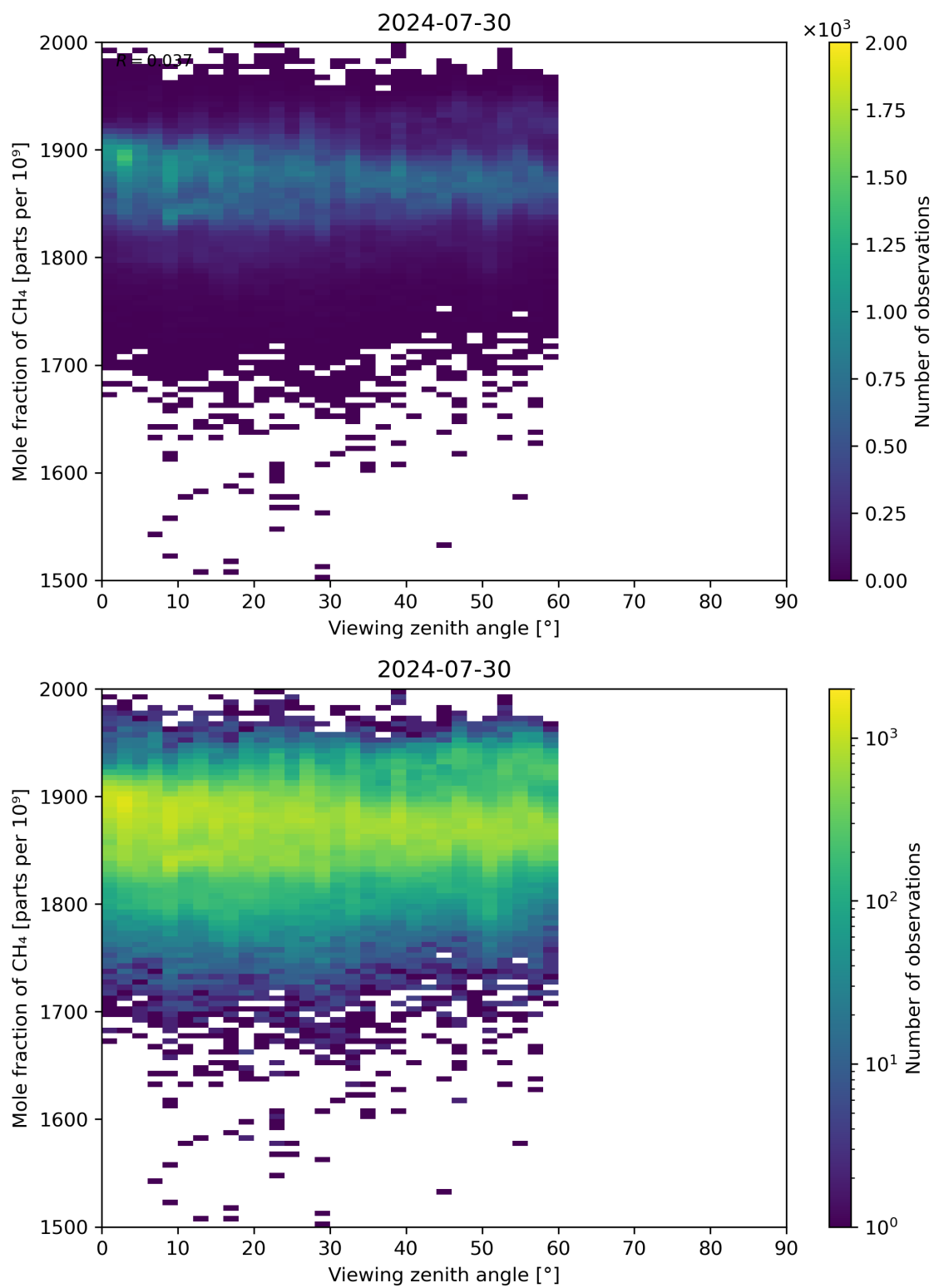
Figure 110: Scatter density plot of “Viewing zenith angle” against “Mole fraction of CH 4 ” for 2024-07-29 to 2024-07-31.
