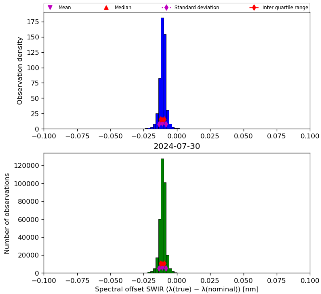
Figure 27: Histogram of “Spectral offset SWIR ( \lambda(\text{true}) - \lambda(\text{nominal}) )” for 2024-07-29 to 2024-07-31
