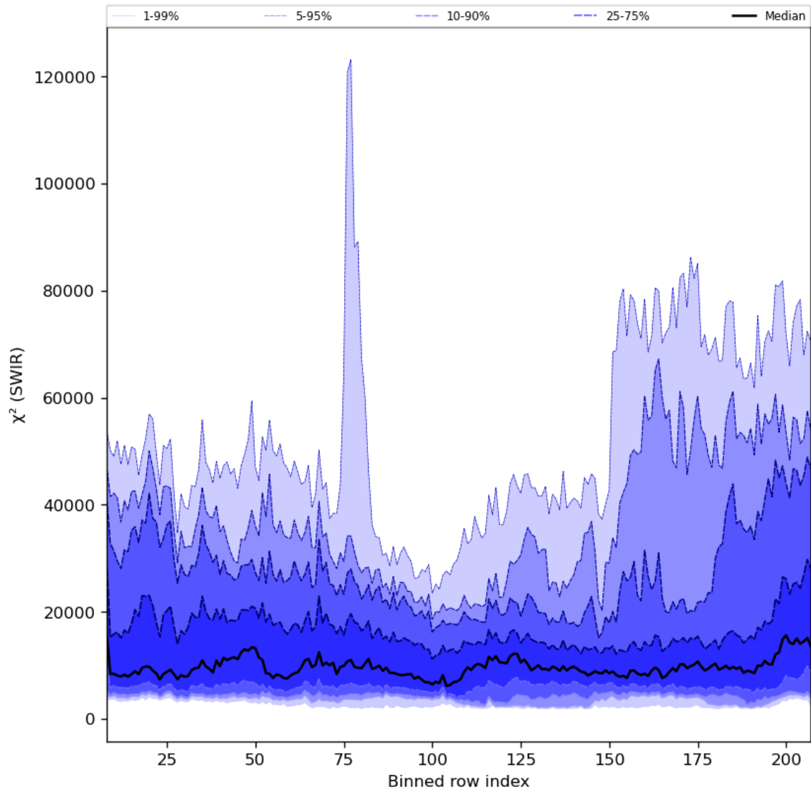
Figure 39: Along track statistics of " \chi^2 (SWIR)" for 2024-07-29 to 2024-07-31
