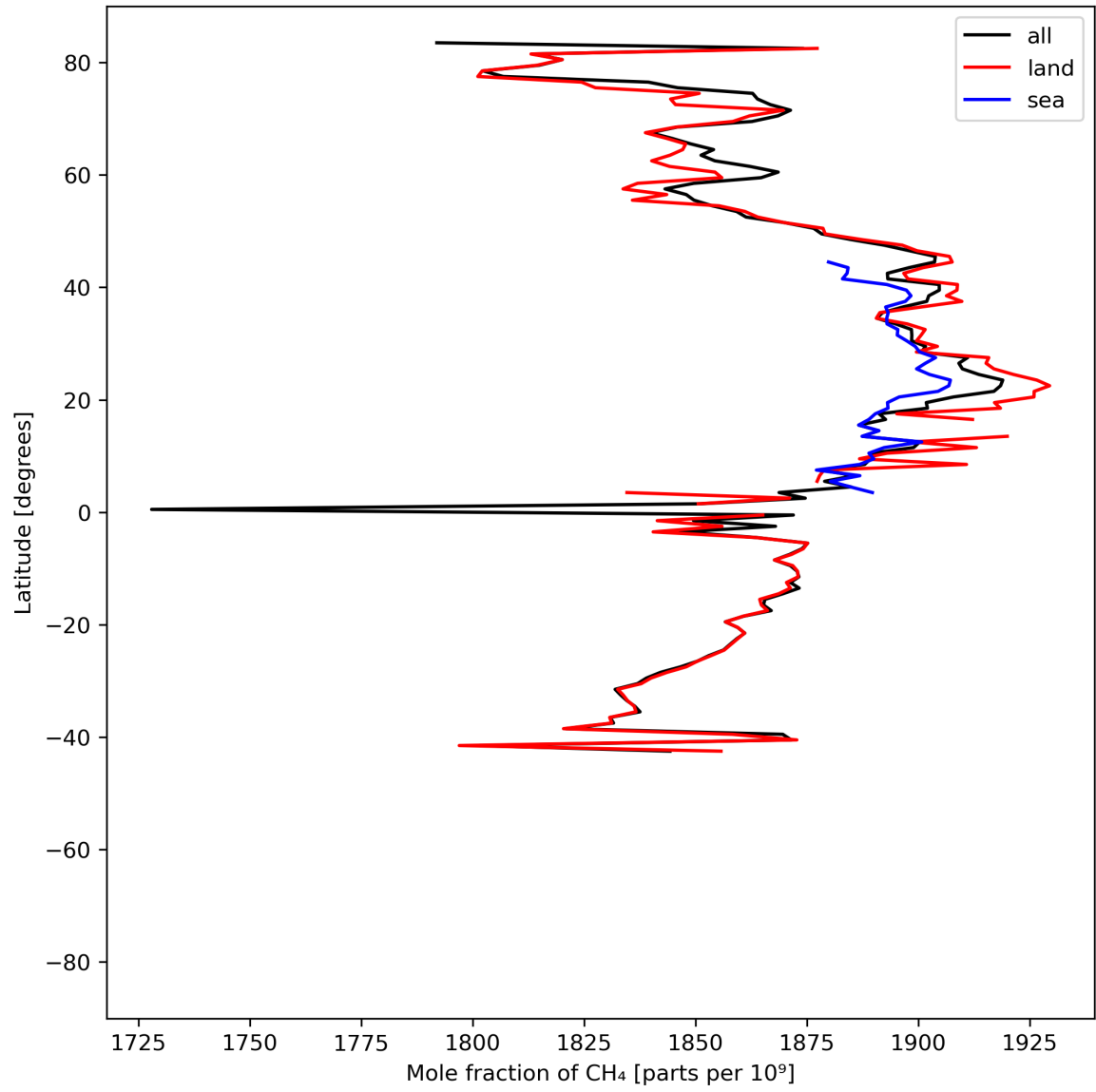
Figure 12: Zonal average of “Mole fraction of CH 4 ” for 2024-07-29 to 2024-07-31.
