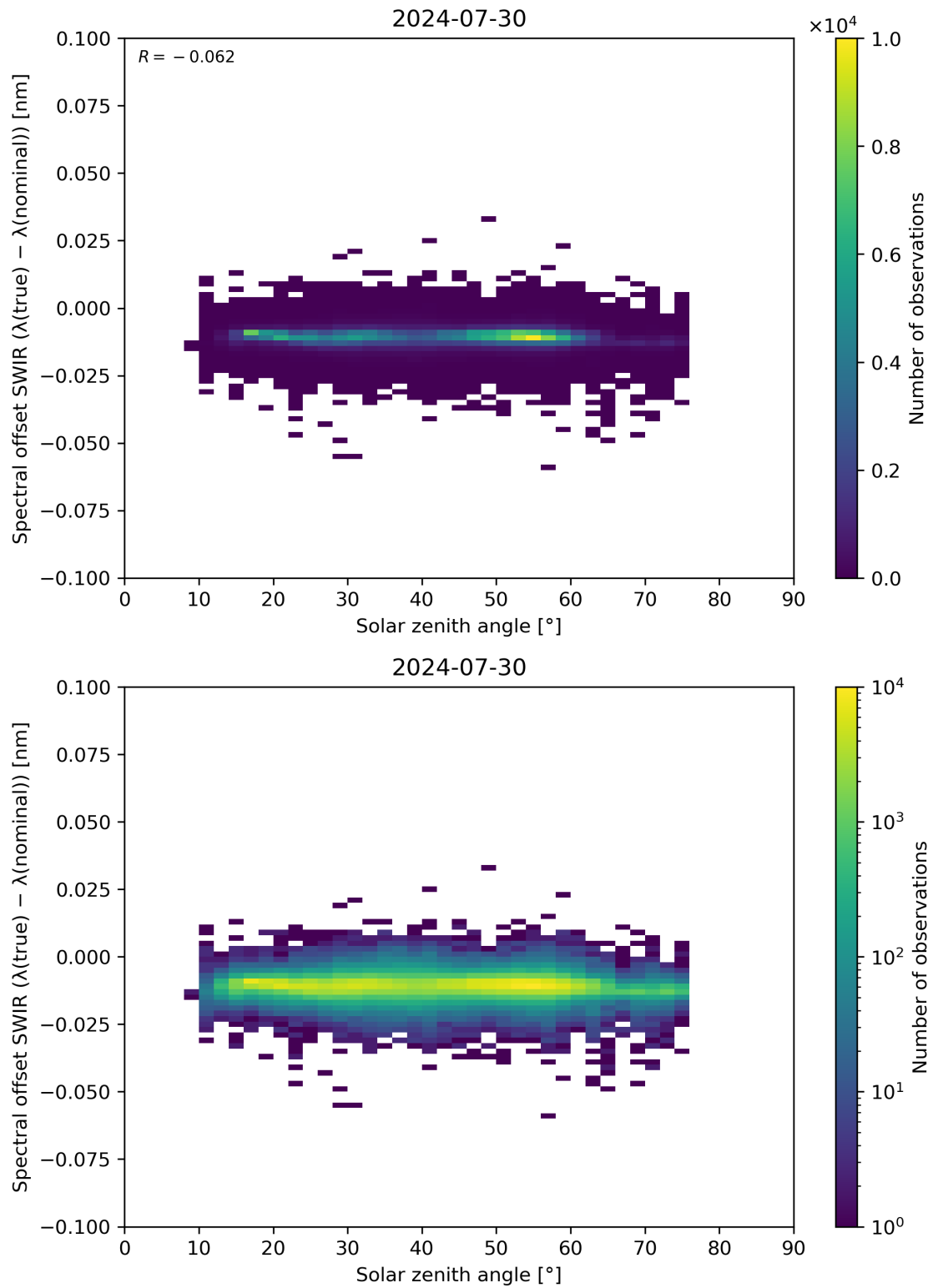
Figure 104: Scatter density plot of “Solar zenith angle” against “Spectral offset SWIR ( \lambda(\text{true}) - \lambda(\text{nominal}) )” for 2024-07-29 to 2024-07-31.
