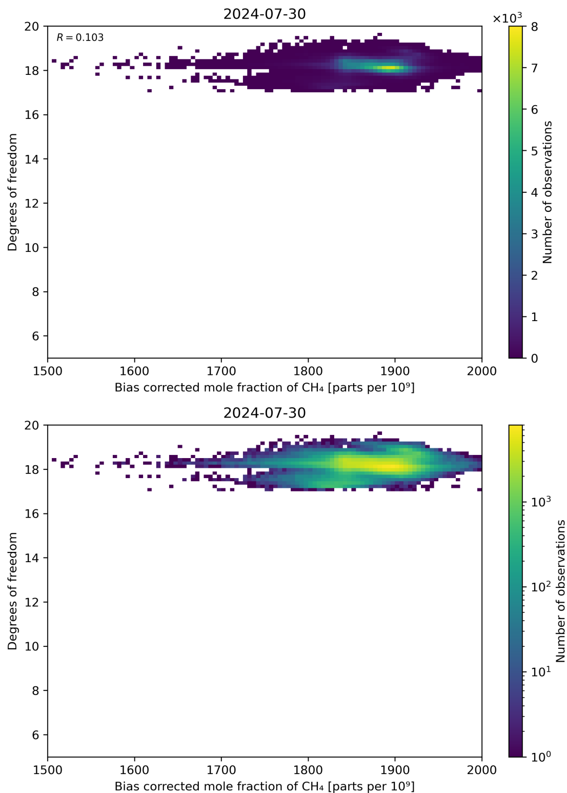
Figure 65: Scatter density plot of “Bias corrected mole fraction of CH 4 ” against “Degrees of freedom” for 2024-07-29 to 2024-07-31.
