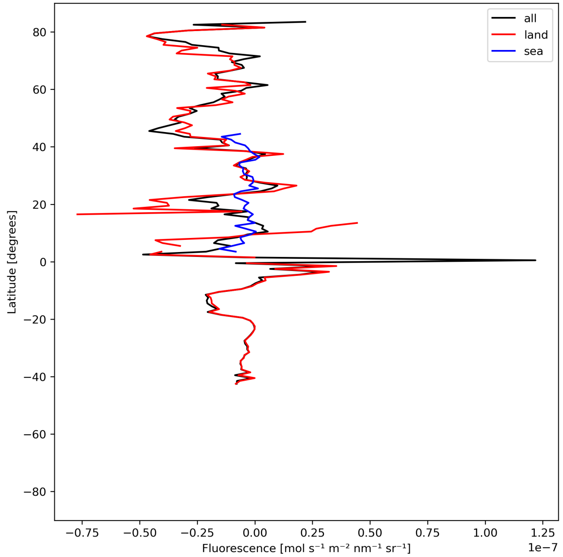
Figure 21: Zonal average of “Fluorescence” for 2024-07-29 to 2024-07-31.
