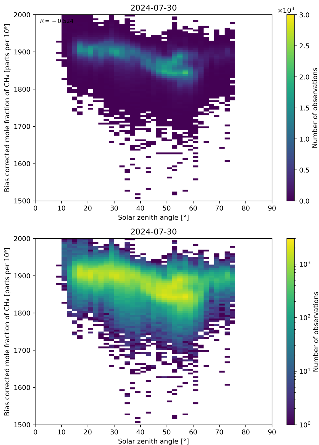
Figure 100: Scatter density plot of “Solar zenith angle” against “Bias corrected mole fraction of CH 4 ” for 2024-07-29 to 2024-07-31.
