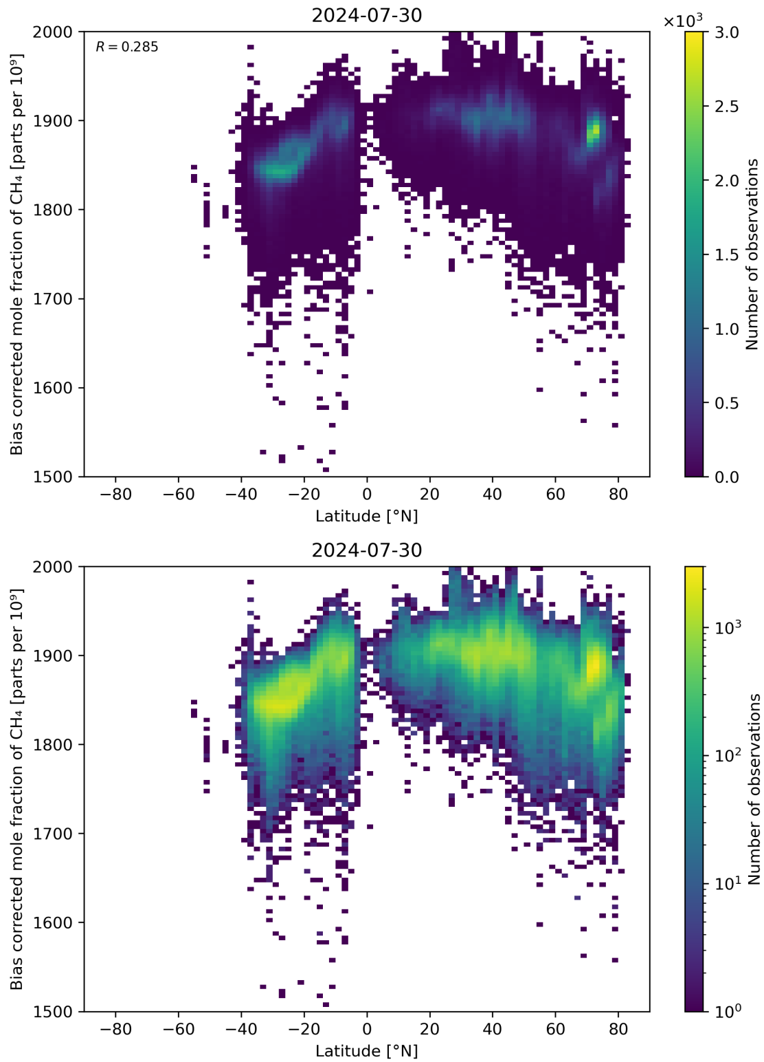
Figure 58: Scatter density plot of “Latitude” against “Bias corrected mole fraction of CH 4 ” for 2024-07-29 to 2024-07-31.
