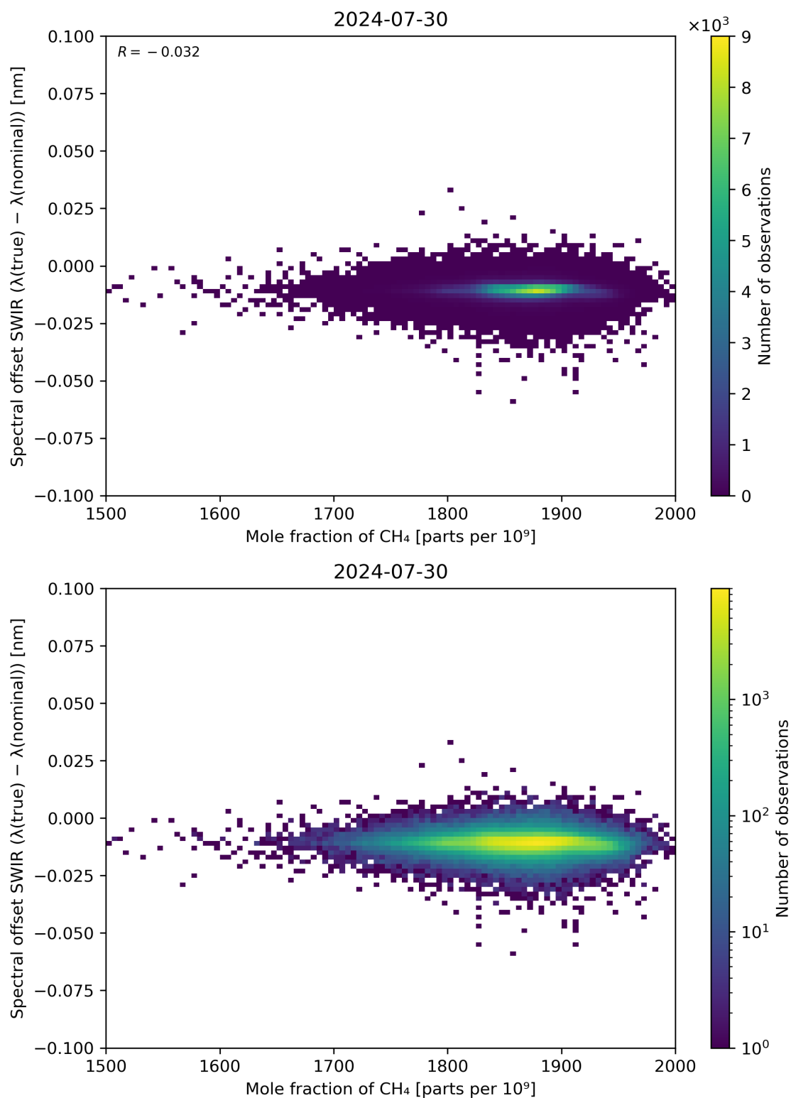
Figure 86: Scatter density plot of “Mole fraction of CH 4 ” against “Spectral offset SWIR ( \lambda(\text{true}) - \lambda(\text{nominal}) )” for 2024-07-29 to 2024-07-31.
