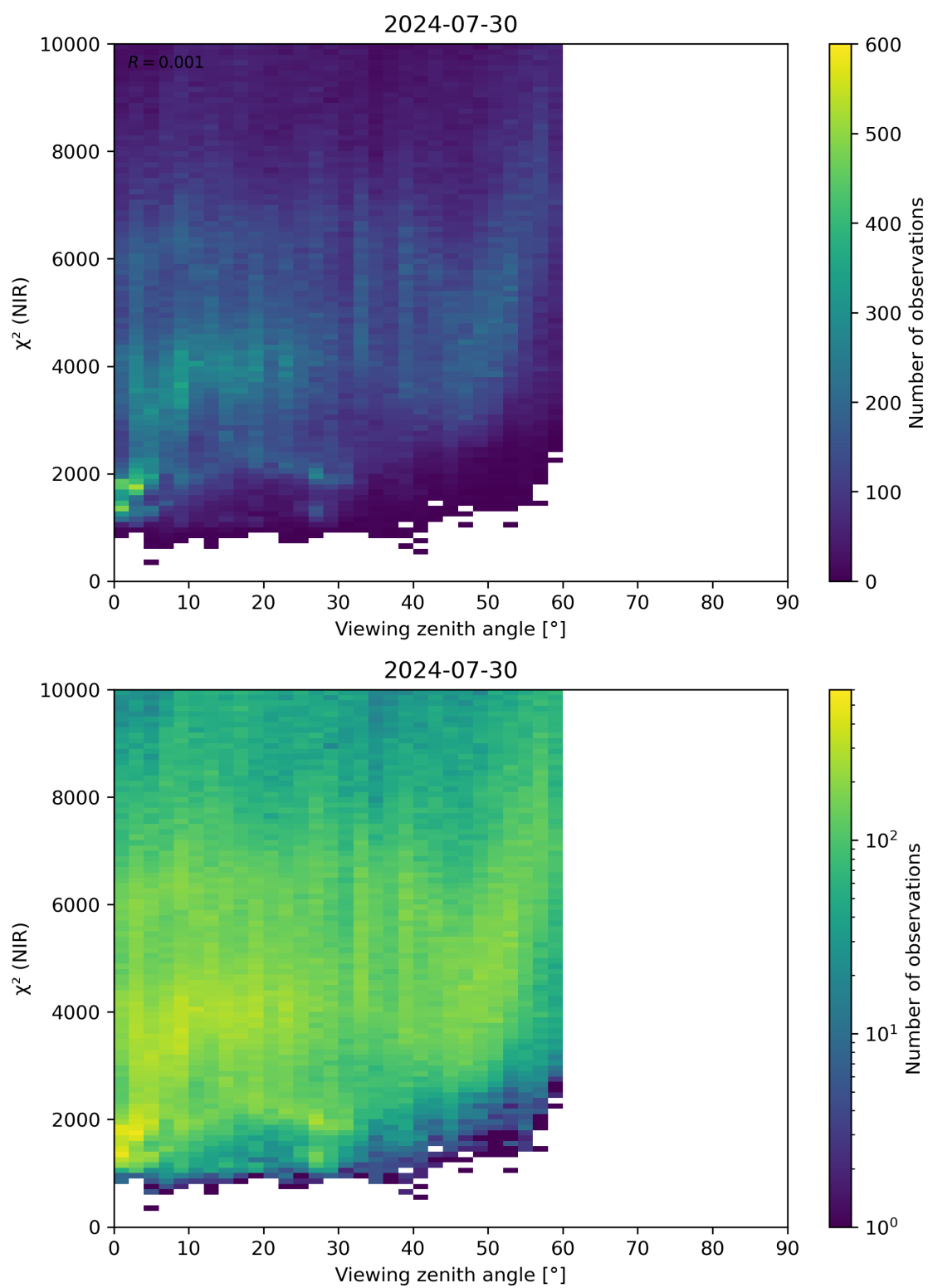
Figure 105: Scatter density plot of “Viewing zenith angle” against “ \chi^2 (NIR)” for 2024-07-29 to 2024-07-31.
