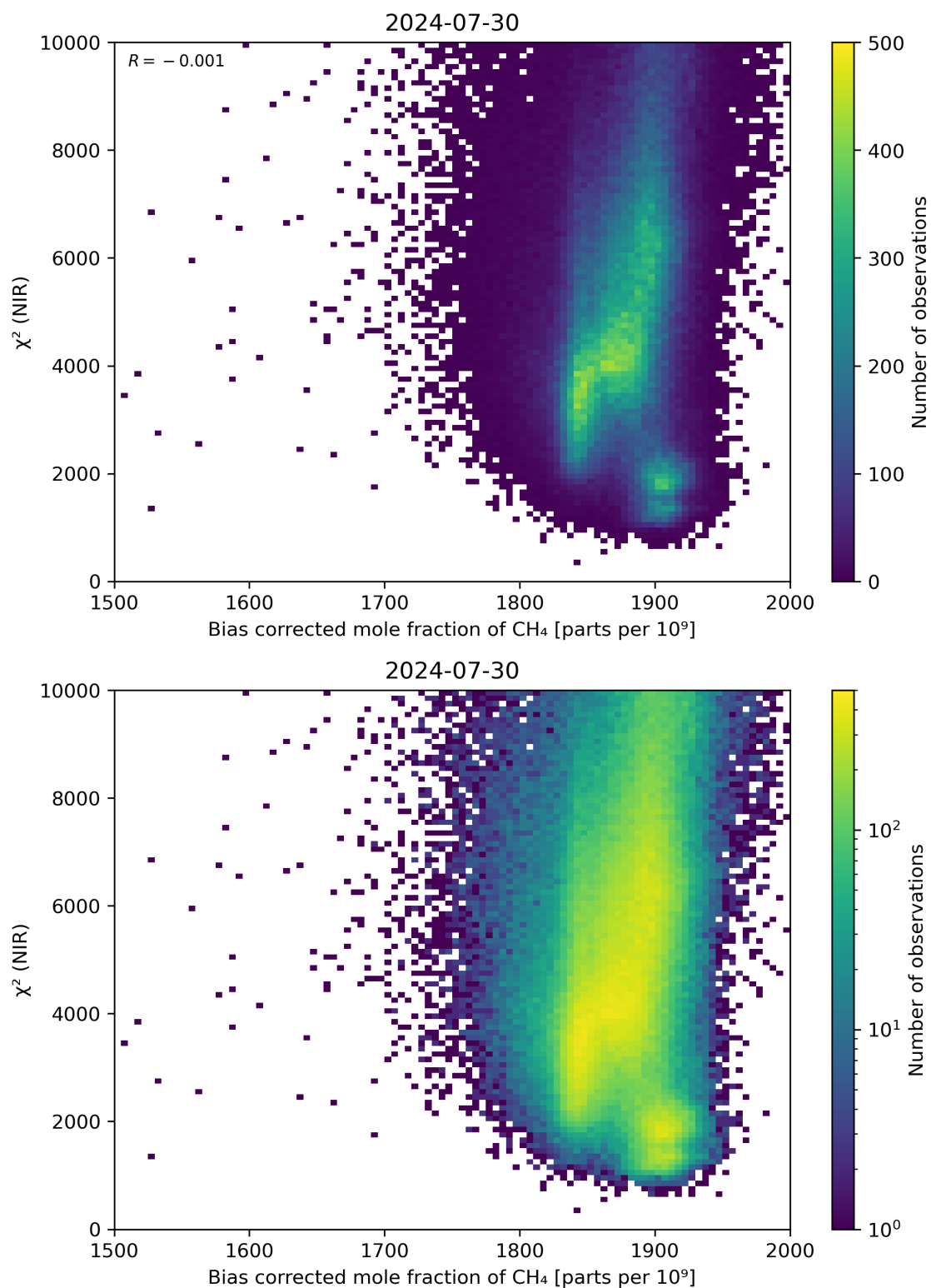
Figure 63: Scatter density plot of “Bias corrected mole fraction of CH 4 ” against “ \chi^2 (NIR)” for 2024-07-29 to 2024-07-31.
