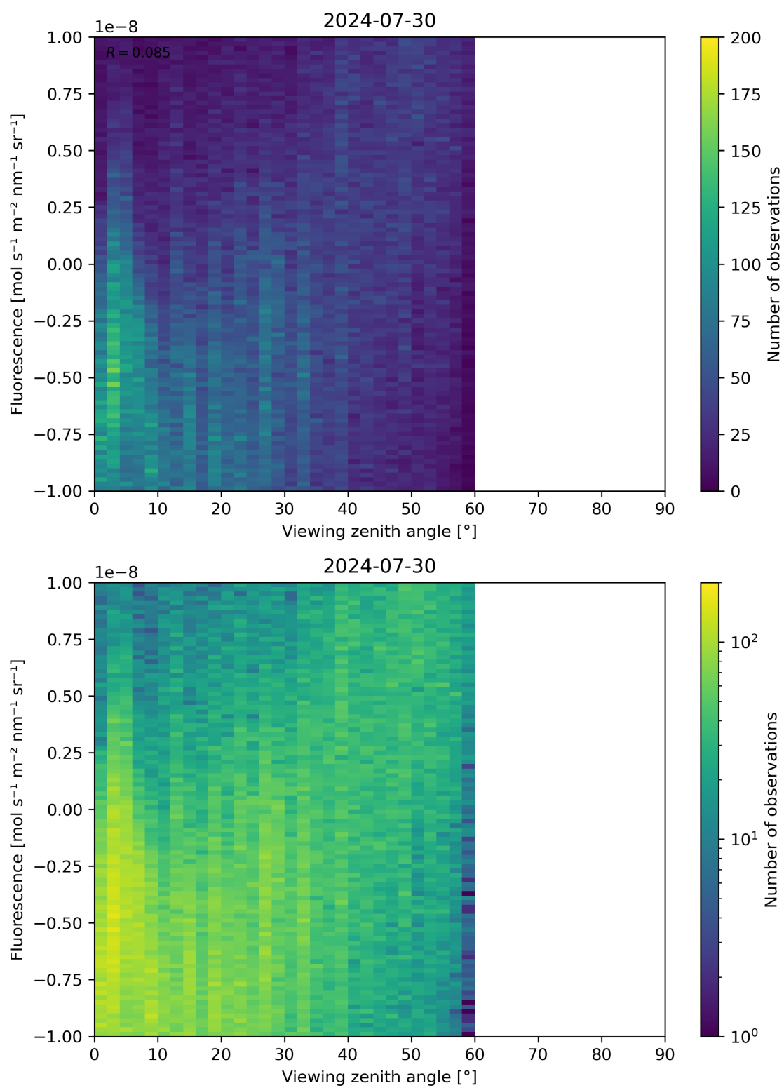
Figure 108: Scatter density plot of “Viewing zenith angle” against “Fluorescence” for 2024-07-29 to 2024-07-31.
