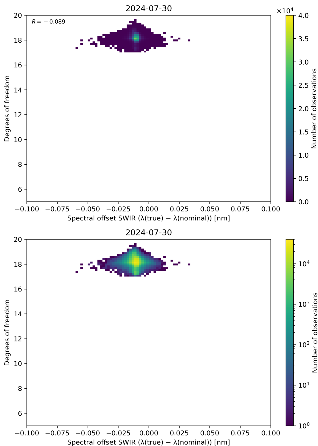
Figure 119: Scatter density plot of “Spectral offset SWIR ( \lambda(\text{true}) - \lambda(\text{nominal}) )” against “Degrees of freedom” for 2024-07-29 to 2024-07-31.
