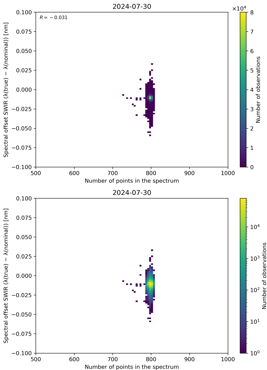
Figure 93: Scatter density plot of “Number of points in the spectrum” against “Spectral offset SWIR ( \lambda(\text{true}) - \lambda(\text{nominal}) )” for 2024-07-29 to 2024-07-31.
