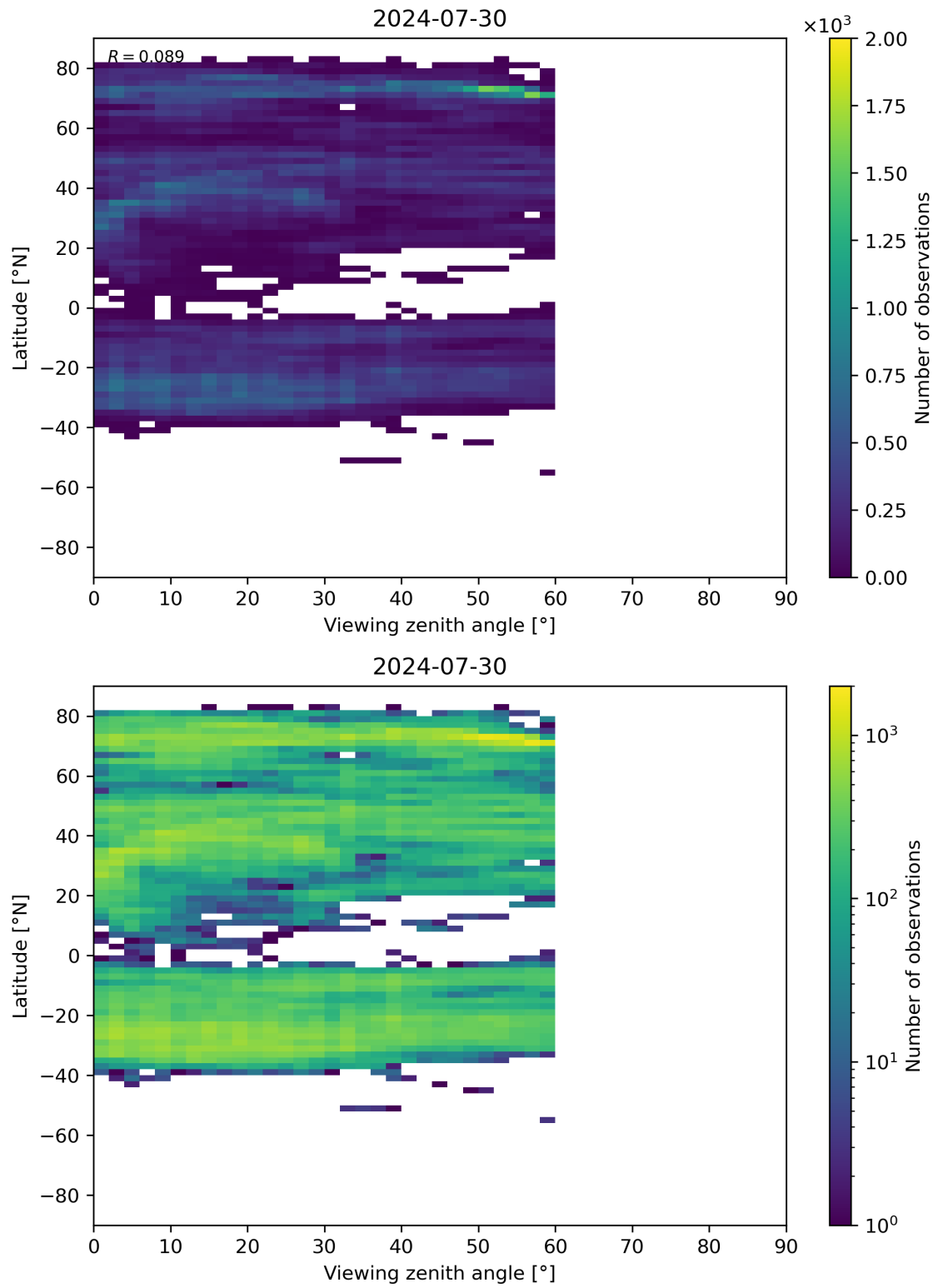
Figure 109: Scatter density plot of “Viewing zenith angle” against “Latitude” for 2024-07-29 to 2024-07-31.
