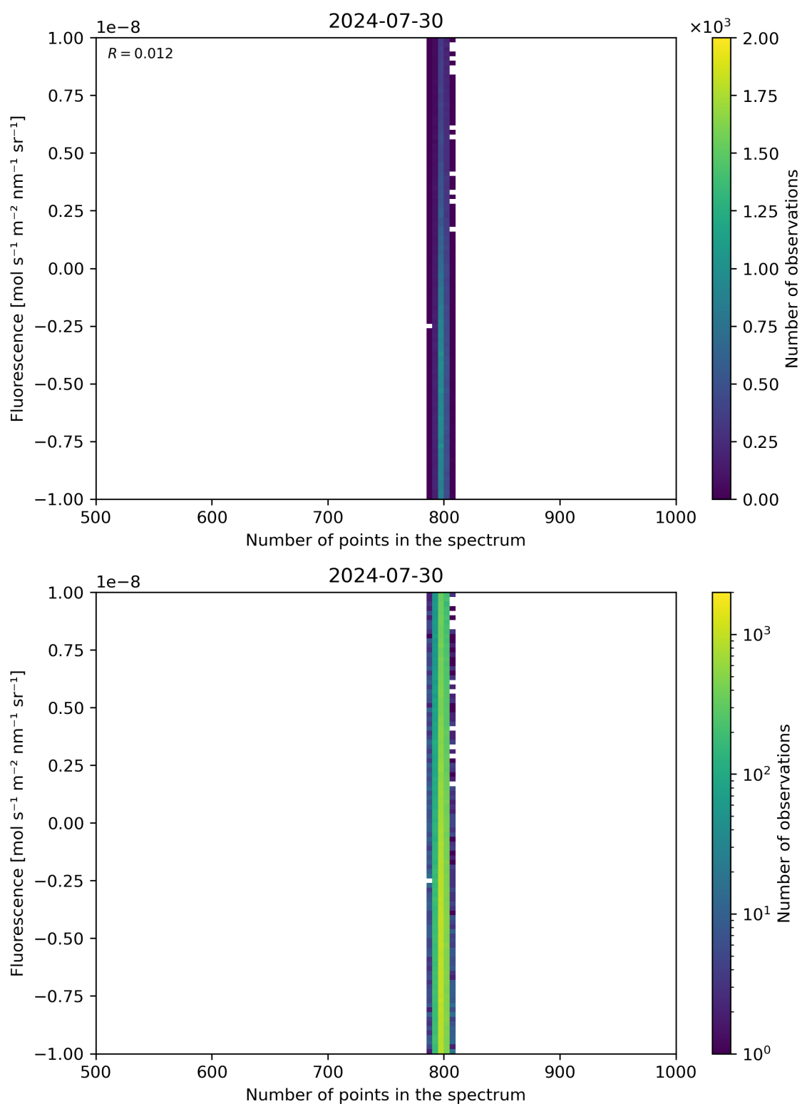
Figure 91: Scatter density plot of “Number of points in the spectrum” against “Fluorescence” for 2024-07-29 to 2024-07-31.
