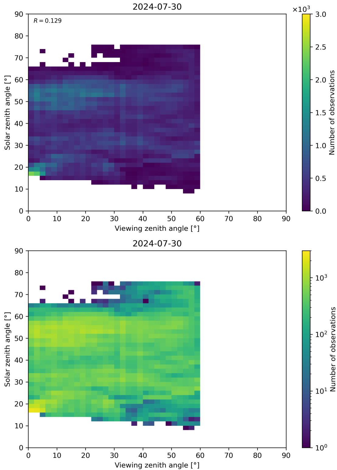
Figure 115: Scatter density plot of “Viewing zenith angle” against “Solar zenith angle” for 2024-07-29 to 2024-07-31.
