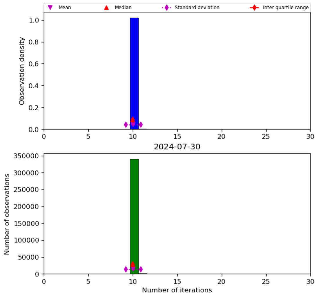
Figure 31: Histogram of “Number of iterations” for 2024-07-29 to 2024-07-31
