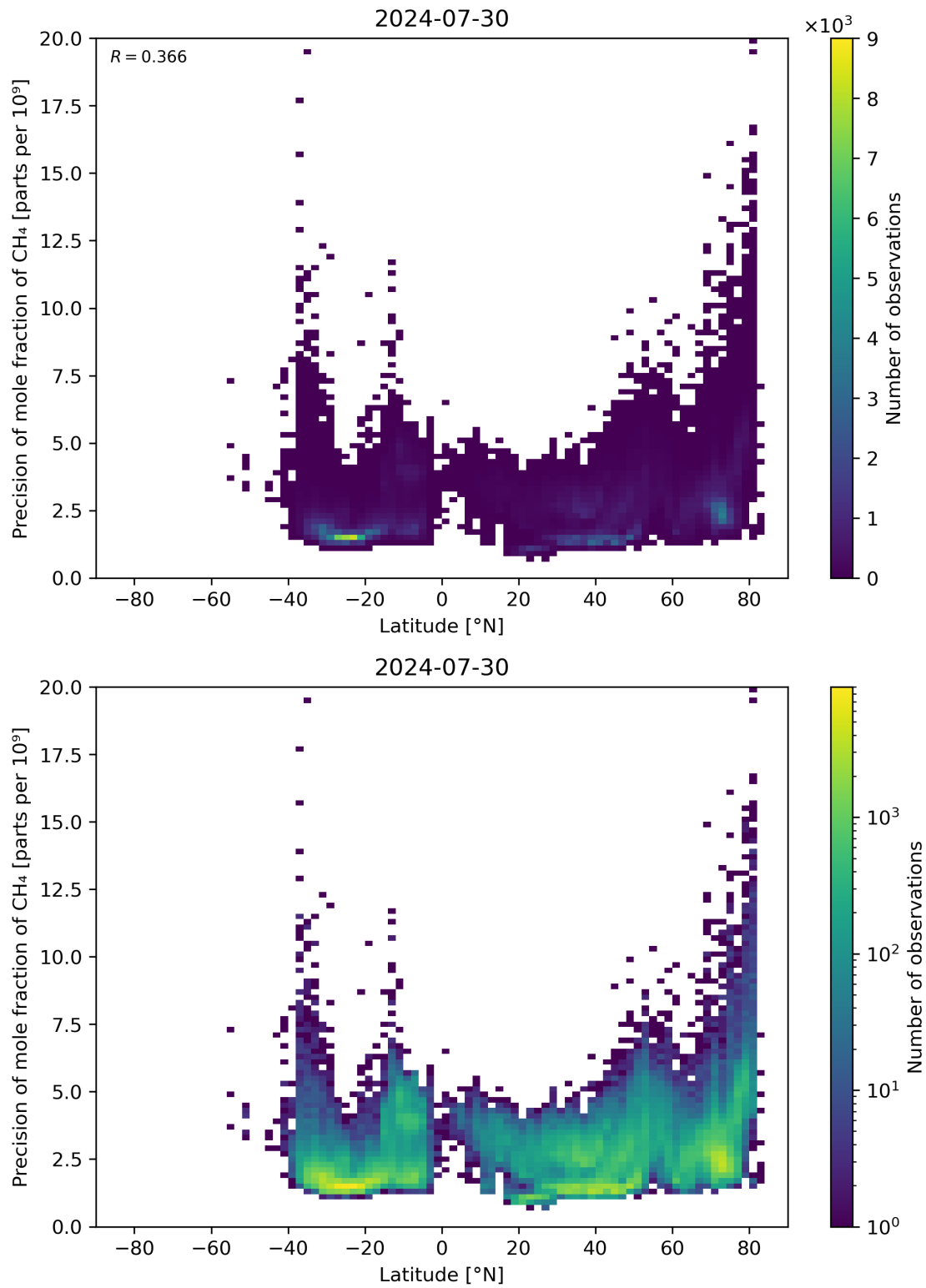
Figure 59: Scatter density plot of “Latitude” against “Precision of mole fraction of \text{CH}_4 ” for 2024-07-29 to 2024-07-31.
