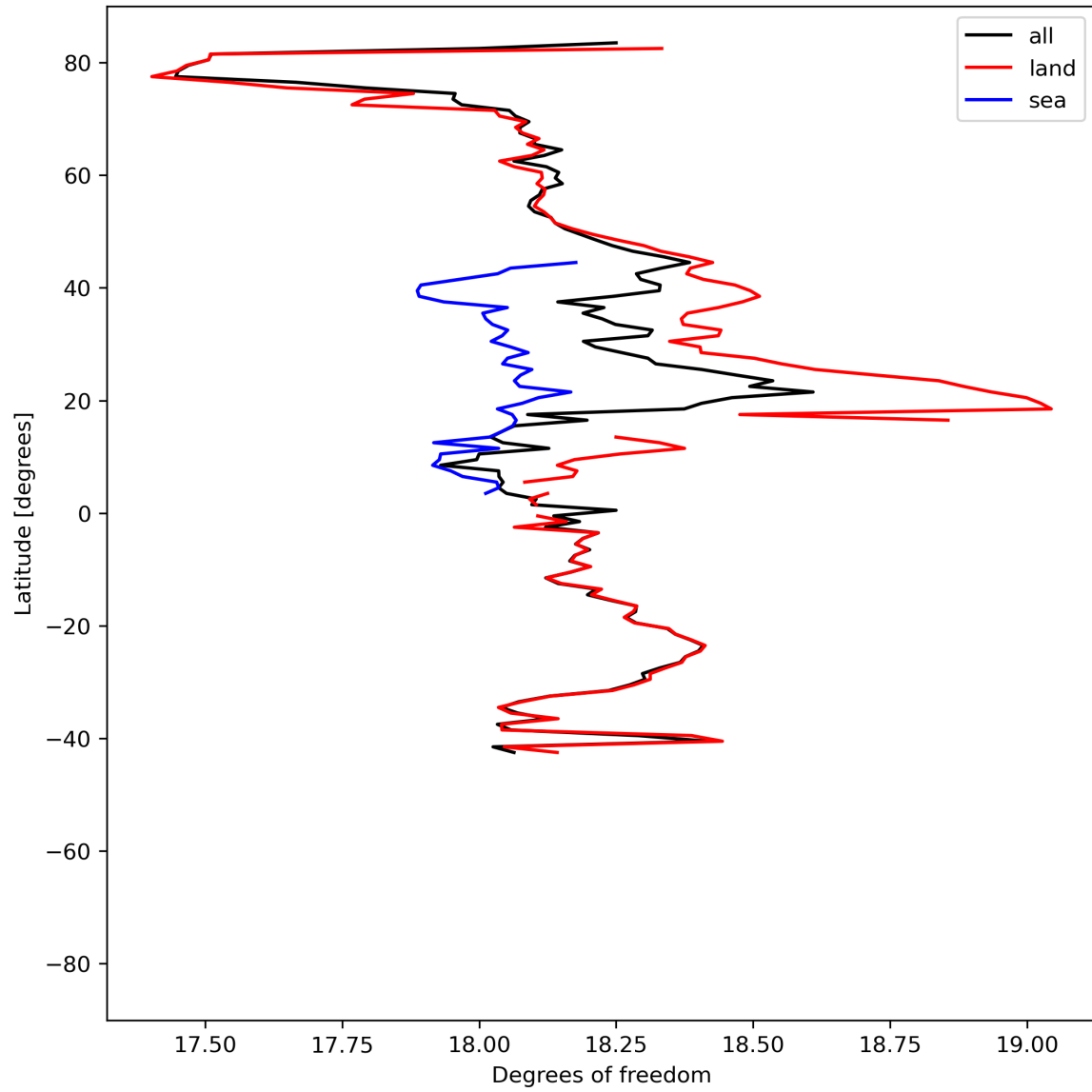
Figure 19: Zonal average of “Degrees of freedom” for 2024-07-29 to 2024-07-31.
