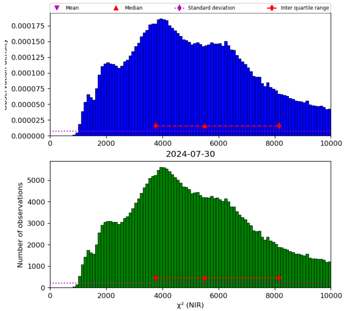
Figure 29: Histogram of “ \chi^2 (NIR)” for 2024-07-29 to 2024-07-31
