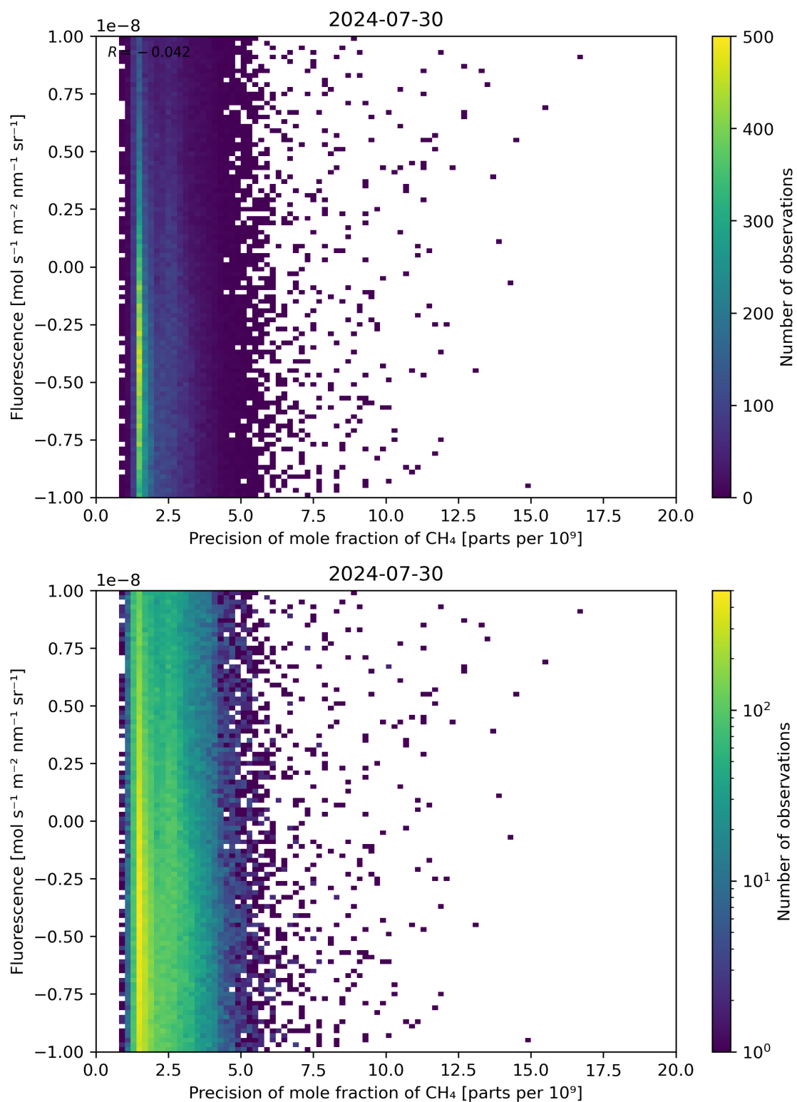
Figure 81: Scatter density plot of “Precision of mole fraction of \text{CH}_4 ” against “Fluorescence” for 2024-07-29 to 2024-07-31.
