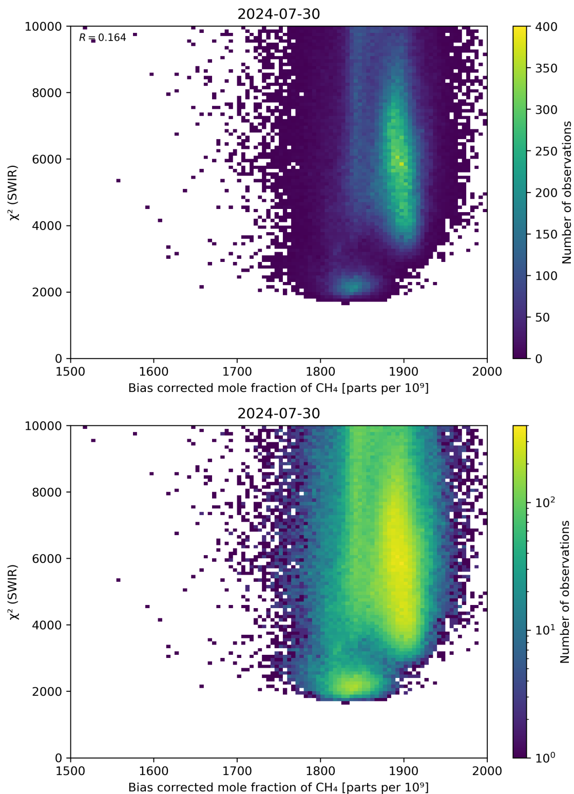
Figure 64: Scatter density plot of “Bias corrected mole fraction of CH 4 ” against “ \chi^2 (SWIR)” for 2024-07-29 to 2024-07-31.
