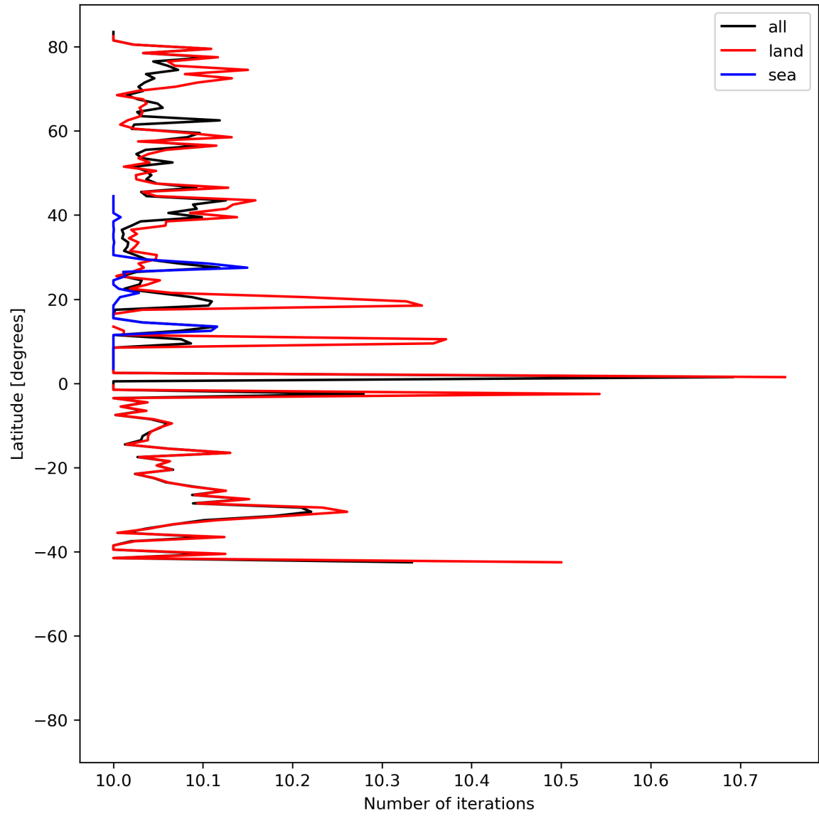
Figure 20: Zonal average of “Number of iterations” for 2024-07-29 to 2024-07-31.
