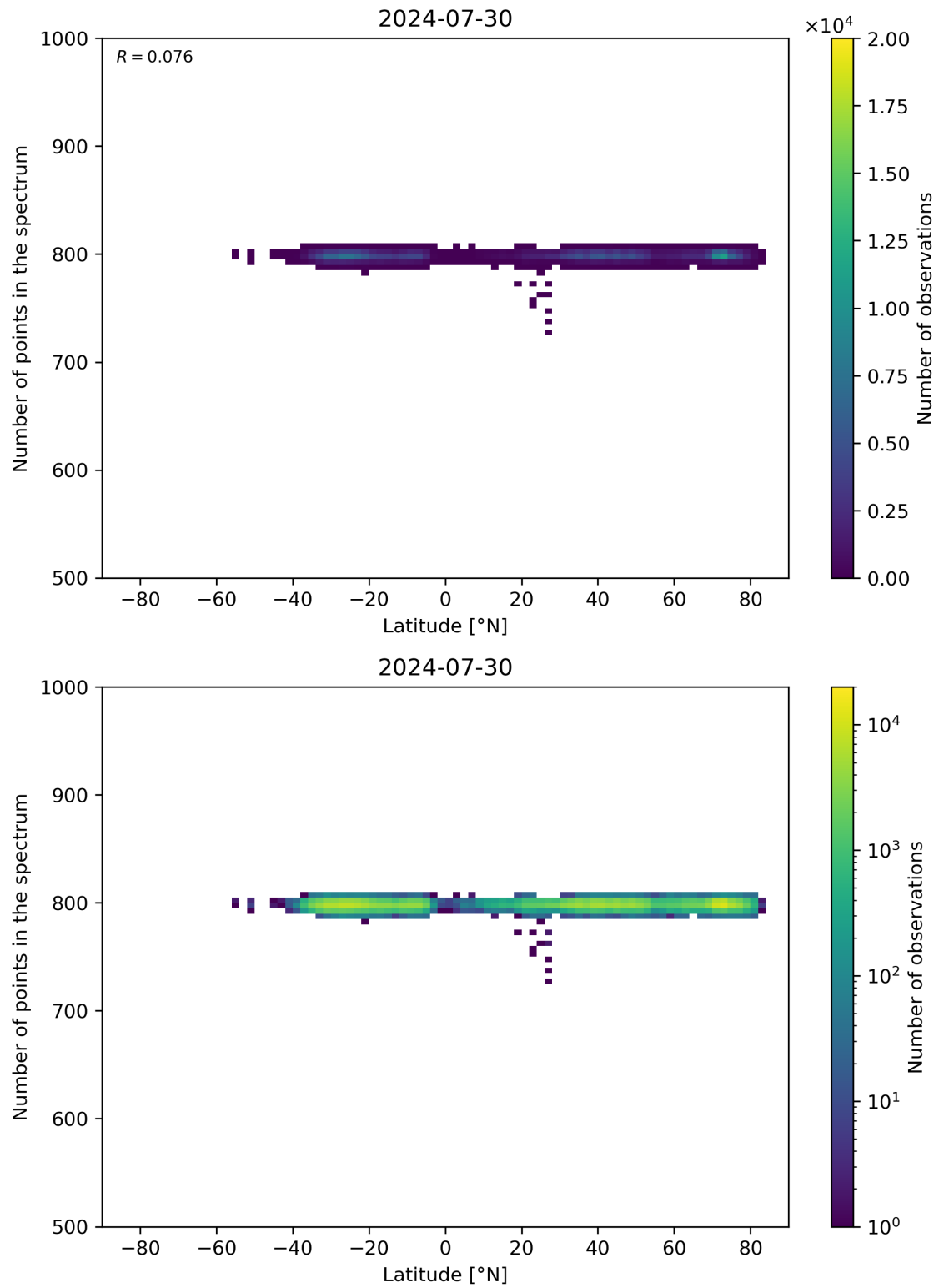
Figure 61: Scatter density plot of “Latitude” against “Number of points in the spectrum” for 2024-07-29 to 2024-07-31.
