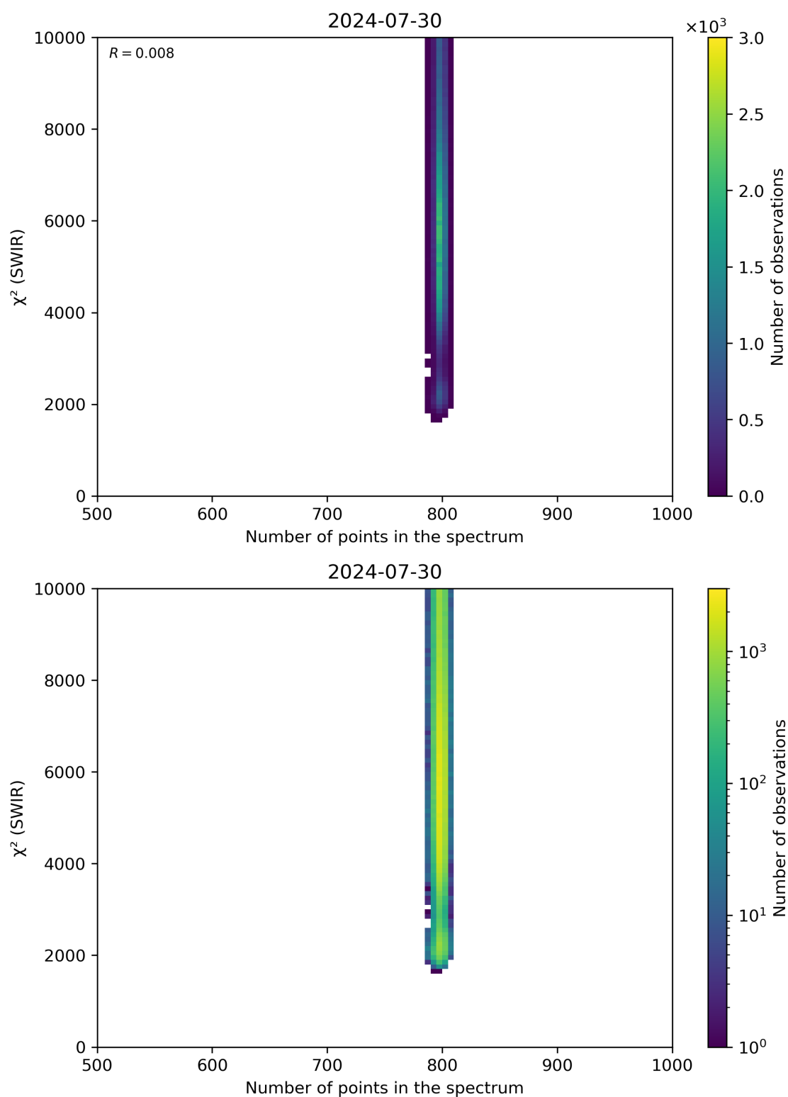
Figure 89: Scatter density plot of “Number of points in the spectrum” against “ \chi^2 (SWIR)” for 2024-07-29 to 2024-07-31.
