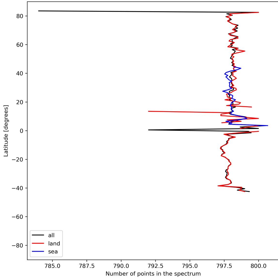
Figure 15: Zonal average of “Number of points in the spectrum” for 2024-07-29 to 2024-07-31.
