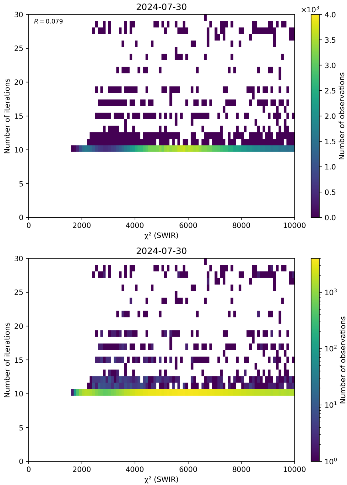
Figure 50: Scatter density plot of “ \chi^2 (SWIR)” against “Number of iterations” for 2024-07-29 to 2024-07-31.
