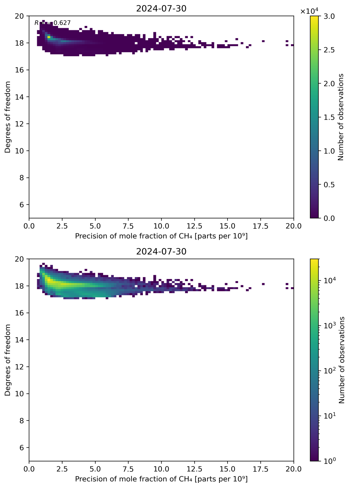
Figure 80: Scatter density plot of “Precision of mole fraction of CH 4 ” against “Degrees of freedom” for 2024-07-29 to 2024-07-31.
