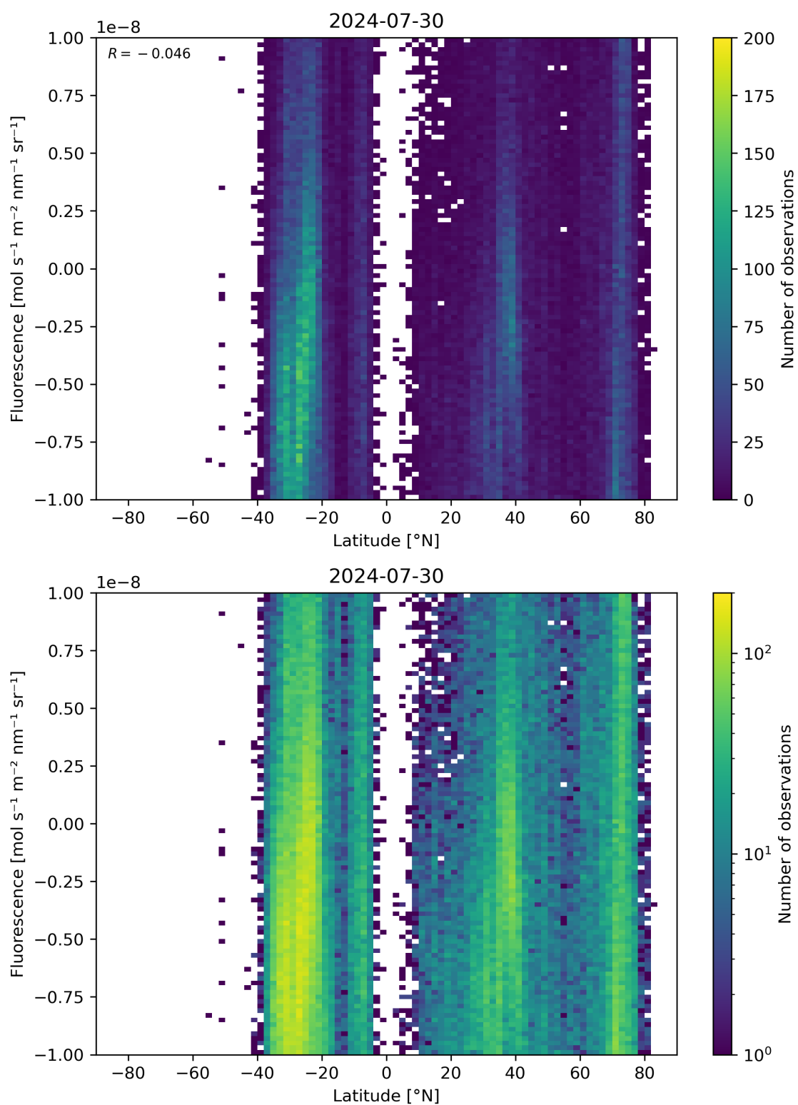
Figure 56: Scatter density plot of “Latitude” against “Fluorescence” for 2024-07-29 to 2024-07-31.
