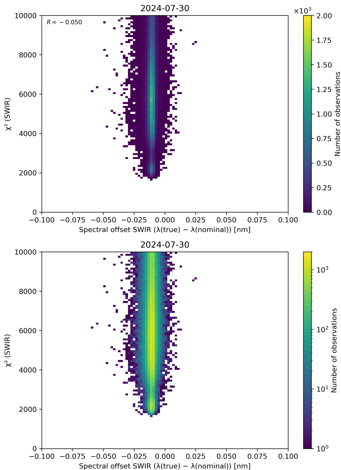
Figure 118: Scatter density plot of “Spectral offset SWIR ( \lambda(\text{true}) - \lambda(\text{nominal}) )” against “ \chi^2 (SWIR)” for 2024-07-29 to 2024-07-31.
