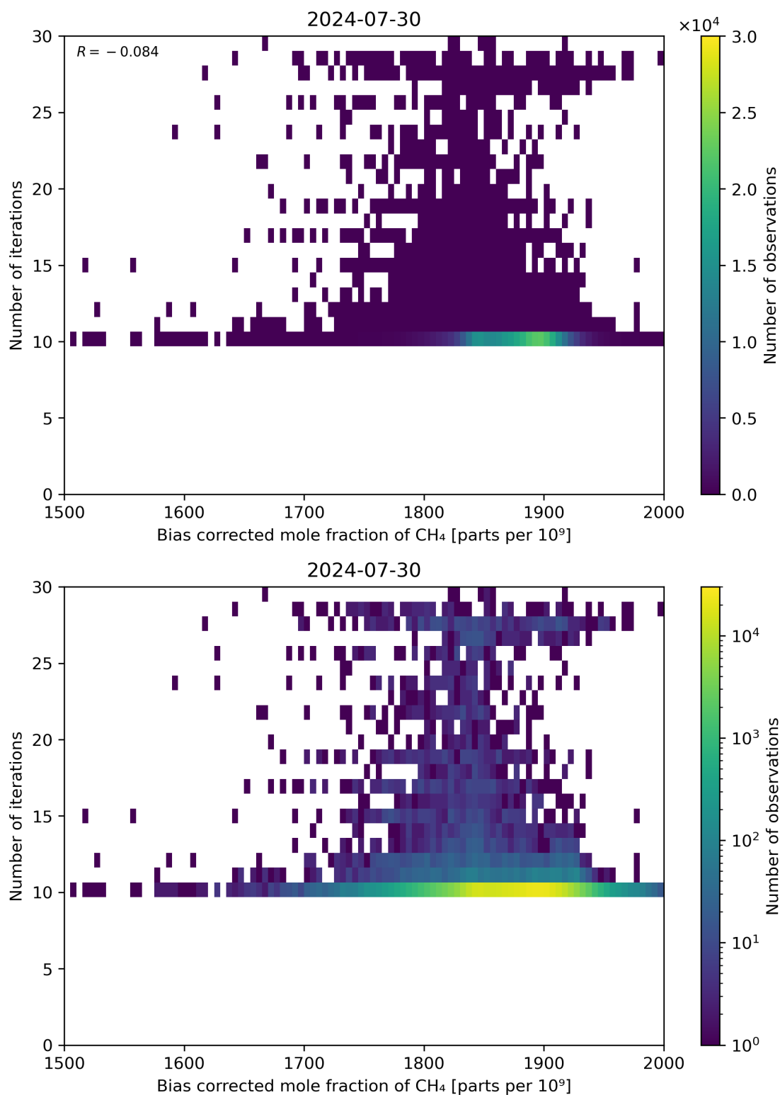
Figure 67: Scatter density plot of “Bias corrected mole fraction of CH 4 ” against “Number of iterations” for 2024-07-29 to 2024-07-31.
