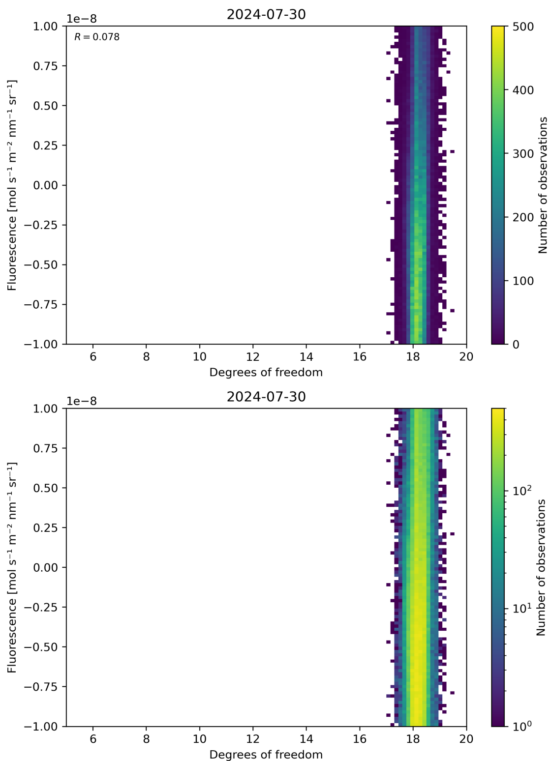
Figure 51: Scatter density plot of “Degrees of freedom” against “Fluorescence” for 2024-07-29 to 2024-07-31.
