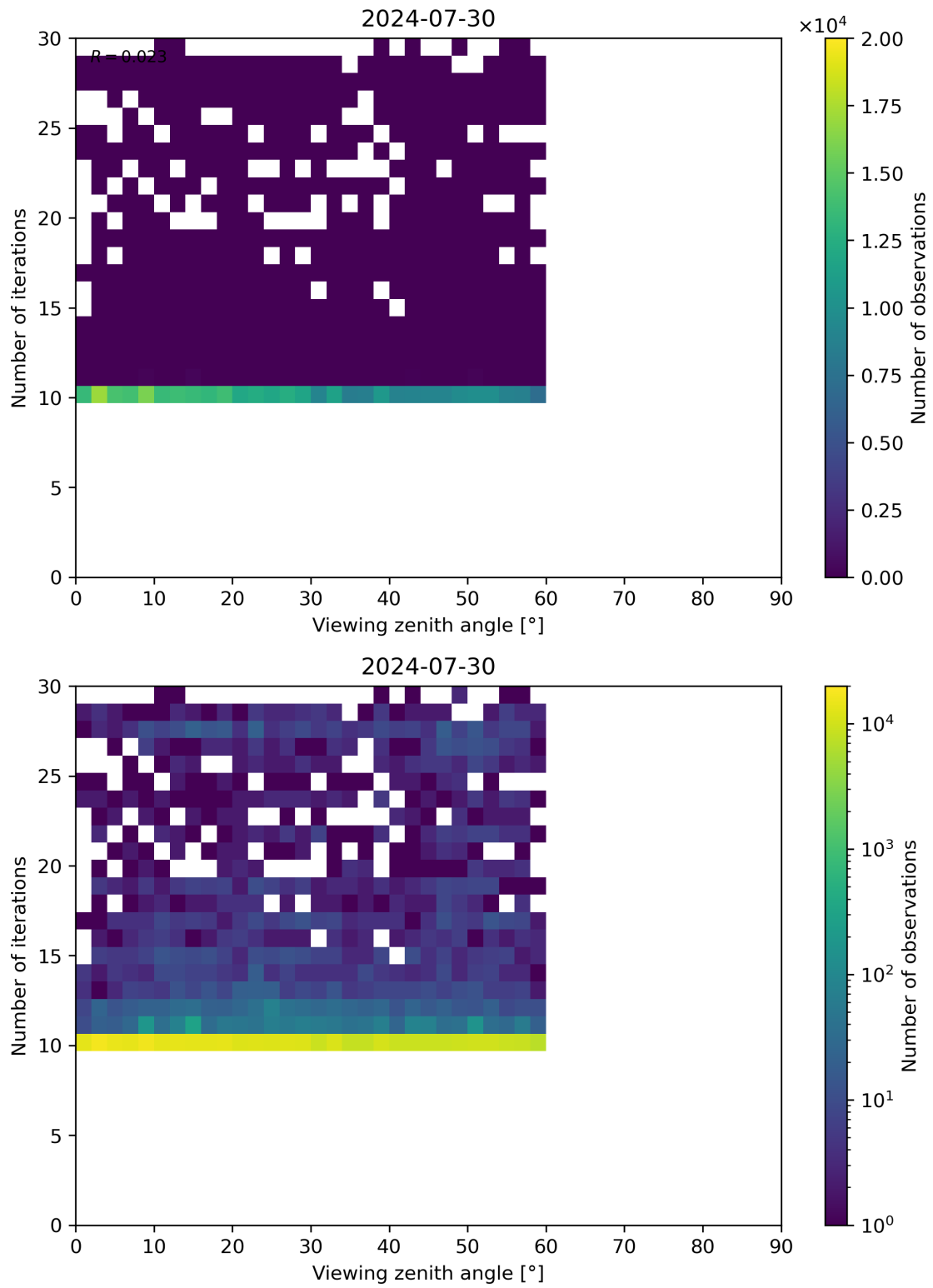
Figure 113: Scatter density plot of “Viewing zenith angle” against “Number of iterations” for 2024-07-29 to 2024-07-31.
