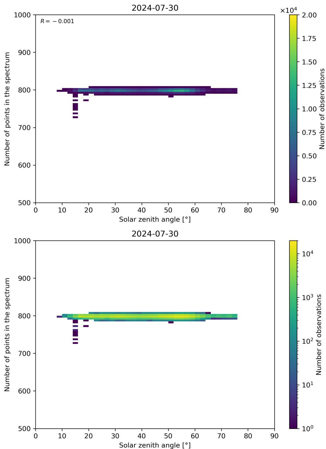
Figure 103: Scatter density plot of “Solar zenith angle” against “Number of points in the spectrum” for 2024-07-29 to 2024-07-31.
