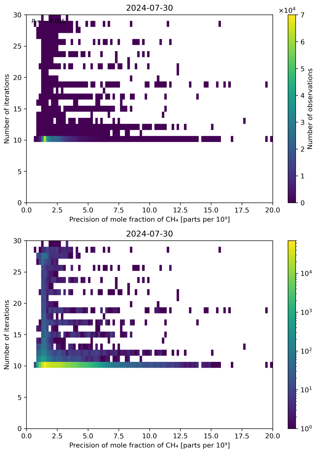
Figure 83: Scatter density plot of “Precision of mole fraction of CH 4 ” against “Number of iterations” for 2024-07-29 to 2024-07-31.
