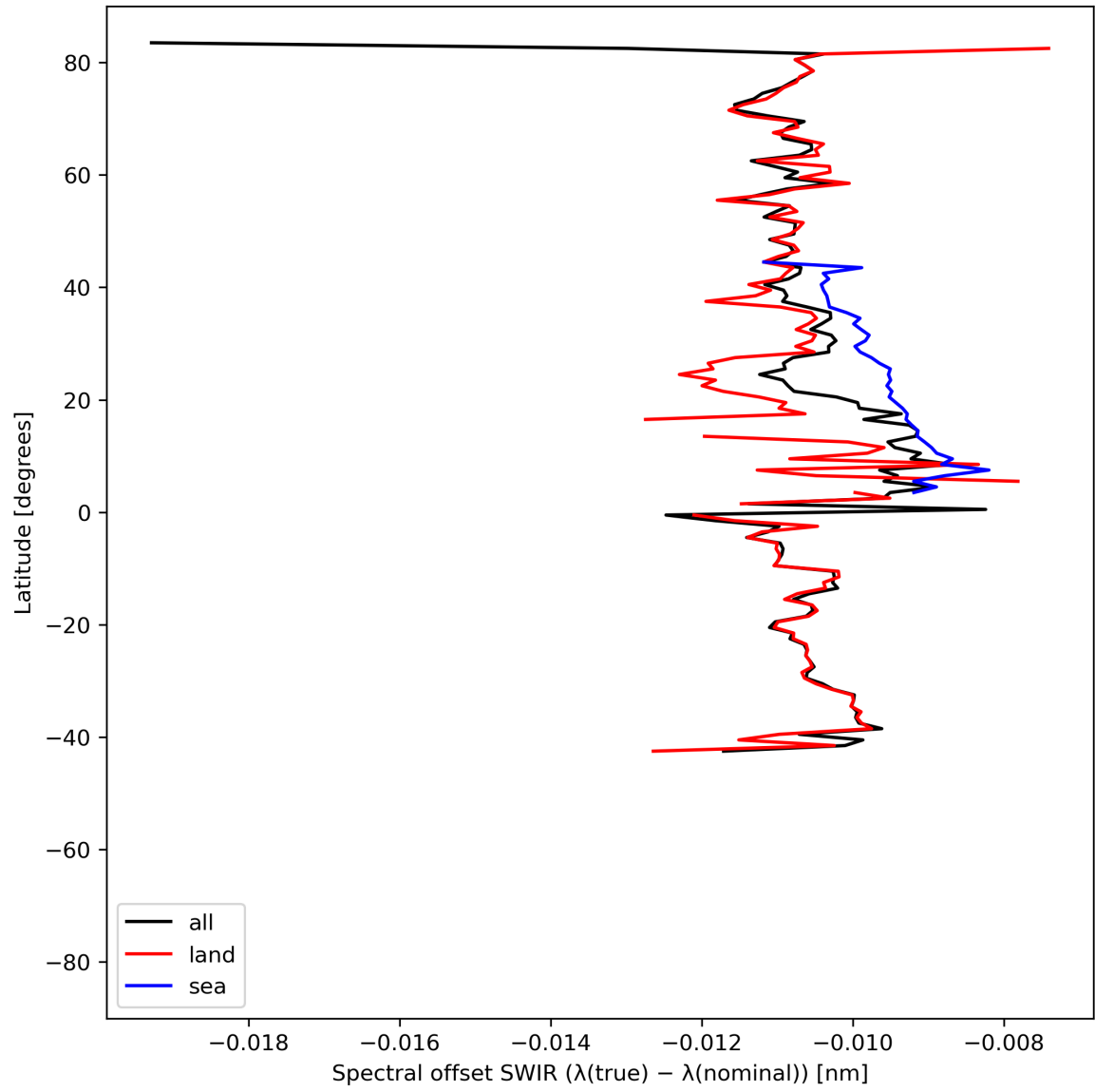
Figure 16: Zonal average of “Spectral offset SWIR ( \lambda(\text{true}) - \lambda(\text{nominal}) )” for 2024-07-29 to 2024-07-31.
