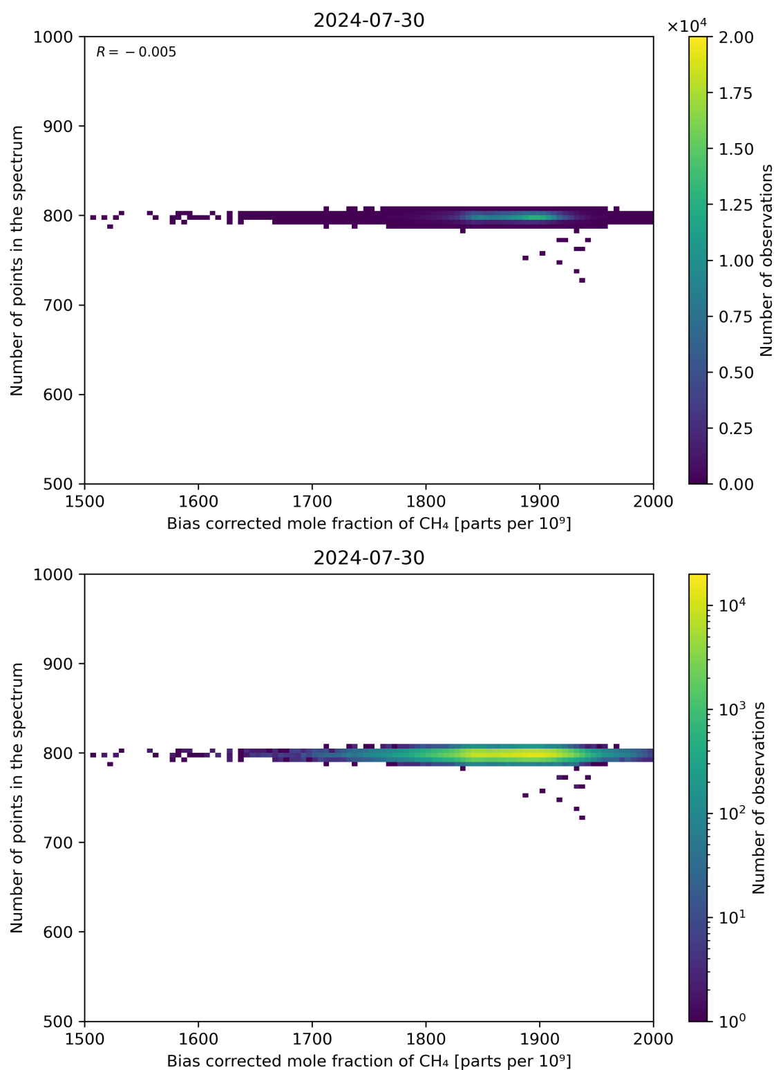
Figure 68: Scatter density plot of “Bias corrected mole fraction of CH 4 ” against “Number of points in the spectrum” for 2024-07-29 to 2024-07-31.
