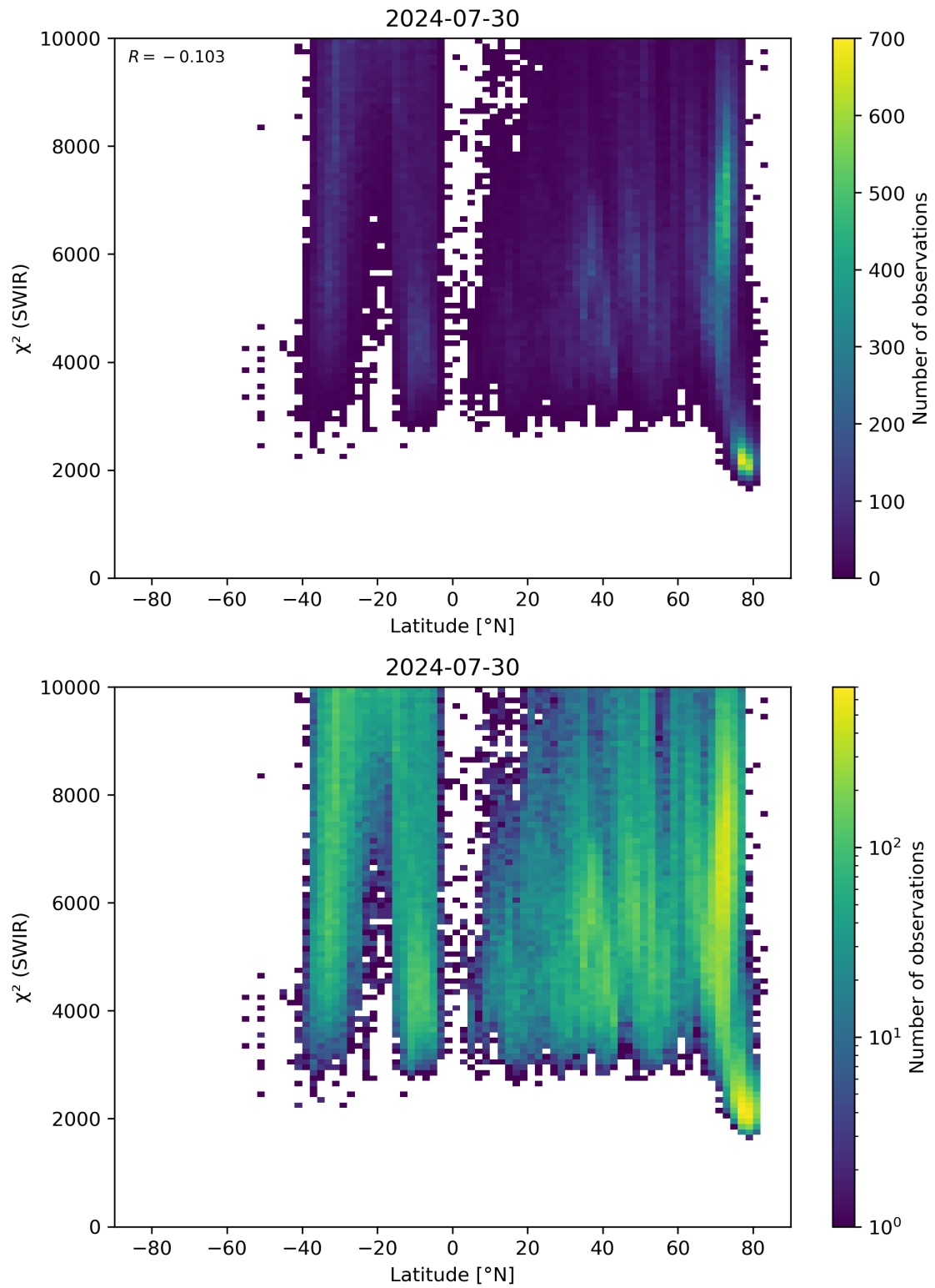
Figure 54: Scatter density plot of “Latitude” against “ \chi^2 (SWIR)” for 2024-07-29 to 2024-07-31.
