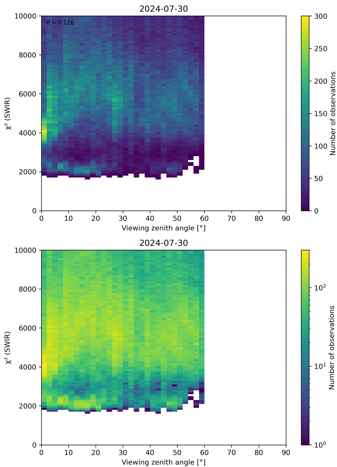
Figure 106: Scatter density plot of “Viewing zenith angle” against “ \chi^2 (SWIR)” for 2024-07-29 to 2024-07-31.
