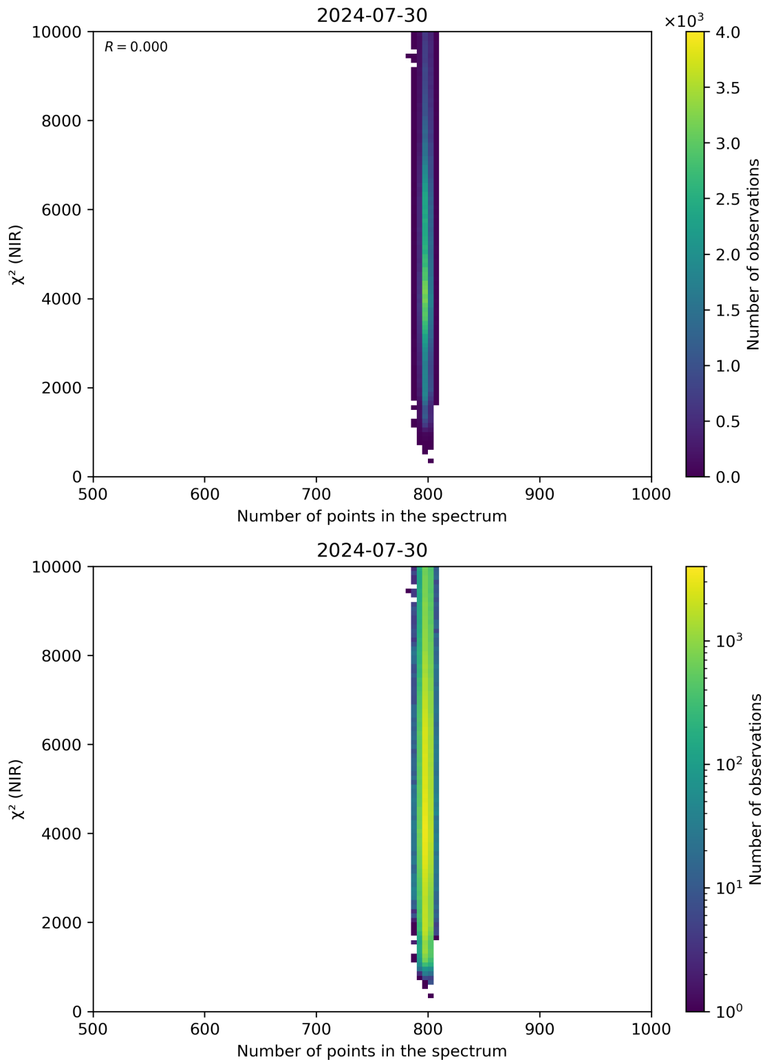
Figure 88: Scatter density plot of “Number of points in the spectrum” against “ \chi^2 (NIR)” for 2024-07-29 to 2024-07-31.
