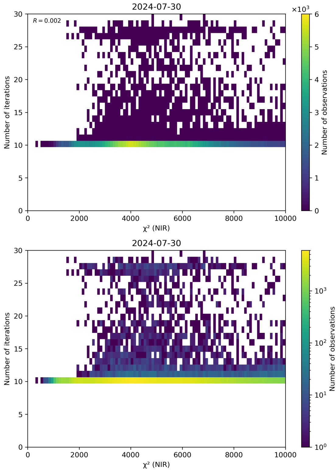
Figure 46: Scatter density plot of “ \chi^2 (NIR)” against “Number of iterations” for 2024-07-29 to 2024-07-31.
