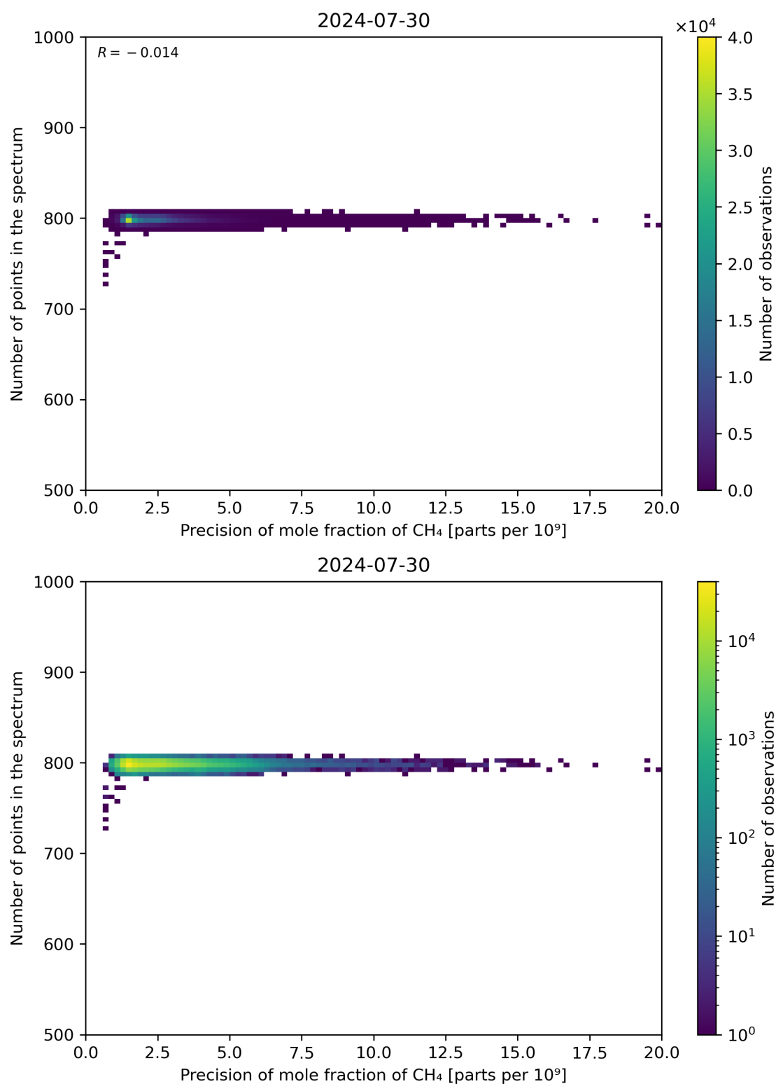
Figure 84: Scatter density plot of “Precision of mole fraction of CH 4 ” against “Number of points in the spectrum” for 2024-07-29 to 2024-07-31.
