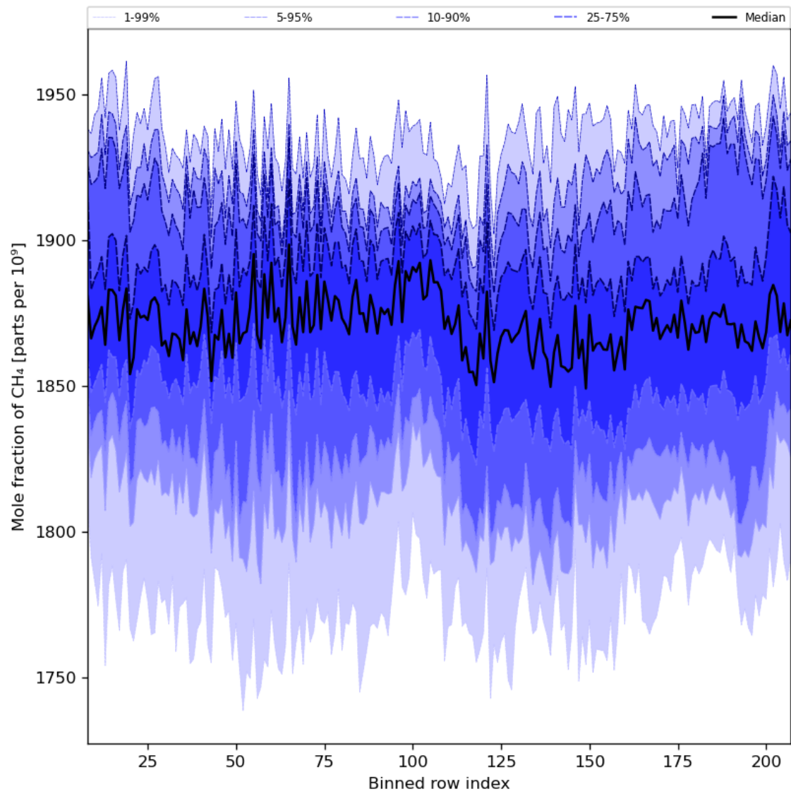
Figure 34: Along track statistics of “Mole fraction of CH 4 ” for 2024-07-29 to 2024-07-31
