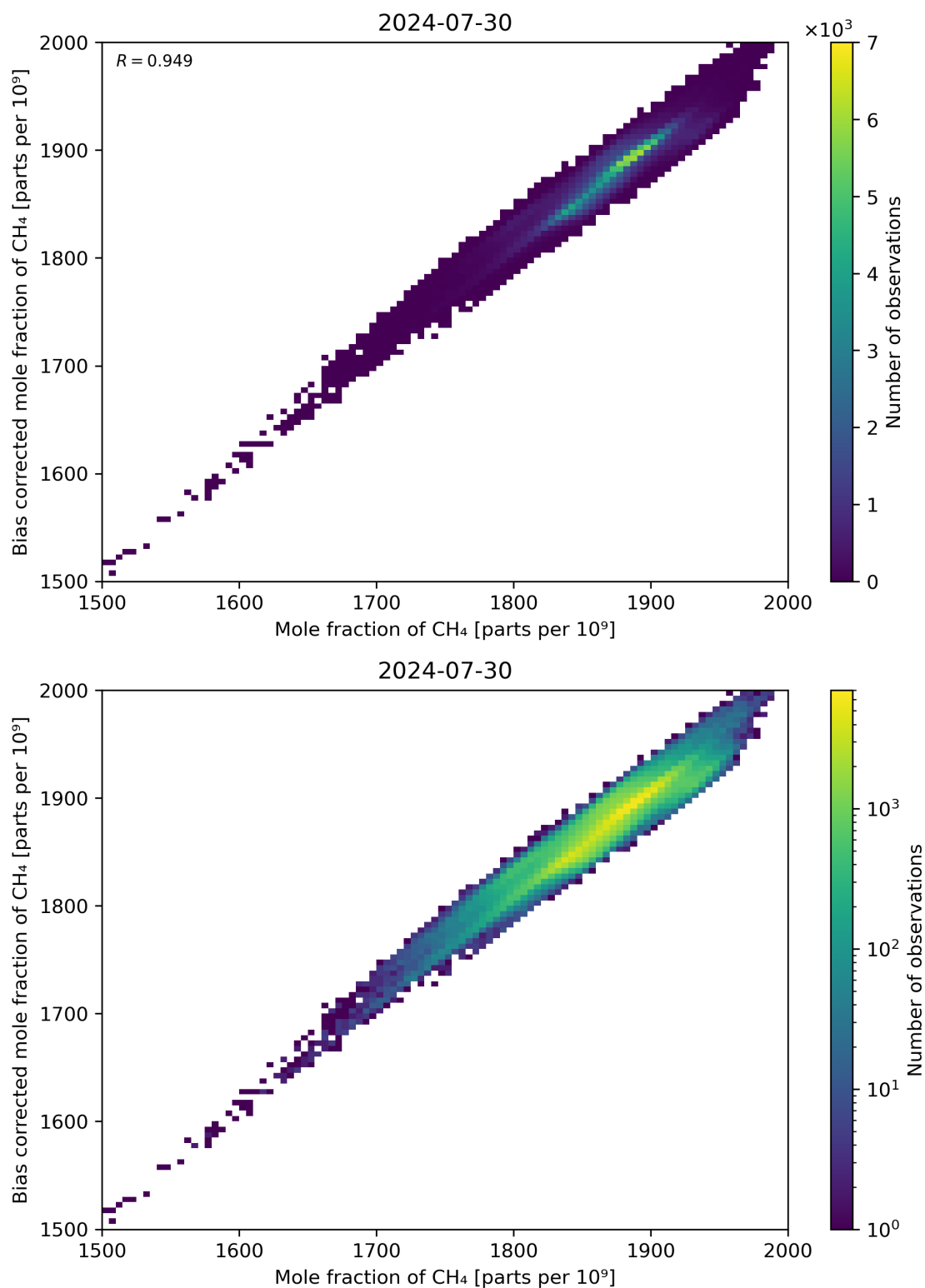
Figure 74: Scatter density plot of “Mole fraction of CH 4 ” against “Bias corrected mole fraction of CH 4 ” for 2024-07-29 to 2024-07-31.
