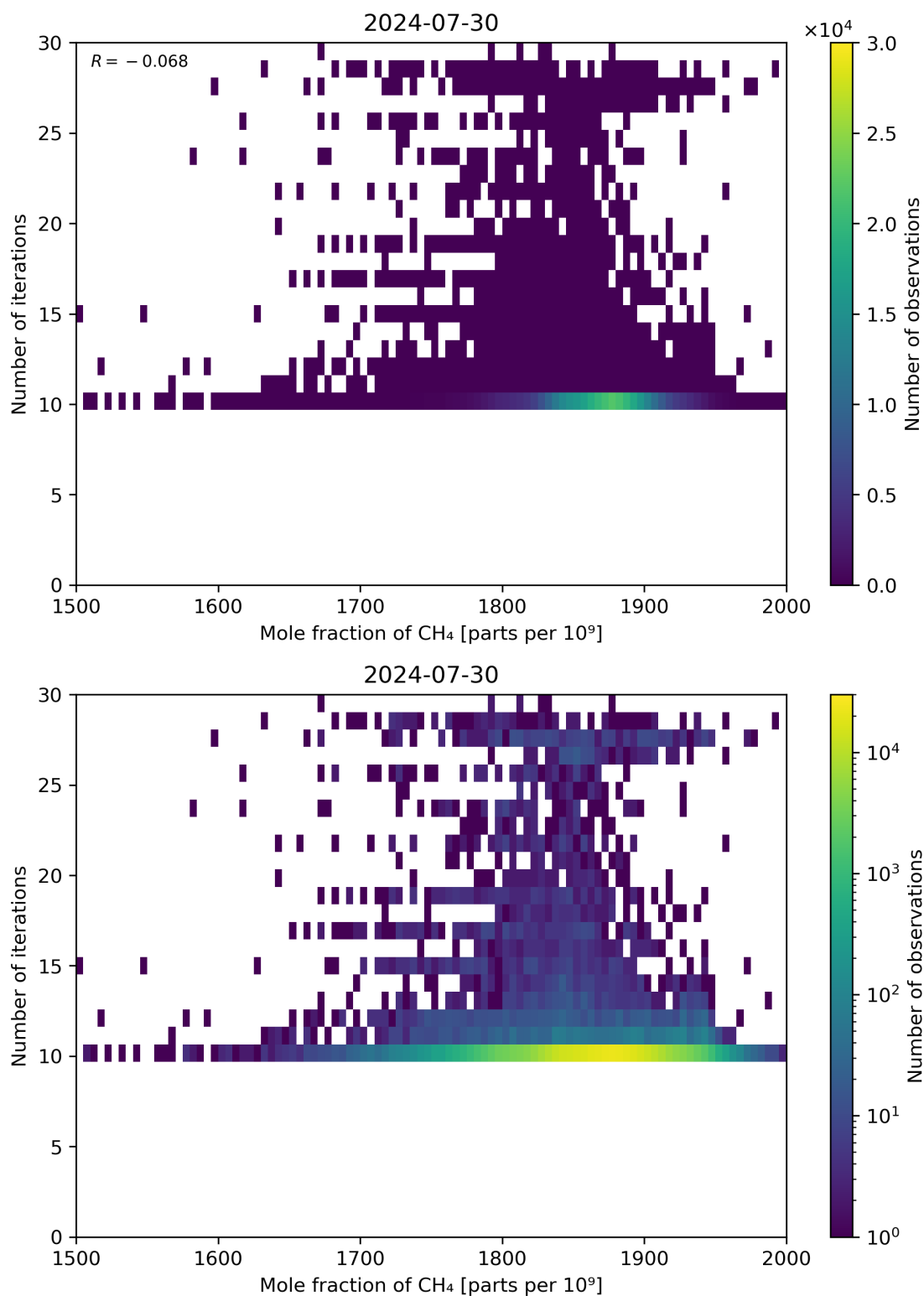
Figure 76: Scatter density plot of “Mole fraction of CH 4 ” against “Number of iterations” for 2024-07-29 to 2024-07-31.
