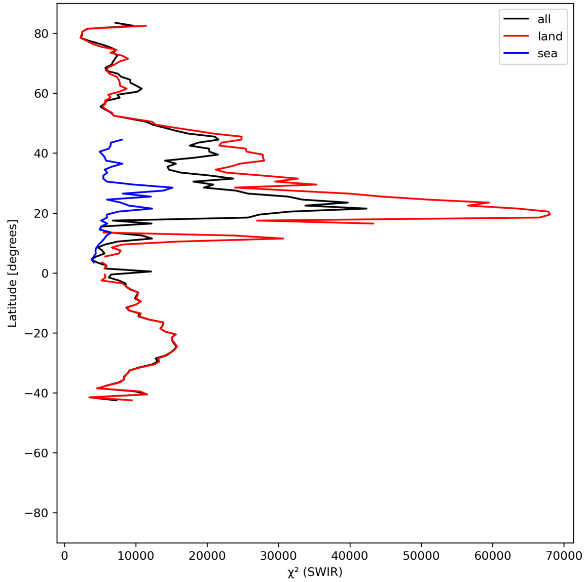
Figure 17: Zonal average of “ \chi^2 (SWIR)” for 2024-07-29 to 2024-07-31.
