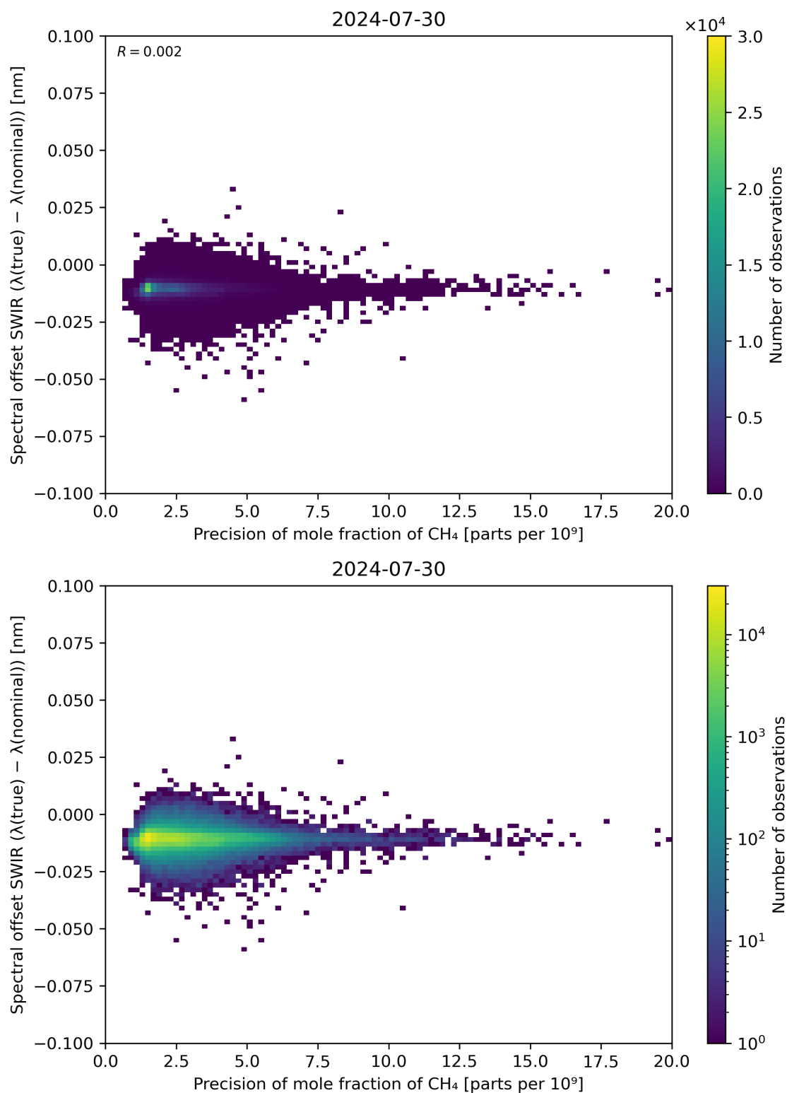
Figure 85: Scatter density plot of “Precision of mole fraction of CH 4 ” against “Spectral offset SWIR ( \lambda(\text{true}) - \lambda(\text{nominal}) )” for 2024-07-29 to 2024-07-31.
