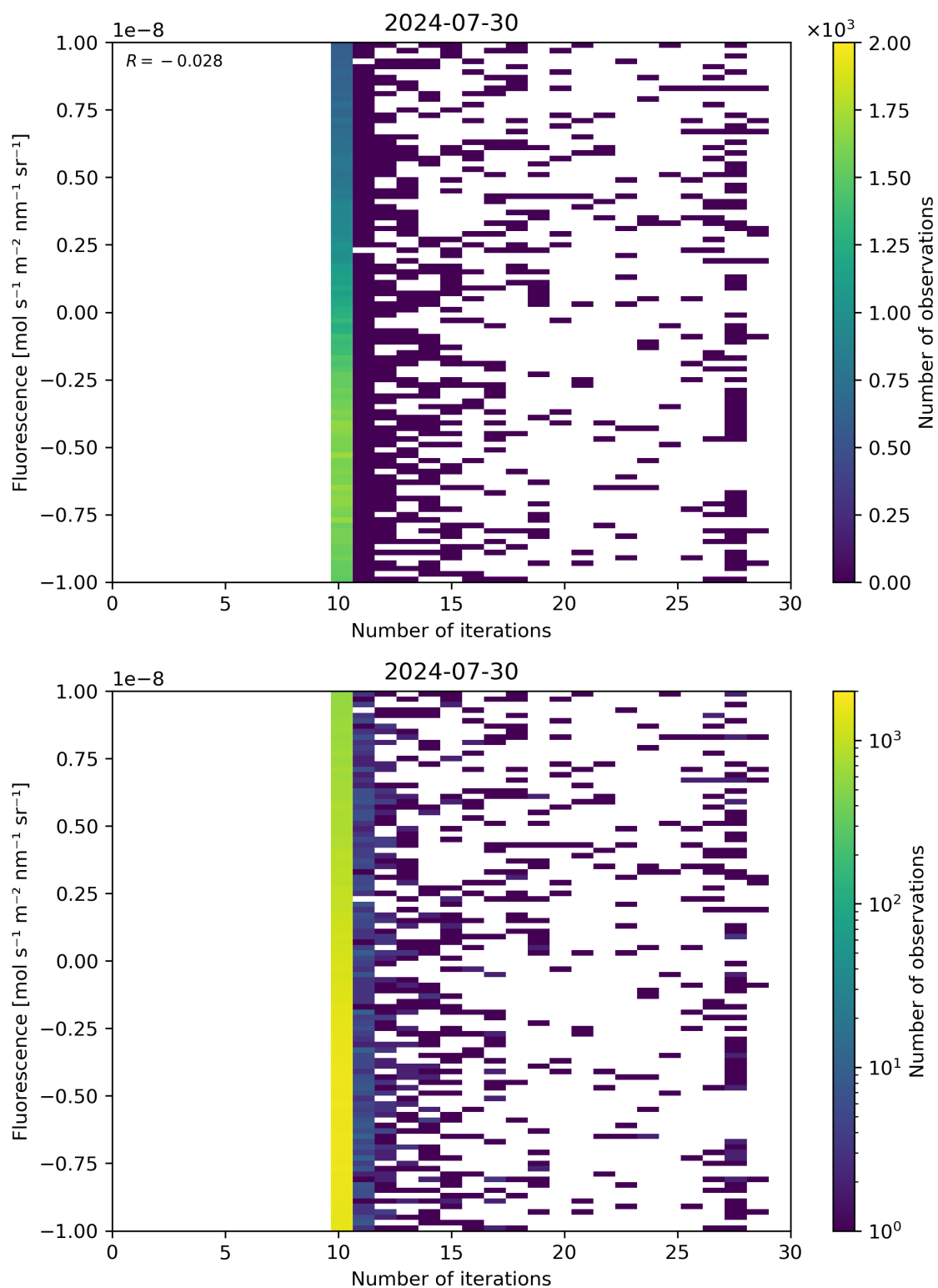
Figure 87: Scatter density plot of “Number of iterations” against “Fluorescence” for 2024-07-29 to 2024-07-31.
