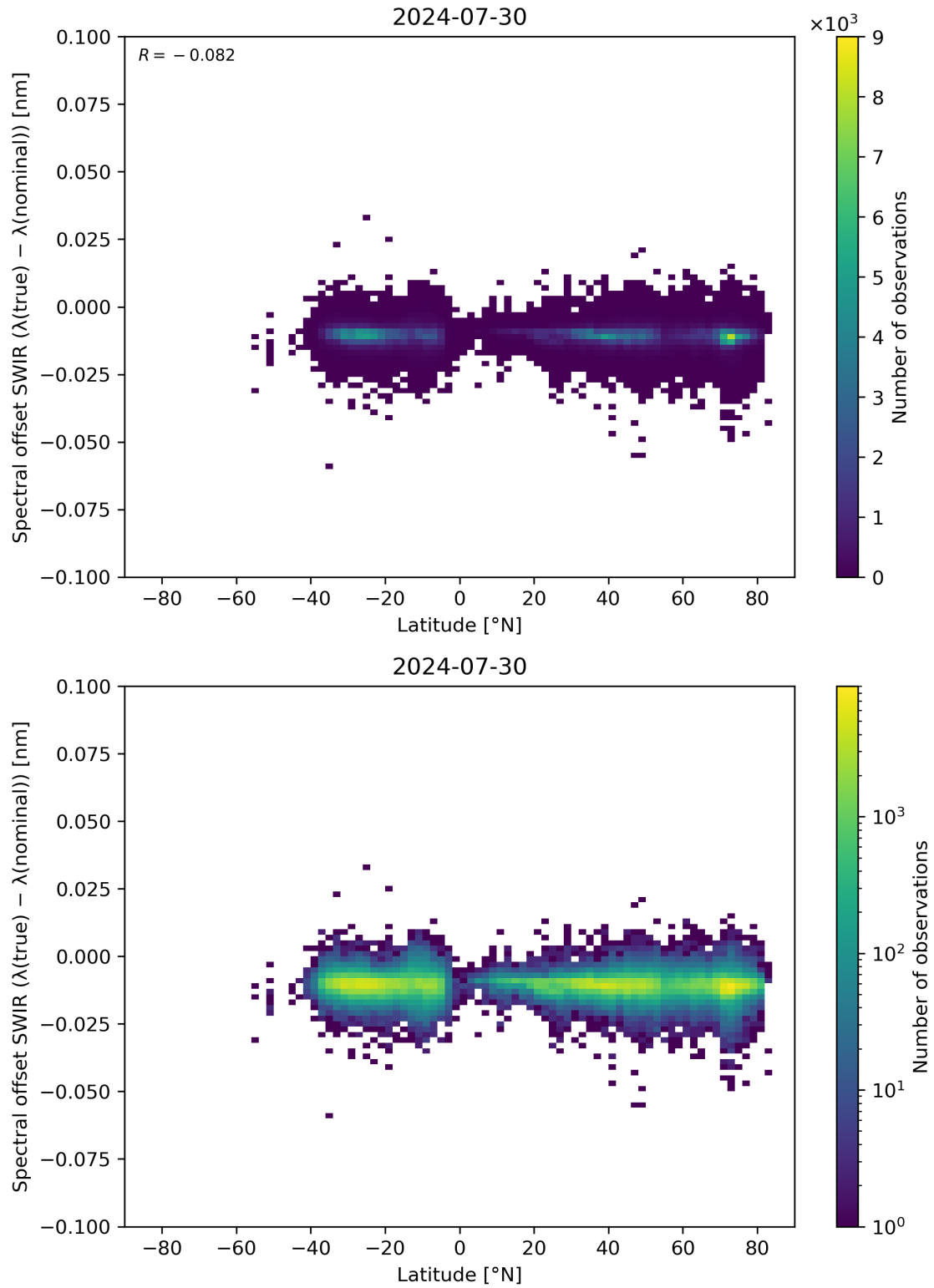
Figure 62: Scatter density plot of “Latitude” against “Spectral offset SWIR ( \lambda(\text{true}) - \lambda(\text{nominal}) )” for 2024-07-29 to 2024-07-31.
