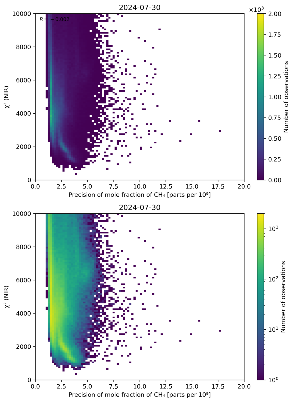
Figure 78: Scatter density plot of “Precision of mole fraction of \text{CH}_4 ” against “ \chi^2 (NIR)” for 2024-07-29 to 2024-07-31.
