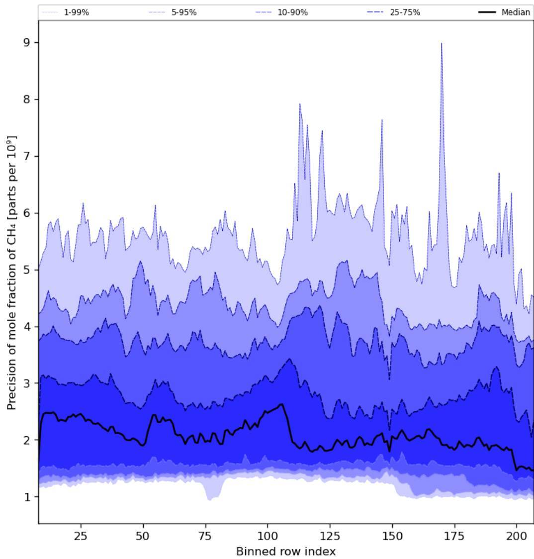
Figure 35: Along track statistics of “Precision of mole fraction of CH 4 ” for 2024-07-29 to 2024-07-31
