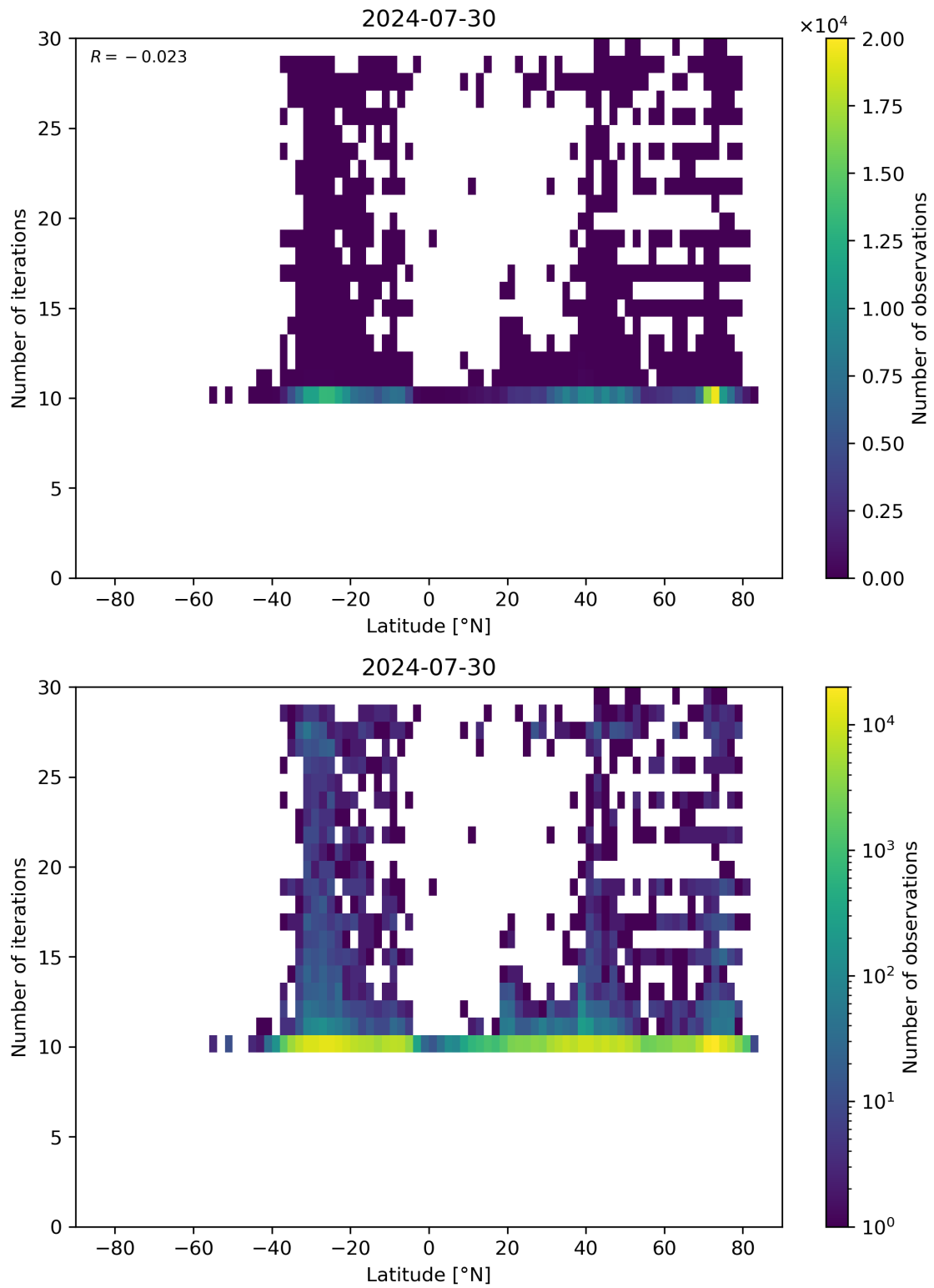
Figure 60: Scatter density plot of “Latitude” against “Number of iterations” for 2024-07-29 to 2024-07-31.
