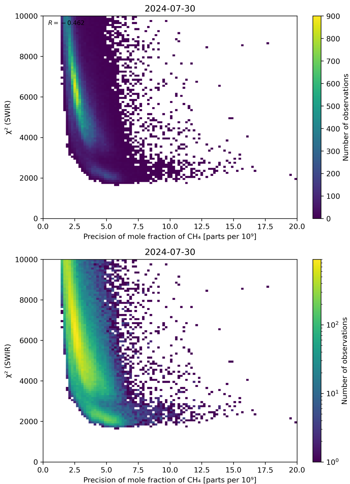
Figure 79: Scatter density plot of “Precision of mole fraction of CH 4 ” against “ \chi^2 (SWIR)” for 2024-07-29 to 2024-07-31.
