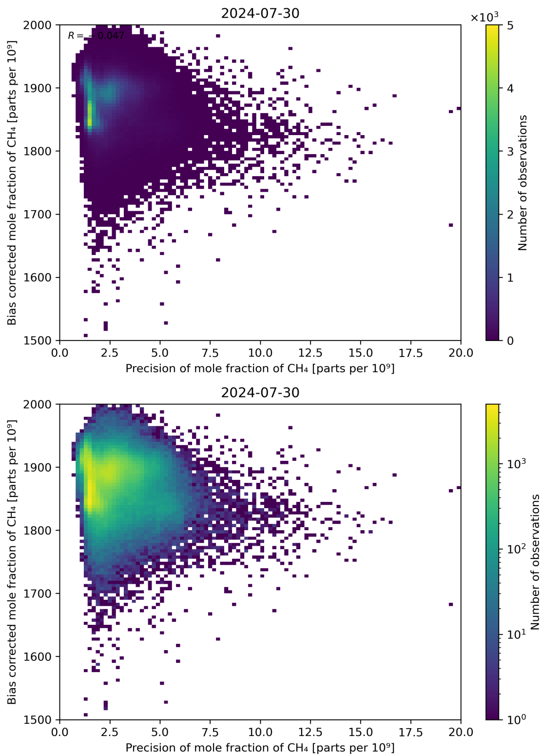
Figure 82: Scatter density plot of “Precision of mole fraction of CH 4 ” against “Bias corrected mole fraction of CH 4 ” for 2024-07-29 to 2024-07-31.
