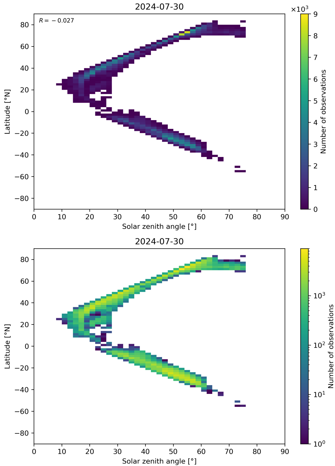
Figure 98: Scatter density plot of “Solar zenith angle” against “Latitude” for 2024-07-29 to 2024-07-31.
