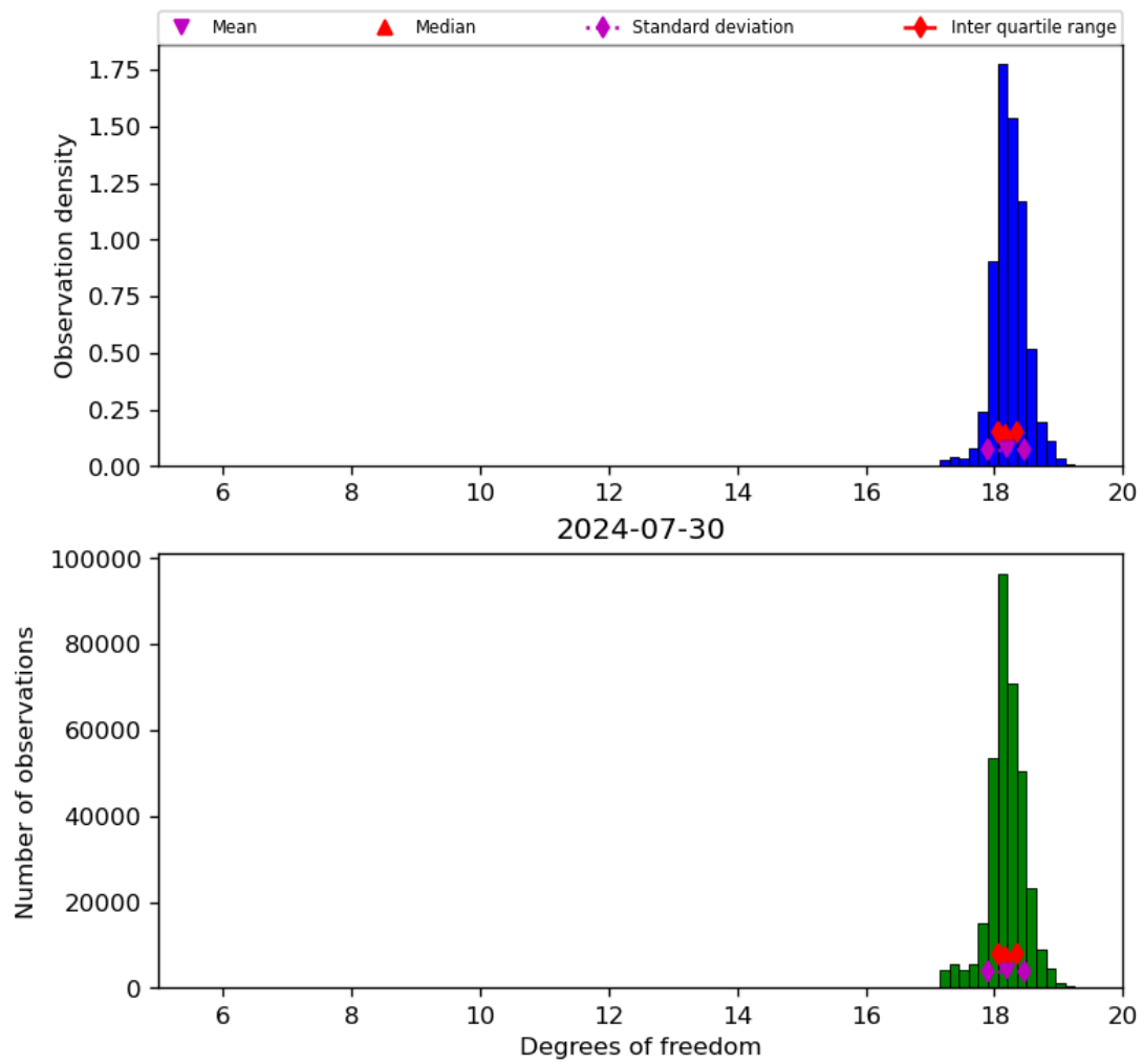
Figure 30: Histogram of “Degrees of freedom” for 2024-07-29 to 2024-07-31
