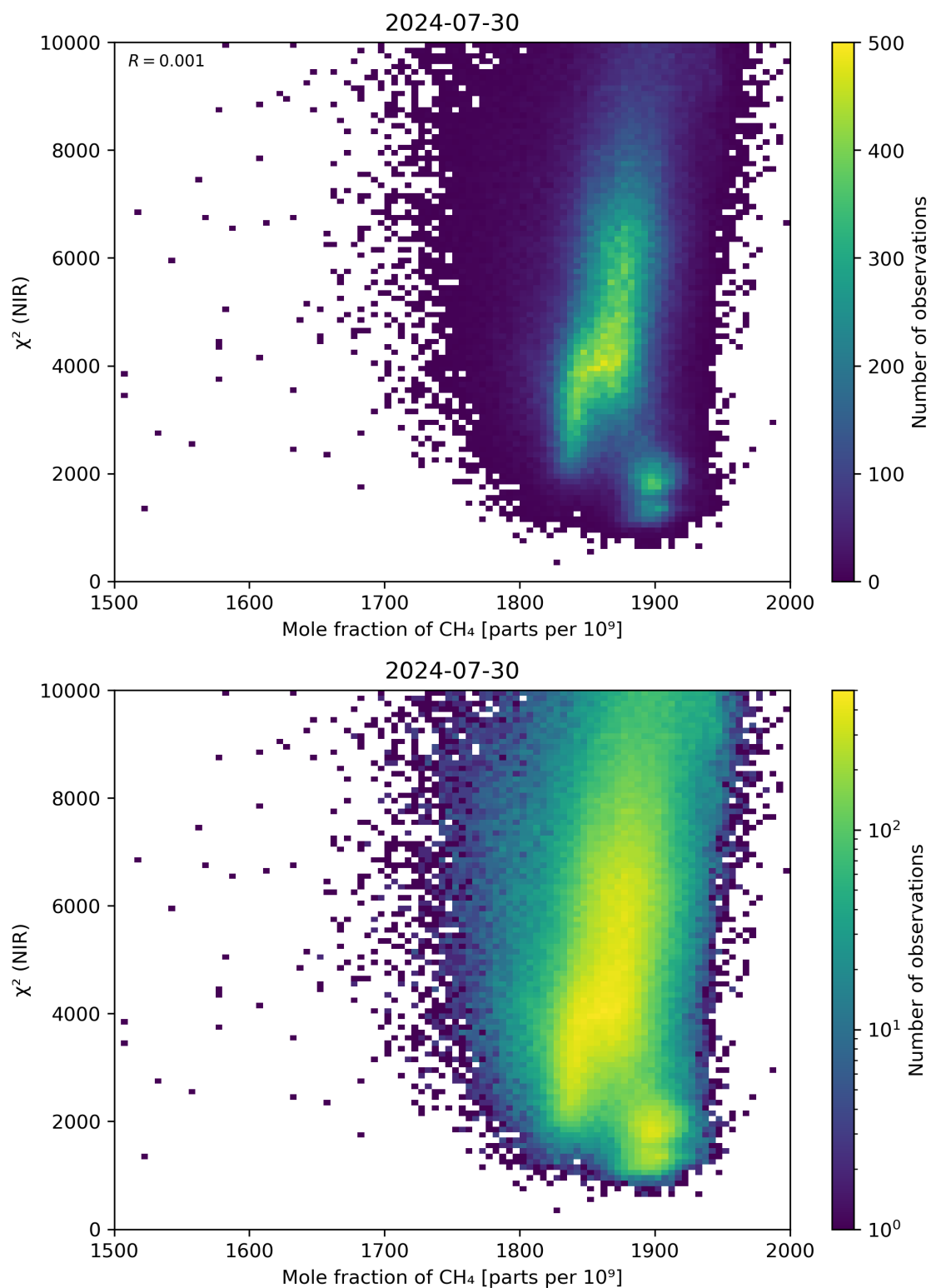
Figure 70: Scatter density plot of “Mole fraction of \text{CH}_4 ” against “ \chi^2 (NIR)” for 2024-07-29 to 2024-07-31.
