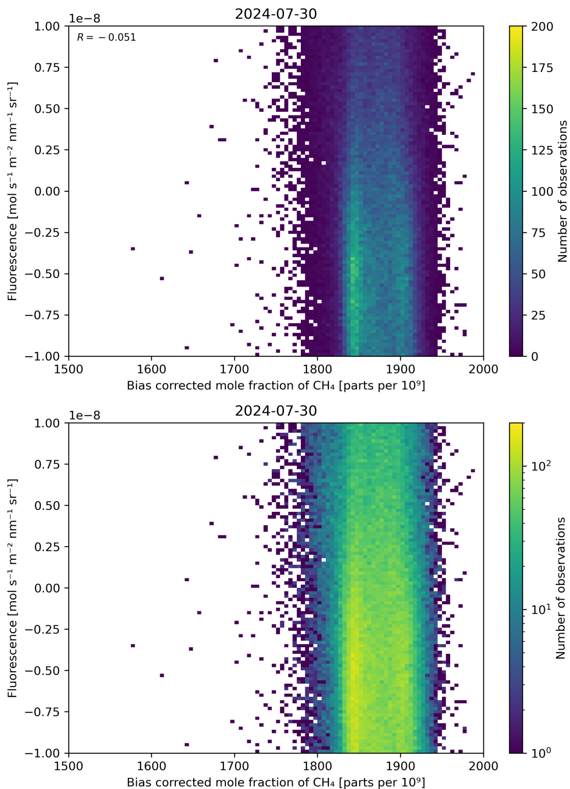
Figure 66: Scatter density plot of “Bias corrected mole fraction of \text{CH}_4 ” against “Fluorescence” for 2024-07-29 to 2024-07-31.
