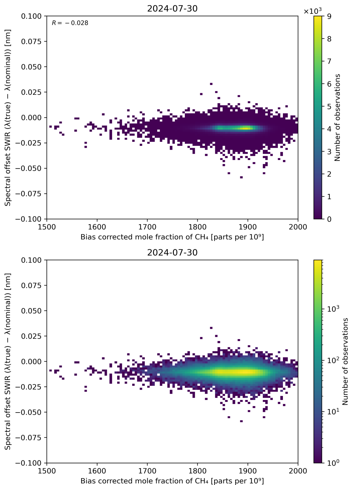
Figure 69: Scatter density plot of “Bias corrected mole fraction of CH 4 ” against “Spectral offset SWIR ( \lambda(\text{true}) - \lambda(\text{nominal}) )” for 2024-07-29 to 2024-07-31.
