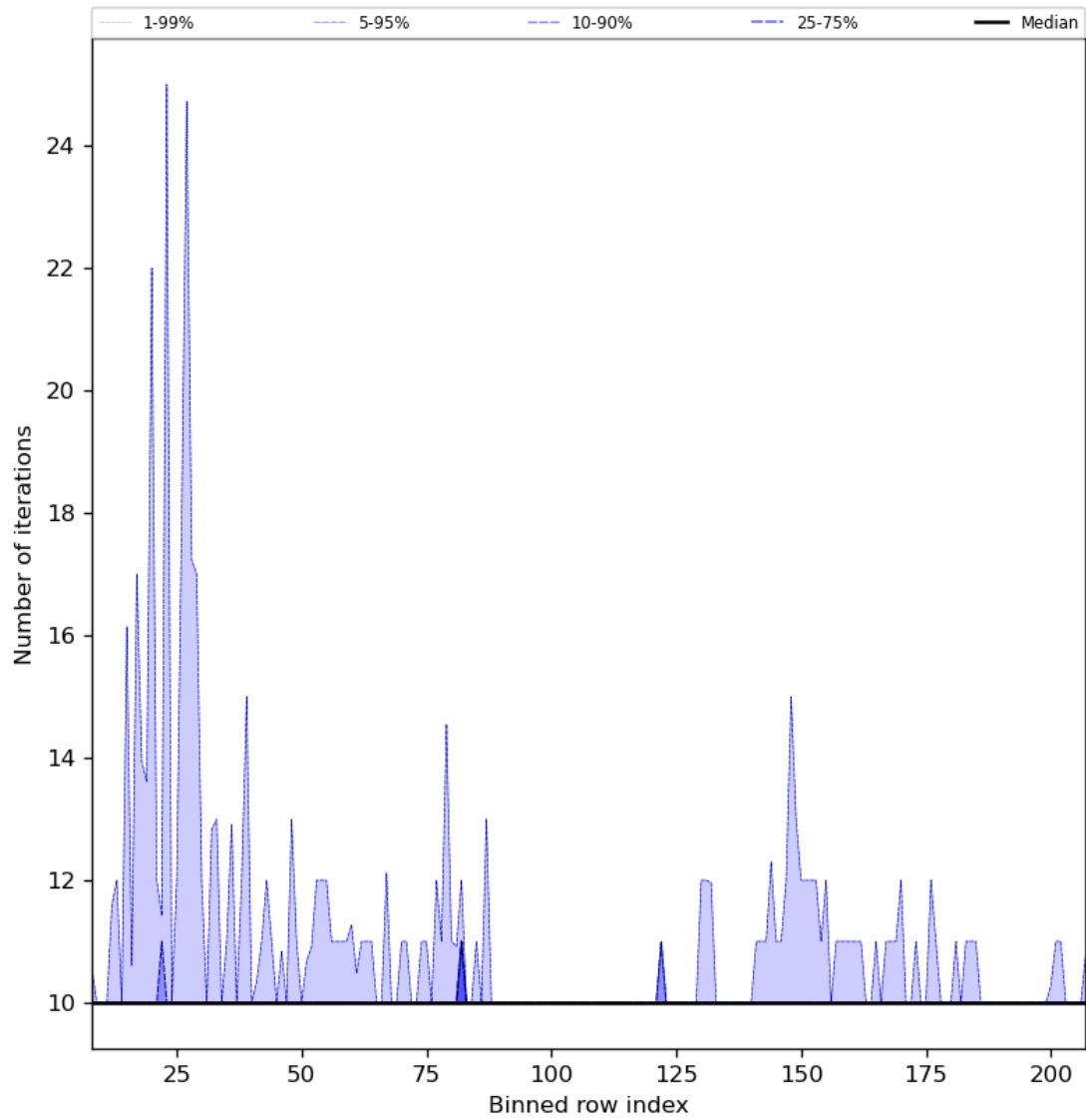
Figure 42: Along track statistics of “Number of iterations” for 2024-07-29 to 2024-07-31
