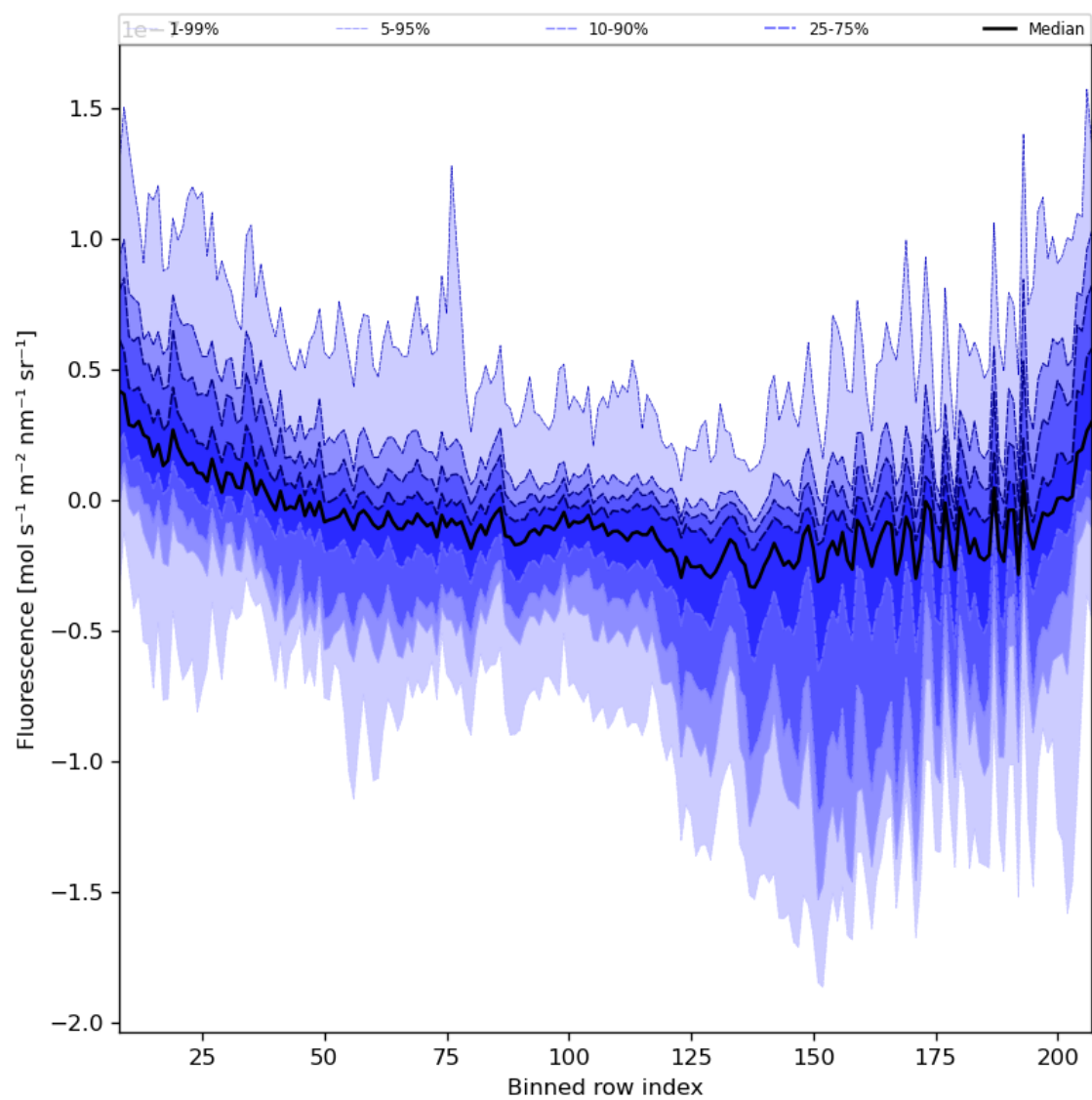
Figure 43: Along track statistics of “Fluorescence” for 2024-07-29 to 2024-07-31
