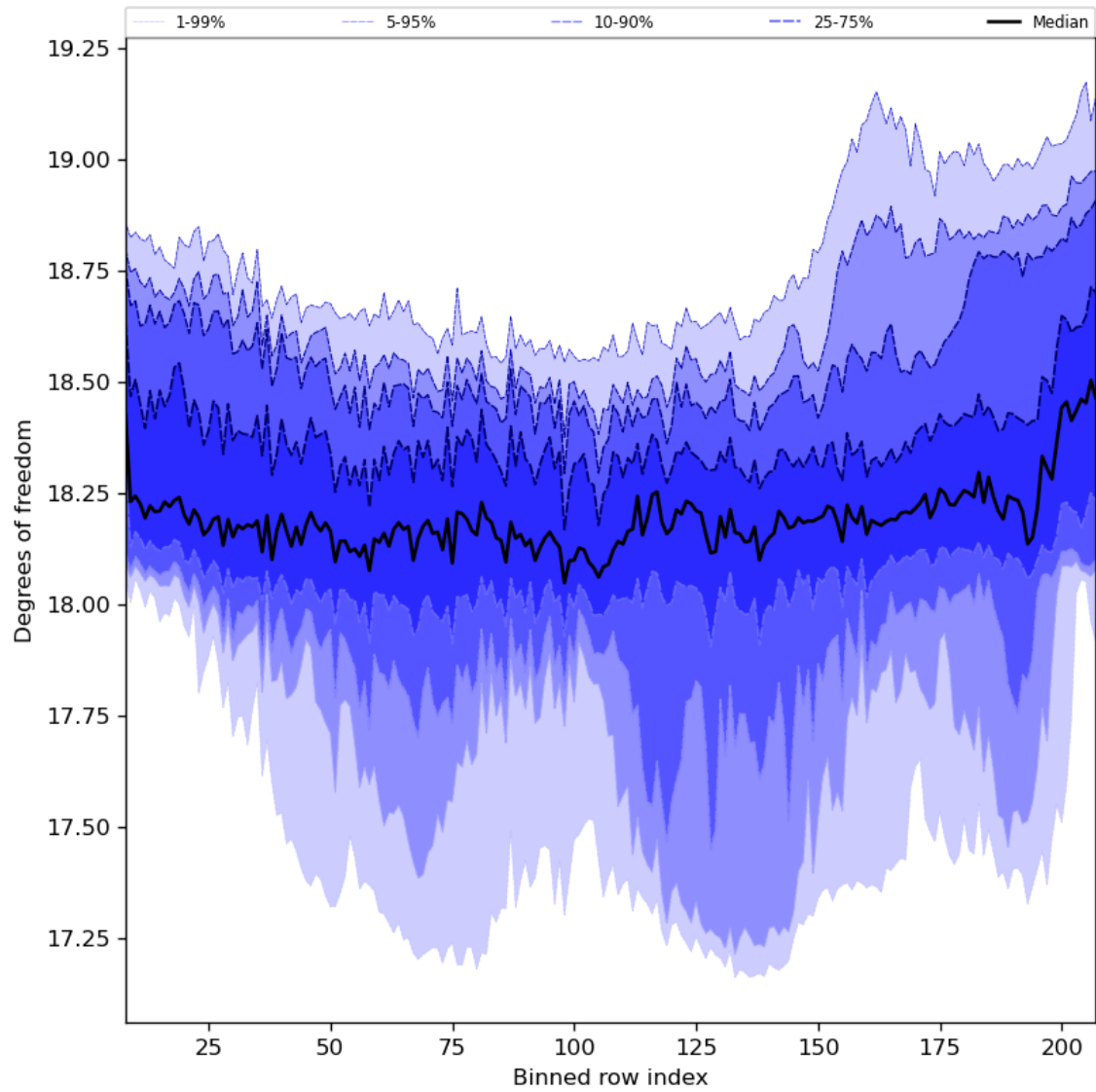
Figure 41: Along track statistics of “Degrees of freedom” for 2024-07-29 to 2024-07-31
