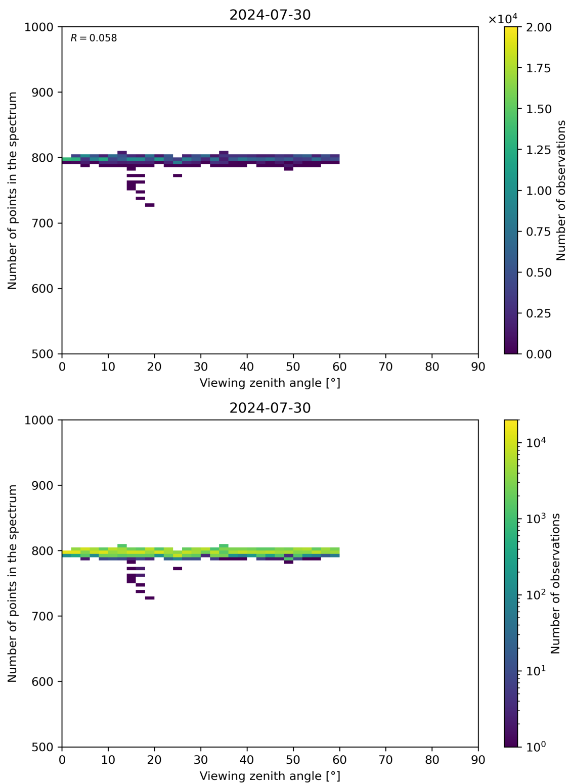
Figure 114: Scatter density plot of “Viewing zenith angle” against “Number of points in the spectrum” for 2024-07-29 to 2024-07-31.
