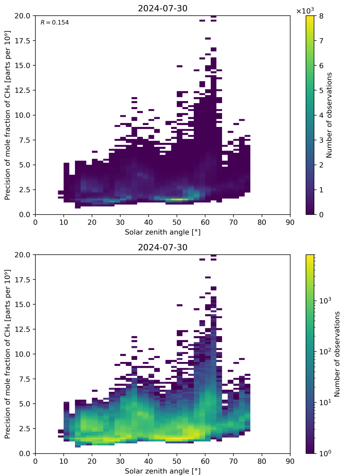
Figure 101: Scatter density plot of “Solar zenith angle” against “Precision of mole fraction of \text{CH}_4 ” for 2024-07-29 to 2024-07-31.
