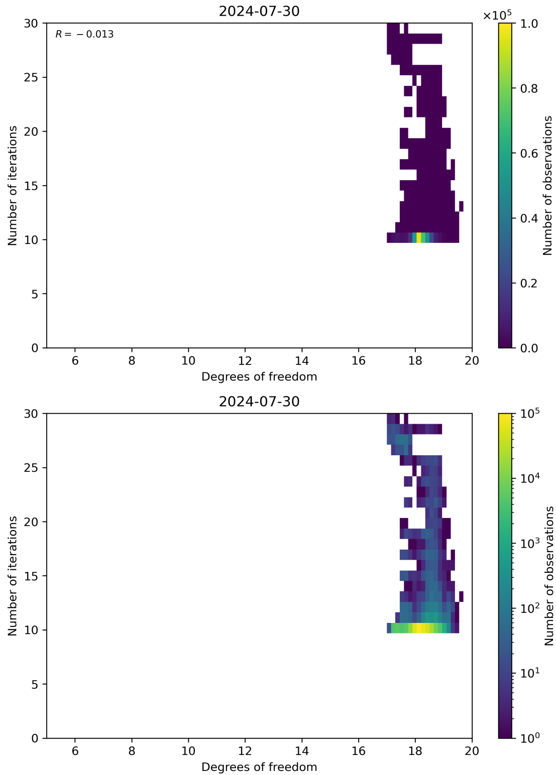
Figure 52: Scatter density plot of “Degrees of freedom” against “Number of iterations” for 2024-07-29 to 2024-07-31.
