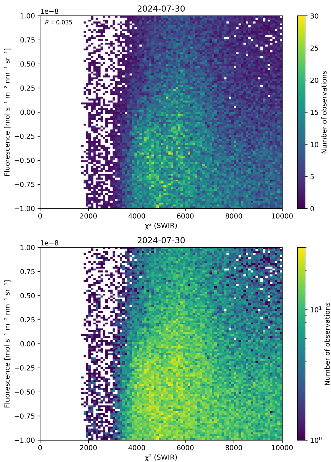
Figure 49: Scatter density plot of “ \chi^2 (SWIR)” against “Fluorescence” for 2024-07-29 to 2024-07-31.
