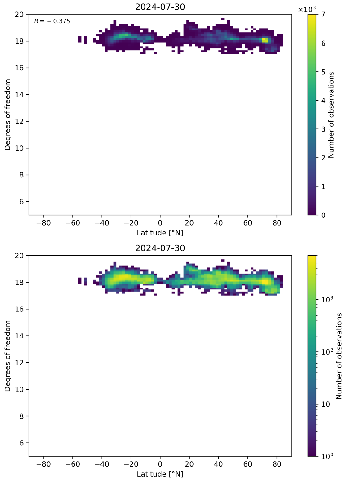
Figure 55: Scatter density plot of “Latitude” against “Degrees of freedom” for 2024-07-29 to 2024-07-31.
