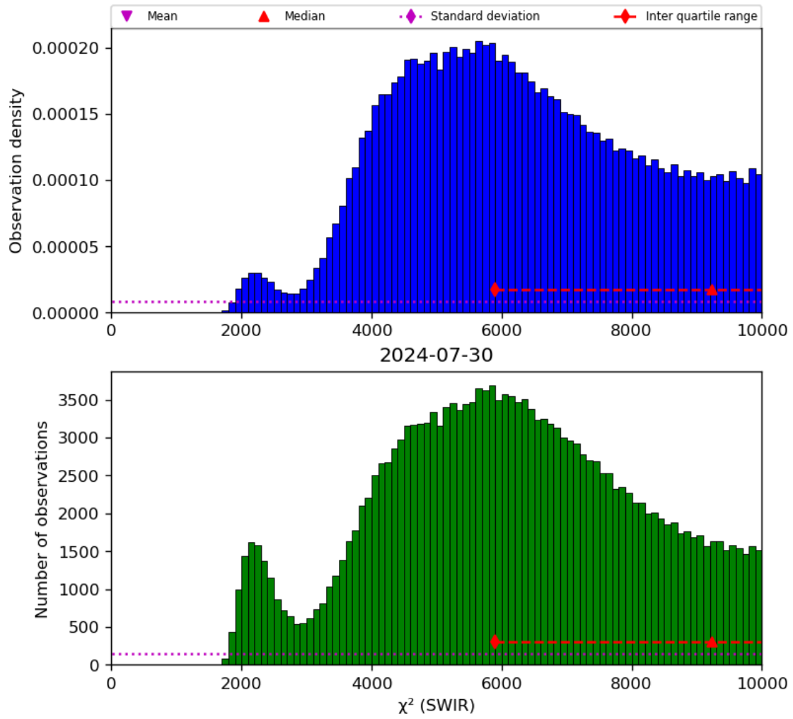
Figure 28: Histogram of " \chi^2 (SWIR)" for 2024-07-29 to 2024-07-31
