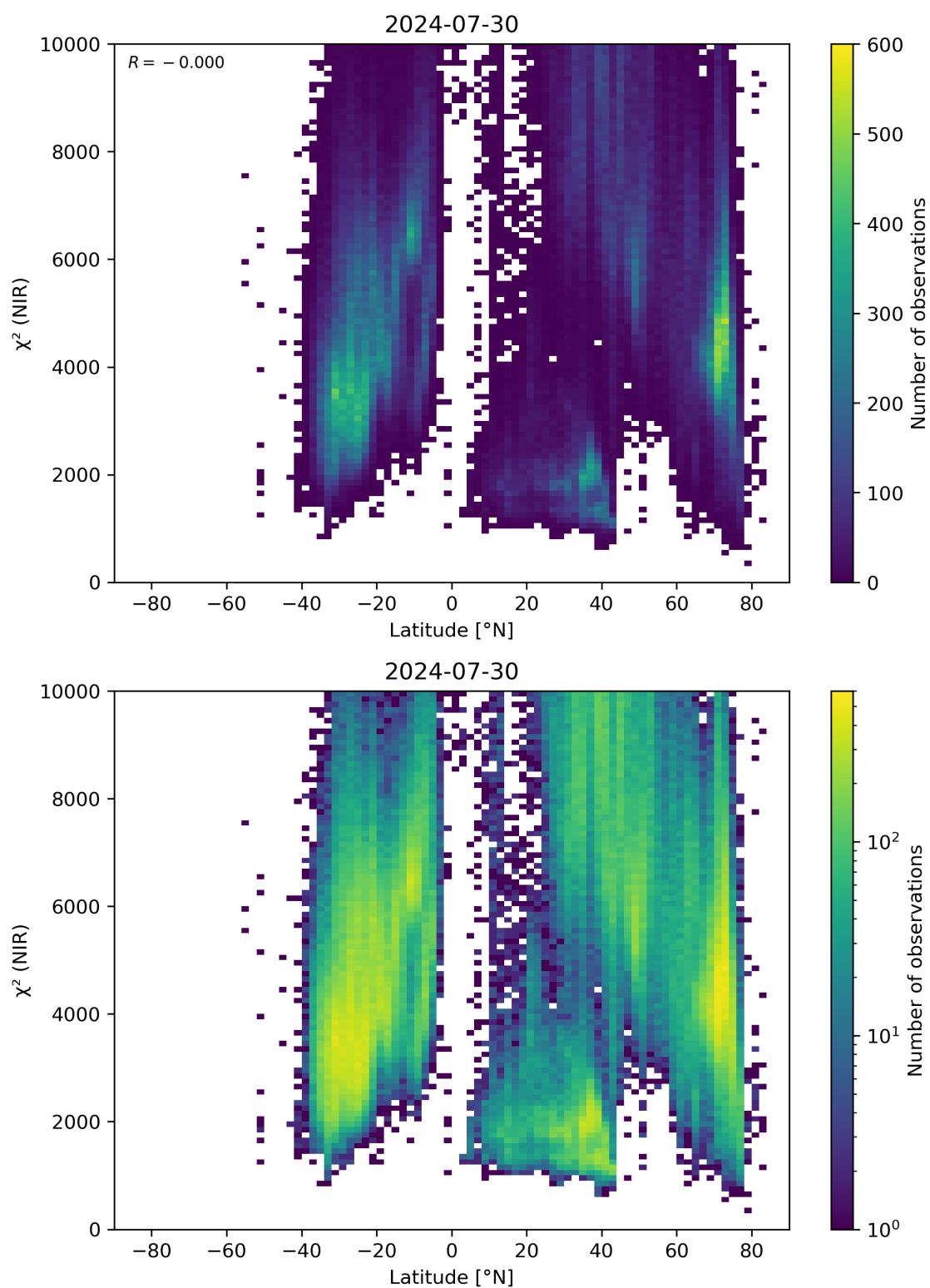
Figure 53: Scatter density plot of “Latitude” against “ \chi^2 (NIR)” for 2024-07-29 to 2024-07-31.
