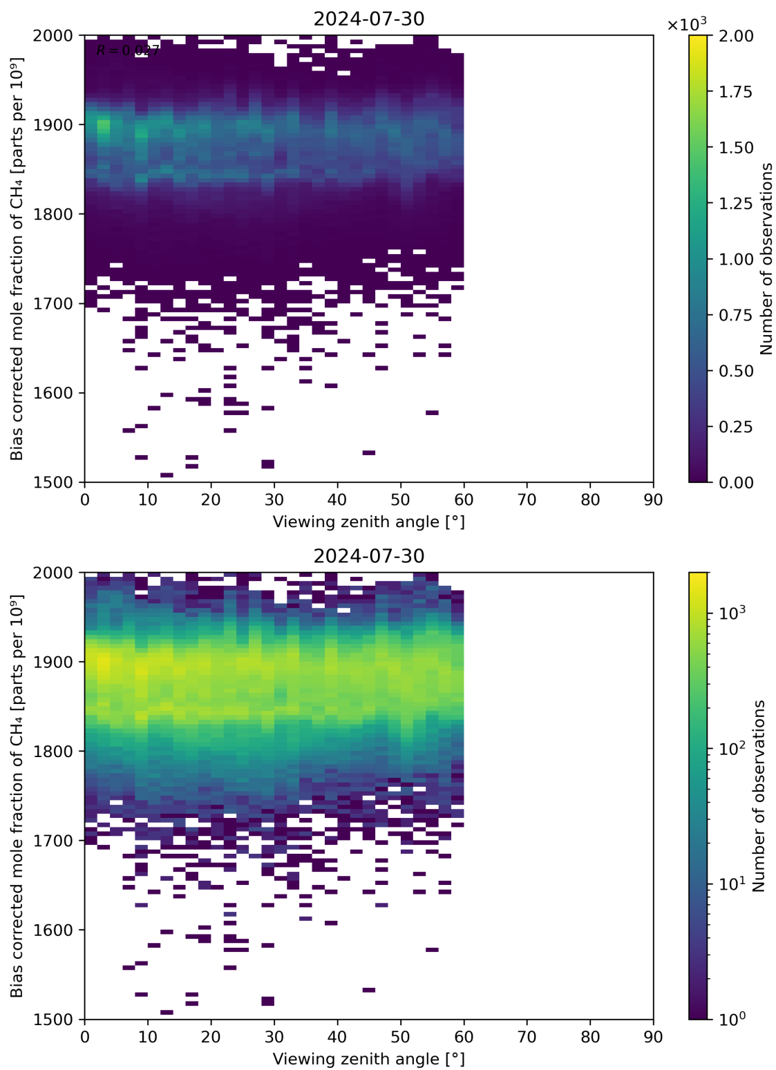
Figure 111: Scatter density plot of “Viewing zenith angle” against “Bias corrected mole fraction of CH 4 ” for 2024-07-29 to 2024-07-31.
