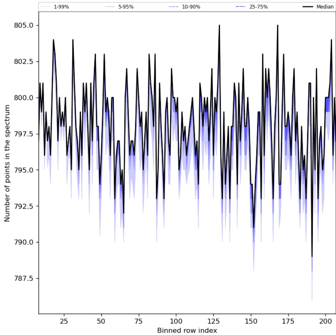
Figure 37: Along track statistics of “Number of points in the spectrum” for 2024-07-29 to 2024-07-31
