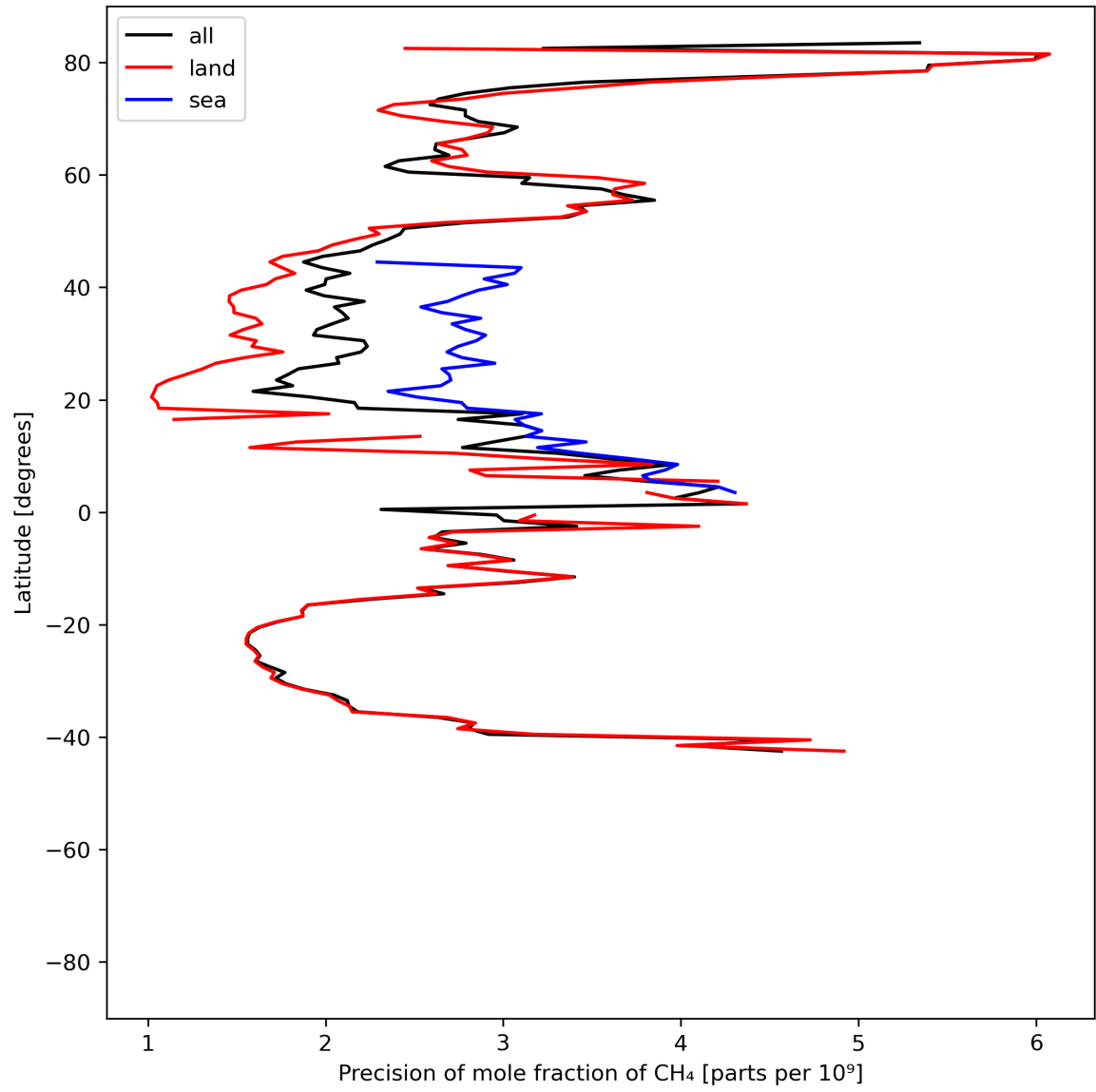
Figure 13: Zonal average of “Precision of mole fraction of CH 4 ” for 2024-07-29 to 2024-07-31.
