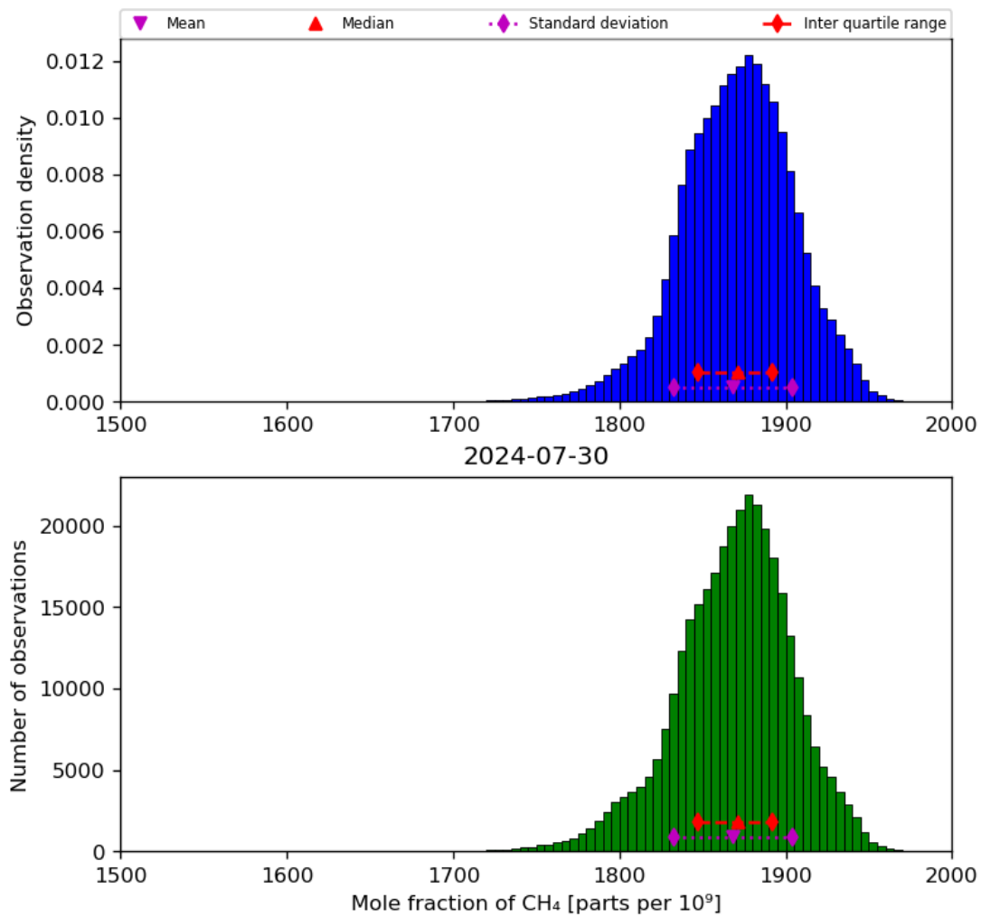
Figure 23: Histogram of “Mole fraction of CH 4 ” for 2024-07-29 to 2024-07-31
