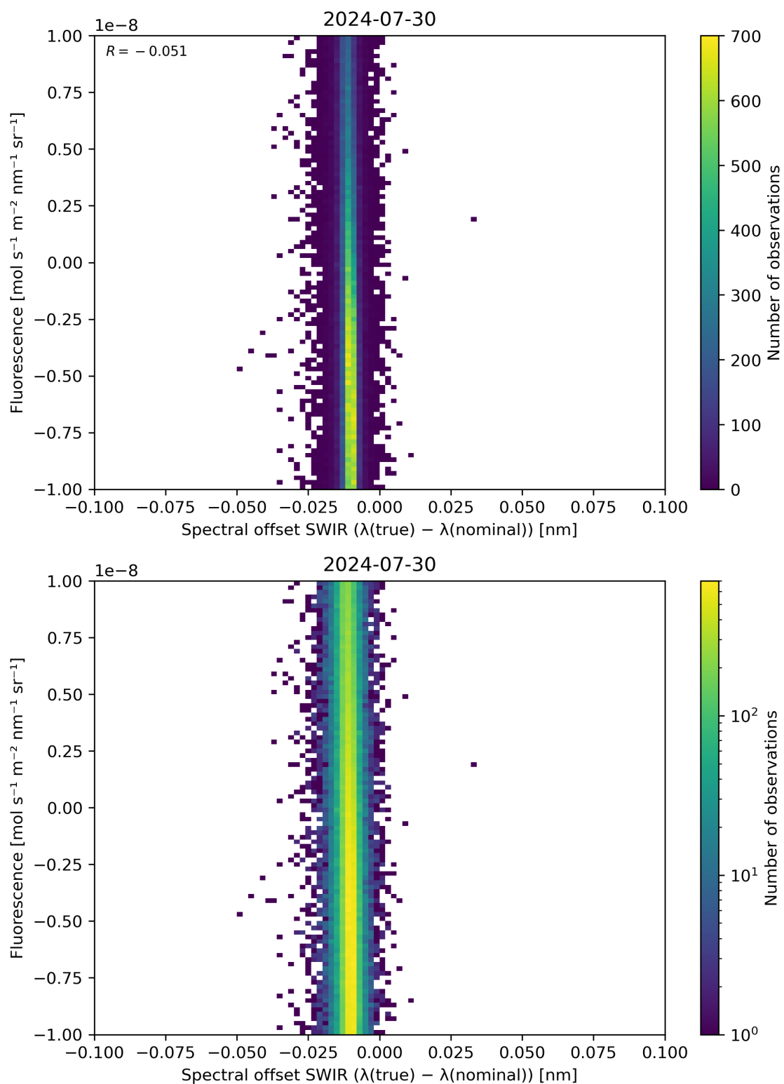
Figure 120: Scatter density plot of “Spectral offset SWIR ( \lambda(\text{true}) - \lambda(\text{nominal}) )” against “Fluorescence” for 2024-07-29 to 2024-07-31.
