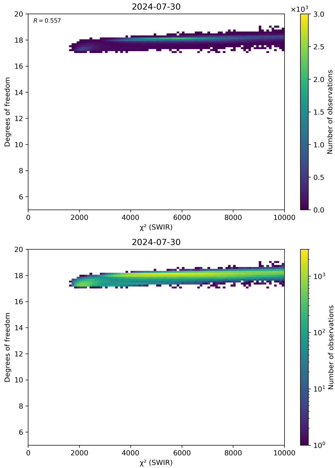
Figure 48: Scatter density plot of “ \chi^2 (SWIR)” against “Degrees of freedom” for 2024-07-29 to 2024-07-31.
