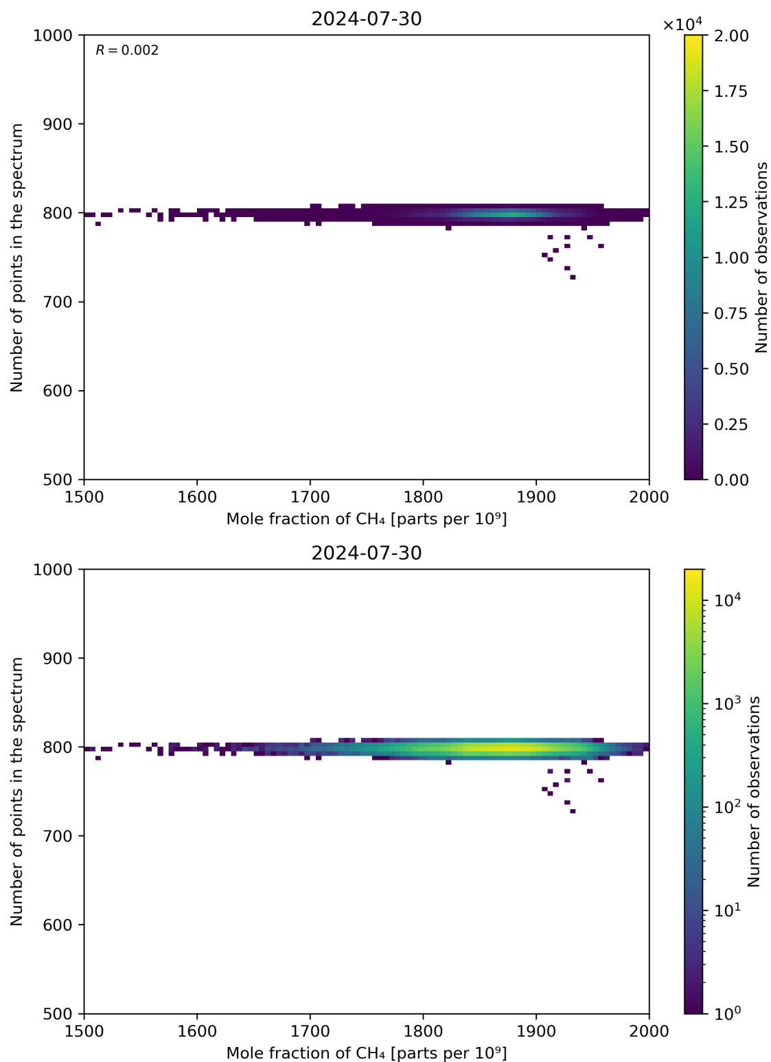
Figure 77: Scatter density plot of “Mole fraction of CH 4 ” against “Number of points in the spectrum” for 2024-07-29 to 2024-07-31.
