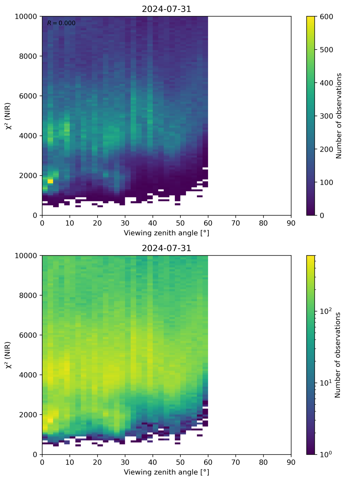
Figure 105: Scatter density plot of “Viewing zenith angle” against “ \chi^2 (NIR)” for 2024-07-31 to 2024-08-01.
