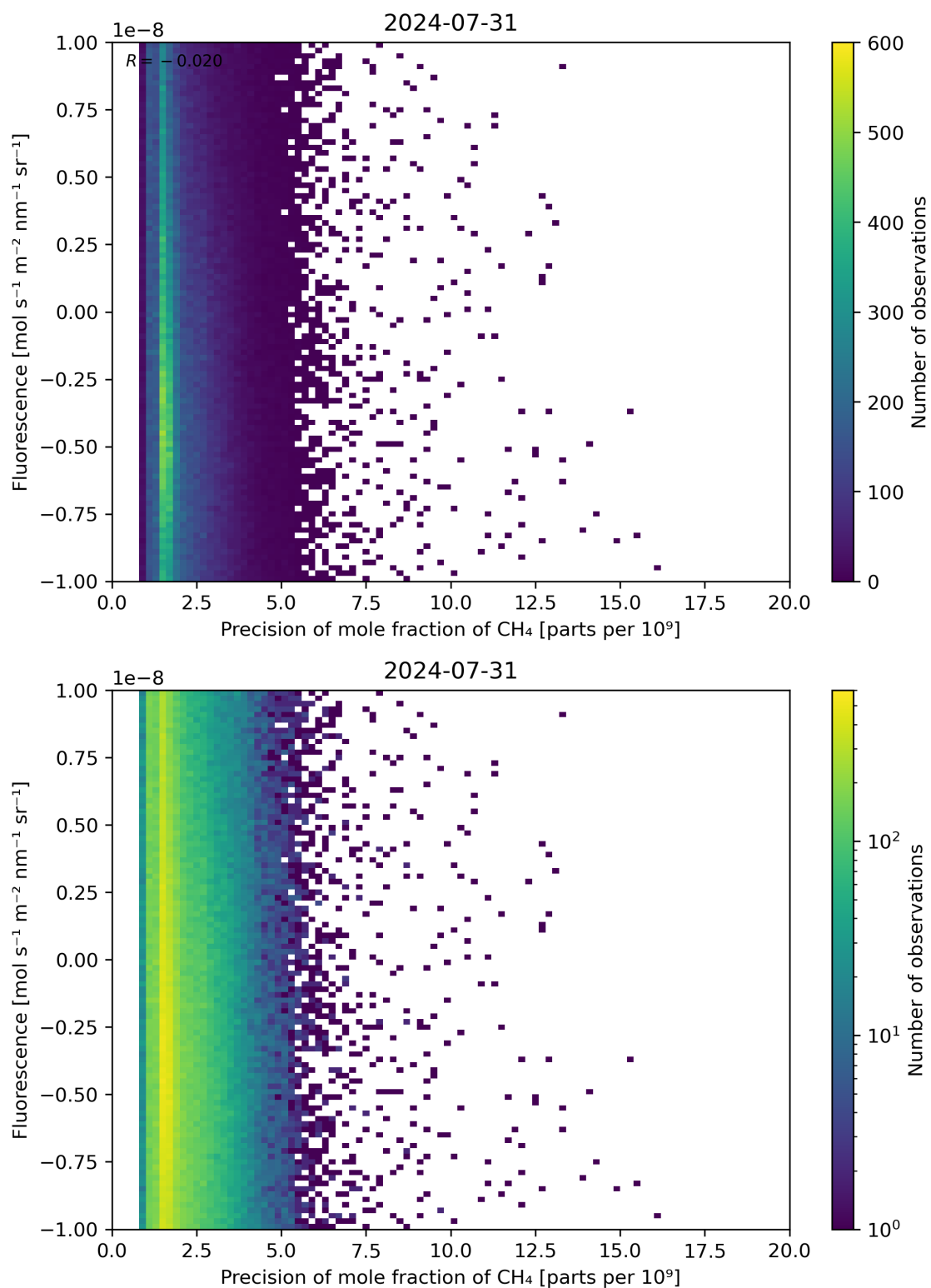
Figure 81: Scatter density plot of “Precision of mole fraction of CH 4 ” against “Fluorescence” for 2024-07-31 to 2024-08-01.
