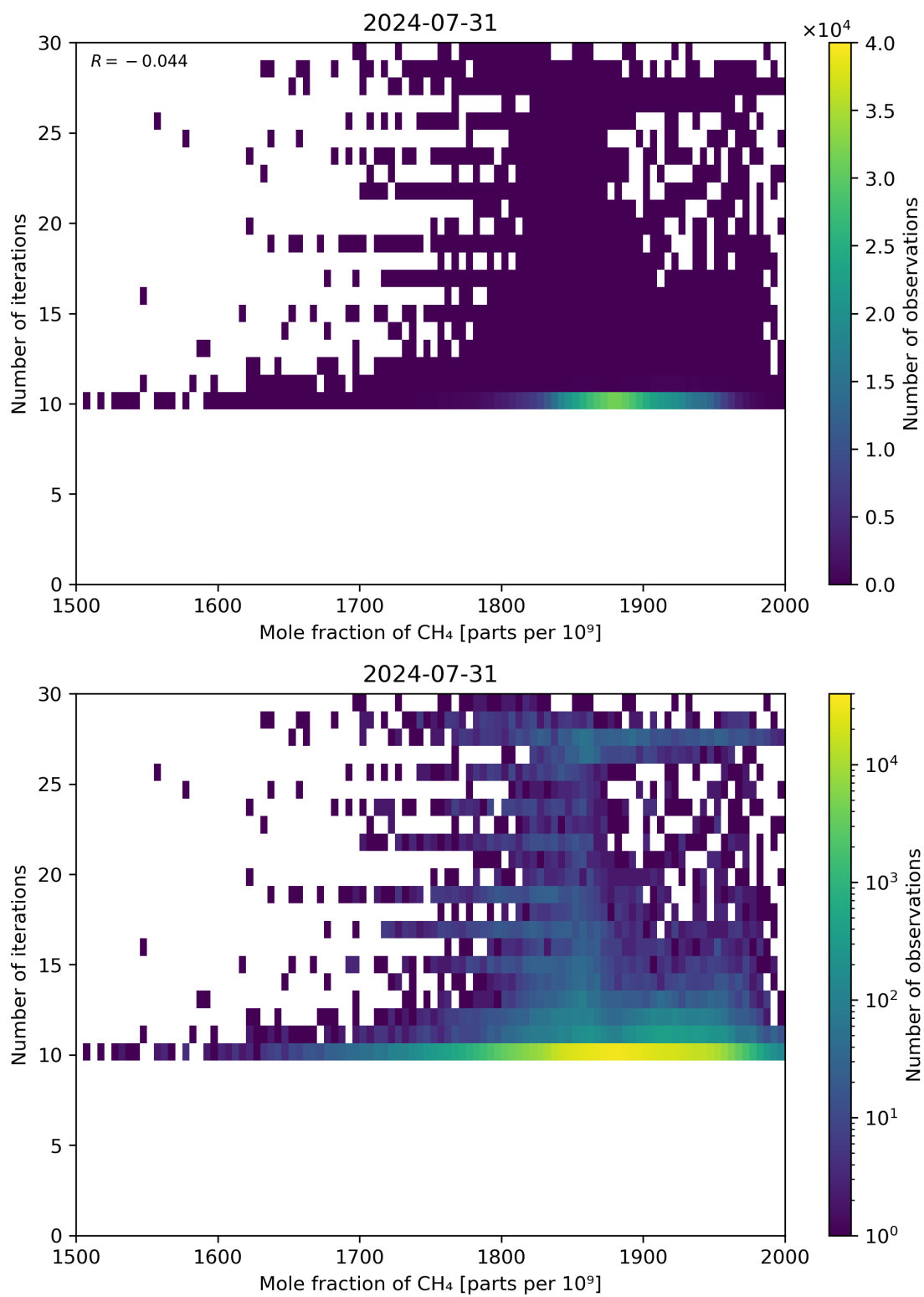
Figure 76: Scatter density plot of “Mole fraction of CH 4 ” against “Number of iterations” for 2024-07-31 to 2024-08-01.
