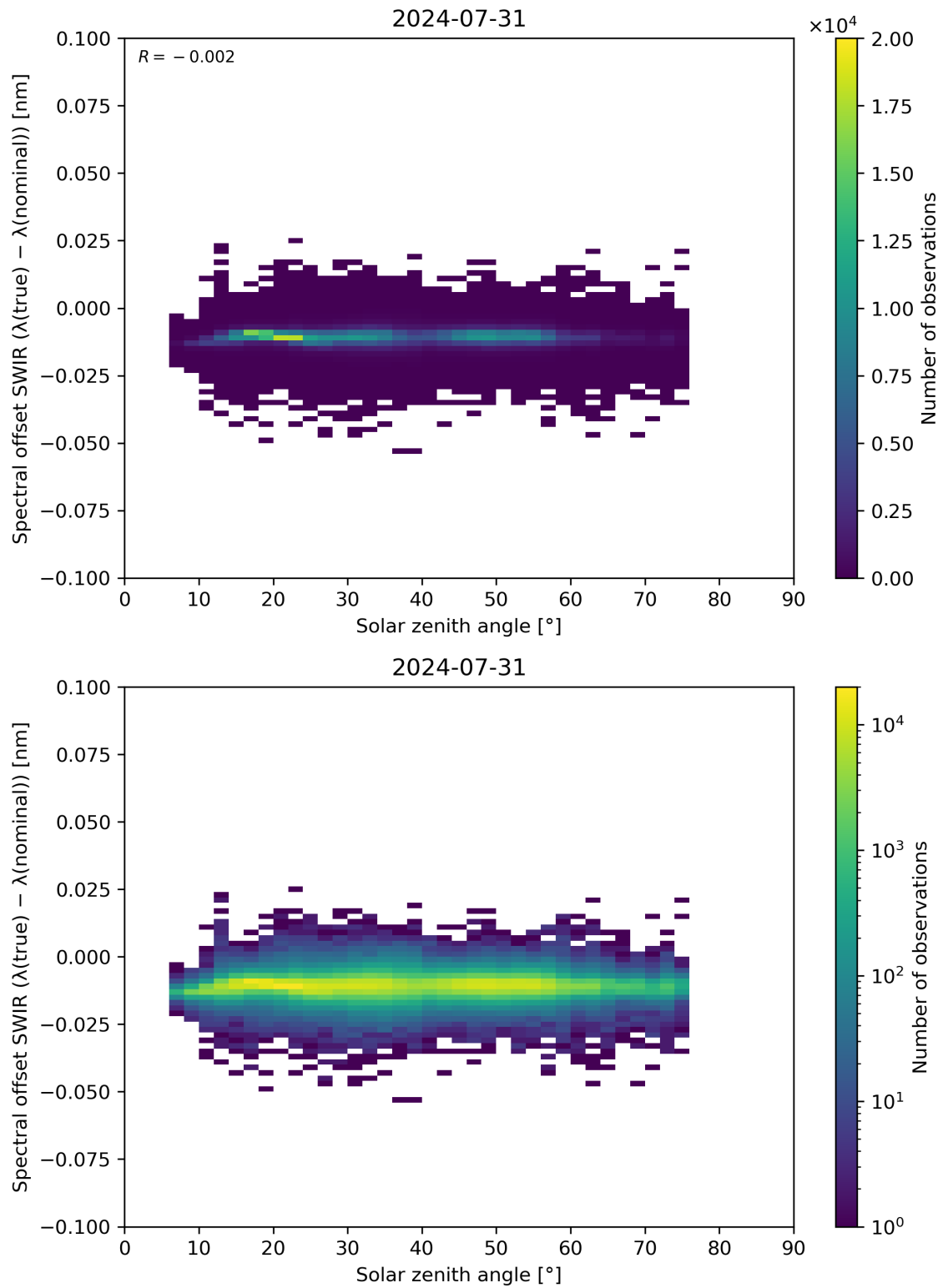
Figure 104: Scatter density plot of “Solar zenith angle” against “Spectral offset SWIR ( \lambda(\text{true}) - \lambda(\text{nominal}) )” for 2024-07-31 to 2024-08-01.
