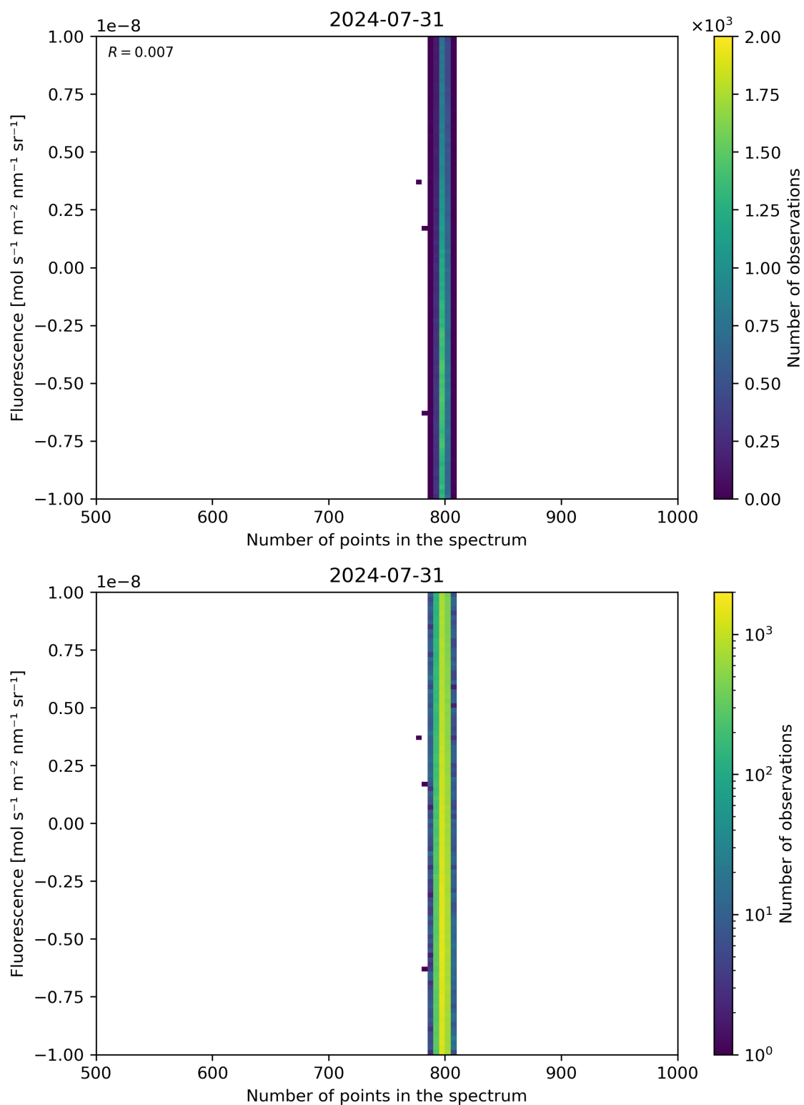
Figure 91: Scatter density plot of “Number of points in the spectrum” against “Fluorescence” for 2024-07-31 to 2024-08-01.
