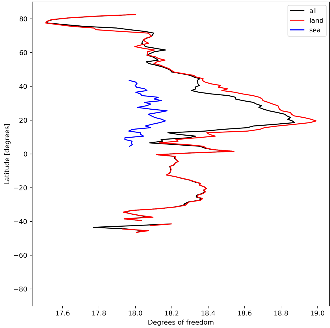
Figure 19: Zonal average of “Degrees of freedom” for 2024-07-31 to 2024-08-01.
