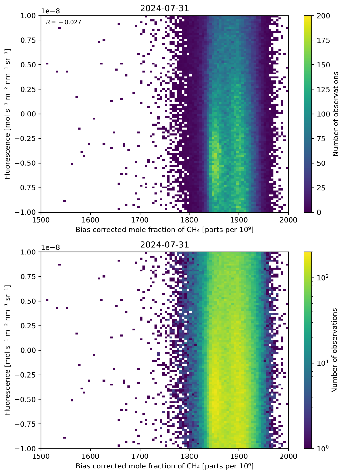
Figure 66: Scatter density plot of “Bias corrected mole fraction of CH 4 ” against “Fluorescence” for 2024-07-31 to 2024-08-01.
