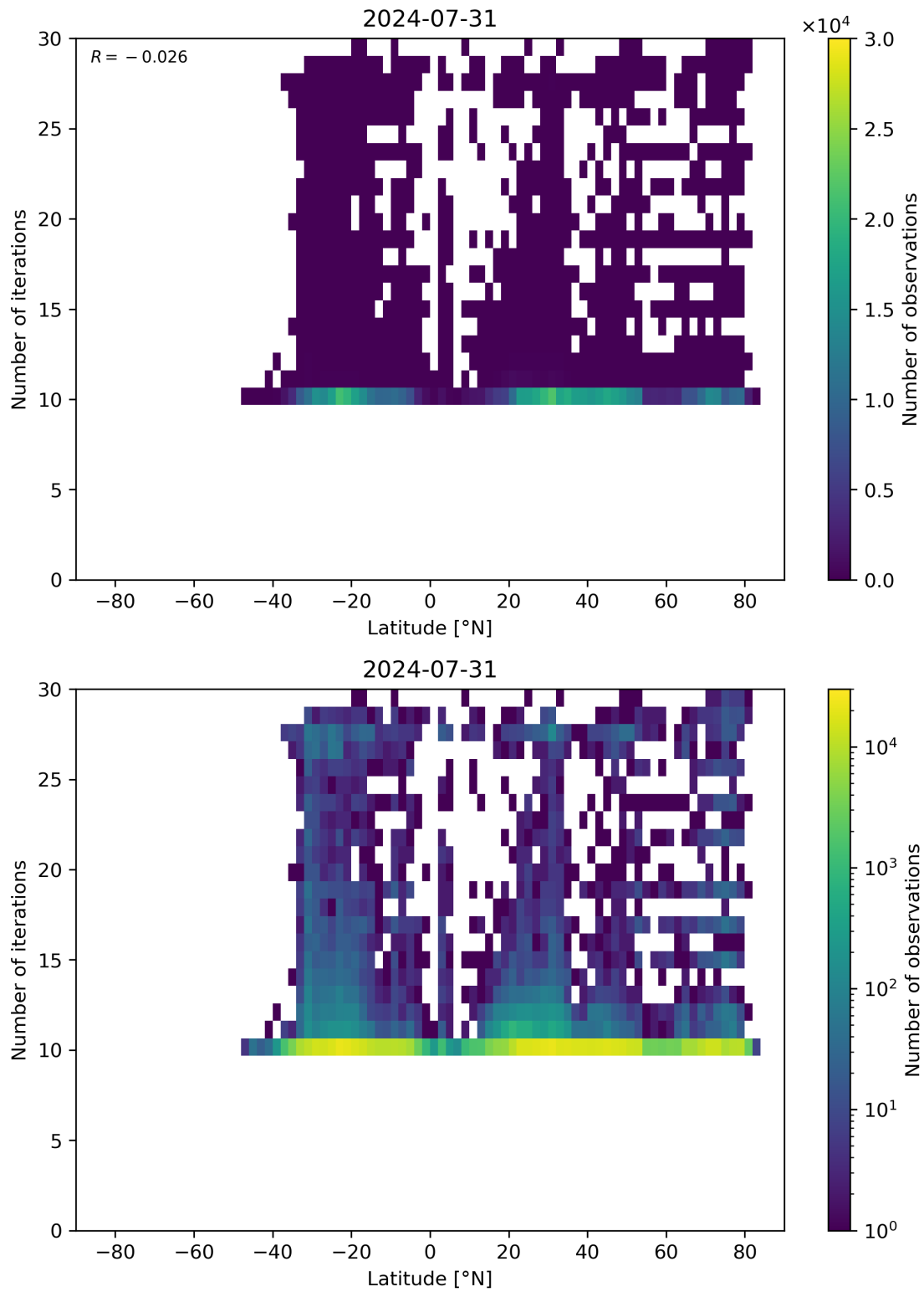
Figure 60: Scatter density plot of “Latitude” against “Number of iterations” for 2024-07-31 to 2024-08-01.
