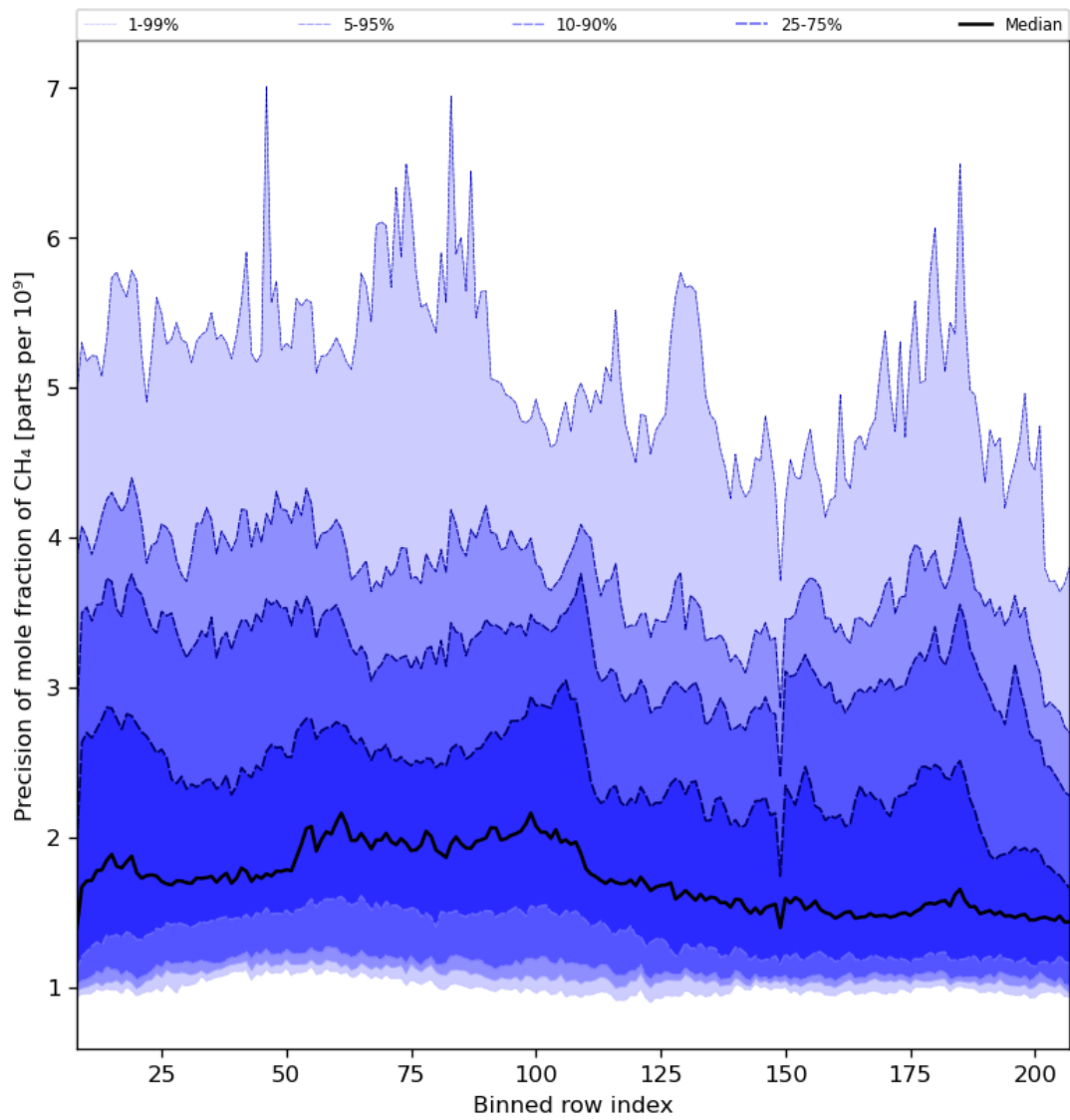
Figure 35: Along track statistics of “Precision of mole fraction of CH 4 ” for 2024-07-31 to 2024-08-01
