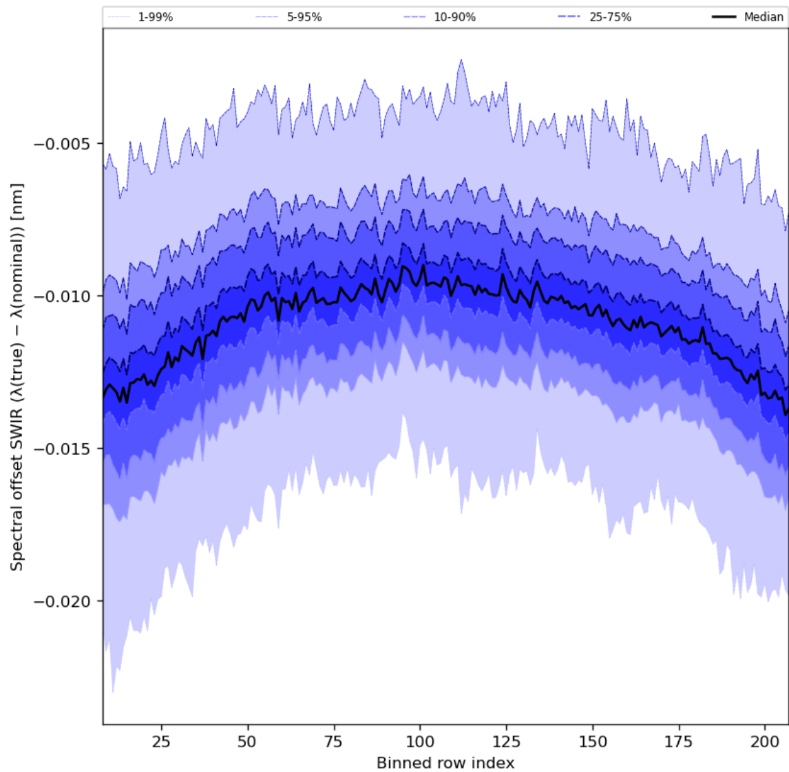
Figure 38: Along track statistics of “Spectral offset SWIR ( \lambda(\text{true}) - \lambda(\text{nominal}) )” for 2024-07-31 to 2024-08-01
