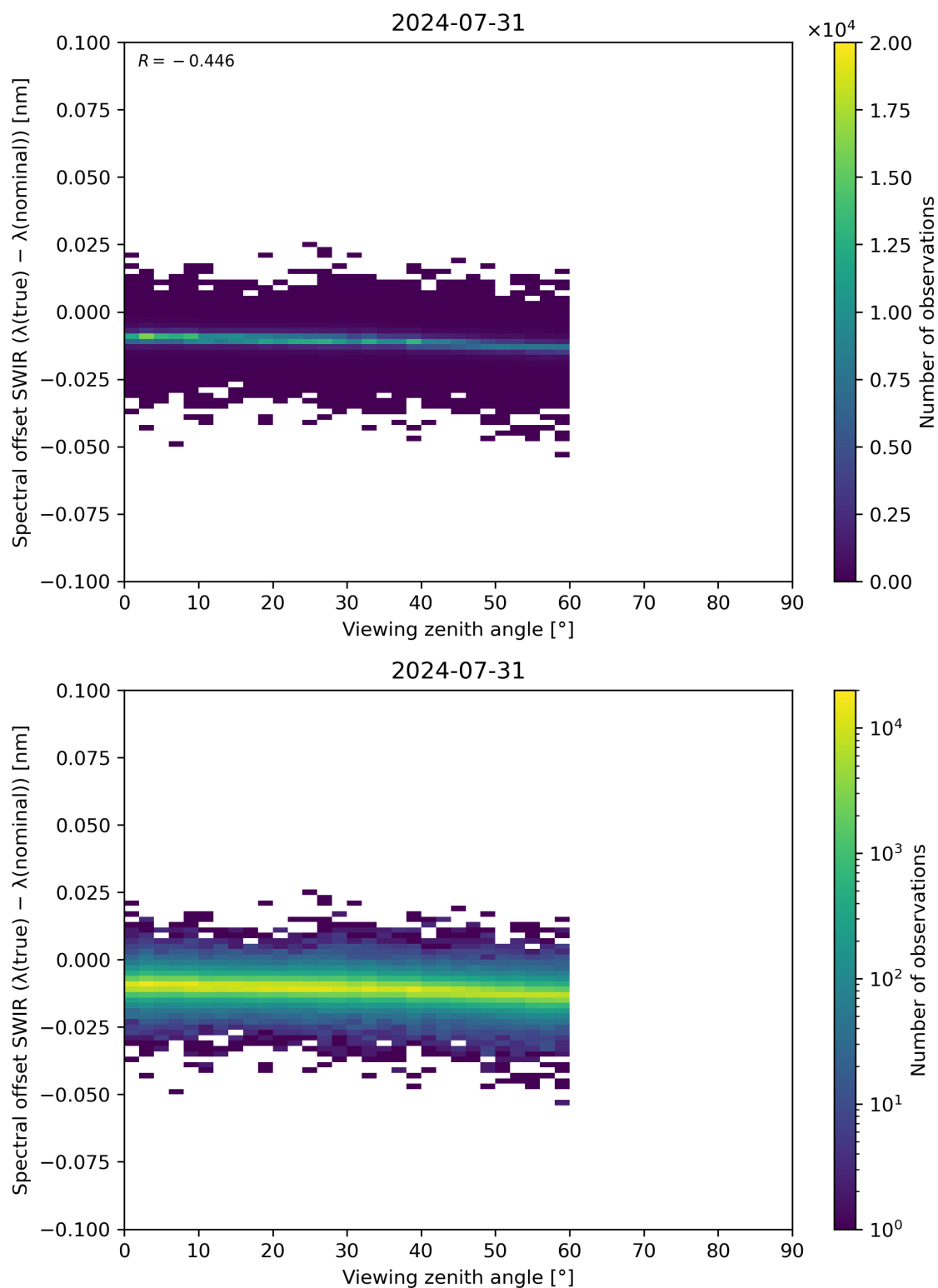
Figure 116: Scatter density plot of “Viewing zenith angle” against “Spectral offset SWIR ( \lambda(\text{true}) - \lambda(\text{nominal}) )” for 2024-07-31 to 2024-08-01.
