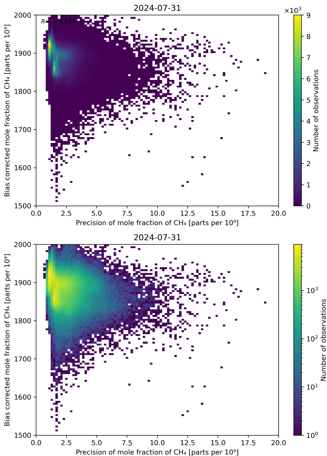
Figure 82: Scatter density plot of “Precision of mole fraction of \text{CH}_4 ” against “Bias corrected mole fraction of \text{CH}_4 ” for 2024-07-31 to 2024-08-01.
