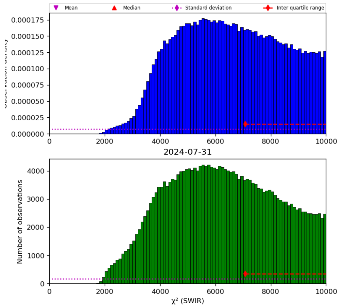
Figure 28: Histogram of “ \chi^2 (SWIR)” for 2024-07-31 to 2024-08-01
