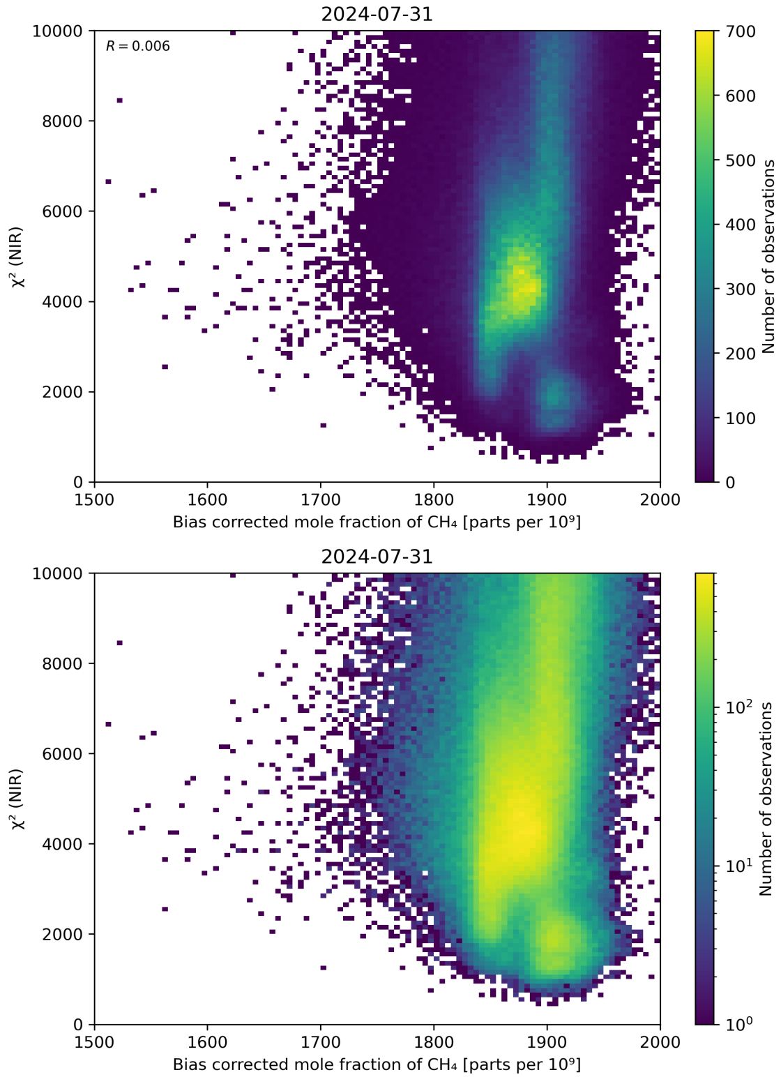
Figure 63: Scatter density plot of “Bias corrected mole fraction of CH 4 ” against “ \chi^2 (NIR)” for 2024-07-31 to 2024-08-01.
