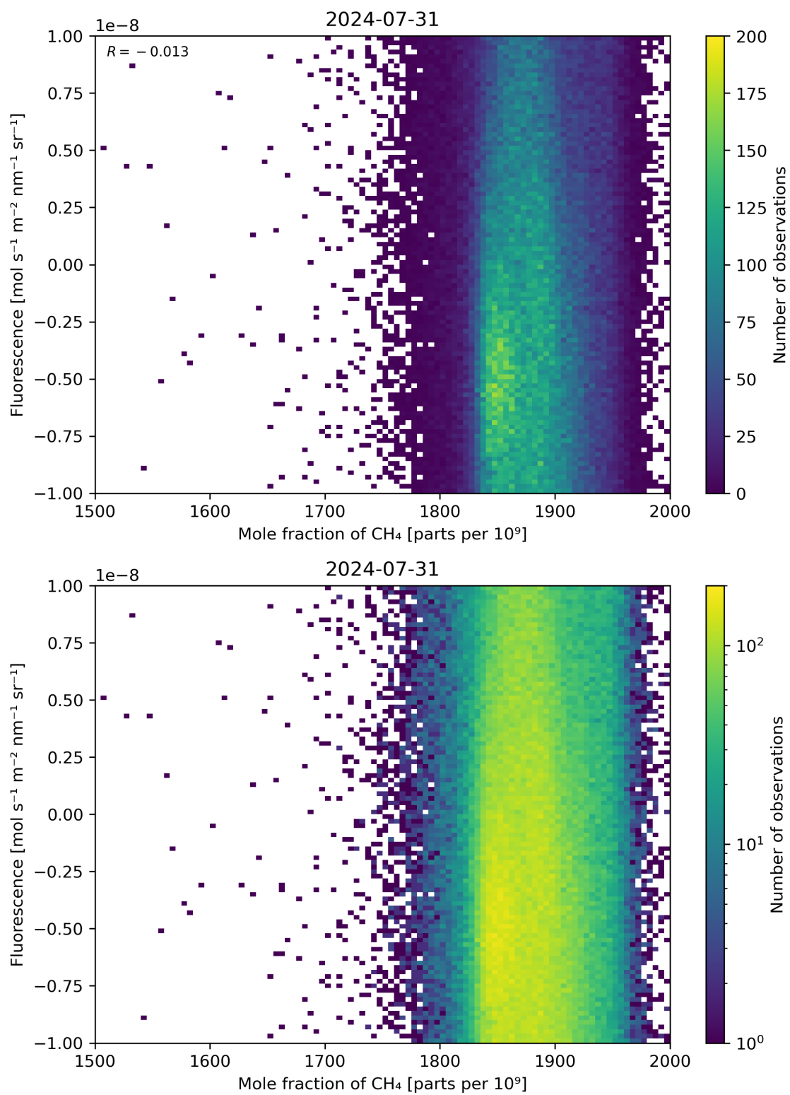
Figure 73: Scatter density plot of “Mole fraction of \text{CH}_4 ” against “Fluorescence” for 2024-07-31 to 2024-08-01.
