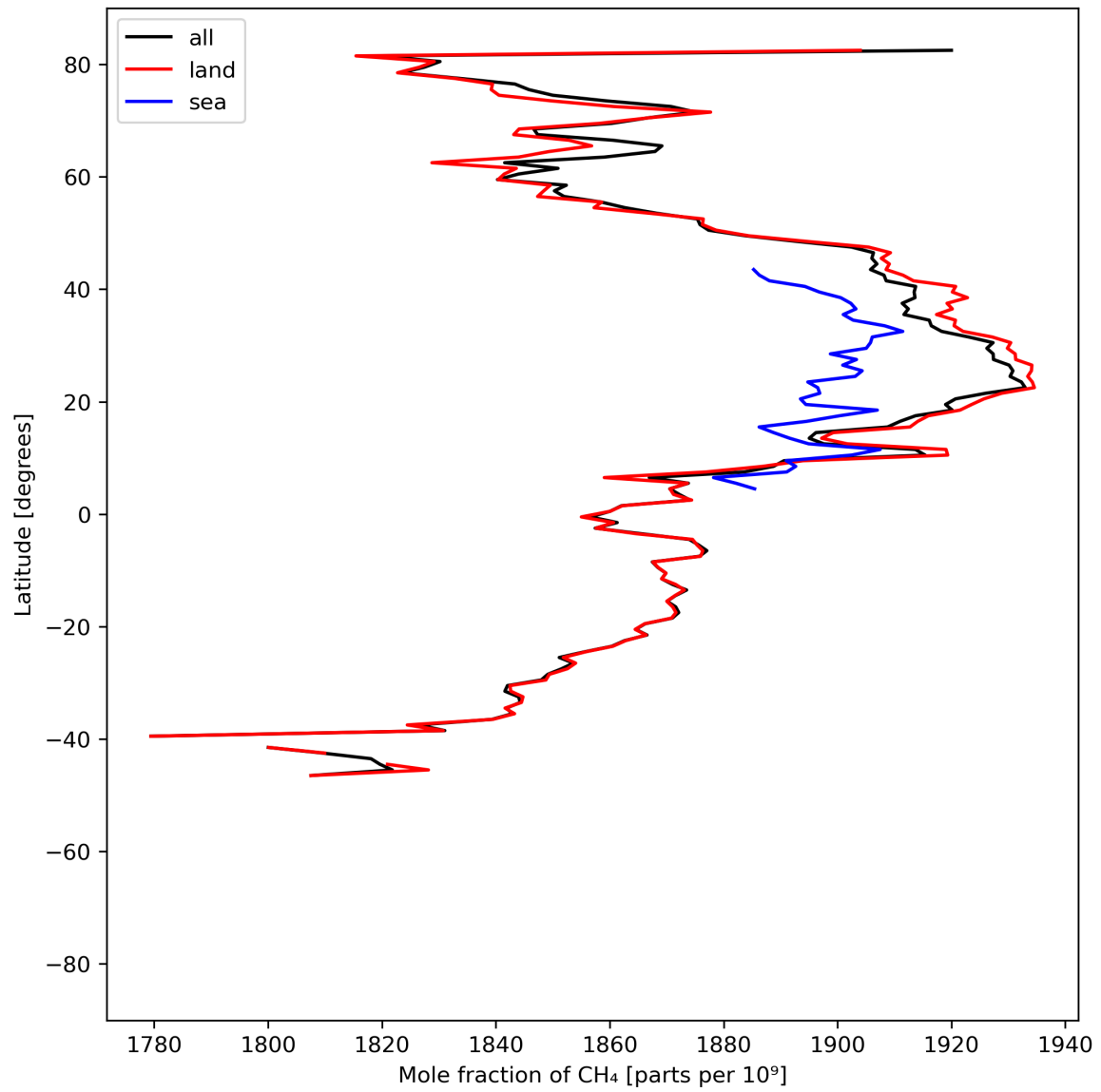
Figure 12: Zonal average of “Mole fraction of \text{CH}_4 ” for 2024-07-31 to 2024-08-01.
