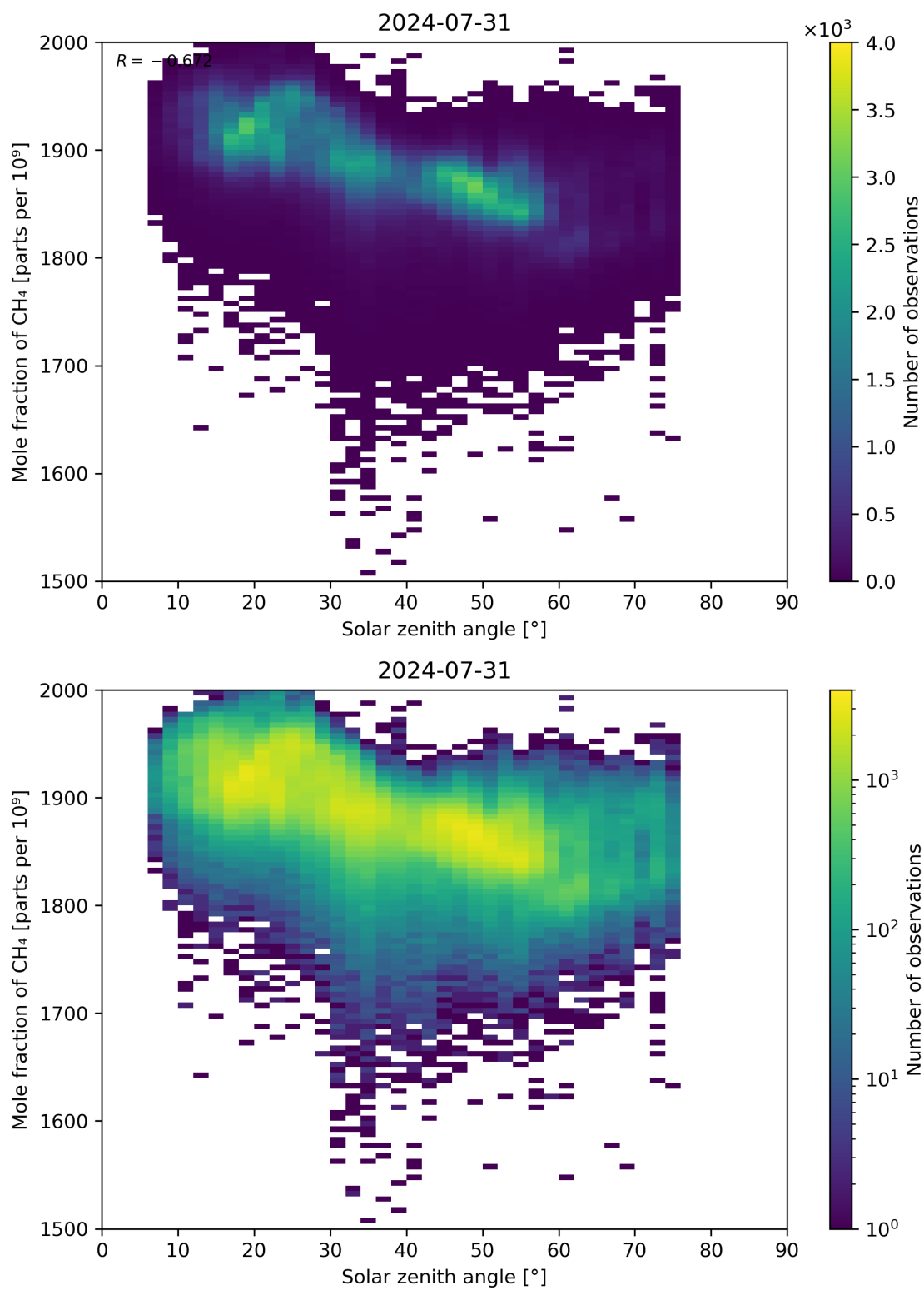
Figure 99: Scatter density plot of “Solar zenith angle” against “Mole fraction of CH 4 ” for 2024-07-31 to 2024-08-01.
