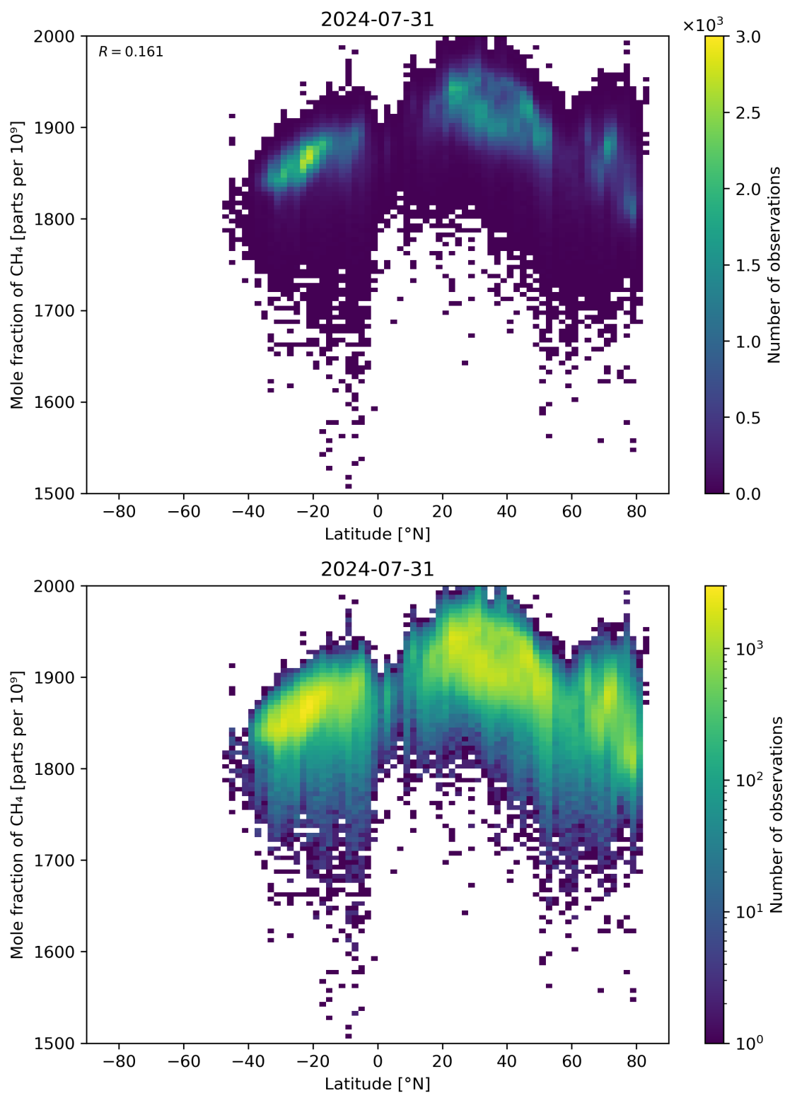
Figure 57: Scatter density plot of “Latitude” against “Mole fraction of \text{CH}_4 ” for 2024-07-31 to 2024-08-01.
