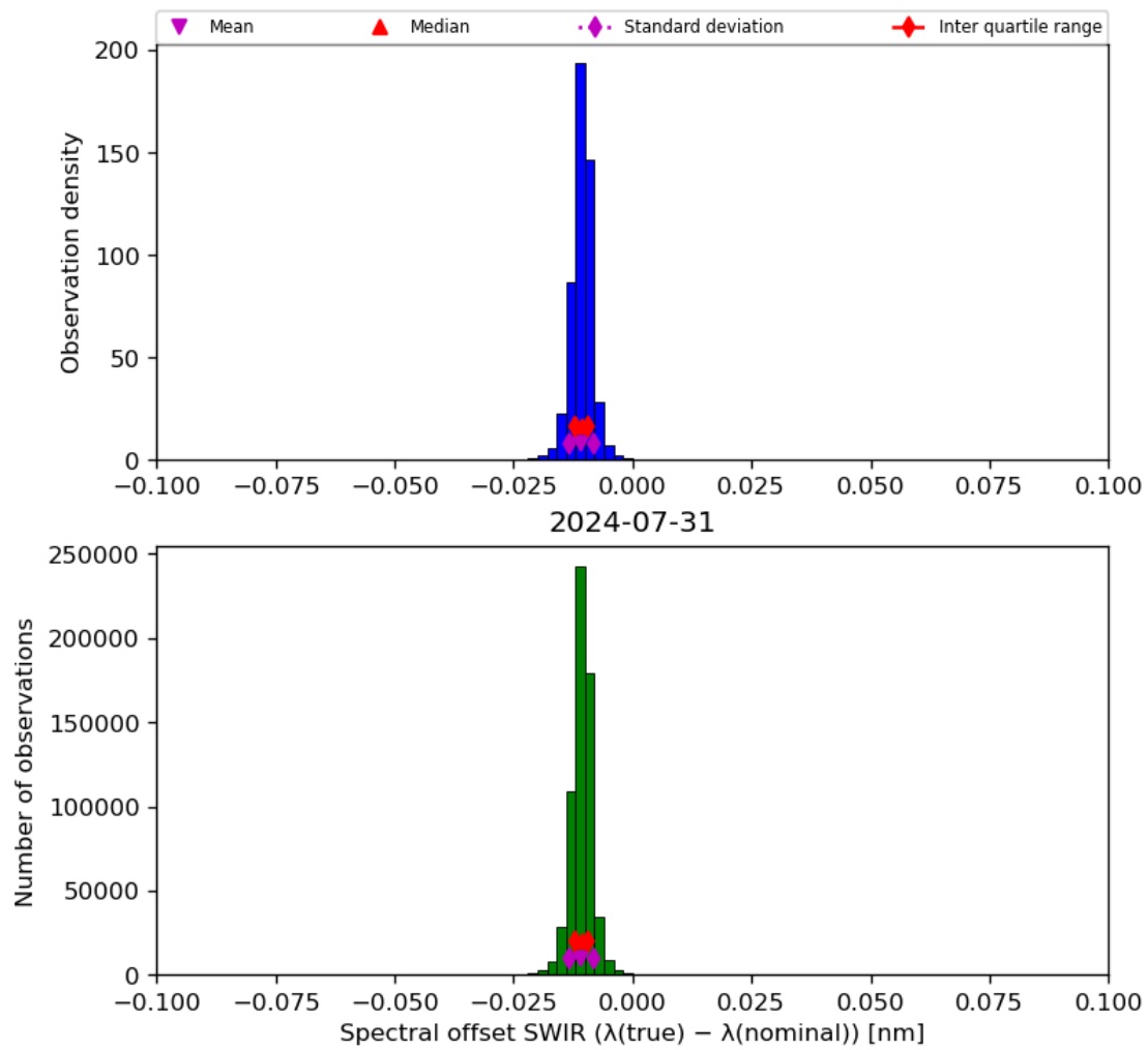
Figure 27: Histogram of “Spectral offset SWIR ( \lambda(\text{true}) - \lambda(\text{nominal}) )” for 2024-07-31 to 2024-08-01
