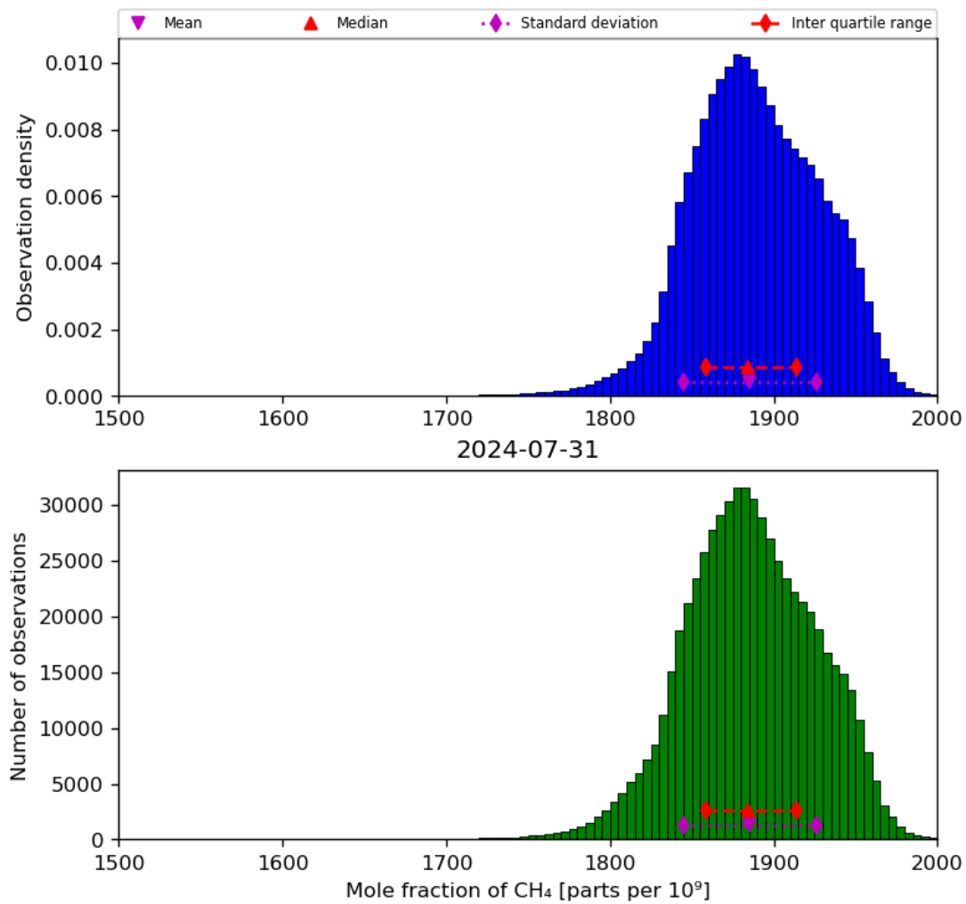
Figure 23: Histogram of “Mole fraction of CH 4 ” for 2024-07-31 to 2024-08-01
