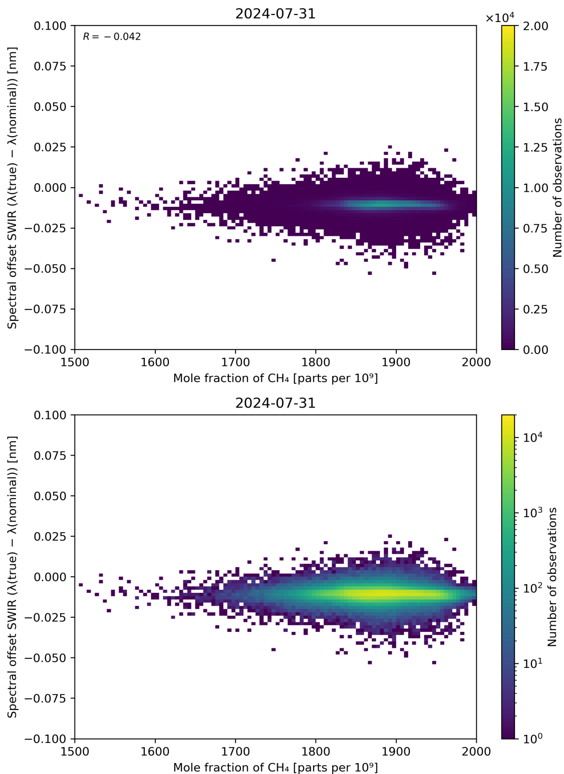
Figure 86: Scatter density plot of “Mole fraction of CH 4 ” against “Spectral offset SWIR ( \lambda(\text{true}) - \lambda(\text{nominal}) )” for 2024-07-31 to 2024-08-01.
