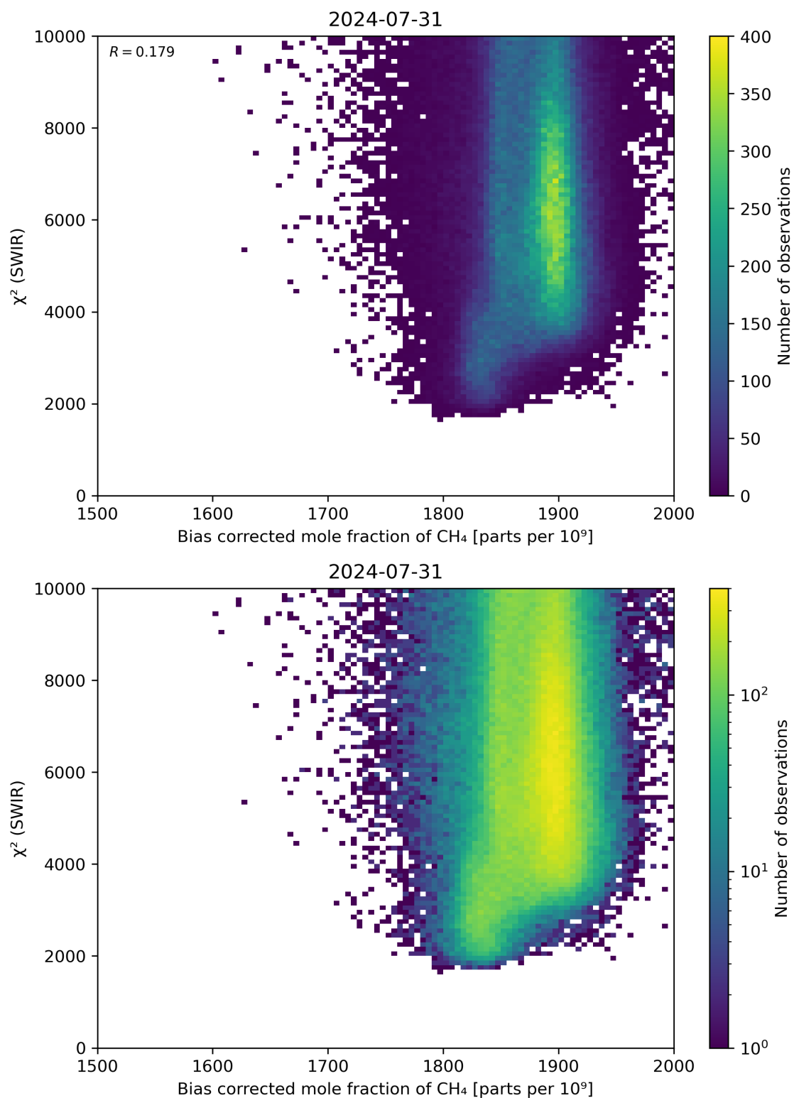
Figure 64: Scatter density plot of “Bias corrected mole fraction of \text{CH}_4 ” against “ \chi^2 (SWIR)” for 2024-07-31 to 2024-08-01.
