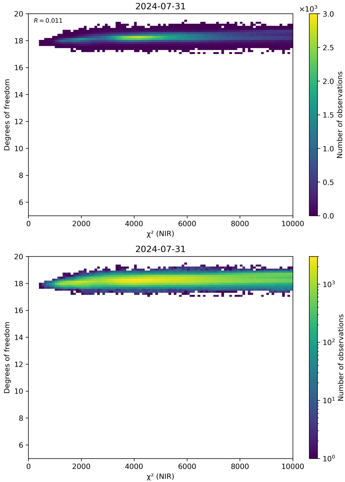
Figure 44: Scatter density plot of “ \chi^2 (NIR)” against “Degrees of freedom” for 2024-07-31 to 2024-08-01.
