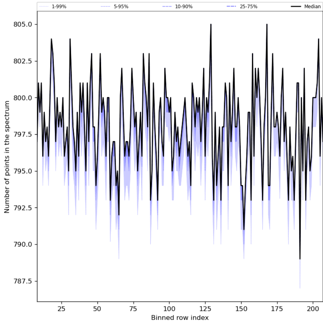
Figure 37: Along track statistics of “Number of points in the spectrum” for 2024-07-31 to 2024-08-01
