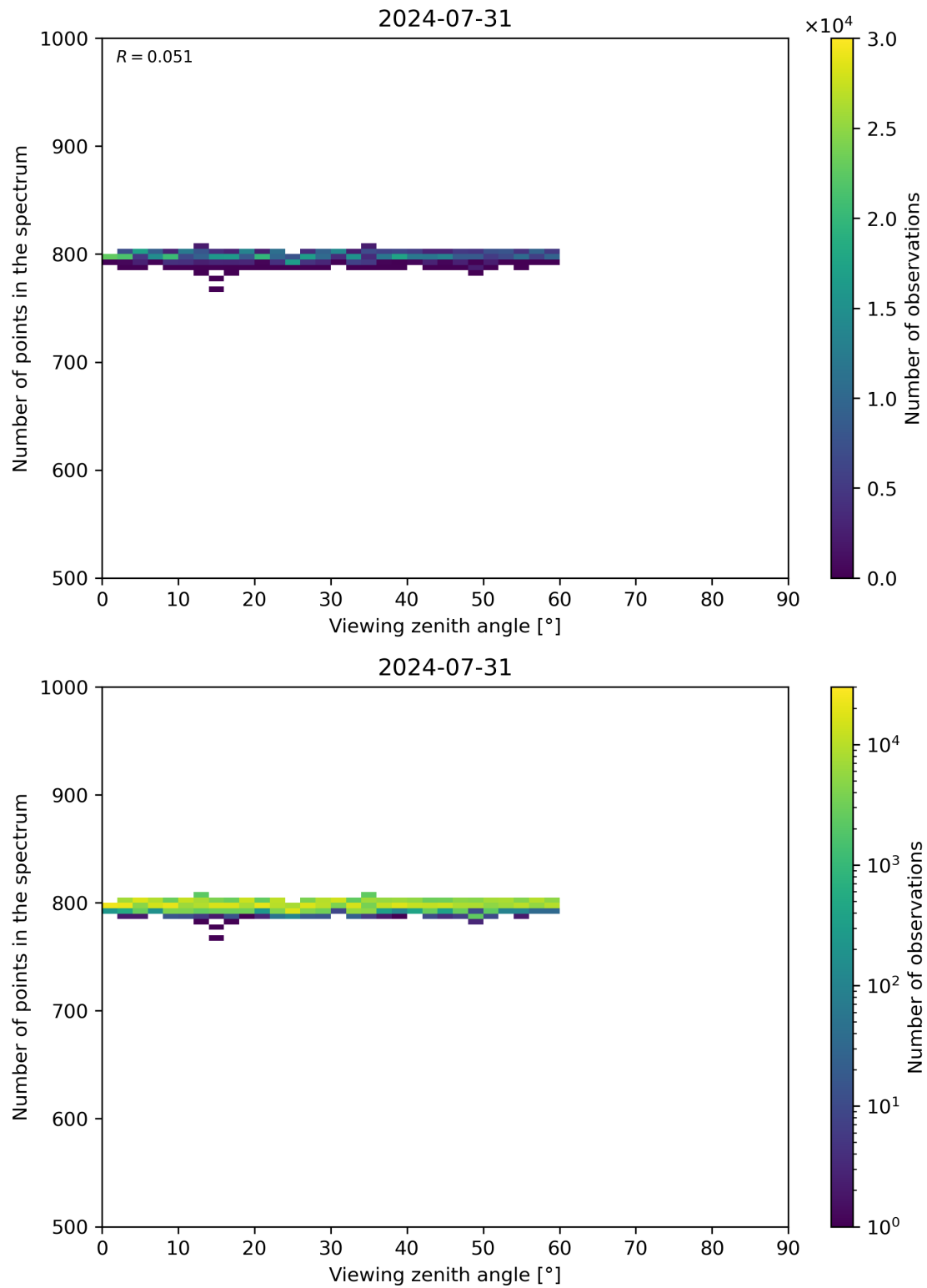
Figure 114: Scatter density plot of “Viewing zenith angle” against “Number of points in the spectrum” for 2024-07-31 to 2024-08-01.
