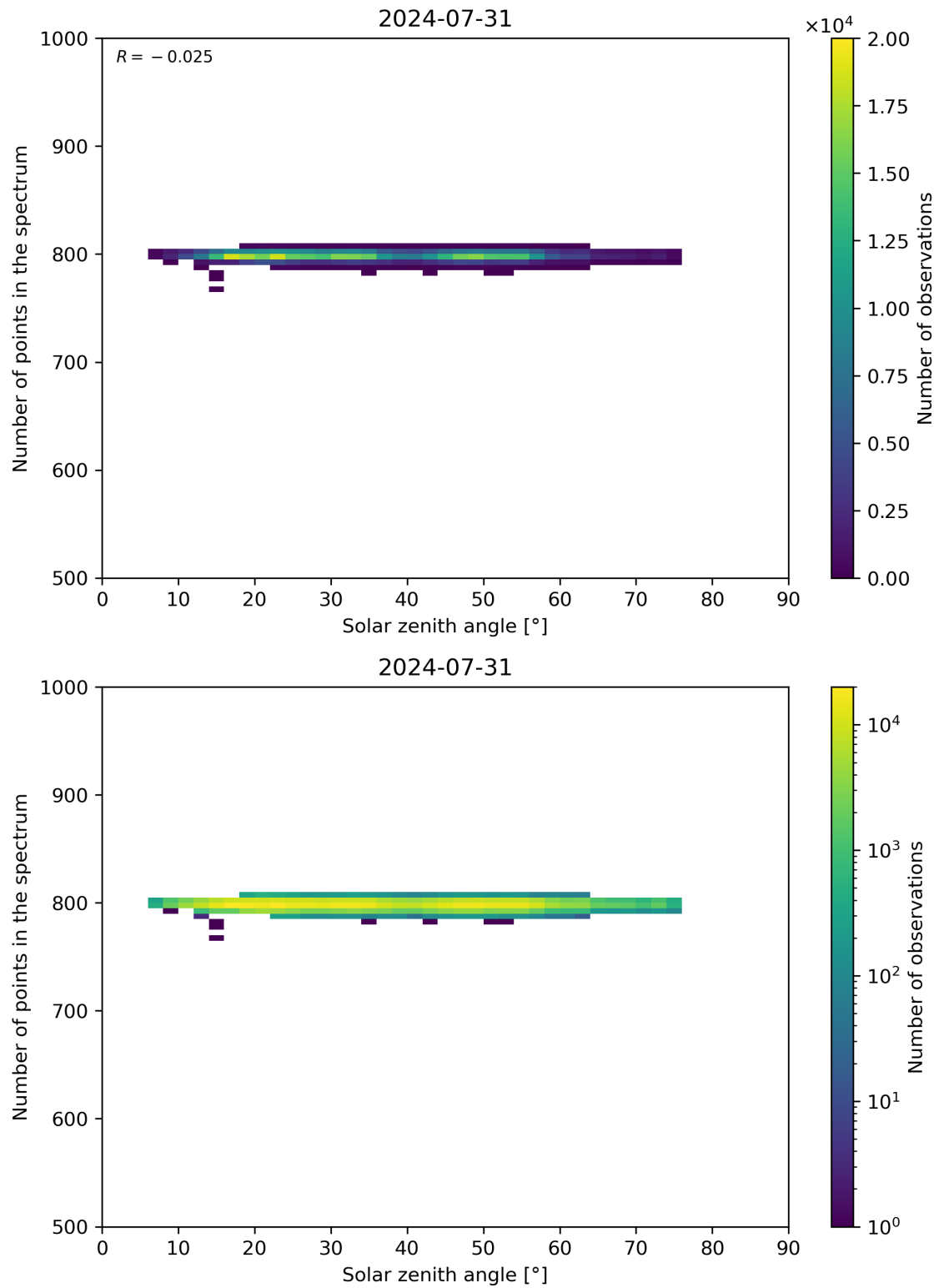
Figure 103: Scatter density plot of “Solar zenith angle” against “Number of points in the spectrum” for 2024-07-31 to 2024-08-01.
