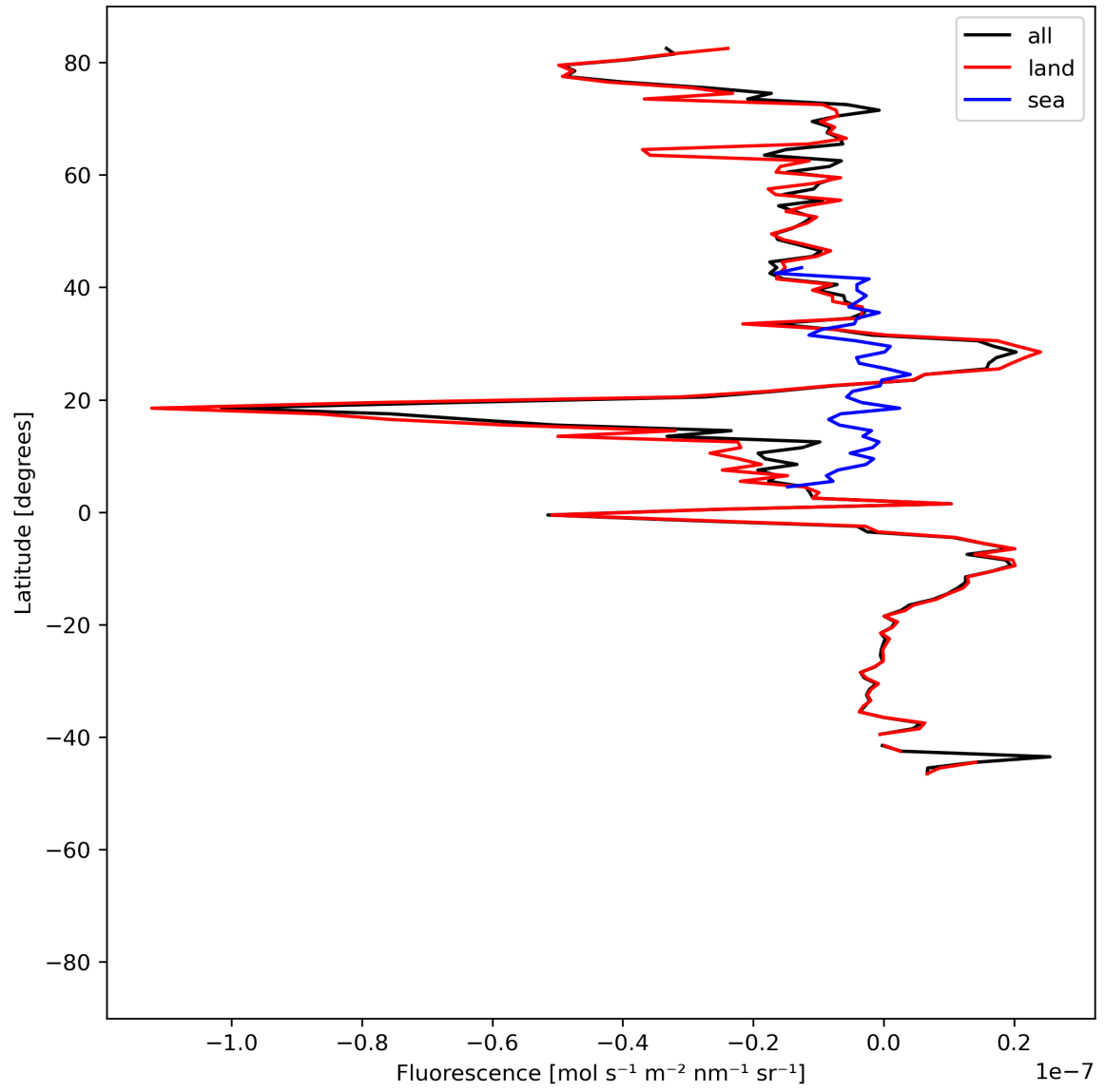
Figure 21: Zonal average of “Fluorescence” for 2024-07-31 to 2024-08-01.
