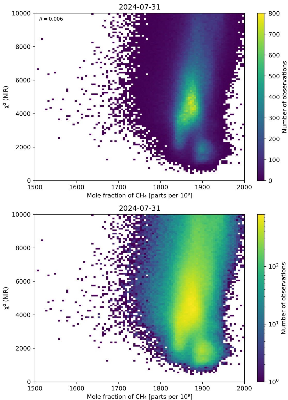
Figure 70: Scatter density plot of “Mole fraction of \text{CH}_4 ” against “ \chi^2 (NIR)” for 2024-07-31 to 2024-08-01.
