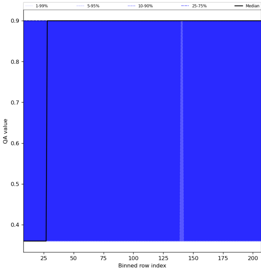
Figure 33: Along track statistics of “QA value” for 2024-07-31 to 2024-08-01
