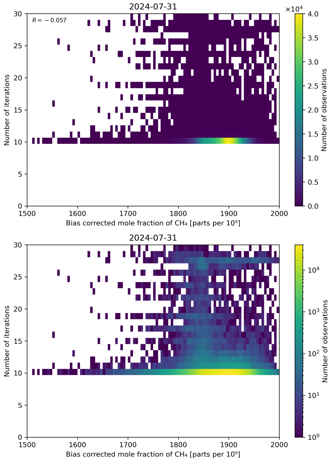
Figure 67: Scatter density plot of “Bias corrected mole fraction of CH 4 ” against “Number of iterations” for 2024-07-31 to 2024-08-01.
