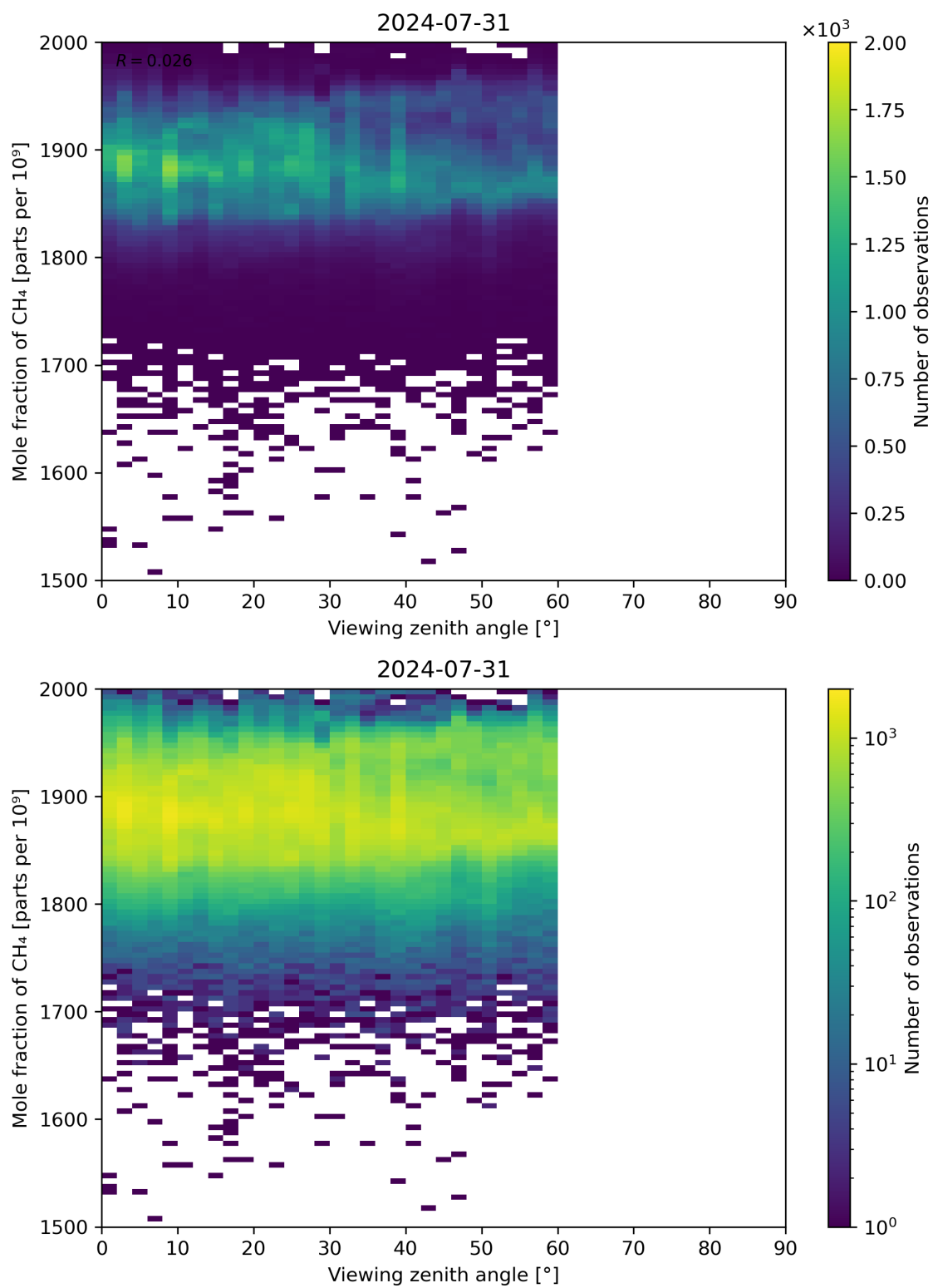
Figure 110: Scatter density plot of “Viewing zenith angle” against “Mole fraction of CH 4 ” for 2024-07-31 to 2024-08-01.
