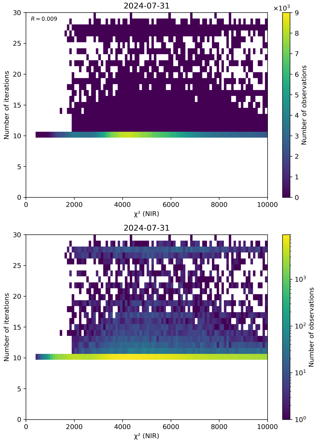
Figure 46: Scatter density plot of “ \chi^2 (NIR)” against “Number of iterations” for 2024-07-31 to 2024-08-01.
