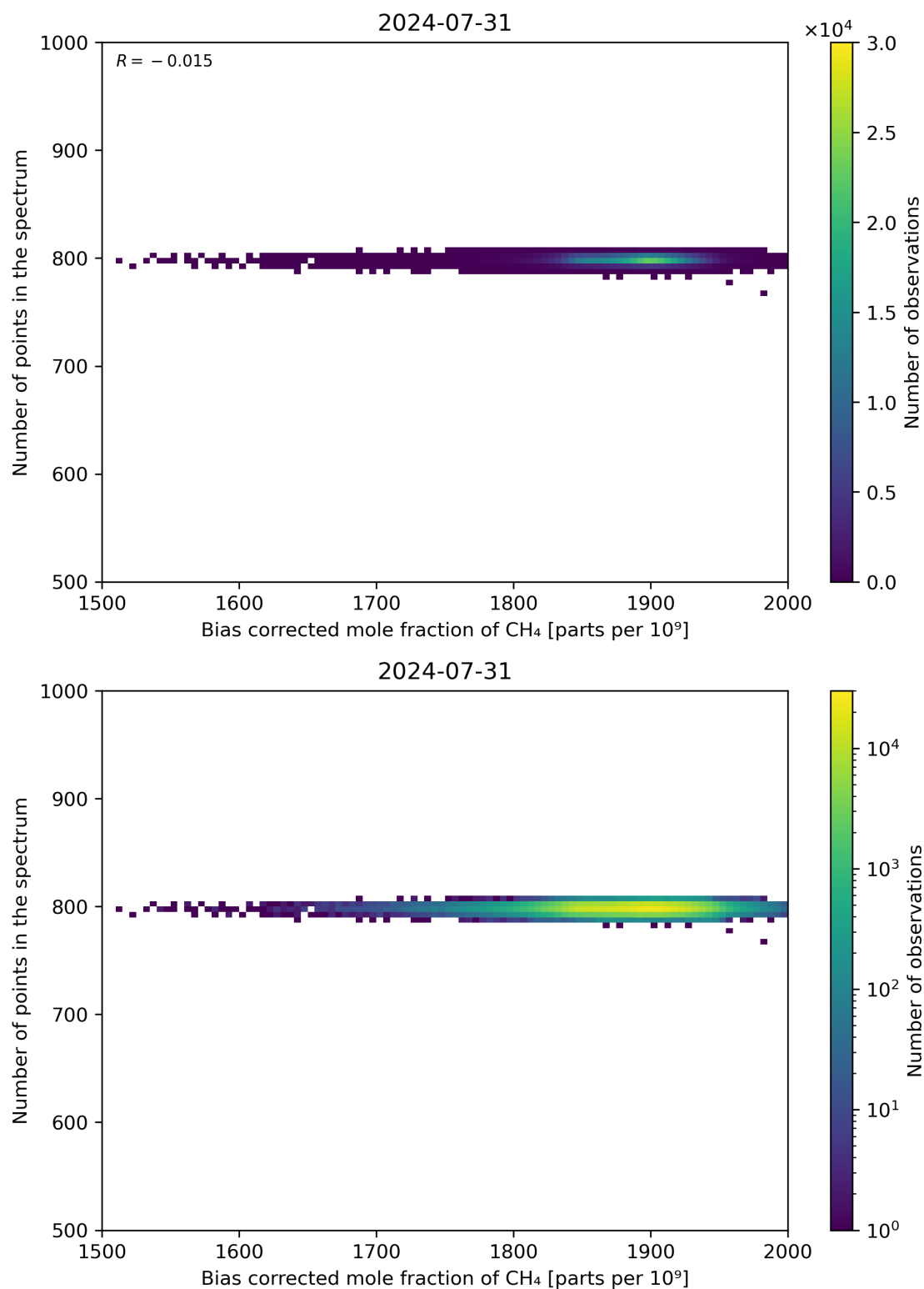
Figure 68: Scatter density plot of “Bias corrected mole fraction of CH 4 ” against “Number of points in the spectrum” for 2024-07-31 to 2024-08-01.
