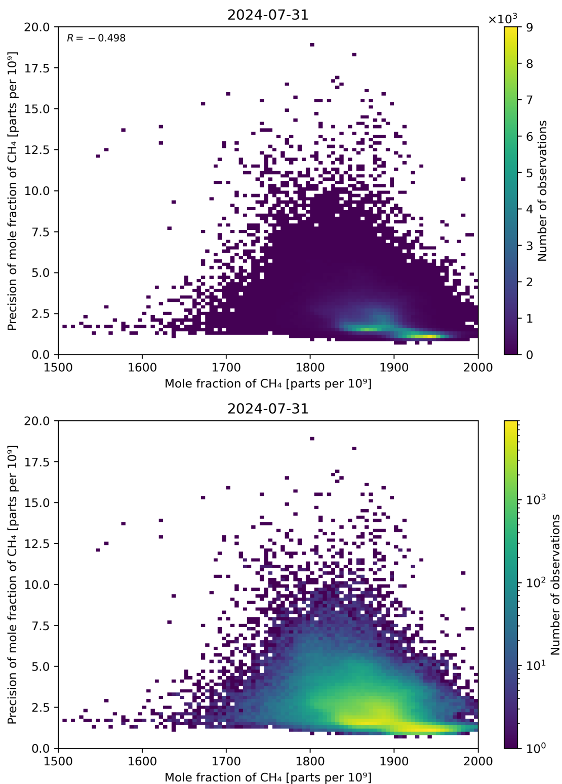
Figure 75: Scatter density plot of “Mole fraction of CH 4 ” against “Precision of mole fraction of CH 4 ” for 2024-07-31 to 2024-08-01.
