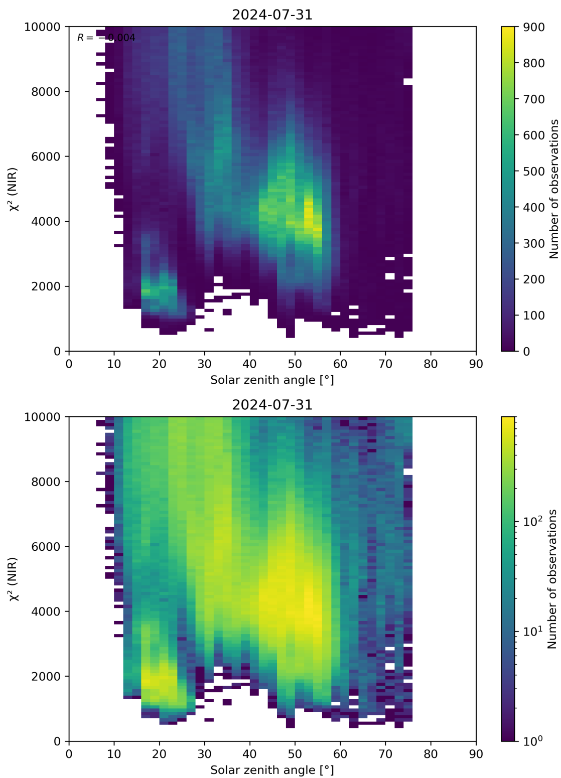
Figure 94: Scatter density plot of “Solar zenith angle” against “ \chi^2 (NIR)” for 2024-07-31 to 2024-08-01.
