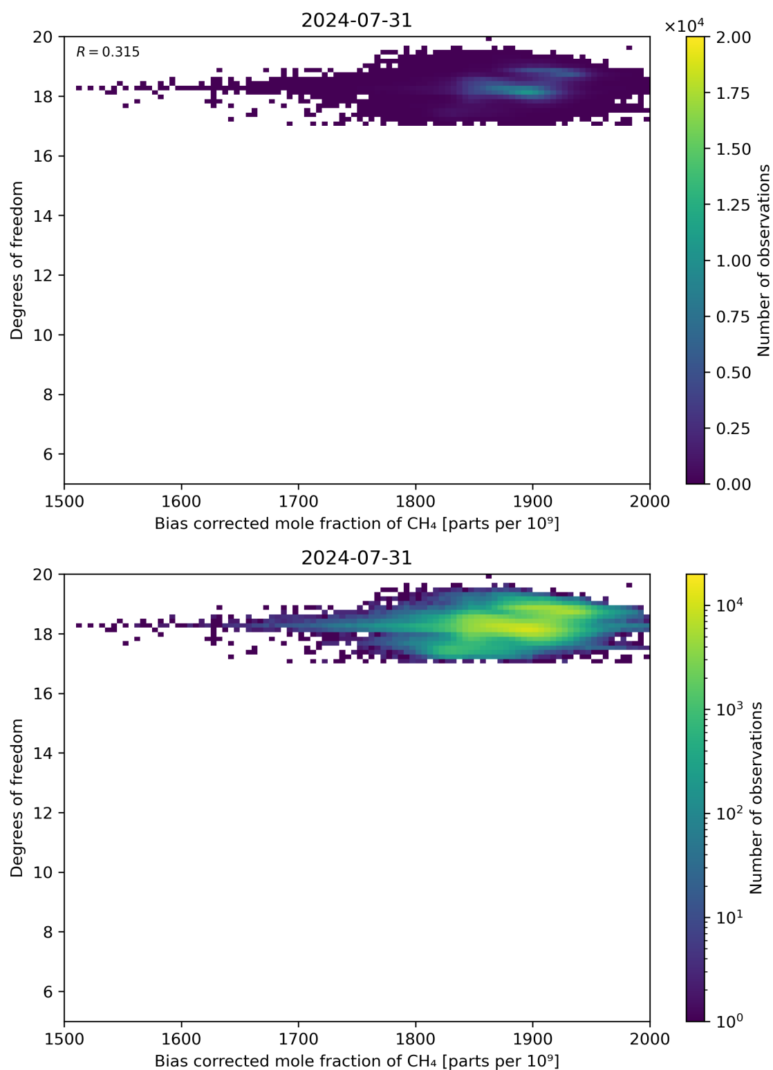
Figure 65: Scatter density plot of “Bias corrected mole fraction of CH 4 ” against “Degrees of freedom” for 2024-07-31 to 2024-08-01.
