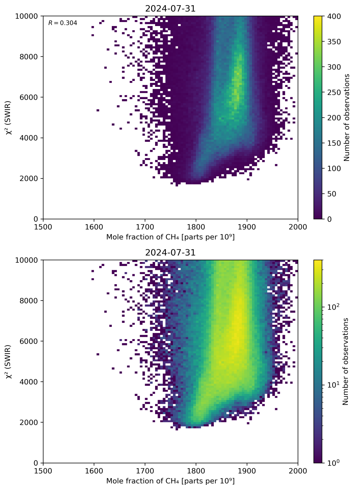
Figure 71: Scatter density plot of “Mole fraction of \text{CH}_4 ” against “ \chi^2 (SWIR)” for 2024-07-31 to 2024-08-01.
