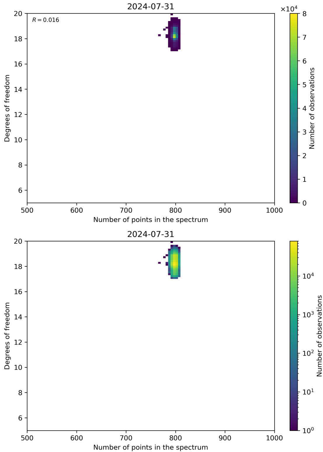
Figure 90: Scatter density plot of “Number of points in the spectrum” against “Degrees of freedom” for 2024-07-31 to 2024-08-01.
