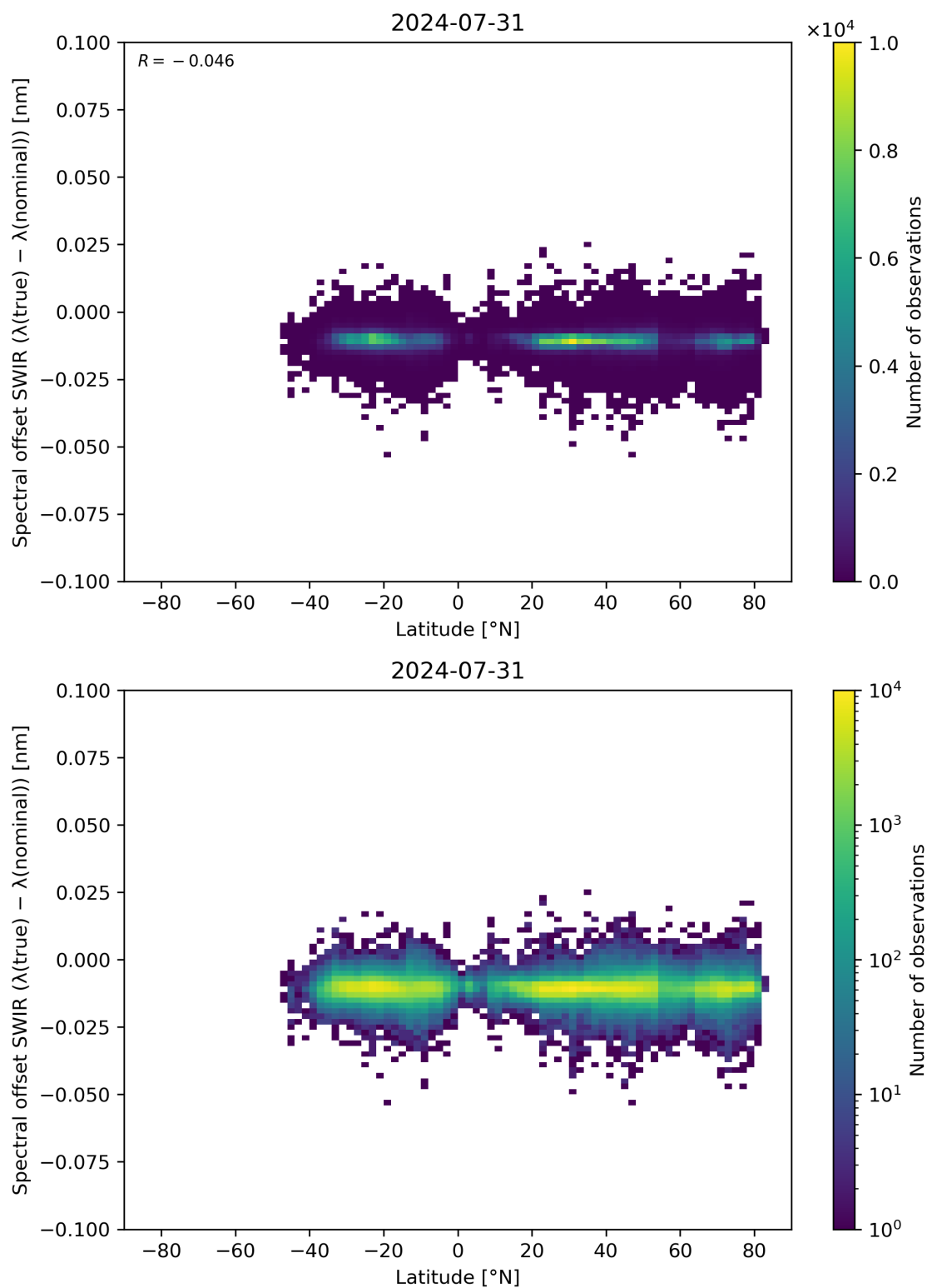
Figure 62: Scatter density plot of “Latitude” against “Spectral offset SWIR ( \lambda(\text{true}) - \lambda(\text{nominal}) )” for 2024-07-31 to 2024-08-01.
