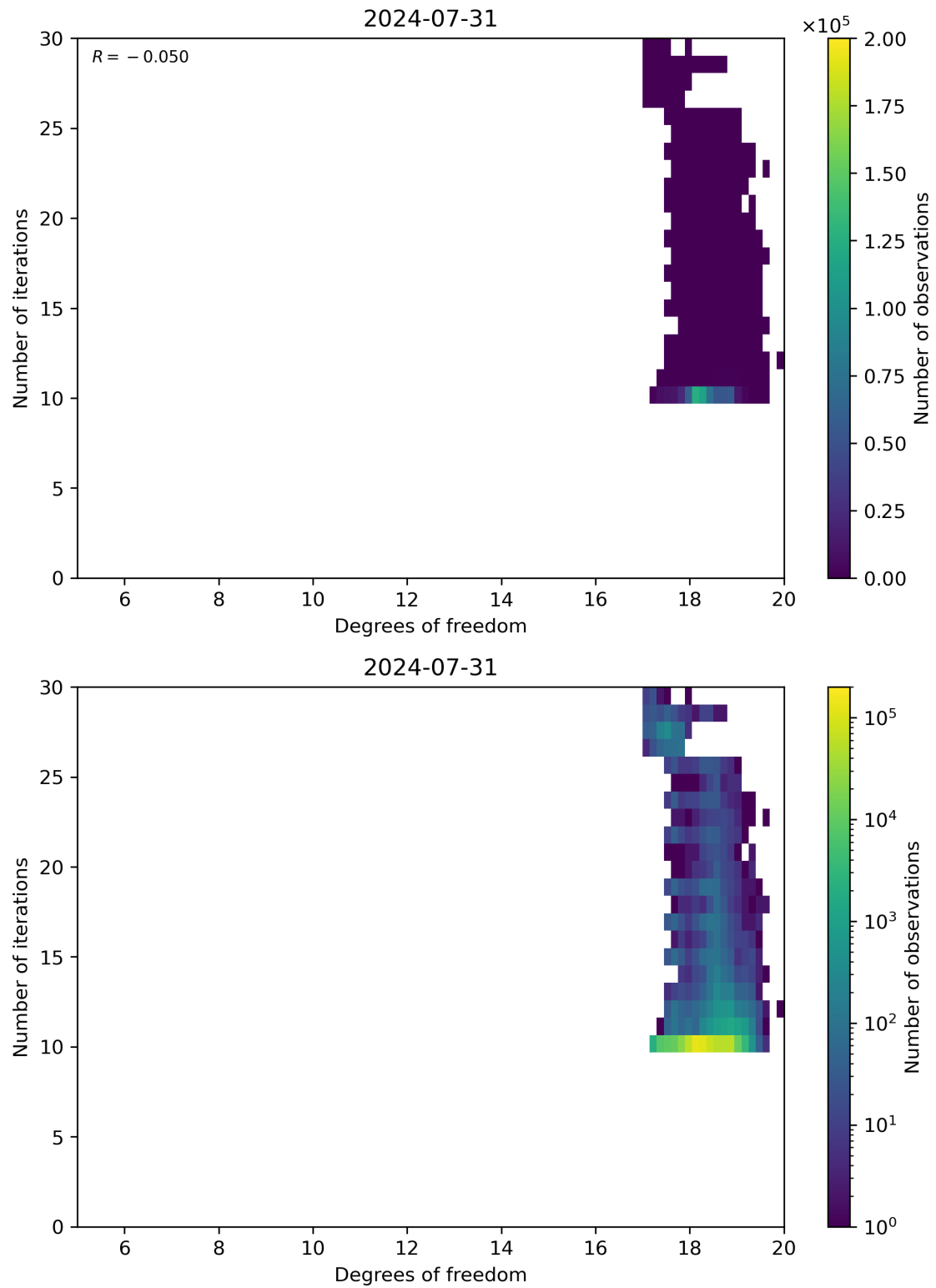
Figure 52: Scatter density plot of “Degrees of freedom” against “Number of iterations” for 2024-07-31 to 2024-08-01.
