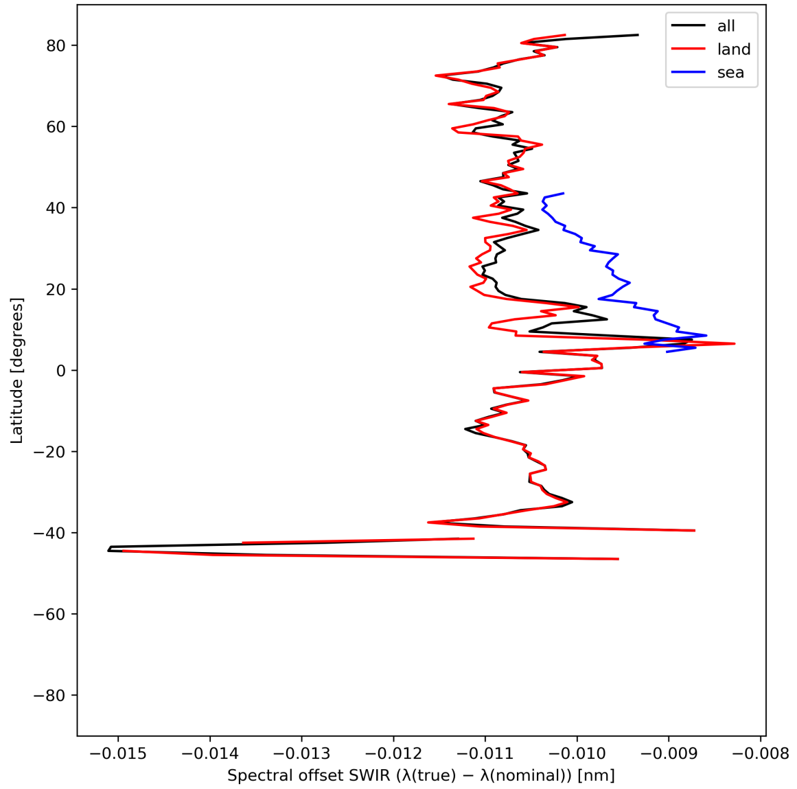
Figure 16: Zonal average of “Spectral offset SWIR ( \lambda(\text{true}) - \lambda(\text{nominal}) )” for 2024-07-31 to 2024-08-01.
