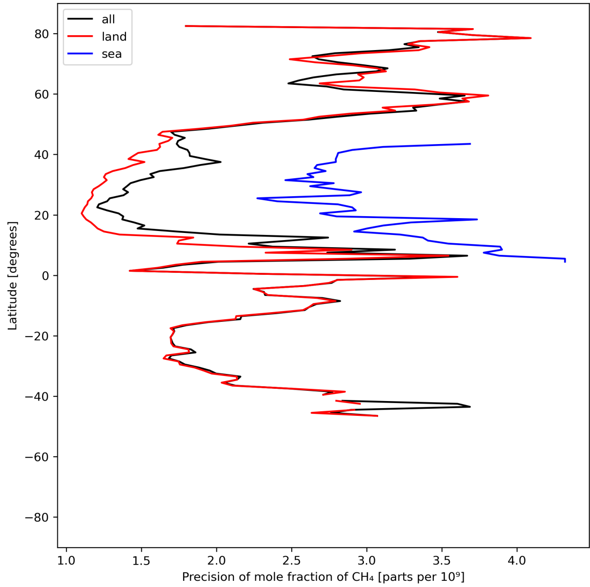
Figure 13: Zonal average of “Precision of mole fraction of CH 4 ” for 2024-07-31 to 2024-08-01.
