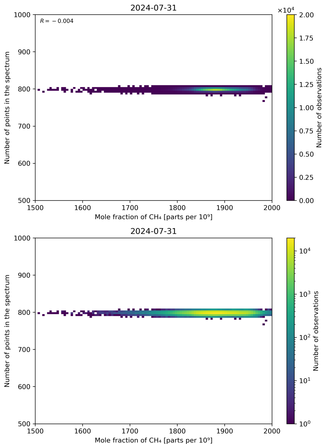
Figure 77: Scatter density plot of “Mole fraction of CH 4 ” against “Number of points in the spectrum” for 2024-07-31 to 2024-08-01.
