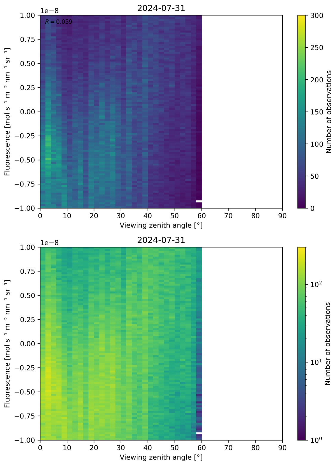
Figure 108: Scatter density plot of “Viewing zenith angle” against “Fluorescence” for 2024-07-31 to 2024-08-01.
