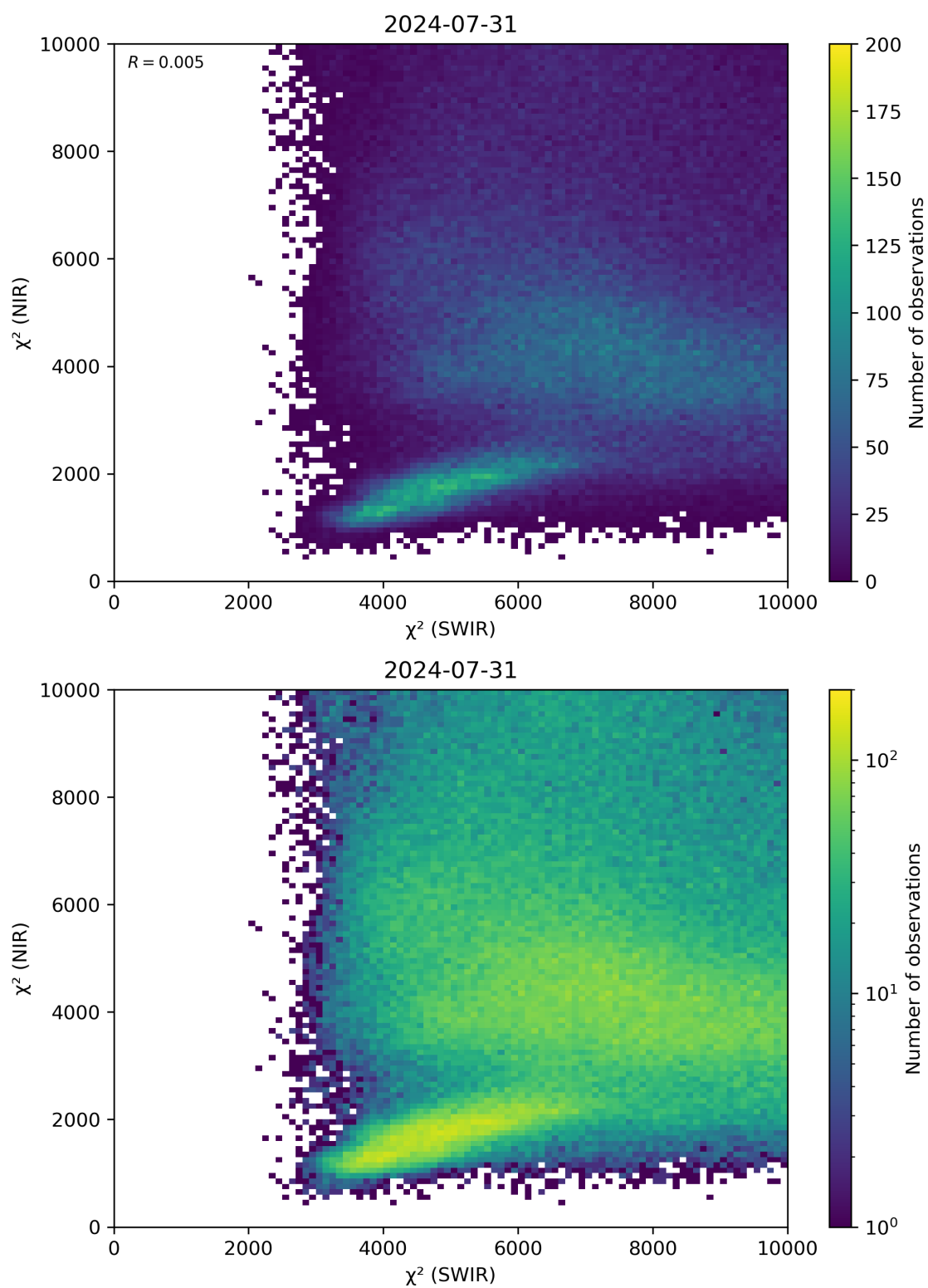
Figure 47: Scatter density plot of “ \chi^2 (SWIR)” against “ \chi^2 (NIR)” for 2024-07-31 to 2024-08-01.
