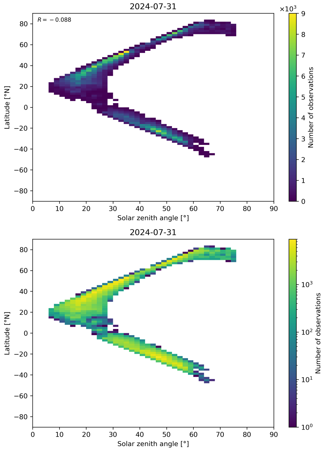
Figure 98: Scatter density plot of “Solar zenith angle” against “Latitude” for 2024-07-31 to 2024-08-01.
