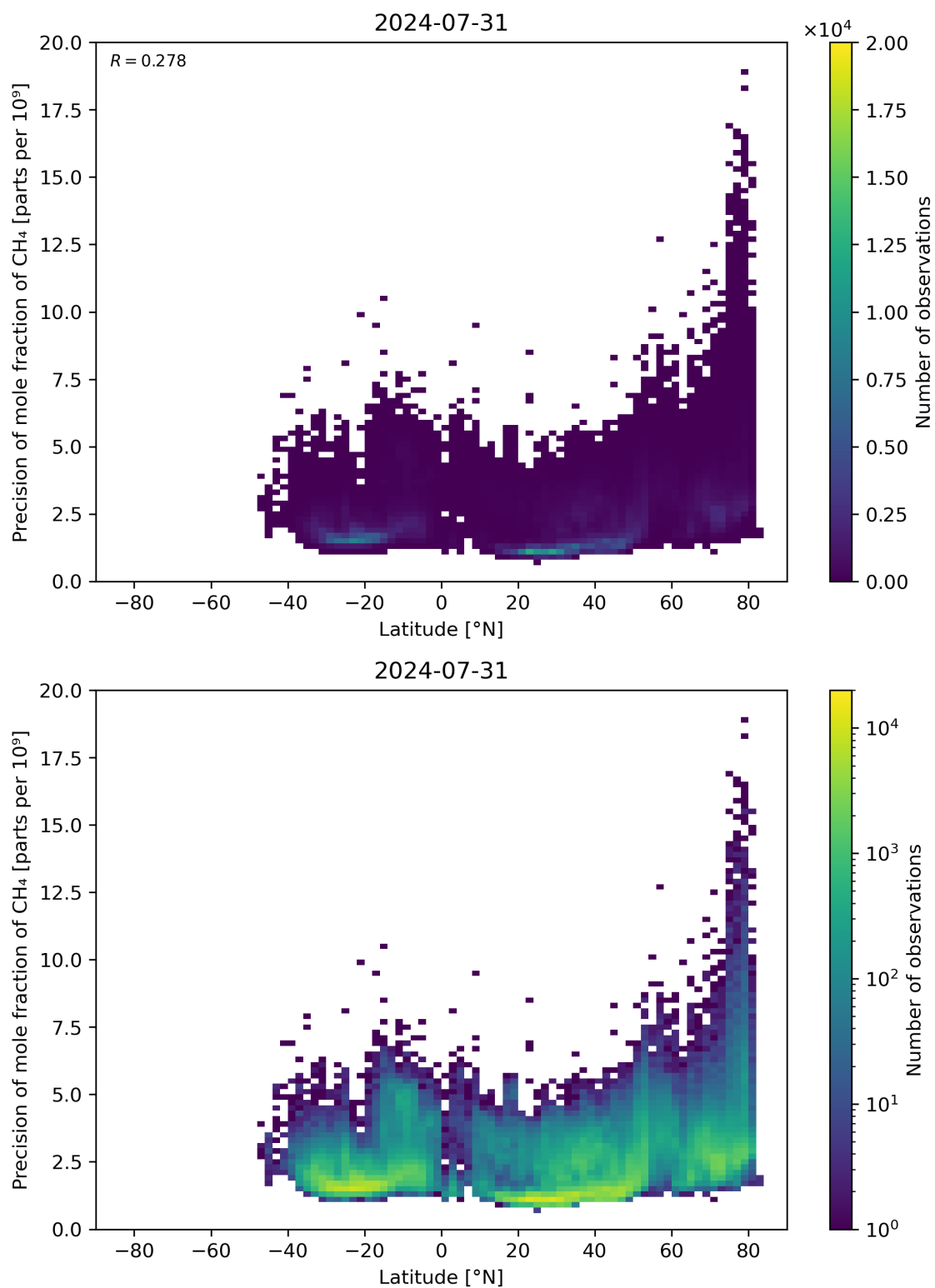
Figure 59: Scatter density plot of “Latitude” against “Precision of mole fraction of \text{CH}_4 ” for 2024-07-31 to 2024-08-01.
