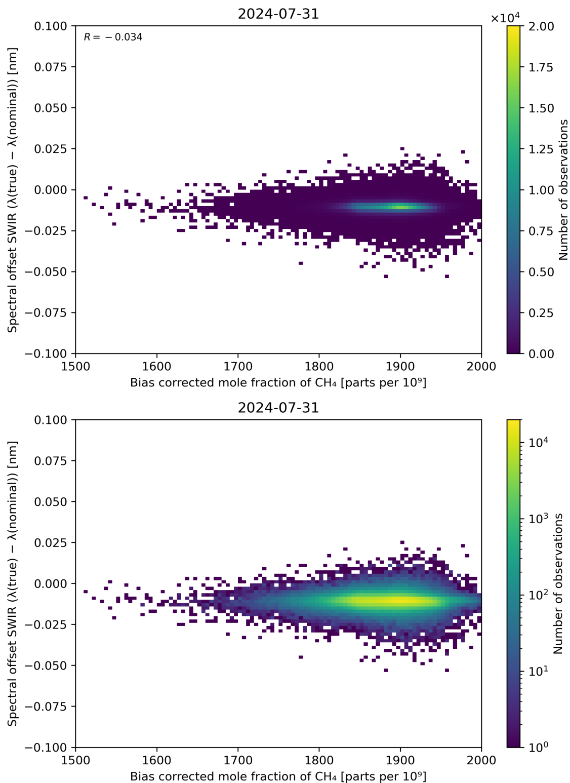
Figure 69: Scatter density plot of “Bias corrected mole fraction of \text{CH}_4 ” against “Spectral offset SWIR ( \lambda(\text{true}) - \lambda(\text{nominal}) )” for 2024-07-31 to 2024-08-01.
