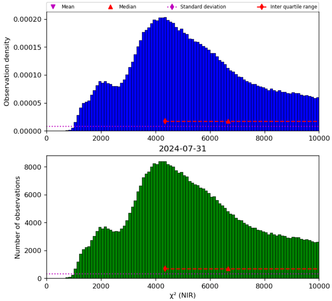
Figure 29: Histogram of " \chi^2 (NIR)" for 2024-07-31 to 2024-08-01
