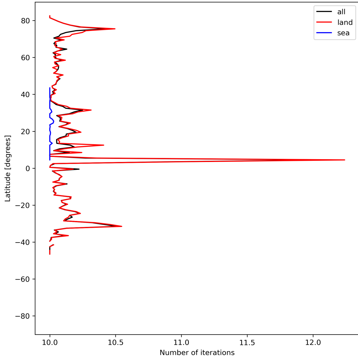
Figure 20: Zonal average of “Number of iterations” for 2024-07-31 to 2024-08-01.
