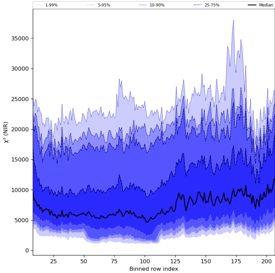
Figure 40: Along track statistics of “ \chi^2 (NIR)” for 2024-07-31 to 2024-08-01
