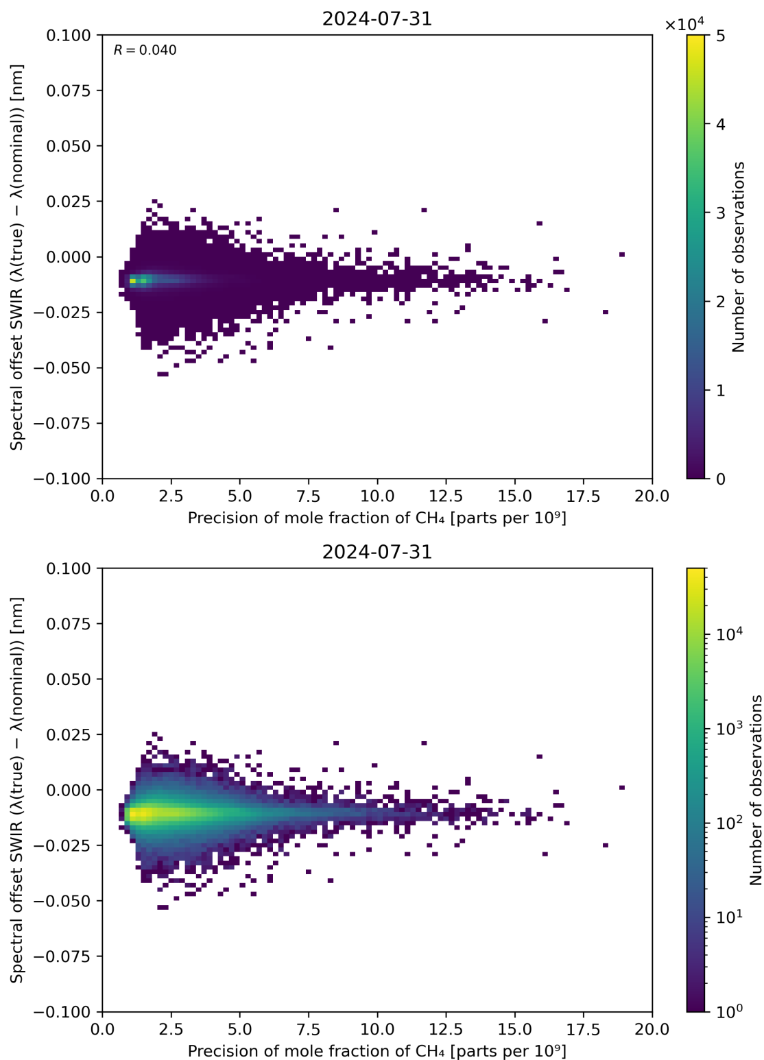
Figure 85: Scatter density plot of “Precision of mole fraction of CH 4 ” against “Spectral offset SWIR ( \lambda(\text{true}) - \lambda(\text{nominal}) )” for 2024-07-31 to 2024-08-01.
