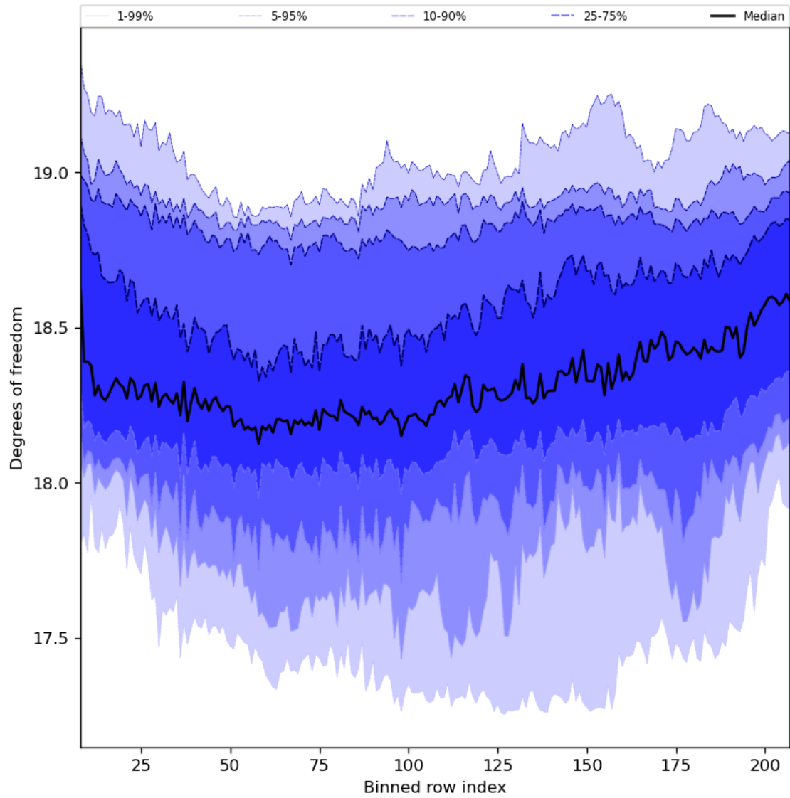
Figure 41: Along track statistics of “Degrees of freedom” for 2024-07-31 to 2024-08-01
