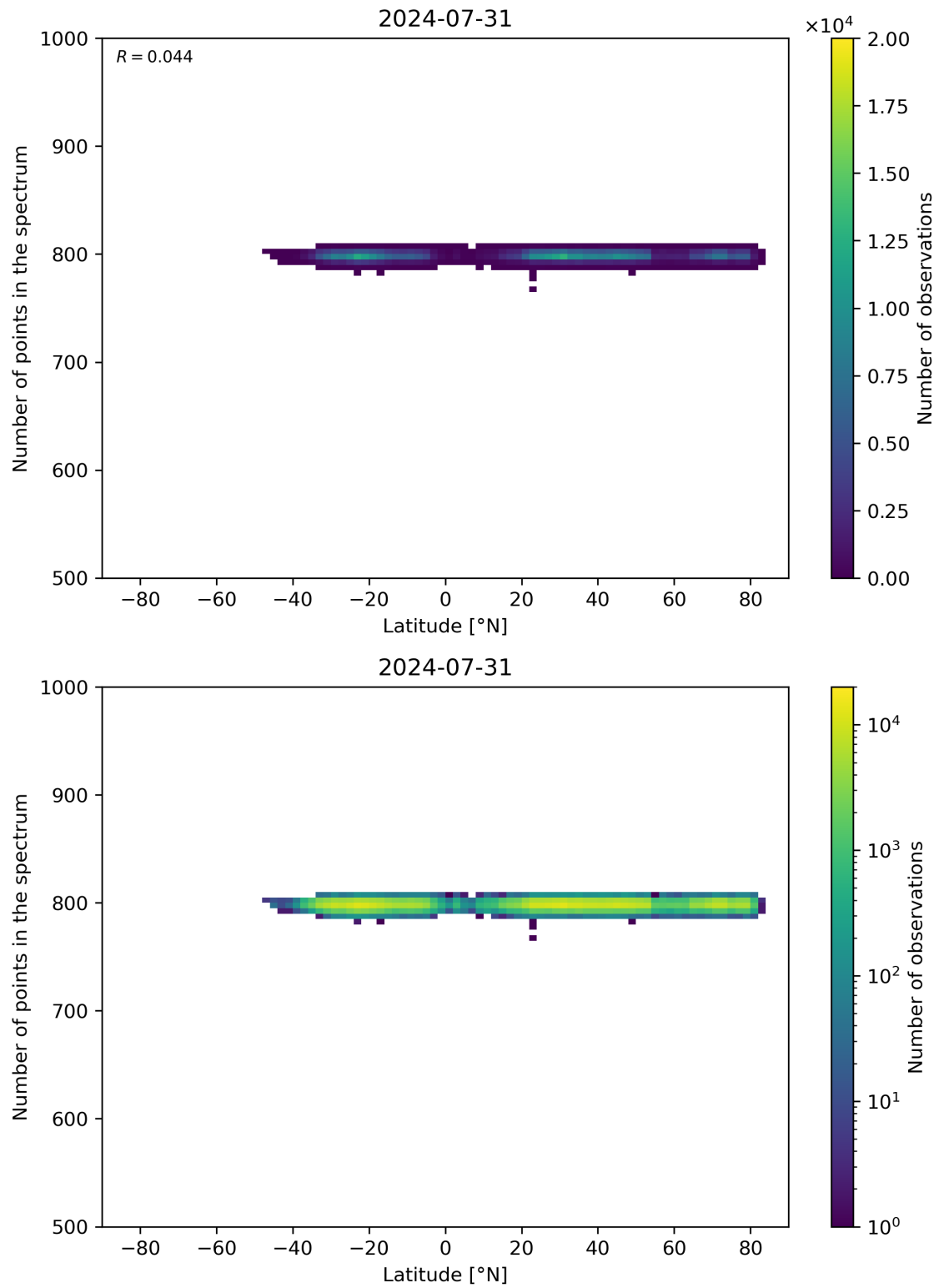
Figure 61: Scatter density plot of “Latitude” against “Number of points in the spectrum” for 2024-07-31 to 2024-08-01.
