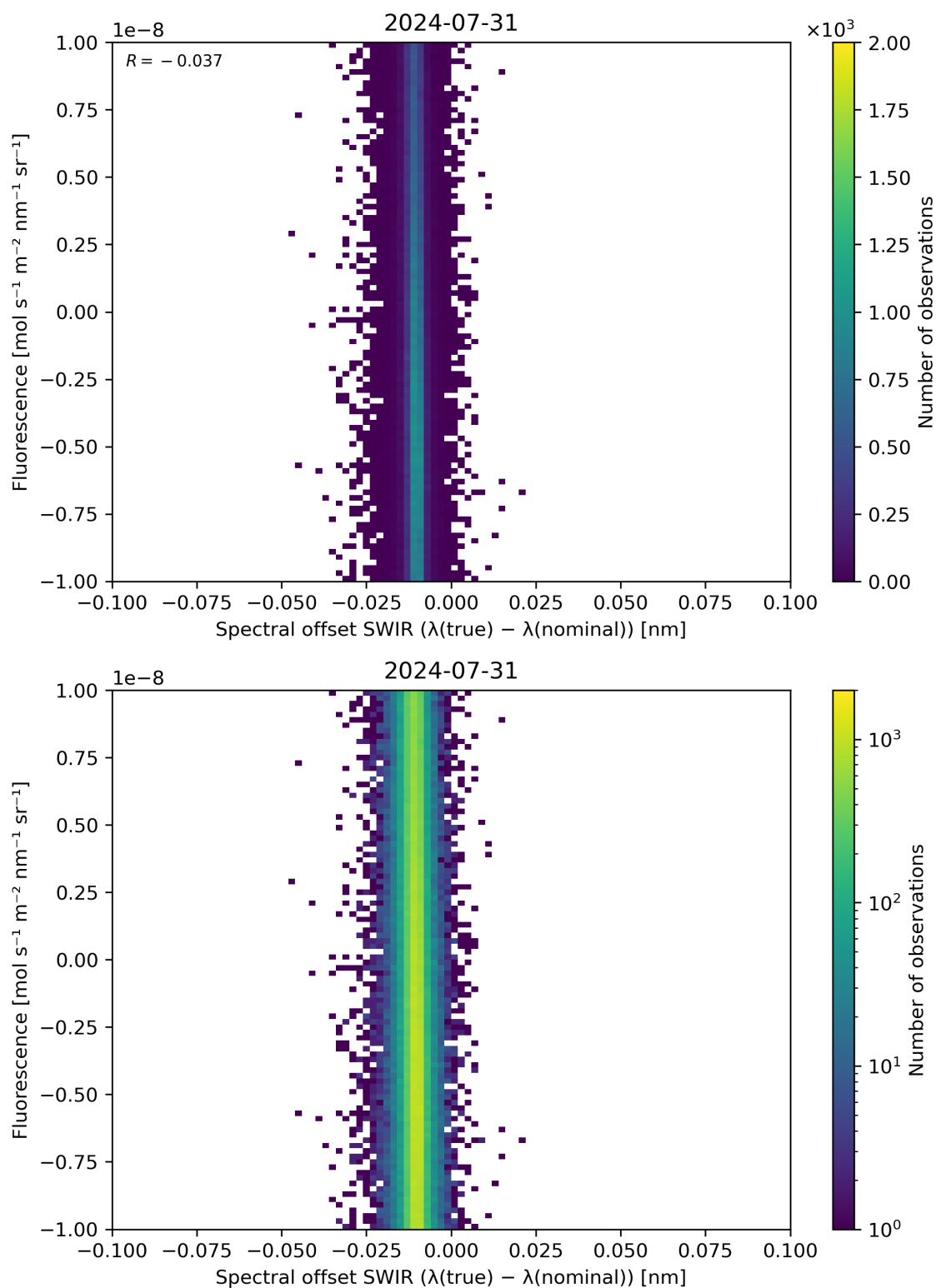
Figure 120: Scatter density plot of “Spectral offset SWIR ( \lambda(\text{true}) - \lambda(\text{nominal}) )” against “Fluorescence” for 2024-07-31 to 2024-08-01.
