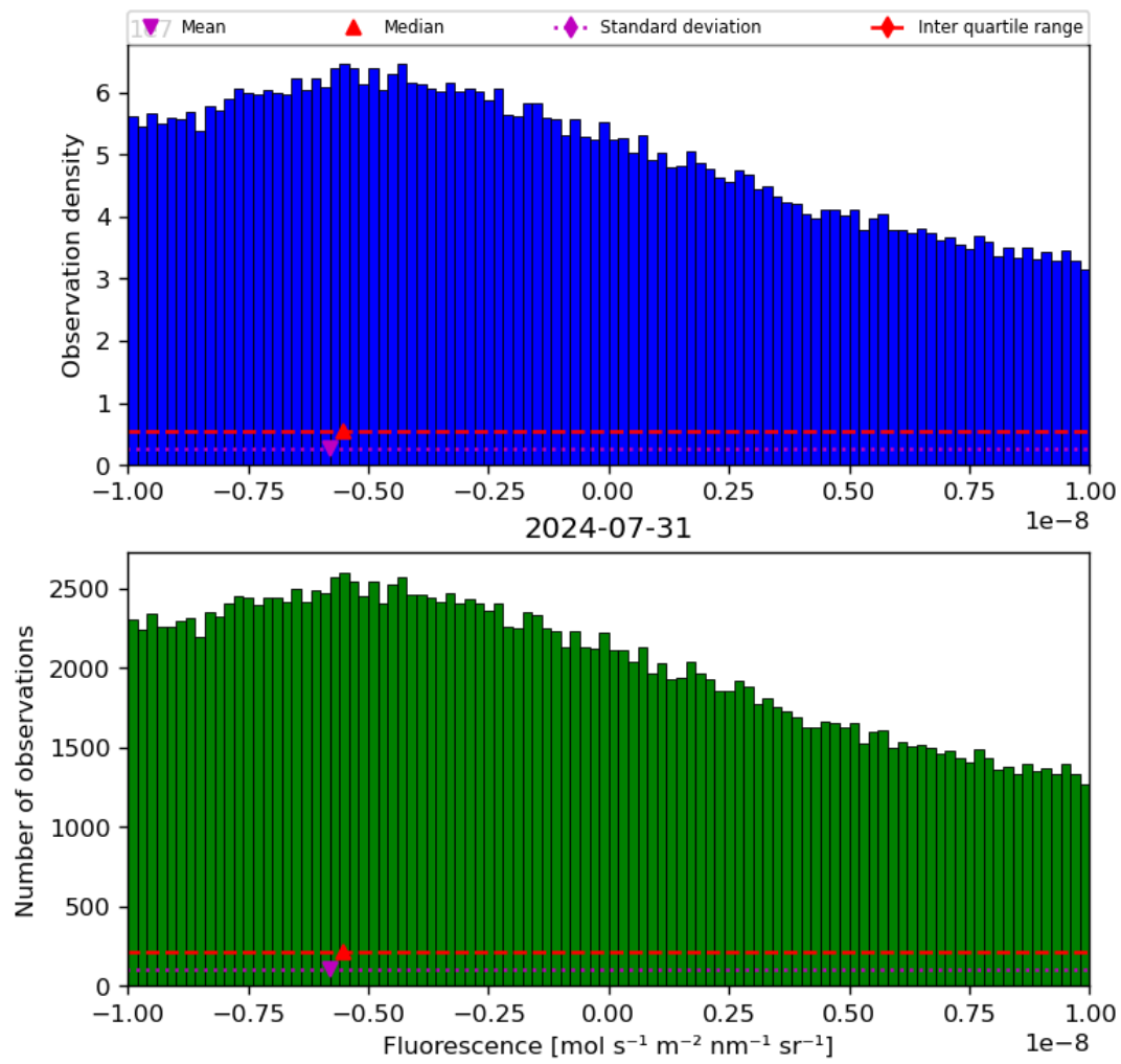
Figure 32: Histogram of “Fluorescence” for 2024-07-31 to 2024-08-01
