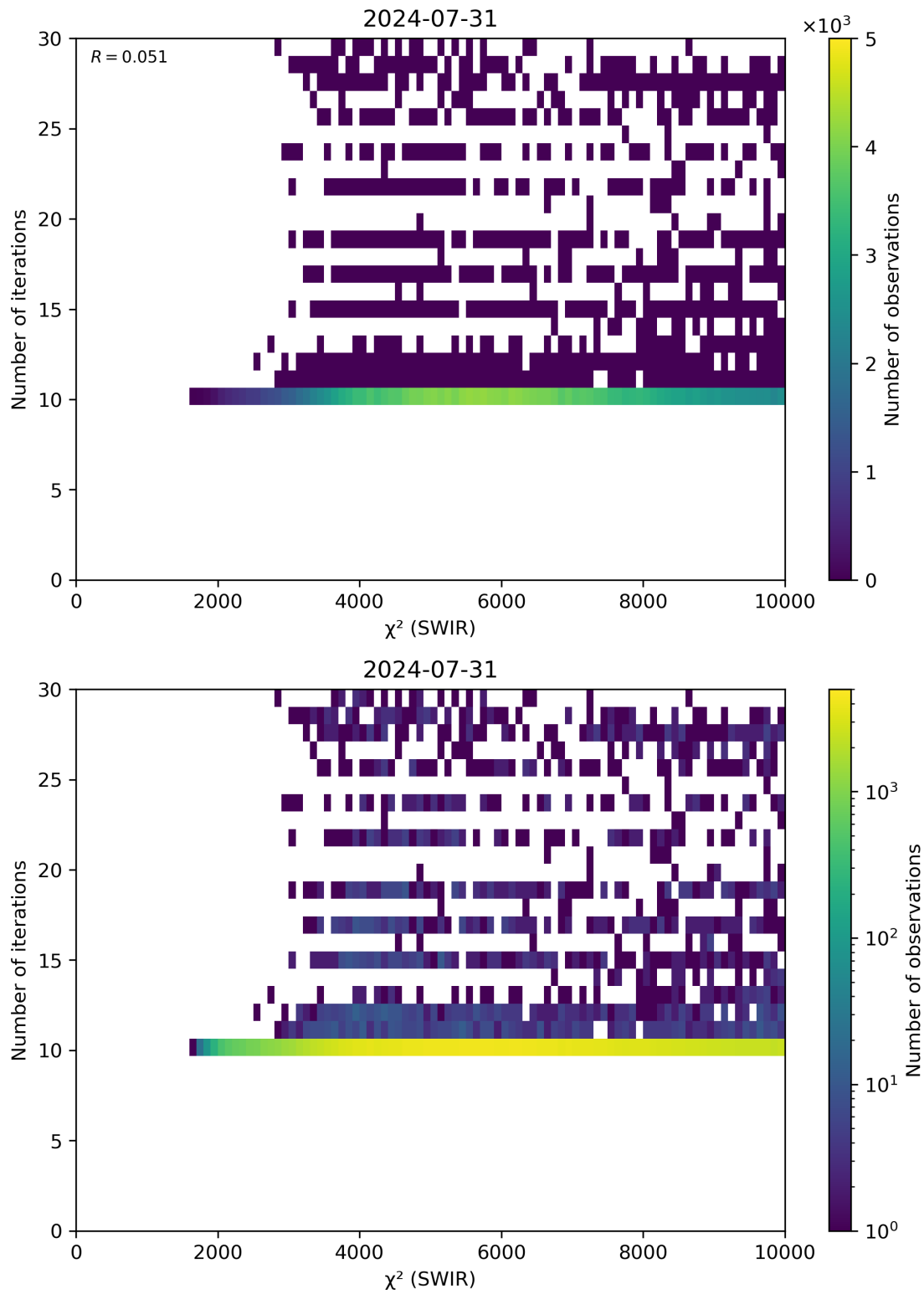
Figure 50: Scatter density plot of “ \chi^2 (SWIR)” against “Number of iterations” for 2024-07-31 to 2024-08-01.
