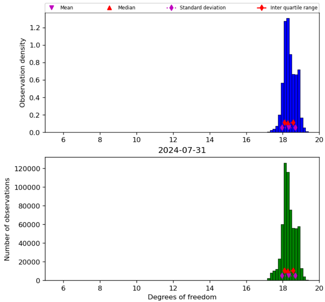
Figure 30: Histogram of “Degrees of freedom” for 2024-07-31 to 2024-08-01
