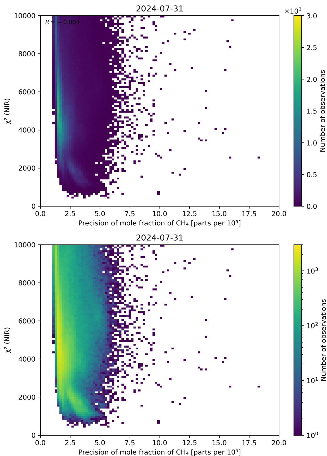
Figure 78: Scatter density plot of “Precision of mole fraction of \text{CH}_4 ” against “ \chi^2 (NIR)” for 2024-07-31 to 2024-08-01.
