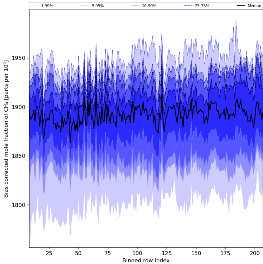
Figure 36: Along track statistics of “Bias corrected mole fraction of CH 4 ” for 2024-07-31 to 2024-08-01
