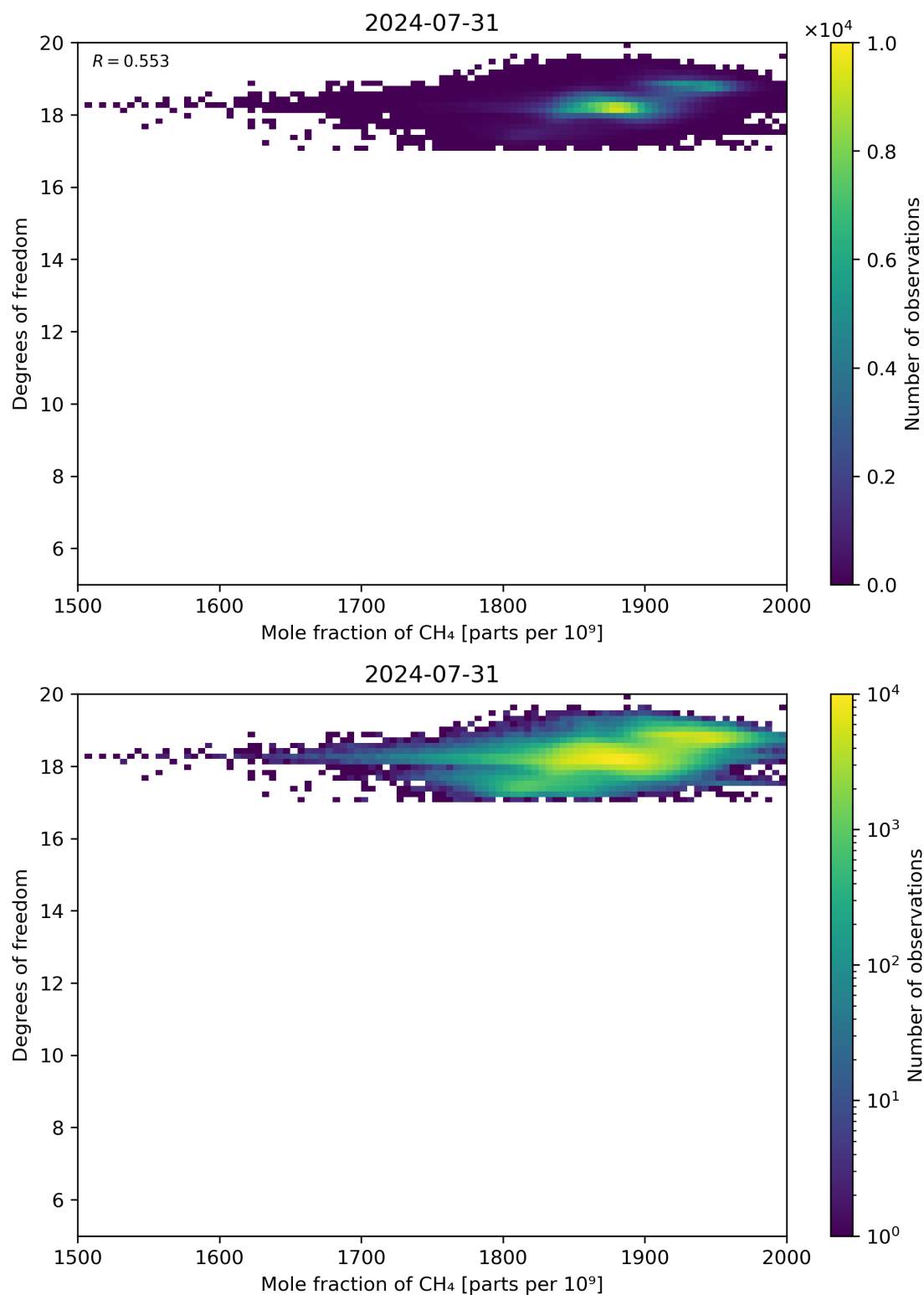
Figure 72: Scatter density plot of “Mole fraction of CH 4 ” against “Degrees of freedom” for 2024-07-31 to 2024-08-01.
