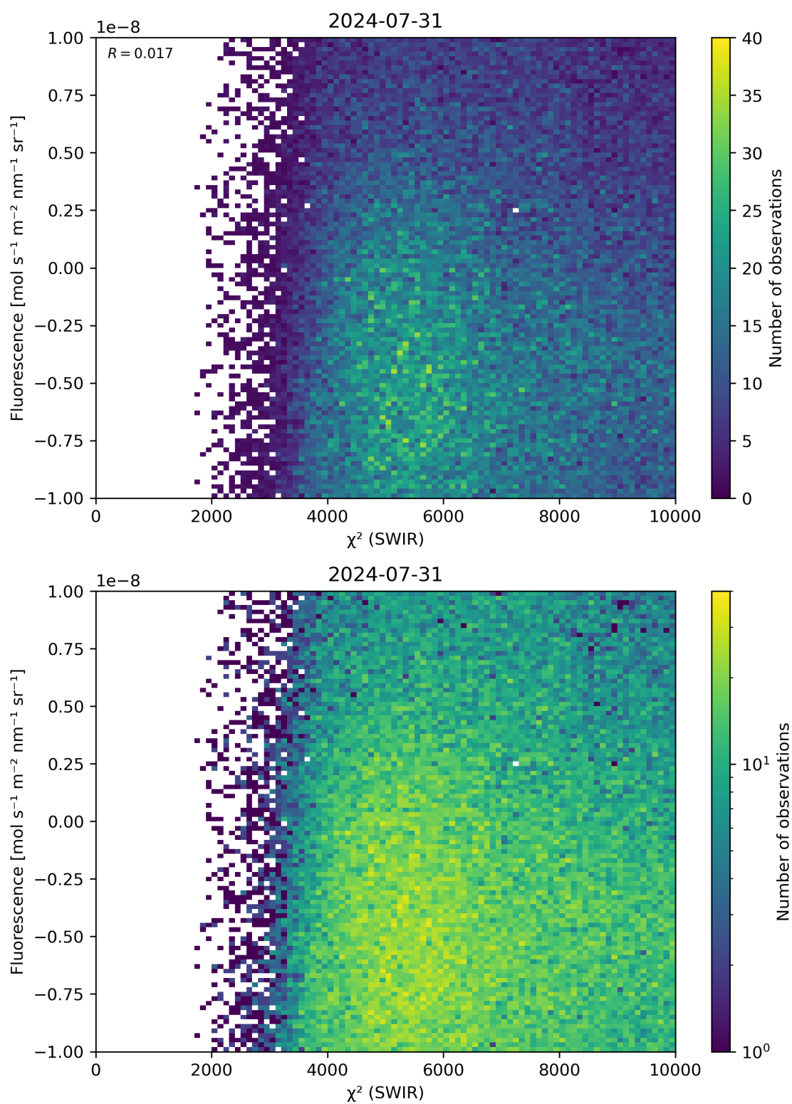
Figure 49: Scatter density plot of “ \chi^2 (SWIR)” against “Fluorescence” for 2024-07-31 to 2024-08-01.
