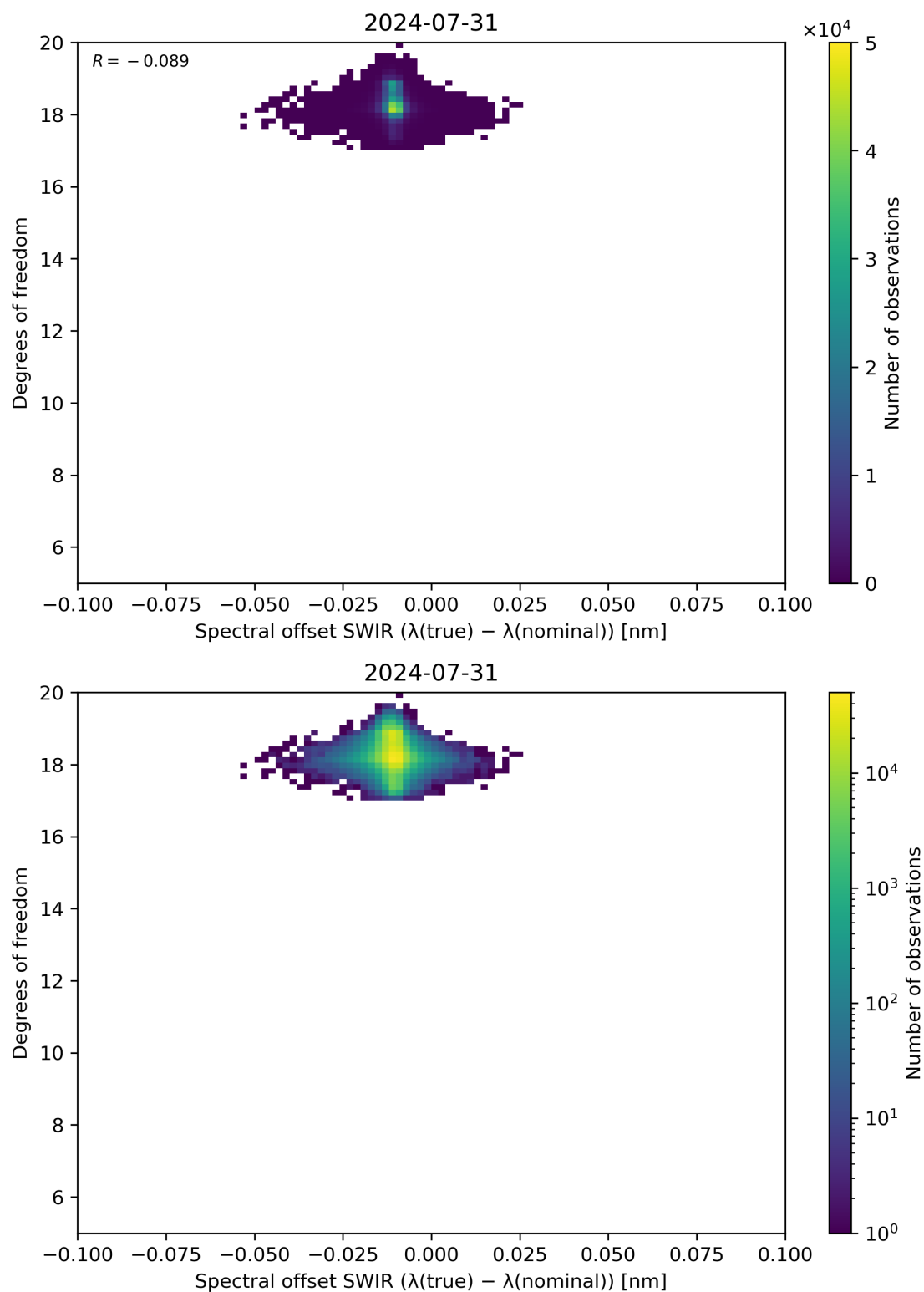
Figure 119: Scatter density plot of “Spectral offset SWIR ( \lambda(\text{true}) - \lambda(\text{nominal}) )” against “Degrees of freedom” for 2024-07-31 to 2024-08-01.
