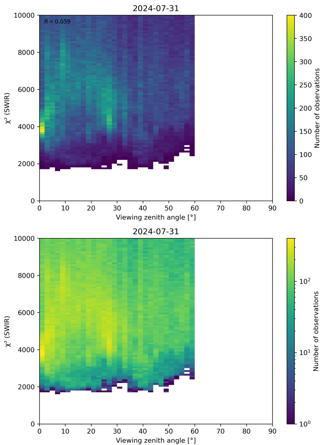
Figure 106: Scatter density plot of “Viewing zenith angle” against “ \chi^2 (SWIR)” for 2024-07-31 to 2024-08-01.
