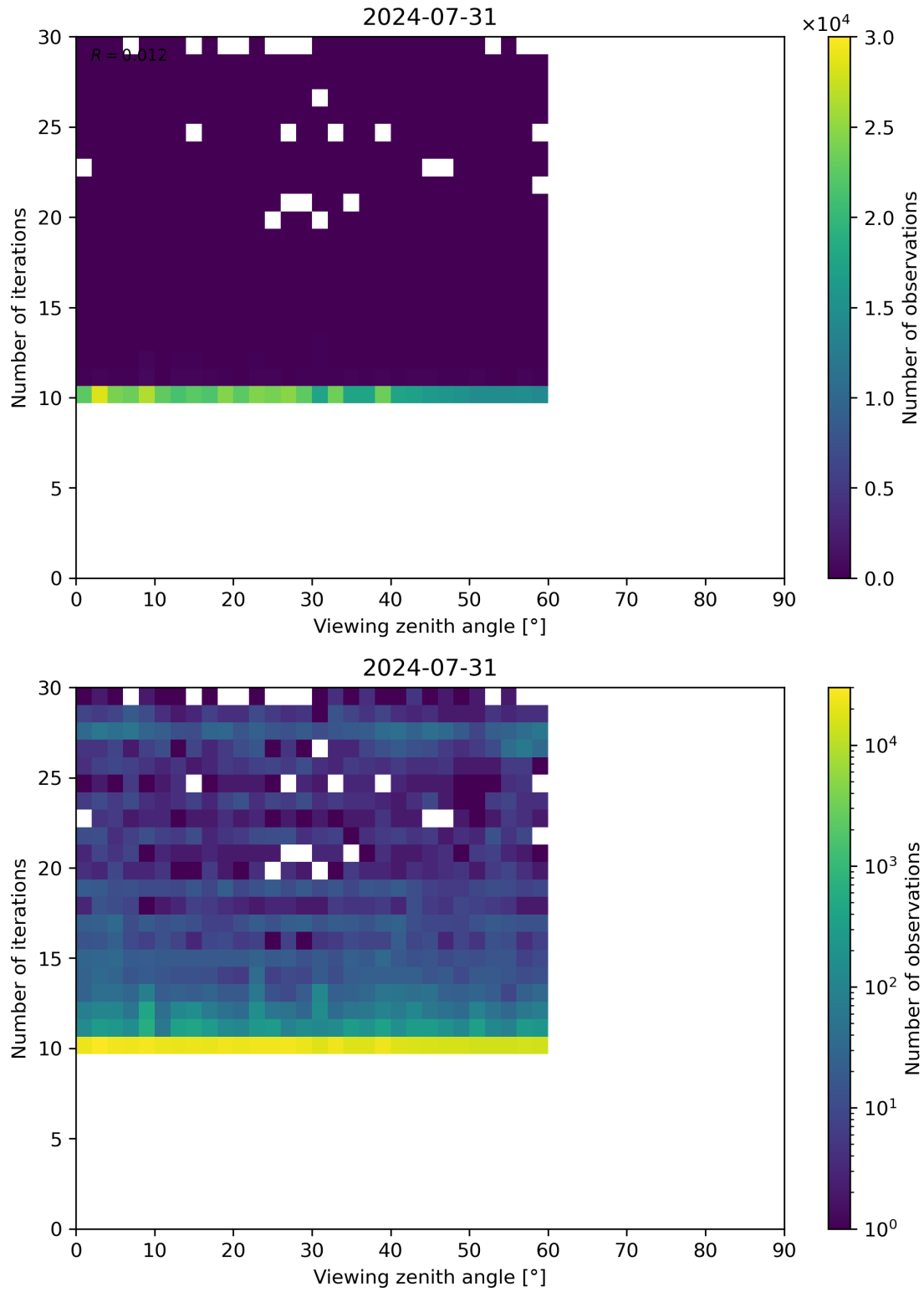
Figure 113: Scatter density plot of “Viewing zenith angle” against “Number of iterations” for 2024-07-31 to 2024-08-01.
