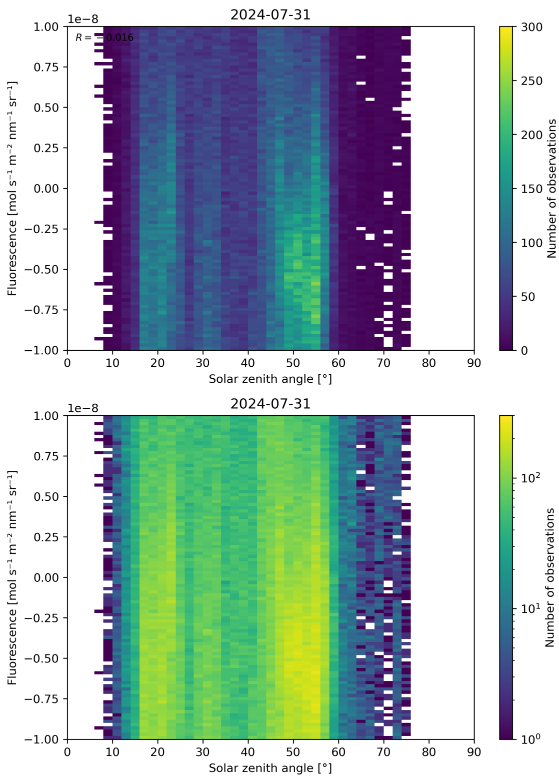
Figure 97: Scatter density plot of “Solar zenith angle” against “Fluorescence” for 2024-07-31 to 2024-08-01.
