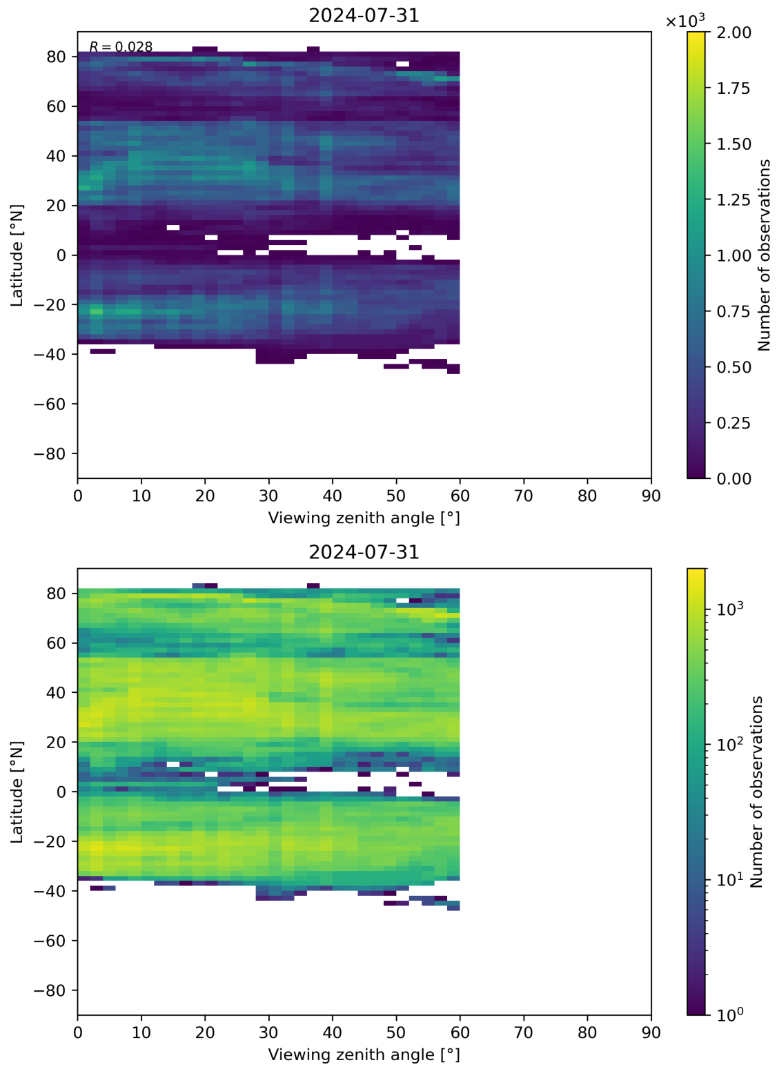
Figure 109: Scatter density plot of “Viewing zenith angle” against “Latitude” for 2024-07-31 to 2024-08-01.
