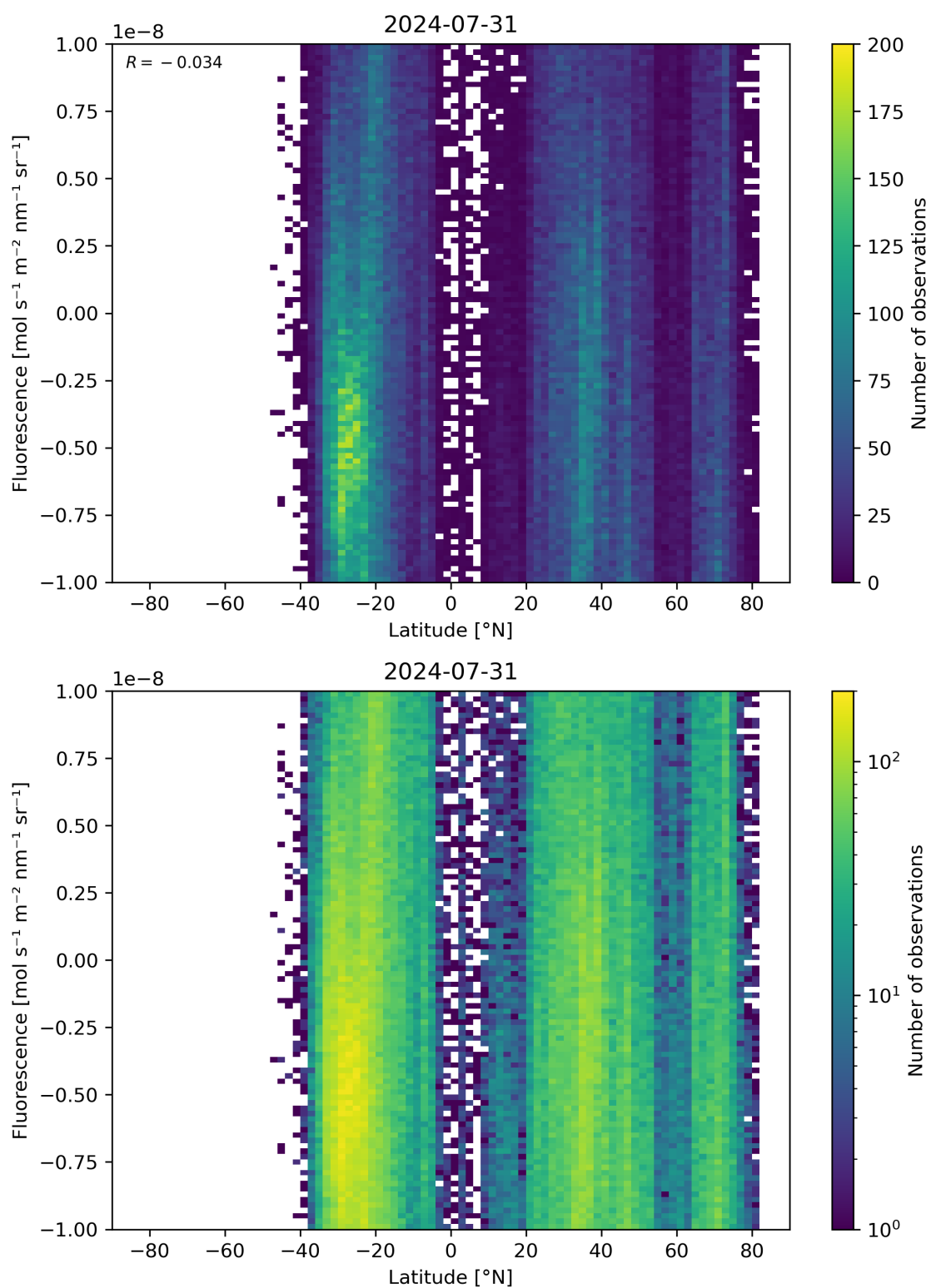
Figure 56: Scatter density plot of “Latitude” against “Fluorescence” for 2024-07-31 to 2024-08-01.
