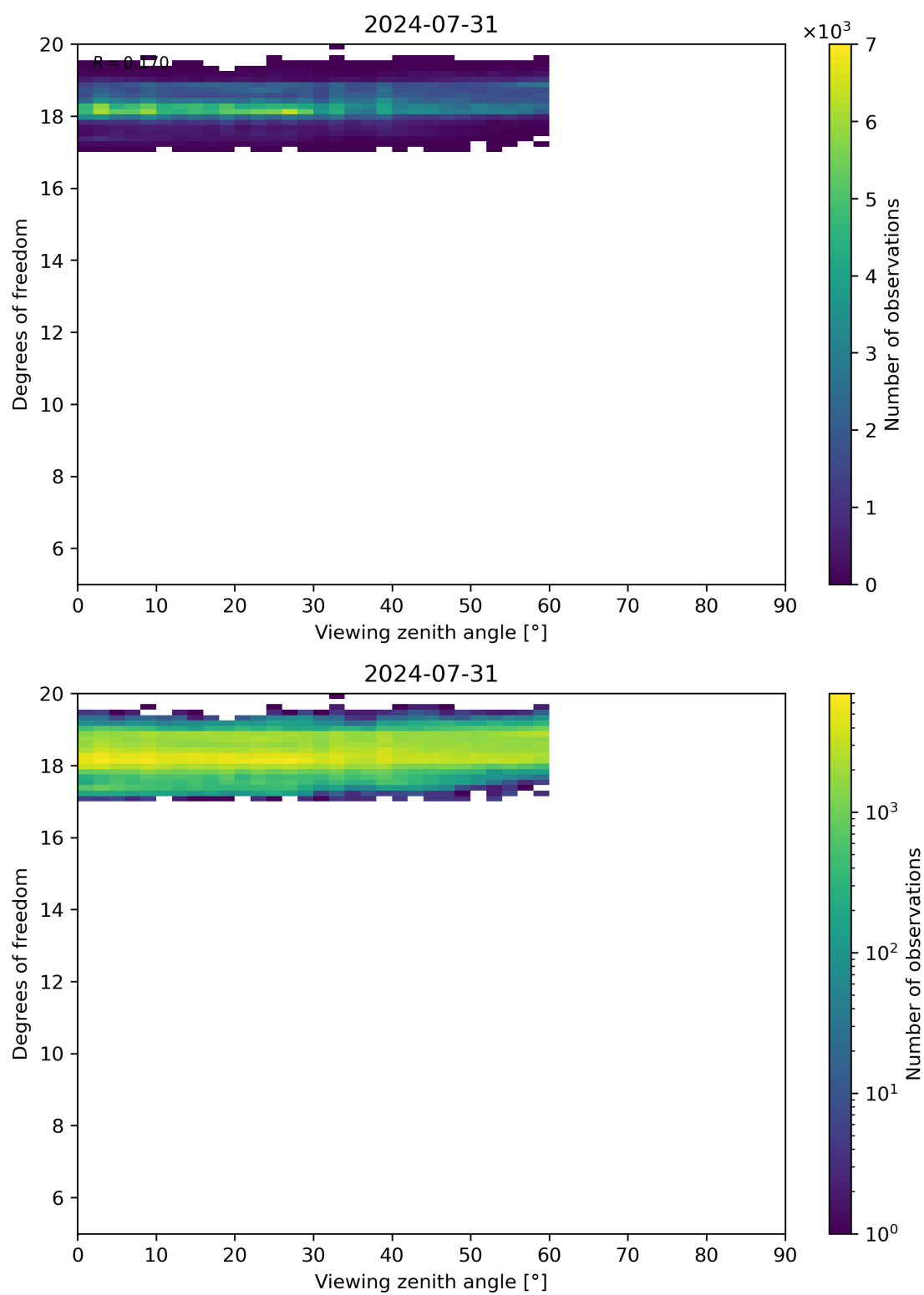
Figure 107: Scatter density plot of “Viewing zenith angle” against “Degrees of freedom” for 2024-07-31 to 2024-08-01.
