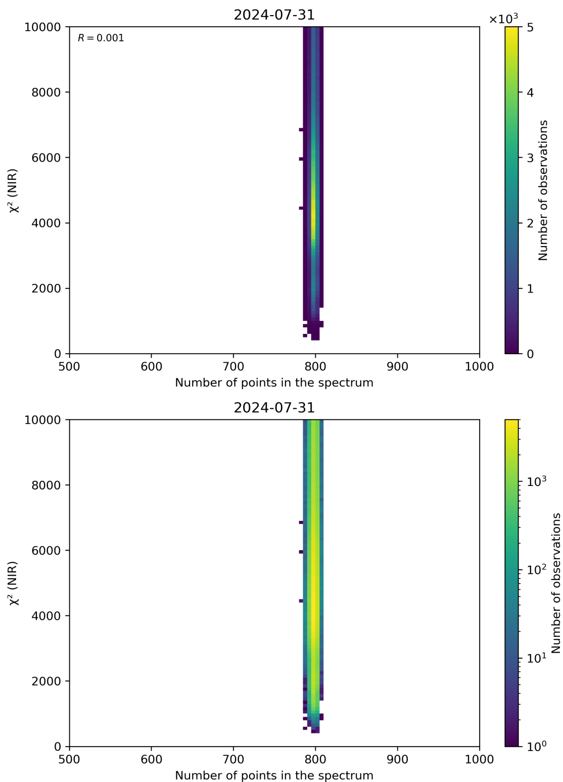
Figure 88: Scatter density plot of “Number of points in the spectrum” against “ \chi^2 (NIR)” for 2024-07-31 to 2024-08-01.
