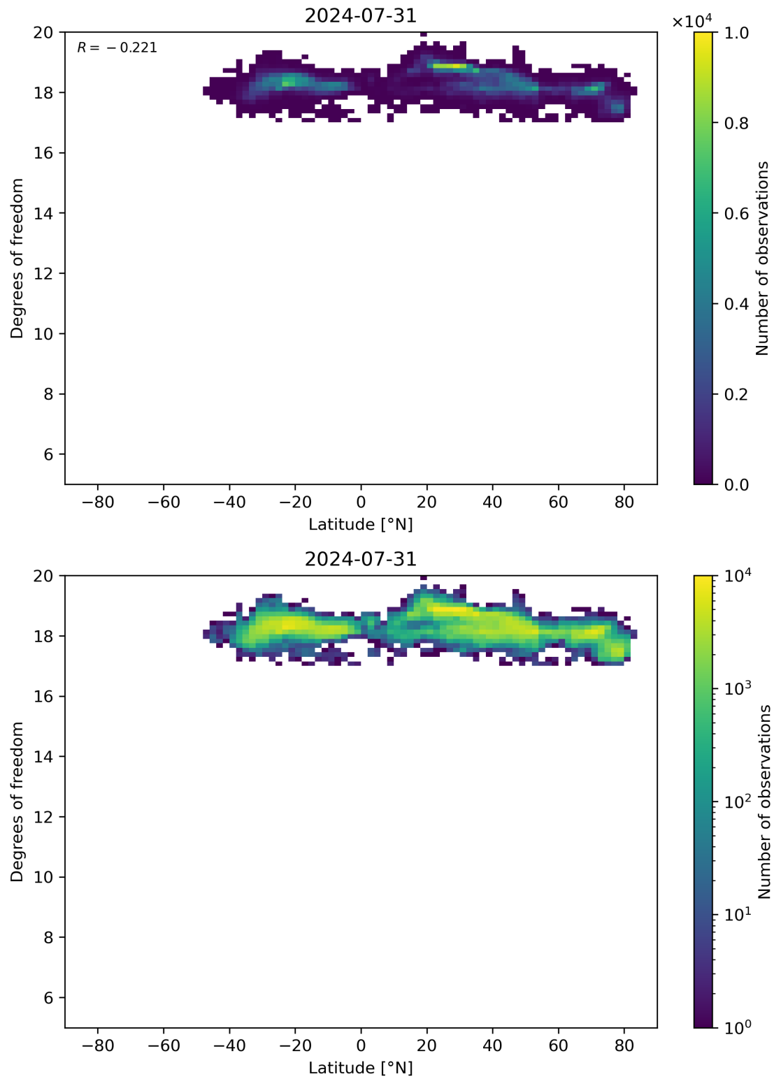
Figure 55: Scatter density plot of “Latitude” against “Degrees of freedom” for 2024-07-31 to 2024-08-01.
