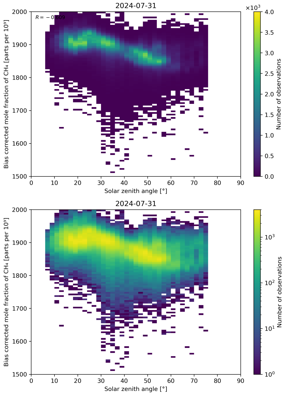
Figure 100: Scatter density plot of “Solar zenith angle” against “Bias corrected mole fraction of CH 4 ” for 2024-07-31 to 2024-08-01.
