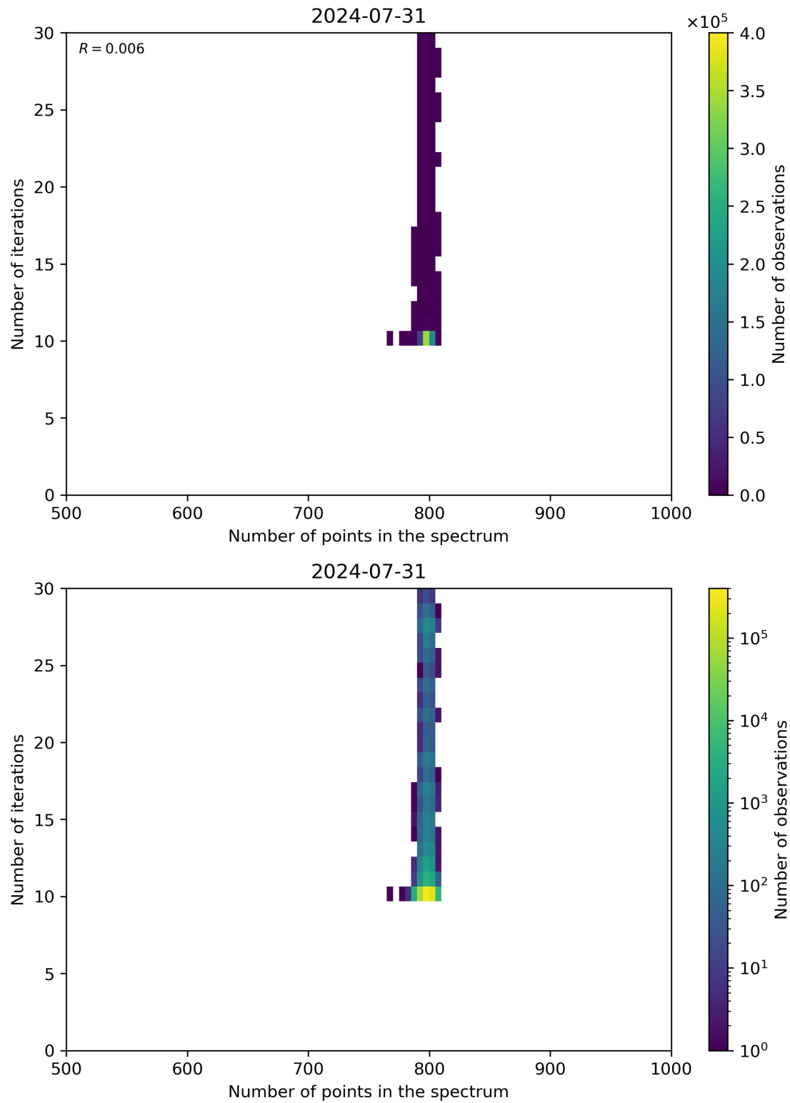
Figure 92: Scatter density plot of “Number of points in the spectrum” against “Number of iterations” for 2024-07-31 to 2024-08-01.
