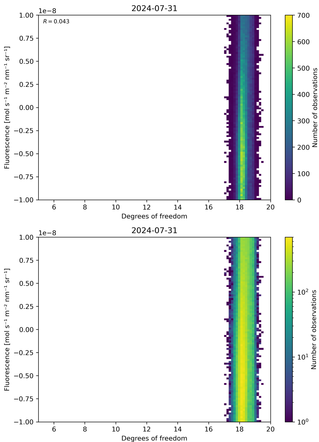
Figure 51: Scatter density plot of “Degrees of freedom” against “Fluorescence” for 2024-07-31 to 2024-08-01.
