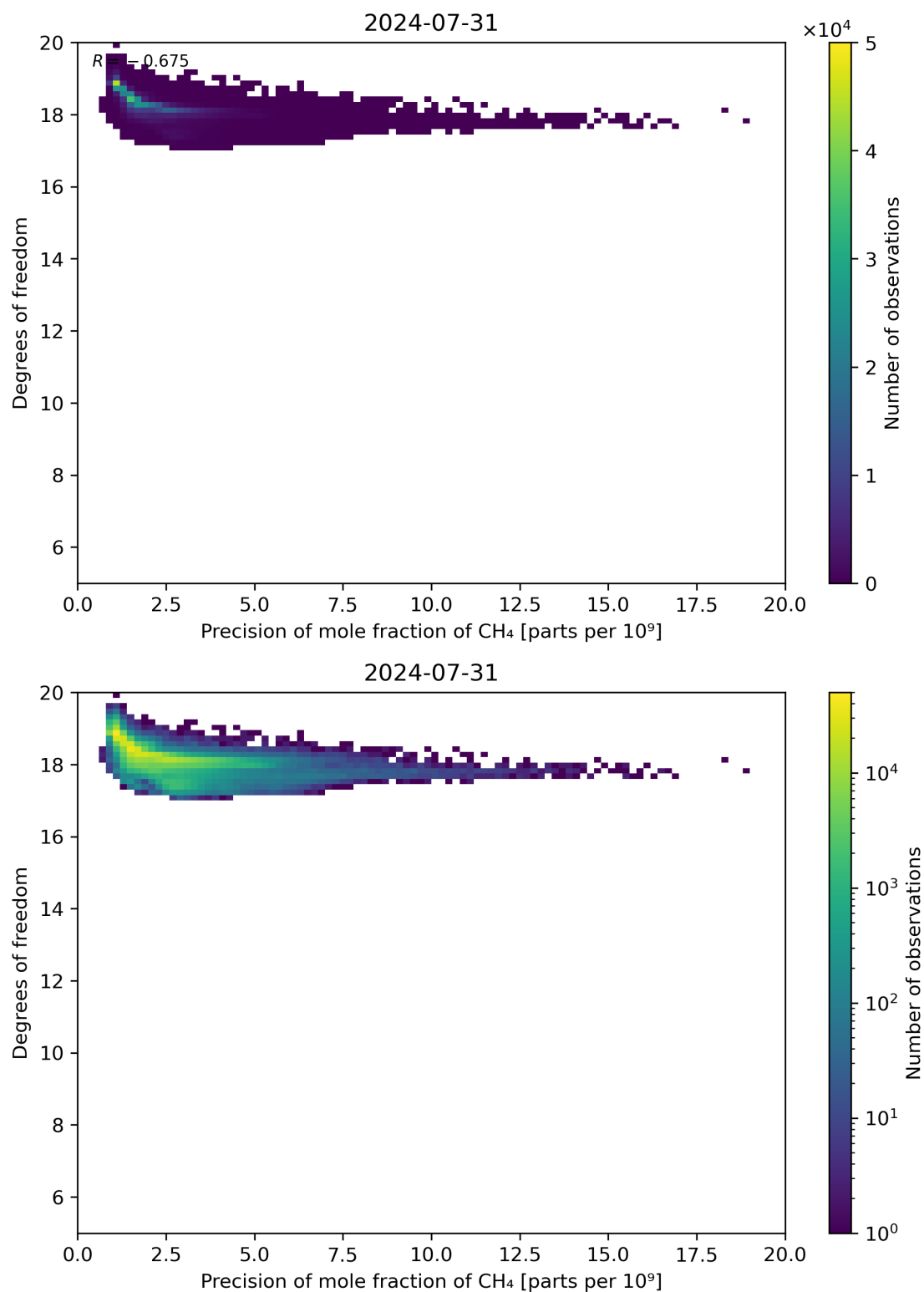
Figure 80: Scatter density plot of “Precision of mole fraction of CH 4 ” against “Degrees of freedom” for 2024-07-31 to 2024-08-01.
