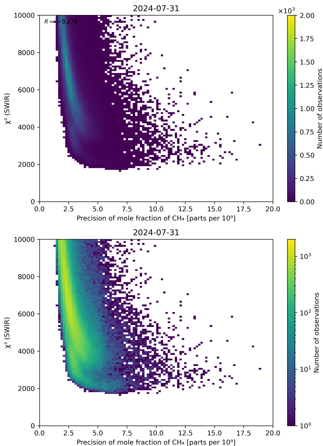
Figure 79: Scatter density plot of “Precision of mole fraction of \text{CH}_4 ” against “ \chi^2 (SWIR)” for 2024-07-31 to 2024-08-01.
