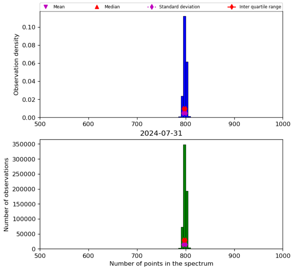
Figure 26: Histogram of “Number of points in the spectrum” for 2024-07-31 to 2024-08-01
