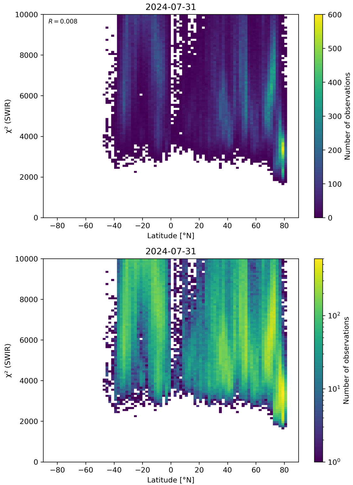
Figure 54: Scatter density plot of “Latitude” against “ \chi^2 (SWIR)” for 2024-07-31 to 2024-08-01.
