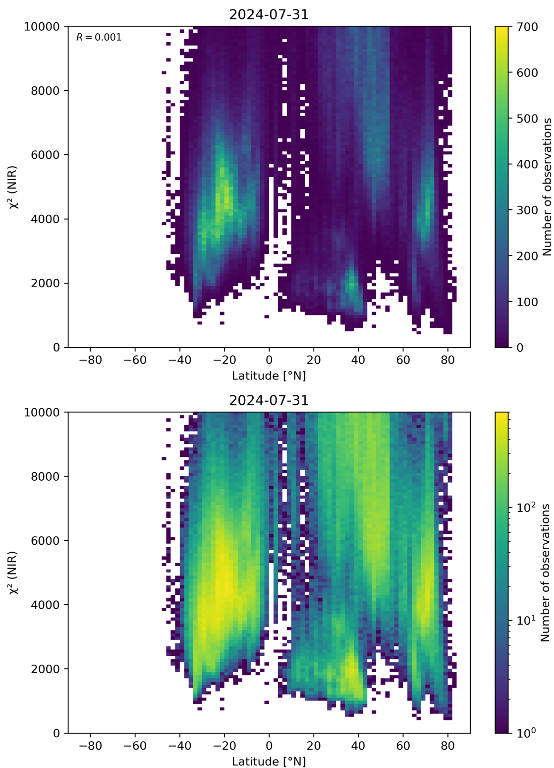
Figure 53: Scatter density plot of “Latitude” against “ \chi^2 (NIR)” for 2024-07-31 to 2024-08-01.
