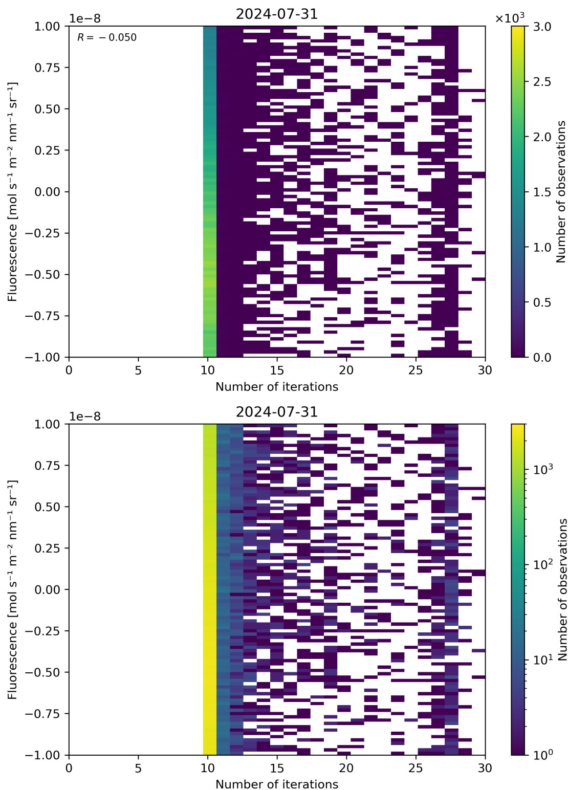
Figure 87: Scatter density plot of “Number of iterations” against “Fluorescence” for 2024-07-31 to 2024-08-01.
