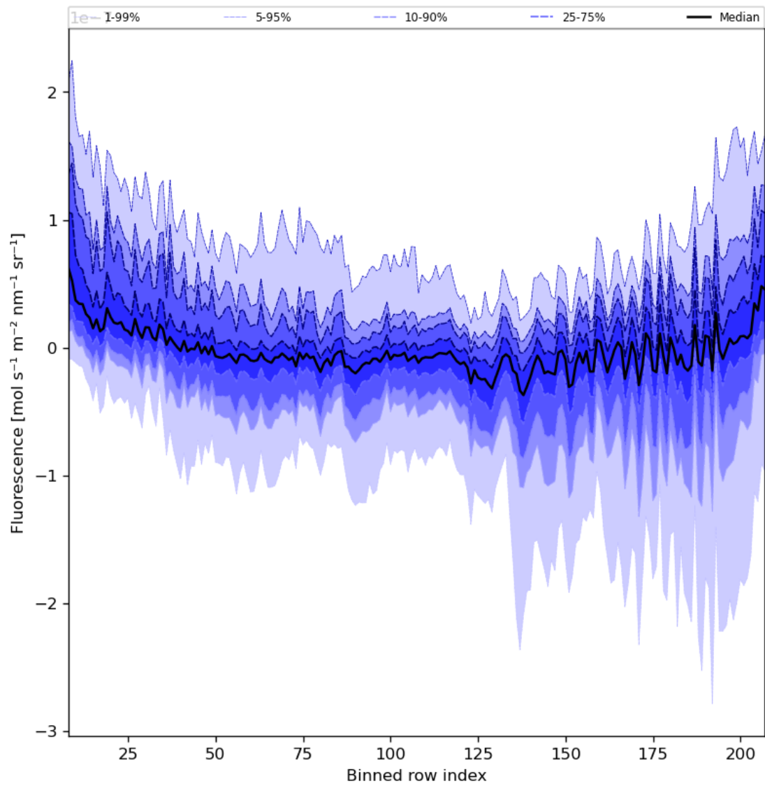
Figure 43: Along track statistics of “Fluorescence” for 2024-07-31 to 2024-08-01
