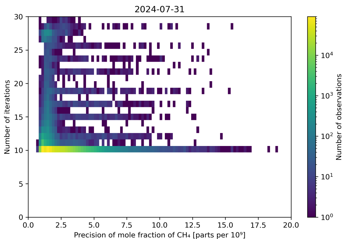
Figure 83: Scatter density plot of “Precision of mole fraction of CH 4 ” against “Number of iterations” for 2024-07-31 to 2024-08-01.
