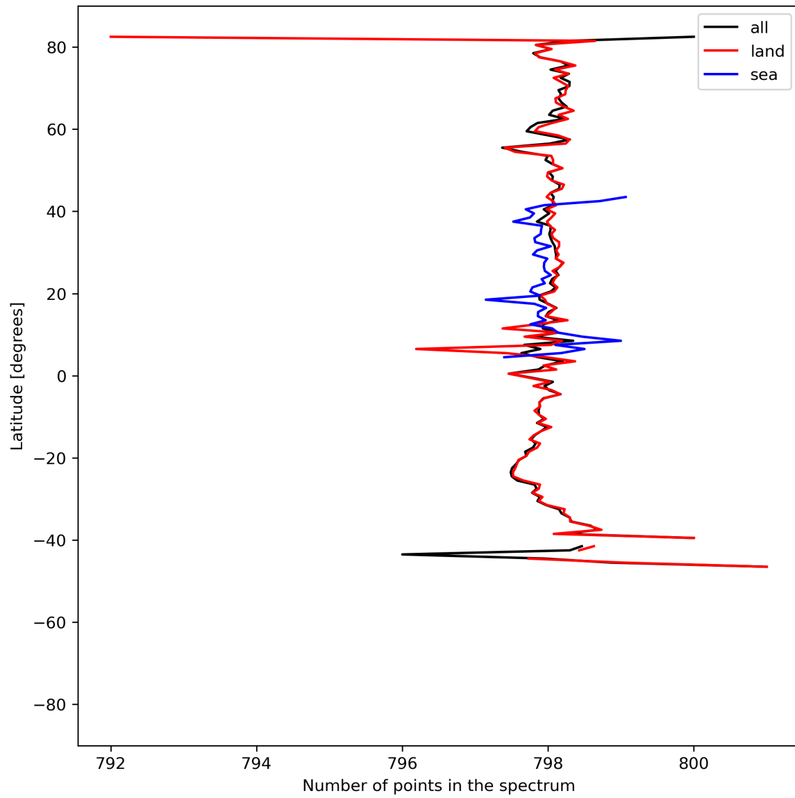
Figure 15: Zonal average of “Number of points in the spectrum” for 2024-07-31 to 2024-08-01.
