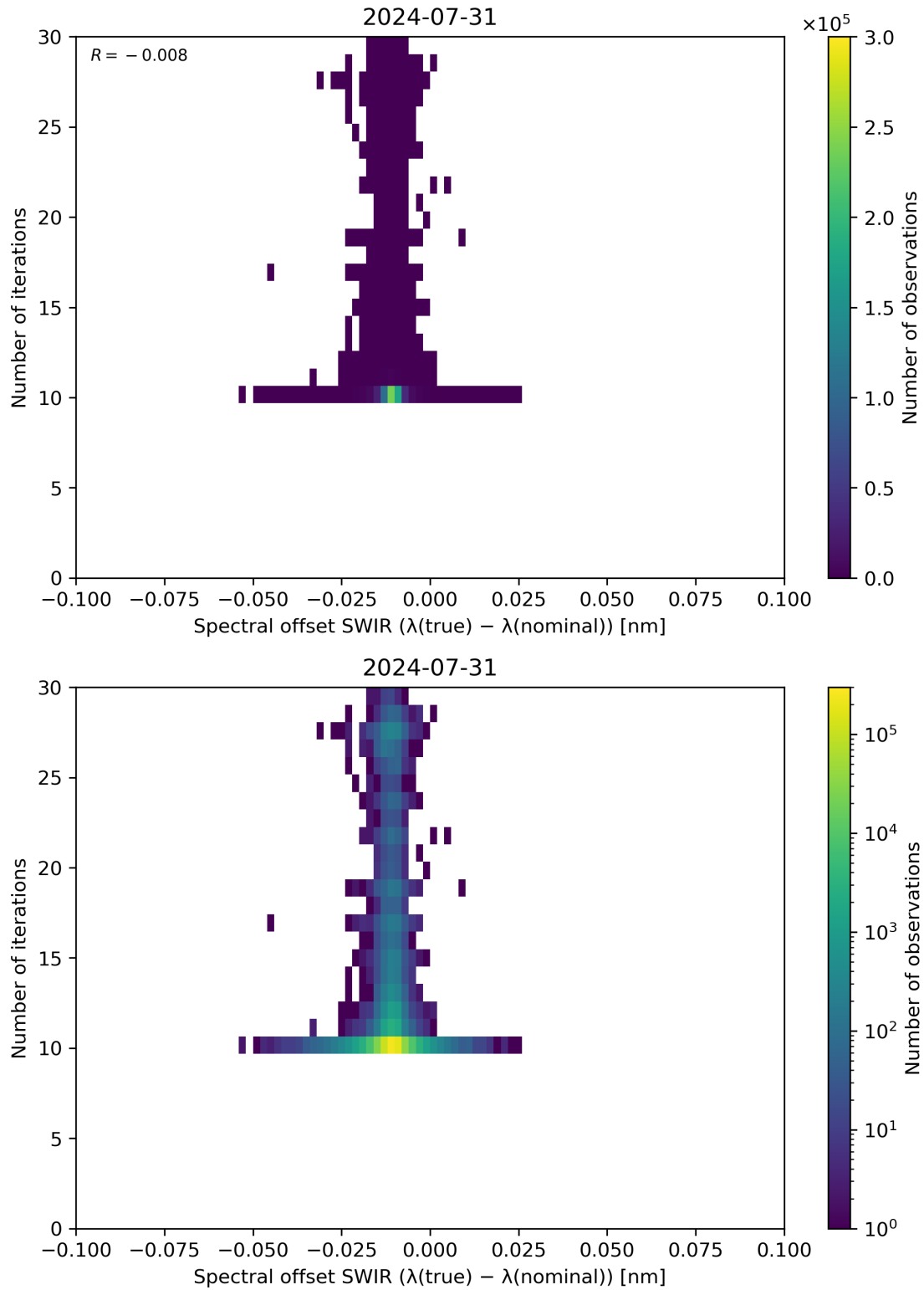
Figure 121: Scatter density plot of “Spectral offset SWIR ( \lambda(\text{true}) - \lambda(\text{nominal}) )” against “Number of iterations” for 2024-07-31 to 2024-08-01.
