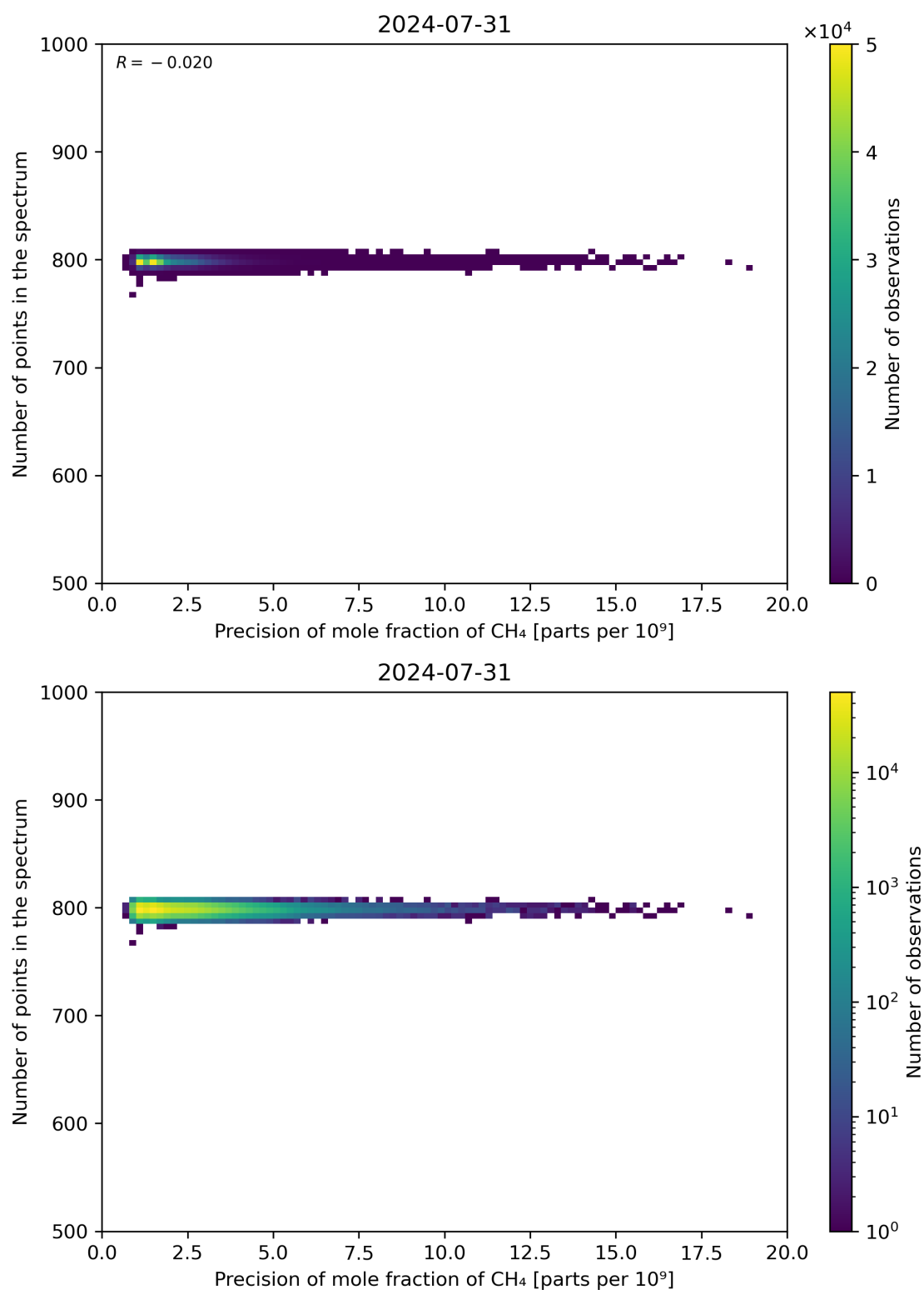
Figure 84: Scatter density plot of “Precision of mole fraction of CH 4 ” against “Number of points in the spectrum” for 2024-07-31 to 2024-08-01.
