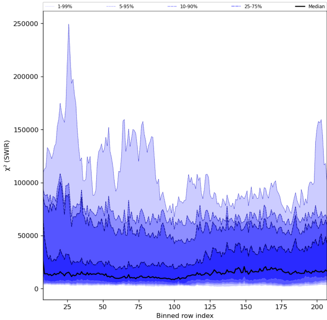
Figure 39: Along track statistics of “ \chi^2 (SWIR)” for 2024-07-31 to 2024-08-01
