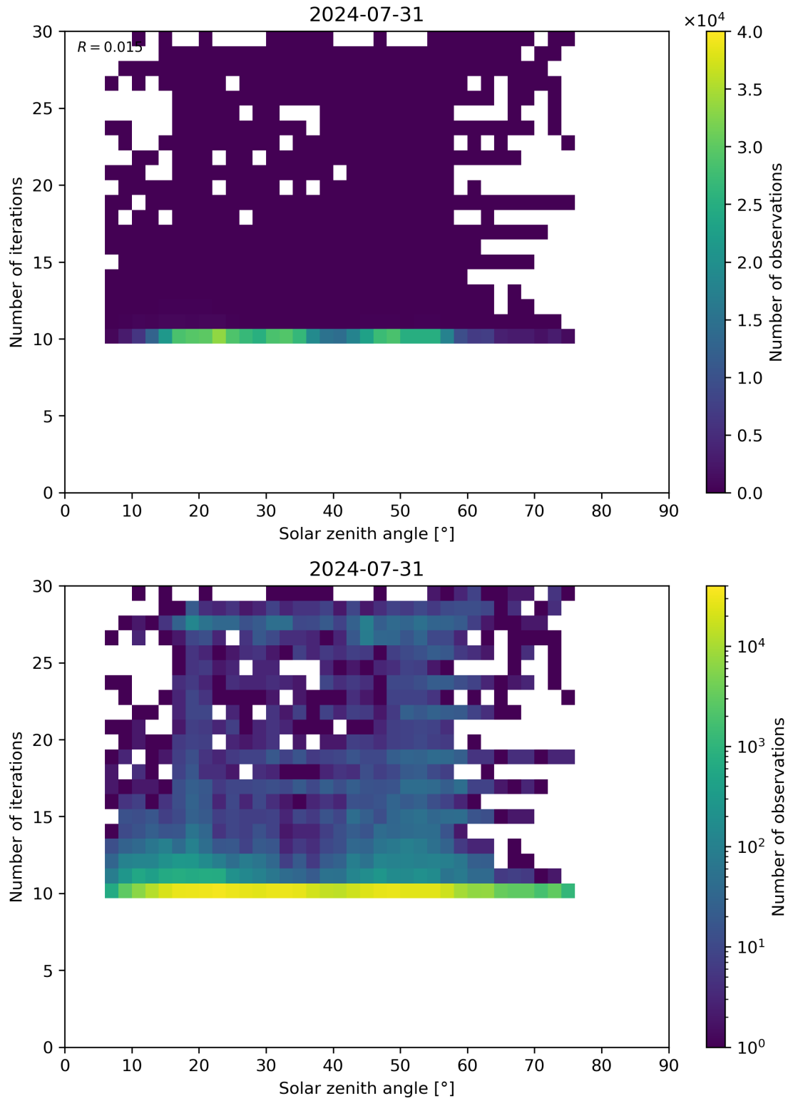
Figure 102: Scatter density plot of “Solar zenith angle” against “Number of iterations” for 2024-07-31 to 2024-08-01.
