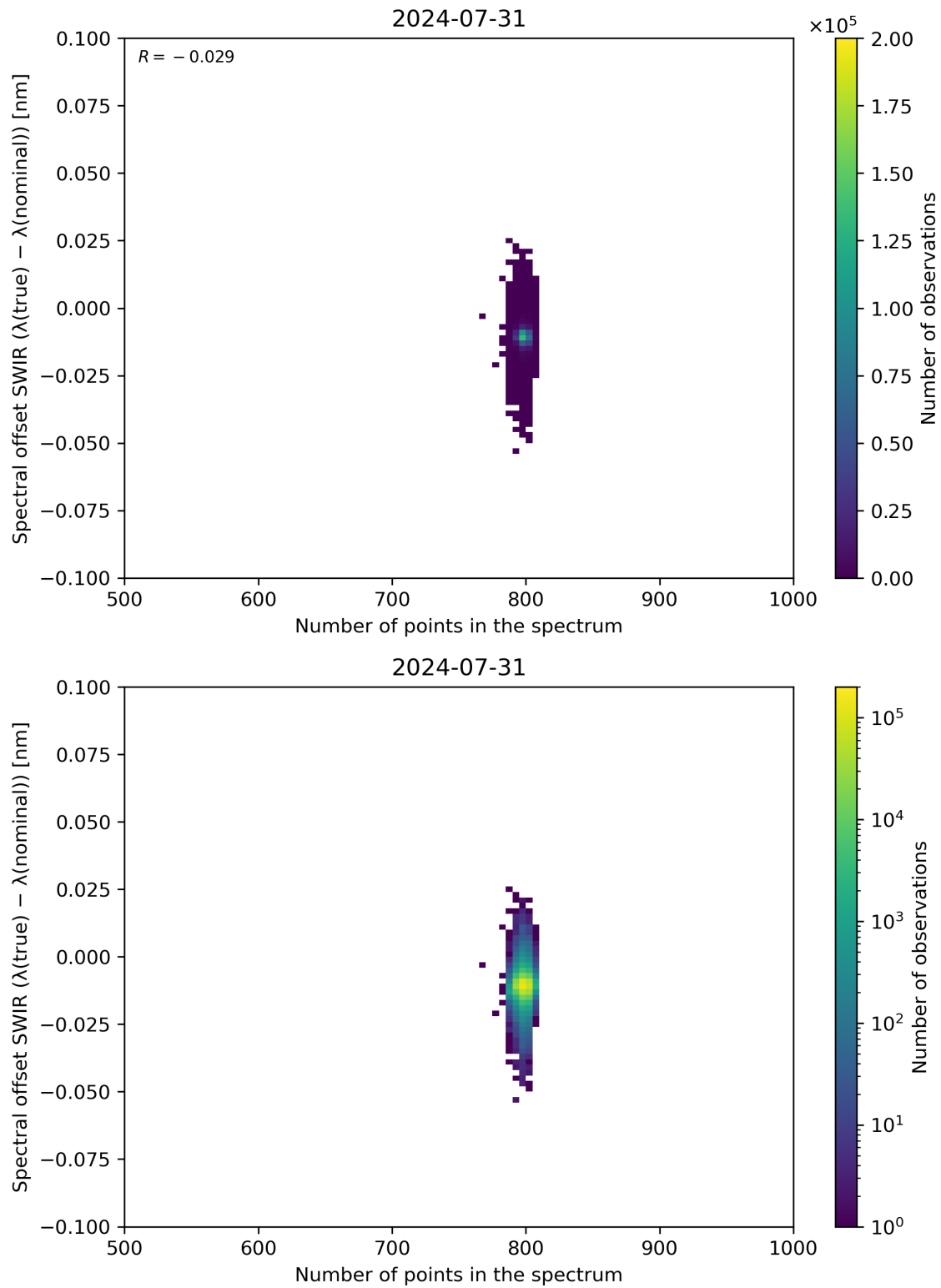
Figure 93: Scatter density plot of “Number of points in the spectrum” against “Spectral offset SWIR ( \lambda(\text{true}) - \lambda(\text{nominal}) )” for 2024-07-31 to 2024-08-01.
