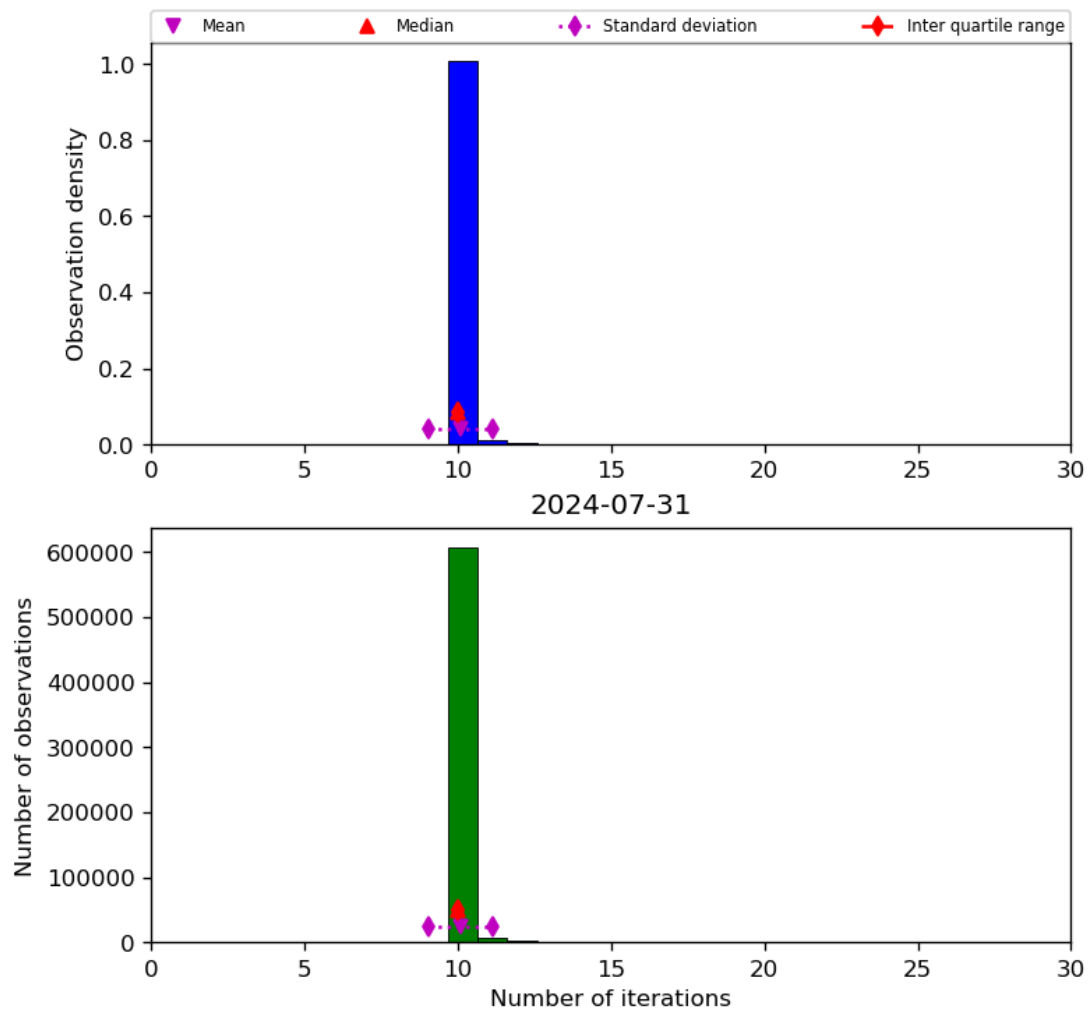
Figure 31: Histogram of “Number of iterations” for 2024-07-31 to 2024-08-01
