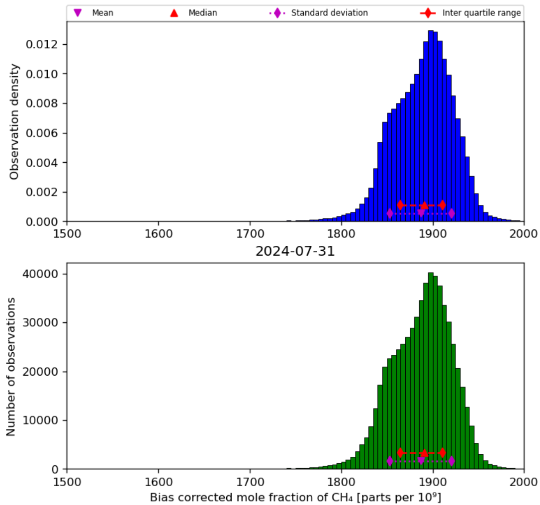
Figure 25: Histogram of “Bias corrected mole fraction of CH 4 ” for 2024-07-31 to 2024-08-01
