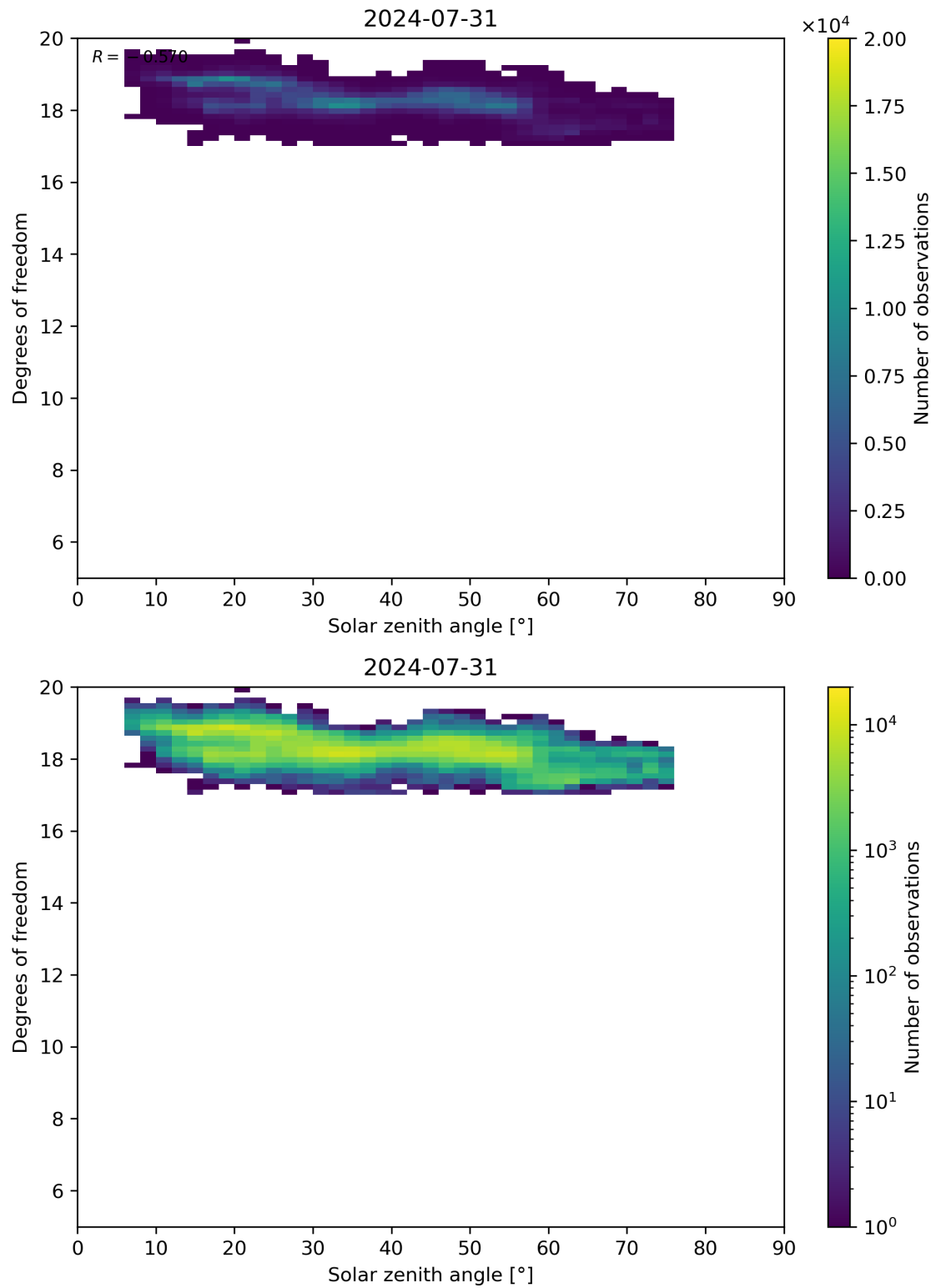
Figure 96: Scatter density plot of “Solar zenith angle” against “Degrees of freedom” for 2024-07-31 to 2024-08-01.
