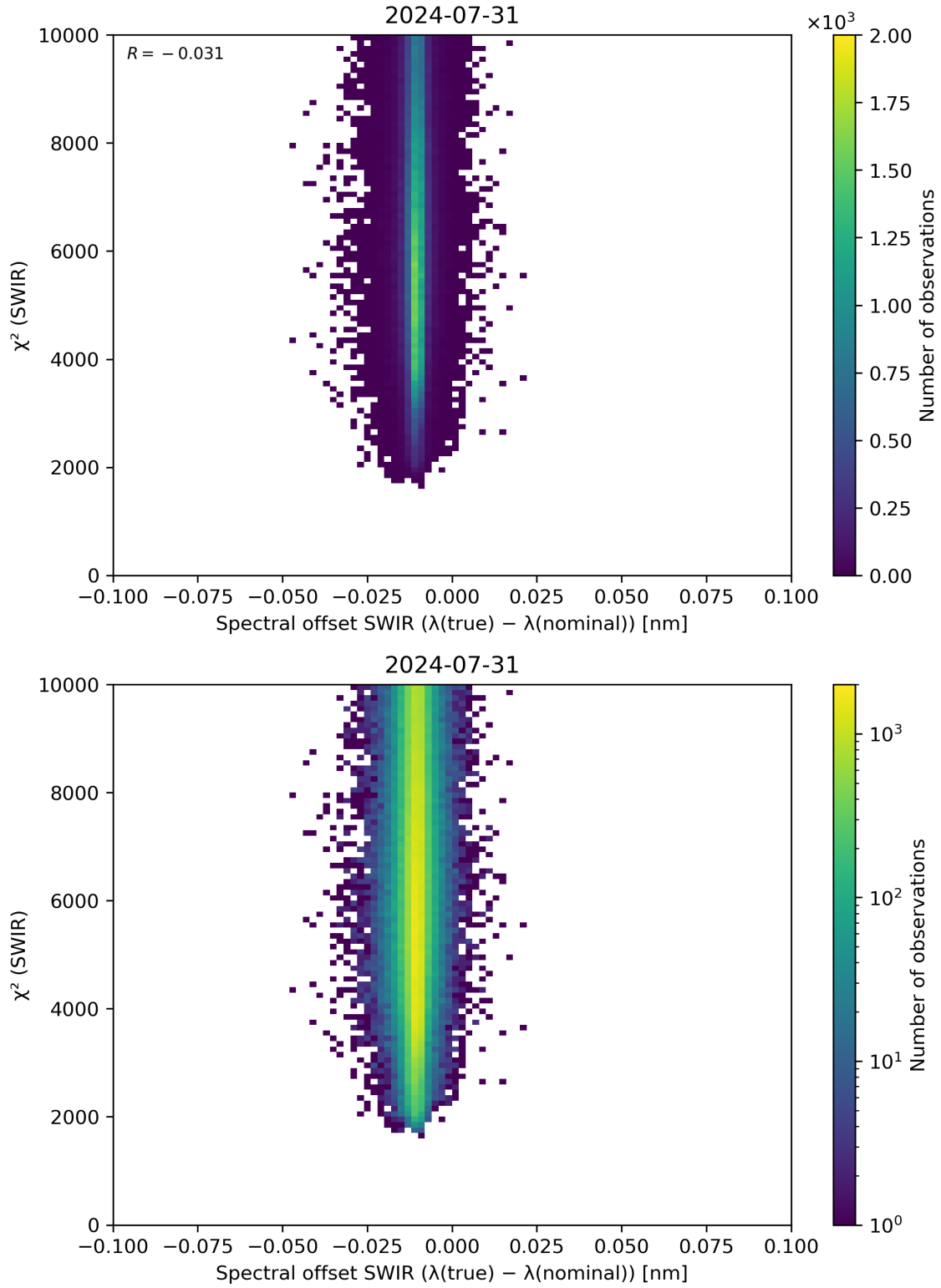
Figure 118: Scatter density plot of “Spectral offset SWIR ( \lambda(\text{true}) - \lambda(\text{nominal}) )” against “ \chi^2 (SWIR)” for 2024-07-31 to 2024-08-01.
