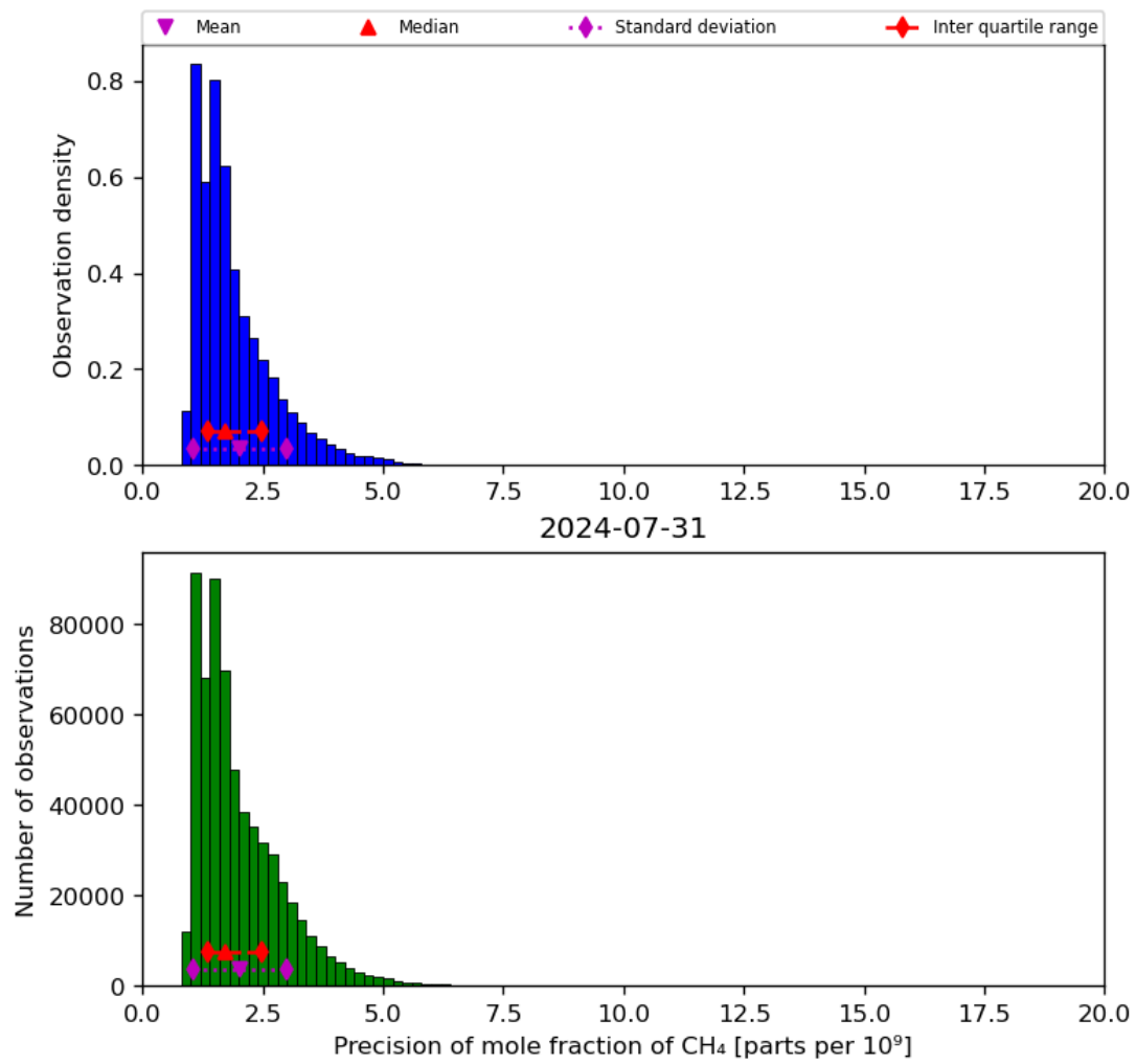
Figure 24: Histogram of “Precision of mole fraction of CH 4 ” for 2024-07-31 to 2024-08-01
