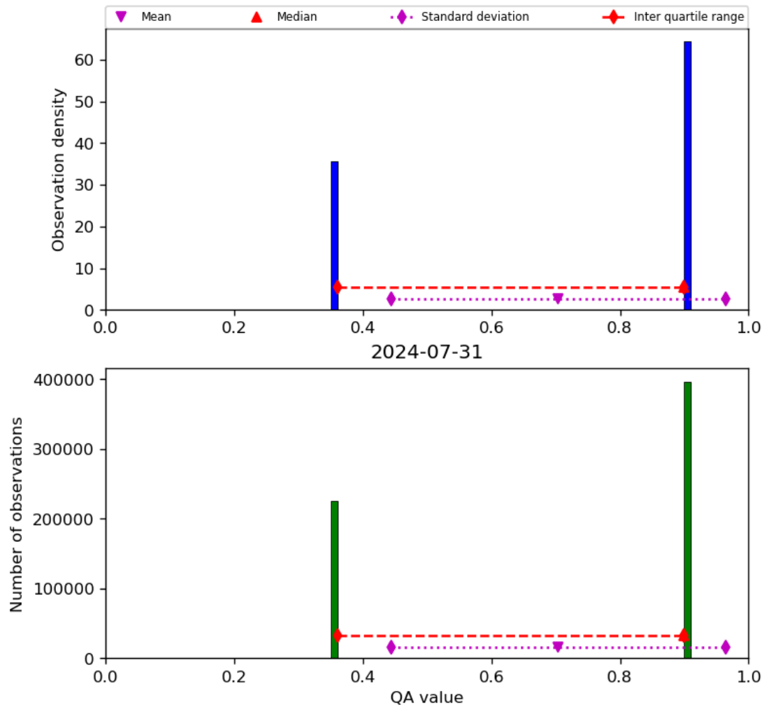
Figure 22: Histogram of “QA value” for 2024-07-31 to 2024-08-01
