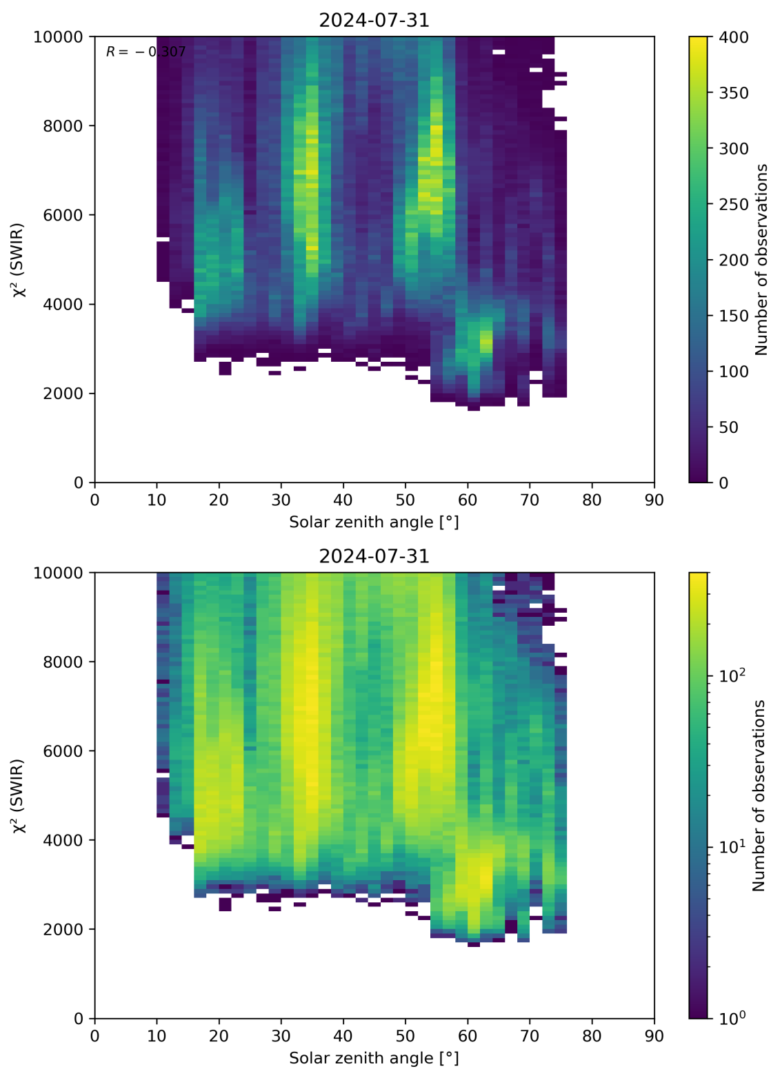
Figure 95: Scatter density plot of “Solar zenith angle” against “ \chi^2 (SWIR)” for 2024-07-31 to 2024-08-01.
