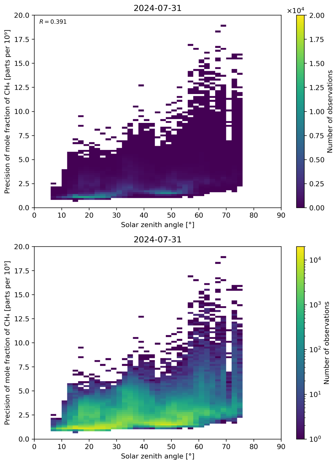
Figure 101: Scatter density plot of “Solar zenith angle” against “Precision of mole fraction of CH 4 ” for 2024-07-31 to 2024-08-01.
