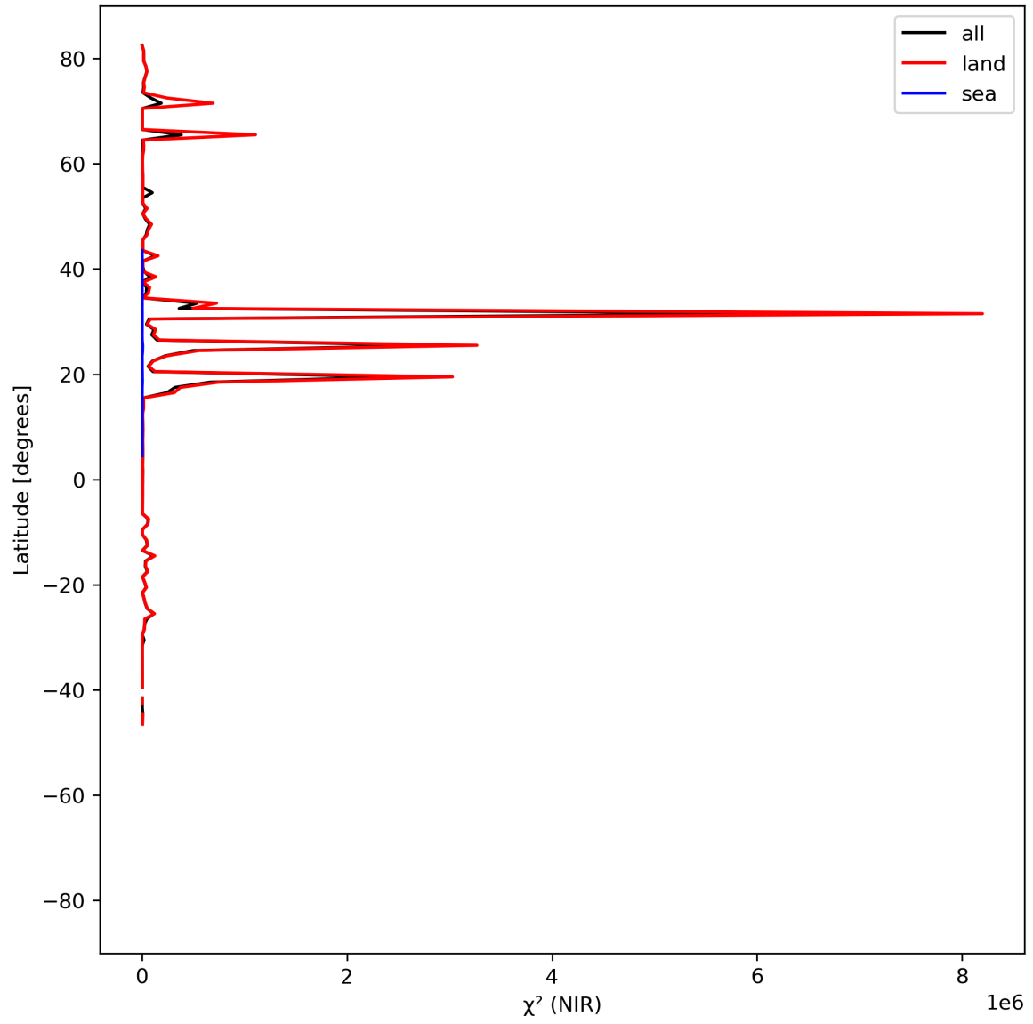
Figure 18: Zonal average of “ \chi^2 (NIR)” for 2024-07-31 to 2024-08-01.
