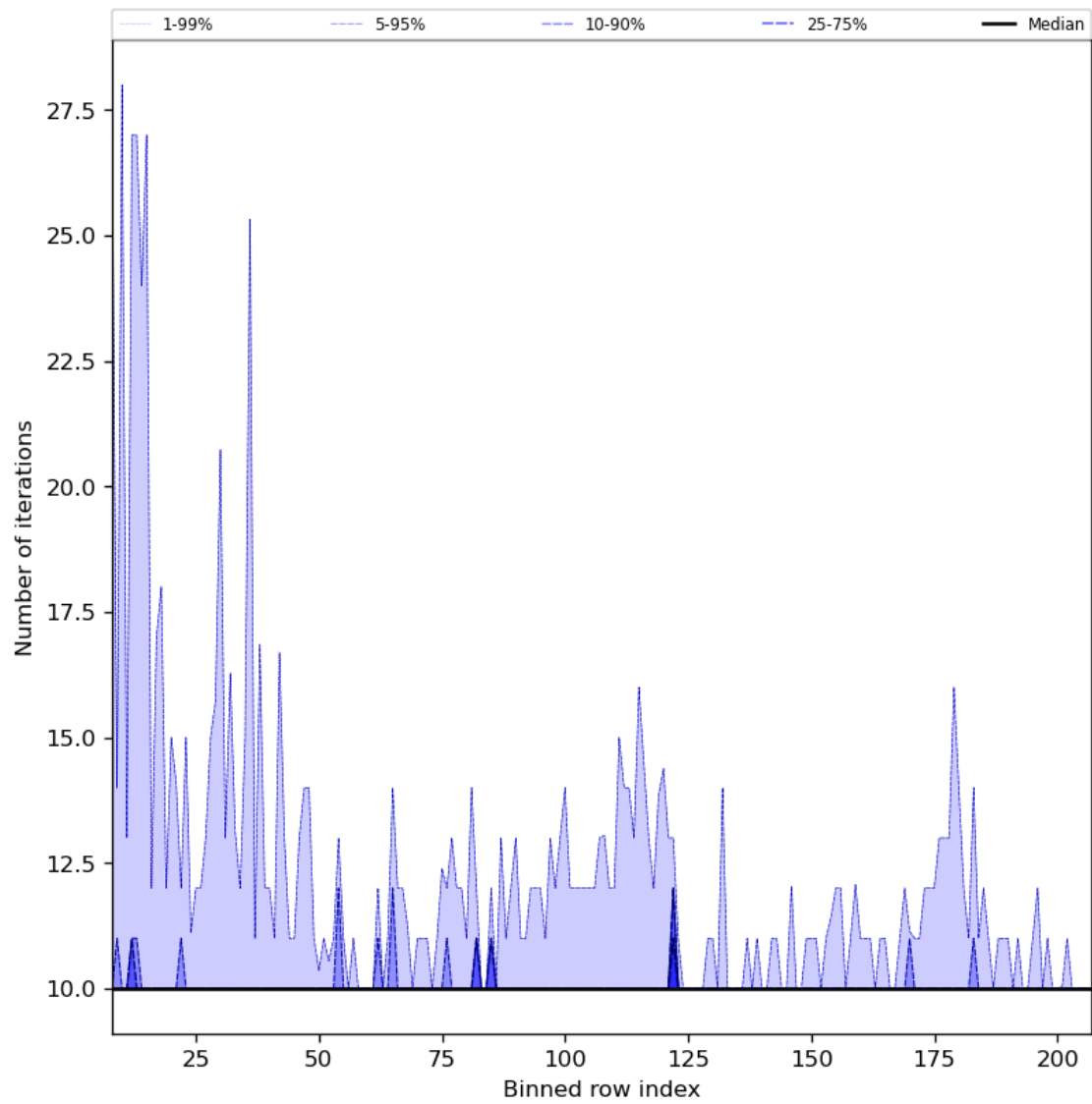
Figure 42: Along track statistics of “Number of iterations” for 2024-07-31 to 2024-08-01
