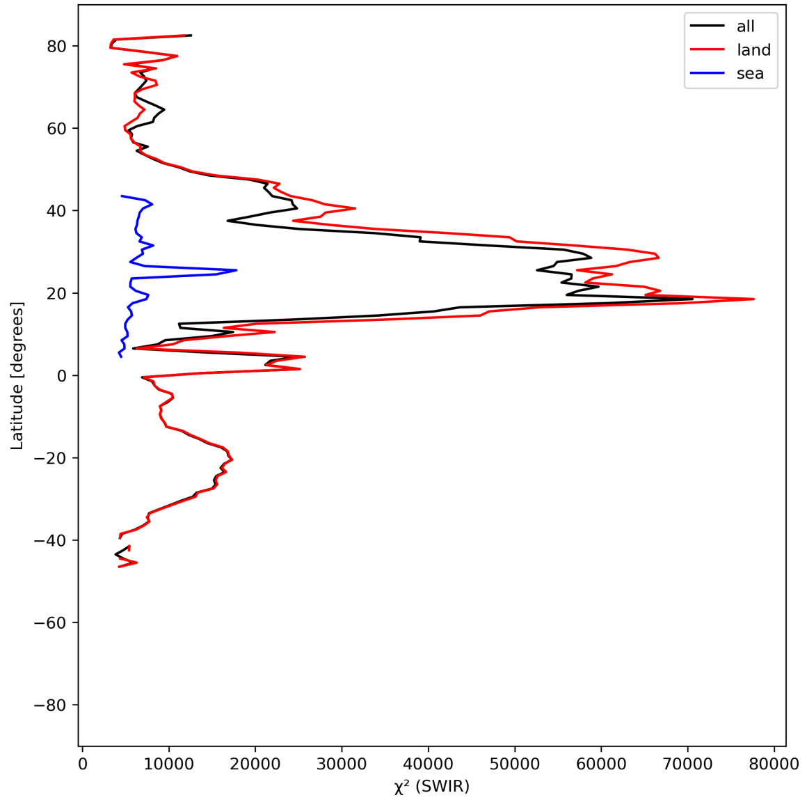
Figure 17: Zonal average of “ \chi^2 (SWIR)” for 2024-07-31 to 2024-08-01.
