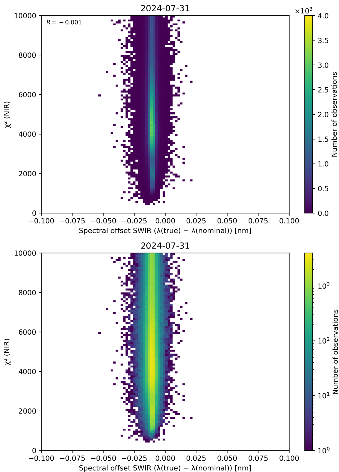
Figure 117: Scatter density plot of “Spectral offset SWIR ( \lambda(\text{true}) - \lambda(\text{nominal}) )” against “ \chi^2 (NIR)” for 2024-07-31 to 2024-08-01.
