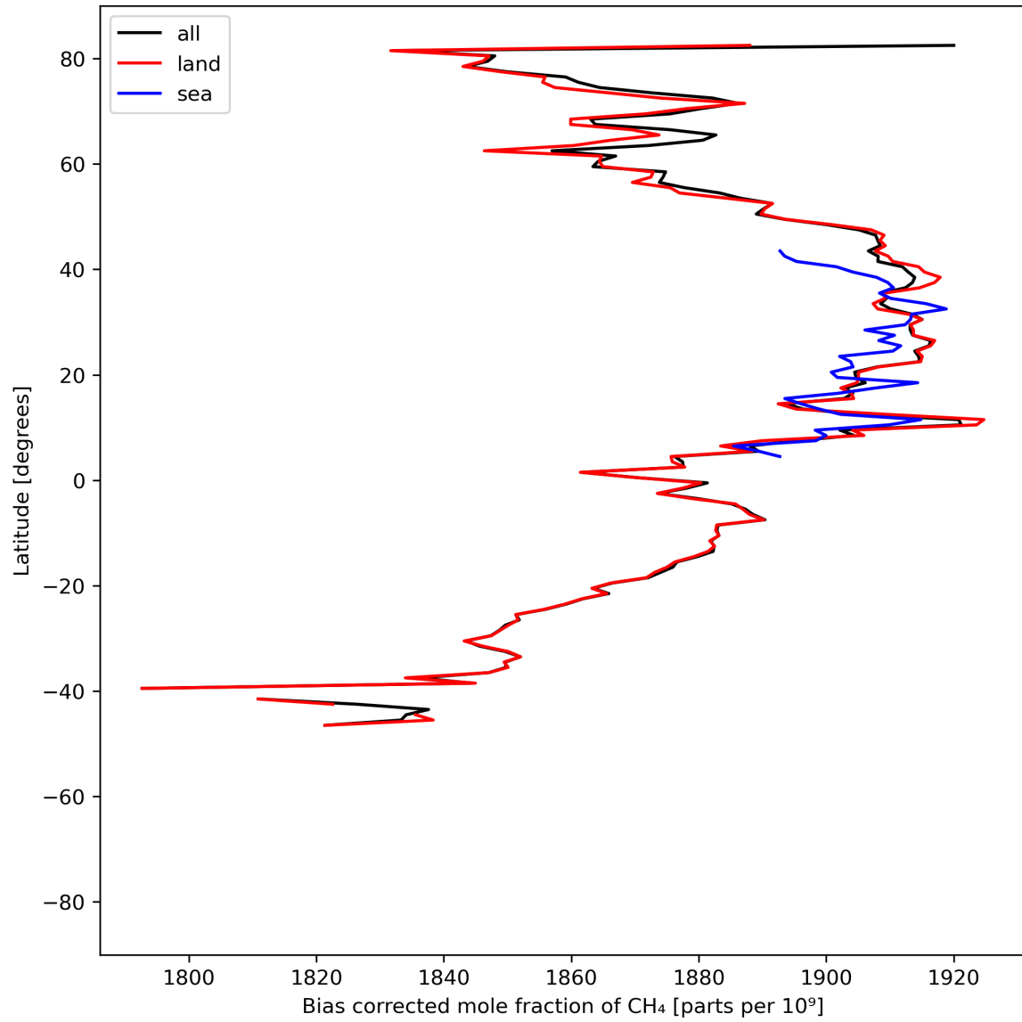
Figure 14: Zonal average of “Bias corrected mole fraction of CH 4 ” for 2024-07-31 to 2024-08-01.
