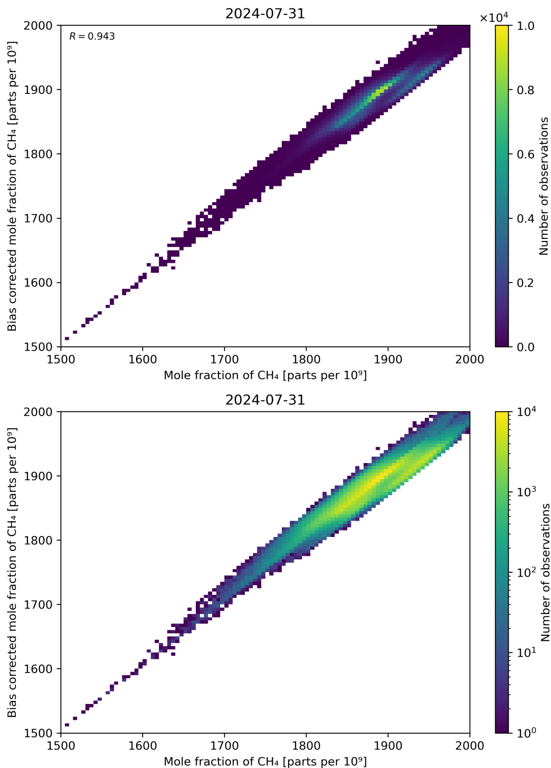
Figure 74: Scatter density plot of “Mole fraction of CH 4 ” against “Bias corrected mole fraction of CH 4 ” for 2024-07-31 to 2024-08-01.
