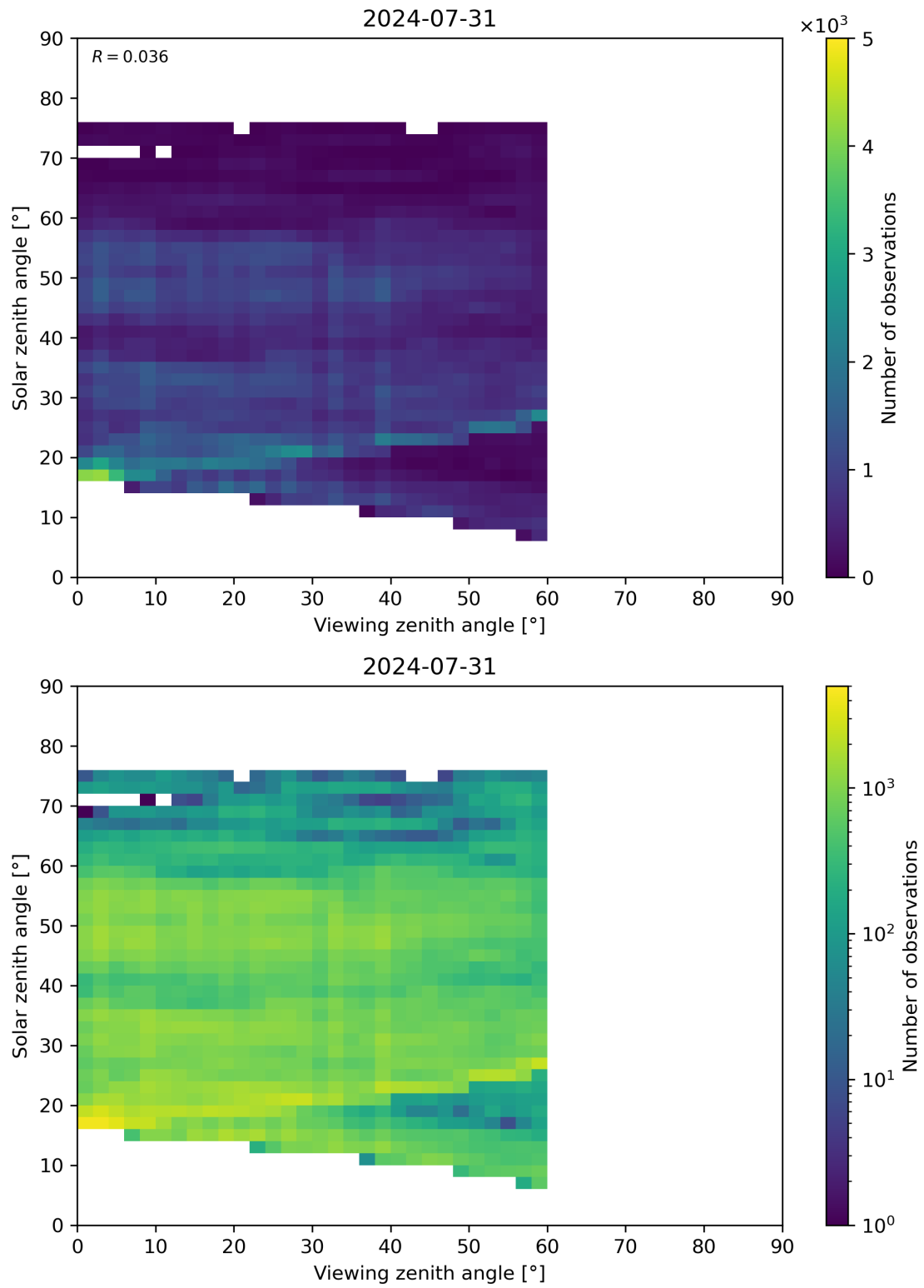
Figure 115: Scatter density plot of “Viewing zenith angle” against “Solar zenith angle” for 2024-07-31 to 2024-08-01.
