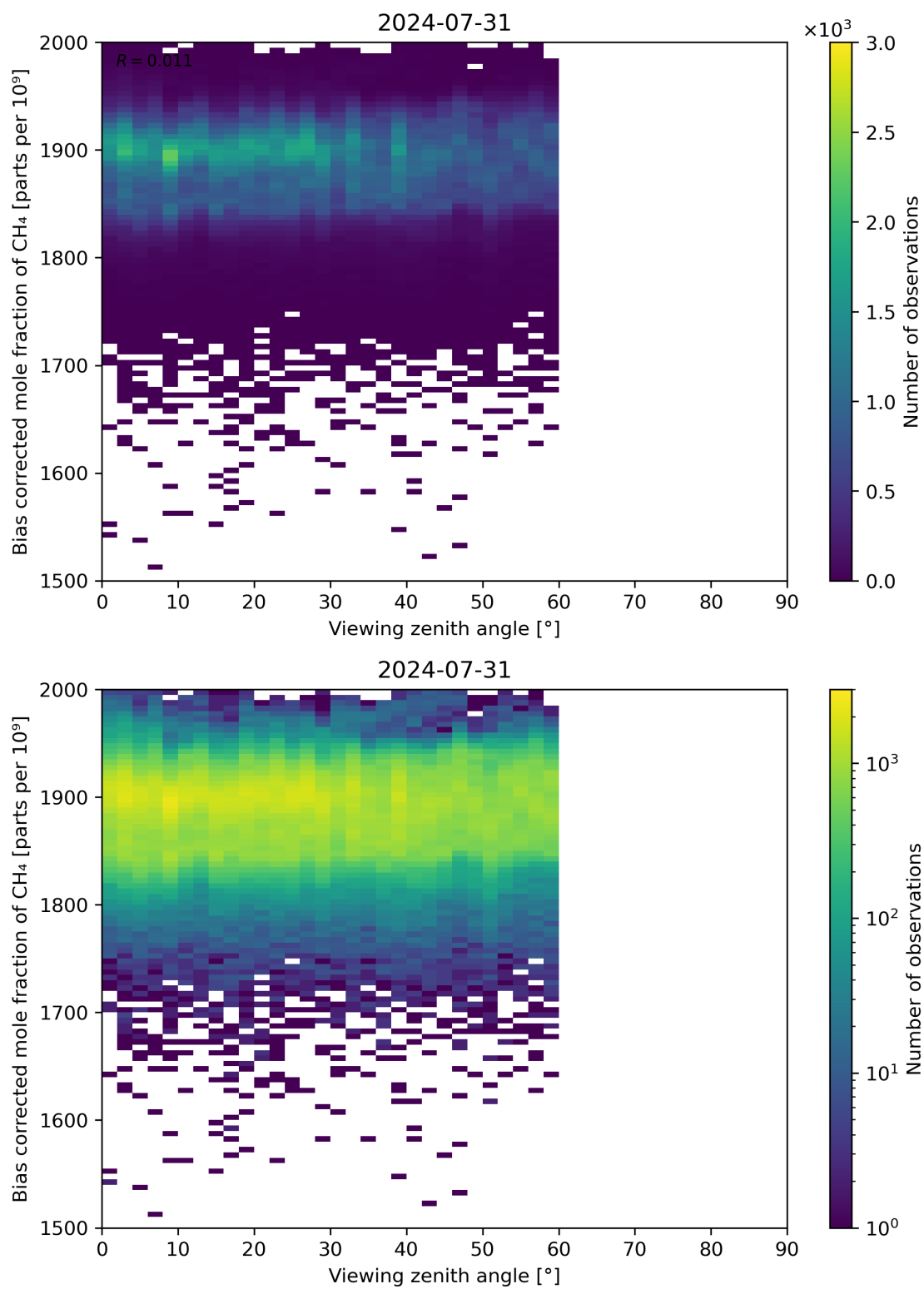
Figure 111: Scatter density plot of “Viewing zenith angle” against “Bias corrected mole fraction of CH 4 ” for 2024-07-31 to 2024-08-01.
