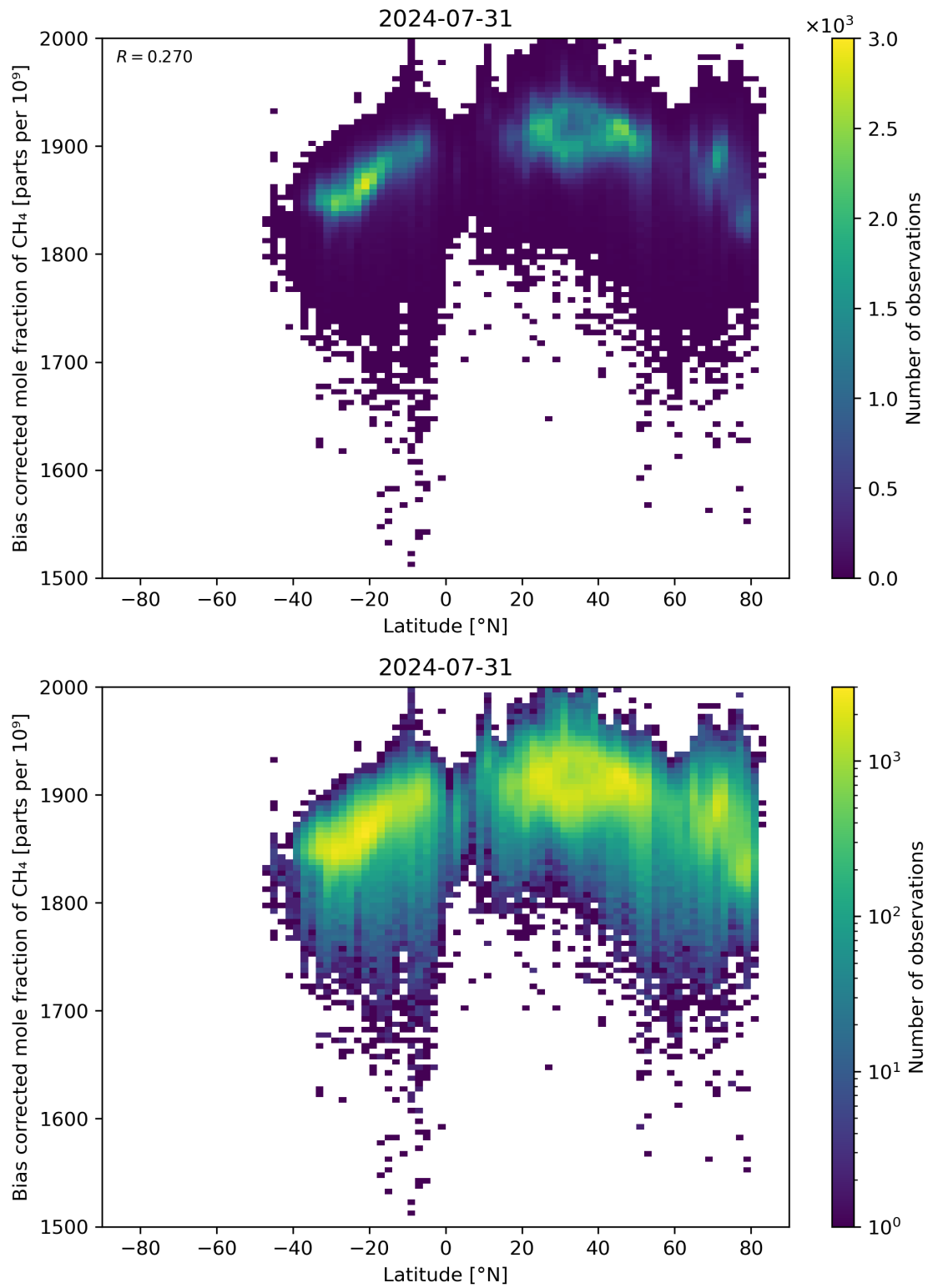
Figure 58: Scatter density plot of “Latitude” against “Bias corrected mole fraction of CH 4 ” for 2024-07-31 to 2024-08-01.
