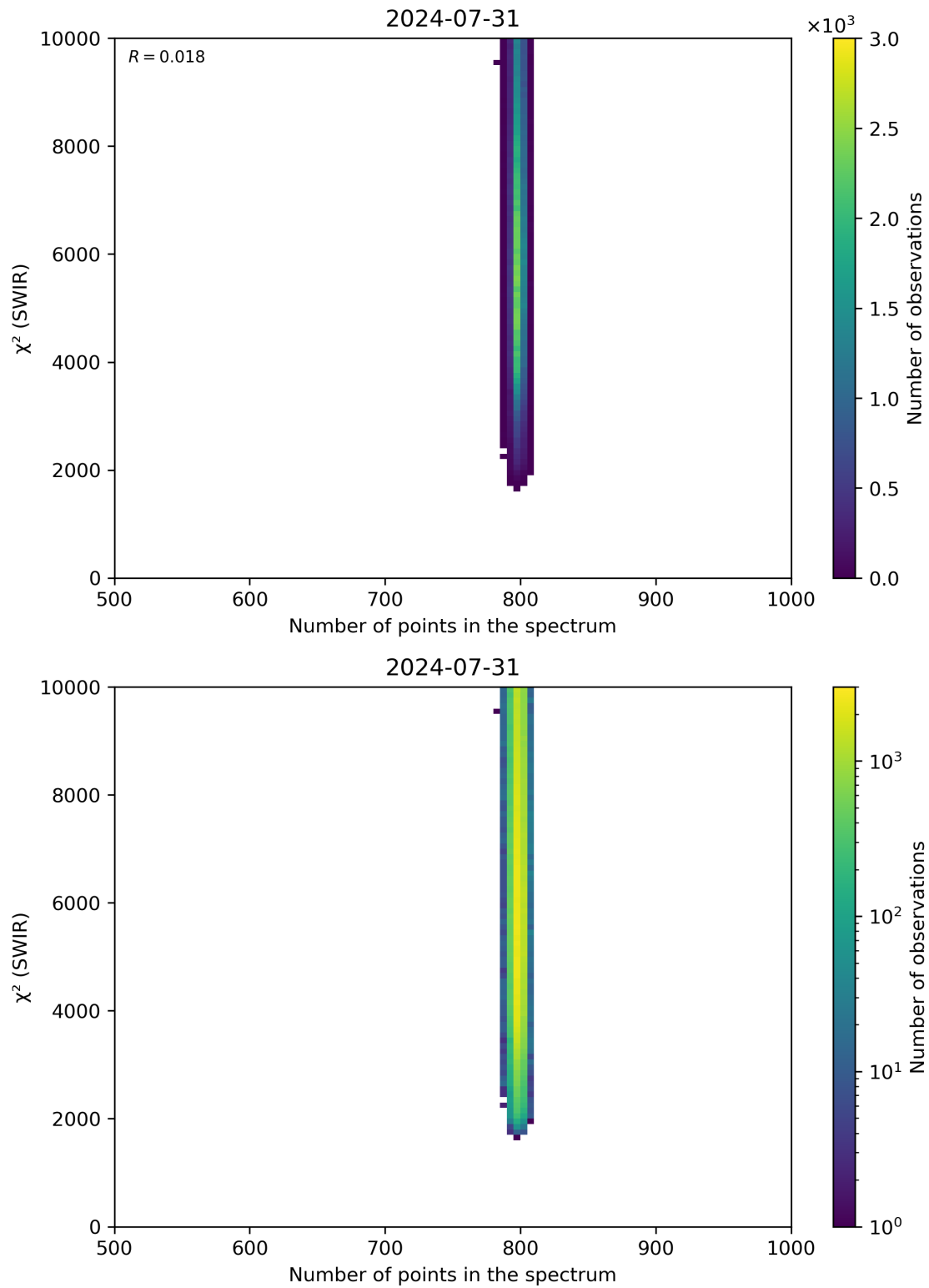
Figure 89: Scatter density plot of “Number of points in the spectrum” against “ \chi^2 (SWIR)” for 2024-07-31 to 2024-08-01.
