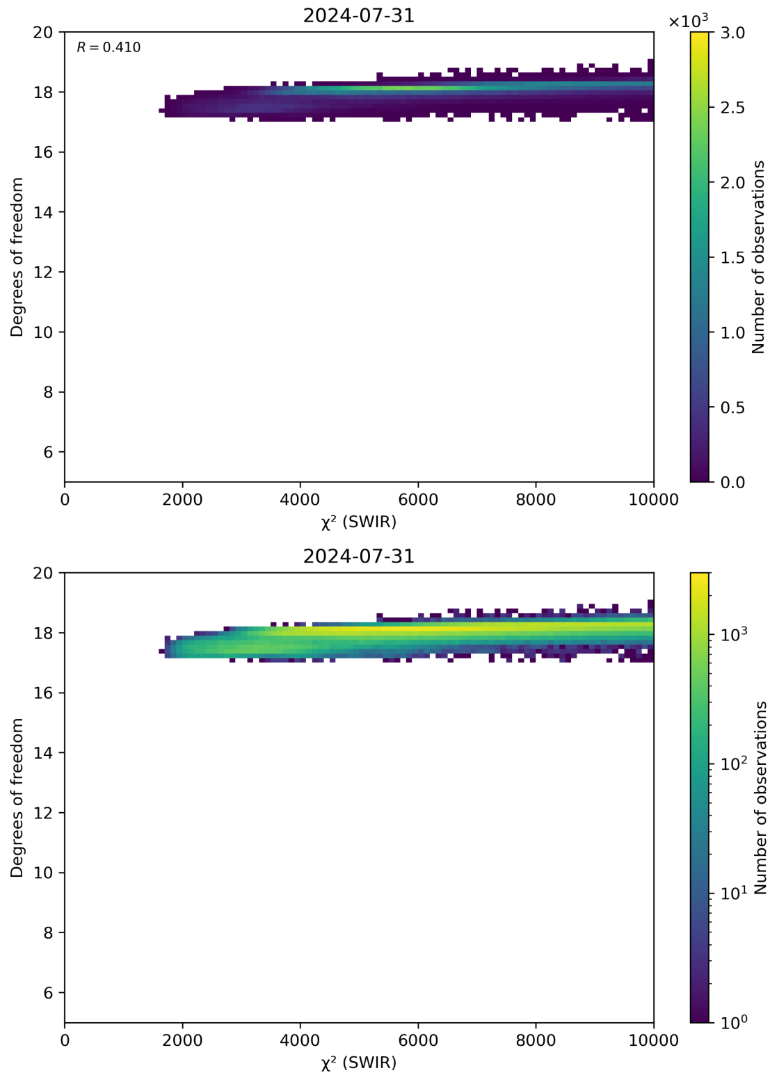
Figure 48: Scatter density plot of “ \chi^2 (SWIR)” against “Degrees of freedom” for 2024-07-31 to 2024-08-01.
