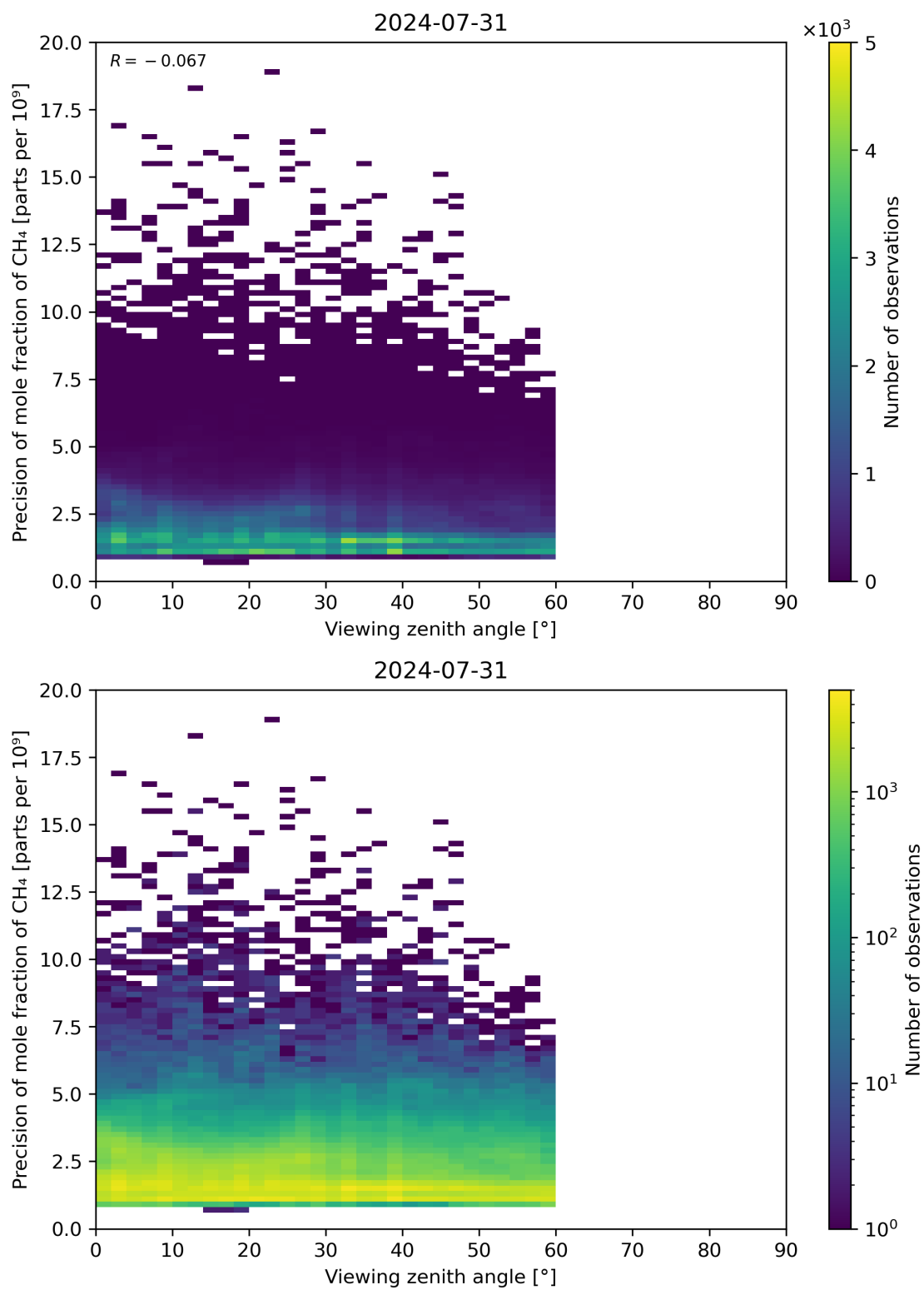
Figure 112: Scatter density plot of “Viewing zenith angle” against “Precision of mole fraction of CH 4 ” for 2024-07-31 to 2024-08-01.
