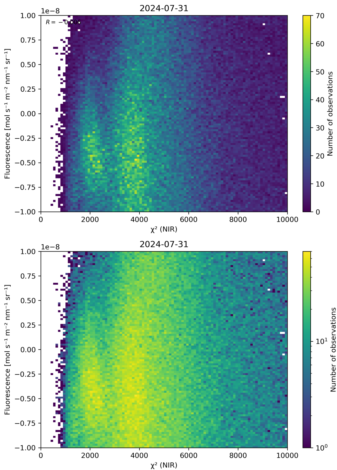
Figure 45: Scatter density plot of “ \chi^2 (NIR)” against “Fluorescence” for 2024-07-31 to 2024-08-01.
