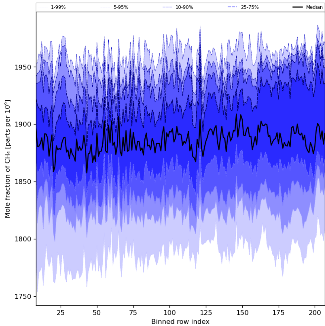
Figure 34: Along track statistics of “Mole fraction of CH 4 ” for 2024-07-31 to 2024-08-01
