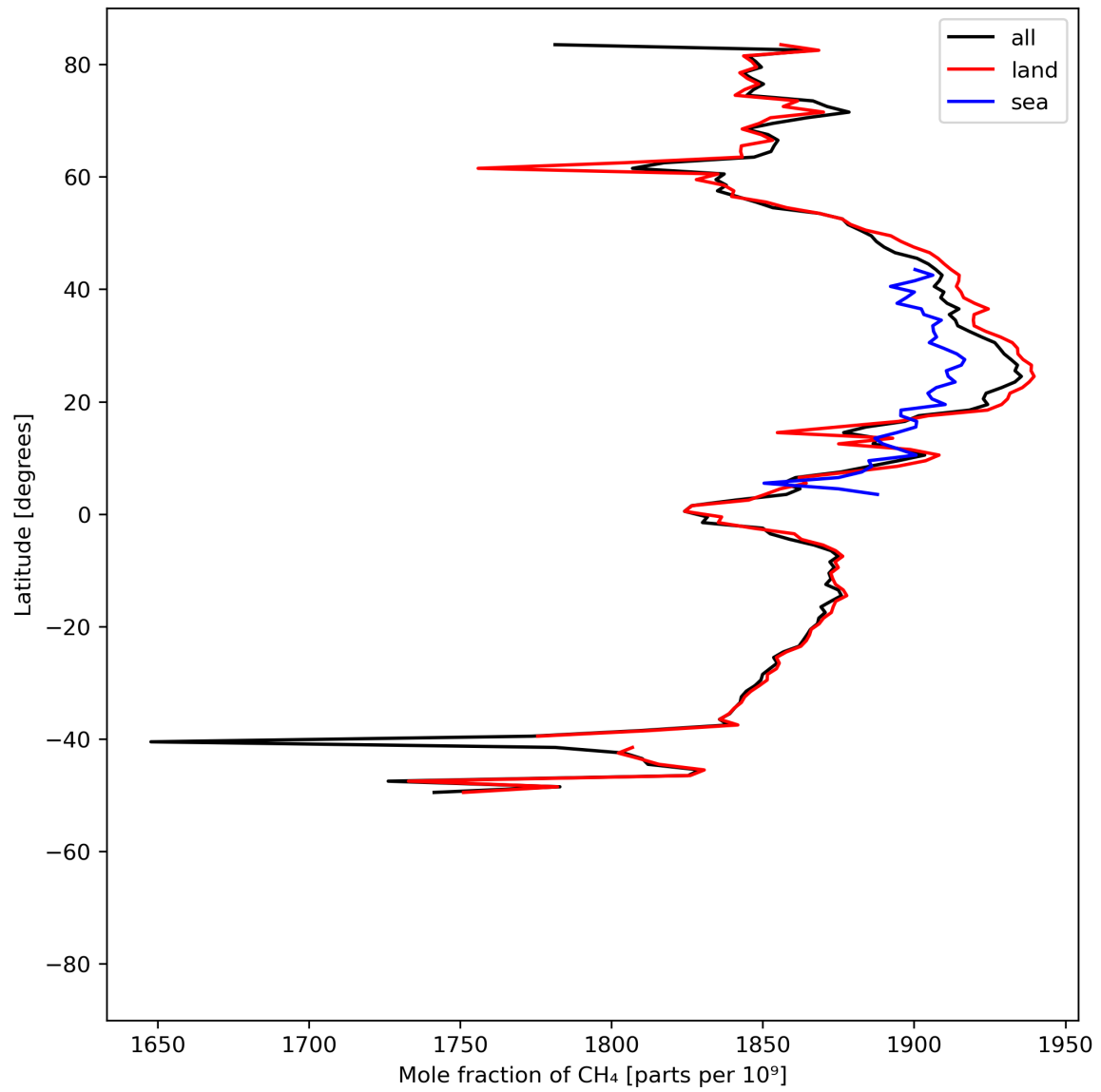
Figure 12: Zonal average of “Mole fraction of \text{CH}_4 ” for 2024-07-31 to 2024-08-02.
