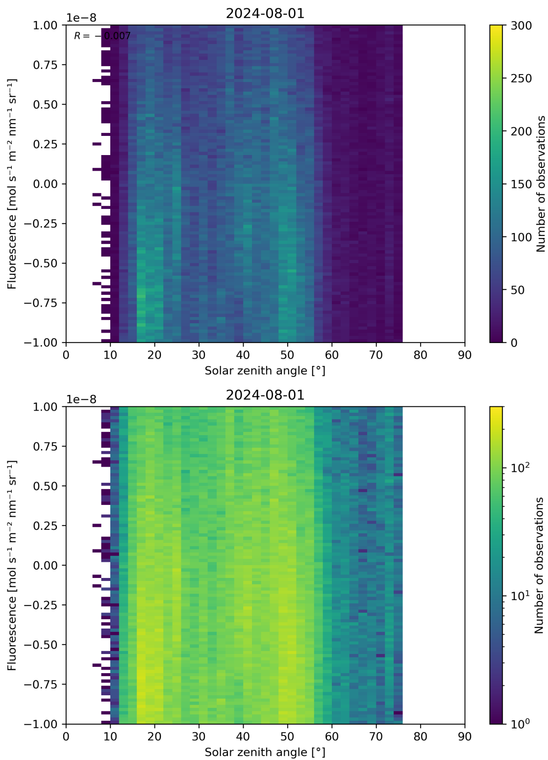
Figure 97: Scatter density plot of “Solar zenith angle” against “Fluorescence” for 2024-07-31 to 2024-08-02.
