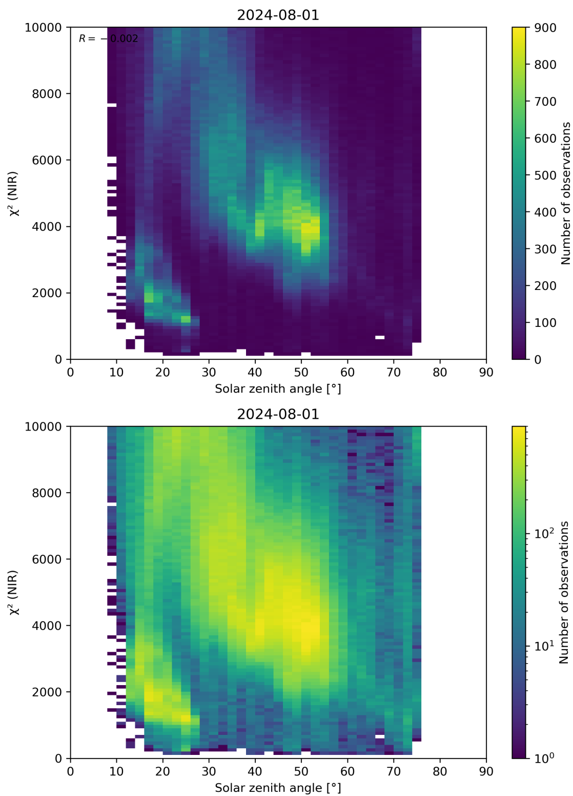
Figure 94: Scatter density plot of “Solar zenith angle” against “ \chi^2 (NIR)” for 2024-07-31 to 2024-08-02.
