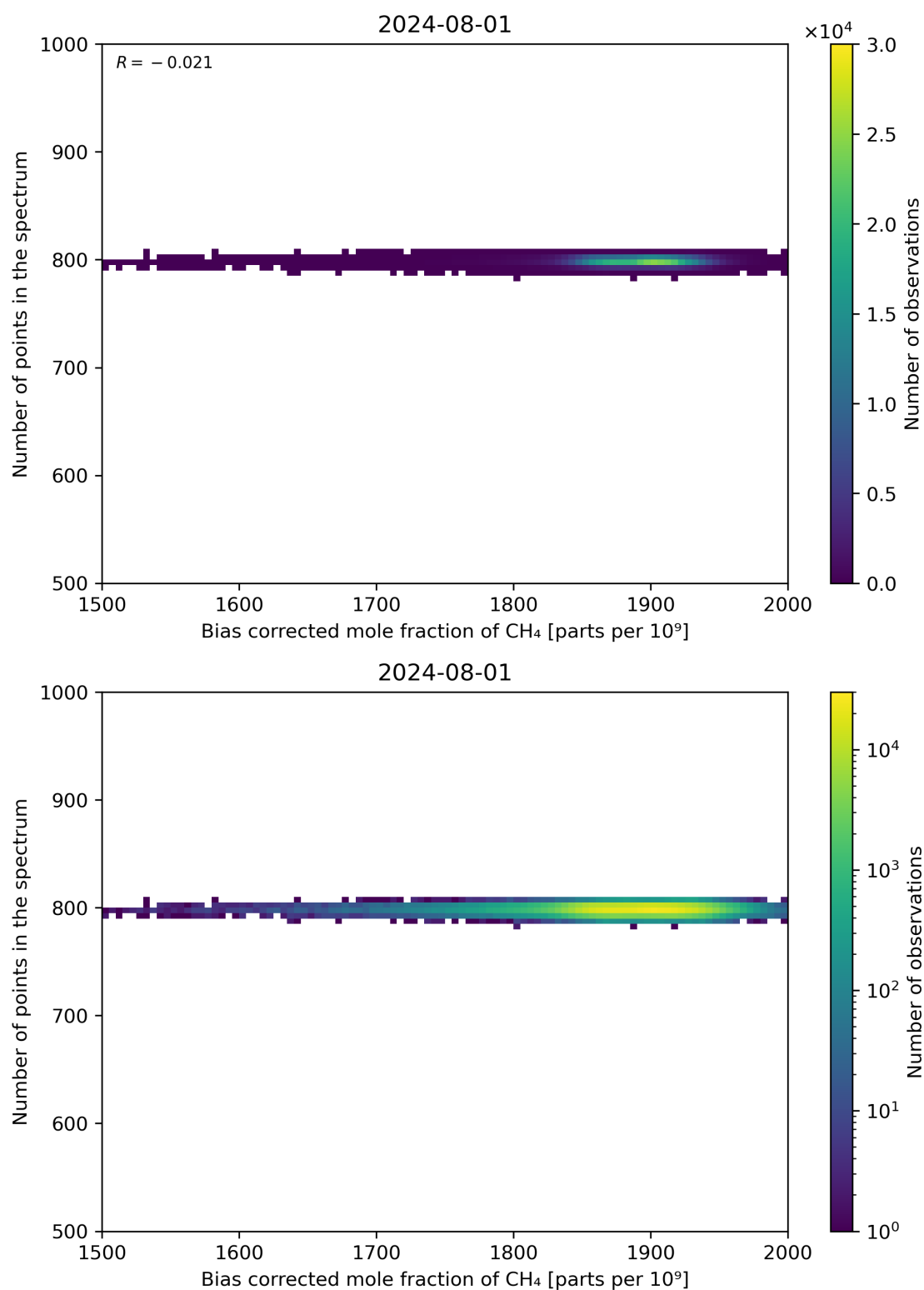
Figure 68: Scatter density plot of “Bias corrected mole fraction of CH 4 ” against “Number of points in the spectrum” for 2024-07-31 to 2024-08-02.
