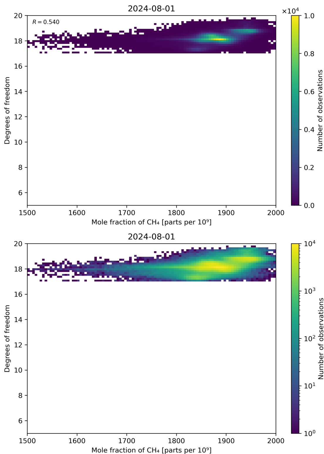
Figure 72: Scatter density plot of “Mole fraction of CH 4 ” against “Degrees of freedom” for 2024-07-31 to 2024-08-02.
