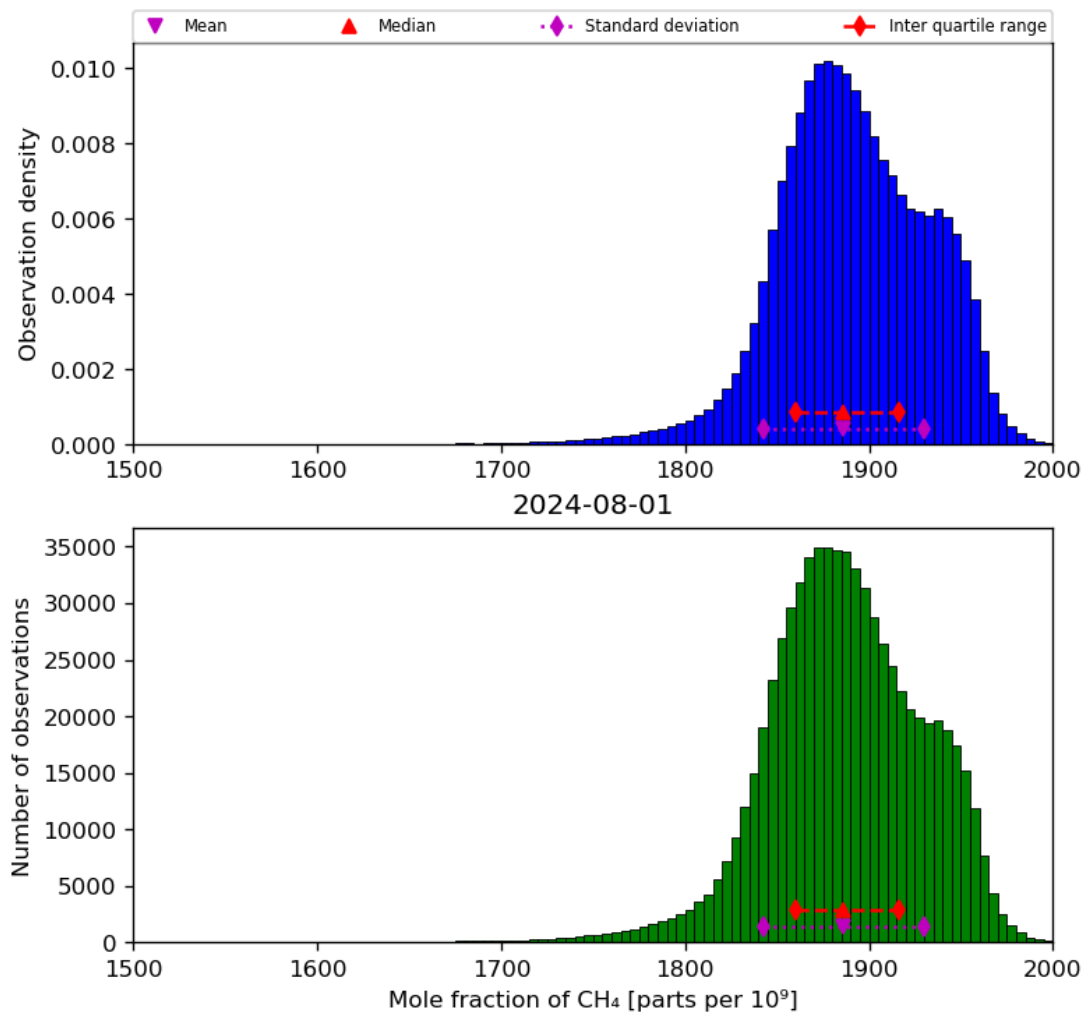
Figure 23: Histogram of “Mole fraction of CH 4 ” for 2024-07-31 to 2024-08-02
