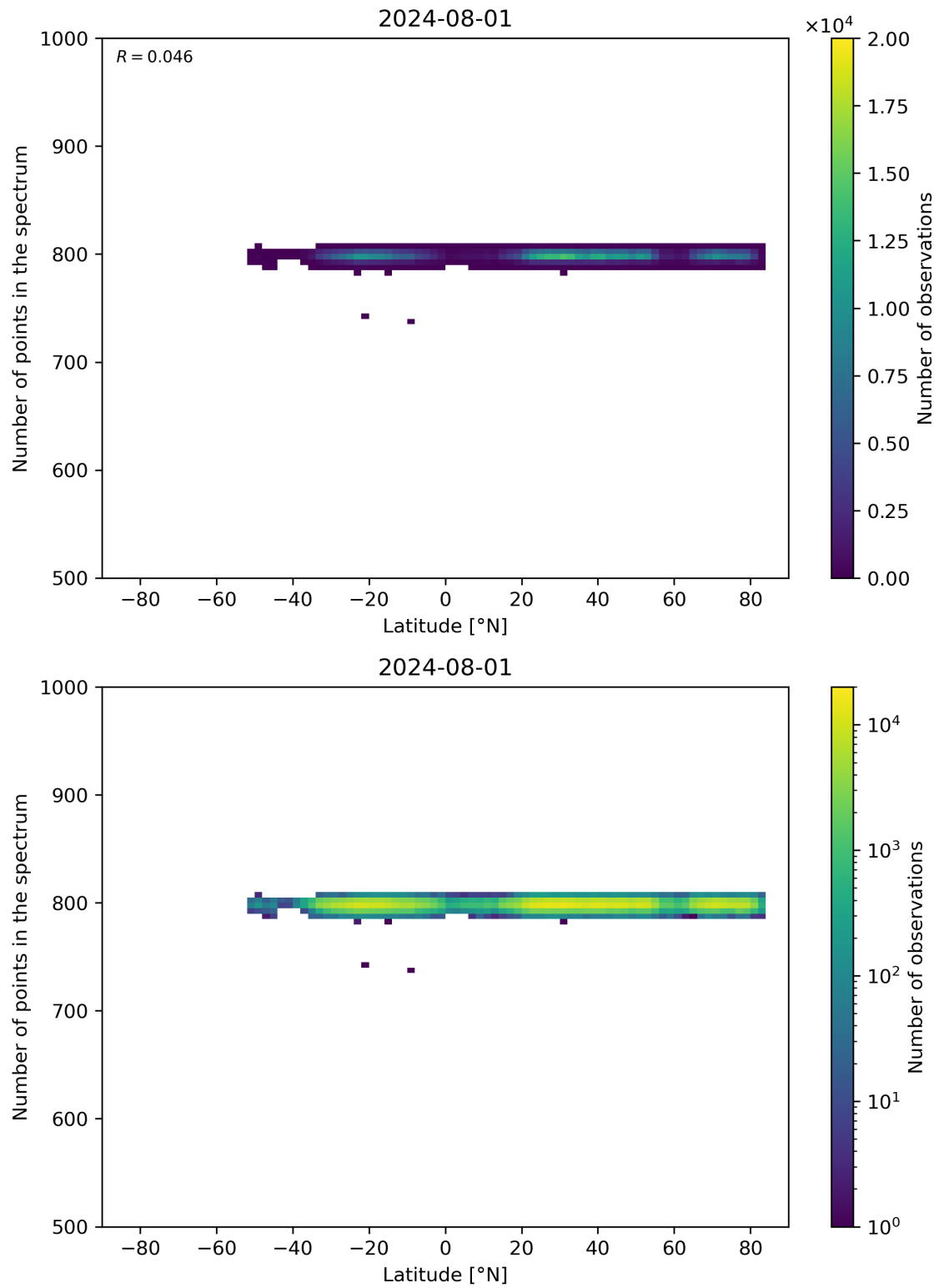
Figure 61: Scatter density plot of “Latitude” against “Number of points in the spectrum” for 2024-07-31 to 2024-08-02.
