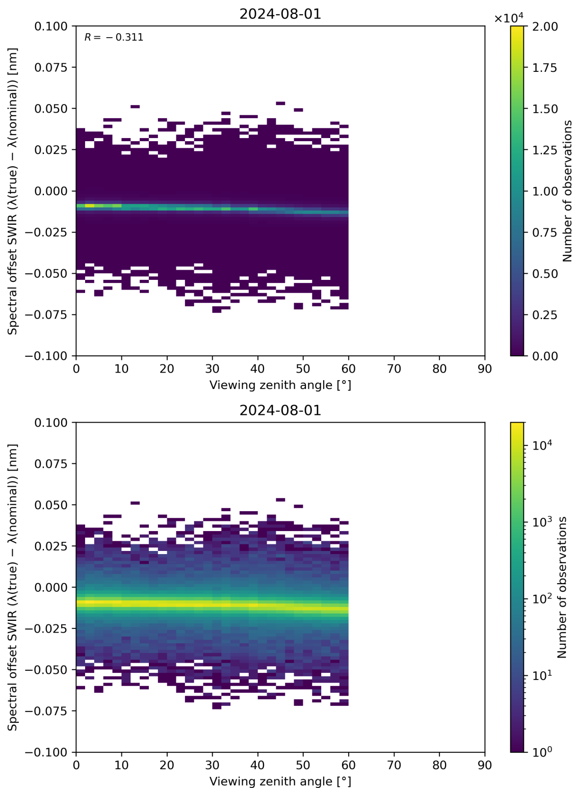
Figure 116: Scatter density plot of “Viewing zenith angle” against “Spectral offset SWIR ( \lambda(\text{true}) - \lambda(\text{nominal}) )” for 2024-07-31 to 2024-08-02.
