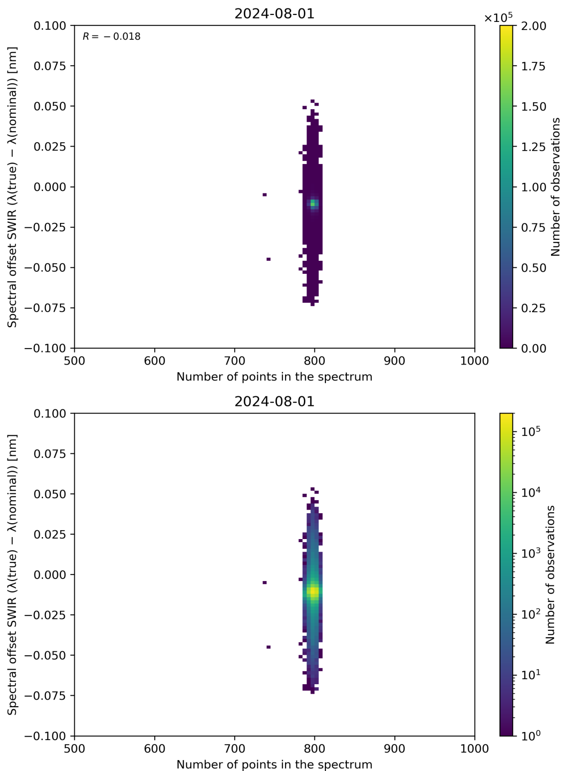
Figure 93: Scatter density plot of “Number of points in the spectrum” against “Spectral offset SWIR ( \lambda(\text{true}) - \lambda(\text{nominal}) )” for 2024-07-31 to 2024-08-02.
