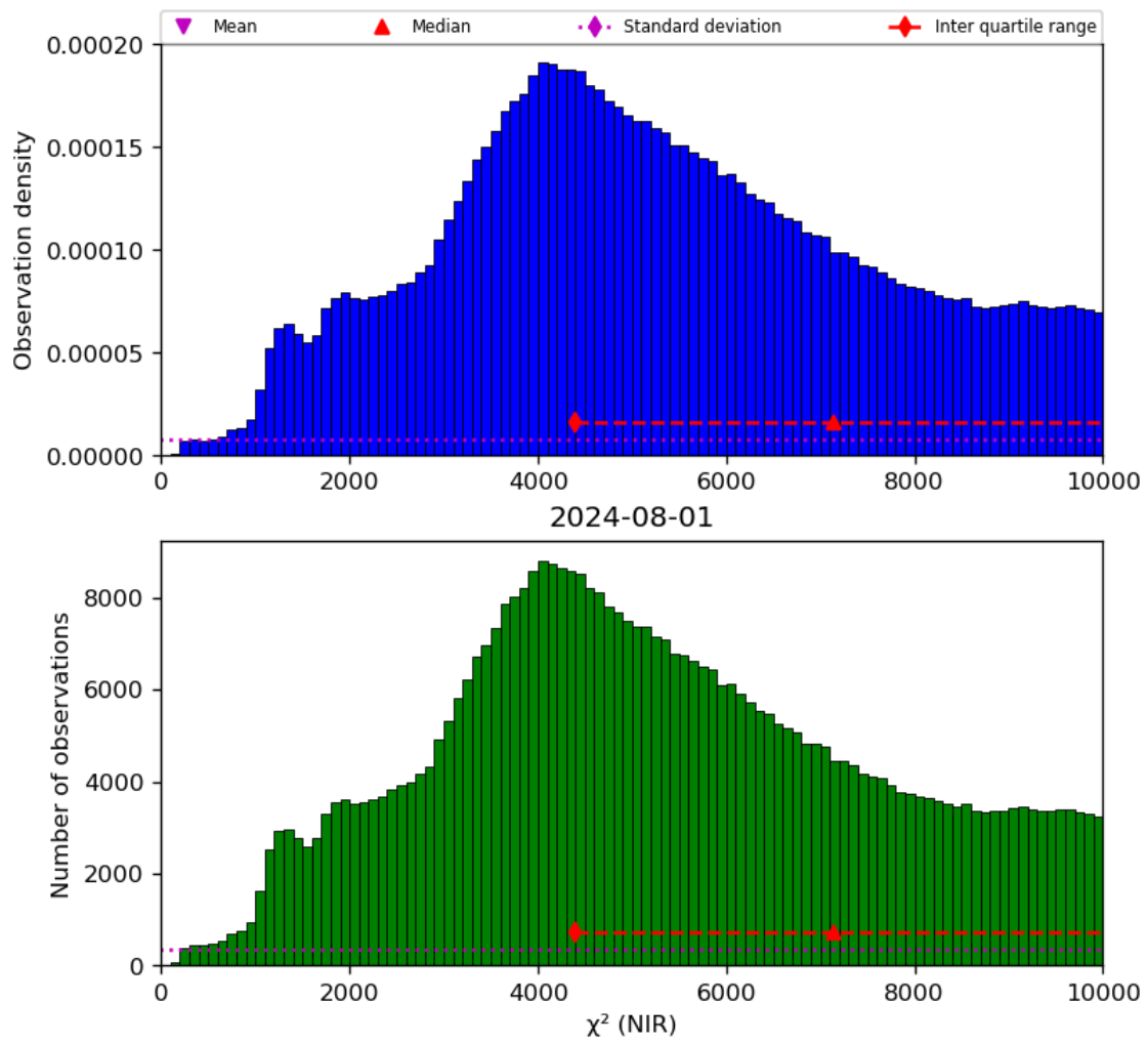
Figure 29: Histogram of “ \chi^2 (NIR)” for 2024-07-31 to 2024-08-02
