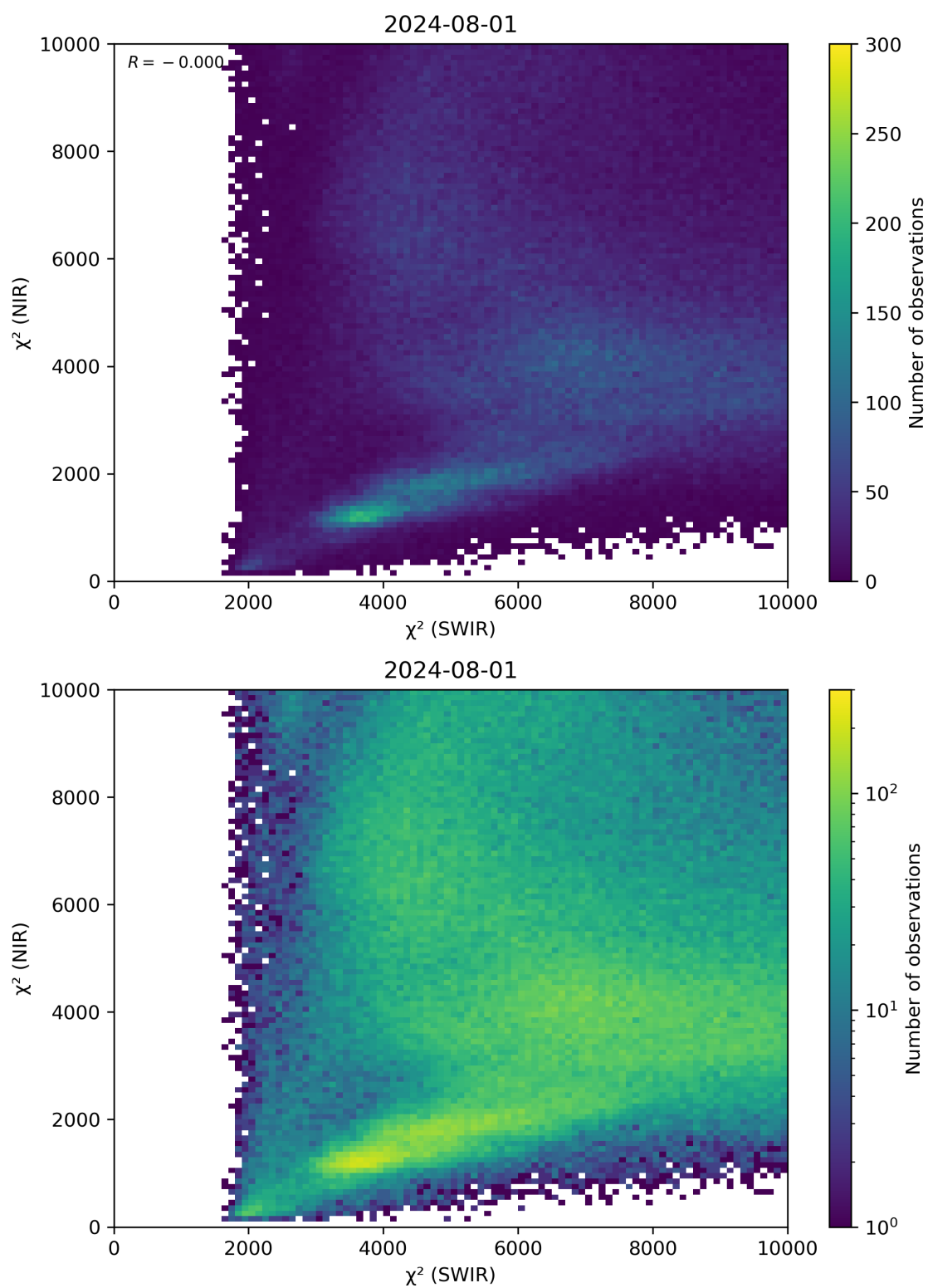
Figure 47: Scatter density plot of “ \chi^2 (SWIR)” against “ \chi^2 (NIR)” for 2024-07-31 to 2024-08-02.
