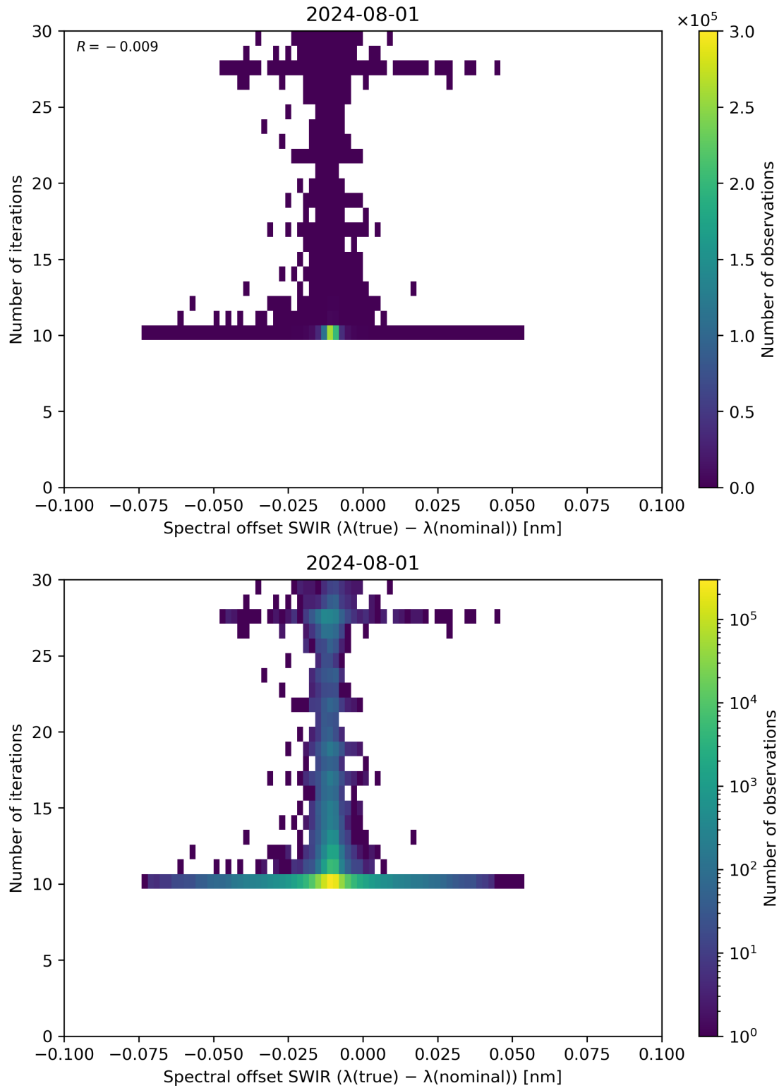
Figure 121: Scatter density plot of “Spectral offset SWIR ( \lambda(\text{true}) - \lambda(\text{nominal}) )” against “Number of iterations” for 2024-07-31 to 2024-08-02.
