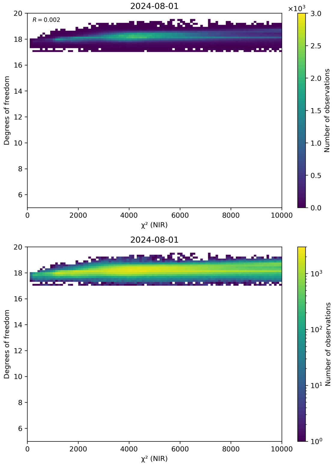
Figure 44: Scatter density plot of “ \chi^2 (NIR)” against “Degrees of freedom” for 2024-07-31 to 2024-08-02.
