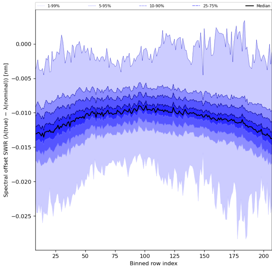
Figure 38: Along track statistics of “Spectral offset SWIR ( \lambda(\text{true}) - \lambda(\text{nominal}) )” for 2024-07-31 to 2024-08-02
