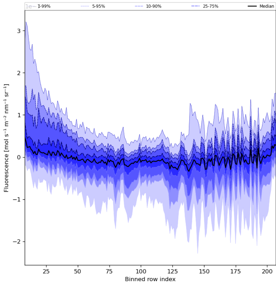
Figure 43: Along track statistics of “Fluorescence” for 2024-07-31 to 2024-08-02
