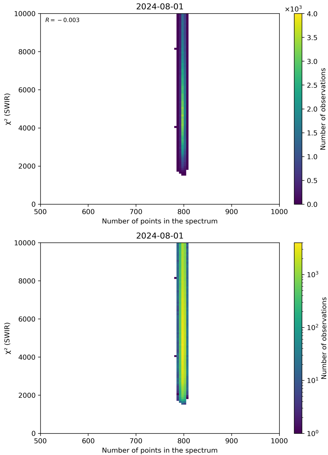
Figure 89: Scatter density plot of “Number of points in the spectrum” against “ \chi^2 (SWIR)” for 2024-07-31 to 2024-08-02.
