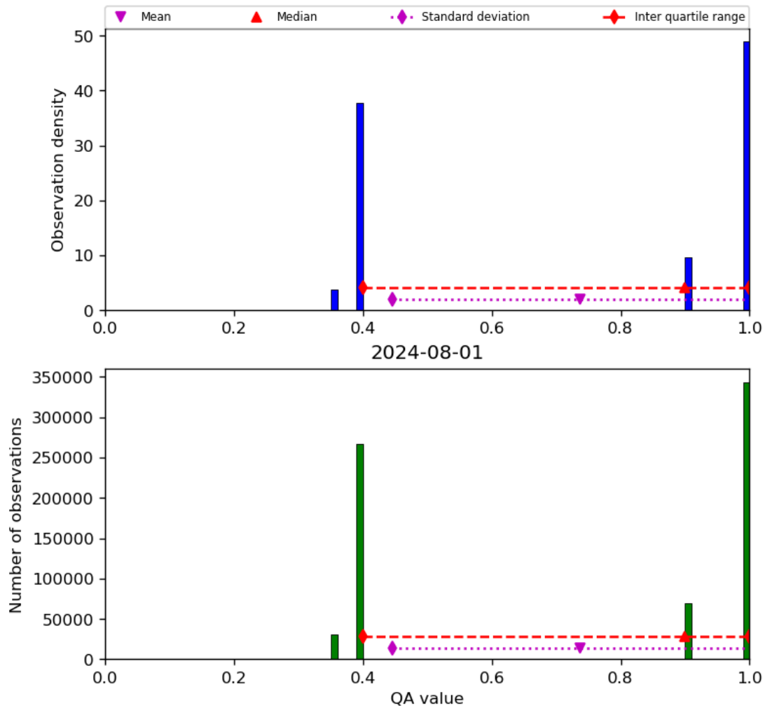
Figure 22: Histogram of “QA value” for 2024-07-31 to 2024-08-02
