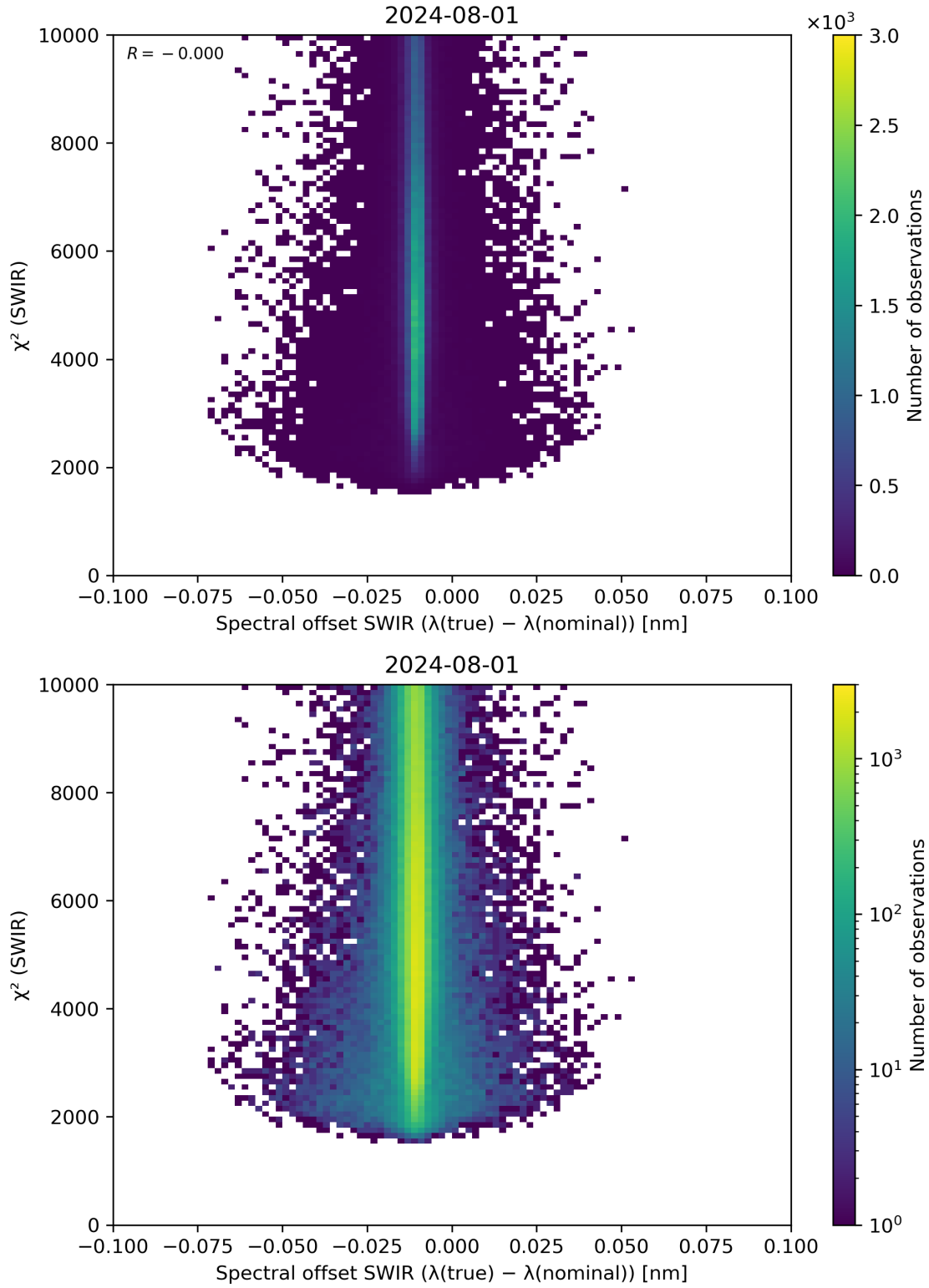
Figure 118: Scatter density plot of “Spectral offset SWIR ( \lambda(\text{true}) - \lambda(\text{nominal}) )” against “ \chi^2 (SWIR)” for 2024-07-31 to 2024-08-02.
