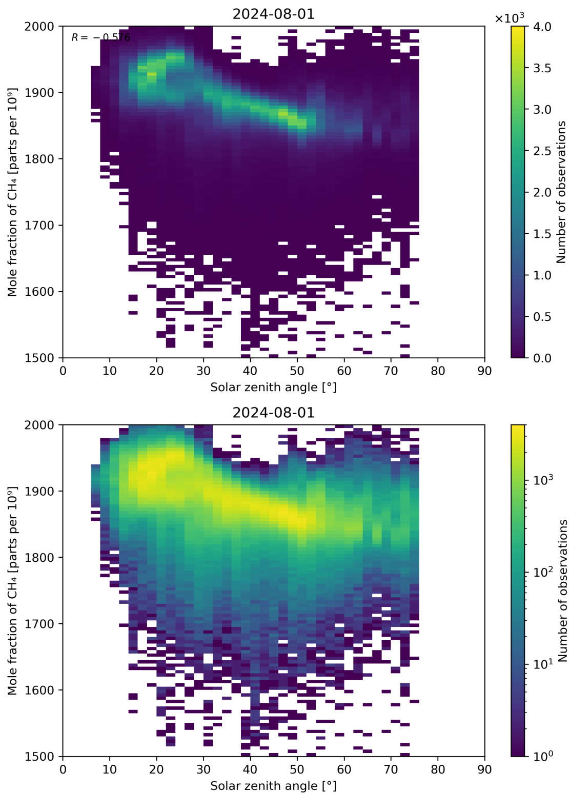
Figure 99: Scatter density plot of “Solar zenith angle” against “Mole fraction of CH 4 ” for 2024-07-31 to 2024-08-02.
