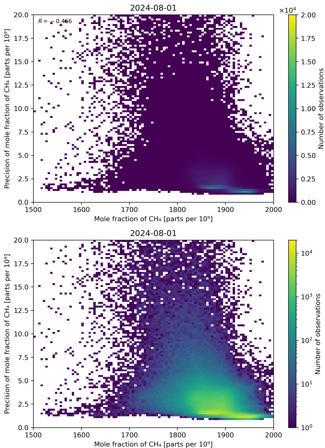
Figure 75: Scatter density plot of “Mole fraction of CH 4 ” against “Precision of mole fraction of CH 4 ” for 2024-07-31 to 2024-08-02.
