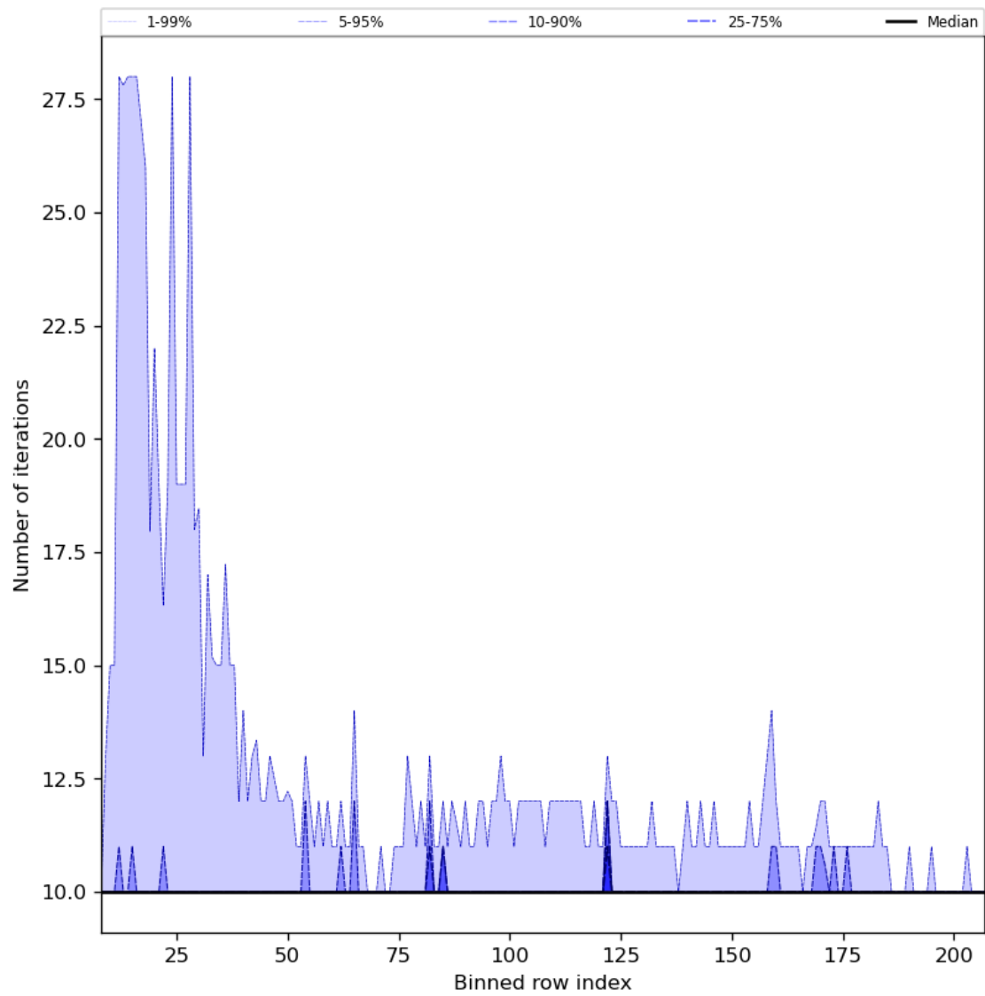
Figure 42: Along track statistics of “Number of iterations” for 2024-07-31 to 2024-08-02
