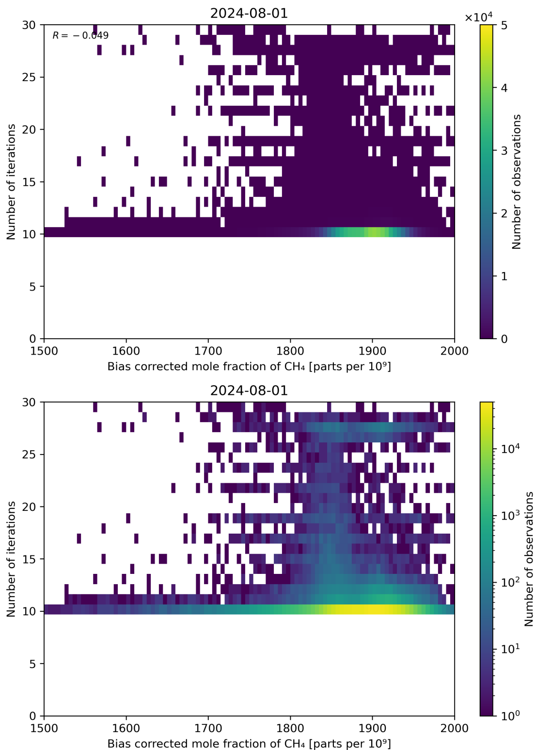
Figure 67: Scatter density plot of “Bias corrected mole fraction of CH 4 ” against “Number of iterations” for 2024-07-31 to 2024-08-02.
