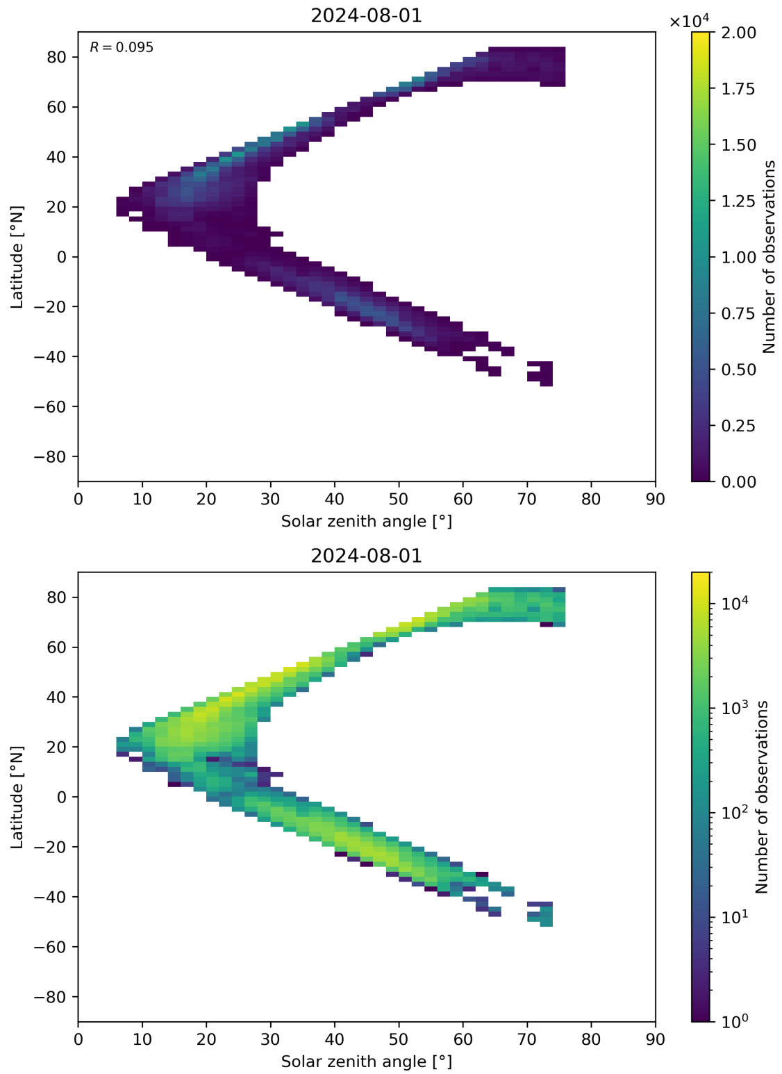
Figure 98: Scatter density plot of “Solar zenith angle” against “Latitude” for 2024-07-31 to 2024-08-02.
