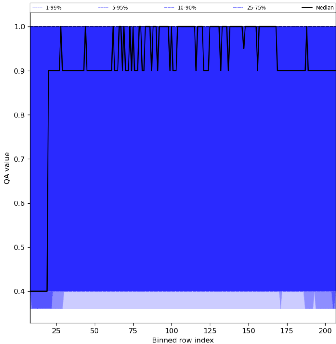
Figure 33: Along track statistics of “QA value” for 2024-07-31 to 2024-08-02
