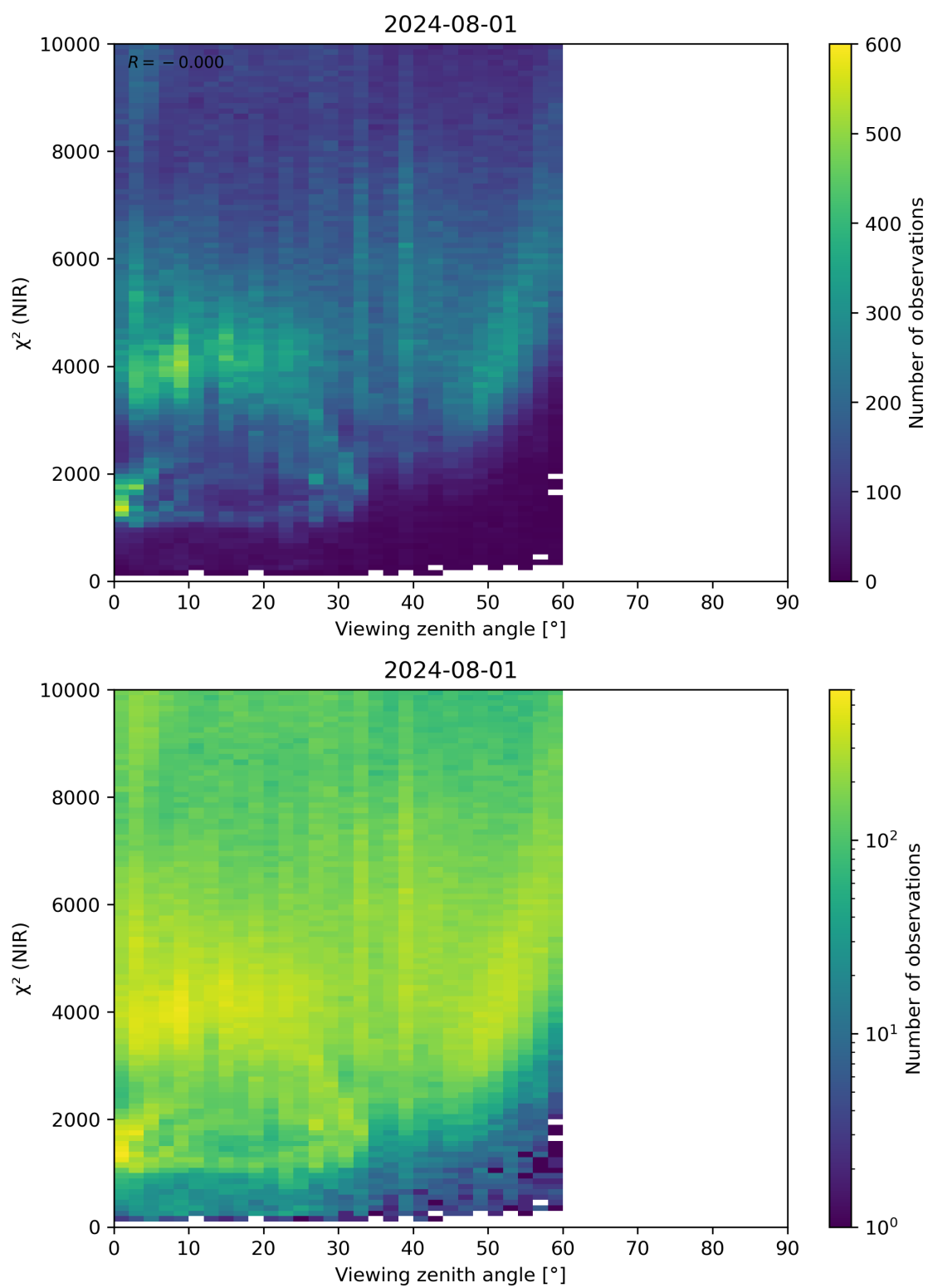
Figure 105: Scatter density plot of “Viewing zenith angle” against “ \chi^2 (NIR)” for 2024-07-31 to 2024-08-02.
