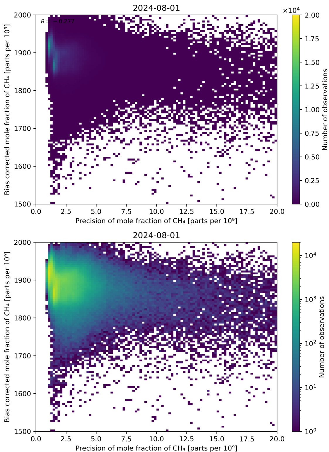
Figure 82: Scatter density plot of “Precision of mole fraction of CH 4 ” against “Bias corrected mole fraction of CH 4 ” for 2024-07-31 to 2024-08-02.
