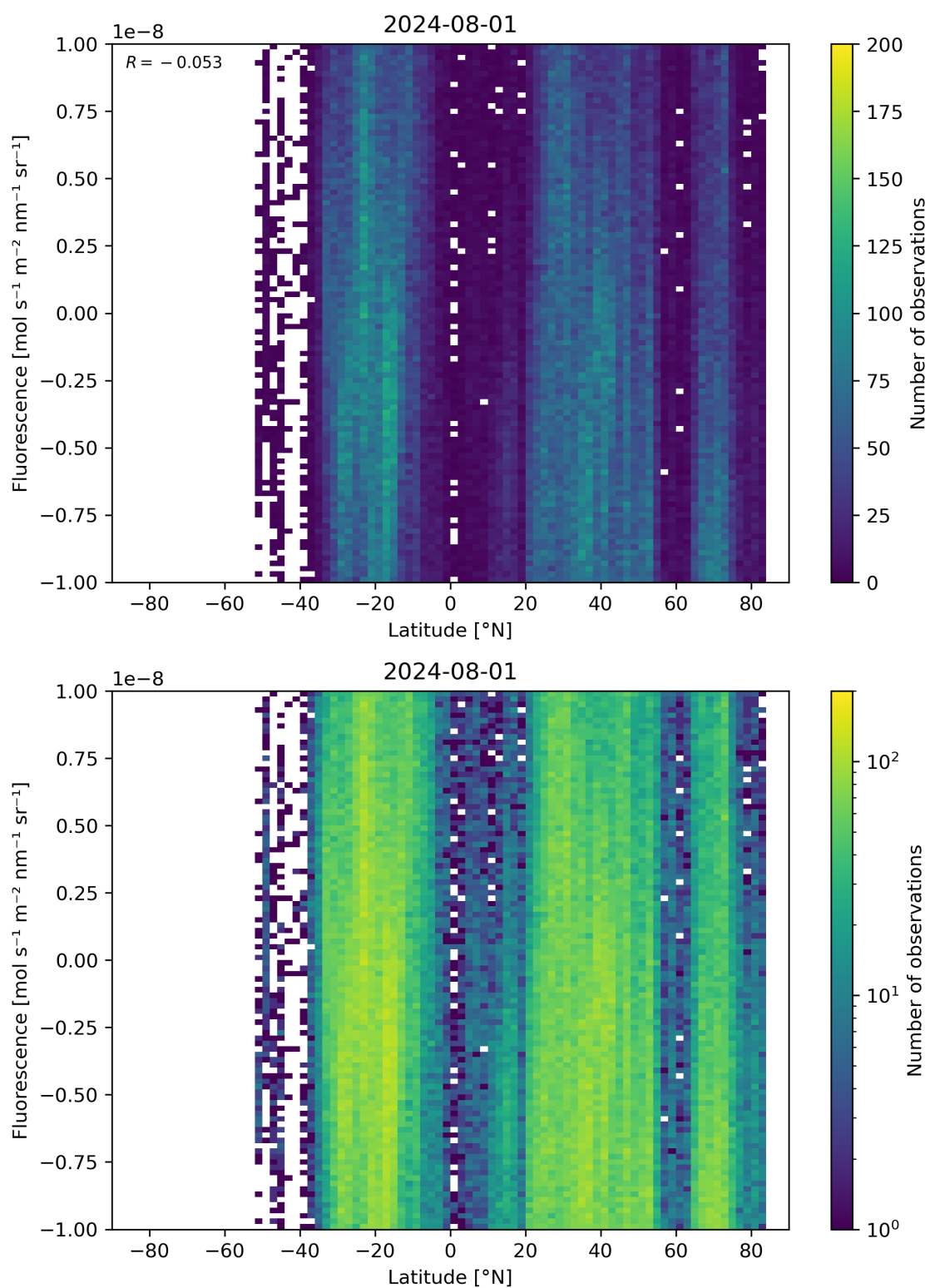
Figure 56: Scatter density plot of “Latitude” against “Fluorescence” for 2024-07-31 to 2024-08-02.
