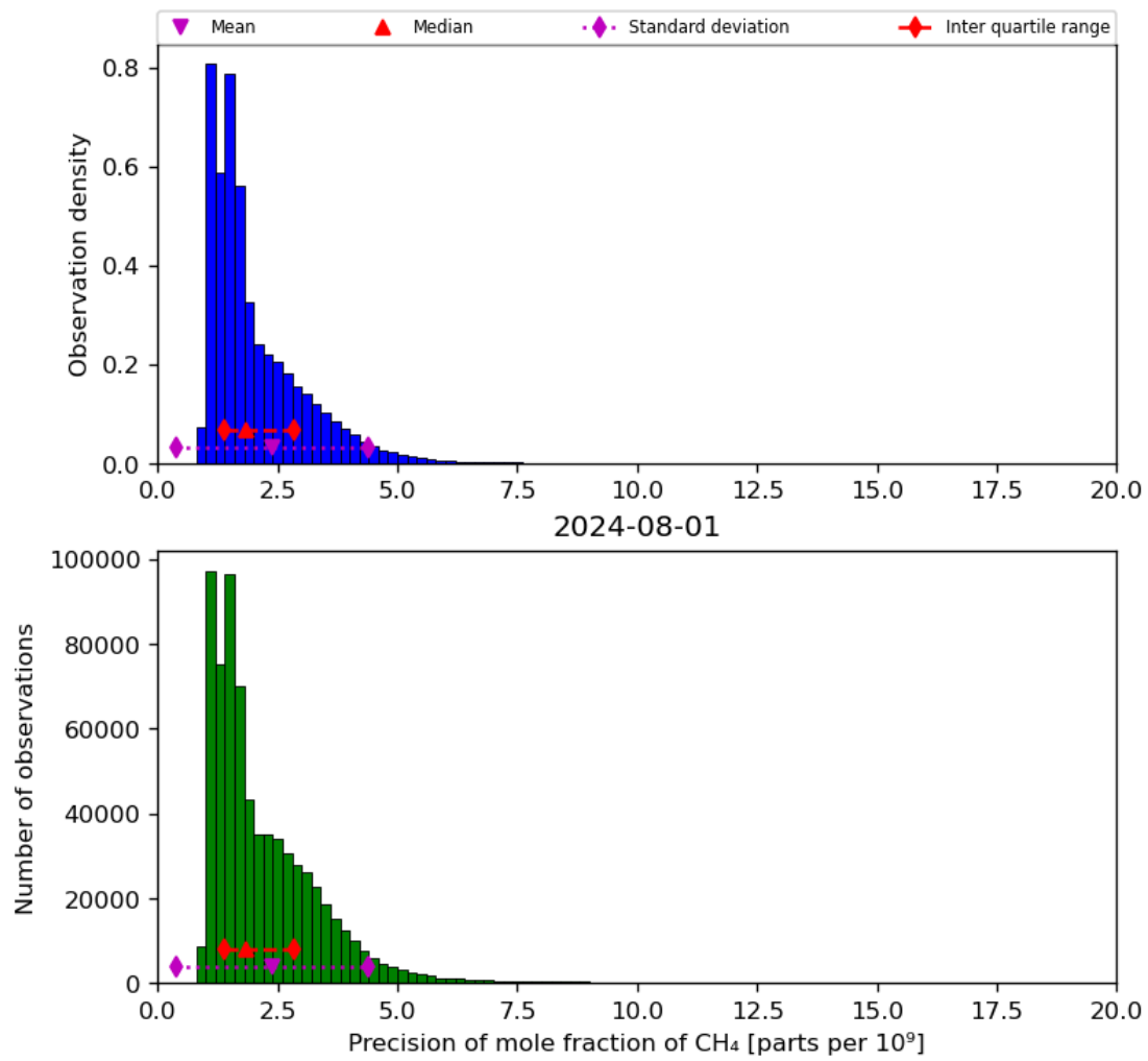
Figure 24: Histogram of “Precision of mole fraction of CH 4 ” for 2024-07-31 to 2024-08-02
