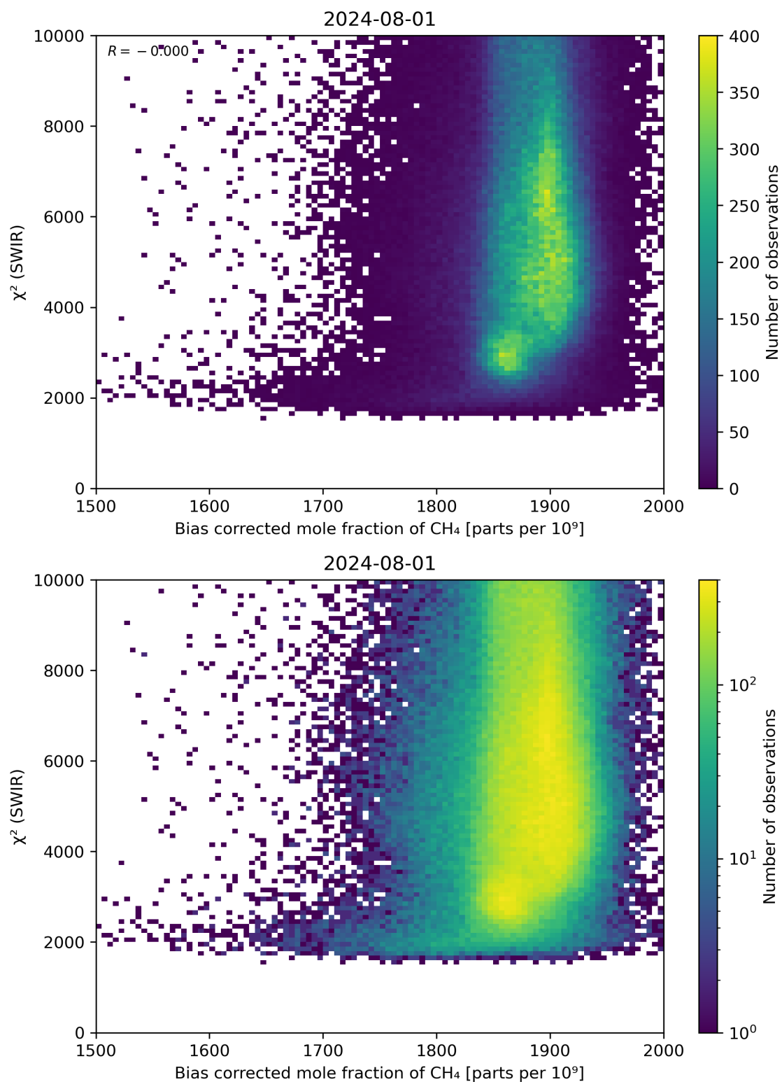
Figure 64: Scatter density plot of “Bias corrected mole fraction of \text{CH}_4 ” against “ \chi^2 (SWIR)” for 2024-07-31 to 2024-08-02.
