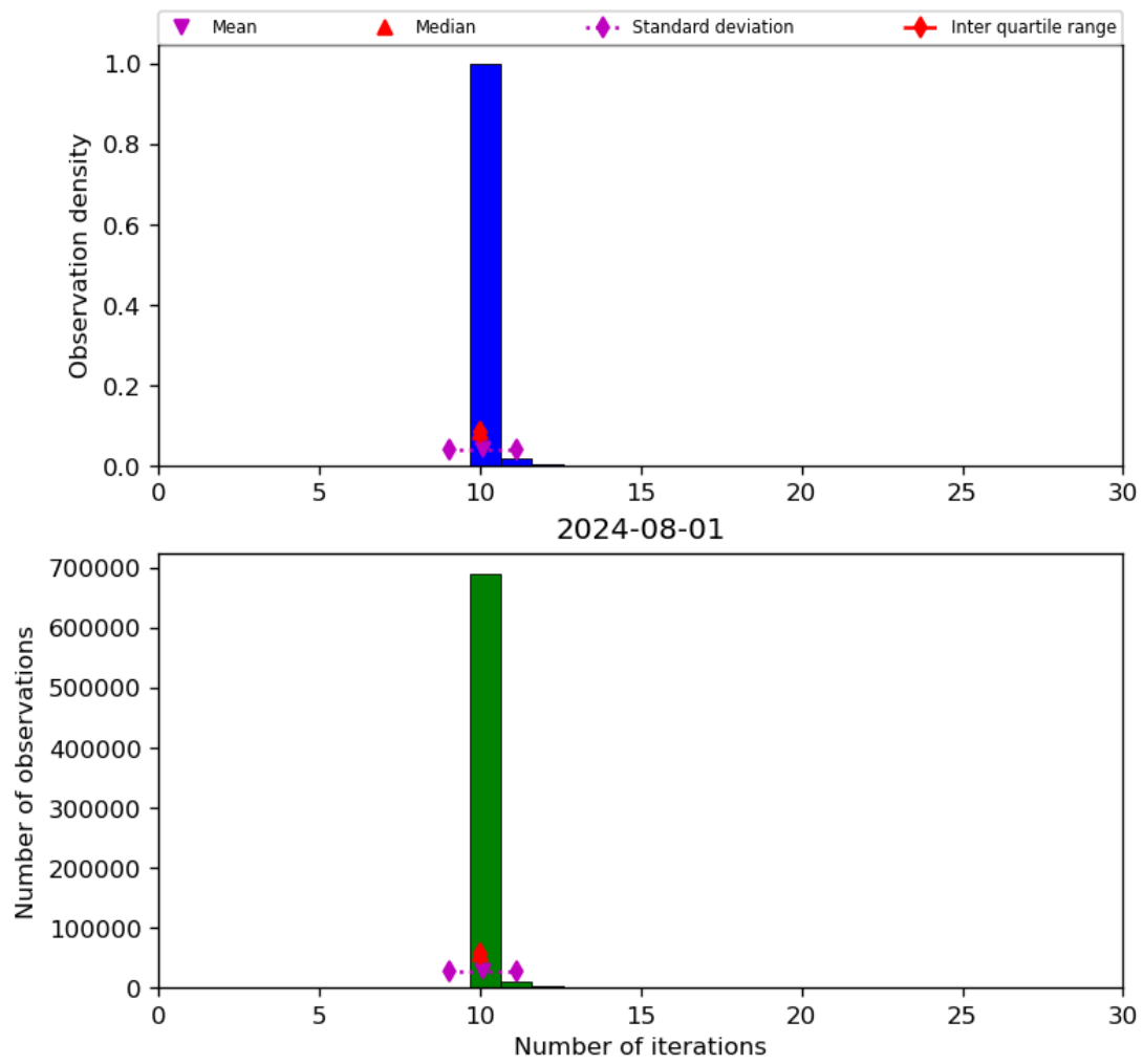
Figure 31: Histogram of “Number of iterations” for 2024-07-31 to 2024-08-02
