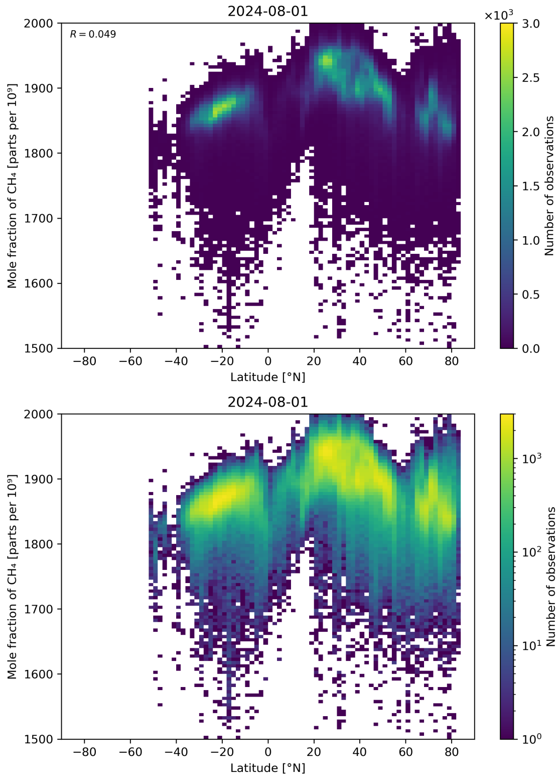
Figure 57: Scatter density plot of “Latitude” against “Mole fraction of CH 4 ” for 2024-07-31 to 2024-08-02.
