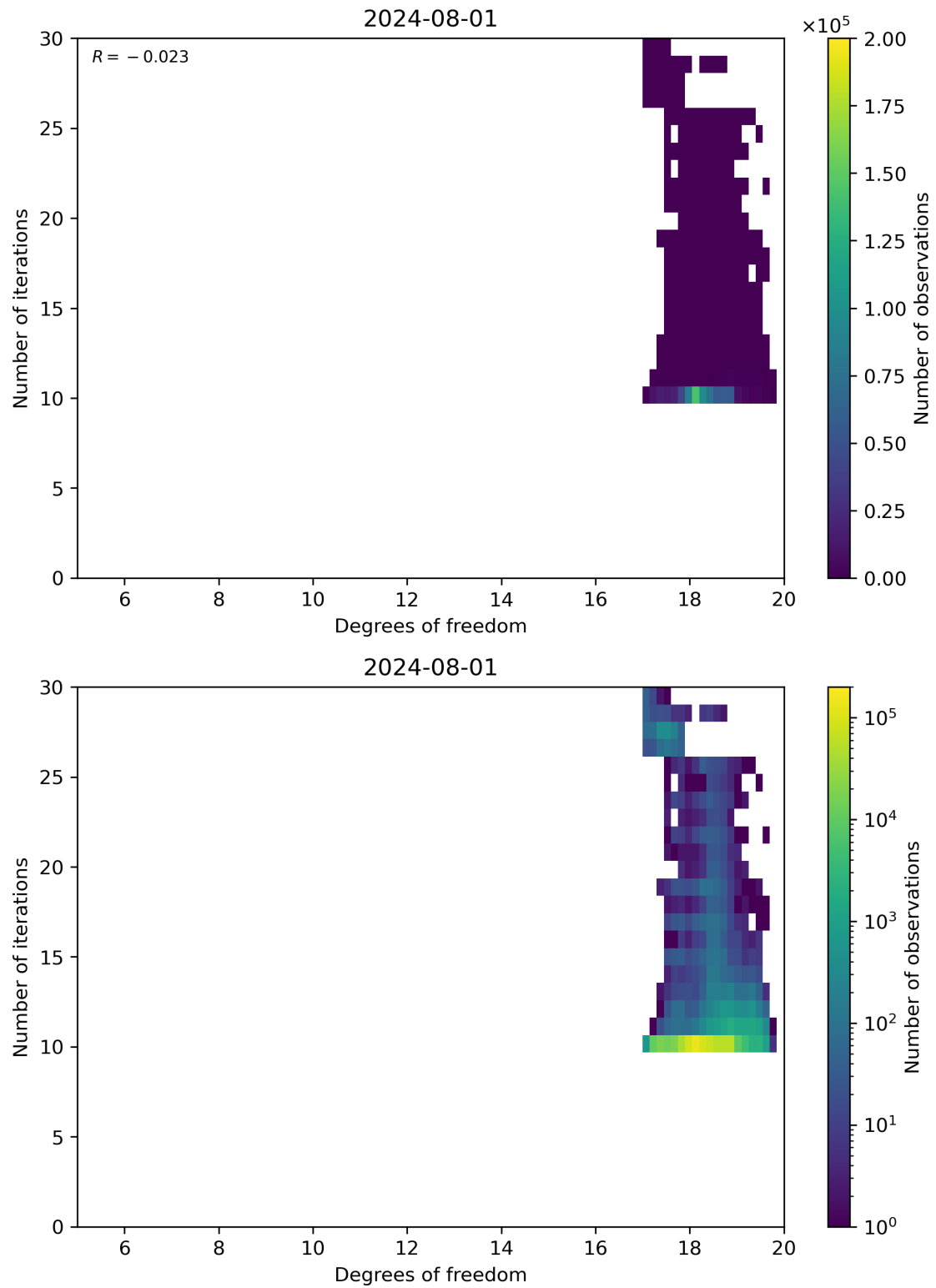
Figure 52: Scatter density plot of “Degrees of freedom” against “Number of iterations” for 2024-07-31 to 2024-08-02.
