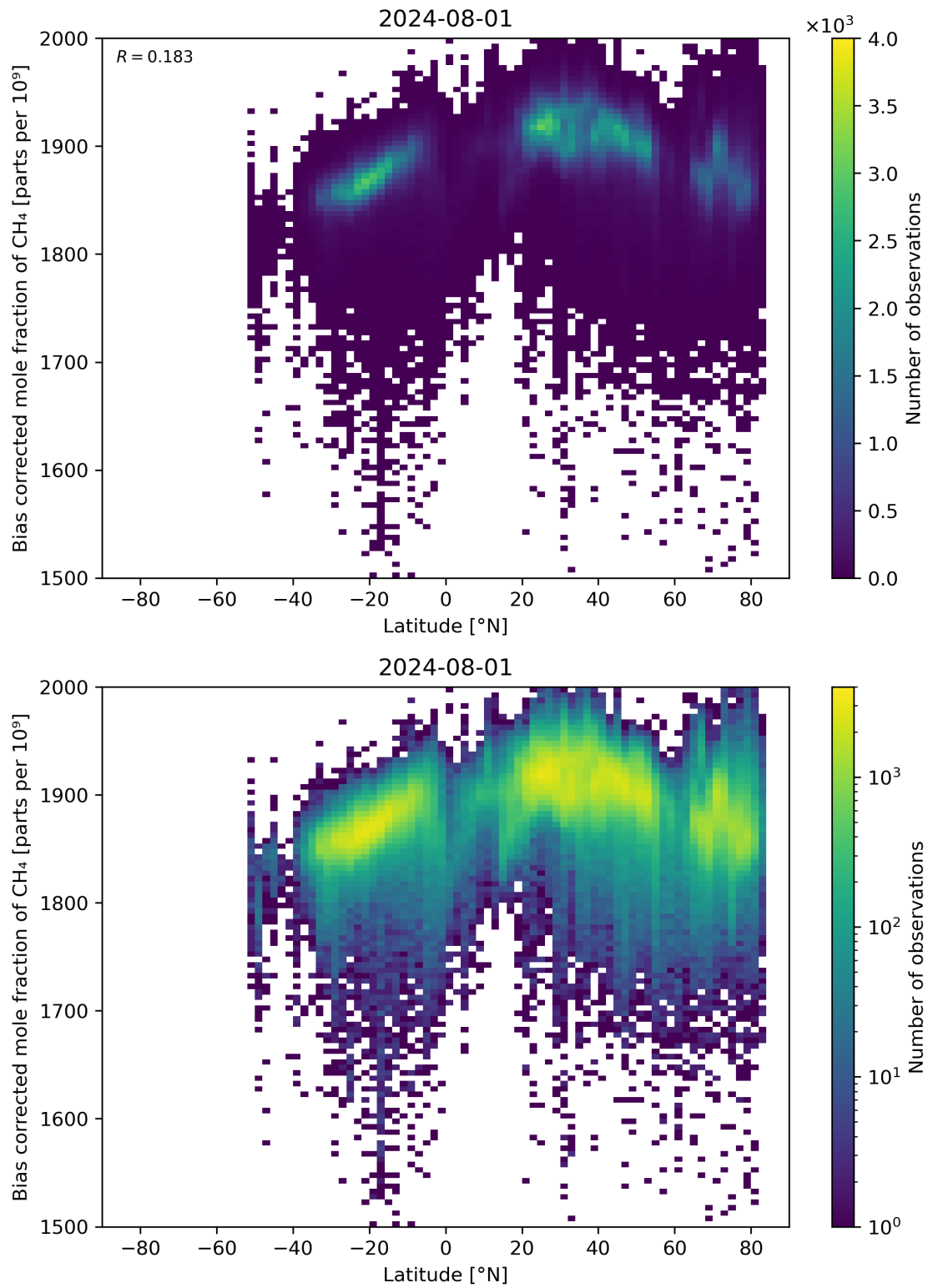
Figure 58: Scatter density plot of “Latitude” against “Bias corrected mole fraction of CH 4 ” for 2024-07-31 to 2024-08-02.
