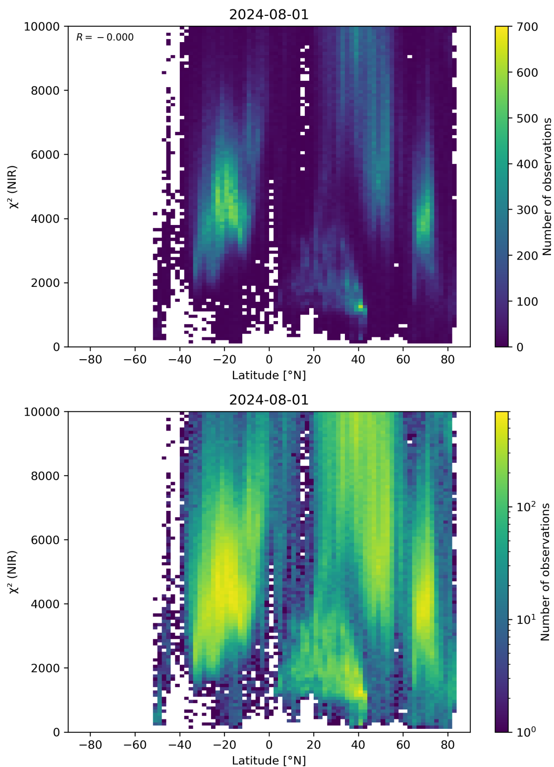
Figure 53: Scatter density plot of “Latitude” against “ \chi^2 (NIR)” for 2024-07-31 to 2024-08-02.
