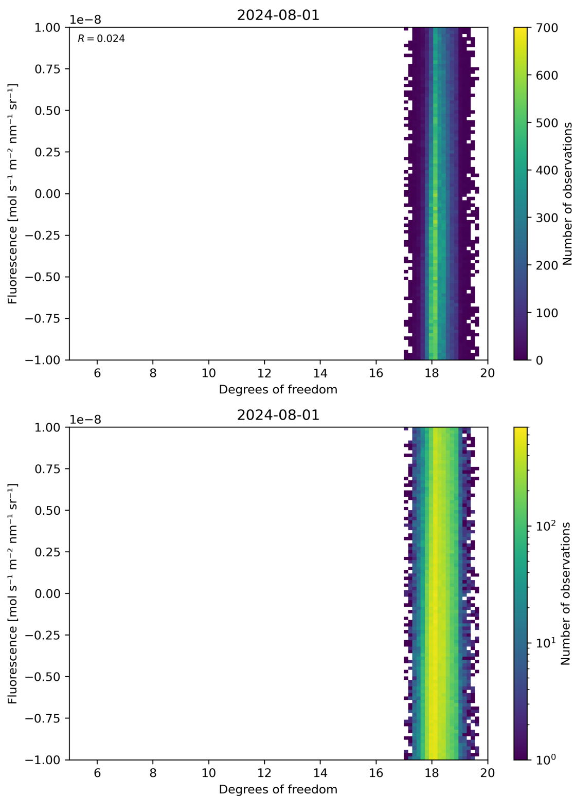
Figure 51: Scatter density plot of “Degrees of freedom” against “Fluorescence” for 2024-07-31 to 2024-08-02.
