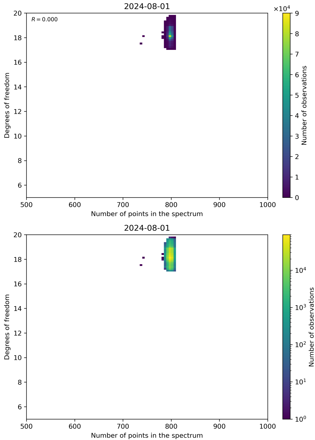
Figure 90: Scatter density plot of “Number of points in the spectrum” against “Degrees of freedom” for 2024-07-31 to 2024-08-02.
