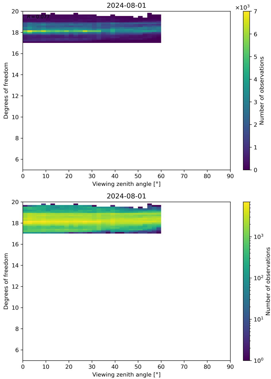
Figure 107: Scatter density plot of “Viewing zenith angle” against “Degrees of freedom” for 2024-07-31 to 2024-08-02.
