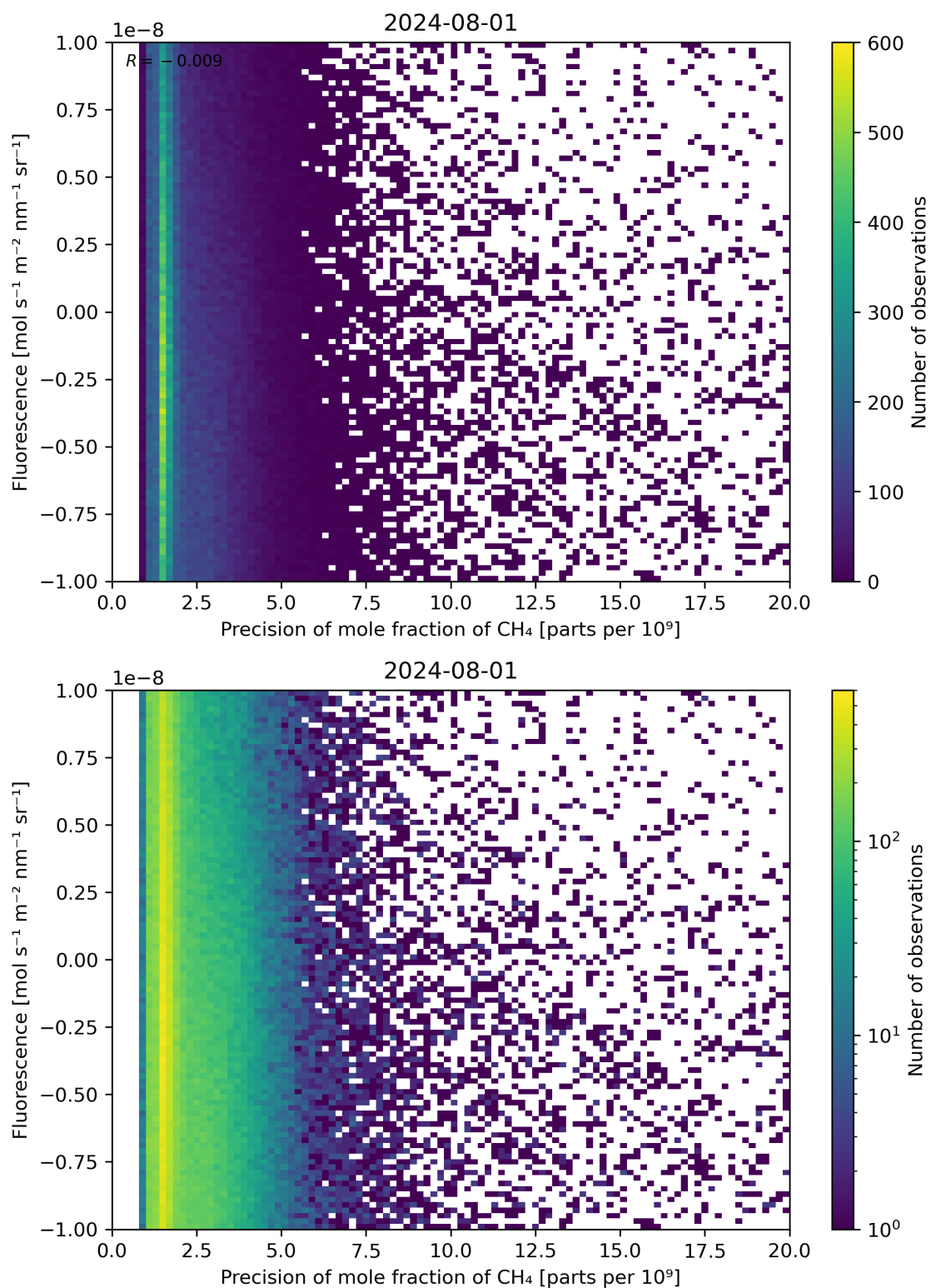
Figure 81: Scatter density plot of “Precision of mole fraction of \text{CH}_4 ” against “Fluorescence” for 2024-07-31 to 2024-08-02.
