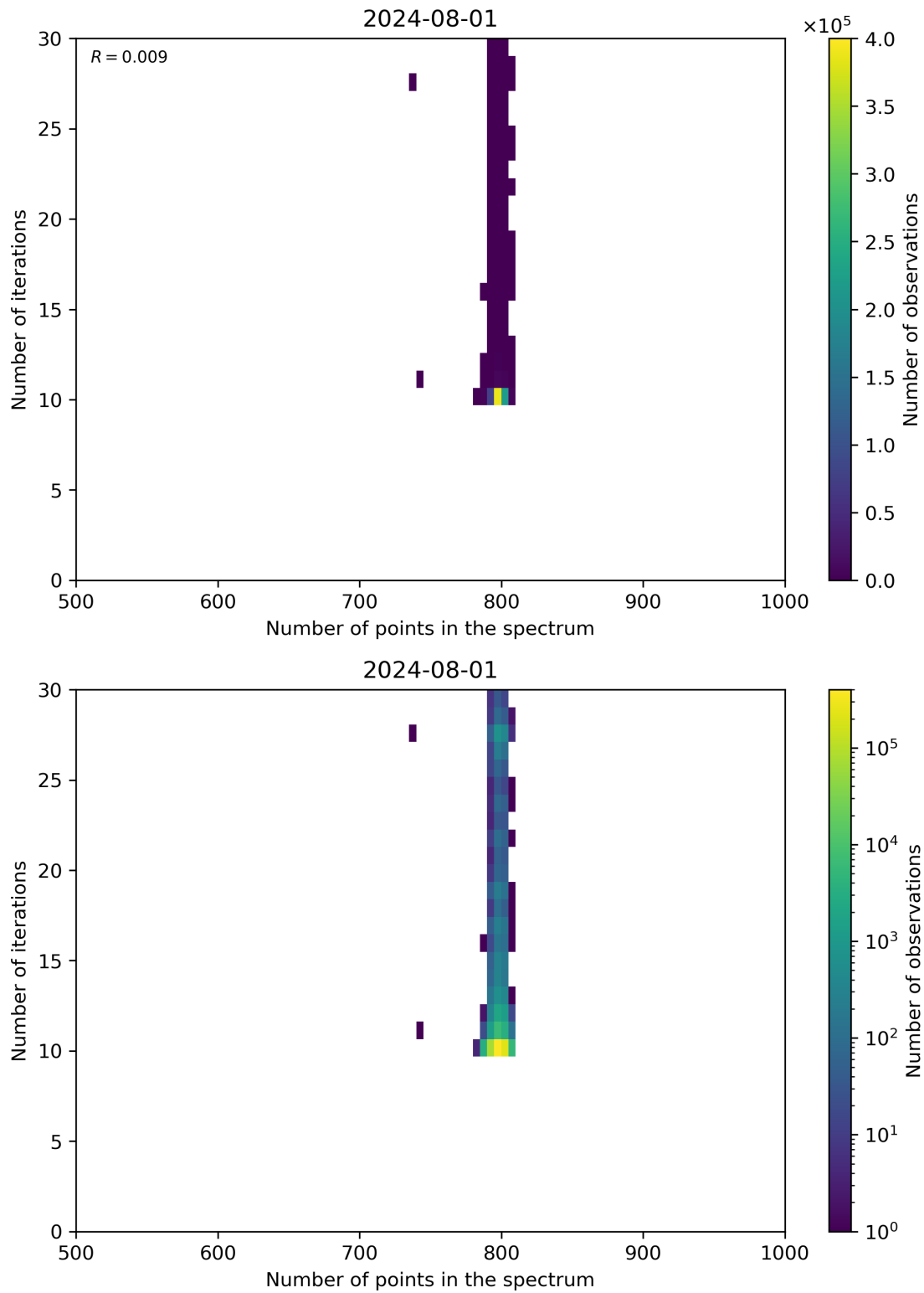
Figure 92: Scatter density plot of “Number of points in the spectrum” against “Number of iterations” for 2024-07-31 to 2024-08-02.
