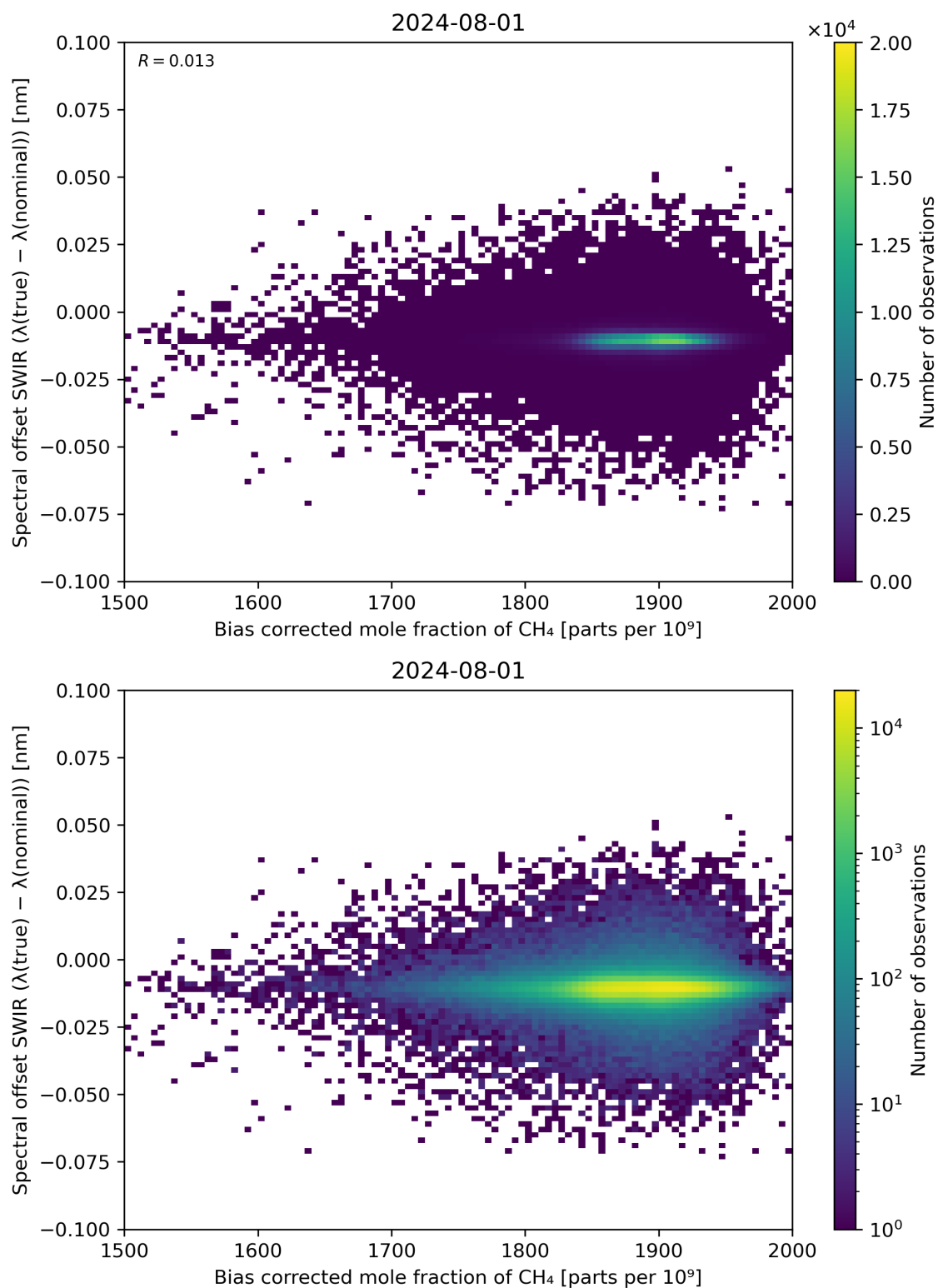
Figure 69: Scatter density plot of “Bias corrected mole fraction of \text{CH}_4 ” against “Spectral offset SWIR ( \lambda(\text{true}) - \lambda(\text{nominal}) )” for 2024-07-31 to 2024-08-02.
