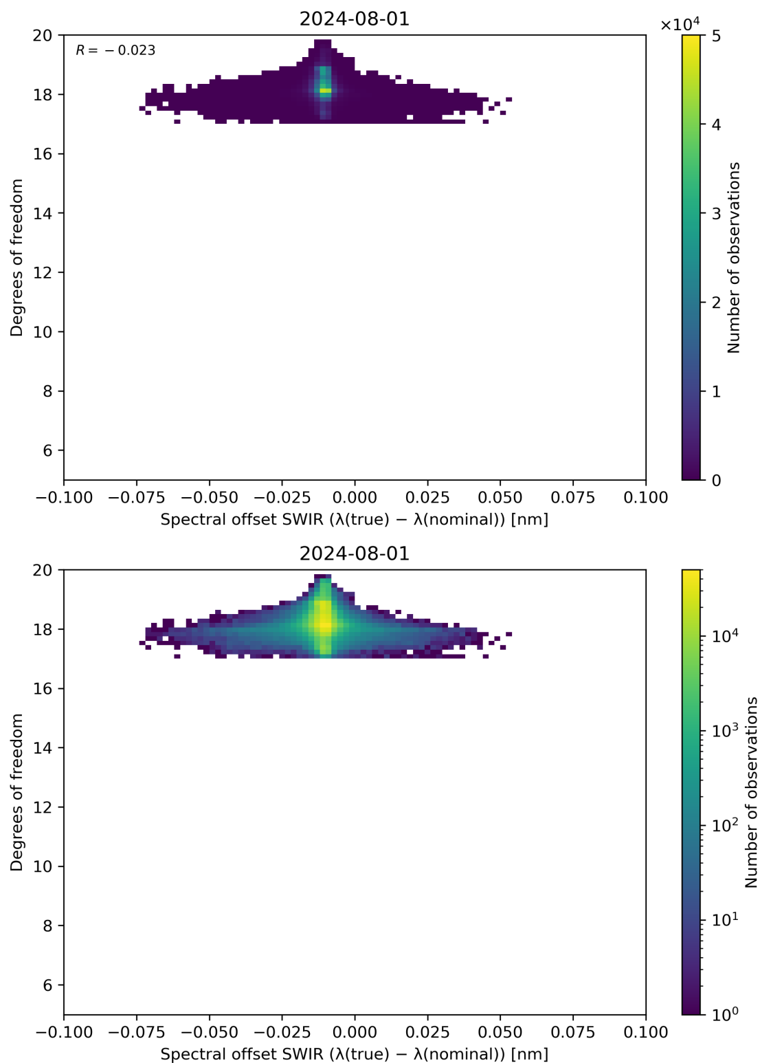
Figure 119: Scatter density plot of “Spectral offset SWIR ( \lambda(\text{true}) - \lambda(\text{nominal}) )” against “Degrees of freedom” for 2024-07-31 to 2024-08-02.
