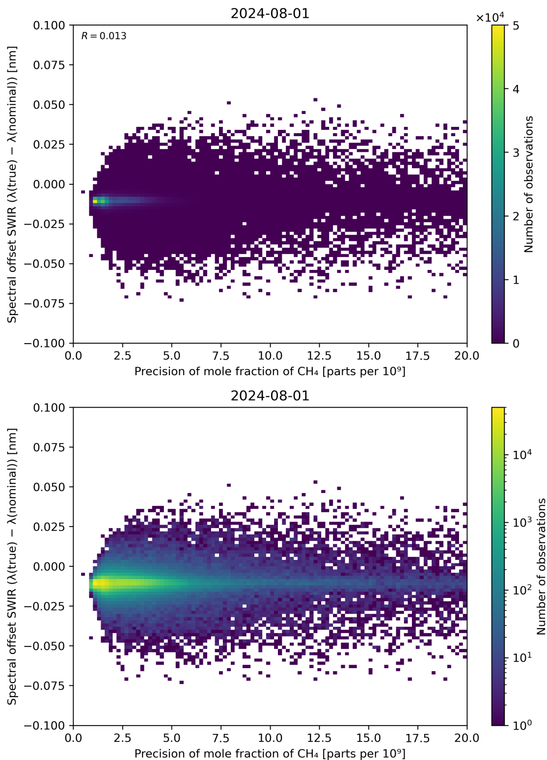
Figure 85: Scatter density plot of “Precision of mole fraction of CH 4 ” against “Spectral offset SWIR ( \lambda(\text{true}) - \lambda(\text{nominal}) )” for 2024-07-31 to 2024-08-02.
