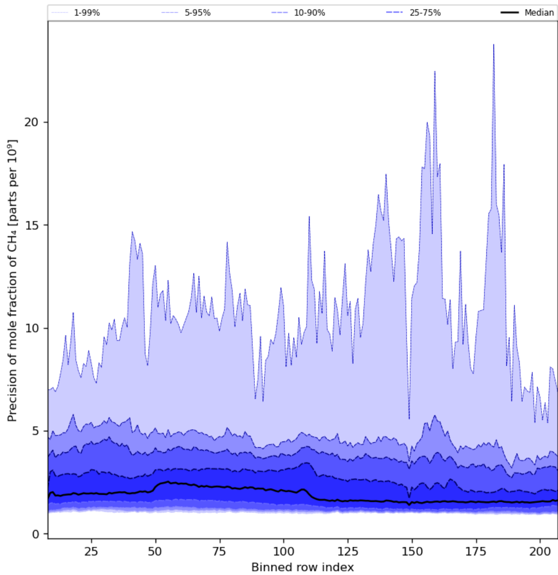
Figure 35: Along track statistics of “Precision of mole fraction of CH 4 ” for 2024-07-31 to 2024-08-02
