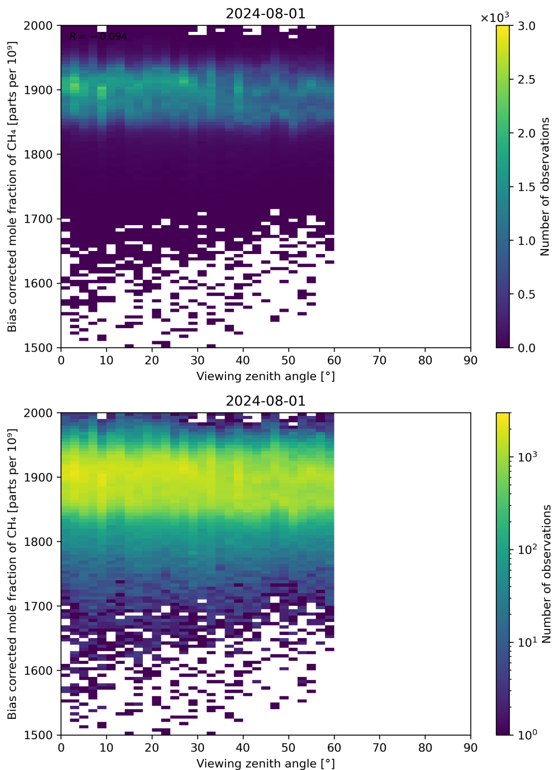
Figure 111: Scatter density plot of “Viewing zenith angle” against “Bias corrected mole fraction of CH 4 ” for 2024-07-31 to 2024-08-02.
