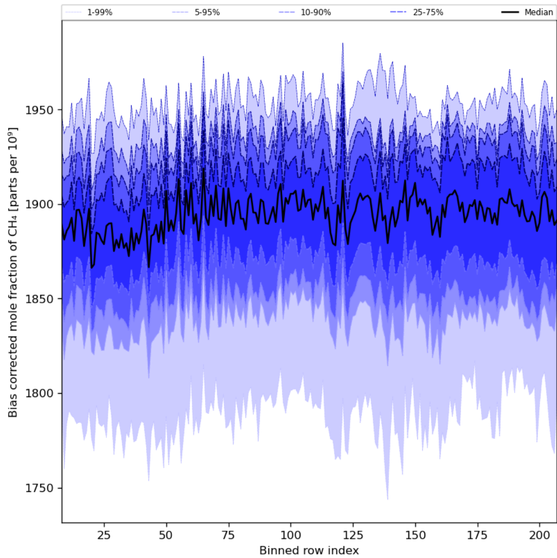
Figure 36: Along track statistics of “Bias corrected mole fraction of CH 4 ” for 2024-07-31 to 2024-08-02
