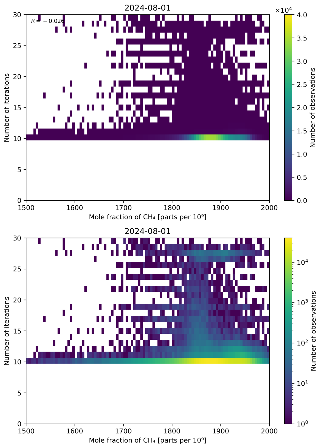
Figure 76: Scatter density plot of “Mole fraction of CH 4 ” against “Number of iterations” for 2024-07-31 to 2024-08-02.
