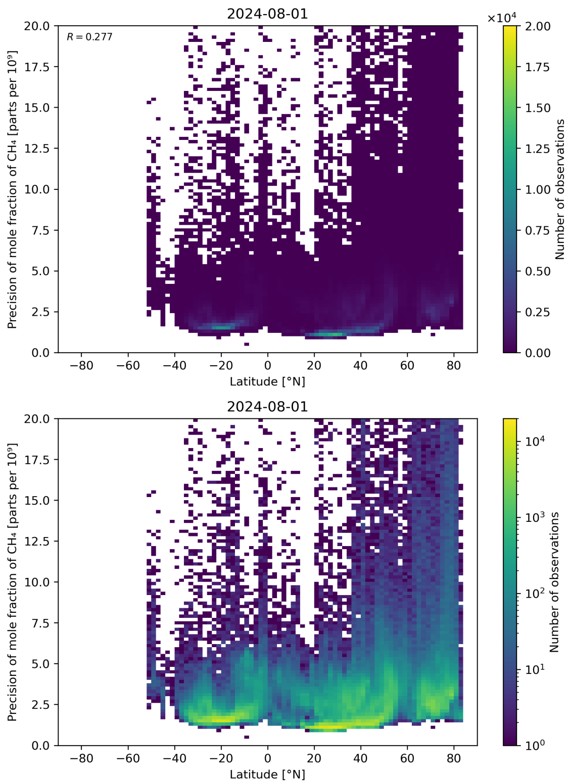
Figure 59: Scatter density plot of “Latitude” against “Precision of mole fraction of \text{CH}_4 ” for 2024-07-31 to 2024-08-02.
