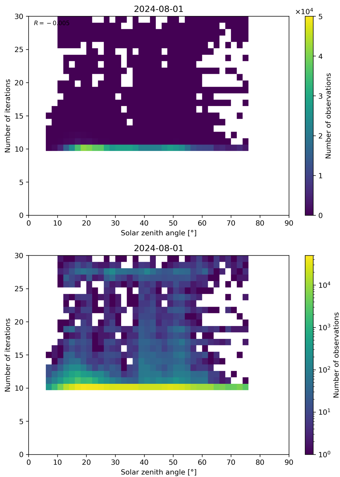
Figure 102: Scatter density plot of “Solar zenith angle” against “Number of iterations” for 2024-07-31 to 2024-08-02.
