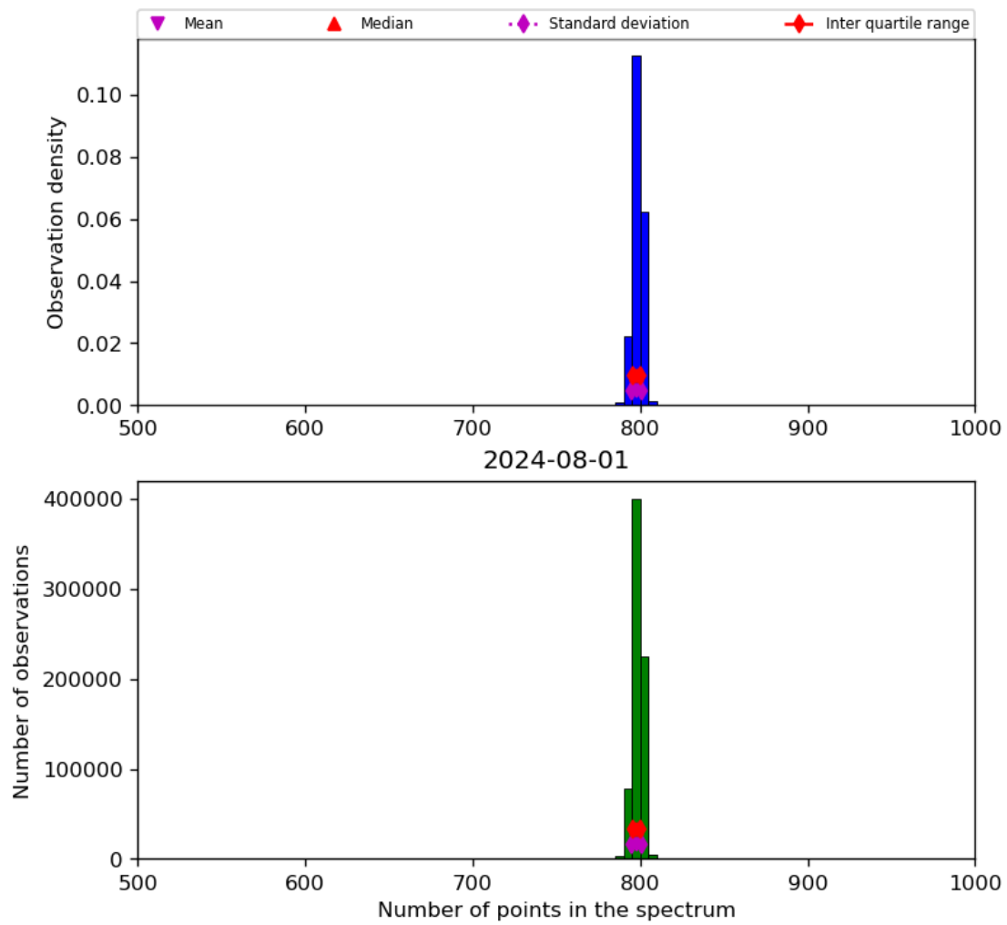
Figure 26: Histogram of “Number of points in the spectrum” for 2024-07-31 to 2024-08-02
