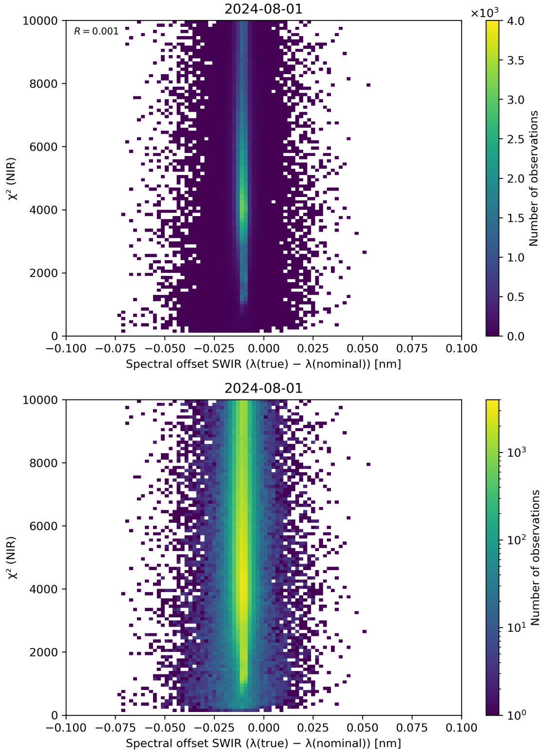
Figure 117: Scatter density plot of “Spectral offset SWIR ( \lambda(\text{true}) - \lambda(\text{nominal}) )” against “ \chi^2 (NIR)” for 2024-07-31 to 2024-08-02.
