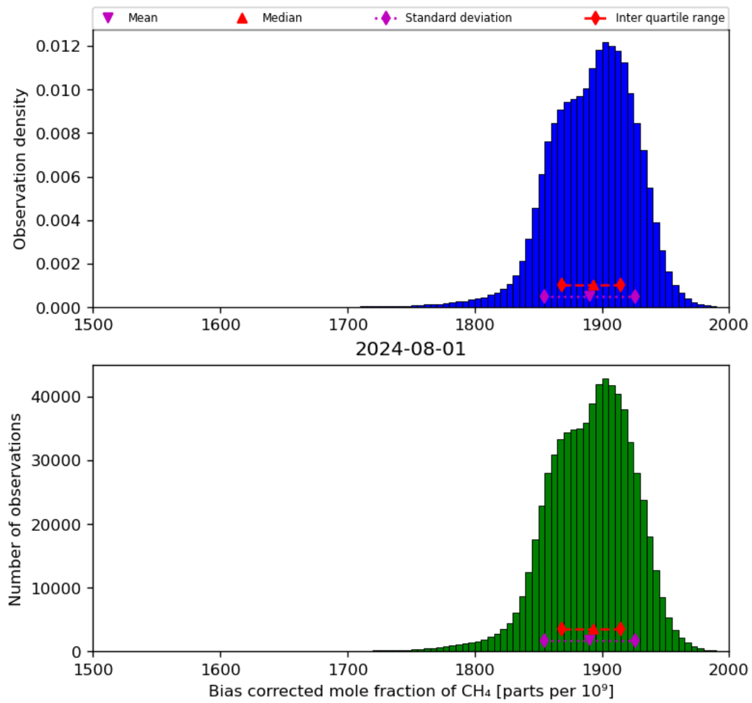
Figure 25: Histogram of “Bias corrected mole fraction of CH 4 ” for 2024-07-31 to 2024-08-02
