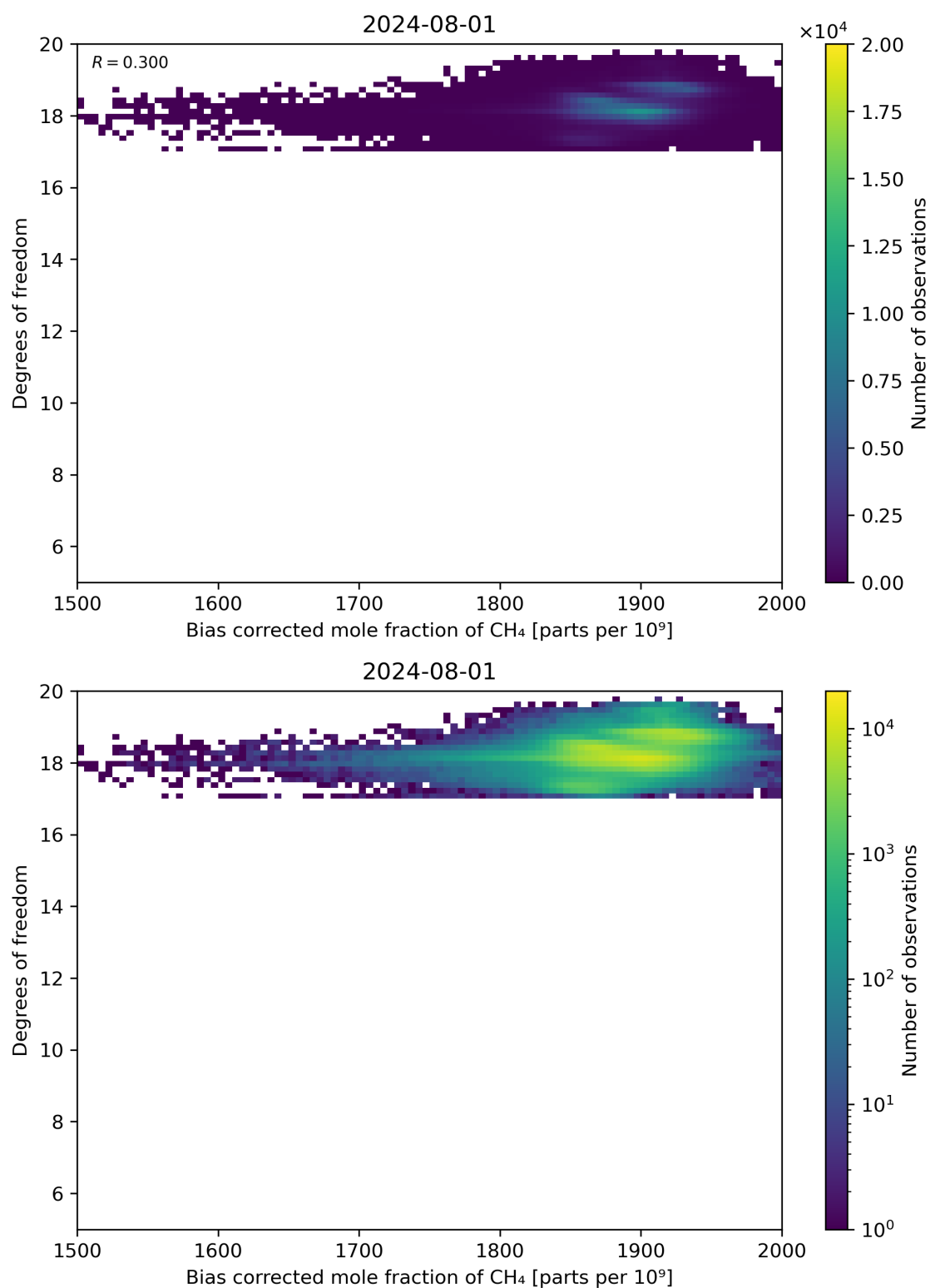
Figure 65: Scatter density plot of “Bias corrected mole fraction of CH 4 ” against “Degrees of freedom” for 2024-07-31 to 2024-08-02.
