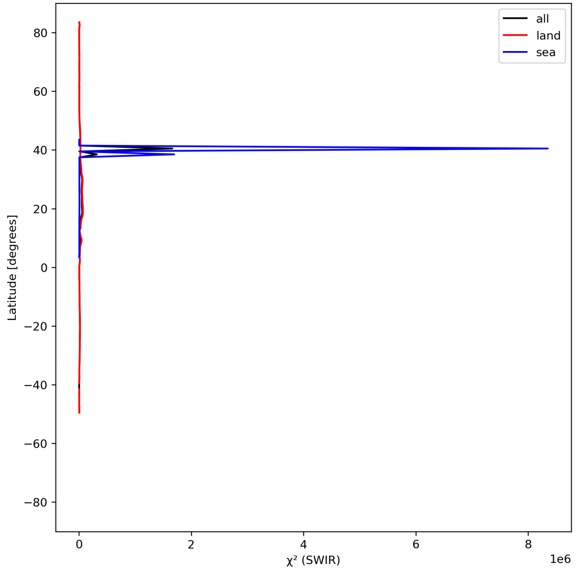
Figure 17: Zonal average of “ \chi^2 (SWIR)” for 2024-07-31 to 2024-08-02.
