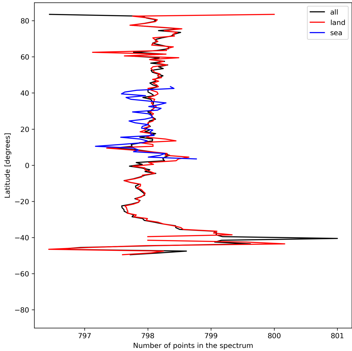
Figure 15: Zonal average of “Number of points in the spectrum” for 2024-07-31 to 2024-08-02.
