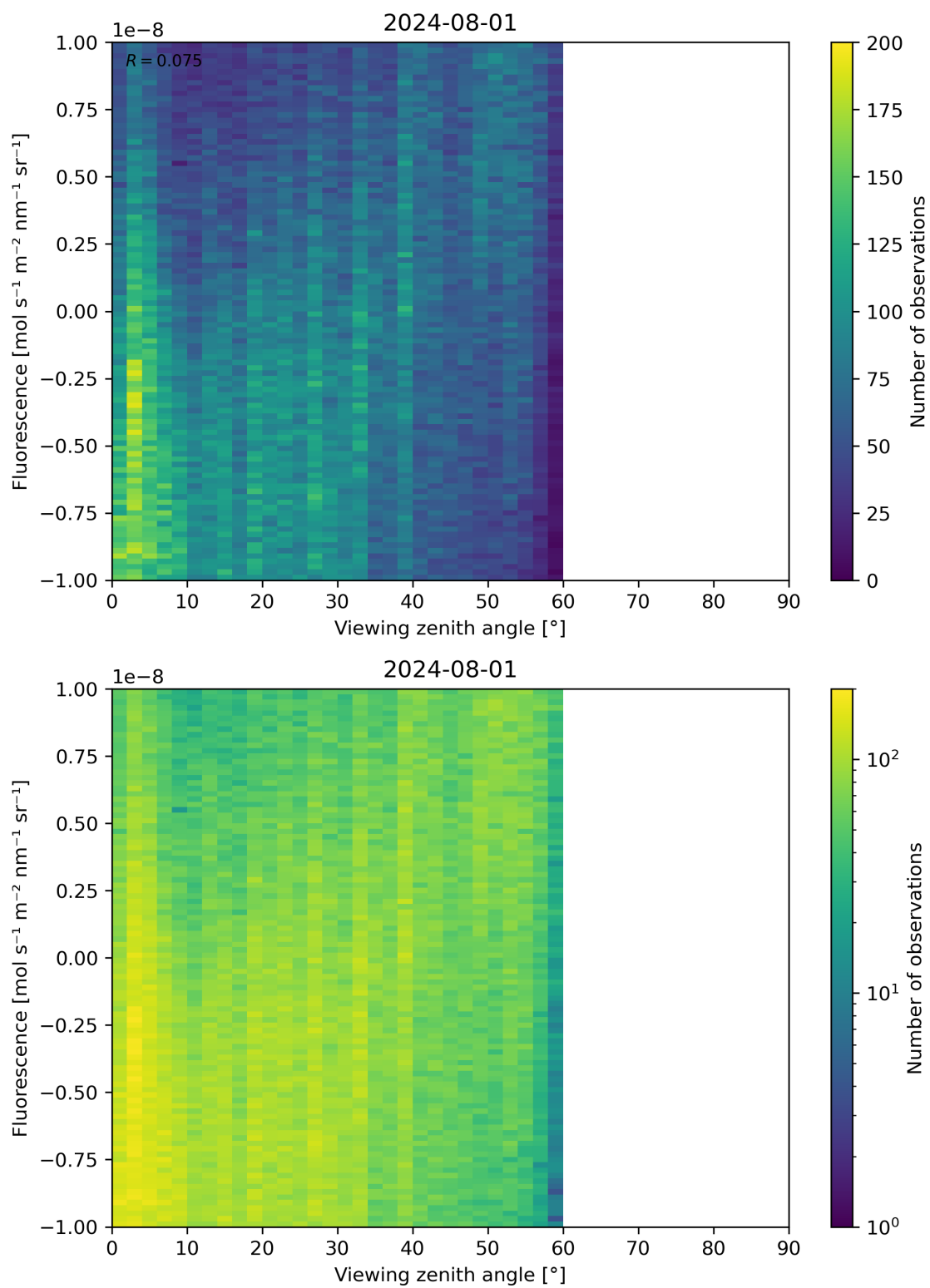
Figure 108: Scatter density plot of “Viewing zenith angle” against “Fluorescence” for 2024-07-31 to 2024-08-02.
