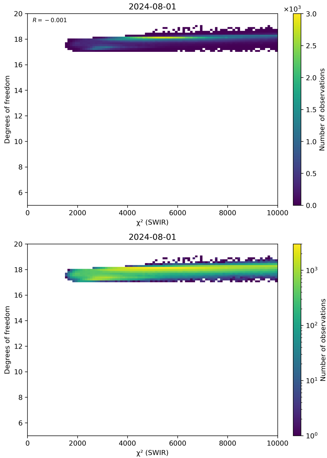
Figure 48: Scatter density plot of “ \chi^2 (SWIR)” against “Degrees of freedom” for 2024-07-31 to 2024-08-02.
