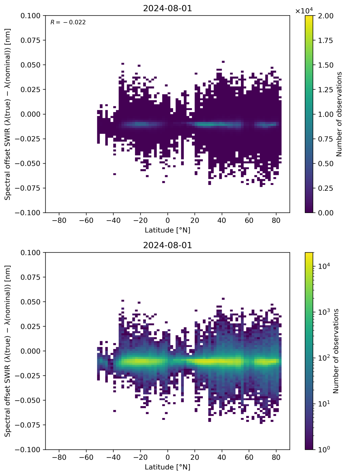
Figure 62: Scatter density plot of “Latitude” against “Spectral offset SWIR ( \lambda(\text{true}) - \lambda(\text{nominal}) )” for 2024-07-31 to 2024-08-02.
