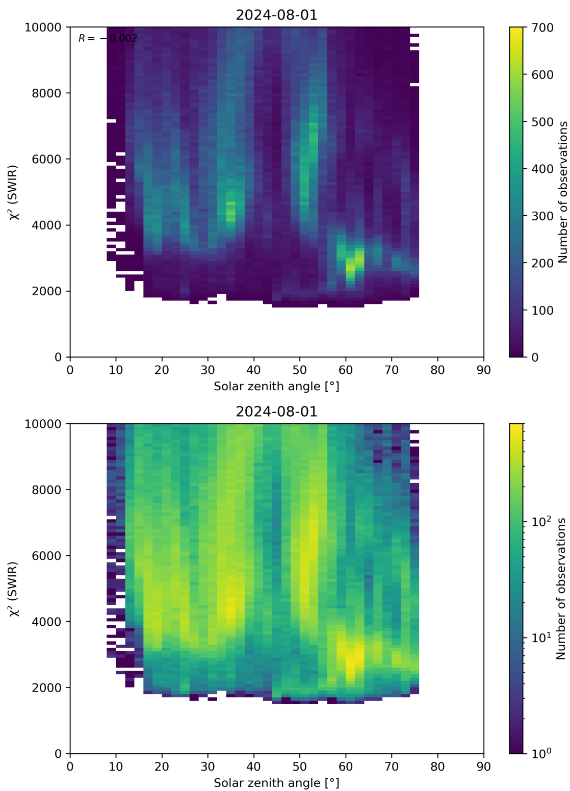
Figure 95: Scatter density plot of “Solar zenith angle” against “ \chi^2 (SWIR)” for 2024-07-31 to 2024-08-02.
