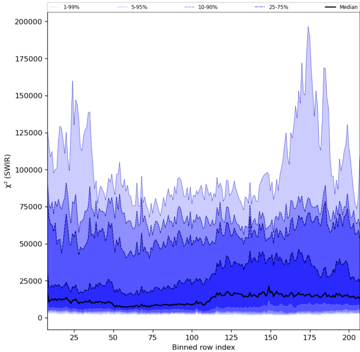
Figure 39: Along track statistics of “ \chi^2 (SWIR)” for 2024-07-31 to 2024-08-02
