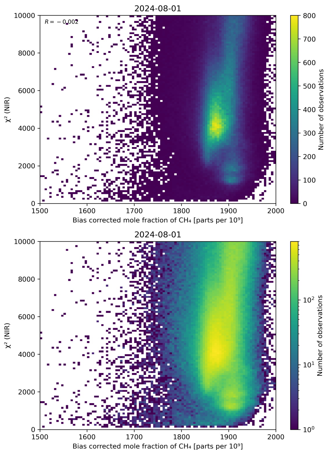
Figure 63: Scatter density plot of “Bias corrected mole fraction of CH 4 ” against “ \chi^2 (NIR)” for 2024-07-31 to 2024-08-02.
