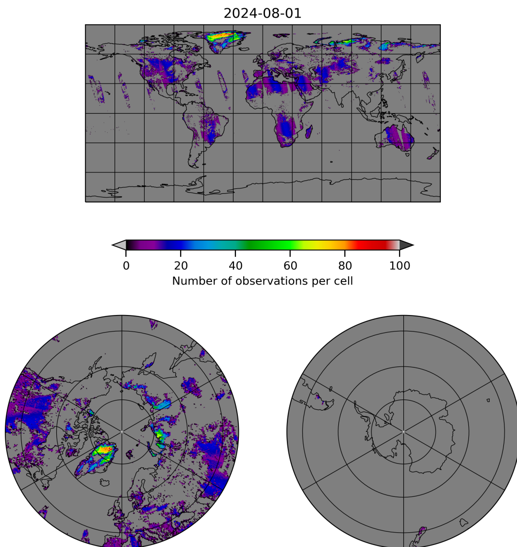
Figure 10: Map of the number of observations for 2024-07-31 to 2024-08-02
