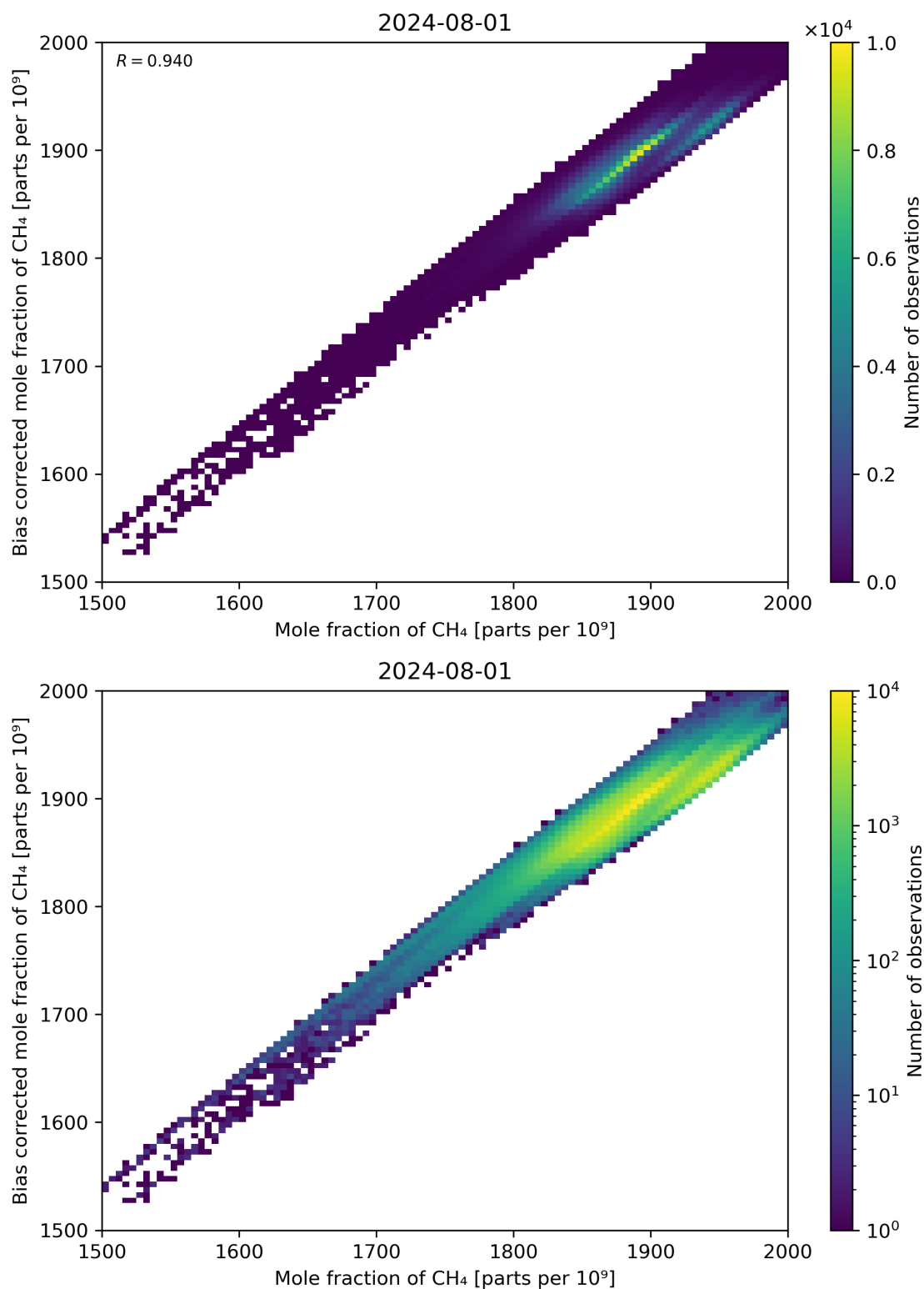
Figure 74: Scatter density plot of “Mole fraction of CH 4 ” against “Bias corrected mole fraction of CH 4 ” for 2024-07-31 to 2024-08-02.
