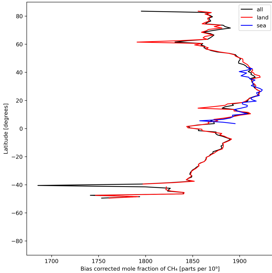
Figure 14: Zonal average of “Bias corrected mole fraction of CH 4 ” for 2024-07-31 to 2024-08-02.
