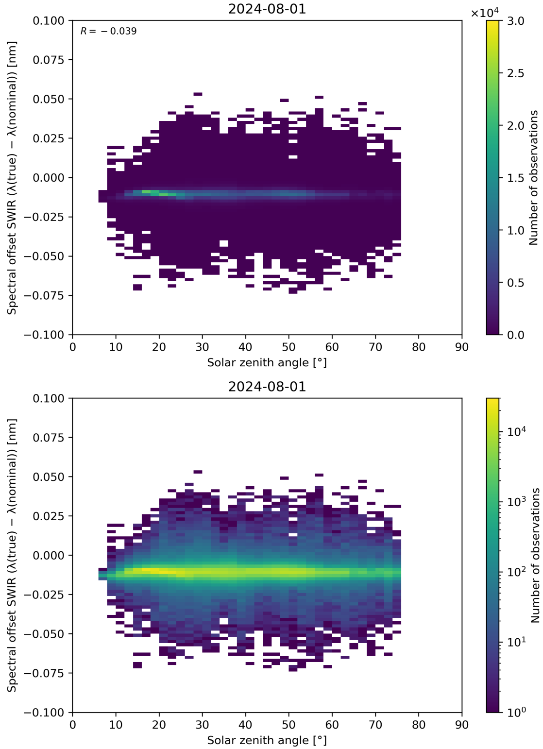
Figure 104: Scatter density plot of “Solar zenith angle” against “Spectral offset SWIR ( \lambda(\text{true}) - \lambda(\text{nominal}) )” for 2024-07-31 to 2024-08-02.
