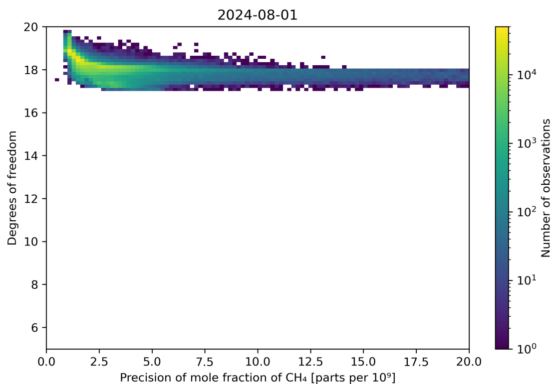
Figure 80: Scatter density plot of “Precision of mole fraction of CH 4 ” against “Degrees of freedom” for 2024-07-31 to 2024-08-02.
