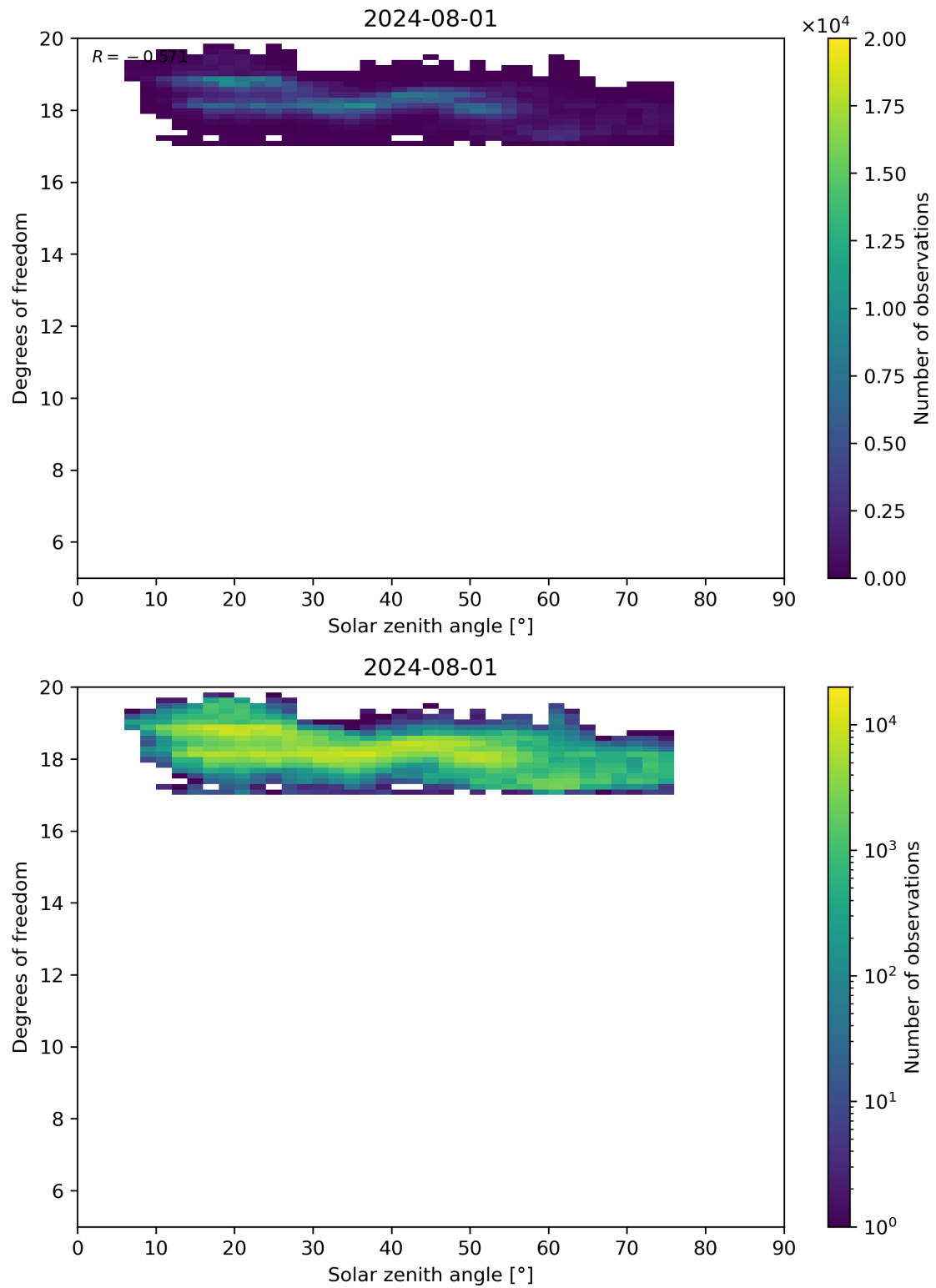
Figure 96: Scatter density plot of “Solar zenith angle” against “Degrees of freedom” for 2024-07-31 to 2024-08-02.
