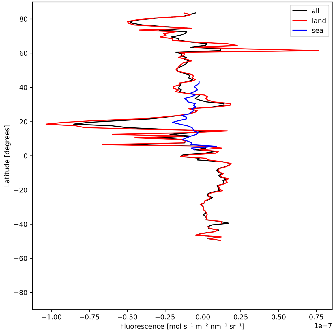
Figure 21: Zonal average of “Fluorescence” for 2024-07-31 to 2024-08-02.
