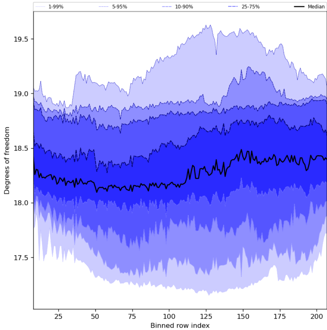
Figure 41: Along track statistics of “Degrees of freedom” for 2024-07-31 to 2024-08-02
