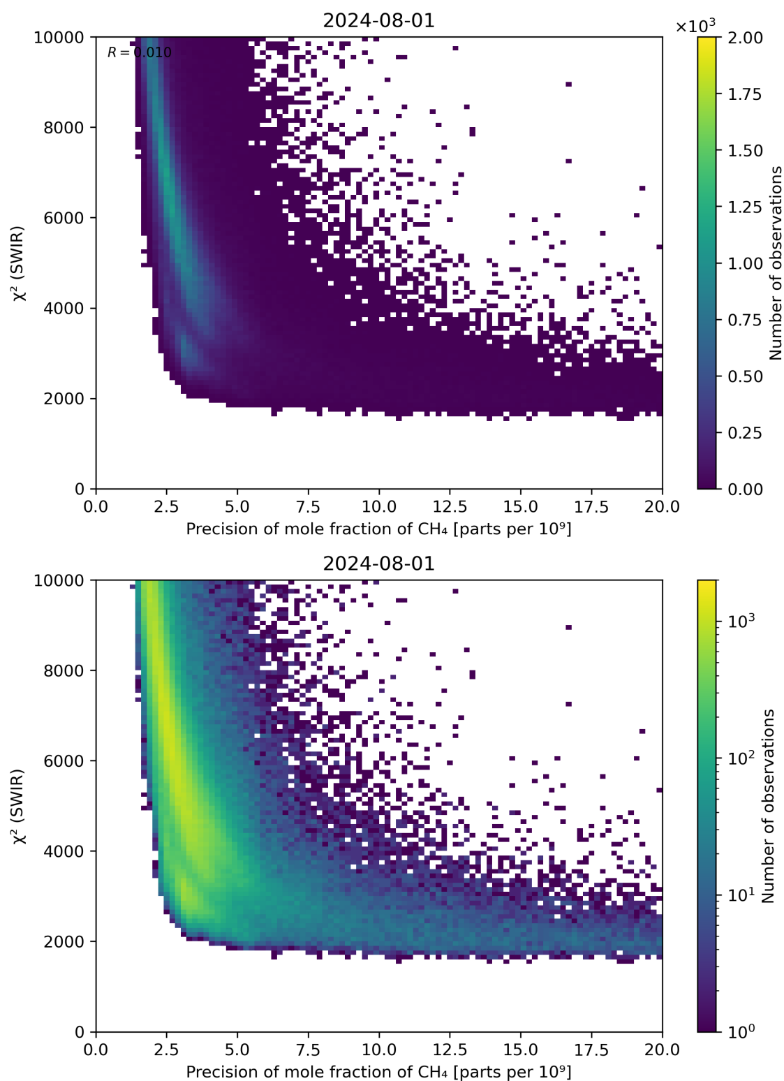
Figure 79: Scatter density plot of “Precision of mole fraction of \text{CH}_4 ” against “ \chi^2 (SWIR)” for 2024-07-31 to 2024-08-02.
