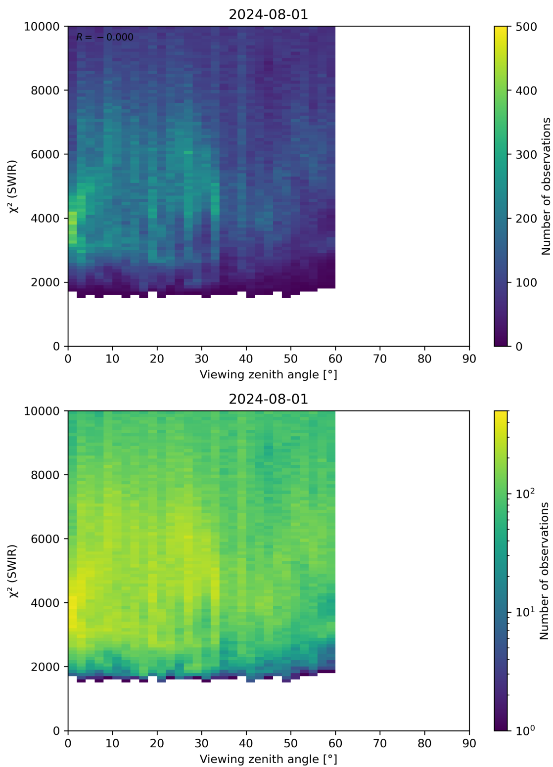
Figure 106: Scatter density plot of “Viewing zenith angle” against “ \chi^2 (SWIR)” for 2024-07-31 to 2024-08-02.
