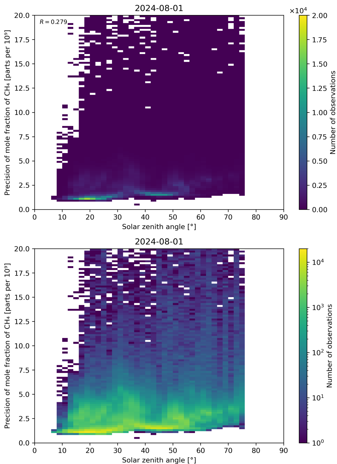
Figure 101: Scatter density plot of “Solar zenith angle” against “Precision of mole fraction of CH 4 ” for 2024-07-31 to 2024-08-02.
