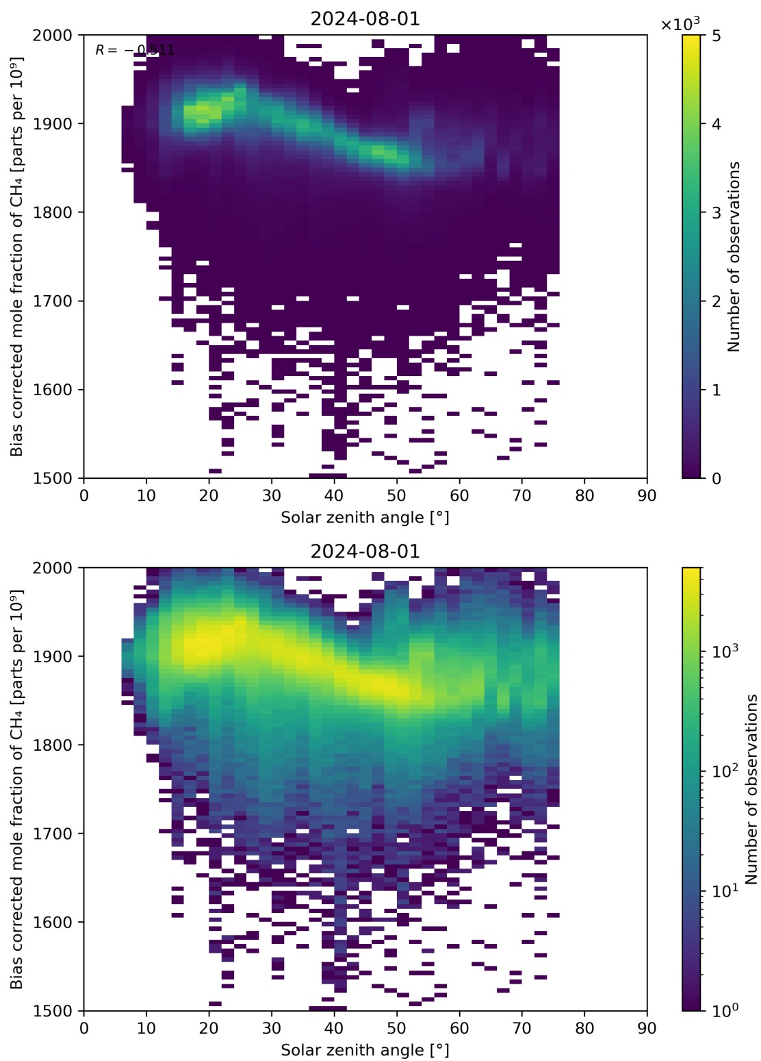
Figure 100: Scatter density plot of “Solar zenith angle” against “Bias corrected mole fraction of CH 4 ” for 2024-07-31 to 2024-08-02.
