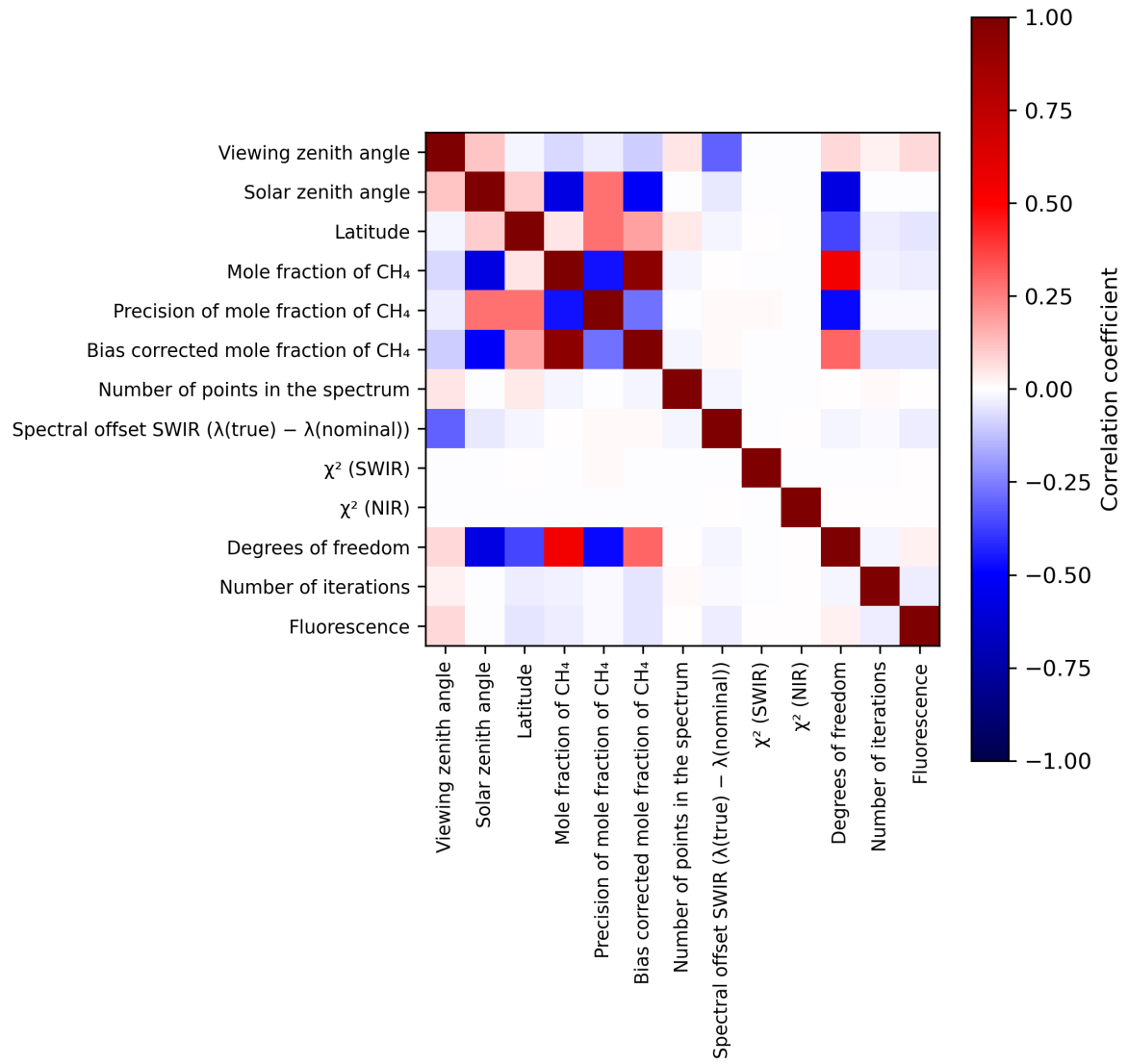
Figure 2: Map of correlation matrix for 2024-07-31 to 2024-08-02.
