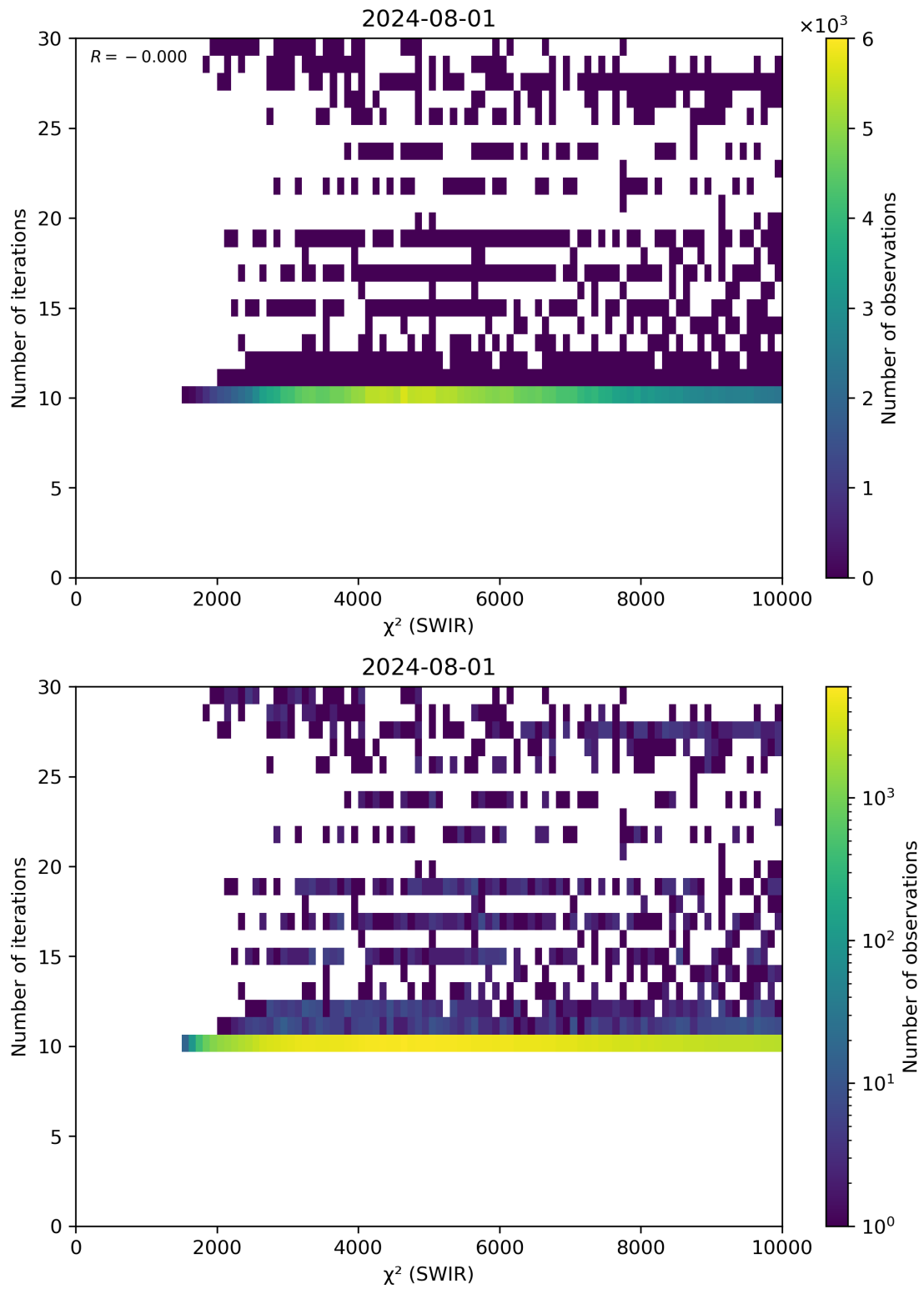
Figure 50: Scatter density plot of " \chi^2 (SWIR)" against "Number of iterations" for 2024-07-31 to 2024-08-02.
