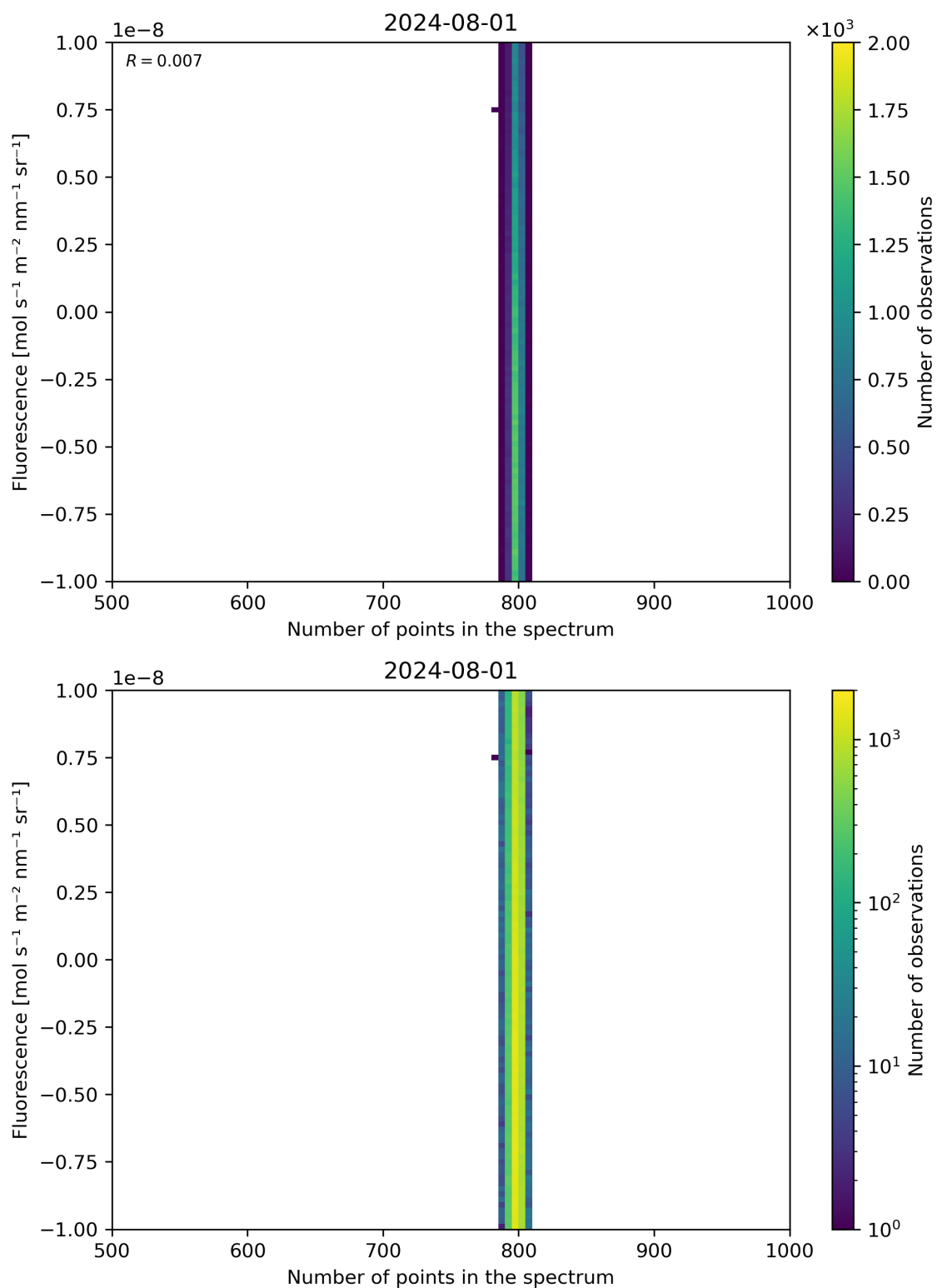
Figure 91: Scatter density plot of “Number of points in the spectrum” against “Fluorescence” for 2024-07-31 to 2024-08-02.
