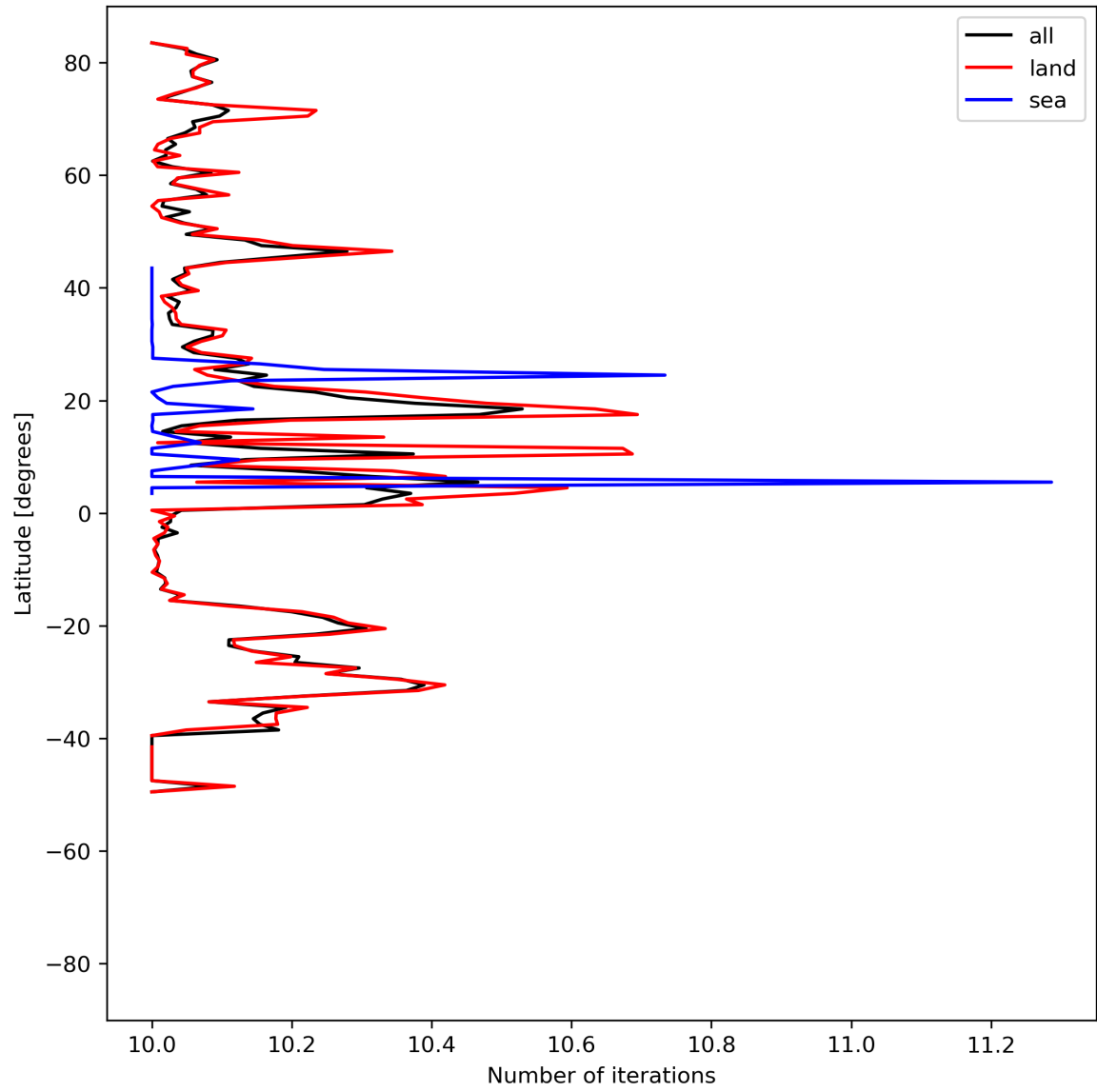
Figure 20: Zonal average of “Number of iterations” for 2024-07-31 to 2024-08-02.
