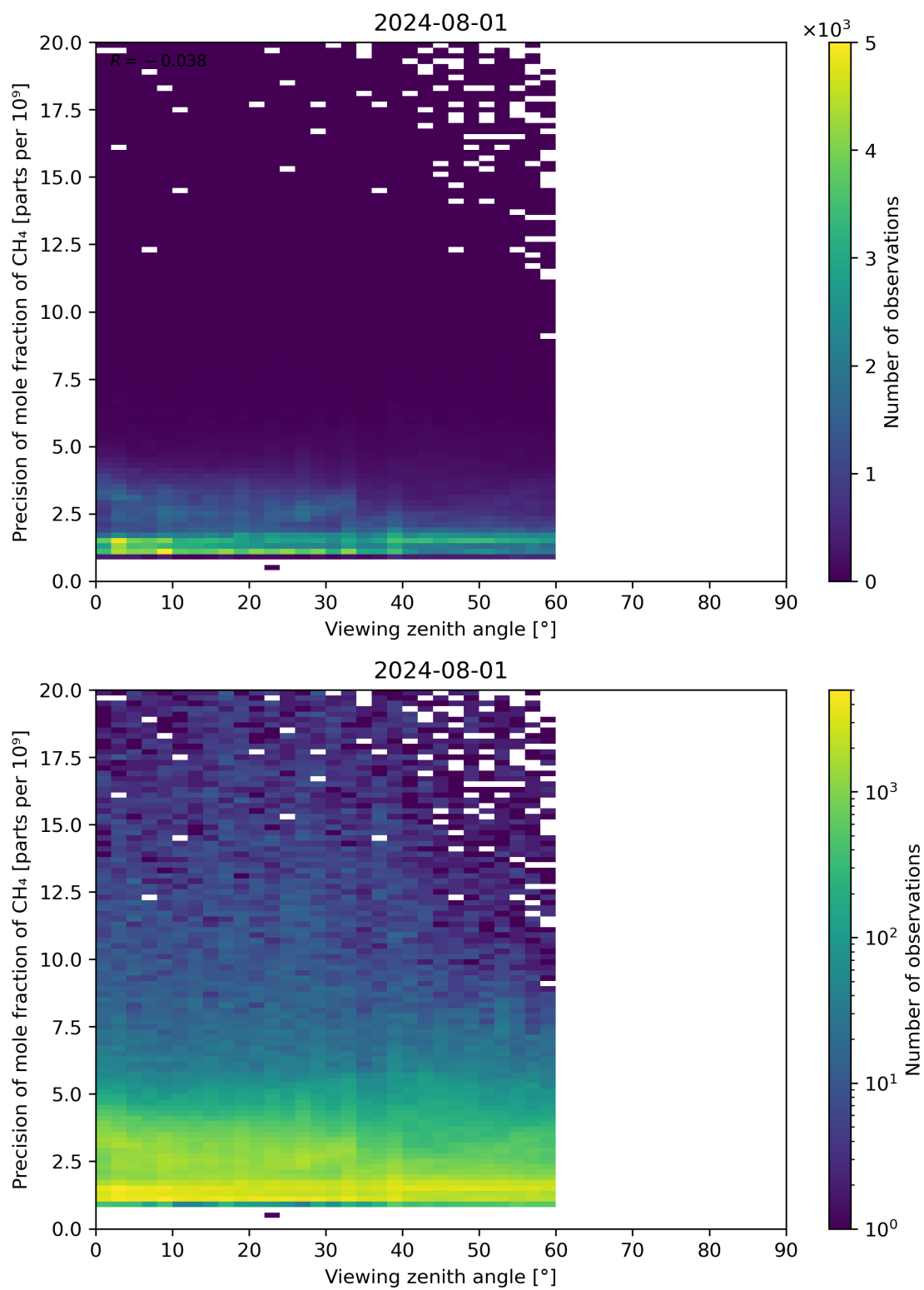
Figure 112: Scatter density plot of “Viewing zenith angle” against “Precision of mole fraction of CH 4 ” for 2024-07-31 to 2024-08-02.
