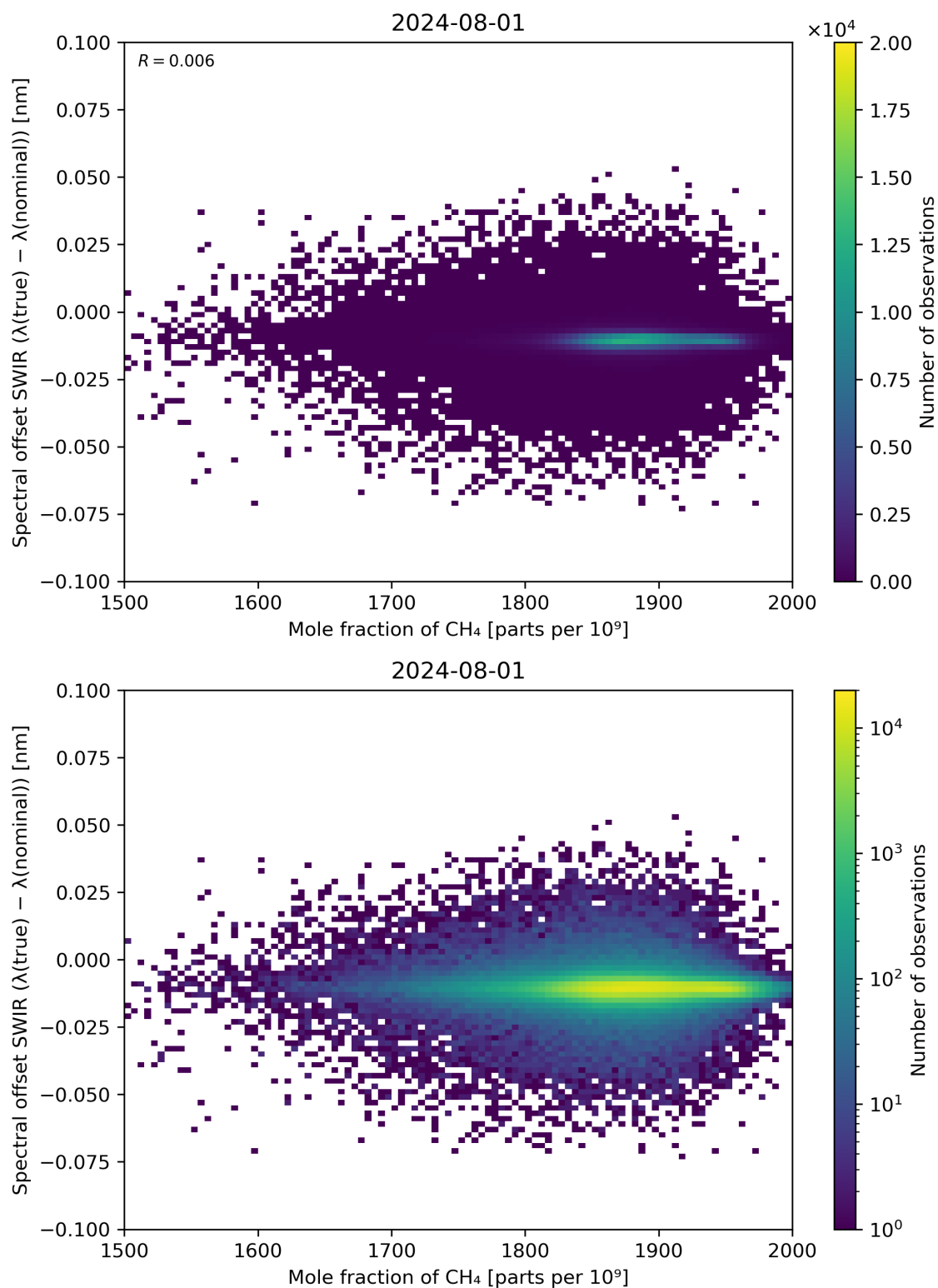
Figure 86: Scatter density plot of “Mole fraction of CH 4 ” against “Spectral offset SWIR ( \lambda(\text{true}) - \lambda(\text{nominal}) )” for 2024-07-31 to 2024-08-02.
