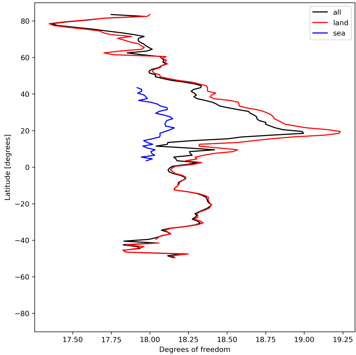
Figure 19: Zonal average of “Degrees of freedom” for 2024-07-31 to 2024-08-02.
