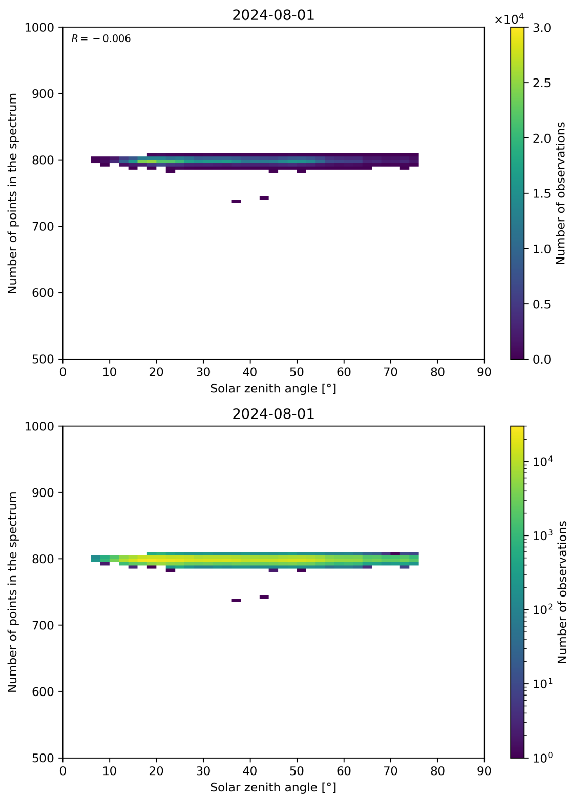
Figure 103: Scatter density plot of “Solar zenith angle” against “Number of points in the spectrum” for 2024-07-31 to 2024-08-02.
