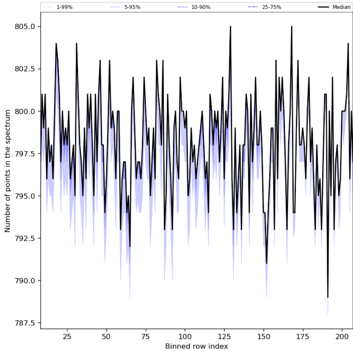
Figure 37: Along track statistics of “Number of points in the spectrum” for 2024-07-31 to 2024-08-02
