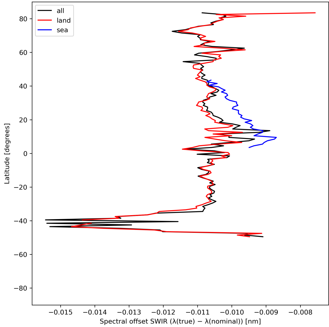
Figure 16: Zonal average of “Spectral offset SWIR ( \lambda(\text{true}) - \lambda(\text{nominal}) )” for 2024-07-31 to 2024-08-02.
