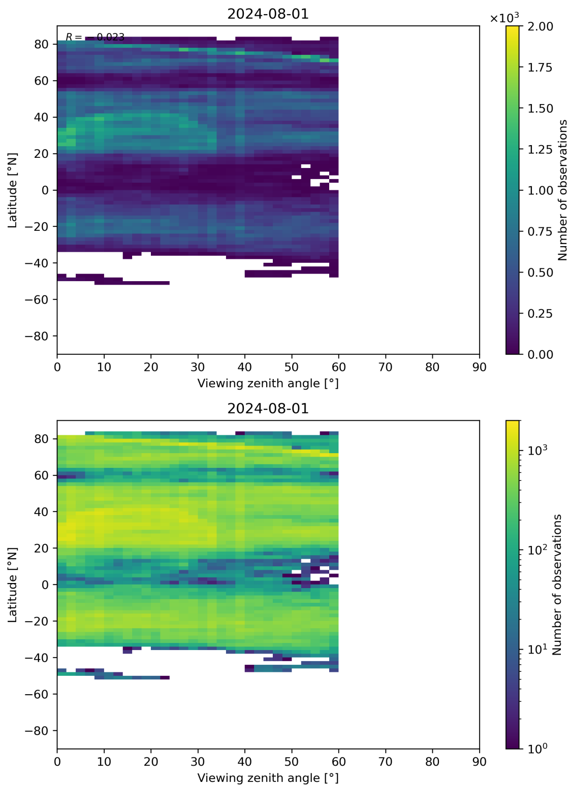
Figure 109: Scatter density plot of “Viewing zenith angle” against “Latitude” for 2024-07-31 to 2024-08-02.
