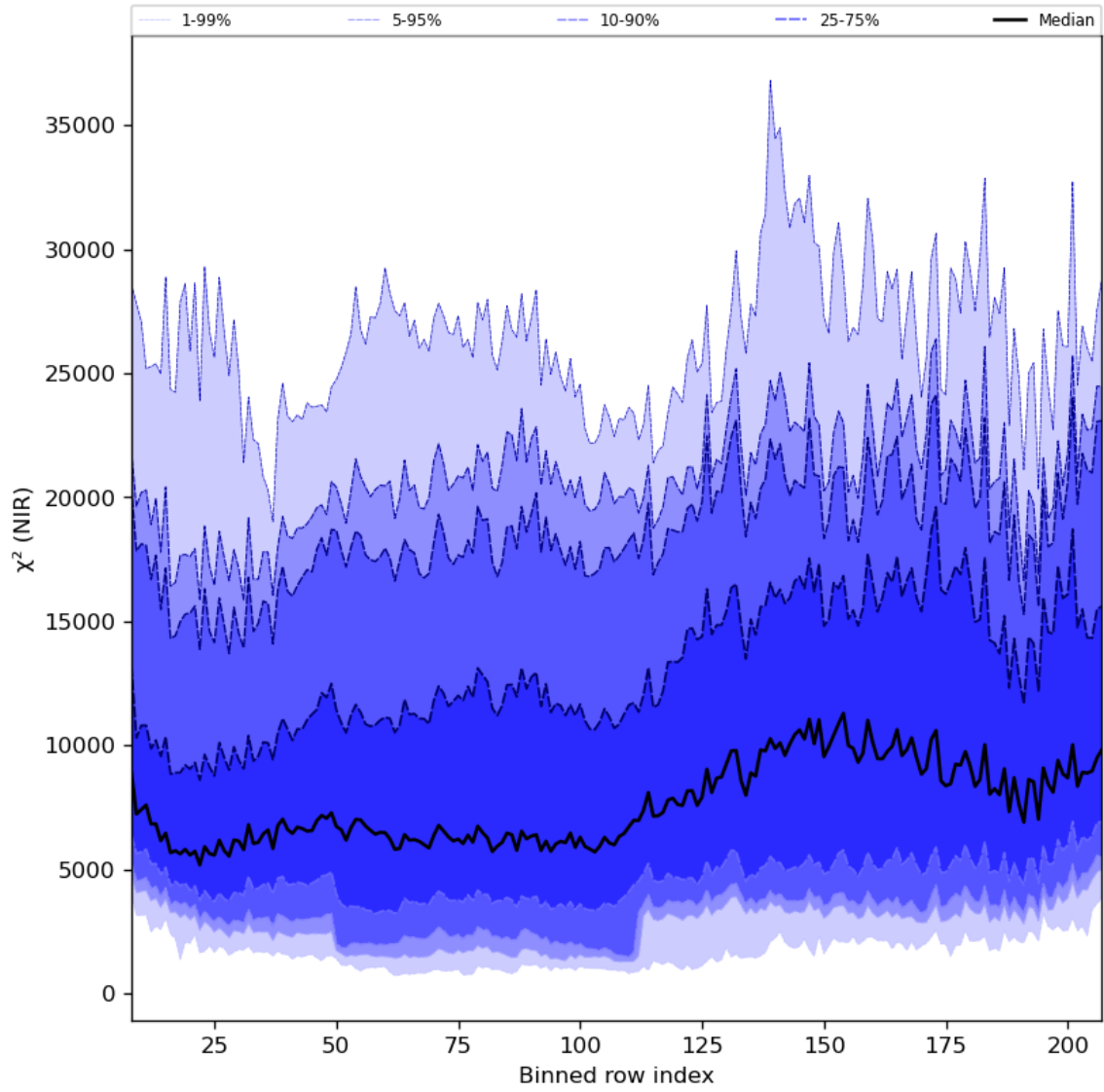
Figure 40: Along track statistics of " \chi^2 (NIR)" for 2024-07-31 to 2024-08-02
