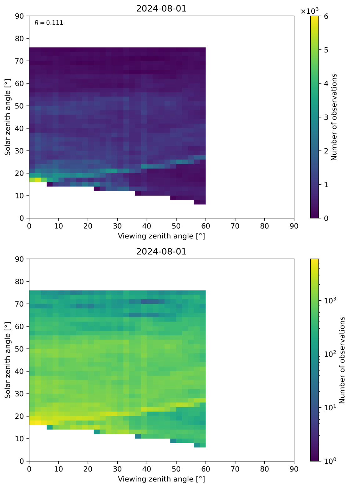
Figure 115: Scatter density plot of “Viewing zenith angle” against “Solar zenith angle” for 2024-07-31 to 2024-08-02.
