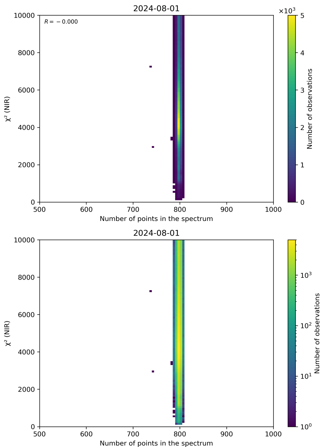
Figure 88: Scatter density plot of “Number of points in the spectrum” against “ \chi^2 (NIR)” for 2024-07-31 to 2024-08-02.
