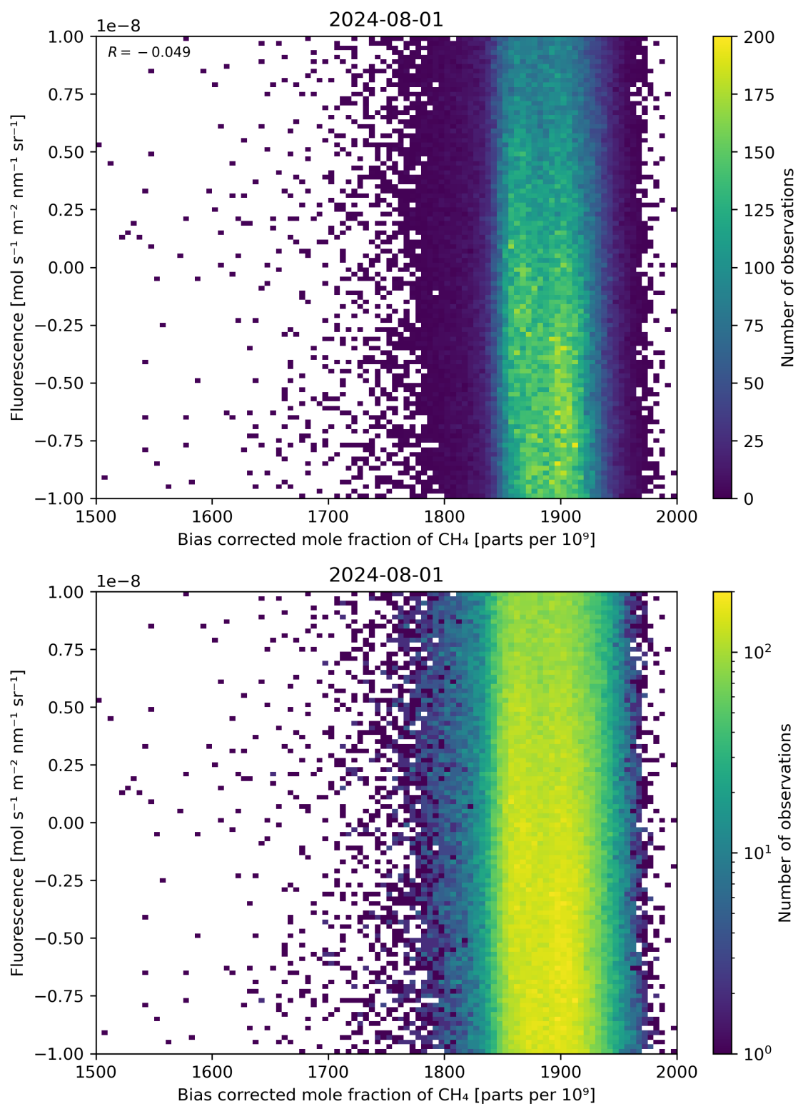
Figure 66: Scatter density plot of “Bias corrected mole fraction of \text{CH}_4 ” against “Fluorescence” for 2024-07-31 to 2024-08-02.
