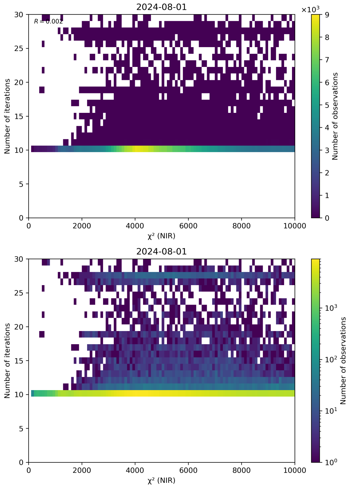
Figure 46: Scatter density plot of “ \chi^2 (NIR)” against “Number of iterations” for 2024-07-31 to 2024-08-02.
