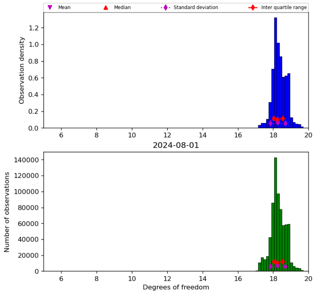
Figure 30: Histogram of “Degrees of freedom” for 2024-07-31 to 2024-08-02
