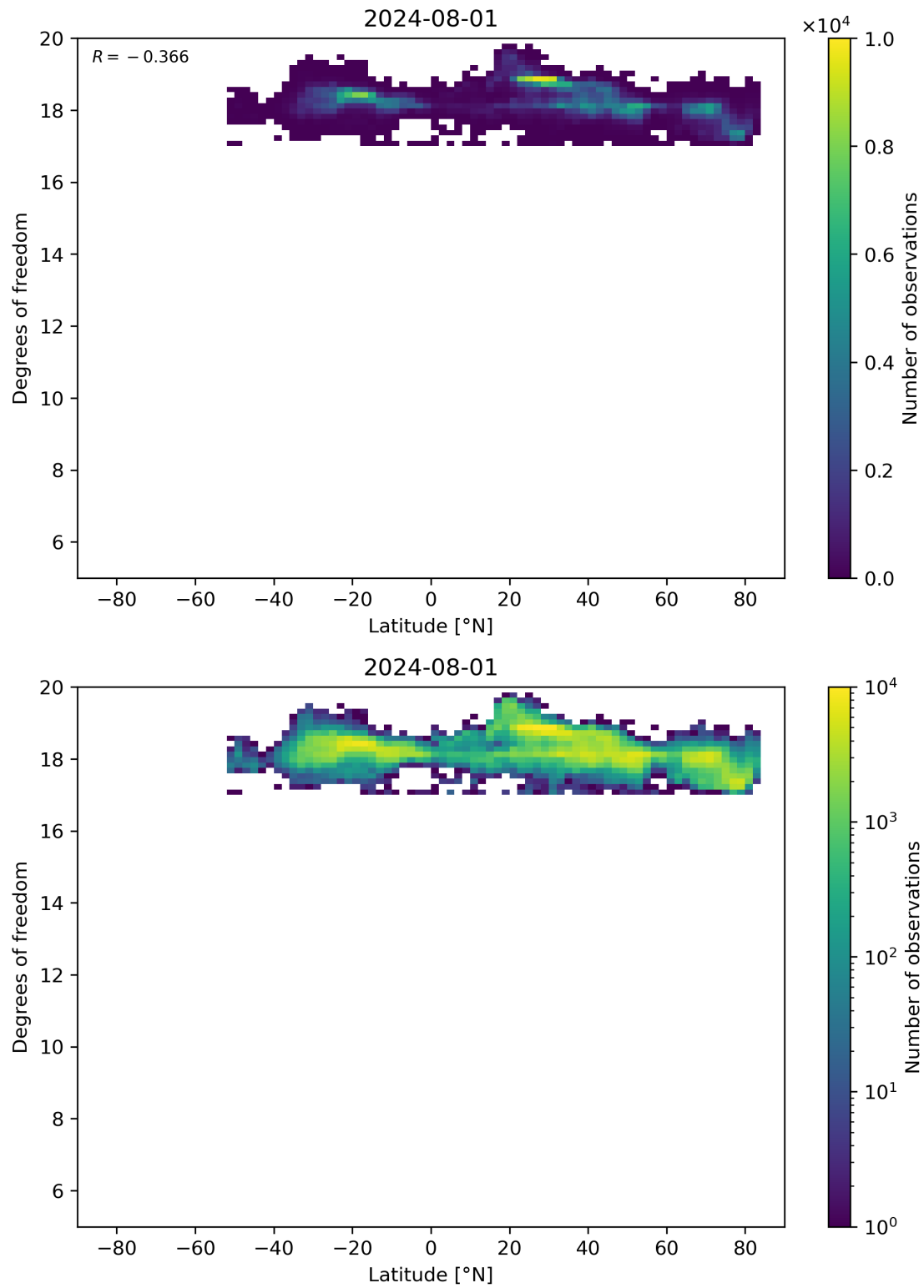
Figure 55: Scatter density plot of “Latitude” against “Degrees of freedom” for 2024-07-31 to 2024-08-02.
