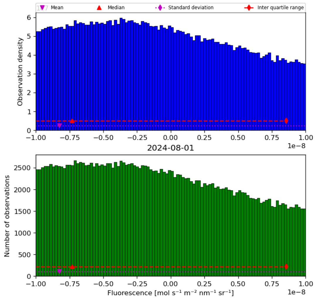
Figure 32: Histogram of “Fluorescence” for 2024-07-31 to 2024-08-02
