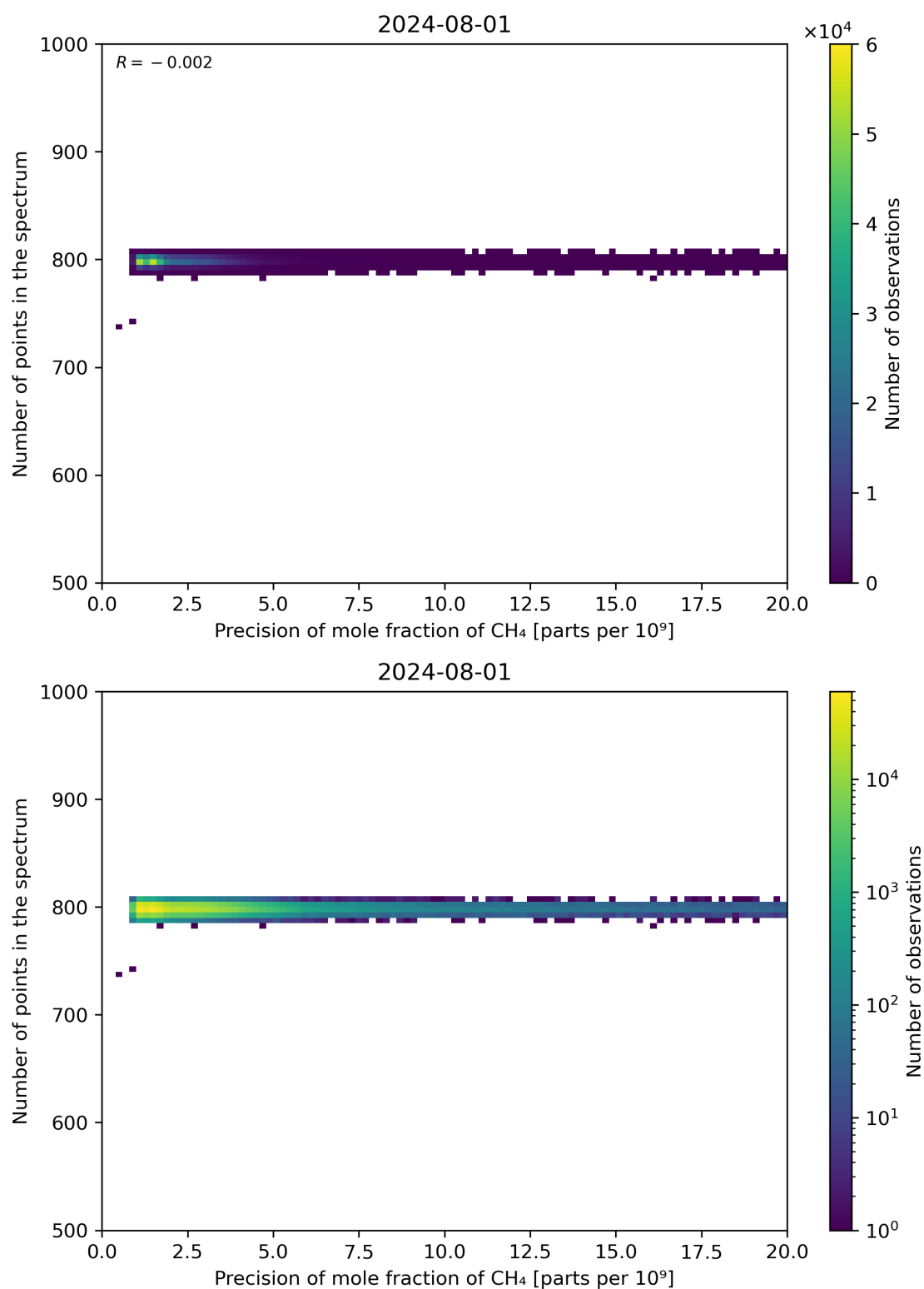
Figure 84: Scatter density plot of “Precision of mole fraction of CH 4 ” against “Number of points in the spectrum” for 2024-07-31 to 2024-08-02.
