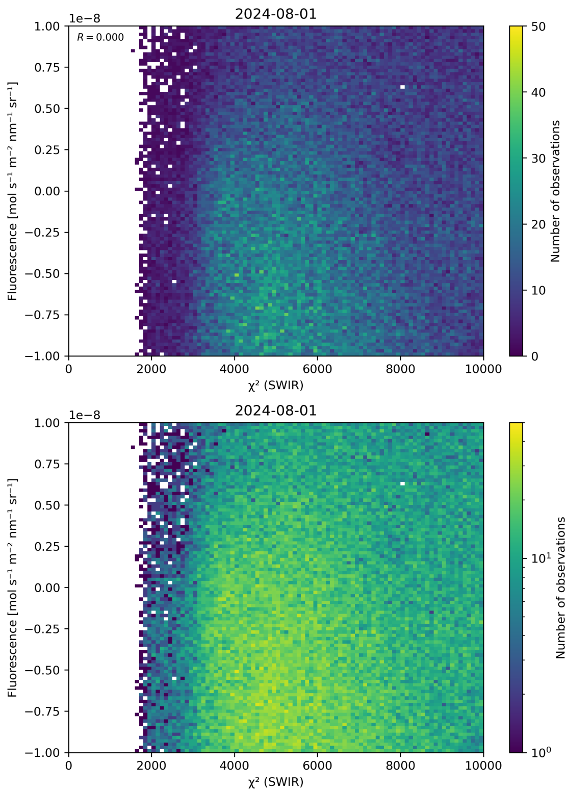
Figure 49: Scatter density plot of “ \chi^2 (SWIR)” against “Fluorescence” for 2024-07-31 to 2024-08-02.
