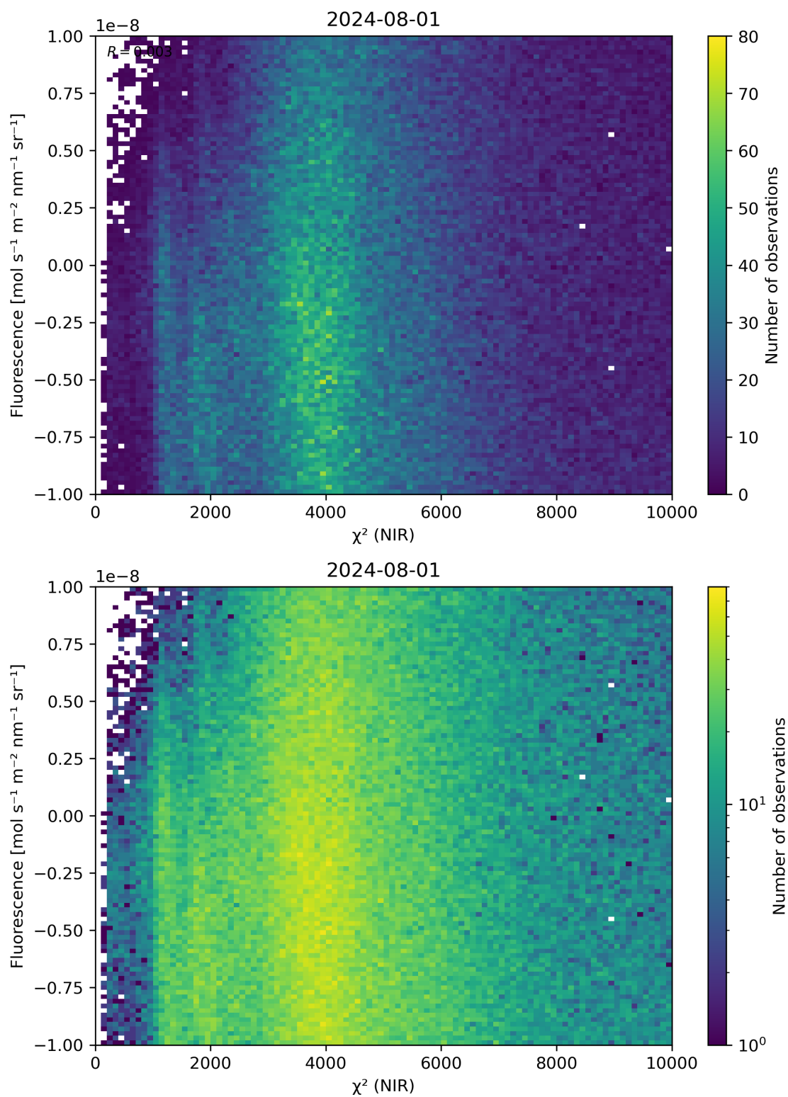
Figure 45: Scatter density plot of “ \chi^2 (NIR)” against “Fluorescence” for 2024-07-31 to 2024-08-02.
