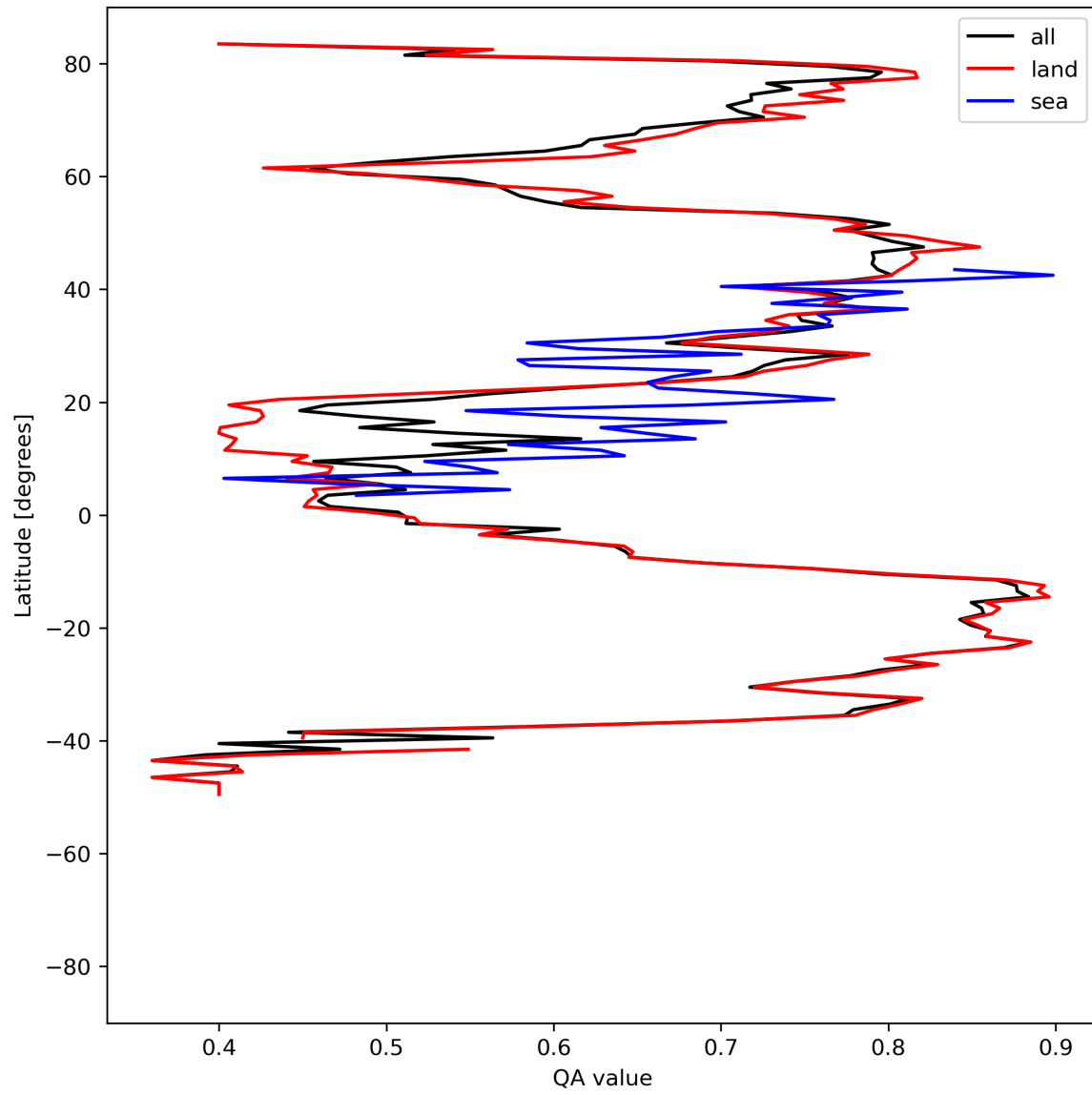
Figure 11: Zonal average of “QA value” for 2024-07-31 to 2024-08-02.
