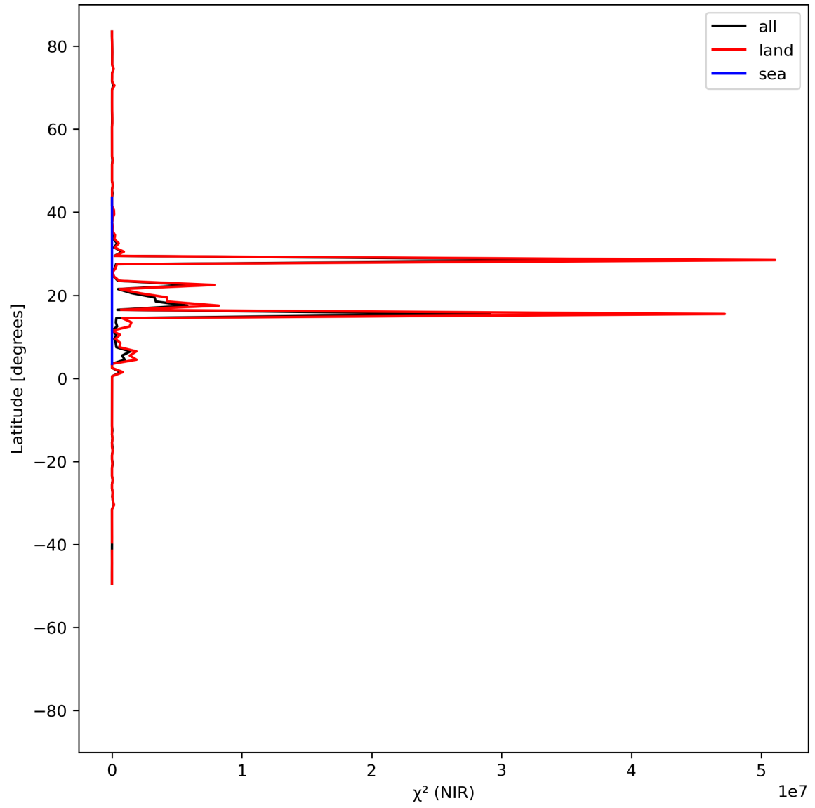
Figure 18: Zonal average of “ \chi^2 (NIR)” for 2024-07-31 to 2024-08-02.
