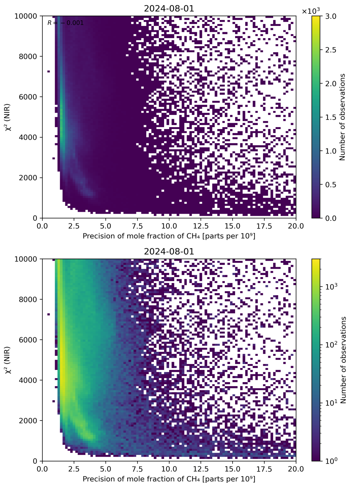
Figure 78: Scatter density plot of “Precision of mole fraction of CH 4 ” against “ \chi^2 (NIR)” for 2024-07-31 to 2024-08-02.
