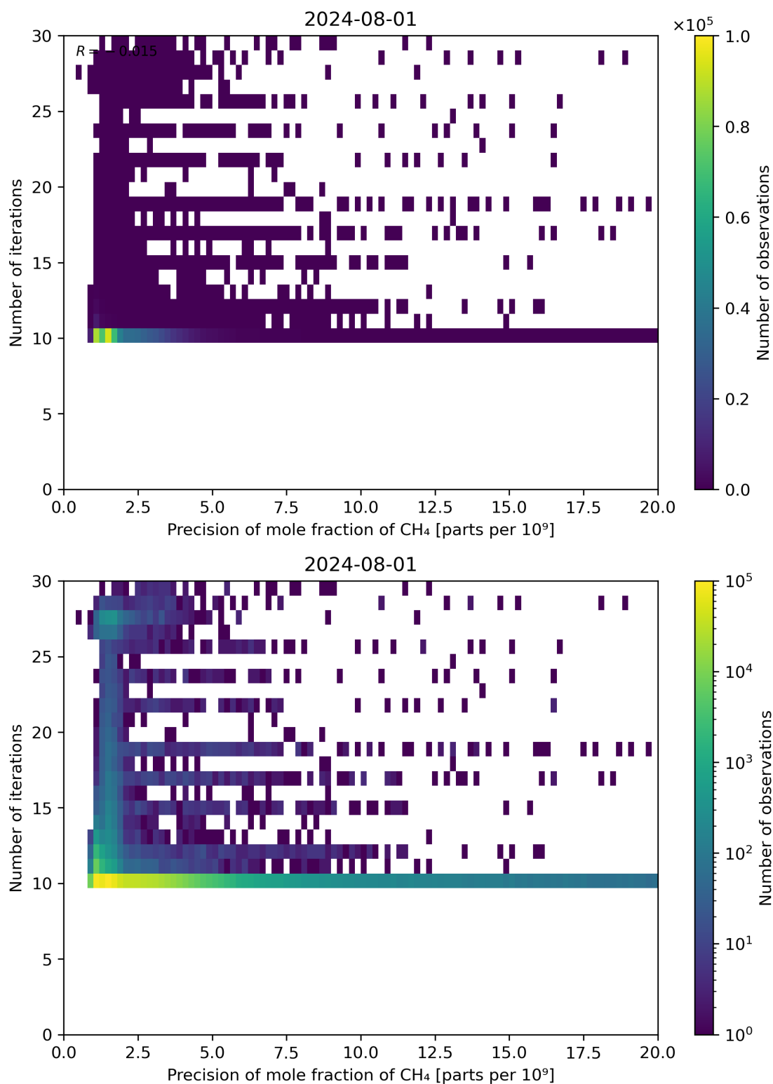
Figure 83: Scatter density plot of “Precision of mole fraction of CH 4 ” against “Number of iterations” for 2024-07-31 to 2024-08-02.
