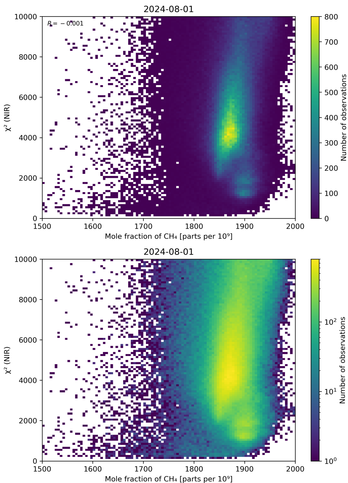
Figure 70: Scatter density plot of “Mole fraction of CH 4 ” against “ \chi^2 (NIR)” for 2024-07-31 to 2024-08-02.
