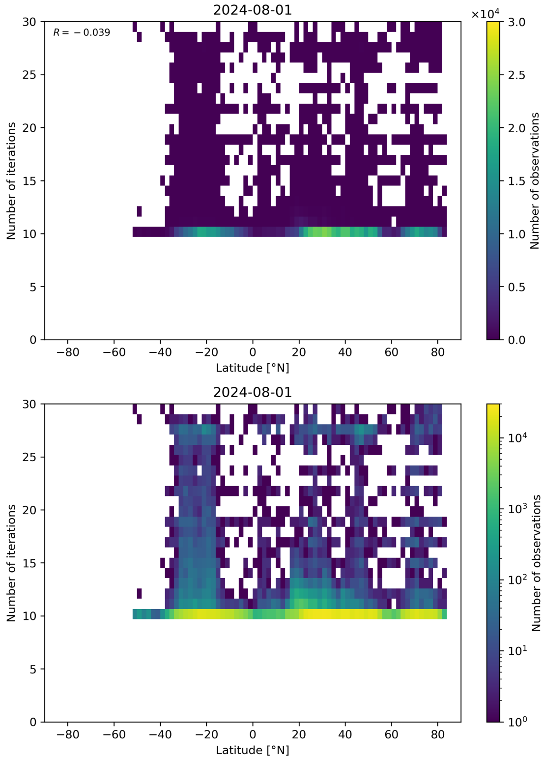
Figure 60: Scatter density plot of “Latitude” against “Number of iterations” for 2024-07-31 to 2024-08-02.
