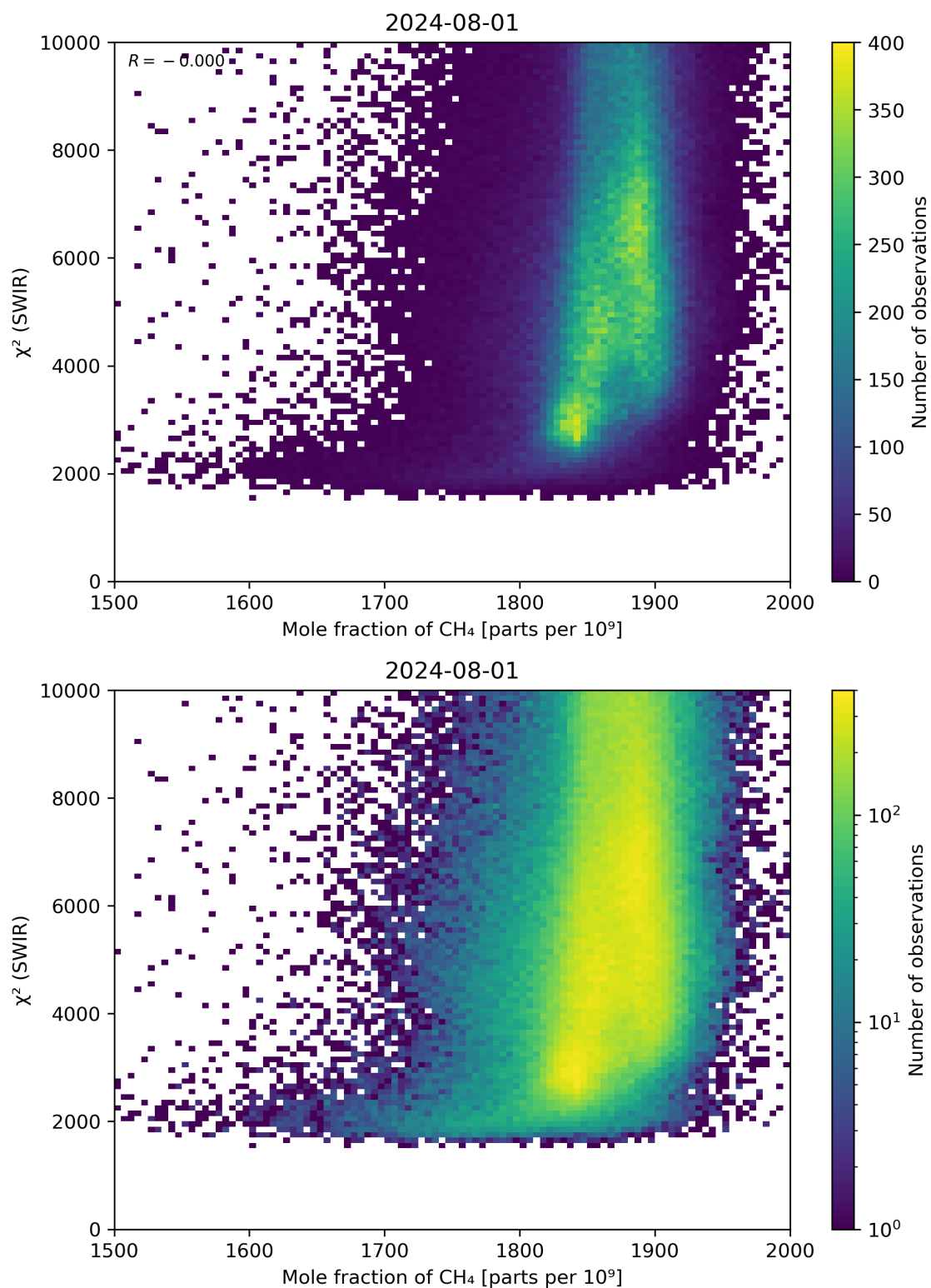
Figure 71: Scatter density plot of “Mole fraction of \text{CH}_4 ” against “ \chi^2 (SWIR)” for 2024-07-31 to 2024-08-02.
