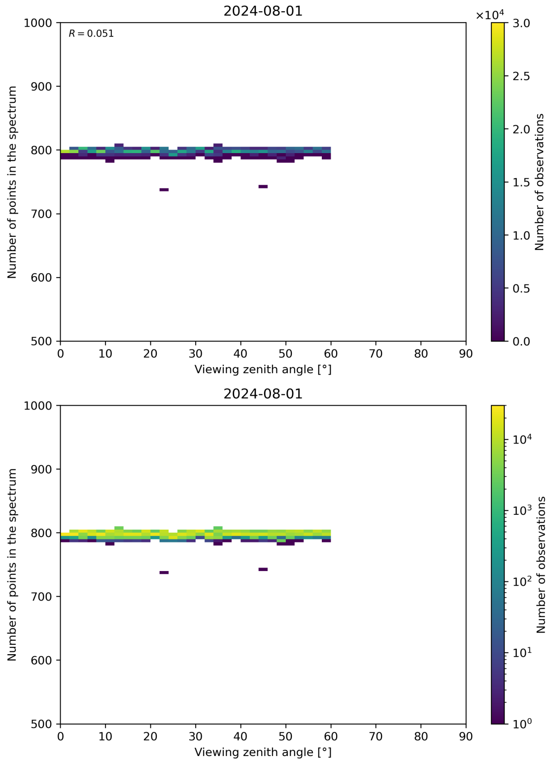
Figure 114: Scatter density plot of “Viewing zenith angle” against “Number of points in the spectrum” for 2024-07-31 to 2024-08-02.
