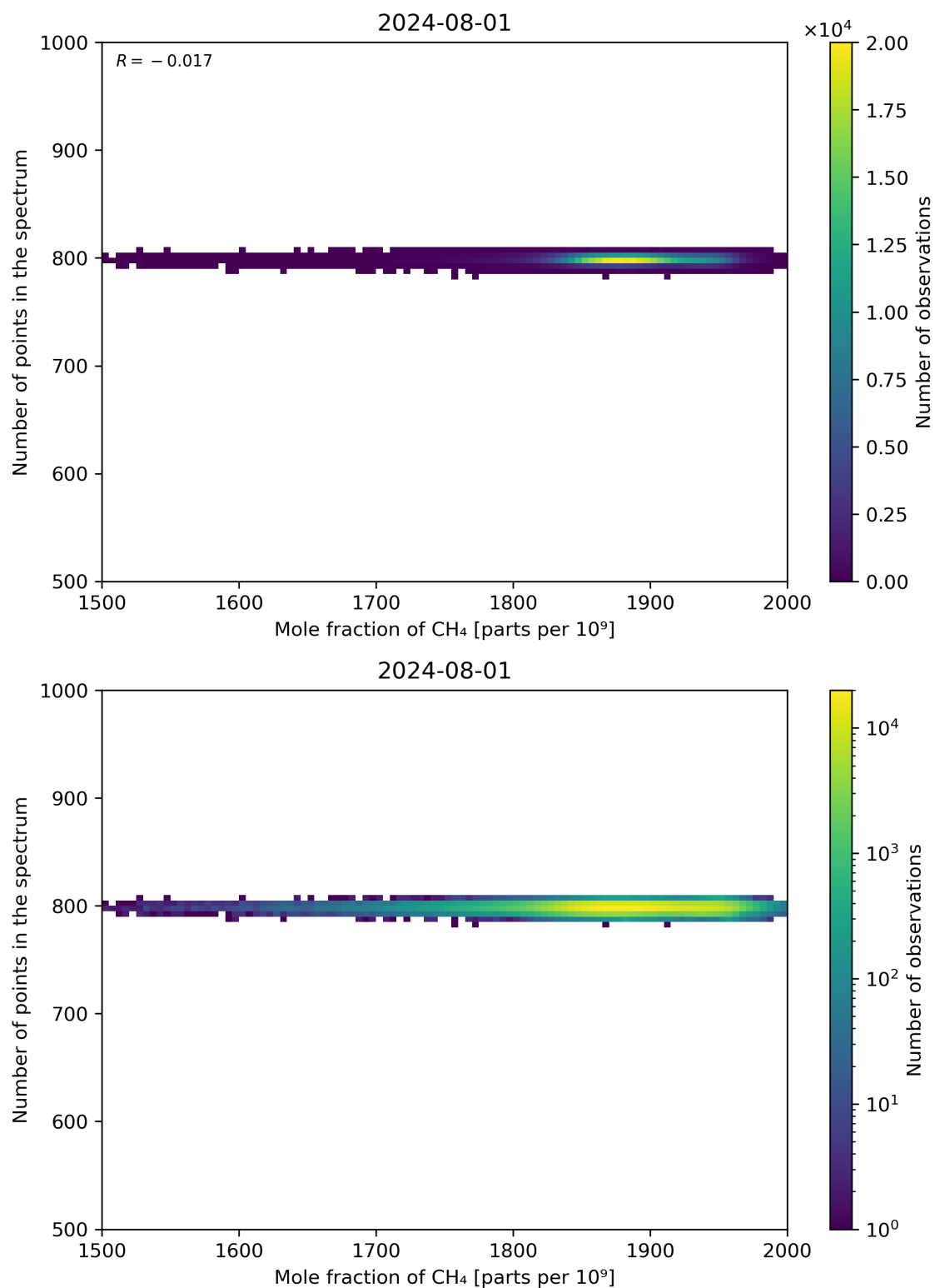
Figure 77: Scatter density plot of “Mole fraction of CH 4 ” against “Number of points in the spectrum” for 2024-07-31 to 2024-08-02.
