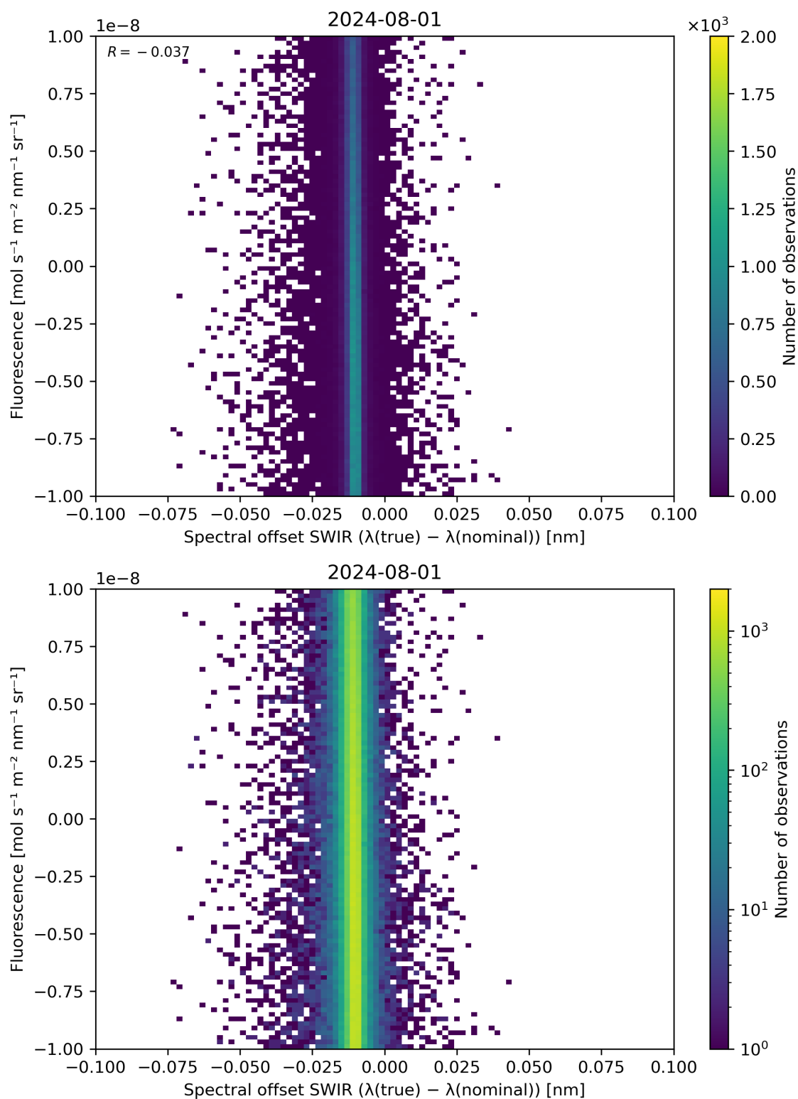
Figure 120: Scatter density plot of “Spectral offset SWIR ( \lambda(\text{true}) - \lambda(\text{nominal}) )” against “Fluorescence” for 2024-07-31 to 2024-08-02.
