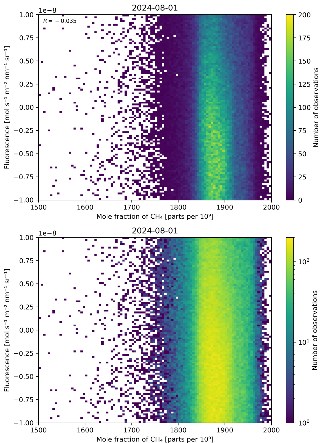
Figure 73: Scatter density plot of “Mole fraction of \text{CH}_4 ” against “Fluorescence” for 2024-07-31 to 2024-08-02.
