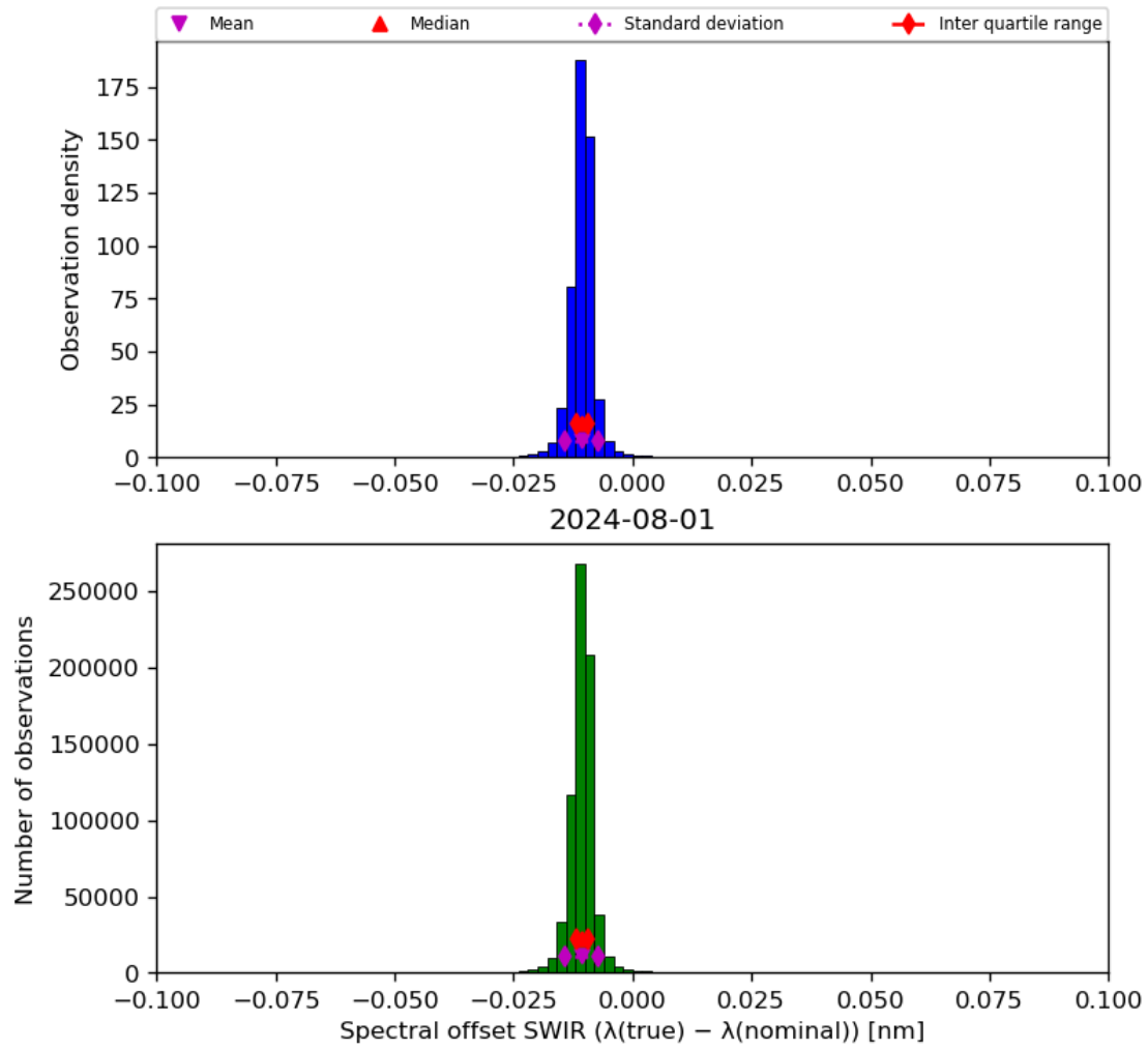
Figure 27: Histogram of “Spectral offset SWIR ( \lambda(\text{true}) - \lambda(\text{nominal}) )” for 2024-07-31 to 2024-08-02
