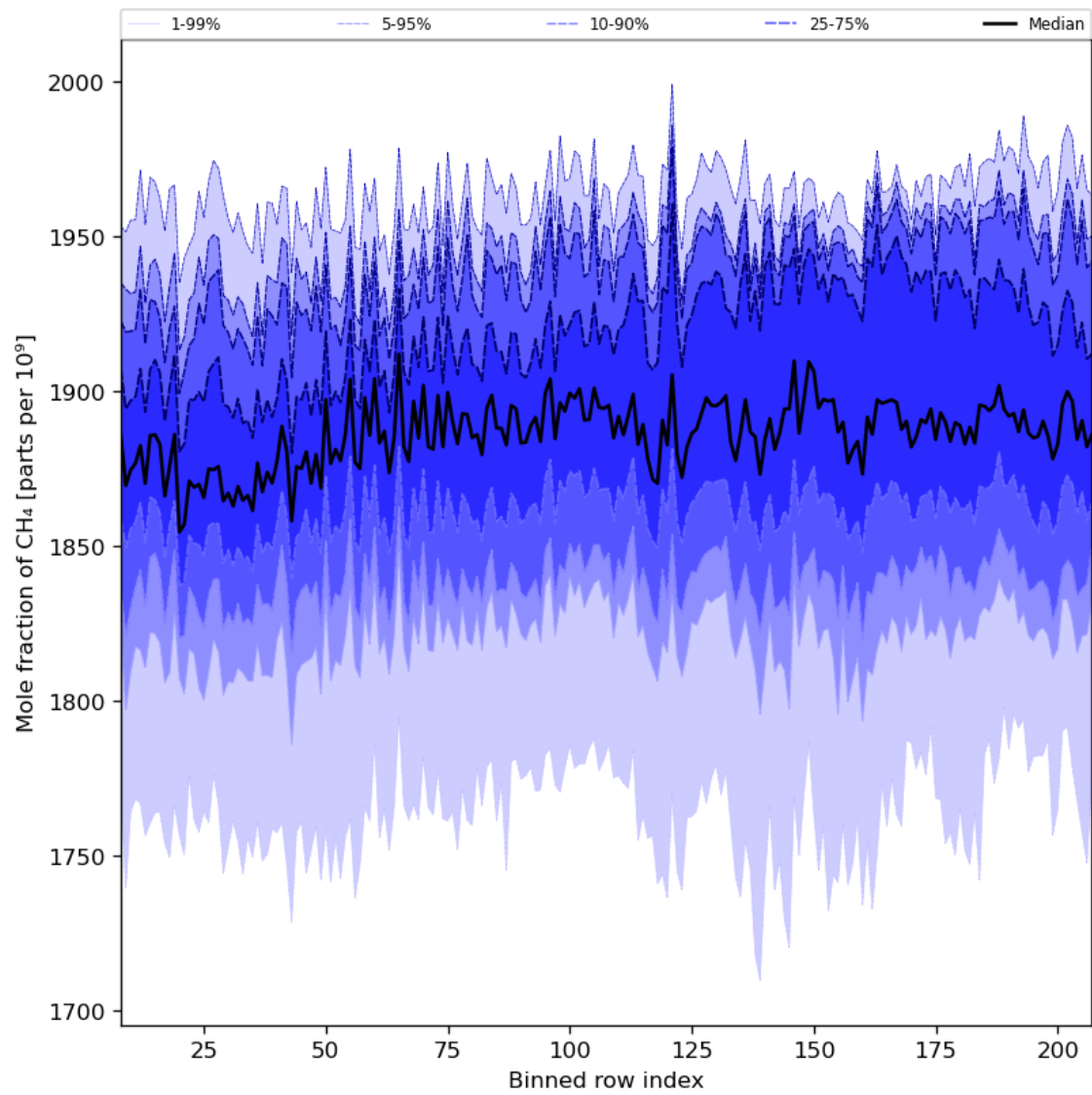
Figure 34: Along track statistics of “Mole fraction of CH 4 ” for 2024-07-31 to 2024-08-02
