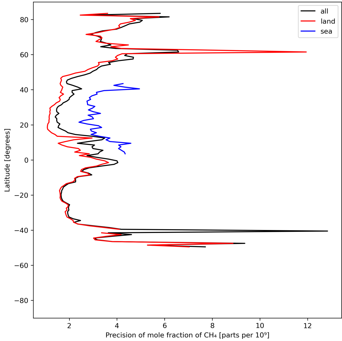
Figure 13: Zonal average of “Precision of mole fraction of CH 4 ” for 2024-07-31 to 2024-08-02.
