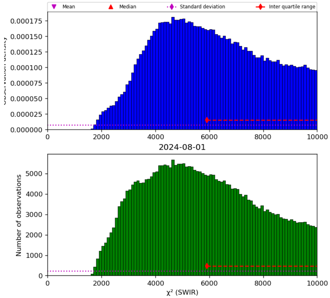
Figure 28: Histogram of “ \chi^2 (SWIR)” for 2024-07-31 to 2024-08-02
