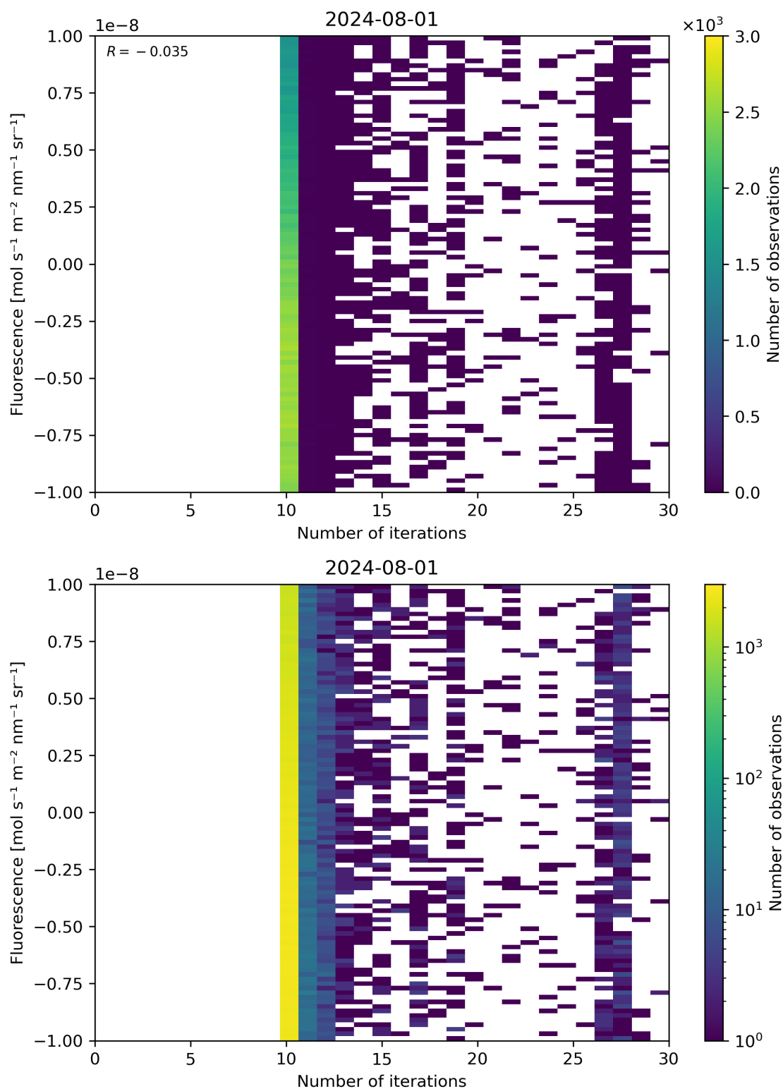
Figure 87: Scatter density plot of “Number of iterations” against “Fluorescence” for 2024-07-31 to 2024-08-02.
