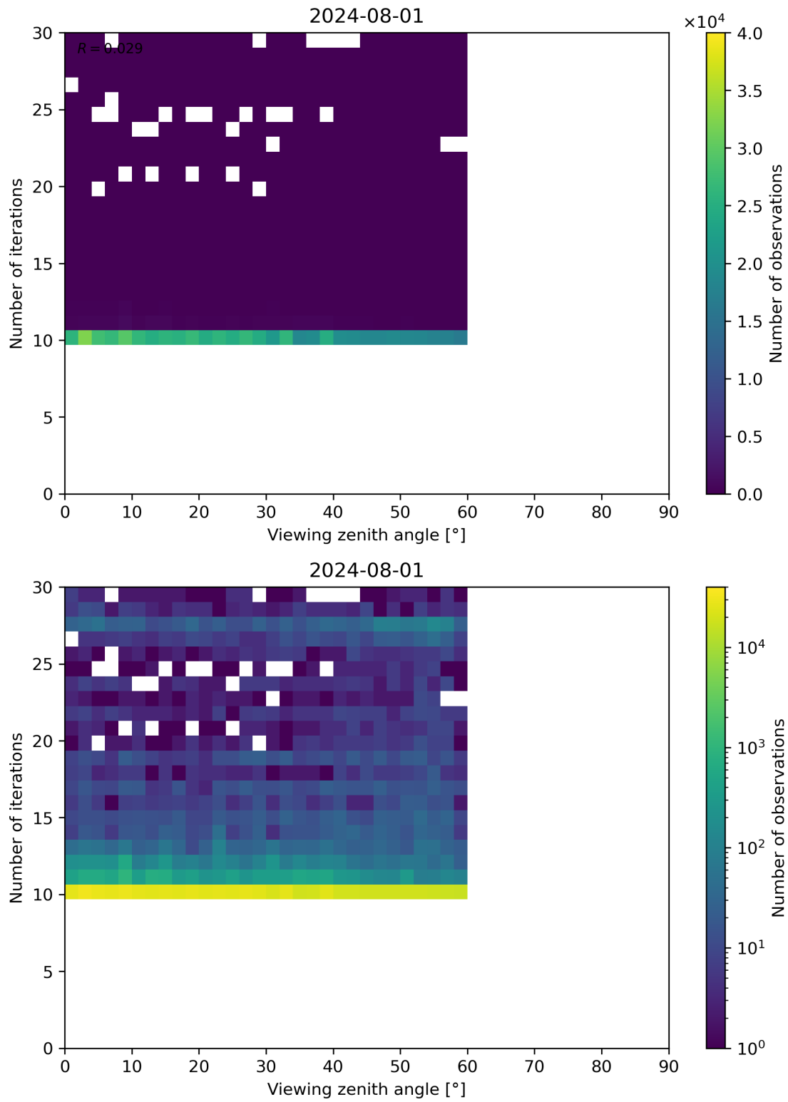
Figure 113: Scatter density plot of “Viewing zenith angle” against “Number of iterations” for 2024-07-31 to 2024-08-02.
