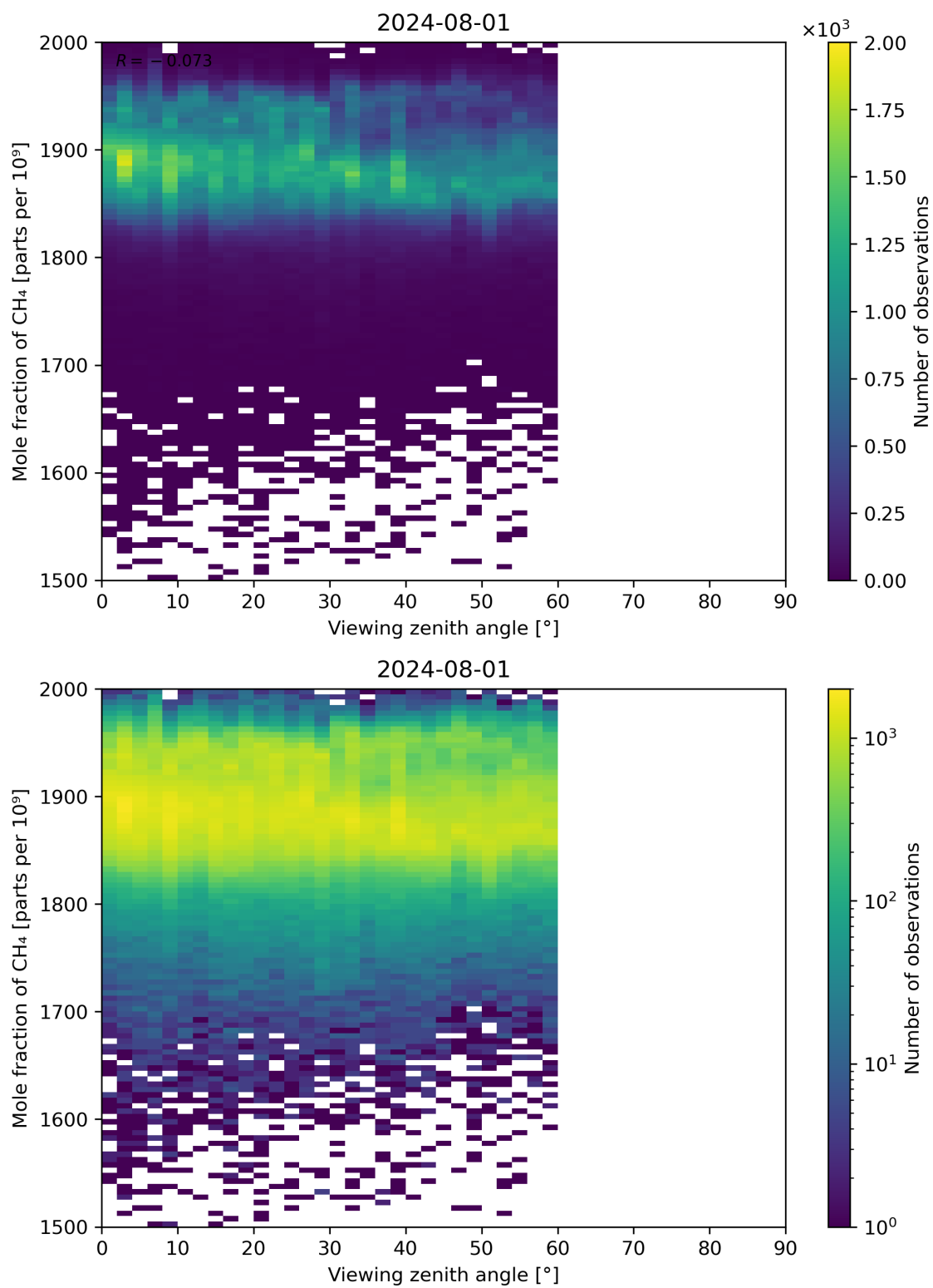
Figure 110: Scatter density plot of “Viewing zenith angle” against “Mole fraction of CH 4 ” for 2024-07-31 to 2024-08-02.
