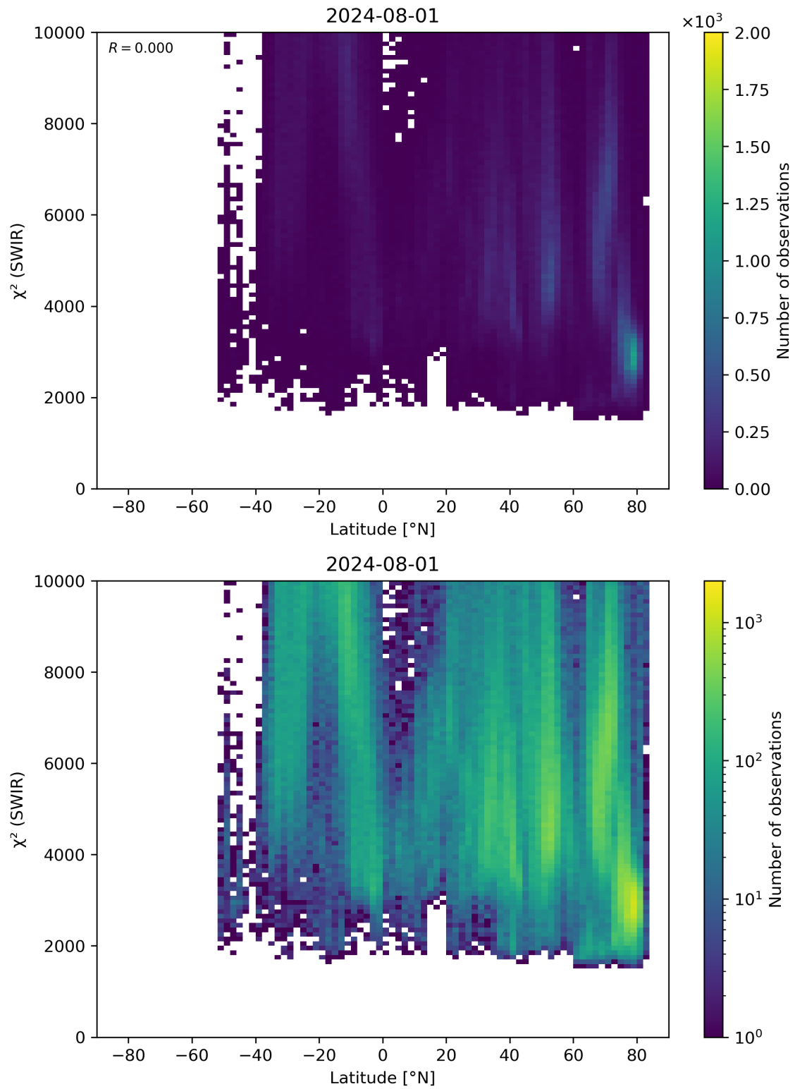
Figure 54: Scatter density plot of “Latitude” against “ \chi^2 (SWIR)” for 2024-07-31 to 2024-08-02.
