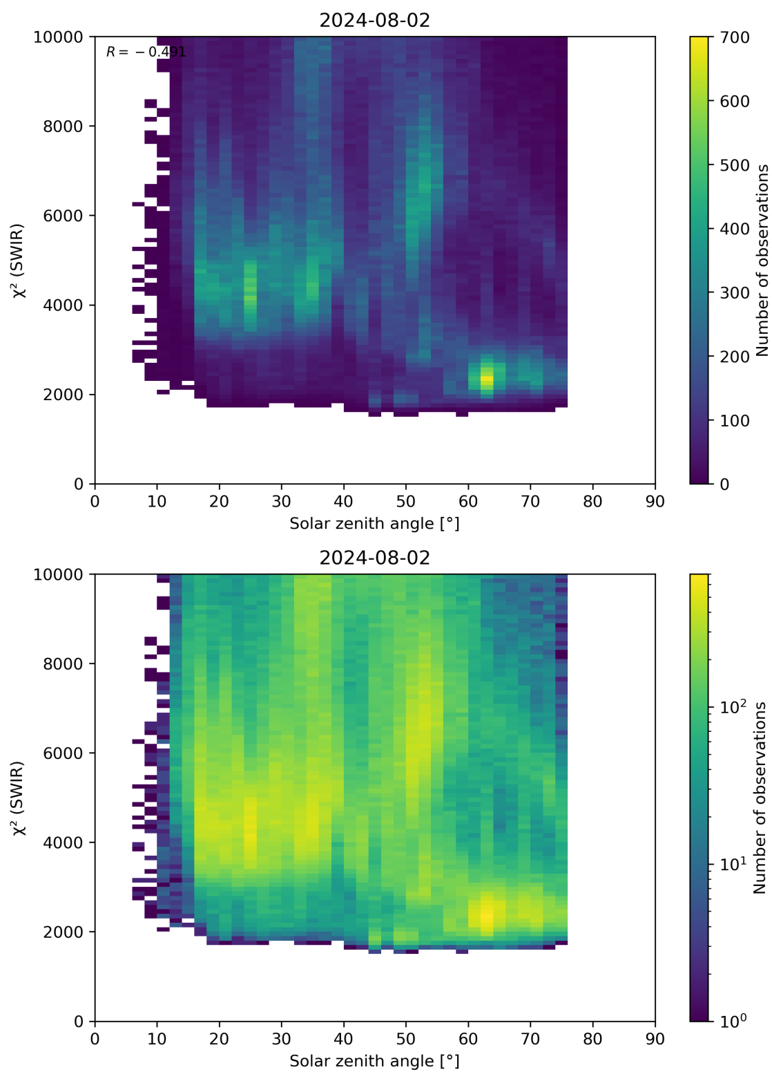
Figure 95: Scatter density plot of “Solar zenith angle” against “ \chi^2 (SWIR)” for 2024-08-01 to 2024-08-03.
