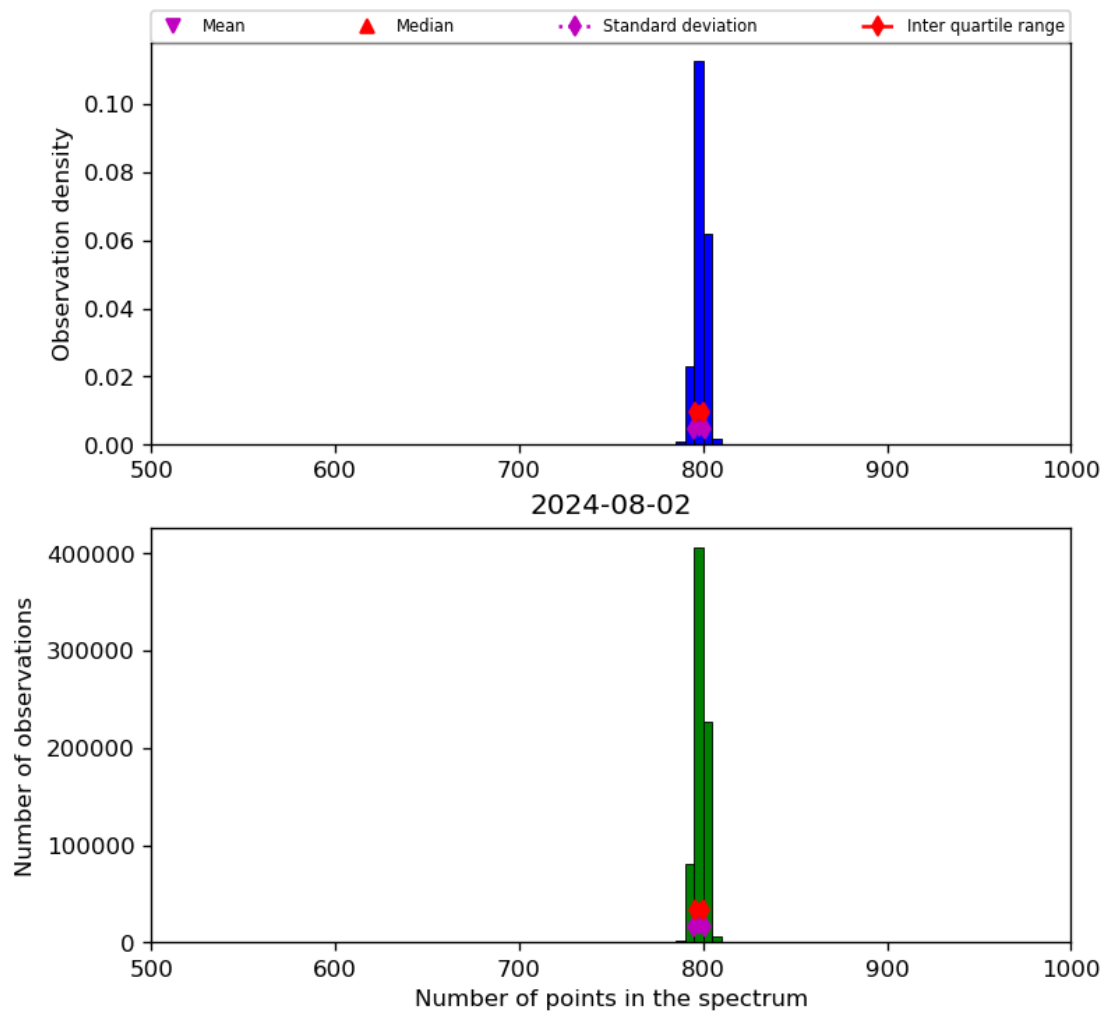
Figure 26: Histogram of “Number of points in the spectrum” for 2024-08-01 to 2024-08-03
