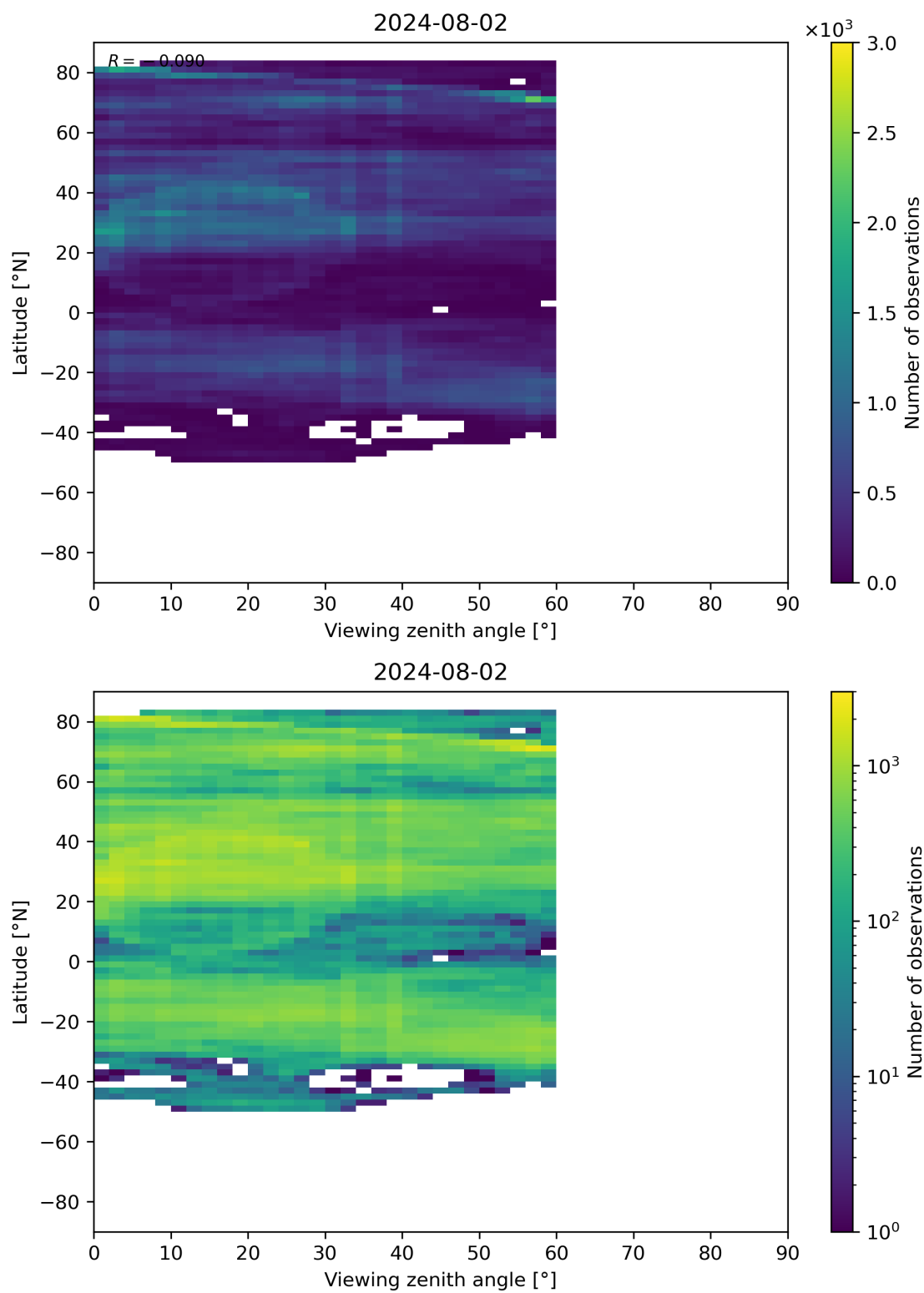
Figure 109: Scatter density plot of “Viewing zenith angle” against “Latitude” for 2024-08-01 to 2024-08-03.
