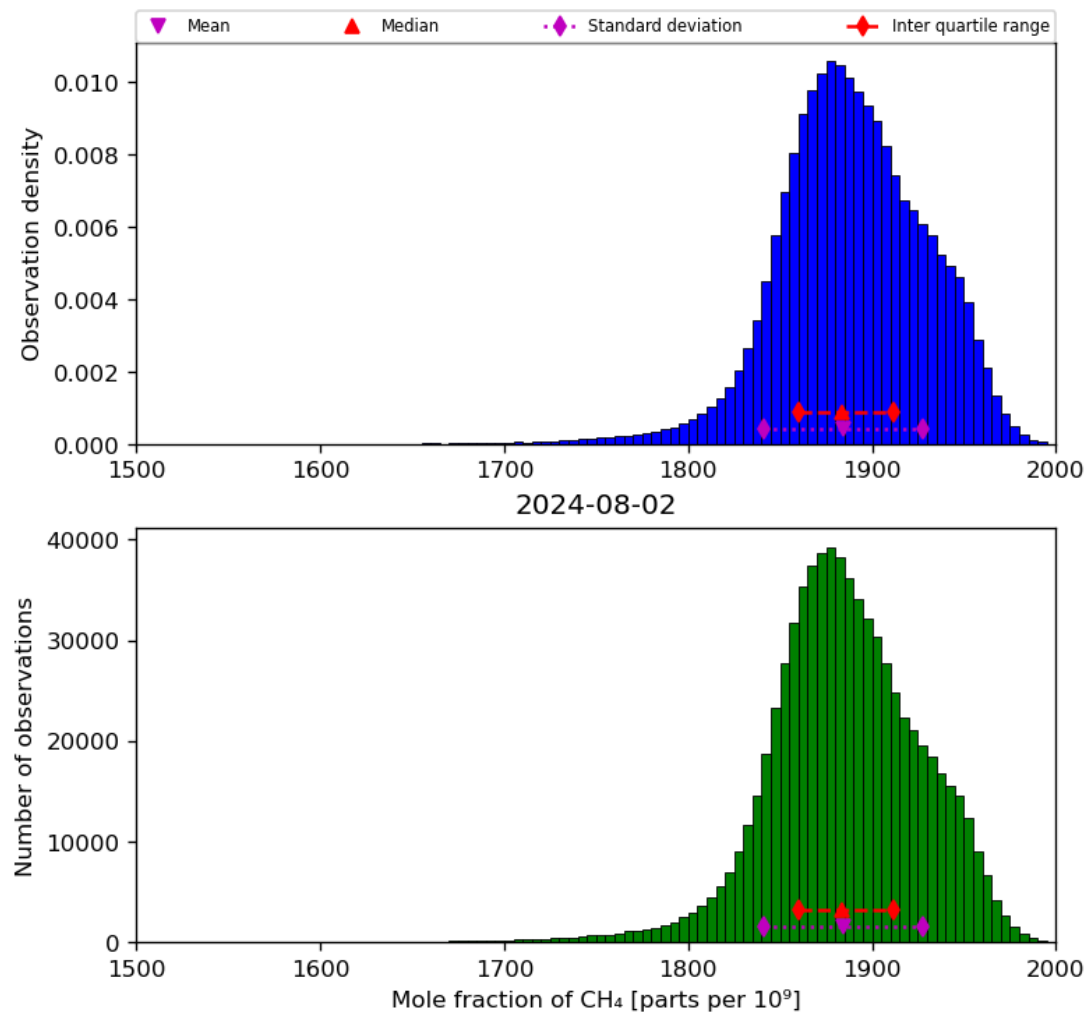
Figure 23: Histogram of “Mole fraction of CH 4 ” for 2024-08-01 to 2024-08-03
