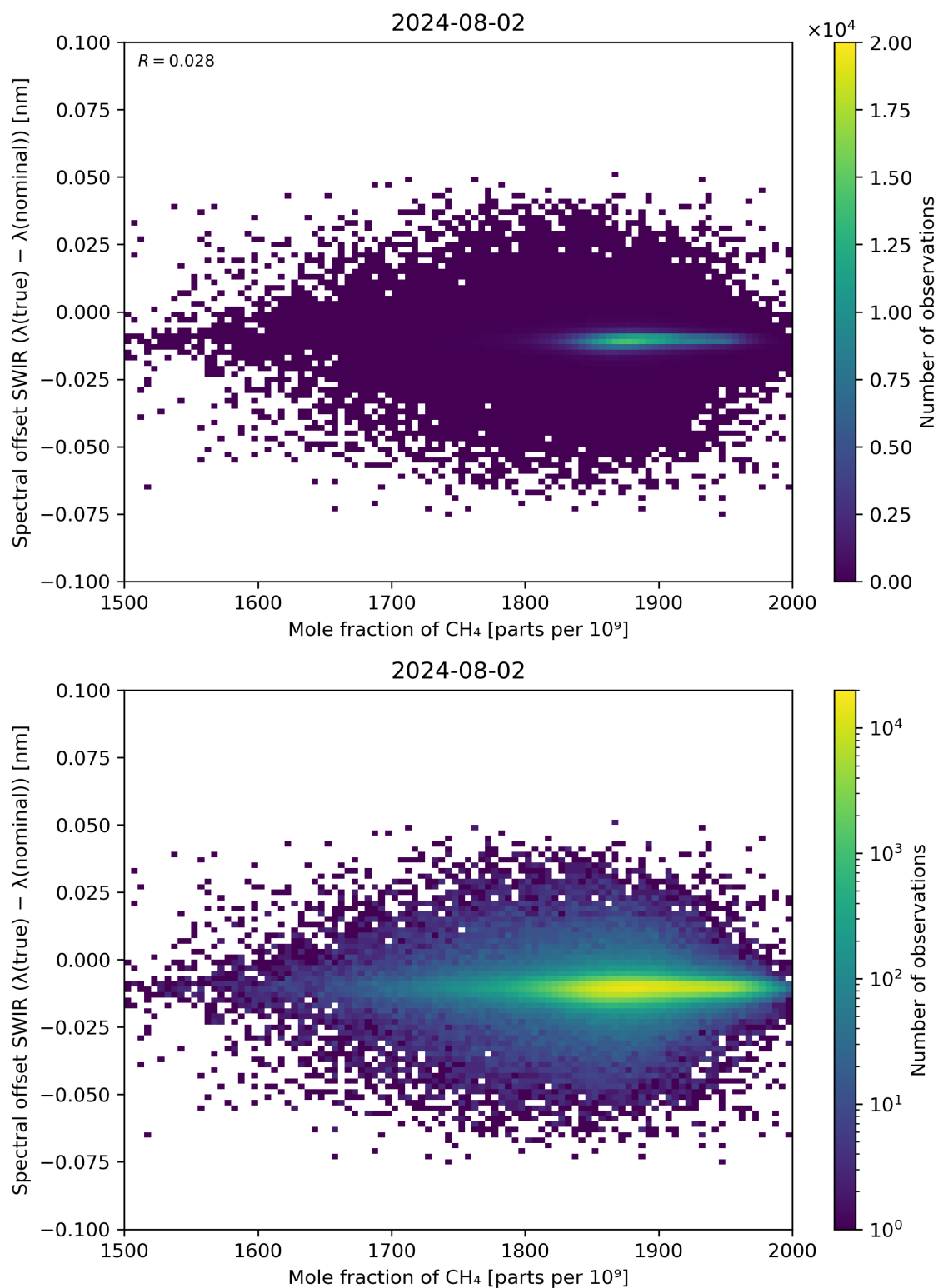
Figure 86: Scatter density plot of “Mole fraction of CH 4 ” against “Spectral offset SWIR ( \lambda(\text{true}) - \lambda(\text{nominal}) )” for 2024-08-01 to 2024-08-03.
