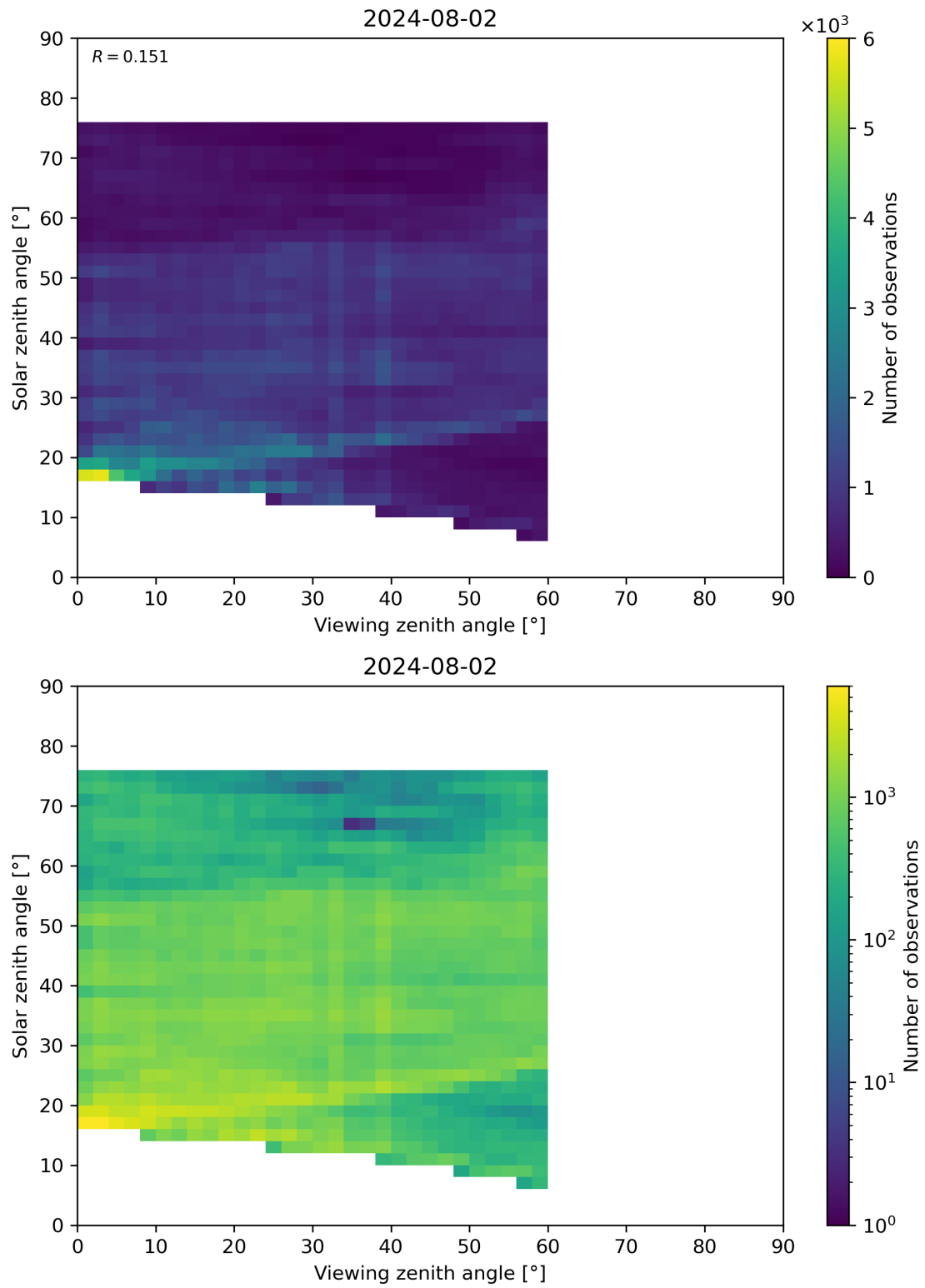
Figure 115: Scatter density plot of “Viewing zenith angle” against “Solar zenith angle” for 2024-08-01 to 2024-08-03.
