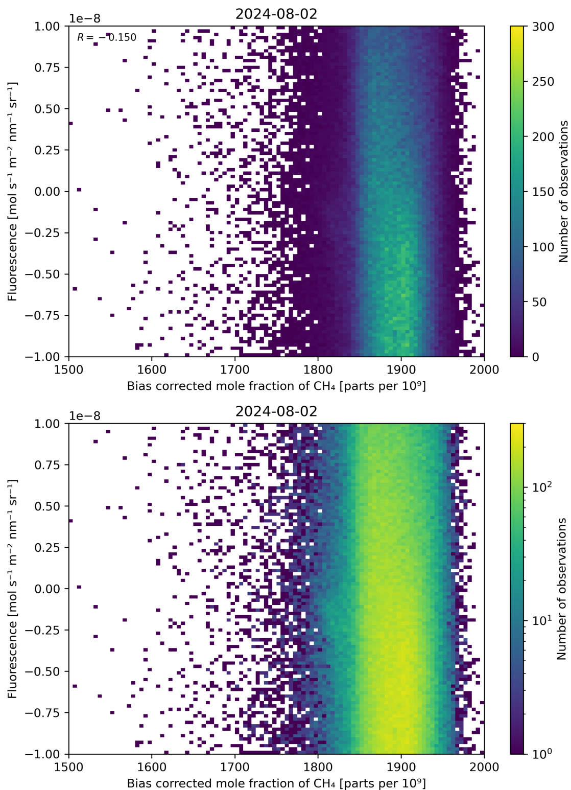
Figure 66: Scatter density plot of “Bias corrected mole fraction of \text{CH}_4 ” against “Fluorescence” for 2024-08-01 to 2024-08-03.
