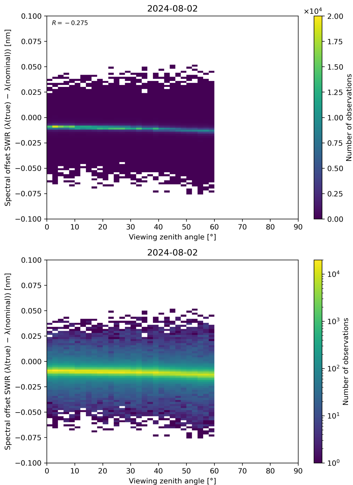
Figure 116: Scatter density plot of “Viewing zenith angle” against “Spectral offset SWIR ( \lambda(\text{true}) - \lambda(\text{nominal}) )” for 2024-08-01 to 2024-08-03.
