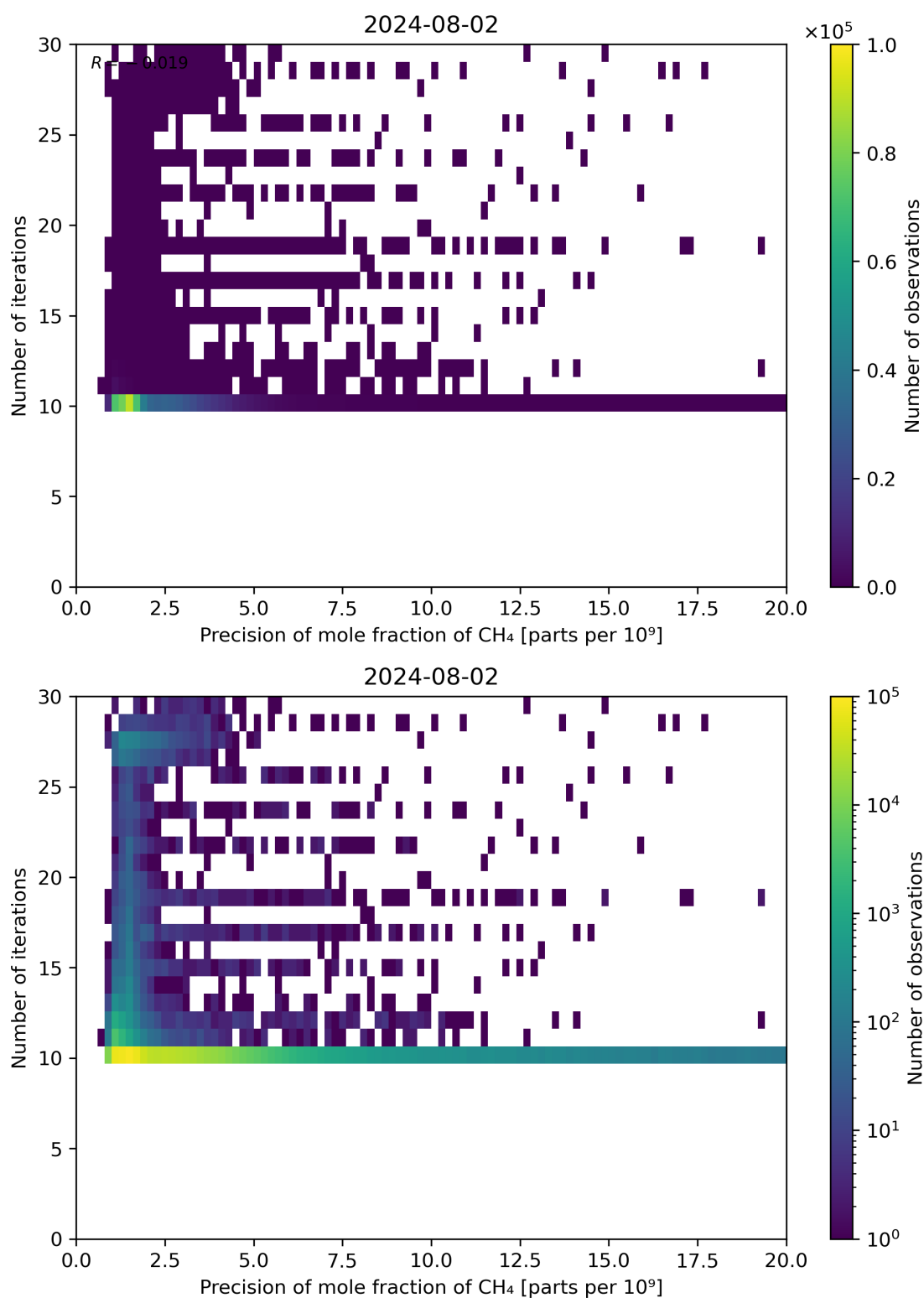
Figure 83: Scatter density plot of “Precision of mole fraction of CH 4 ” against “Number of iterations” for 2024-08-01 to 2024-08-03.
