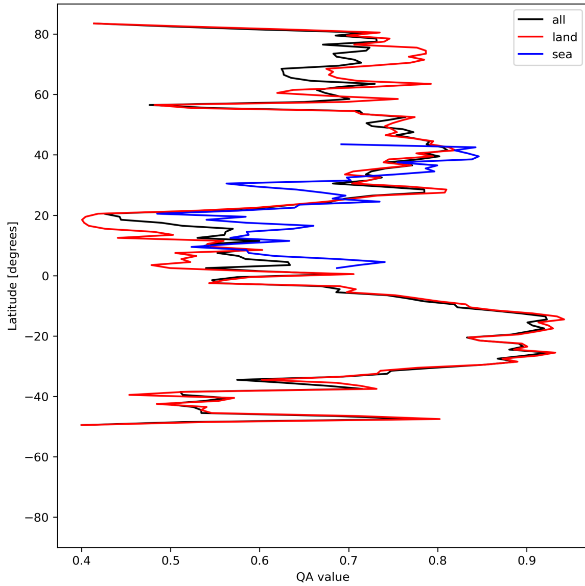
Figure 11: Zonal average of “QA value” for 2024-08-01 to 2024-08-03.
