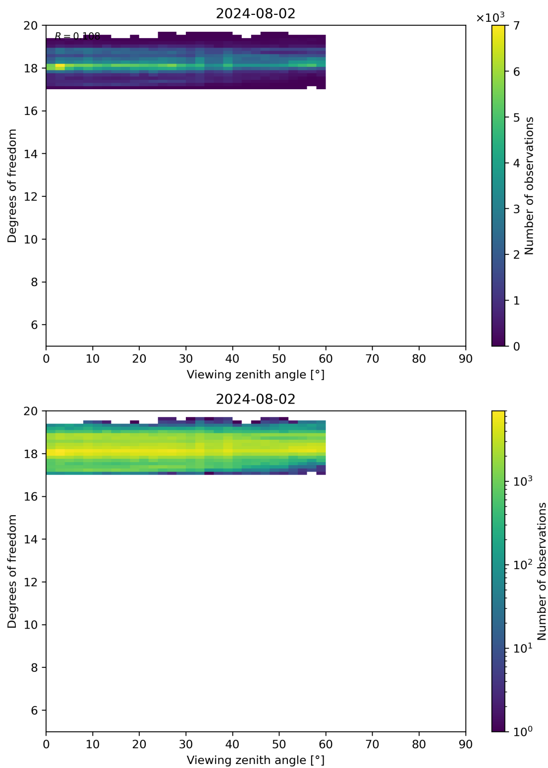
Figure 107: Scatter density plot of “Viewing zenith angle” against “Degrees of freedom” for 2024-08-01 to 2024-08-03.
