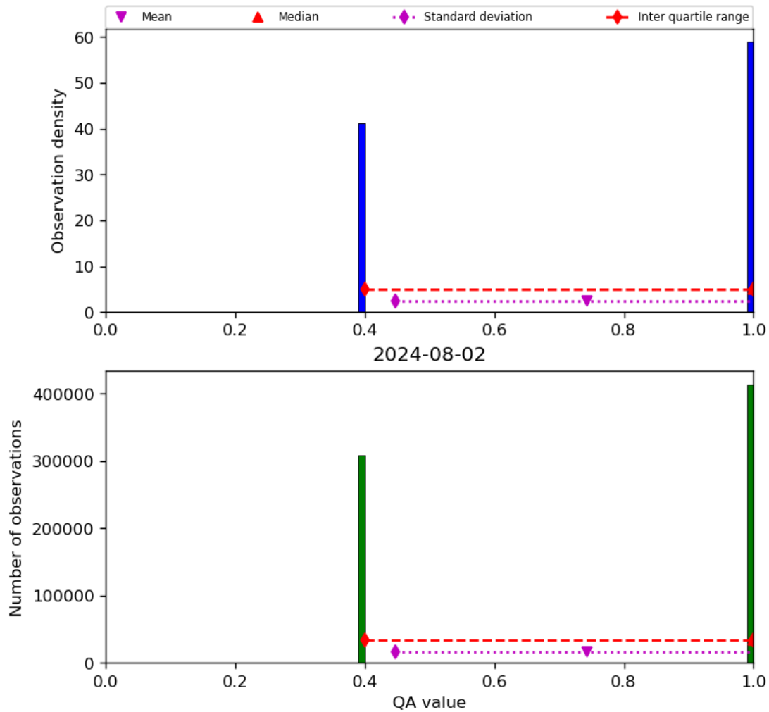
Figure 22: Histogram of “QA value” for 2024-08-01 to 2024-08-03
