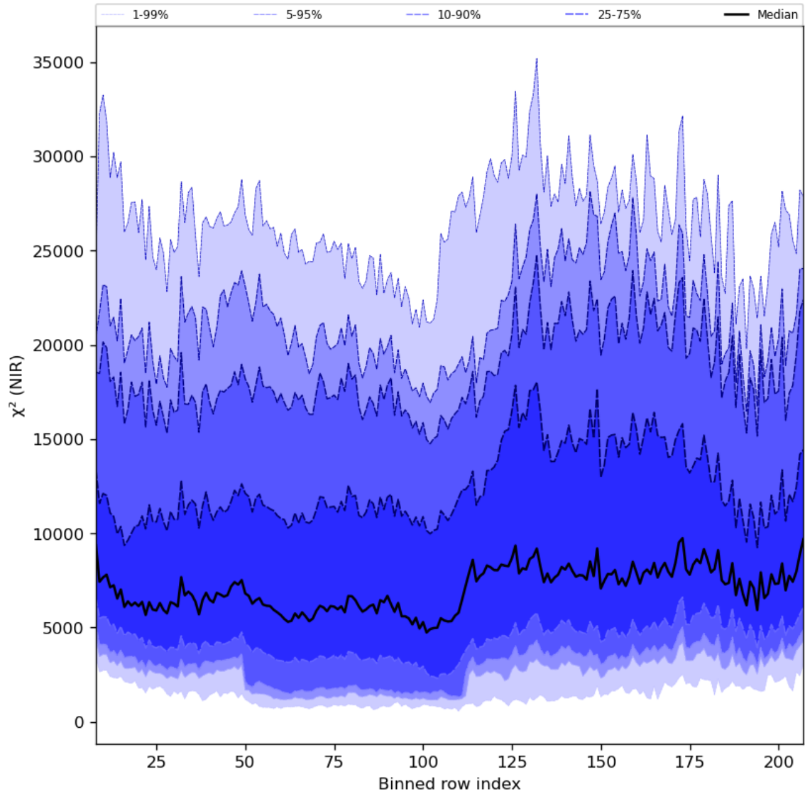
Figure 40: Along track statistics of “ \chi^2 (NIR)” for 2024-08-01 to 2024-08-03
