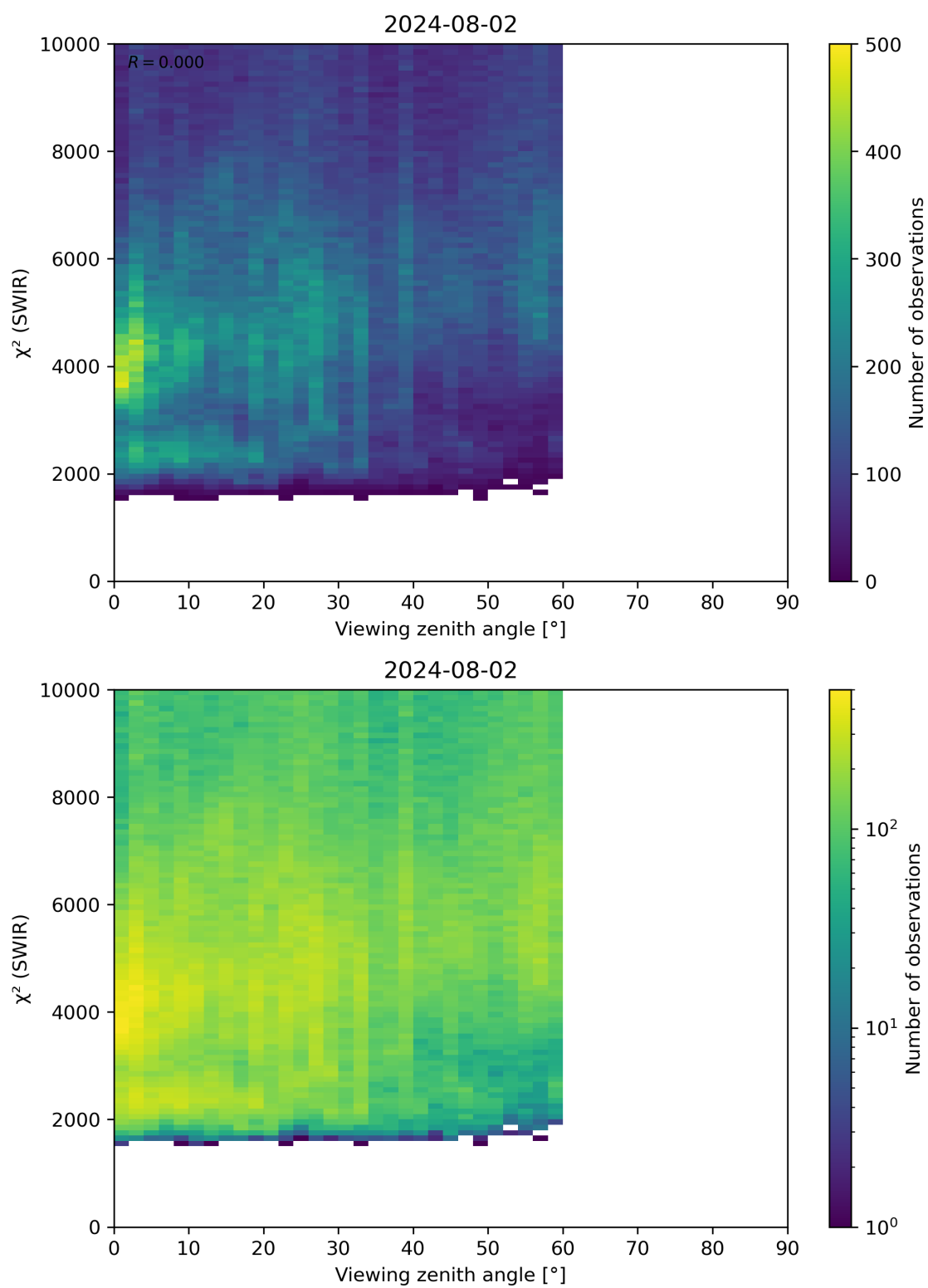
Figure 106: Scatter density plot of “Viewing zenith angle” against “ \chi^2 (SWIR)” for 2024-08-01 to 2024-08-03.
