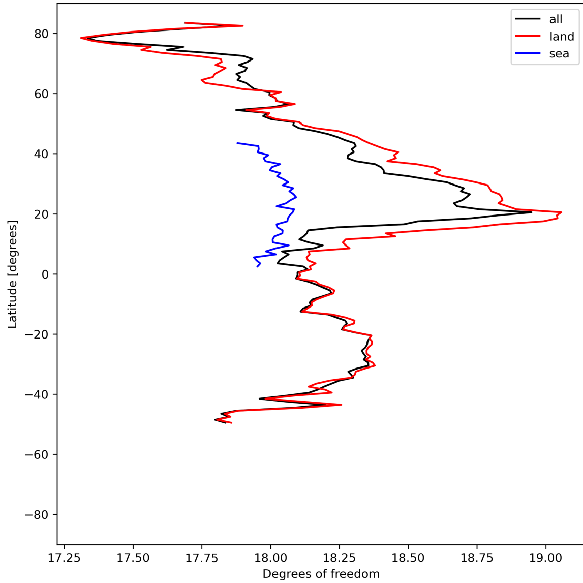
Figure 19: Zonal average of “Degrees of freedom” for 2024-08-01 to 2024-08-03.
