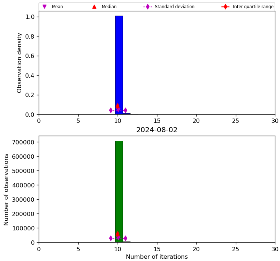
Figure 31: Histogram of “Number of iterations” for 2024-08-01 to 2024-08-03
