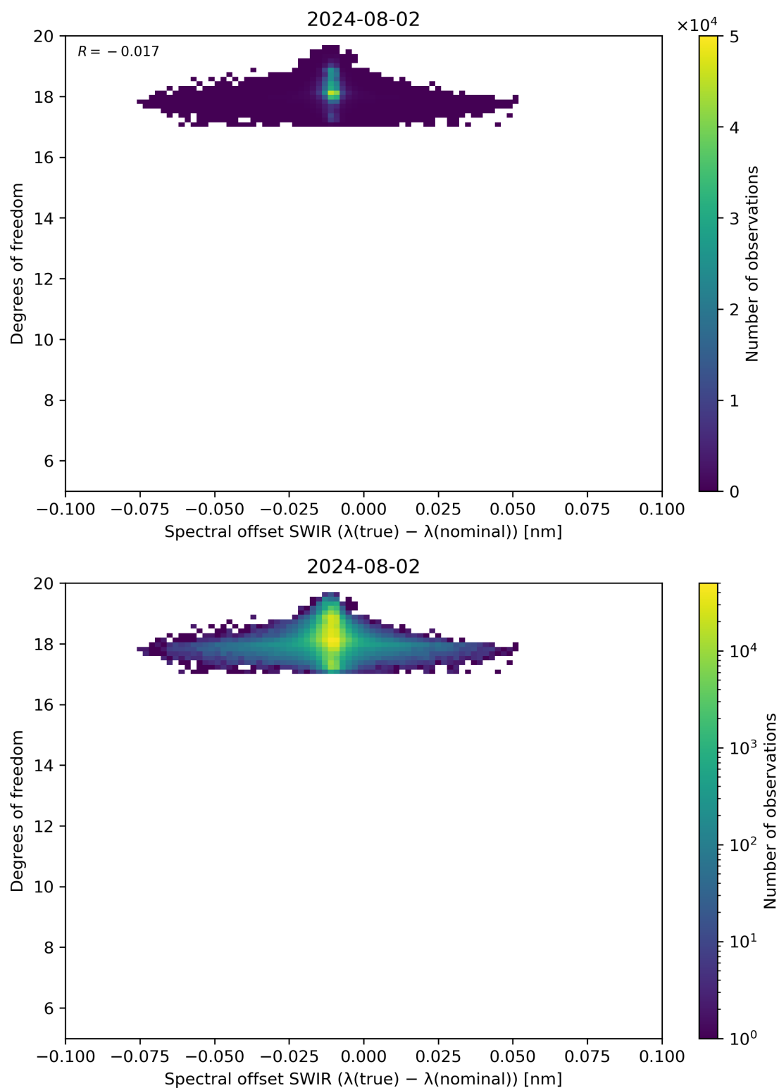
Figure 119: Scatter density plot of “Spectral offset SWIR ( \lambda(\text{true}) - \lambda(\text{nominal}) )” against “Degrees of freedom” for 2024-08-01 to 2024-08-03.
