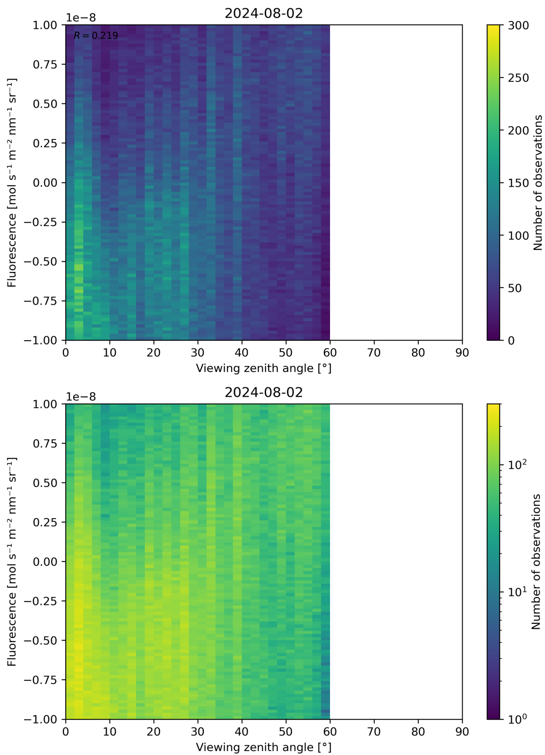
Figure 108: Scatter density plot of “Viewing zenith angle” against “Fluorescence” for 2024-08-01 to 2024-08-03.
