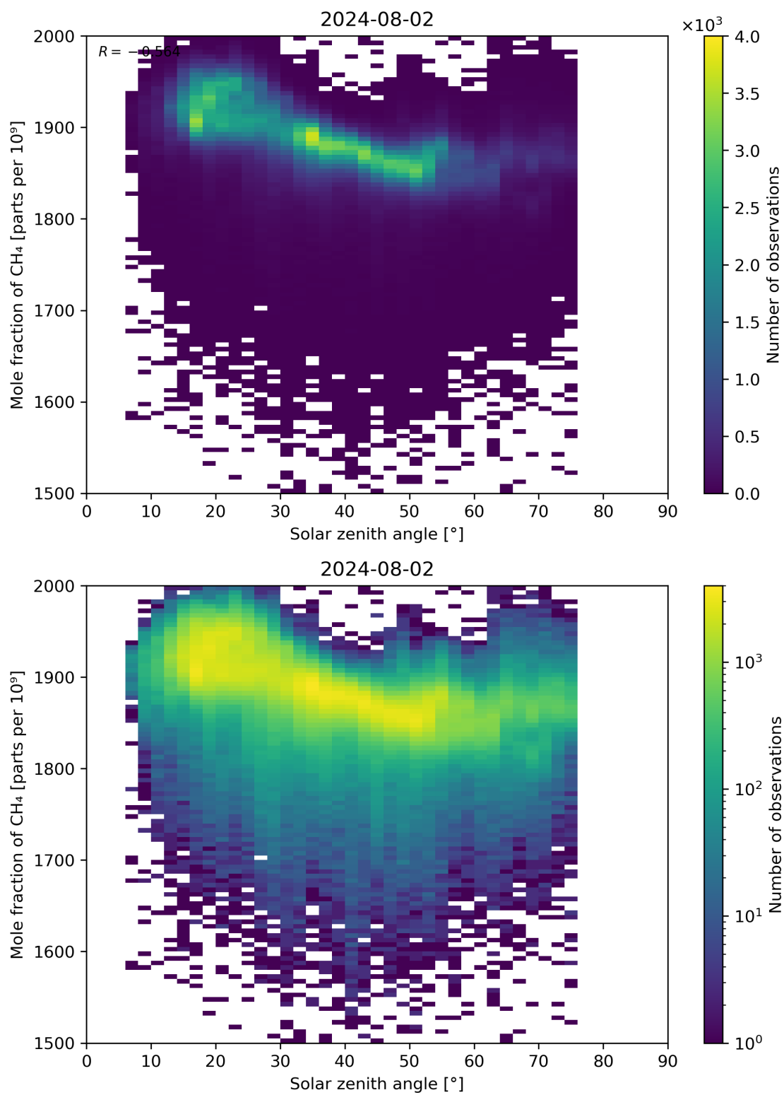
Figure 99: Scatter density plot of “Solar zenith angle” against “Mole fraction of CH 4 ” for 2024-08-01 to 2024-08-03.
