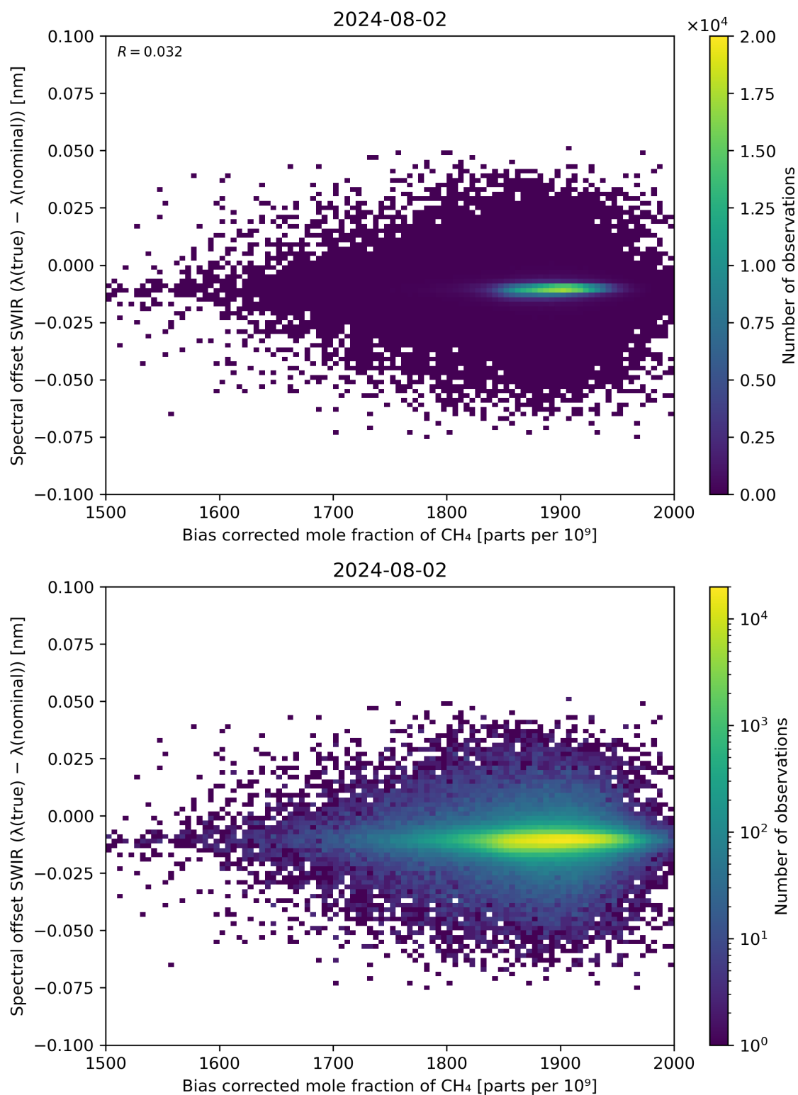
Figure 69: Scatter density plot of “Bias corrected mole fraction of \text{CH}_4 ” against “Spectral offset SWIR ( \lambda(\text{true}) - \lambda(\text{nominal}) )” for 2024-08-01 to 2024-08-03.
