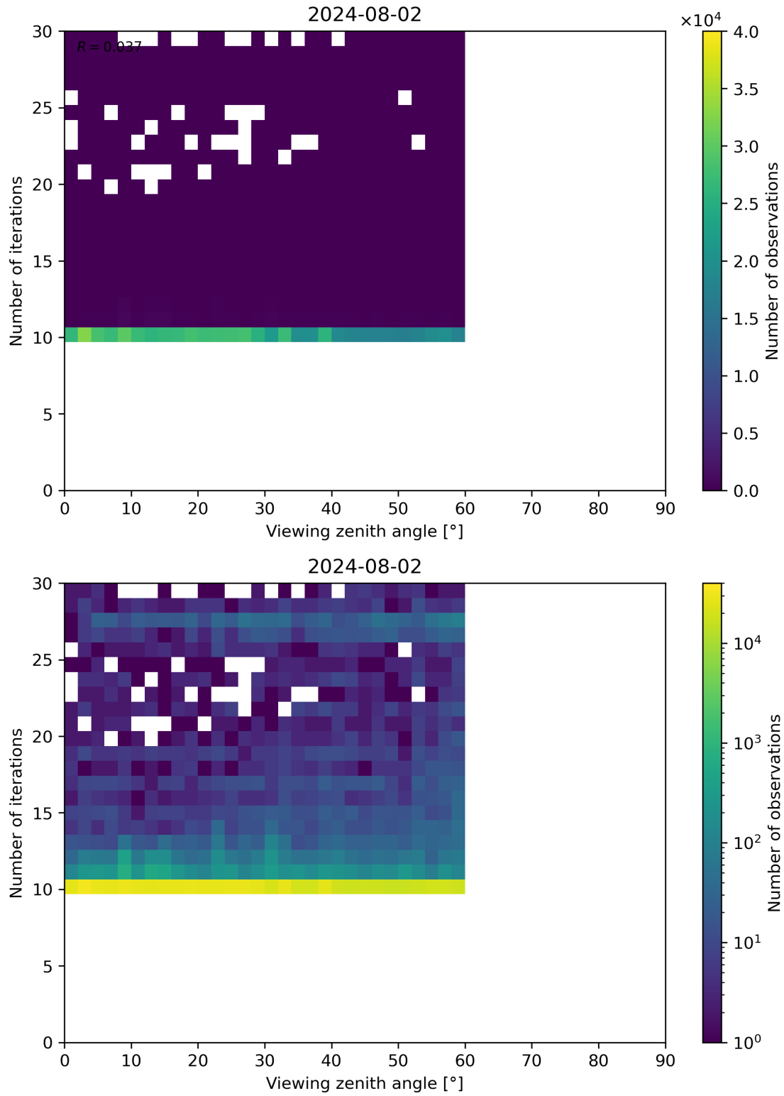
Figure 113: Scatter density plot of “Viewing zenith angle” against “Number of iterations” for 2024-08-01 to 2024-08-03.
