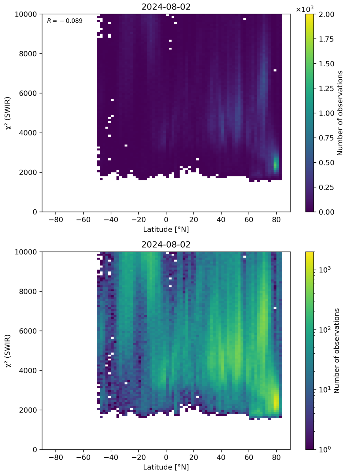
Figure 54: Scatter density plot of “Latitude” against “ \chi^2 (SWIR)” for 2024-08-01 to 2024-08-03.
