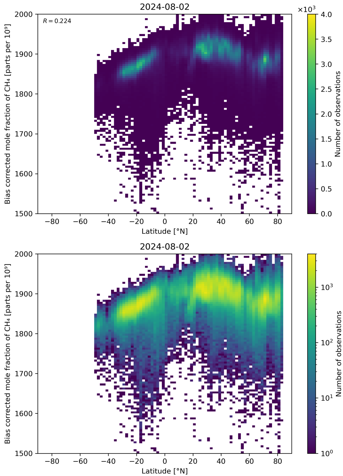
Figure 58: Scatter density plot of “Latitude” against “Bias corrected mole fraction of CH 4 ” for 2024-08-01 to 2024-08-03.
