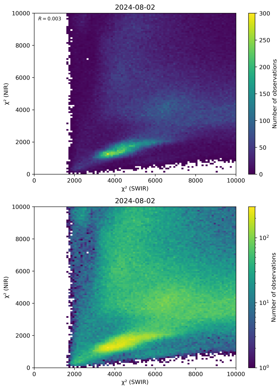
Figure 47: Scatter density plot of “ \chi^2 (SWIR)” against “ \chi^2 (NIR)” for 2024-08-01 to 2024-08-03.
