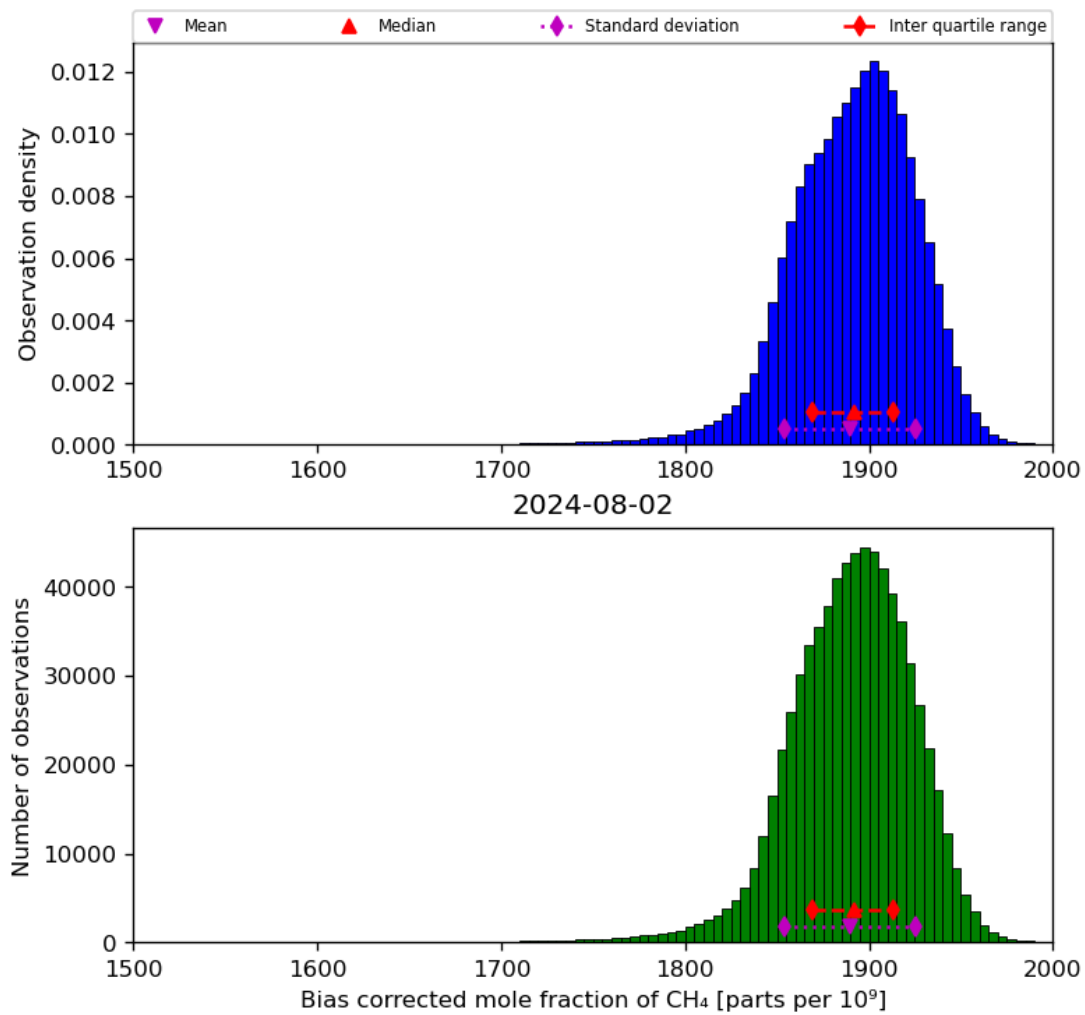
Figure 25: Histogram of “Bias corrected mole fraction of CH 4 ” for 2024-08-01 to 2024-08-03
