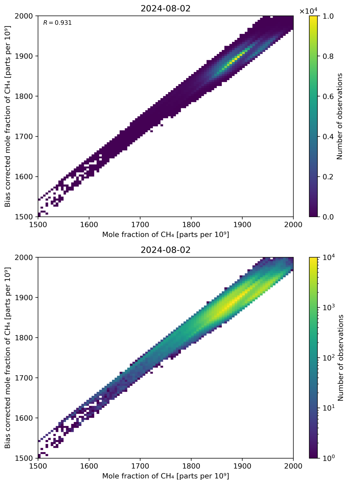
Figure 74: Scatter density plot of “Mole fraction of CH 4 ” against “Bias corrected mole fraction of CH 4 ” for 2024-08-01 to 2024-08-03.
