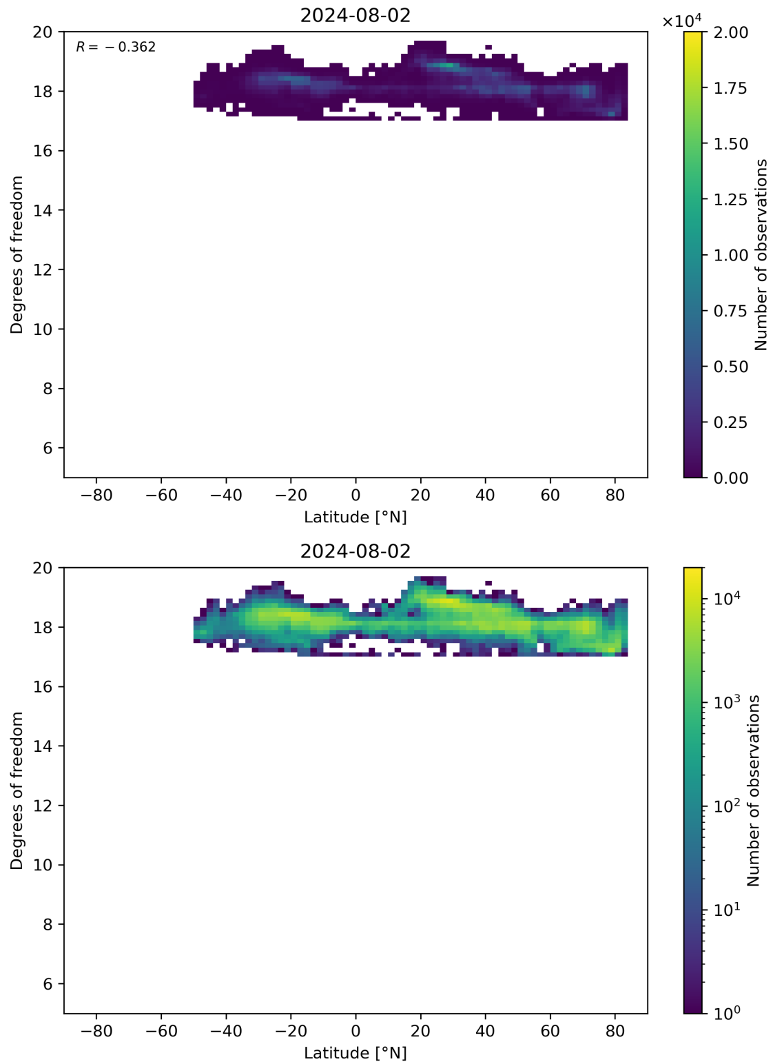
Figure 55: Scatter density plot of “Latitude” against “Degrees of freedom” for 2024-08-01 to 2024-08-03.
