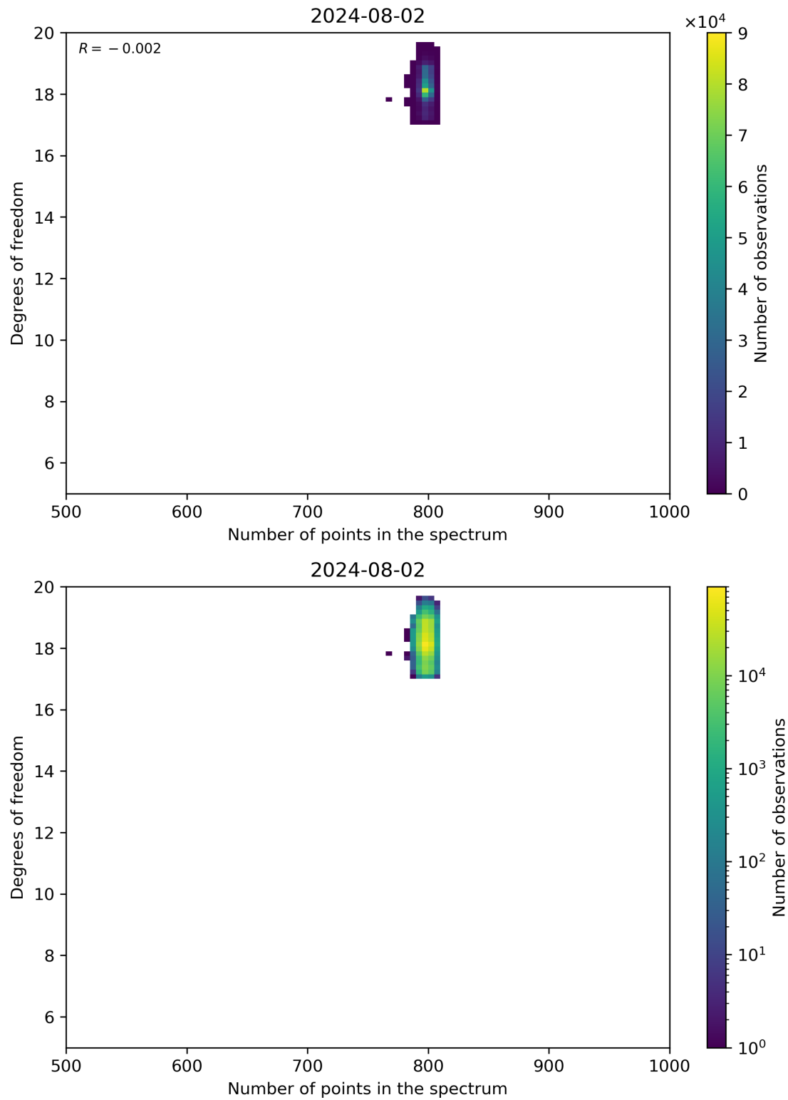
Figure 90: Scatter density plot of “Number of points in the spectrum” against “Degrees of freedom” for 2024-08-01 to 2024-08-03.
