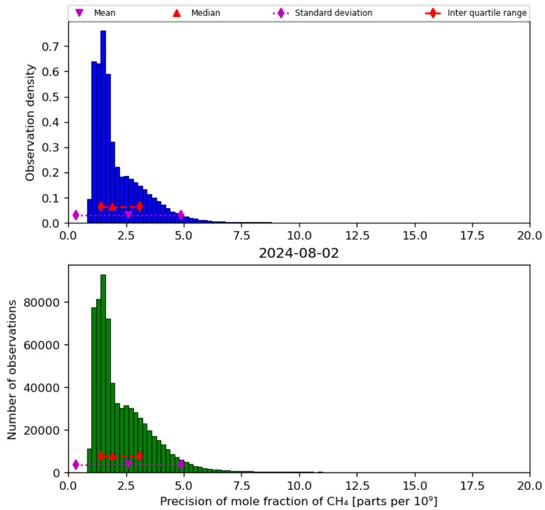
Figure 24: Histogram of “Precision of mole fraction of CH 4 ” for 2024-08-01 to 2024-08-03
