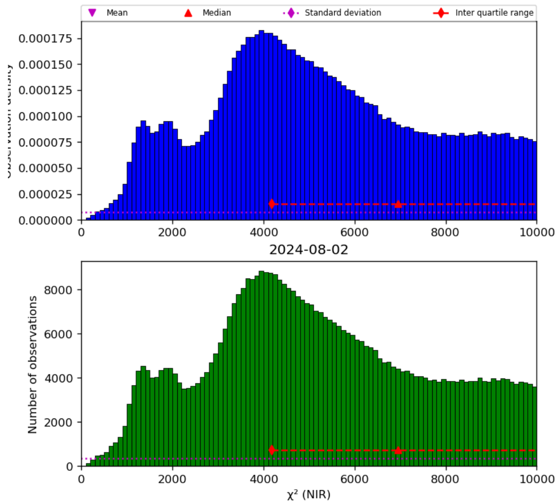
Figure 29: Histogram of “ \chi^2 (NIR)” for 2024-08-01 to 2024-08-03
