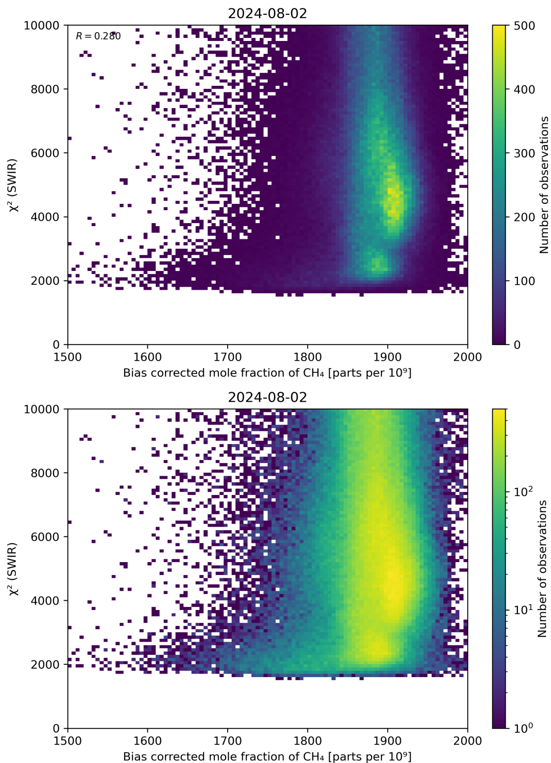
Figure 64: Scatter density plot of “Bias corrected mole fraction of CH 4 ” against “ \chi^2 (SWIR)” for 2024-08-01 to 2024-08-03.
