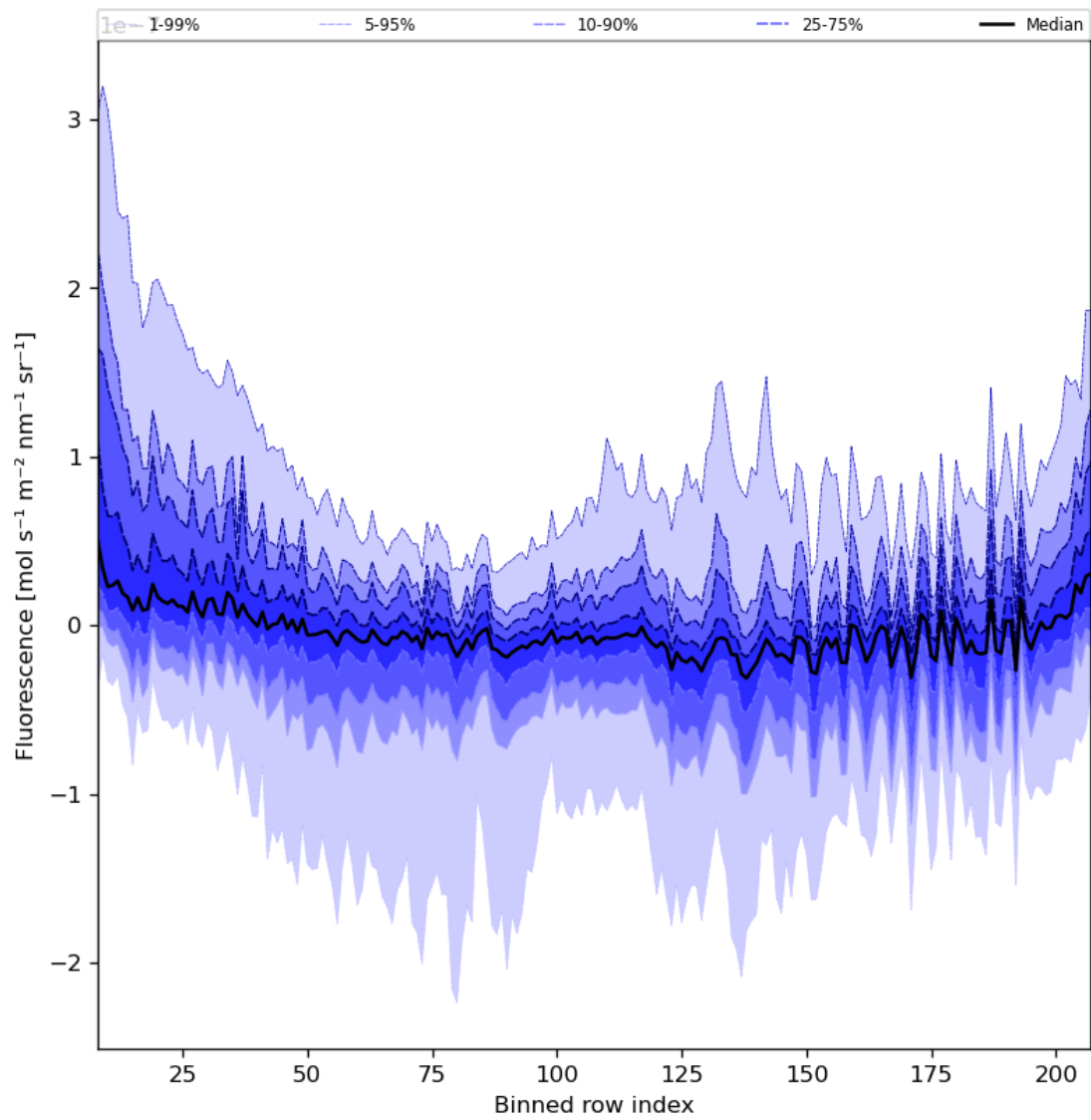
Figure 43: Along track statistics of “Fluorescence” for 2024-08-01 to 2024-08-03
