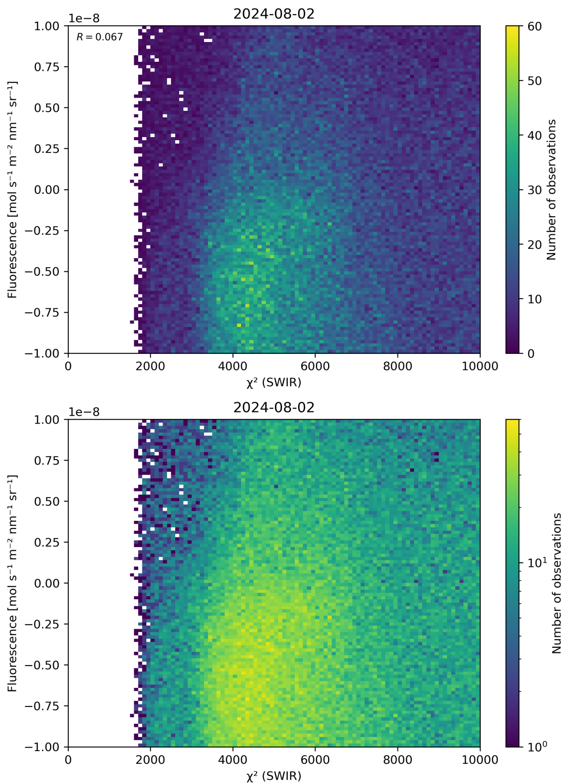
Figure 49: Scatter density plot of “ \chi^2 (SWIR)” against “Fluorescence” for 2024-08-01 to 2024-08-03.
