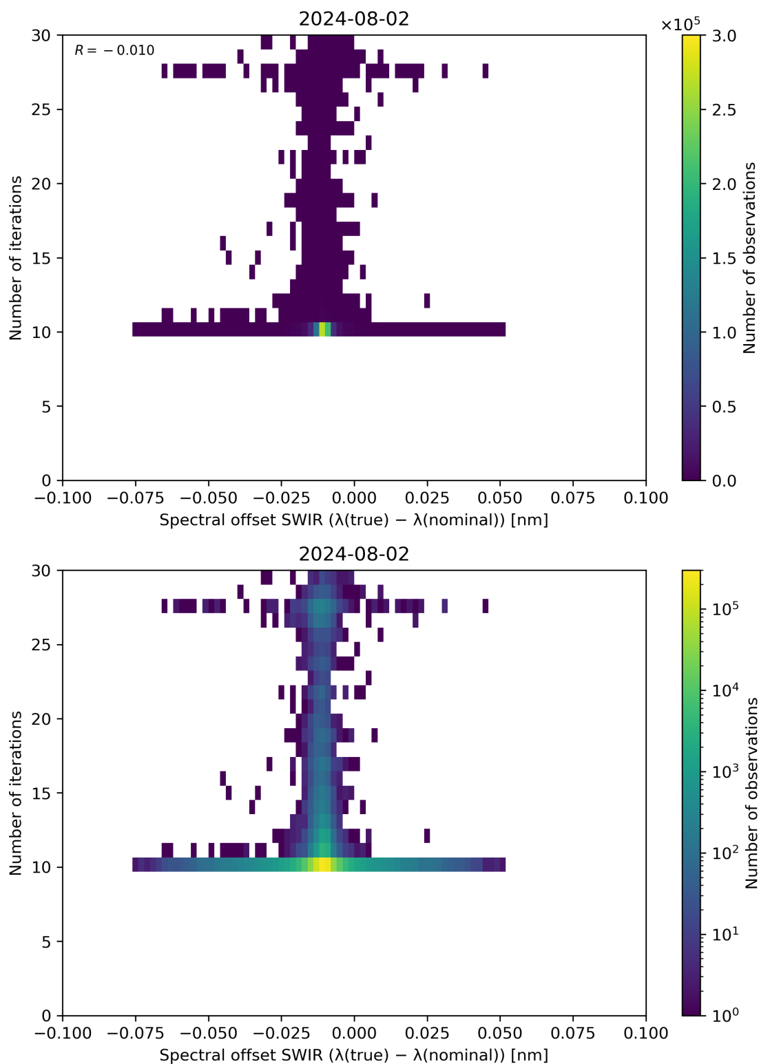
Figure 121: Scatter density plot of “Spectral offset SWIR ( \lambda(\text{true}) - \lambda(\text{nominal}) )” against “Number of iterations” for 2024-08-01 to 2024-08-03.
