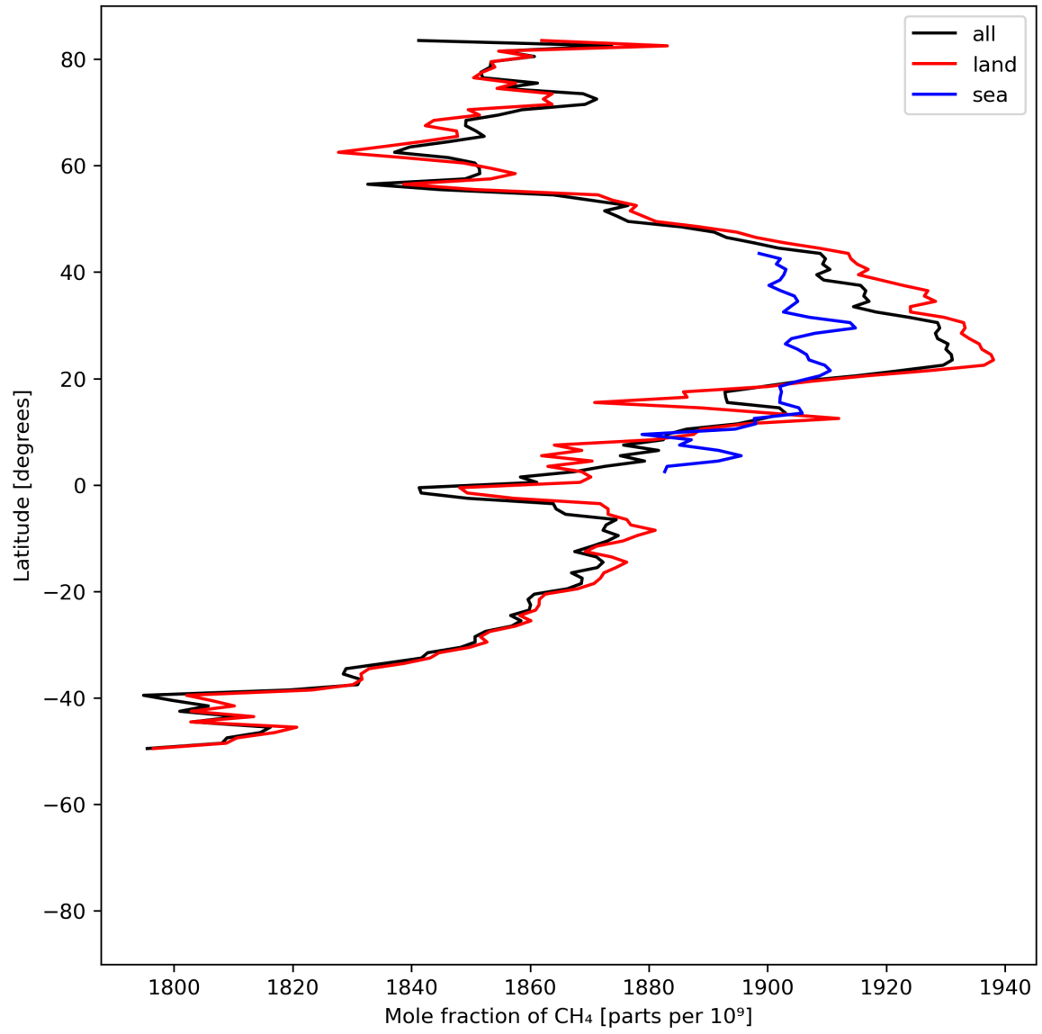
Figure 12: Zonal average of “Mole fraction of \text{CH}_4 ” for 2024-08-01 to 2024-08-03.
