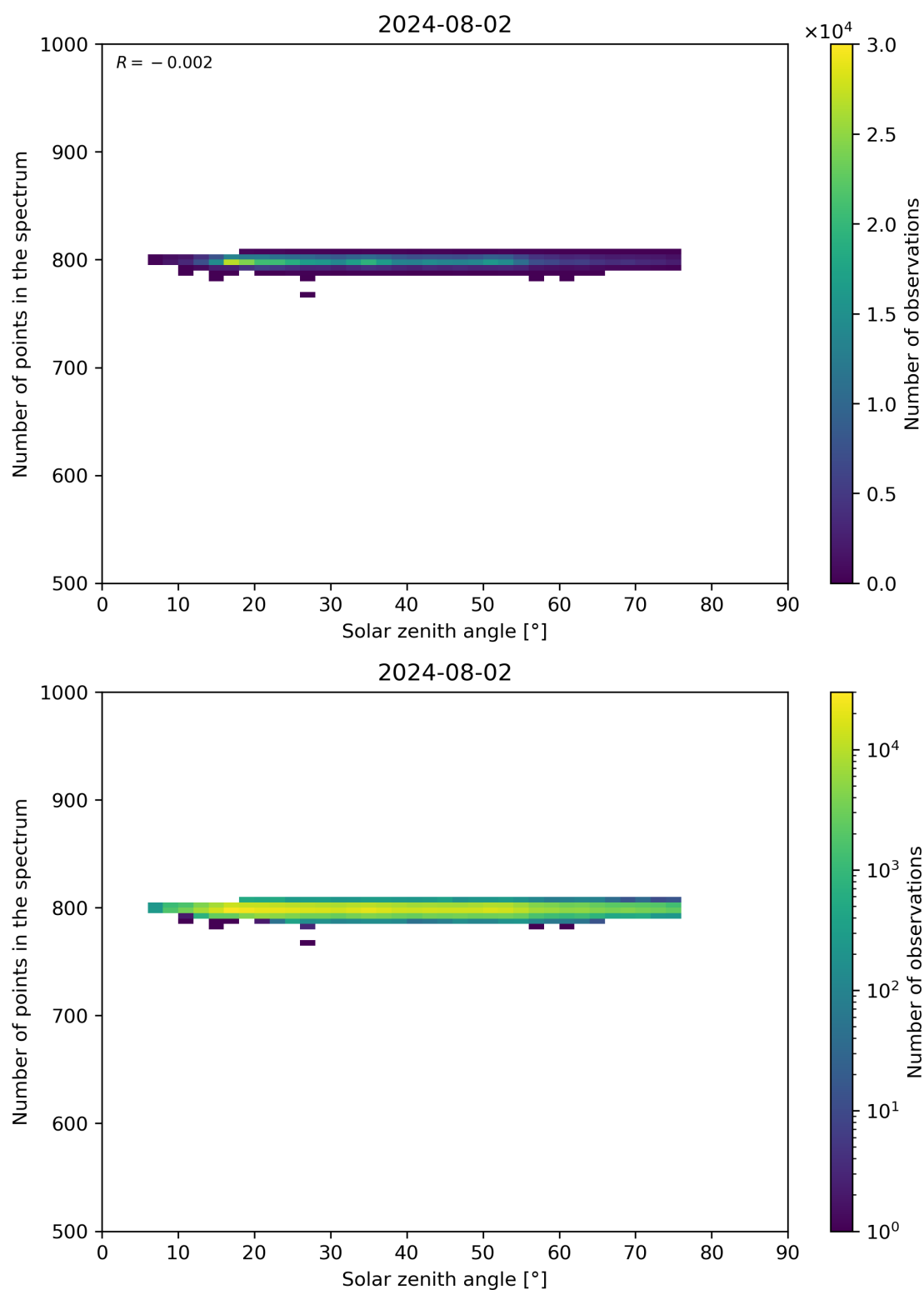
Figure 103: Scatter density plot of “Solar zenith angle” against “Number of points in the spectrum” for 2024-08-01 to 2024-08-03.
