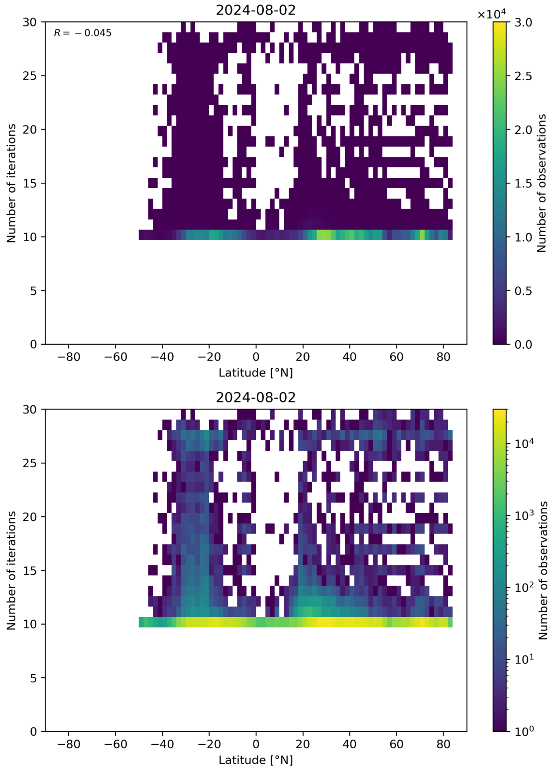
Figure 60: Scatter density plot of “Latitude” against “Number of iterations” for 2024-08-01 to 2024-08-03.
