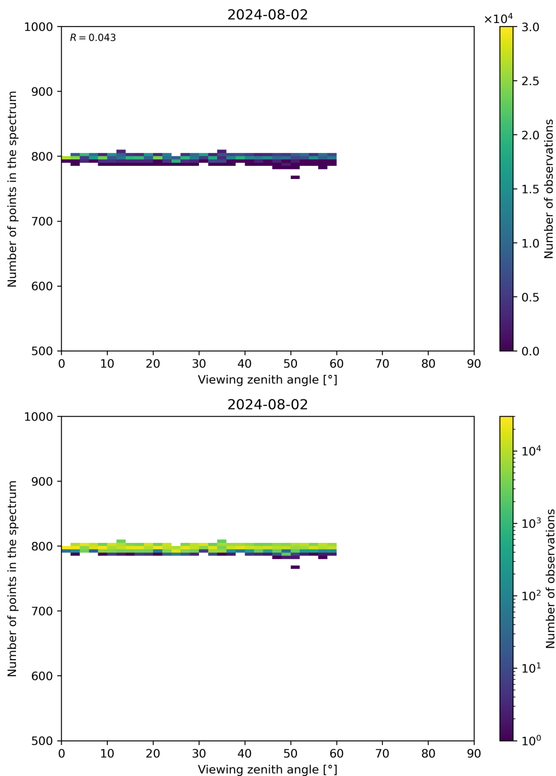
Figure 114: Scatter density plot of “Viewing zenith angle” against “Number of points in the spectrum” for 2024-08-01 to 2024-08-03.
