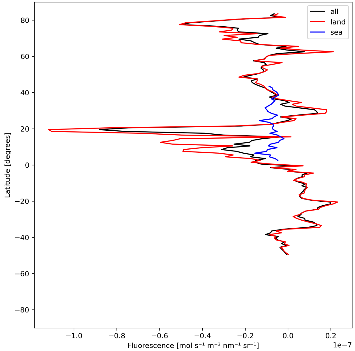
Figure 21: Zonal average of “Fluorescence” for 2024-08-01 to 2024-08-03.
