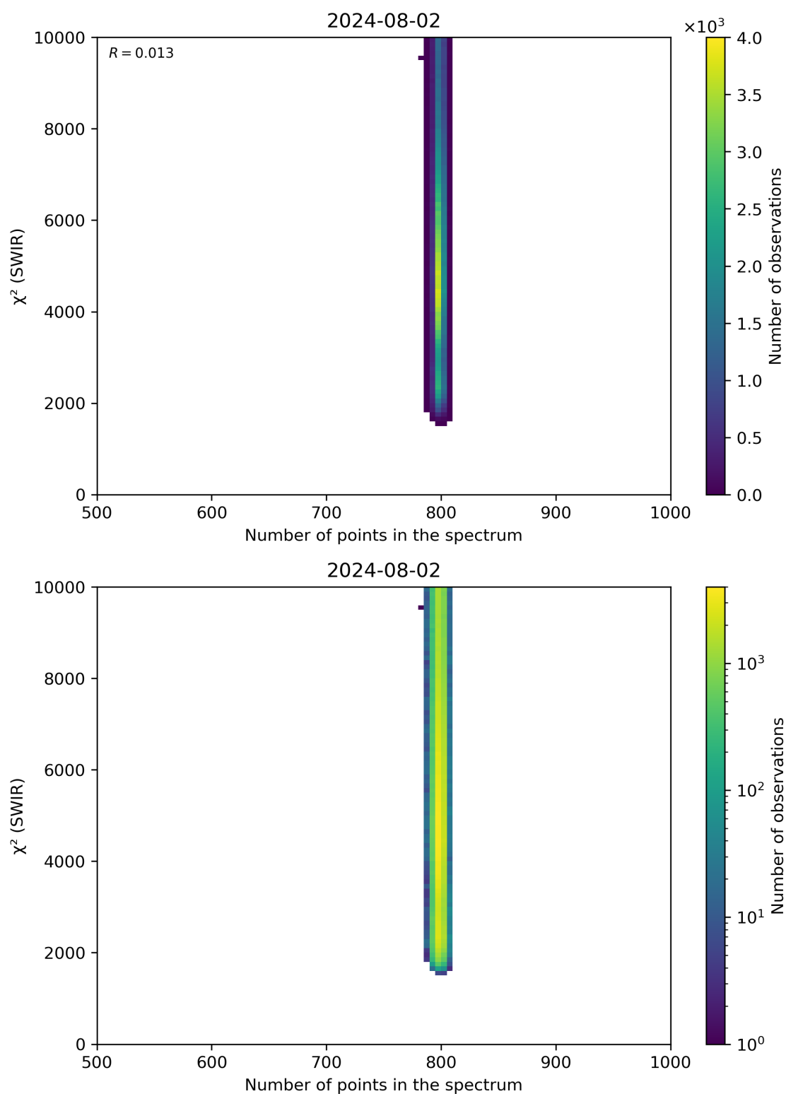
Figure 89: Scatter density plot of “Number of points in the spectrum” against “ \chi^2 (SWIR)” for 2024-08-01 to 2024-08-03.
