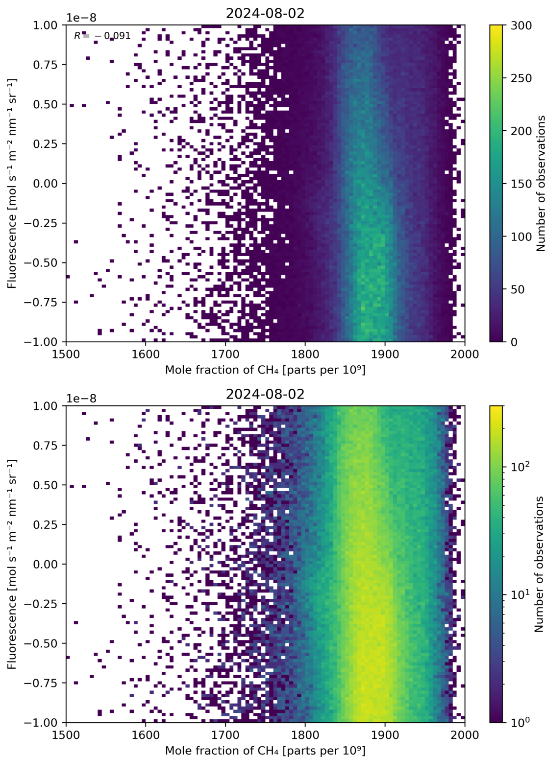
Figure 73: Scatter density plot of “Mole fraction of \text{CH}_4 ” against “Fluorescence” for 2024-08-01 to 2024-08-03.
