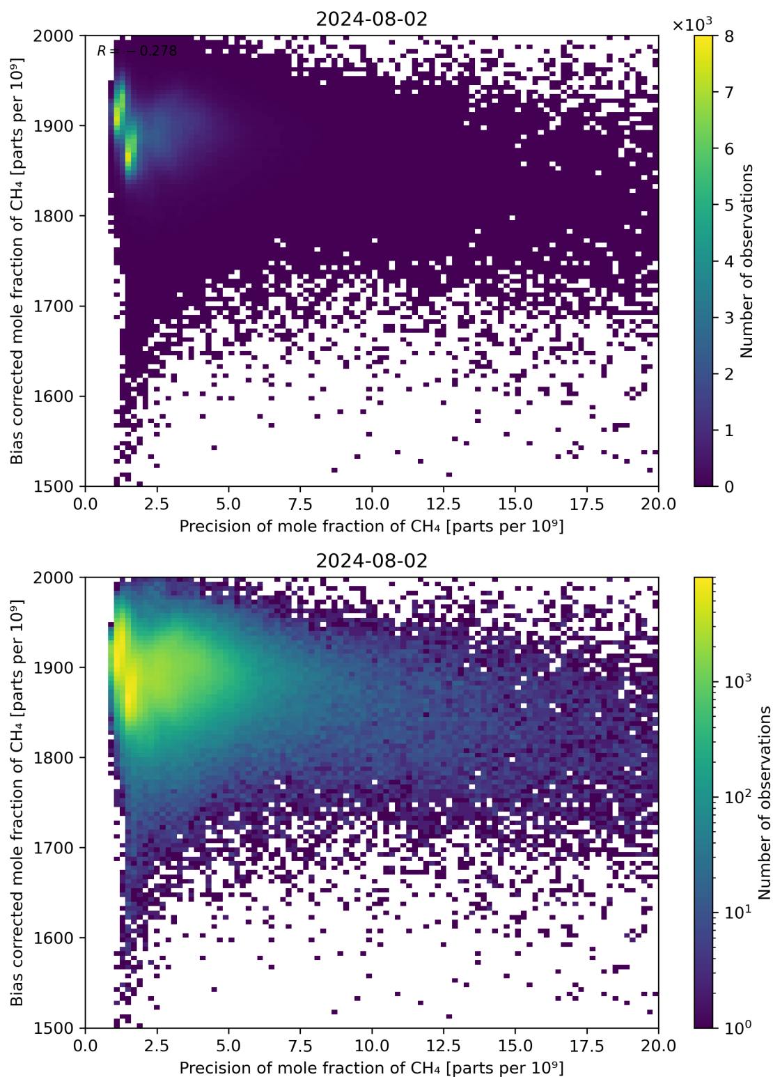
Figure 82: Scatter density plot of “Precision of mole fraction of CH 4 ” against “Bias corrected mole fraction of CH 4 ” for 2024-08-01 to 2024-08-03.
