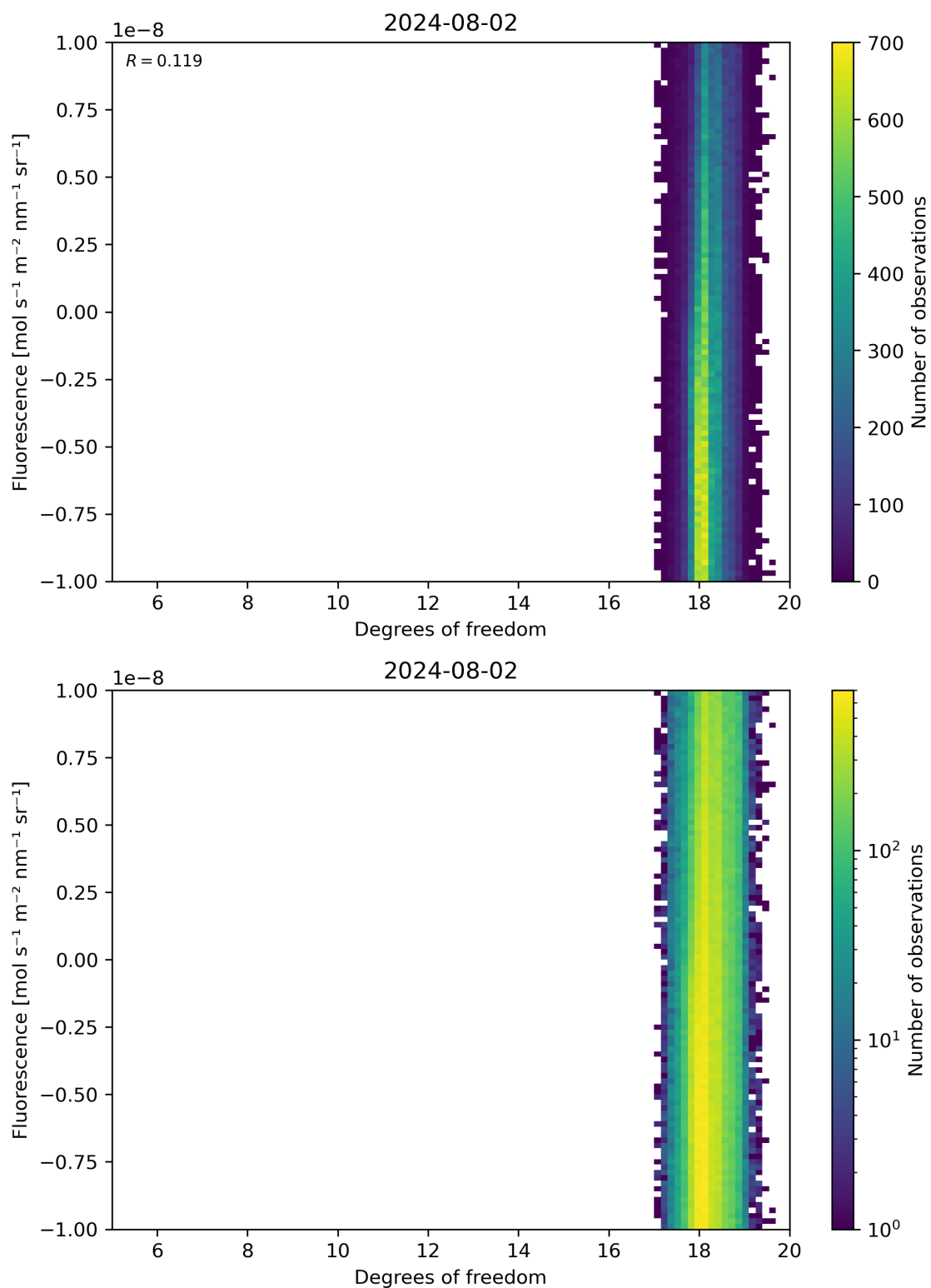
Figure 51: Scatter density plot of “Degrees of freedom” against “Fluorescence” for 2024-08-01 to 2024-08-03.
