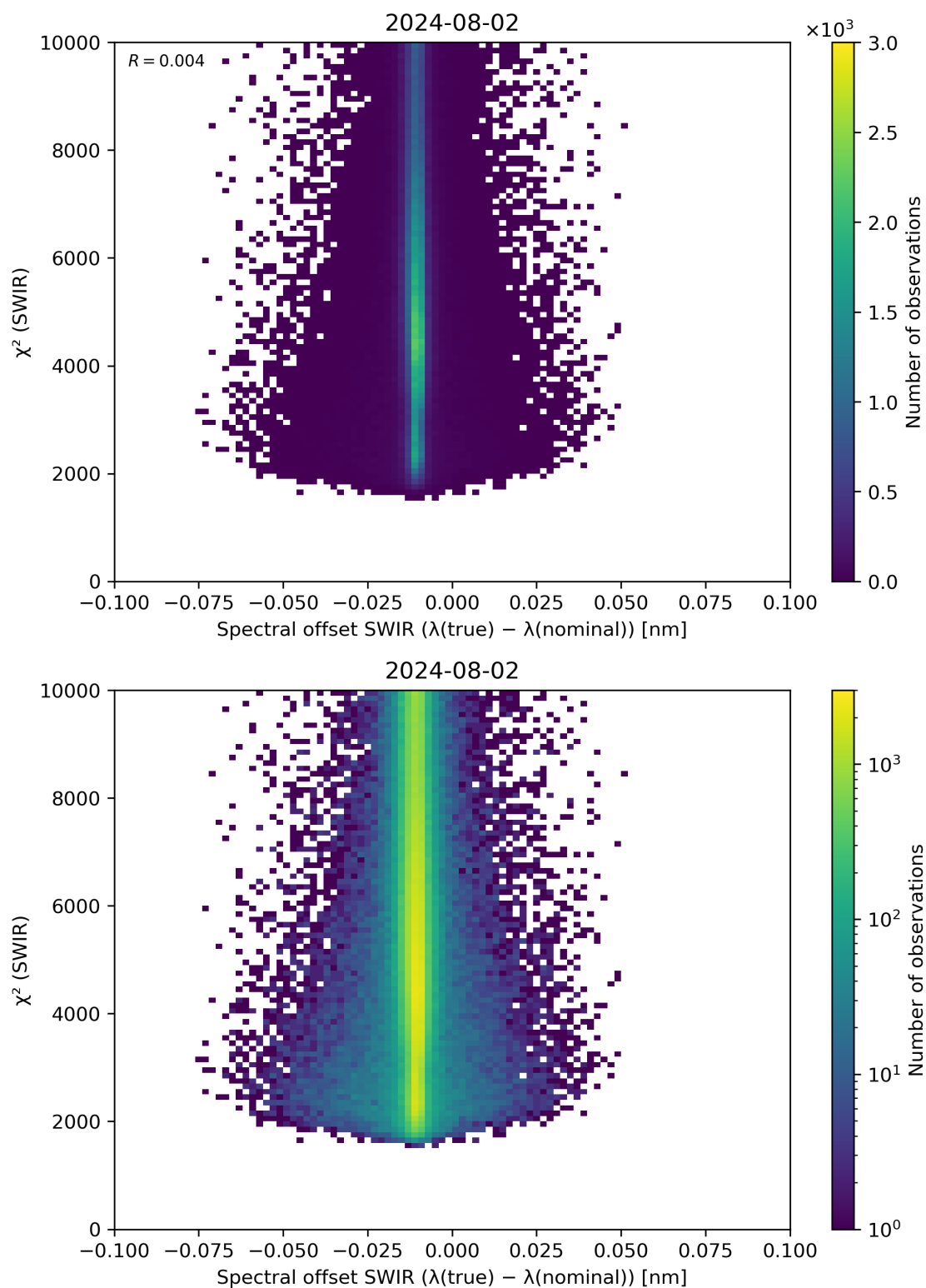
Figure 118: Scatter density plot of “Spectral offset SWIR ( \lambda(\text{true}) - \lambda(\text{nominal}) )” against “ \chi^2 (SWIR)” for 2024-08-01 to 2024-08-03.
