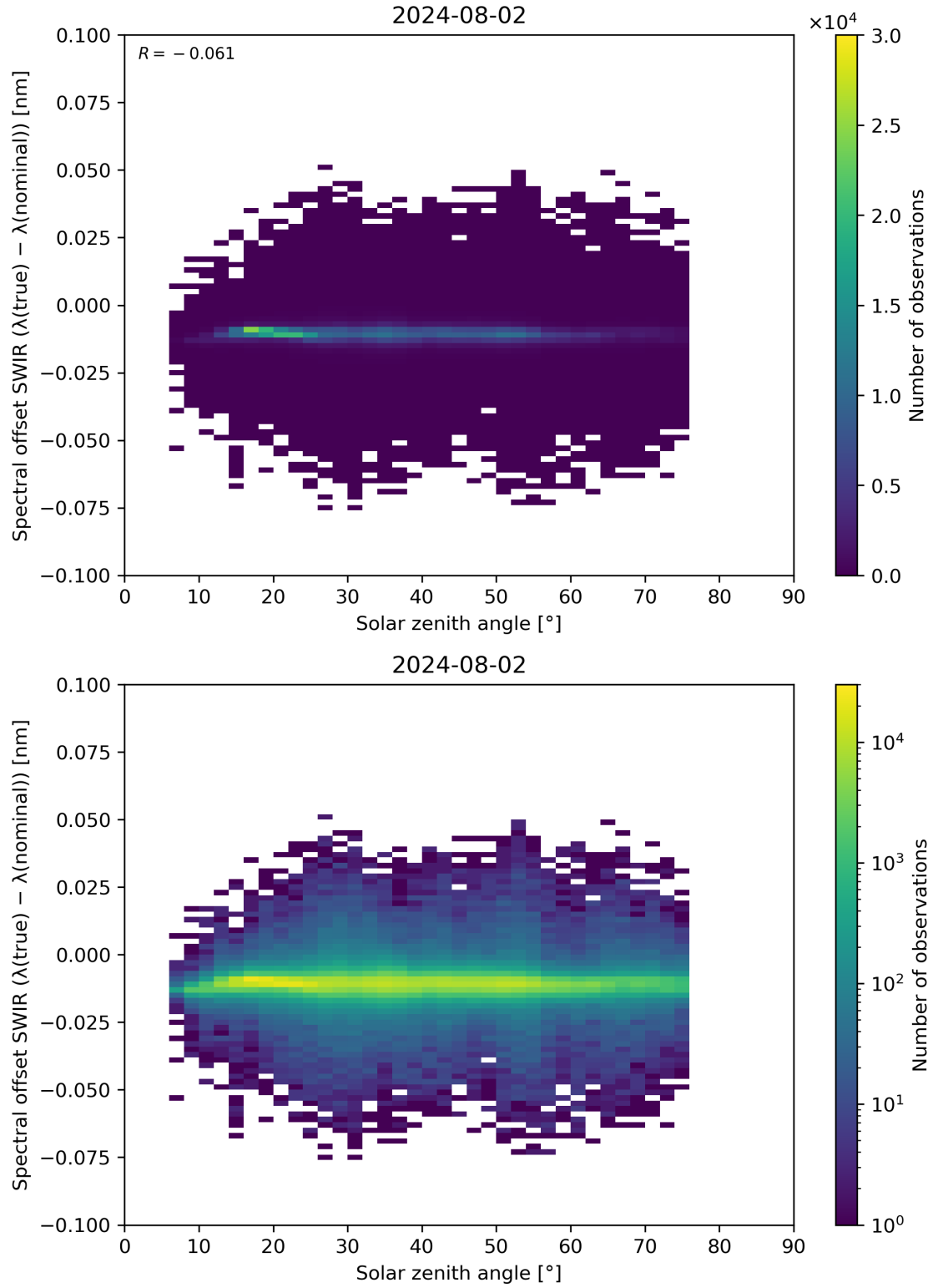
Figure 104: Scatter density plot of “Solar zenith angle” against “Spectral offset SWIR ( \lambda(\text{true}) - \lambda(\text{nominal}) )” for 2024-08-01 to 2024-08-03.
