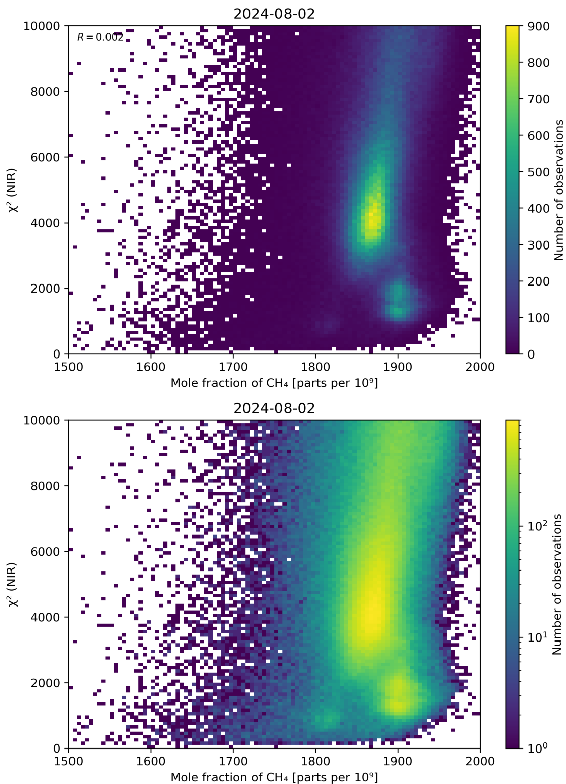
Figure 70: Scatter density plot of “Mole fraction of \text{CH}_4 ” against “ \chi^2 (NIR)” for 2024-08-01 to 2024-08-03.
