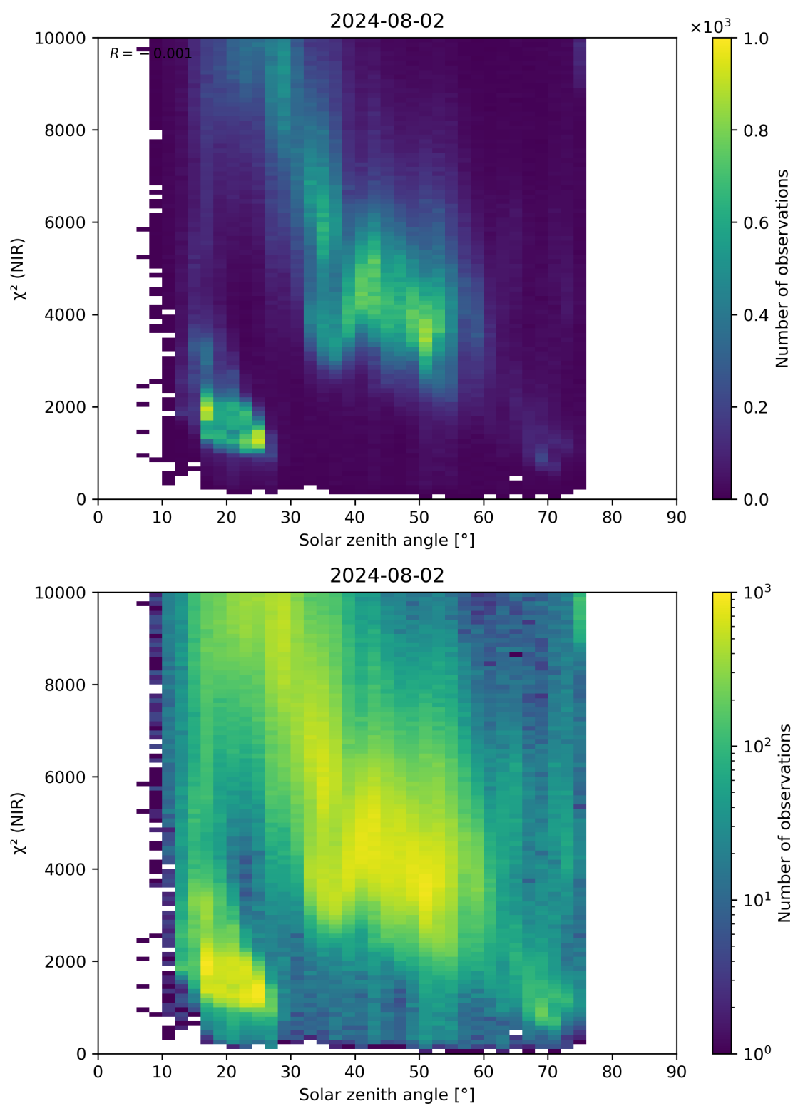
Figure 94: Scatter density plot of “Solar zenith angle” against “ \chi^2 (NIR)” for 2024-08-01 to 2024-08-03.
