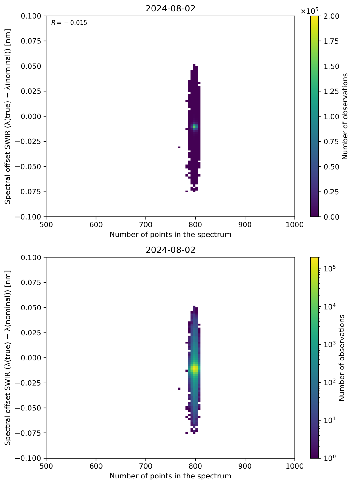
Figure 93: Scatter density plot of “Number of points in the spectrum” against “Spectral offset SWIR ( \lambda(\text{true}) - \lambda(\text{nominal}) )” for 2024-08-01 to 2024-08-03.
