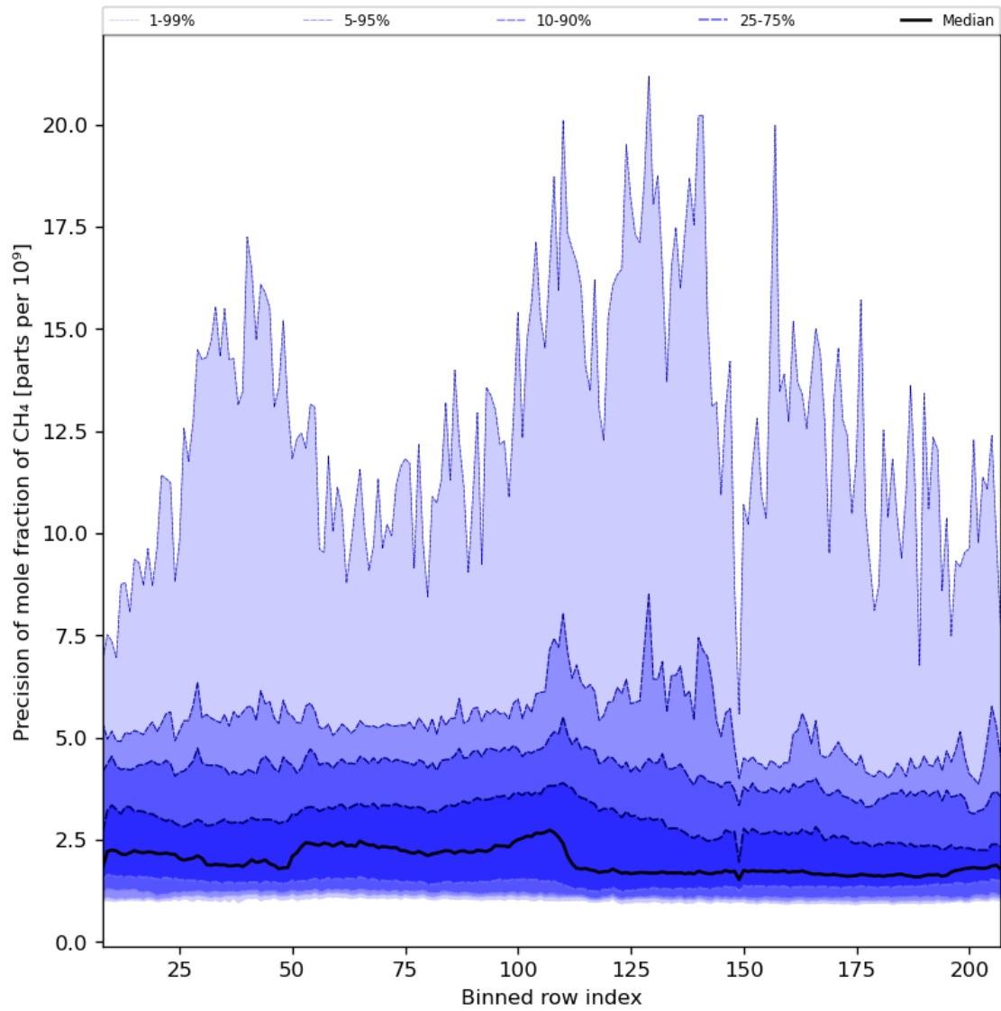
Figure 35: Along track statistics of “Precision of mole fraction of CH 4 ” for 2024-08-01 to 2024-08-03
