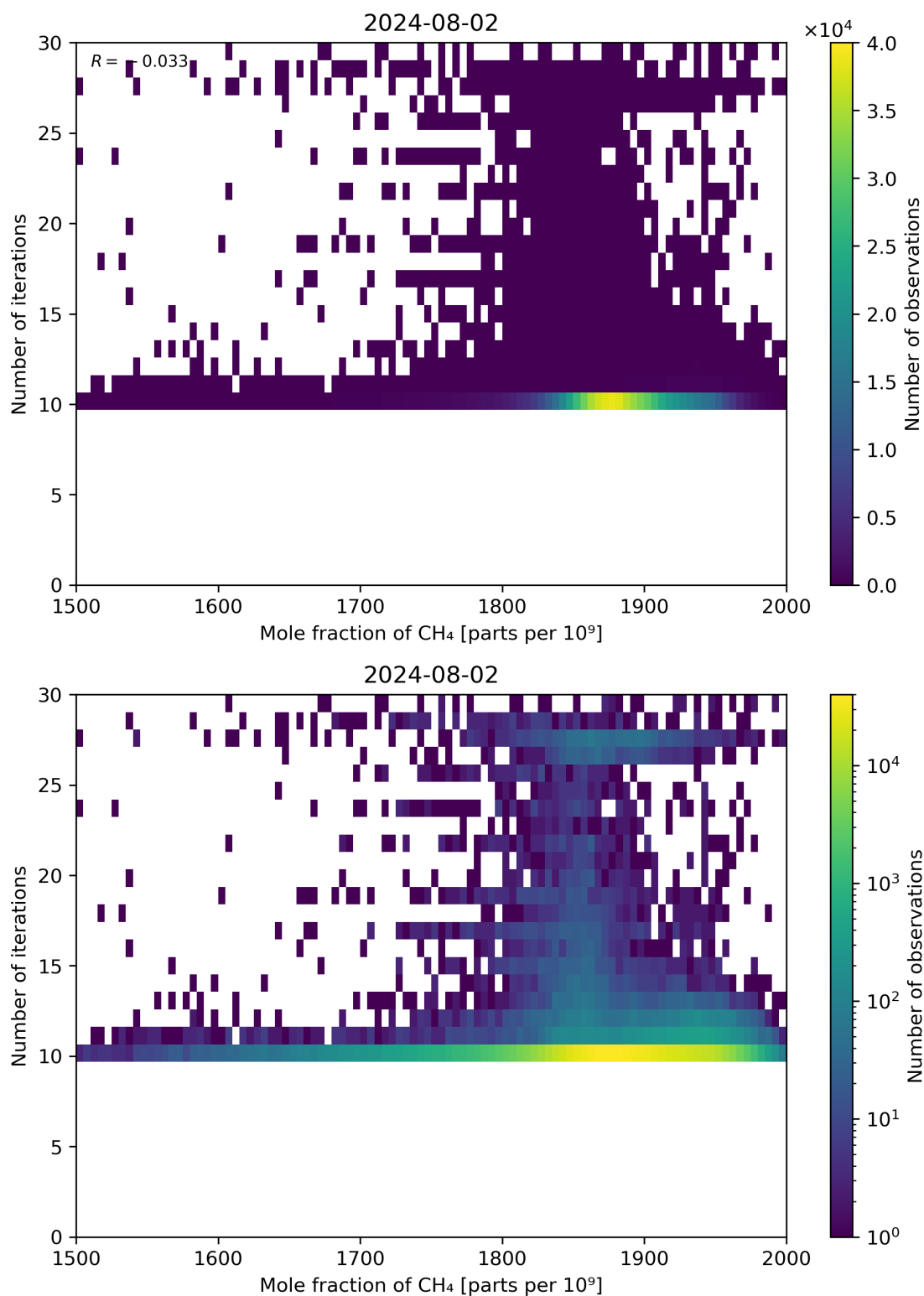
Figure 76: Scatter density plot of “Mole fraction of CH 4 ” against “Number of iterations” for 2024-08-01 to 2024-08-03.
