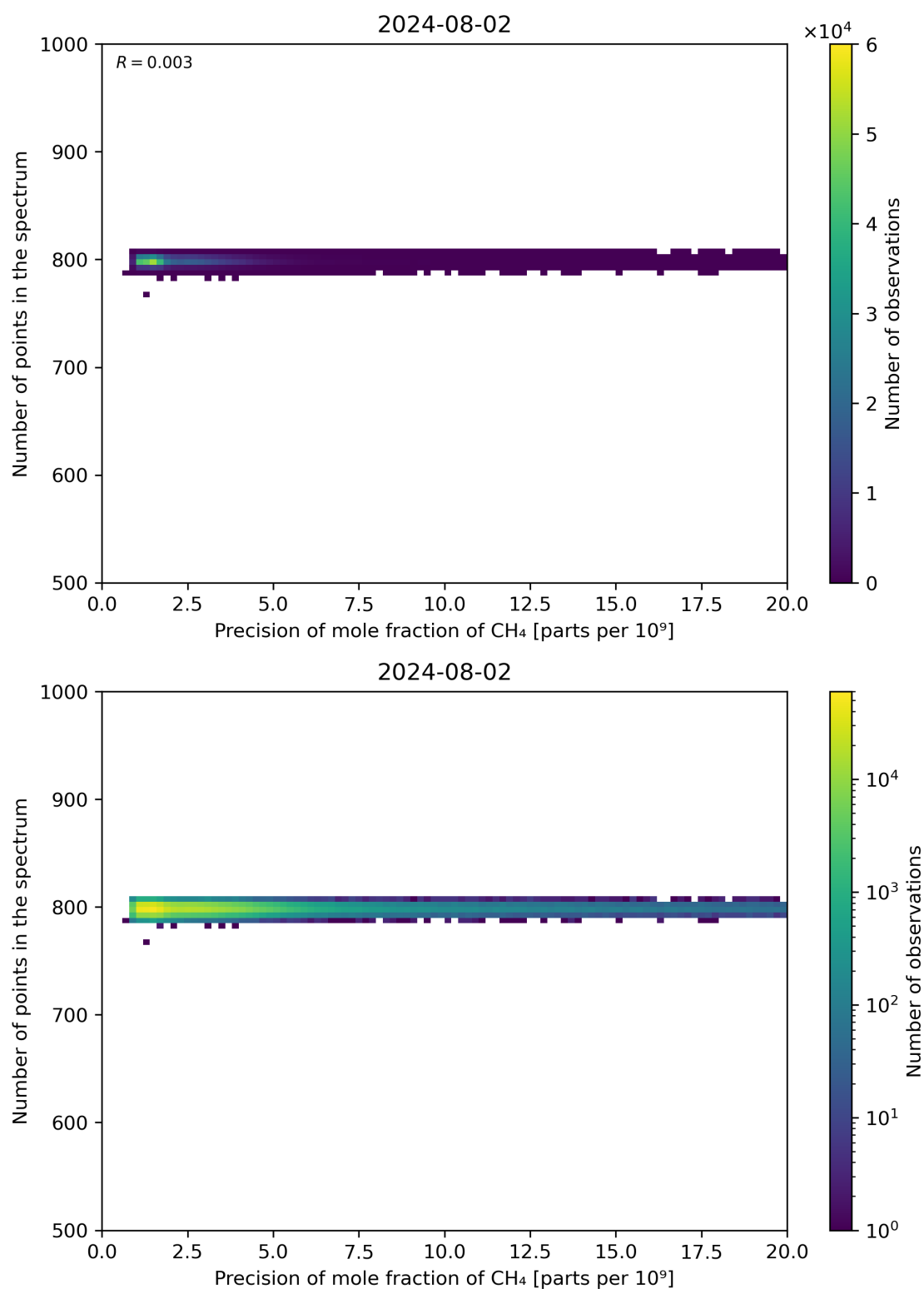
Figure 84: Scatter density plot of “Precision of mole fraction of CH 4 ” against “Number of points in the spectrum” for 2024-08-01 to 2024-08-03.
