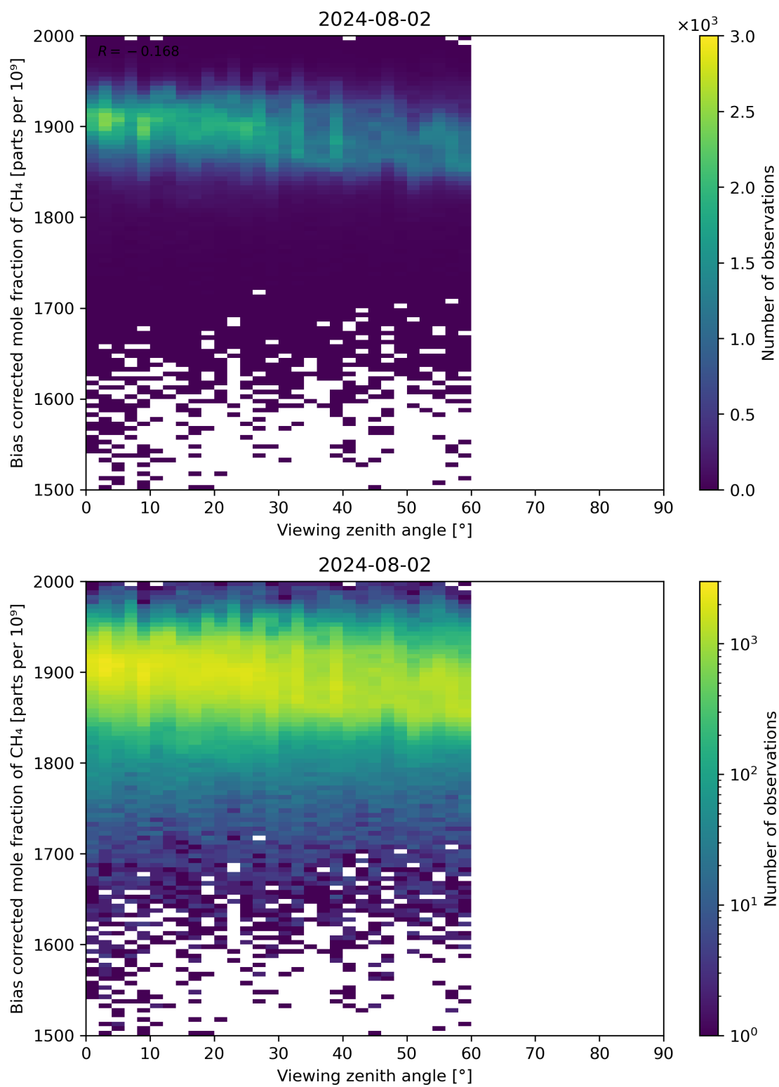
Figure 111: Scatter density plot of “Viewing zenith angle” against “Bias corrected mole fraction of CH 4 ” for 2024-08-01 to 2024-08-03.
