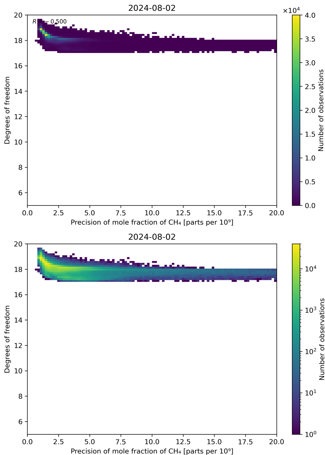
Figure 80: Scatter density plot of “Precision of mole fraction of CH 4 ” against “Degrees of freedom” for 2024-08-01 to 2024-08-03.
