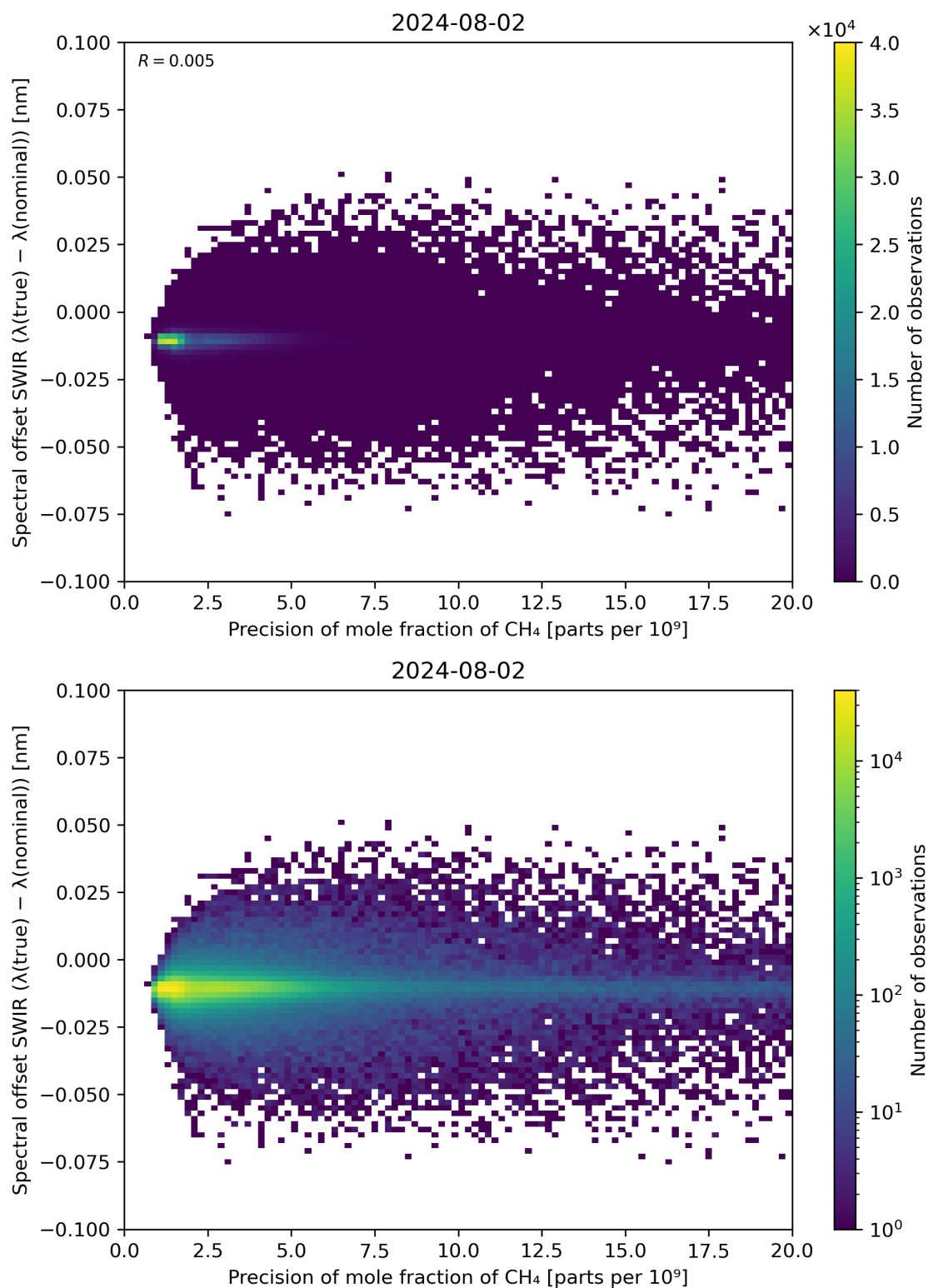
Figure 85: Scatter density plot of “Precision of mole fraction of \text{CH}_4 ” against “Spectral offset SWIR ( \lambda(\text{true}) - \lambda(\text{nominal}) )” for 2024-08-01 to 2024-08-03.
