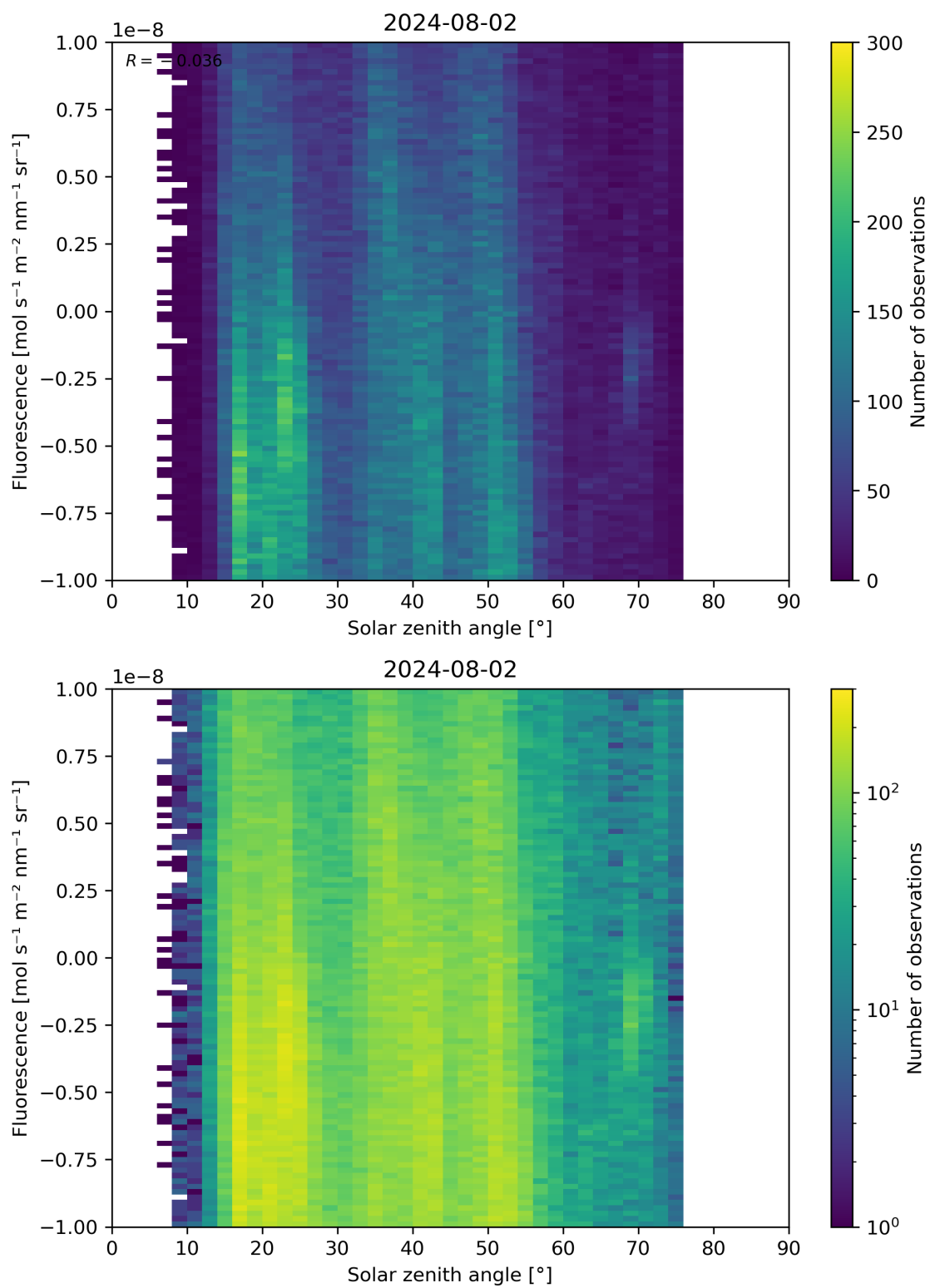
Figure 97: Scatter density plot of “Solar zenith angle” against “Fluorescence” for 2024-08-01 to 2024-08-03.
