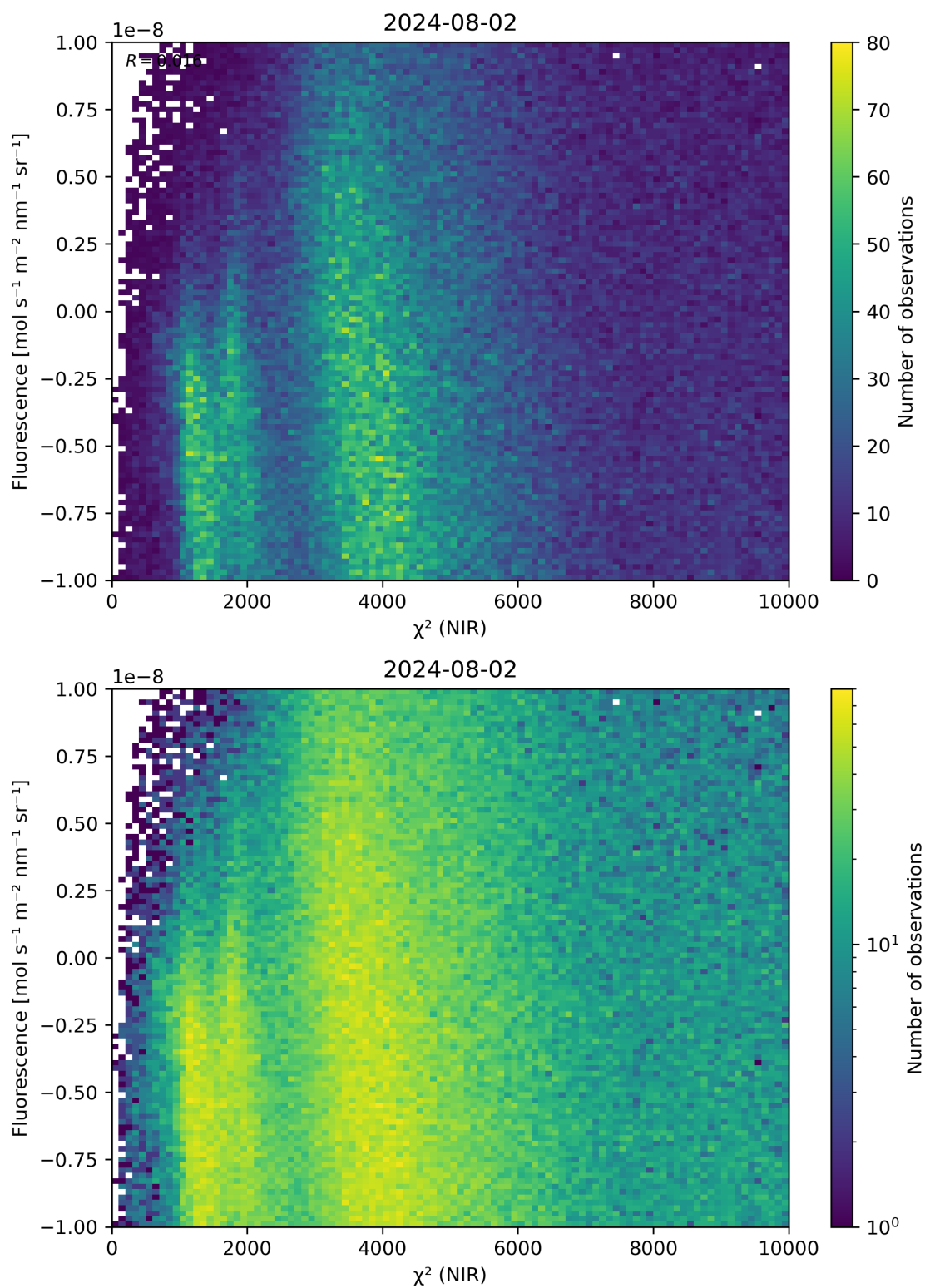
Figure 45: Scatter density plot of “ \chi^2 (NIR)” against “Fluorescence” for 2024-08-01 to 2024-08-03.
