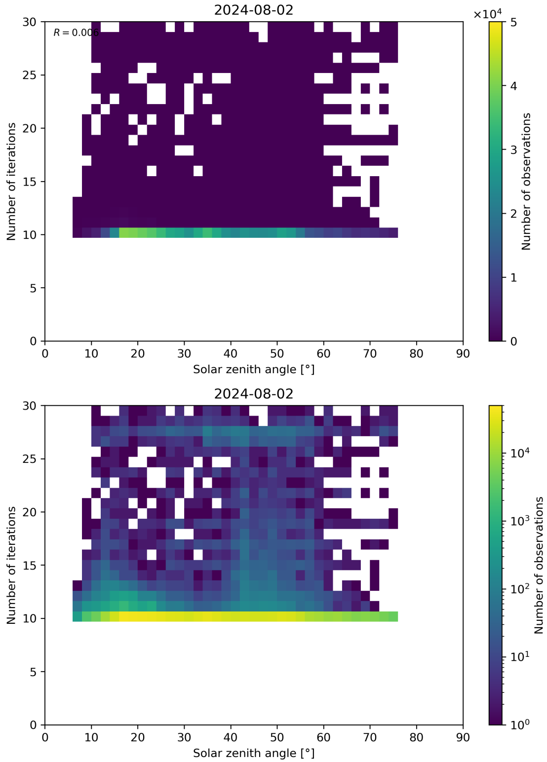
Figure 102: Scatter density plot of “Solar zenith angle” against “Number of iterations” for 2024-08-01 to 2024-08-03.
