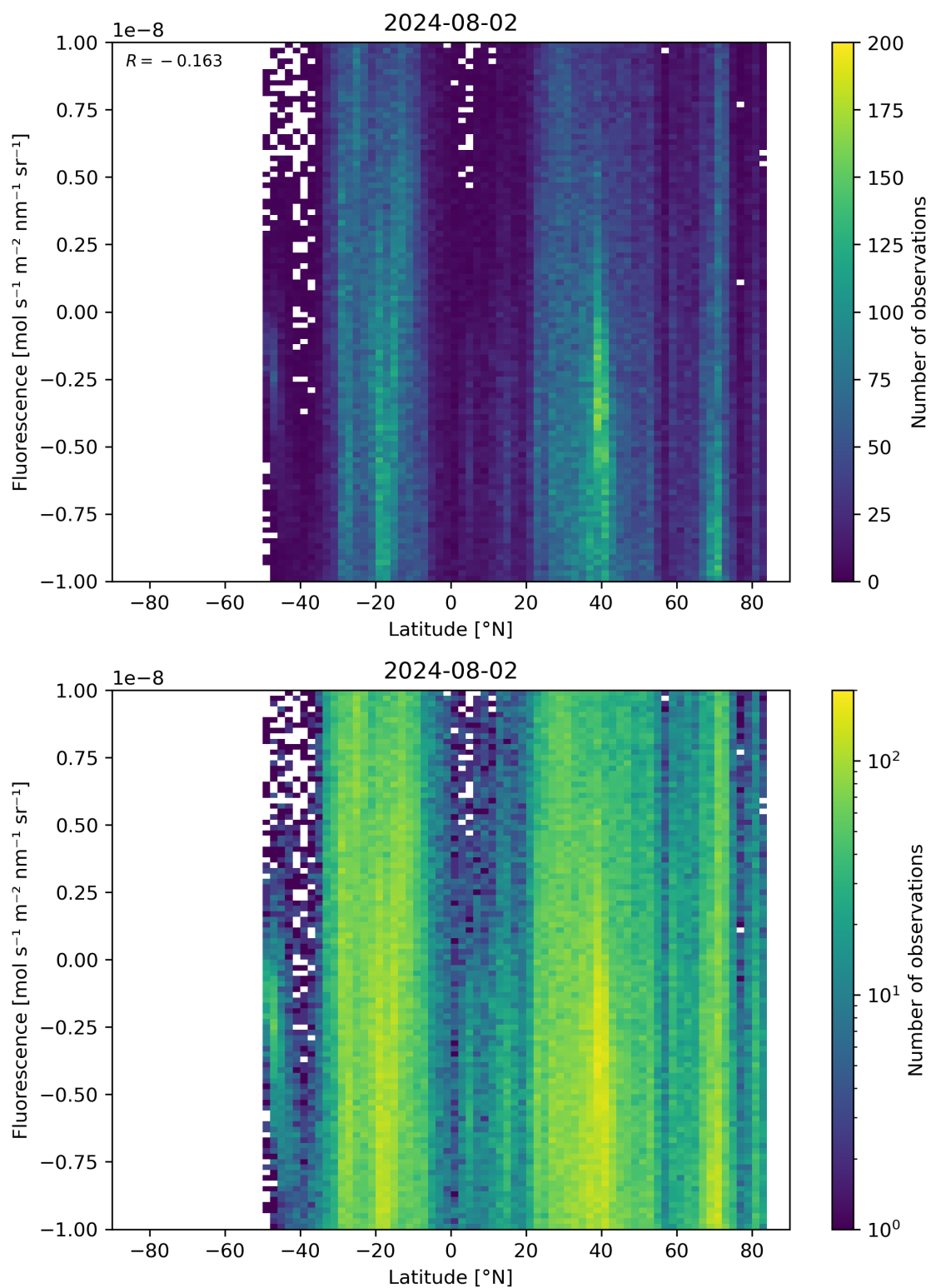
Figure 56: Scatter density plot of “Latitude” against “Fluorescence” for 2024-08-01 to 2024-08-03.
