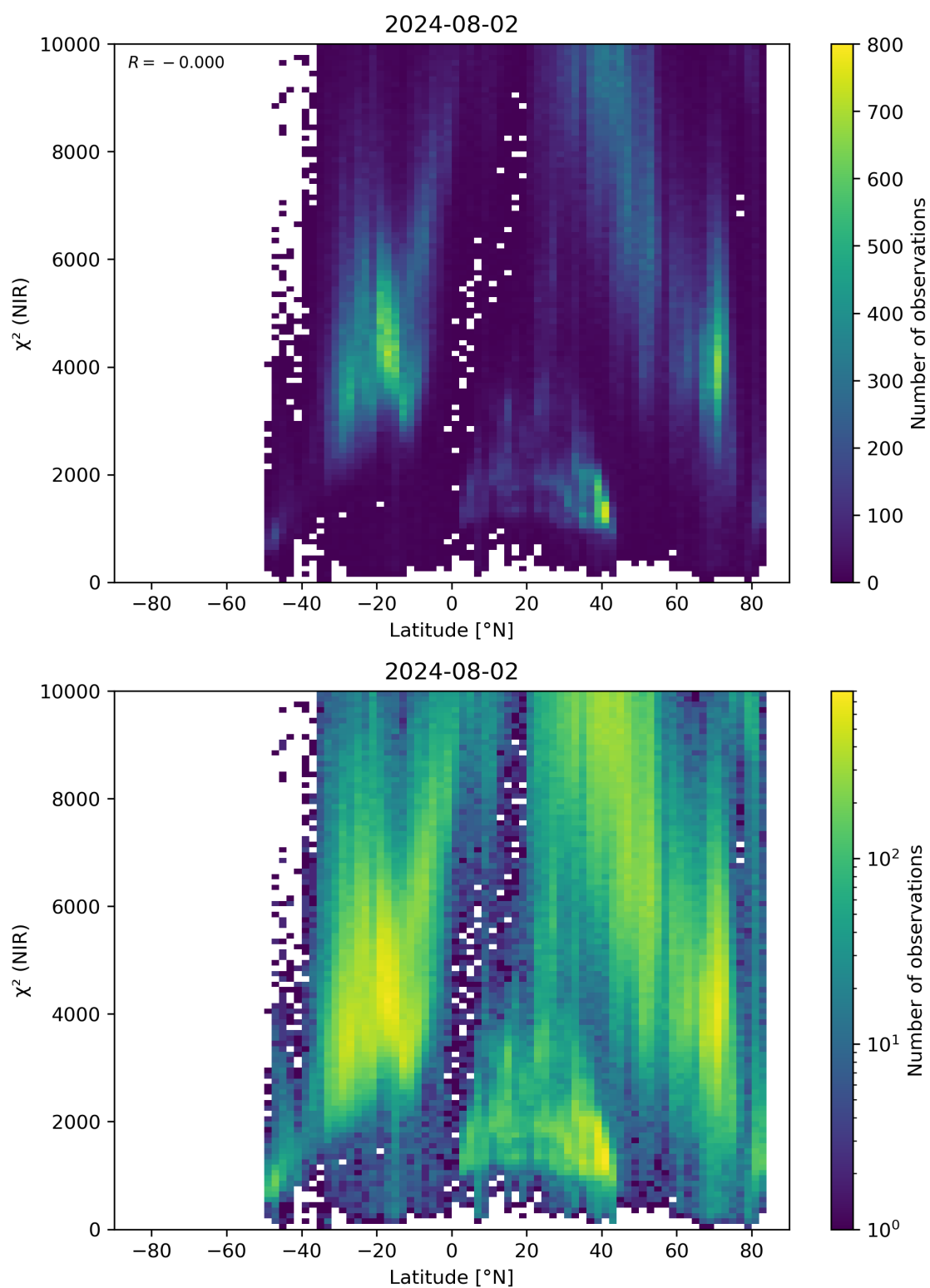
Figure 53: Scatter density plot of “Latitude” against “ \chi^2 (NIR)” for 2024-08-01 to 2024-08-03.
