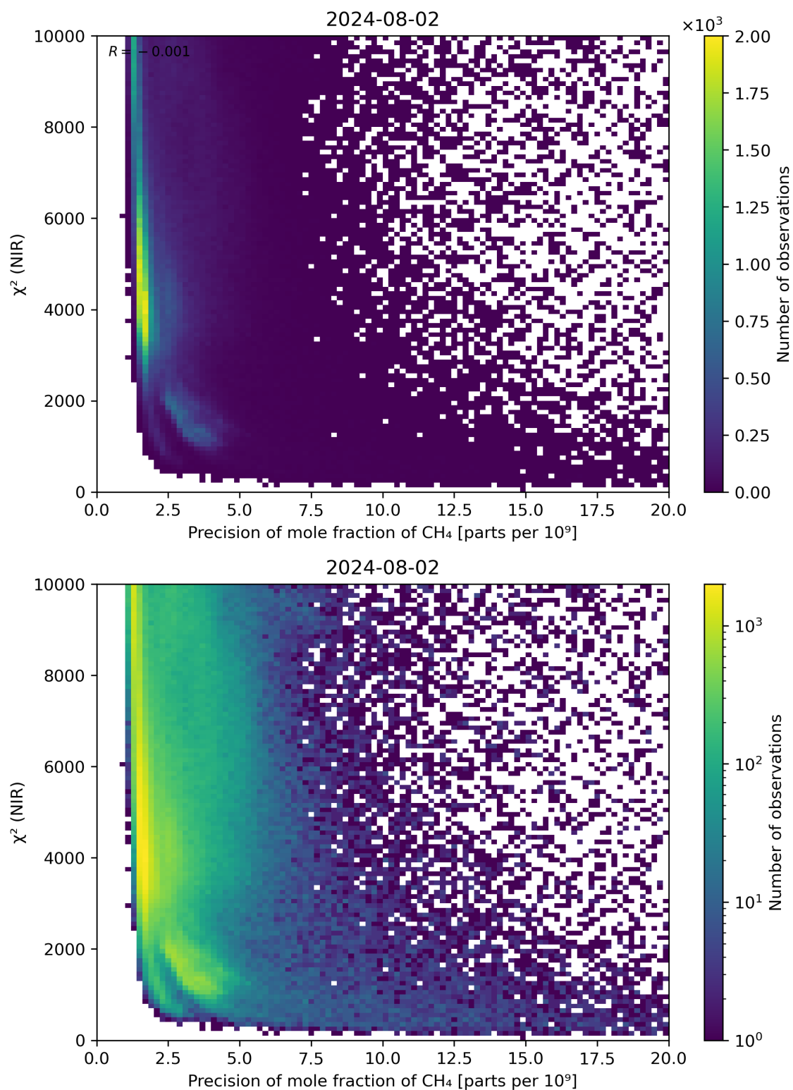
Figure 78: Scatter density plot of “Precision of mole fraction of \text{CH}_4 ” against “ \chi^2 (NIR)” for 2024-08-01 to 2024-08-03.
