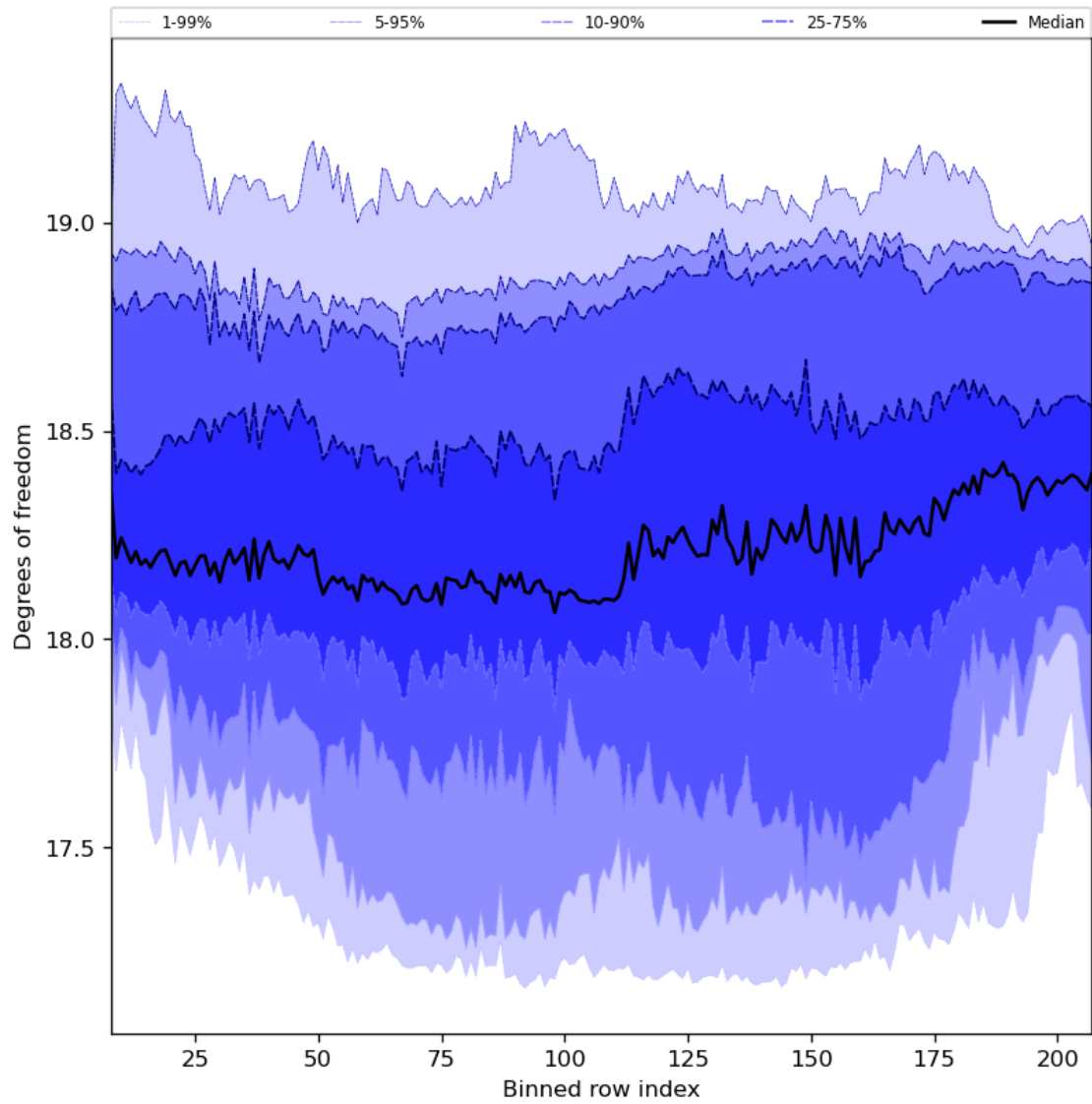
Figure 41: Along track statistics of “Degrees of freedom” for 2024-08-01 to 2024-08-03
