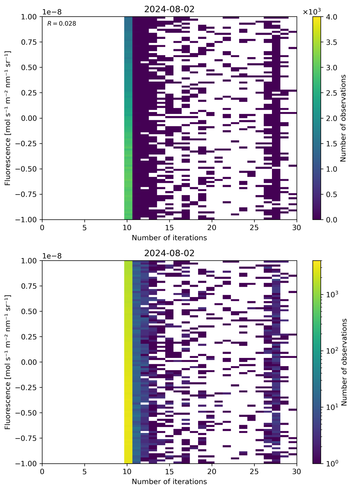
Figure 87: Scatter density plot of “Number of iterations” against “Fluorescence” for 2024-08-01 to 2024-08-03.
