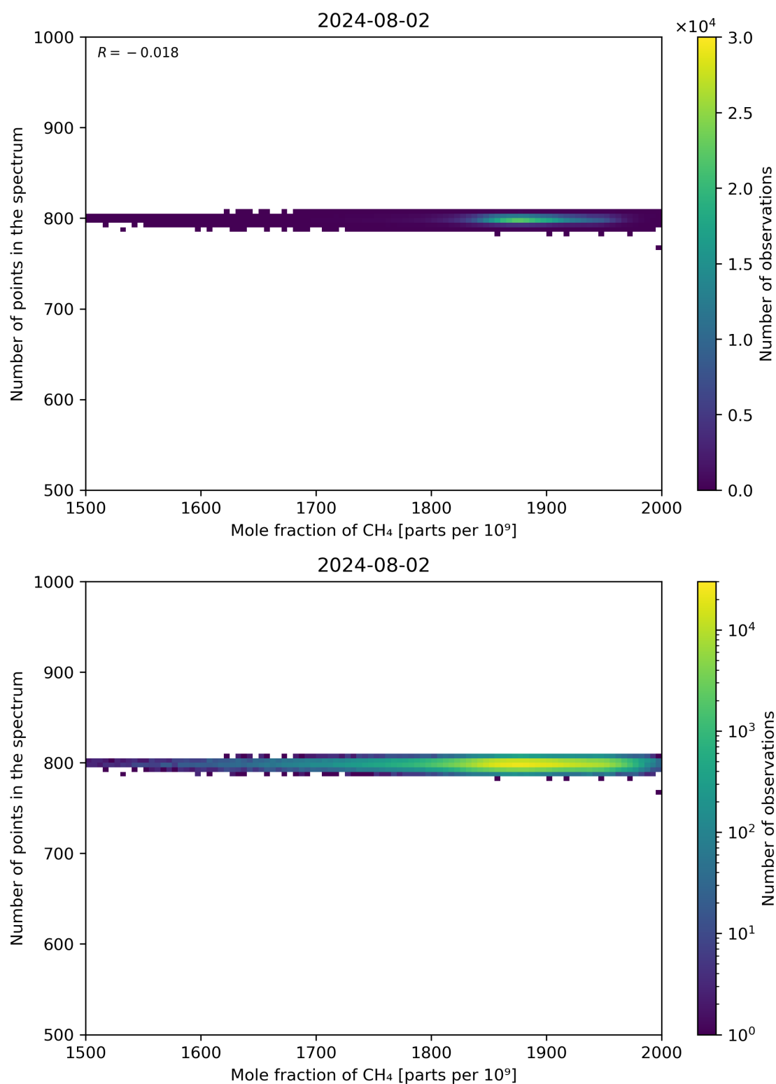
Figure 77: Scatter density plot of “Mole fraction of CH 4 ” against “Number of points in the spectrum” for 2024-08-01 to 2024-08-03.
