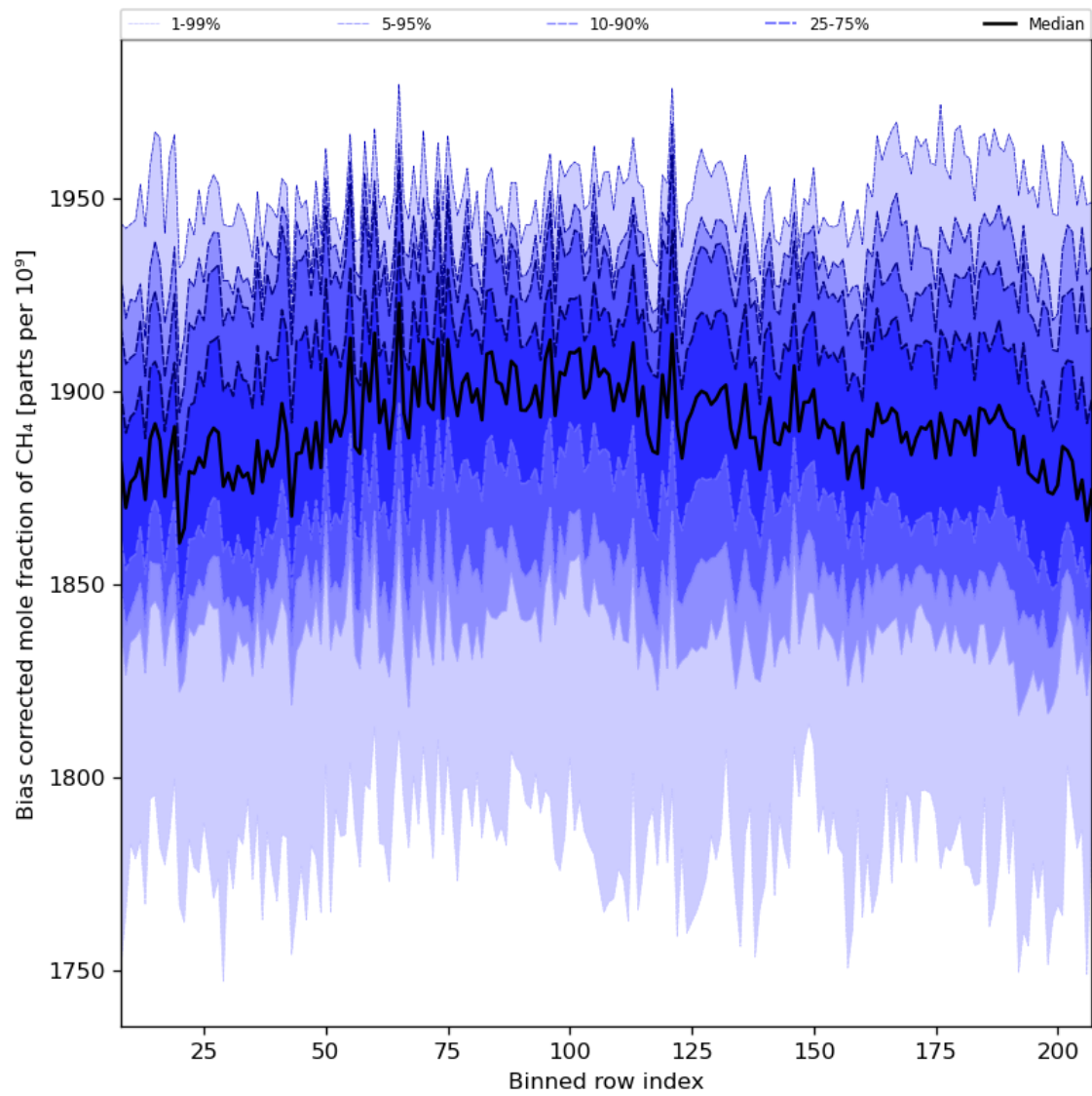
Figure 36: Along track statistics of “Bias corrected mole fraction of CH 4 ” for 2024-08-01 to 2024-08-03
