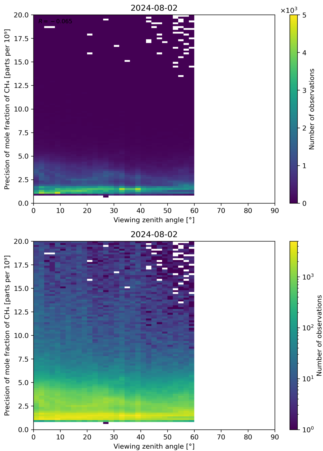
Figure 112: Scatter density plot of “Viewing zenith angle” against “Precision of mole fraction of CH 4 ” for 2024-08-01 to 2024-08-03.
