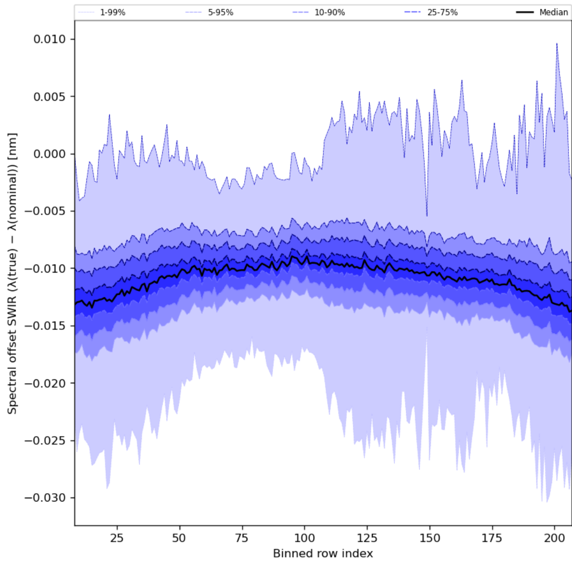
Figure 38: Along track statistics of “Spectral offset SWIR ( \lambda(\text{true}) - \lambda(\text{nominal}) )” for 2024-08-01 to 2024-08-03
