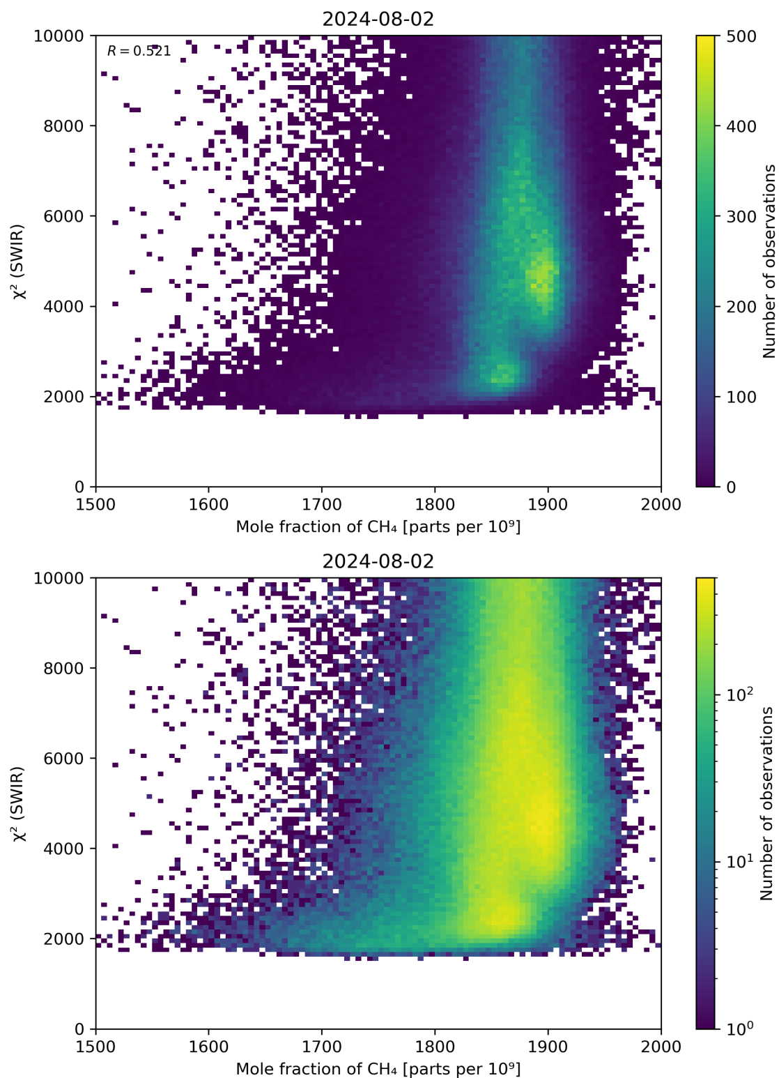
Figure 71: Scatter density plot of “Mole fraction of \text{CH}_4 ” against “ \chi^2 (SWIR)” for 2024-08-01 to 2024-08-03.
