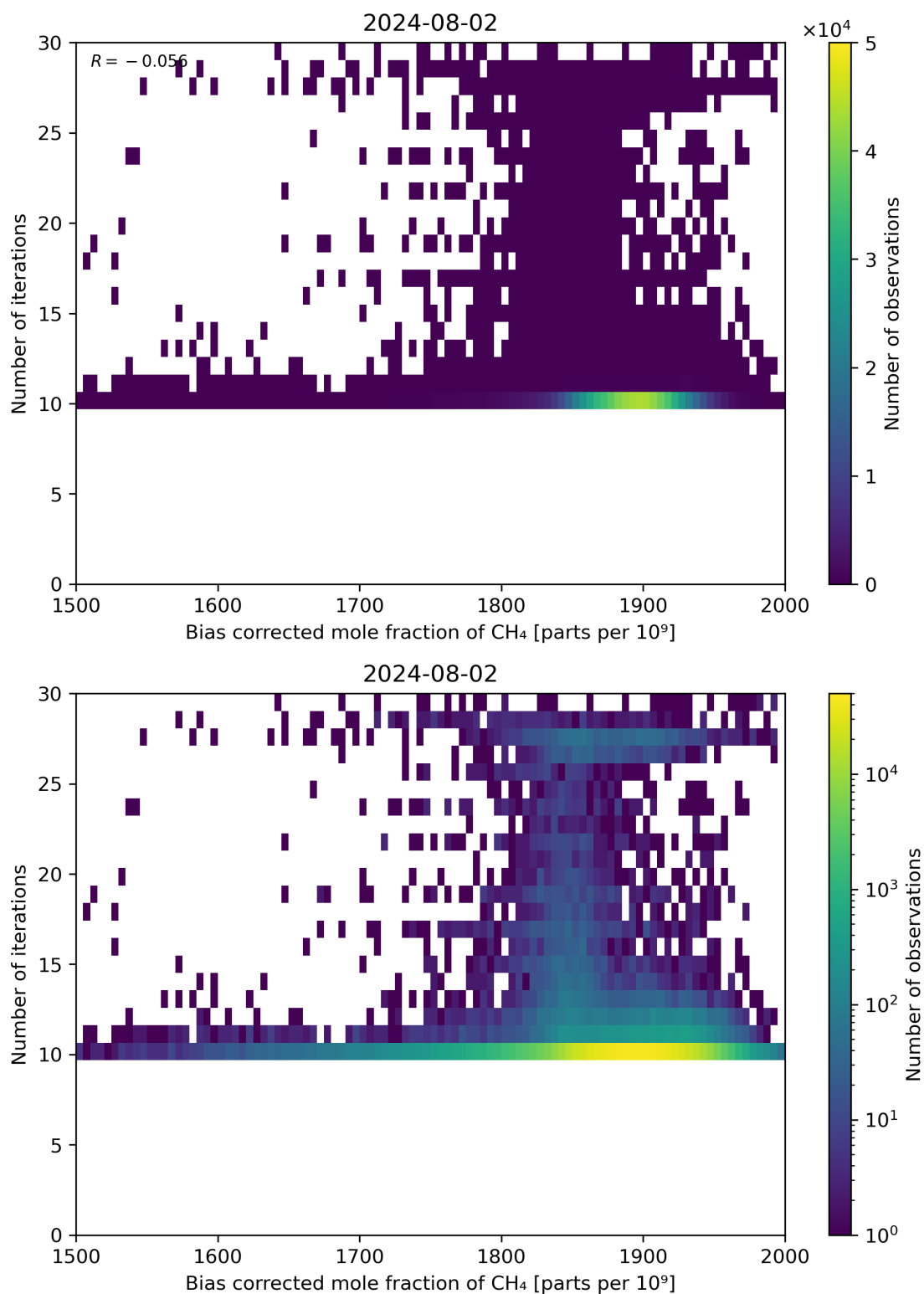
Figure 67: Scatter density plot of “Bias corrected mole fraction of CH 4 ” against “Number of iterations” for 2024-08-01 to 2024-08-03.
