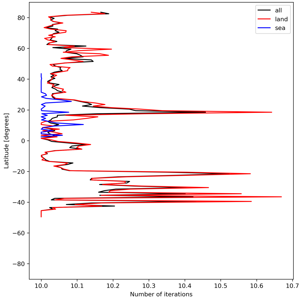
Figure 20: Zonal average of “Number of iterations” for 2024-08-01 to 2024-08-03.
