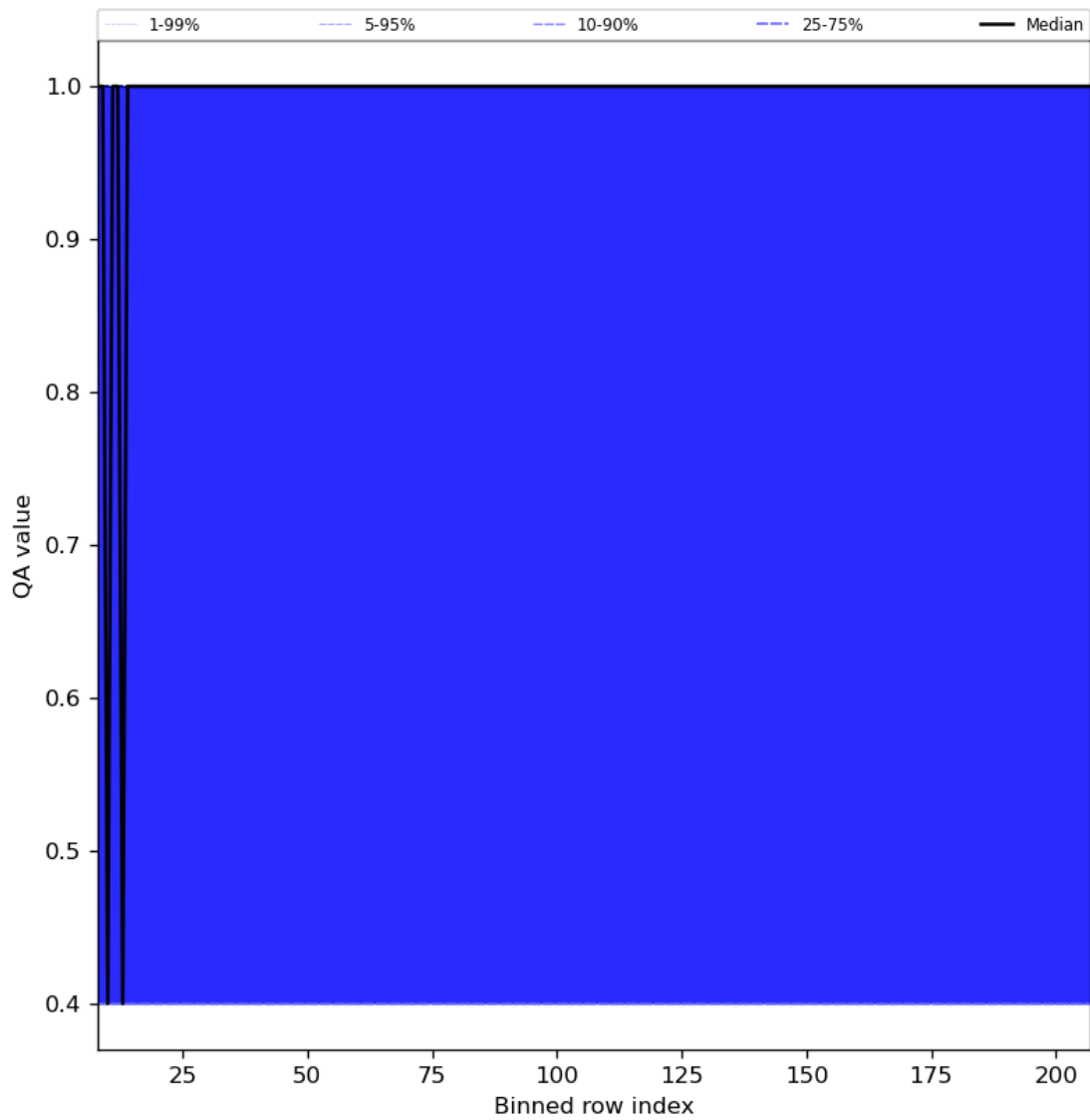
Figure 33: Along track statistics of “QA value” for 2024-08-01 to 2024-08-03
