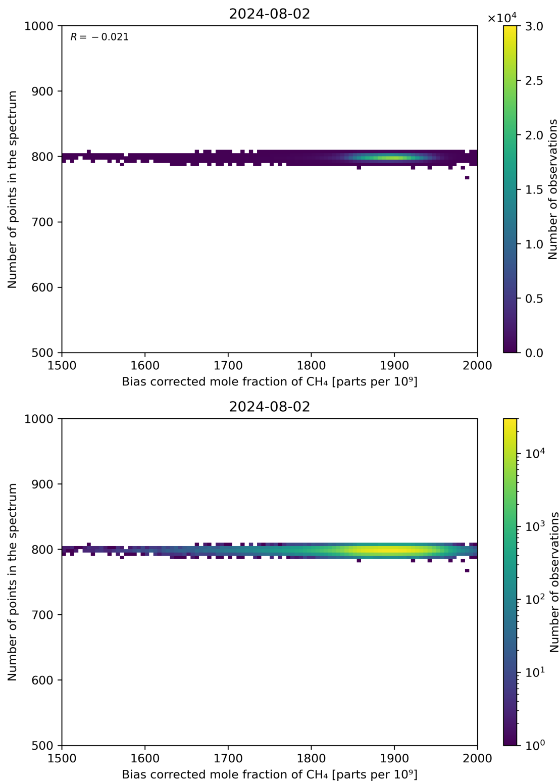
Figure 68: Scatter density plot of “Bias corrected mole fraction of CH 4 ” against “Number of points in the spectrum” for 2024-08-01 to 2024-08-03.
