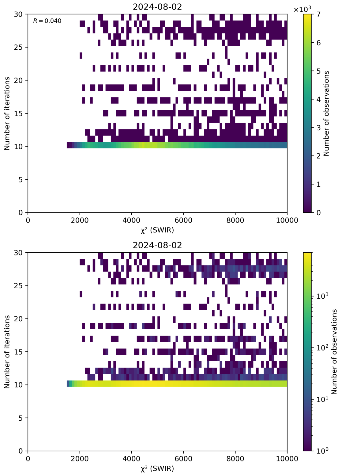
Figure 50: Scatter density plot of “ \chi^2 (SWIR)” against “Number of iterations” for 2024-08-01 to 2024-08-03.
