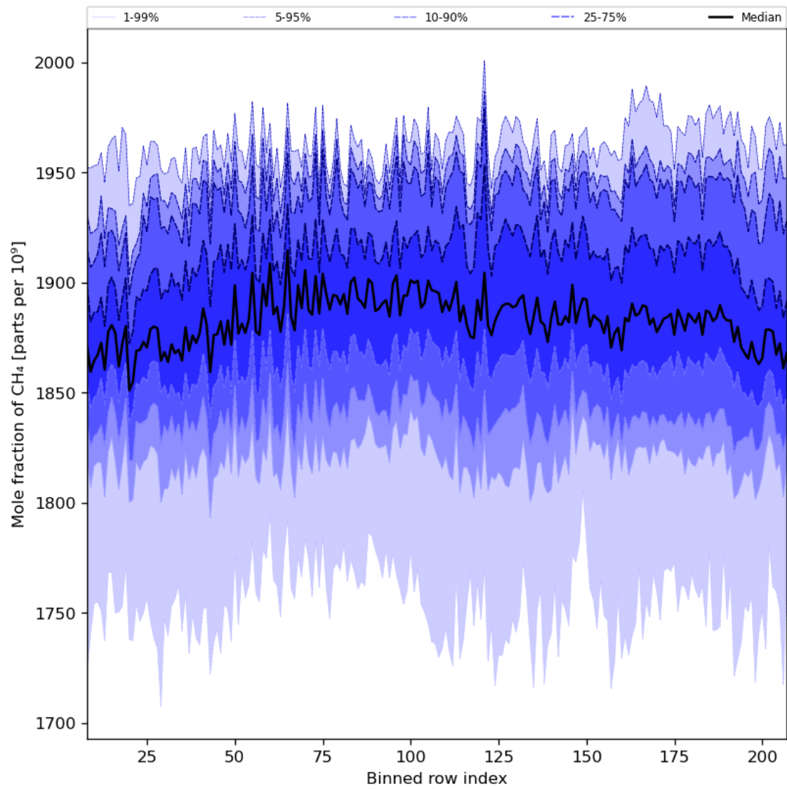
Figure 34: Along track statistics of “Mole fraction of CH 4 ” for 2024-08-01 to 2024-08-03
