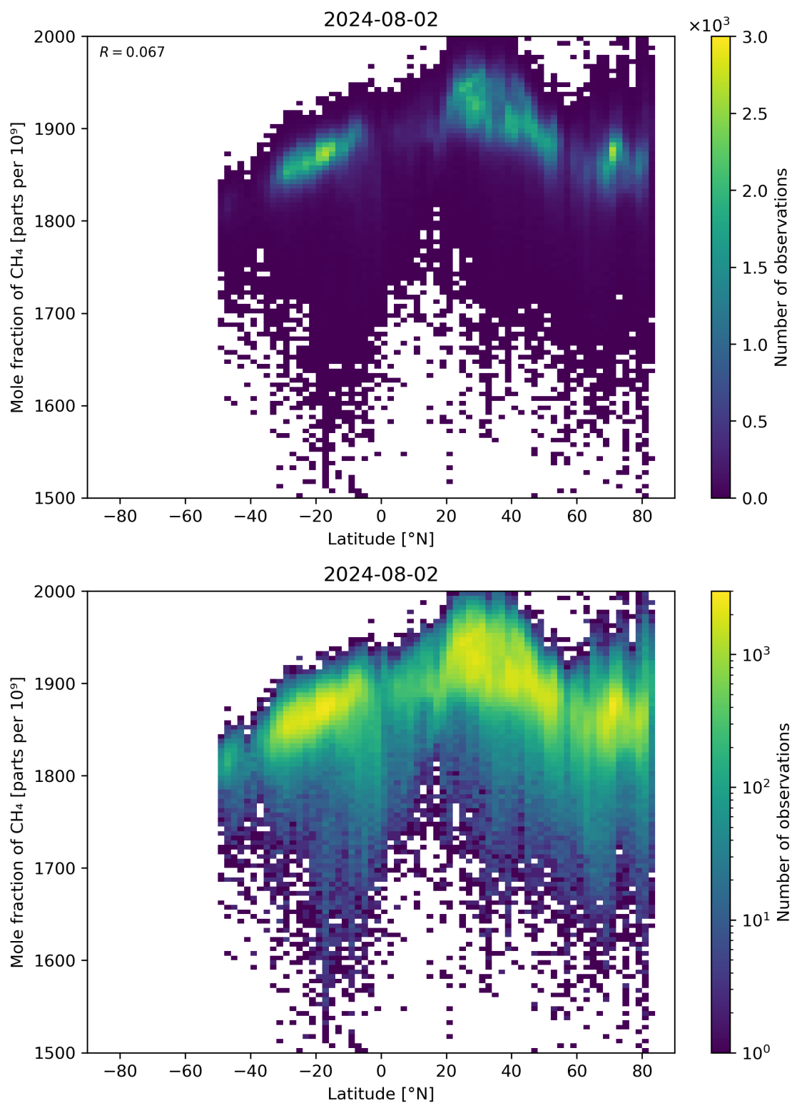
Figure 57: Scatter density plot of “Latitude” against “Mole fraction of CH 4 ” for 2024-08-01 to 2024-08-03.
