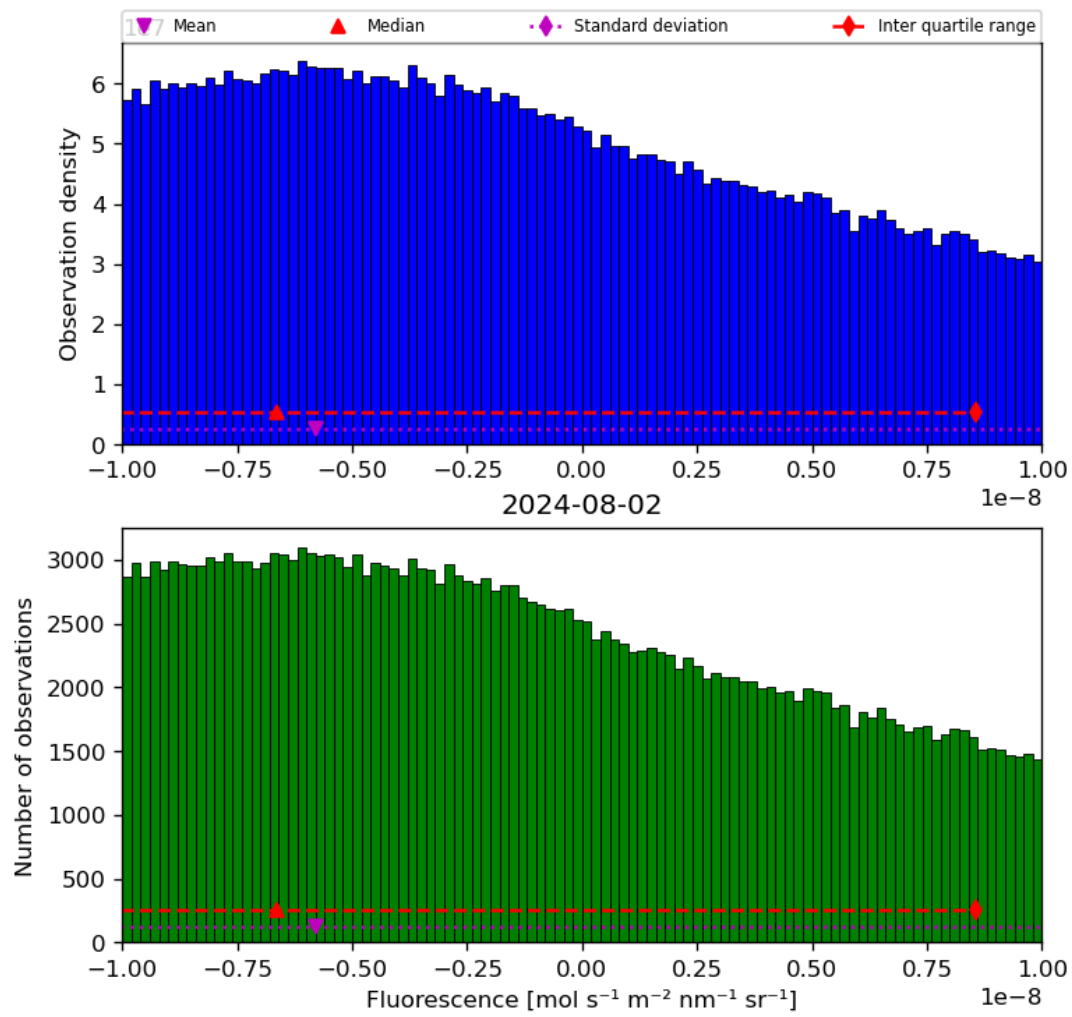
Figure 32: Histogram of “Fluorescence” for 2024-08-01 to 2024-08-03
