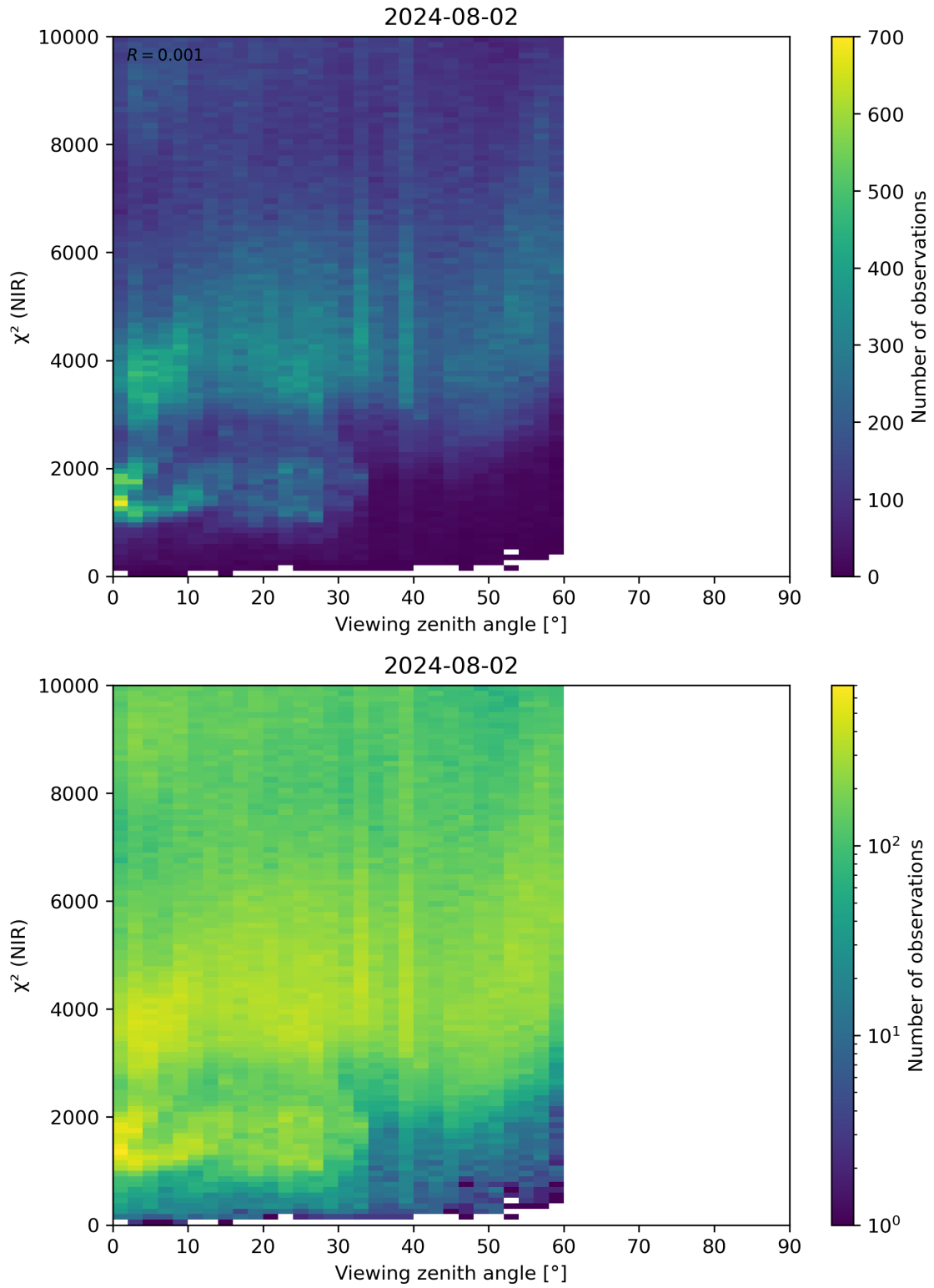
Figure 105: Scatter density plot of “Viewing zenith angle” against “ \chi^2 (NIR)” for 2024-08-01 to 2024-08-03.
