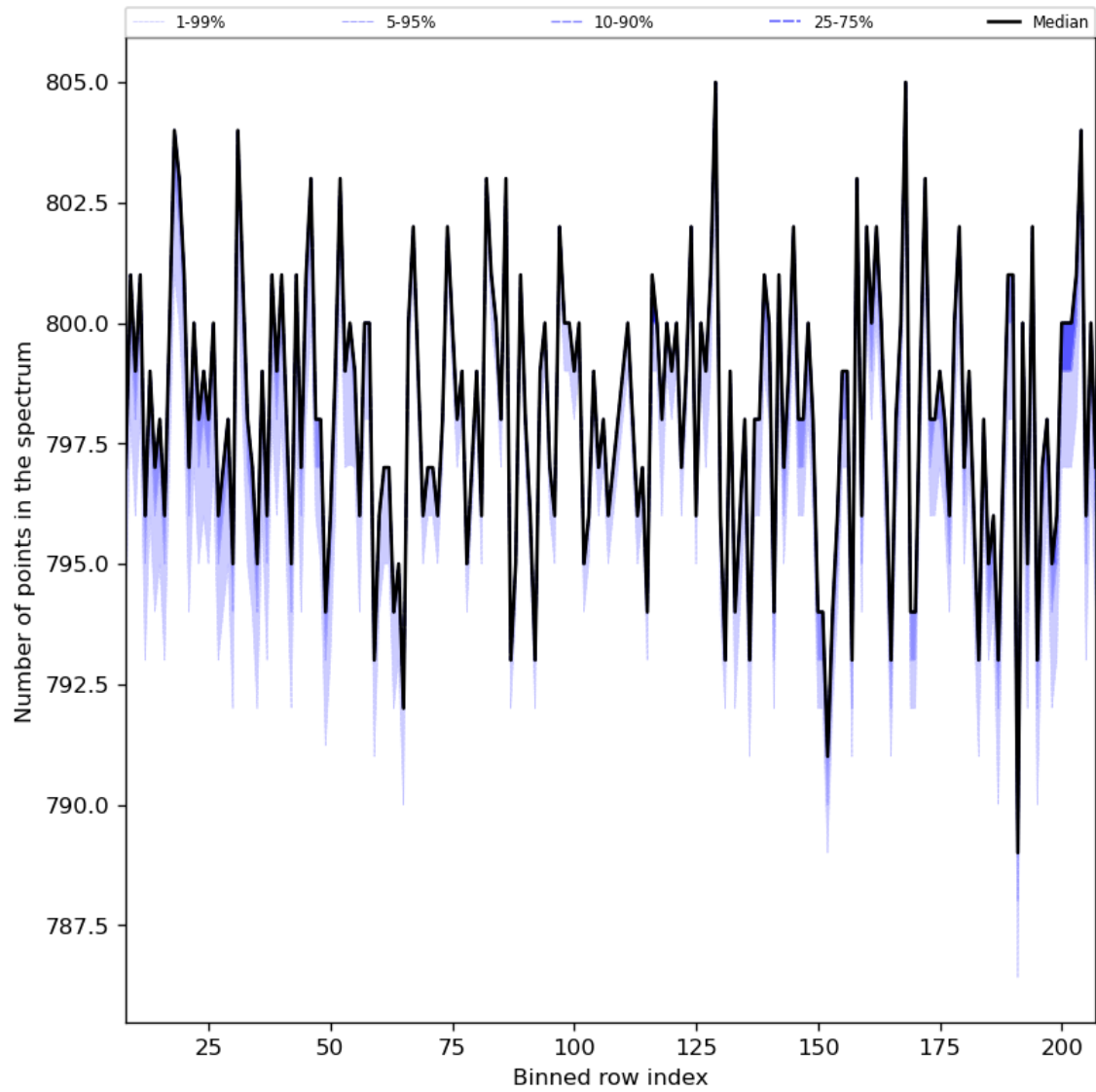
Figure 37: Along track statistics of “Number of points in the spectrum” for 2024-08-01 to 2024-08-03
