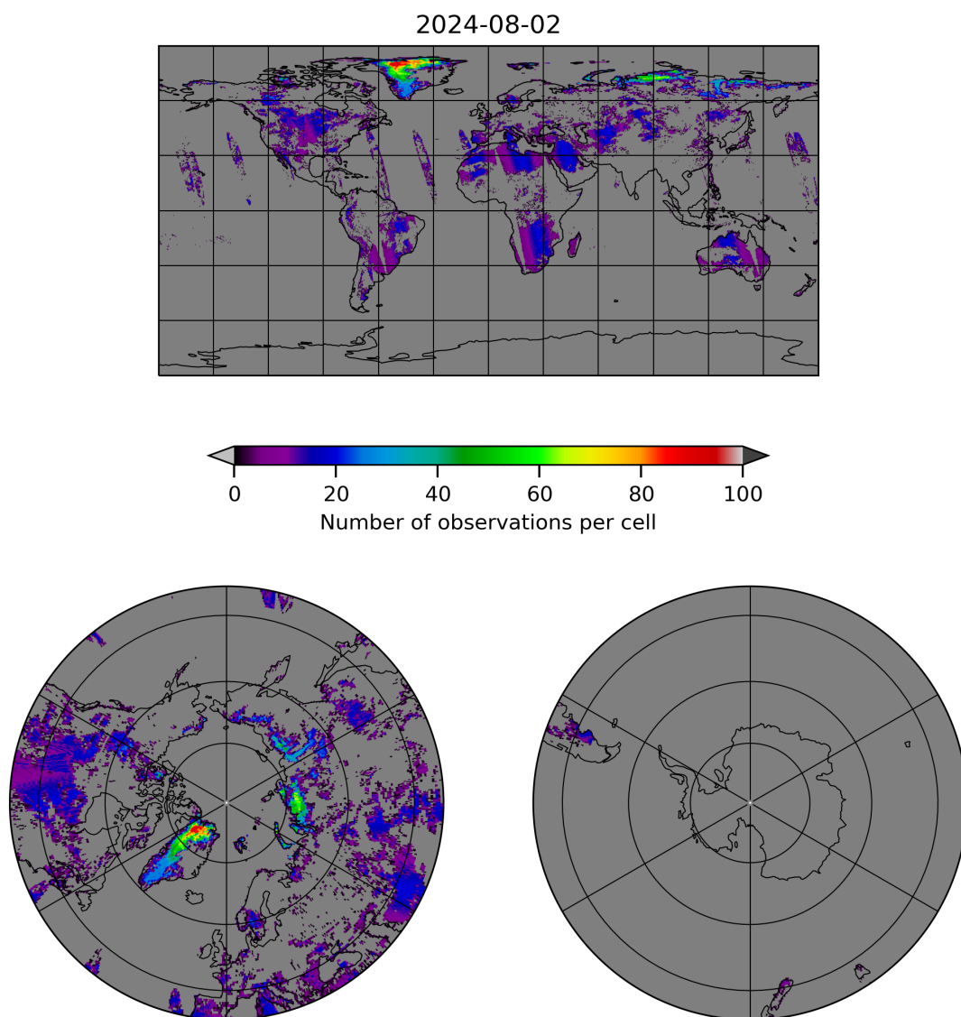
Figure 10: Map of the number of observations for 2024-08-01 to 2024-08-03
