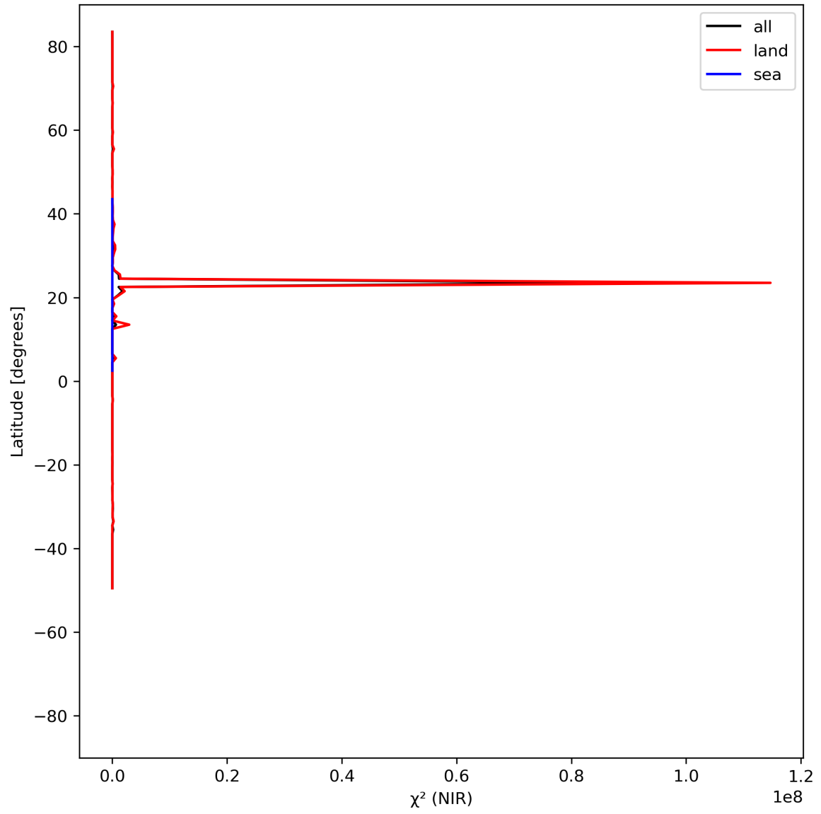
Figure 18: Zonal average of “ \chi^2 (NIR)” for 2024-08-01 to 2024-08-03.
