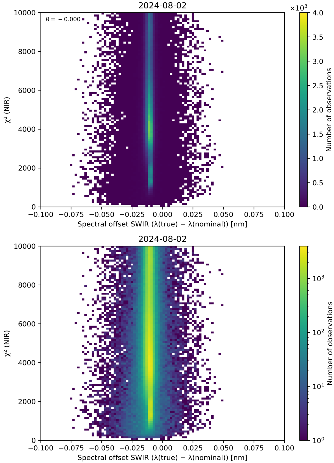
Figure 117: Scatter density plot of “Spectral offset SWIR ( \lambda(\text{true}) - \lambda(\text{nominal}) )” against “ \chi^2 (NIR)” for 2024-08-01 to 2024-08-03.
