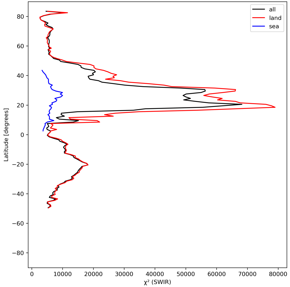
Figure 17: Zonal average of “ \chi^2 (SWIR)” for 2024-08-01 to 2024-08-03.
