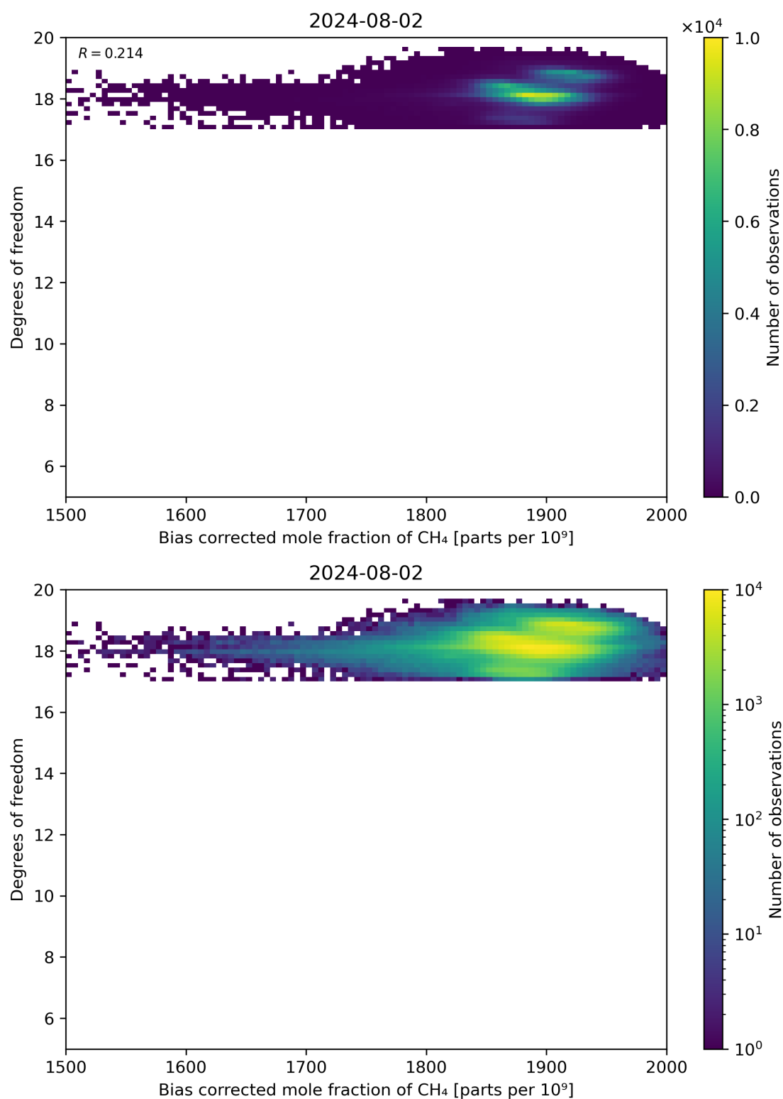
Figure 65: Scatter density plot of “Bias corrected mole fraction of CH 4 ” against “Degrees of freedom” for 2024-08-01 to 2024-08-03.
