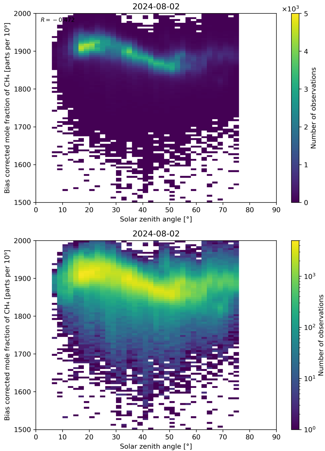
Figure 100: Scatter density plot of “Solar zenith angle” against “Bias corrected mole fraction of CH 4 ” for 2024-08-01 to 2024-08-03.
