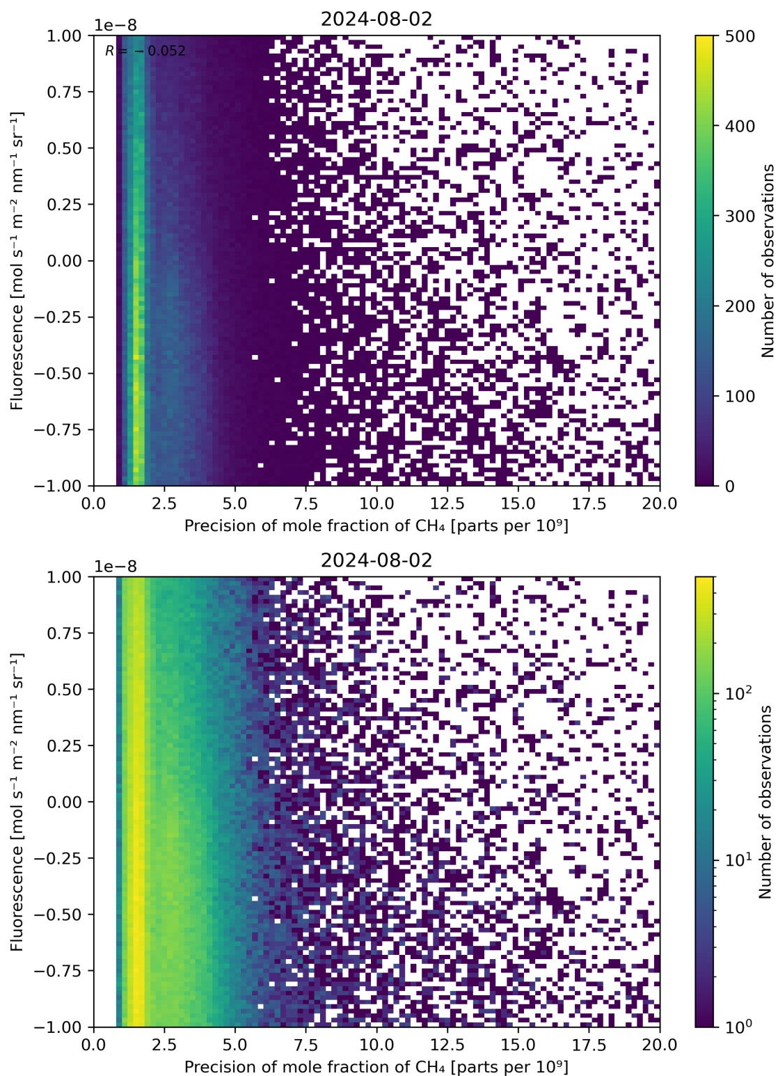
Figure 81: Scatter density plot of “Precision of mole fraction of \text{CH}_4 ” against “Fluorescence” for 2024-08-01 to 2024-08-03.
