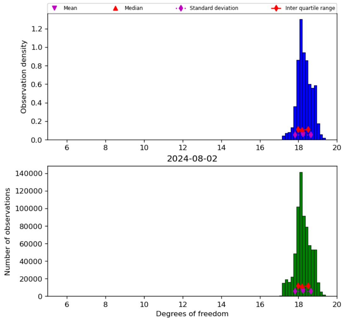
Figure 30: Histogram of “Degrees of freedom” for 2024-08-01 to 2024-08-03
