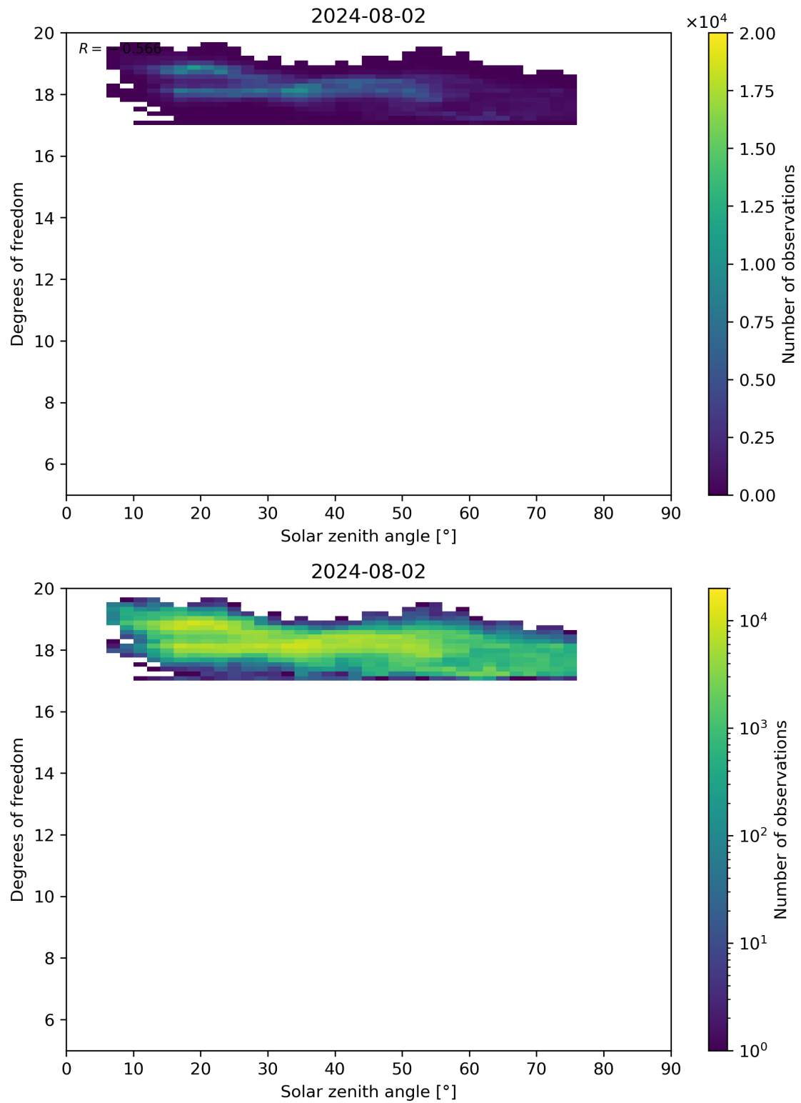
Figure 96: Scatter density plot of “Solar zenith angle” against “Degrees of freedom” for 2024-08-01 to 2024-08-03.
