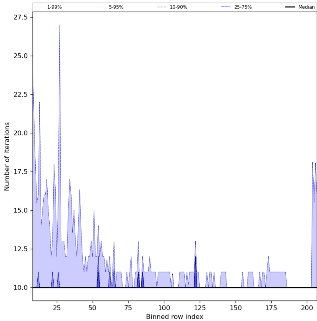
Figure 42: Along track statistics of “Number of iterations” for 2024-08-01 to 2024-08-03
