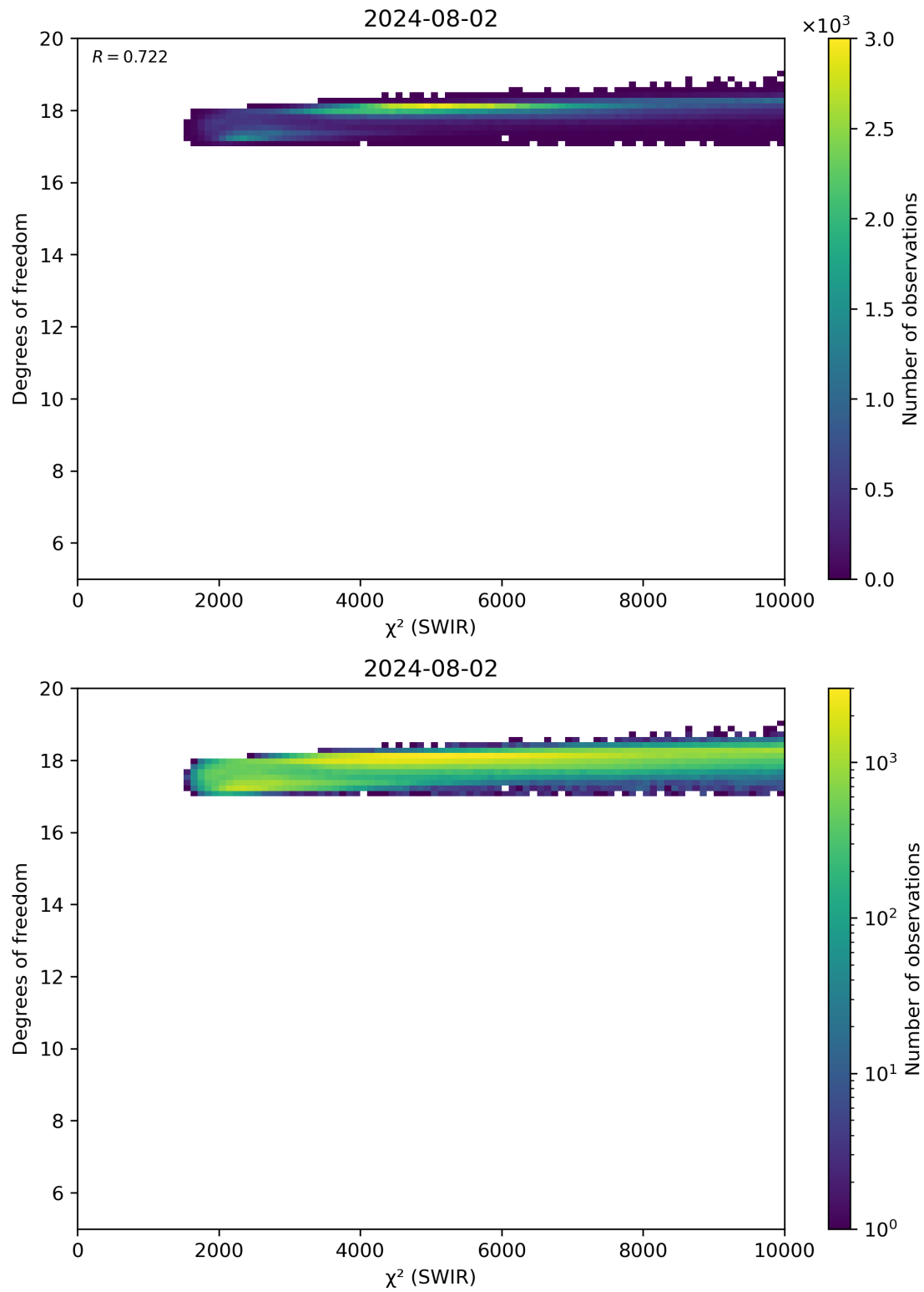
Figure 48: Scatter density plot of “ \chi^2 (SWIR)” against “Degrees of freedom” for 2024-08-01 to 2024-08-03.
