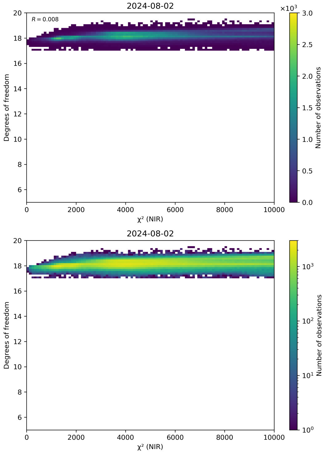
Figure 44: Scatter density plot of “ \chi^2 (NIR)” against “Degrees of freedom” for 2024-08-01 to 2024-08-03.
