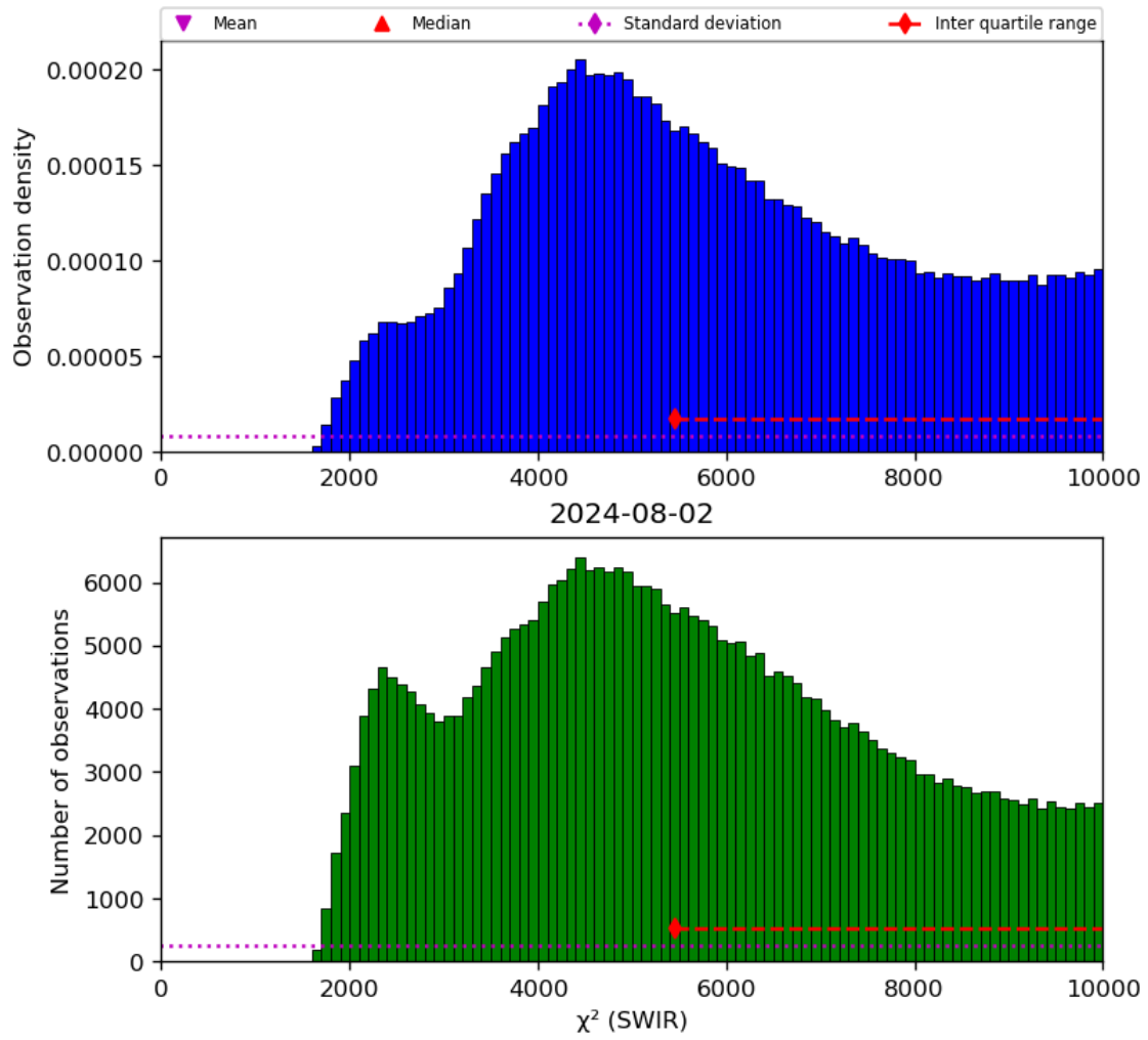
Figure 28: Histogram of " \chi^2 (SWIR)" for 2024-08-01 to 2024-08-03
