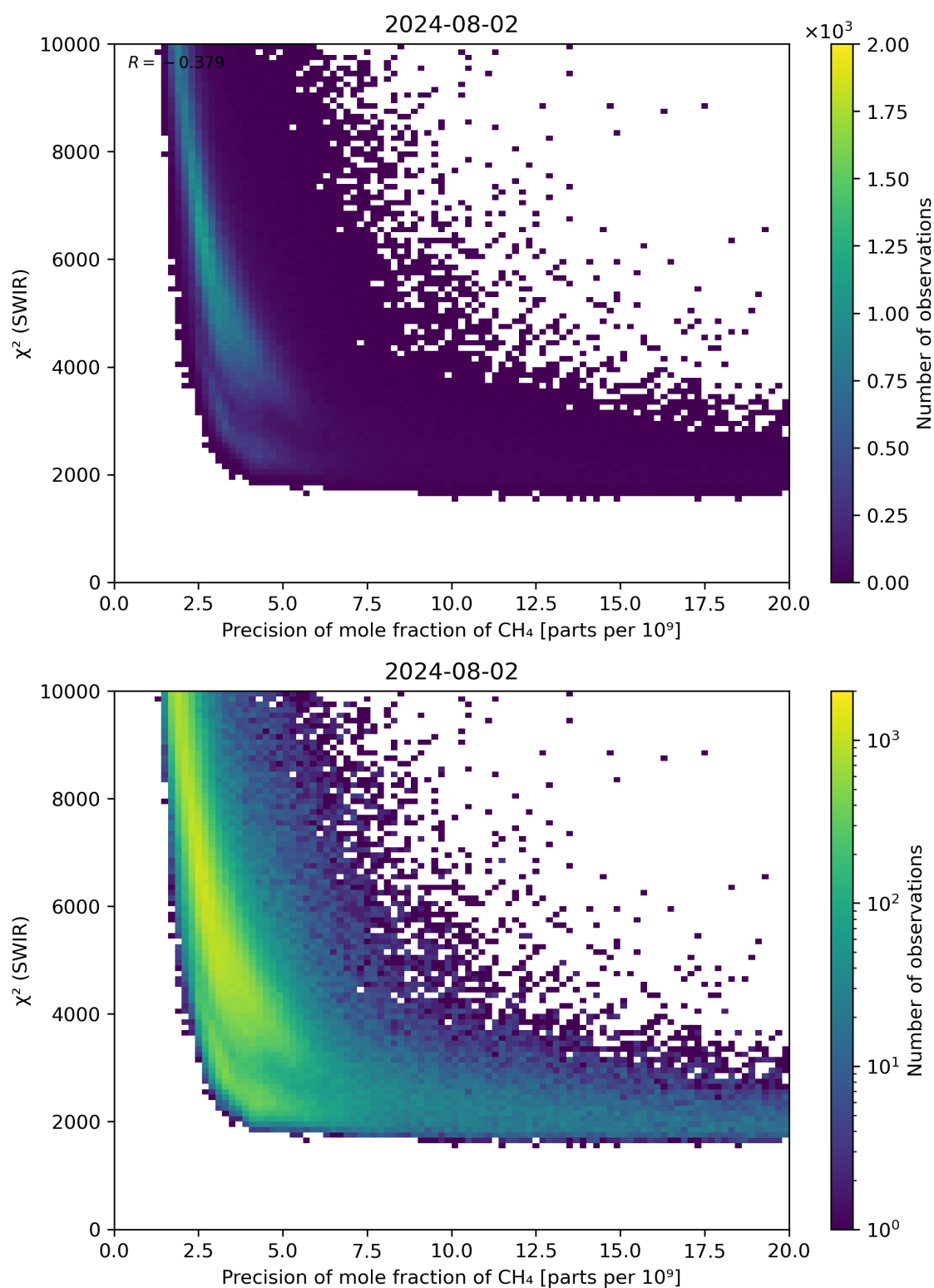
Figure 79: Scatter density plot of “Precision of mole fraction of \text{CH}_4 ” against “ \chi^2 (SWIR)” for 2024-08-01 to 2024-08-03.
