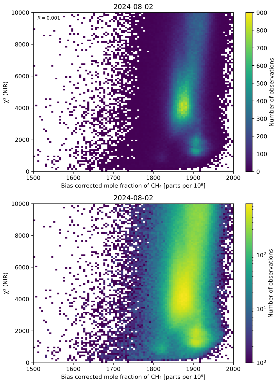
Figure 63: Scatter density plot of “Bias corrected mole fraction of CH 4 ” against “ \chi^2 (NIR)” for 2024-08-01 to 2024-08-03.
