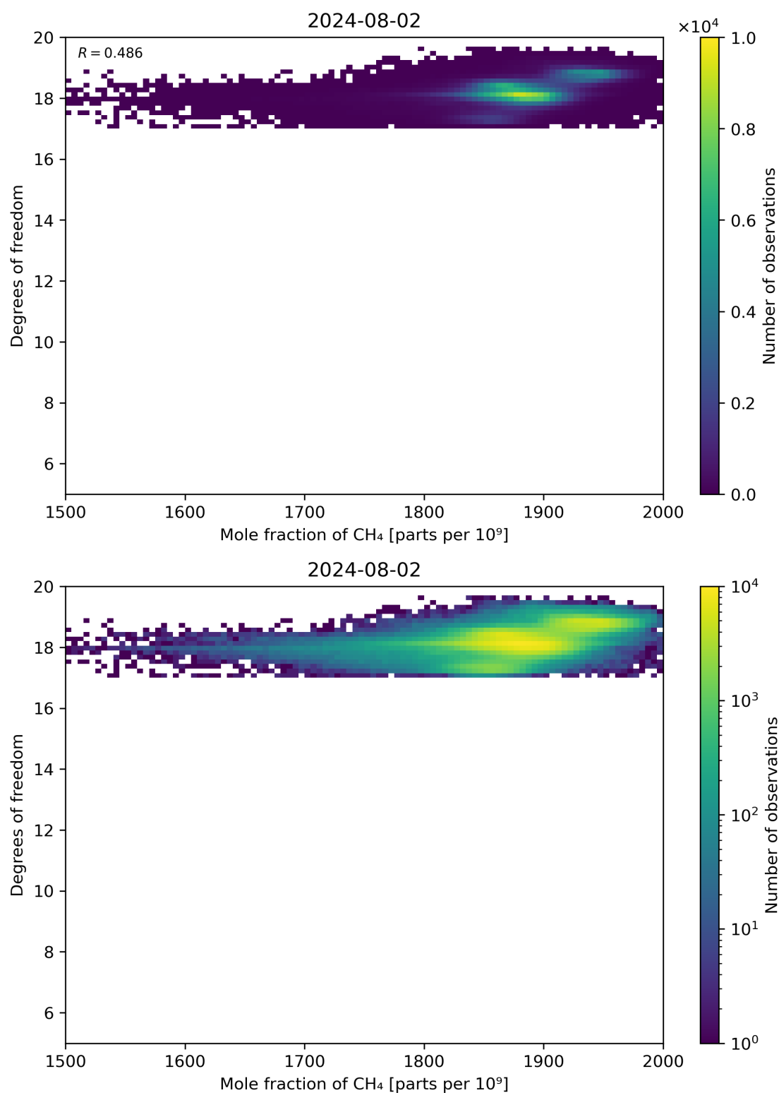
Figure 72: Scatter density plot of “Mole fraction of CH 4 ” against “Degrees of freedom” for 2024-08-01 to 2024-08-03.
