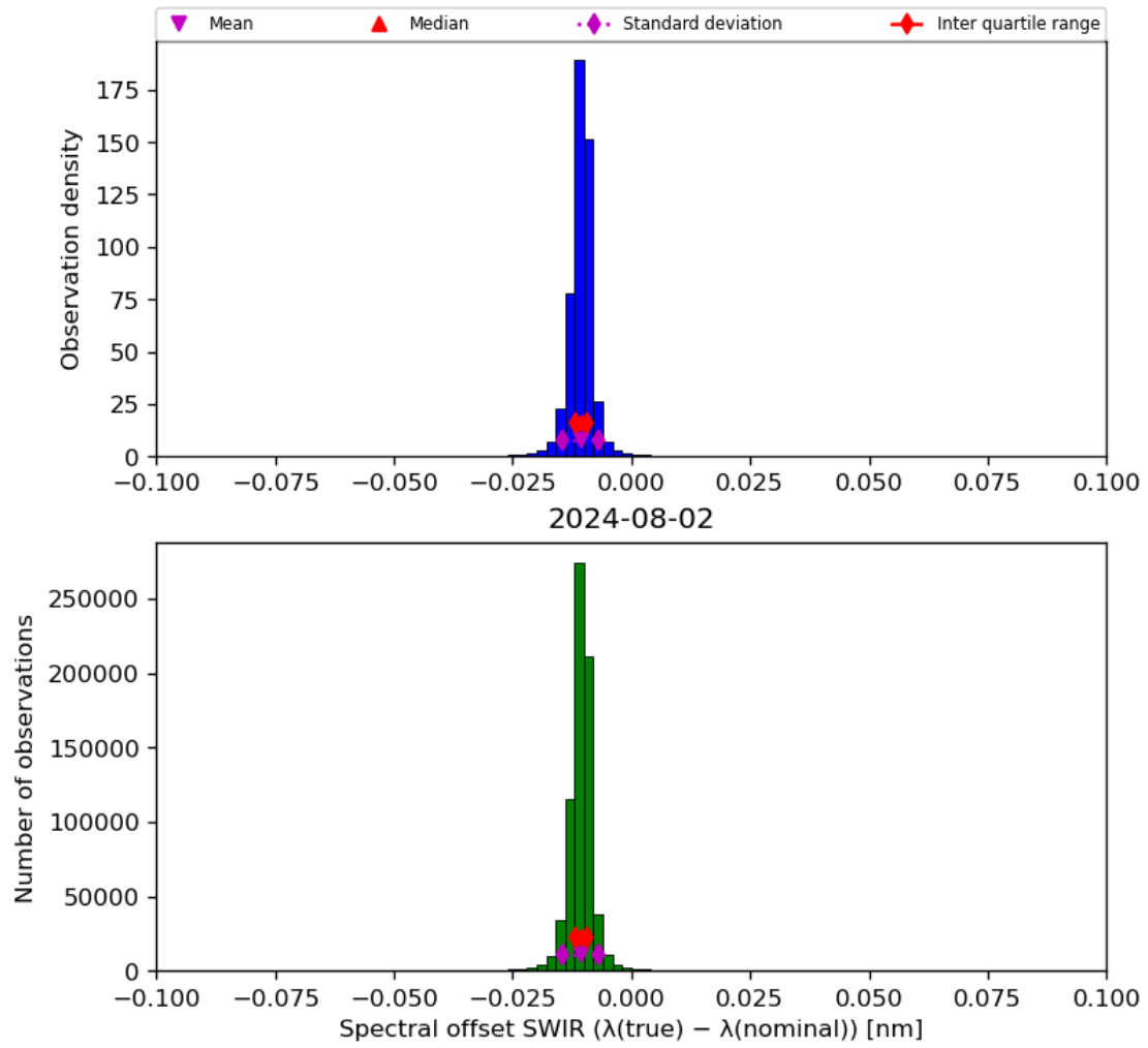
Figure 27: Histogram of “Spectral offset SWIR ( \lambda(\text{true}) - \lambda(\text{nominal}) )” for 2024-08-01 to 2024-08-03
