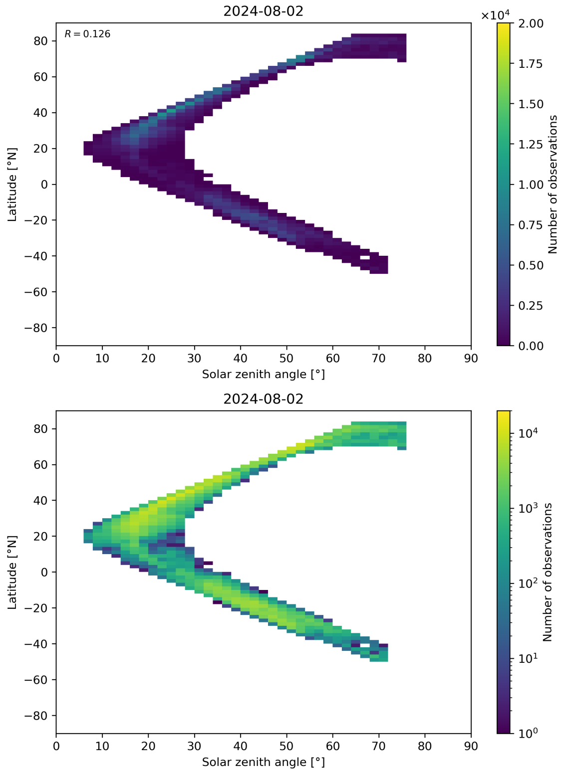
Figure 98: Scatter density plot of “Solar zenith angle” against “Latitude” for 2024-08-01 to 2024-08-03.
