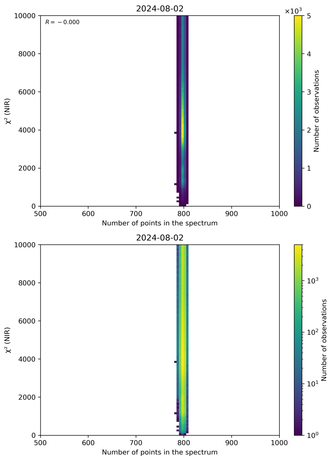
Figure 88: Scatter density plot of “Number of points in the spectrum” against “ \chi^2 (NIR)” for 2024-08-01 to 2024-08-03.
