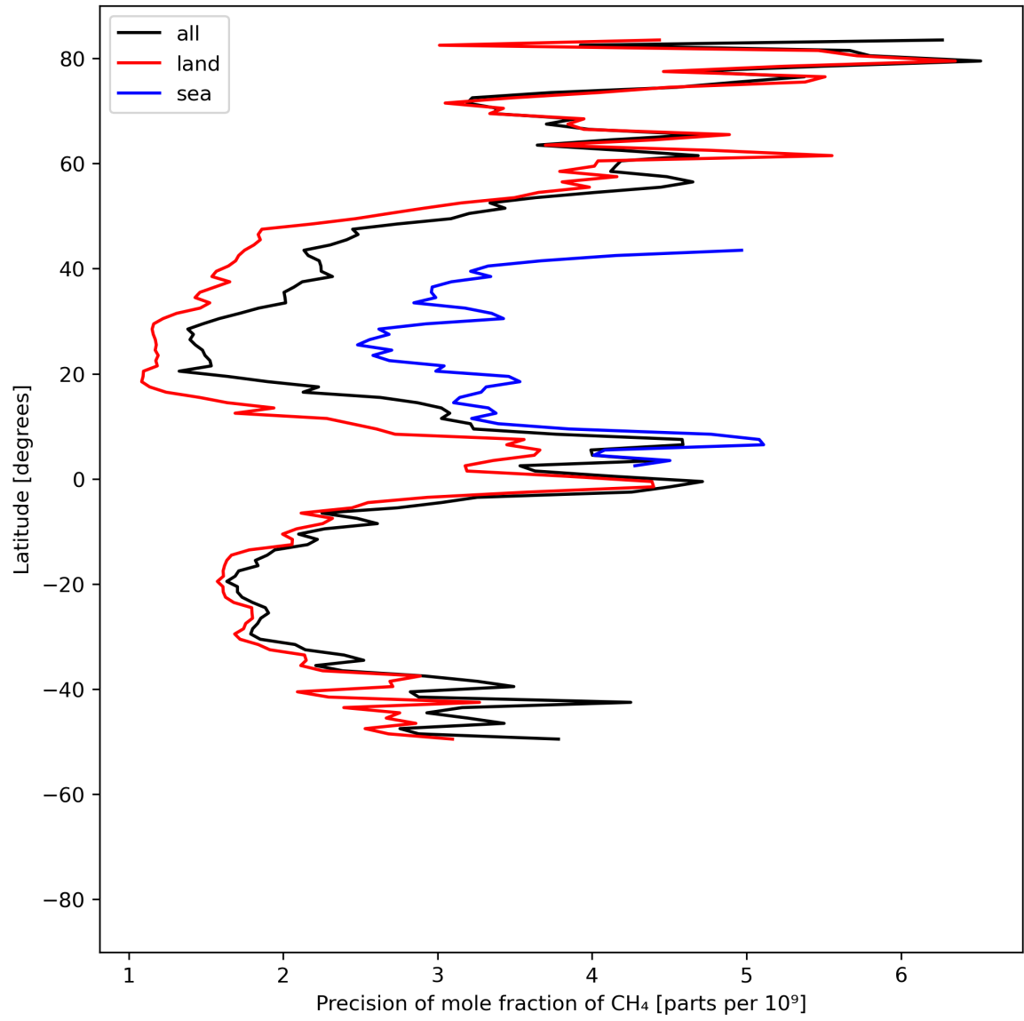
Figure 13: Zonal average of “Precision of mole fraction of CH 4 ” for 2024-08-01 to 2024-08-03.
