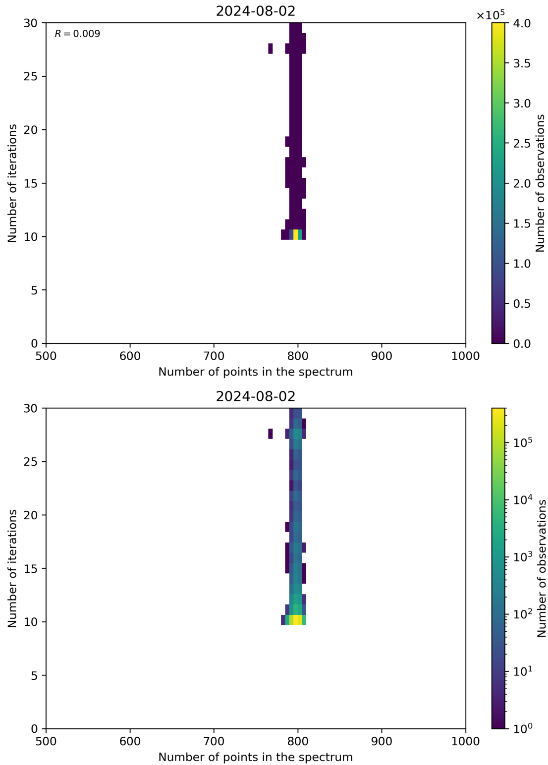
Figure 92: Scatter density plot of “Number of points in the spectrum” against “Number of iterations” for 2024-08-01 to 2024-08-03.
