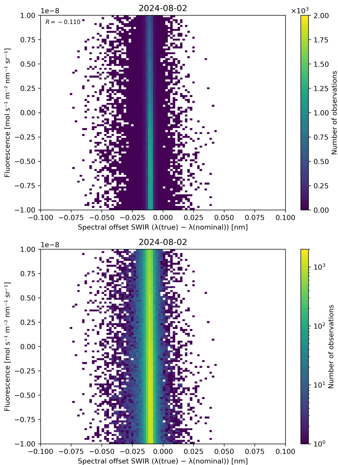
Figure 120: Scatter density plot of “Spectral offset SWIR ( \lambda(\text{true}) - \lambda(\text{nominal}) )” against “Fluorescence” for 2024-08-01 to 2024-08-03.
