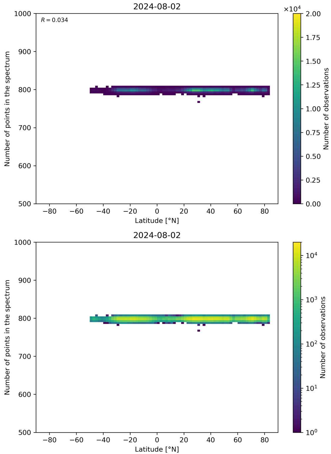
Figure 61: Scatter density plot of “Latitude” against “Number of points in the spectrum” for 2024-08-01 to 2024-08-03.
