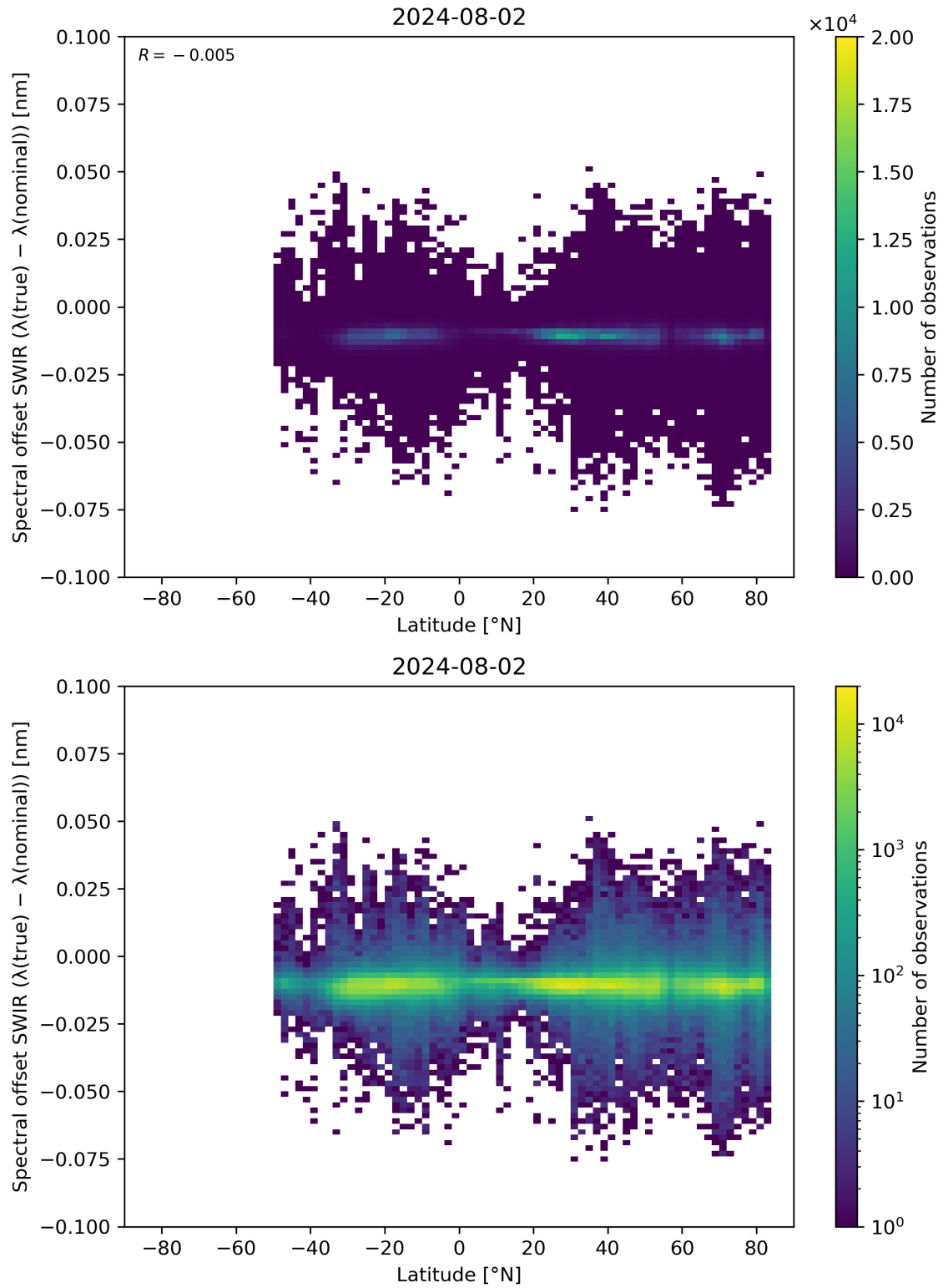
Figure 62: Scatter density plot of “Latitude” against “Spectral offset SWIR ( \lambda(\text{true}) - \lambda(\text{nominal}) )” for 2024-08-01 to 2024-08-03.
