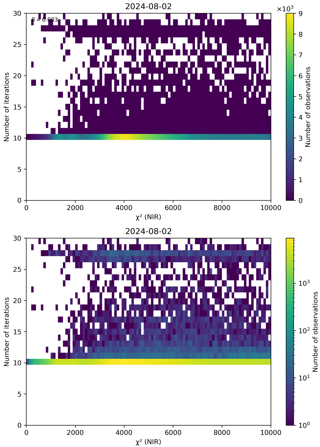
Figure 46: Scatter density plot of “ \chi^2 (NIR)” against “Number of iterations” for 2024-08-01 to 2024-08-03.
