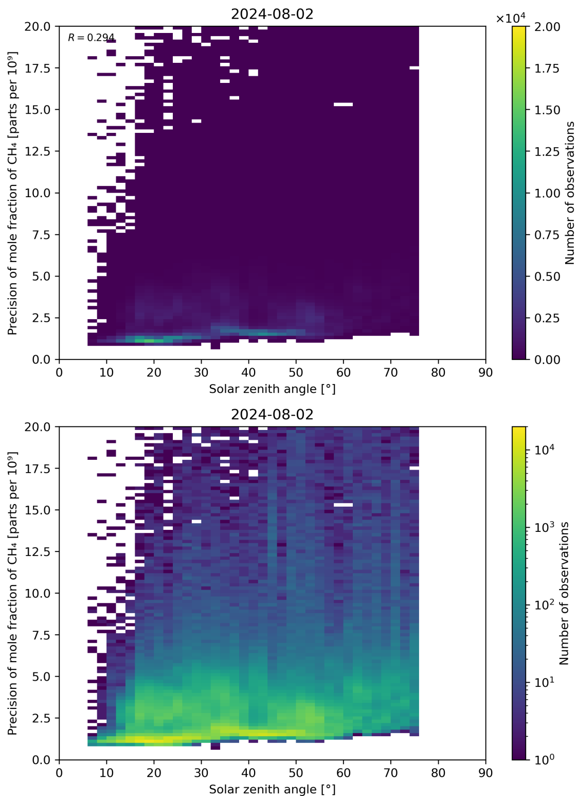
Figure 101: Scatter density plot of “Solar zenith angle” against “Precision of mole fraction of CH 4 ” for 2024-08-01 to 2024-08-03.
