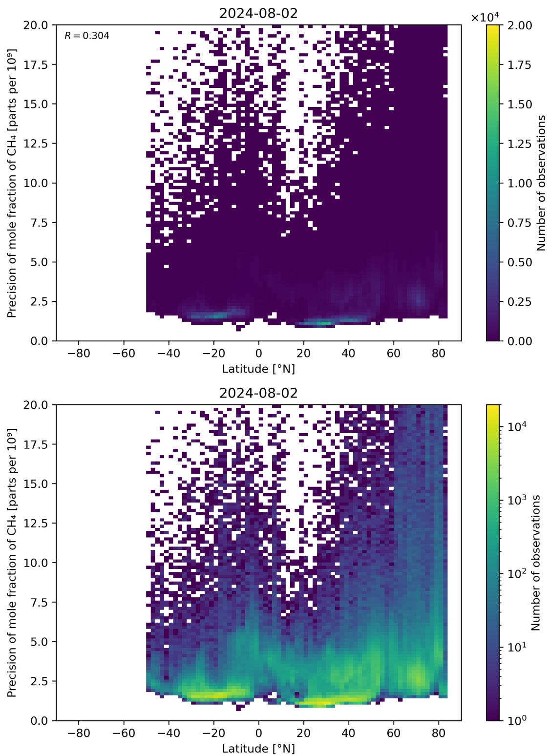
Figure 59: Scatter density plot of “Latitude” against “Precision of mole fraction of \text{CH}_4 ” for 2024-08-01 to 2024-08-03.
