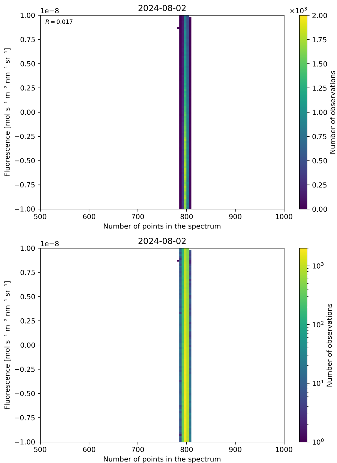
Figure 91: Scatter density plot of “Number of points in the spectrum” against “Fluorescence” for 2024-08-01 to 2024-08-03.
