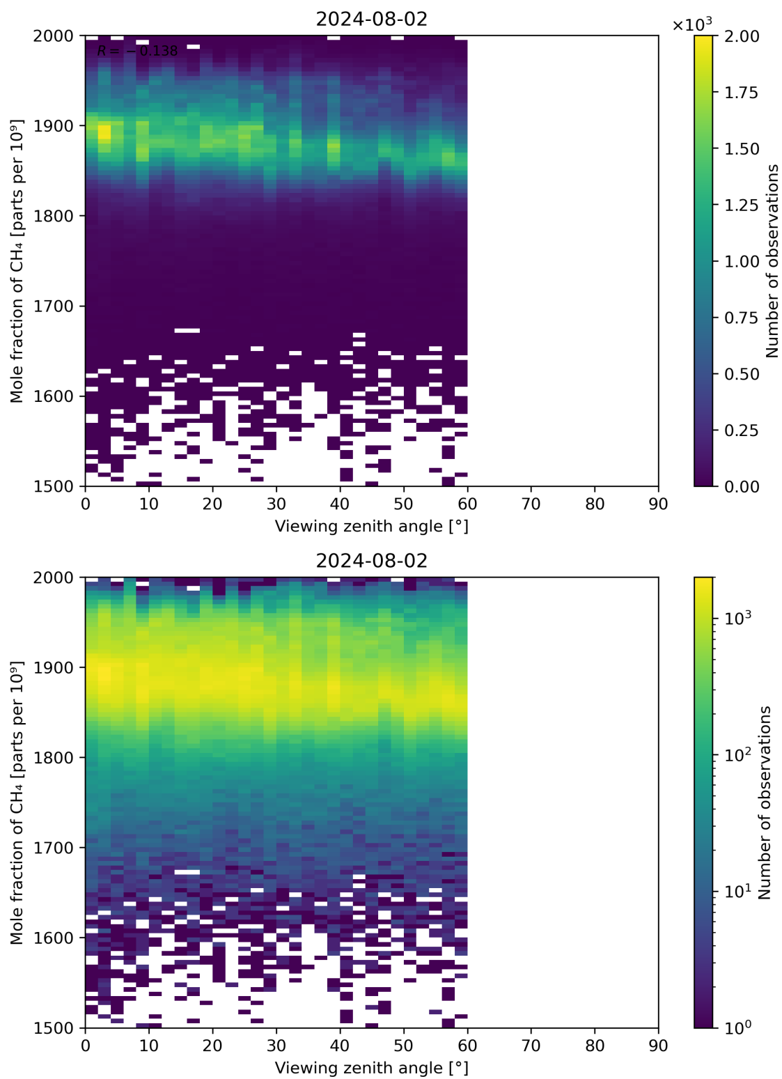
Figure 110: Scatter density plot of “Viewing zenith angle” against “Mole fraction of CH 4 ” for 2024-08-01 to 2024-08-03.
