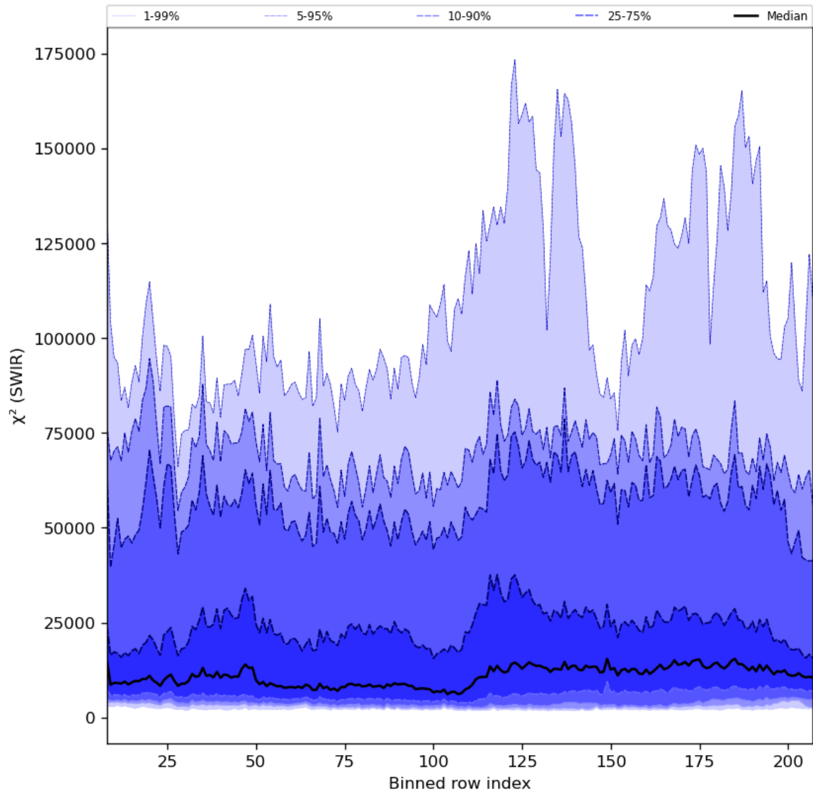
Figure 39: Along track statistics of “ \chi^2 (SWIR)” for 2024-08-01 to 2024-08-03
