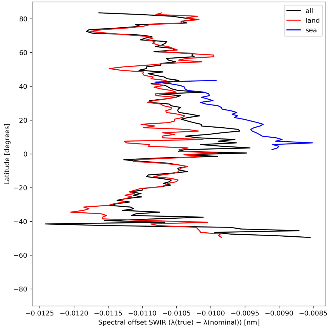
Figure 16: Zonal average of “Spectral offset SWIR ( \lambda(\text{true}) - \lambda(\text{nominal}) )” for 2024-08-01 to 2024-08-03.
