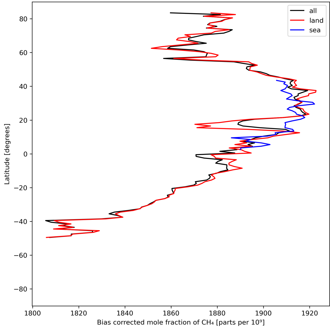
Figure 14: Zonal average of “Bias corrected mole fraction of \text{CH}_4 ” for 2024-08-01 to 2024-08-03.
