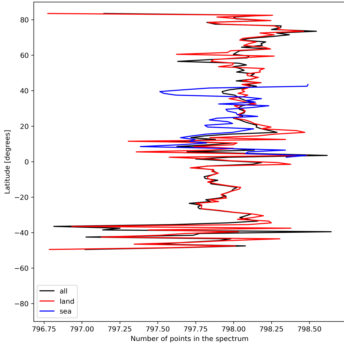
Figure 15: Zonal average of “Number of points in the spectrum” for 2024-08-01 to 2024-08-03.
