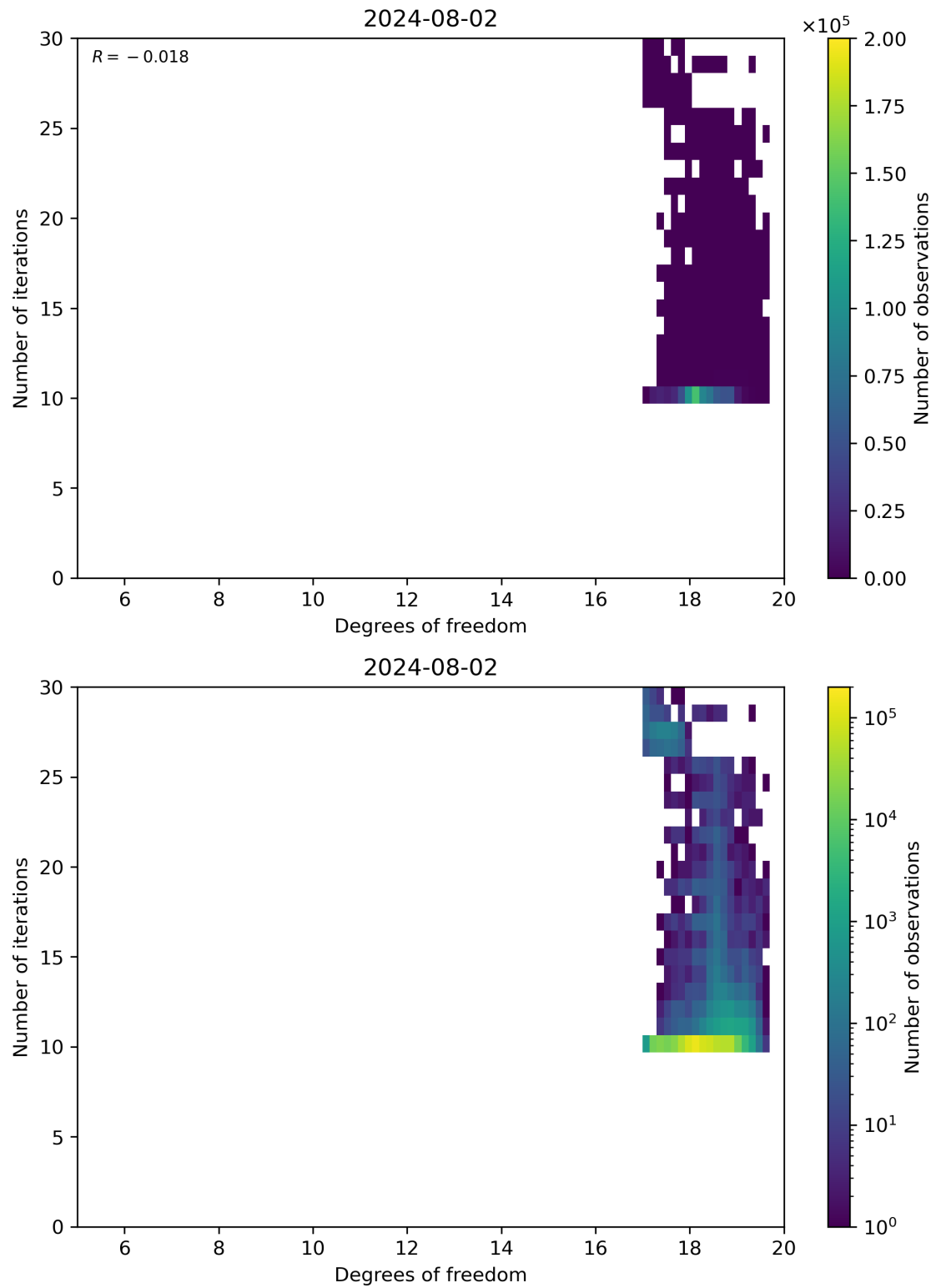
Figure 52: Scatter density plot of “Degrees of freedom” against “Number of iterations” for 2024-08-01 to 2024-08-03.
