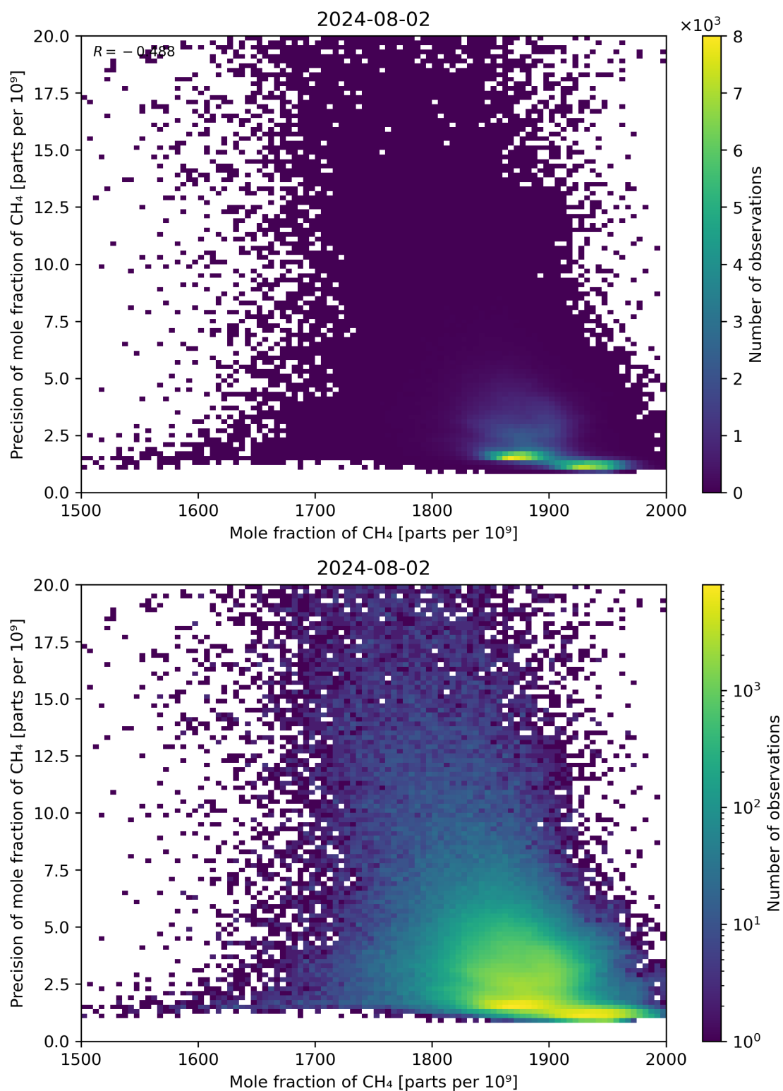
Figure 75: Scatter density plot of “Mole fraction of CH 4 ” against “Precision of mole fraction of CH 4 ” for 2024-08-01 to 2024-08-03.
