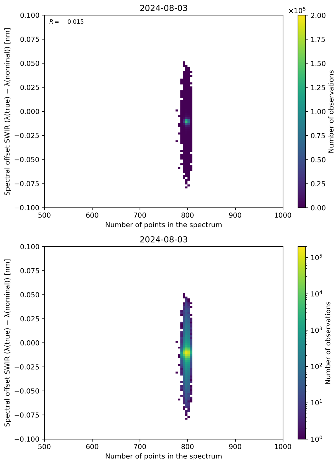
Figure 93: Scatter density plot of “Number of points in the spectrum” against “Spectral offset SWIR ( \lambda(\text{true}) - \lambda(\text{nominal}) )” for 2024-08-02 to 2024-08-04.
