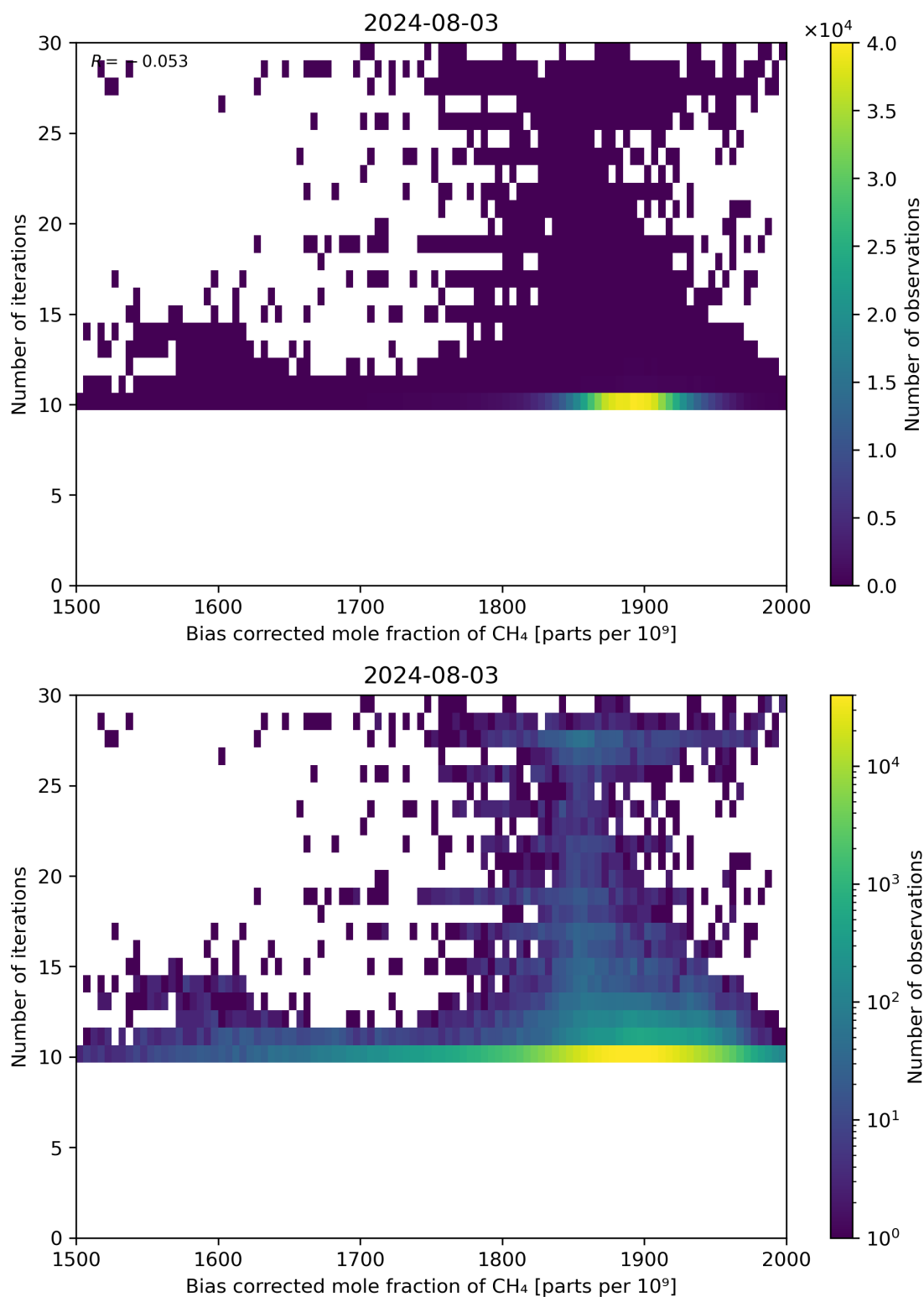
Figure 67: Scatter density plot of “Bias corrected mole fraction of CH 4 ” against “Number of iterations” for 2024-08-02 to 2024-08-04.
