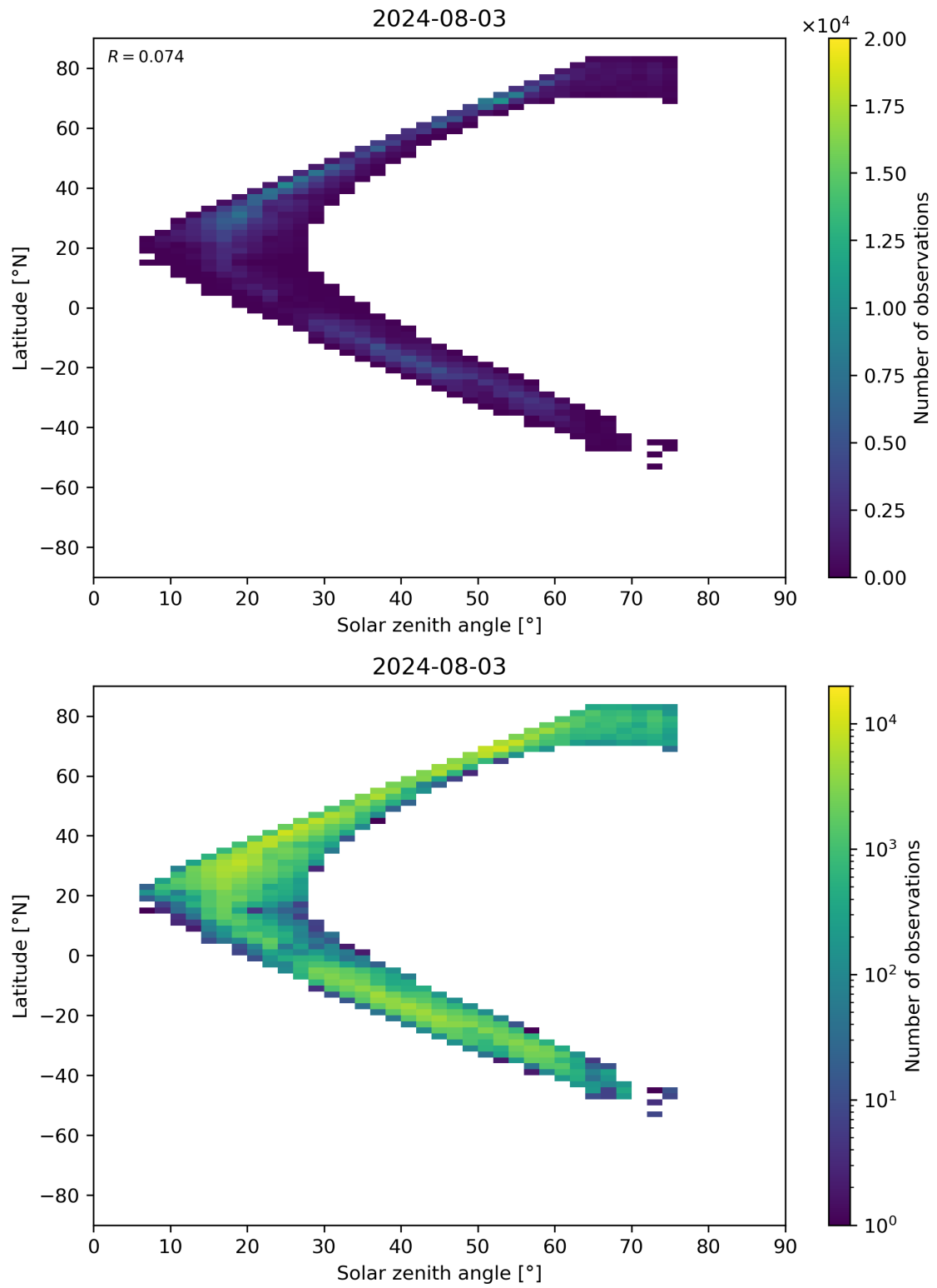
Figure 98: Scatter density plot of “Solar zenith angle” against “Latitude” for 2024-08-02 to 2024-08-04.
