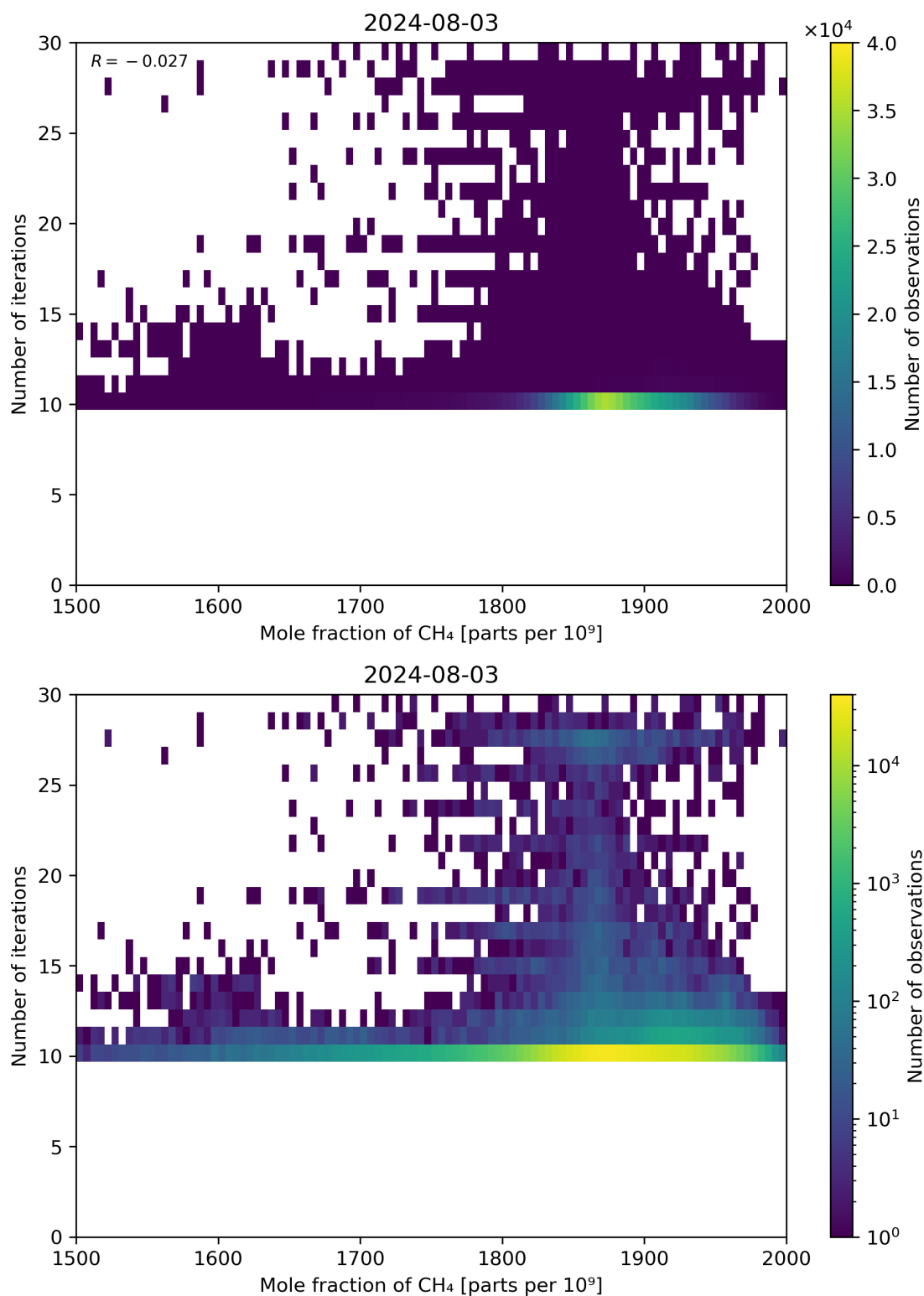
Figure 76: Scatter density plot of “Mole fraction of CH 4 ” against “Number of iterations” for 2024-08-02 to 2024-08-04.
