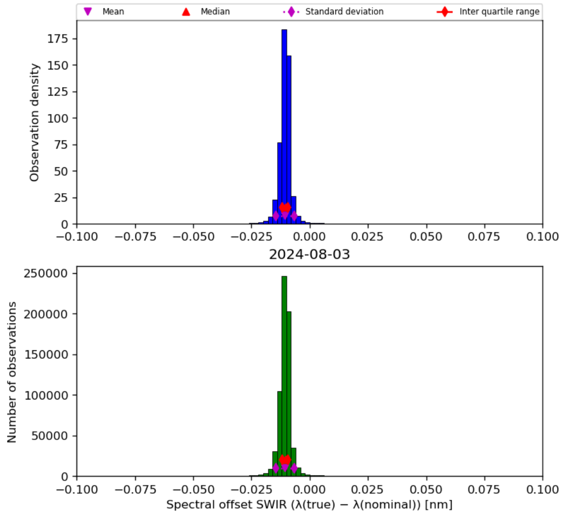
Figure 27: Histogram of “Spectral offset SWIR ( \lambda(\text{true}) - \lambda(\text{nominal}) )” for 2024-08-02 to 2024-08-04
