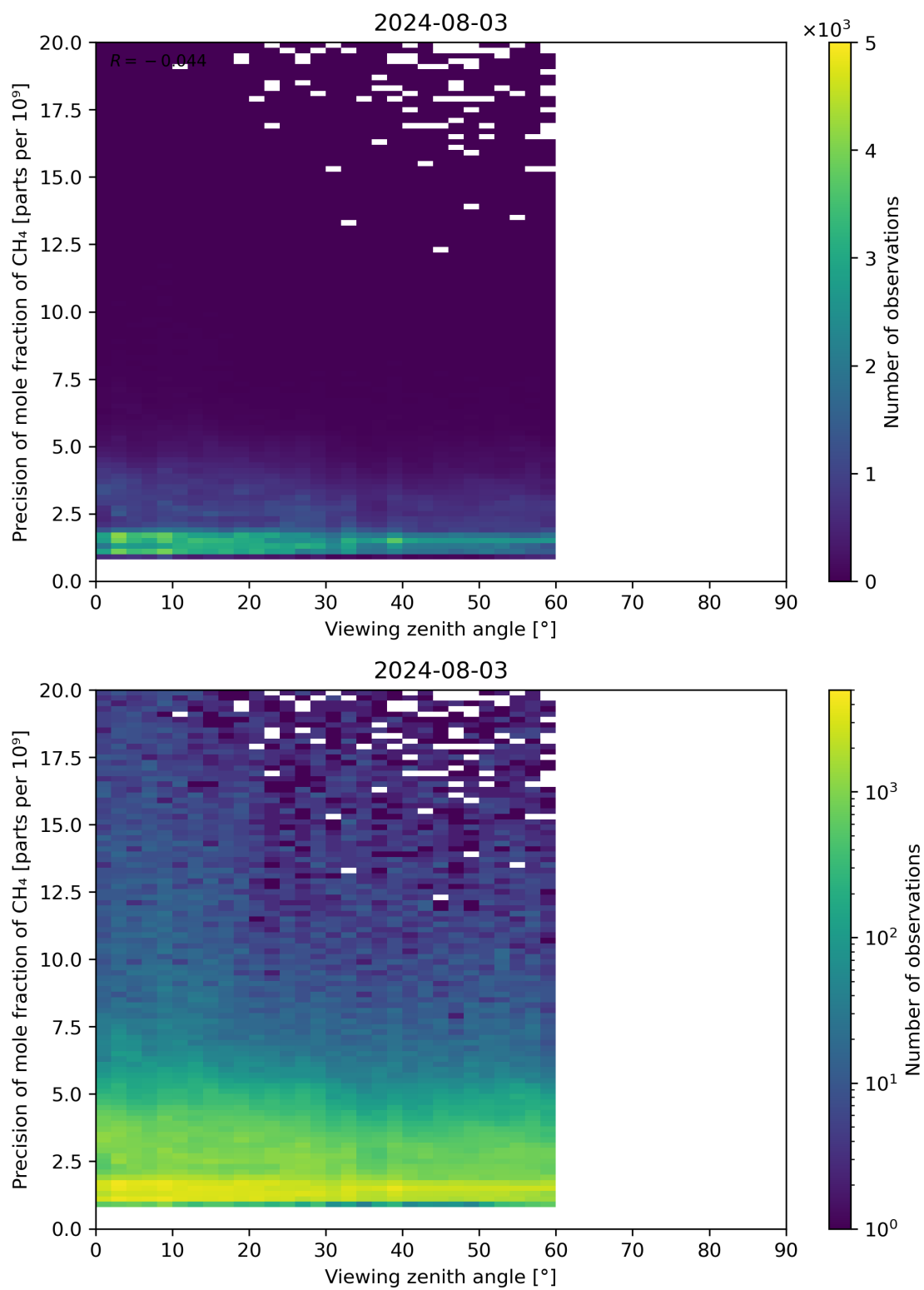
Figure 112: Scatter density plot of “Viewing zenith angle” against “Precision of mole fraction of CH 4 ” for 2024-08-02 to 2024-08-04.
