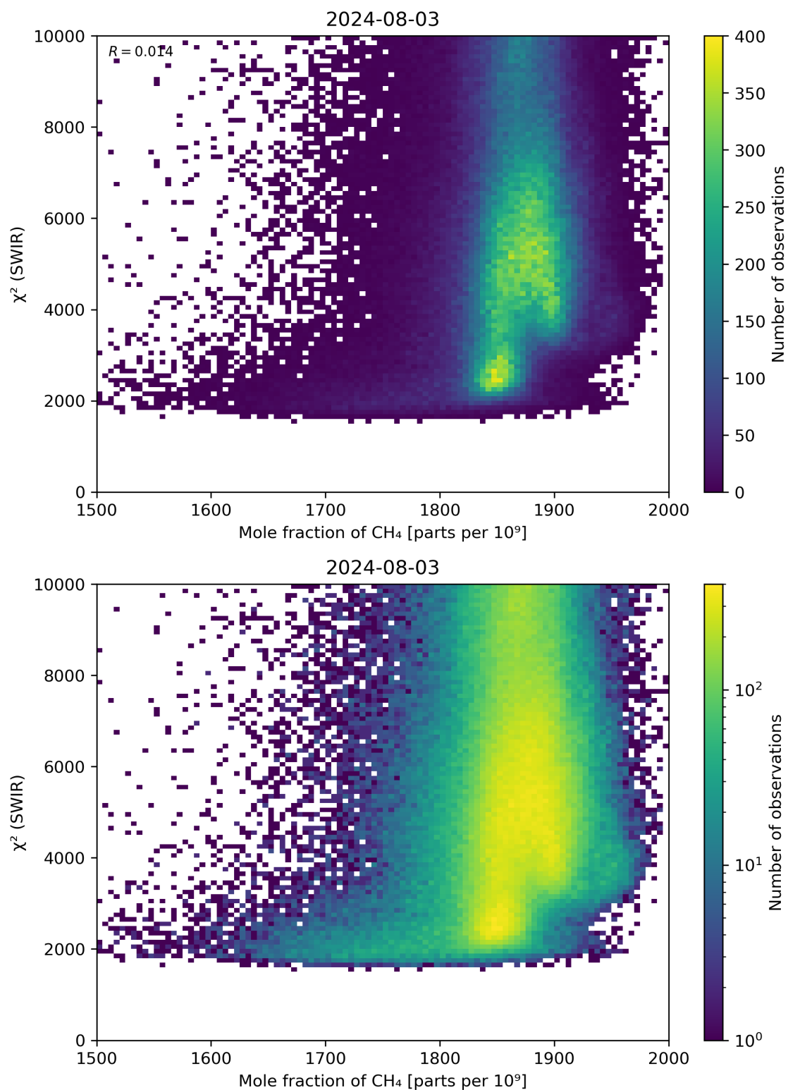
Figure 71: Scatter density plot of “Mole fraction of \text{CH}_4 ” against “ \chi^2 (SWIR)” for 2024-08-02 to 2024-08-04.
