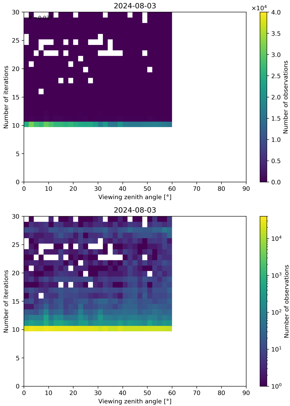
Figure 113: Scatter density plot of “Viewing zenith angle” against “Number of iterations” for 2024-08-02 to 2024-08-04.
