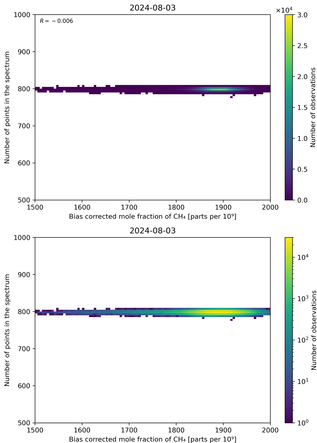
Figure 68: Scatter density plot of “Bias corrected mole fraction of CH 4 ” against “Number of points in the spectrum” for 2024-08-02 to 2024-08-04.
