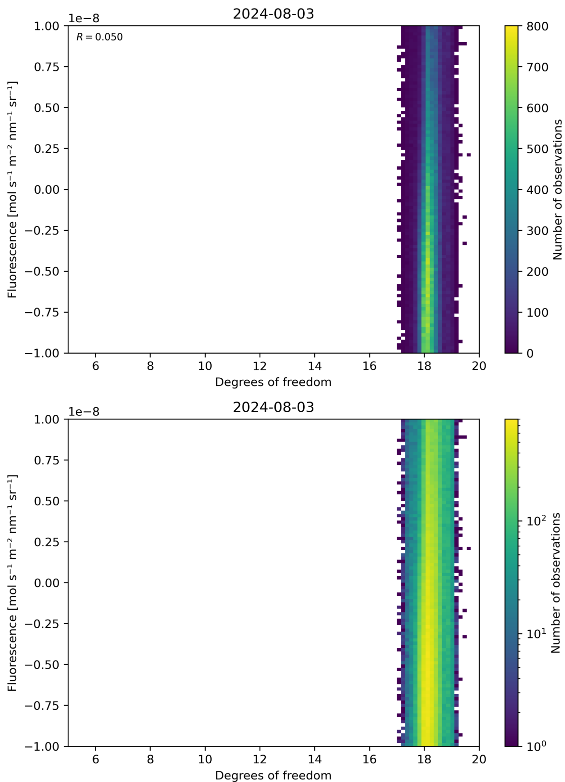
Figure 51: Scatter density plot of “Degrees of freedom” against “Fluorescence” for 2024-08-02 to 2024-08-04.
