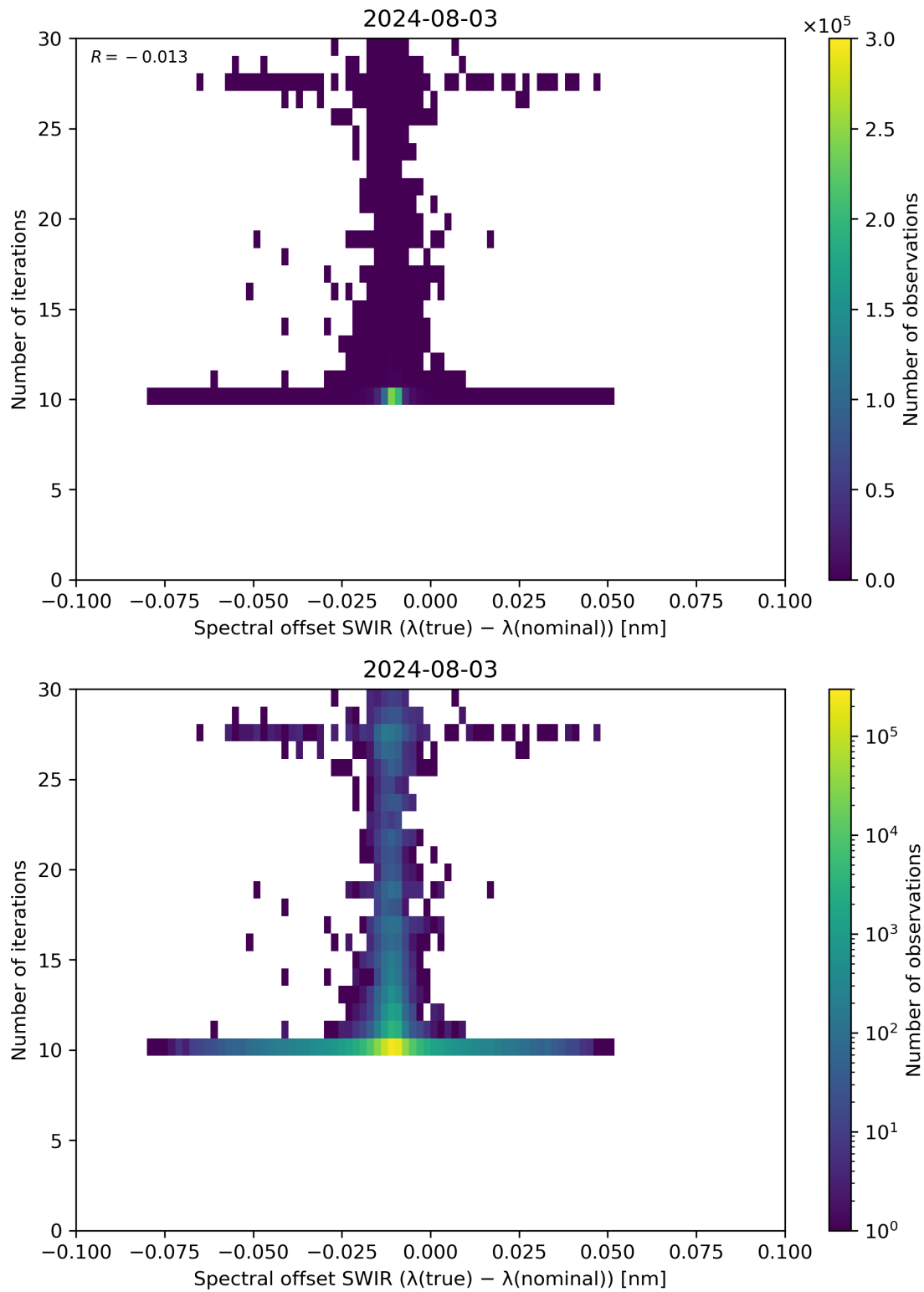
Figure 121: Scatter density plot of “Spectral offset SWIR ( \lambda(\text{true}) - \lambda(\text{nominal}) )” against “Number of iterations” for 2024-08-02 to 2024-08-04.
