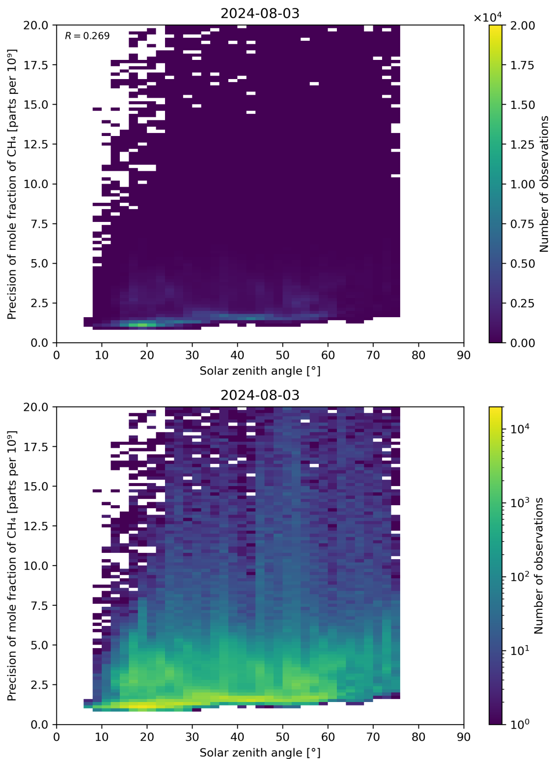
Figure 101: Scatter density plot of “Solar zenith angle” against “Precision of mole fraction of CH 4 ” for 2024-08-02 to 2024-08-04.
