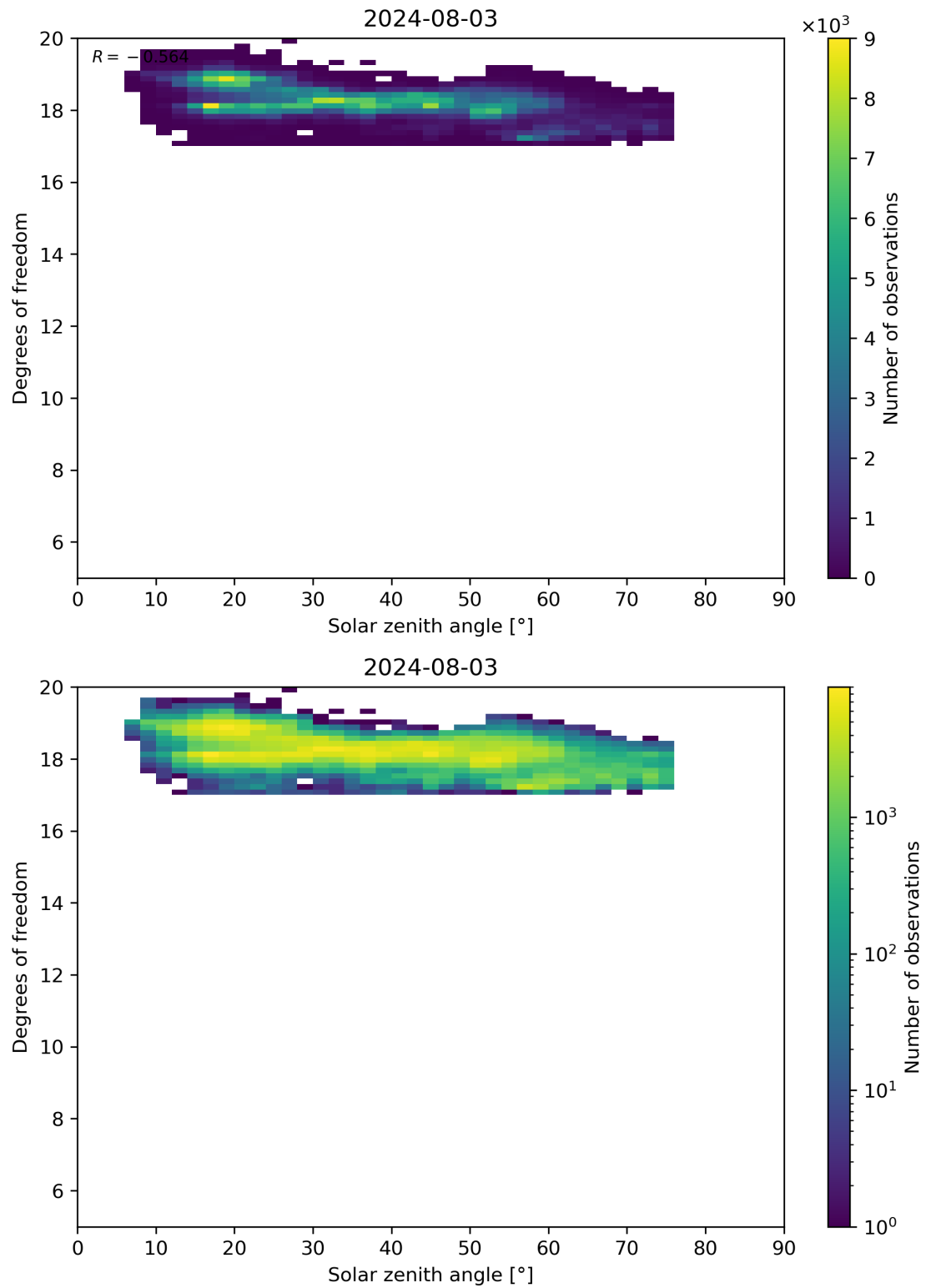
Figure 96: Scatter density plot of “Solar zenith angle” against “Degrees of freedom” for 2024-08-02 to 2024-08-04.
