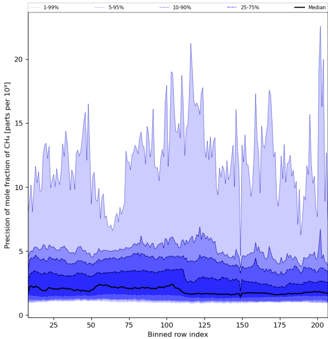
Figure 35: Along track statistics of “Precision of mole fraction of CH 4 ” for 2024-08-02 to 2024-08-04
