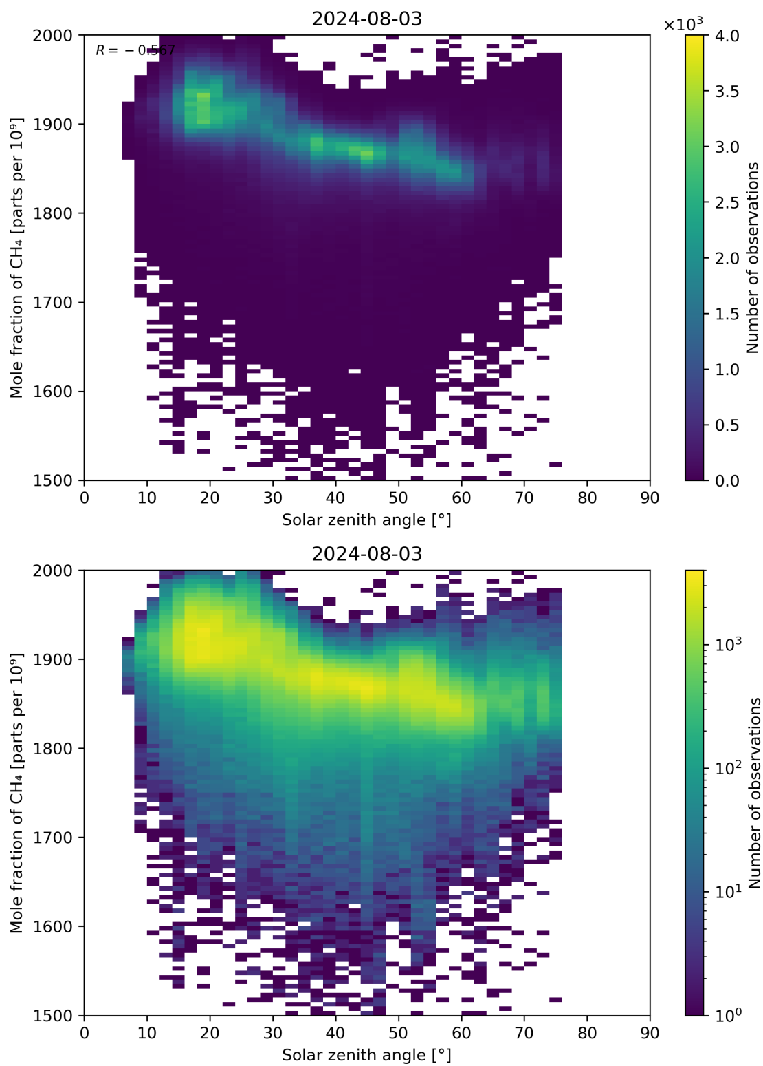
Figure 99: Scatter density plot of “Solar zenith angle” against “Mole fraction of CH 4 ” for 2024-08-02 to 2024-08-04.
