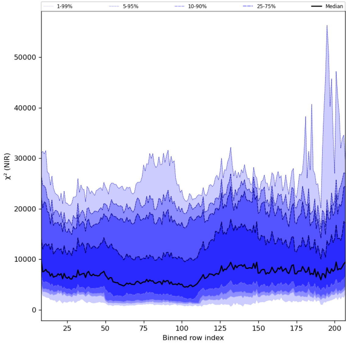
Figure 40: Along track statistics of “ \chi^2 (NIR)” for 2024-08-02 to 2024-08-04
