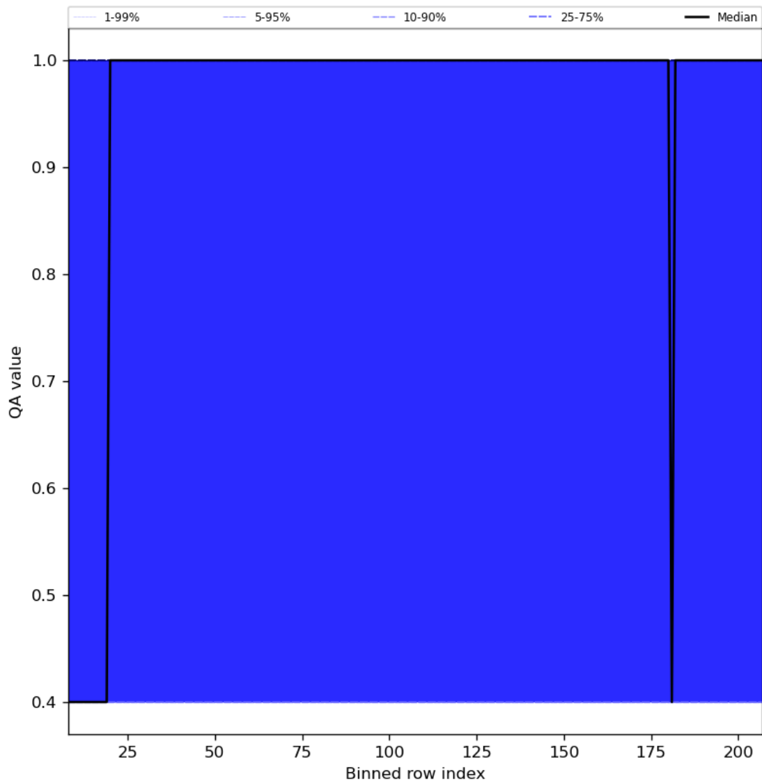
Figure 33: Along track statistics of “QA value” for 2024-08-02 to 2024-08-04
