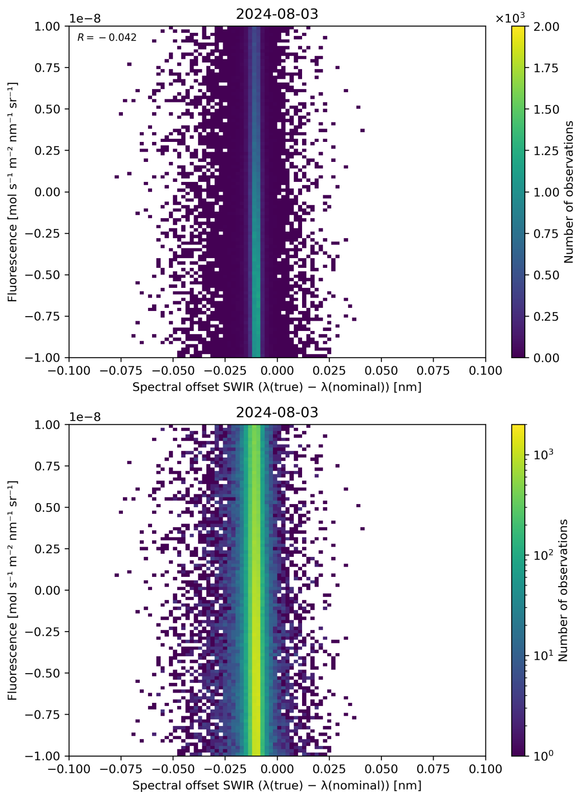
Figure 120: Scatter density plot of “Spectral offset SWIR ( \lambda(\text{true}) - \lambda(\text{nominal}) )” against “Fluorescence” for 2024-08-02 to 2024-08-04.
