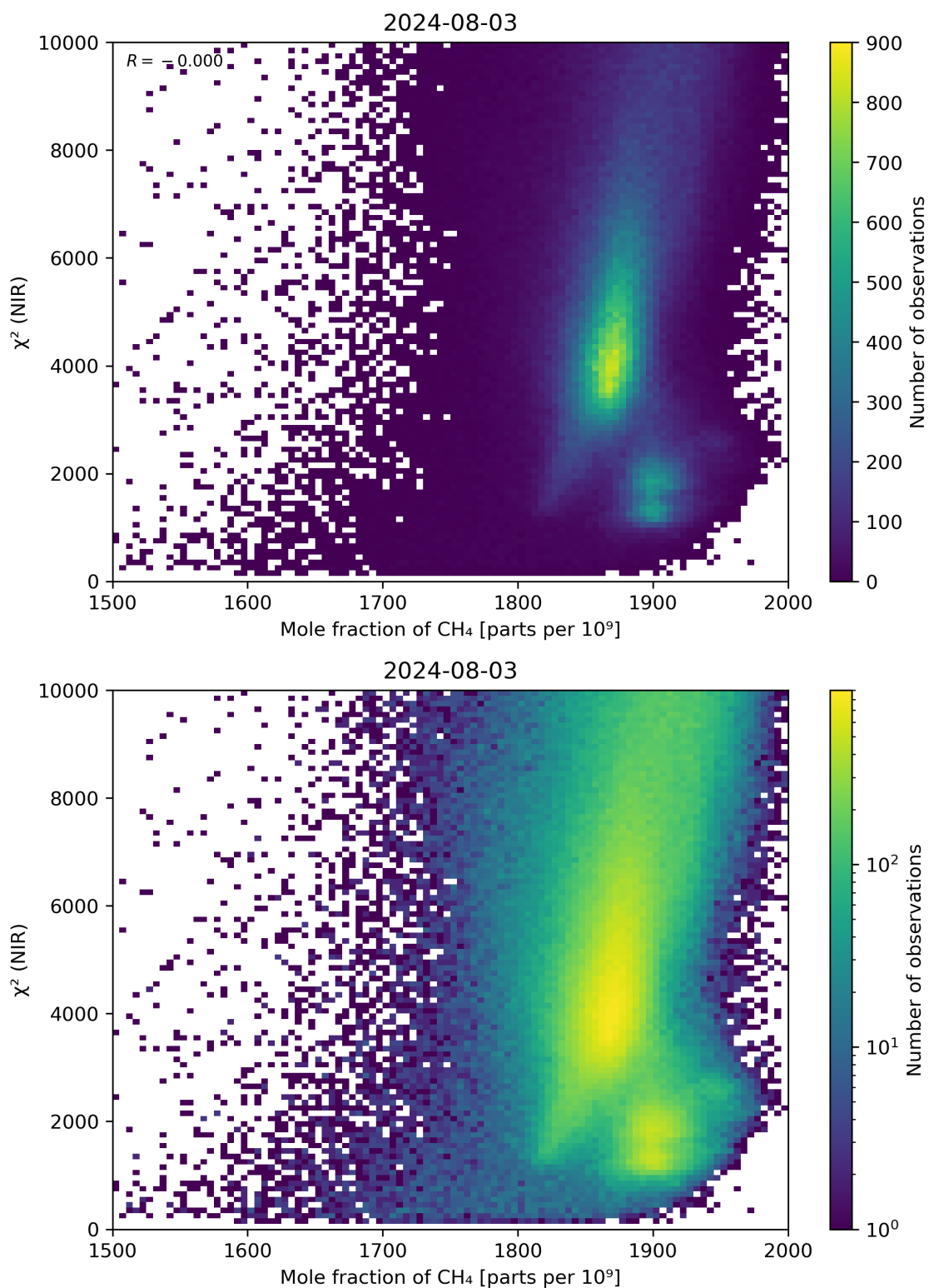
Figure 70: Scatter density plot of “Mole fraction of CH 4 ” against “ \chi^2 (NIR)” for 2024-08-02 to 2024-08-04.
