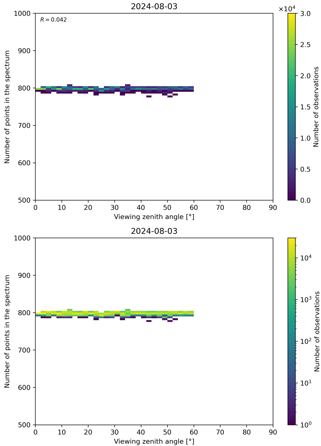
Figure 114: Scatter density plot of “Viewing zenith angle” against “Number of points in the spectrum” for 2024-08-02 to 2024-08-04.
