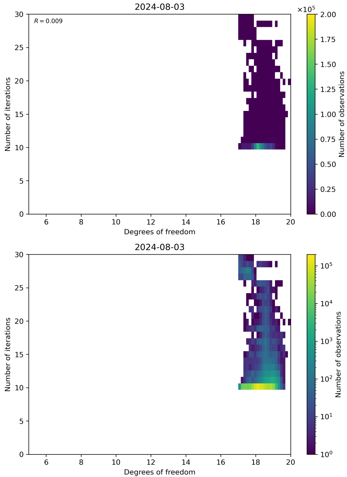
Figure 52: Scatter density plot of “Degrees of freedom” against “Number of iterations” for 2024-08-02 to 2024-08-04.
