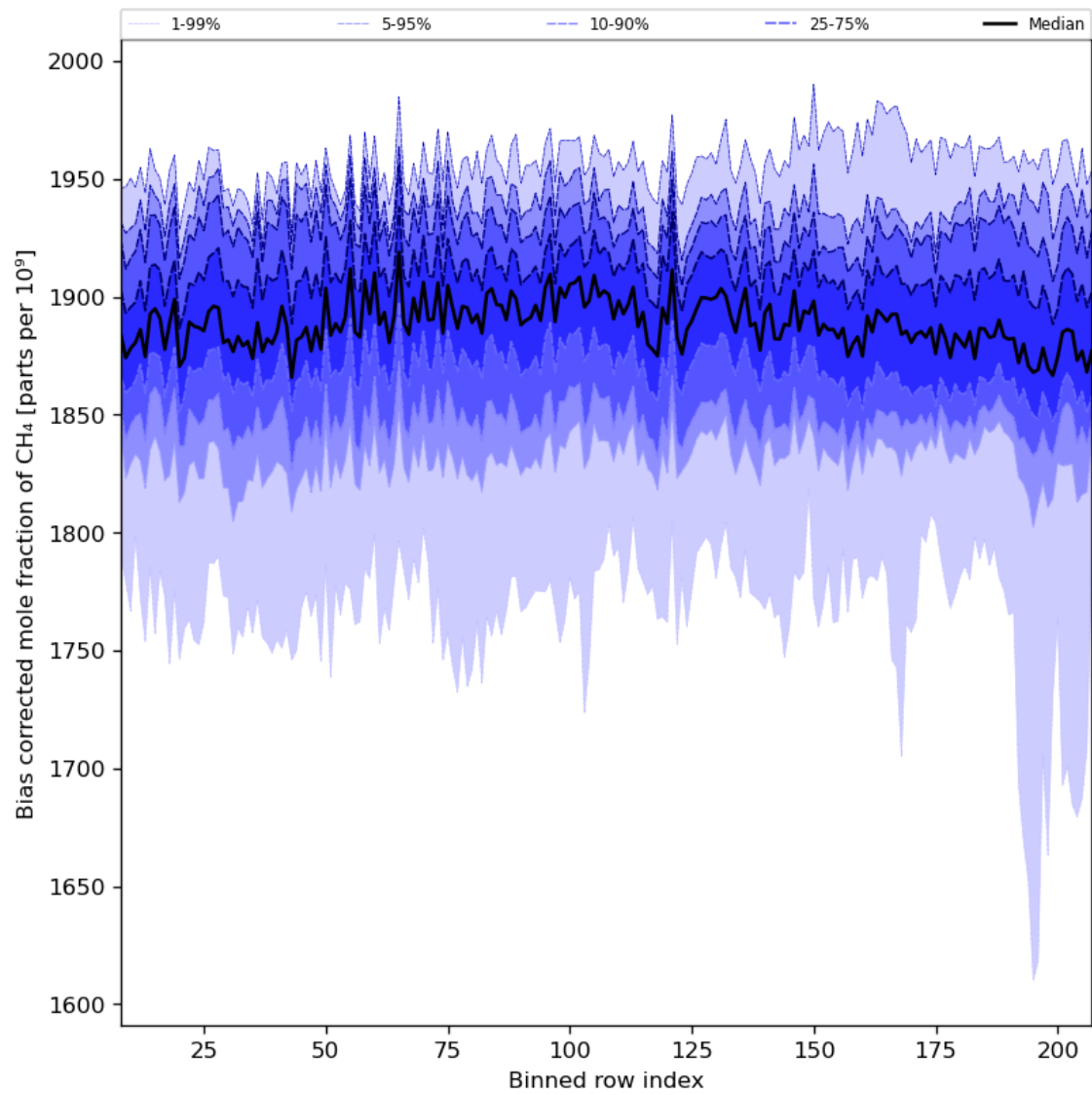
Figure 36: Along track statistics of “Bias corrected mole fraction of CH 4 ” for 2024-08-02 to 2024-08-04
