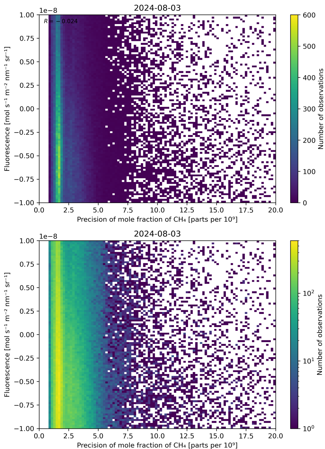
Figure 81: Scatter density plot of “Precision of mole fraction of \text{CH}_4 ” against “Fluorescence” for 2024-08-02 to 2024-08-04.
