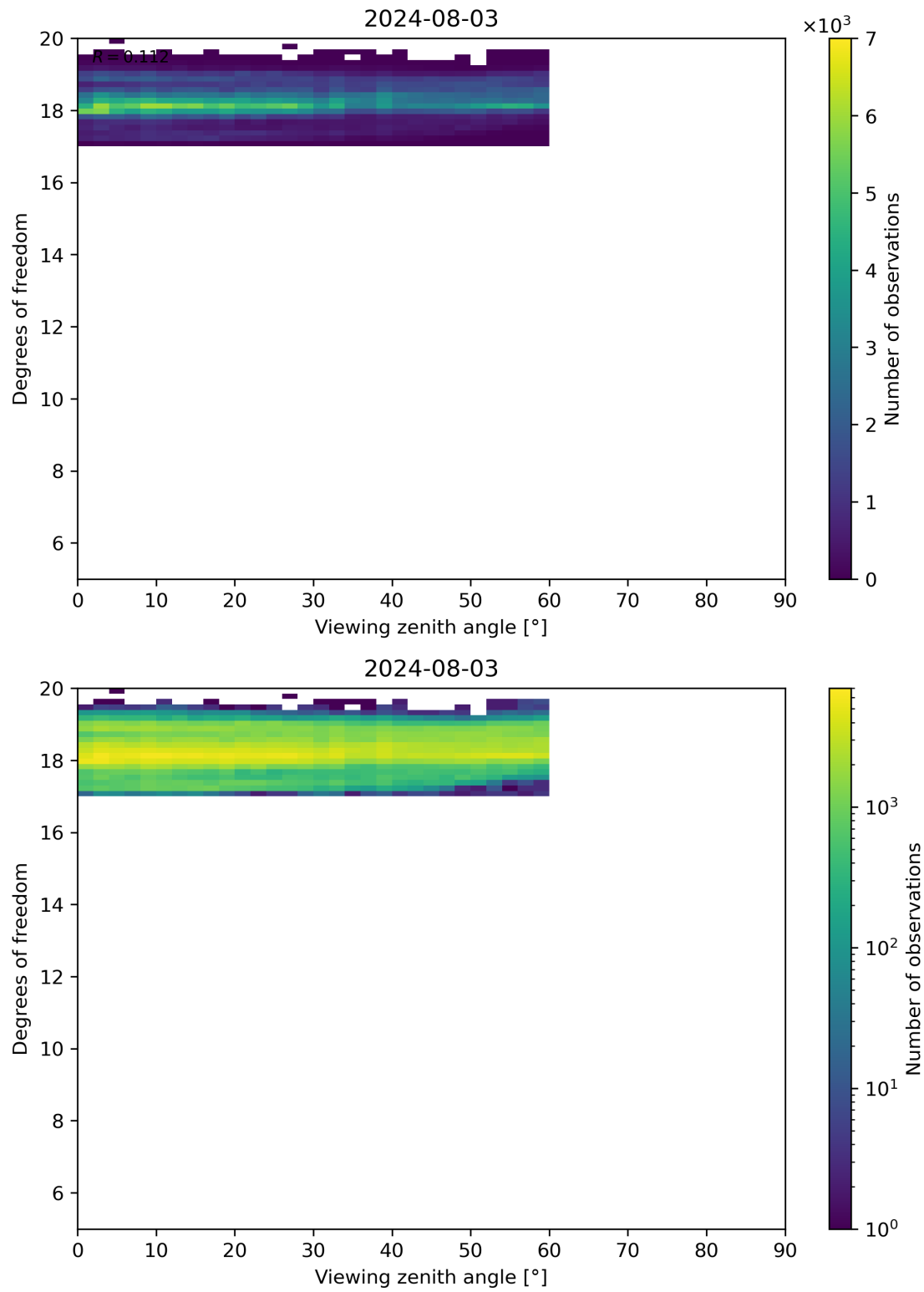
Figure 107: Scatter density plot of “Viewing zenith angle” against “Degrees of freedom” for 2024-08-02 to 2024-08-04.
