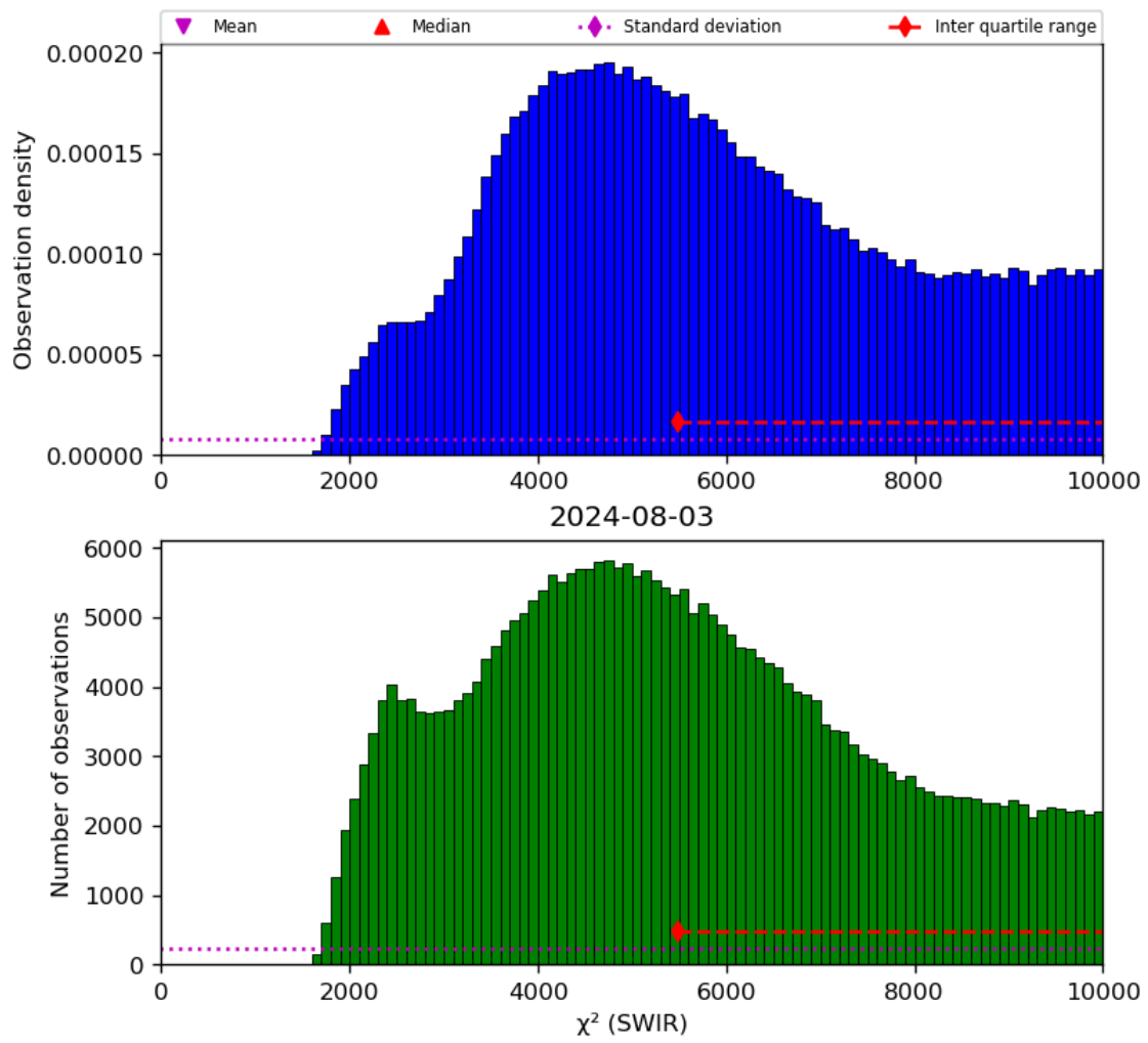
Figure 28: Histogram of “ \chi^2 (SWIR)” for 2024-08-02 to 2024-08-04
