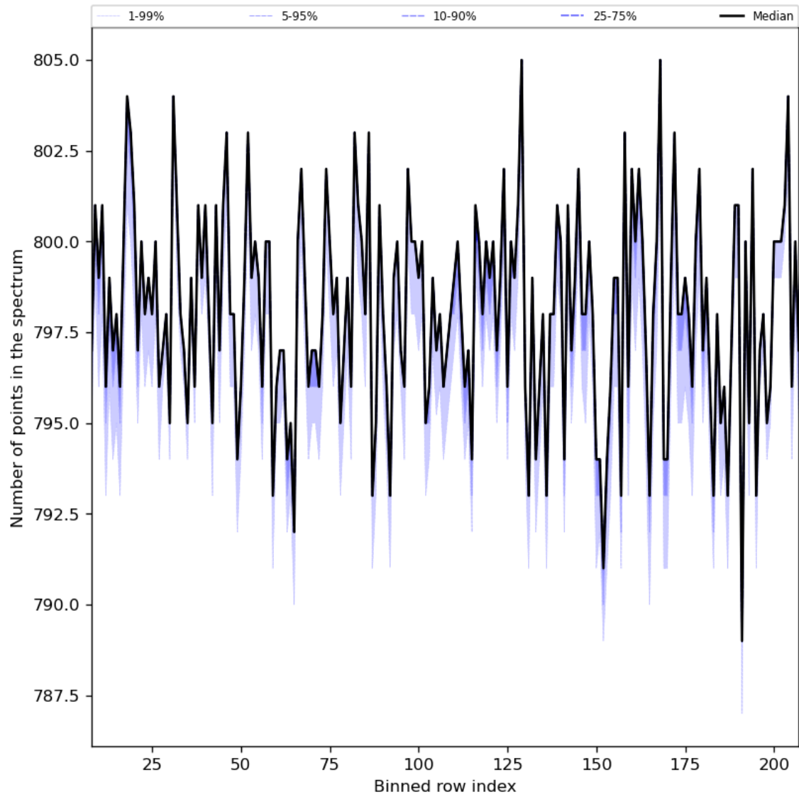
Figure 37: Along track statistics of “Number of points in the spectrum” for 2024-08-02 to 2024-08-04
