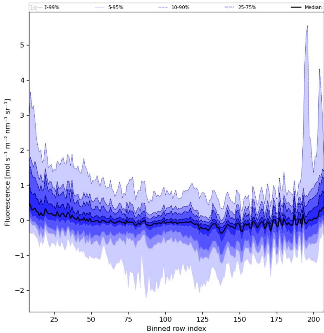
Figure 43: Along track statistics of "Fluorescence" for 2024-08-02 to 2024-08-04
