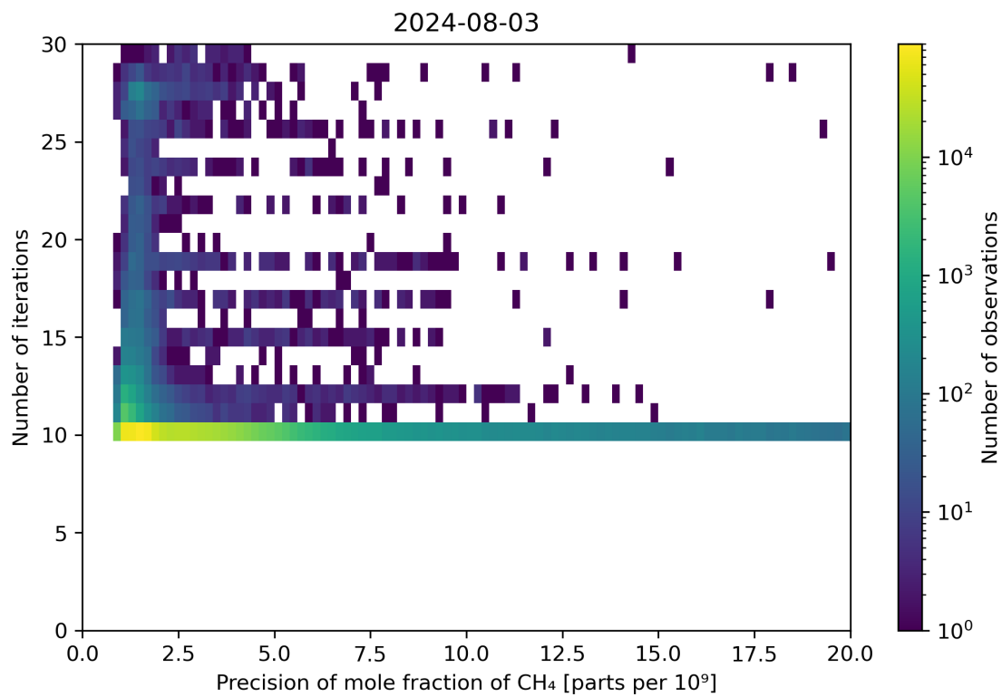
Figure 83: Scatter density plot of “Precision of mole fraction of CH 4 ” against “Number of iterations” for 2024-08-02 to 2024-08-04.
