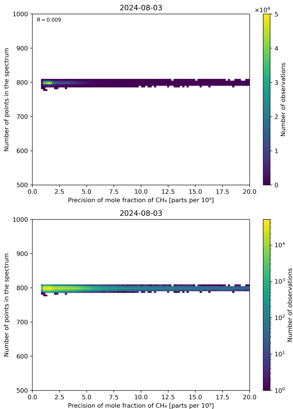
Figure 84: Scatter density plot of “Precision of mole fraction of CH 4 ” against “Number of points in the spectrum” for 2024-08-02 to 2024-08-04.
