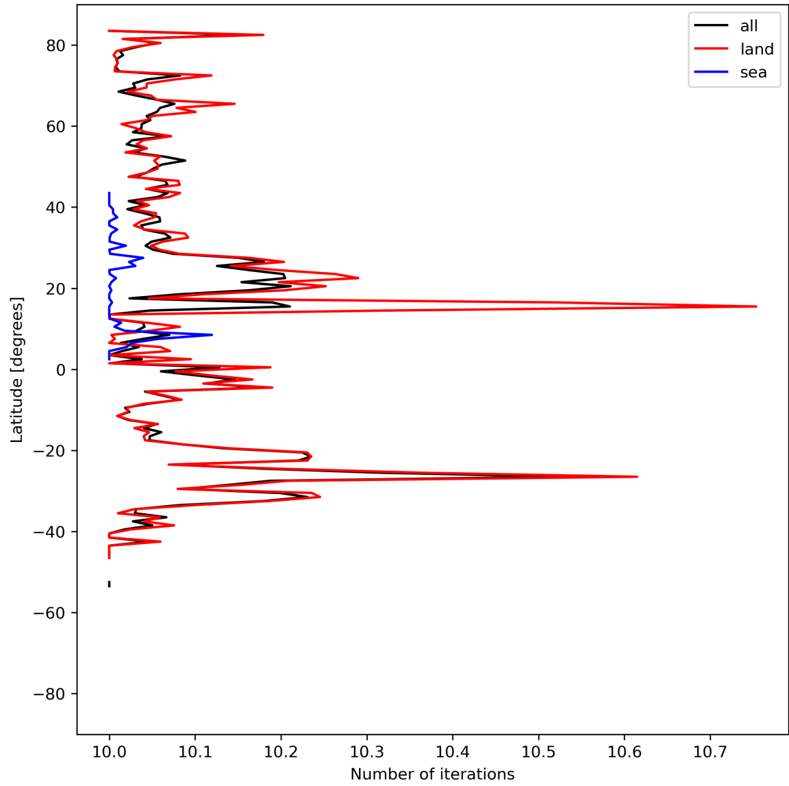
Figure 20: Zonal average of “Number of iterations” for 2024-08-02 to 2024-08-04.
