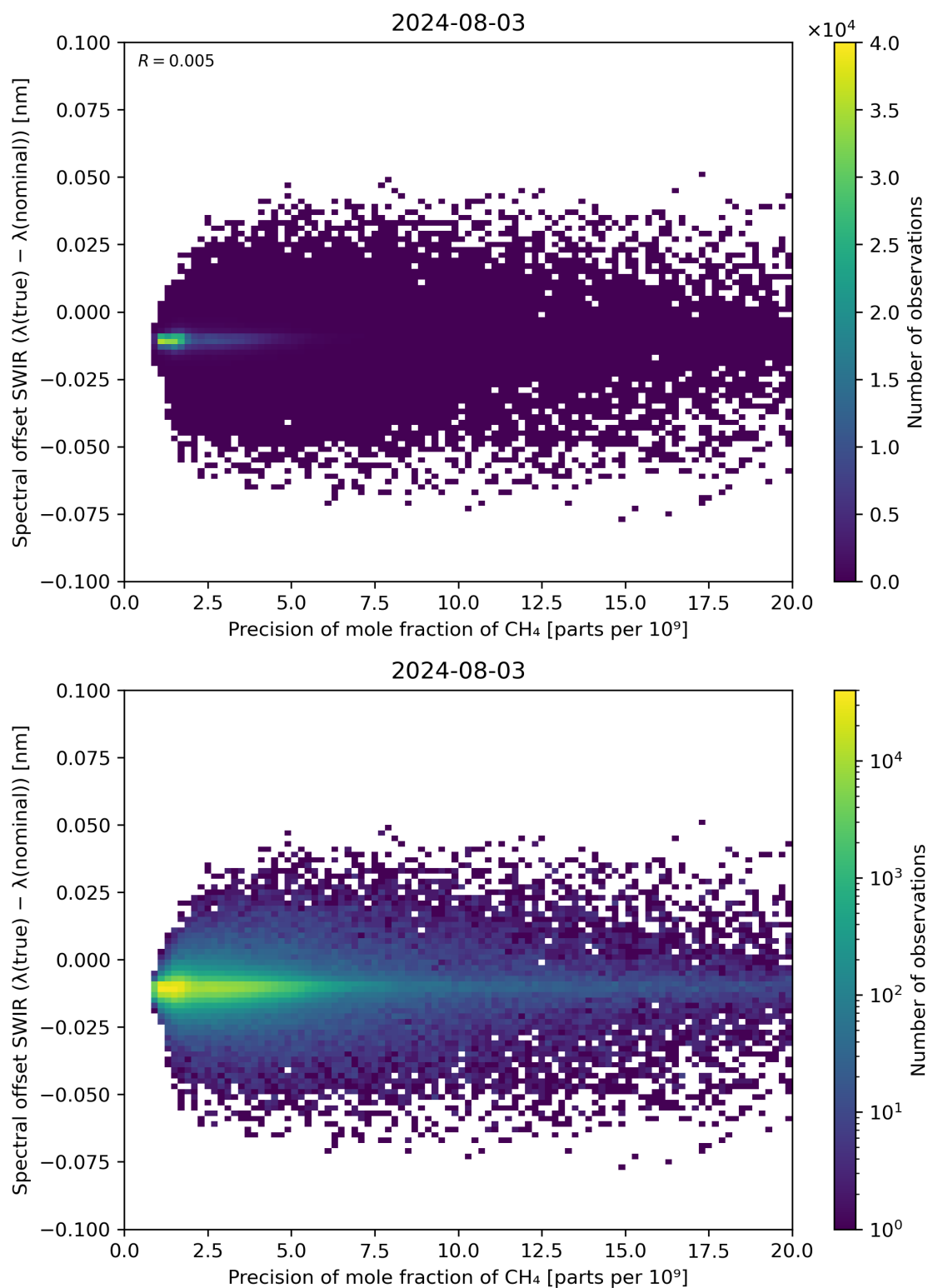
Figure 85: Scatter density plot of “Precision of mole fraction of CH 4 ” against “Spectral offset SWIR ( \lambda(\text{true}) - \lambda(\text{nominal}) )” for 2024-08-02 to 2024-08-04.
