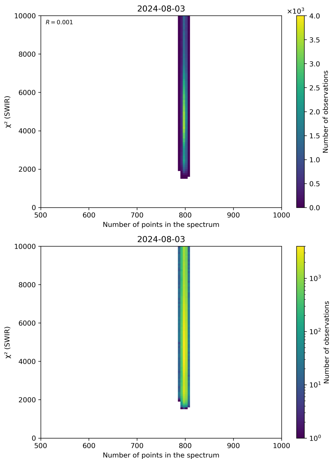
Figure 89: Scatter density plot of “Number of points in the spectrum” against “ \chi^2 (SWIR)” for 2024-08-02 to 2024-08-04.
