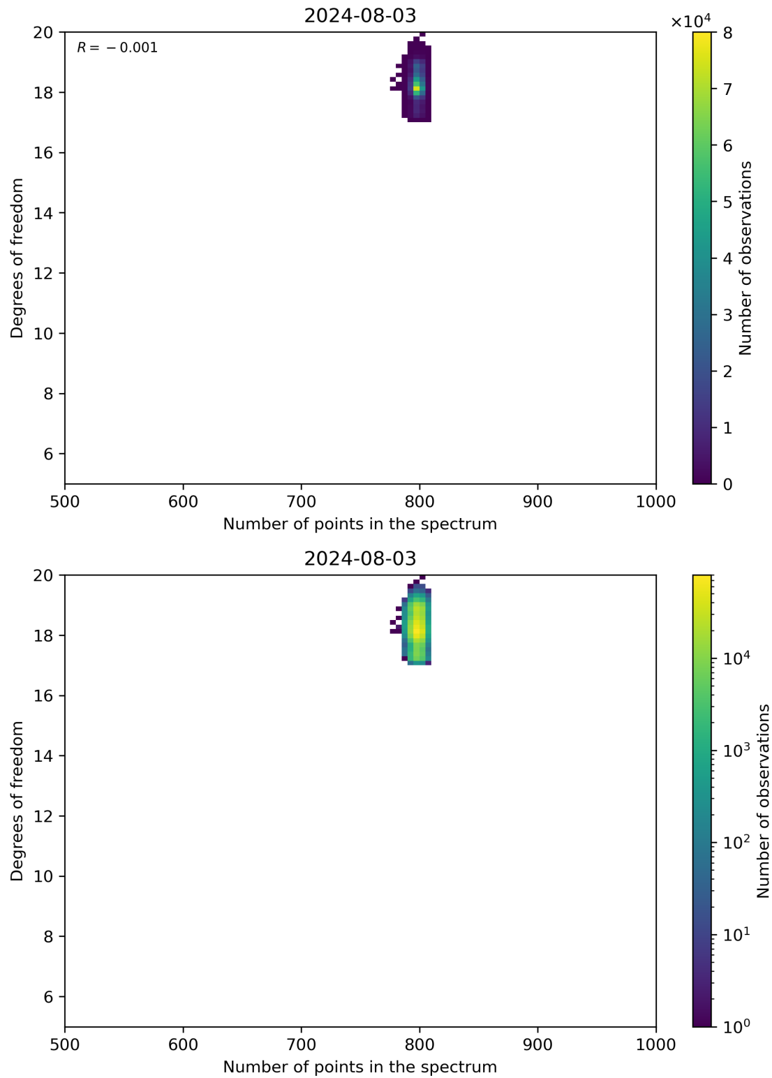
Figure 90: Scatter density plot of “Number of points in the spectrum” against “Degrees of freedom” for 2024-08-02 to 2024-08-04.
