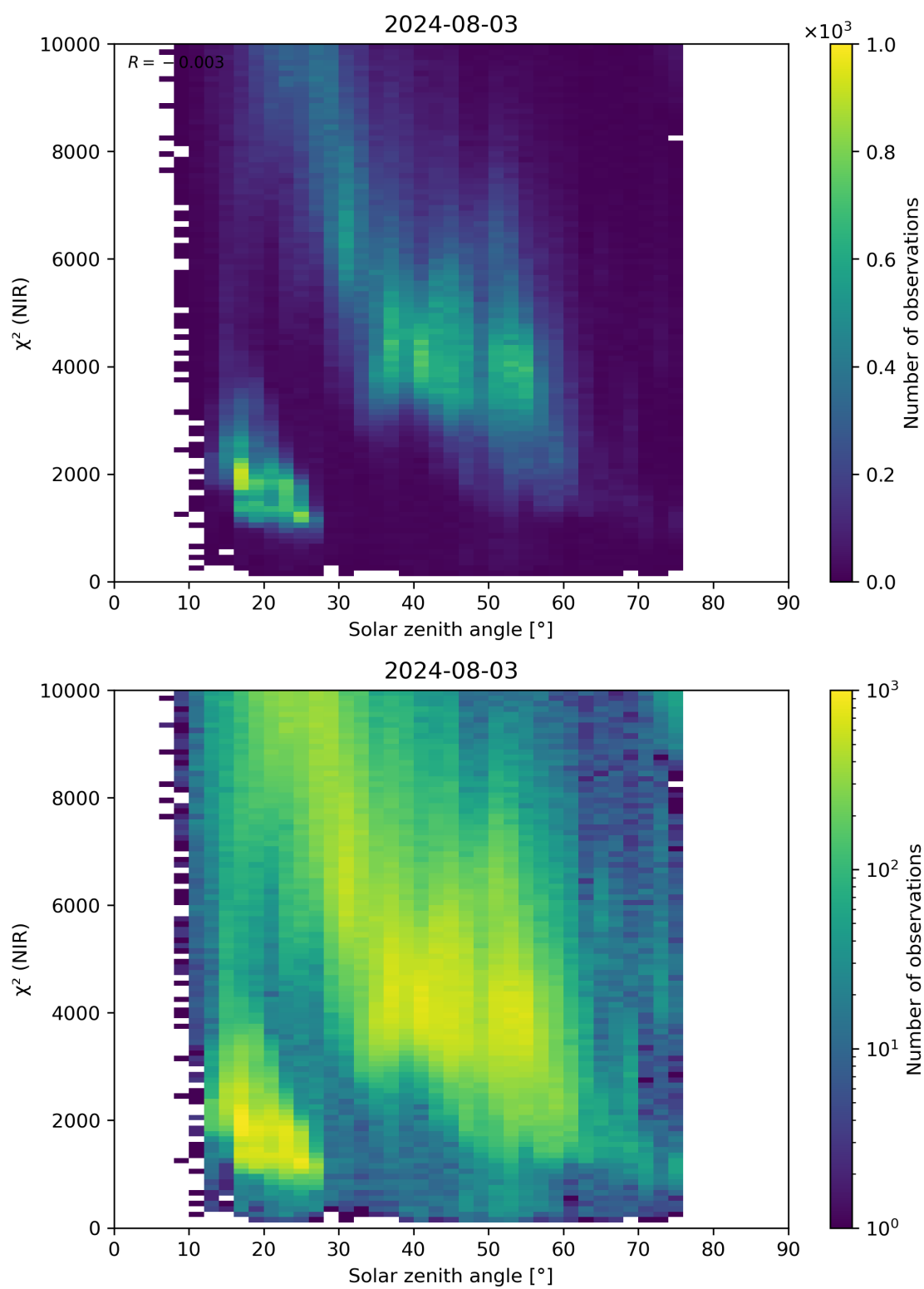
Figure 94: Scatter density plot of “Solar zenith angle” against “ \chi^2 (NIR)” for 2024-08-02 to 2024-08-04.
