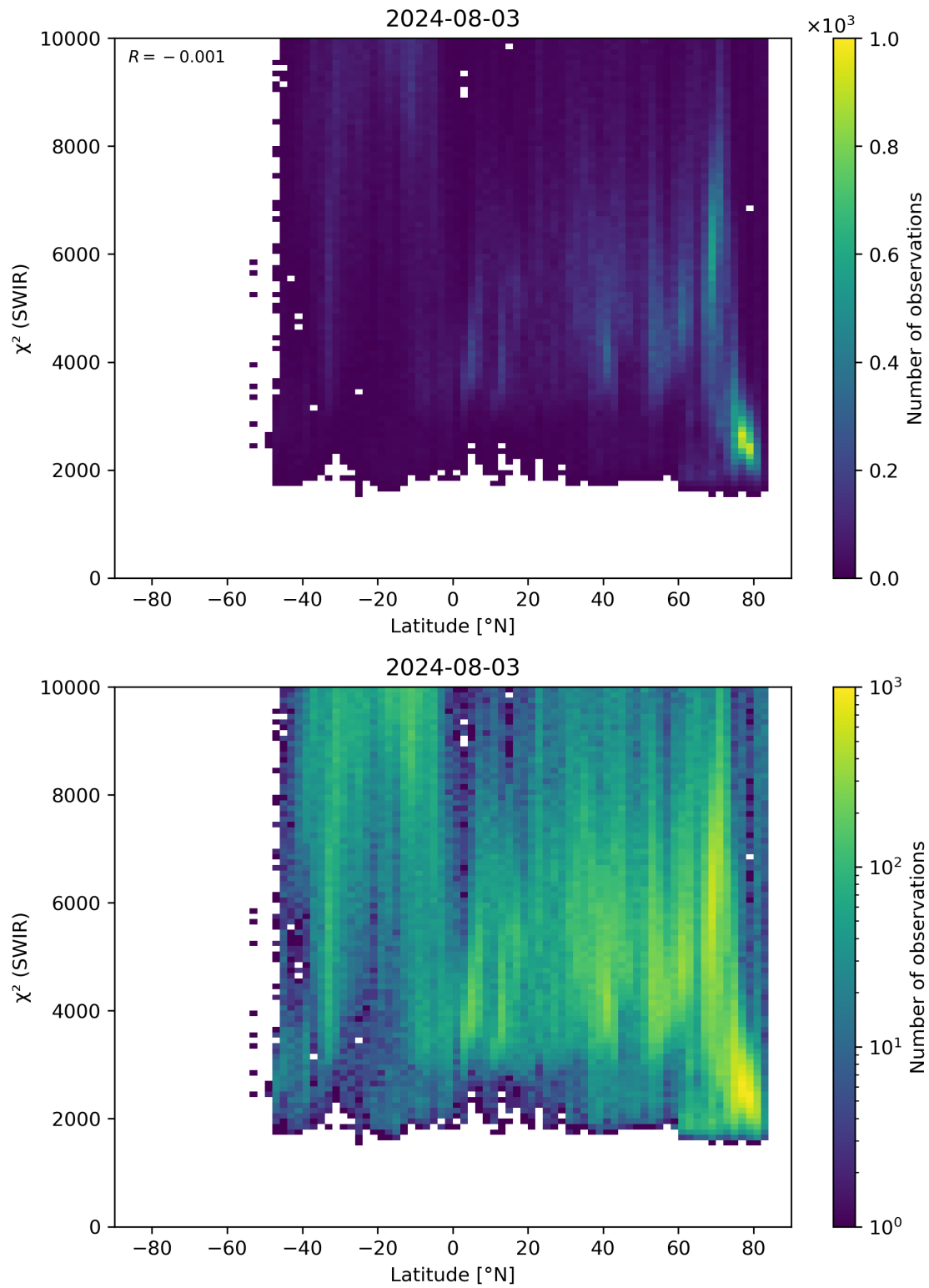
Figure 54: Scatter density plot of “Latitude” against “ \chi^2 (SWIR)” for 2024-08-02 to 2024-08-04.
