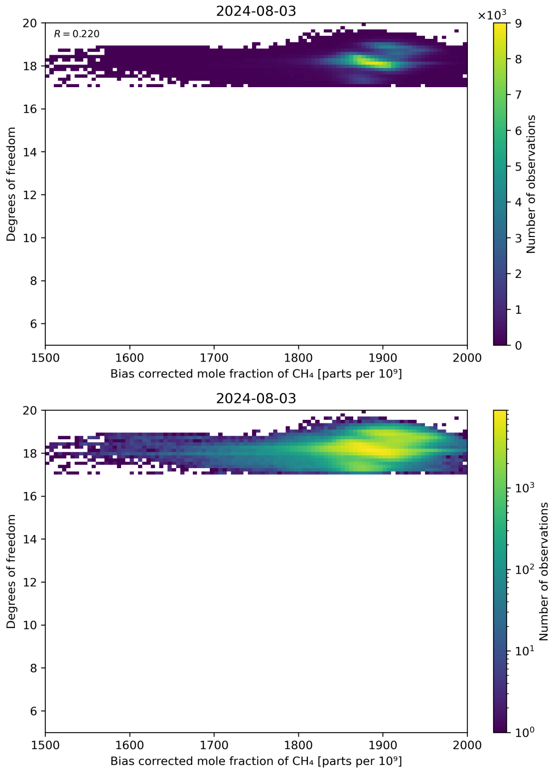
Figure 65: Scatter density plot of “Bias corrected mole fraction of CH 4 ” against “Degrees of freedom” for 2024-08-02 to 2024-08-04.
