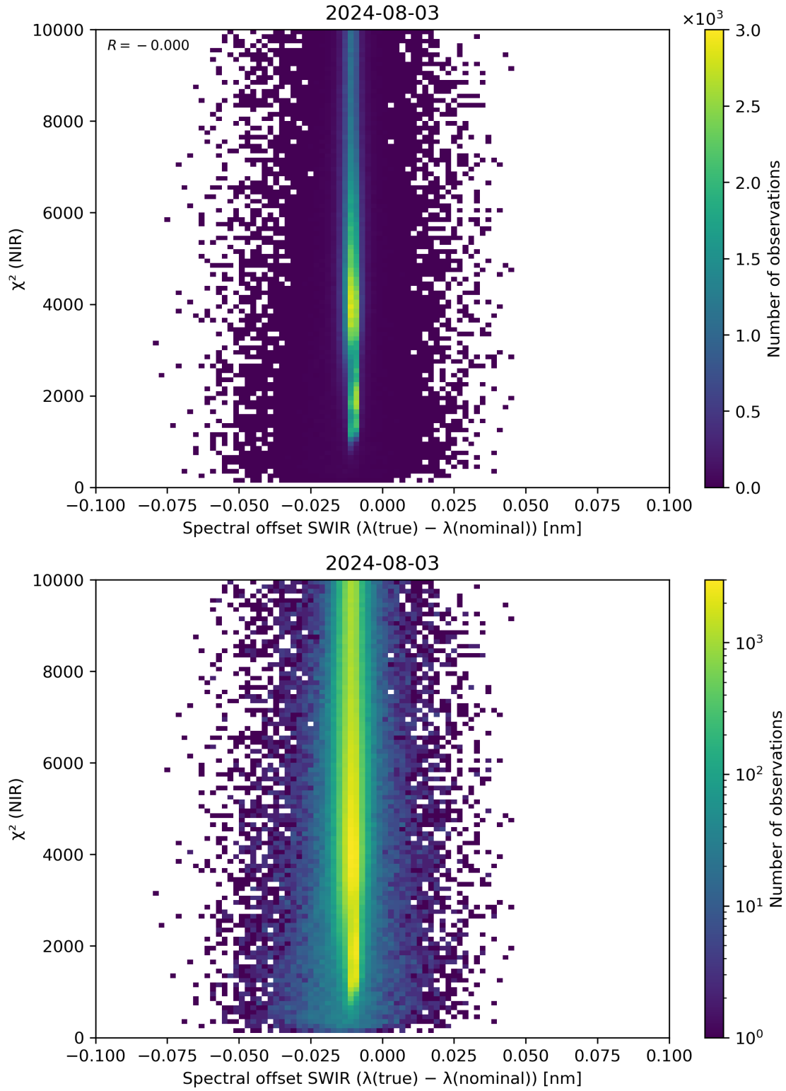
Figure 117: Scatter density plot of “Spectral offset SWIR ( \lambda(\text{true}) - \lambda(\text{nominal}) )” against “ \chi^2 (NIR)” for 2024-08-02 to 2024-08-04.
