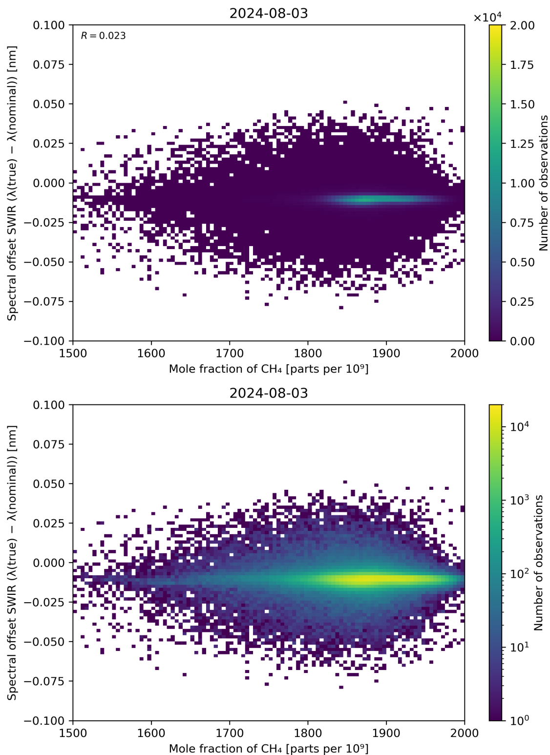
Figure 86: Scatter density plot of “Mole fraction of CH 4 ” against “Spectral offset SWIR ( \lambda(\text{true}) - \lambda(\text{nominal}) )” for 2024-08-02 to 2024-08-04.
