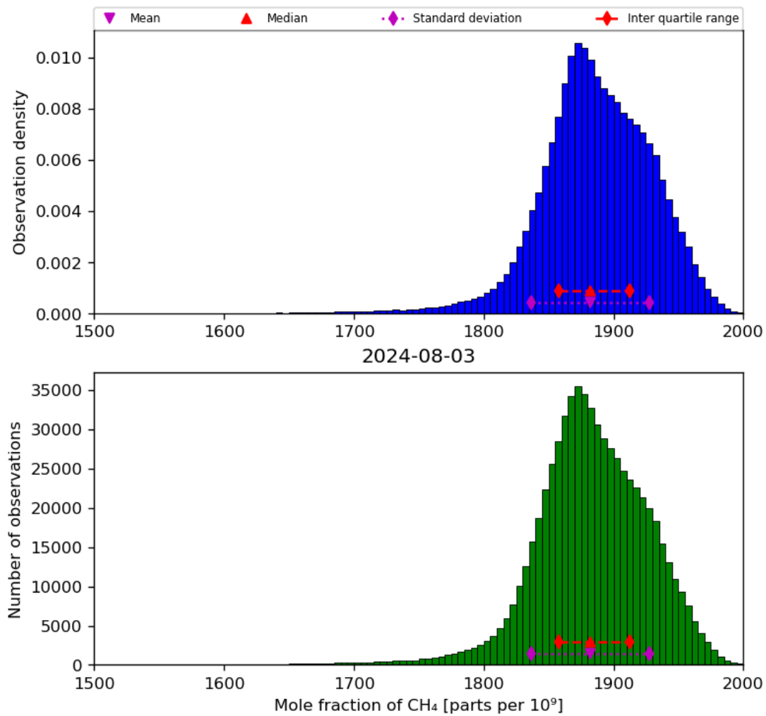
Figure 23: Histogram of “Mole fraction of CH 4 ” for 2024-08-02 to 2024-08-04
