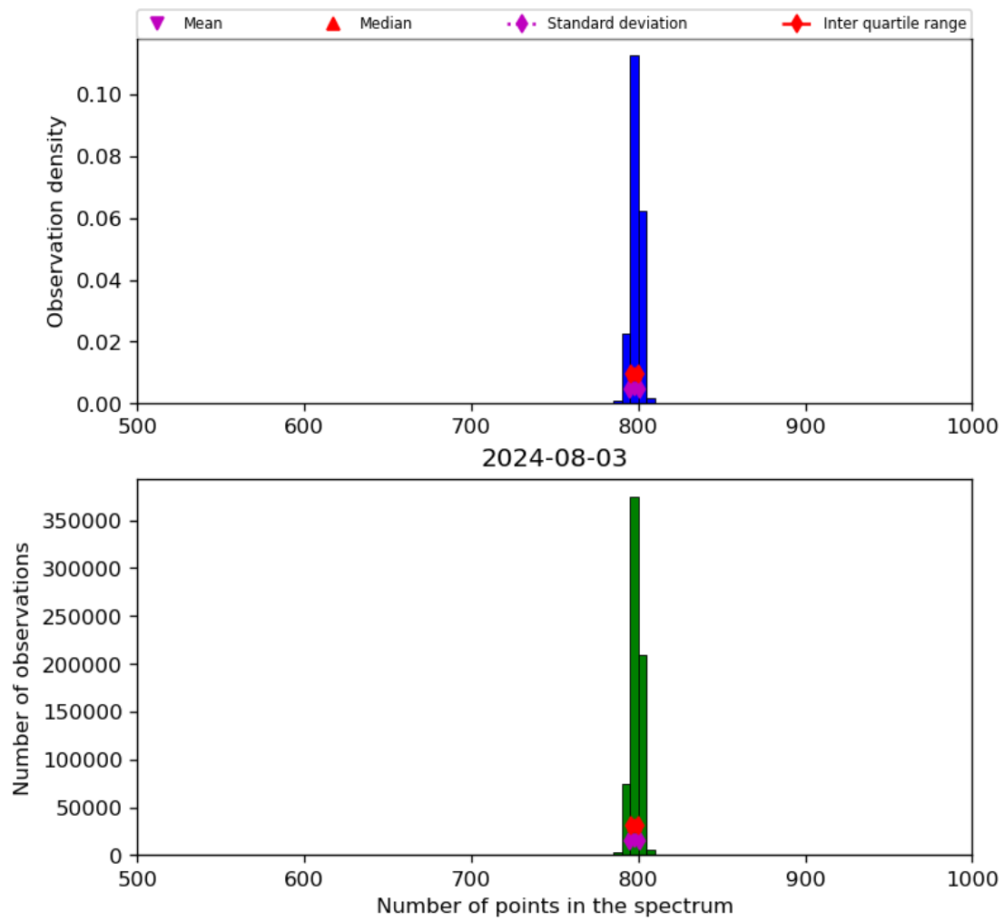
Figure 26: Histogram of “Number of points in the spectrum” for 2024-08-02 to 2024-08-04
