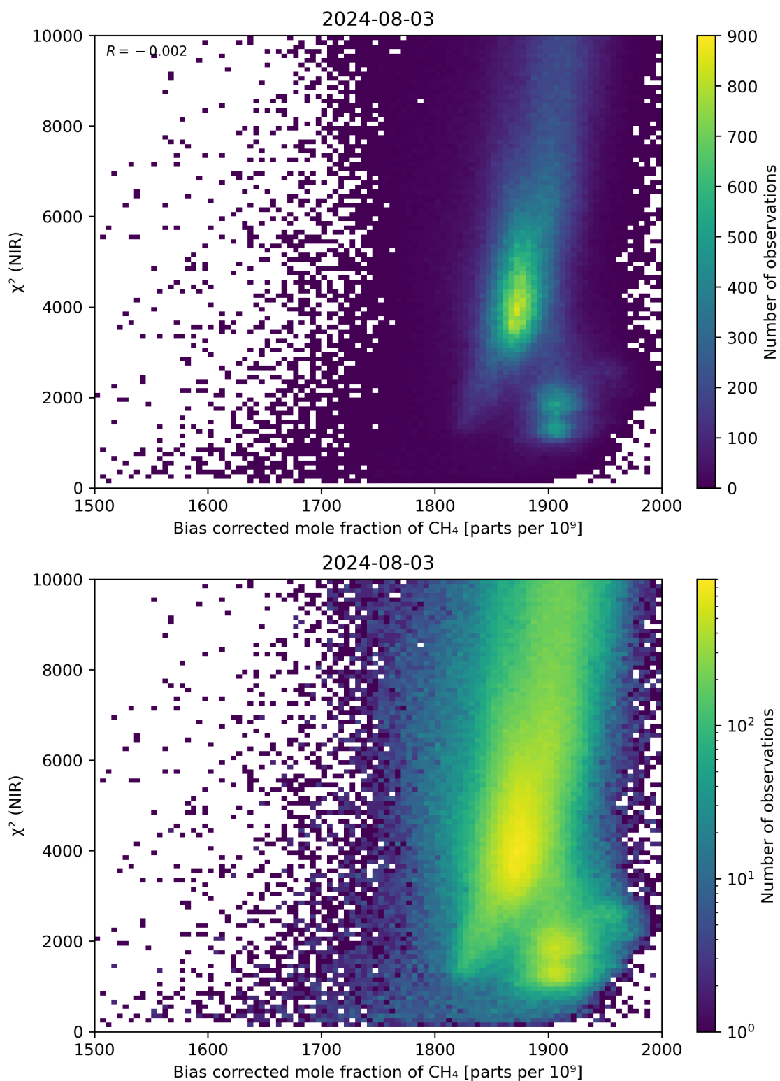
Figure 63: Scatter density plot of “Bias corrected mole fraction of \text{CH}_4 ” against “ \chi^2 (NIR)” for 2024-08-02 to 2024-08-04.
