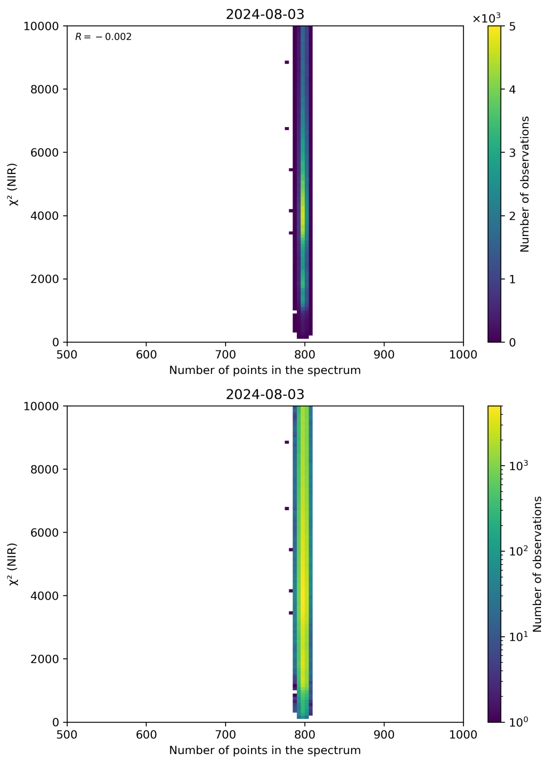
Figure 88: Scatter density plot of “Number of points in the spectrum” against “ \chi^2 (NIR)” for 2024-08-02 to 2024-08-04.
