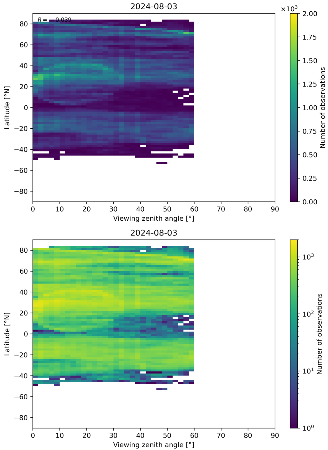
Figure 109: Scatter density plot of “Viewing zenith angle” against “Latitude” for 2024-08-02 to 2024-08-04.
