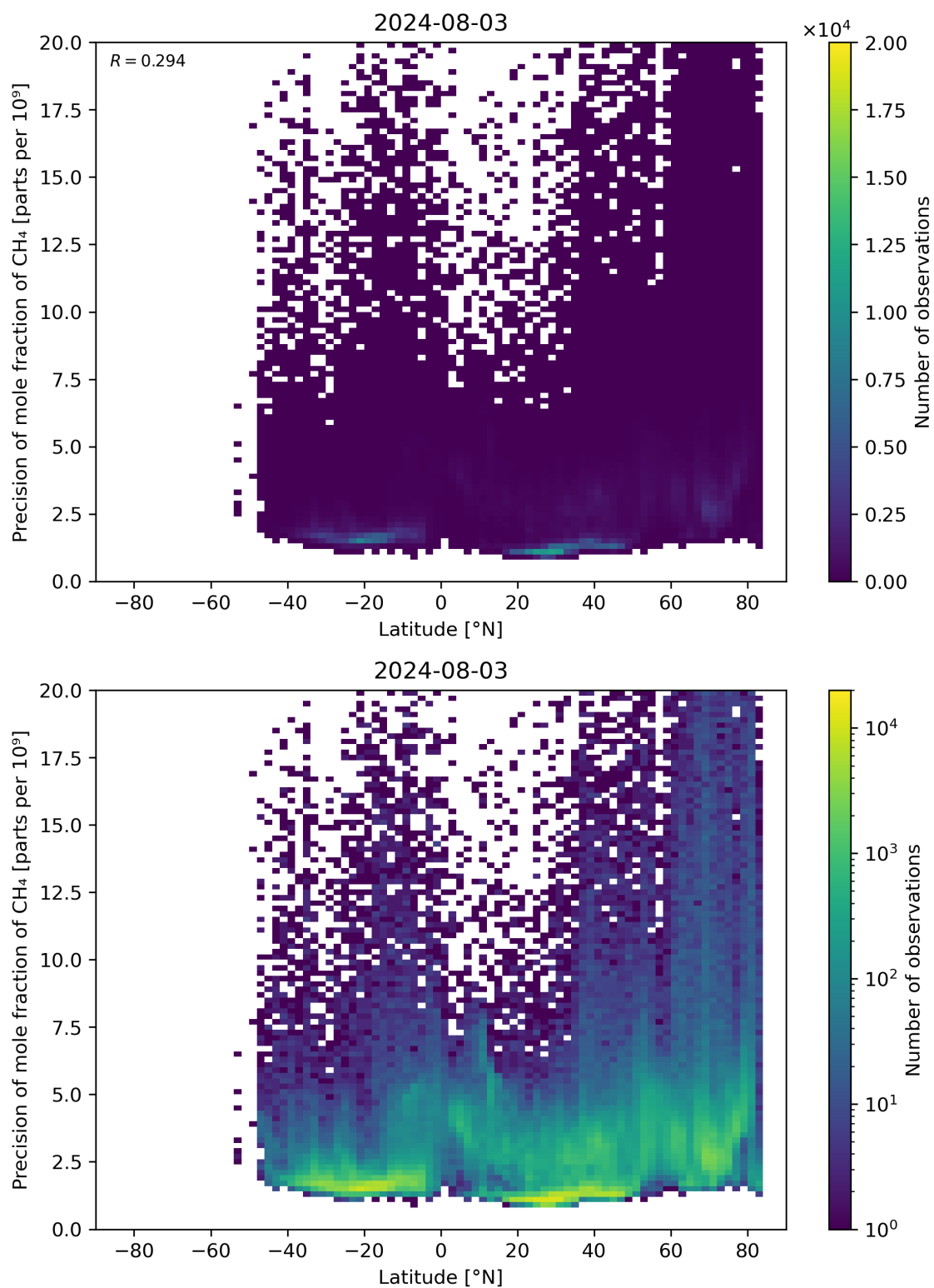
Figure 59: Scatter density plot of “Latitude” against “Precision of mole fraction of \text{CH}_4 ” for 2024-08-02 to 2024-08-04.
