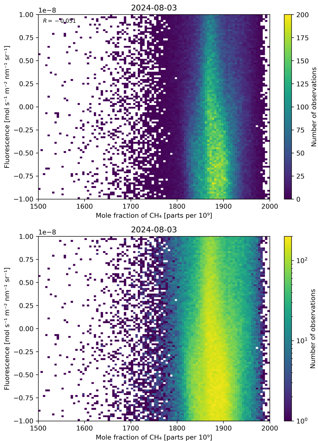
Figure 73: Scatter density plot of “Mole fraction of \text{CH}_4 ” against “Fluorescence” for 2024-08-02 to 2024-08-04.
