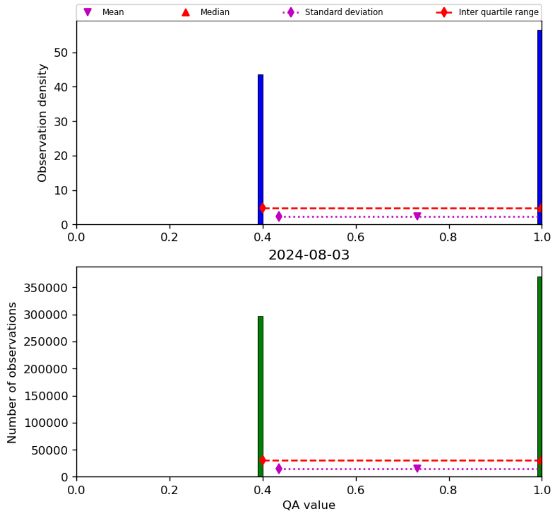
Figure 22: Histogram of “QA value” for 2024-08-02 to 2024-08-04
