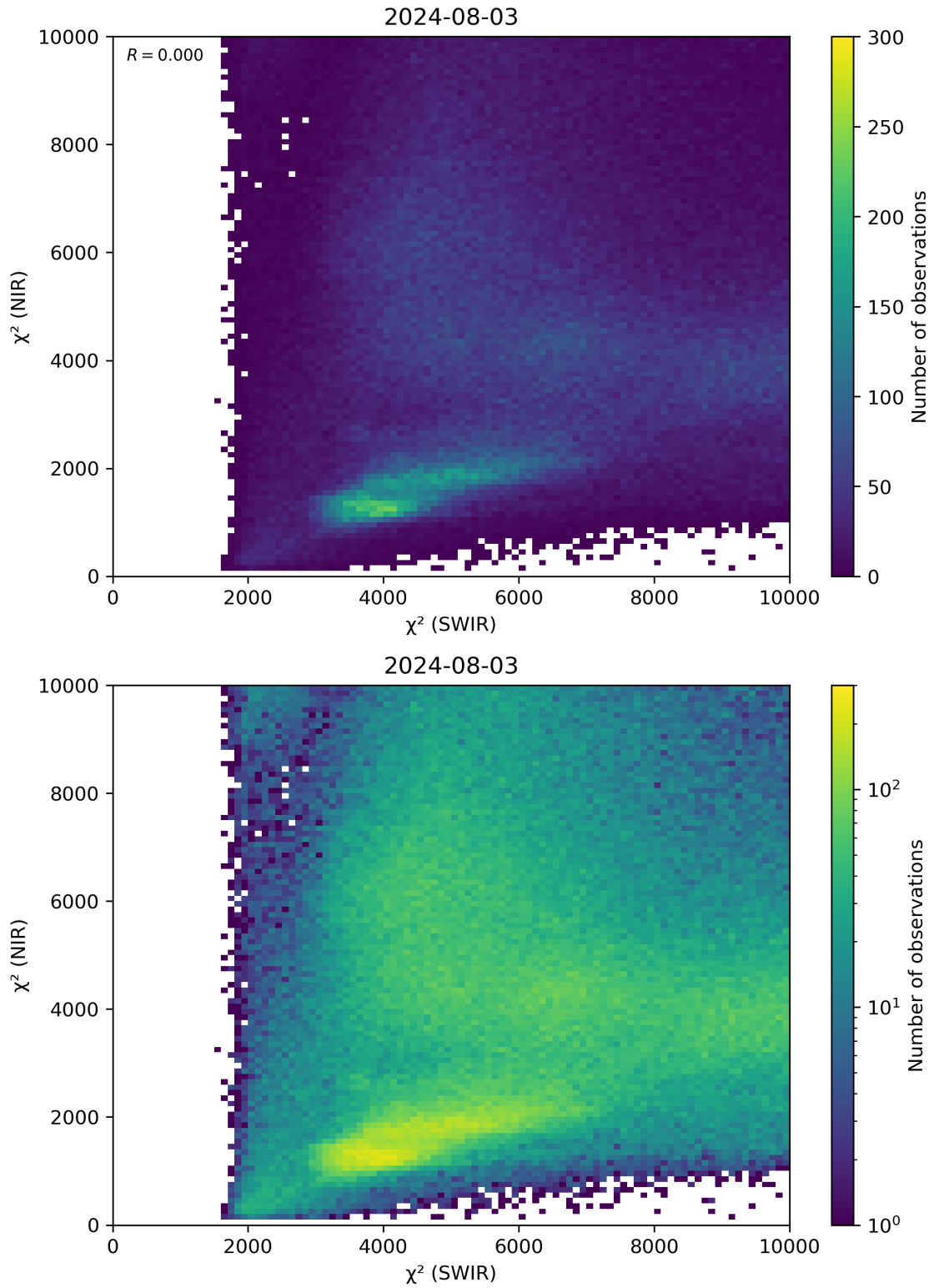
Figure 47: Scatter density plot of “ \chi^2 (SWIR)” against “ \chi^2 (NIR)” for 2024-08-02 to 2024-08-04.
