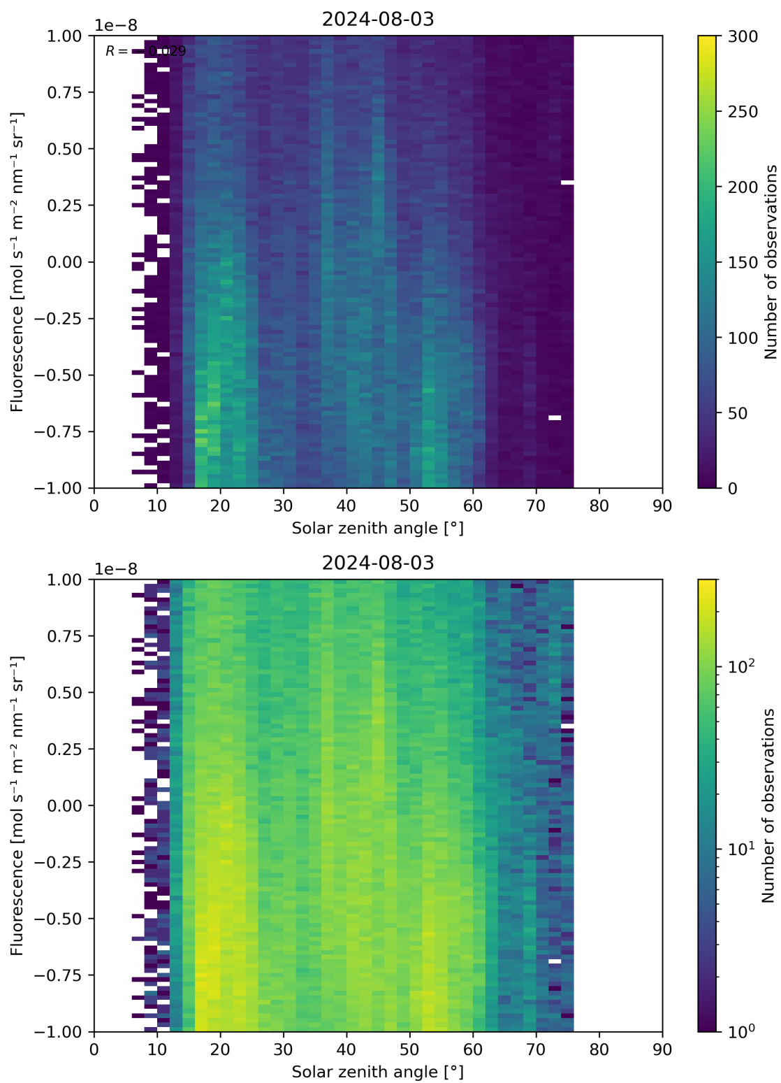
Figure 97: Scatter density plot of “Solar zenith angle” against “Fluorescence” for 2024-08-02 to 2024-08-04.
