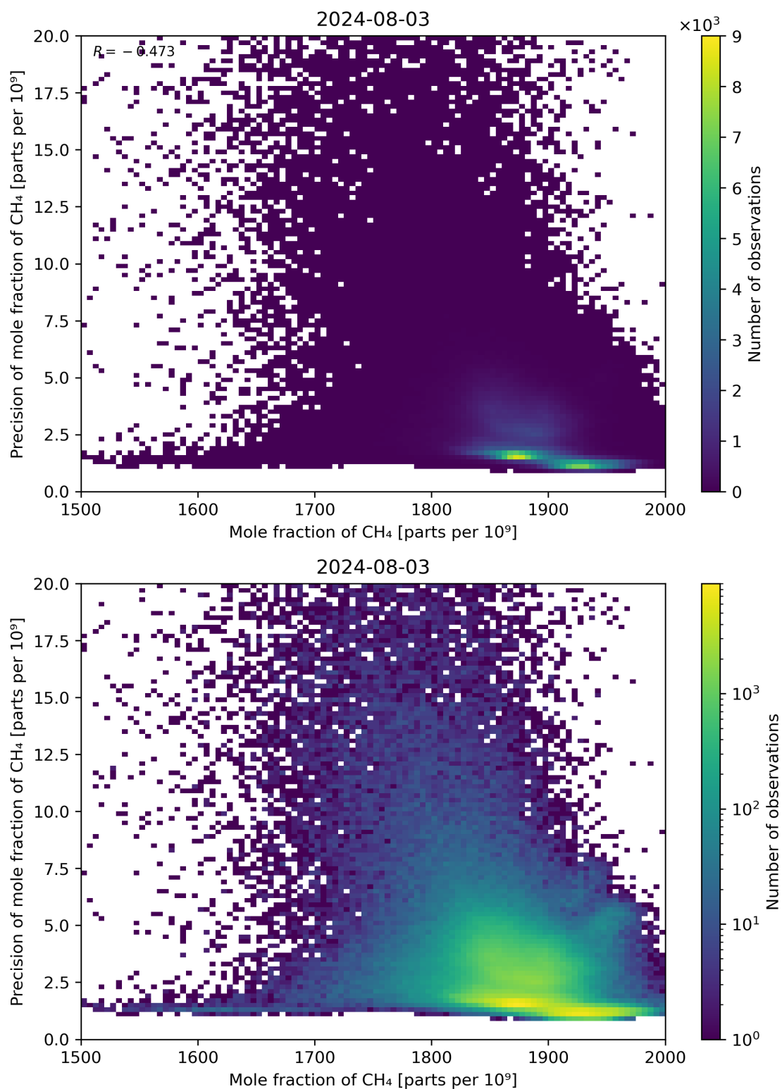
Figure 75: Scatter density plot of “Mole fraction of CH 4 ” against “Precision of mole fraction of CH 4 ” for 2024-08-02 to 2024-08-04.
