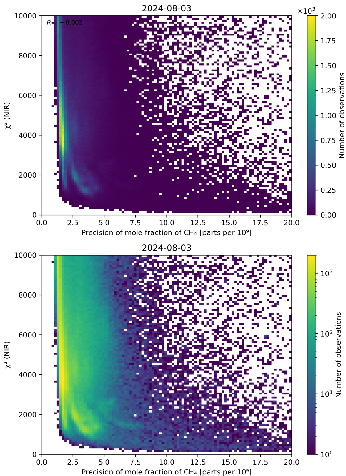
Figure 78: Scatter density plot of “Precision of mole fraction of \text{CH}_4 ” against “ \chi^2 (NIR)” for 2024-08-02 to 2024-08-04.
