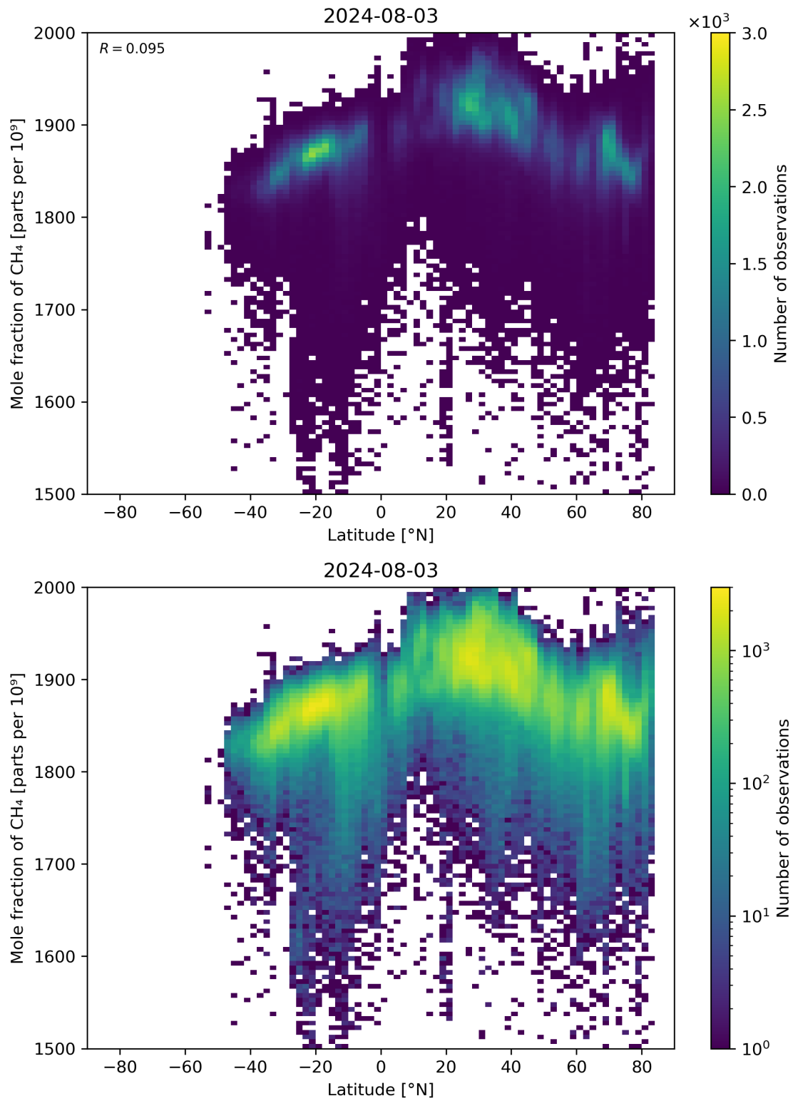
Figure 57: Scatter density plot of “Latitude” against “Mole fraction of CH 4 ” for 2024-08-02 to 2024-08-04.
