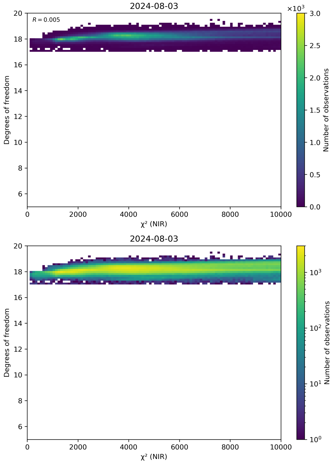
Figure 44: Scatter density plot of “ \chi^2 (NIR)” against “Degrees of freedom” for 2024-08-02 to 2024-08-04.
