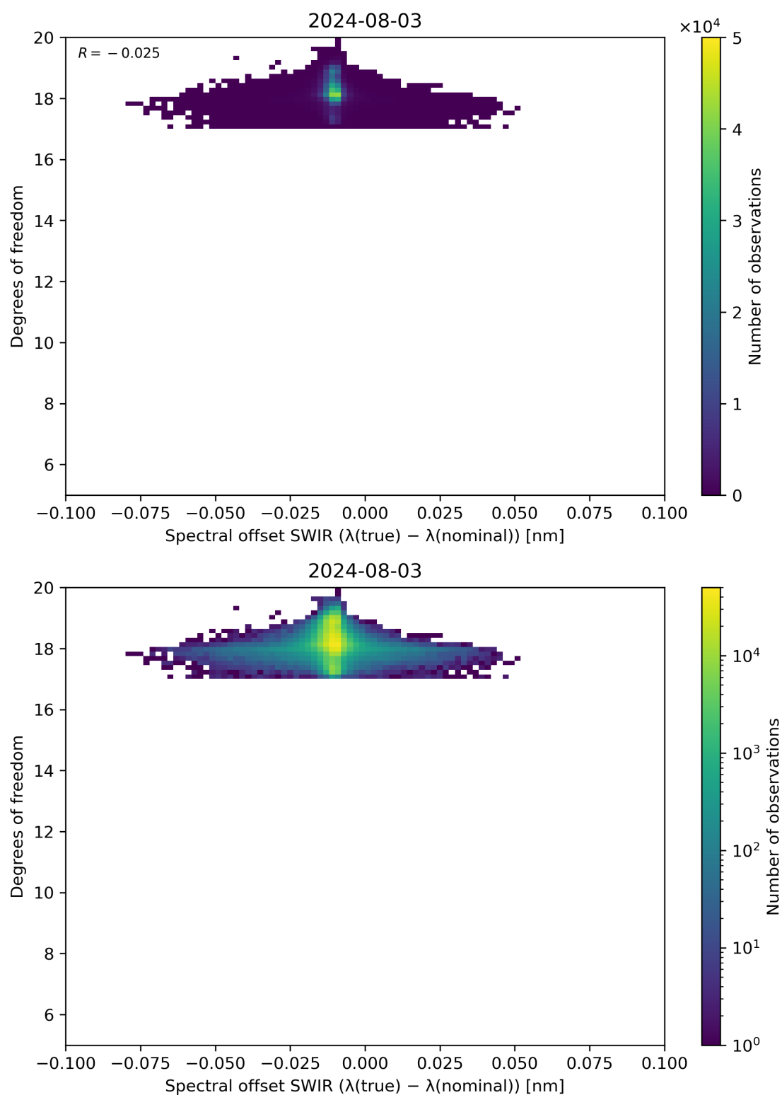
Figure 119: Scatter density plot of “Spectral offset SWIR ( \lambda(\text{true}) - \lambda(\text{nominal}) )” against “Degrees of freedom” for 2024-08-02 to 2024-08-04.
