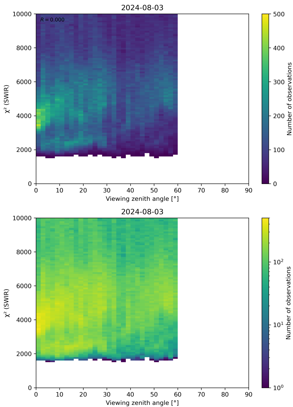
Figure 106: Scatter density plot of “Viewing zenith angle” against “ \chi^2 (SWIR)” for 2024-08-02 to 2024-08-04.
