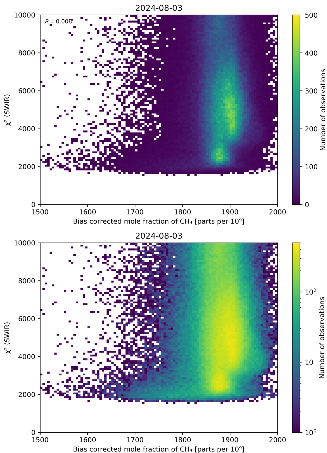
Figure 64: Scatter density plot of “Bias corrected mole fraction of CH 4 ” against “ \chi^2 (SWIR)” for 2024-08-02 to 2024-08-04.
