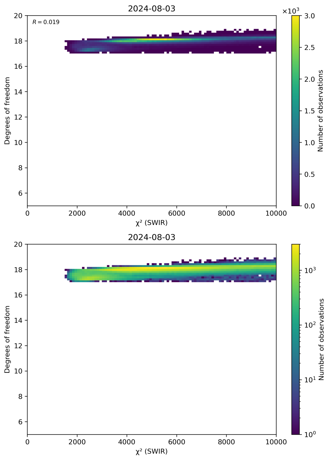
Figure 48: Scatter density plot of “ \chi^2 (SWIR)” against “Degrees of freedom” for 2024-08-02 to 2024-08-04.
