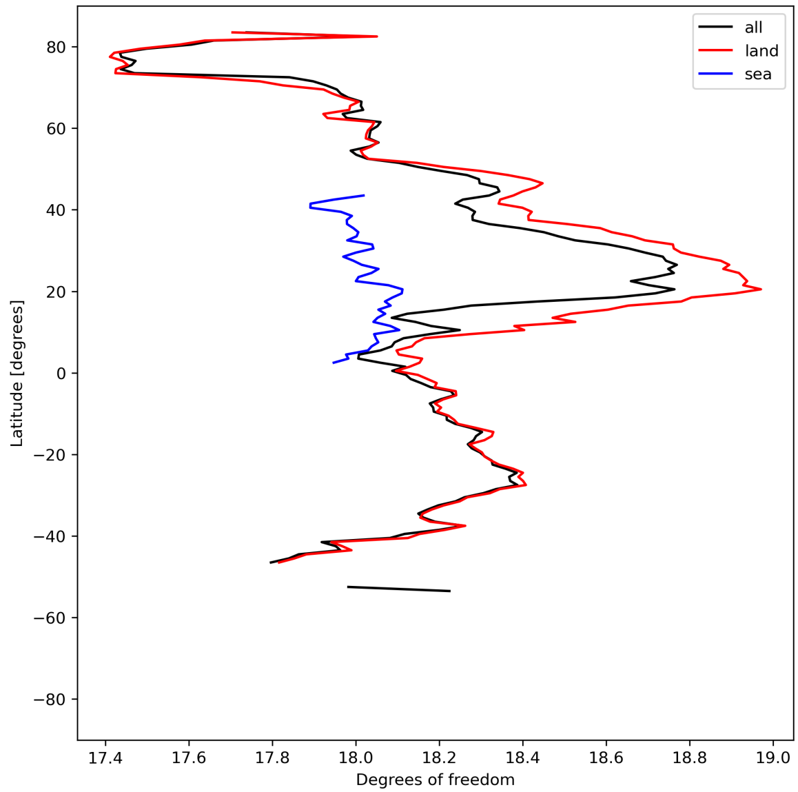
Figure 19: Zonal average of “Degrees of freedom” for 2024-08-02 to 2024-08-04.
