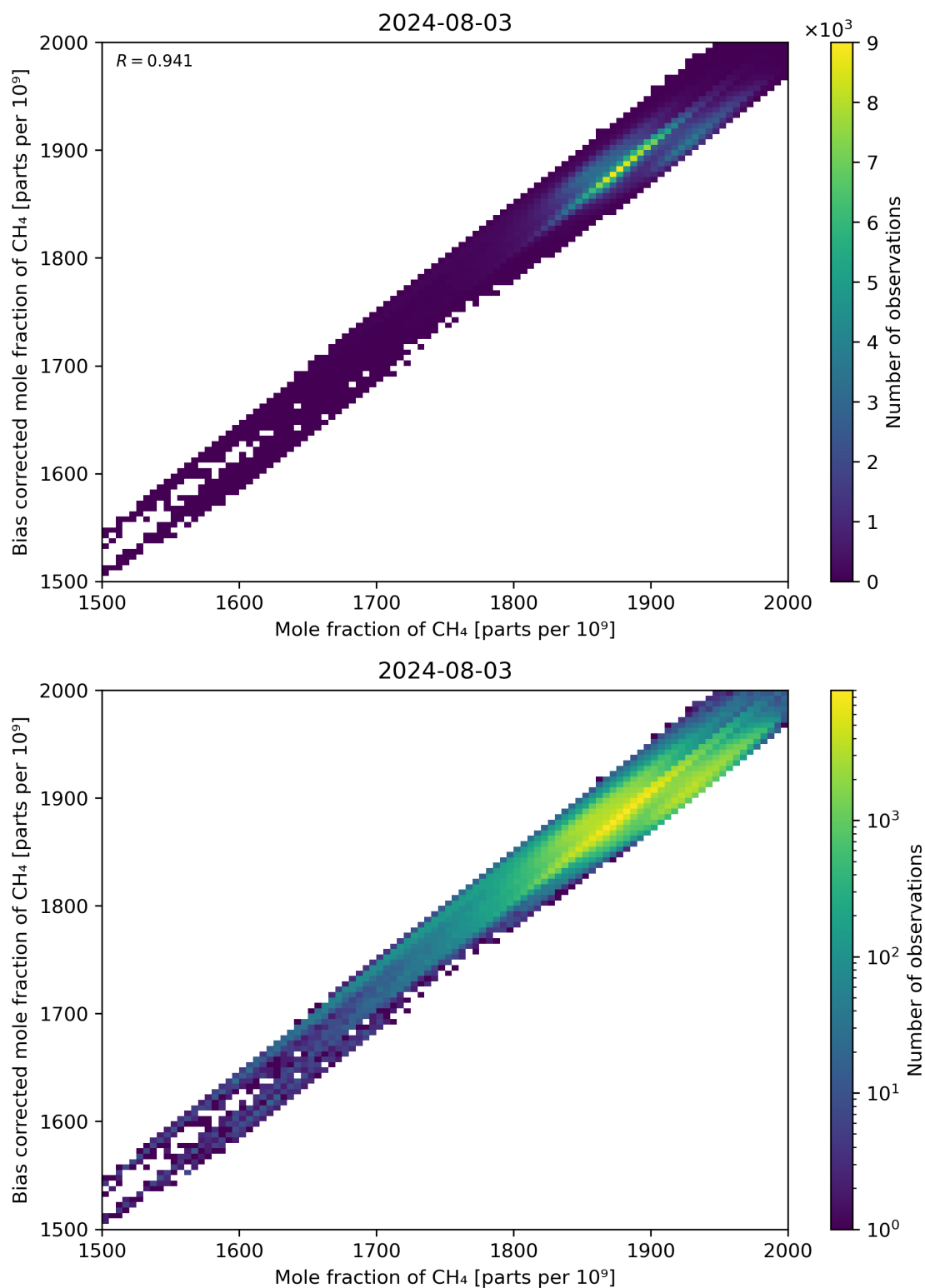
Figure 74: Scatter density plot of “Mole fraction of CH 4 ” against “Bias corrected mole fraction of CH 4 ” for 2024-08-02 to 2024-08-04.
