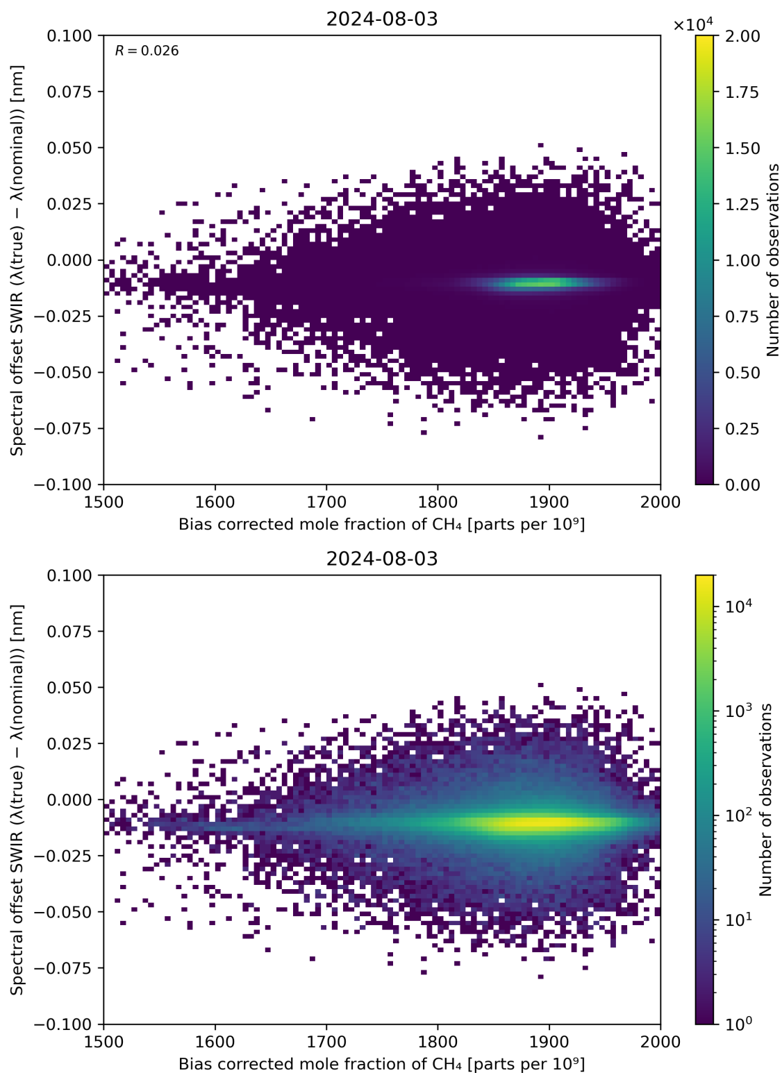
Figure 69: Scatter density plot of “Bias corrected mole fraction of \text{CH}_4 ” against “Spectral offset SWIR ( \lambda(\text{true}) - \lambda(\text{nominal}) )” for 2024-08-02 to 2024-08-04.
