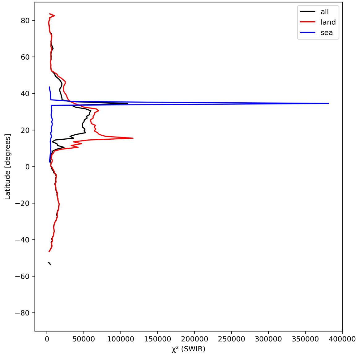
Figure 17: Zonal average of “ \chi^2 (SWIR)” for 2024-08-02 to 2024-08-04.
