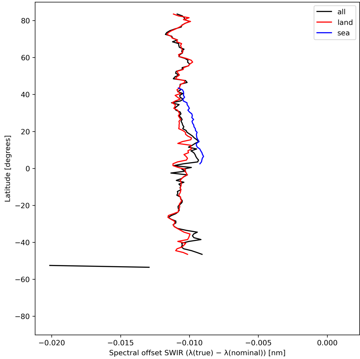
Figure 16: Zonal average of “Spectral offset SWIR ( \lambda(\text{true}) - \lambda(\text{nominal}) )” for 2024-08-02 to 2024-08-04.
