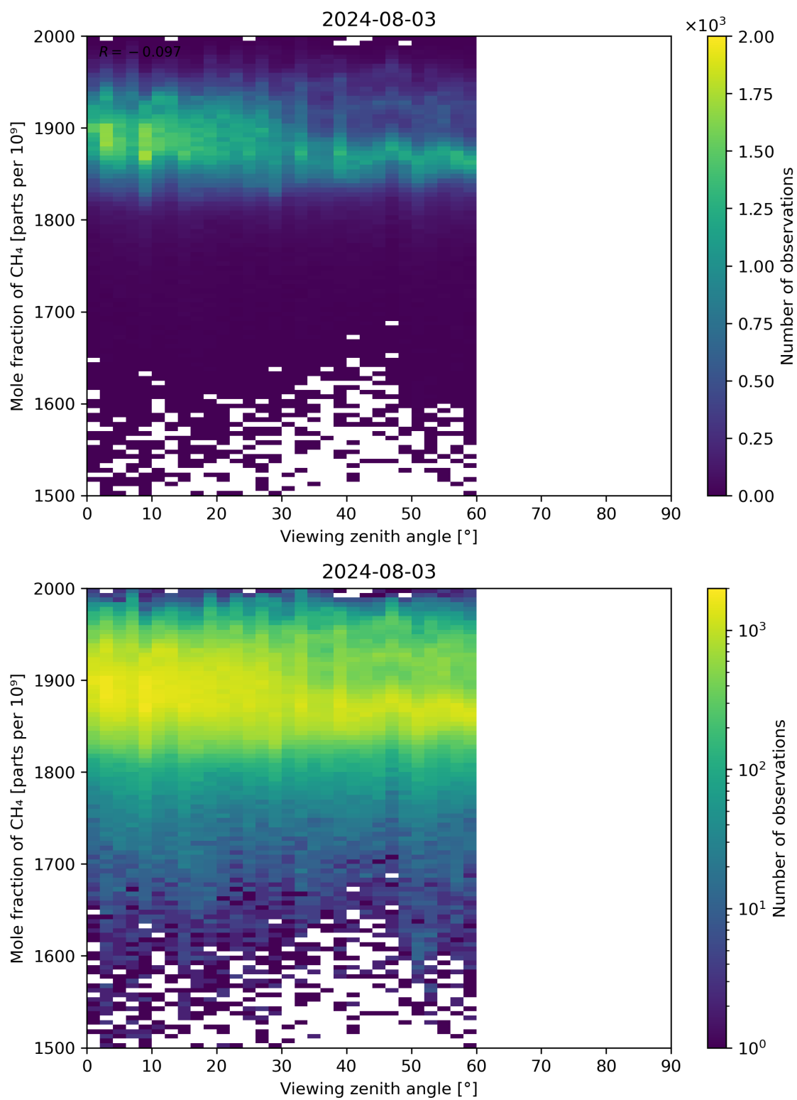
Figure 110: Scatter density plot of “Viewing zenith angle” against “Mole fraction of CH 4 ” for 2024-08-02 to 2024-08-04.
