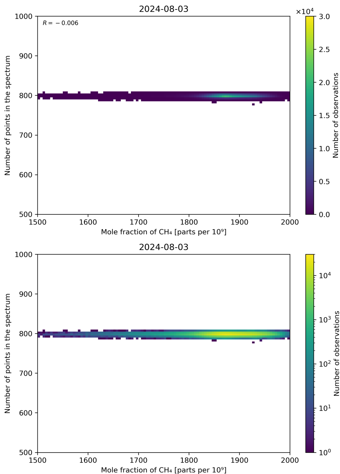
Figure 77: Scatter density plot of “Mole fraction of CH 4 ” against “Number of points in the spectrum” for 2024-08-02 to 2024-08-04.
