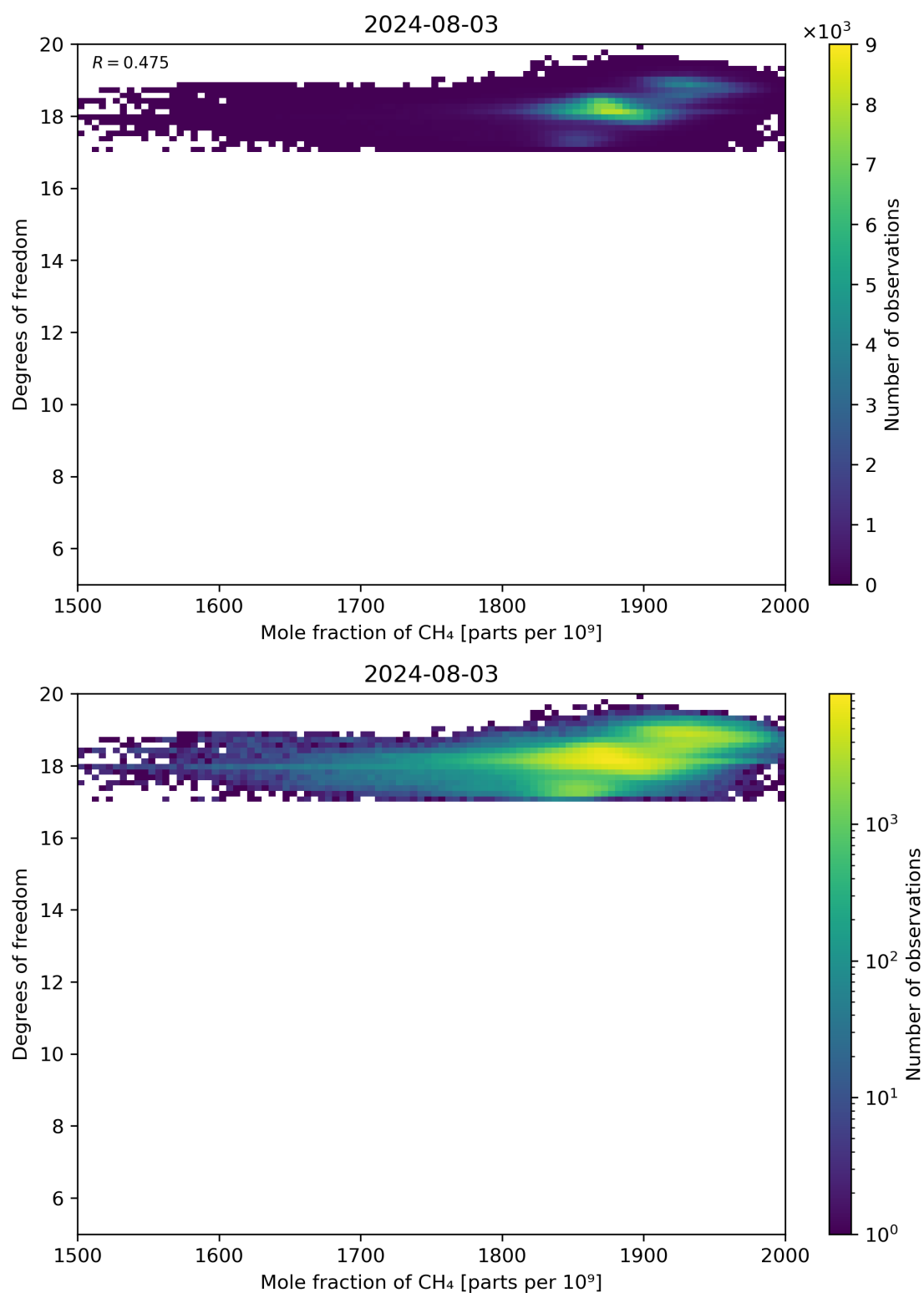
Figure 72: Scatter density plot of “Mole fraction of CH 4 ” against “Degrees of freedom” for 2024-08-02 to 2024-08-04.
