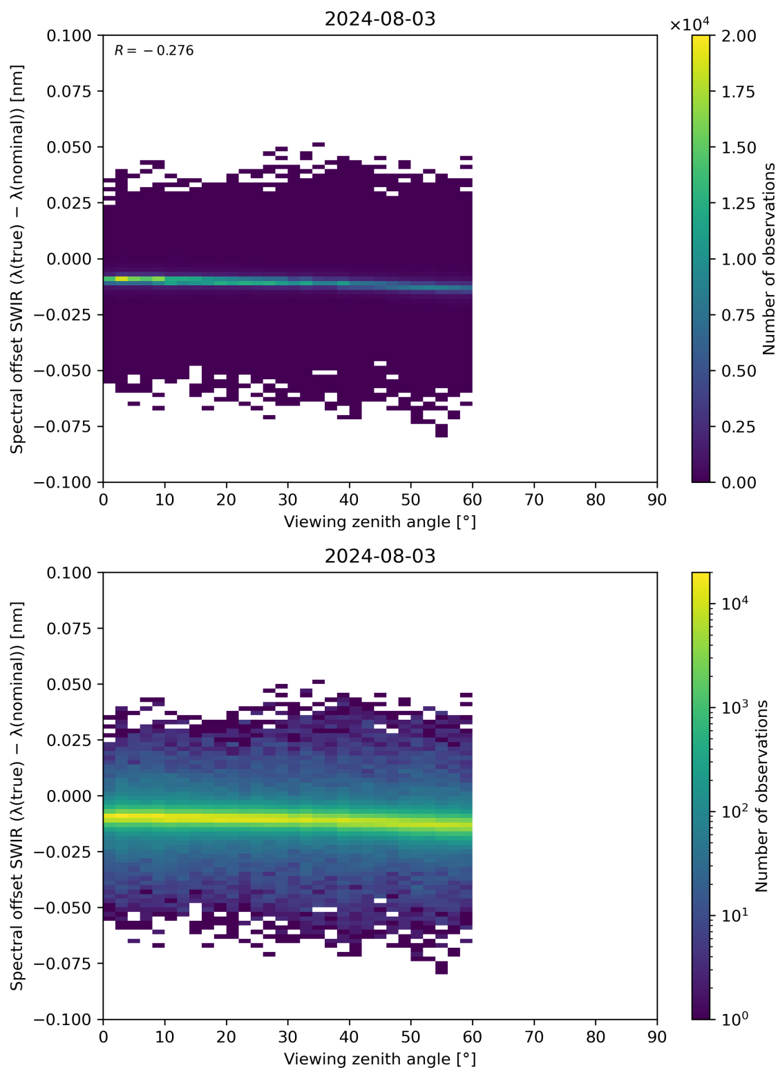
Figure 116: Scatter density plot of “Viewing zenith angle” against “Spectral offset SWIR ( \lambda(\text{true}) - \lambda(\text{nominal}) )” for 2024-08-02 to 2024-08-04.
