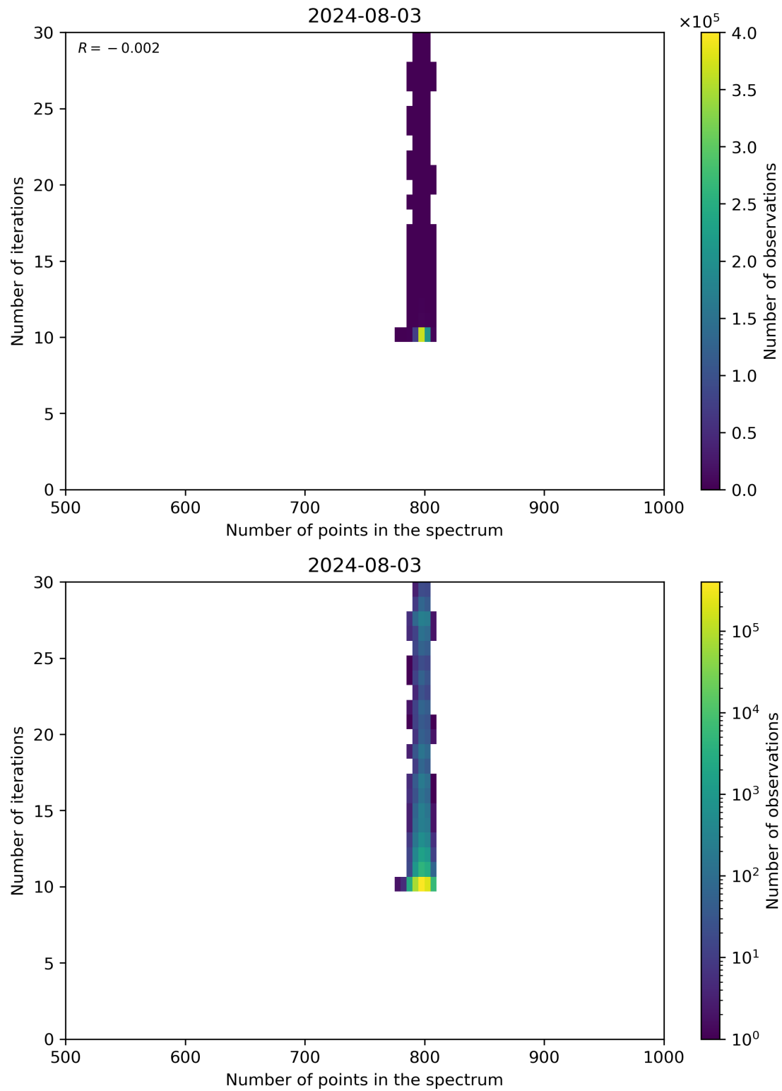
Figure 92: Scatter density plot of “Number of points in the spectrum” against “Number of iterations” for 2024-08-02 to 2024-08-04.
