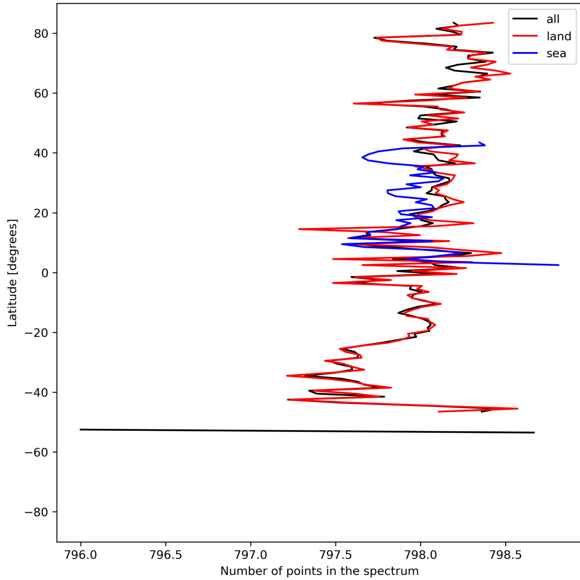
Figure 15: Zonal average of “Number of points in the spectrum” for 2024-08-02 to 2024-08-04.
