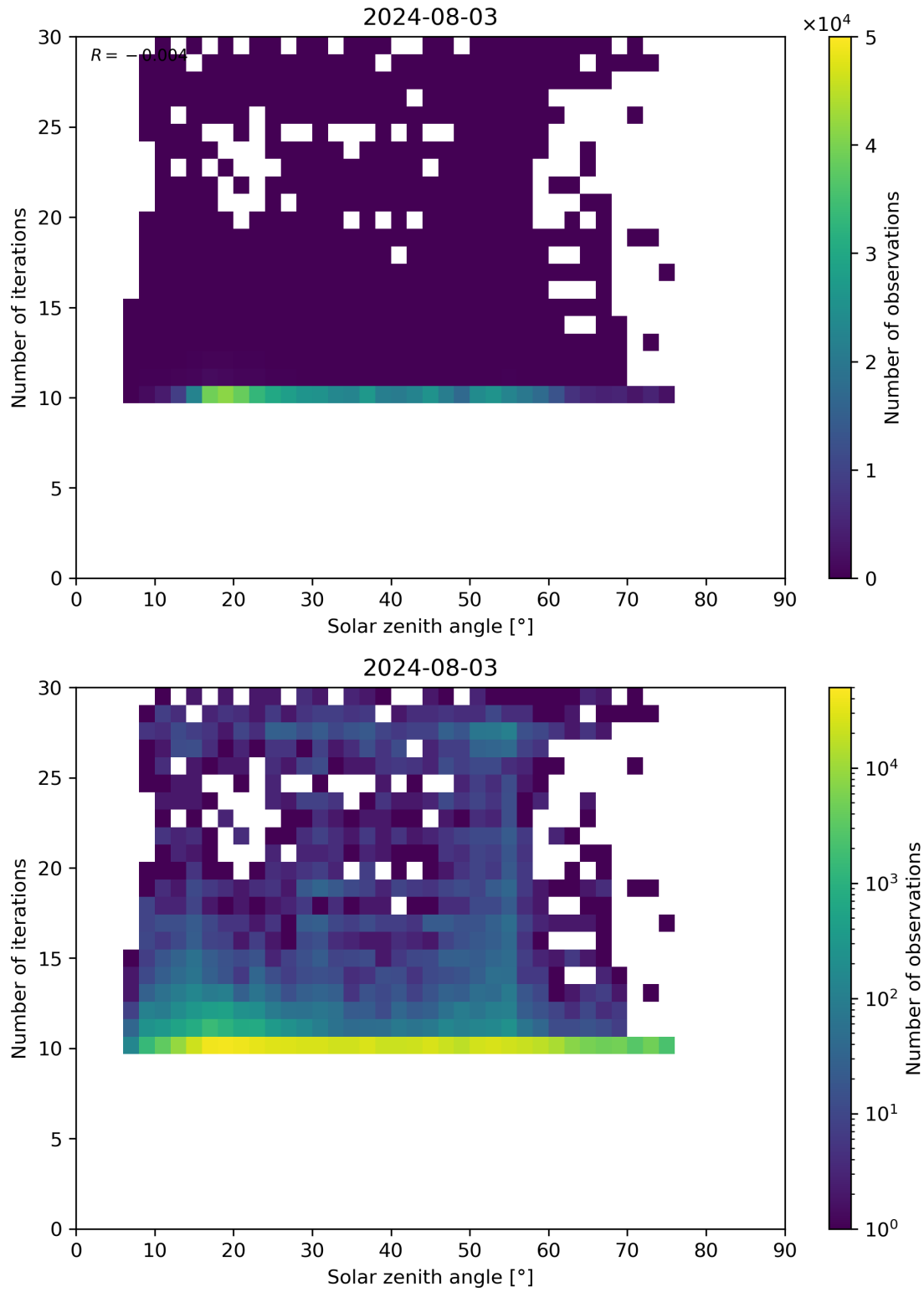
Figure 102: Scatter density plot of “Solar zenith angle” against “Number of iterations” for 2024-08-02 to 2024-08-04.
