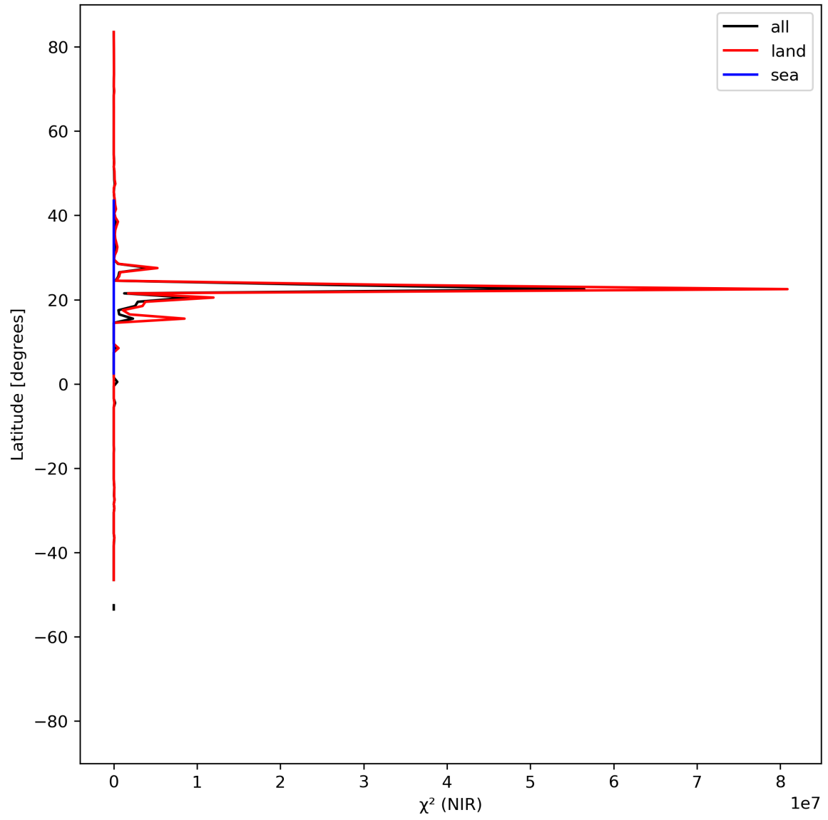
Figure 18: Zonal average of “ \chi^2 (NIR)” for 2024-08-02 to 2024-08-04.
