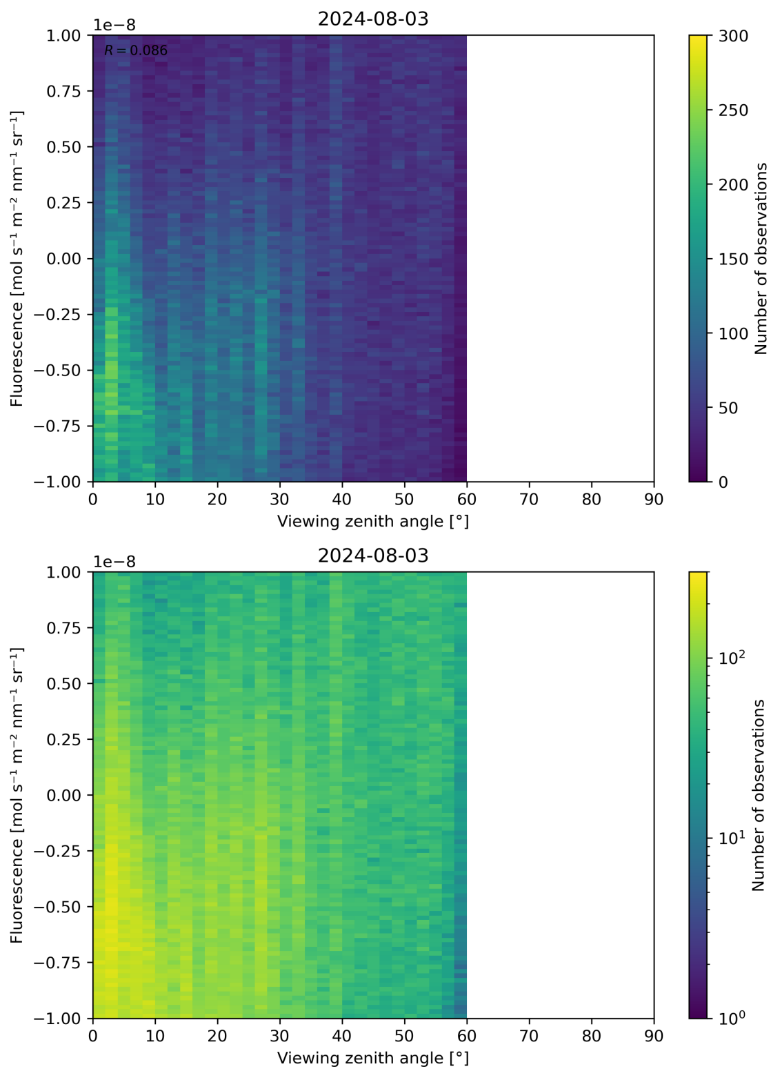
Figure 108: Scatter density plot of “Viewing zenith angle” against “Fluorescence” for 2024-08-02 to 2024-08-04.
