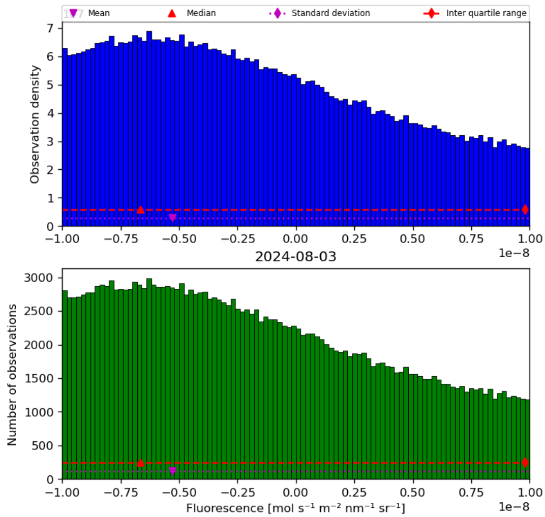
Figure 32: Histogram of “Fluorescence” for 2024-08-02 to 2024-08-04
