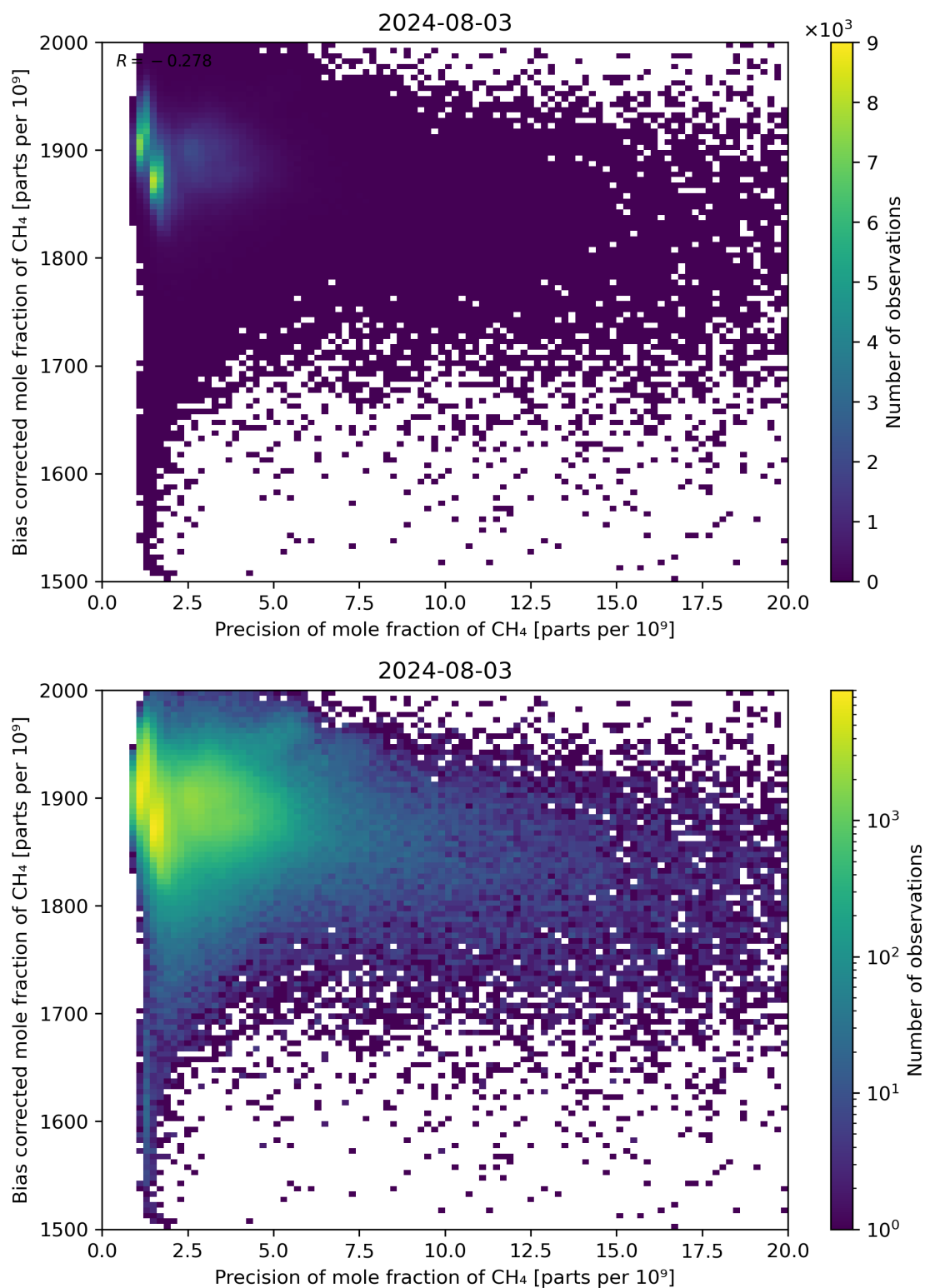
Figure 82: Scatter density plot of “Precision of mole fraction of CH 4 ” against “Bias corrected mole fraction of CH 4 ” for 2024-08-02 to 2024-08-04.
