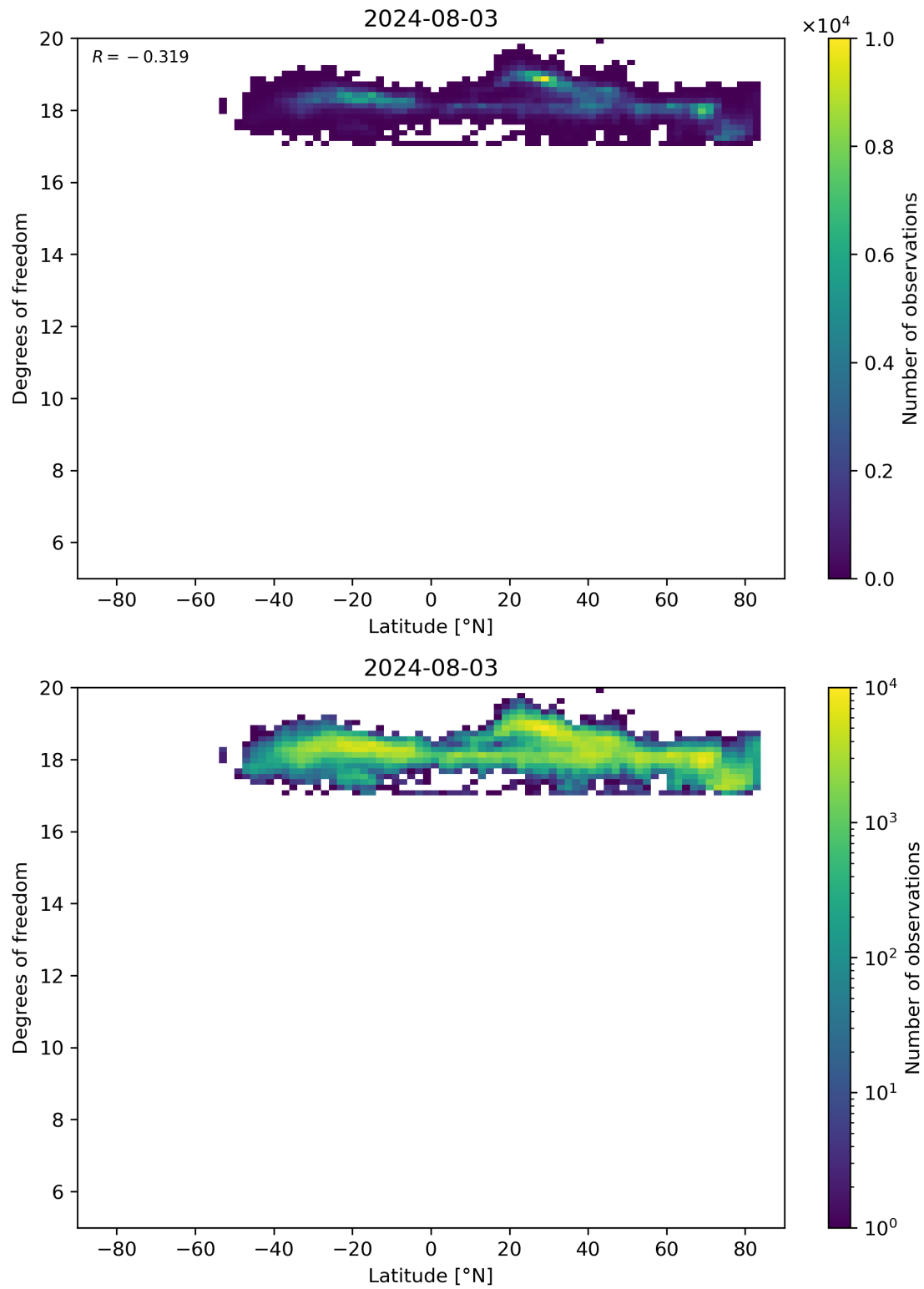
Figure 55: Scatter density plot of “Latitude” against “Degrees of freedom” for 2024-08-02 to 2024-08-04.
