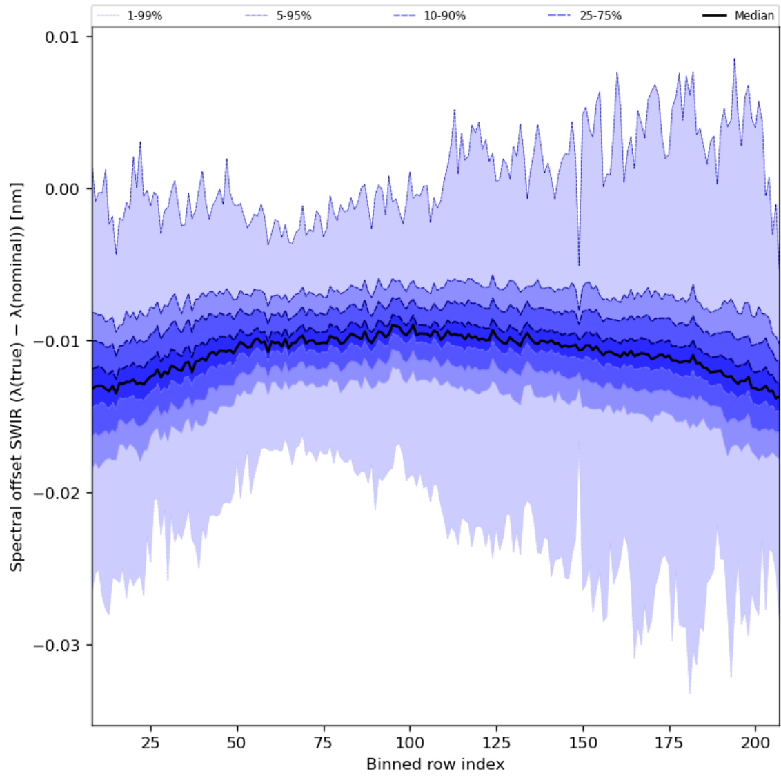
Figure 38: Along track statistics of “Spectral offset SWIR ( \lambda(\text{true}) - \lambda(\text{nominal}) )” for 2024-08-02 to 2024-08-04
