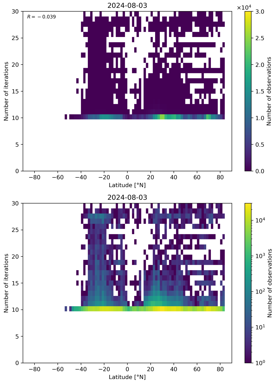
Figure 60: Scatter density plot of “Latitude” against “Number of iterations” for 2024-08-02 to 2024-08-04.
