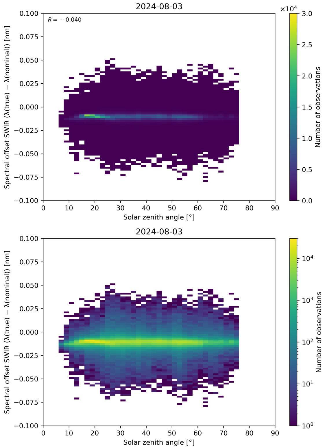
Figure 104: Scatter density plot of “Solar zenith angle” against “Spectral offset SWIR ( \lambda(\text{true}) - \lambda(\text{nominal}) )” for 2024-08-02 to 2024-08-04.
