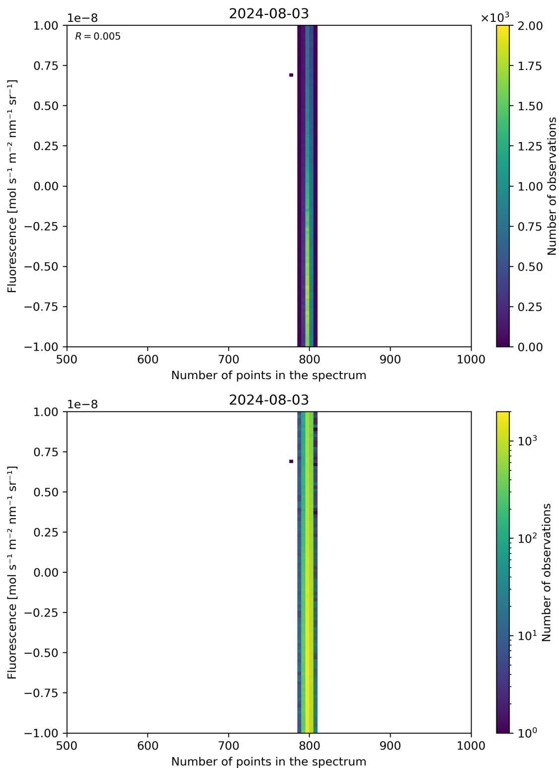
Figure 91: Scatter density plot of “Number of points in the spectrum” against “Fluorescence” for 2024-08-02 to 2024-08-04.
