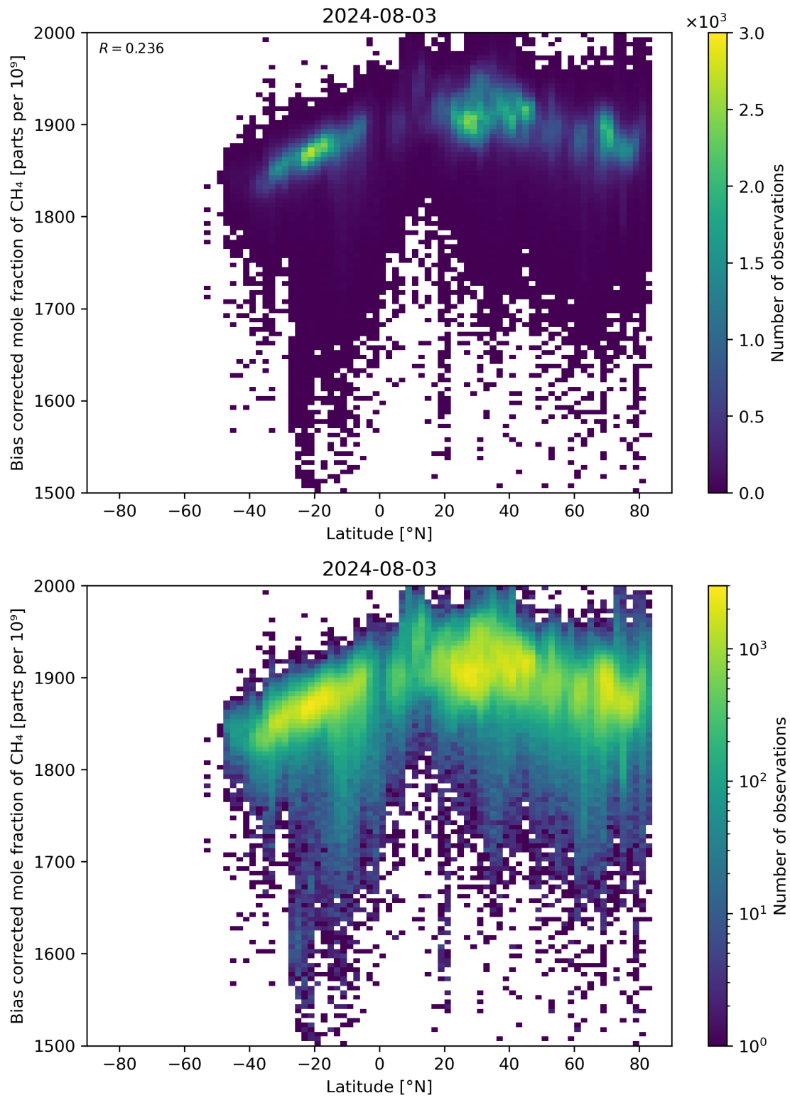
Figure 58: Scatter density plot of “Latitude” against “Bias corrected mole fraction of CH 4 ” for 2024-08-02 to 2024-08-04.
