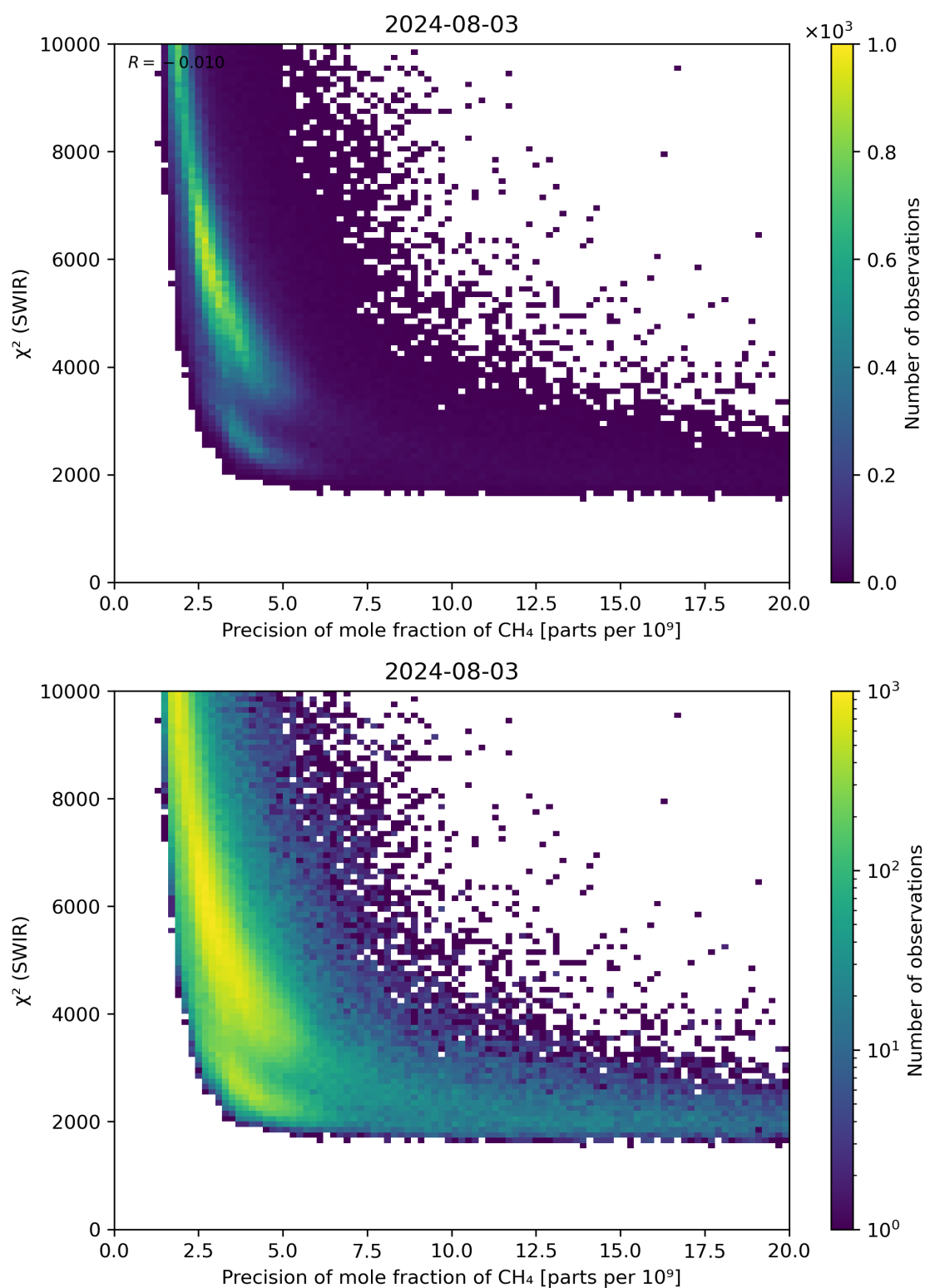
Figure 79: Scatter density plot of “Precision of mole fraction of \text{CH}_4 ” against “ \chi^2 (SWIR)” for 2024-08-02 to 2024-08-04.
