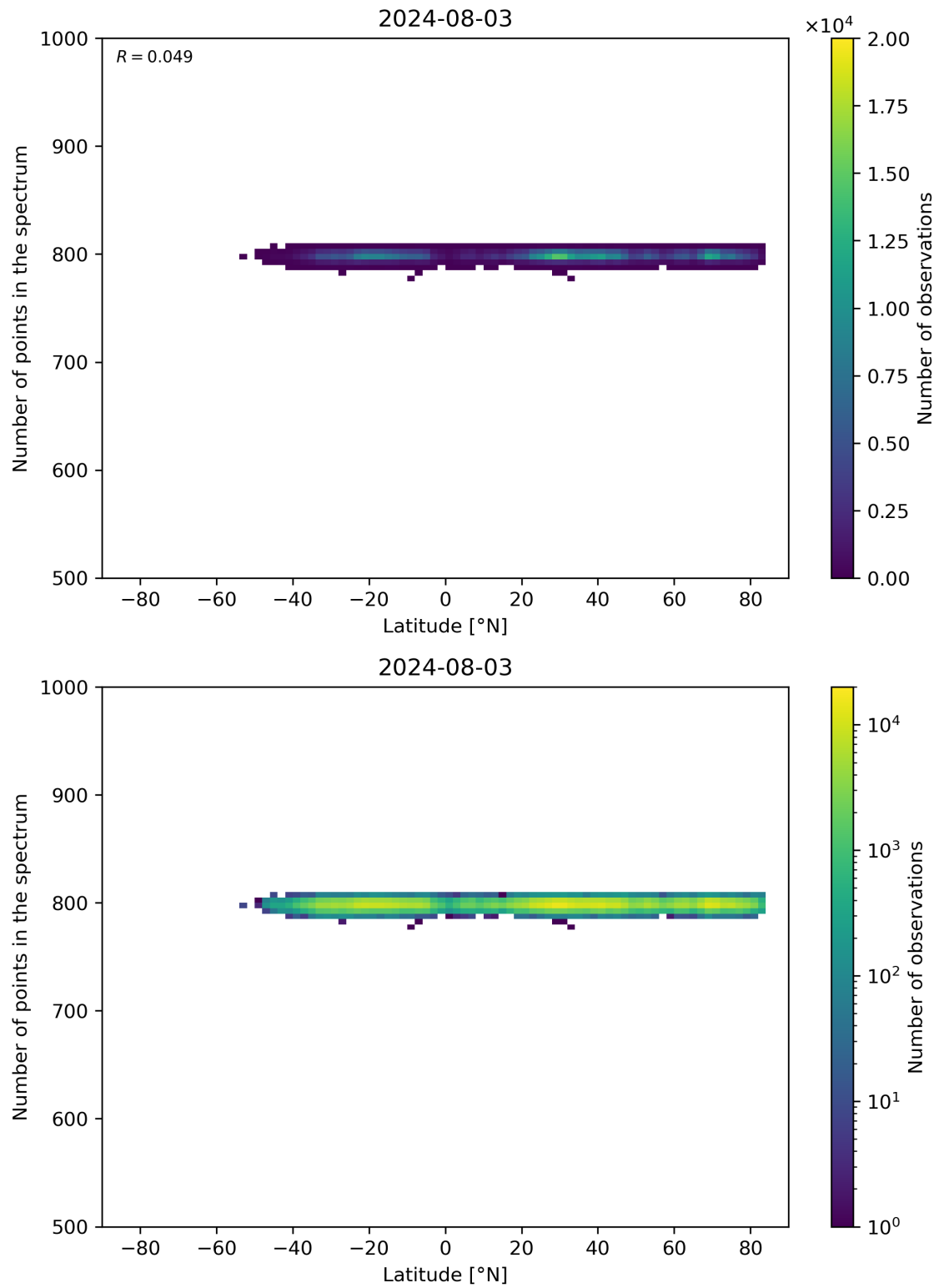
Figure 61: Scatter density plot of “Latitude” against “Number of points in the spectrum” for 2024-08-02 to 2024-08-04.
