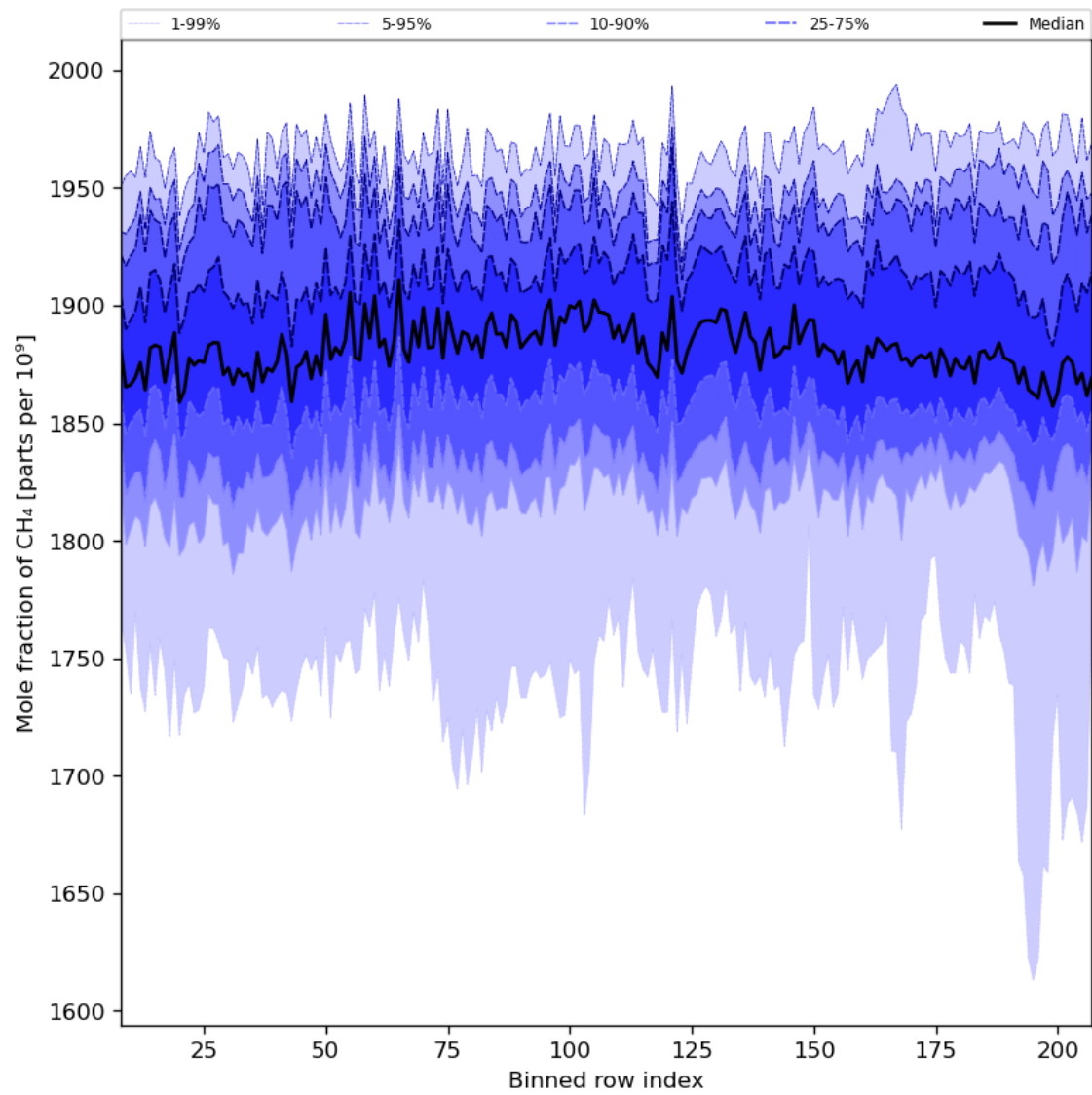
Figure 34: Along track statistics of “Mole fraction of CH 4 ” for 2024-08-02 to 2024-08-04
