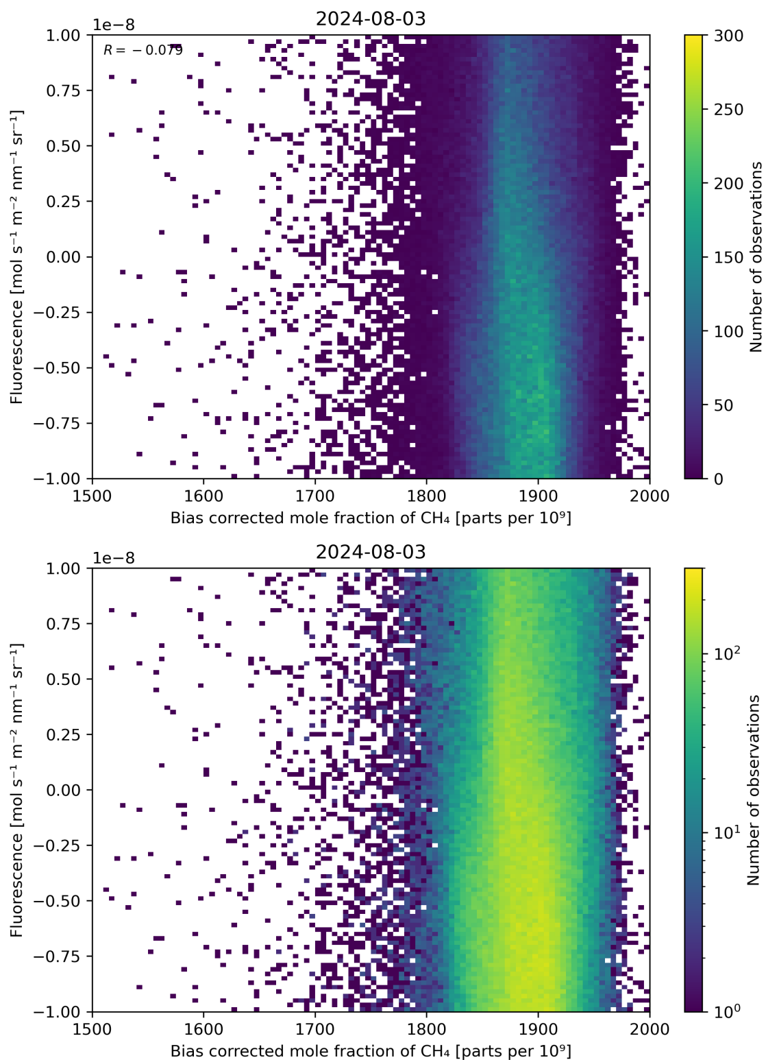
Figure 66: Scatter density plot of “Bias corrected mole fraction of \text{CH}_4 ” against “Fluorescence” for 2024-08-02 to 2024-08-04.
