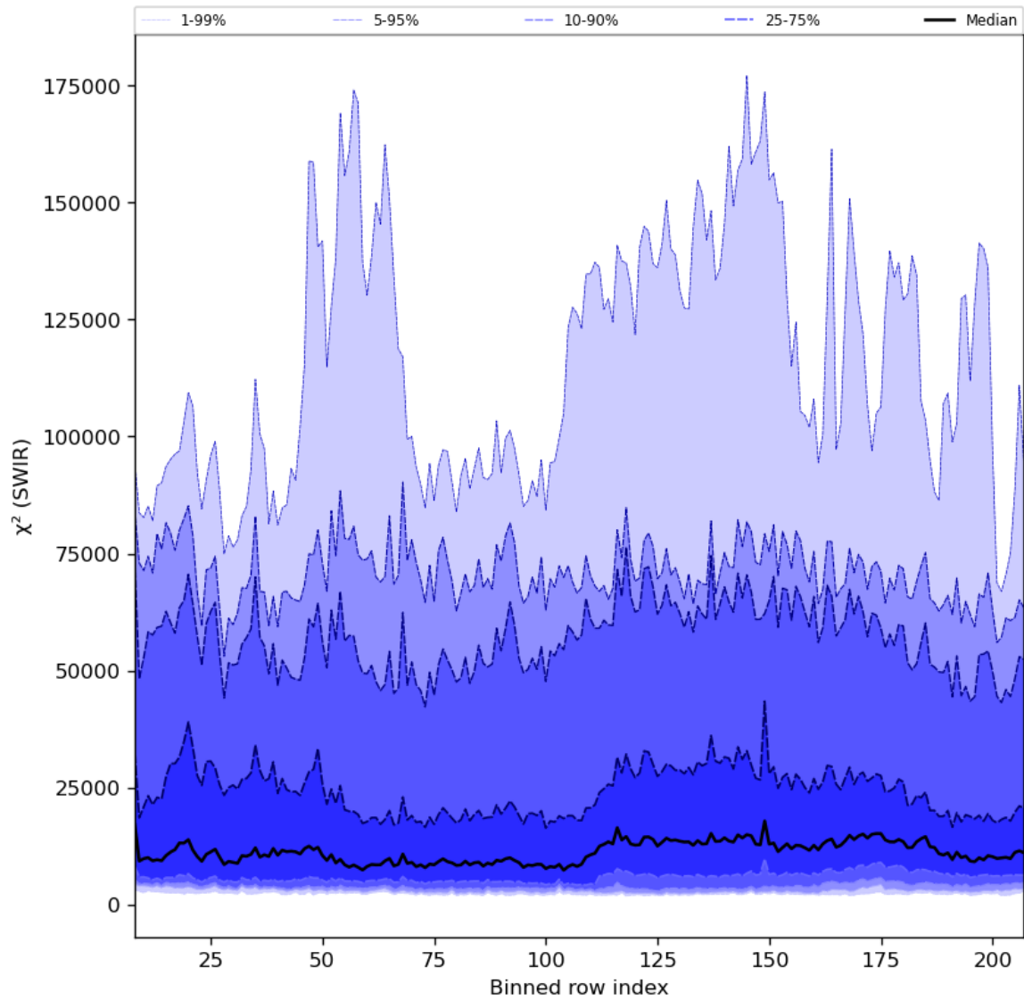
Figure 39: Along track statistics of " \chi^2 (SWIR)" for 2024-08-02 to 2024-08-04
