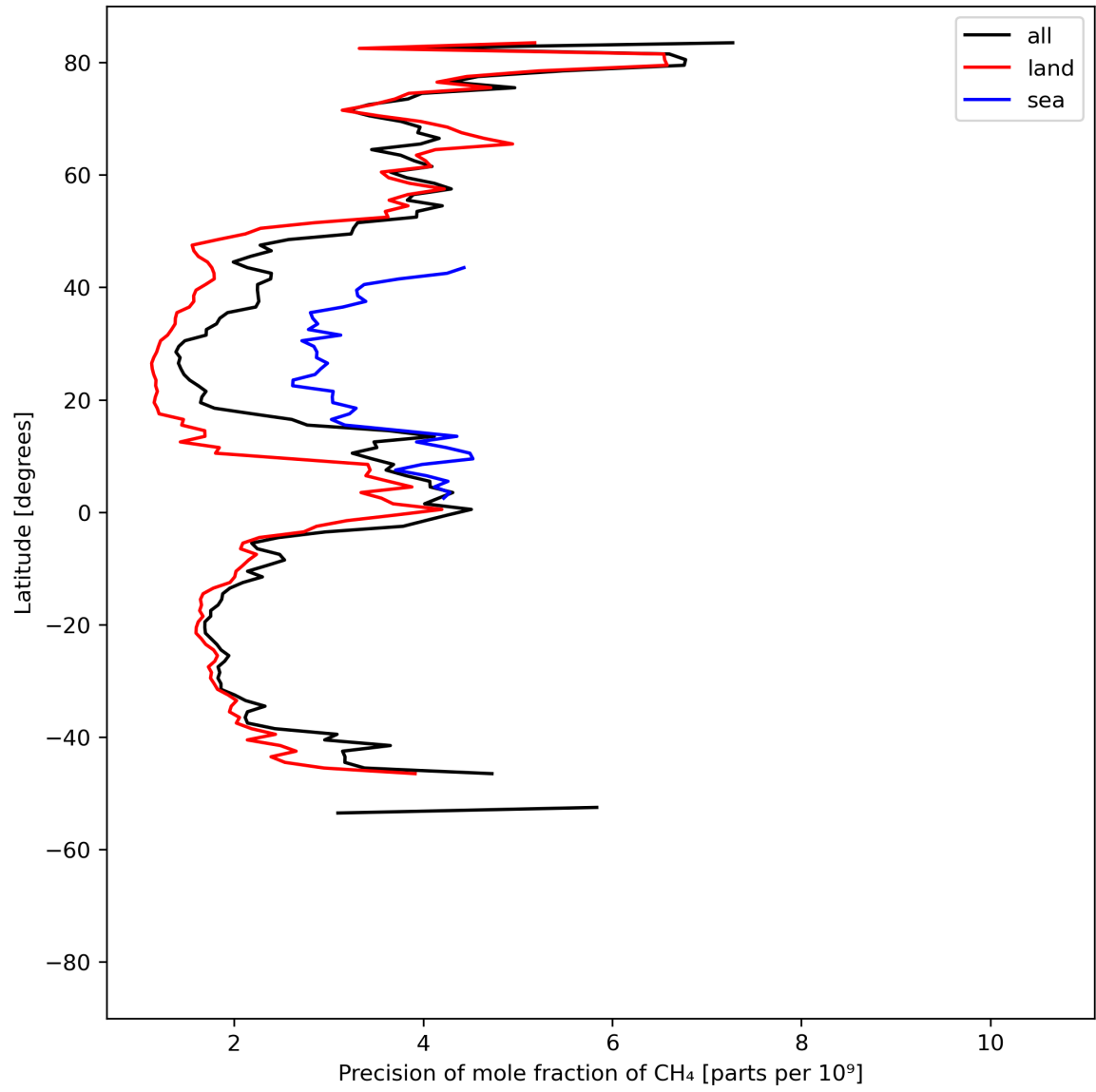
Figure 13: Zonal average of “Precision of mole fraction of CH 4 ” for 2024-08-02 to 2024-08-04.
