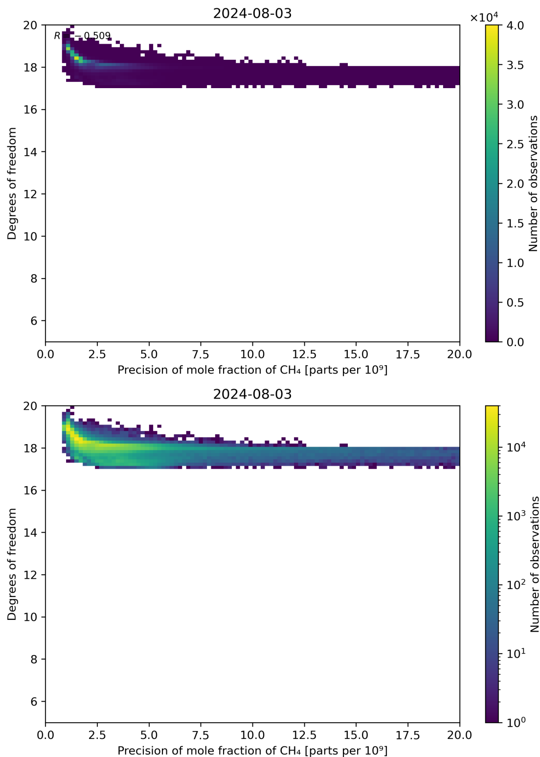
Figure 80: Scatter density plot of “Precision of mole fraction of CH 4 ” against “Degrees of freedom” for 2024-08-02 to 2024-08-04.
