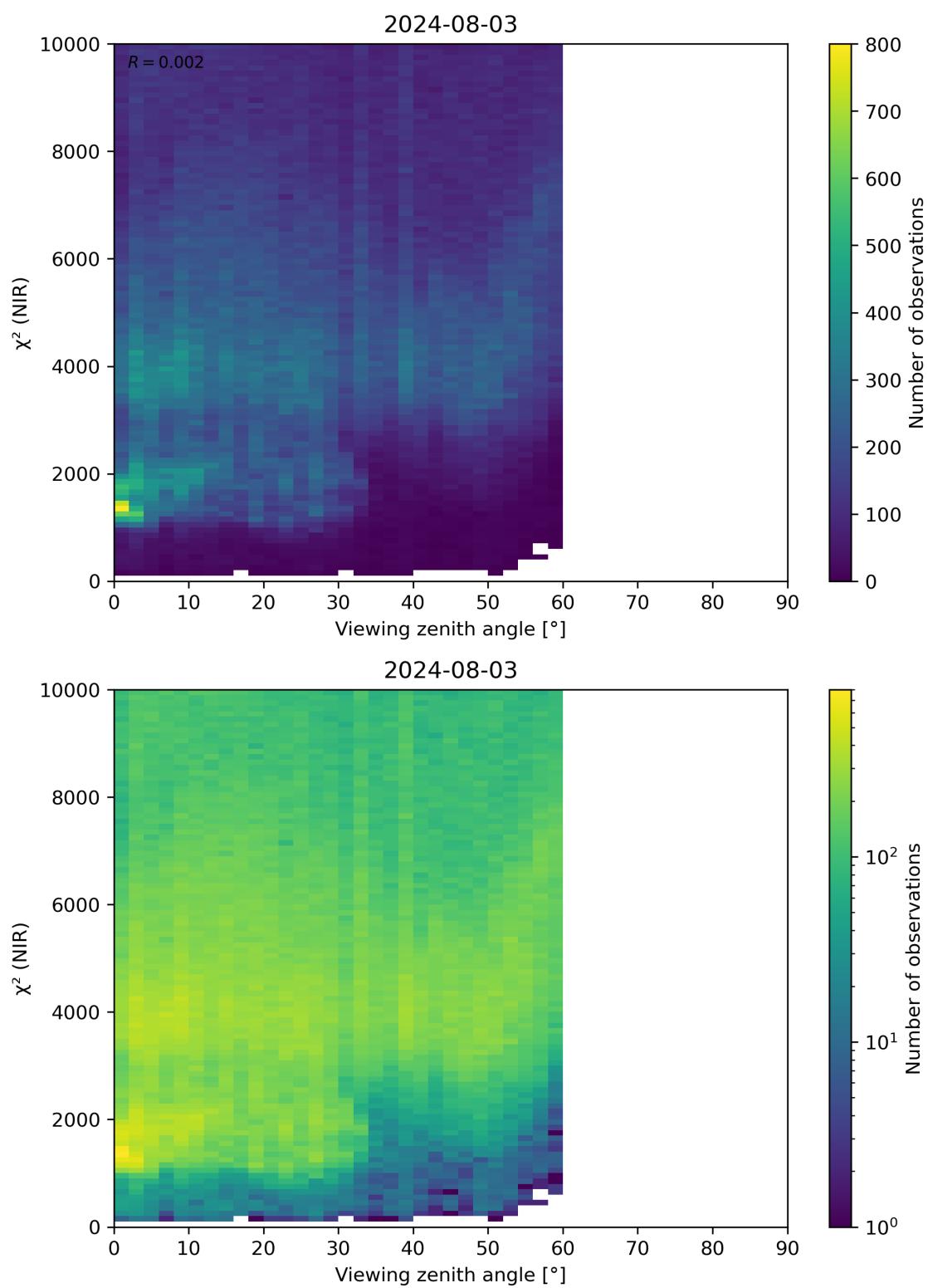
Figure 105: Scatter density plot of “Viewing zenith angle” against “ \chi^2 (NIR)” for 2024-08-02 to 2024-08-04.
