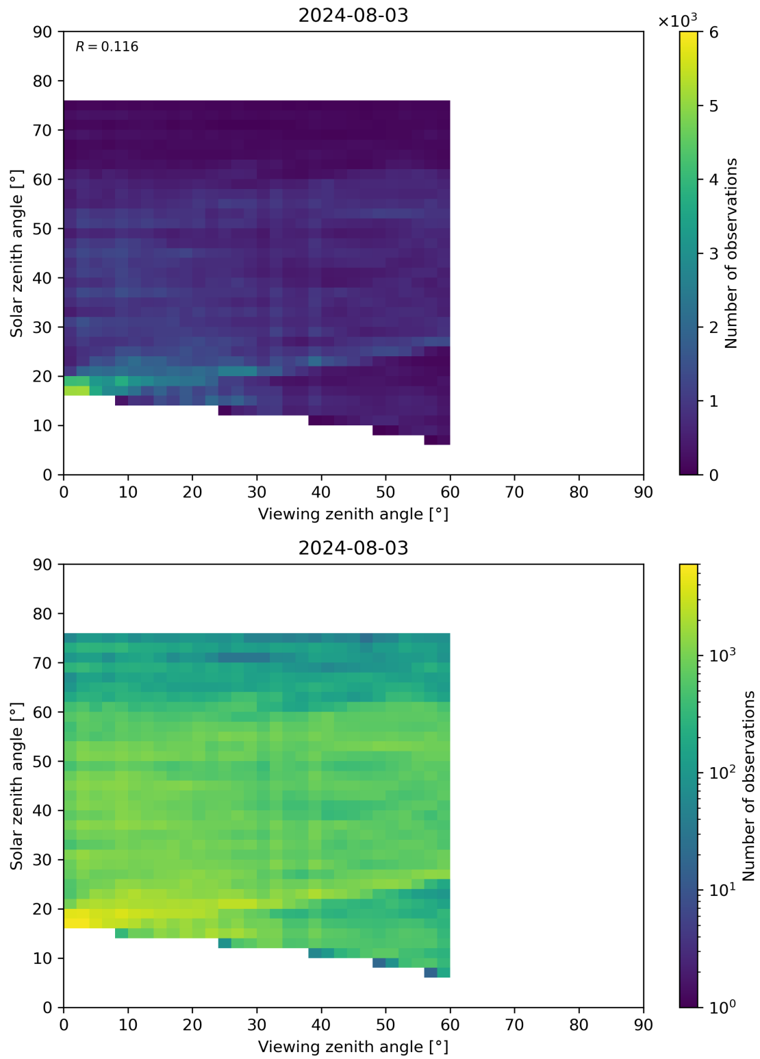
Figure 115: Scatter density plot of “Viewing zenith angle” against “Solar zenith angle” for 2024-08-02 to 2024-08-04.
