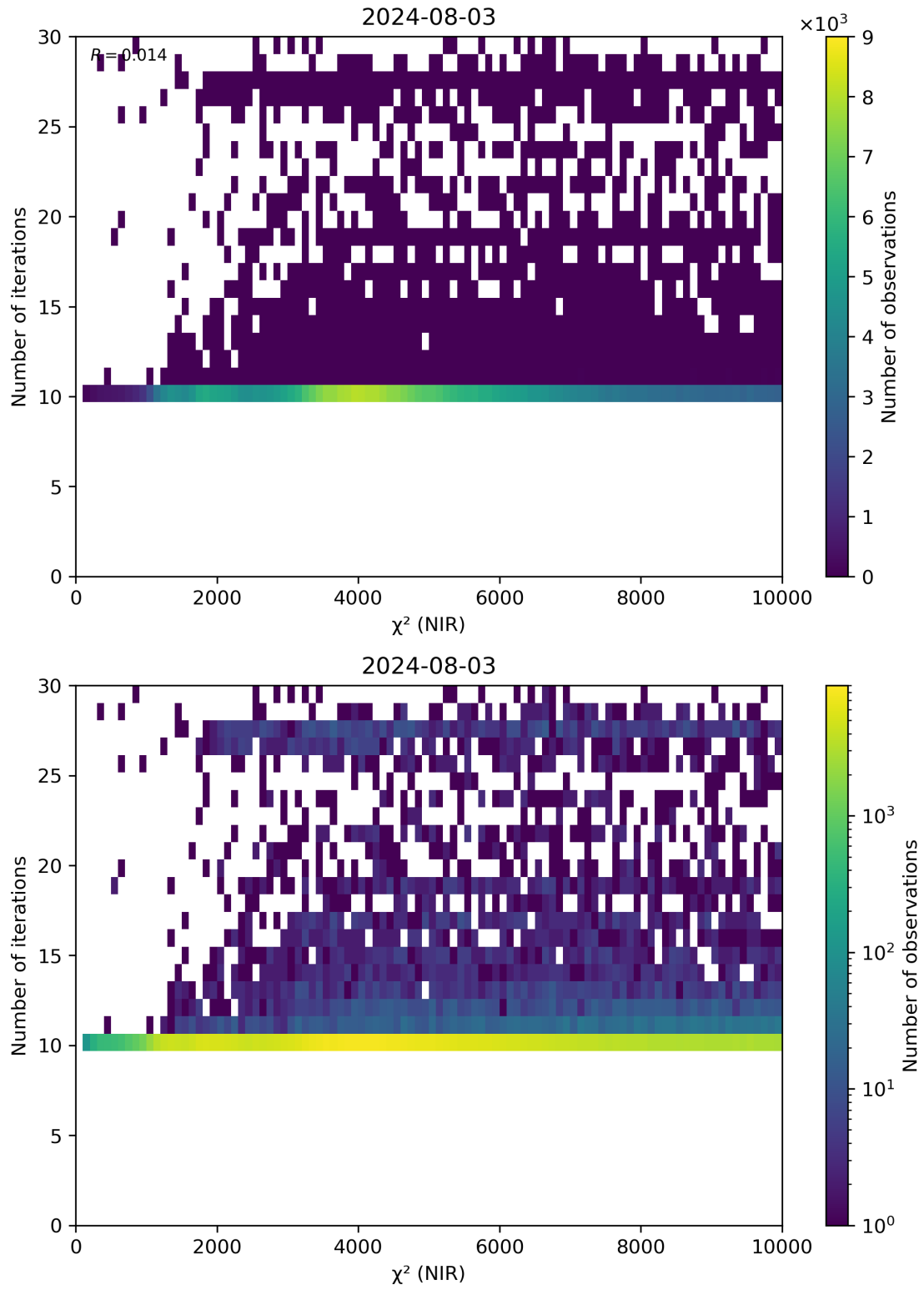
Figure 46: Scatter density plot of “ \chi^2 (NIR)” against “Number of iterations” for 2024-08-02 to 2024-08-04.
