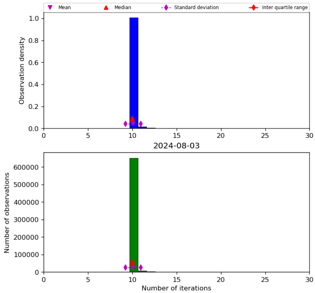
Figure 31: Histogram of “Number of iterations” for 2024-08-02 to 2024-08-04
