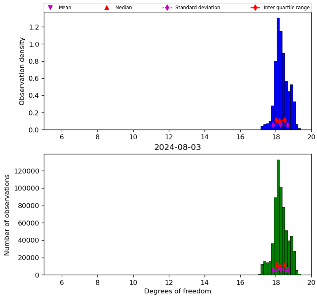
Figure 30: Histogram of “Degrees of freedom” for 2024-08-02 to 2024-08-04
