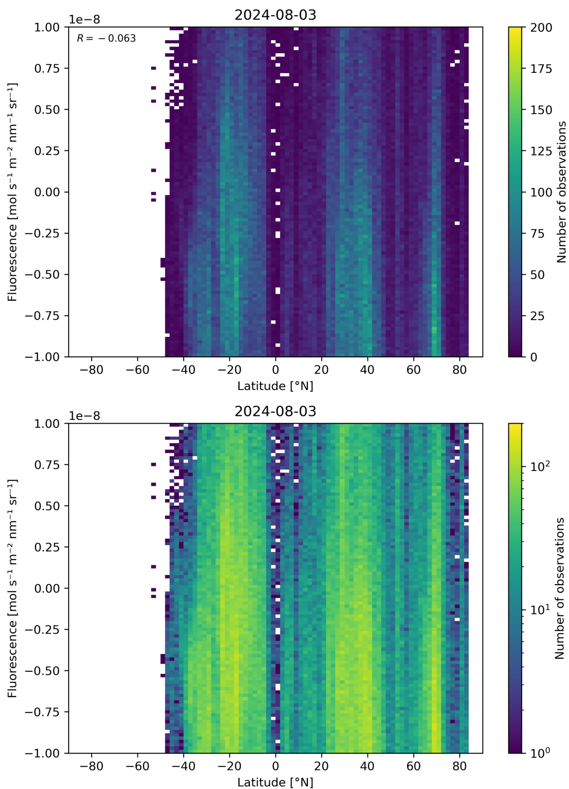
Figure 56: Scatter density plot of “Latitude” against “Fluorescence” for 2024-08-02 to 2024-08-04.
