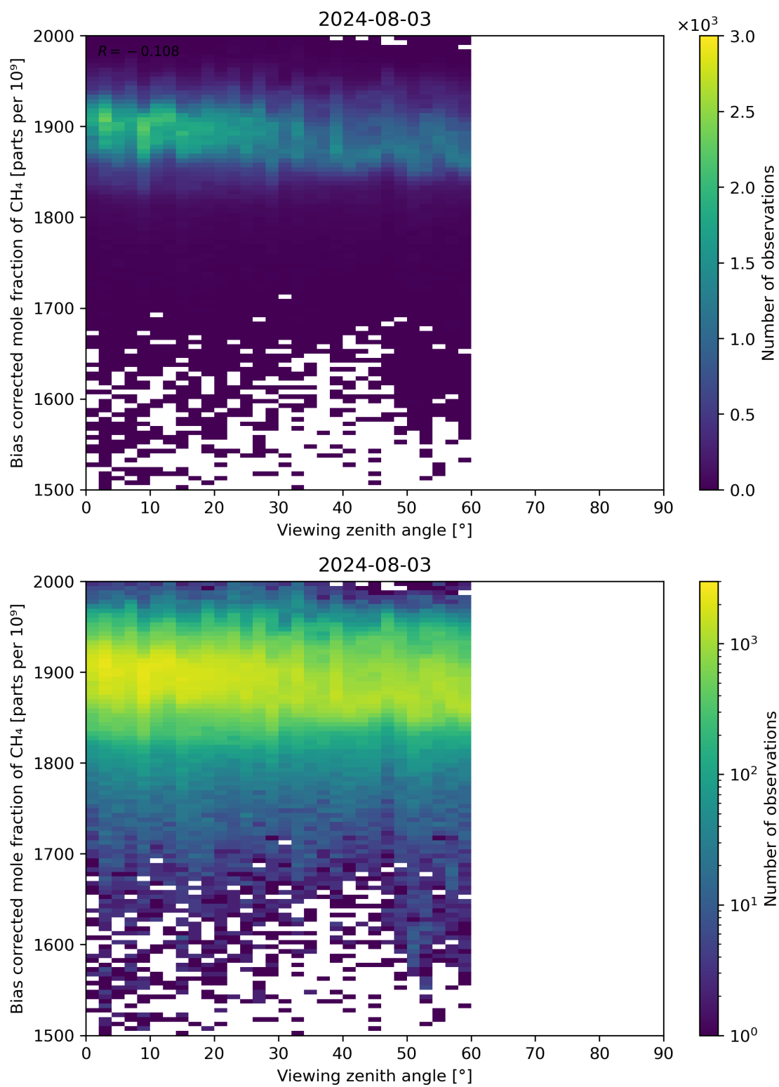
Figure 111: Scatter density plot of “Viewing zenith angle” against “Bias corrected mole fraction of CH 4 ” for 2024-08-02 to 2024-08-04.
