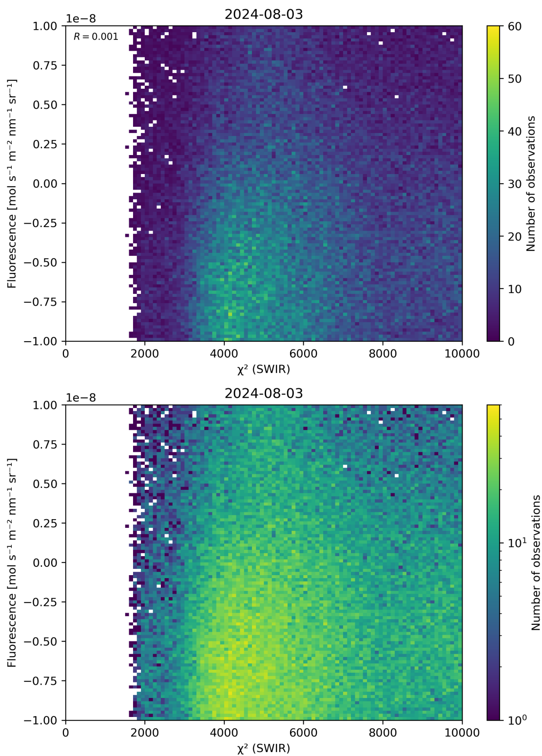
Figure 49: Scatter density plot of “ \chi^2 (SWIR)” against “Fluorescence” for 2024-08-02 to 2024-08-04.
