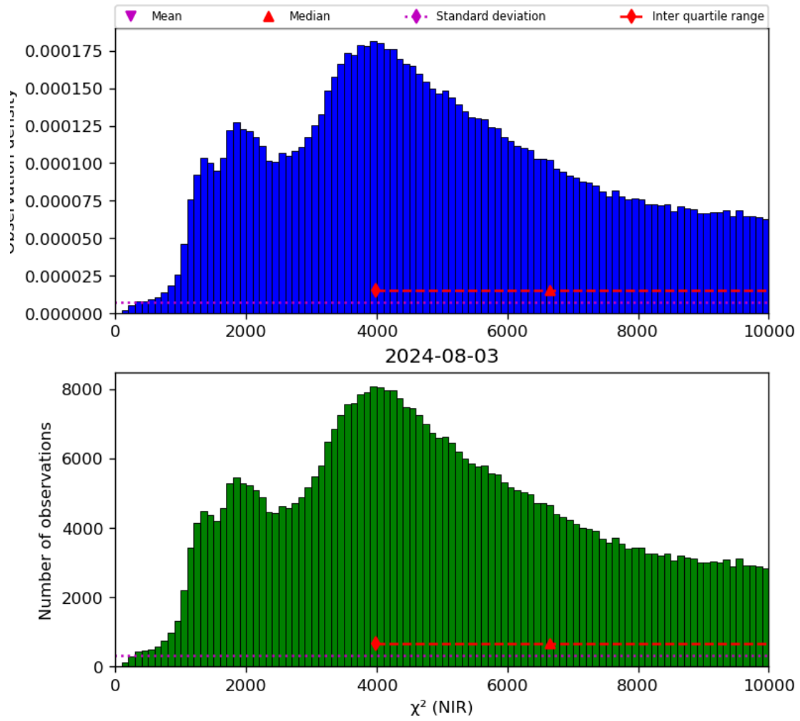
Figure 29: Histogram of “ \chi^2 (NIR)” for 2024-08-02 to 2024-08-04
