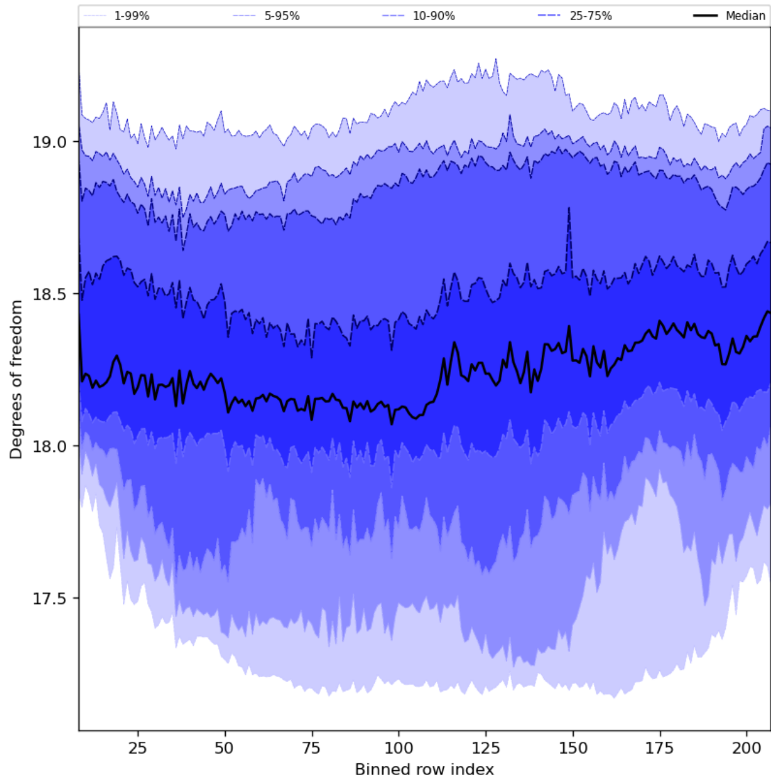
Figure 41: Along track statistics of “Degrees of freedom” for 2024-08-02 to 2024-08-04
