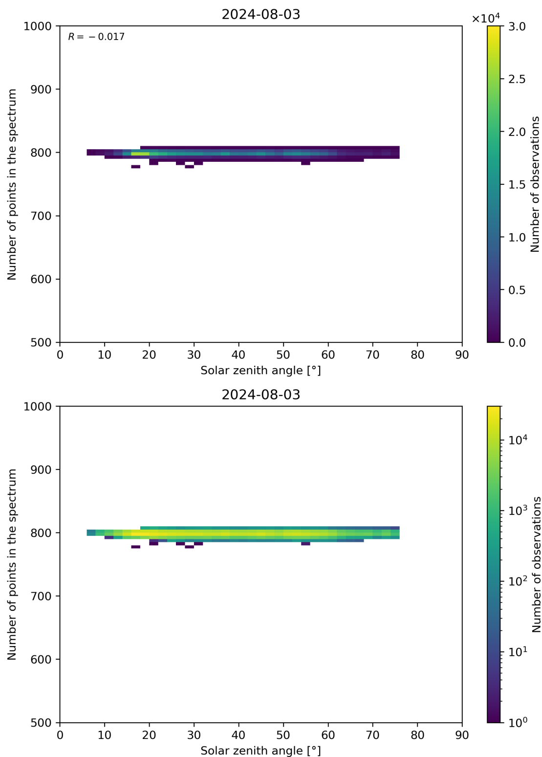
Figure 103: Scatter density plot of “Solar zenith angle” against “Number of points in the spectrum” for 2024-08-02 to 2024-08-04.
