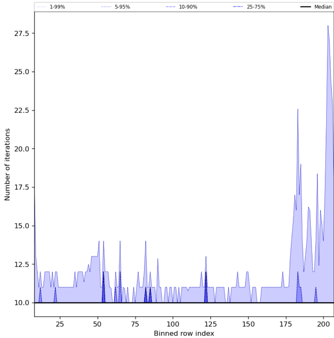
Figure 42: Along track statistics of “Number of iterations” for 2024-08-02 to 2024-08-04
