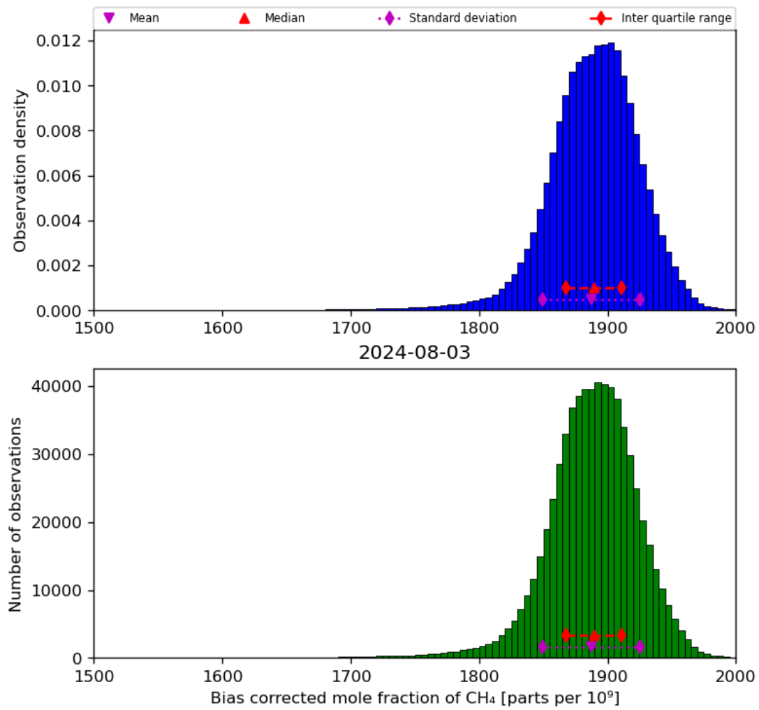
Figure 25: Histogram of “Bias corrected mole fraction of CH 4 ” for 2024-08-02 to 2024-08-04
