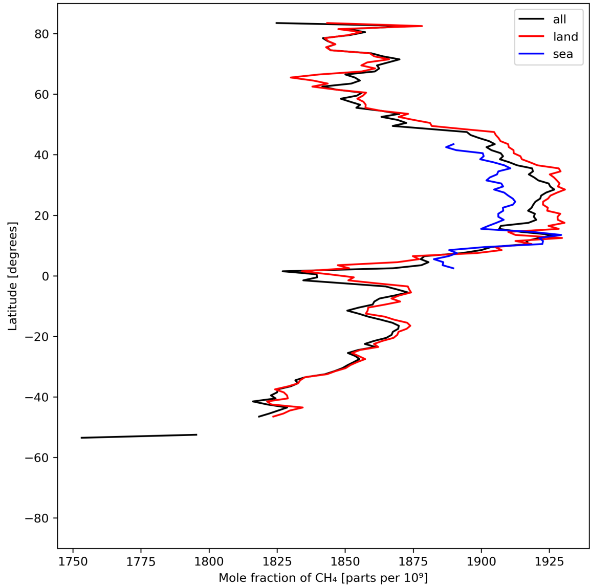
Figure 12: Zonal average of “Mole fraction of \text{CH}_4 ” for 2024-08-02 to 2024-08-04.
