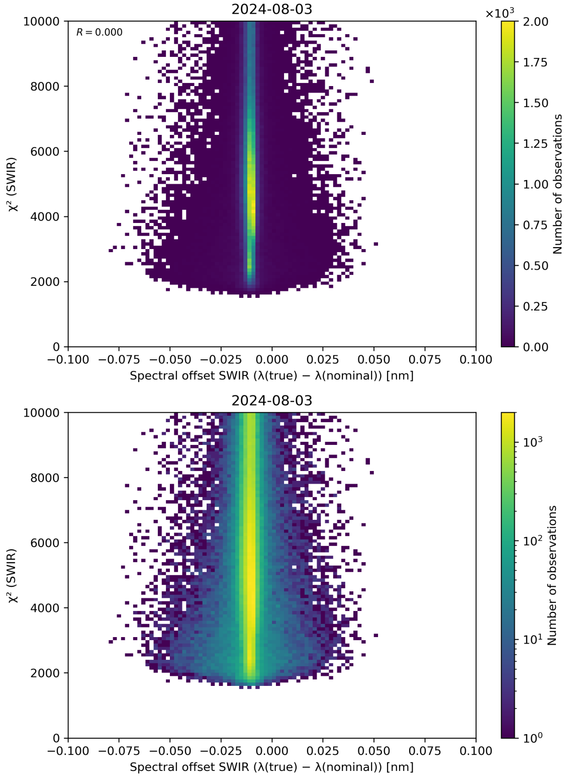
Figure 118: Scatter density plot of “Spectral offset SWIR ( \lambda(\text{true}) - \lambda(\text{nominal}) )” against “ \chi^2 (SWIR)” for 2024-08-02 to 2024-08-04.
