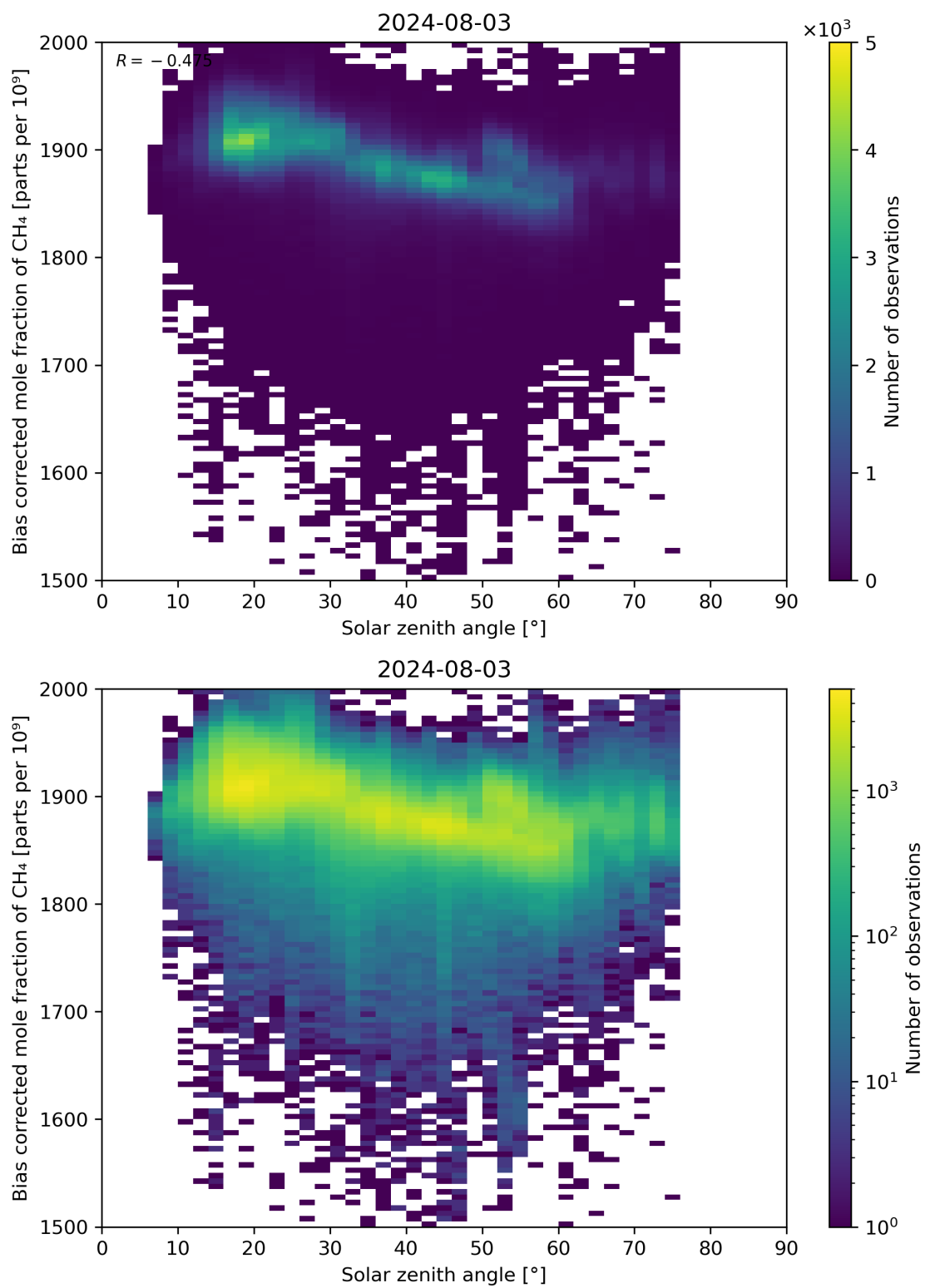
Figure 100: Scatter density plot of “Solar zenith angle” against “Bias corrected mole fraction of \text{CH}_4 ” for 2024-08-02 to 2024-08-04.
