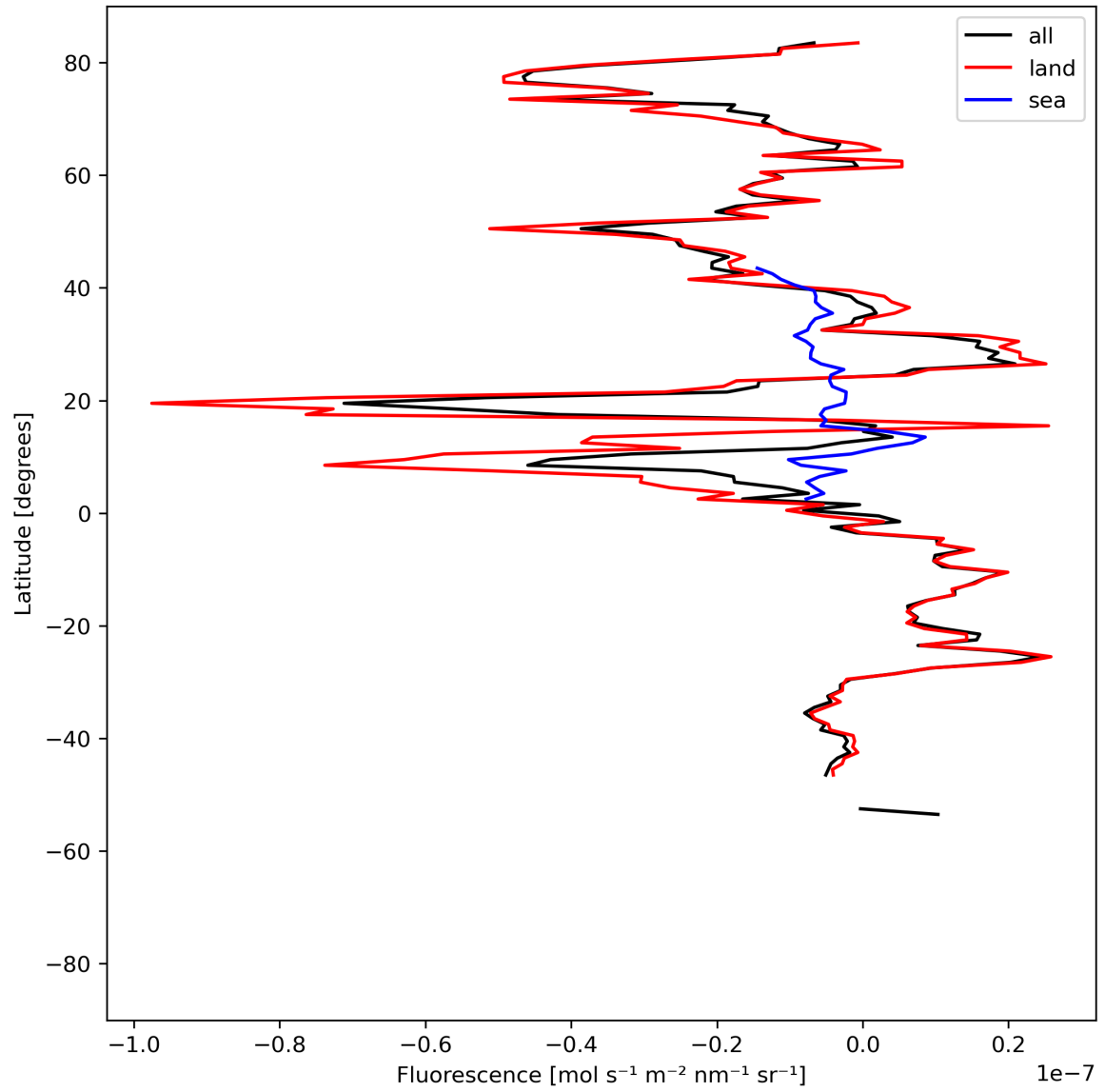
Figure 21: Zonal average of “Fluorescence” for 2024-08-02 to 2024-08-04.
