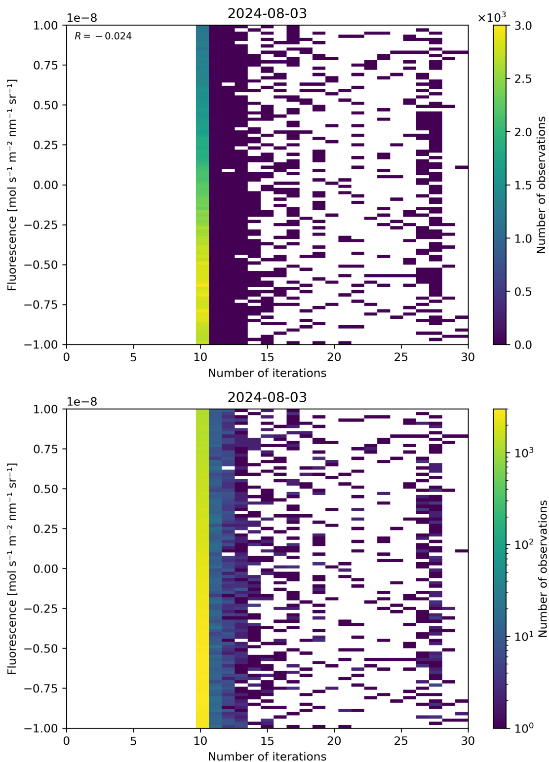
Figure 87: Scatter density plot of “Number of iterations” against “Fluorescence” for 2024-08-02 to 2024-08-04.
