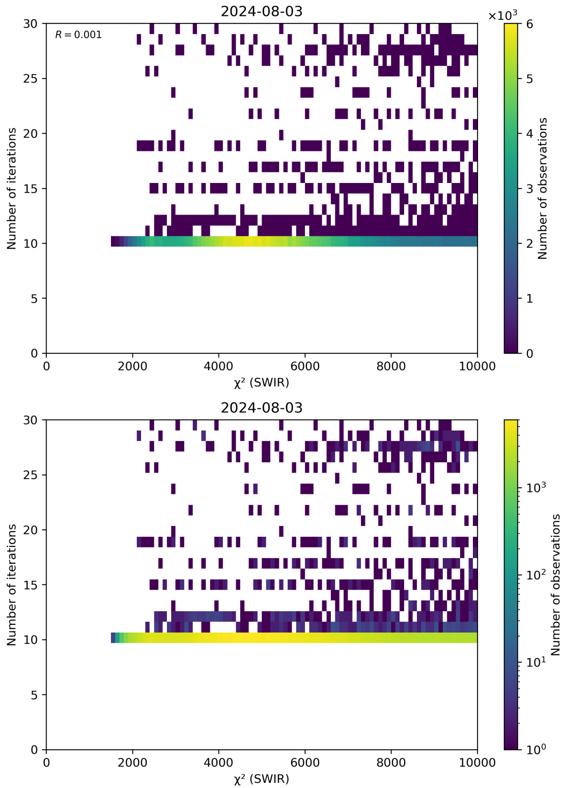
Figure 50: Scatter density plot of “ \chi^2 (SWIR)” against “Number of iterations” for 2024-08-02 to 2024-08-04.
