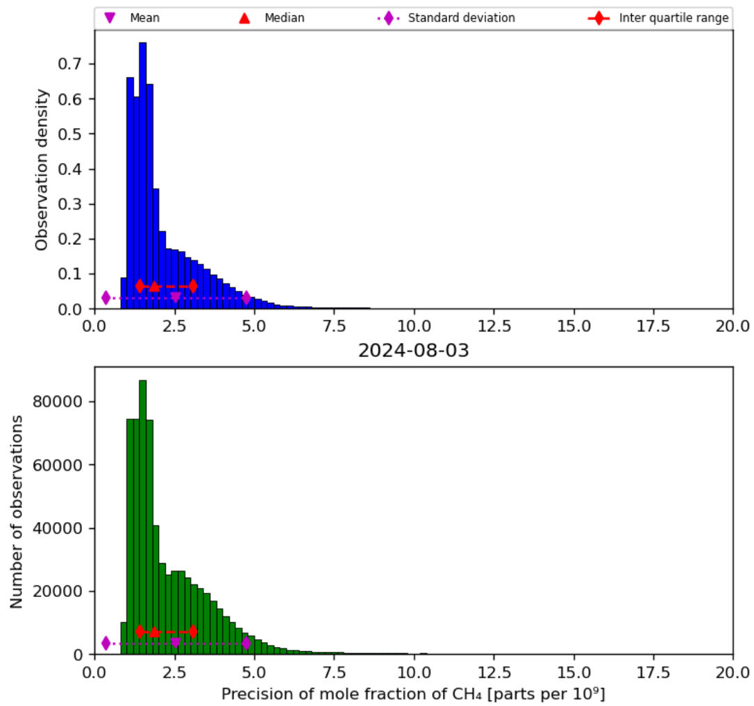
Figure 24: Histogram of “Precision of mole fraction of CH 4 ” for 2024-08-02 to 2024-08-04
