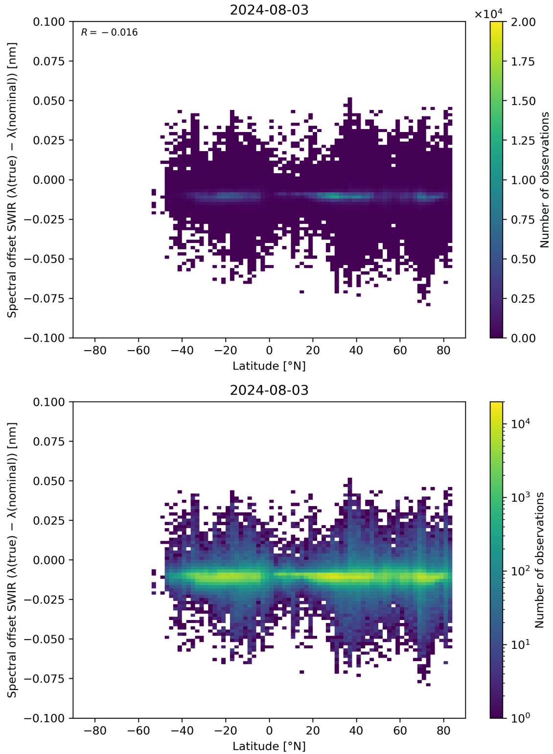
Figure 62: Scatter density plot of “Latitude” against “Spectral offset SWIR ( \lambda(\text{true}) - \lambda(\text{nominal}) )” for 2024-08-02 to 2024-08-04.
