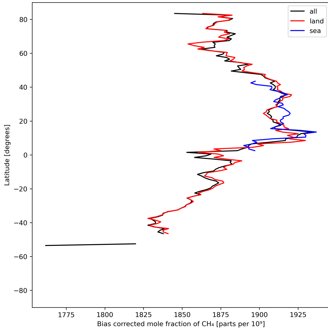
Figure 14: Zonal average of “Bias corrected mole fraction of CH 4 ” for 2024-08-02 to 2024-08-04.
