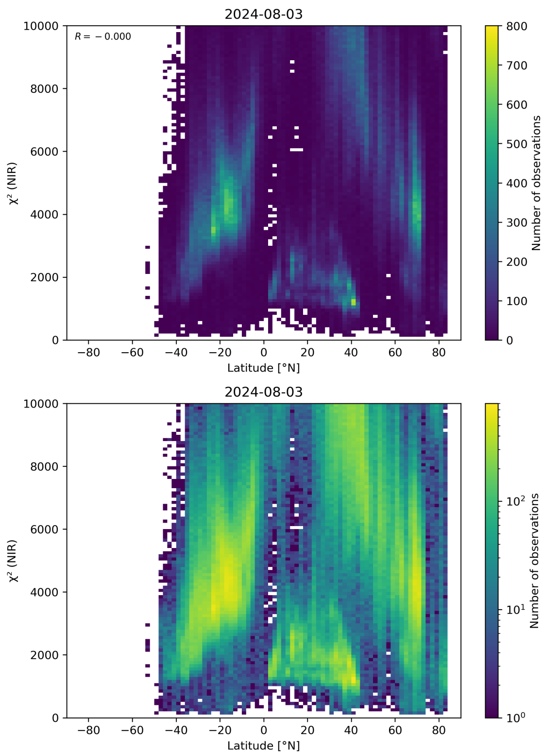
Figure 53: Scatter density plot of “Latitude” against “ \chi^2 (NIR)” for 2024-08-02 to 2024-08-04.
