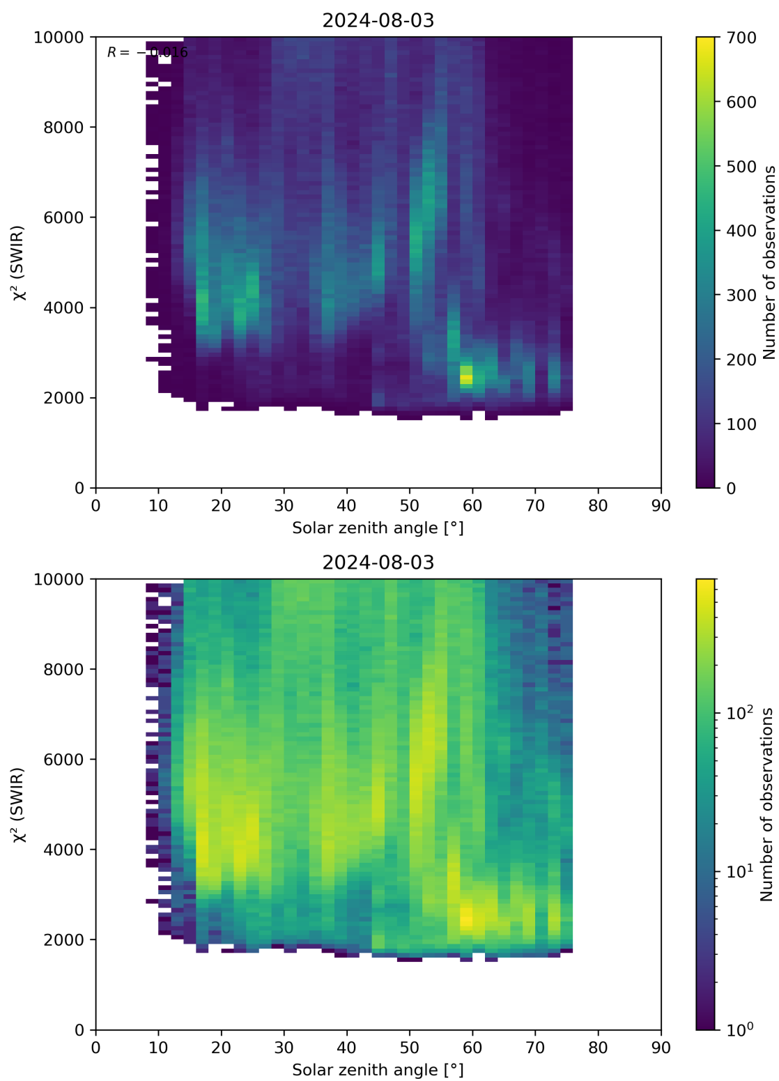
Figure 95: Scatter density plot of “Solar zenith angle” against “ \chi^2 (SWIR)” for 2024-08-02 to 2024-08-04.
