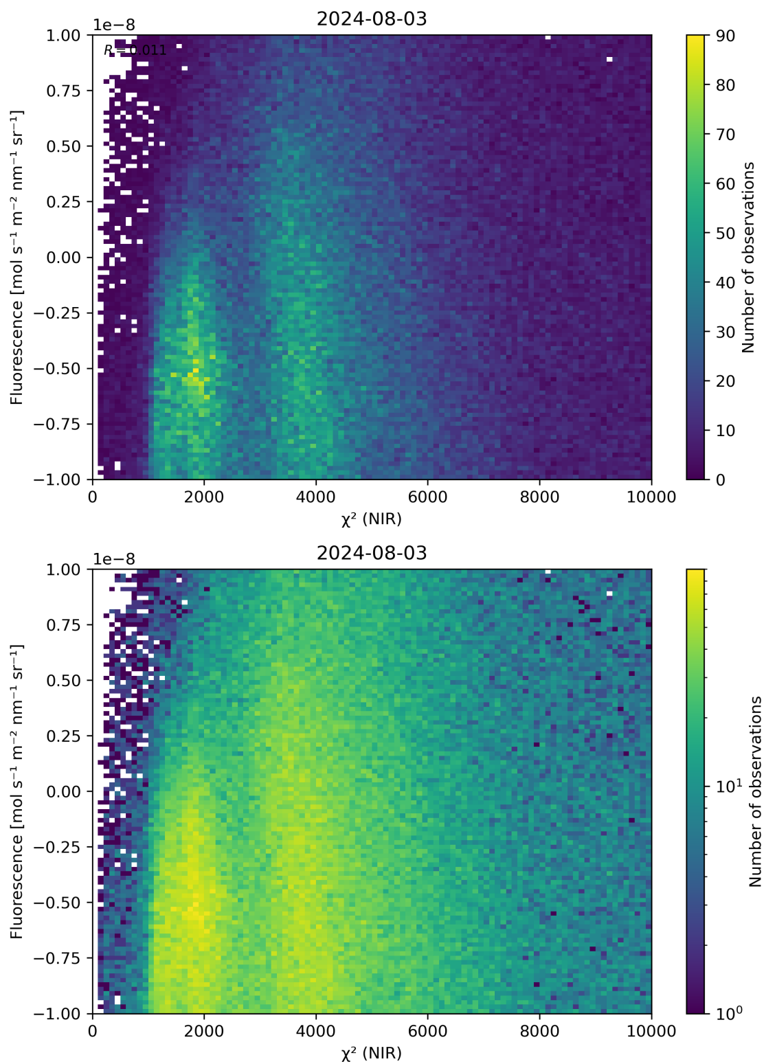
Figure 45: Scatter density plot of “ \chi^2 (NIR)” against “Fluorescence” for 2024-08-02 to 2024-08-04.
