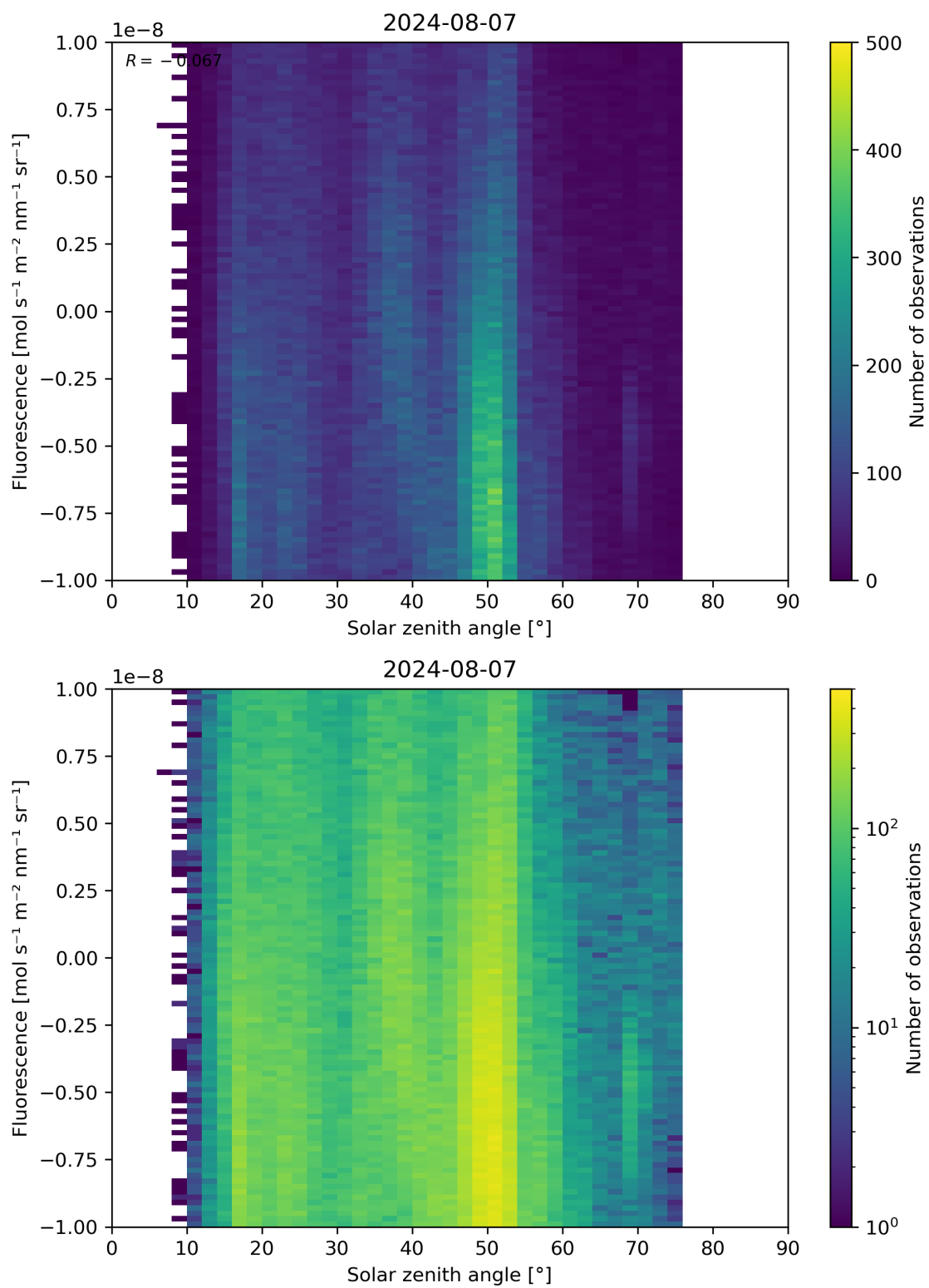
Figure 97: Scatter density plot of “Solar zenith angle” against “Fluorescence” for 2024-08-06 to 2024-08-08.
