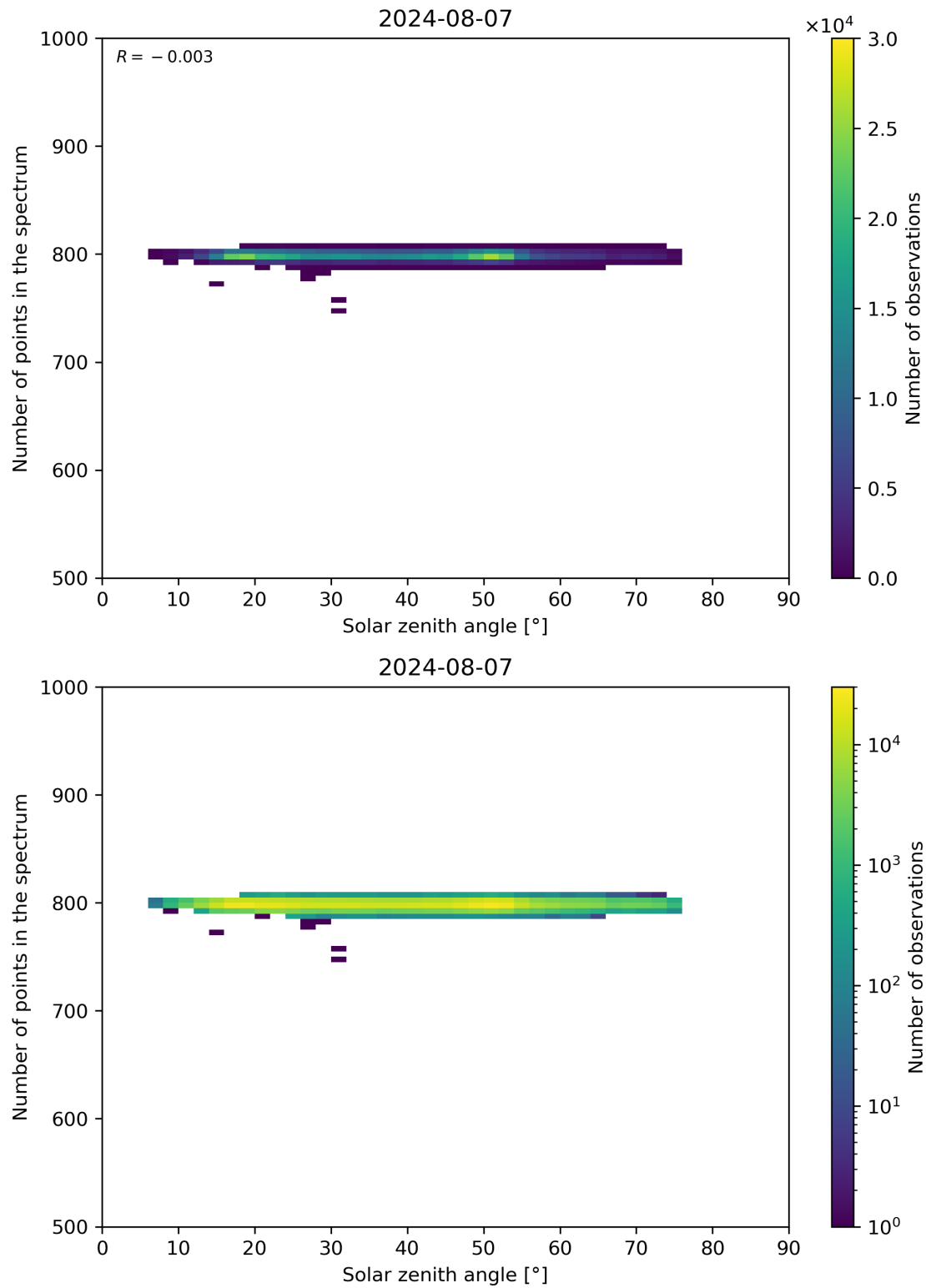
Figure 103: Scatter density plot of “Solar zenith angle” against “Number of points in the spectrum” for 2024-08-06 to 2024-08-08.
