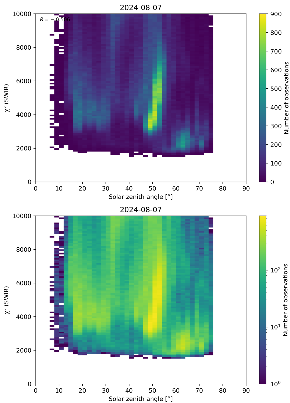
Figure 95: Scatter density plot of “Solar zenith angle” against “ \chi^2 (SWIR)” for 2024-08-06 to 2024-08-08.
