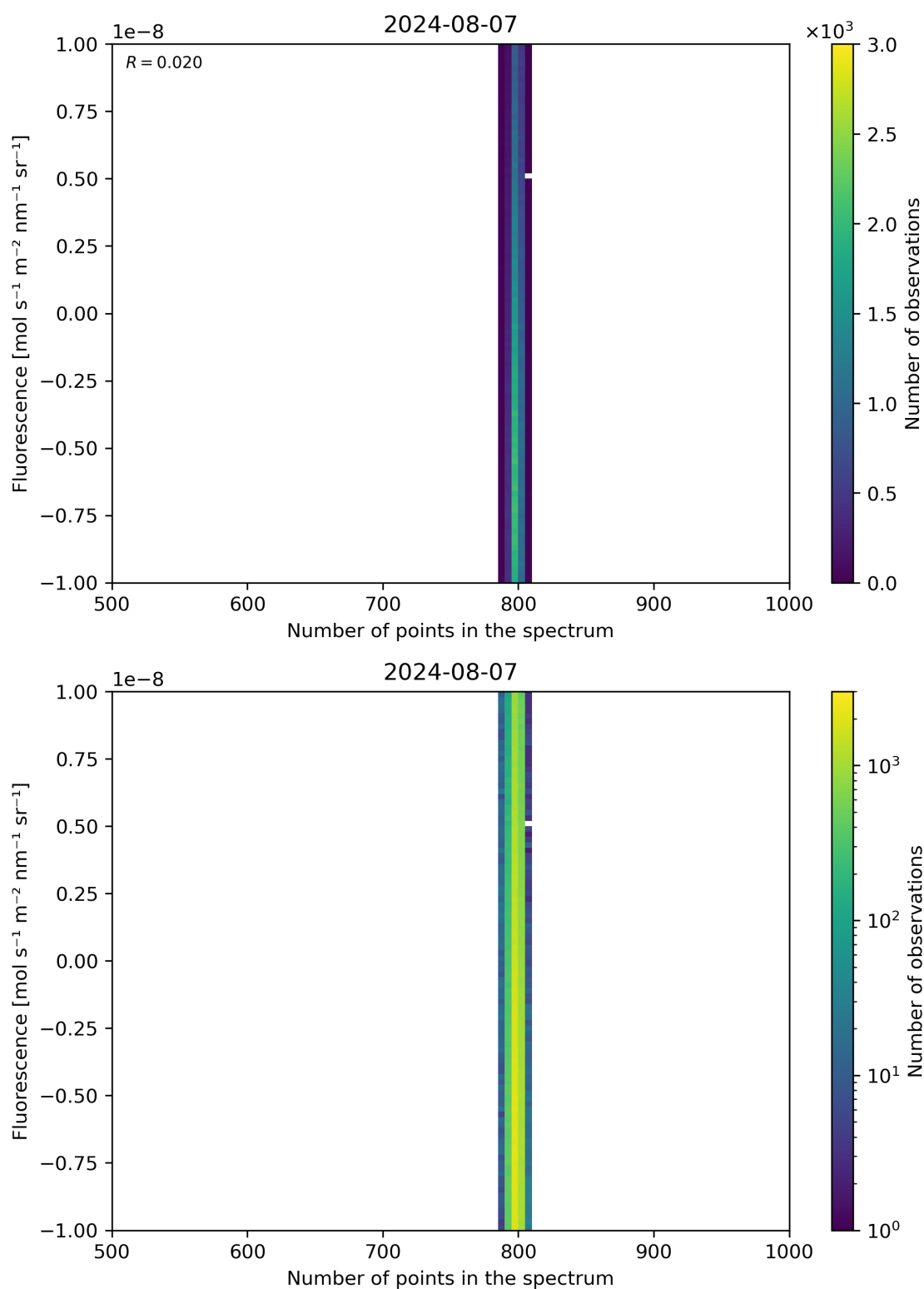
Figure 91: Scatter density plot of “Number of points in the spectrum” against “Fluorescence” for 2024-08-06 to 2024-08-08.
