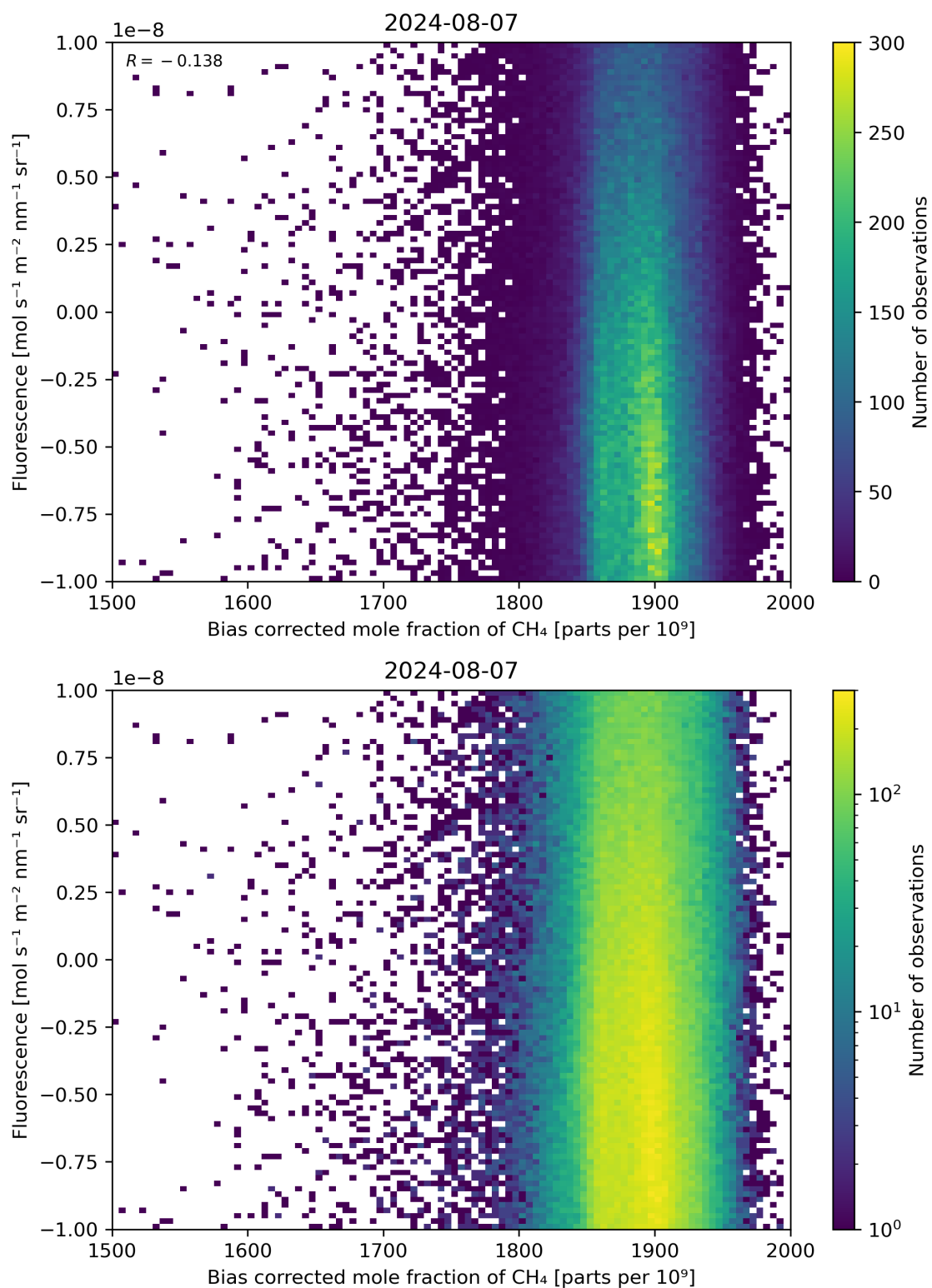
Figure 66: Scatter density plot of “Bias corrected mole fraction of \text{CH}_4 ” against “Fluorescence” for 2024-08-06 to 2024-08-08.
