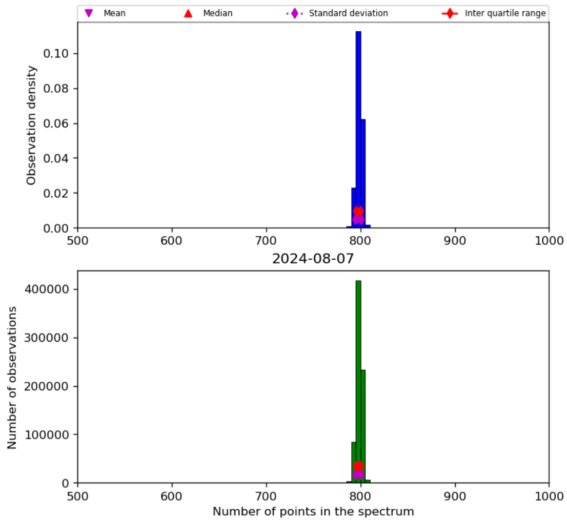
Figure 26: Histogram of “Number of points in the spectrum” for 2024-08-06 to 2024-08-08
