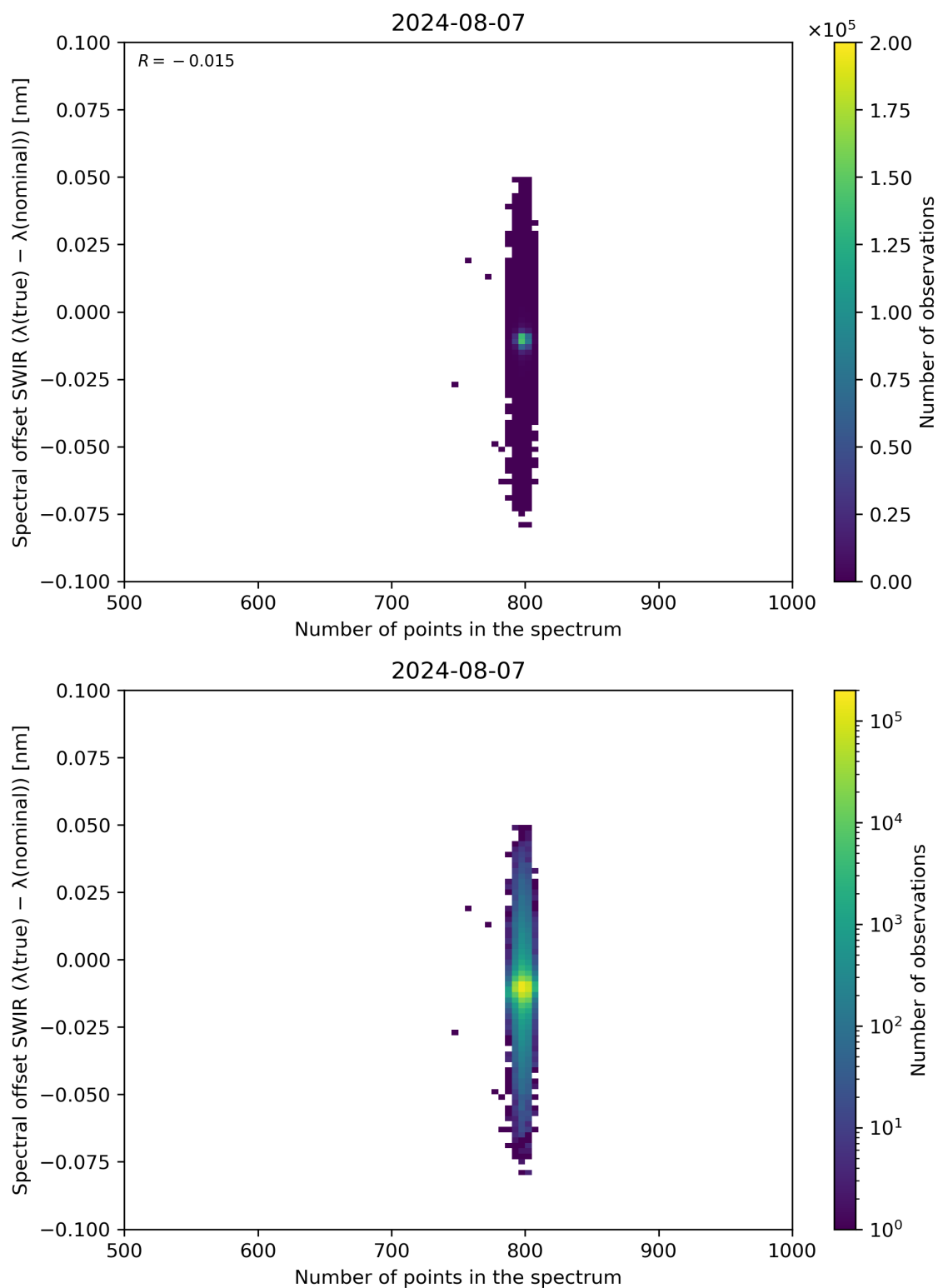
Figure 93: Scatter density plot of “Number of points in the spectrum” against “Spectral offset SWIR ( \lambda(\text{true}) - \lambda(\text{nominal}) )” for 2024-08-06 to 2024-08-08.
