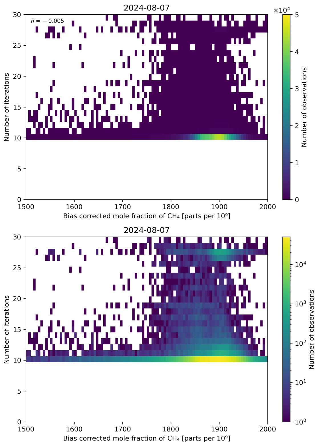
Figure 67: Scatter density plot of “Bias corrected mole fraction of CH 4 ” against “Number of iterations” for 2024-08-06 to 2024-08-08.
