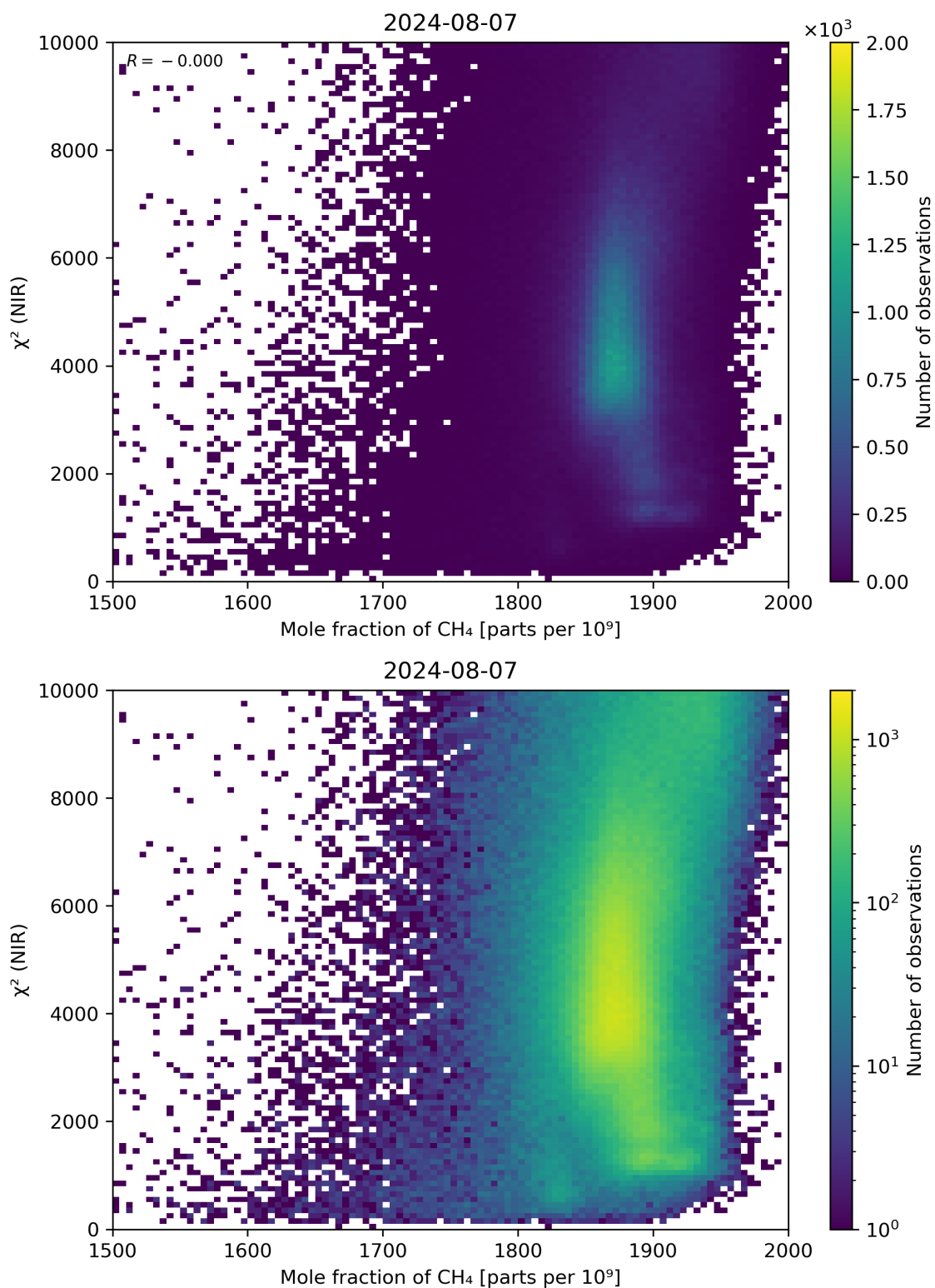
Figure 70: Scatter density plot of “Mole fraction of \text{CH}_4 ” against “ \chi^2 (NIR)” for 2024-08-06 to 2024-08-08.
