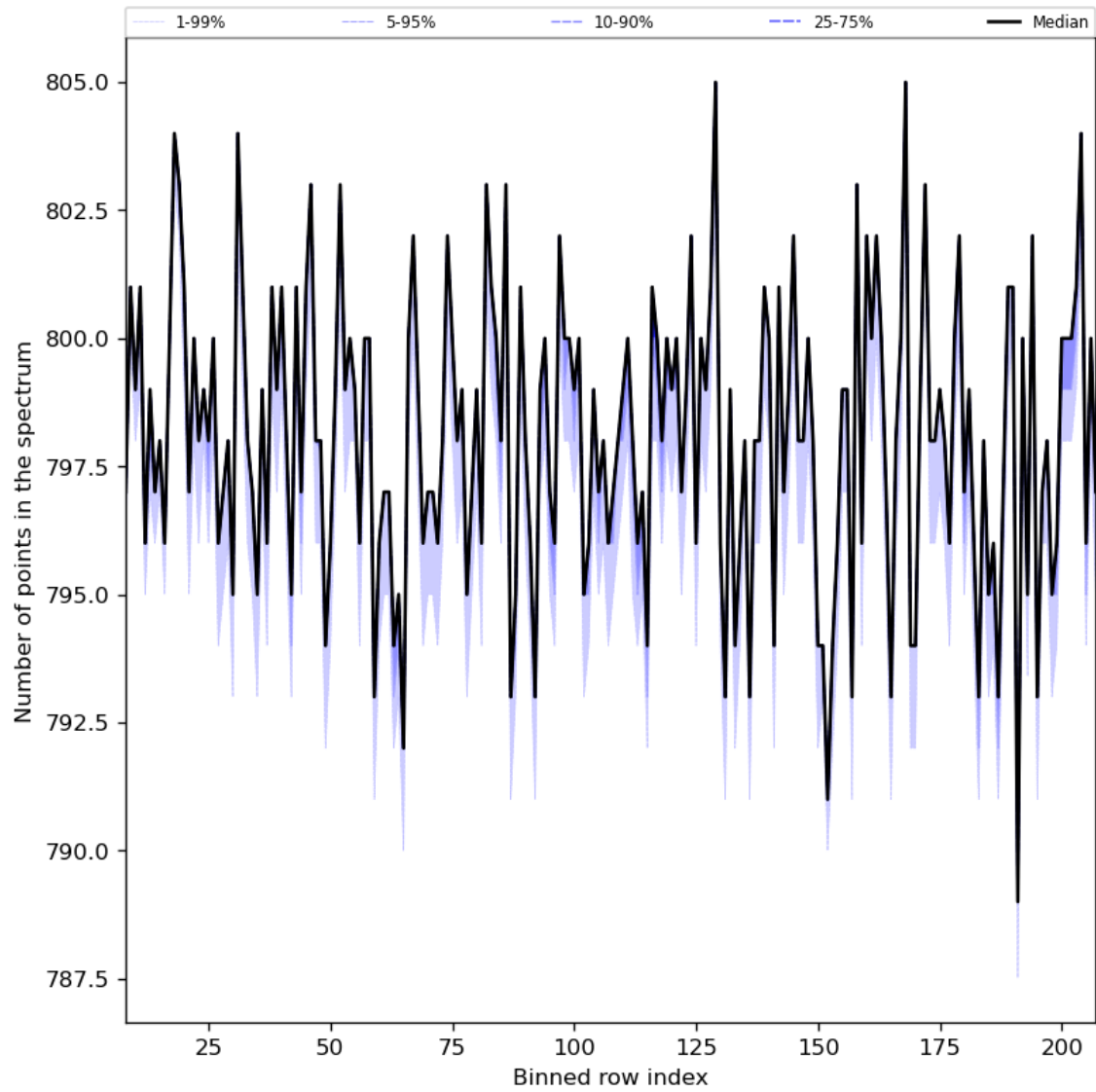
Figure 37: Along track statistics of “Number of points in the spectrum” for 2024-08-06 to 2024-08-08
