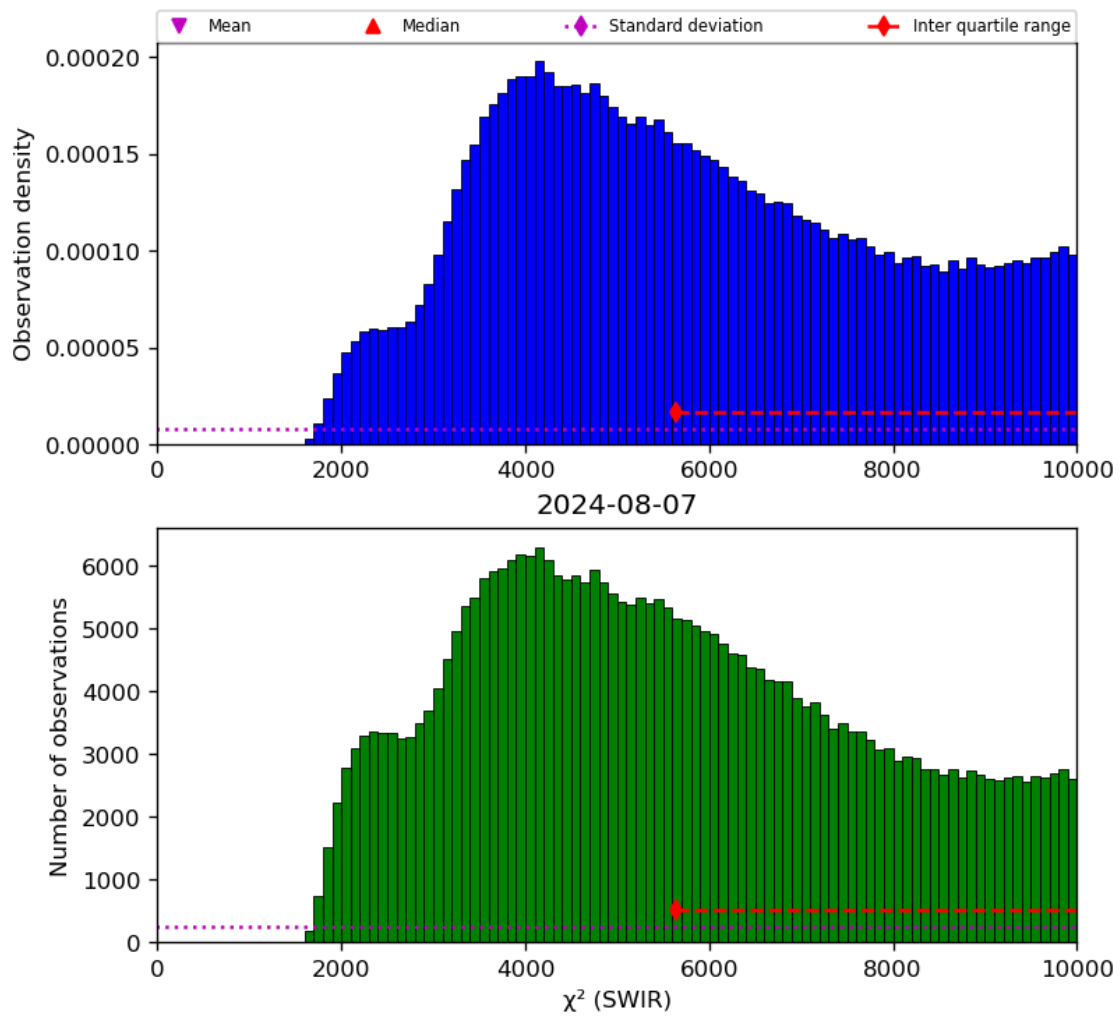
Figure 28: Histogram of “ \chi^2 (SWIR)” for 2024-08-06 to 2024-08-08
