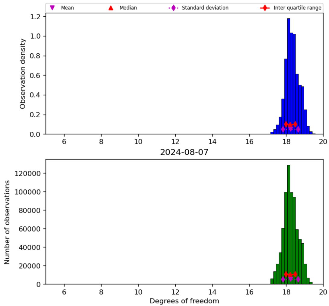
Figure 30: Histogram of “Degrees of freedom” for 2024-08-06 to 2024-08-08
