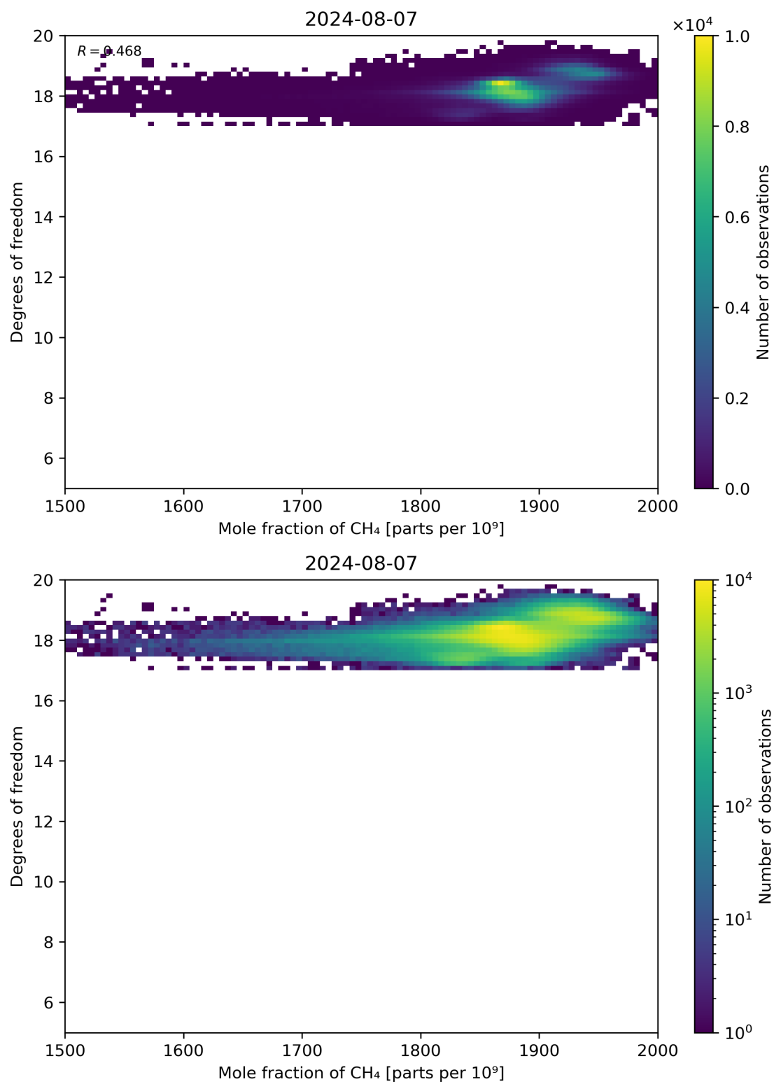
Figure 72: Scatter density plot of “Mole fraction of CH 4 ” against “Degrees of freedom” for 2024-08-06 to 2024-08-08.
