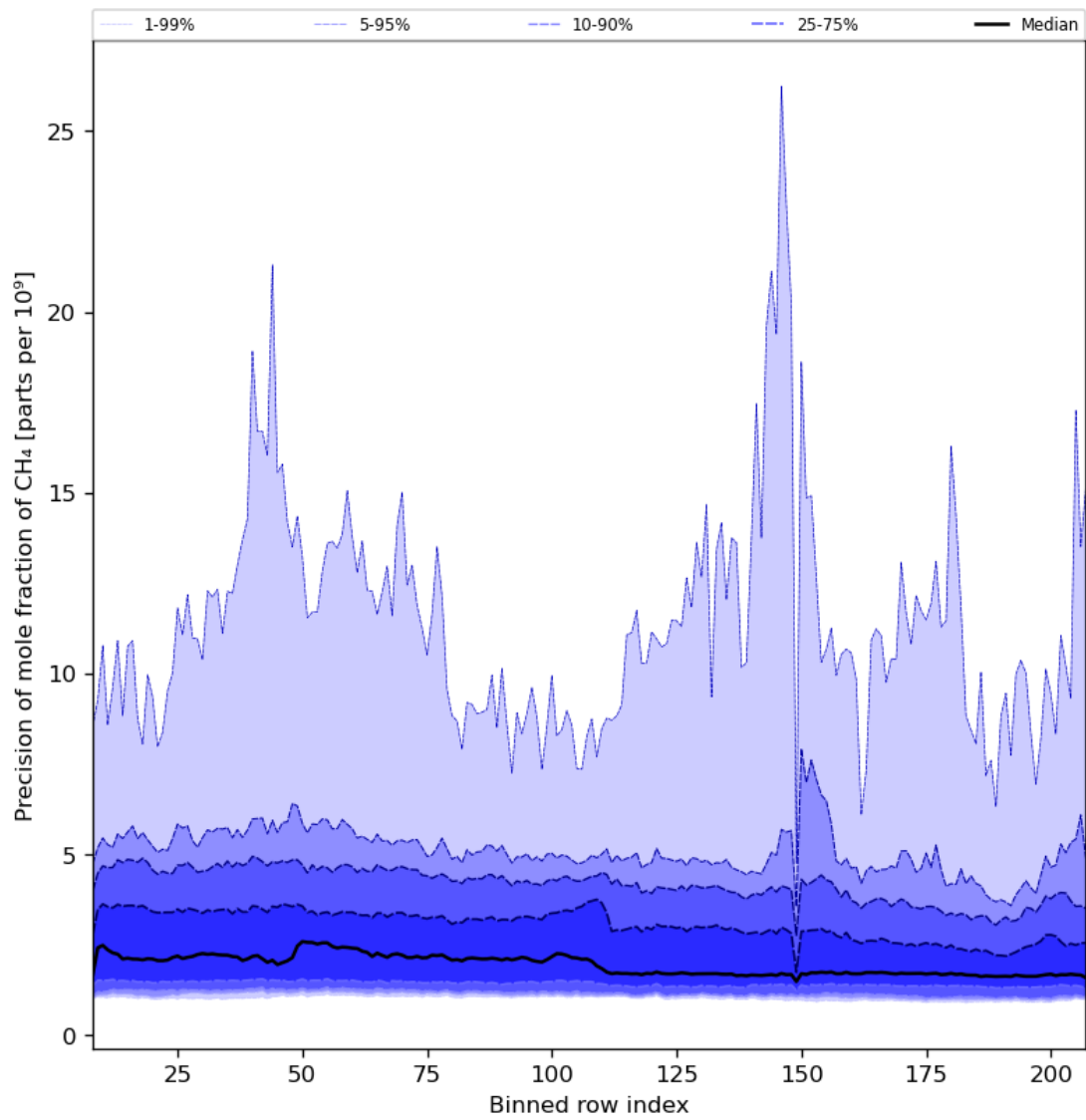
Figure 35: Along track statistics of “Precision of mole fraction of CH 4 ” for 2024-08-06 to 2024-08-08
