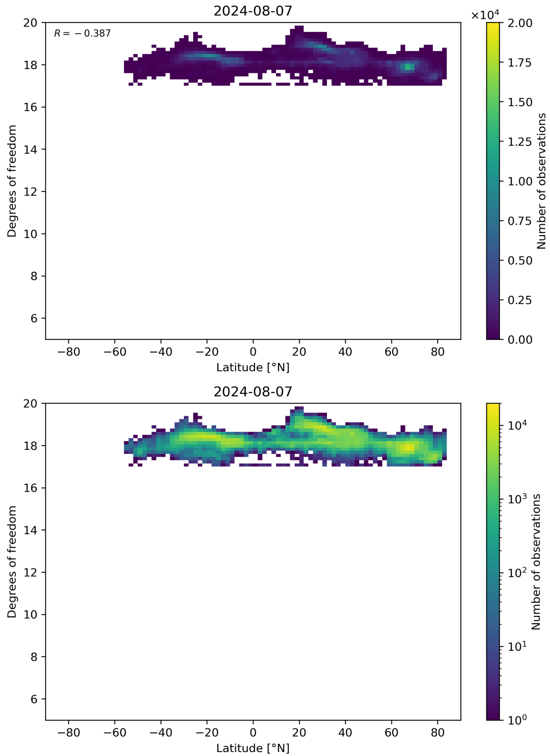
Figure 55: Scatter density plot of “Latitude” against “Degrees of freedom” for 2024-08-06 to 2024-08-08.
