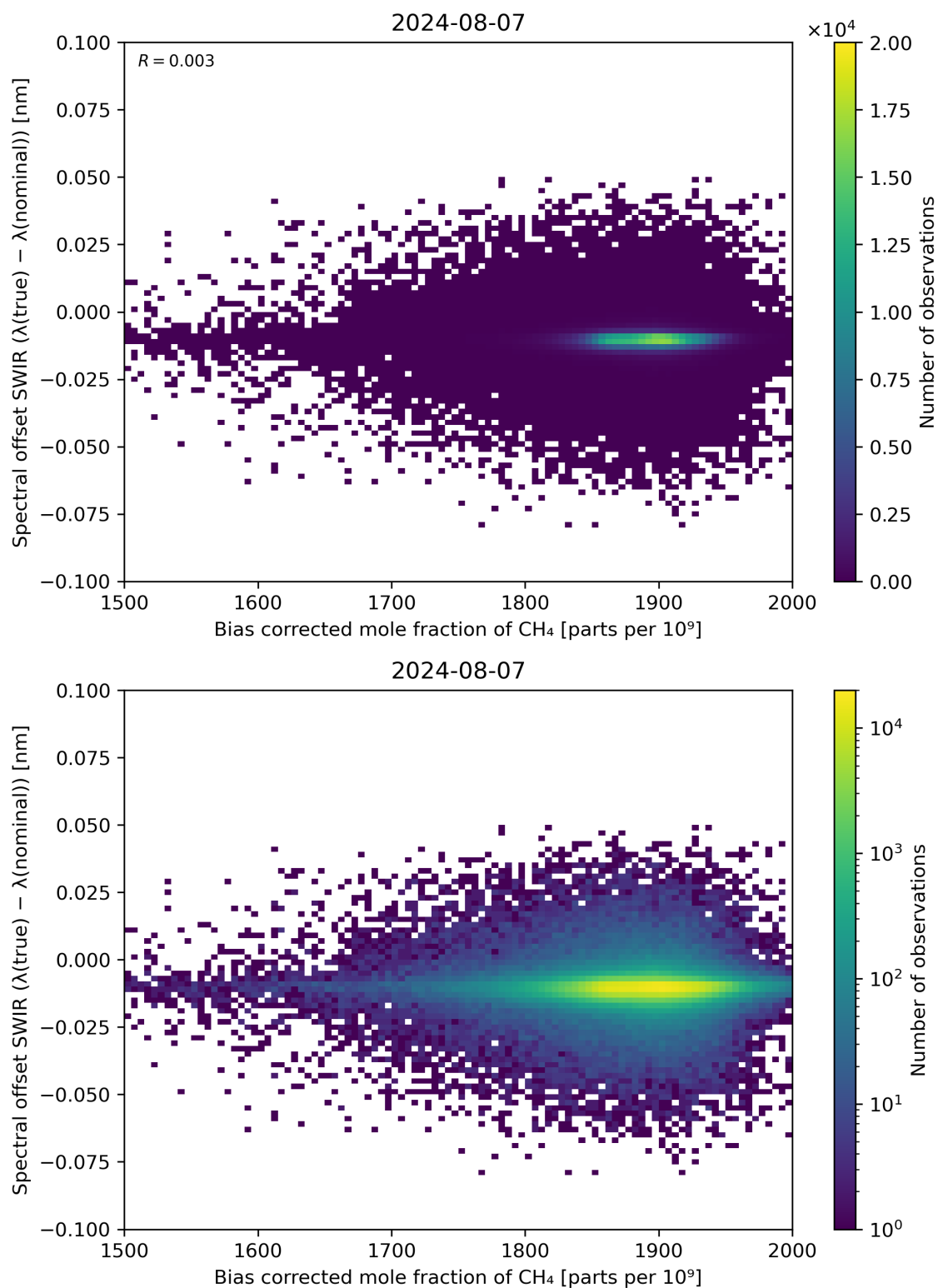
Figure 69: Scatter density plot of “Bias corrected mole fraction of \text{CH}_4 ” against “Spectral offset SWIR ( \lambda(\text{true}) - \lambda(\text{nominal}) )” for 2024-08-06 to 2024-08-08.
