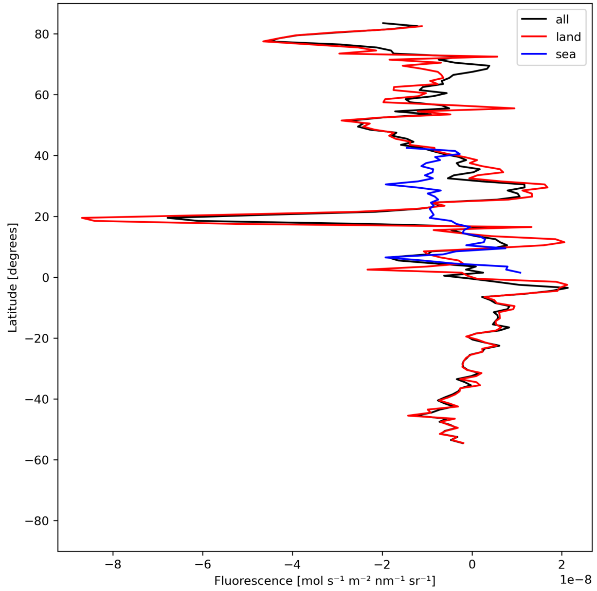
Figure 21: Zonal average of “Fluorescence” for 2024-08-06 to 2024-08-08.
