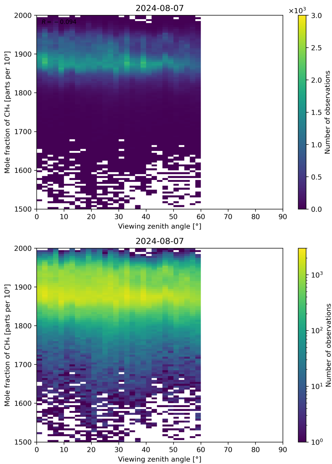
Figure 110: Scatter density plot of “Viewing zenith angle” against “Mole fraction of CH 4 ” for 2024-08-06 to 2024-08-08.
