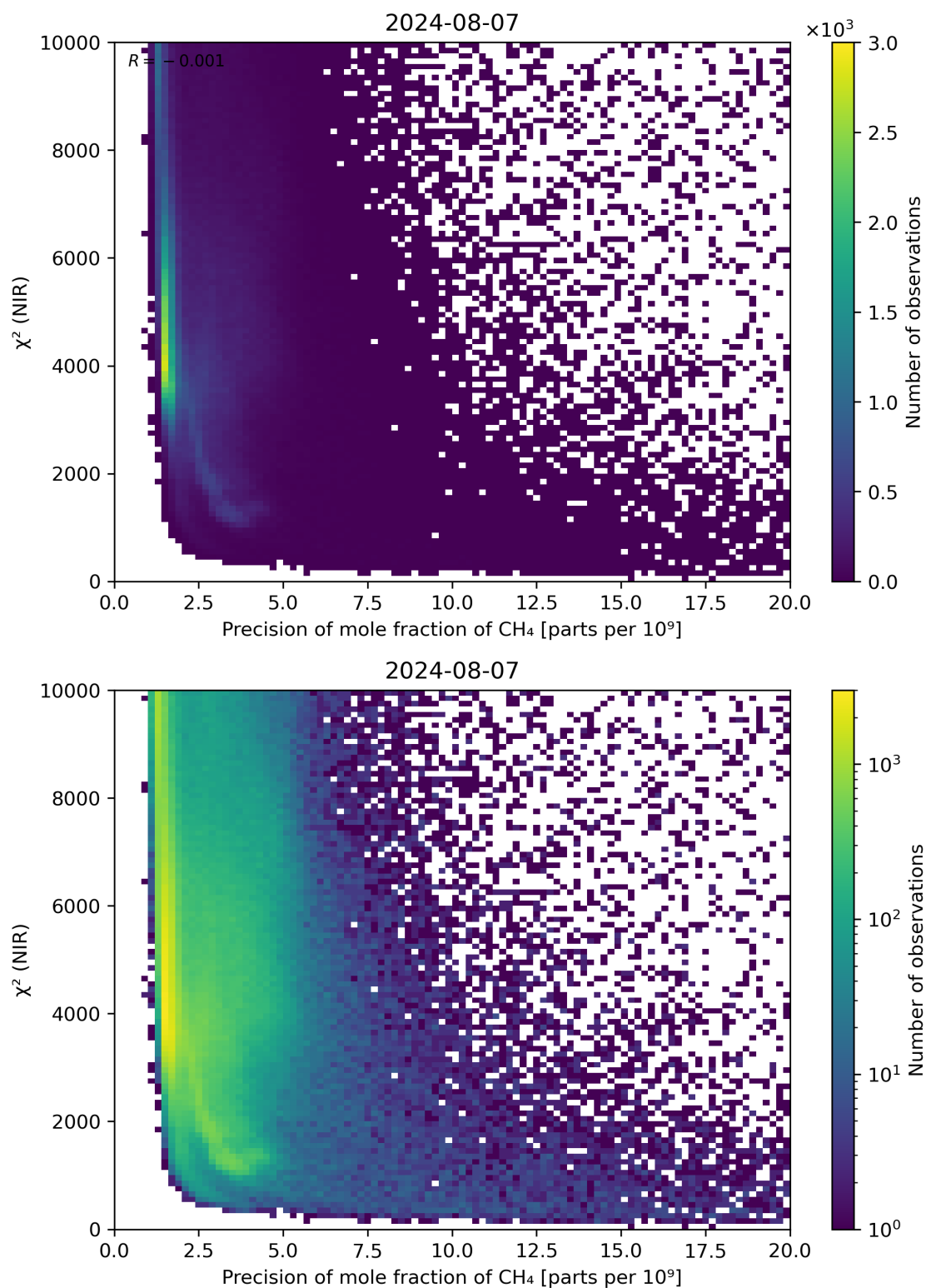
Figure 78: Scatter density plot of “Precision of mole fraction of CH 4 ” against “ \chi^2 (NIR)” for 2024-08-06 to 2024-08-08.
