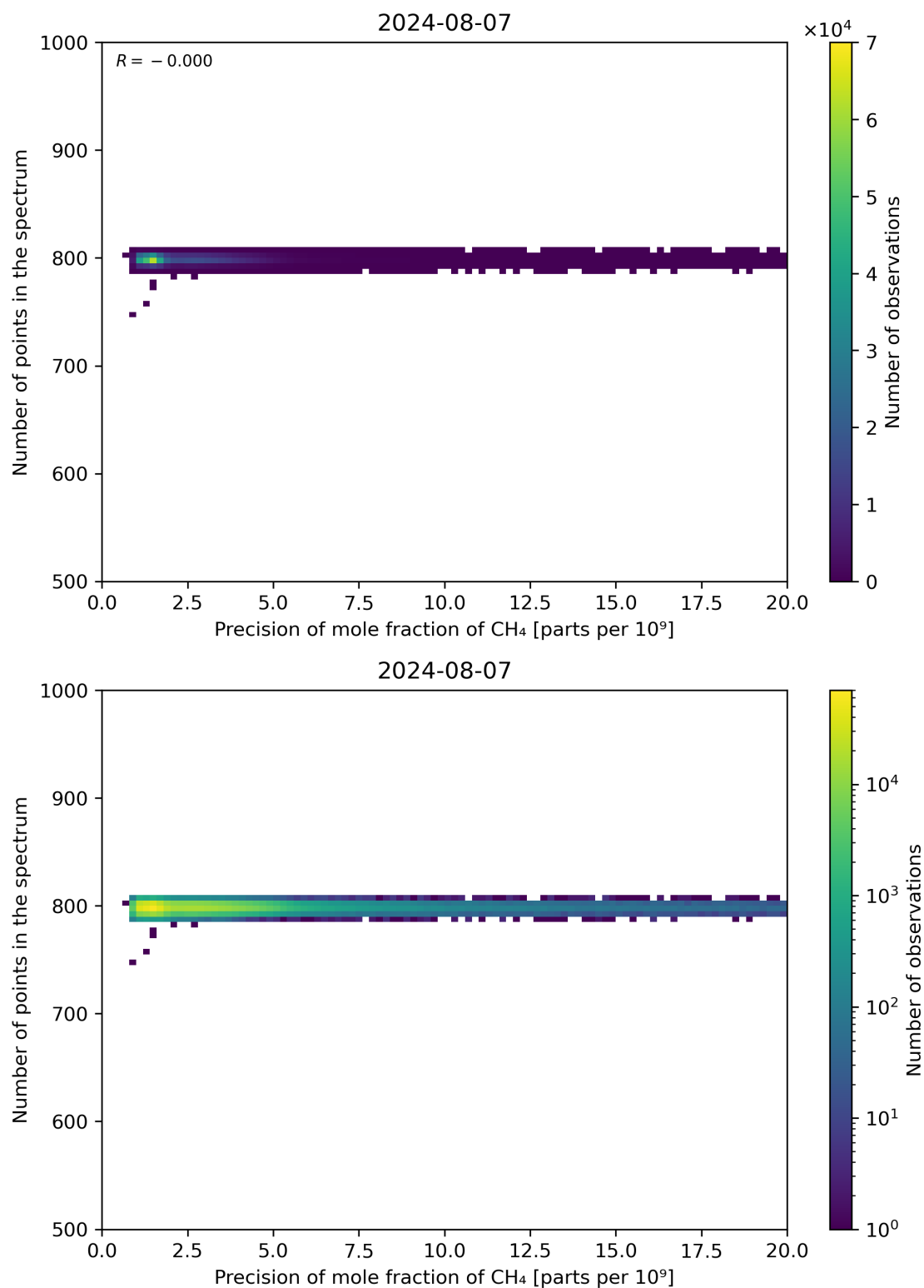
Figure 84: Scatter density plot of “Precision of mole fraction of CH 4 ” against “Number of points in the spectrum” for 2024-08-06 to 2024-08-08.
