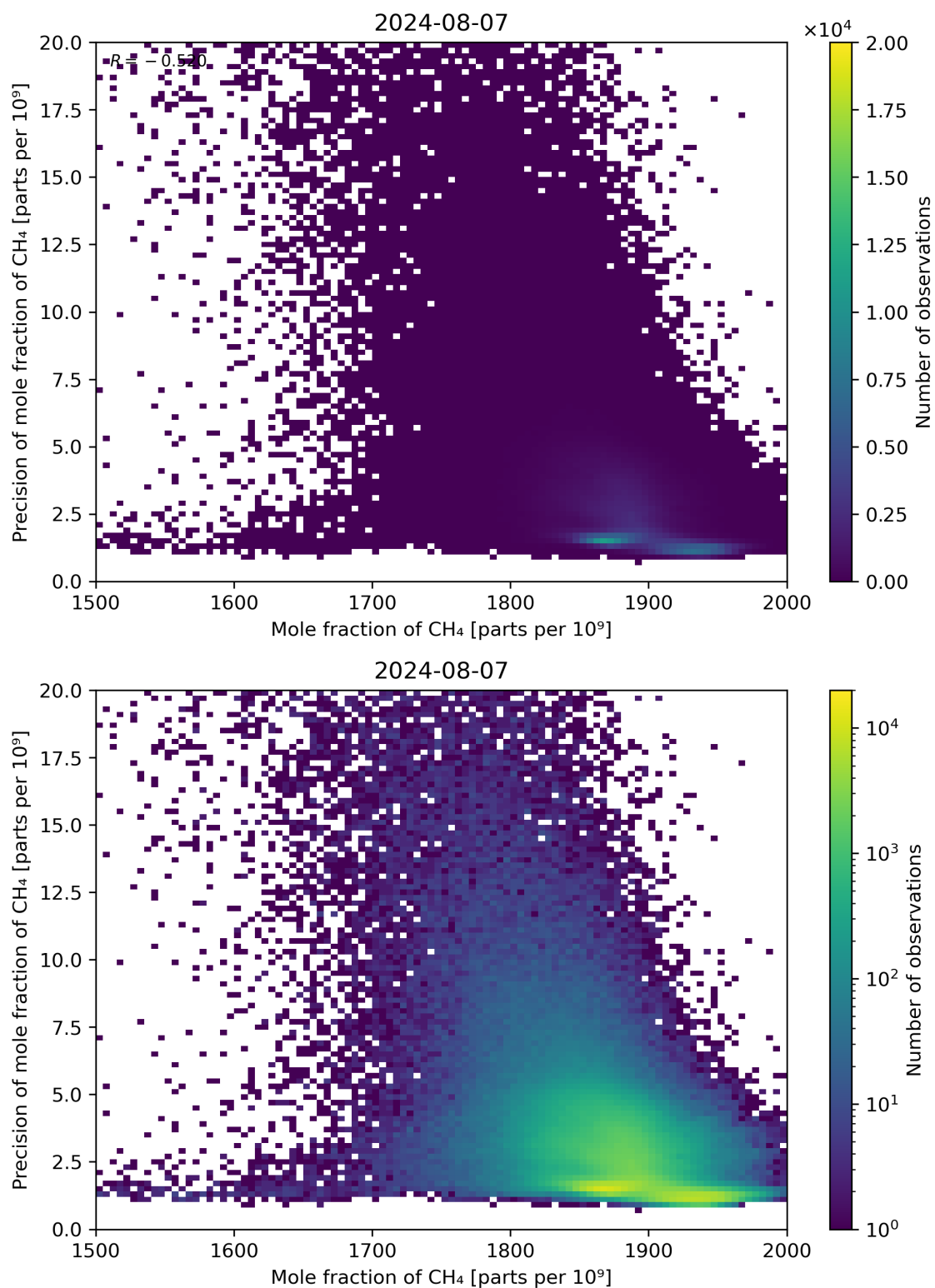
Figure 75: Scatter density plot of “Mole fraction of CH 4 ” against “Precision of mole fraction of CH 4 ” for 2024-08-06 to 2024-08-08.
