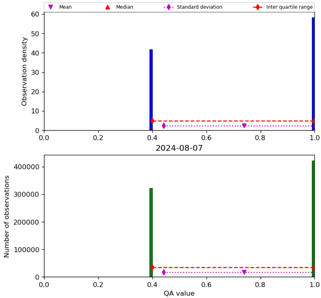
Figure 22: Histogram of “QA value” for 2024-08-06 to 2024-08-08
