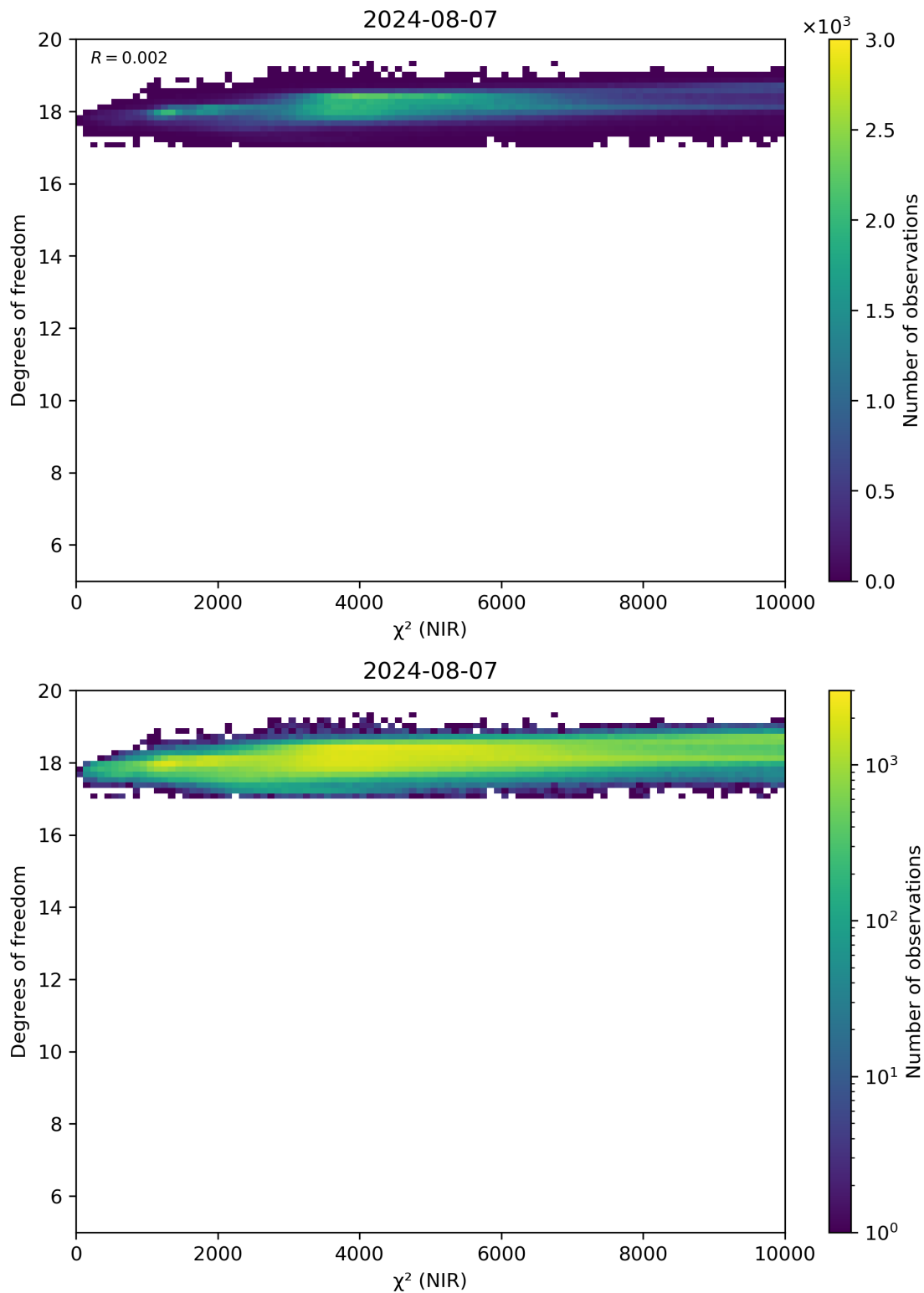
Figure 44: Scatter density plot of “ \chi^2 (NIR)” against “Degrees of freedom” for 2024-08-06 to 2024-08-08.
