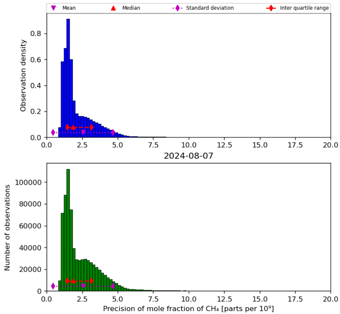
Figure 24: Histogram of “Precision of mole fraction of CH 4 ” for 2024-08-06 to 2024-08-08
