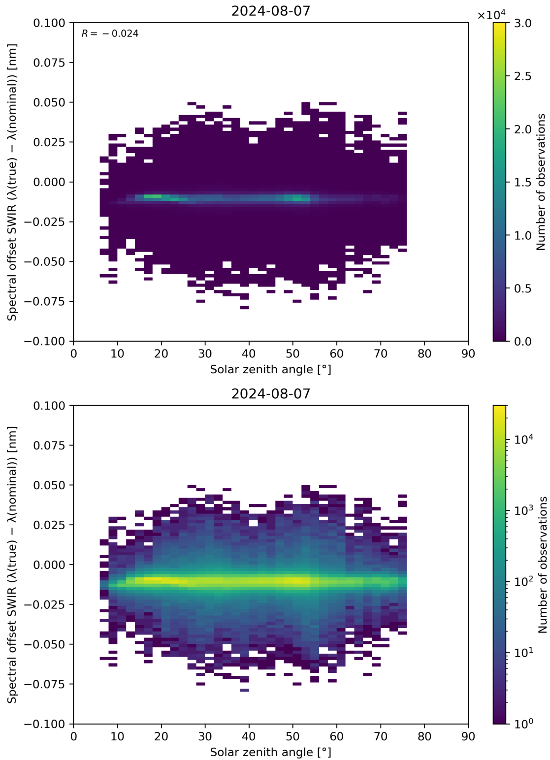
Figure 104: Scatter density plot of “Solar zenith angle” against “Spectral offset SWIR ( \lambda(\text{true}) - \lambda(\text{nominal}) )” for 2024-08-06 to 2024-08-08.
