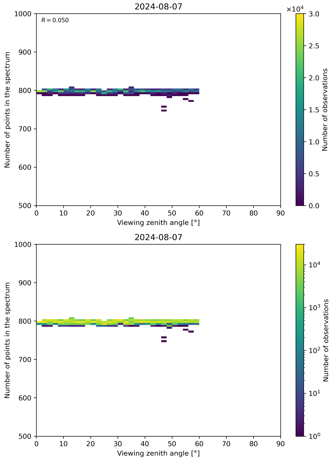
Figure 114: Scatter density plot of “Viewing zenith angle” against “Number of points in the spectrum” for 2024-08-06 to 2024-08-08.
