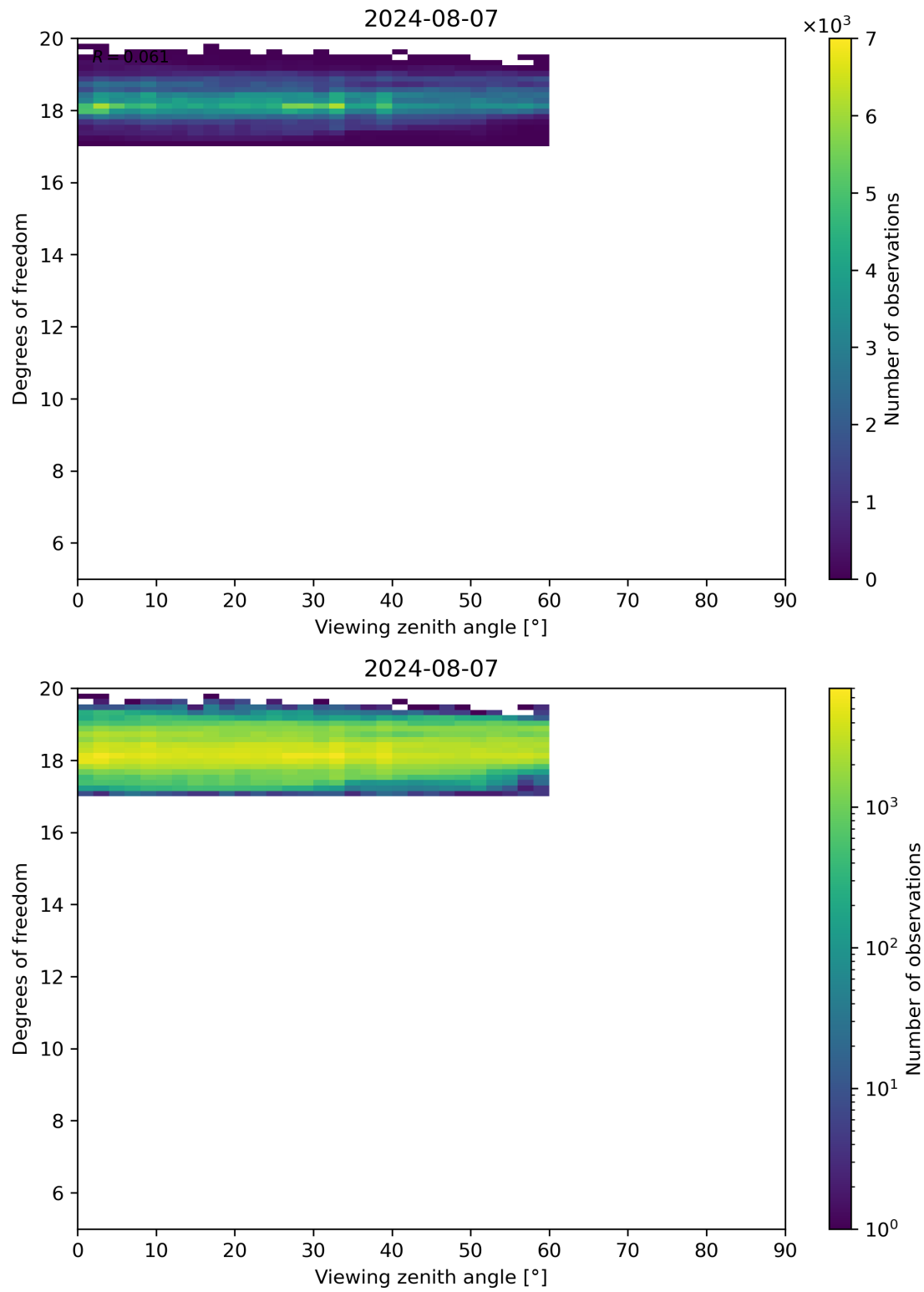
Figure 107: Scatter density plot of “Viewing zenith angle” against “Degrees of freedom” for 2024-08-06 to 2024-08-08.
