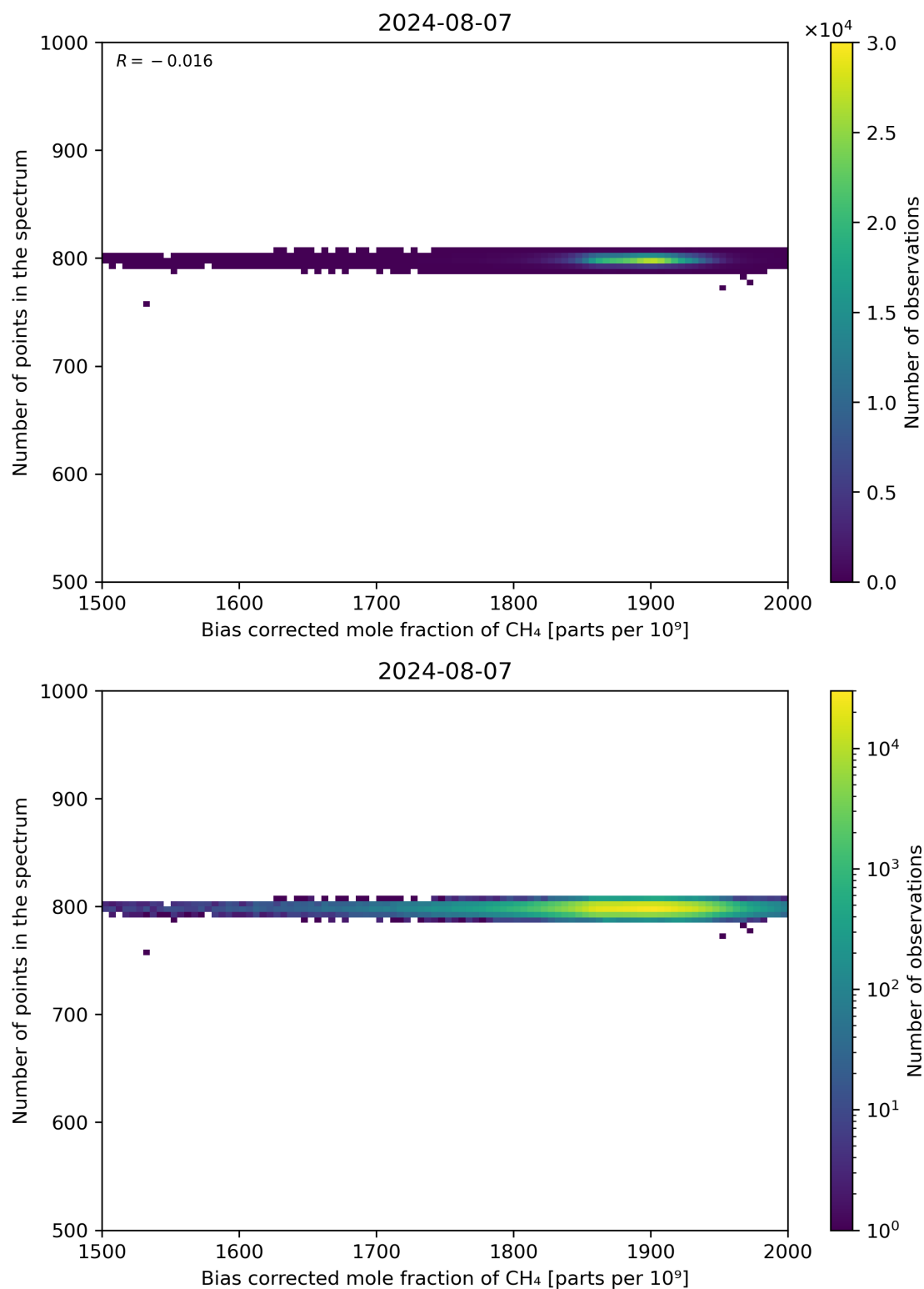
Figure 68: Scatter density plot of “Bias corrected mole fraction of CH 4 ” against “Number of points in the spectrum” for 2024-08-06 to 2024-08-08.
