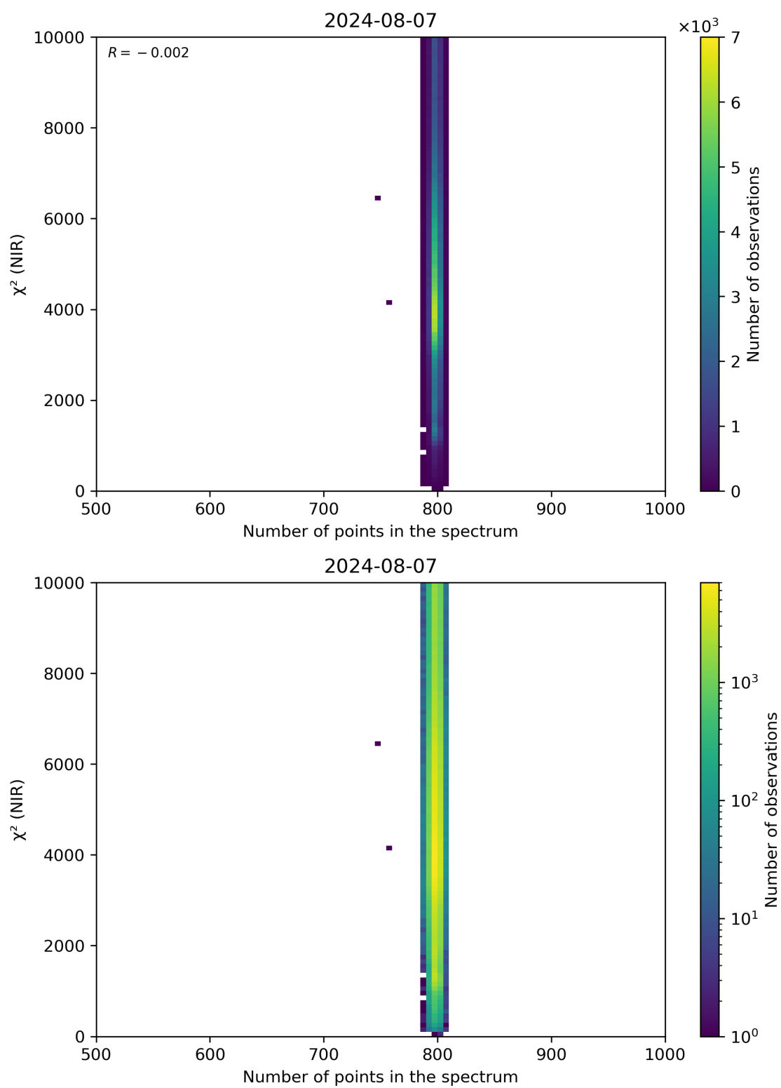
Figure 88: Scatter density plot of “Number of points in the spectrum” against “ \chi^2 (NIR)” for 2024-08-06 to 2024-08-08.
