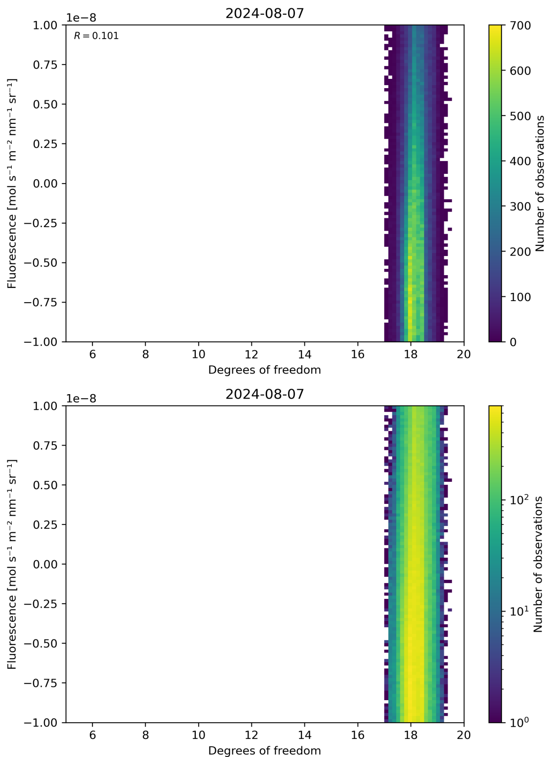
Figure 51: Scatter density plot of “Degrees of freedom” against “Fluorescence” for 2024-08-06 to 2024-08-08.
