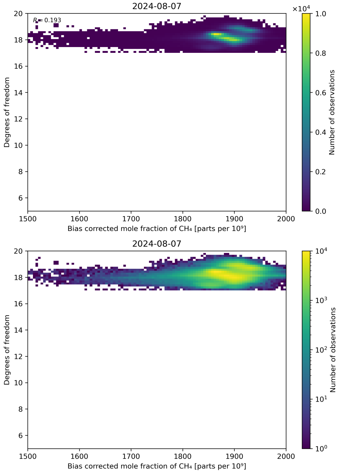
Figure 65: Scatter density plot of “Bias corrected mole fraction of CH 4 ” against “Degrees of freedom” for 2024-08-06 to 2024-08-08.
