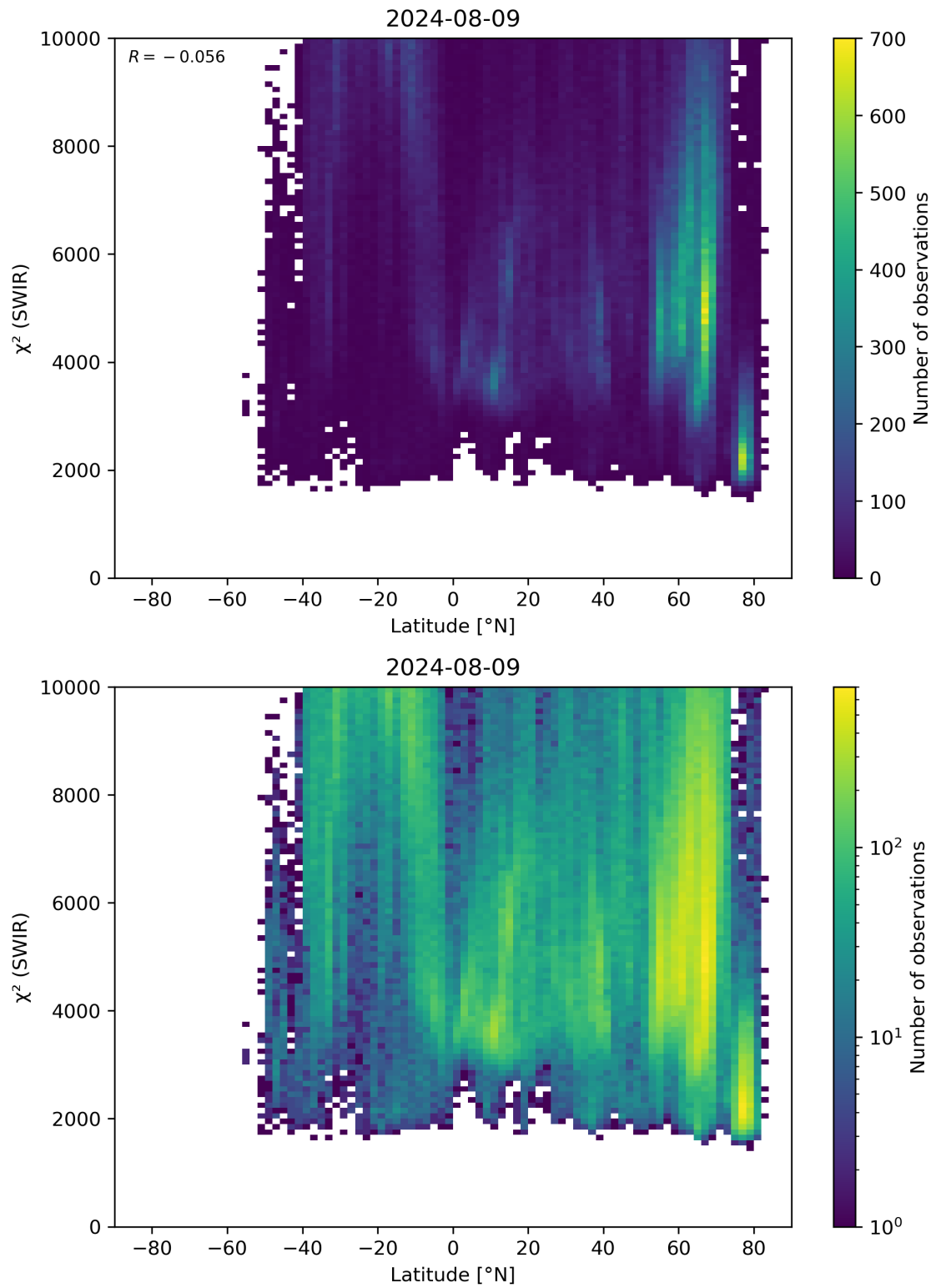
Figure 54: Scatter density plot of “Latitude” against “ \chi^2 (SWIR)” for 2024-08-08 to 2024-08-10.
