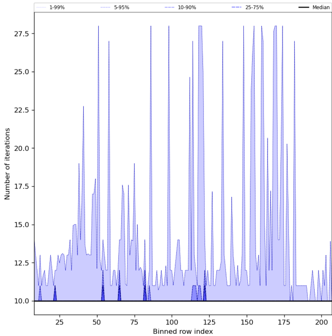
Figure 42: Along track statistics of “Number of iterations” for 2024-08-08 to 2024-08-10
