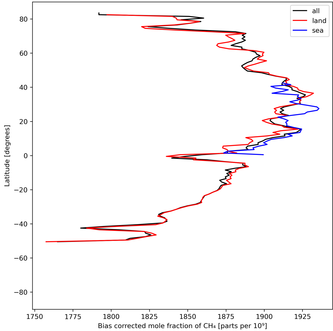
Figure 14: Zonal average of “Bias corrected mole fraction of \text{CH}_4 ” for 2024-08-08 to 2024-08-10.
