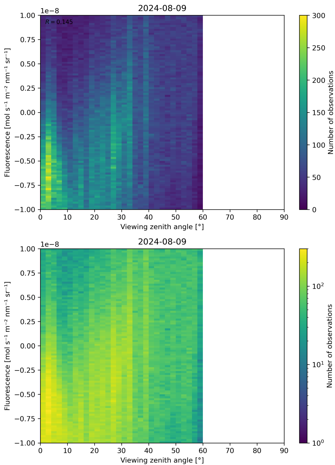
Figure 108: Scatter density plot of “Viewing zenith angle” against “Fluorescence” for 2024-08-08 to 2024-08-10.
