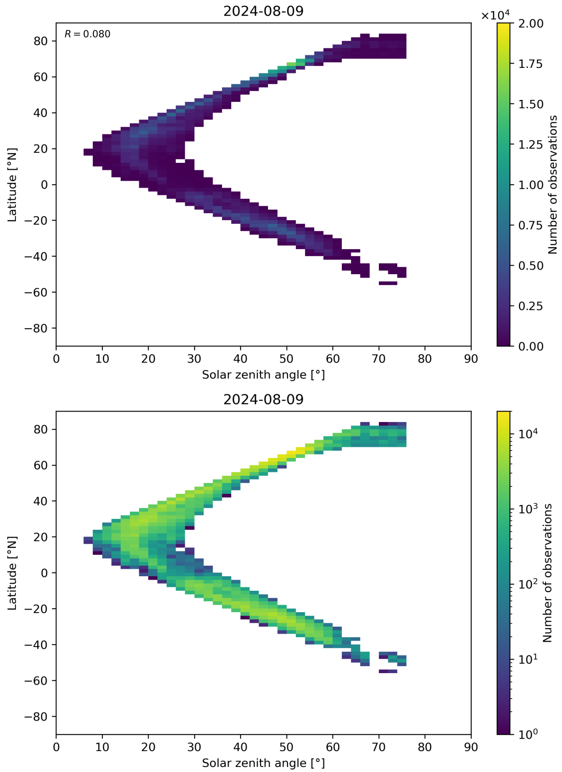
Figure 98: Scatter density plot of “Solar zenith angle” against “Latitude” for 2024-08-08 to 2024-08-10.
