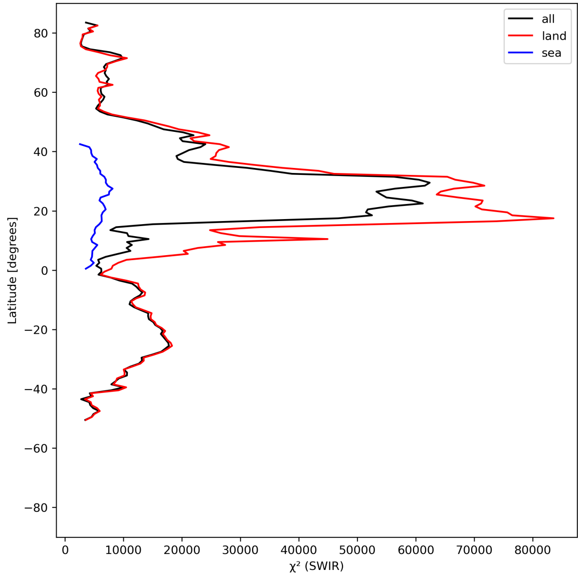
Figure 17: Zonal average of “ \chi^2 (SWIR)” for 2024-08-08 to 2024-08-10.
