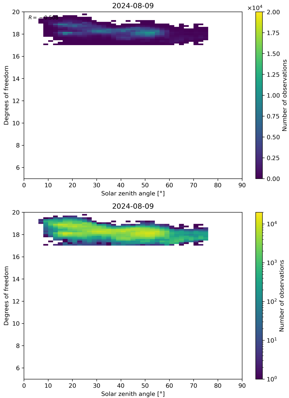
Figure 96: Scatter density plot of “Solar zenith angle” against “Degrees of freedom” for 2024-08-08 to 2024-08-10.
