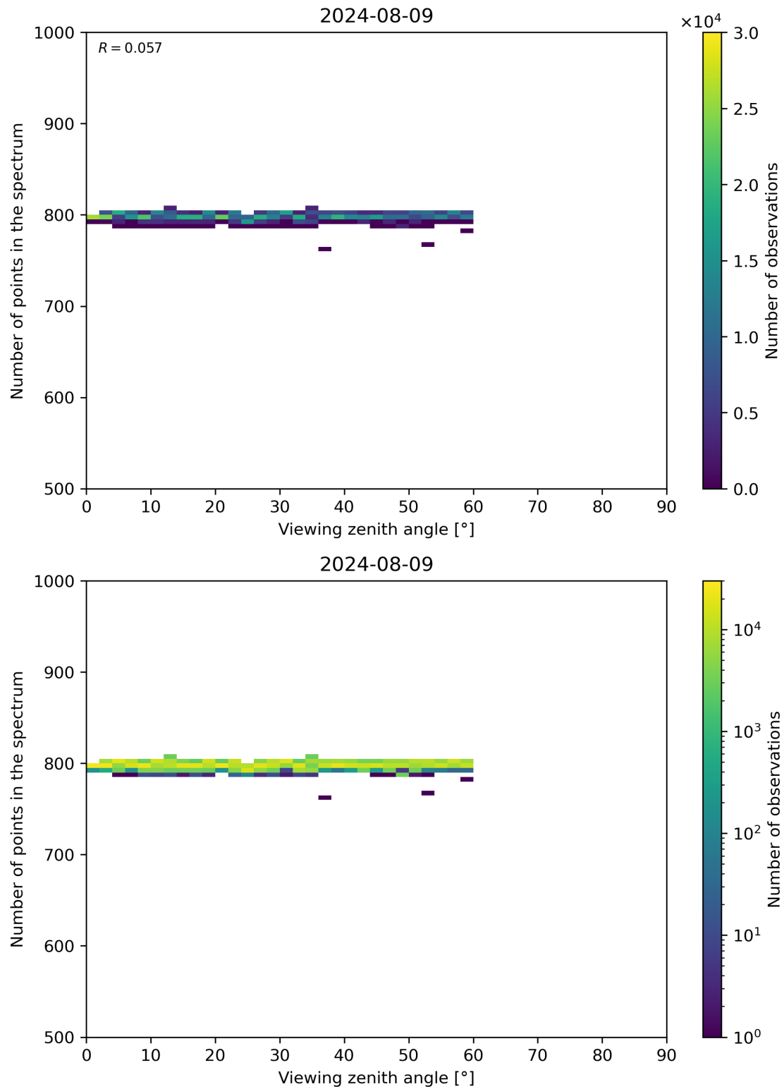
Figure 114: Scatter density plot of “Viewing zenith angle” against “Number of points in the spectrum” for 2024-08-08 to 2024-08-10.
