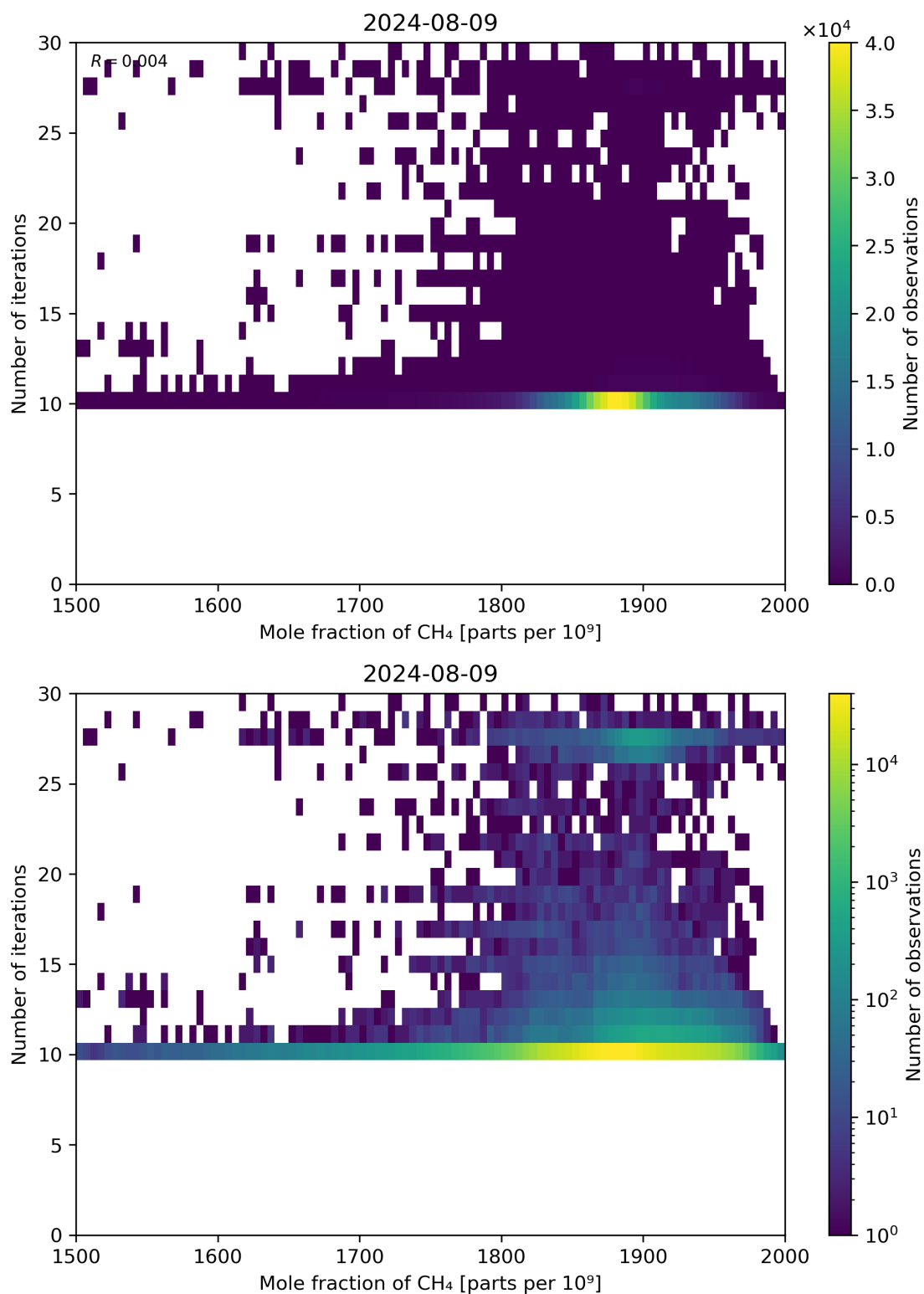
Figure 76: Scatter density plot of “Mole fraction of CH 4 ” against “Number of iterations” for 2024-08-08 to 2024-08-10.
