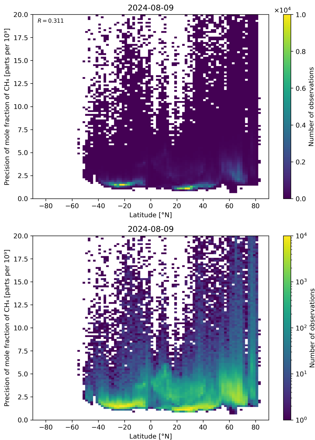
Figure 59: Scatter density plot of “Latitude” against “Precision of mole fraction of \text{CH}_4 ” for 2024-08-08 to 2024-08-10.
