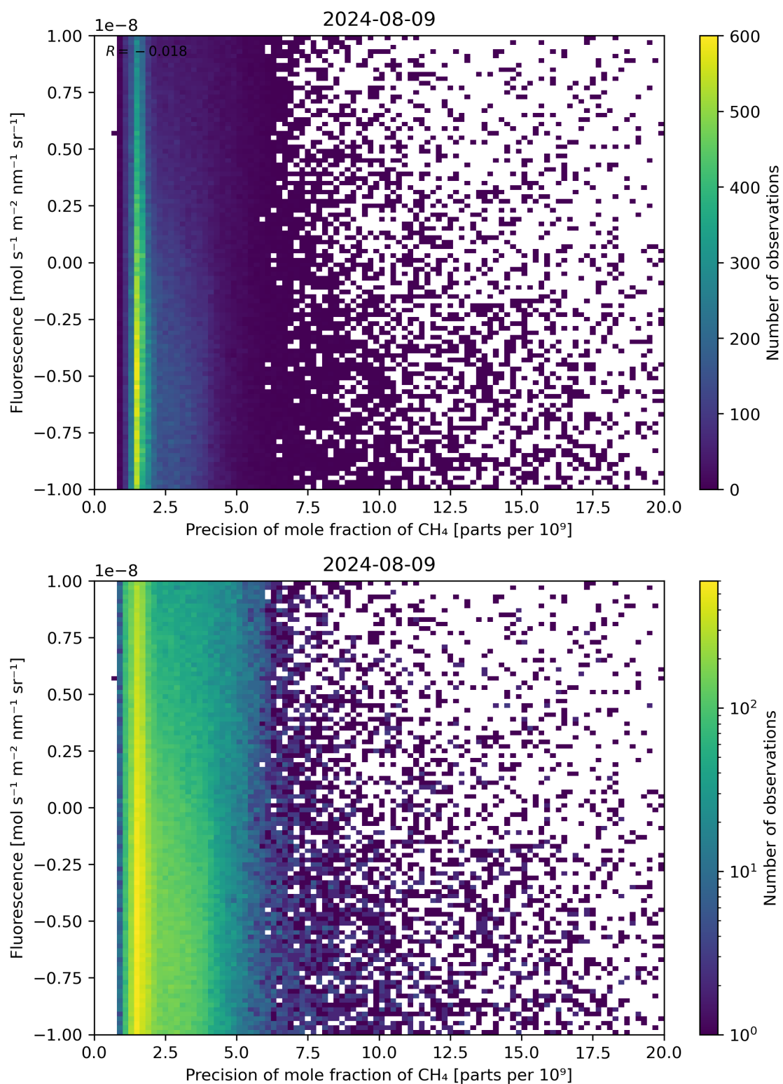
Figure 81: Scatter density plot of “Precision of mole fraction of \text{CH}_4 ” against “Fluorescence” for 2024-08-08 to 2024-08-10.
