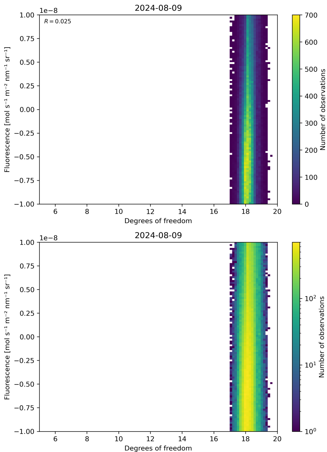
Figure 51: Scatter density plot of “Degrees of freedom” against “Fluorescence” for 2024-08-08 to 2024-08-10.
