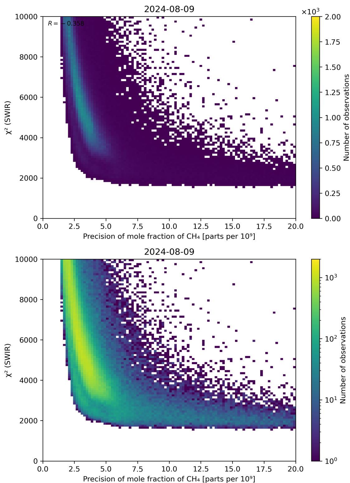
Figure 79: Scatter density plot of “Precision of mole fraction of CH 4 ” against “ \chi^2 (SWIR)” for 2024-08-08 to 2024-08-10.
