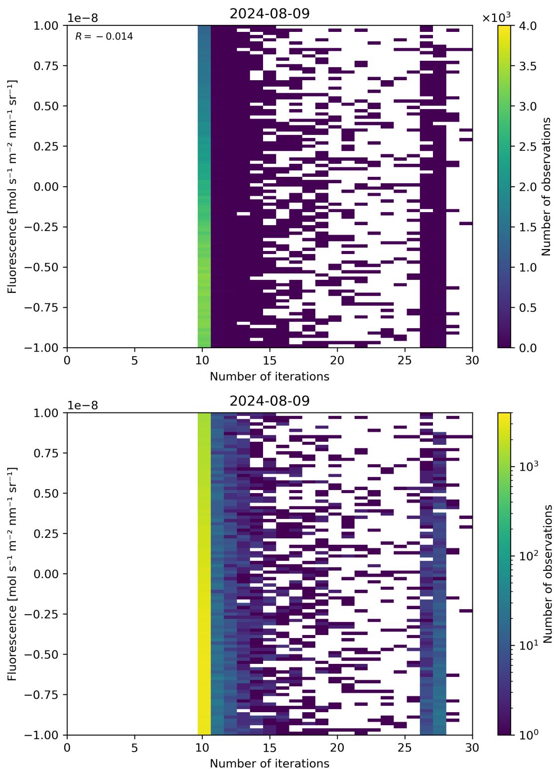
Figure 87: Scatter density plot of “Number of iterations” against “Fluorescence” for 2024-08-08 to 2024-08-10.
