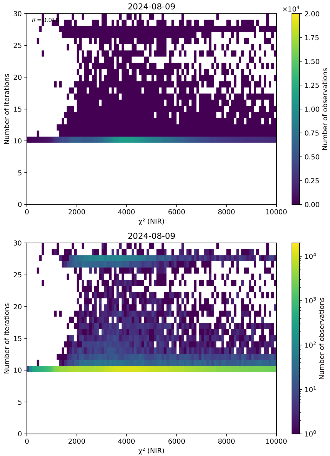
Figure 46: Scatter density plot of “ \chi^2 (NIR)” against “Number of iterations” for 2024-08-08 to 2024-08-10.
