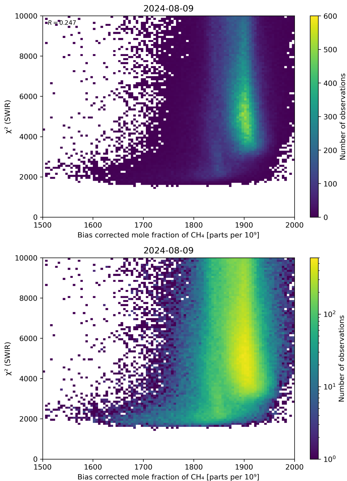
Figure 64: Scatter density plot of “Bias corrected mole fraction of CH 4 ” against “ \chi^2 (SWIR)” for 2024-08-08 to 2024-08-10.
