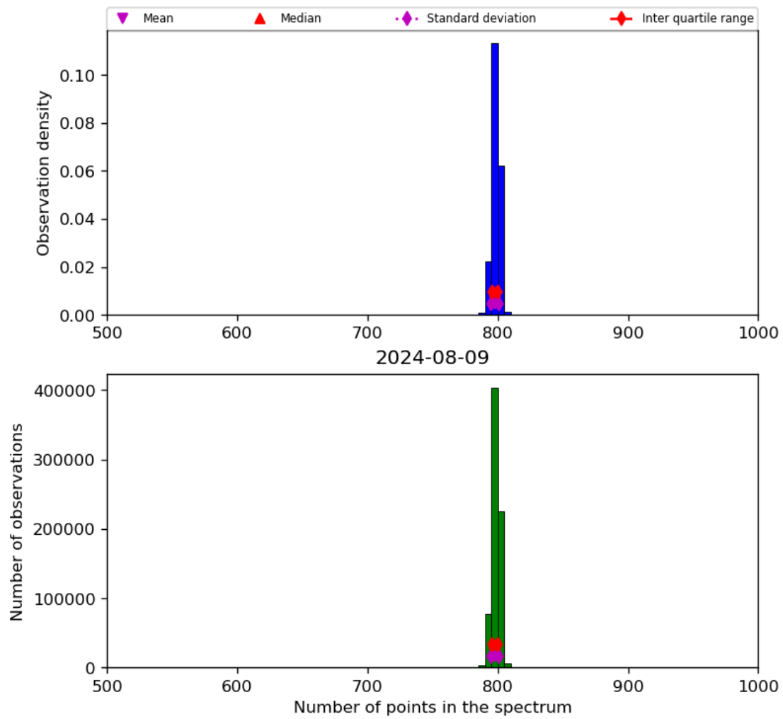
Figure 26: Histogram of “Number of points in the spectrum” for 2024-08-08 to 2024-08-10
