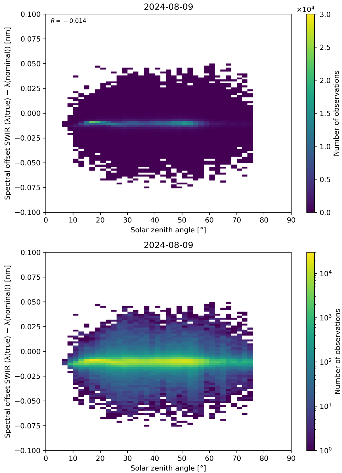
Figure 104: Scatter density plot of “Solar zenith angle” against “Spectral offset SWIR ( \lambda(\text{true}) - \lambda(\text{nominal}) )” for 2024-08-08 to 2024-08-10.
