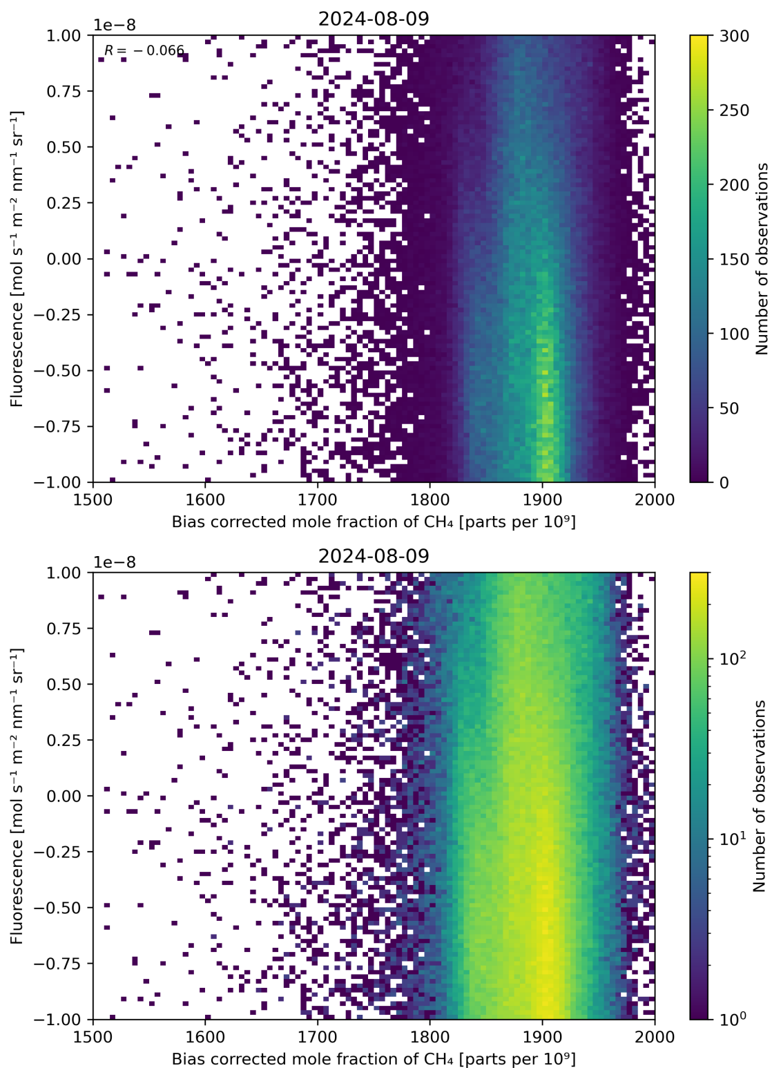
Figure 66: Scatter density plot of “Bias corrected mole fraction of \text{CH}_4 ” against “Fluorescence” for 2024-08-08 to 2024-08-10.
