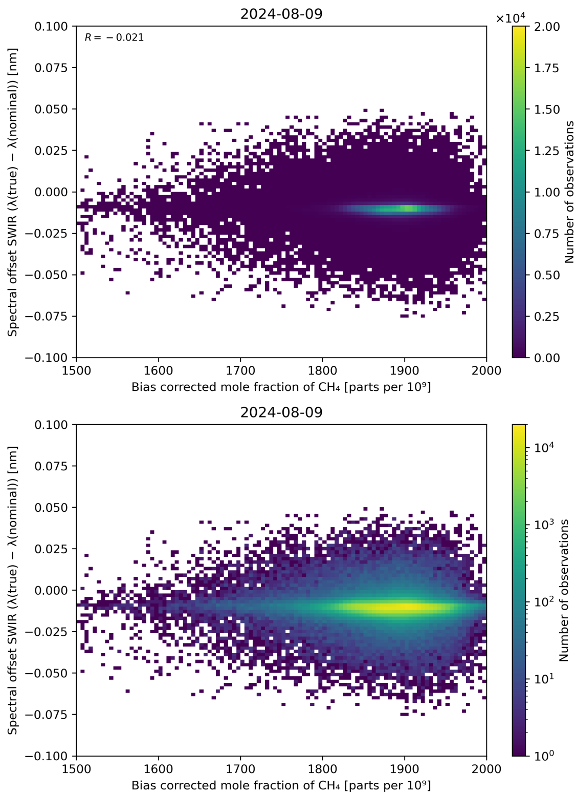
Figure 69: Scatter density plot of “Bias corrected mole fraction of \text{CH}_4 ” against “Spectral offset SWIR ( \lambda(\text{true}) - \lambda(\text{nominal}) )” for 2024-08-08 to 2024-08-10.
