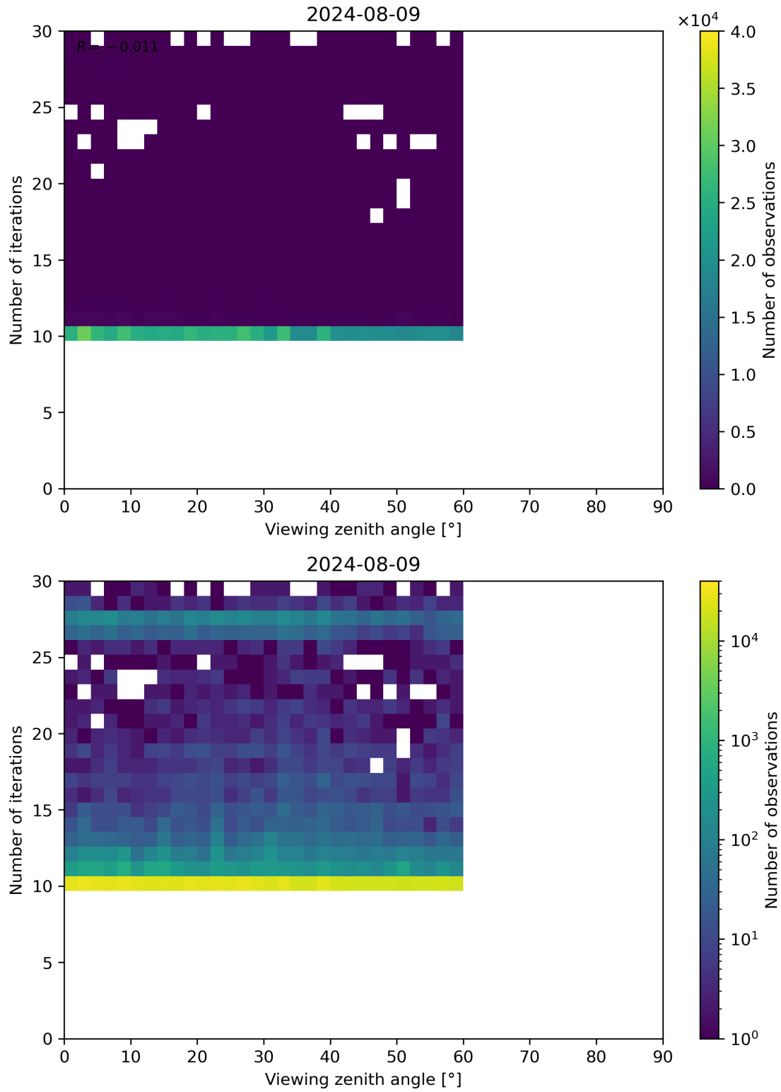
Figure 113: Scatter density plot of “Viewing zenith angle” against “Number of iterations” for 2024-08-08 to 2024-08-10.
