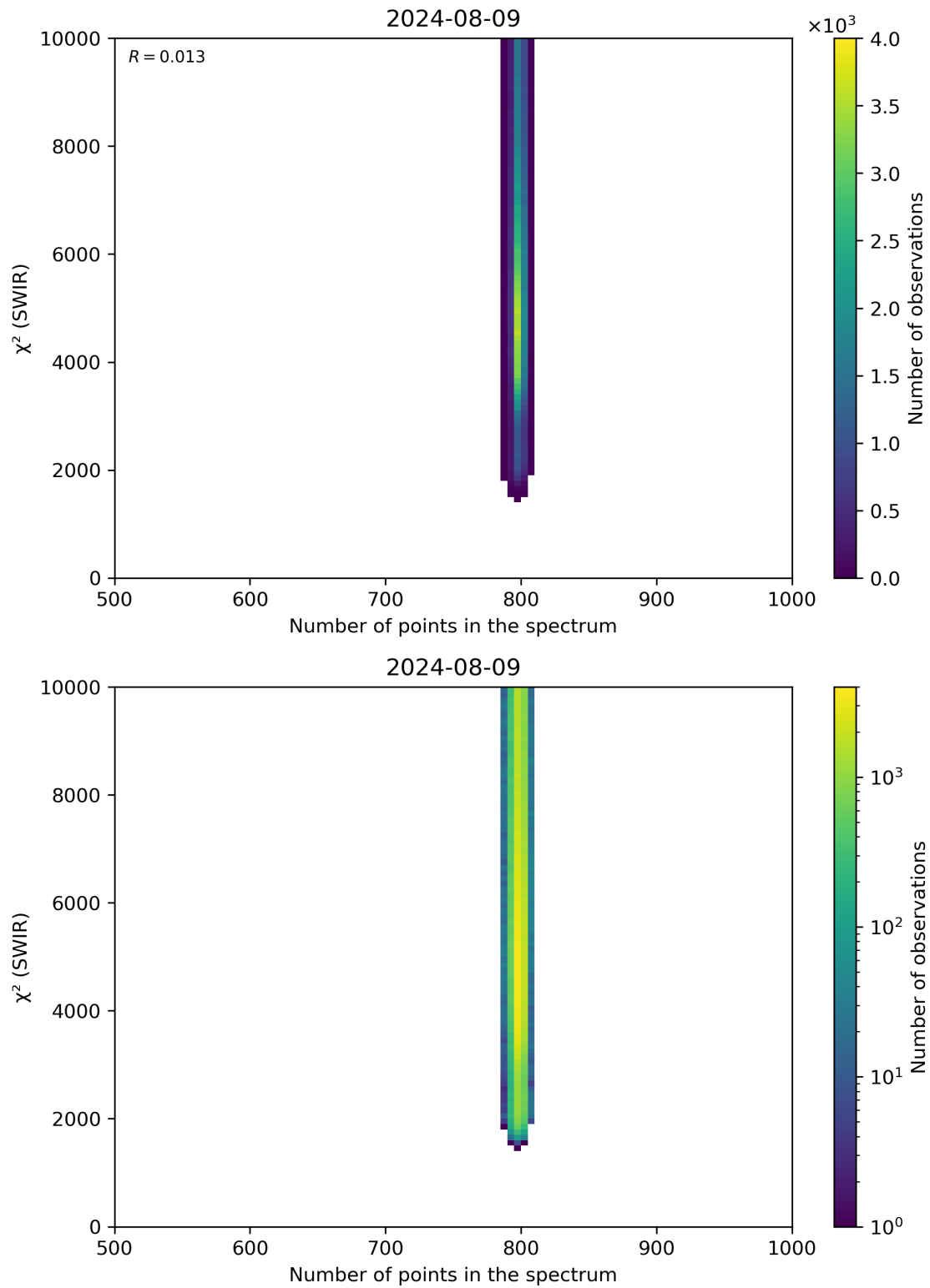
Figure 89: Scatter density plot of “Number of points in the spectrum” against “ \chi^2 (SWIR)” for 2024-08-08 to 2024-08-10.
