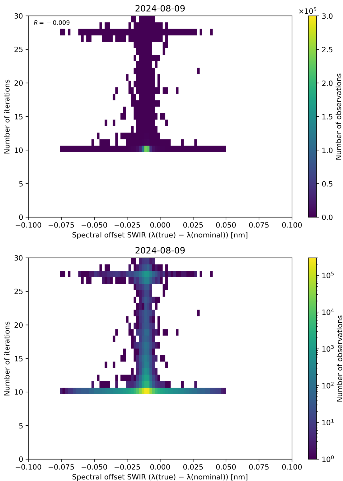
Figure 121: Scatter density plot of “Spectral offset SWIR ( \lambda(\text{true}) - \lambda(\text{nominal}) )” against “Number of iterations” for 2024-08-08 to 2024-08-10.
