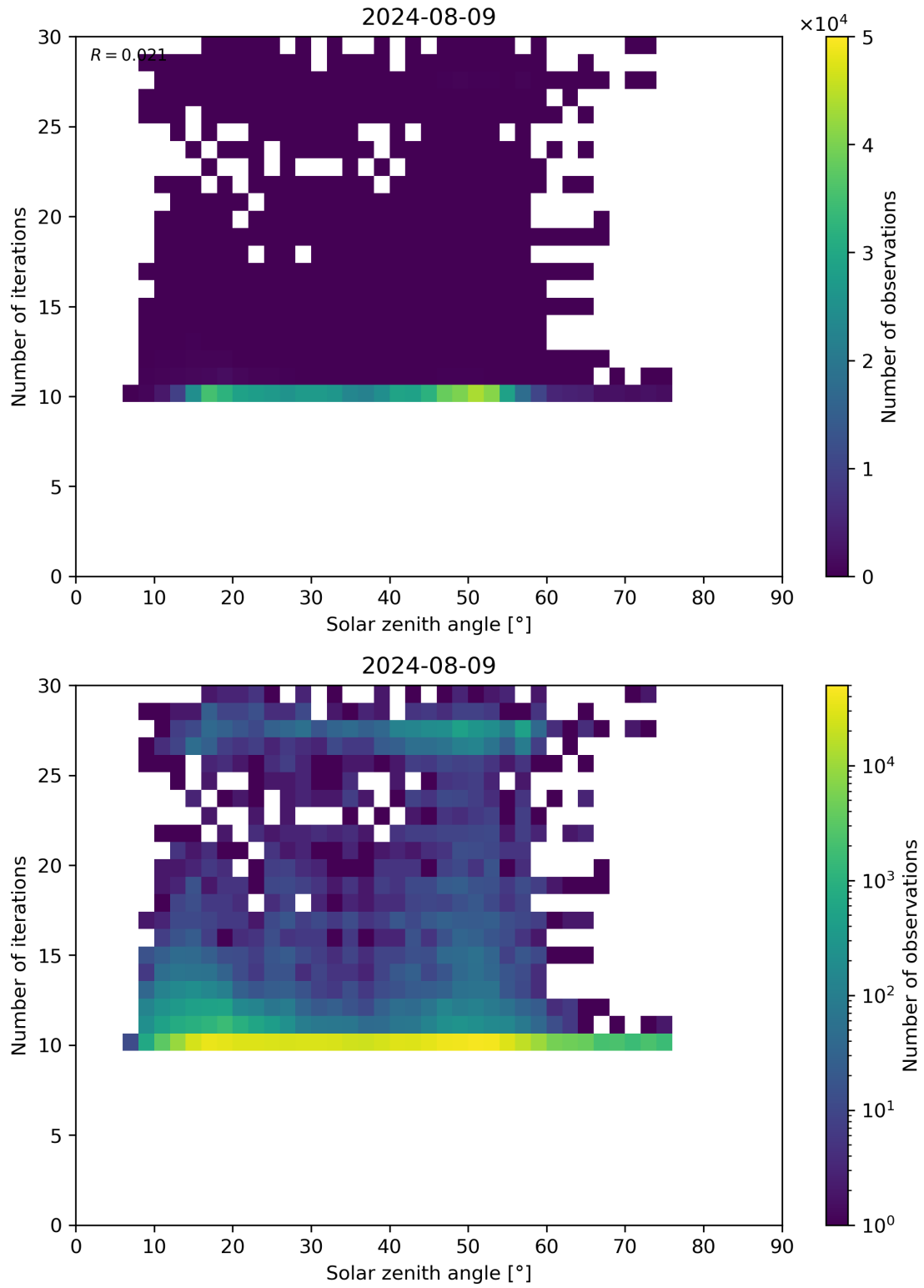
Figure 102: Scatter density plot of “Solar zenith angle” against “Number of iterations” for 2024-08-08 to 2024-08-10.
