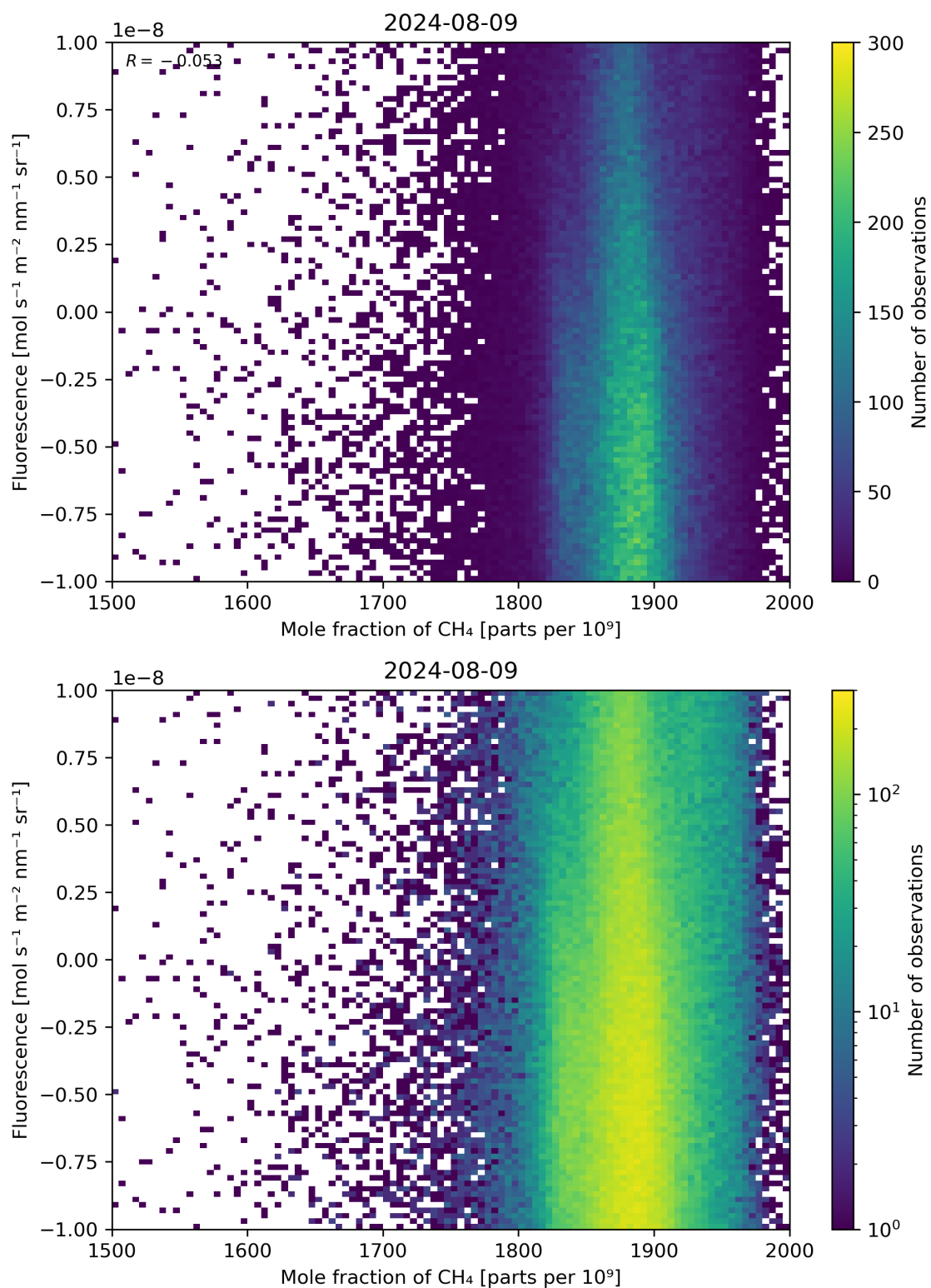
Figure 73: Scatter density plot of “Mole fraction of \text{CH}_4 ” against “Fluorescence” for 2024-08-08 to 2024-08-10.
