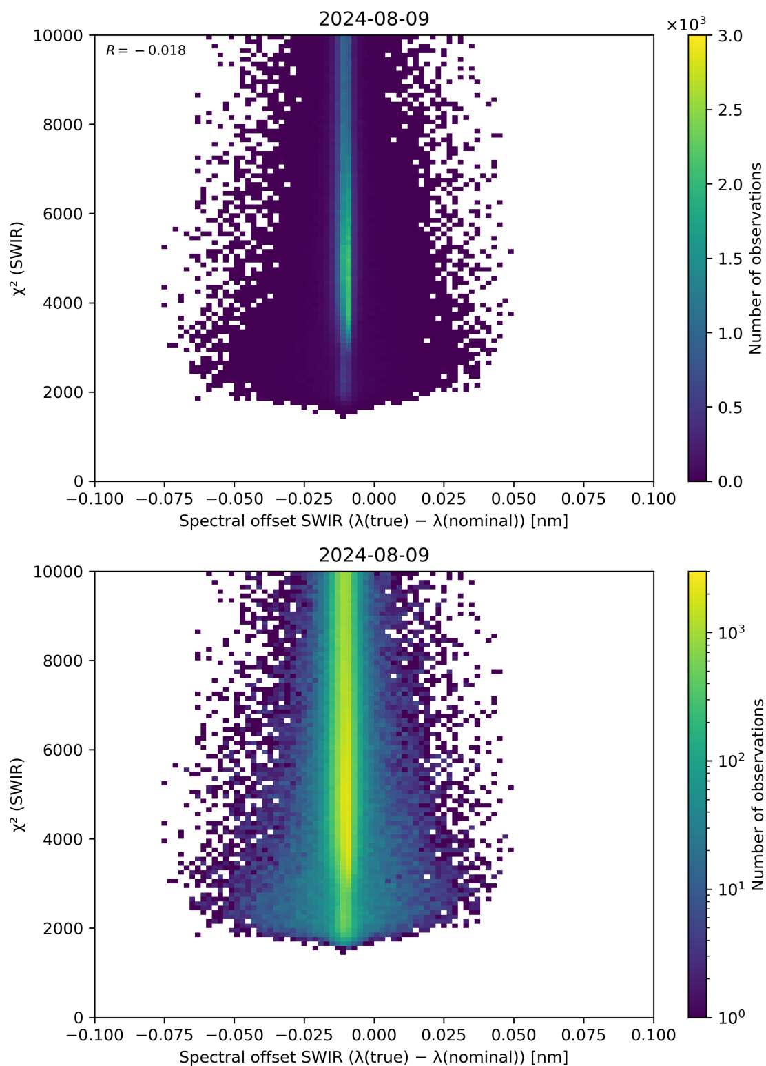
Figure 118: Scatter density plot of “Spectral offset SWIR ( \lambda(\text{true}) - \lambda(\text{nominal}) )” against “ \chi^2 (SWIR)” for 2024-08-08 to 2024-08-10.
