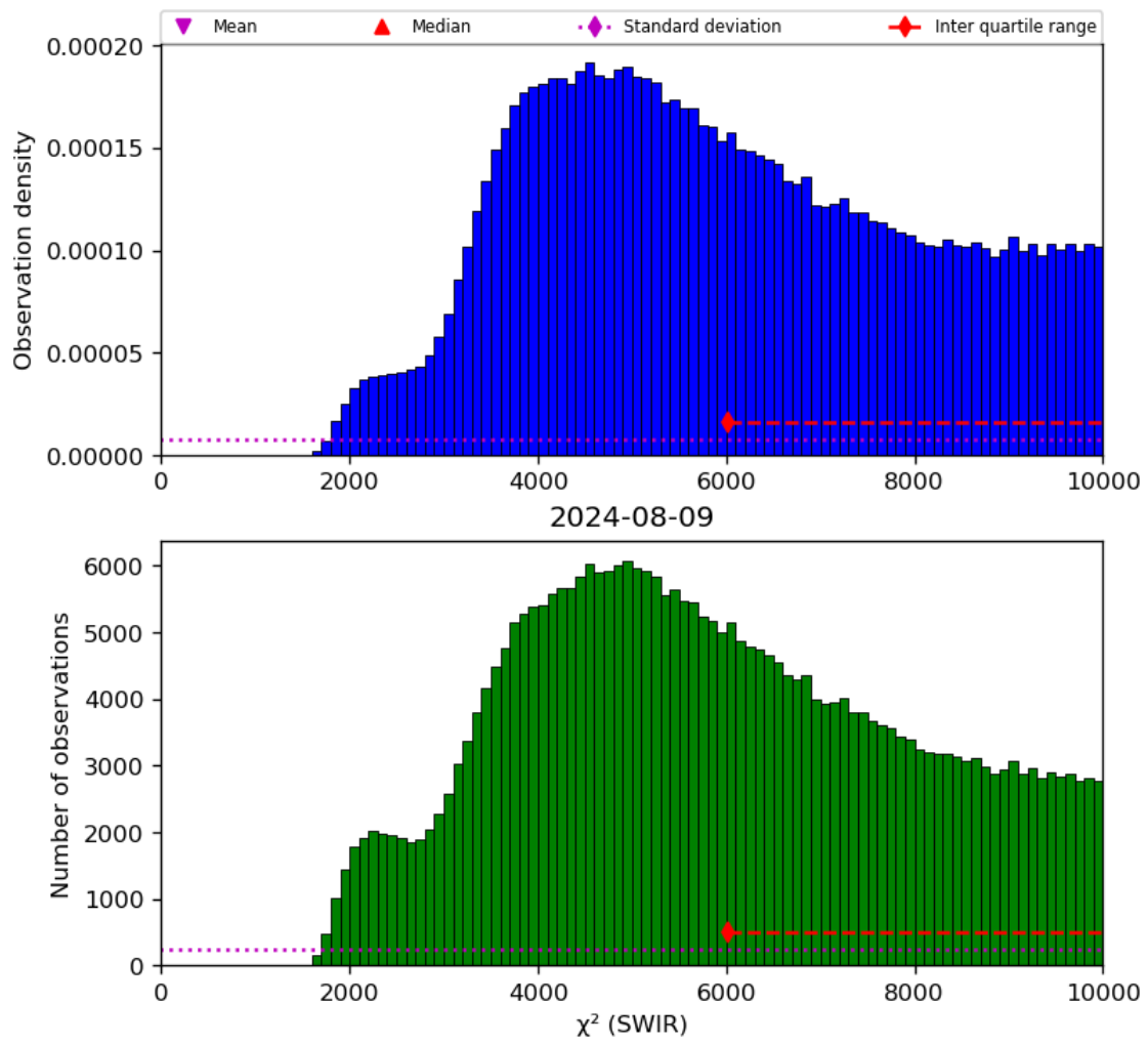
Figure 28: Histogram of " \chi^2 (SWIR)" for 2024-08-08 to 2024-08-10
