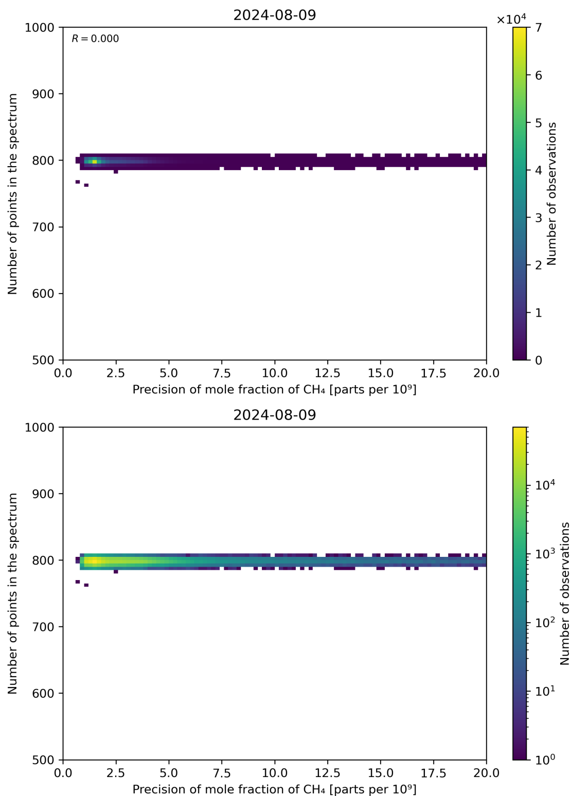
Figure 84: Scatter density plot of “Precision of mole fraction of CH 4 ” against “Number of points in the spectrum” for 2024-08-08 to 2024-08-10.
