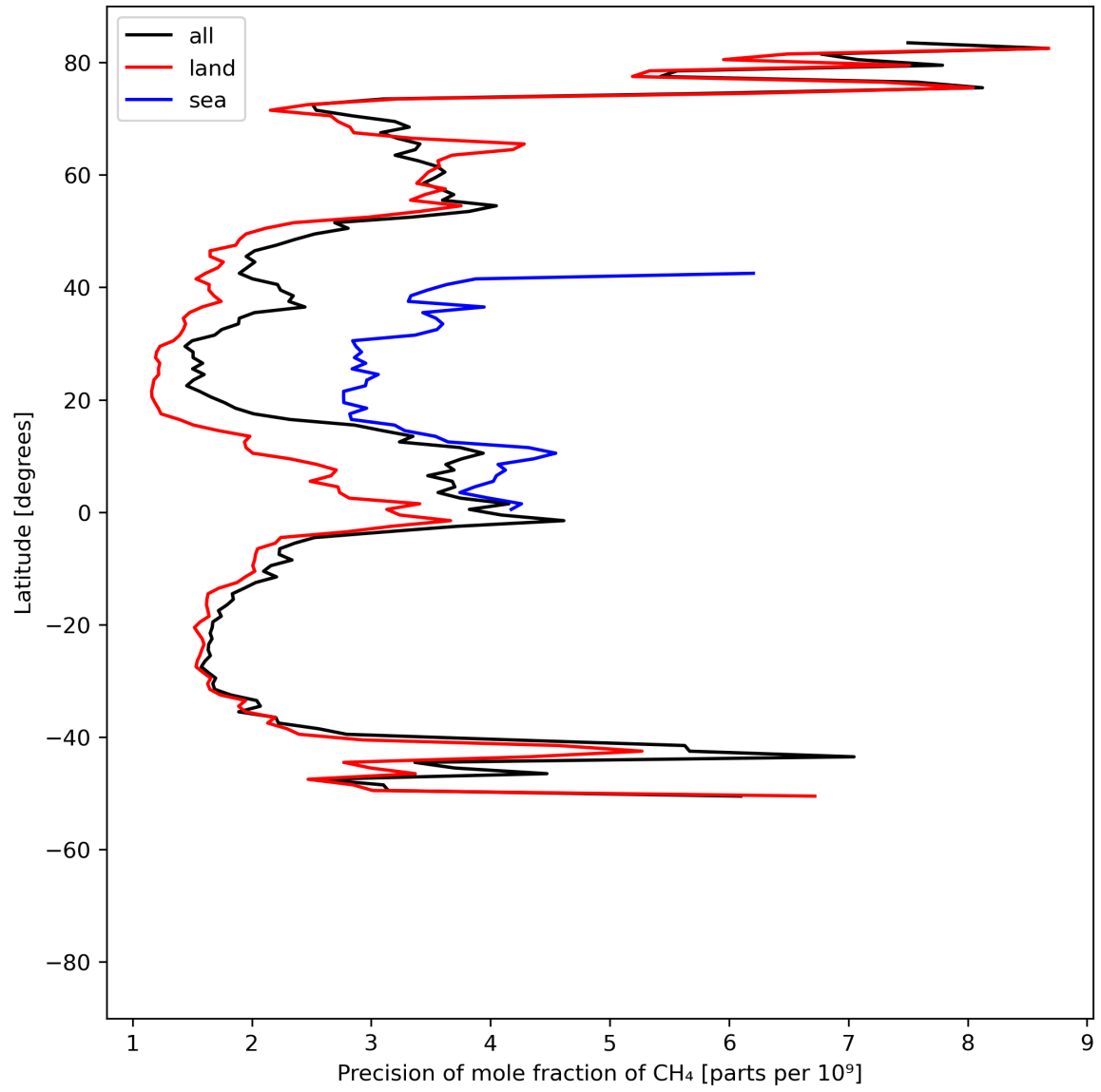
Figure 13: Zonal average of “Precision of mole fraction of \text{CH}_4 ” for 2024-08-08 to 2024-08-10.
