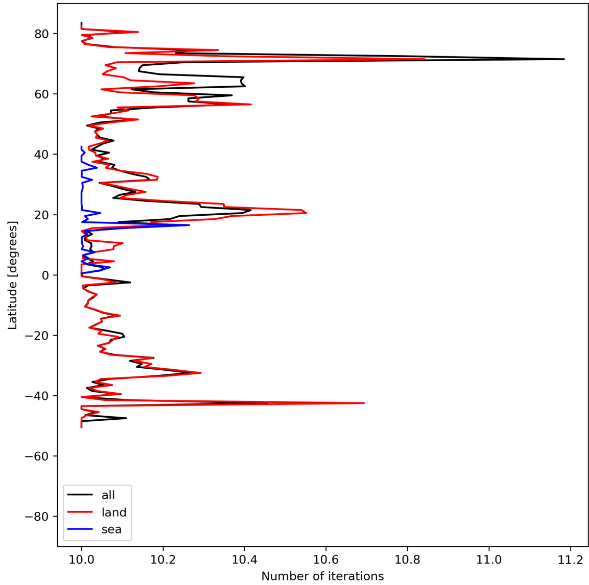
Figure 20: Zonal average of “Number of iterations” for 2024-08-08 to 2024-08-10.
