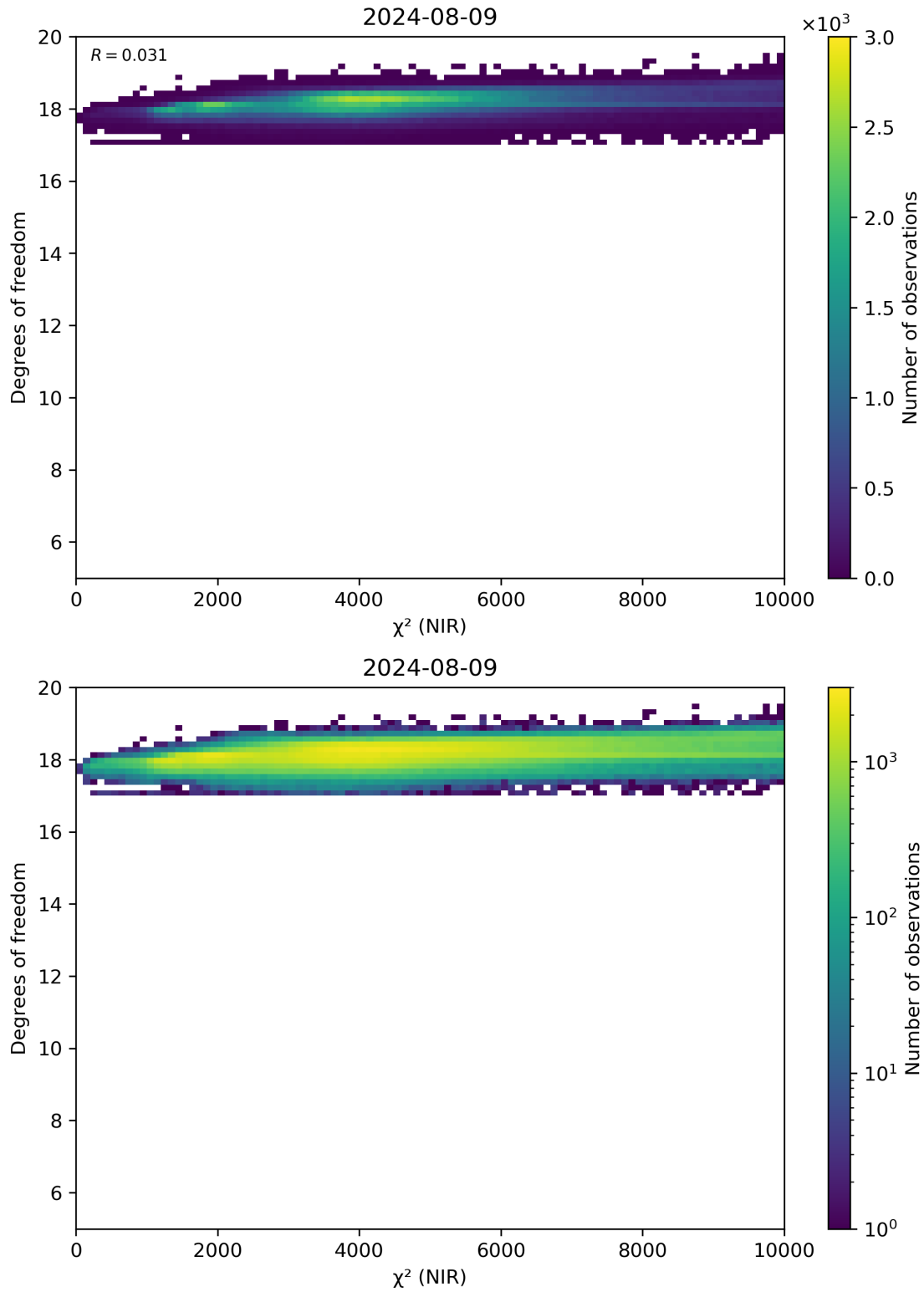
Figure 44: Scatter density plot of “ \chi^2 (NIR)” against “Degrees of freedom” for 2024-08-08 to 2024-08-10.
