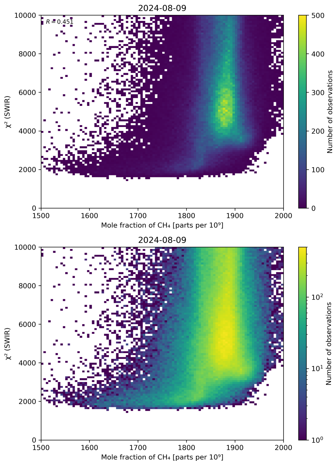
Figure 71: Scatter density plot of “Mole fraction of CH 4 ” against “ \chi^2 (SWIR)” for 2024-08-08 to 2024-08-10.
