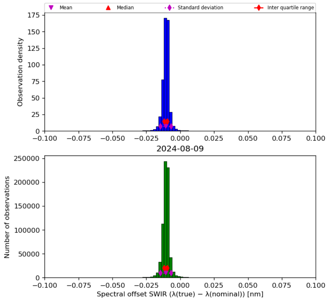
Figure 27: Histogram of “Spectral offset SWIR ( \lambda(\text{true}) - \lambda(\text{nominal}) )” for 2024-08-08 to 2024-08-10
