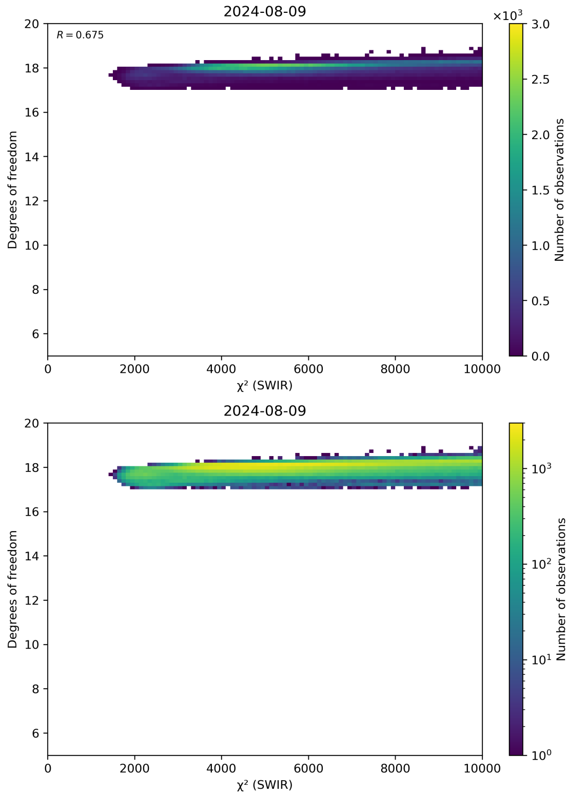
Figure 48: Scatter density plot of “ \chi^2 (SWIR)” against “Degrees of freedom” for 2024-08-08 to 2024-08-10.
