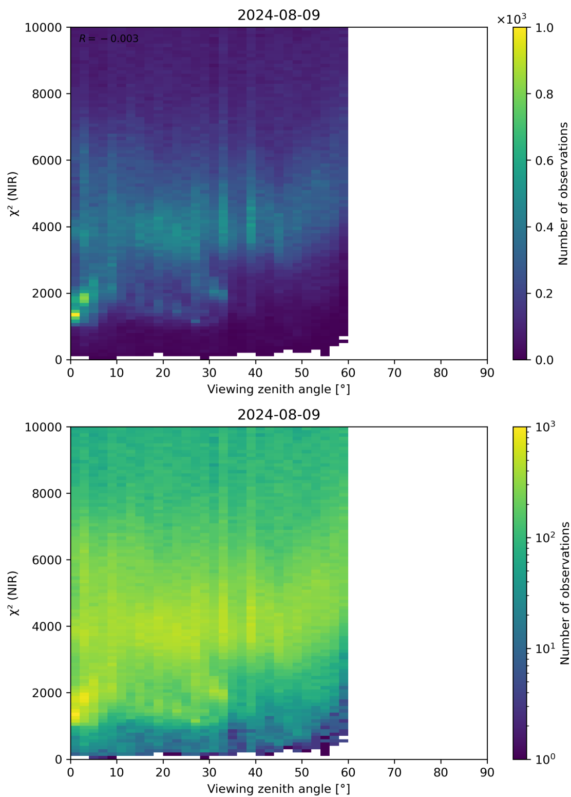
Figure 105: Scatter density plot of “Viewing zenith angle” against “ \chi^2 (NIR)” for 2024-08-08 to 2024-08-10.
