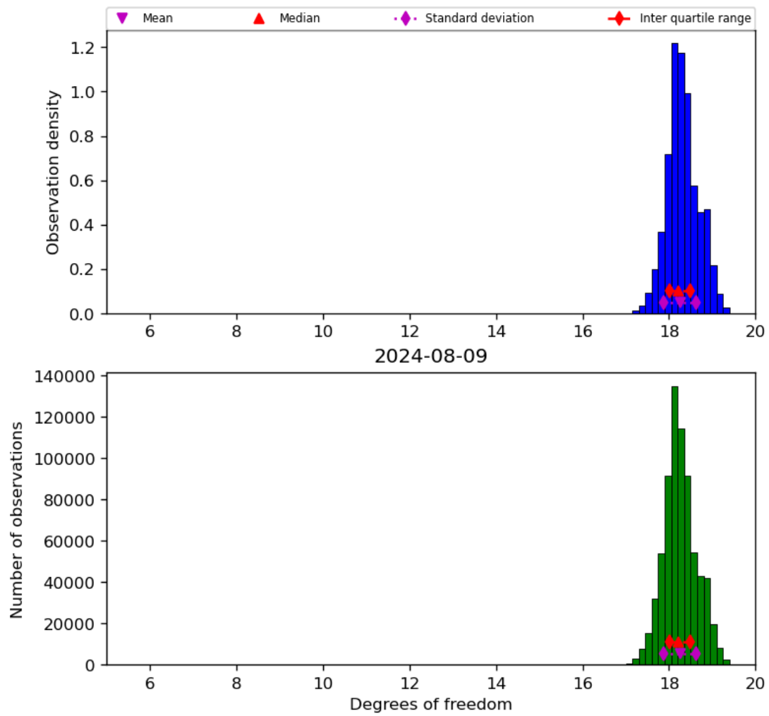
Figure 30: Histogram of “Degrees of freedom” for 2024-08-08 to 2024-08-10
