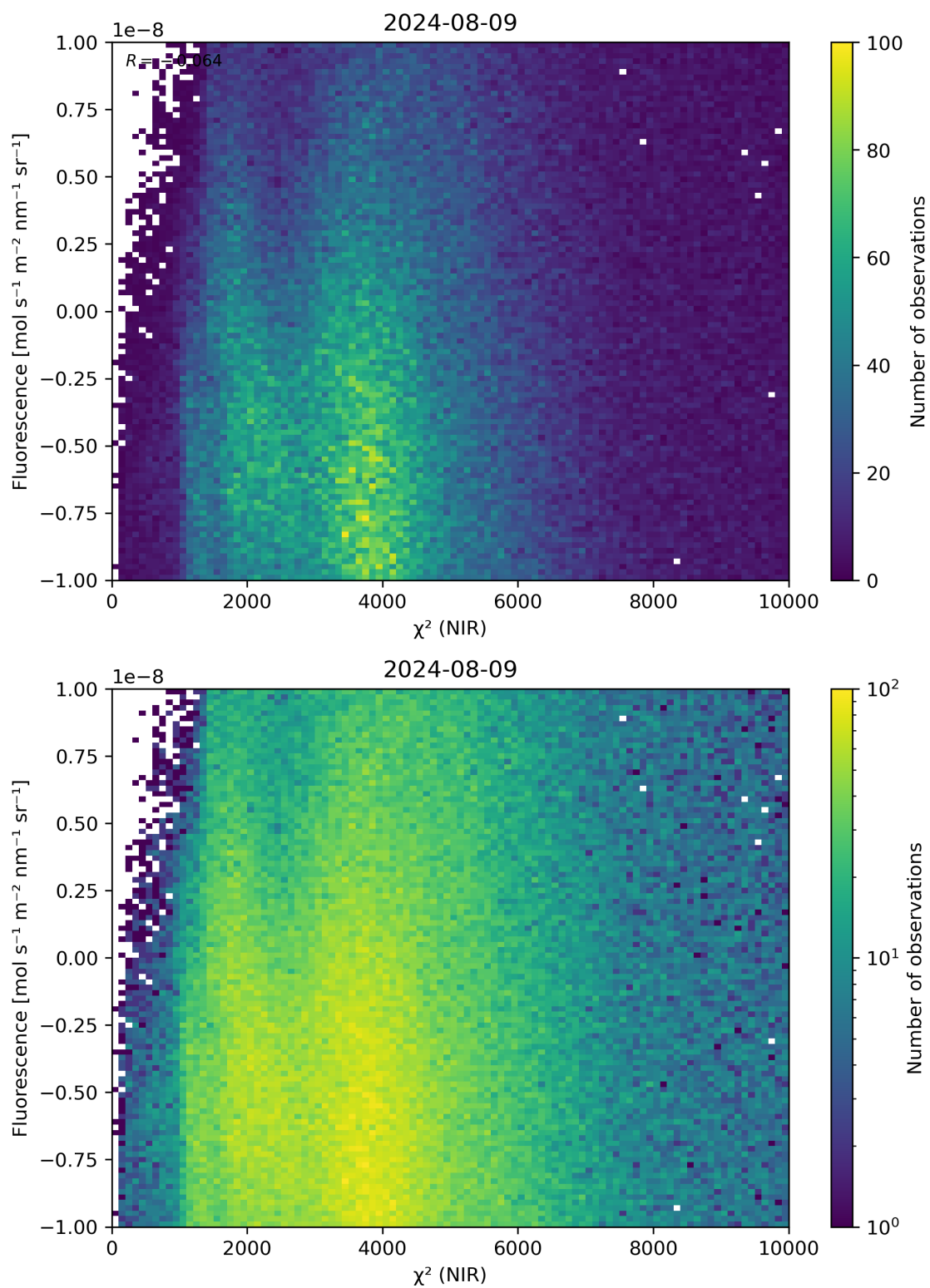
Figure 45: Scatter density plot of “ \chi^2 (NIR)” against “Fluorescence” for 2024-08-08 to 2024-08-10.
