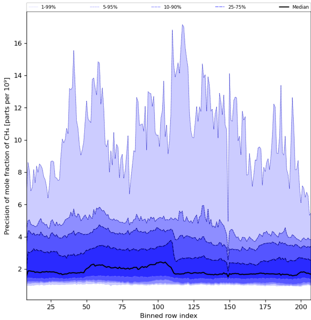
Figure 35: Along track statistics of “Precision of mole fraction of CH 4 ” for 2024-08-08 to 2024-08-10
