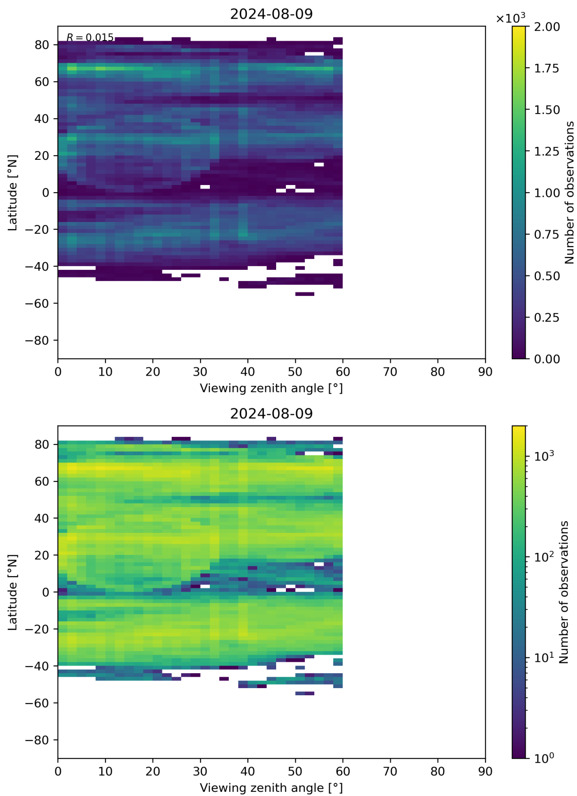
Figure 109: Scatter density plot of “Viewing zenith angle” against “Latitude” for 2024-08-08 to 2024-08-10.
