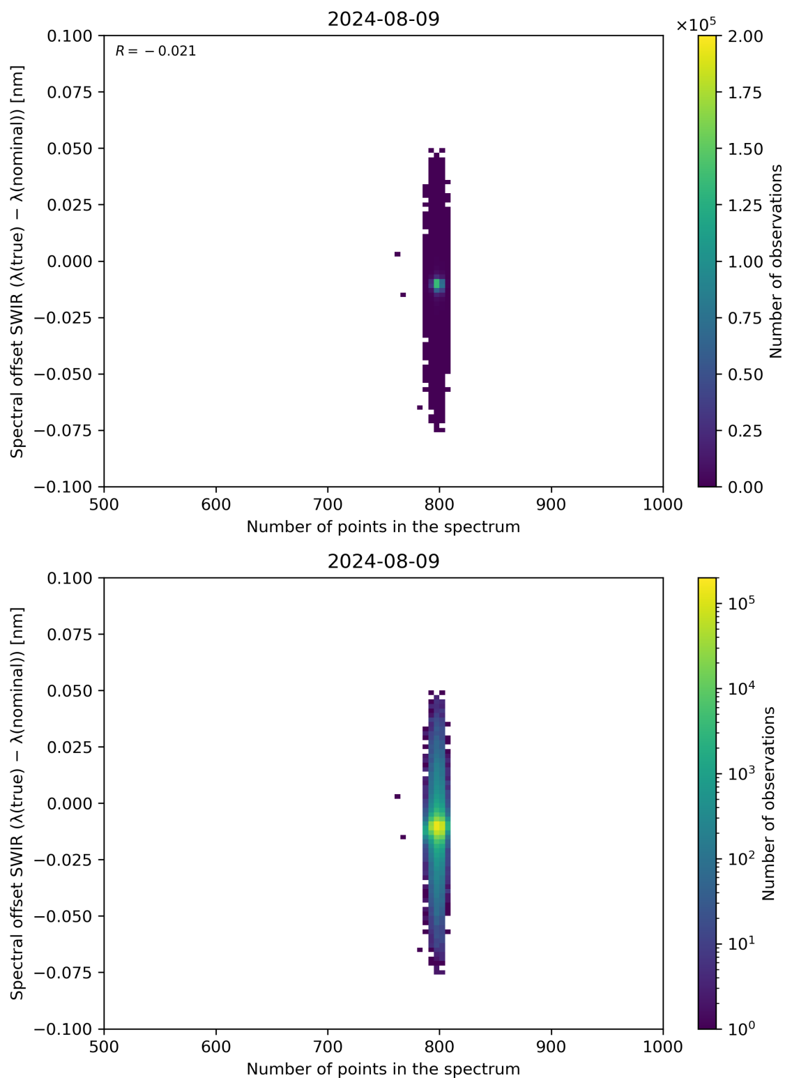
Figure 93: Scatter density plot of “Number of points in the spectrum” against “Spectral offset SWIR ( \lambda(\text{true}) - \lambda(\text{nominal}) )” for 2024-08-08 to 2024-08-10.
