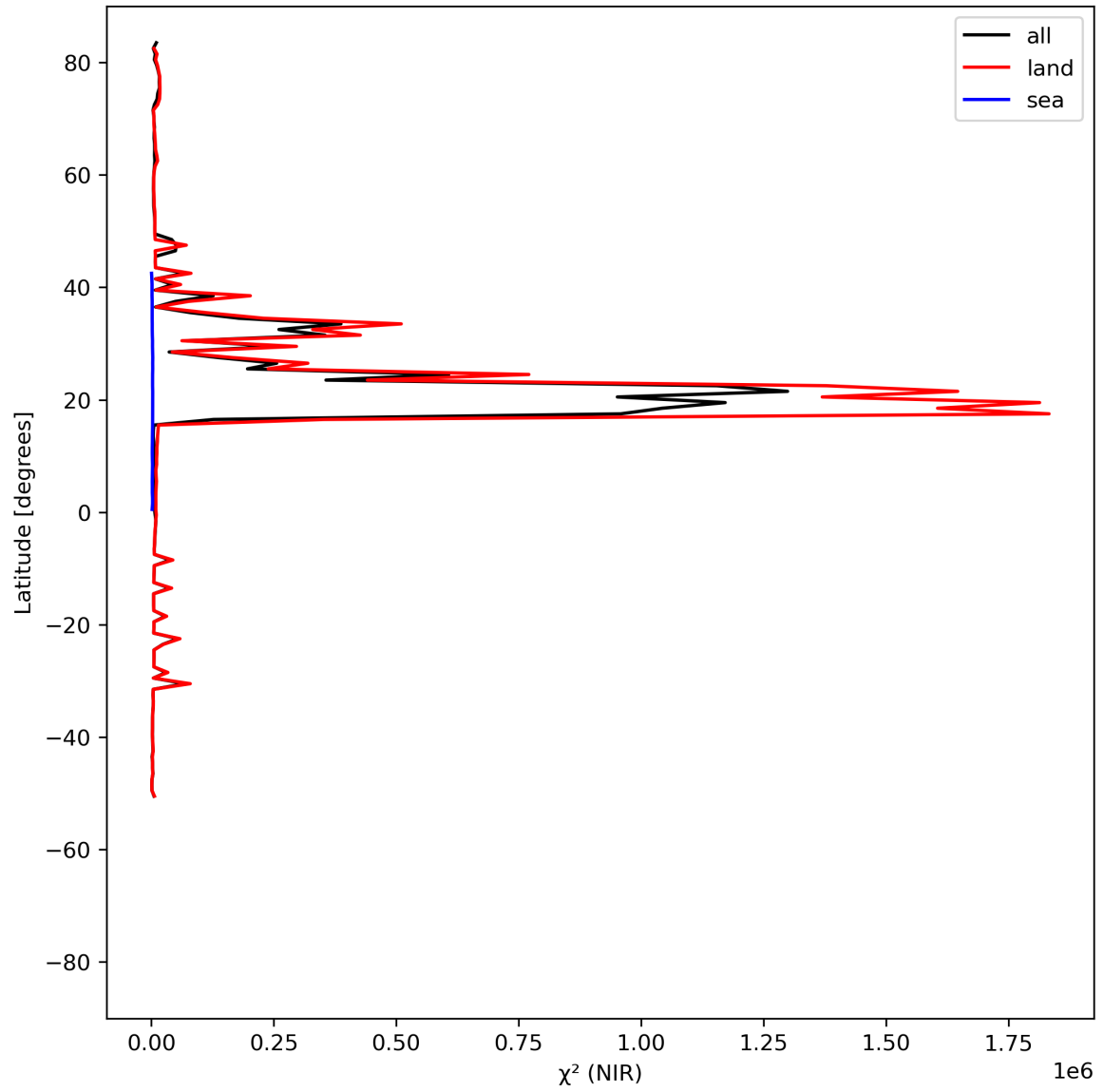
Figure 18: Zonal average of “ \chi^2 (NIR)” for 2024-08-08 to 2024-08-10.
