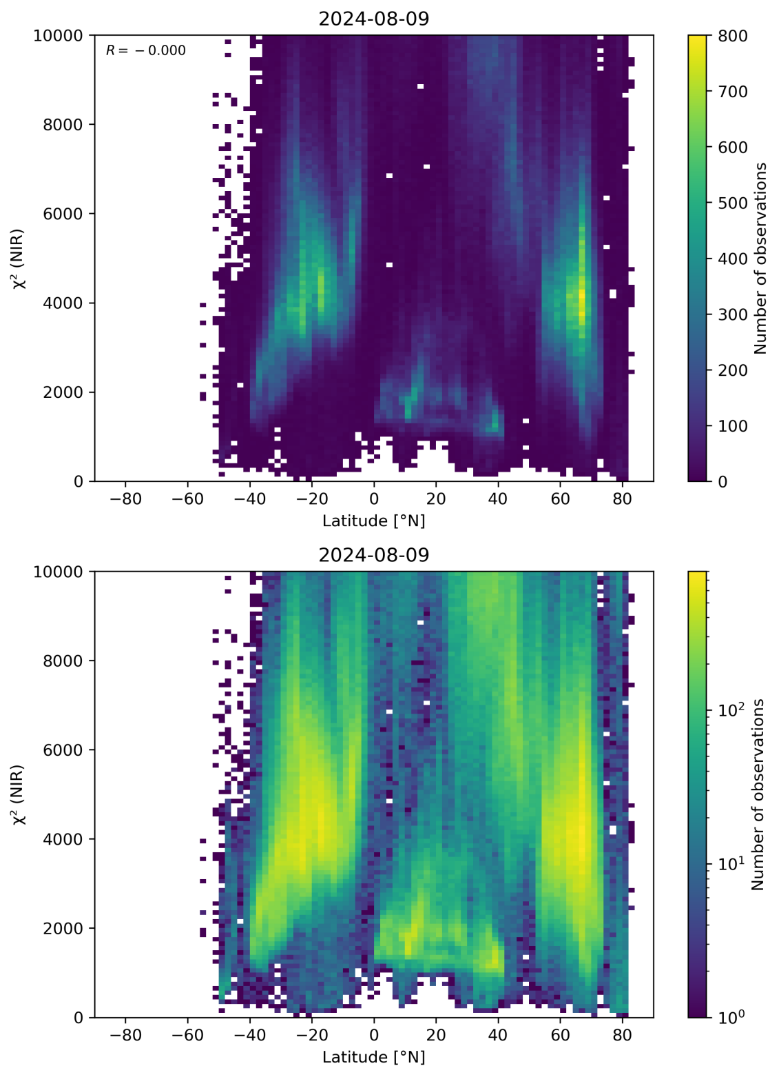
Figure 53: Scatter density plot of “Latitude” against “ \chi^2 (NIR)” for 2024-08-08 to 2024-08-10.
