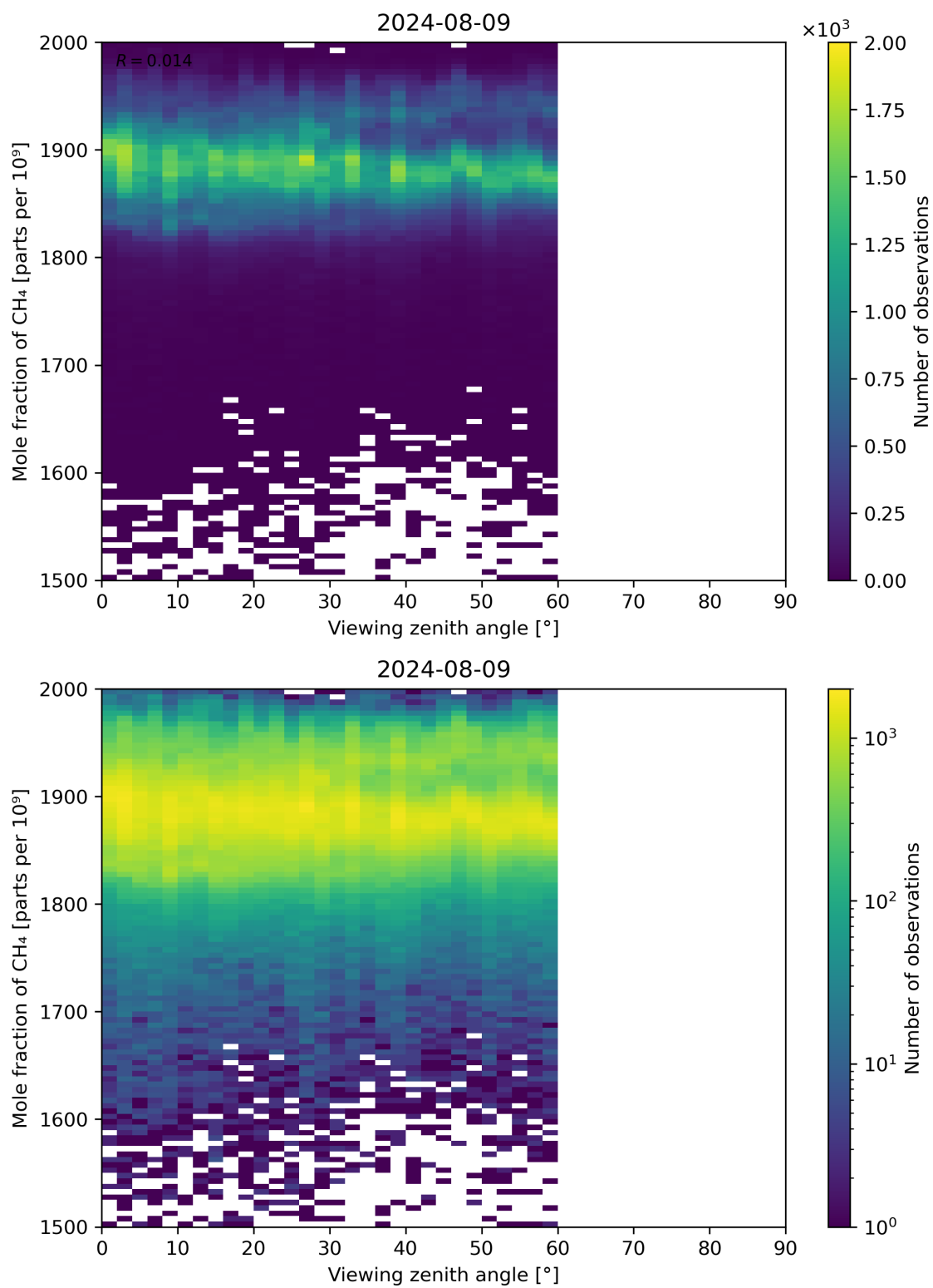
Figure 110: Scatter density plot of “Viewing zenith angle” against “Mole fraction of CH 4 ” for 2024-08-08 to 2024-08-10.
