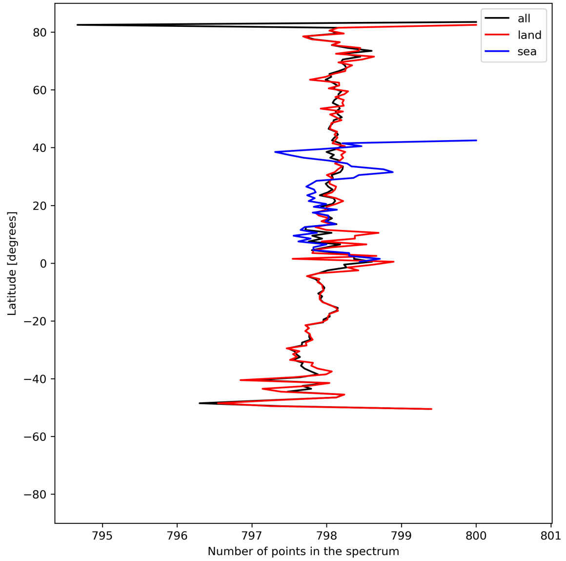
Figure 15: Zonal average of “Number of points in the spectrum” for 2024-08-08 to 2024-08-10.
