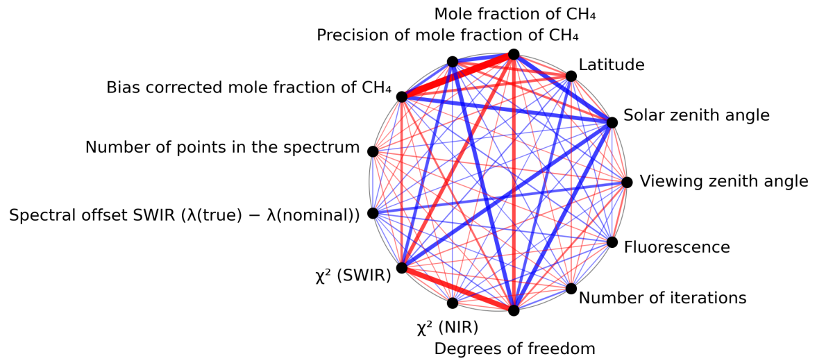
Figure 1: Map of correlation graph for 2024-08-08 to 2024-08-10.
