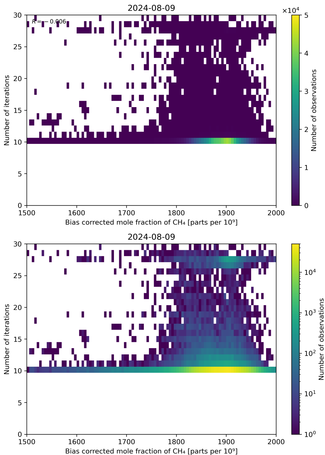
Figure 67: Scatter density plot of “Bias corrected mole fraction of CH 4 ” against “Number of iterations” for 2024-08-08 to 2024-08-10.
