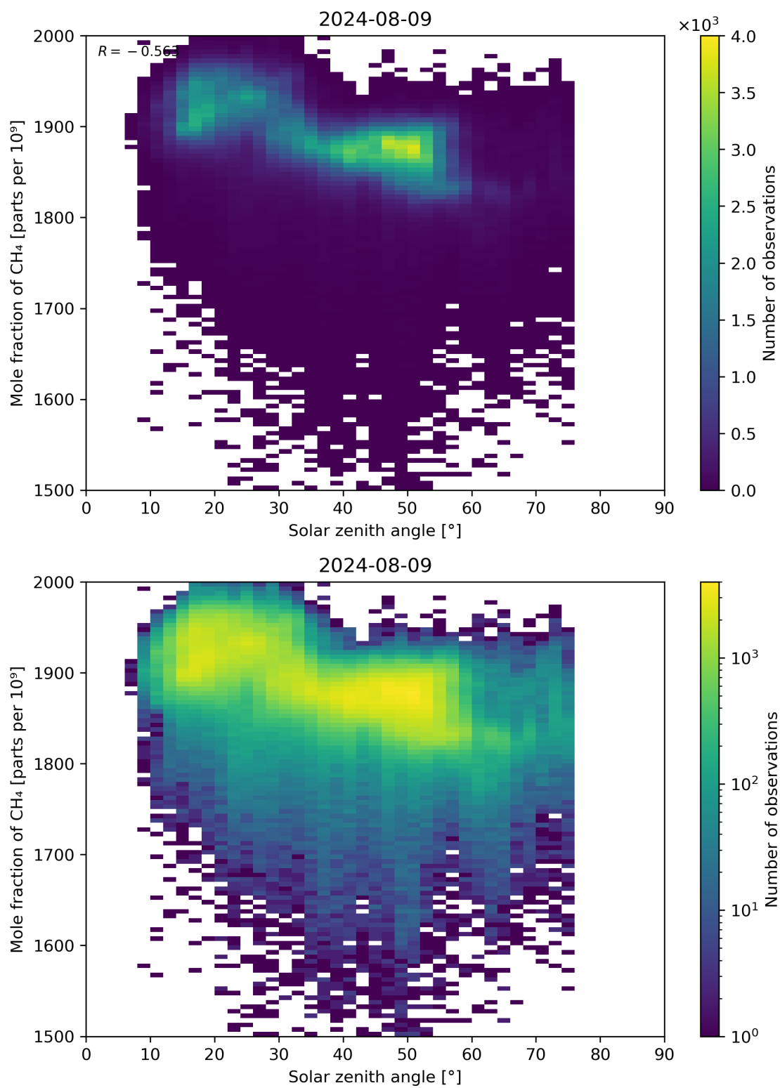
Figure 99: Scatter density plot of “Solar zenith angle” against “Mole fraction of \text{CH}_4 ” for 2024-08-08 to 2024-08-10.
