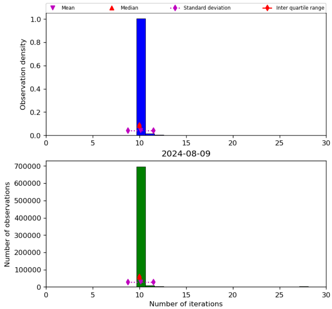
Figure 31: Histogram of “Number of iterations” for 2024-08-08 to 2024-08-10
