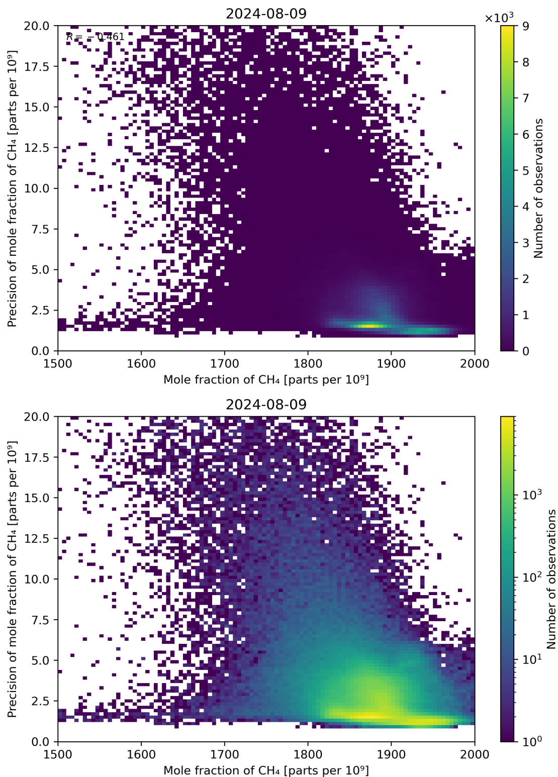
Figure 75: Scatter density plot of “Mole fraction of CH 4 ” against “Precision of mole fraction of CH 4 ” for 2024-08-08 to 2024-08-10.
