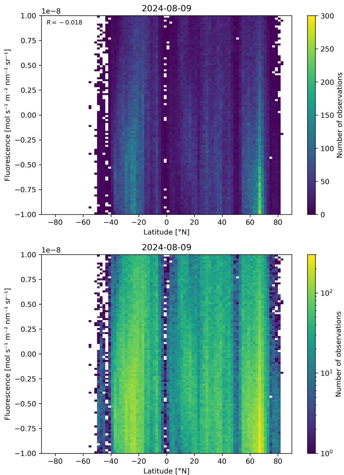
Figure 56: Scatter density plot of “Latitude” against “Fluorescence” for 2024-08-08 to 2024-08-10.
