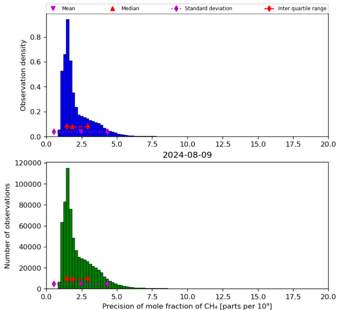
Figure 24: Histogram of “Precision of mole fraction of CH 4 ” for 2024-08-08 to 2024-08-10
