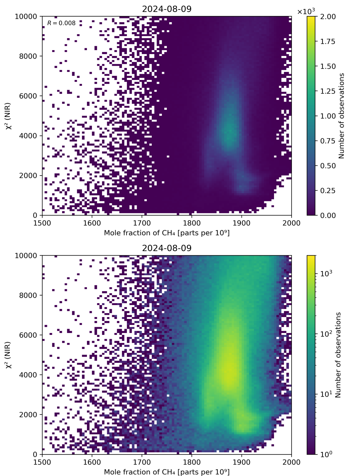
Figure 70: Scatter density plot of “Mole fraction of \text{CH}_4 ” against “ \chi^2 (NIR)” for 2024-08-08 to 2024-08-10.
