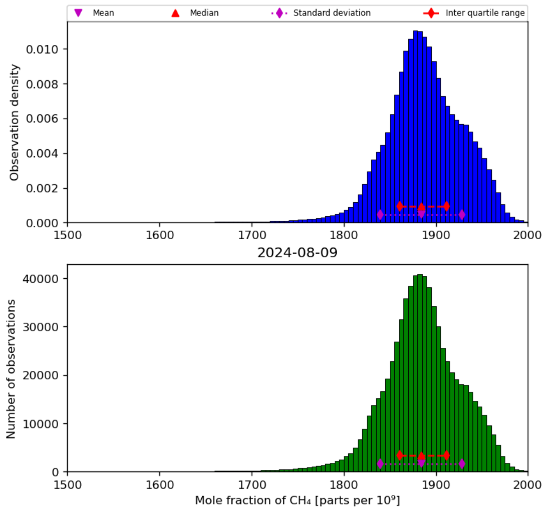
Figure 23: Histogram of “Mole fraction of CH 4 ” for 2024-08-08 to 2024-08-10
