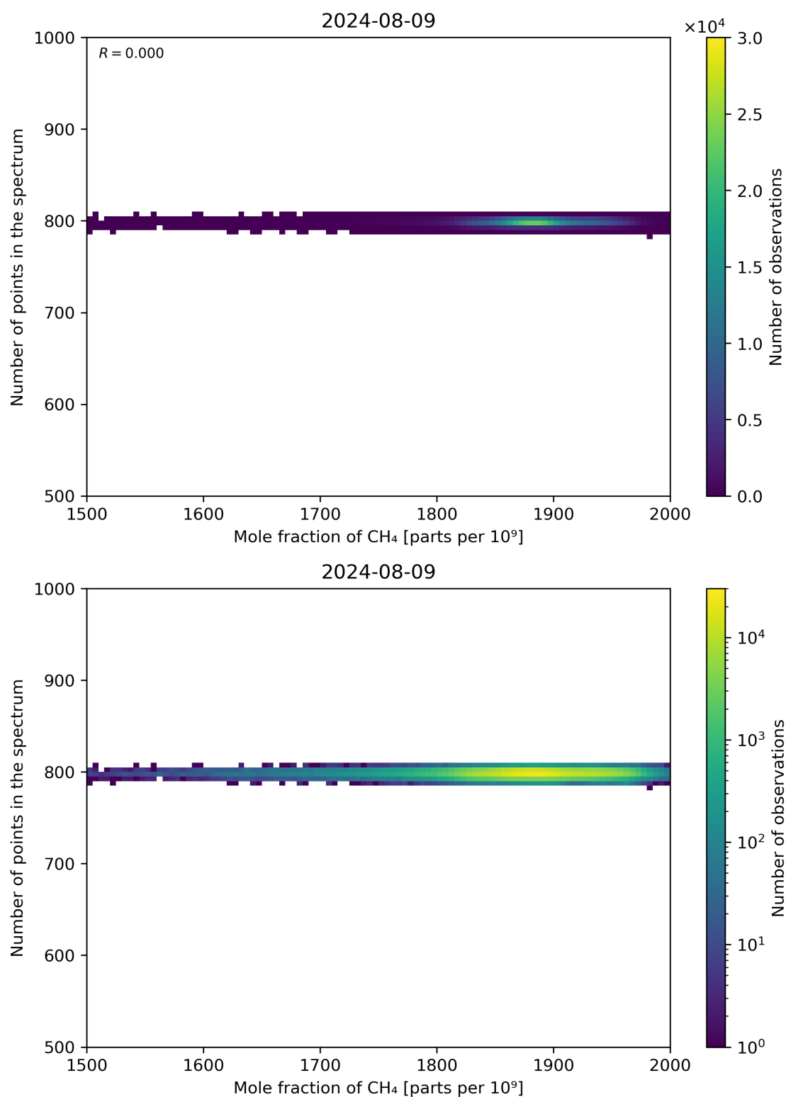
Figure 77: Scatter density plot of “Mole fraction of CH 4 ” against “Number of points in the spectrum” for 2024-08-08 to 2024-08-10.
