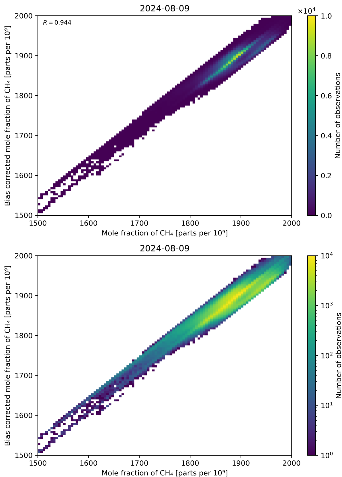
Figure 74: Scatter density plot of “Mole fraction of CH 4 ” against “Bias corrected mole fraction of CH 4 ” for 2024-08-08 to 2024-08-10.
