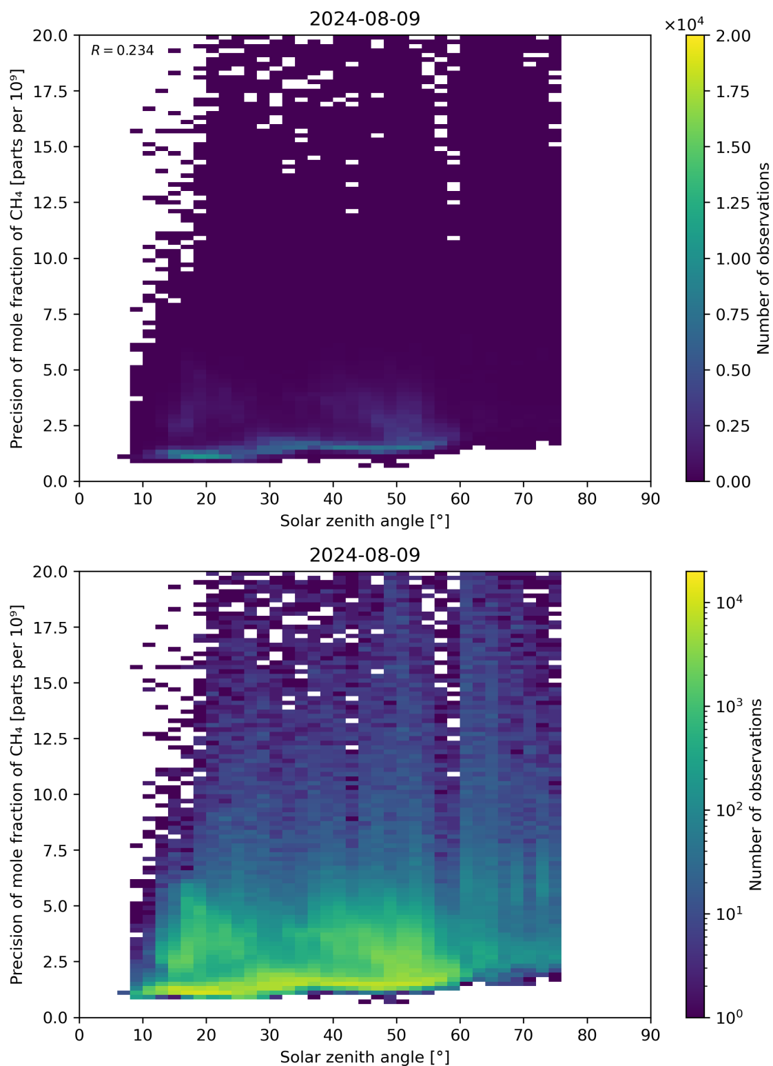
Figure 101: Scatter density plot of “Solar zenith angle” against “Precision of mole fraction of \text{CH}_4 ” for 2024-08-08 to 2024-08-10.
