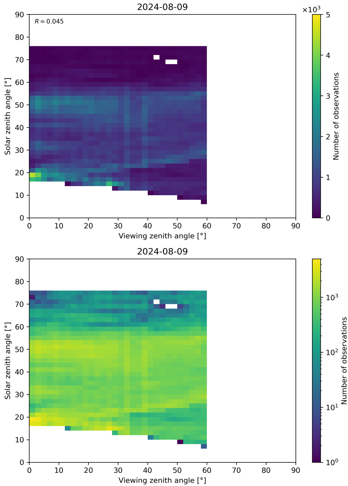
Figure 115: Scatter density plot of “Viewing zenith angle” against “Solar zenith angle” for 2024-08-08 to 2024-08-10.
