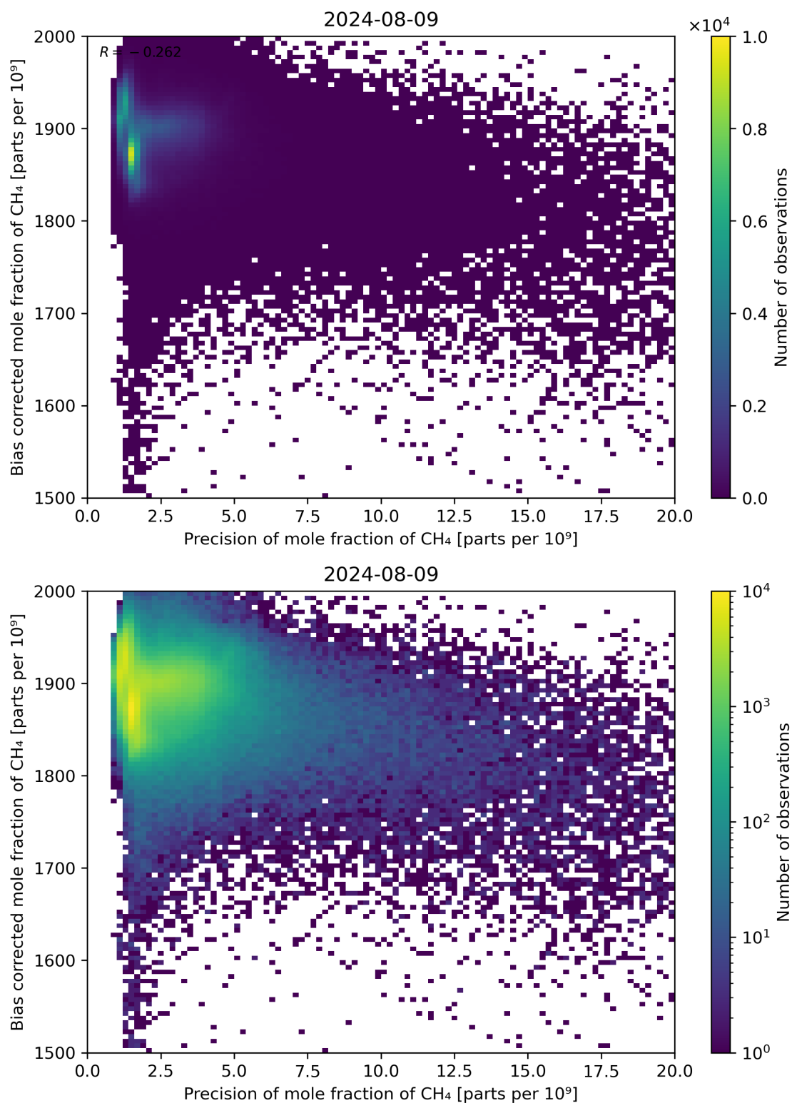
Figure 82: Scatter density plot of “Precision of mole fraction of CH 4 ” against “Bias corrected mole fraction of CH 4 ” for 2024-08-08 to 2024-08-10.
