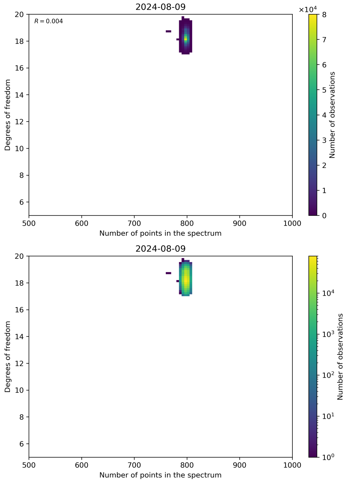
Figure 90: Scatter density plot of “Number of points in the spectrum” against “Degrees of freedom” for 2024-08-08 to 2024-08-10.
