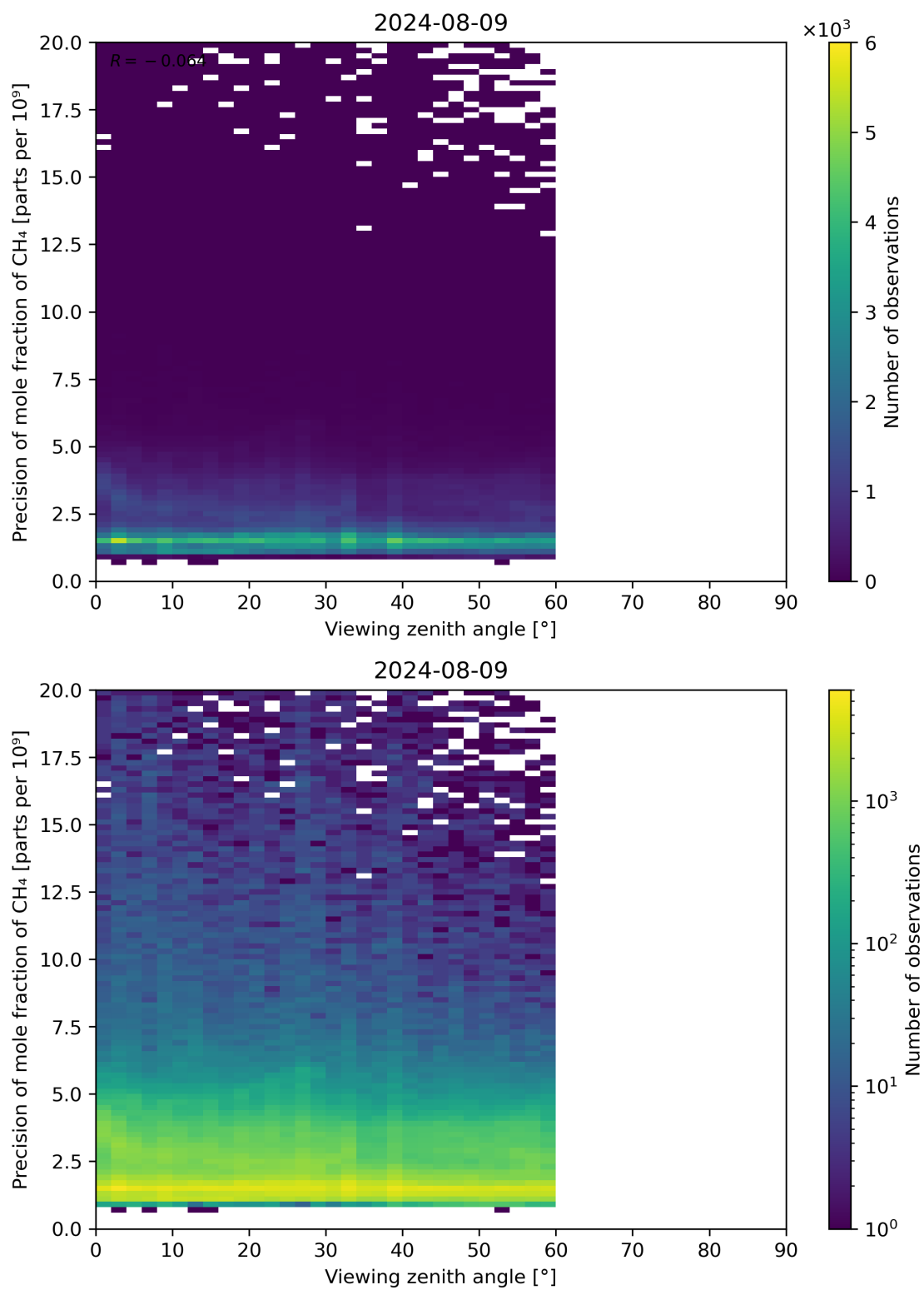
Figure 112: Scatter density plot of “Viewing zenith angle” against “Precision of mole fraction of CH 4 ” for 2024-08-08 to 2024-08-10.
