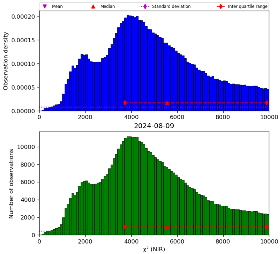
Figure 29: Histogram of “ \chi^2 (NIR)” for 2024-08-08 to 2024-08-10
