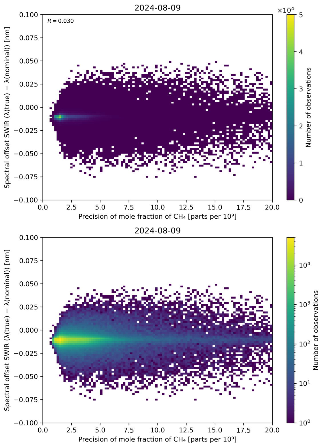
Figure 85: Scatter density plot of “Precision of mole fraction of \text{CH}_4 ” against “Spectral offset SWIR ( \lambda(\text{true}) - \lambda(\text{nominal}) )” for 2024-08-08 to 2024-08-10.
