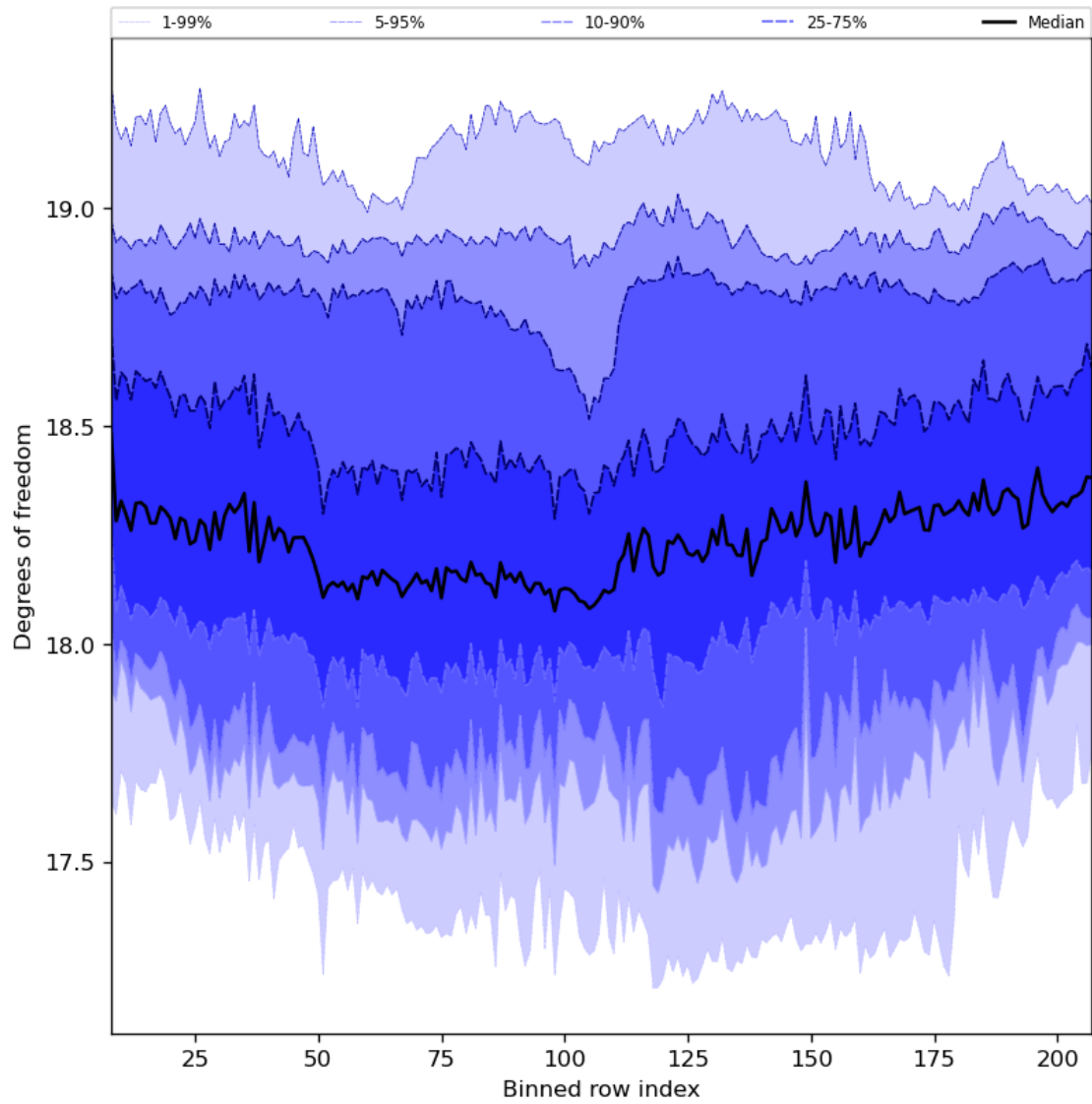
Figure 41: Along track statistics of “Degrees of freedom” for 2024-08-08 to 2024-08-10
