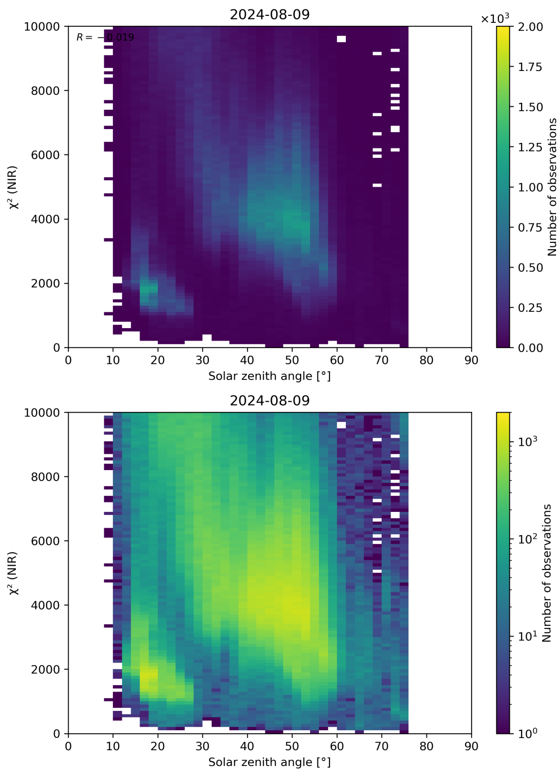
Figure 94: Scatter density plot of “Solar zenith angle” against “ \chi^2 (NIR)” for 2024-08-08 to 2024-08-10.
