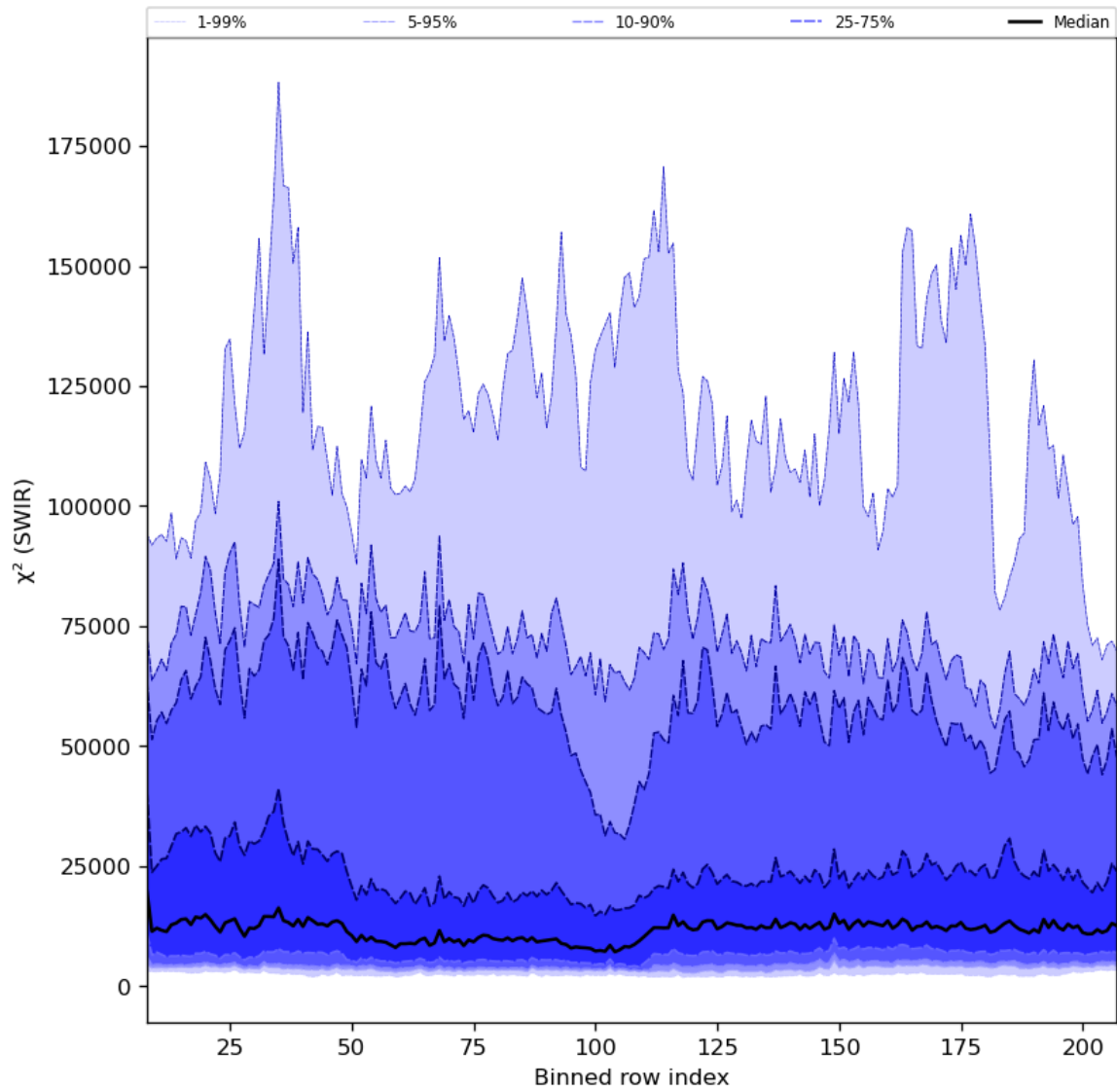
Figure 39: Along track statistics of “ \chi^2 (SWIR)” for 2024-08-08 to 2024-08-10
