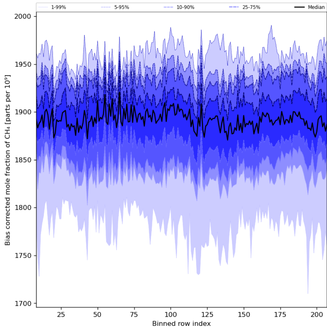
Figure 36: Along track statistics of “Bias corrected mole fraction of CH 4 ” for 2024-08-08 to 2024-08-10
