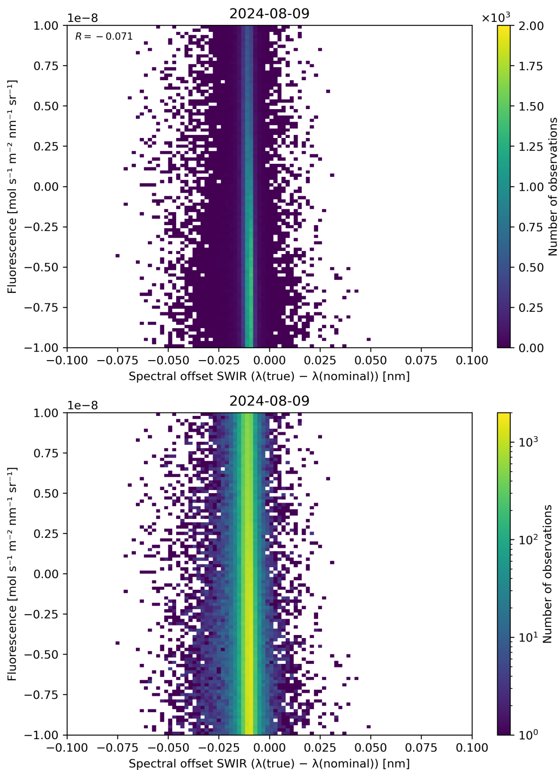
Figure 120: Scatter density plot of “Spectral offset SWIR ( \lambda(\text{true}) - \lambda(\text{nominal}) )” against “Fluorescence” for 2024-08-08 to 2024-08-10.
