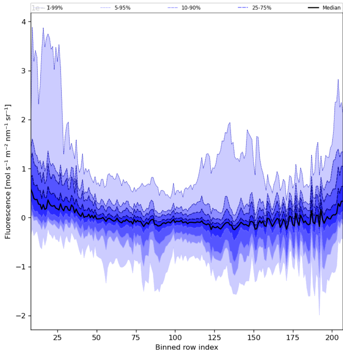
Figure 43: Along track statistics of “Fluorescence” for 2024-08-08 to 2024-08-10
