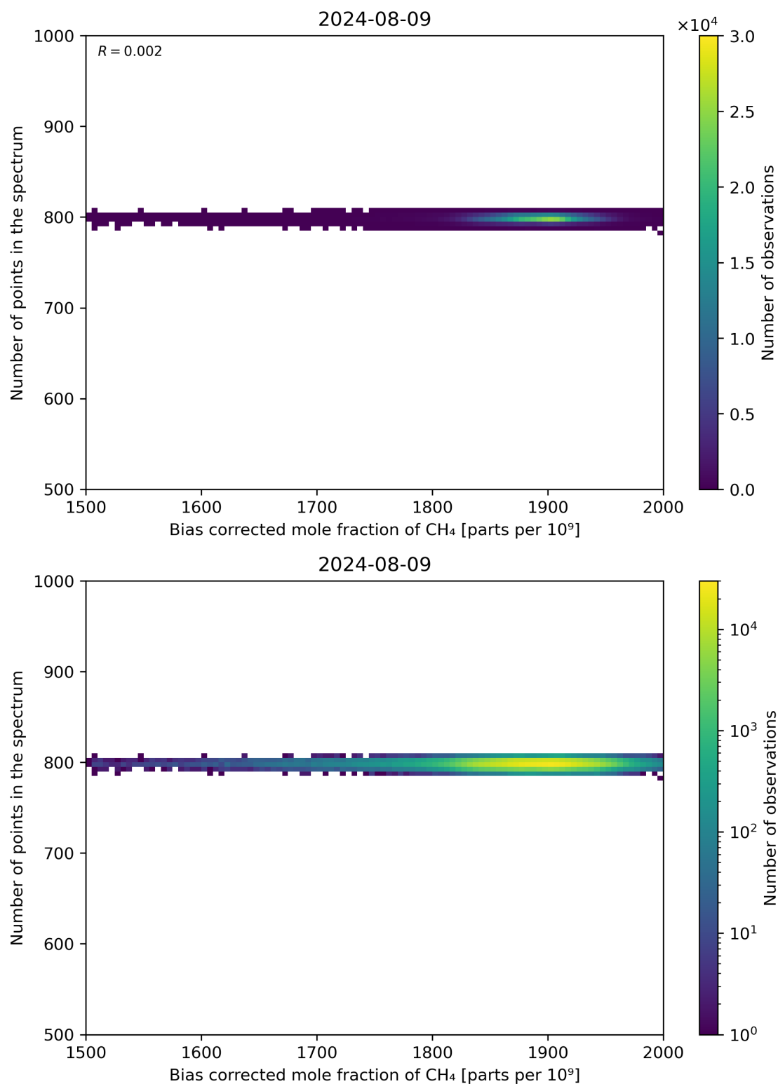
Figure 68: Scatter density plot of “Bias corrected mole fraction of \text{CH}_4 ” against “Number of points in the spectrum” for 2024-08-08 to 2024-08-10.
