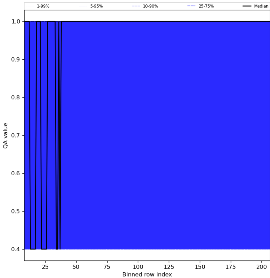
Figure 33: Along track statistics of “QA value” for 2024-08-08 to 2024-08-10
