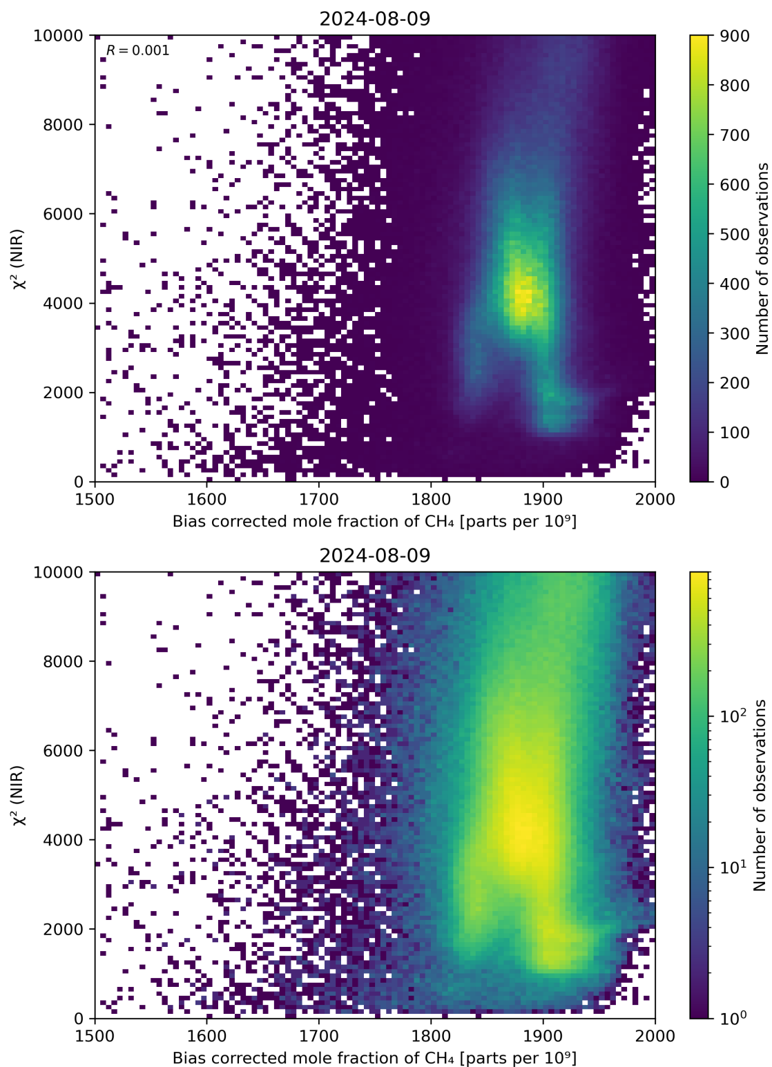
Figure 63: Scatter density plot of “Bias corrected mole fraction of CH 4 ” against “ \chi^2 (NIR)” for 2024-08-08 to 2024-08-10.
