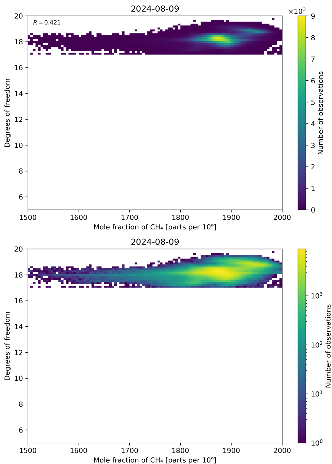
Figure 72: Scatter density plot of “Mole fraction of CH 4 ” against “Degrees of freedom” for 2024-08-08 to 2024-08-10.
