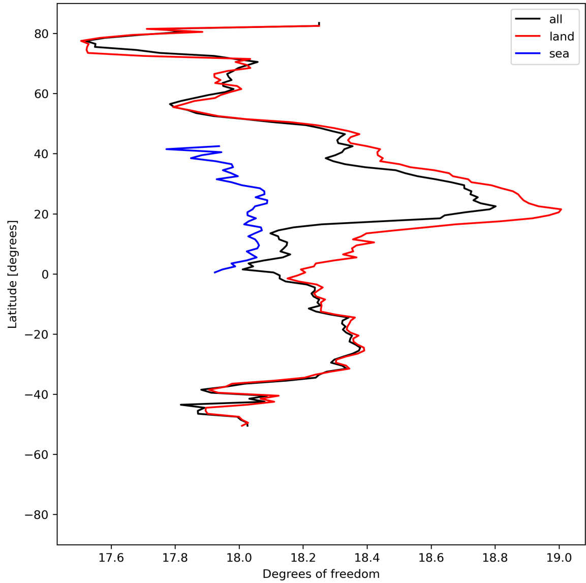
Figure 19: Zonal average of “Degrees of freedom” for 2024-08-08 to 2024-08-10.
