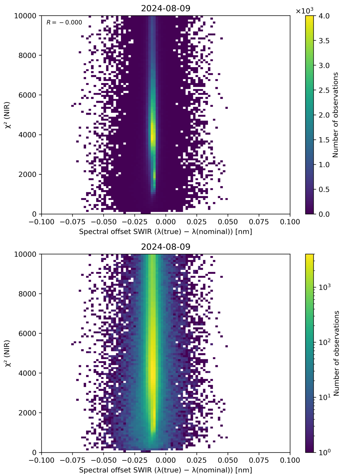
Figure 117: Scatter density plot of “Spectral offset SWIR ( \lambda(\text{true}) - \lambda(\text{nominal}) )” against “ \chi^2 (NIR)” for 2024-08-08 to 2024-08-10.
