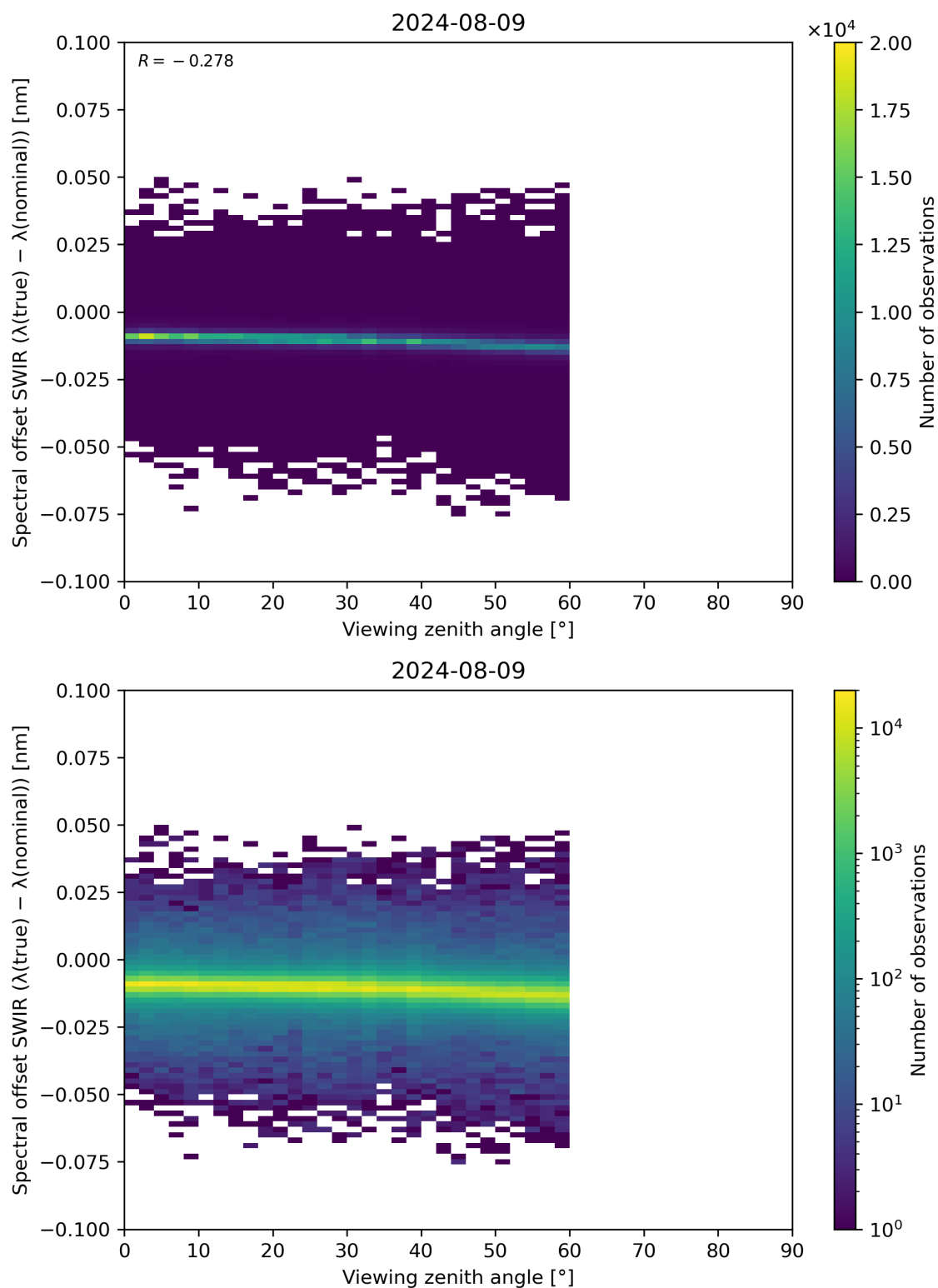
Figure 116: Scatter density plot of “Viewing zenith angle” against “Spectral offset SWIR ( \lambda(\text{true}) - \lambda(\text{nominal}) )” for 2024-08-08 to 2024-08-10.
