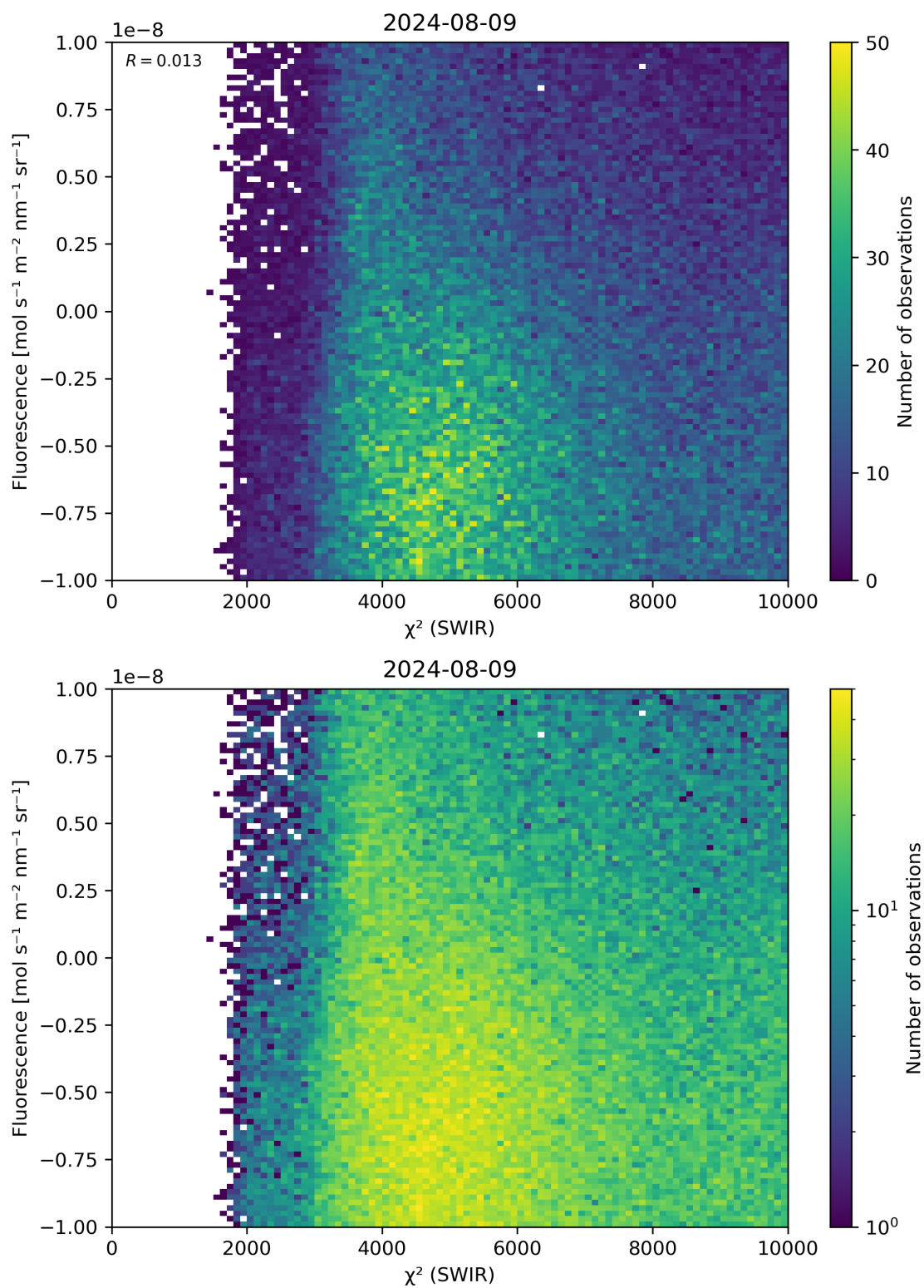
Figure 49: Scatter density plot of “ \chi^2 (SWIR)” against “Fluorescence” for 2024-08-08 to 2024-08-10.
