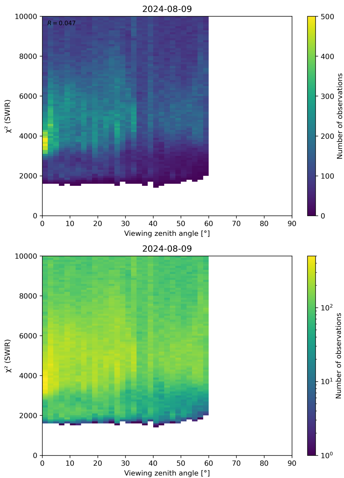
Figure 106: Scatter density plot of “Viewing zenith angle” against “ \chi^2 (SWIR)” for 2024-08-08 to 2024-08-10.
