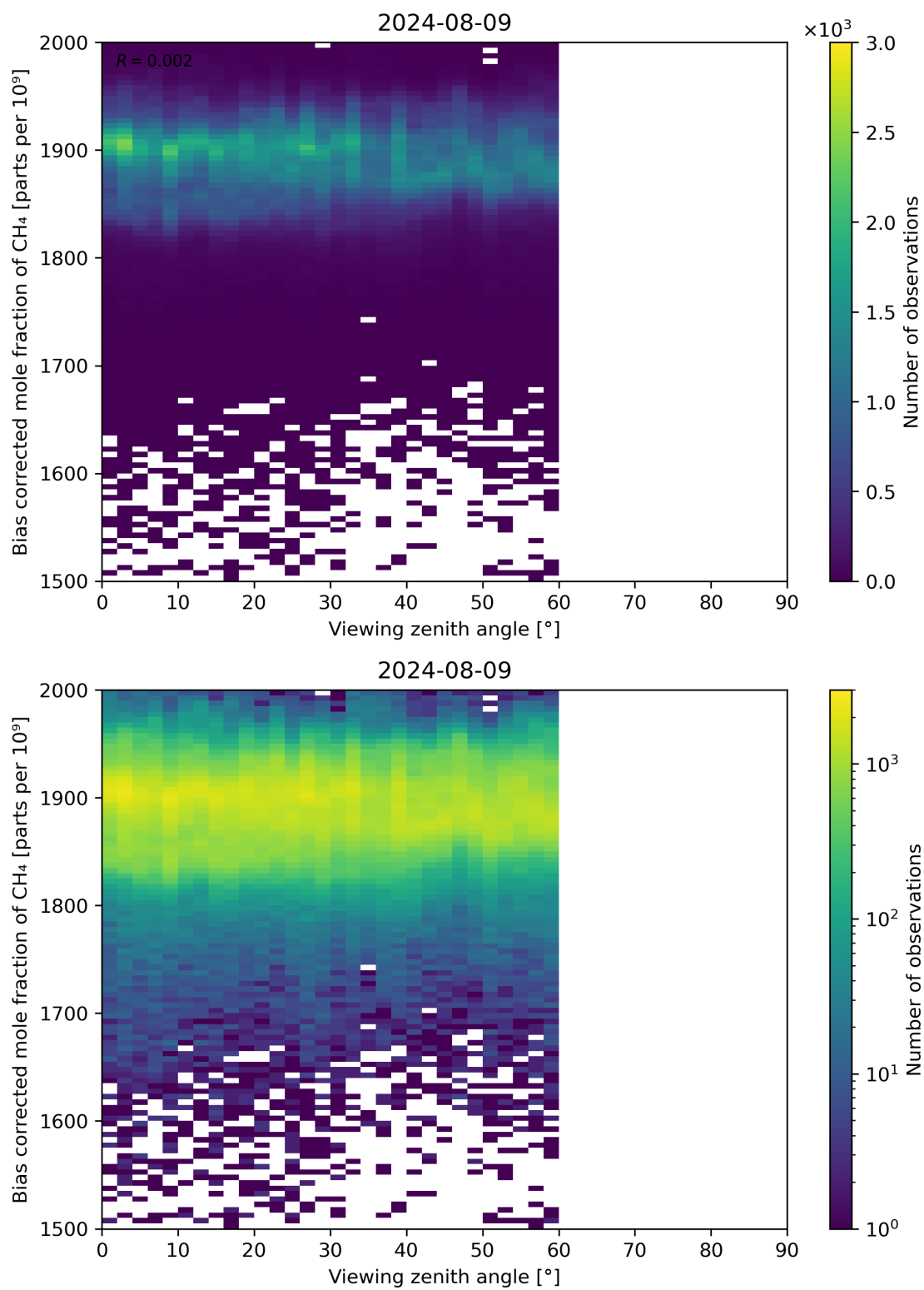
Figure 111: Scatter density plot of “Viewing zenith angle” against “Bias corrected mole fraction of CH 4 ” for 2024-08-08 to 2024-08-10.
