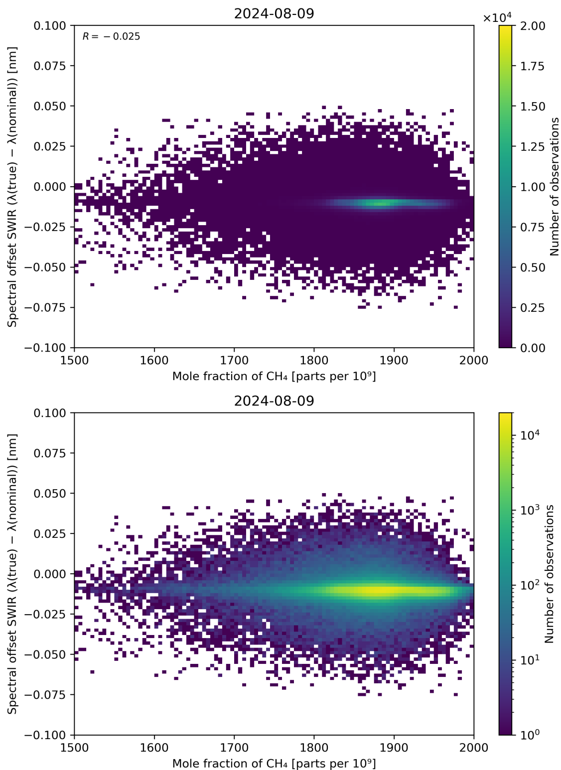
Figure 86: Scatter density plot of “Mole fraction of CH 4 ” against “Spectral offset SWIR ( \lambda(\text{true}) - \lambda(\text{nominal}) )” for 2024-08-08 to 2024-08-10.
