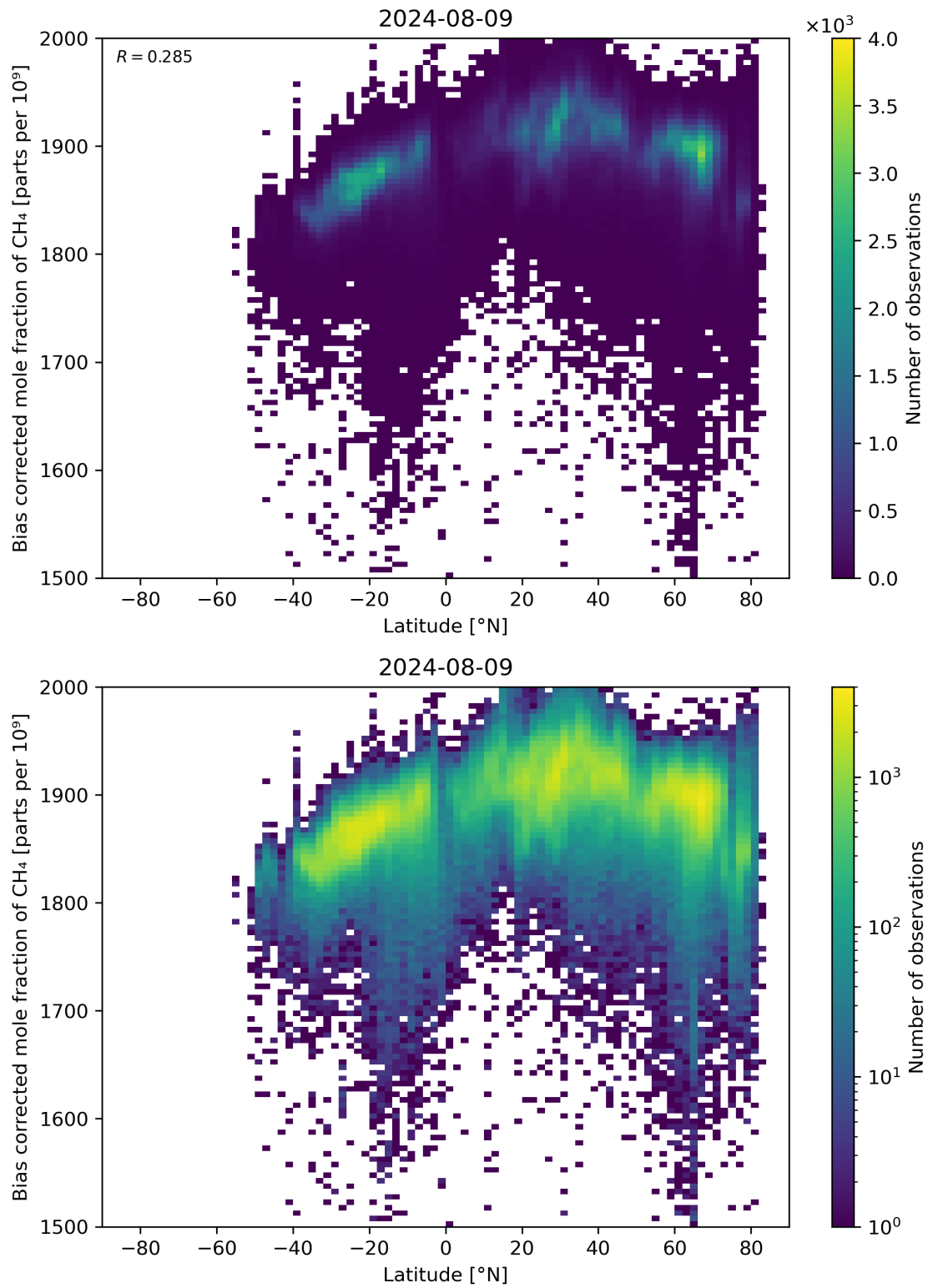
Figure 58: Scatter density plot of “Latitude” against “Bias corrected mole fraction of \text{CH}_4 ” for 2024-08-08 to 2024-08-10.
