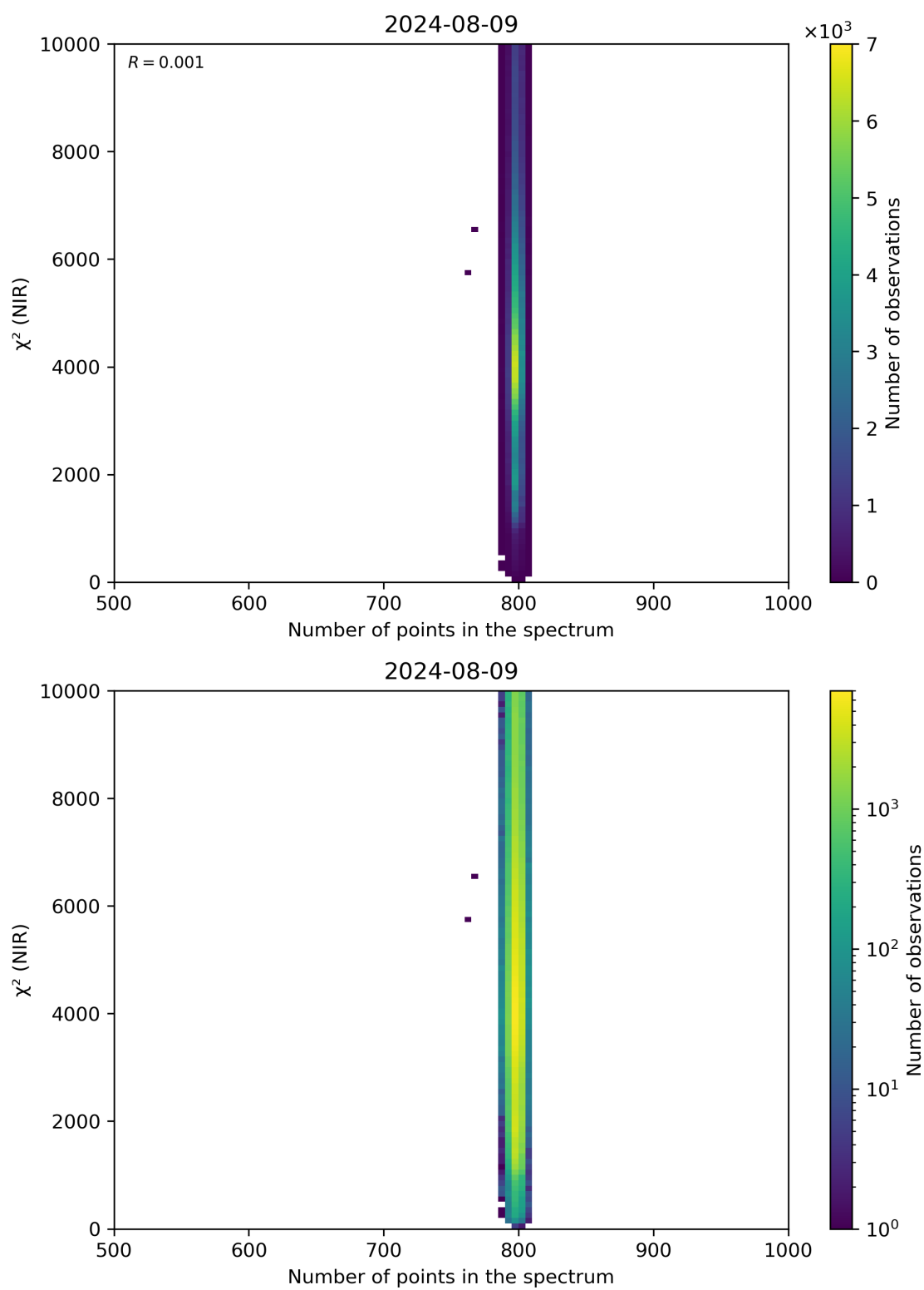
Figure 88: Scatter density plot of “Number of points in the spectrum” against “ \chi^2 (NIR)” for 2024-08-08 to 2024-08-10.
