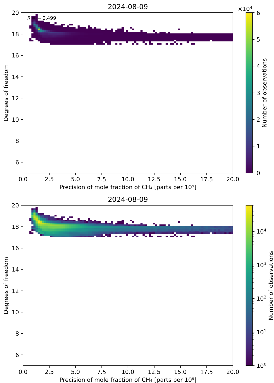
Figure 80: Scatter density plot of “Precision of mole fraction of CH 4 ” against “Degrees of freedom” for 2024-08-08 to 2024-08-10.
