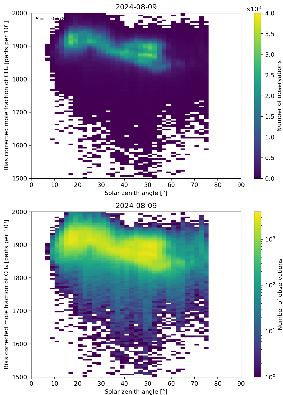
Figure 100: Scatter density plot of “Solar zenith angle” against “Bias corrected mole fraction of CH 4 ” for 2024-08-08 to 2024-08-10.
