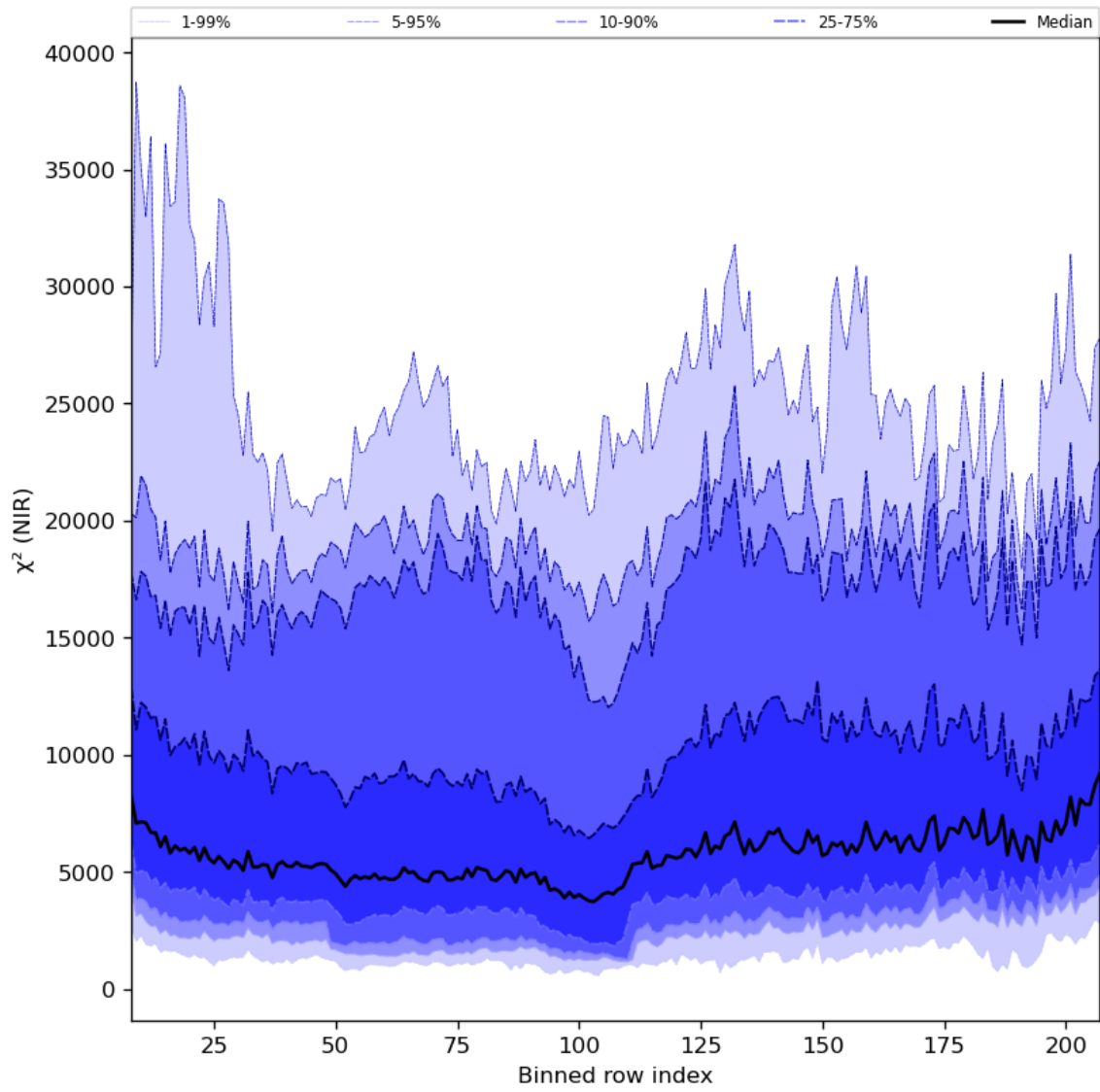
Figure 40: Along track statistics of " \chi^2 (NIR)" for 2024-08-08 to 2024-08-10
