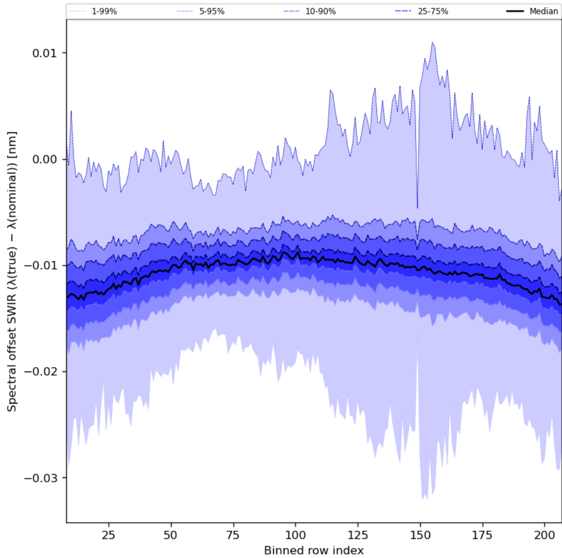
Figure 38: Along track statistics of “Spectral offset SWIR ( \lambda(\text{true}) - \lambda(\text{nominal}) )” for 2024-08-08 to 2024-08-10
