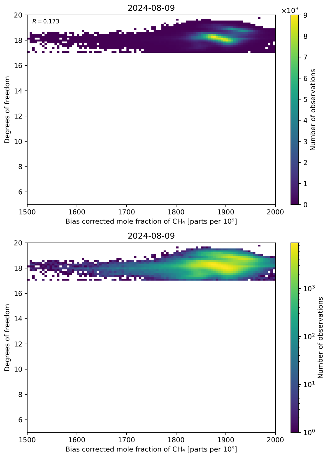
Figure 65: Scatter density plot of “Bias corrected mole fraction of CH 4 ” against “Degrees of freedom” for 2024-08-08 to 2024-08-10.
