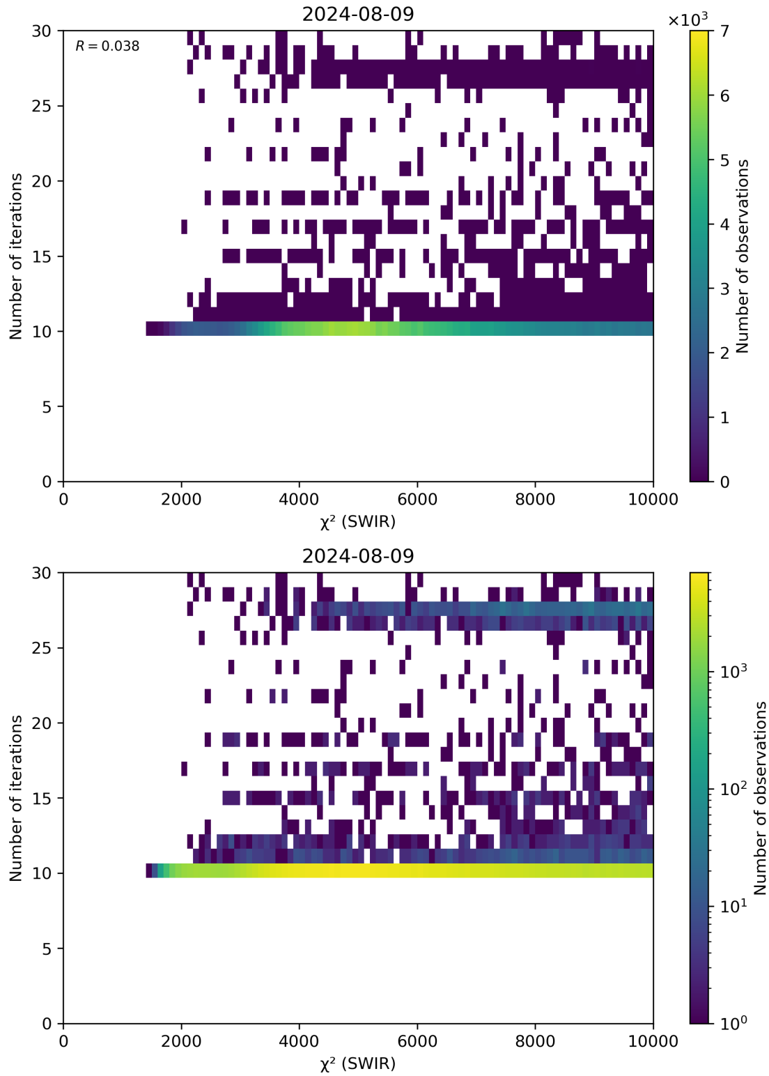
Figure 50: Scatter density plot of “ \chi^2 (SWIR)” against “Number of iterations” for 2024-08-08 to 2024-08-10.
