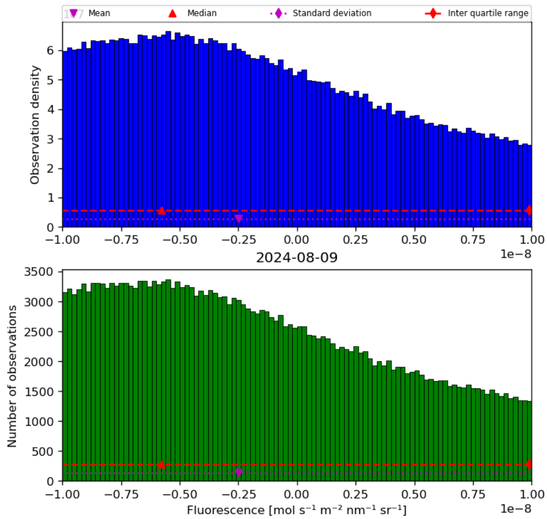
Figure 32: Histogram of “Fluorescence” for 2024-08-08 to 2024-08-10
