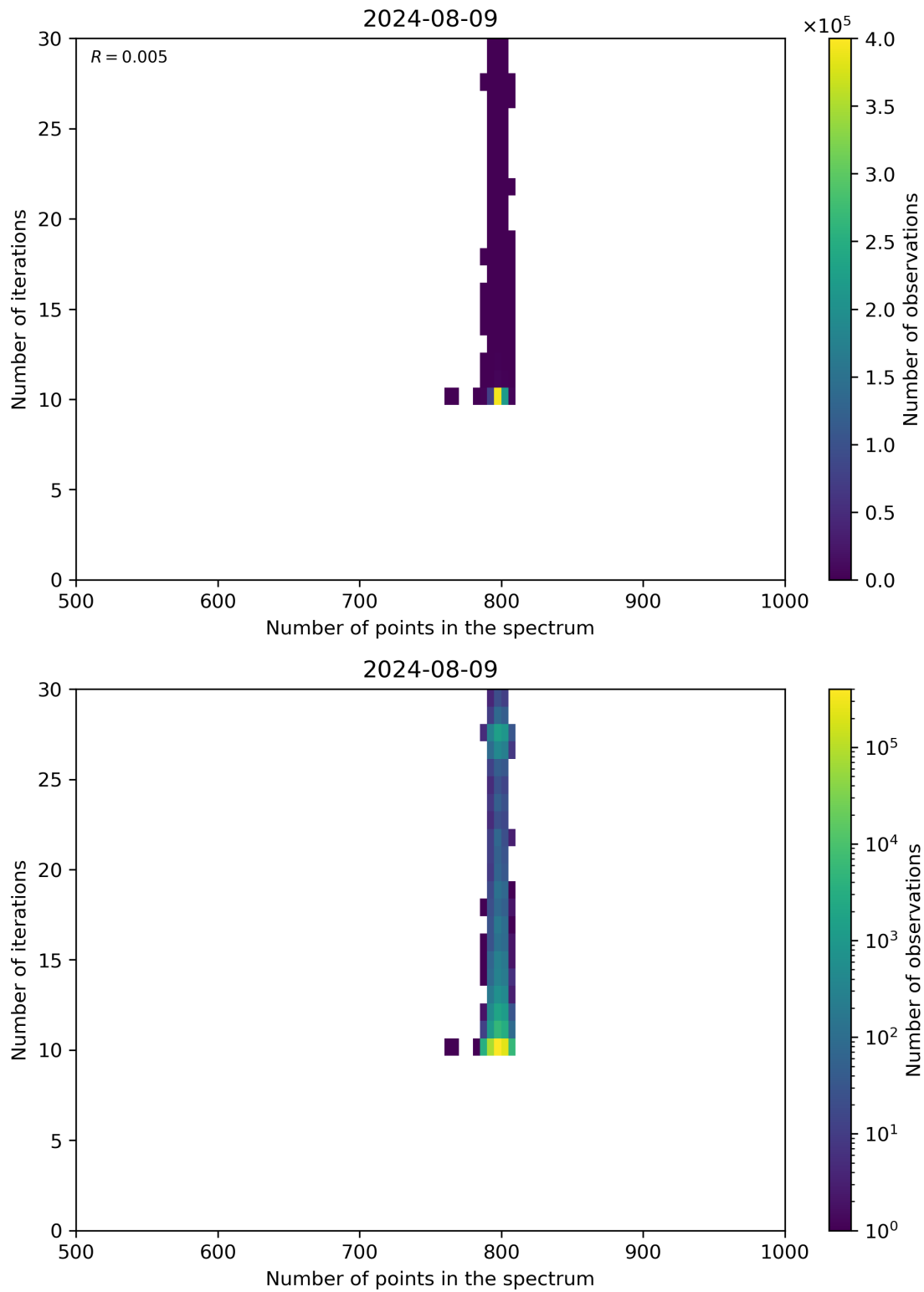
Figure 92: Scatter density plot of “Number of points in the spectrum” against “Number of iterations” for 2024-08-08 to 2024-08-10.
