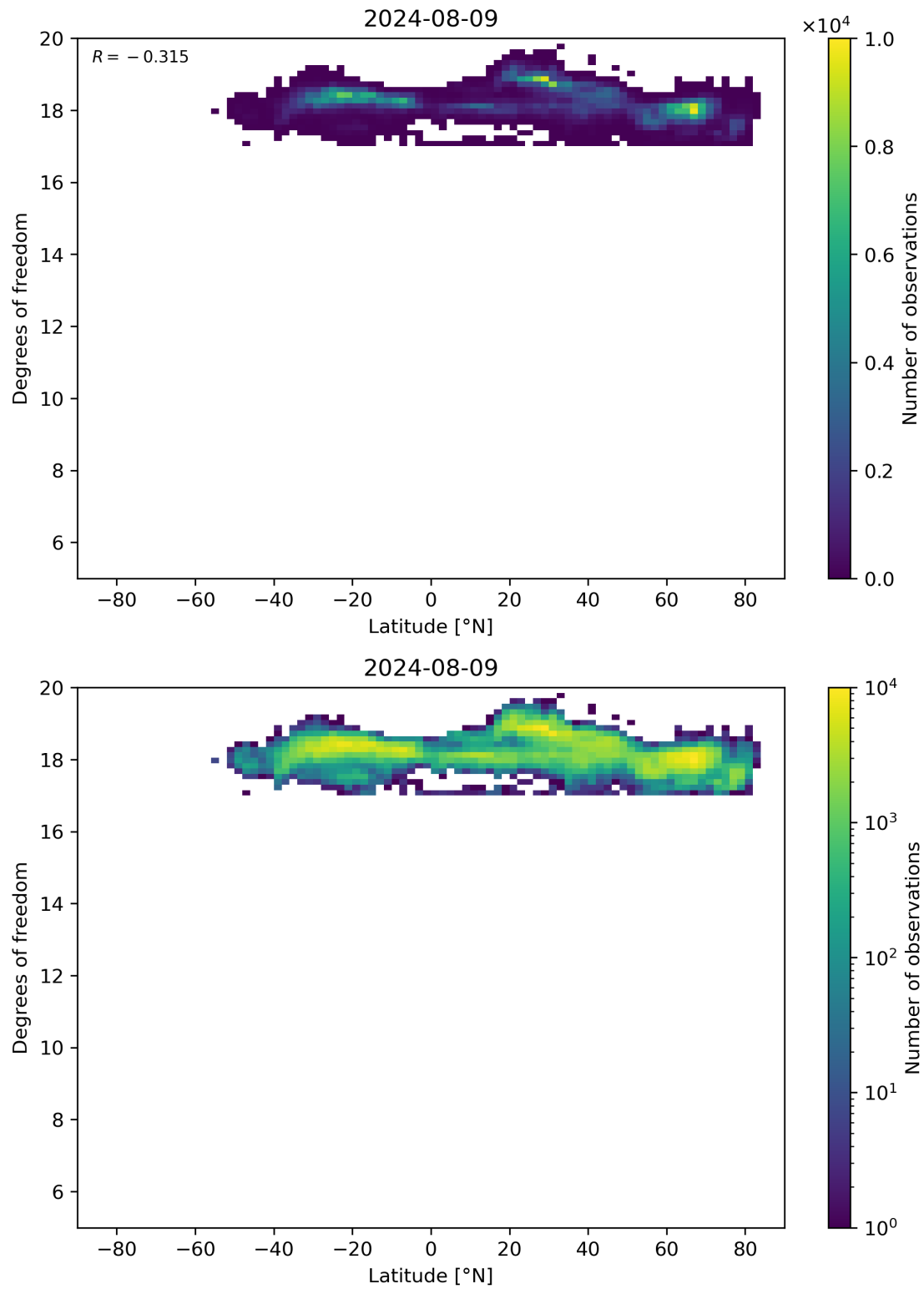
Figure 55: Scatter density plot of “Latitude” against “Degrees of freedom” for 2024-08-08 to 2024-08-10.
