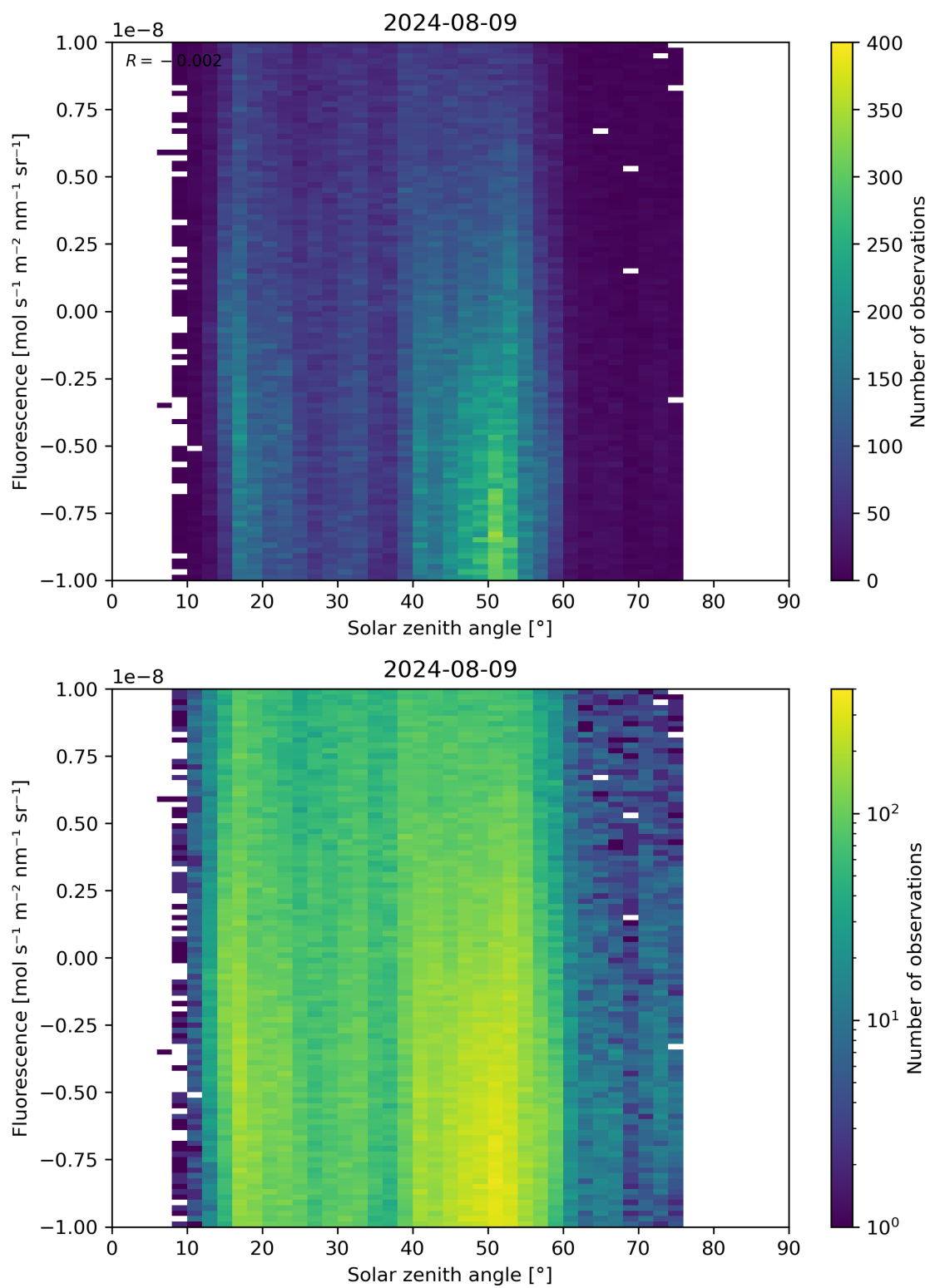
Figure 97: Scatter density plot of “Solar zenith angle” against “Fluorescence” for 2024-08-08 to 2024-08-10.
