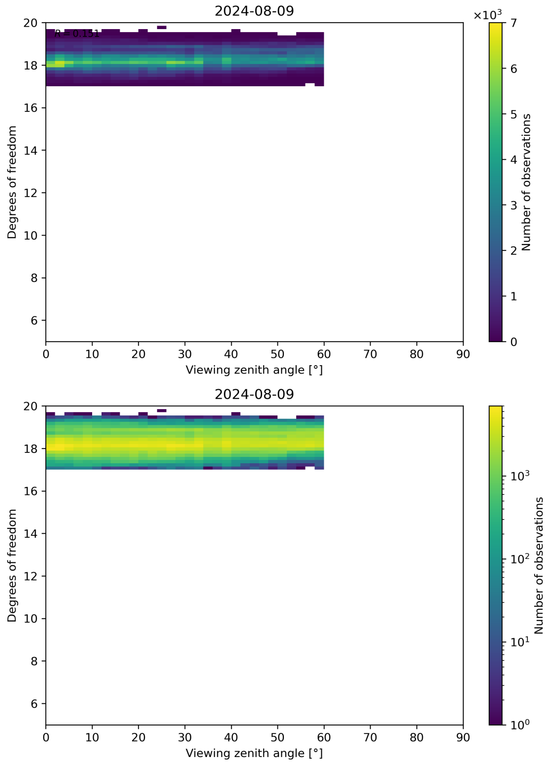
Figure 107: Scatter density plot of “Viewing zenith angle” against “Degrees of freedom” for 2024-08-08 to 2024-08-10.
