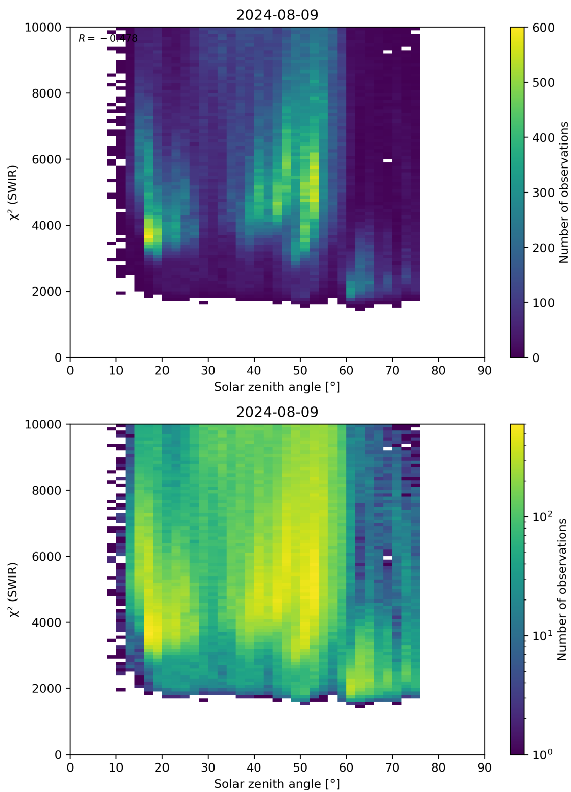
Figure 95: Scatter density plot of “Solar zenith angle” against “ \chi^2 (SWIR)” for 2024-08-08 to 2024-08-10.
