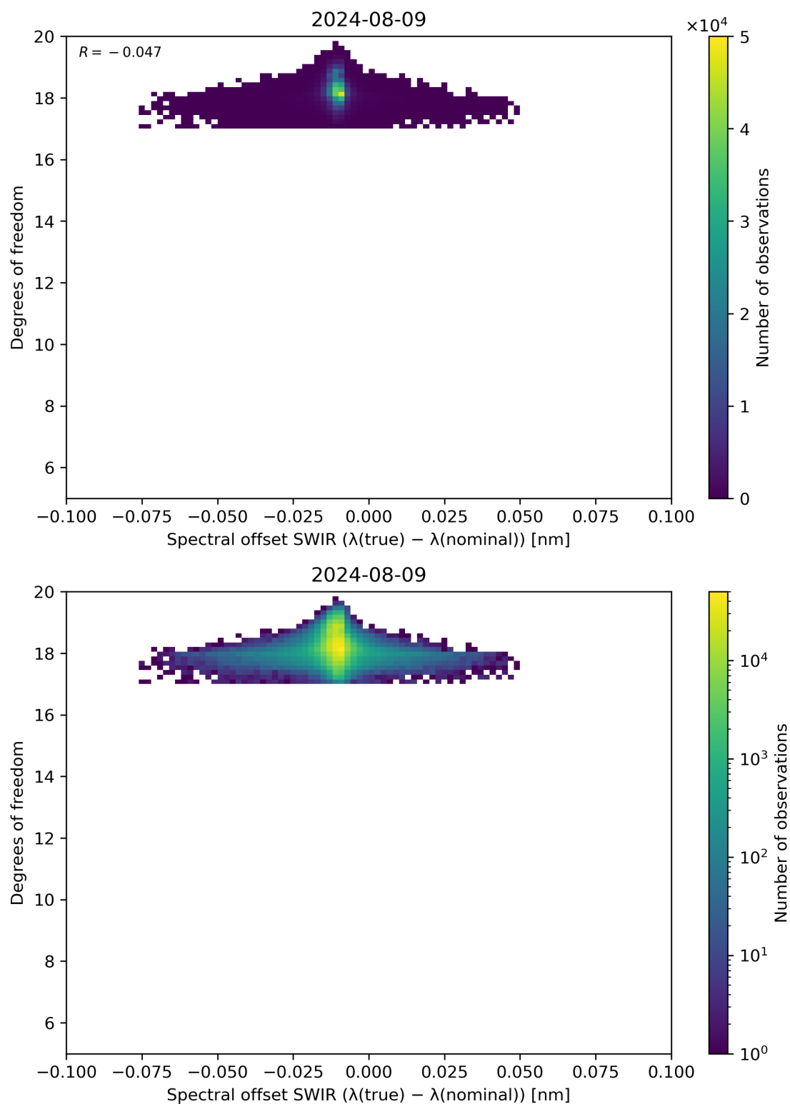
Figure 119: Scatter density plot of “Spectral offset SWIR ( \lambda(\text{true}) - \lambda(\text{nominal}) )” against “Degrees of freedom” for 2024-08-08 to 2024-08-10.
