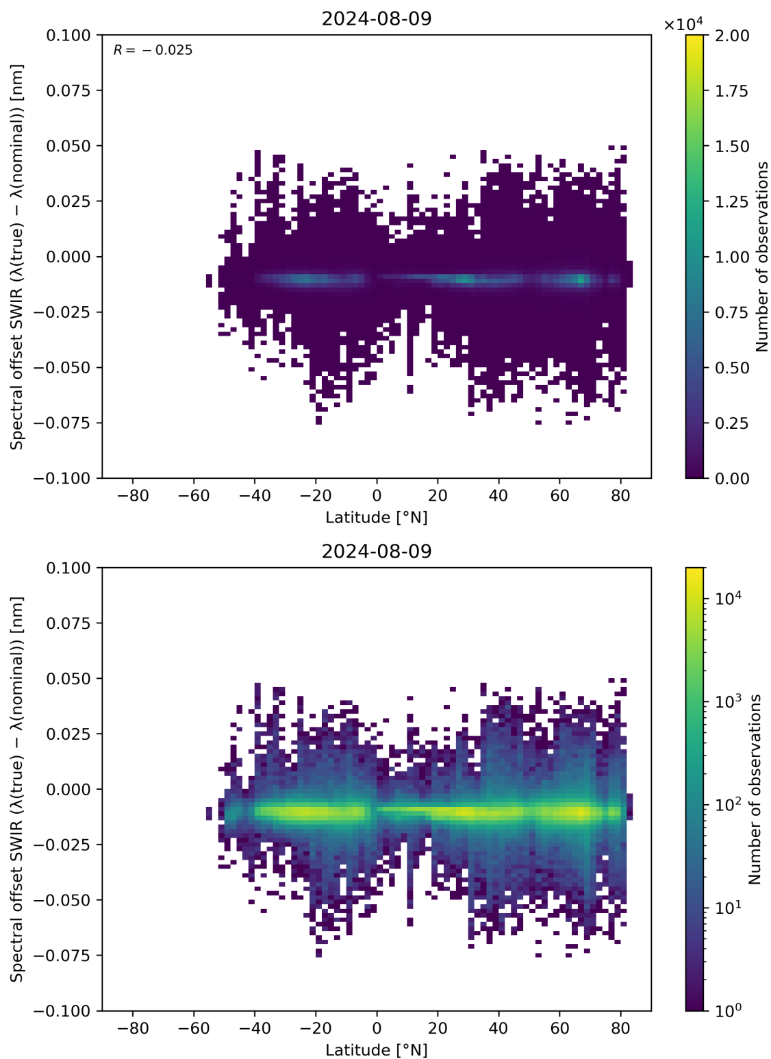
Figure 62: Scatter density plot of “Latitude” against “Spectral offset SWIR ( \lambda(\text{true}) - \lambda(\text{nominal}) )” for 2024-08-08 to 2024-08-10.
