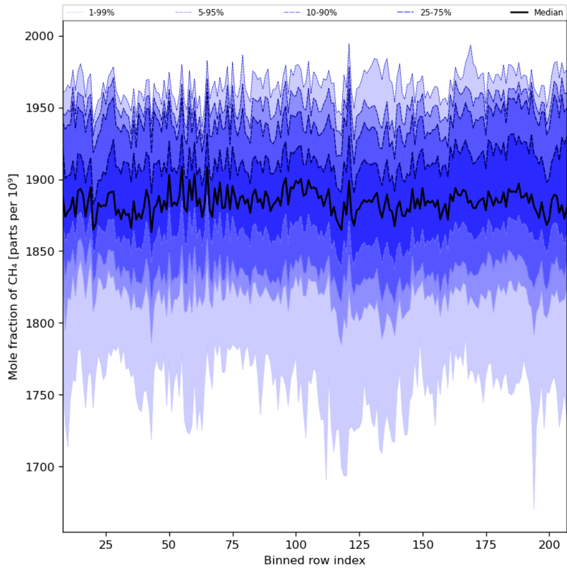
Figure 34: Along track statistics of “Mole fraction of CH 4 ” for 2024-08-08 to 2024-08-10
