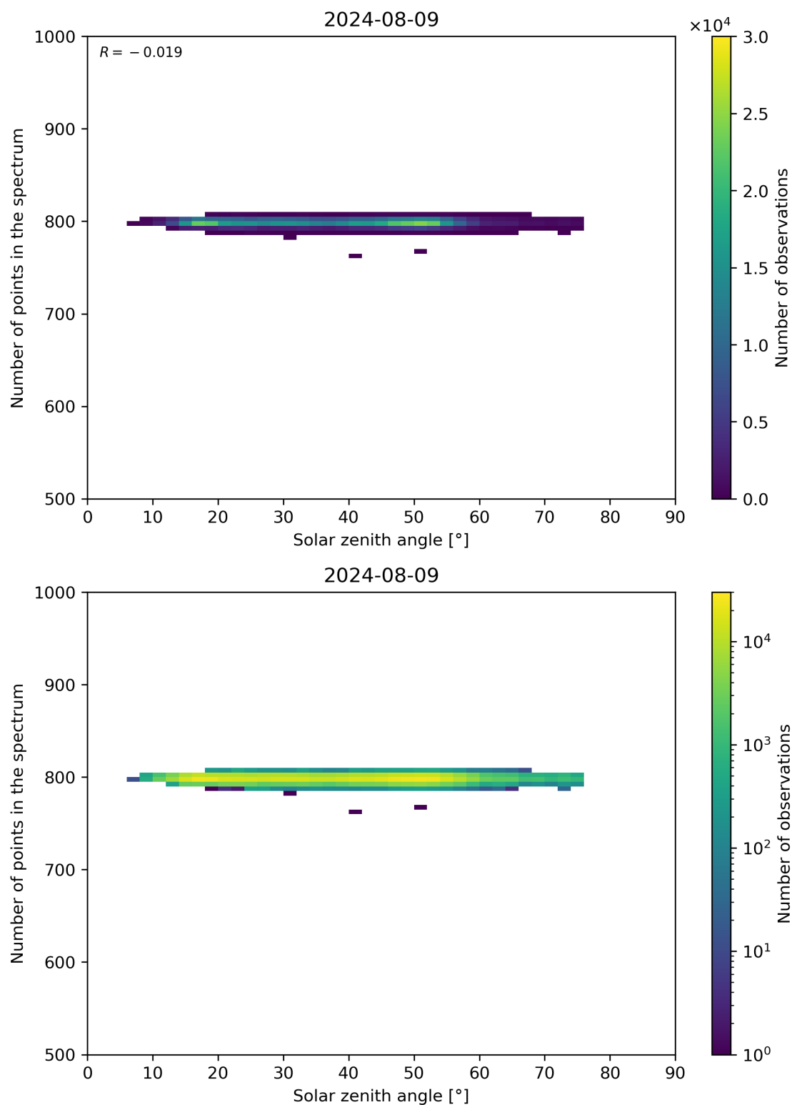
Figure 103: Scatter density plot of “Solar zenith angle” against “Number of points in the spectrum” for 2024-08-08 to 2024-08-10.
