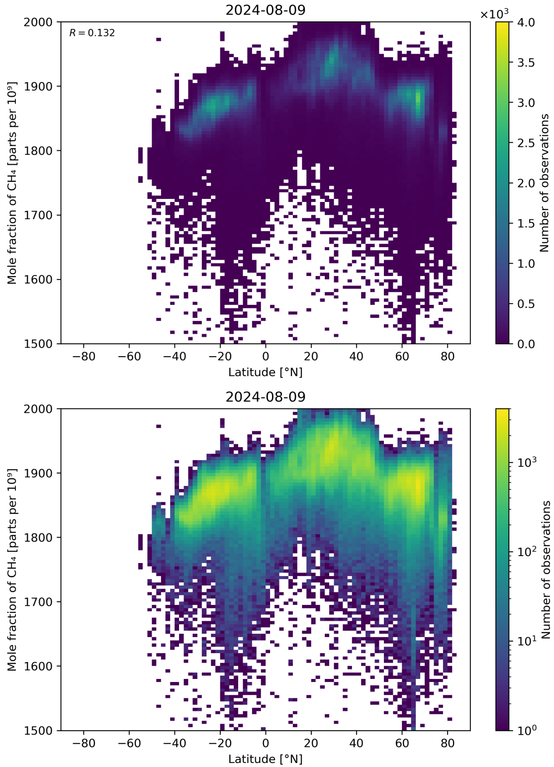
Figure 57: Scatter density plot of “Latitude” against “Mole fraction of CH 4 ” for 2024-08-08 to 2024-08-10.
