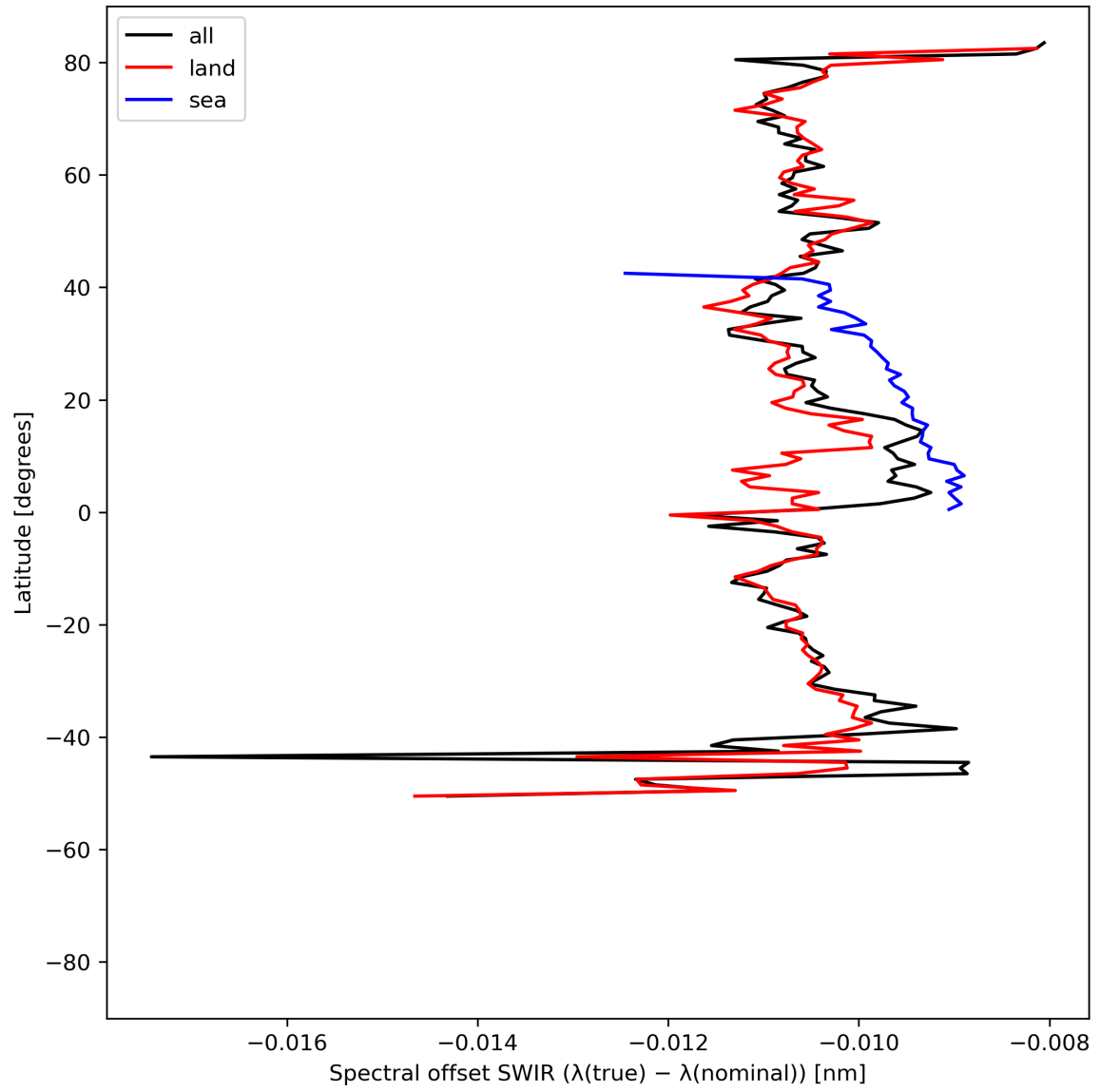
Figure 16: Zonal average of “Spectral offset SWIR ( \lambda(\text{true}) - \lambda(\text{nominal}) )” for 2024-08-08 to 2024-08-10.
