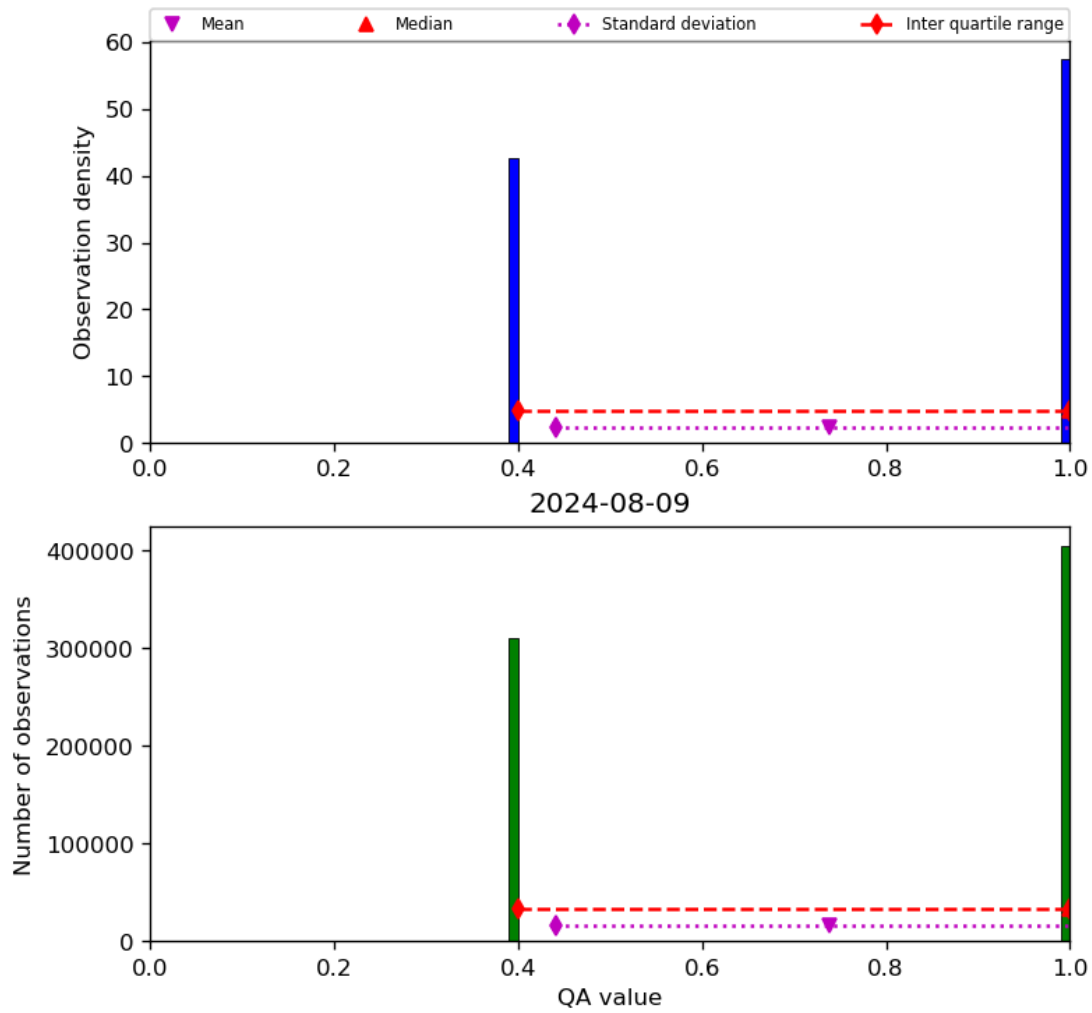
Figure 22: Histogram of “QA value” for 2024-08-08 to 2024-08-10
