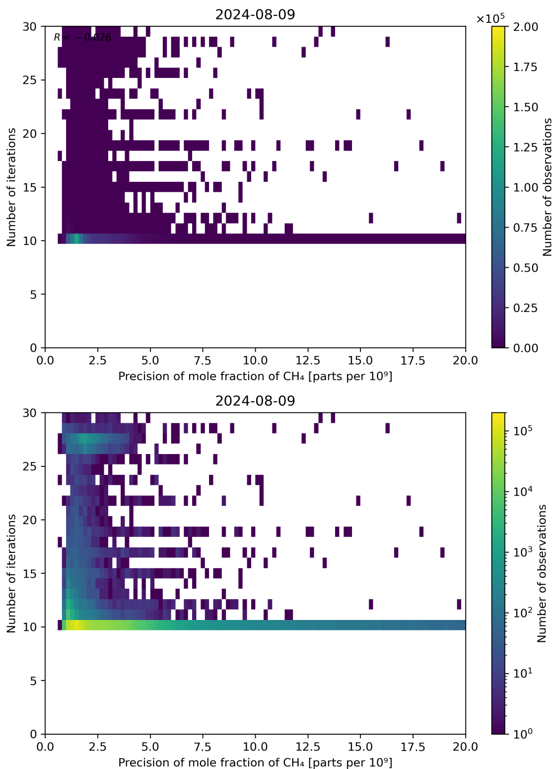
Figure 83: Scatter density plot of “Precision of mole fraction of CH 4 ” against “Number of iterations” for 2024-08-08 to 2024-08-10.
