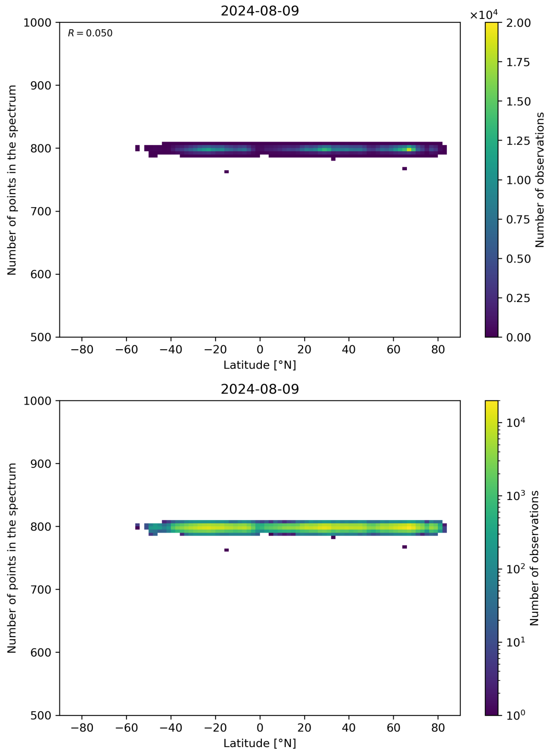
Figure 61: Scatter density plot of “Latitude” against “Number of points in the spectrum” for 2024-08-08 to 2024-08-10.
