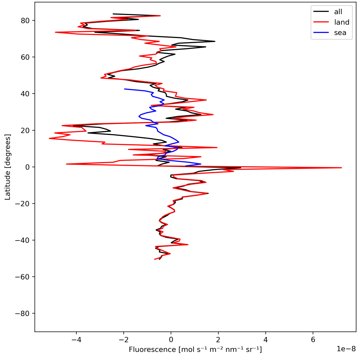
Figure 21: Zonal average of “Fluorescence” for 2024-08-08 to 2024-08-10.
