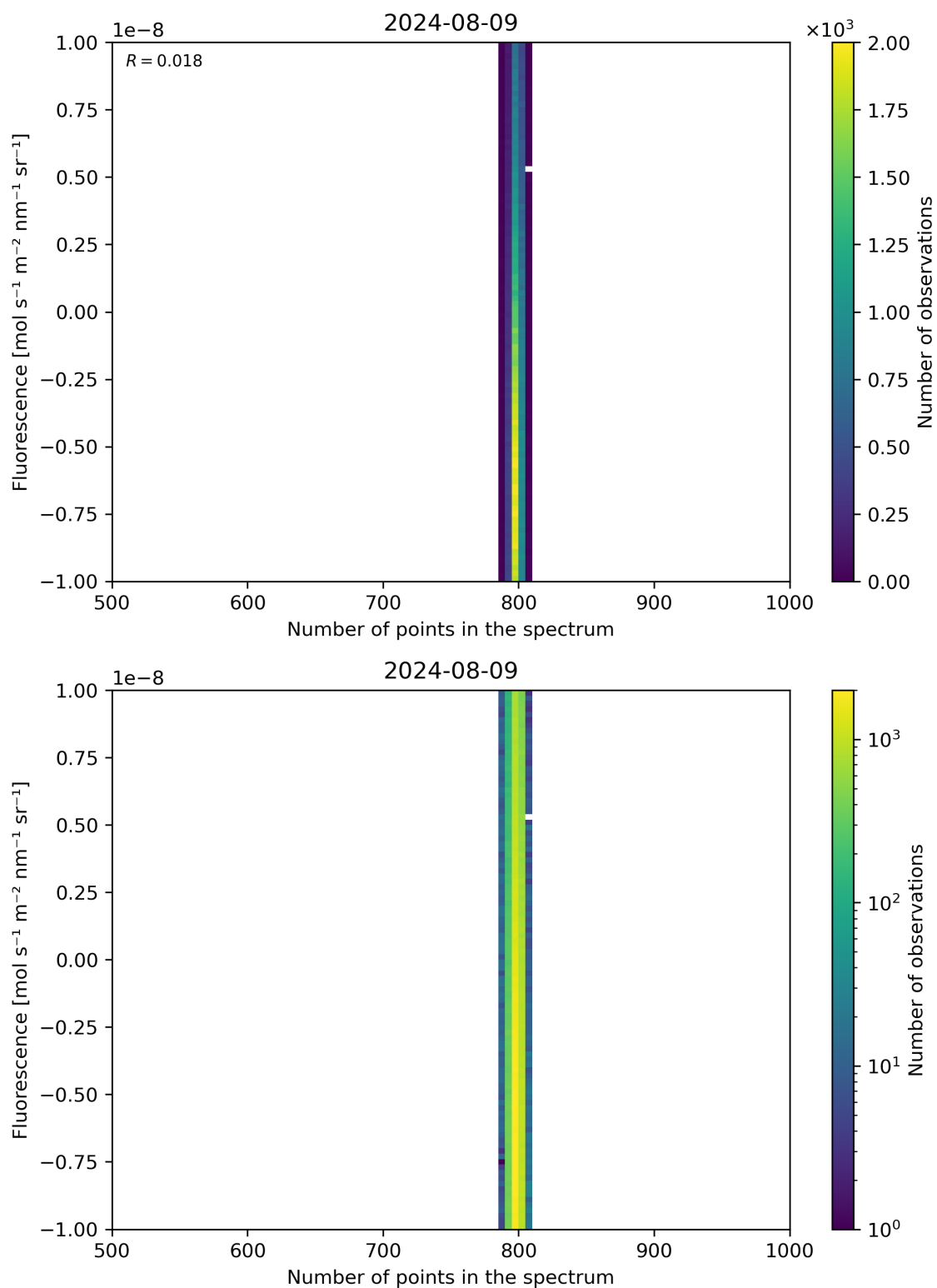
Figure 91: Scatter density plot of “Number of points in the spectrum” against “Fluorescence” for 2024-08-08 to 2024-08-10.
