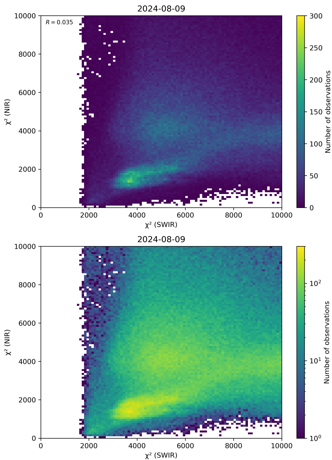
Figure 47: Scatter density plot of “ \chi^2 (SWIR)” against “ \chi^2 (NIR)” for 2024-08-08 to 2024-08-10.
