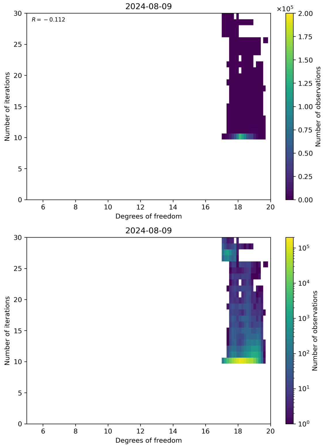
Figure 52: Scatter density plot of “Degrees of freedom” against “Number of iterations” for 2024-08-08 to 2024-08-10.
