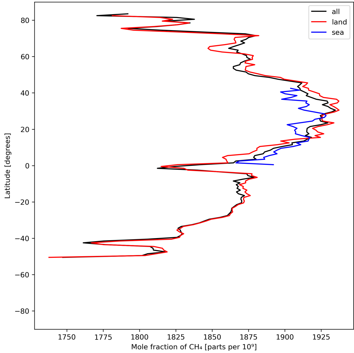
Figure 12: Zonal average of “Mole fraction of \text{CH}_4 ” for 2024-08-08 to 2024-08-10.
