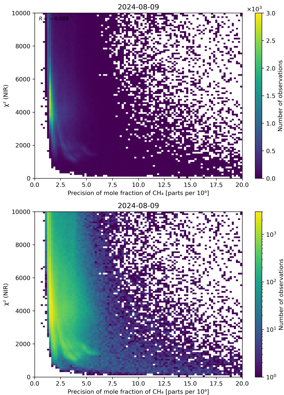
Figure 78: Scatter density plot of “Precision of mole fraction of CH 4 ” against “ \chi^2 (NIR)” for 2024-08-08 to 2024-08-10.
