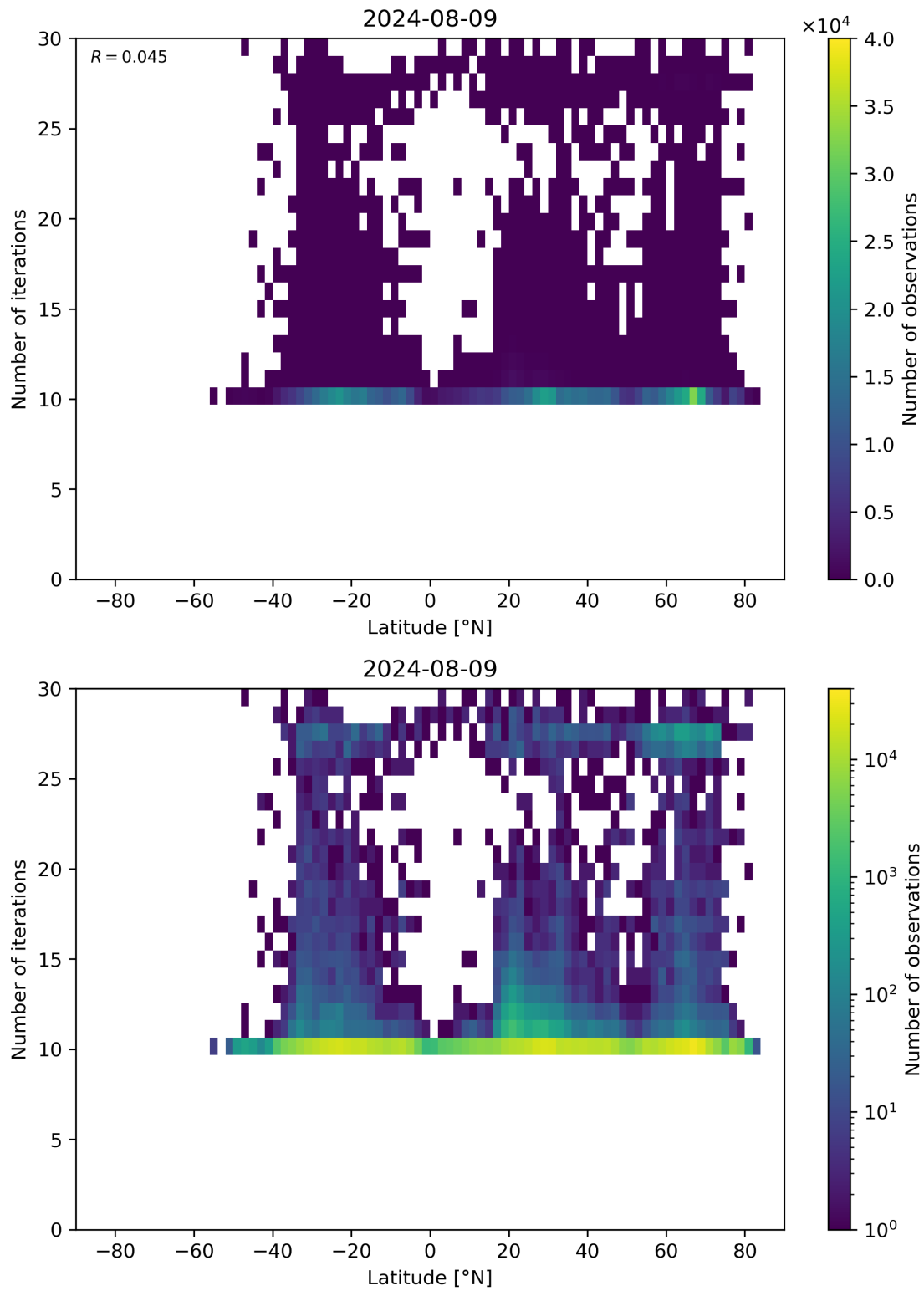
Figure 60: Scatter density plot of “Latitude” against “Number of iterations” for 2024-08-08 to 2024-08-10.
