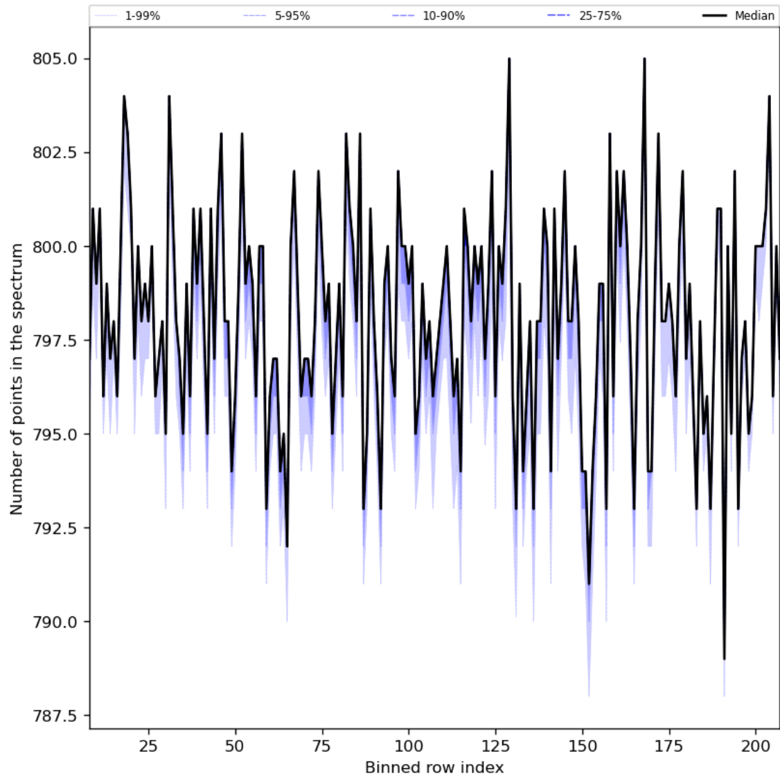
Figure 37: Along track statistics of “Number of points in the spectrum” for 2024-08-08 to 2024-08-10
