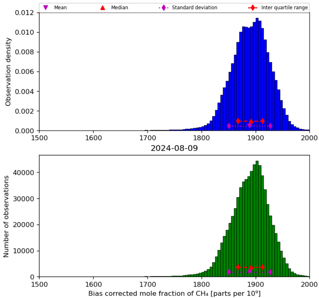
Figure 25: Histogram of “Bias corrected mole fraction of CH 4 ” for 2024-08-08 to 2024-08-10
