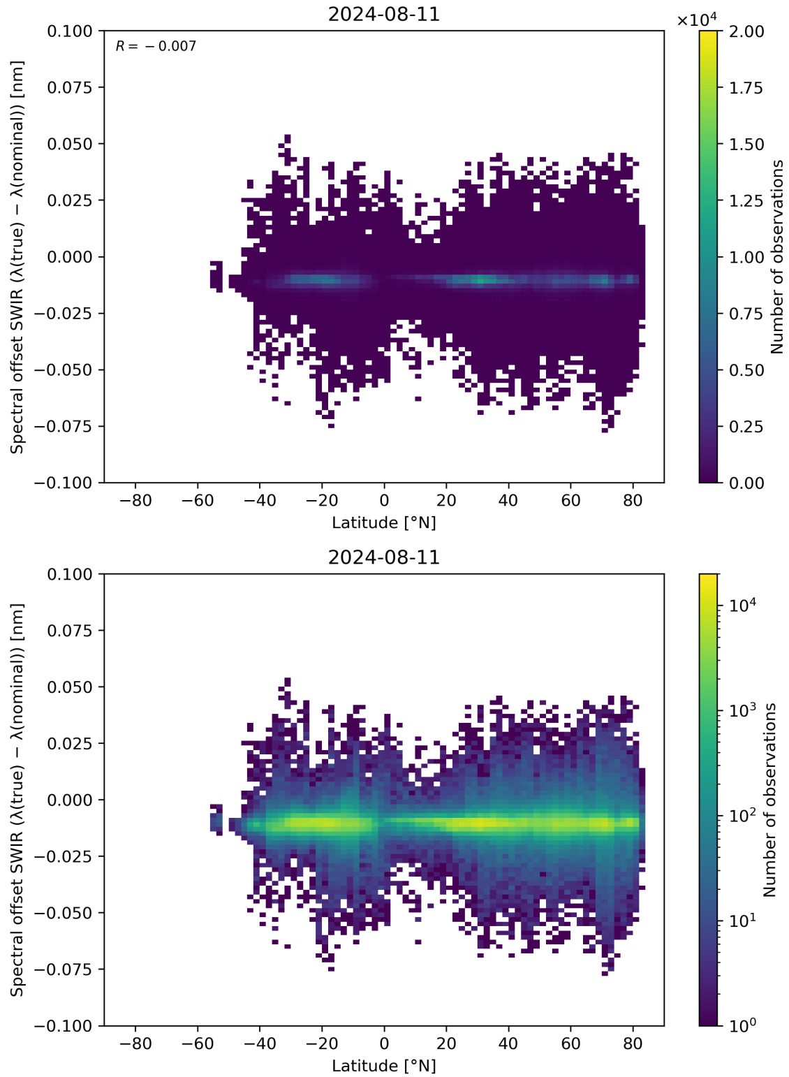
Figure 62: Scatter density plot of “Latitude” against “Spectral offset SWIR ( \lambda(\text{true}) - \lambda(\text{nominal}) )” for 2024-08-11 to 2024-08-11.
