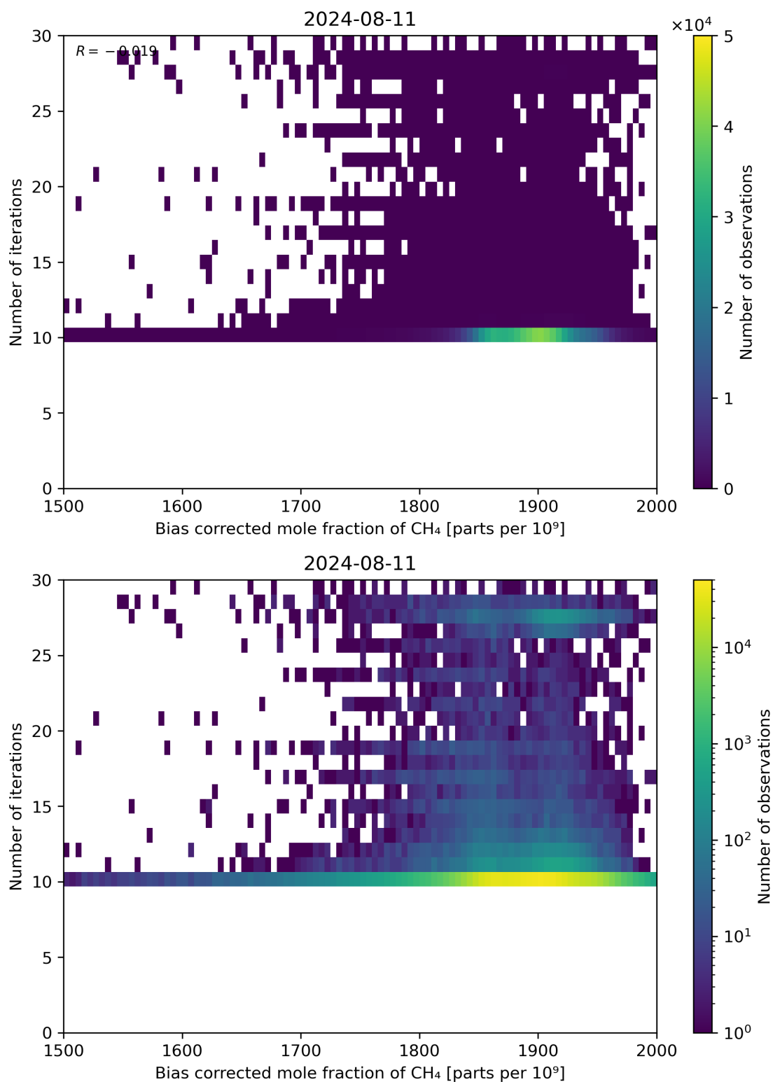
Figure 67: Scatter density plot of “Bias corrected mole fraction of CH 4 ” against “Number of iterations” for 2024-08-11 to 2024-08-11.
