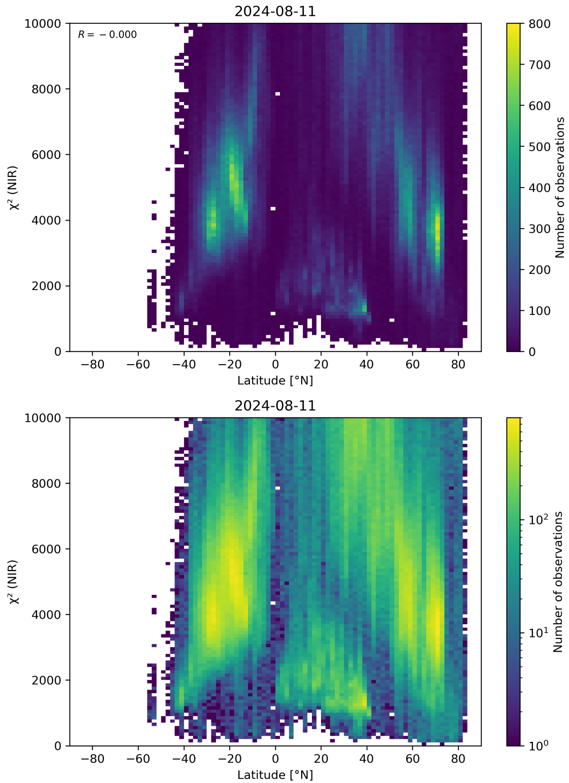
Figure 53: Scatter density plot of “Latitude” against “ \chi^2 (NIR)” for 2024-08-11 to 2024-08-11.
