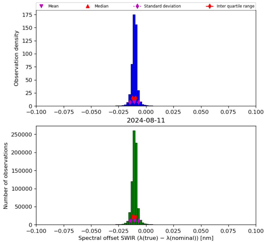
Figure 27: Histogram of “Spectral offset SWIR ( \lambda(\text{true}) - \lambda(\text{nominal}) )” for 2024-08-11 to 2024-08-11
