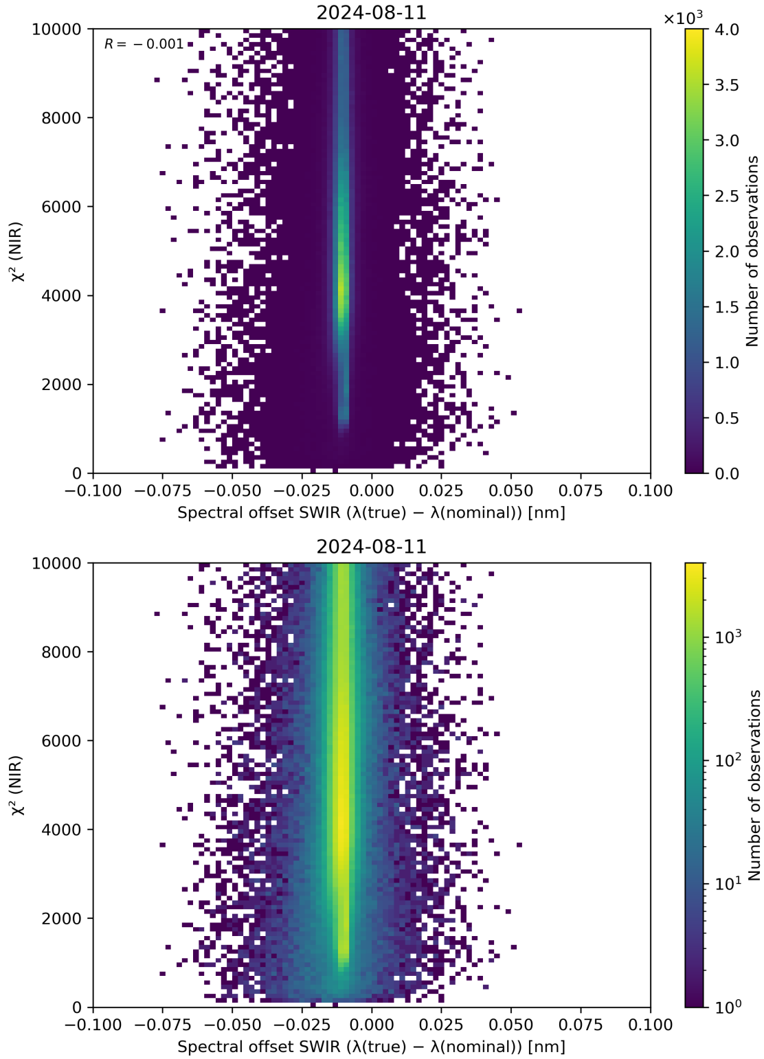
Figure 117: Scatter density plot of “Spectral offset SWIR ( \lambda(\text{true}) - \lambda(\text{nominal}) )” against “ \chi^2 (NIR)” for 2024-08-11 to 2024-08-11.
