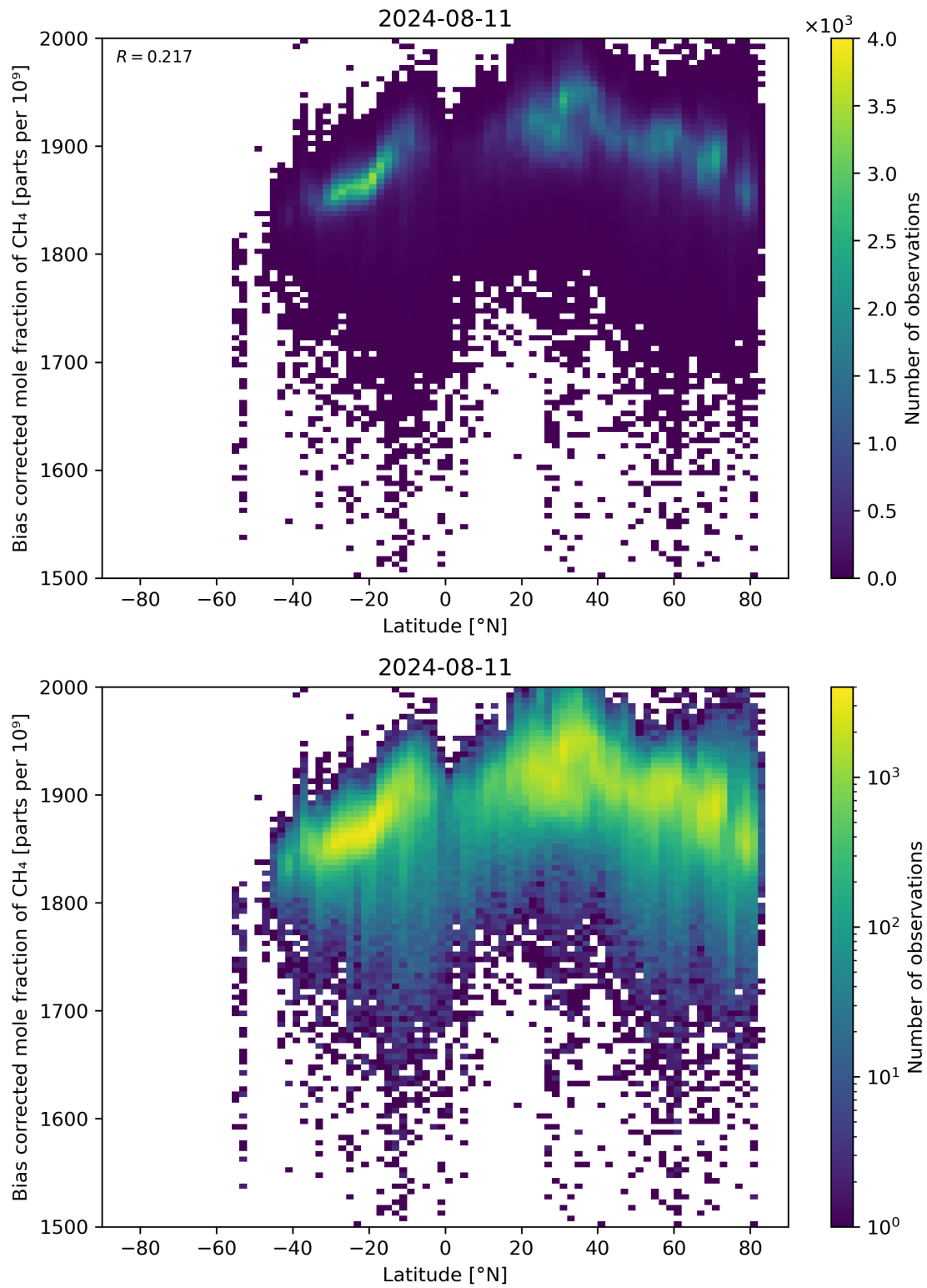
Figure 58: Scatter density plot of “Latitude” against “Bias corrected mole fraction of CH 4 ” for 2024-08-11 to 2024-08-11.
