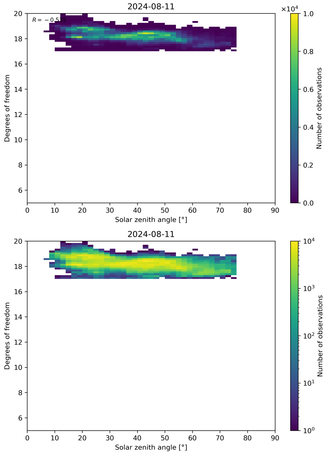
Figure 96: Scatter density plot of “Solar zenith angle” against “Degrees of freedom” for 2024-08-11 to 2024-08-11.
