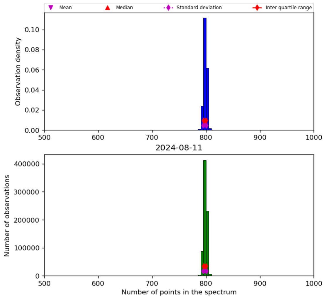
Figure 26: Histogram of “Number of points in the spectrum” for 2024-08-11 to 2024-08-11
