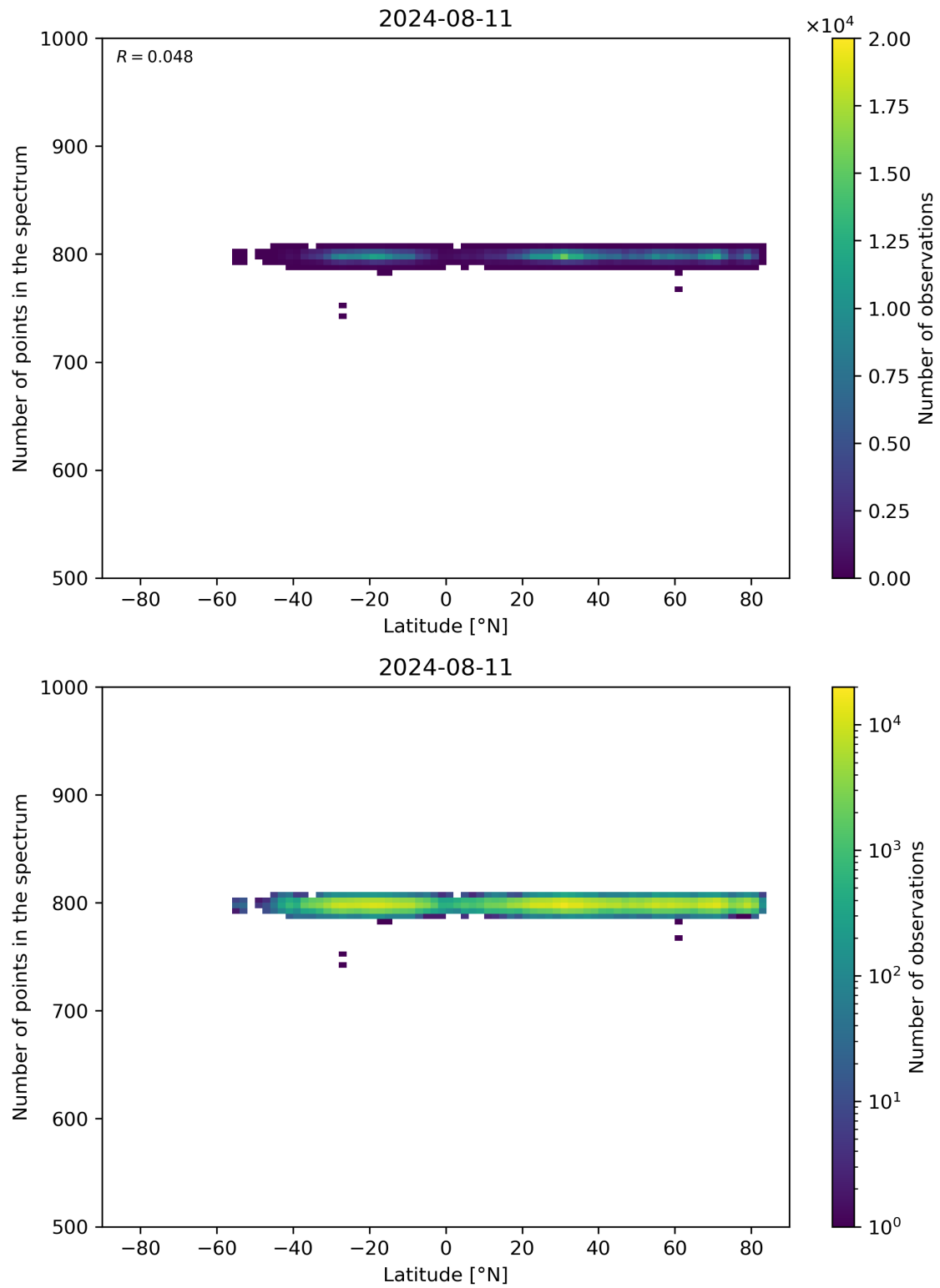
Figure 61: Scatter density plot of “Latitude” against “Number of points in the spectrum” for 2024-08-11 to 2024-08-11.
