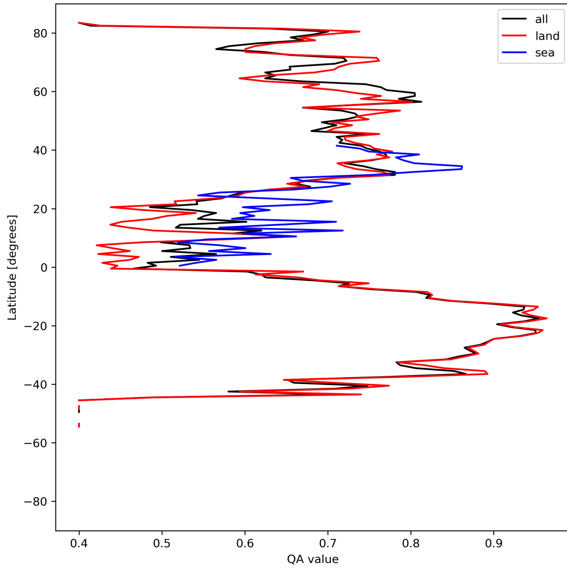
Figure 11: Zonal average of “QA value” for 2024-08-11 to 2024-08-11.
