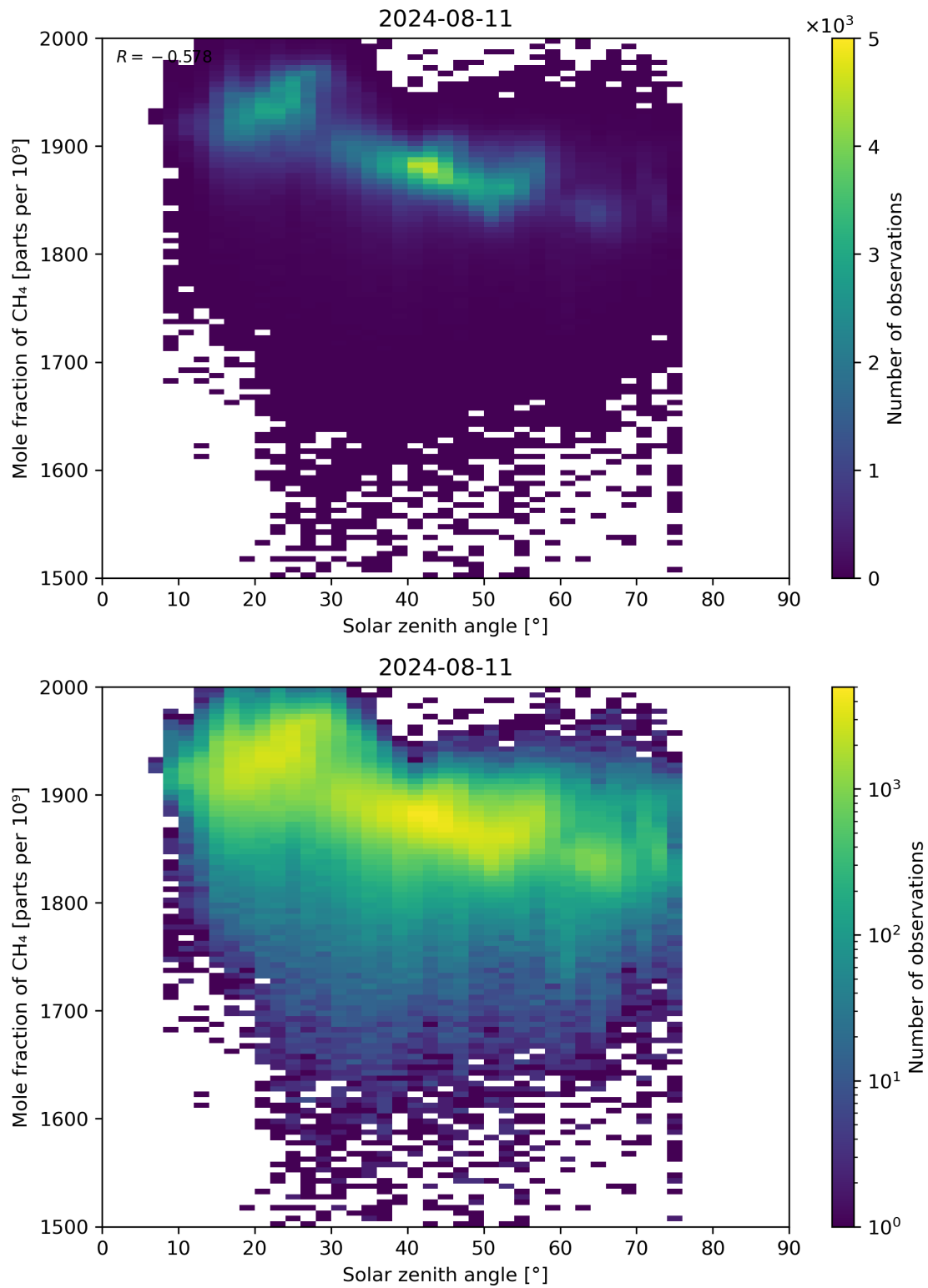
Figure 99: Scatter density plot of “Solar zenith angle” against “Mole fraction of CH 4 ” for 2024-08-11 to 2024-08-11.
