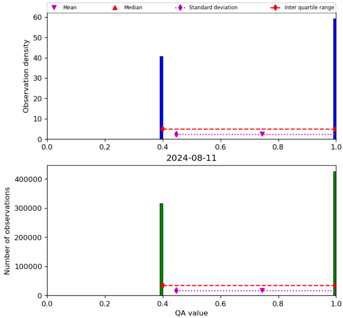
Figure 22: Histogram of “QA value” for 2024-08-11 to 2024-08-11
