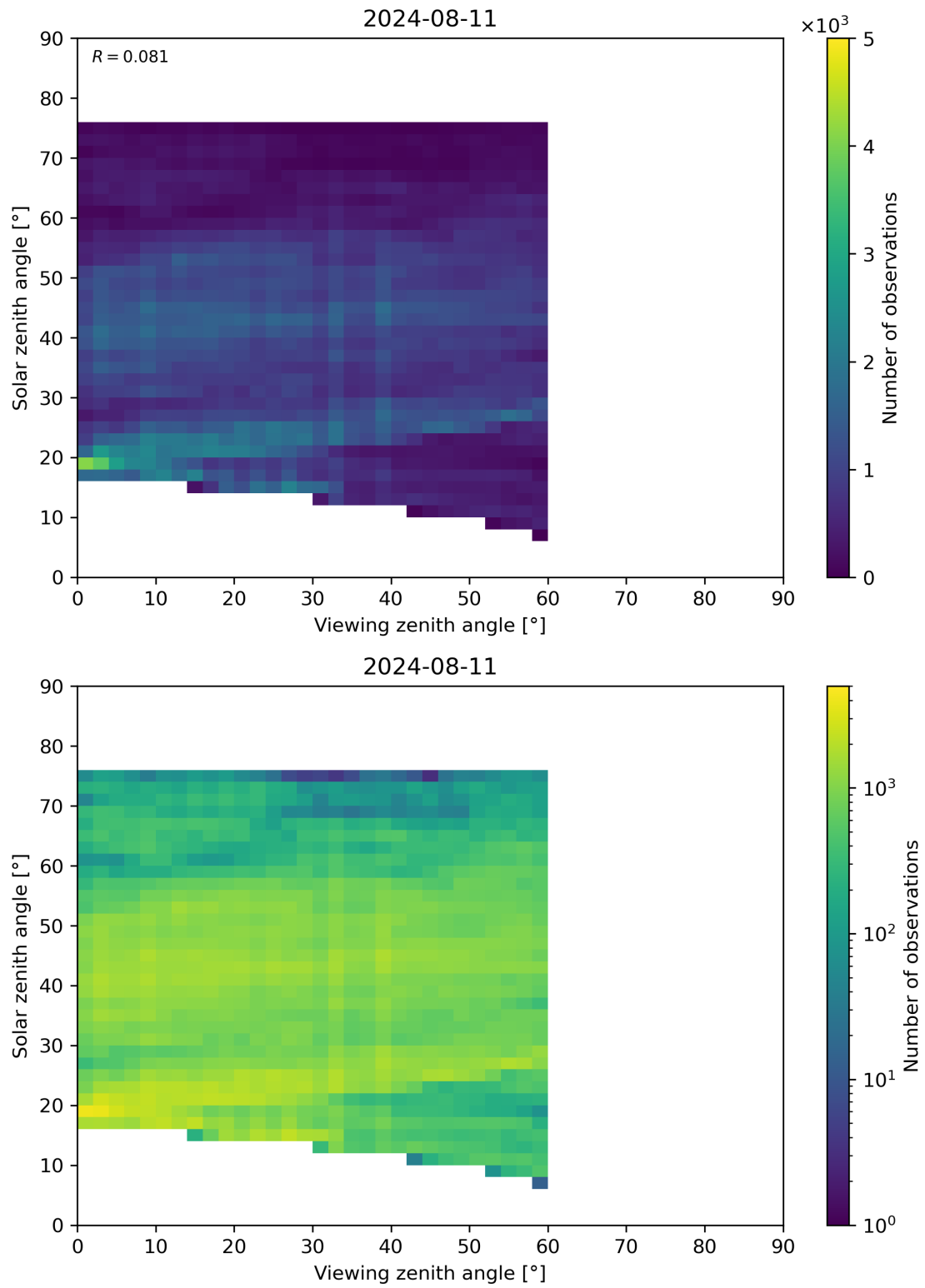
Figure 115: Scatter density plot of “Viewing zenith angle” against “Solar zenith angle” for 2024-08-11 to 2024-08-11.
