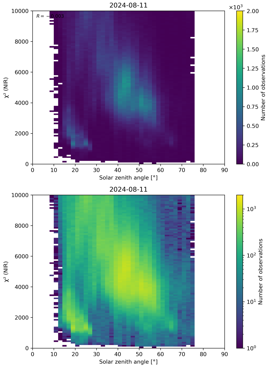
Figure 94: Scatter density plot of “Solar zenith angle” against “ \chi^2 (NIR)” for 2024-08-11 to 2024-08-11.
