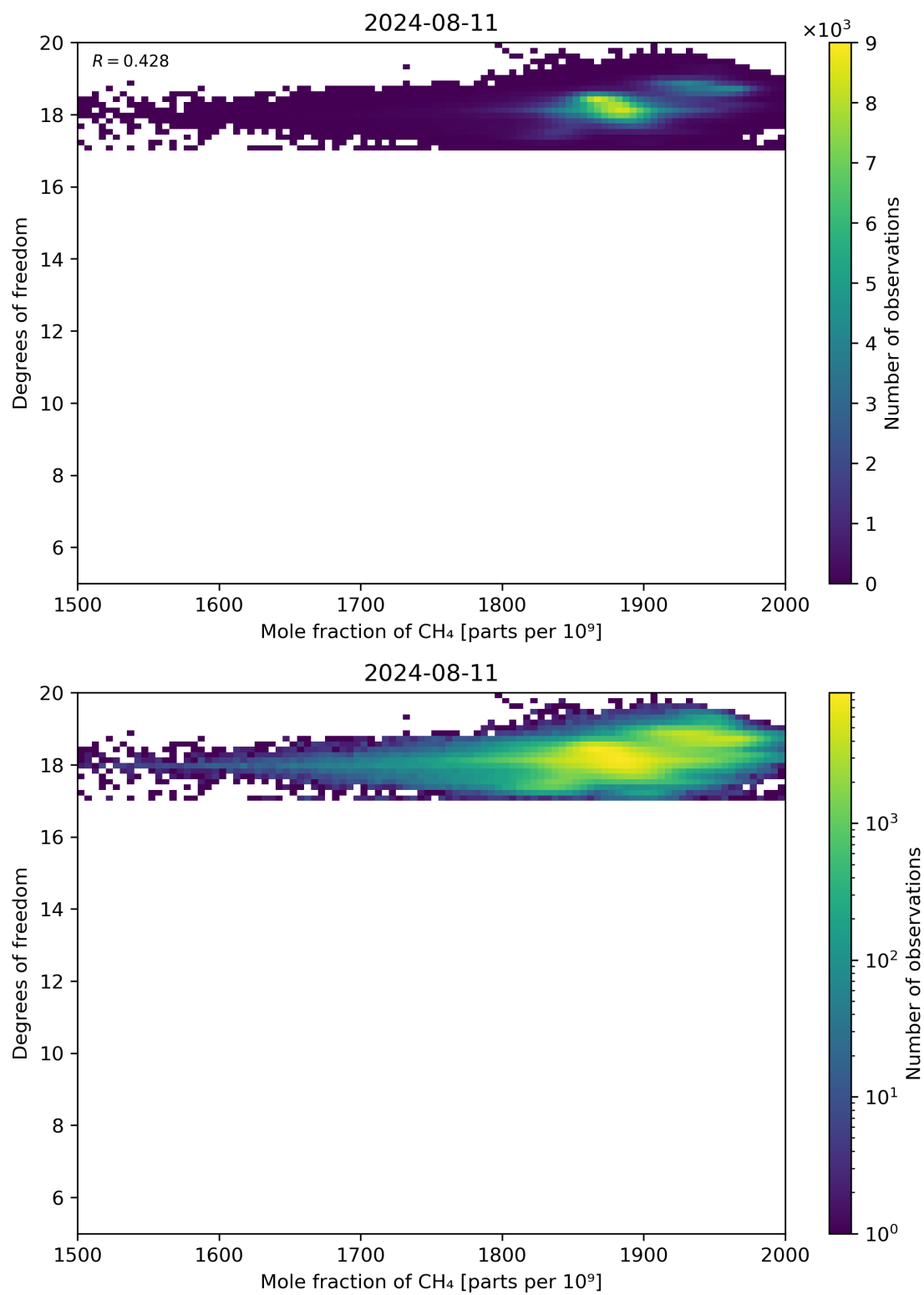
Figure 72: Scatter density plot of “Mole fraction of CH 4 ” against “Degrees of freedom” for 2024-08-11 to 2024-08-11.
