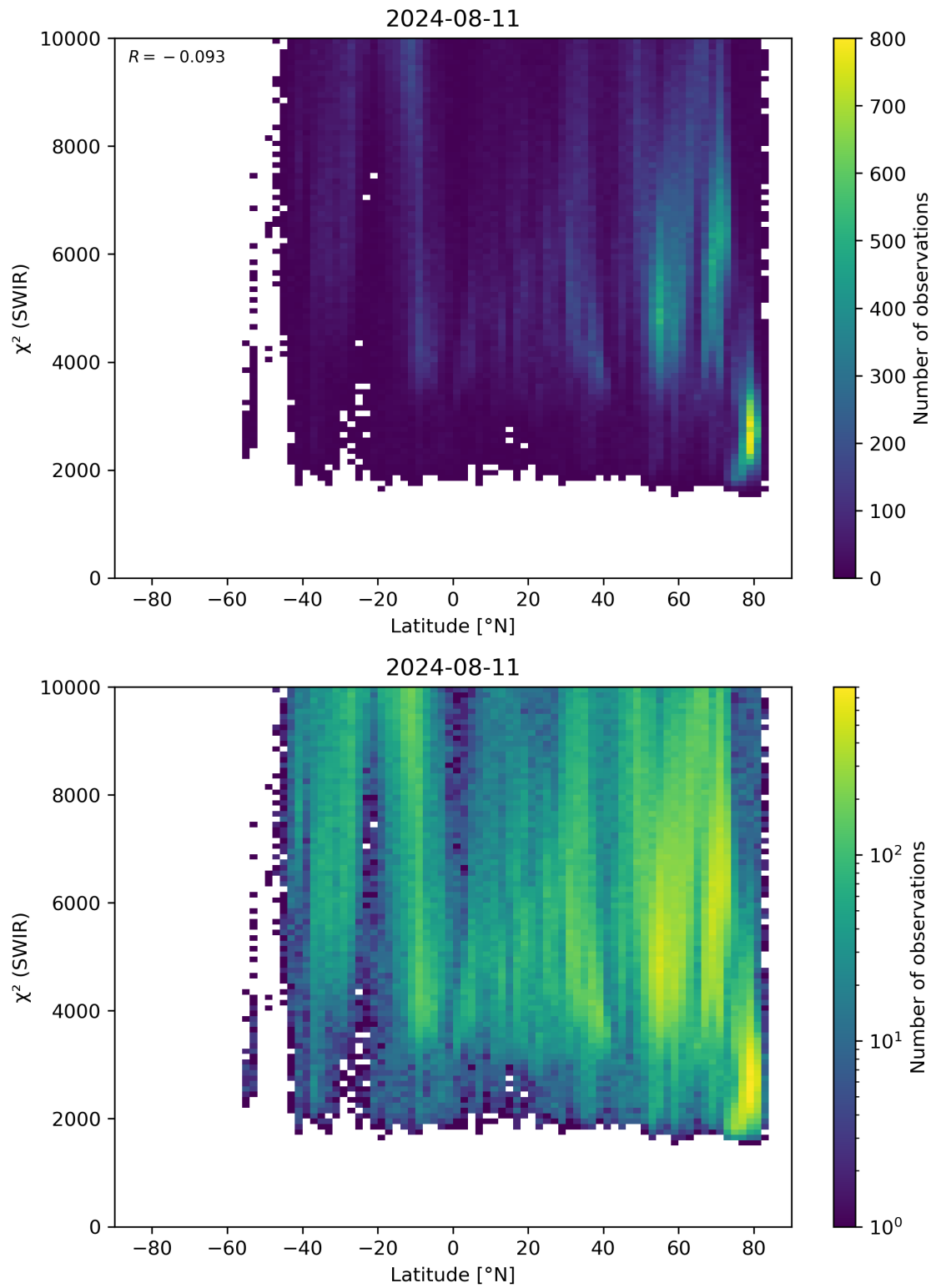
Figure 54: Scatter density plot of “Latitude” against “ \chi^2 (SWIR)” for 2024-08-11 to 2024-08-11.
