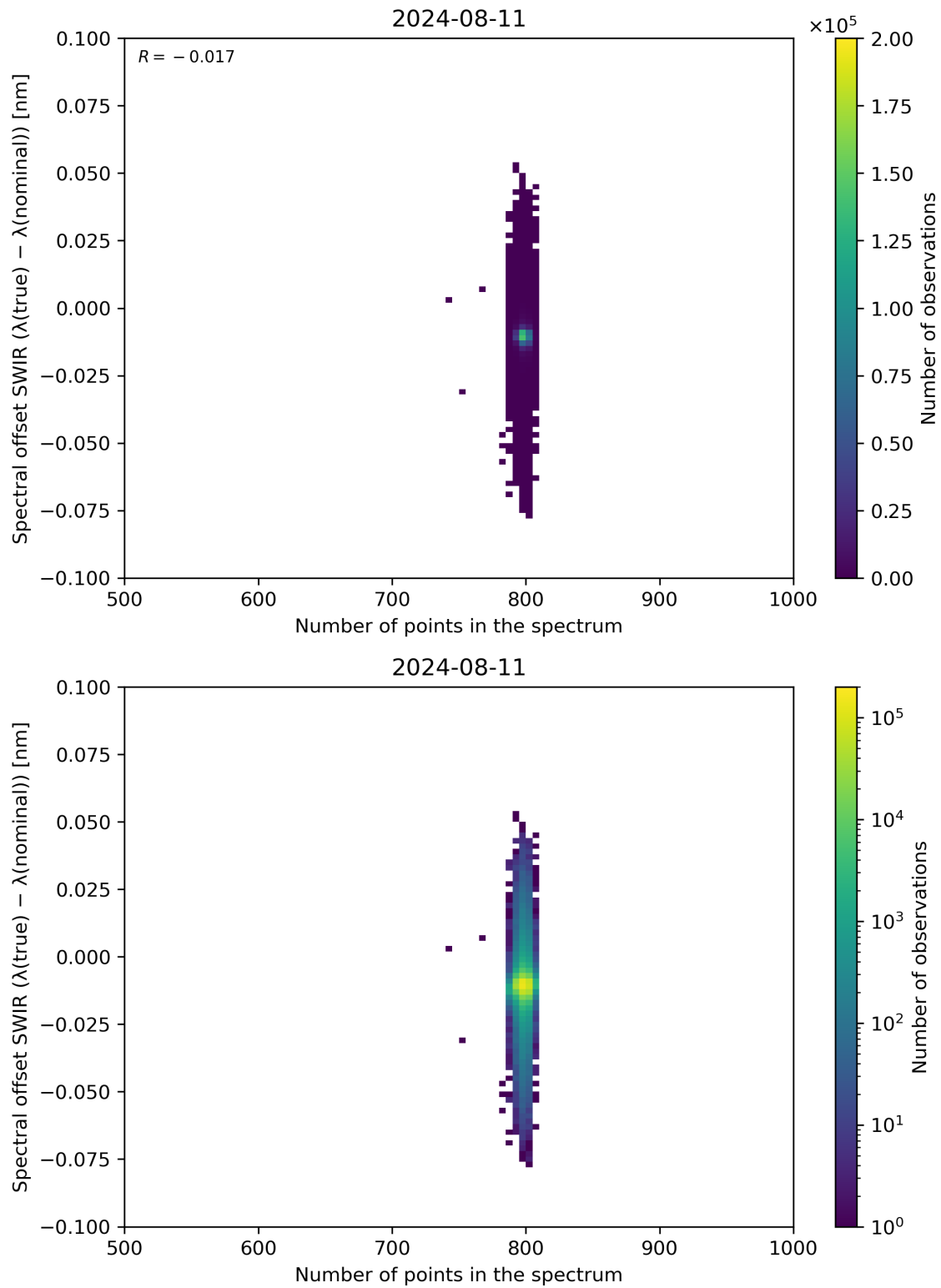
Figure 93: Scatter density plot of “Number of points in the spectrum” against “Spectral offset SWIR ( \lambda(\text{true}) - \lambda(\text{nominal}) )” for 2024-08-11 to 2024-08-11.
