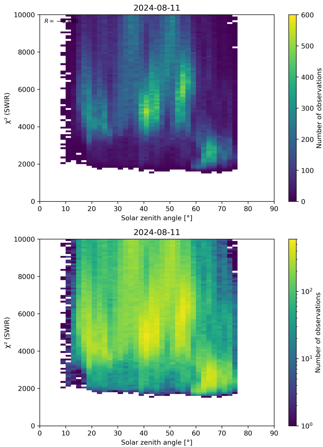
Figure 95: Scatter density plot of “Solar zenith angle” against “ \chi^2 (SWIR)” for 2024-08-11 to 2024-08-11.
