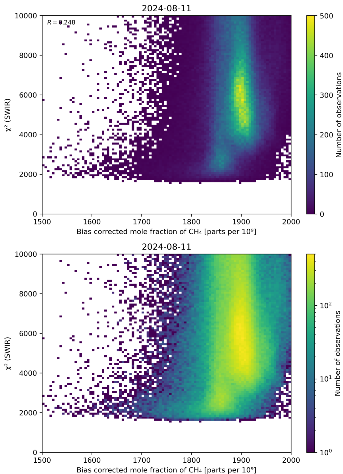
Figure 64: Scatter density plot of “Bias corrected mole fraction of CH 4 ” against “ \chi^2 (SWIR)” for 2024-08-11 to 2024-08-11.
