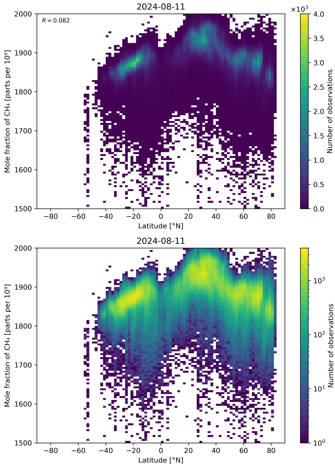
Figure 57: Scatter density plot of “Latitude” against “Mole fraction of \text{CH}_4 ” for 2024-08-11 to 2024-08-11.
