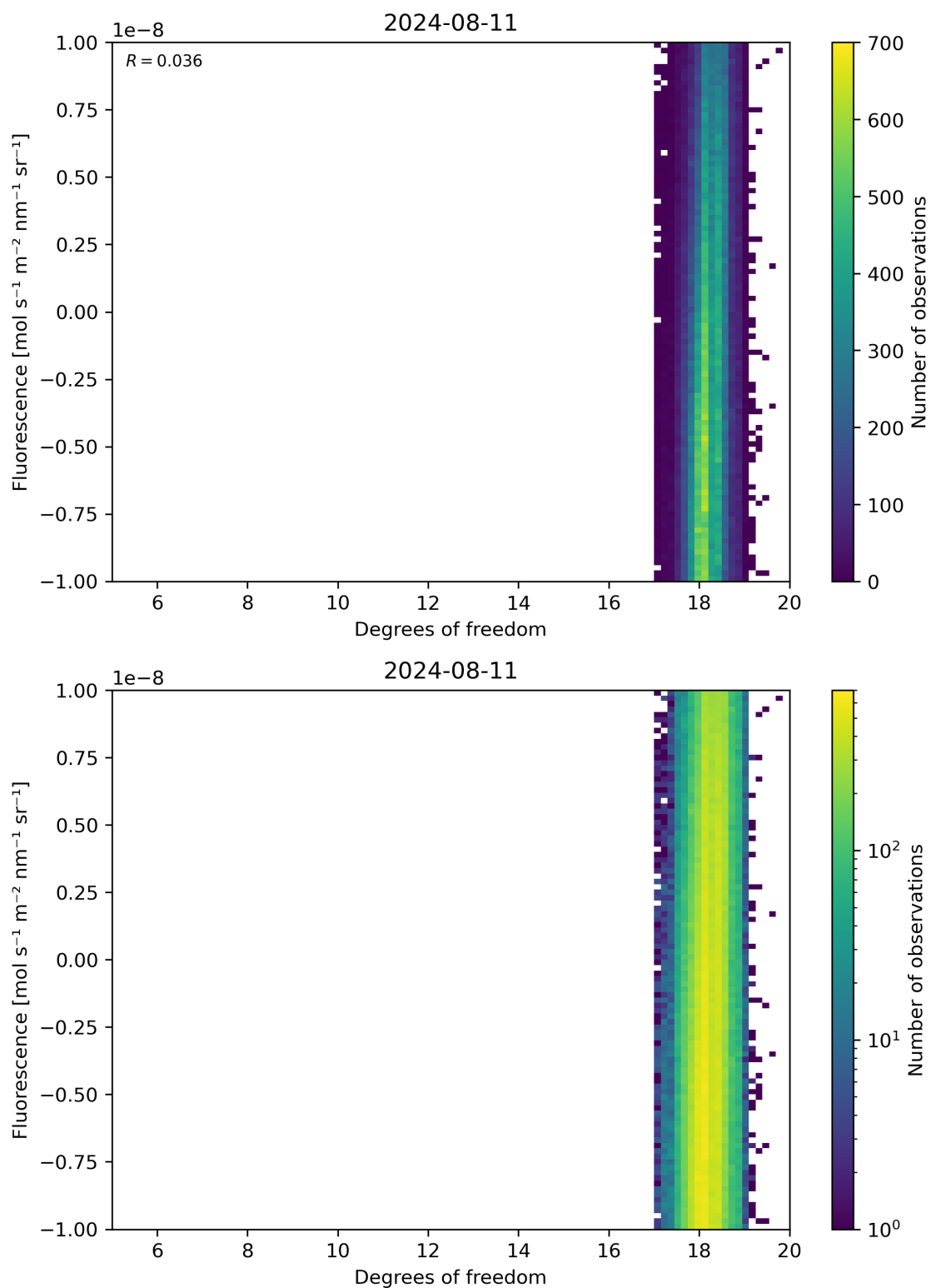
Figure 51: Scatter density plot of “Degrees of freedom” against “Fluorescence” for 2024-08-11 to 2024-08-11.
