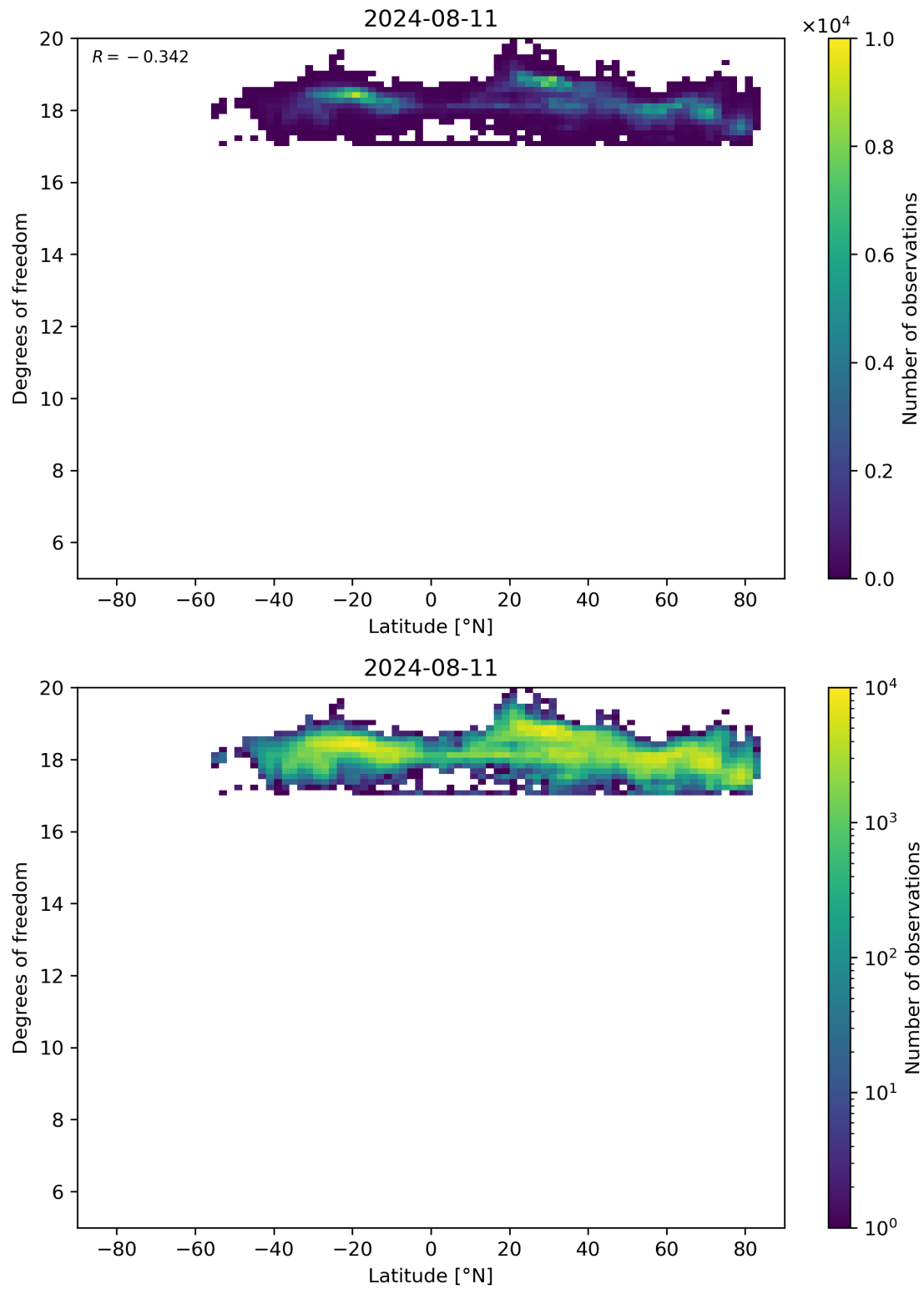
Figure 55: Scatter density plot of “Latitude” against “Degrees of freedom” for 2024-08-11 to 2024-08-11.
