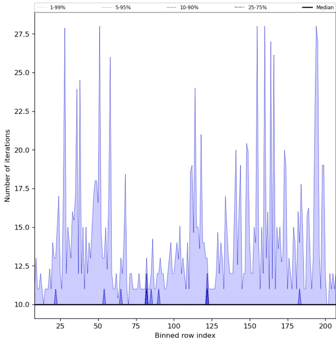
Figure 42: Along track statistics of “Number of iterations” for 2024-08-11 to 2024-08-11
