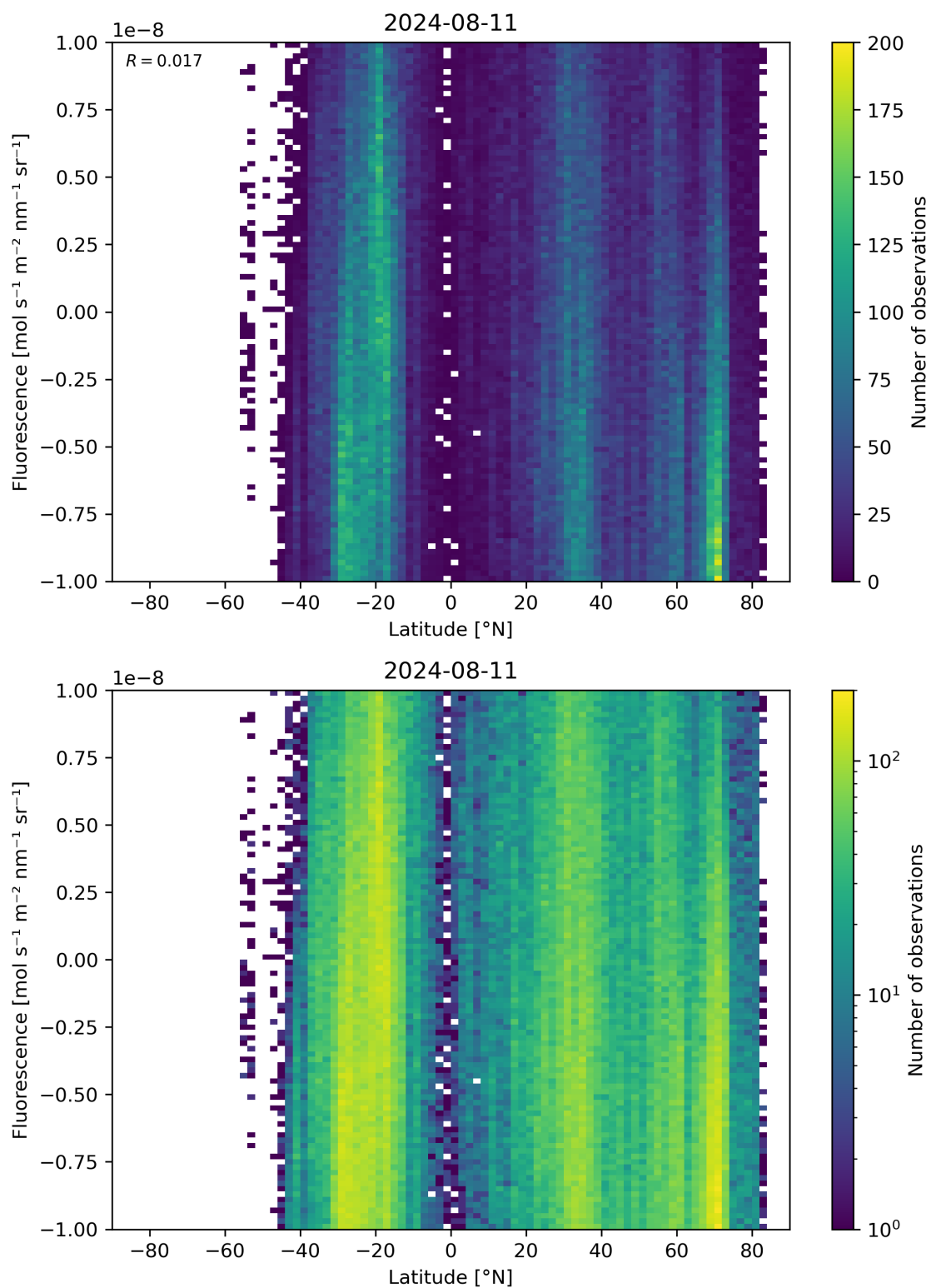
Figure 56: Scatter density plot of “Latitude” against “Fluorescence” for 2024-08-11 to 2024-08-11.
