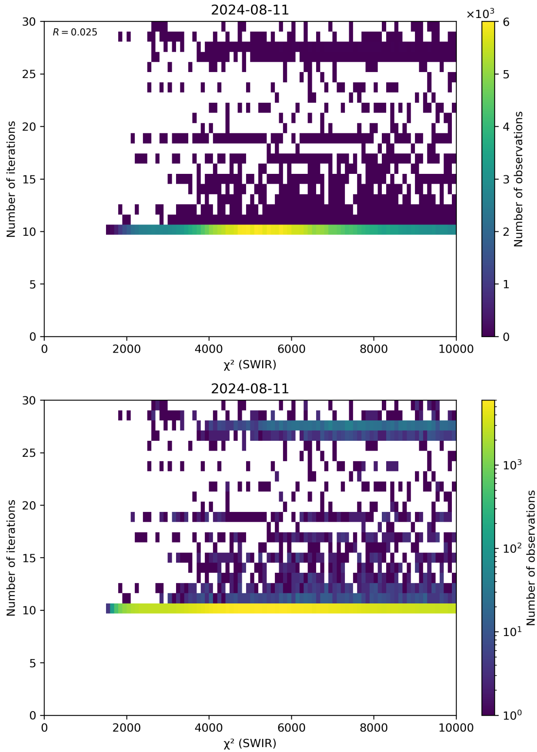
Figure 50: Scatter density plot of " \chi^2 (SWIR)" against "Number of iterations" for 2024-08-11 to 2024-08-11.
