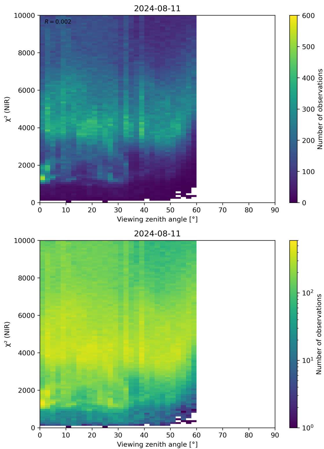
Figure 105: Scatter density plot of “Viewing zenith angle” against “ \chi^2 (NIR)” for 2024-08-11 to 2024-08-11.
