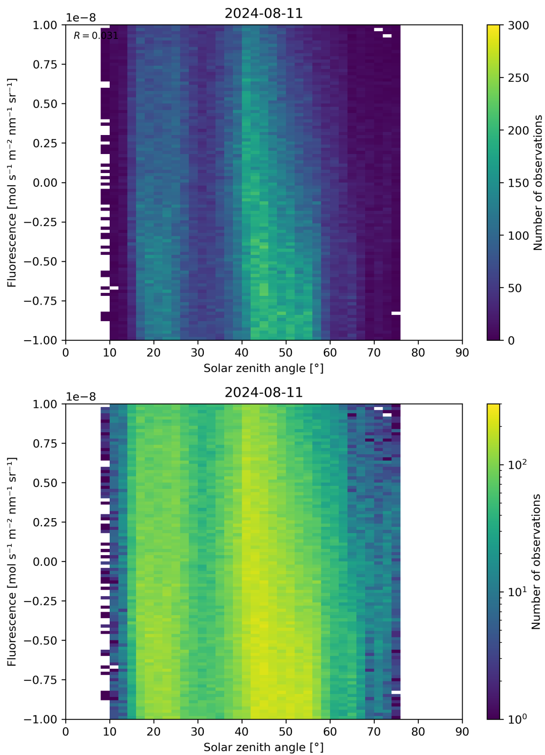
Figure 97: Scatter density plot of “Solar zenith angle” against “Fluorescence” for 2024-08-11 to 2024-08-11.
