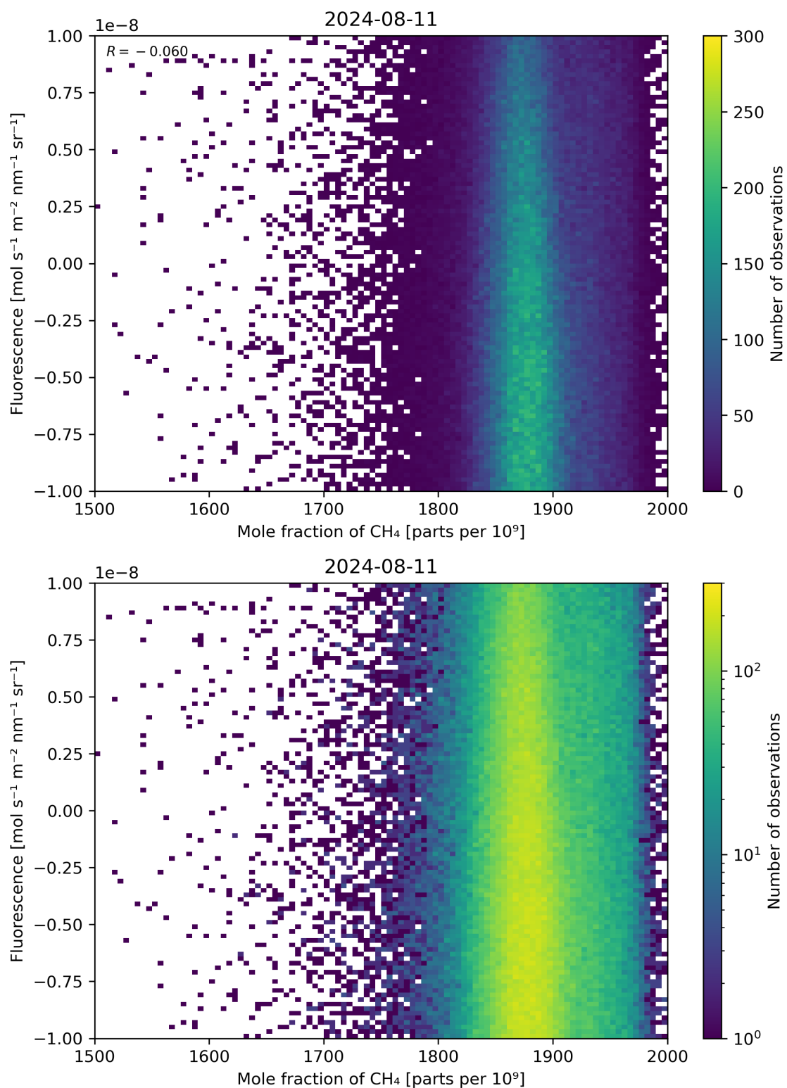
Figure 73: Scatter density plot of “Mole fraction of \text{CH}_4 ” against “Fluorescence” for 2024-08-11 to 2024-08-11.
