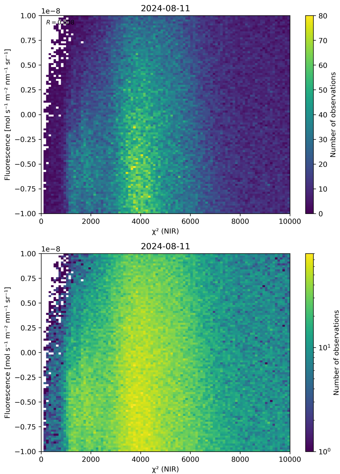
Figure 45: Scatter density plot of “ \chi^2 (NIR)” against “Fluorescence” for 2024-08-11 to 2024-08-11.
