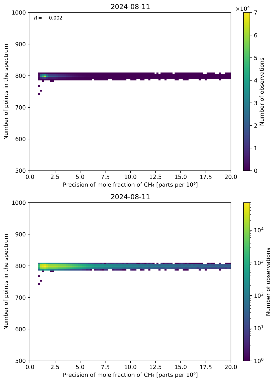
Figure 84: Scatter density plot of “Precision of mole fraction of CH 4 ” against “Number of points in the spectrum” for 2024-08-11 to 2024-08-11.
