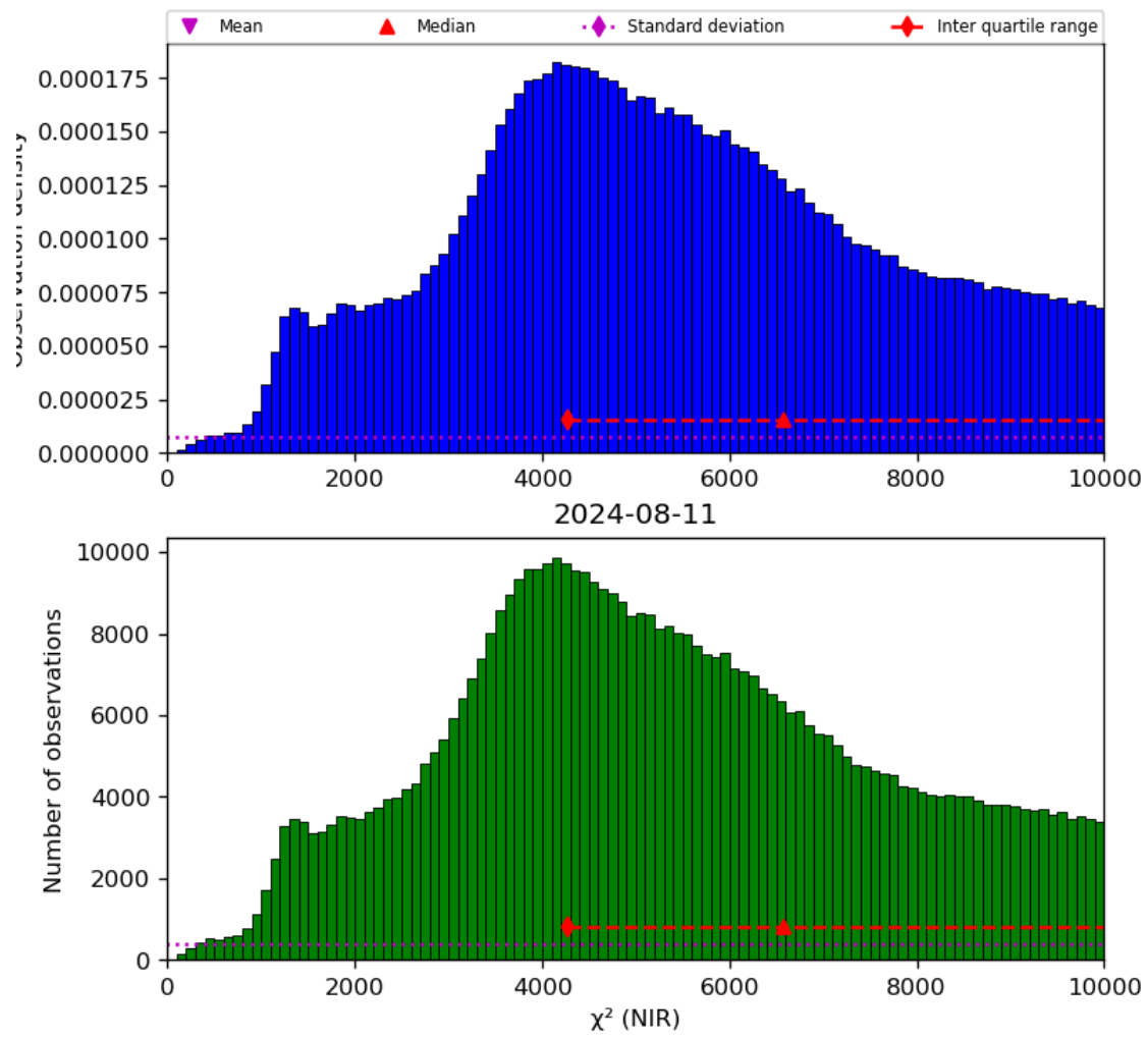
Figure 29: Histogram of “ \chi^2 (NIR)” for 2024-08-11 to 2024-08-11
