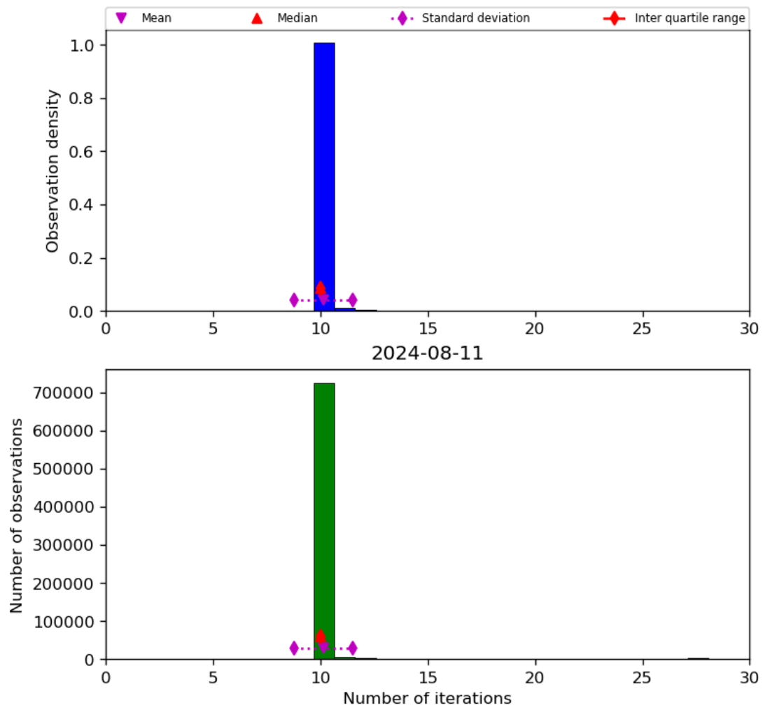
Figure 31: Histogram of “Number of iterations” for 2024-08-11 to 2024-08-11
