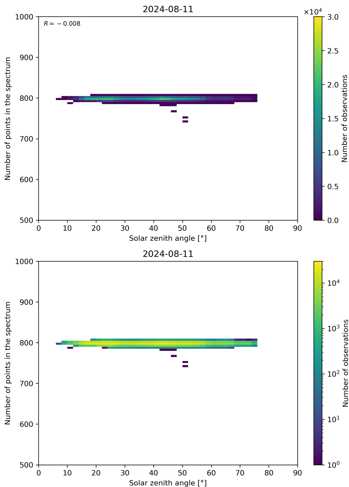
Figure 103: Scatter density plot of “Solar zenith angle” against “Number of points in the spectrum” for 2024-08-11 to 2024-08-11.
