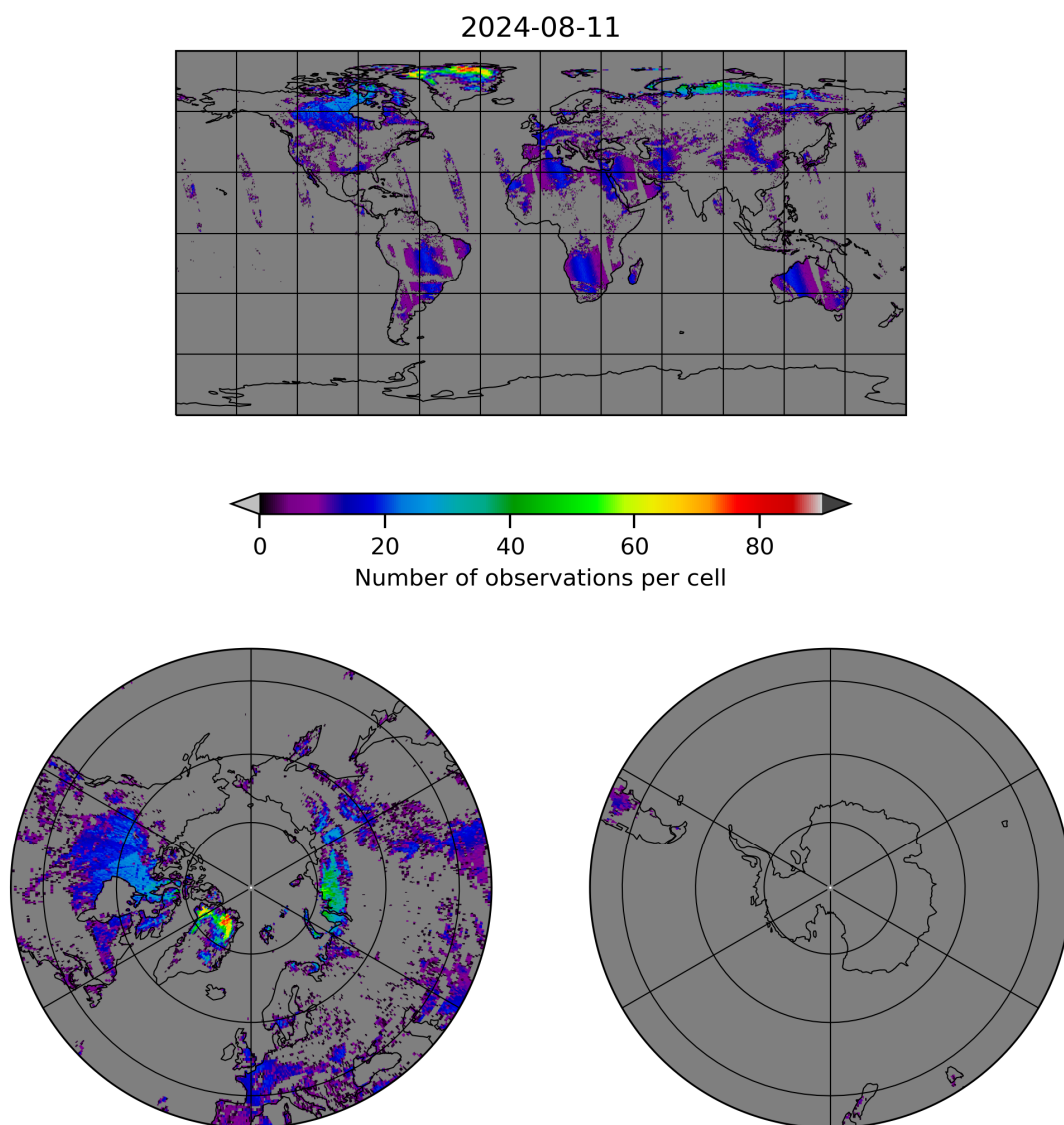
Figure 10: Map of the number of observations for 2024-08-11 to 2024-08-11
