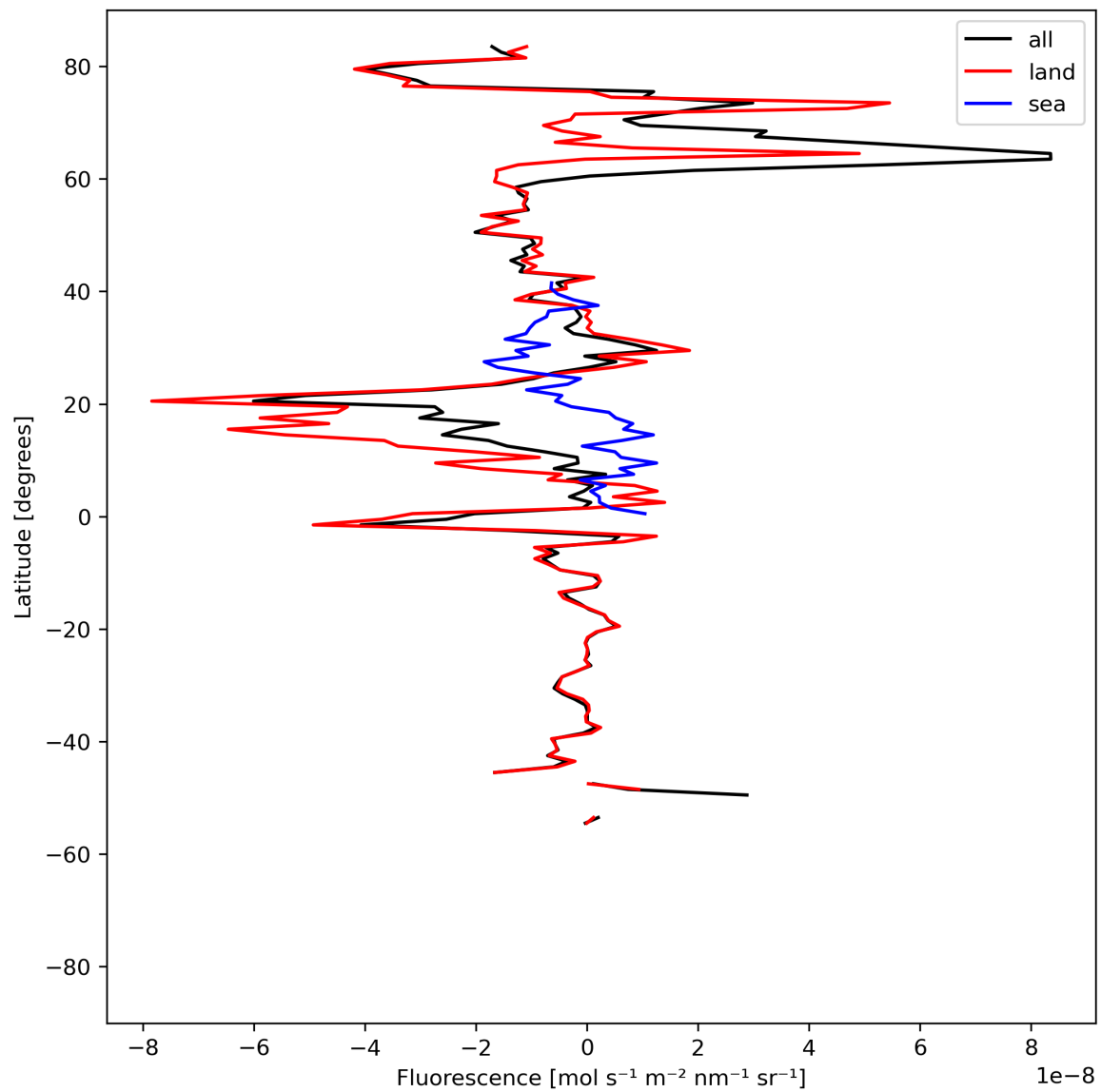
Figure 21: Zonal average of “Fluorescence” for 2024-08-11 to 2024-08-11.
