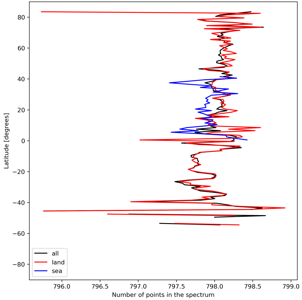
Figure 15: Zonal average of “Number of points in the spectrum” for 2024-08-11 to 2024-08-11.
