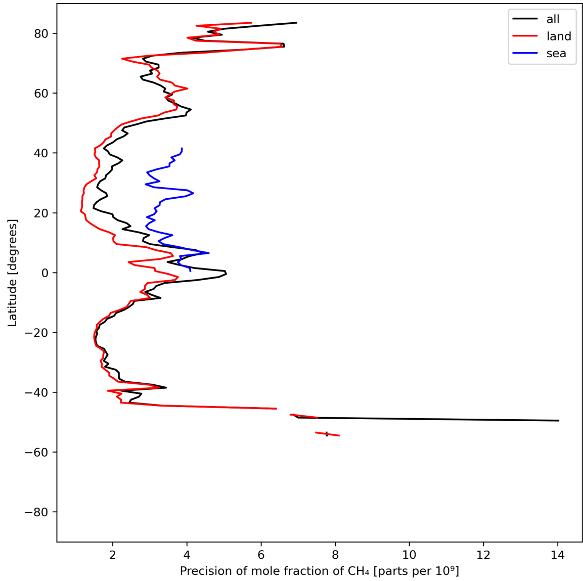
Figure 13: Zonal average of “Precision of mole fraction of CH 4 ” for 2024-08-11 to 2024-08-11.
