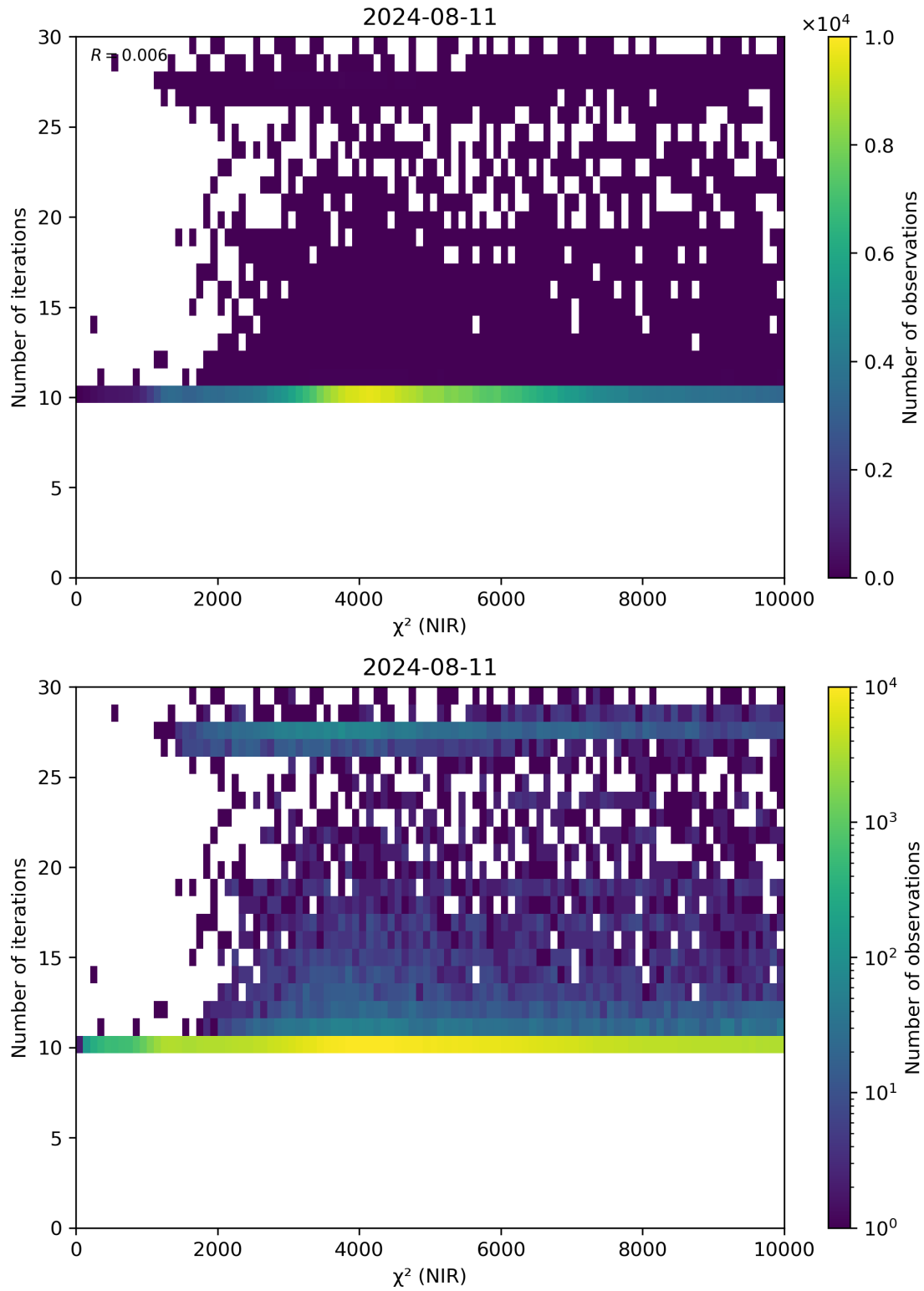
Figure 46: Scatter density plot of " \chi^2 (NIR)" against "Number of iterations" for 2024-08-11 to 2024-08-11.
