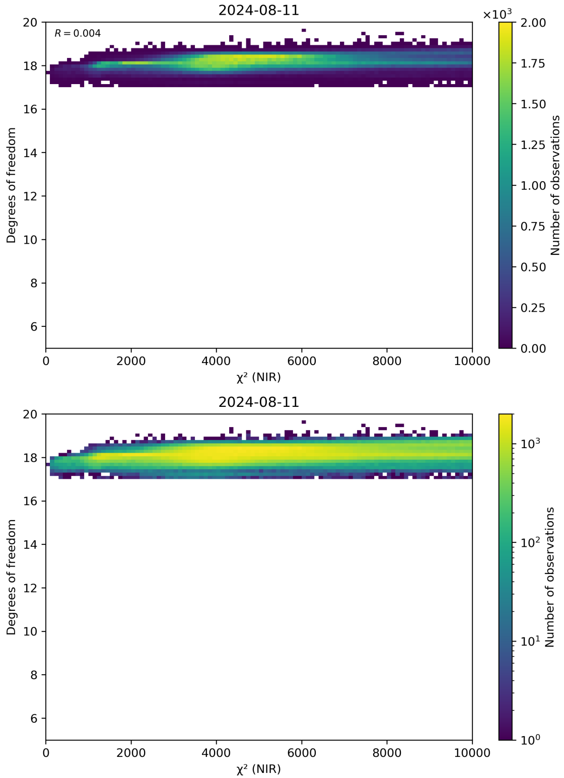
Figure 44: Scatter density plot of “ \chi^2 (NIR)” against “Degrees of freedom” for 2024-08-11 to 2024-08-11.
