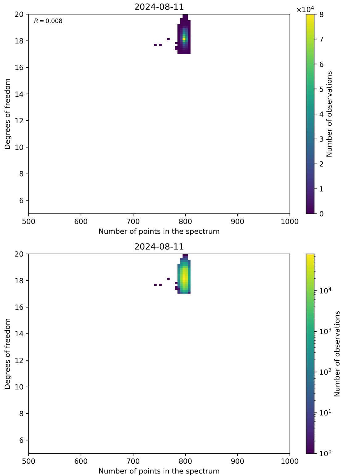
Figure 90: Scatter density plot of “Number of points in the spectrum” against “Degrees of freedom” for 2024-08-11 to 2024-08-11.
