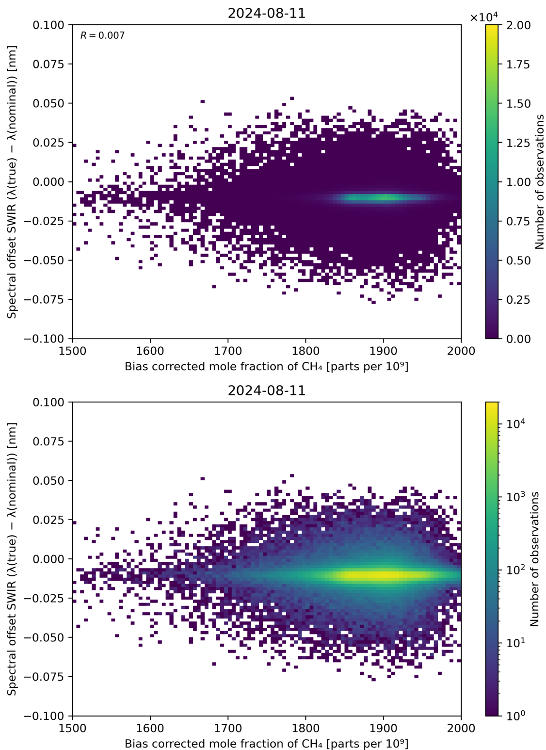
Figure 69: Scatter density plot of “Bias corrected mole fraction of \text{CH}_4 ” against “Spectral offset SWIR ( \lambda(\text{true}) - \lambda(\text{nominal}) )” for 2024-08-11 to 2024-08-11.
