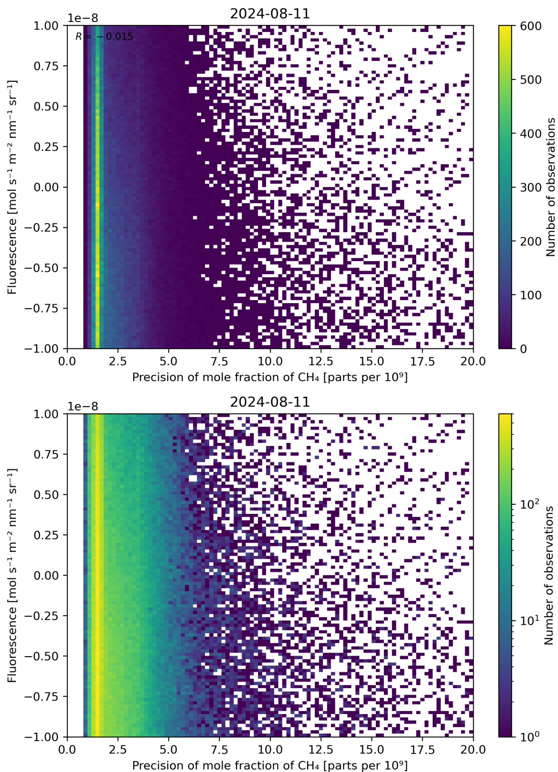
Figure 81: Scatter density plot of “Precision of mole fraction of \text{CH}_4 ” against “Fluorescence” for 2024-08-11 to 2024-08-11.
