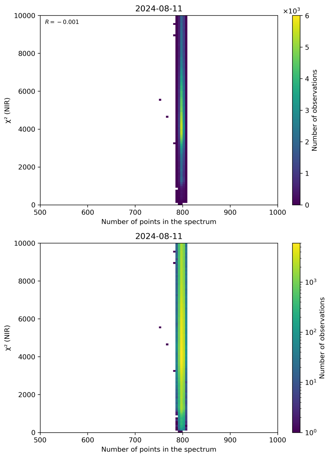
Figure 88: Scatter density plot of “Number of points in the spectrum” against “ \chi^2 (NIR)” for 2024-08-11 to 2024-08-11.
