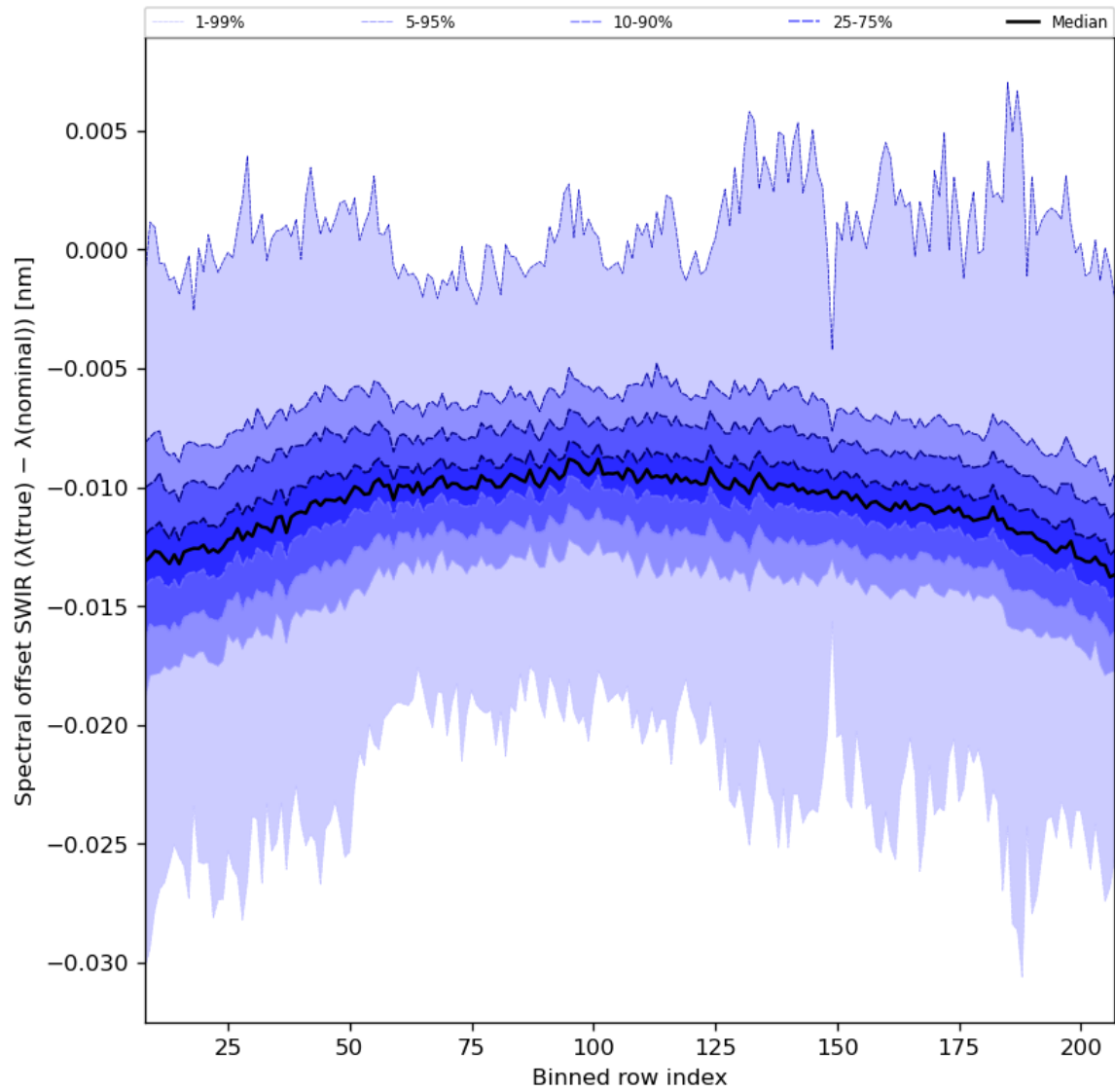
Figure 38: Along track statistics of “Spectral offset SWIR ( \lambda(\text{true}) - \lambda(\text{nominal}) )” for 2024-08-11 to 2024-08-11
