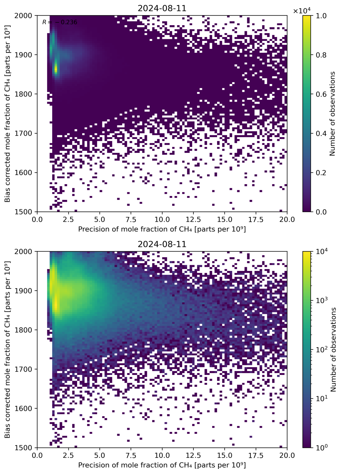
Figure 82: Scatter density plot of “Precision of mole fraction of CH 4 ” against “Bias corrected mole fraction of CH 4 ” for 2024-08-11 to 2024-08-11.
