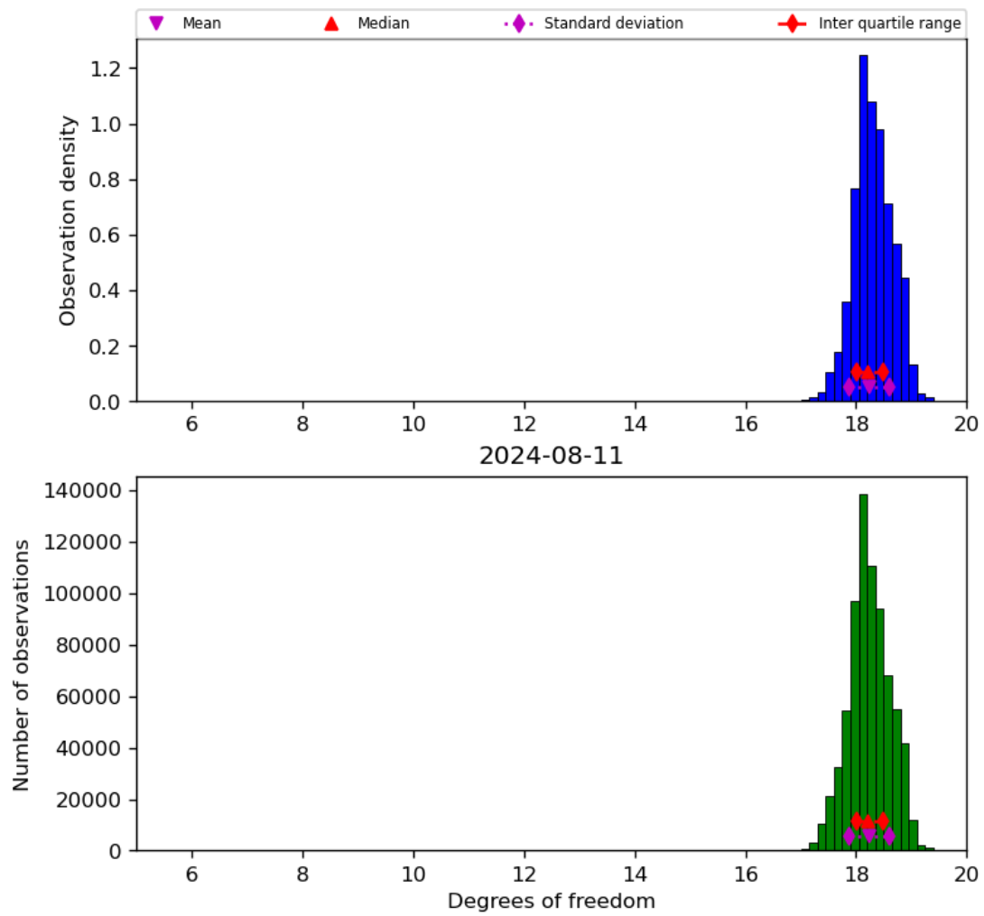
Figure 30: Histogram of “Degrees of freedom” for 2024-08-11 to 2024-08-11
