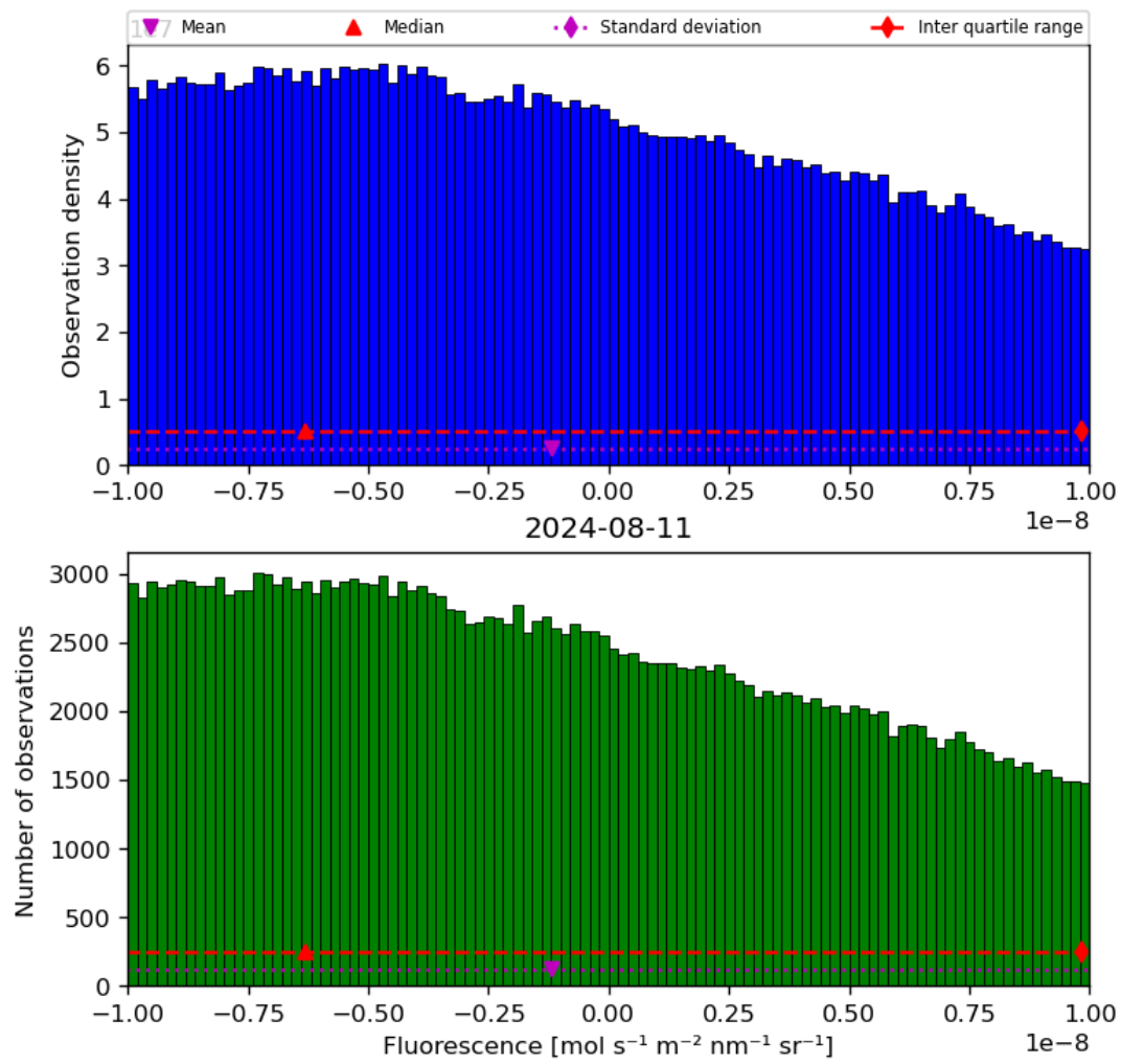
Figure 32: Histogram of “Fluorescence” for 2024-08-11 to 2024-08-11
