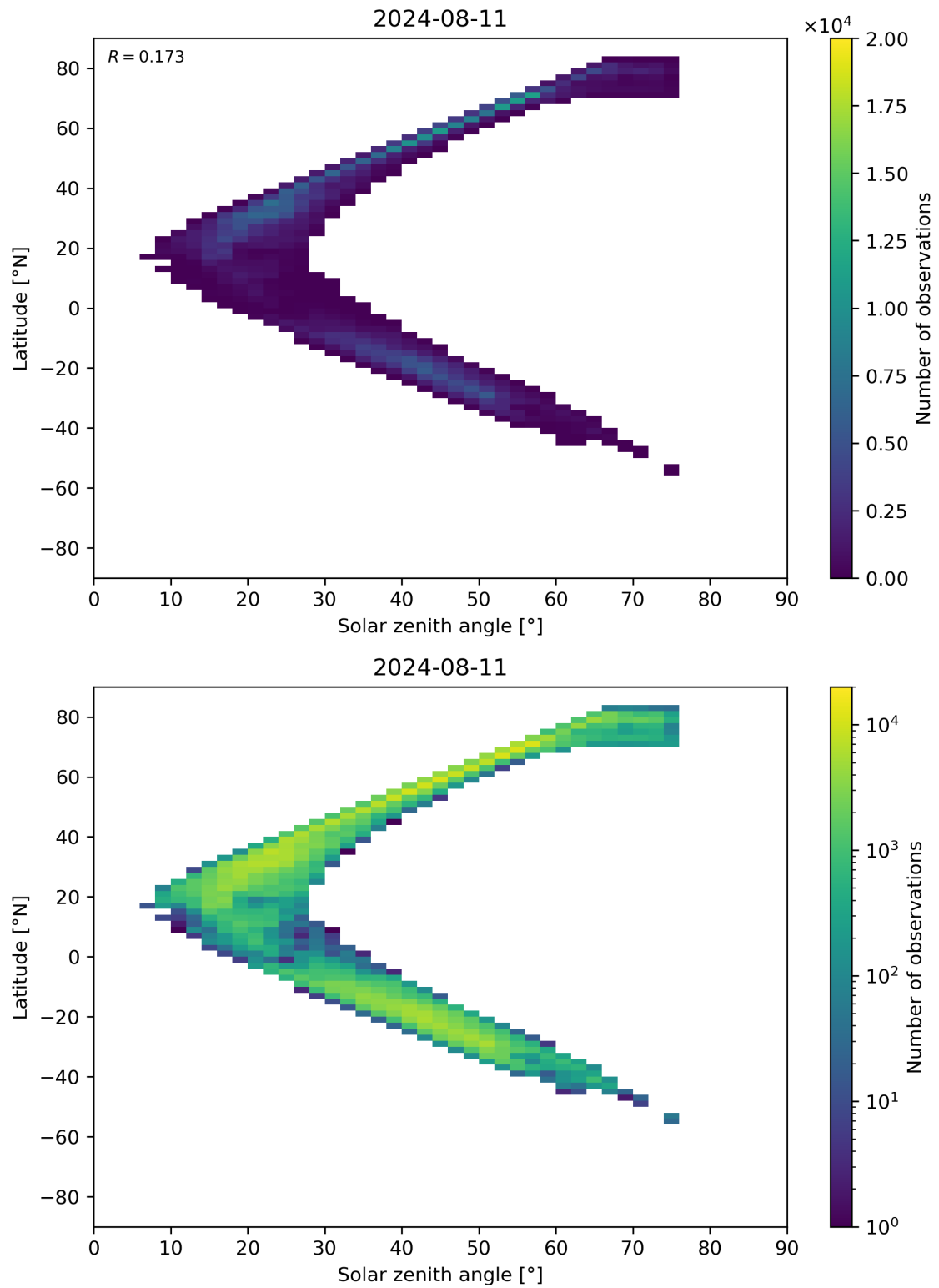
Figure 98: Scatter density plot of “Solar zenith angle” against “Latitude” for 2024-08-11 to 2024-08-11.
