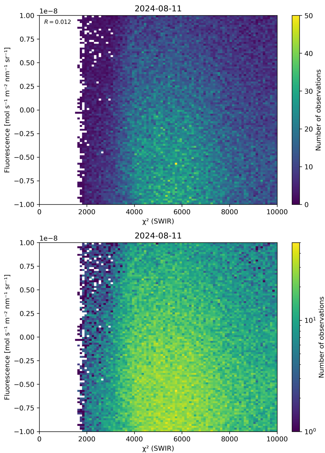
Figure 49: Scatter density plot of “ \chi^2 (SWIR)” against “Fluorescence” for 2024-08-11 to 2024-08-11.
