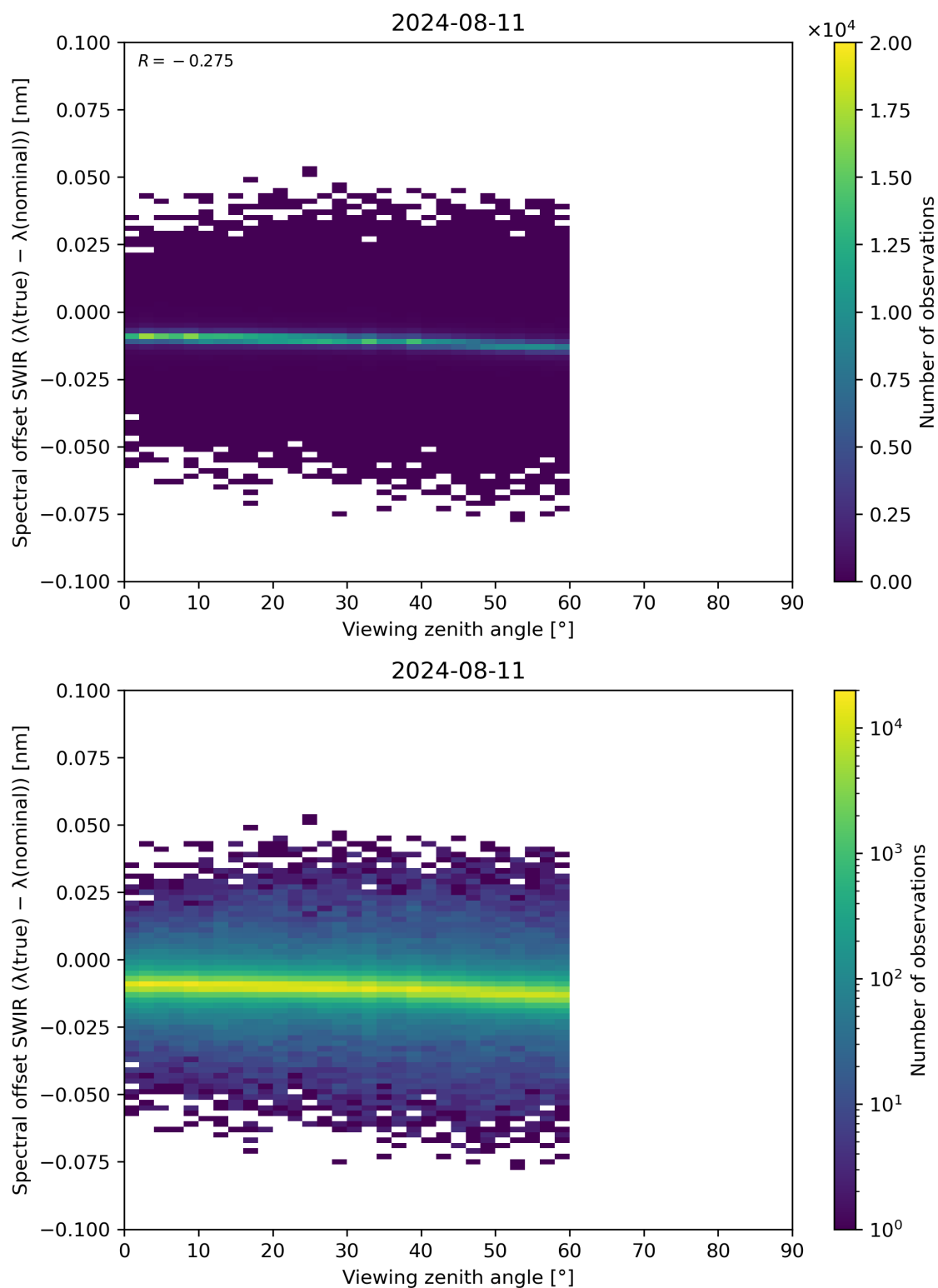
Figure 116: Scatter density plot of “Viewing zenith angle” against “Spectral offset SWIR ( \lambda(\text{true}) - \lambda(\text{nominal}) )” for 2024-08-11 to 2024-08-11.
