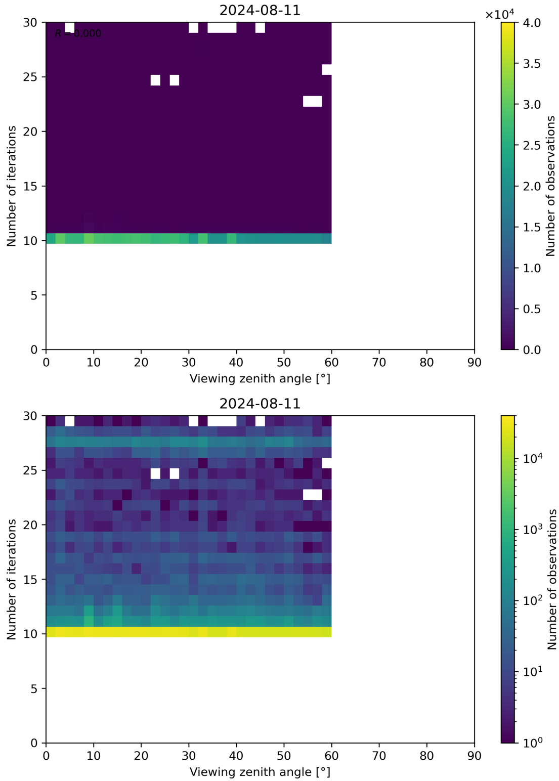
Figure 113: Scatter density plot of “Viewing zenith angle” against “Number of iterations” for 2024-08-11 to 2024-08-11.
