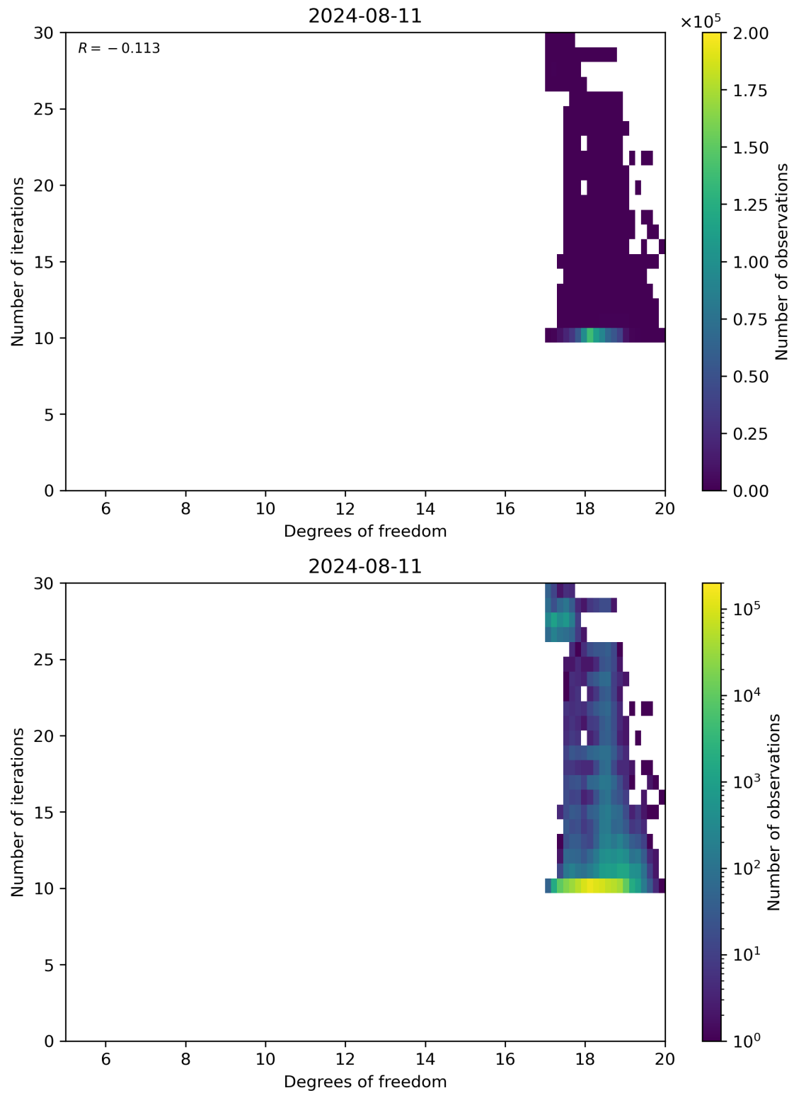
Figure 52: Scatter density plot of “Degrees of freedom” against “Number of iterations” for 2024-08-11 to 2024-08-11.
