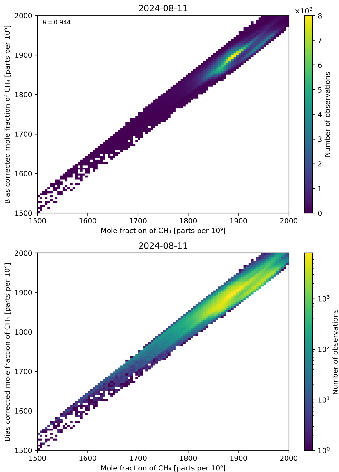
Figure 74: Scatter density plot of “Mole fraction of CH 4 ” against “Bias corrected mole fraction of CH 4 ” for 2024-08-11 to 2024-08-11.
