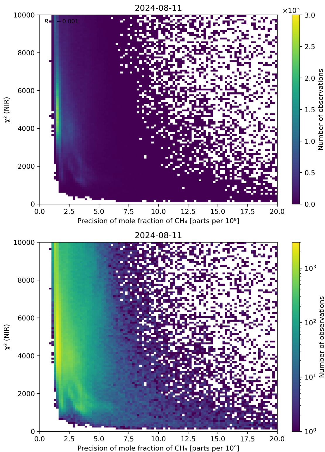
Figure 78: Scatter density plot of “Precision of mole fraction of CH 4 ” against “ \chi^2 (NIR)” for 2024-08-11 to 2024-08-11.
