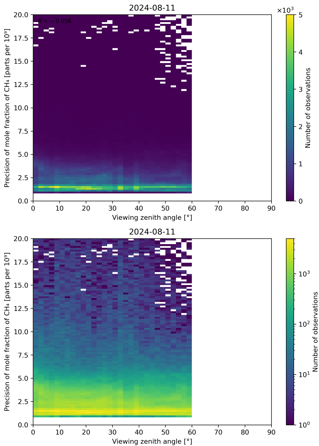
Figure 112: Scatter density plot of “Viewing zenith angle” against “Precision of mole fraction of CH 4 ” for 2024-08-11 to 2024-08-11.
