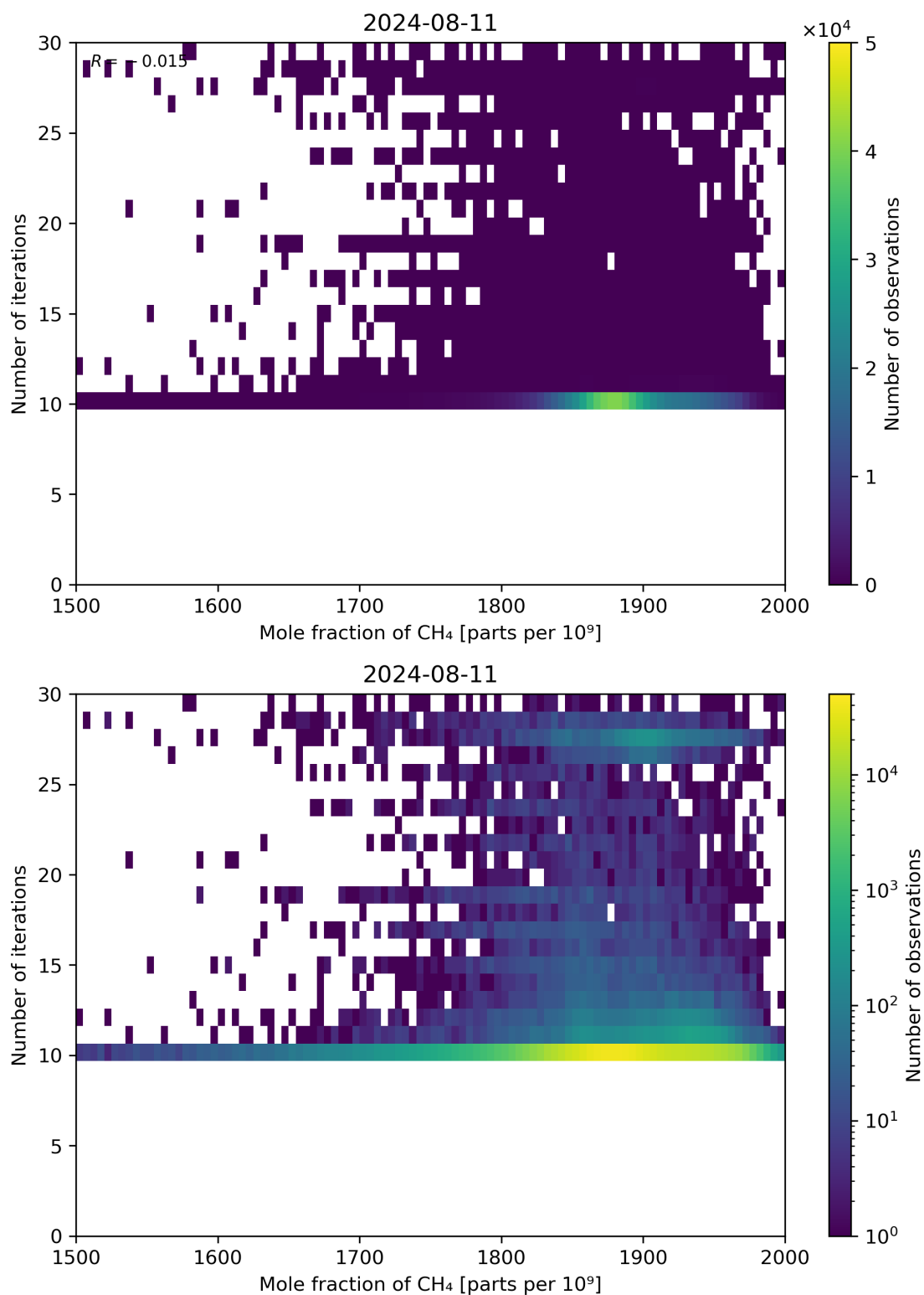
Figure 76: Scatter density plot of “Mole fraction of CH 4 ” against “Number of iterations” for 2024-08-11 to 2024-08-11.
