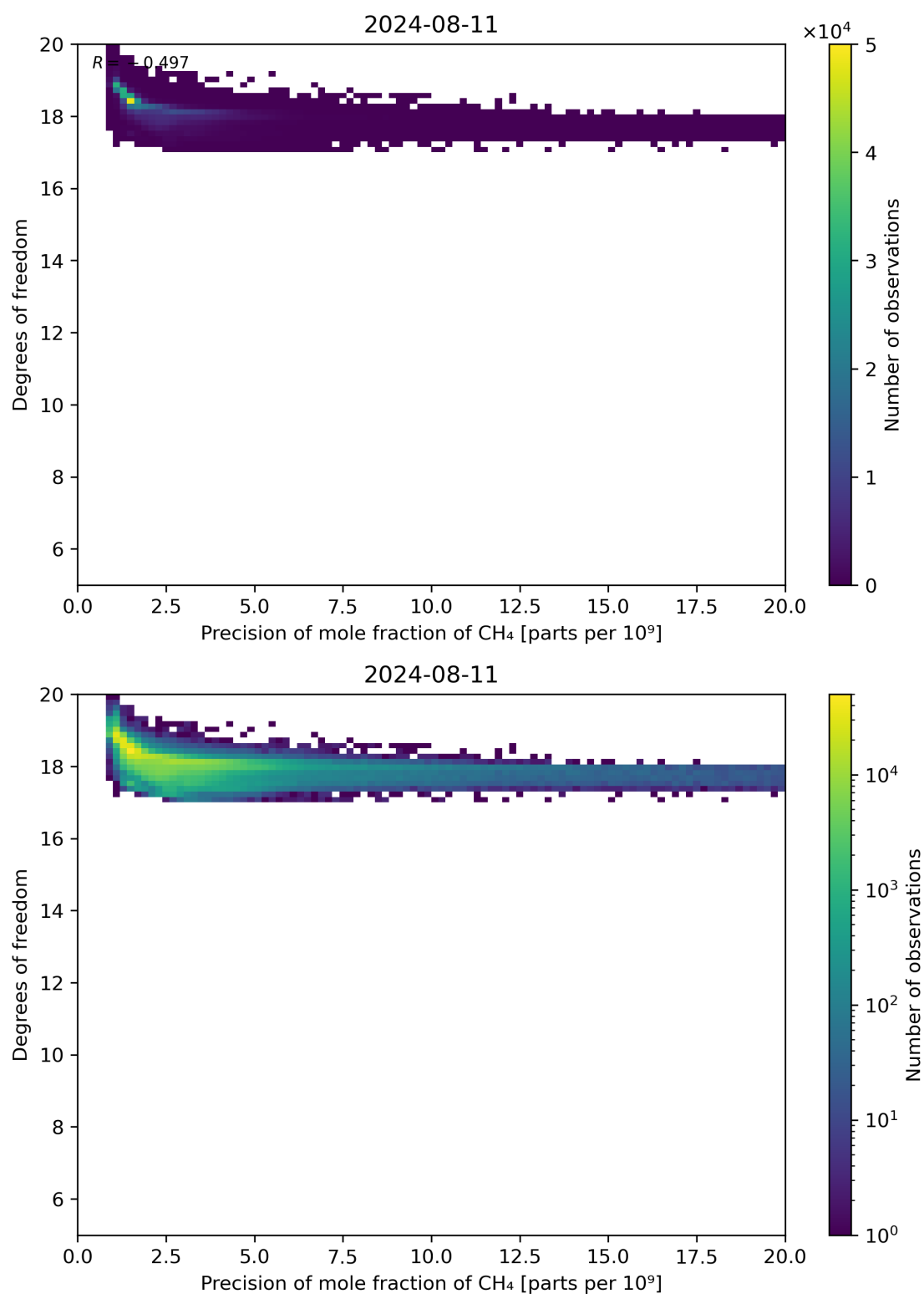
Figure 80: Scatter density plot of “Precision of mole fraction of CH 4 ” against “Degrees of freedom” for 2024-08-11 to 2024-08-11.
