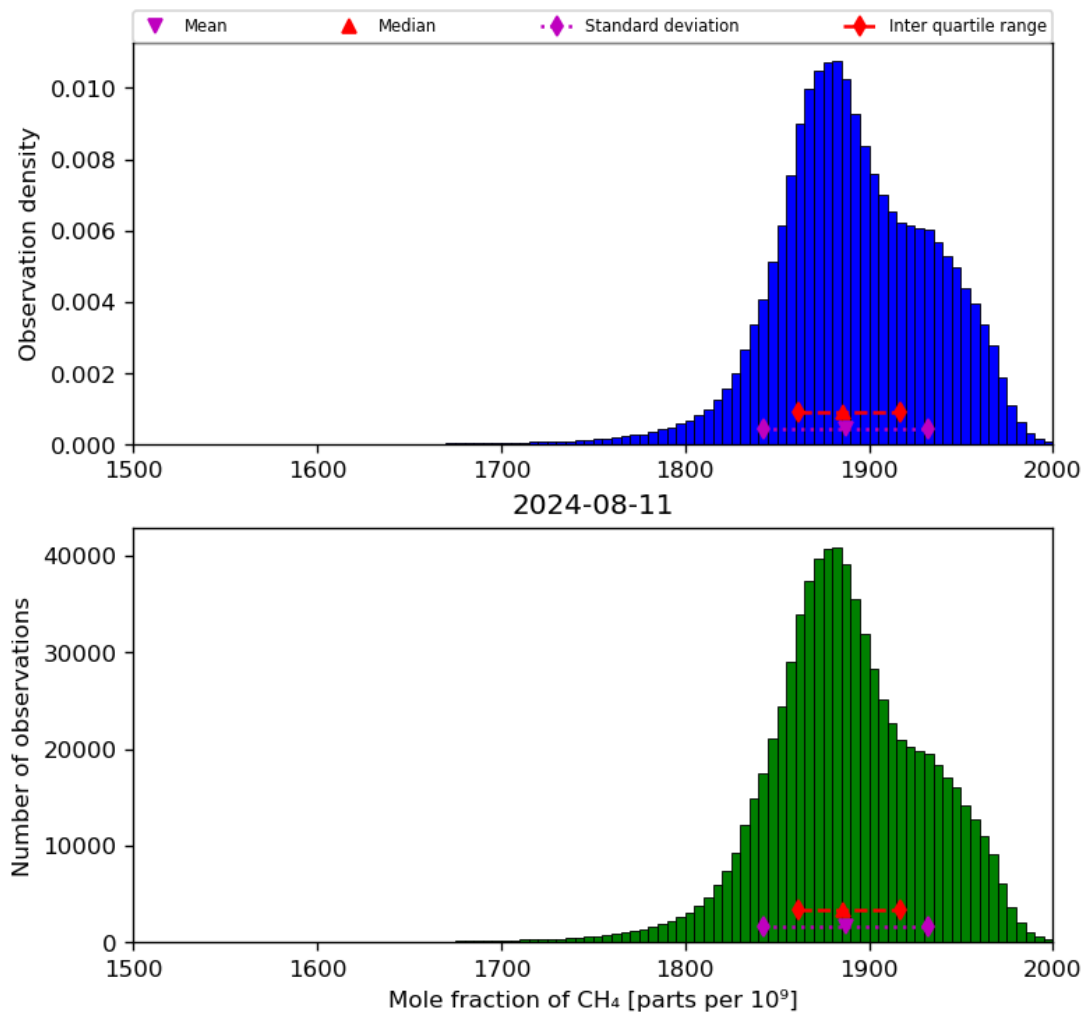
Figure 23: Histogram of “Mole fraction of CH 4 ” for 2024-08-11 to 2024-08-11
