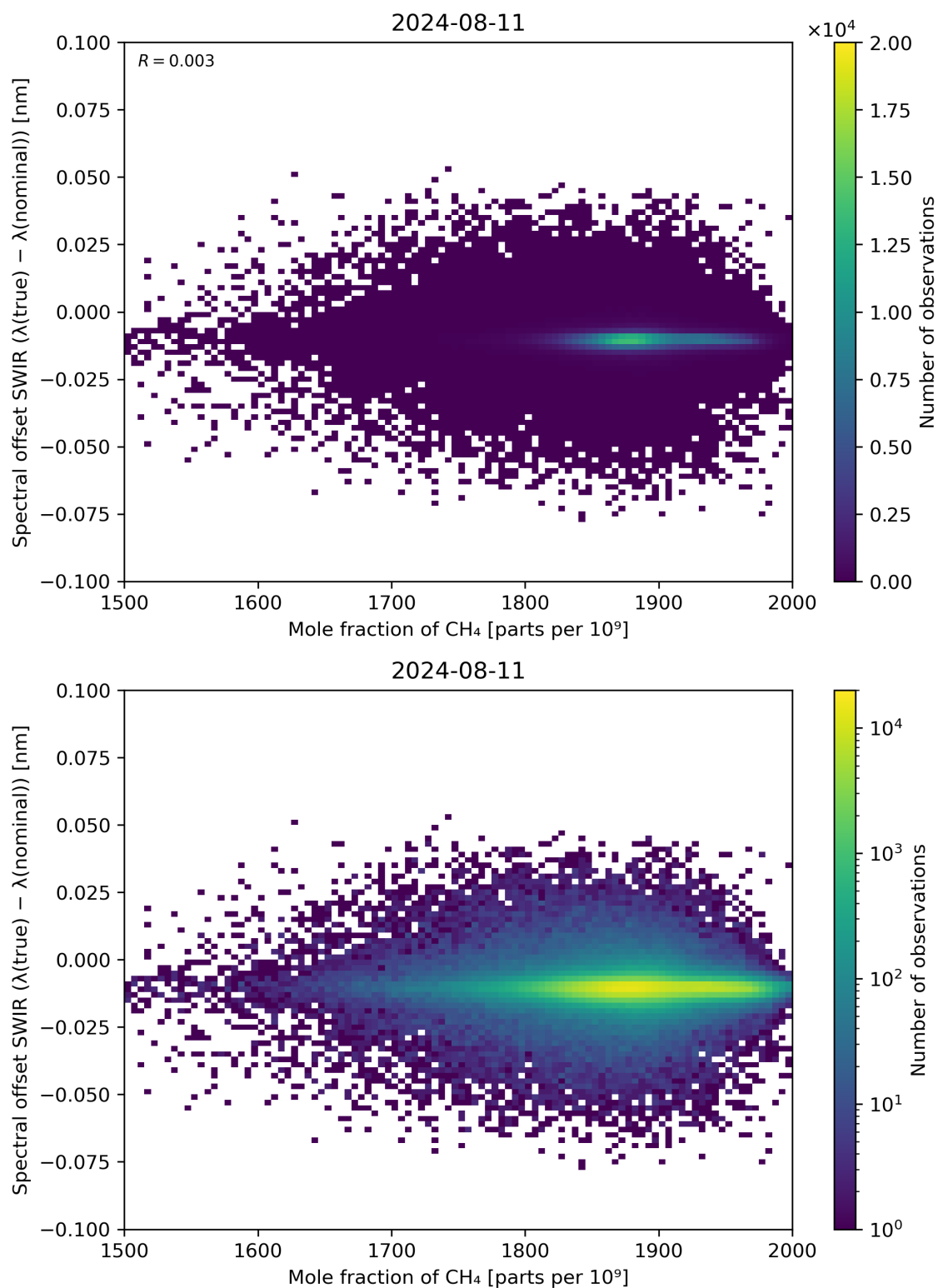
Figure 86: Scatter density plot of “Mole fraction of CH 4 ” against “Spectral offset SWIR ( \lambda(\text{true}) - \lambda(\text{nominal}) )” for 2024-08-11 to 2024-08-11.
