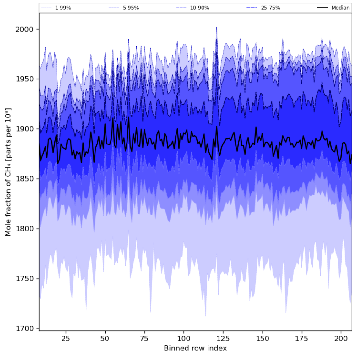
Figure 34: Along track statistics of “Mole fraction of CH 4 ” for 2024-08-11 to 2024-08-11
