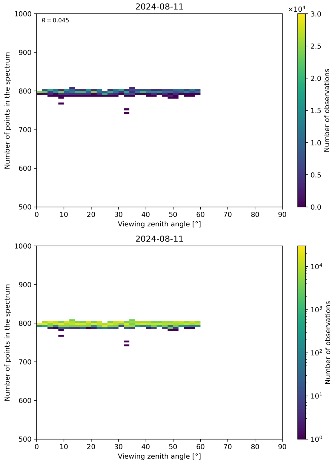
Figure 114: Scatter density plot of “Viewing zenith angle” against “Number of points in the spectrum” for 2024-08-11 to 2024-08-11.
