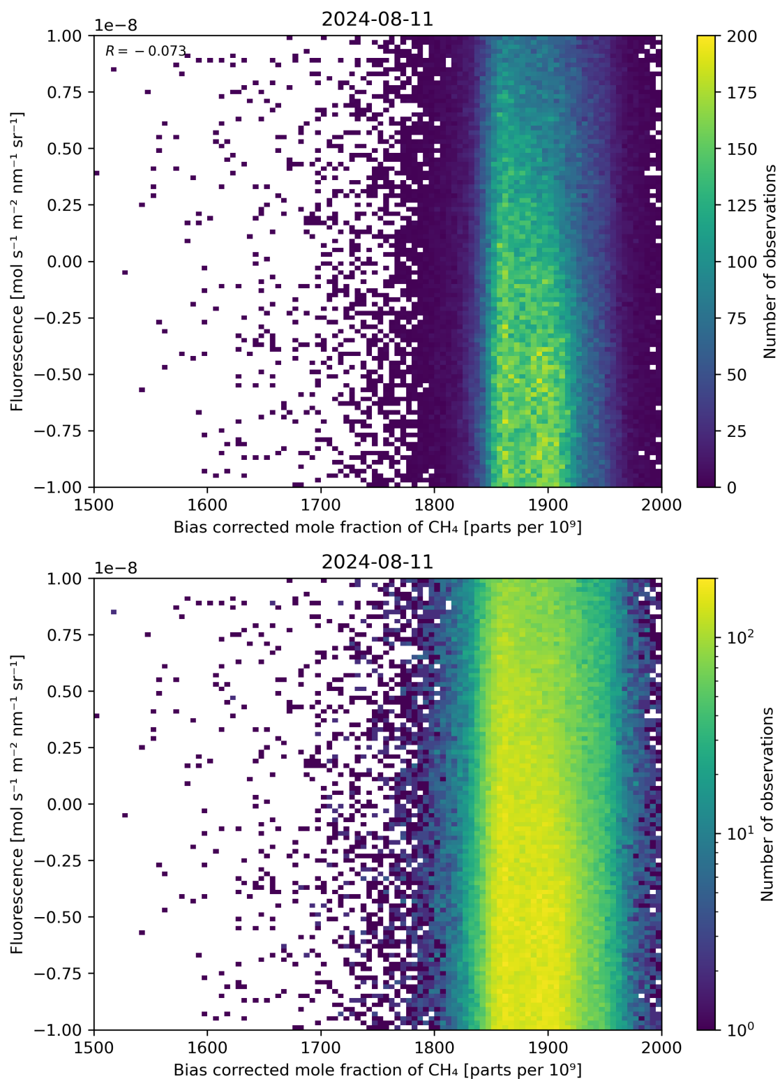
Figure 66: Scatter density plot of “Bias corrected mole fraction of \text{CH}_4 ” against “Fluorescence” for 2024-08-11 to 2024-08-11.
