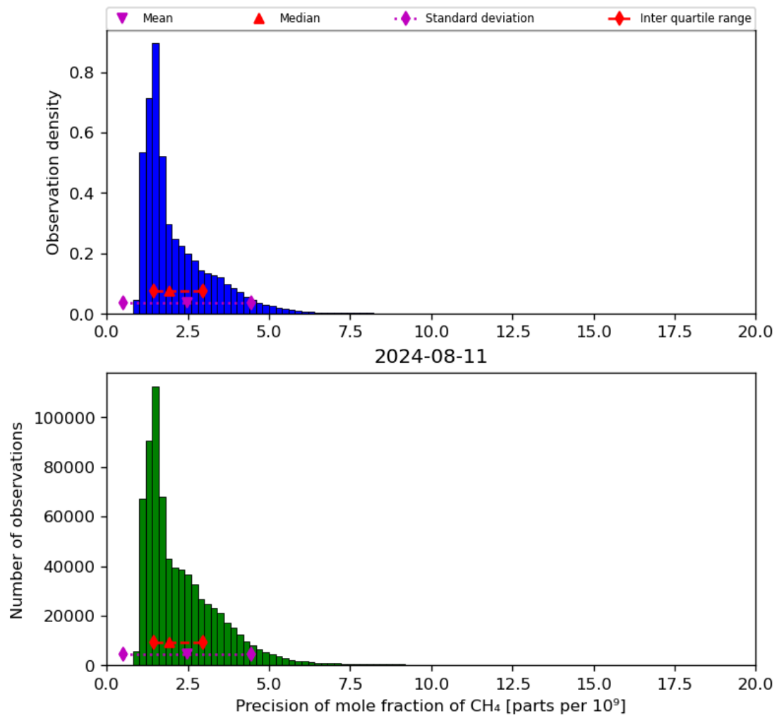
Figure 24: Histogram of “Precision of mole fraction of CH 4 ” for 2024-08-11 to 2024-08-11
