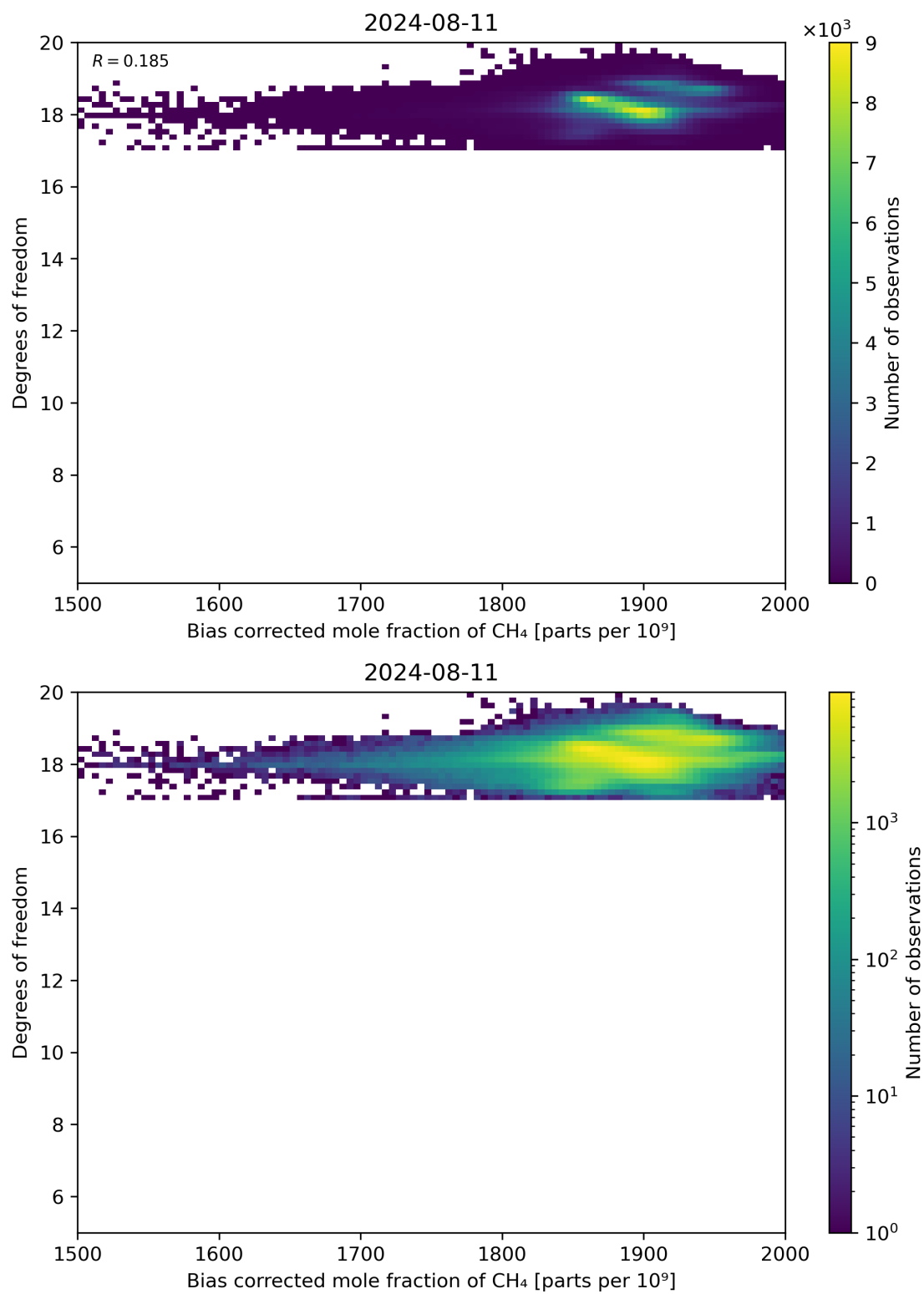
Figure 65: Scatter density plot of “Bias corrected mole fraction of CH 4 ” against “Degrees of freedom” for 2024-08-11 to 2024-08-11.
