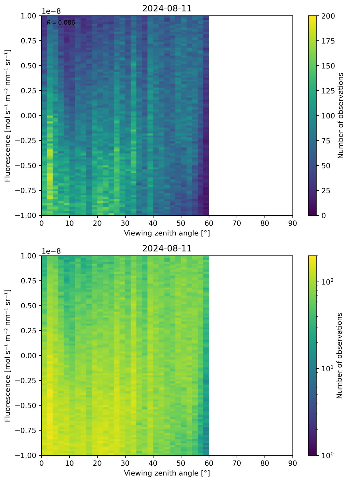
Figure 108: Scatter density plot of “Viewing zenith angle” against “Fluorescence” for 2024-08-11 to 2024-08-11.
