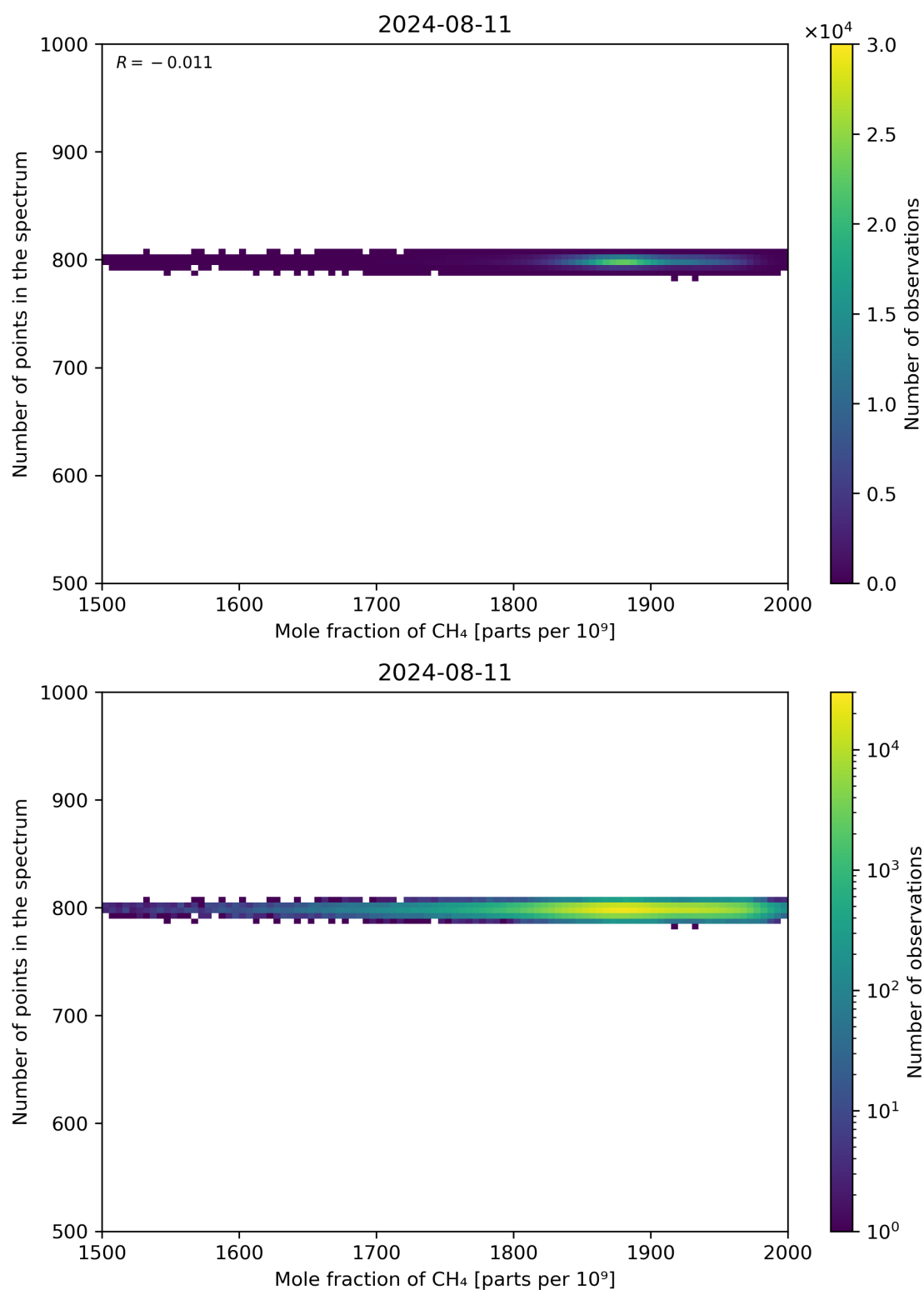
Figure 77: Scatter density plot of “Mole fraction of CH 4 ” against “Number of points in the spectrum” for 2024-08-11 to 2024-08-11.
