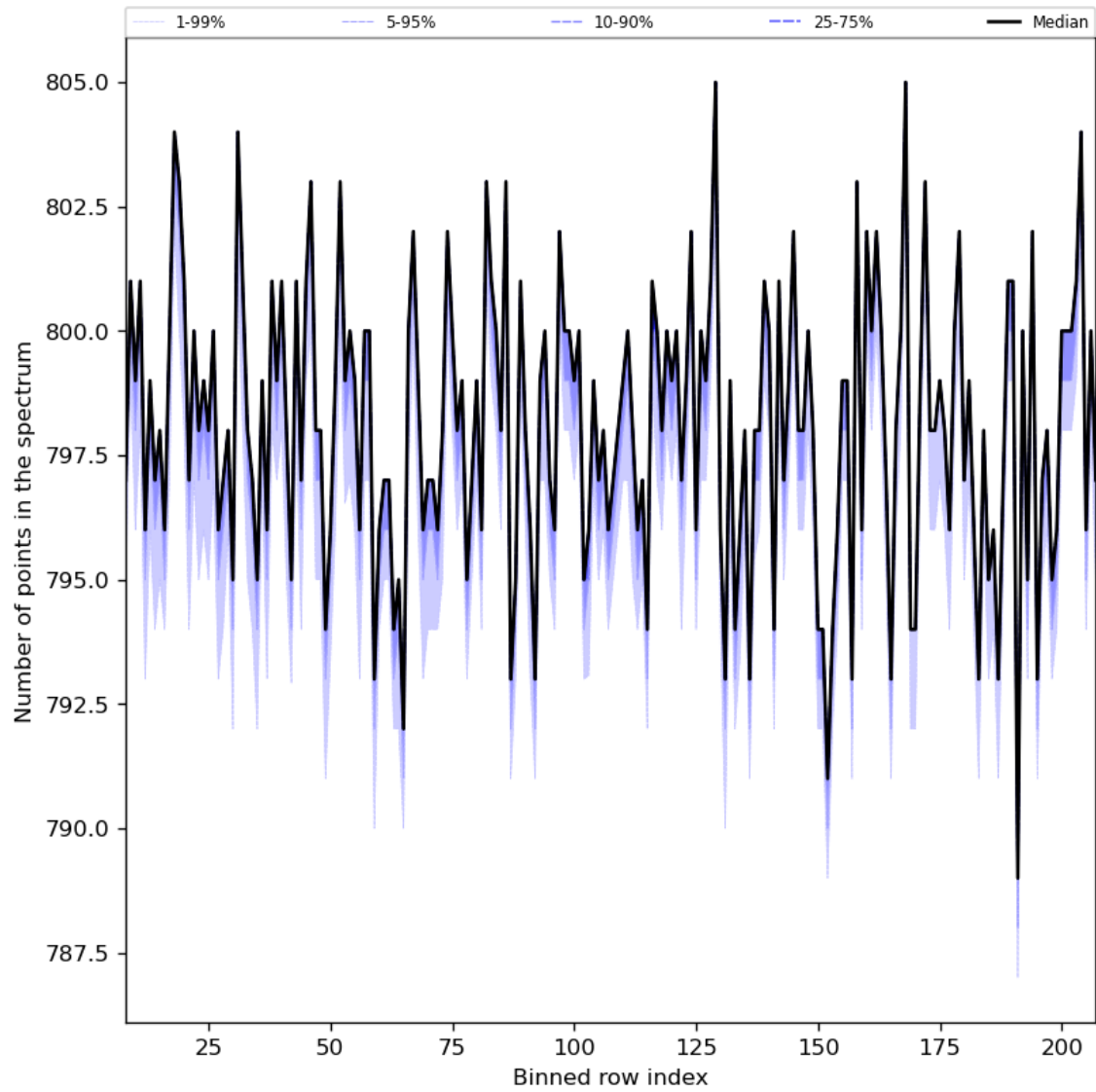
Figure 37: Along track statistics of “Number of points in the spectrum” for 2024-08-11 to 2024-08-11
