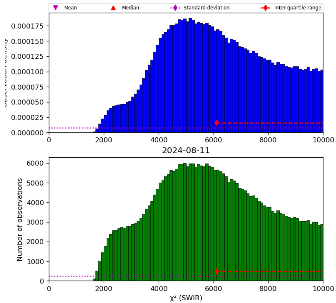
Figure 28: Histogram of “ \chi^2 (SWIR)” for 2024-08-11 to 2024-08-11
