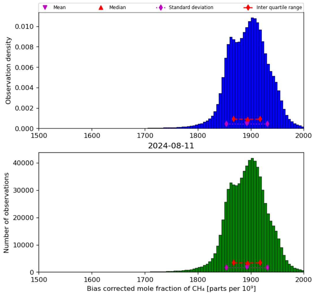
Figure 25: Histogram of “Bias corrected mole fraction of CH 4 ” for 2024-08-11 to 2024-08-11
