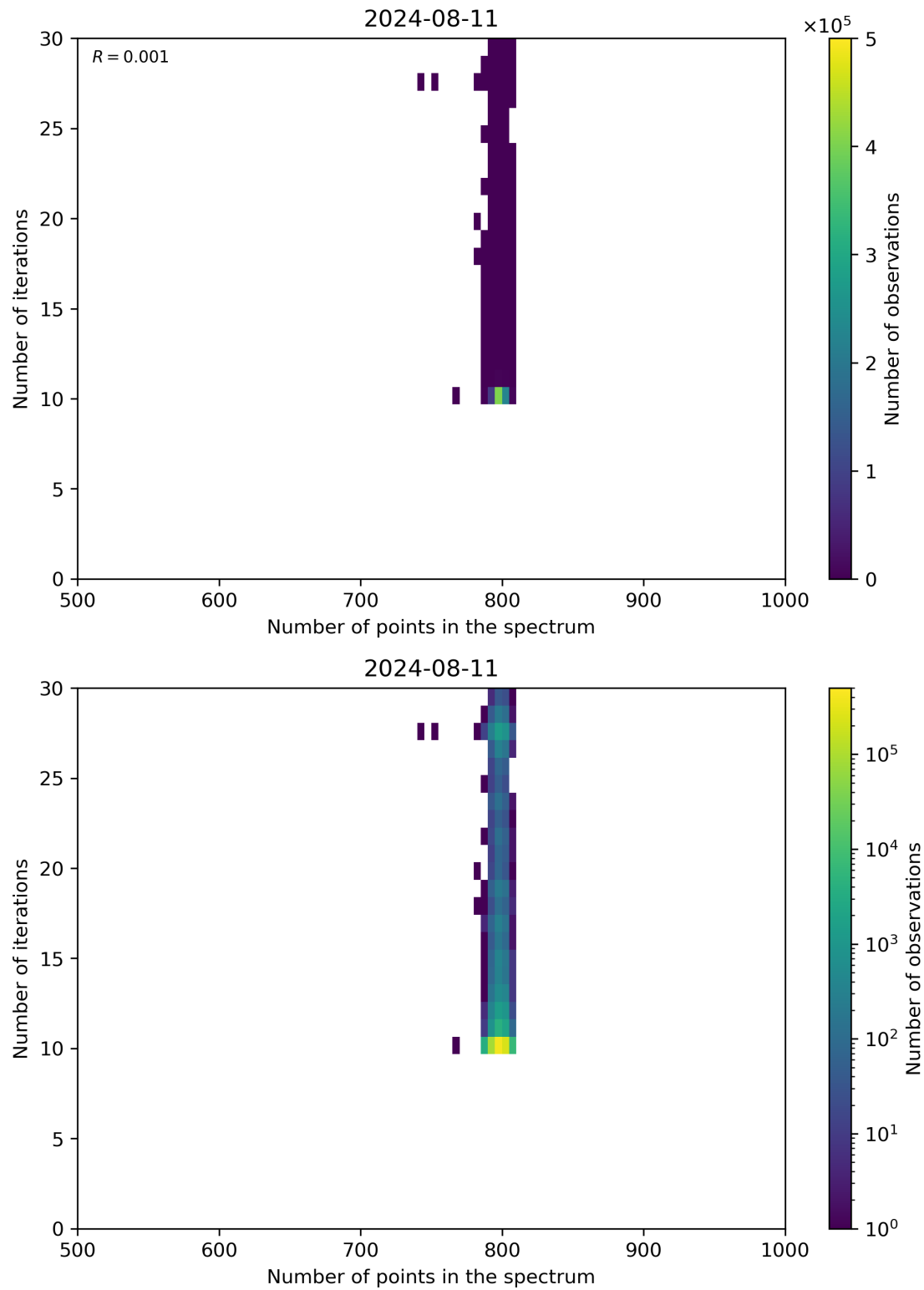
Figure 92: Scatter density plot of “Number of points in the spectrum” against “Number of iterations” for 2024-08-11 to 2024-08-11.
