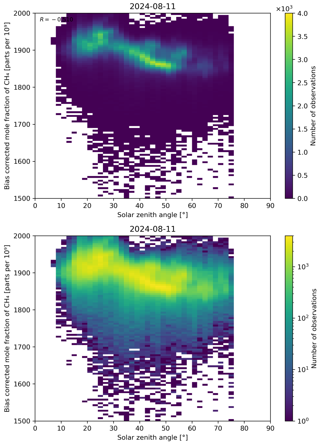
Figure 100: Scatter density plot of “Solar zenith angle” against “Bias corrected mole fraction of CH 4 ” for 2024-08-11 to 2024-08-11.
