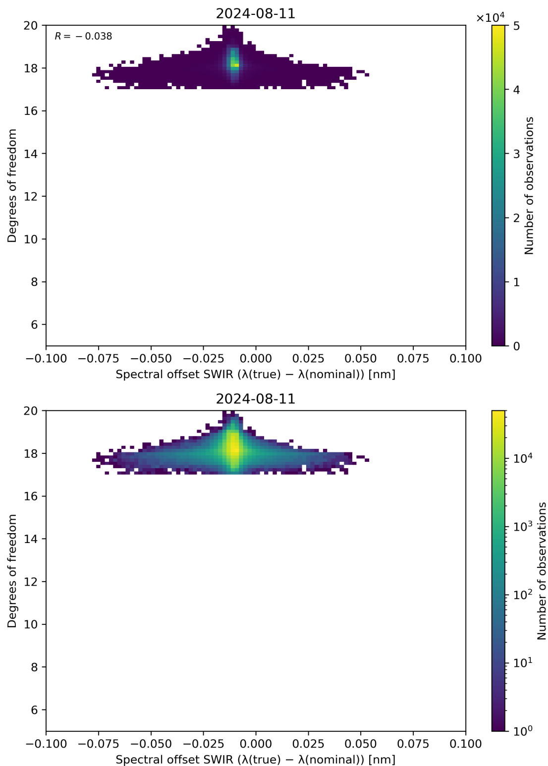
Figure 119: Scatter density plot of “Spectral offset SWIR ( \lambda(\text{true}) - \lambda(\text{nominal}) )” against “Degrees of freedom” for 2024-08-11 to 2024-08-11.
