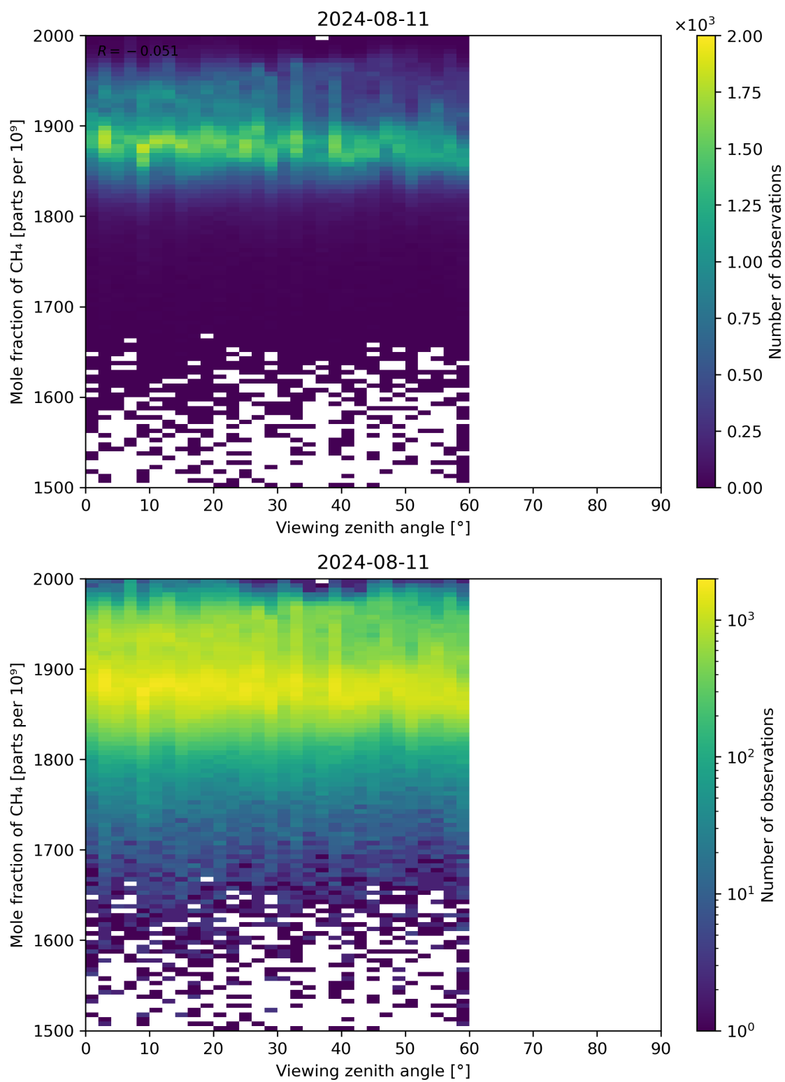
Figure 110: Scatter density plot of “Viewing zenith angle” against “Mole fraction of CH 4 ” for 2024-08-11 to 2024-08-11.
