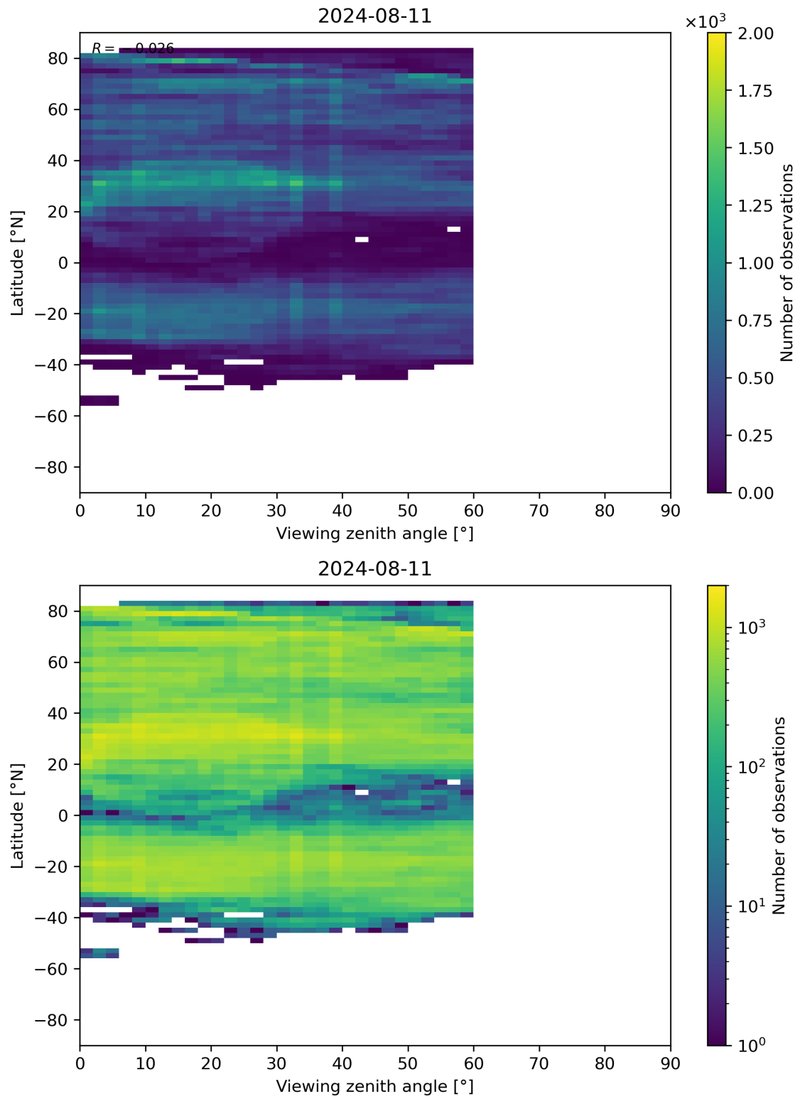
Figure 109: Scatter density plot of “Viewing zenith angle” against “Latitude” for 2024-08-11 to 2024-08-11.
