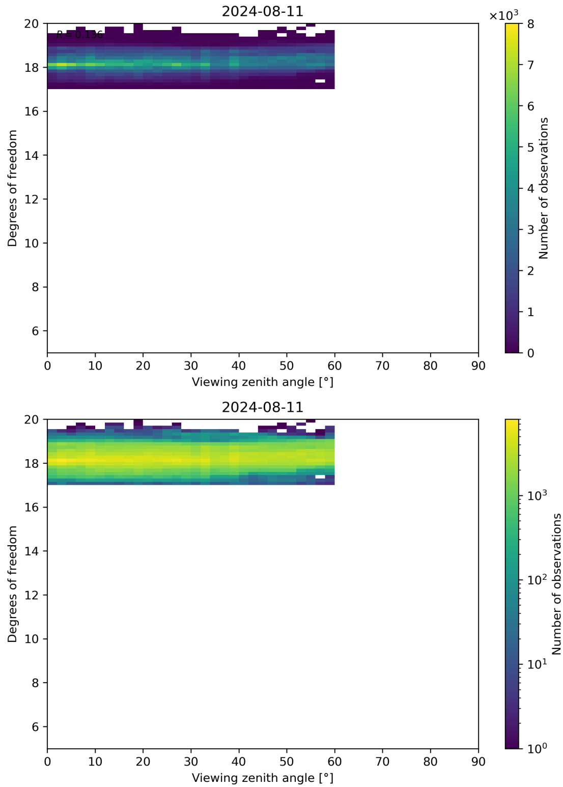
Figure 107: Scatter density plot of “Viewing zenith angle” against “Degrees of freedom” for 2024-08-11 to 2024-08-11.
