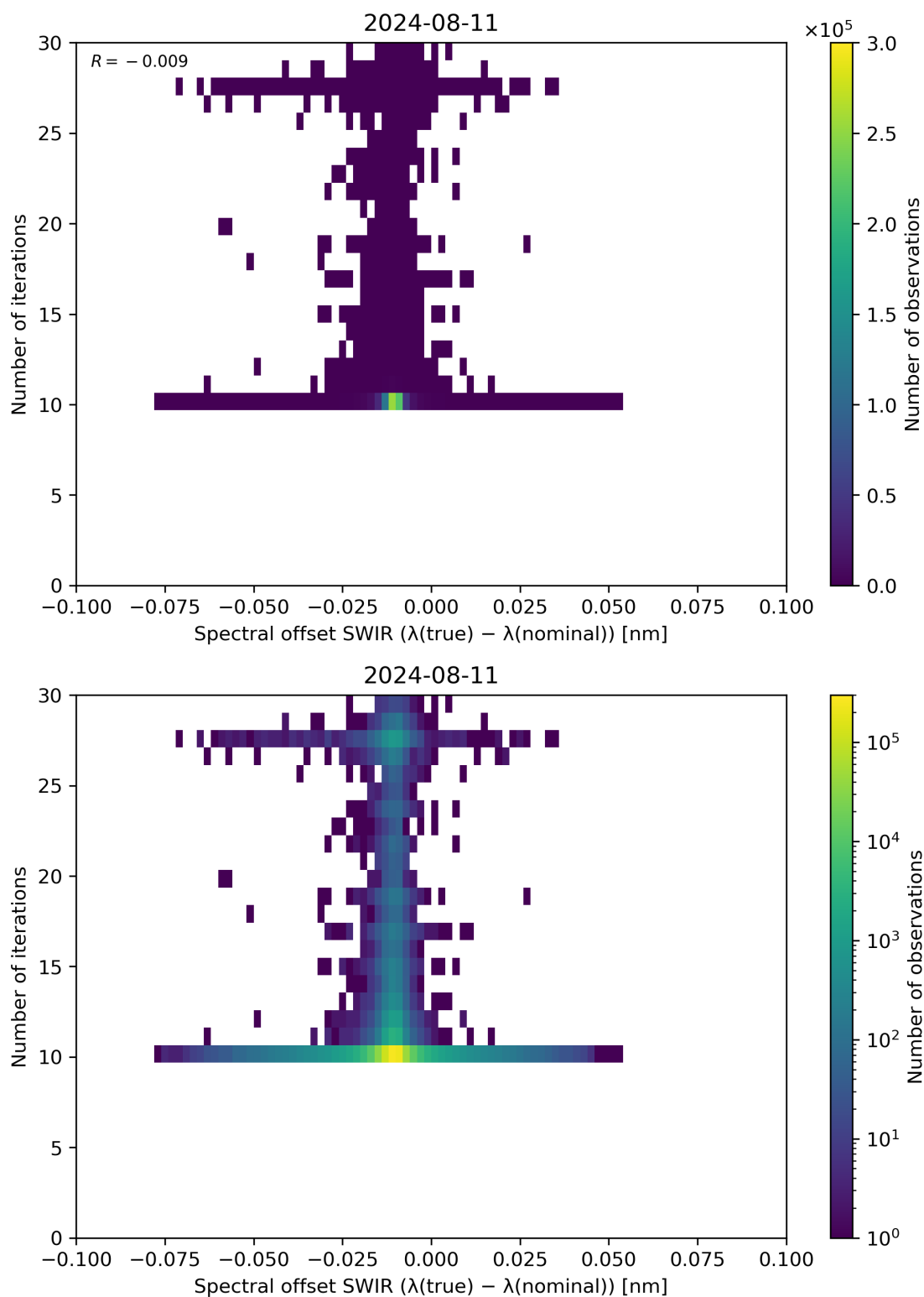
Figure 121: Scatter density plot of “Spectral offset SWIR ( \lambda(\text{true}) - \lambda(\text{nominal}) )” against “Number of iterations” for 2024-08-11 to 2024-08-11.
