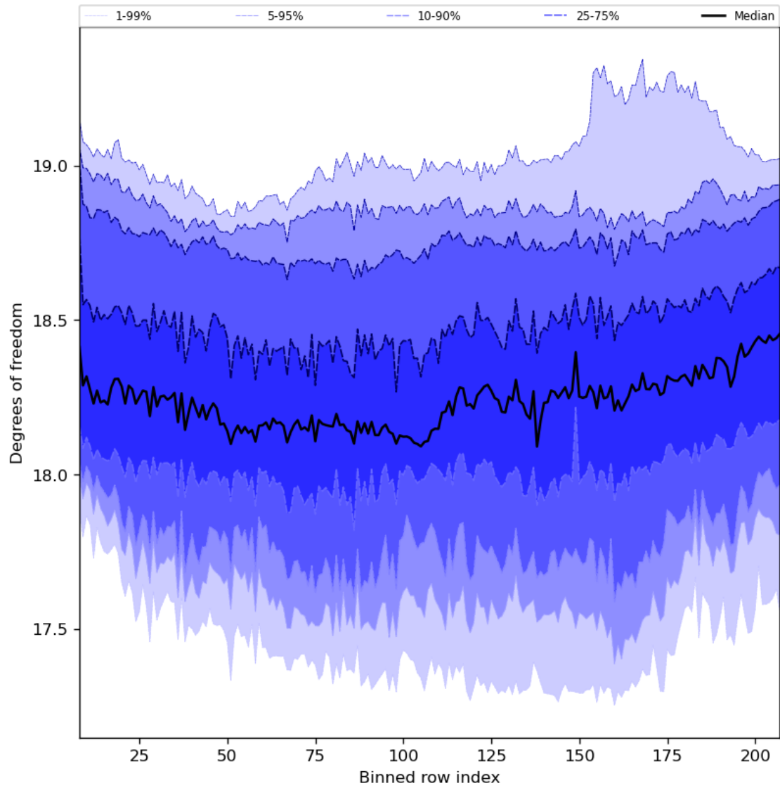
Figure 41: Along track statistics of “Degrees of freedom” for 2024-08-11 to 2024-08-11
