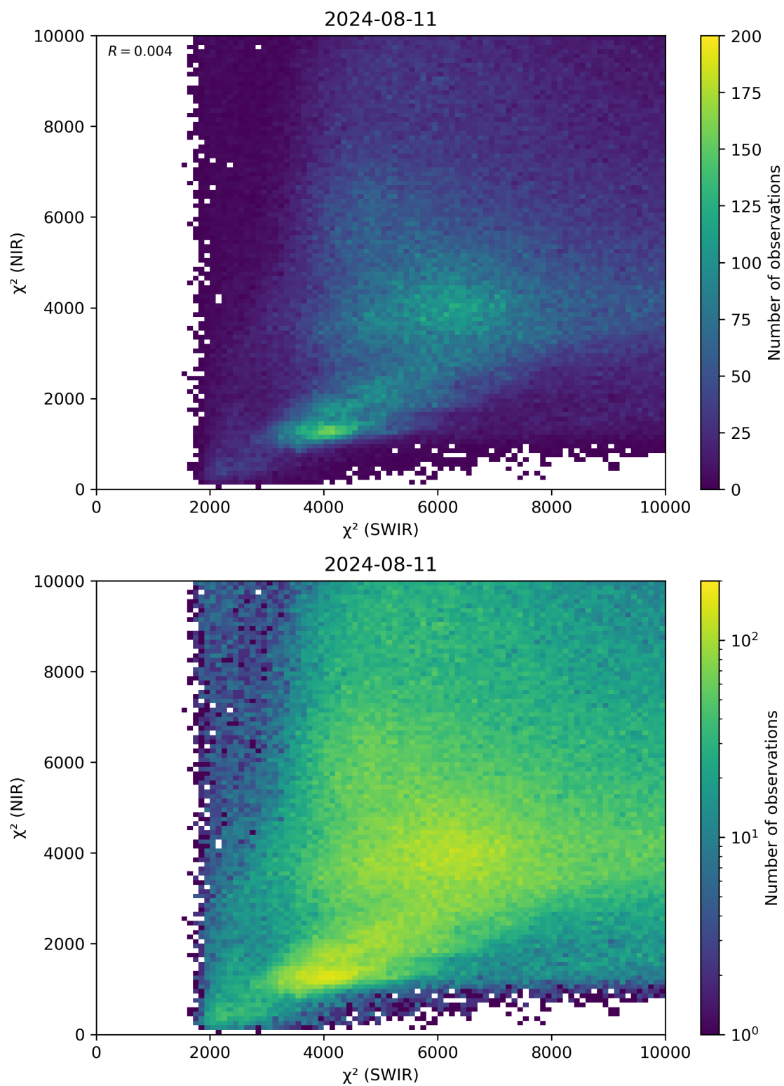
Figure 47: Scatter density plot of “ \chi^2 (SWIR)” against “ \chi^2 (NIR)” for 2024-08-11 to 2024-08-11.
