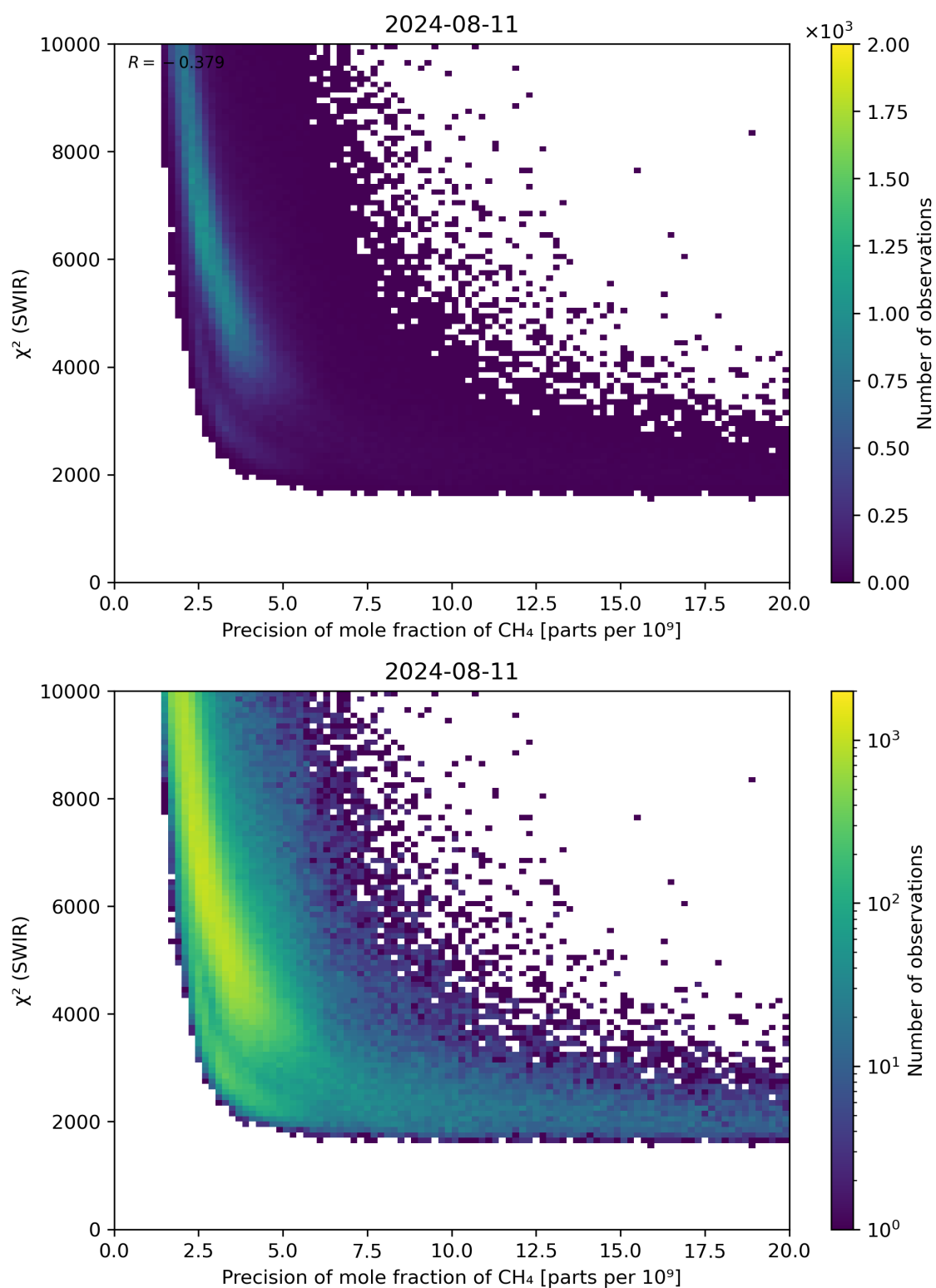
Figure 79: Scatter density plot of “Precision of mole fraction of \text{CH}_4 ” against “ \chi^2 (SWIR)” for 2024-08-11 to 2024-08-11.
