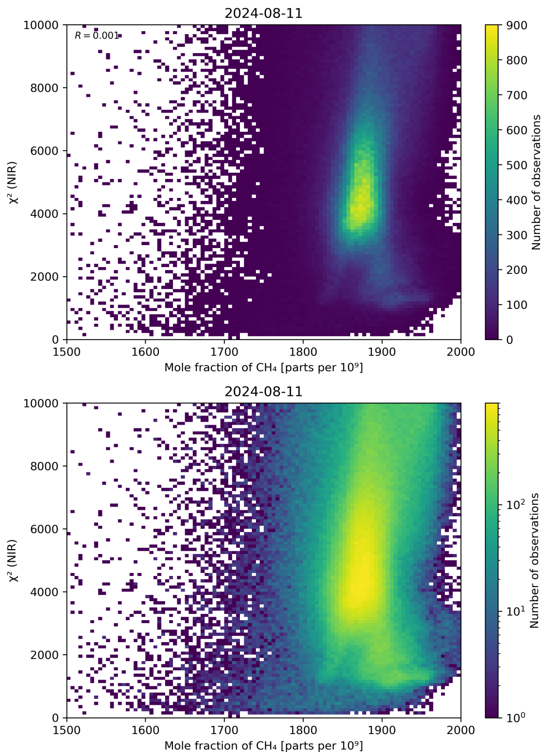
Figure 70: Scatter density plot of “Mole fraction of \text{CH}_4 ” against “ \chi^2 (NIR)” for 2024-08-11 to 2024-08-11.
