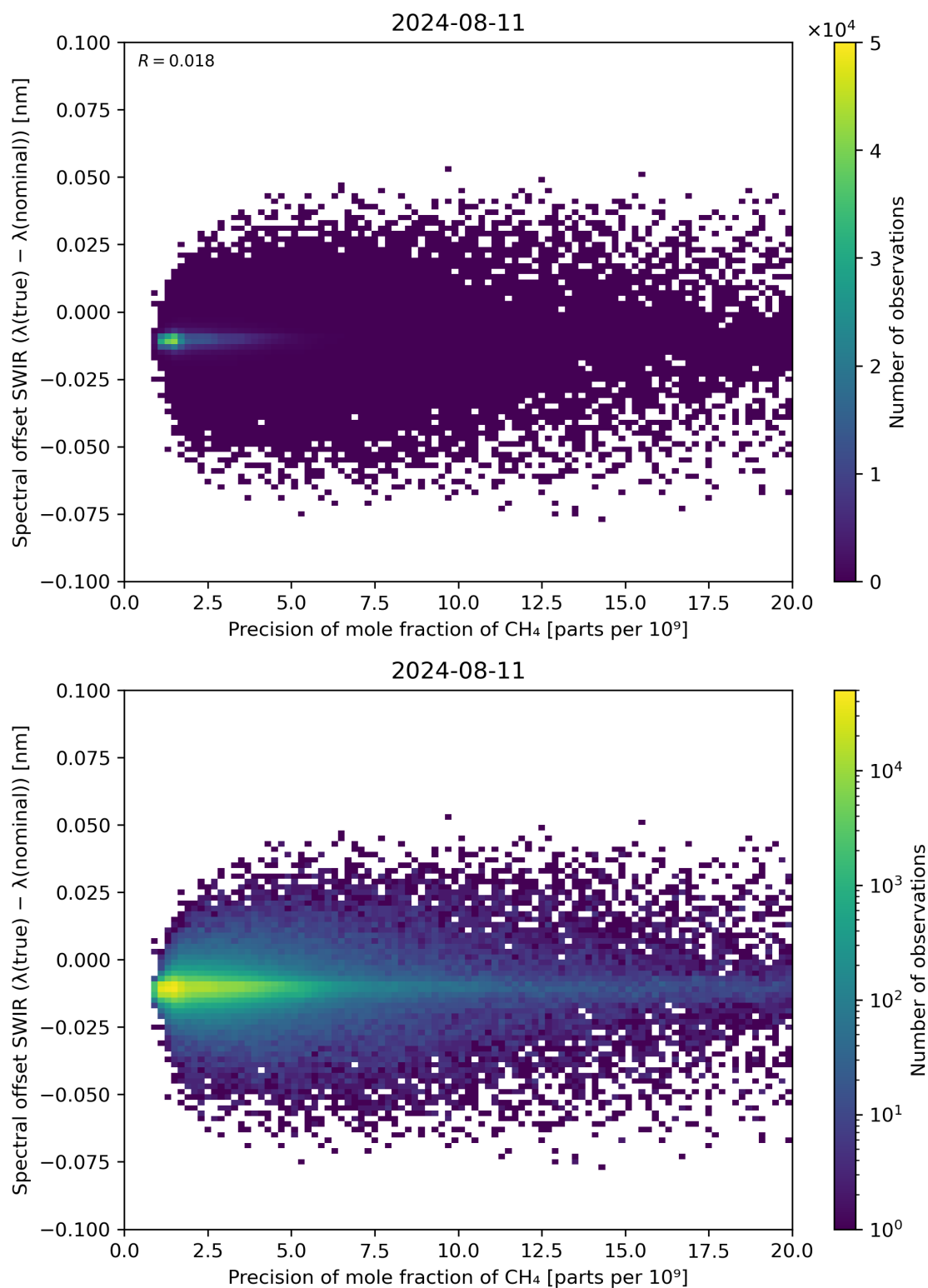
Figure 85: Scatter density plot of “Precision of mole fraction of CH 4 ” against “Spectral offset SWIR ( \lambda(\text{true}) - \lambda(\text{nominal}) )” for 2024-08-11 to 2024-08-11.
