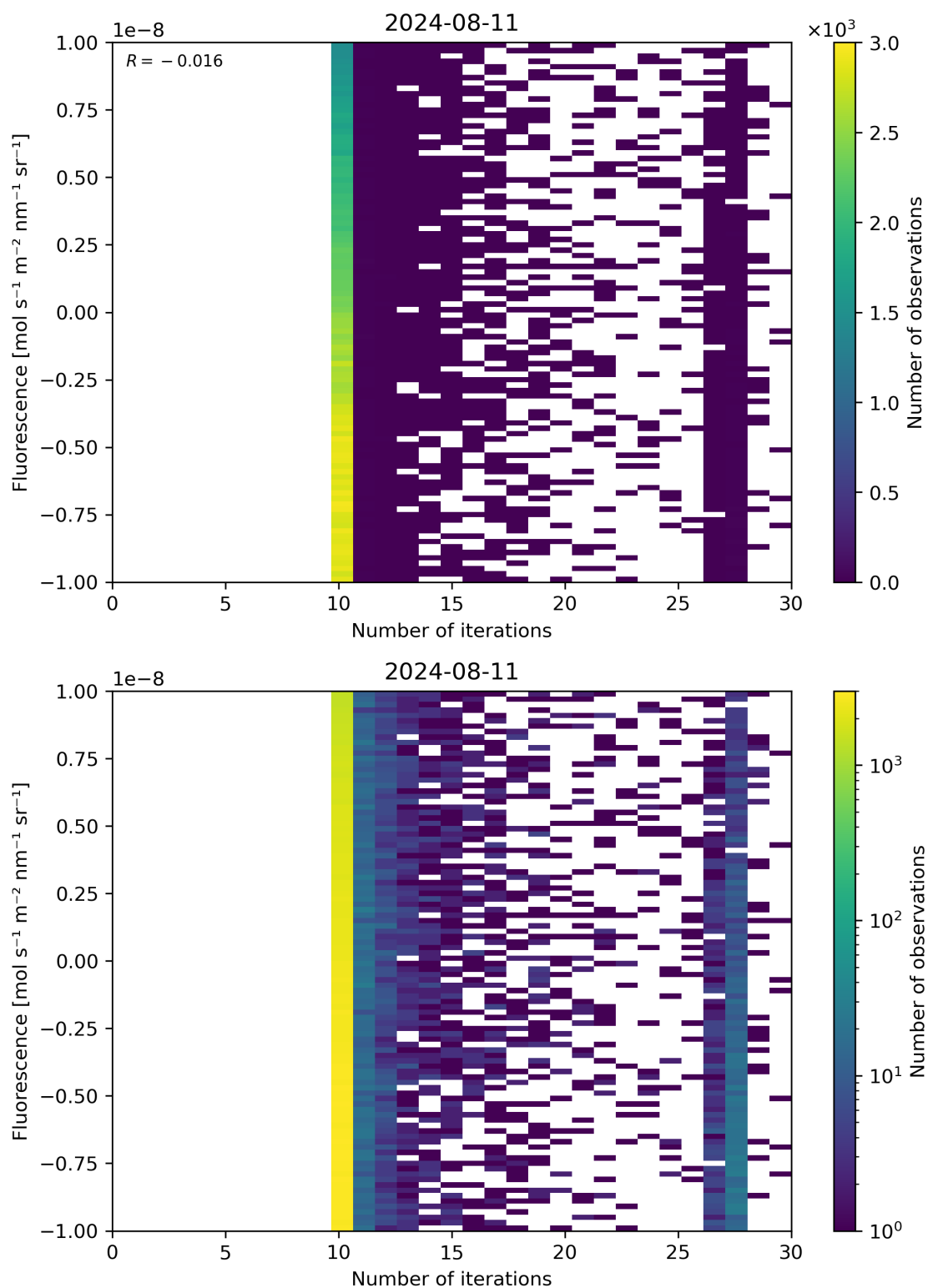
Figure 87: Scatter density plot of “Number of iterations” against “Fluorescence” for 2024-08-11 to 2024-08-11.
