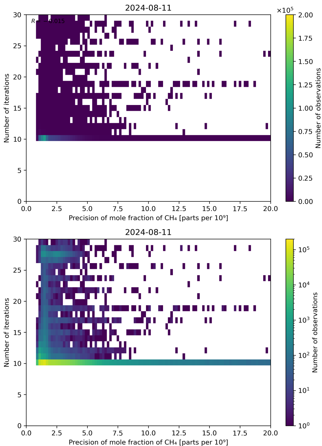
Figure 83: Scatter density plot of “Precision of mole fraction of CH 4 ” against “Number of iterations” for 2024-08-11 to 2024-08-11.
