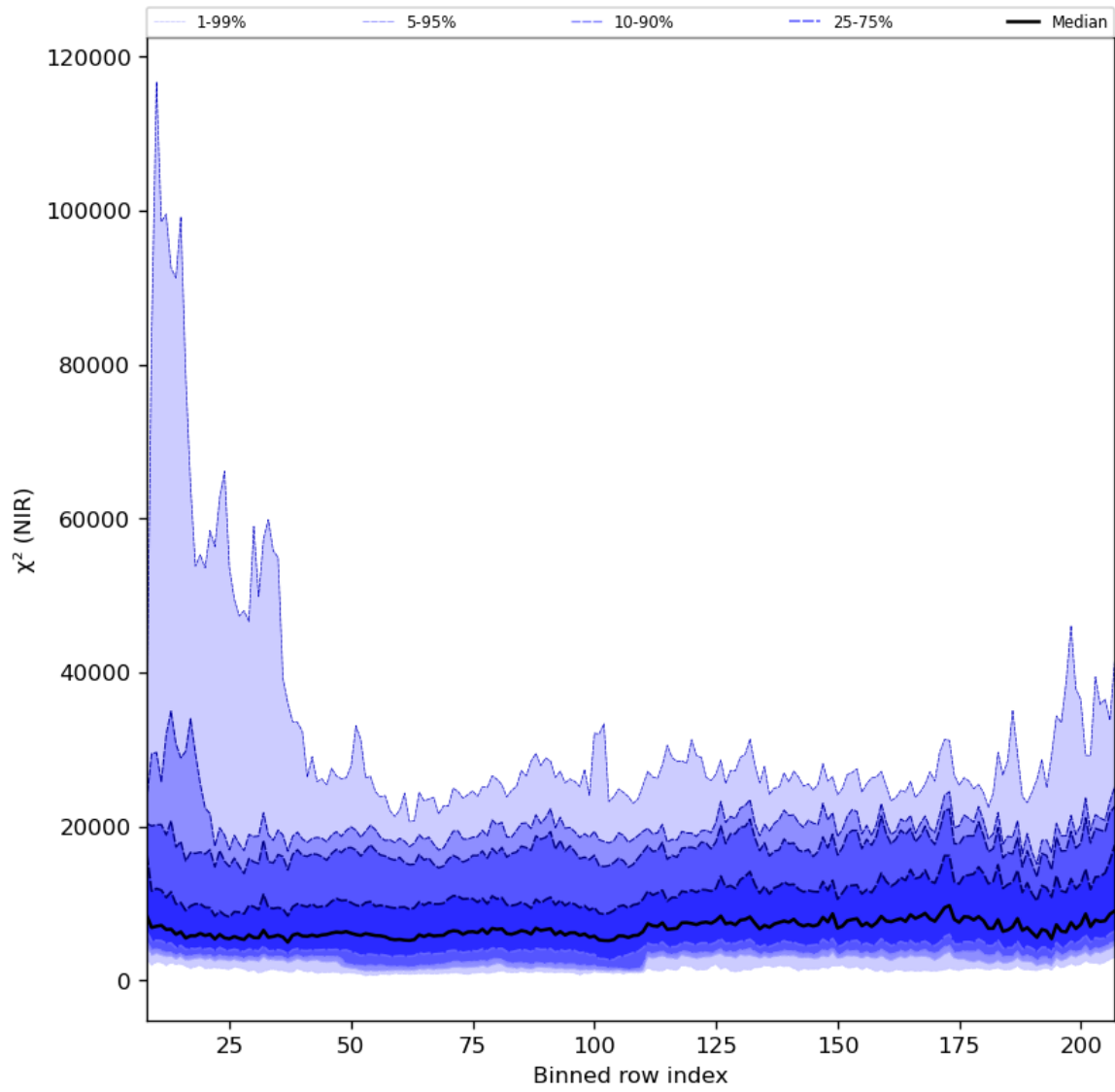
Figure 40: Along track statistics of “ \chi^2 (NIR)” for 2024-08-11 to 2024-08-11
