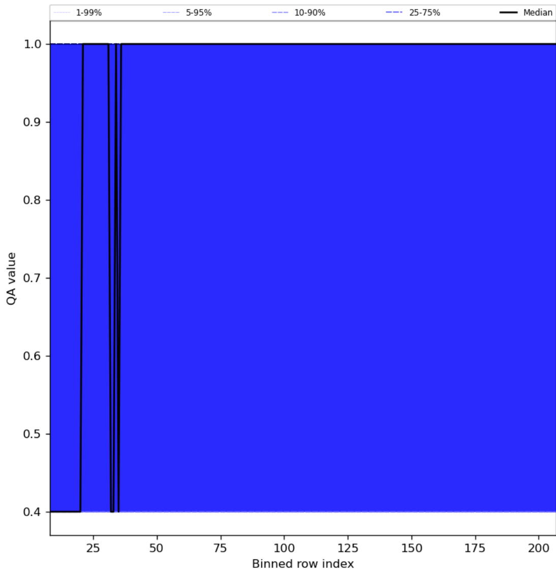
Figure 33: Along track statistics of “QA value” for 2024-08-11 to 2024-08-11
