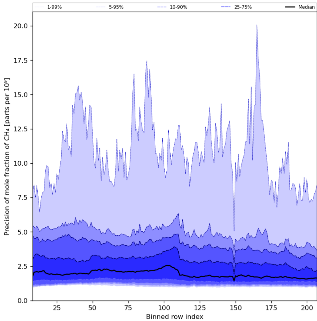
Figure 35: Along track statistics of “Precision of mole fraction of CH 4 ” for 2024-08-11 to 2024-08-11
