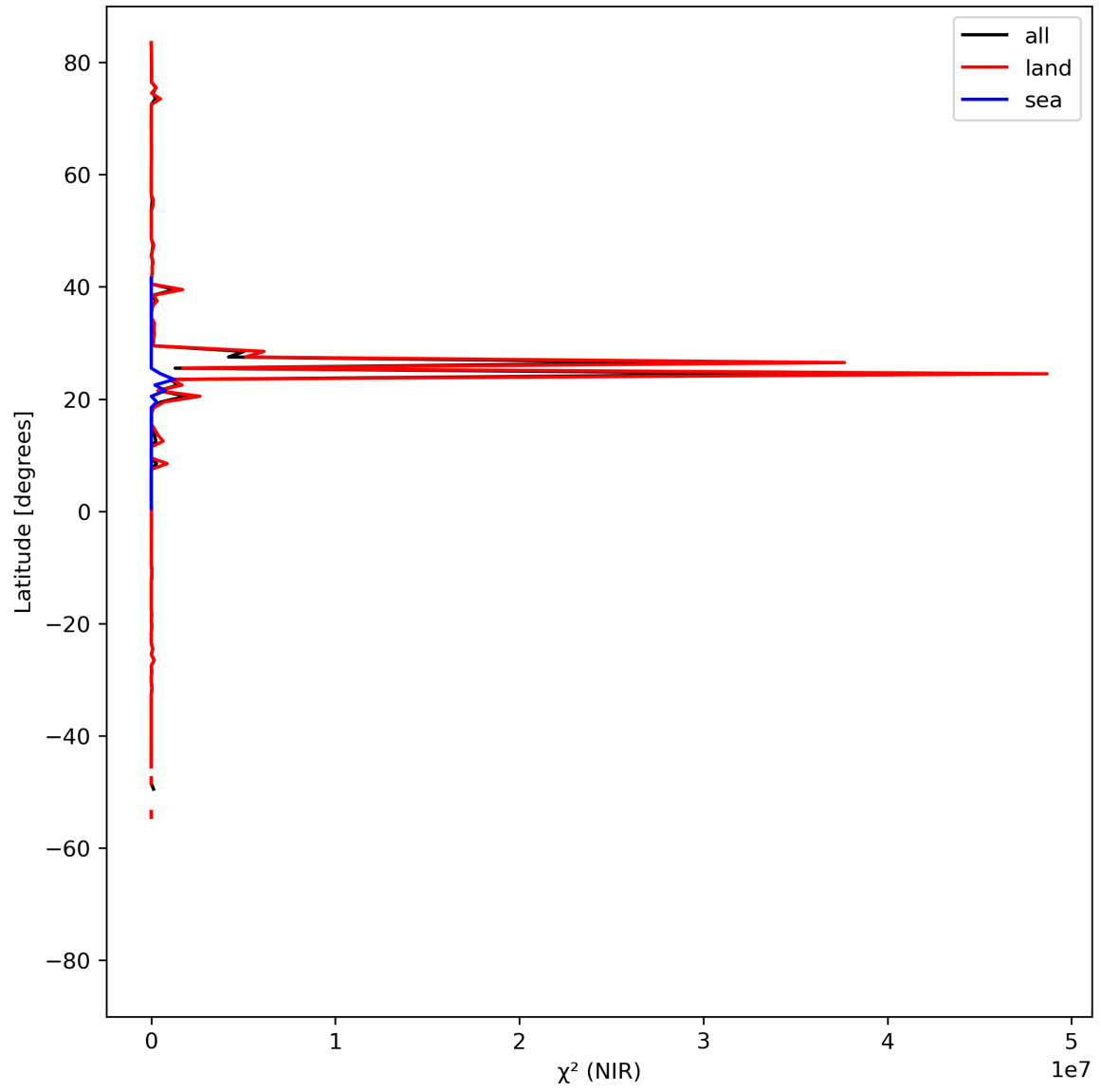
Figure 18: Zonal average of “ \chi^2 (NIR)” for 2024-08-11 to 2024-08-11.
