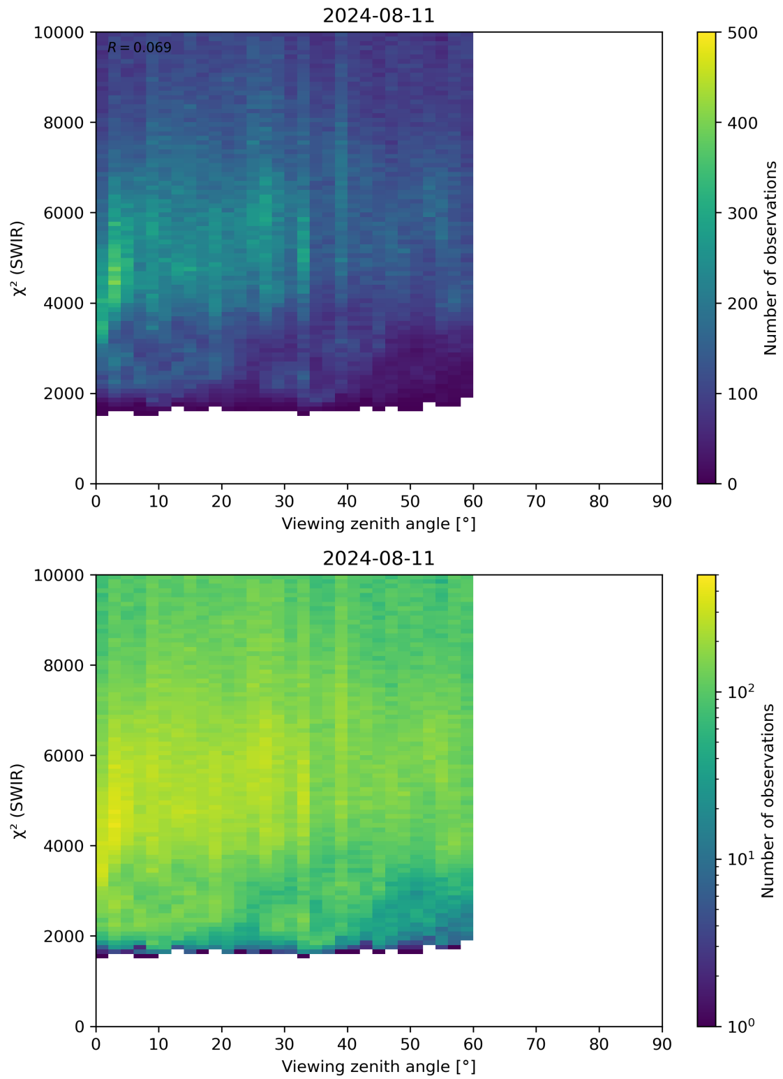
Figure 106: Scatter density plot of “Viewing zenith angle” against “ \chi^2 (SWIR)” for 2024-08-11 to 2024-08-11.
