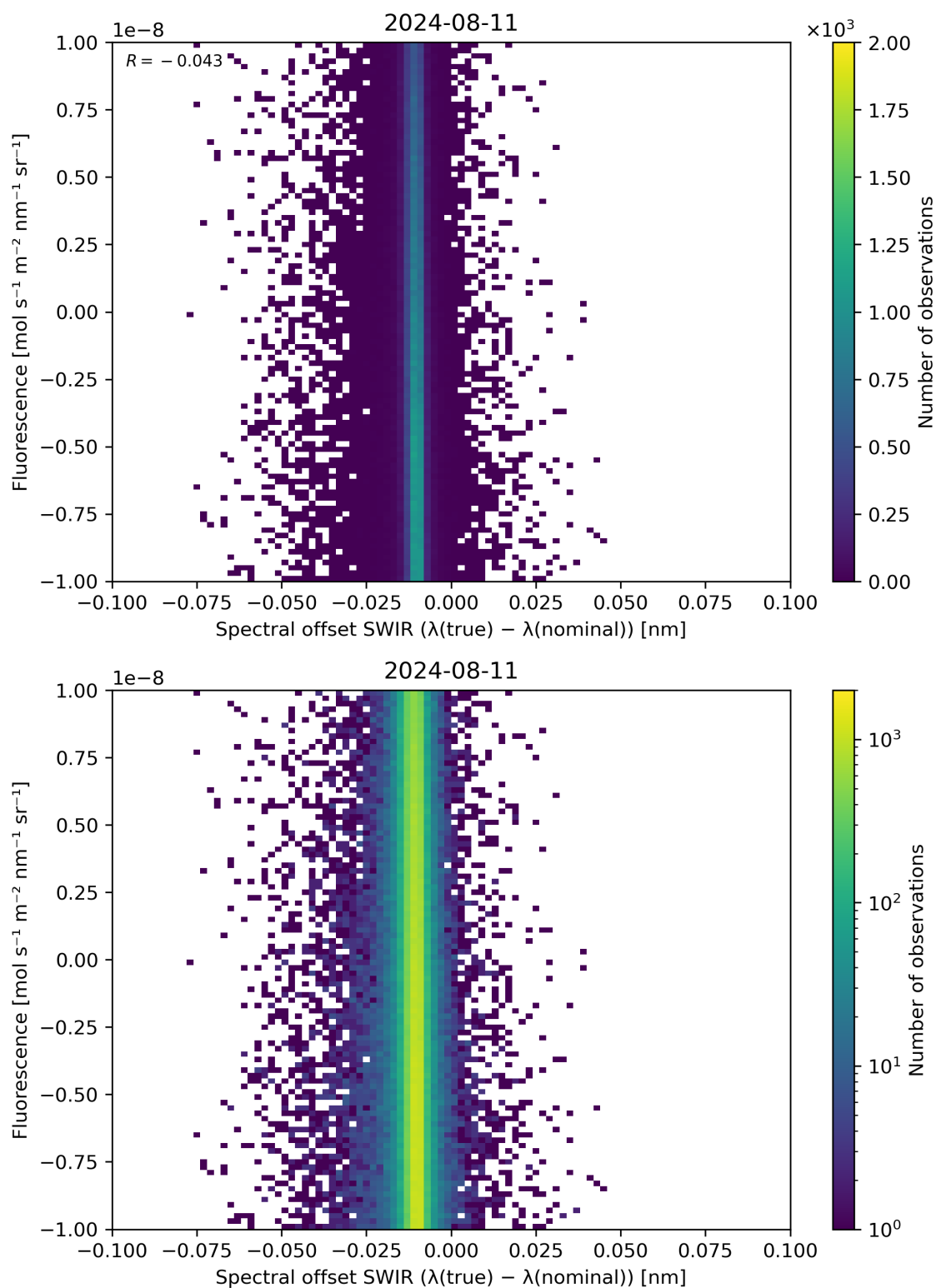
Figure 120: Scatter density plot of “Spectral offset SWIR ( \lambda(\text{true}) - \lambda(\text{nominal}) )” against “Fluorescence” for 2024-08-11 to 2024-08-11.
