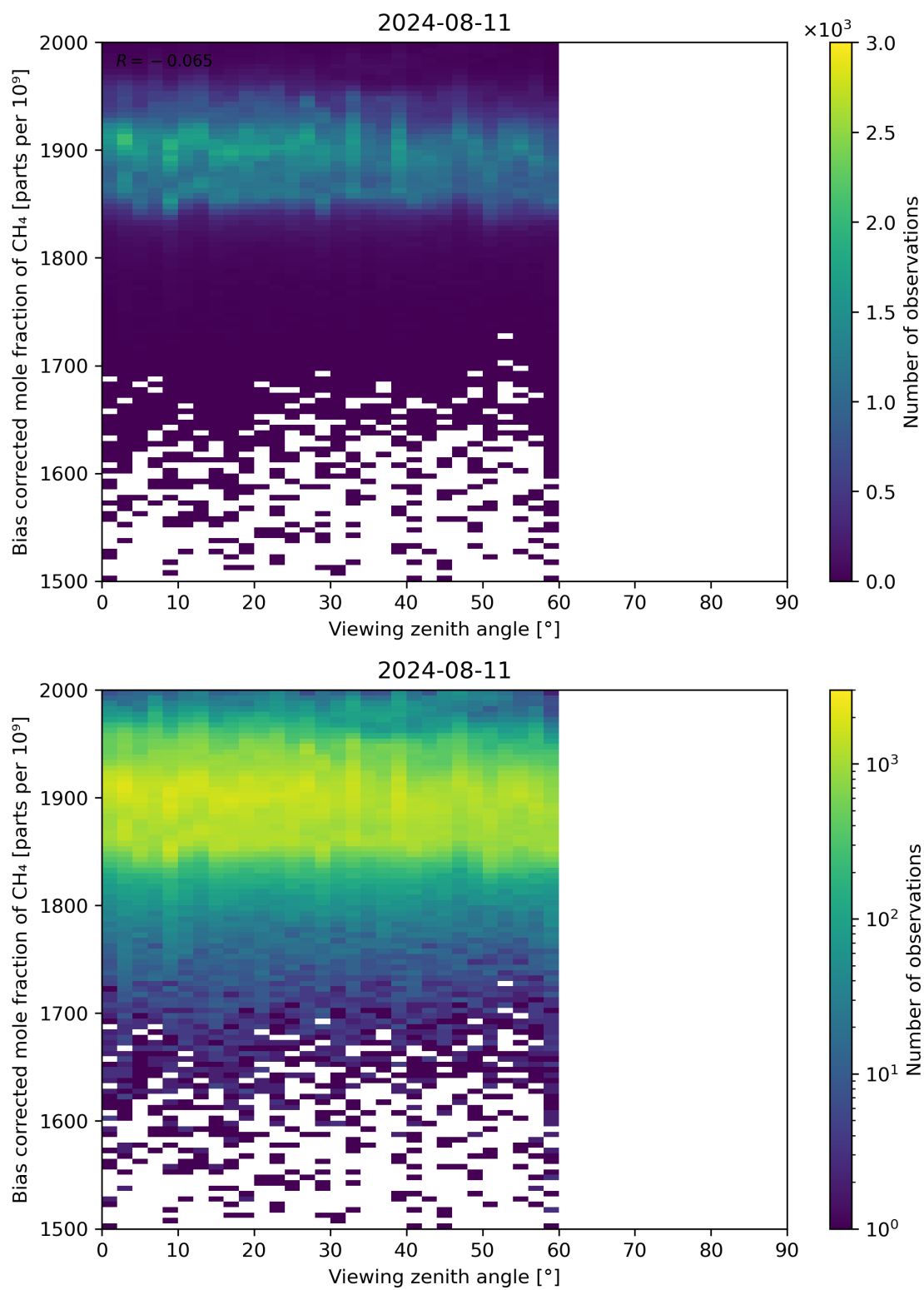
Figure 111: Scatter density plot of “Viewing zenith angle” against “Bias corrected mole fraction of CH 4 ” for 2024-08-11 to 2024-08-11.
