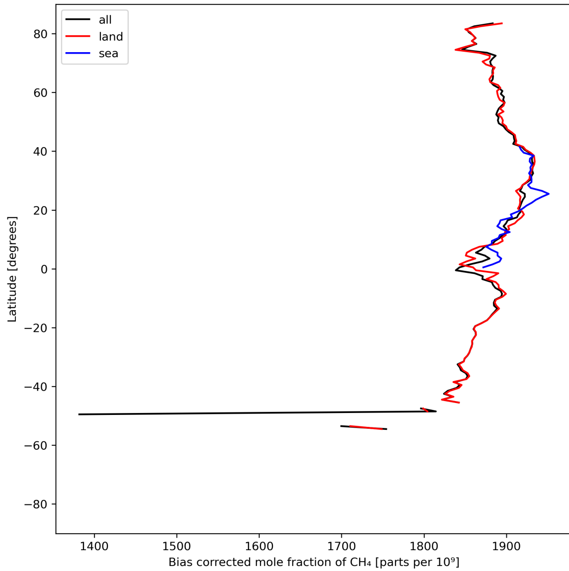
Figure 14: Zonal average of “Bias corrected mole fraction of CH 4 ” for 2024-08-11 to 2024-08-11.
