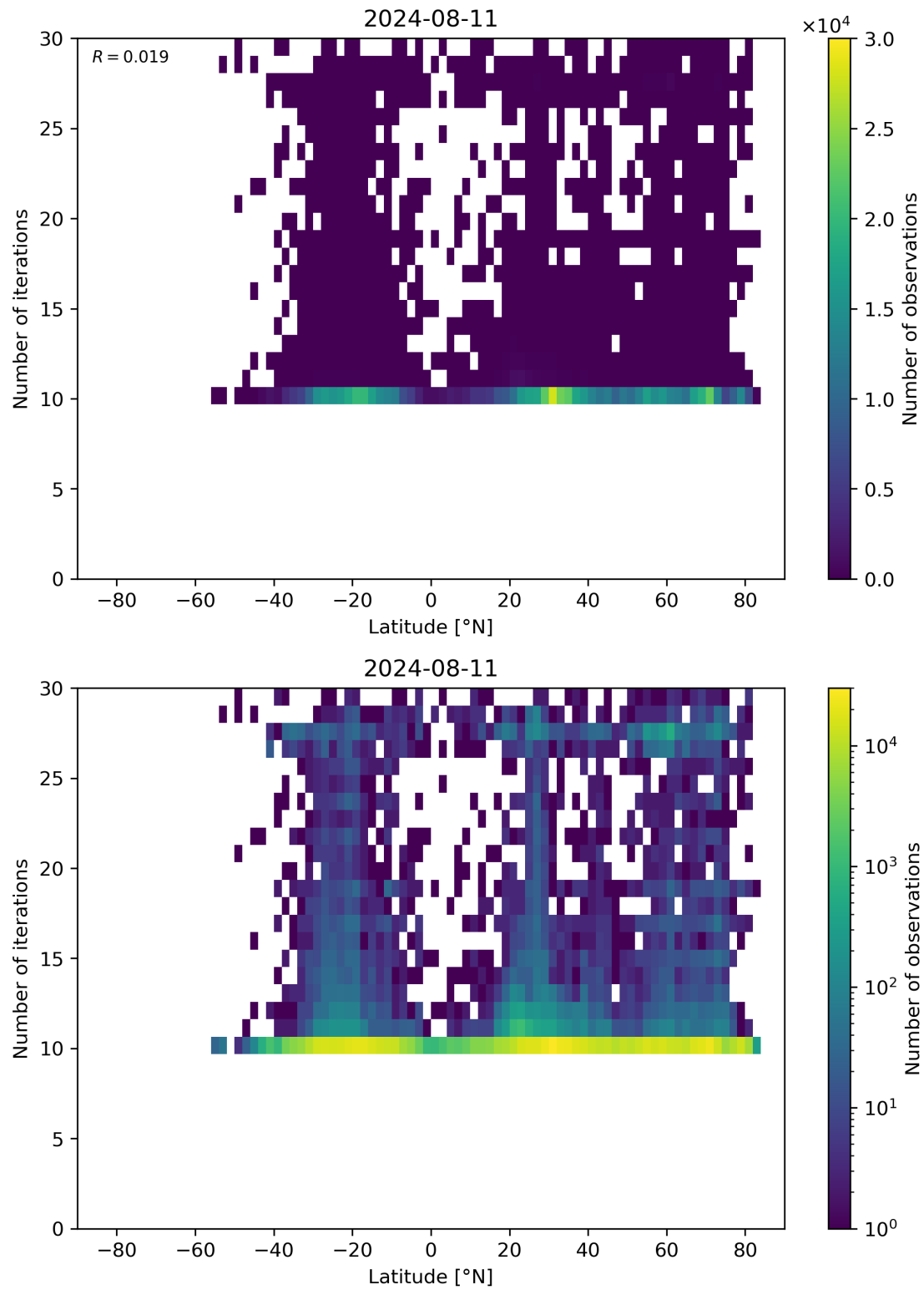
Figure 60: Scatter density plot of “Latitude” against “Number of iterations” for 2024-08-11 to 2024-08-11.
