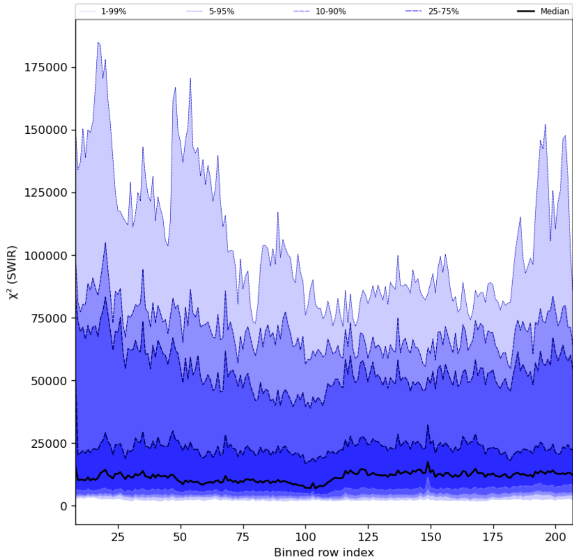
Figure 39: Along track statistics of “ \chi^2 (SWIR)” for 2024-08-11 to 2024-08-11
