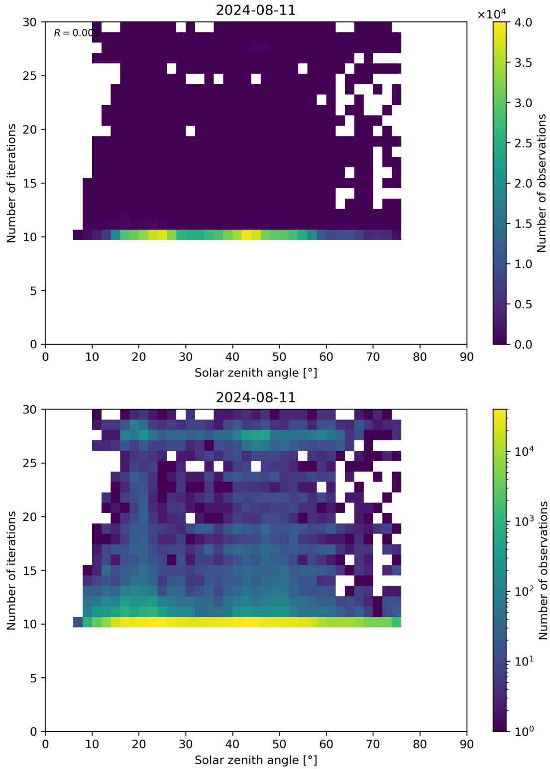
Figure 102: Scatter density plot of “Solar zenith angle” against “Number of iterations” for 2024-08-11 to 2024-08-11.
