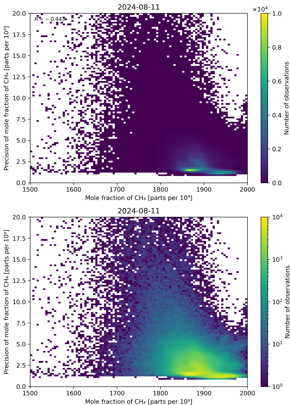
Figure 75: Scatter density plot of “Mole fraction of CH 4 ” against “Precision of mole fraction of CH 4 ” for 2024-08-11 to 2024-08-11.
