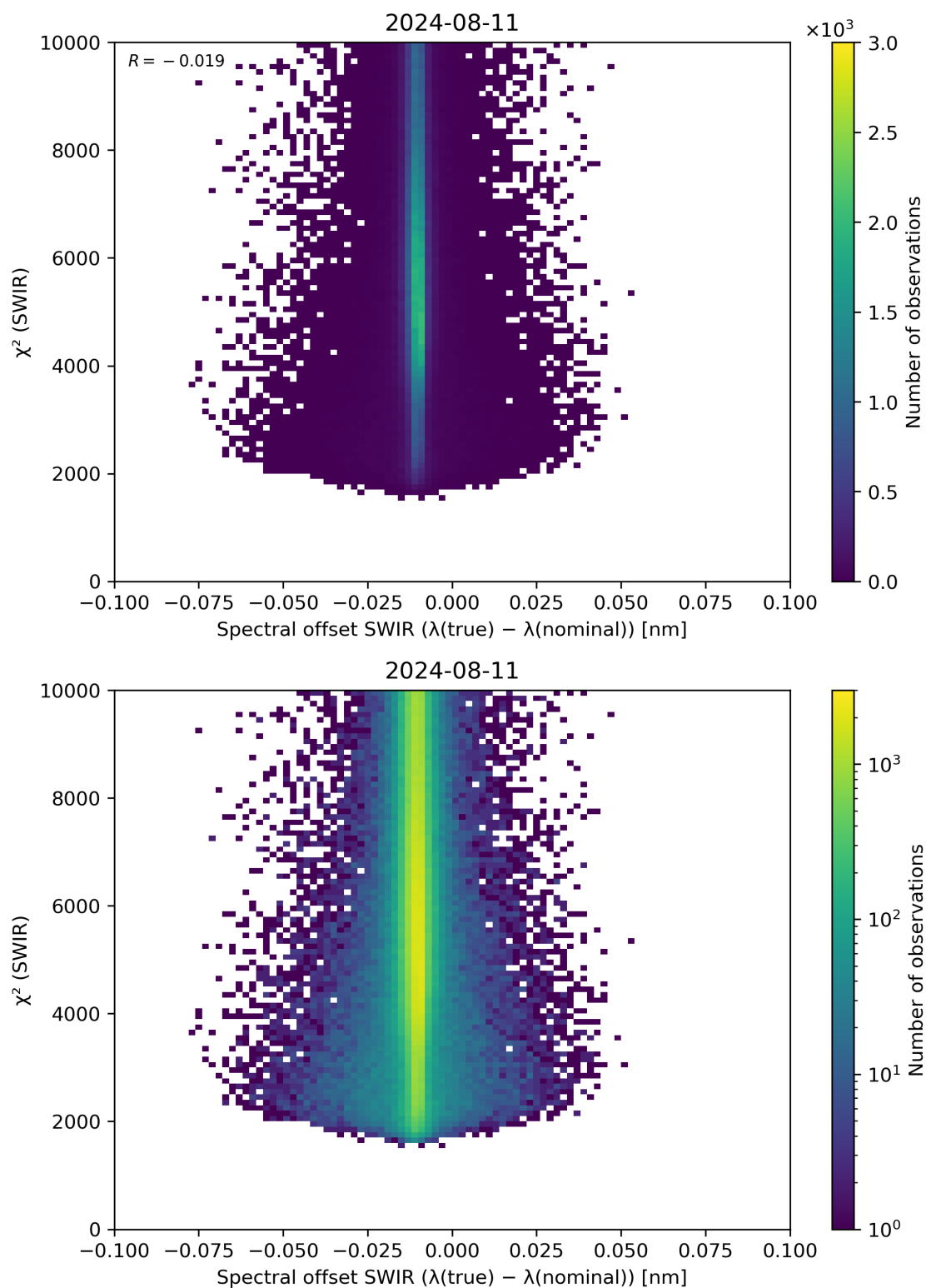
Figure 118: Scatter density plot of “Spectral offset SWIR ( \lambda(\text{true}) - \lambda(\text{nominal}) )” against “ \chi^2 (SWIR)” for 2024-08-11 to 2024-08-11.
