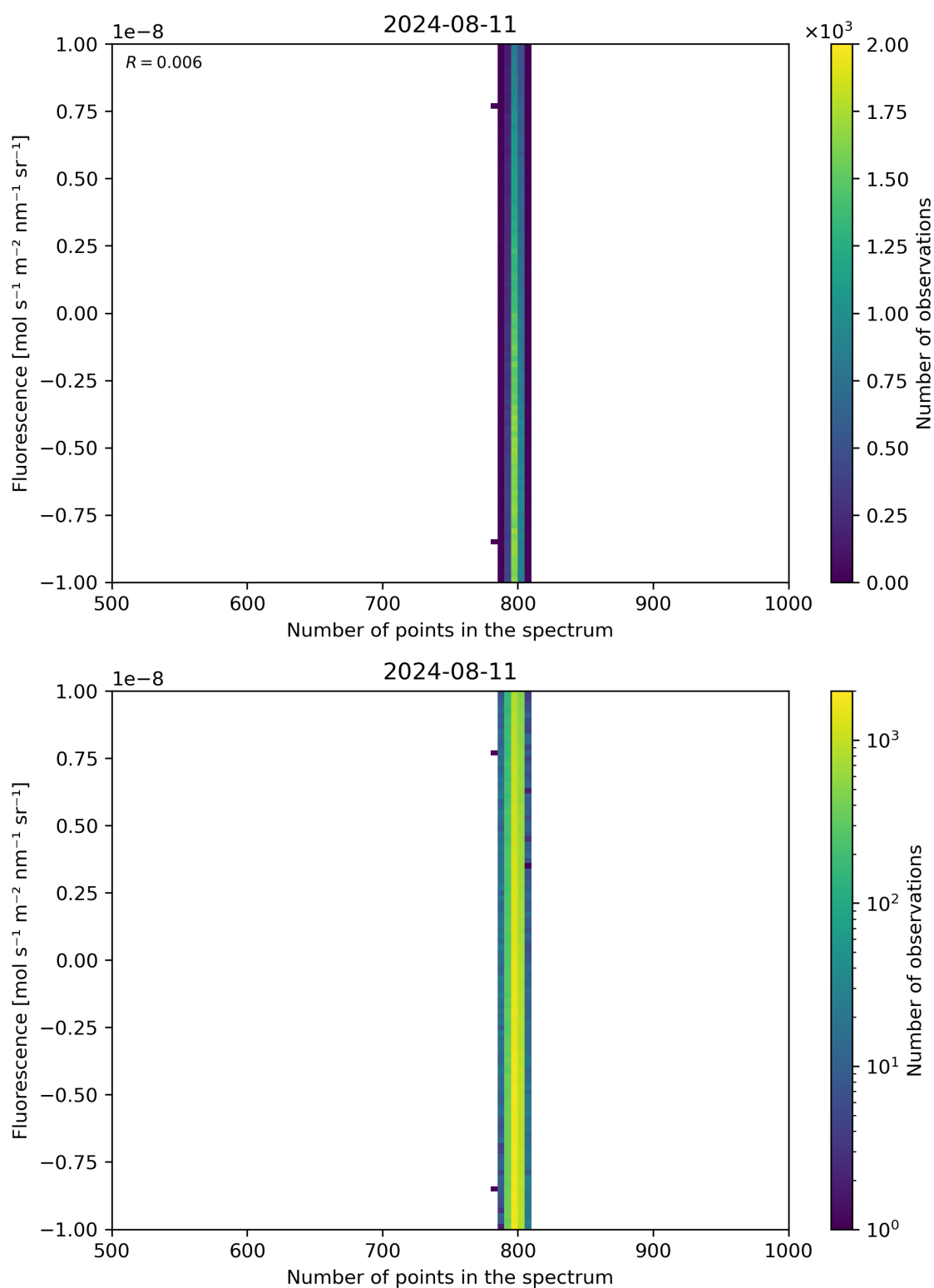
Figure 91: Scatter density plot of “Number of points in the spectrum” against “Fluorescence” for 2024-08-11 to 2024-08-11.
