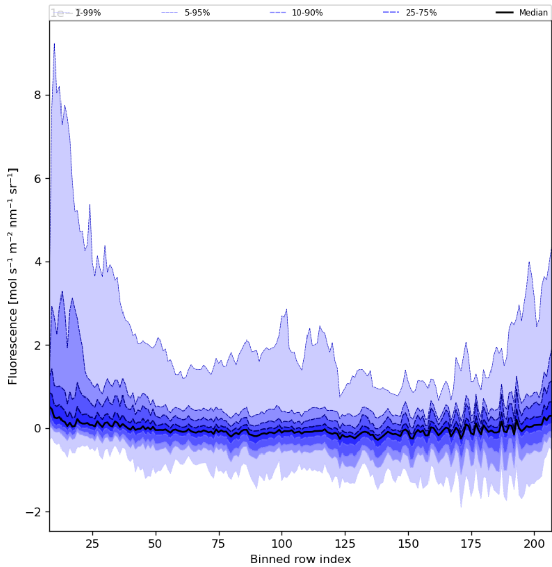
Figure 43: Along track statistics of “Fluorescence” for 2024-08-11 to 2024-08-11
