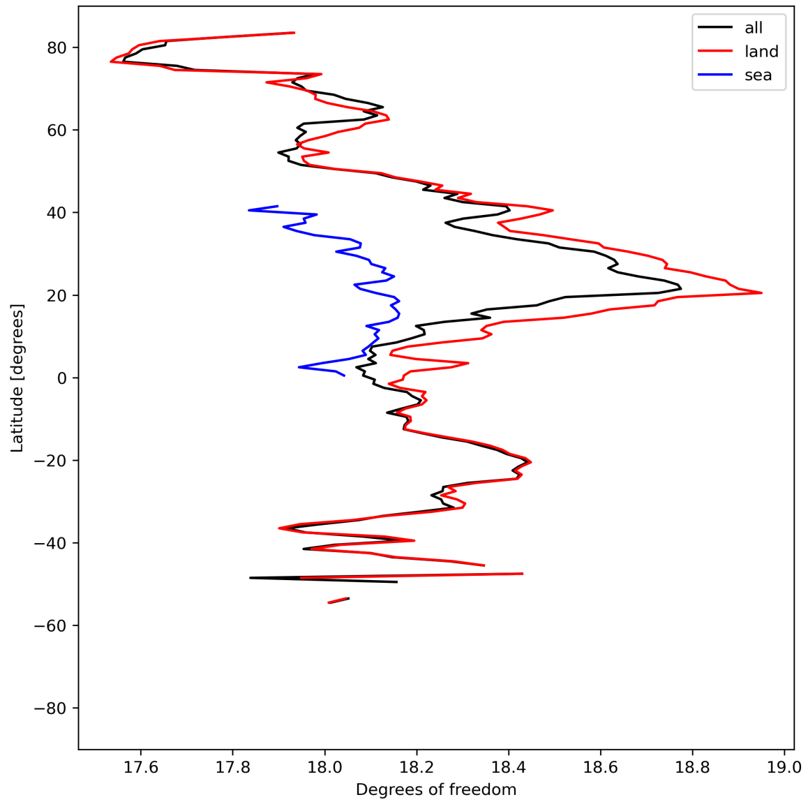
Figure 19: Zonal average of “Degrees of freedom” for 2024-08-11 to 2024-08-11.
