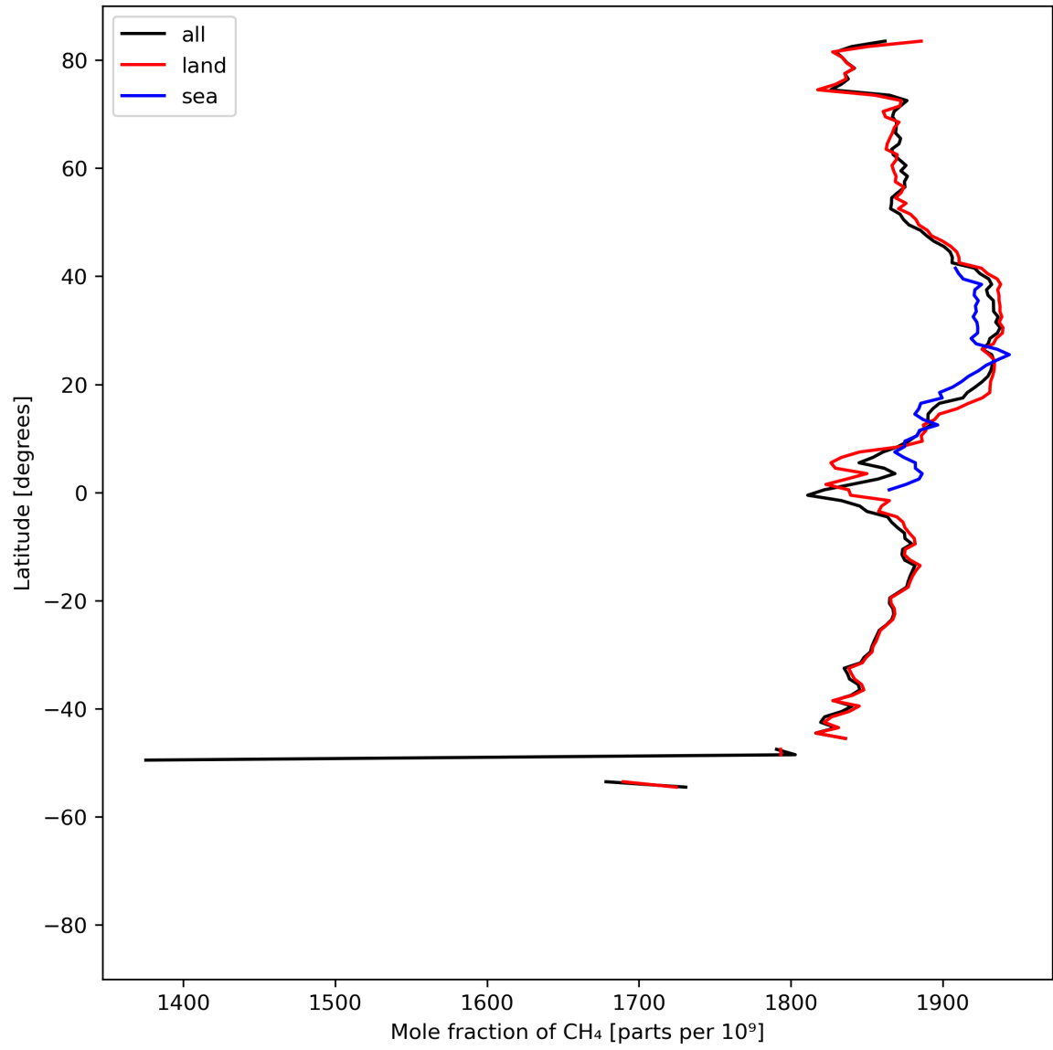
Figure 12: Zonal average of “Mole fraction of \text{CH}_4 ” for 2024-08-11 to 2024-08-11.
