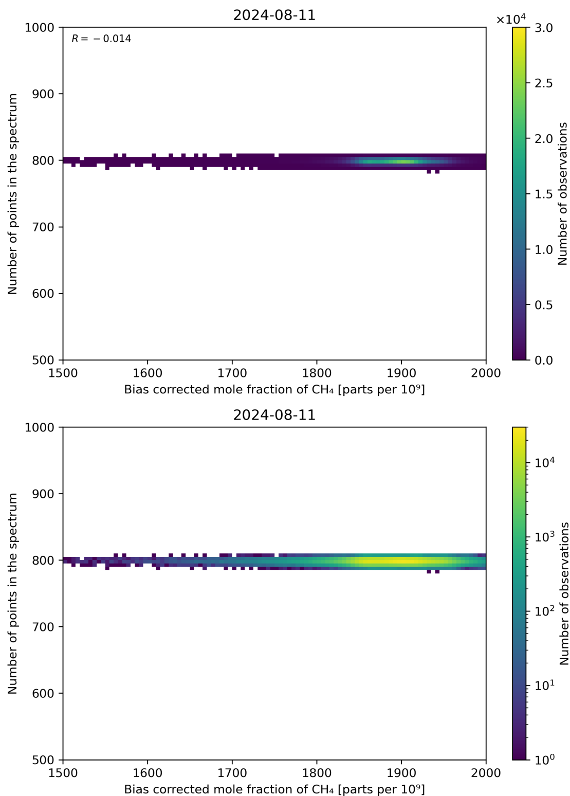
Figure 68: Scatter density plot of “Bias corrected mole fraction of CH 4 ” against “Number of points in the spectrum” for 2024-08-11 to 2024-08-11.
