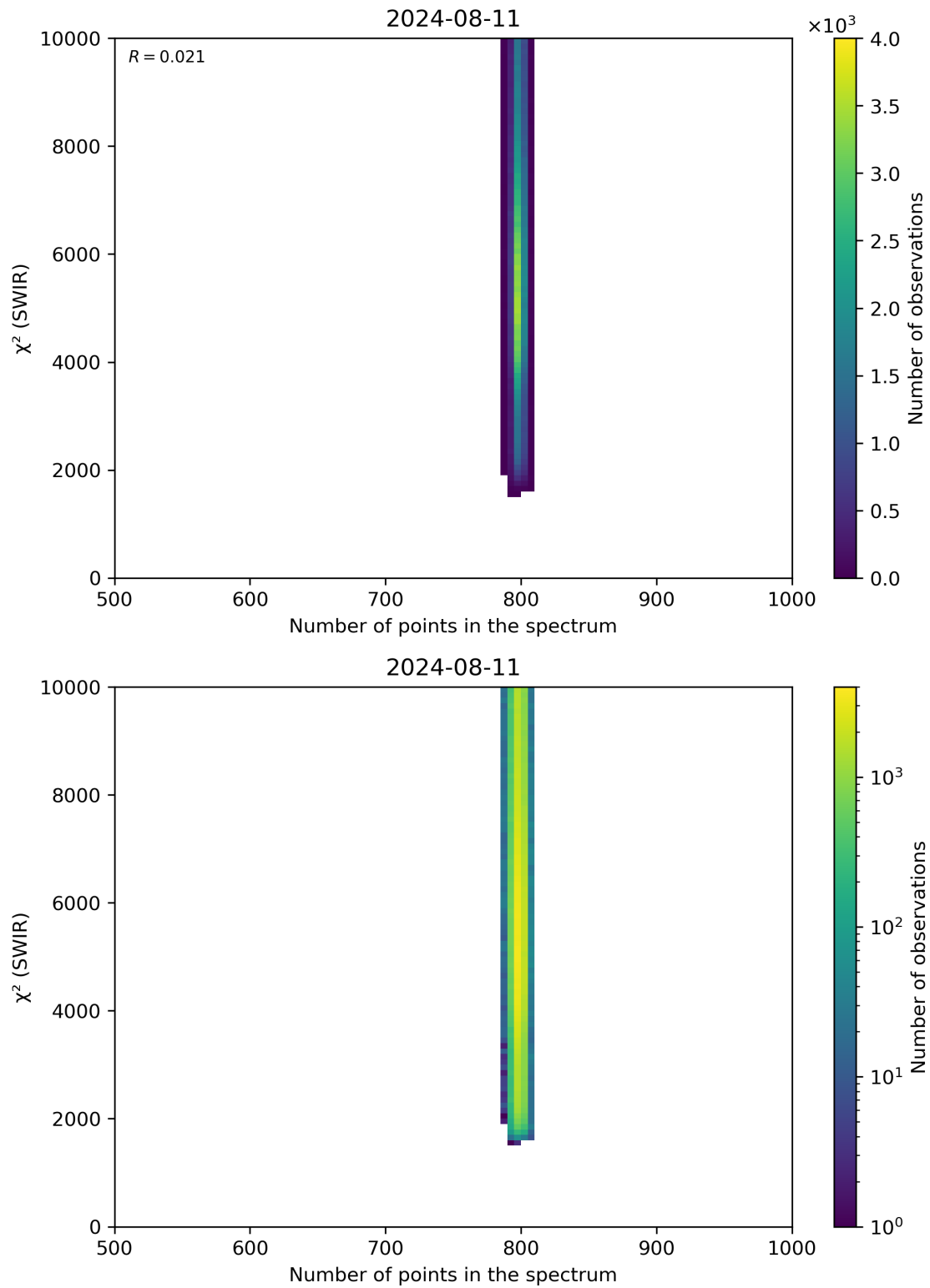
Figure 89: Scatter density plot of “Number of points in the spectrum” against “ \chi^2 (SWIR)” for 2024-08-11 to 2024-08-11.
