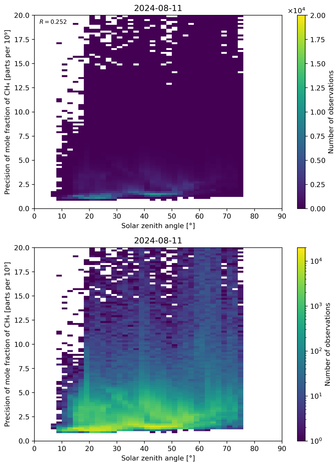
Figure 101: Scatter density plot of “Solar zenith angle” against “Precision of mole fraction of CH 4 ” for 2024-08-11 to 2024-08-11.
