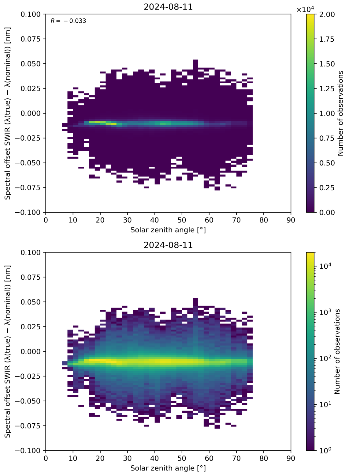
Figure 104: Scatter density plot of “Solar zenith angle” against “Spectral offset SWIR ( \lambda(\text{true}) - \lambda(\text{nominal}) )” for 2024-08-11 to 2024-08-11.
