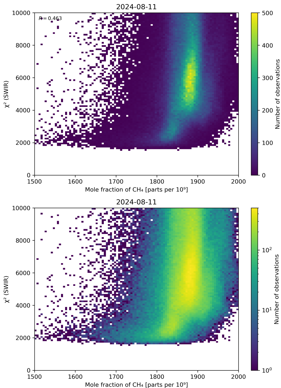
Figure 71: Scatter density plot of “Mole fraction of \text{CH}_4 ” against “ \chi^2 (SWIR)” for 2024-08-11 to 2024-08-11.
