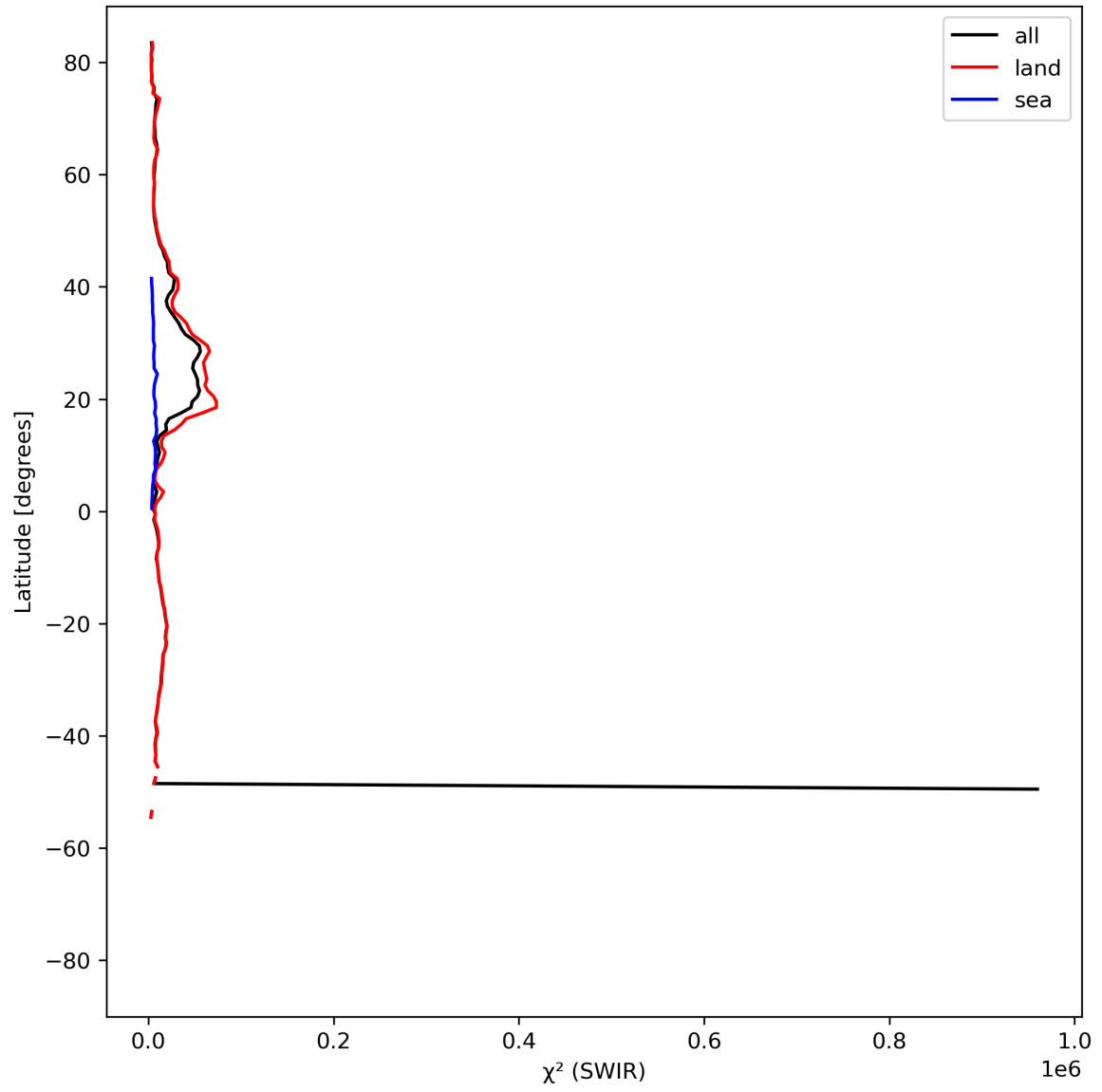
Figure 17: Zonal average of “ \chi^2 (SWIR)” for 2024-08-11 to 2024-08-11.
