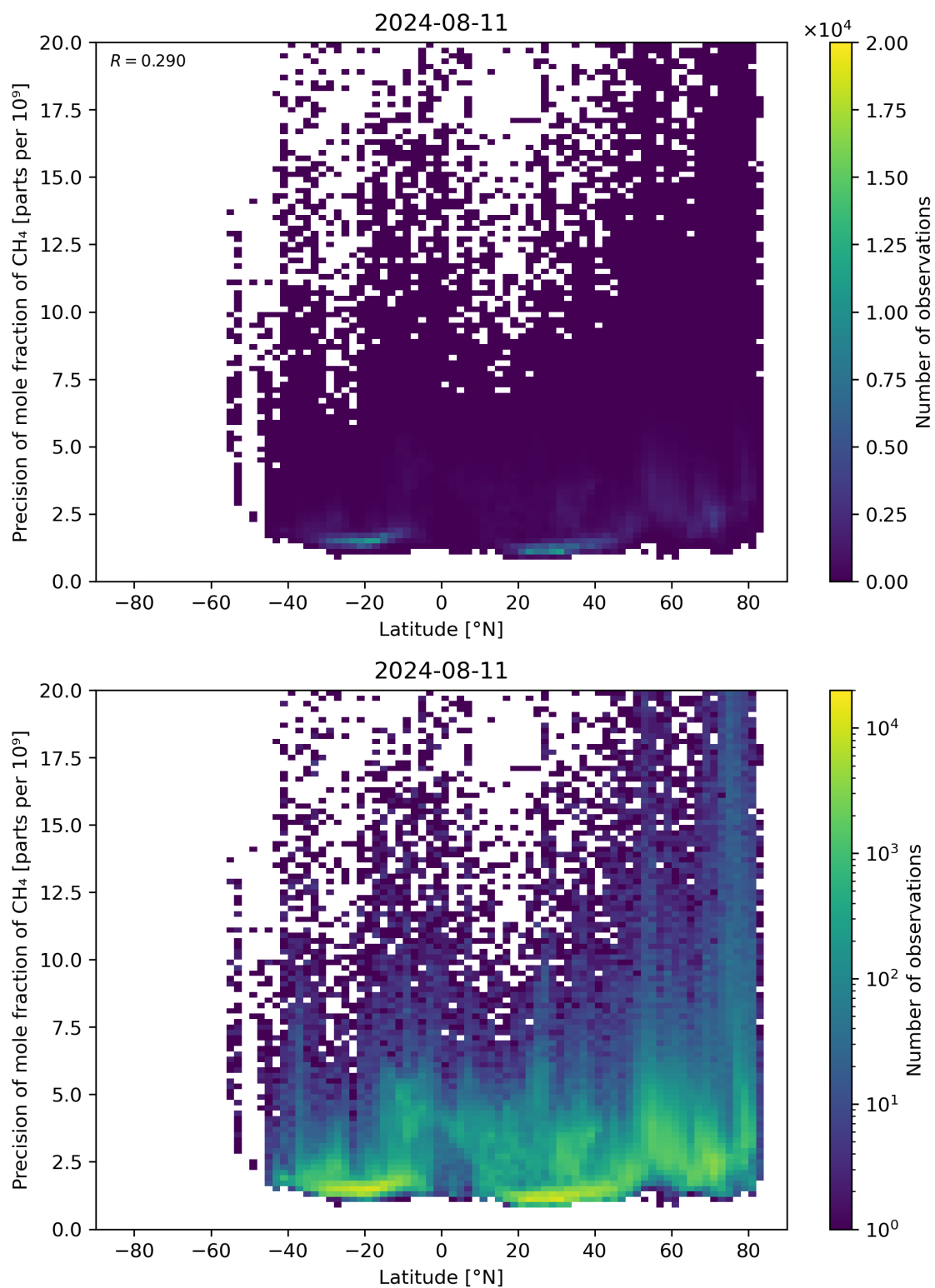
Figure 59: Scatter density plot of “Latitude” against “Precision of mole fraction of \text{CH}_4 ” for 2024-08-11 to 2024-08-11.
