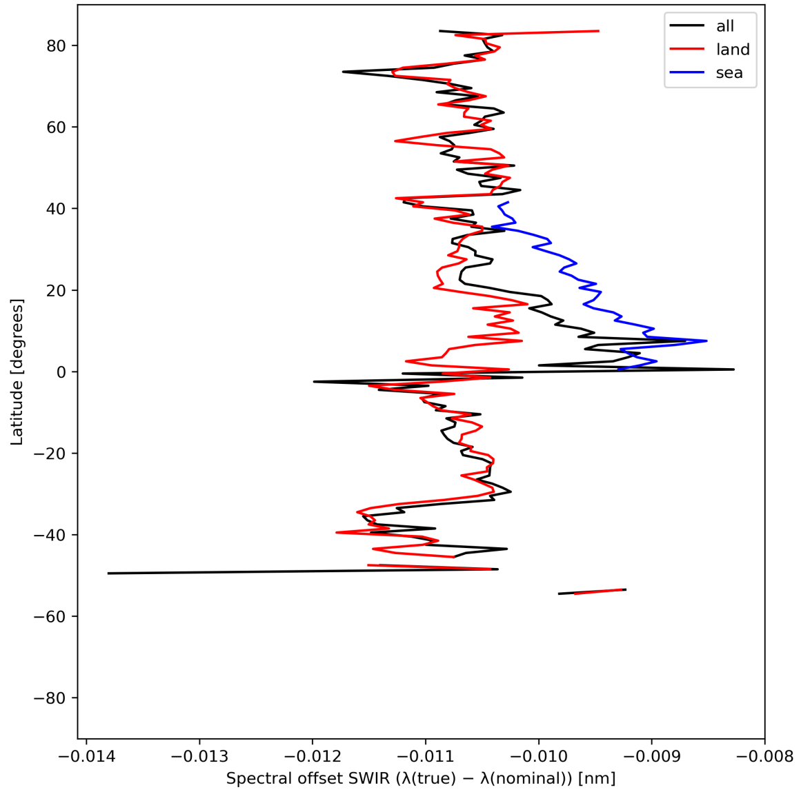
Figure 16: Zonal average of “Spectral offset SWIR ( \lambda(\text{true}) - \lambda(\text{nominal}) )” for 2024-08-11 to 2024-08-11.
