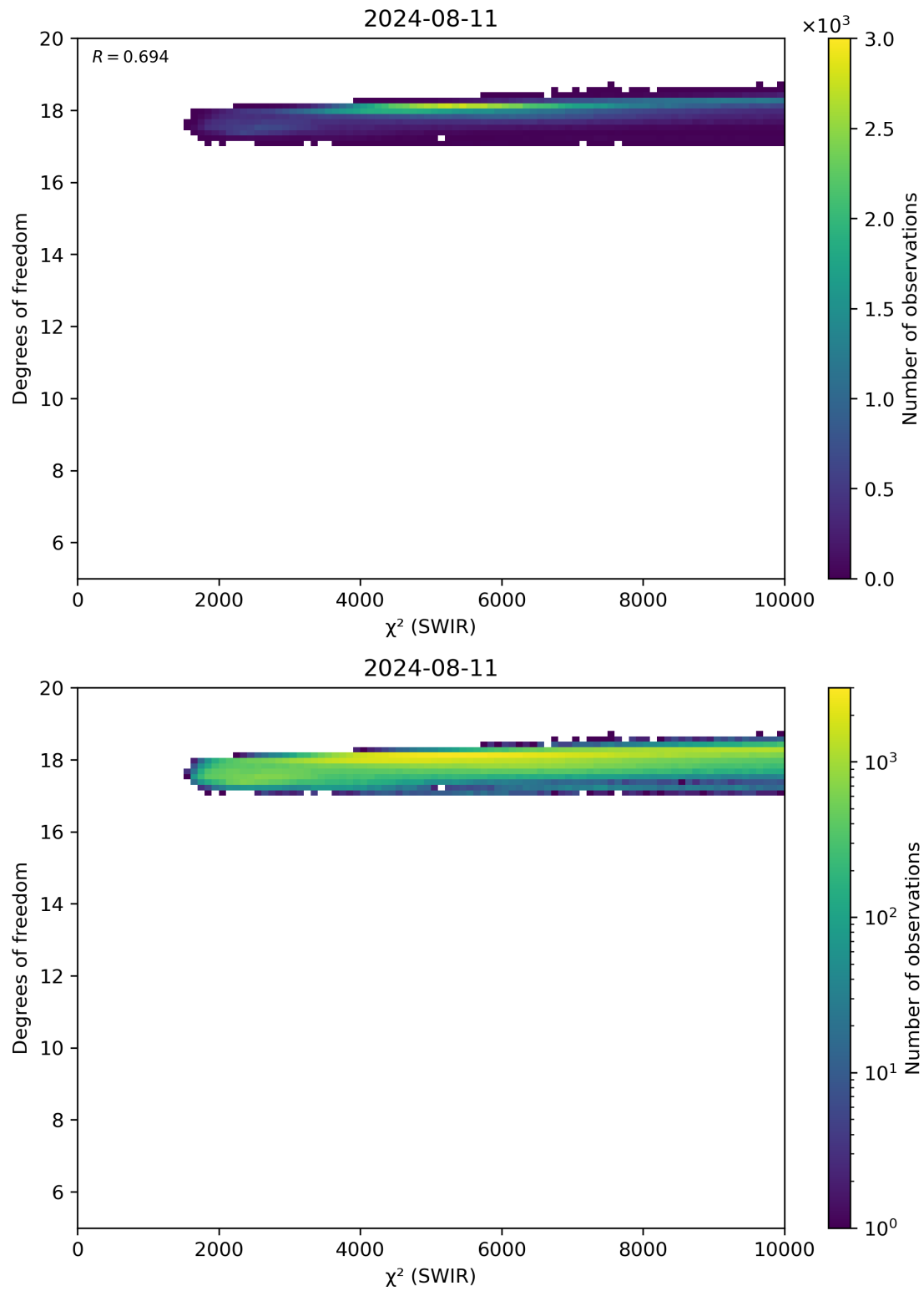
Figure 48: Scatter density plot of “ \chi^2 (SWIR)” against “Degrees of freedom” for 2024-08-11 to 2024-08-11.
