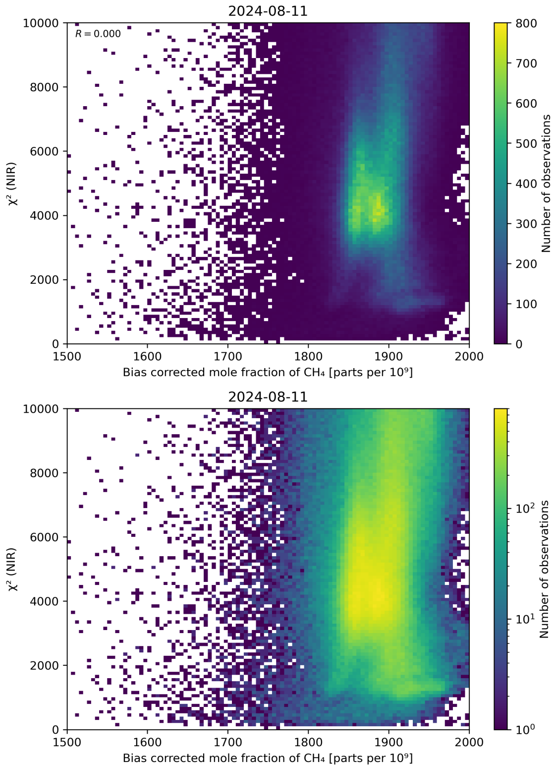
Figure 63: Scatter density plot of “Bias corrected mole fraction of CH 4 ” against “ \chi^2 (NIR)” for 2024-08-11 to 2024-08-11.
