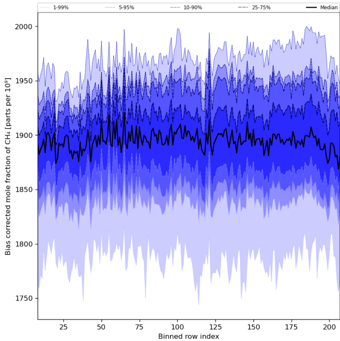
Figure 36: Along track statistics of “Bias corrected mole fraction of CH 4 ” for 2024-08-11 to 2024-08-11
