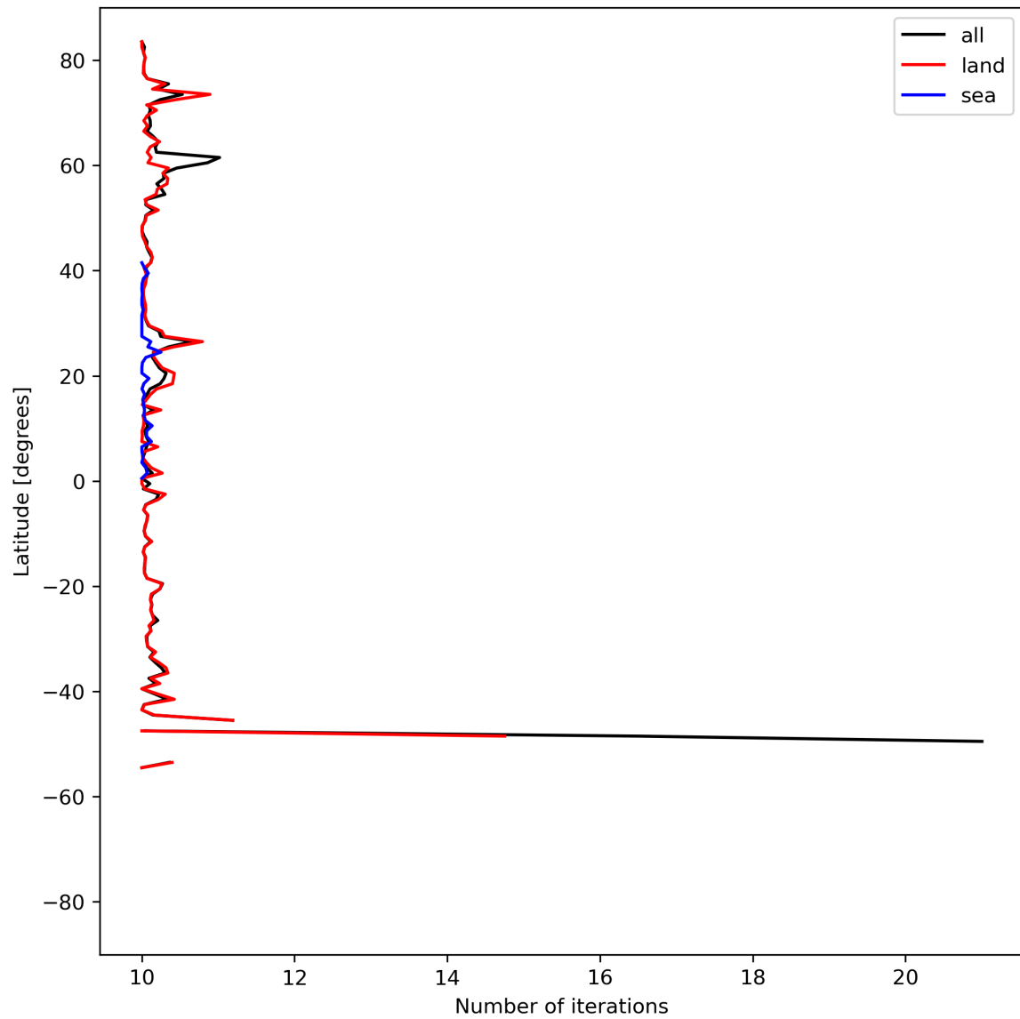
Figure 20: Zonal average of “Number of iterations” for 2024-08-11 to 2024-08-11.
