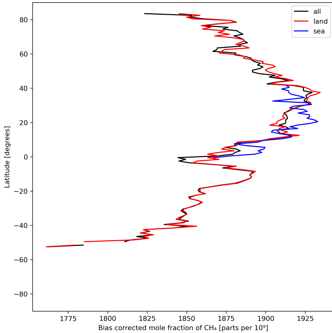
Figure 14: Zonal average of “Bias corrected mole fraction of CH 4 ” for 2024-08-12 to 2024-08-13.
