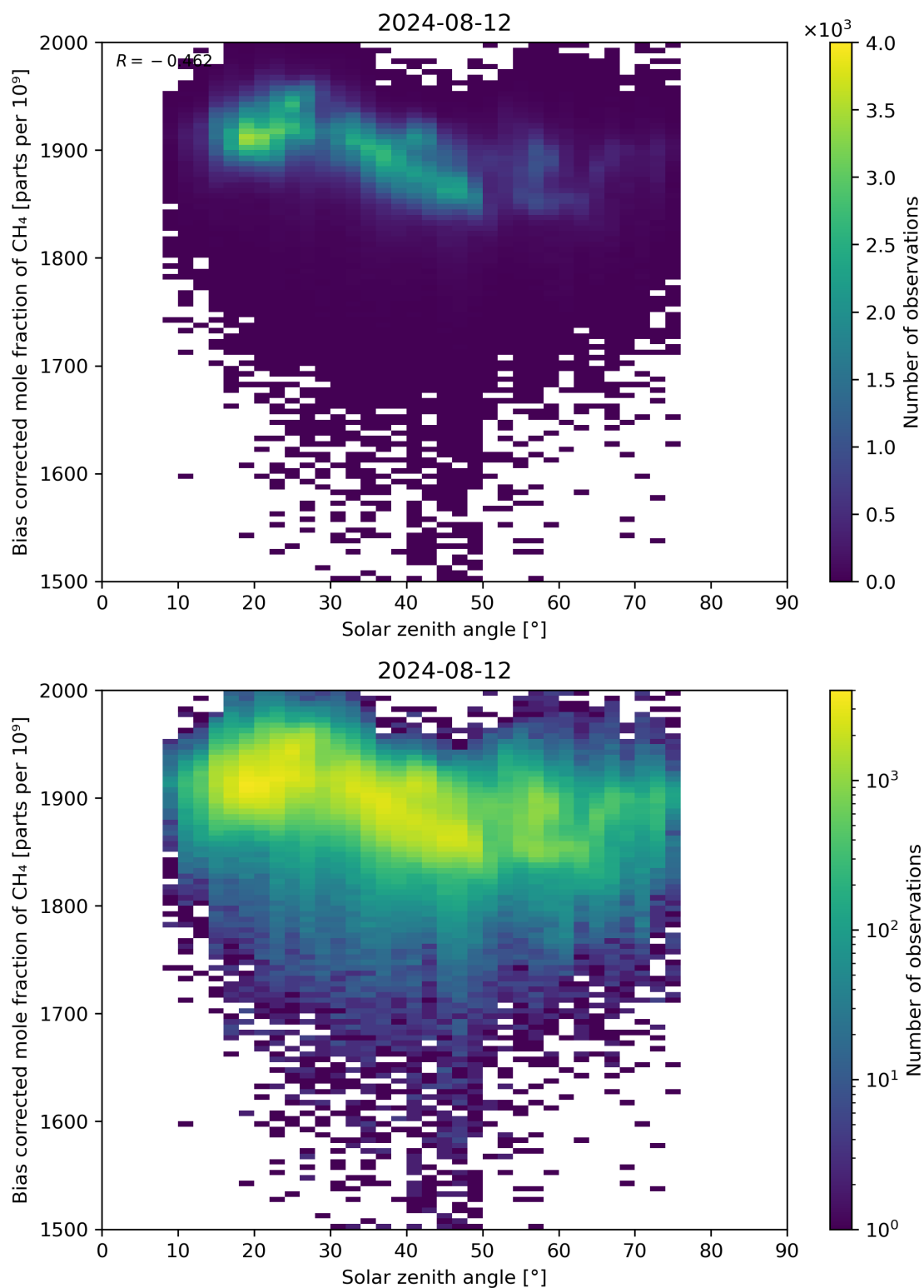
Figure 100: Scatter density plot of “Solar zenith angle” against “Bias corrected mole fraction of CH 4 ” for 2024-08-12 to 2024-08-13.
