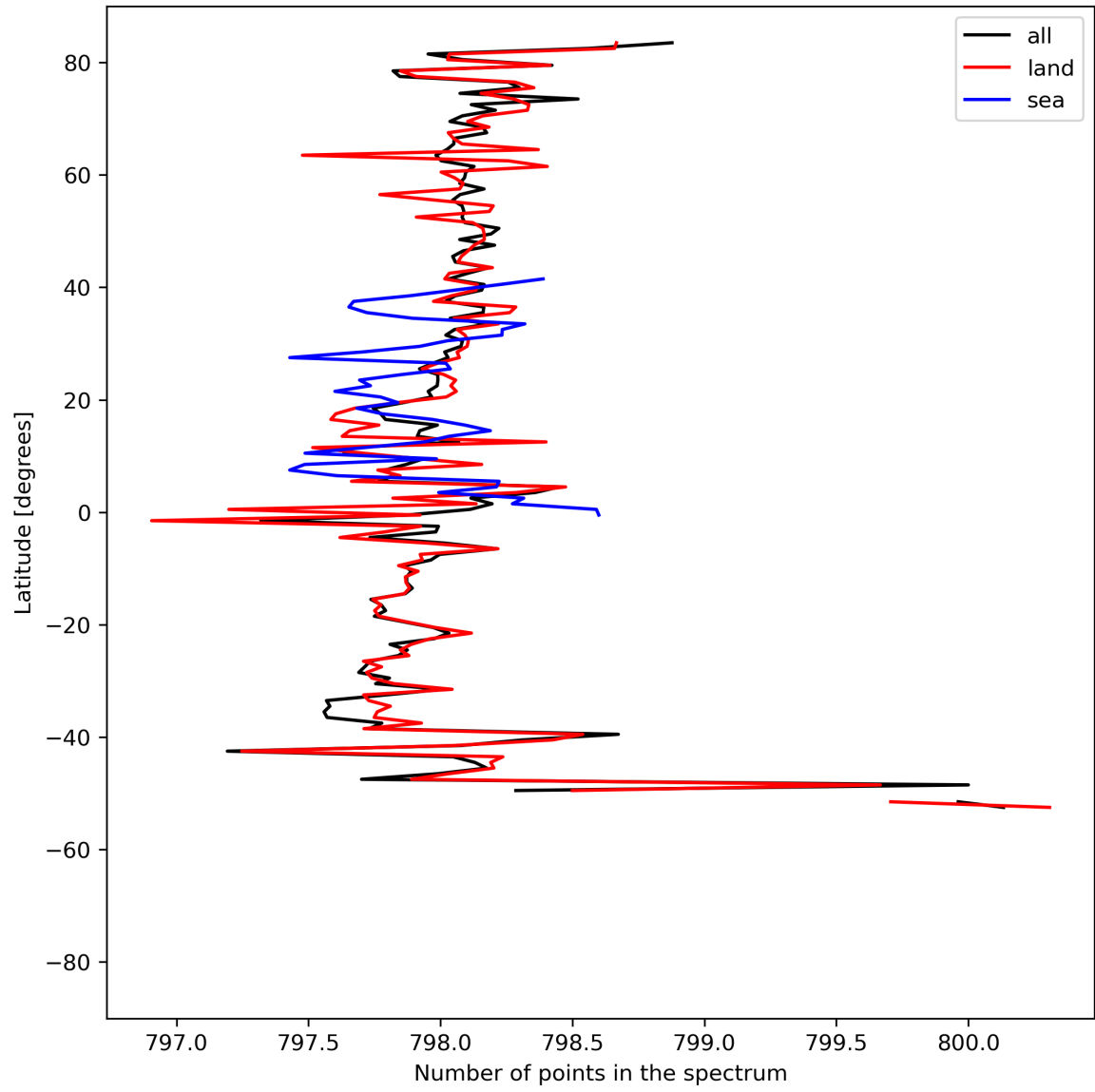
Figure 15: Zonal average of “Number of points in the spectrum” for 2024-08-12 to 2024-08-13.
