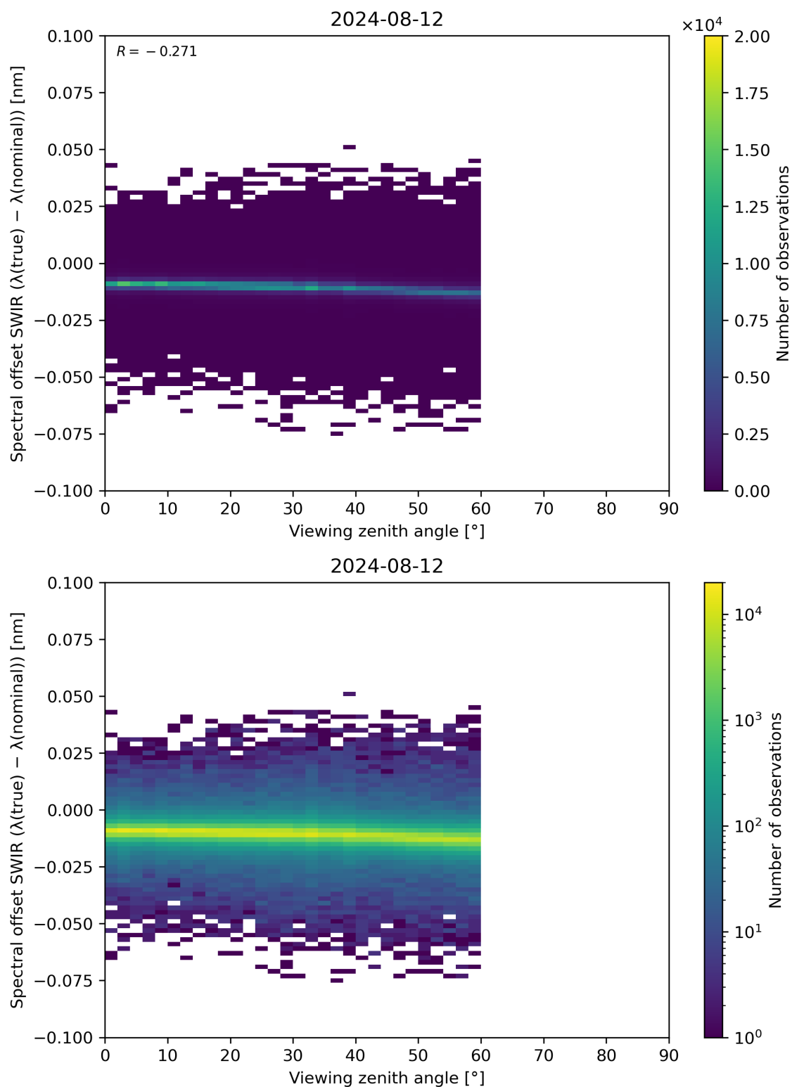
Figure 116: Scatter density plot of “Viewing zenith angle” against “Spectral offset SWIR ( \lambda(\text{true}) - \lambda(\text{nominal}) )” for 2024-08-12 to 2024-08-13.
