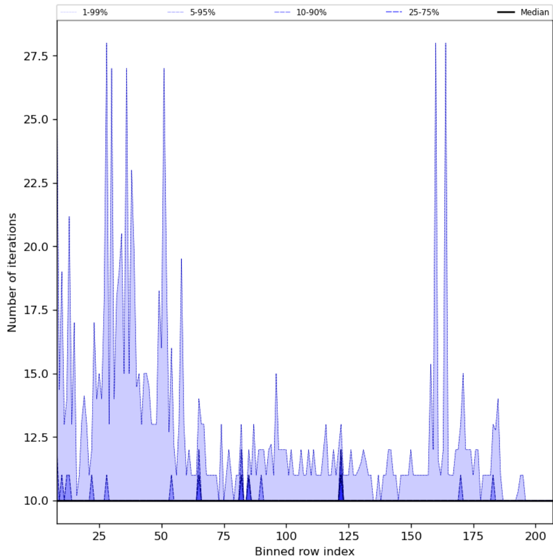
Figure 42: Along track statistics of “Number of iterations” for 2024-08-12 to 2024-08-13
