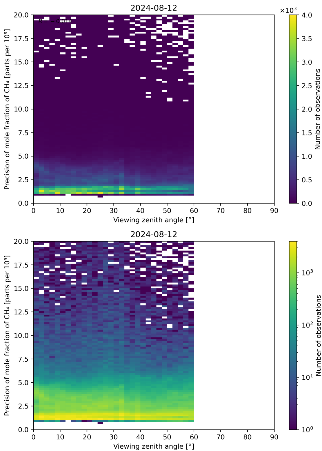
Figure 112: Scatter density plot of “Viewing zenith angle” against “Precision of mole fraction of CH 4 ” for 2024-08-12 to 2024-08-13.
