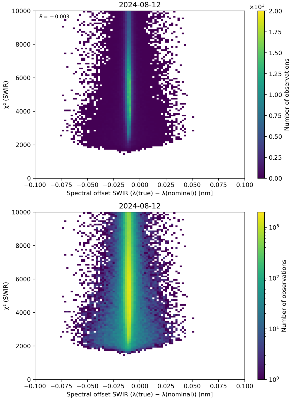
Figure 118: Scatter density plot of “Spectral offset SWIR ( \lambda(\text{true}) - \lambda(\text{nominal}) )” against “ \chi^2 (SWIR)” for 2024-08-12 to 2024-08-13.
