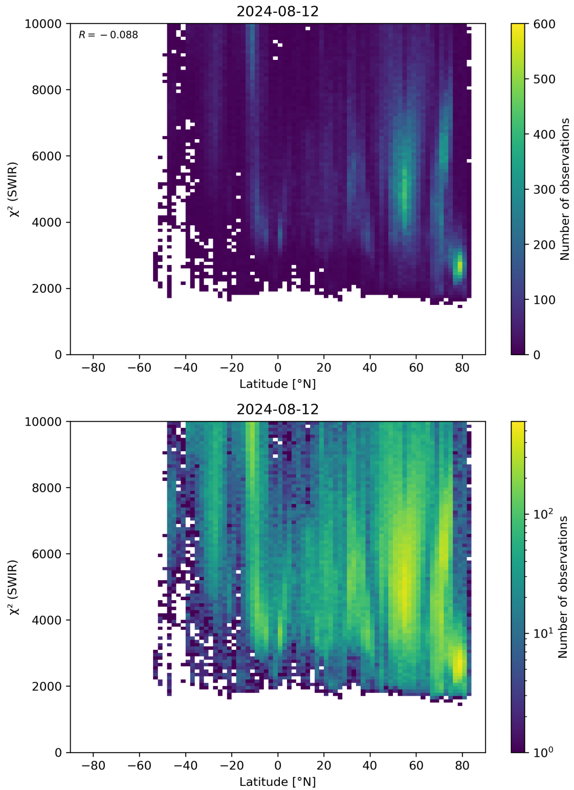
Figure 54: Scatter density plot of “Latitude” against “ \chi^2 (SWIR)” for 2024-08-12 to 2024-08-13.
