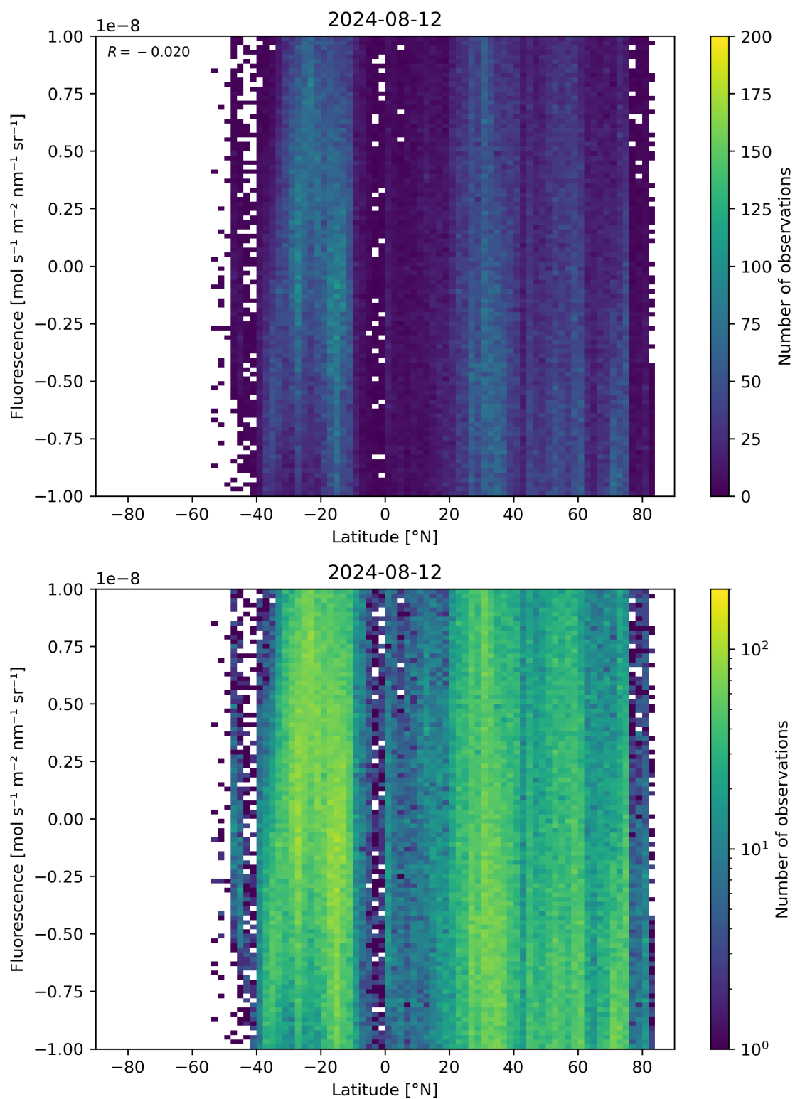
Figure 56: Scatter density plot of “Latitude” against “Fluorescence” for 2024-08-12 to 2024-08-13.
