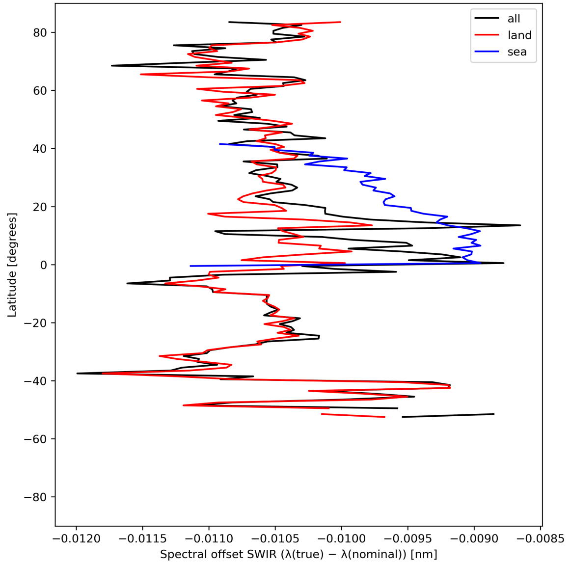
Figure 16: Zonal average of “Spectral offset SWIR ( \lambda(\text{true}) - \lambda(\text{nominal}) )” for 2024-08-12 to 2024-08-13.
