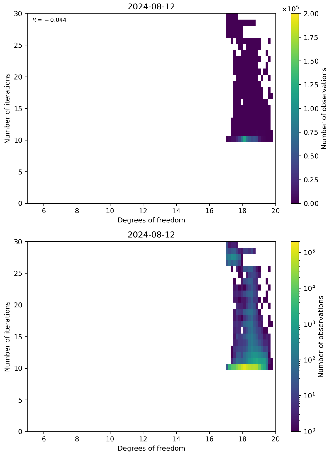
Figure 52: Scatter density plot of “Degrees of freedom” against “Number of iterations” for 2024-08-12 to 2024-08-13.
