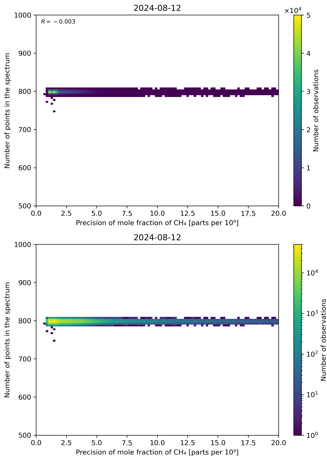
Figure 84: Scatter density plot of “Precision of mole fraction of CH 4 ” against “Number of points in the spectrum” for 2024-08-12 to 2024-08-13.
