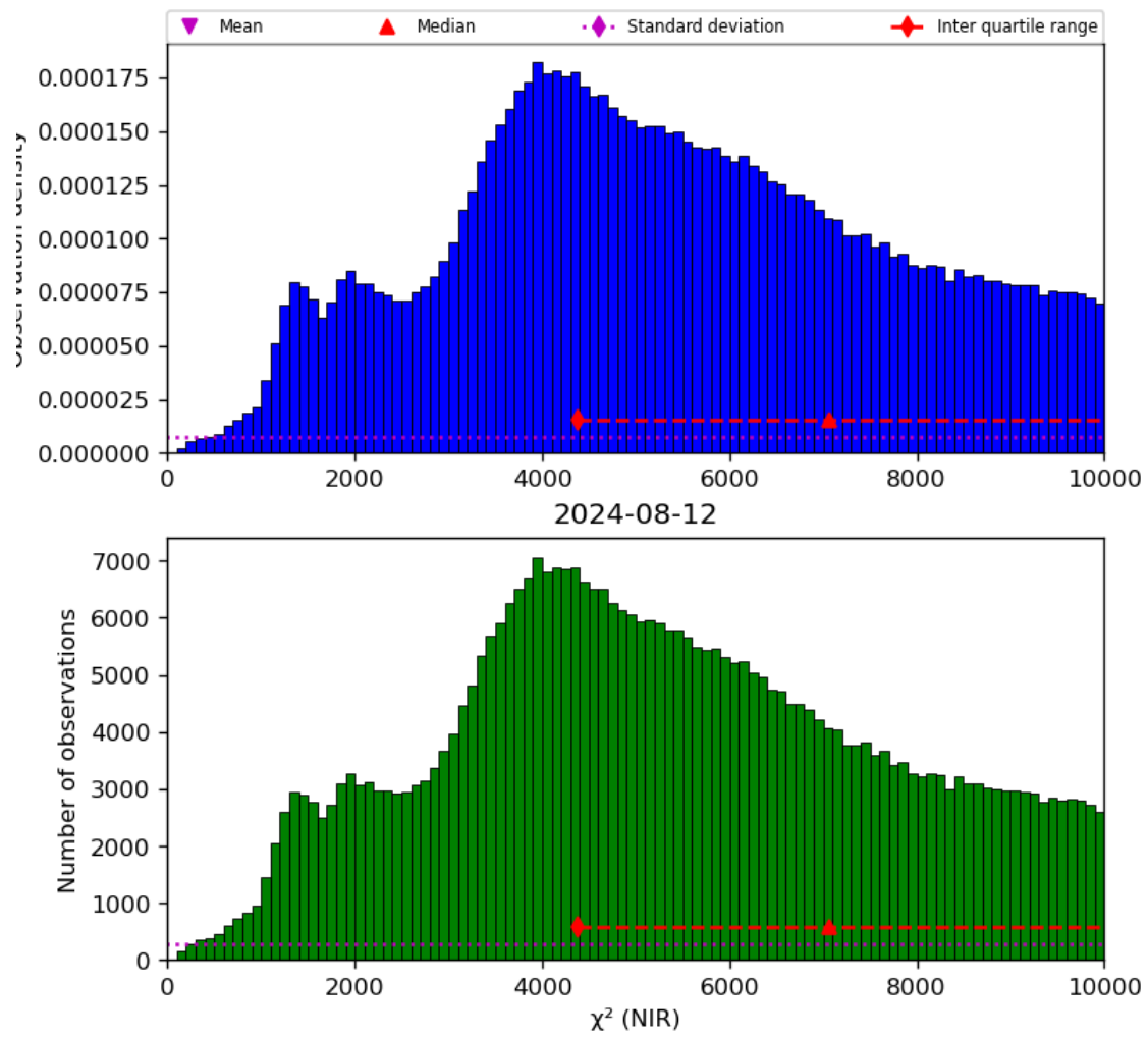
Figure 29: Histogram of “ \chi^2 (NIR)” for 2024-08-12 to 2024-08-13
