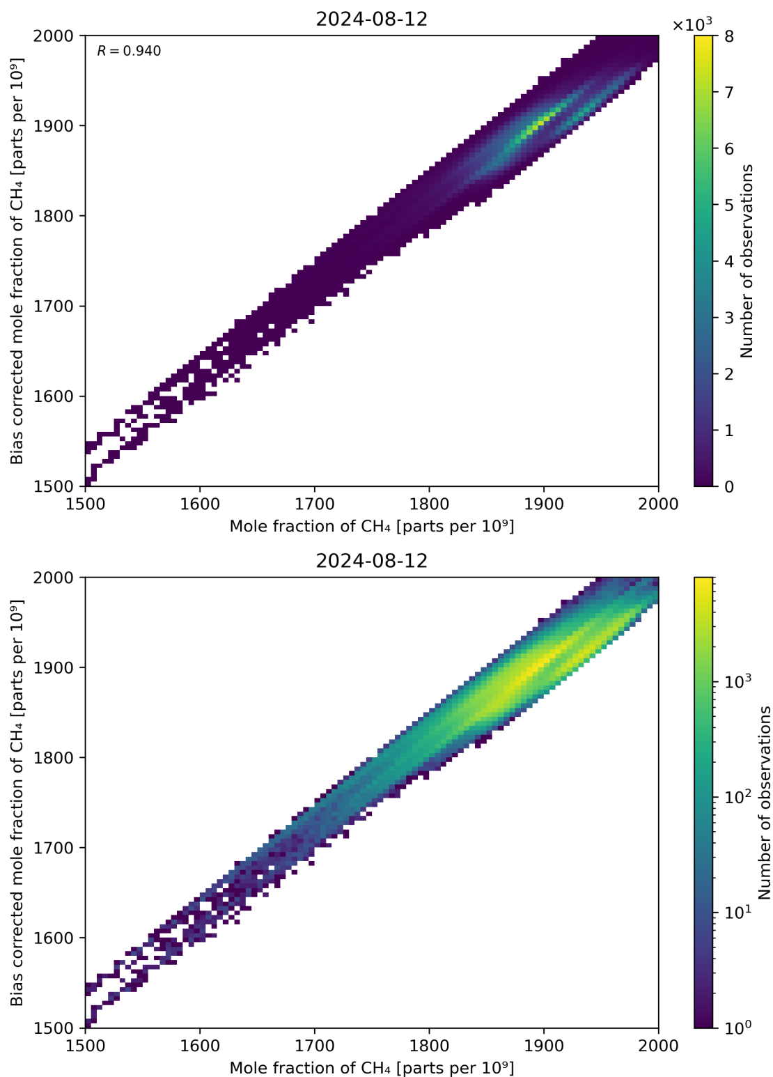
Figure 74: Scatter density plot of “Mole fraction of CH 4 ” against “Bias corrected mole fraction of CH 4 ” for 2024-08-12 to 2024-08-13.
