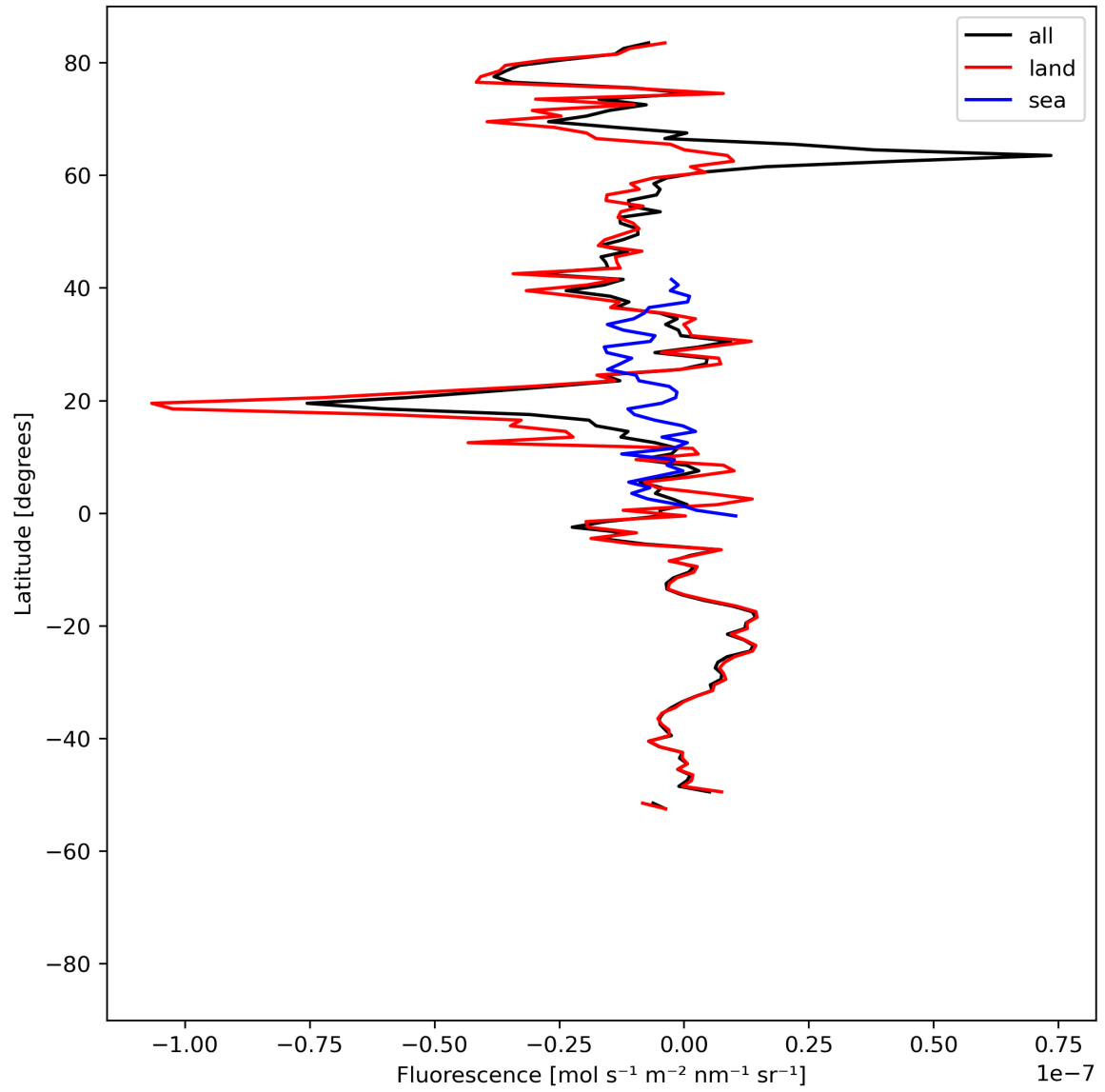
Figure 21: Zonal average of “Fluorescence” for 2024-08-12 to 2024-08-13.
