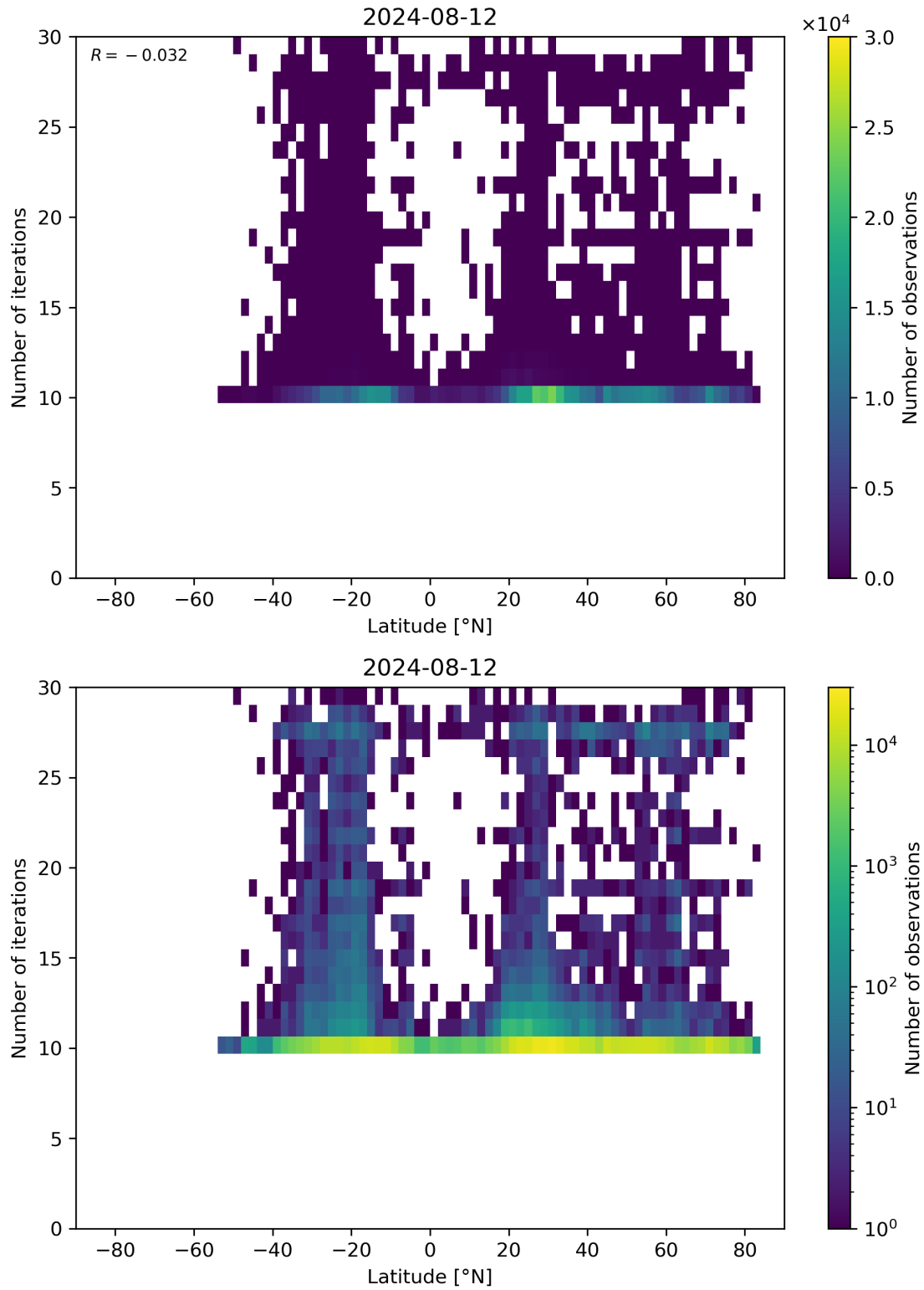
Figure 60: Scatter density plot of “Latitude” against “Number of iterations” for 2024-08-12 to 2024-08-13.
