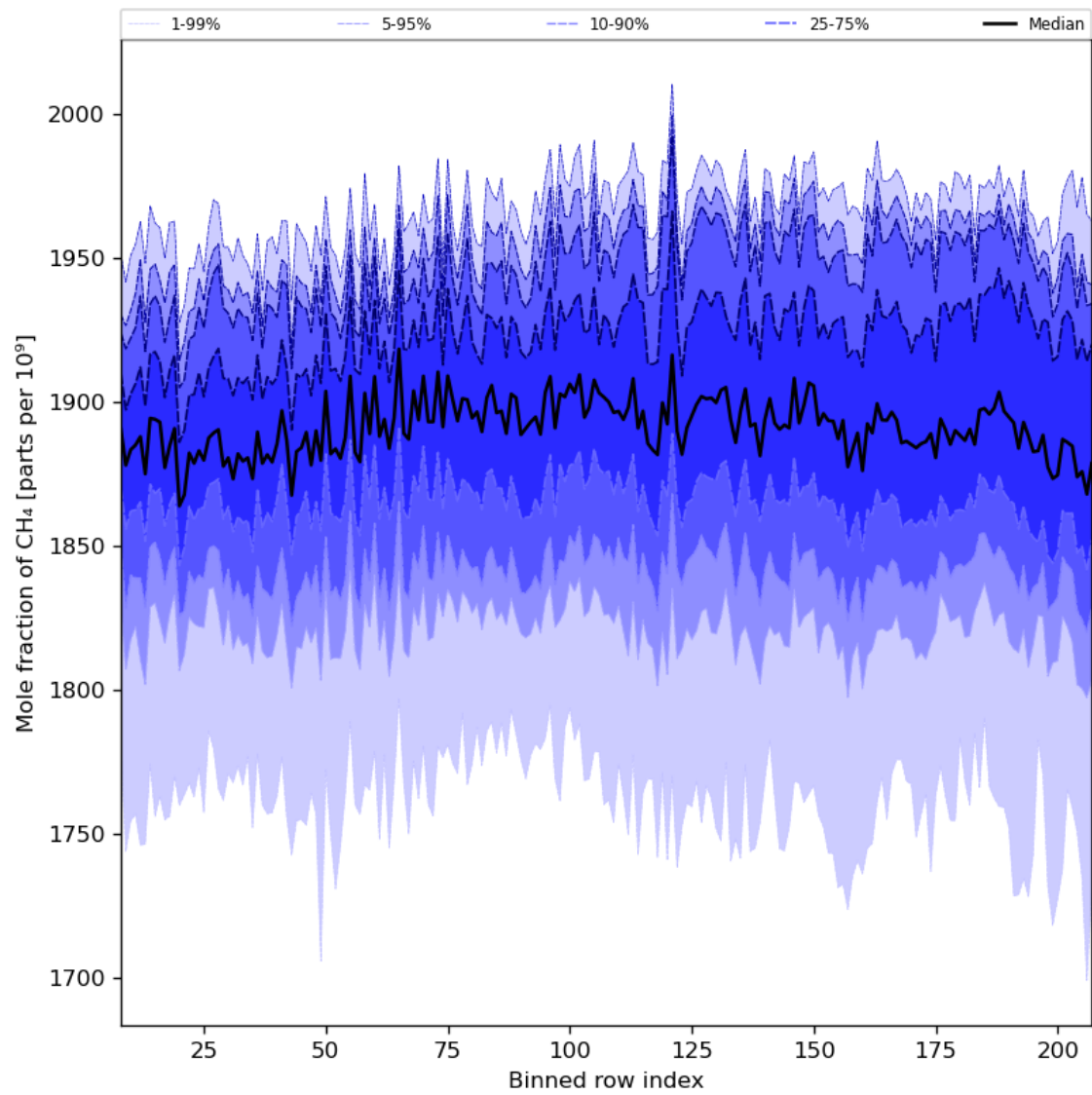
Figure 34: Along track statistics of “Mole fraction of CH 4 ” for 2024-08-12 to 2024-08-13
