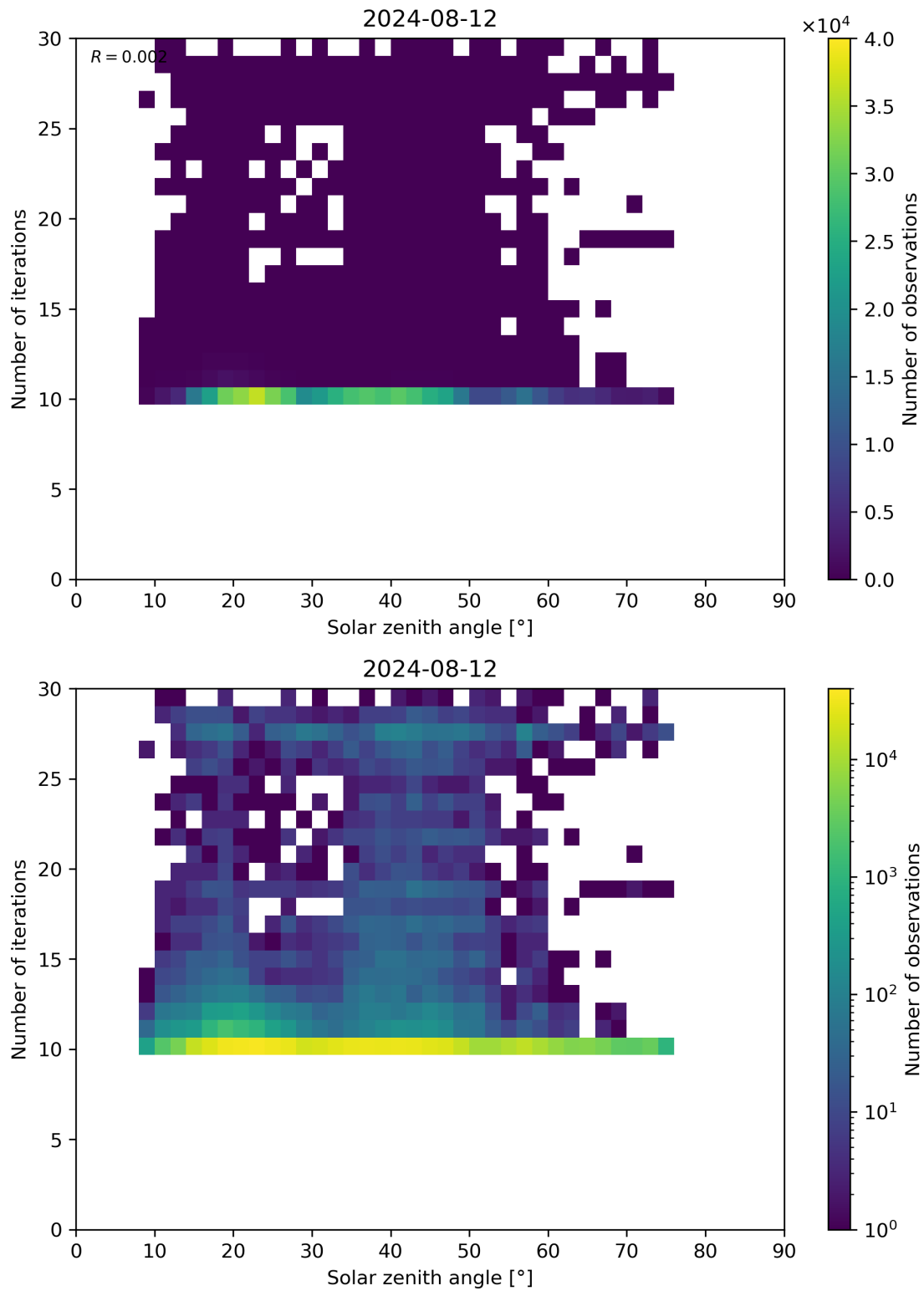
Figure 102: Scatter density plot of “Solar zenith angle” against “Number of iterations” for 2024-08-12 to 2024-08-13.
