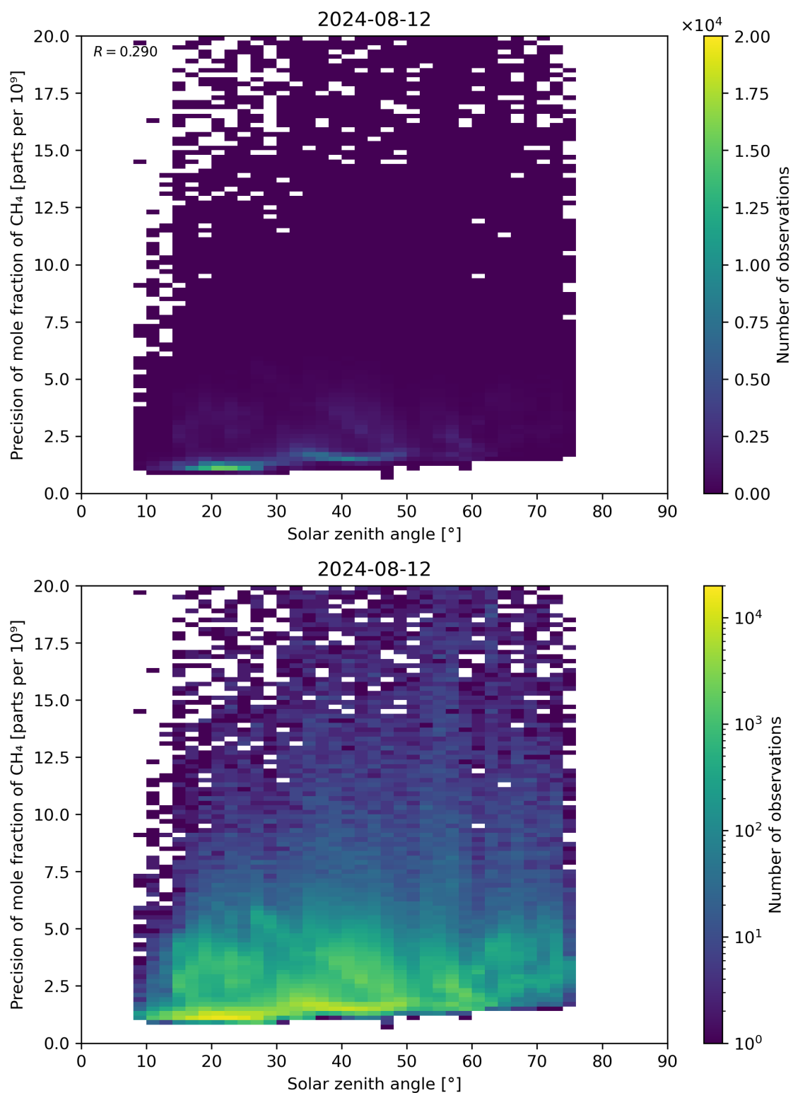
Figure 101: Scatter density plot of “Solar zenith angle” against “Precision of mole fraction of CH 4 ” for 2024-08-12 to 2024-08-13.
