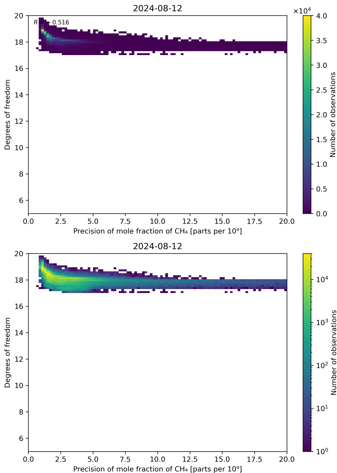
Figure 80: Scatter density plot of “Precision of mole fraction of CH 4 ” against “Degrees of freedom” for 2024-08-12 to 2024-08-13.
