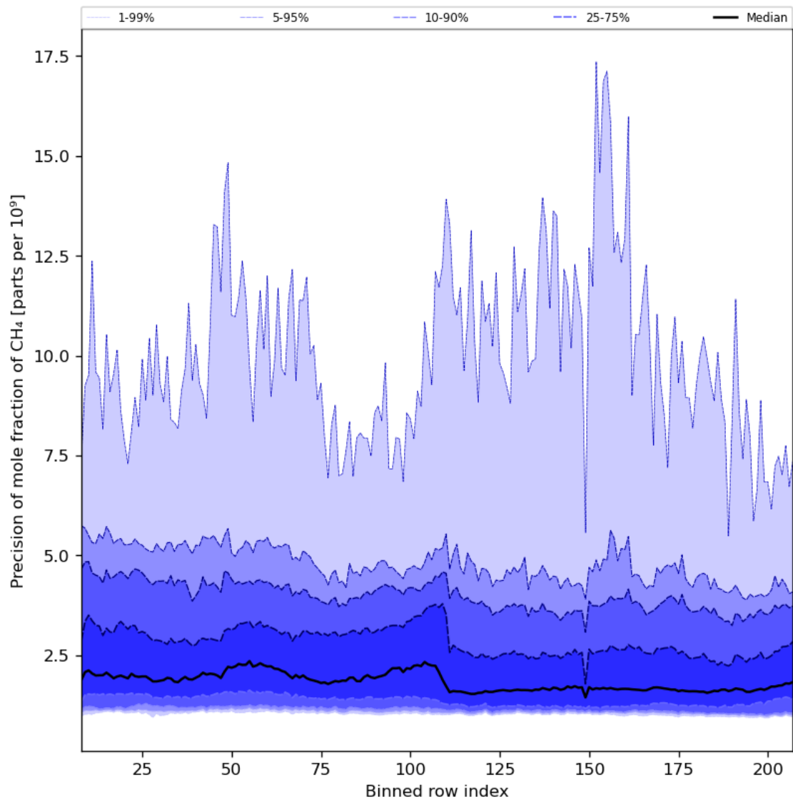
Figure 35: Along track statistics of “Precision of mole fraction of CH 4 ” for 2024-08-12 to 2024-08-13
