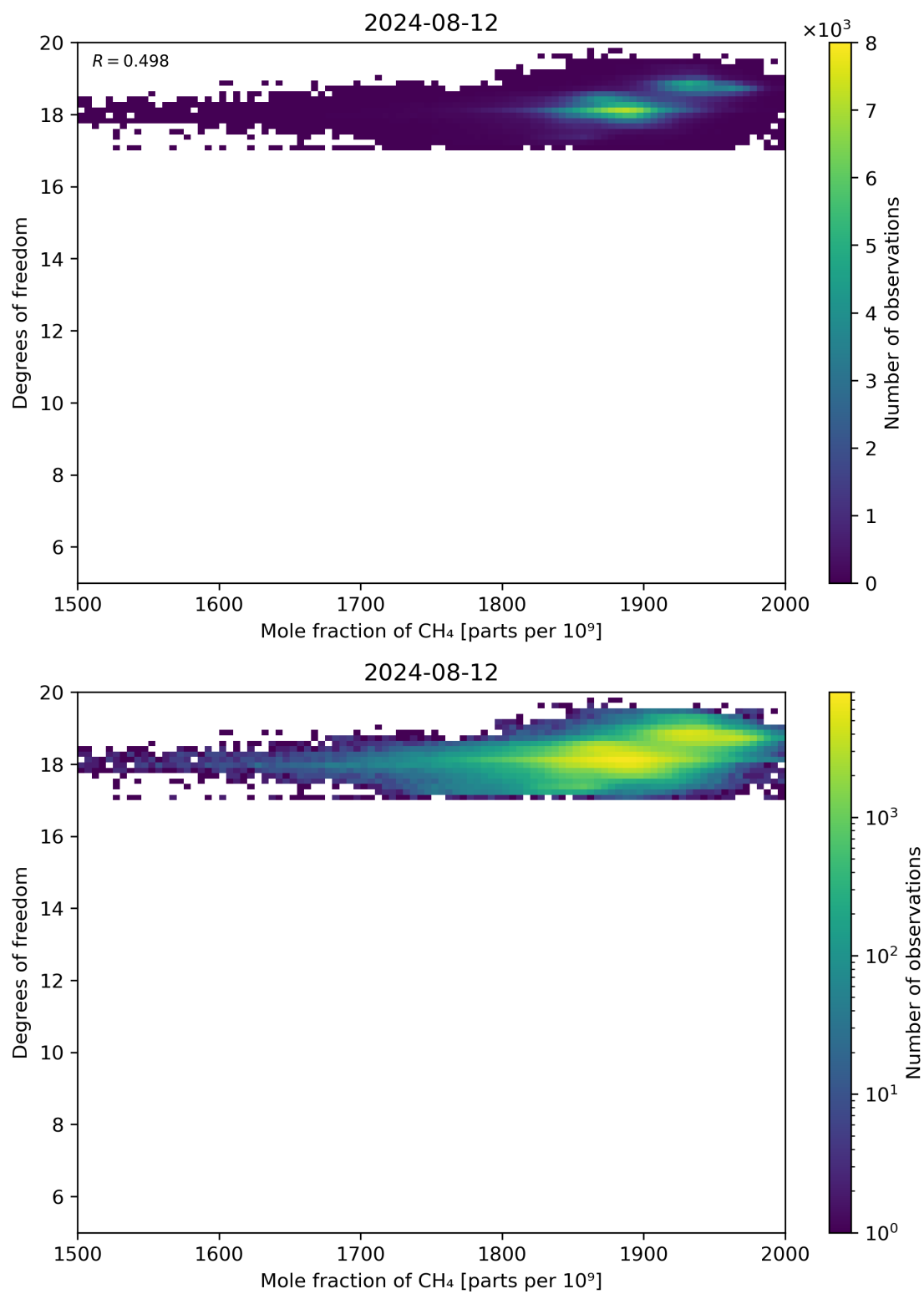
Figure 72: Scatter density plot of “Mole fraction of CH 4 ” against “Degrees of freedom” for 2024-08-12 to 2024-08-13.
