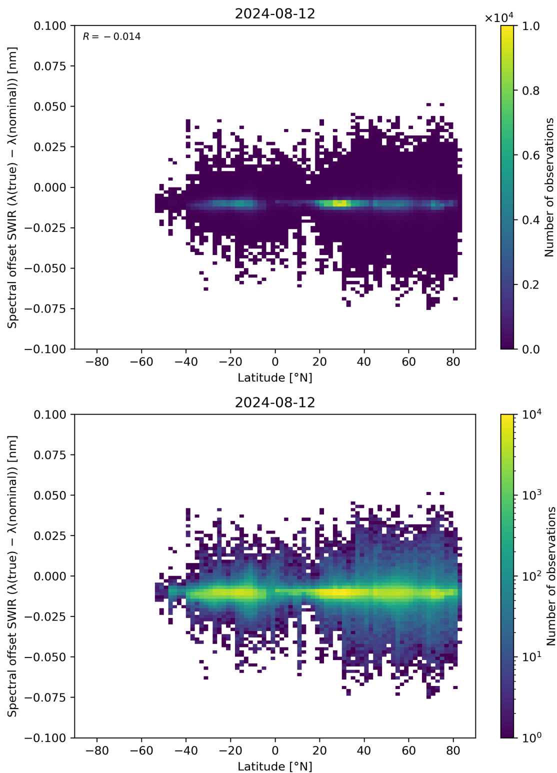
Figure 62: Scatter density plot of “Latitude” against “Spectral offset SWIR ( \lambda(\text{true}) - \lambda(\text{nominal}) )” for 2024-08-12 to 2024-08-13.
