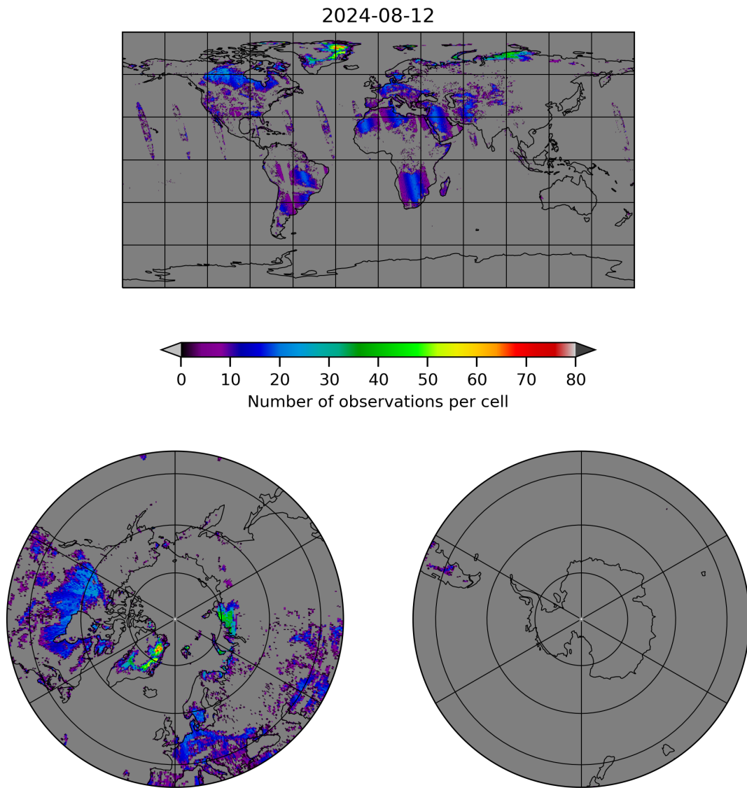
Figure 10: Map of the number of observations for 2024-08-12 to 2024-08-13
