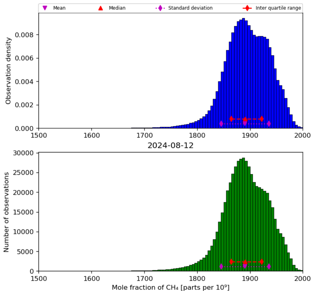
Figure 23: Histogram of “Mole fraction of CH 4 ” for 2024-08-12 to 2024-08-13
