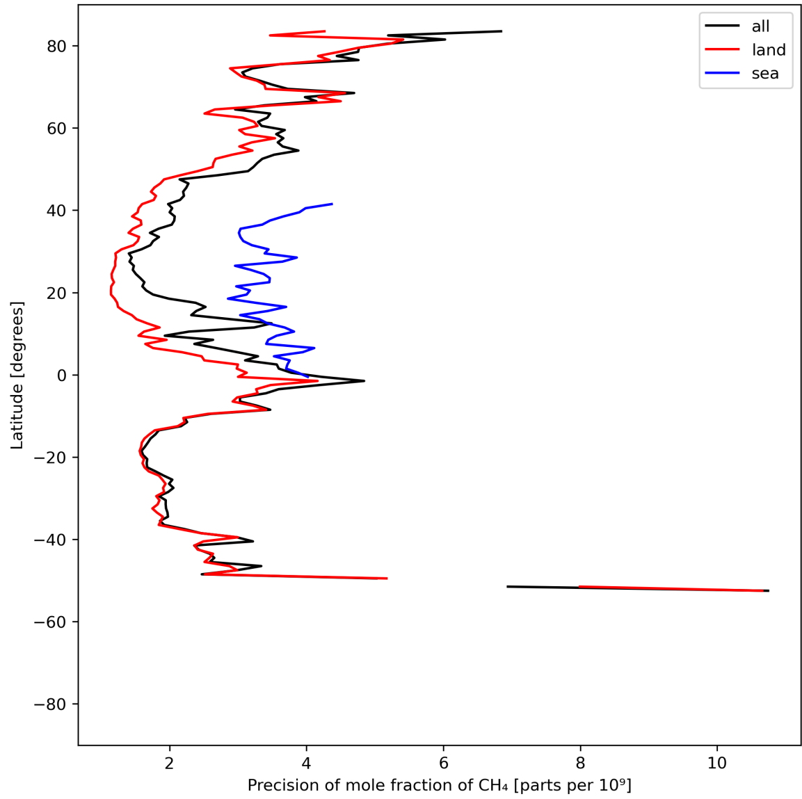
Figure 13: Zonal average of “Precision of mole fraction of CH 4 ” for 2024-08-12 to 2024-08-13.
