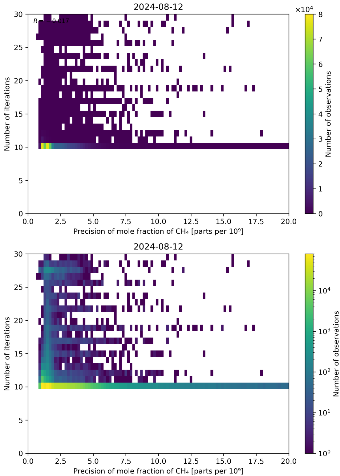
Figure 83: Scatter density plot of “Precision of mole fraction of CH 4 ” against “Number of iterations” for 2024-08-12 to 2024-08-13.
