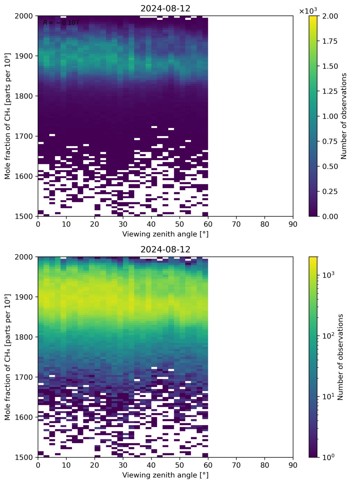
Figure 110: Scatter density plot of “Viewing zenith angle” against “Mole fraction of CH 4 ” for 2024-08-12 to 2024-08-13.
