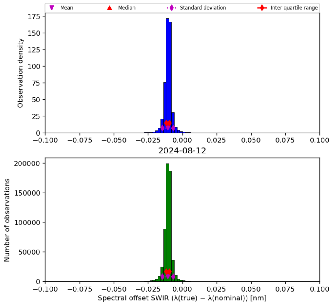
Figure 27: Histogram of “Spectral offset SWIR ( \lambda(\text{true}) - \lambda(\text{nominal}) )” for 2024-08-12 to 2024-08-13
