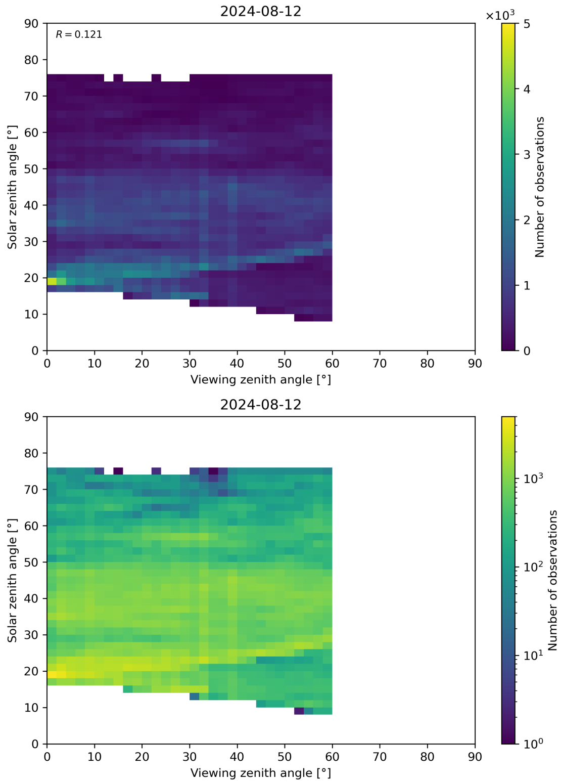
Figure 115: Scatter density plot of “Viewing zenith angle” against “Solar zenith angle” for 2024-08-12 to 2024-08-13.
