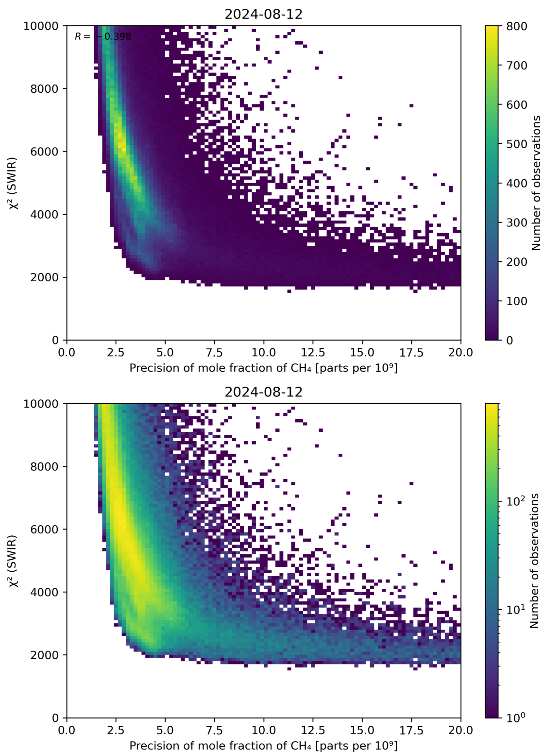
Figure 79: Scatter density plot of “Precision of mole fraction of CH 4 ” against “ \chi^2 (SWIR)” for 2024-08-12 to 2024-08-13.
