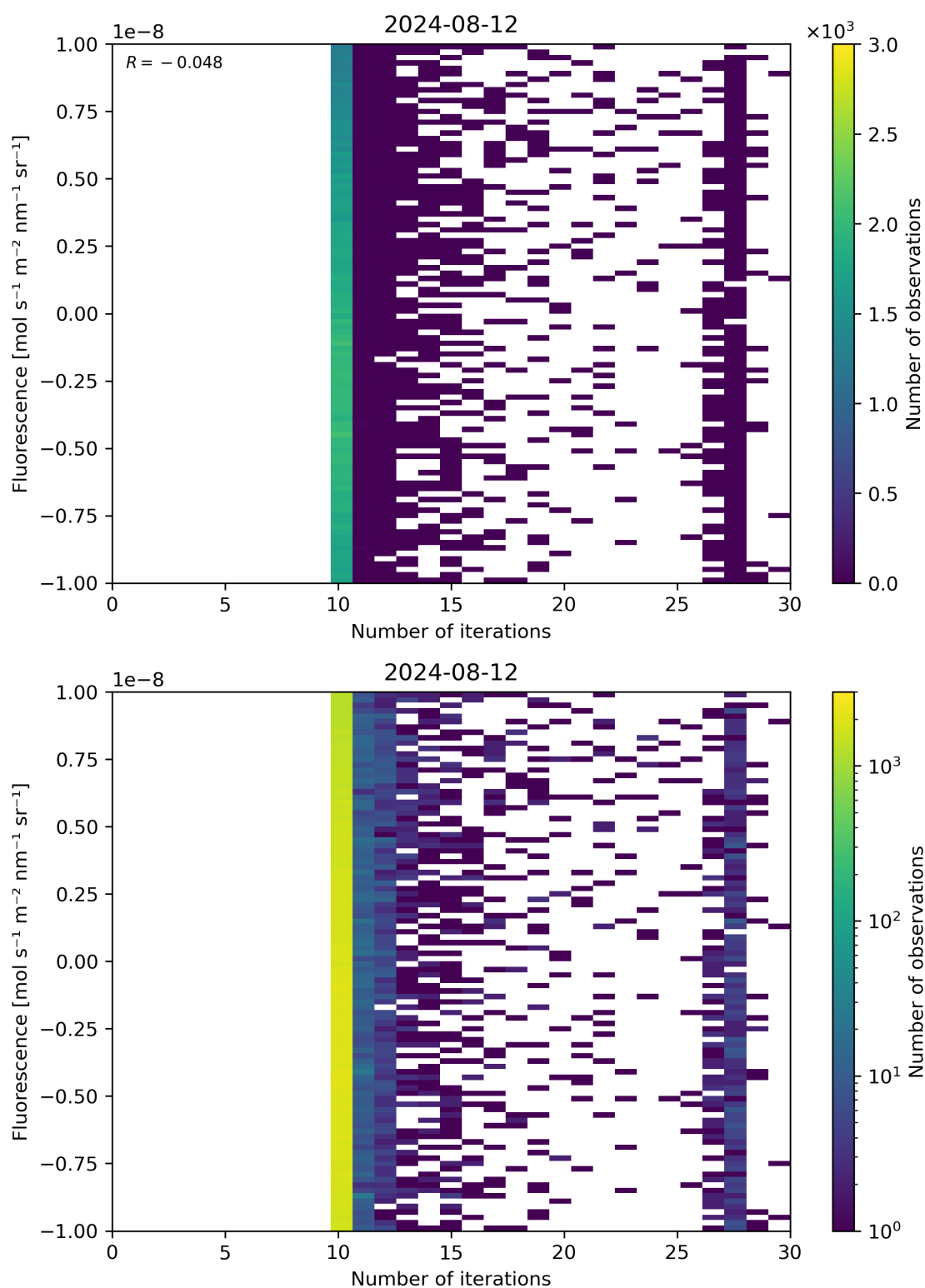
Figure 87: Scatter density plot of “Number of iterations” against “Fluorescence” for 2024-08-12 to 2024-08-13.
