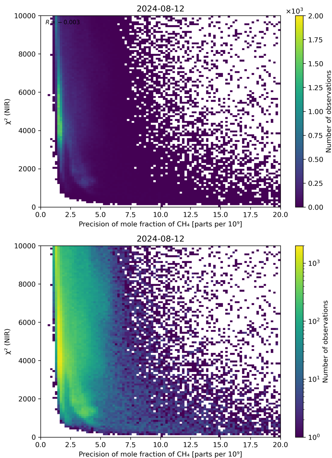
Figure 78: Scatter density plot of “Precision of mole fraction of CH 4 ” against “ \chi^2 (NIR)” for 2024-08-12 to 2024-08-13.
