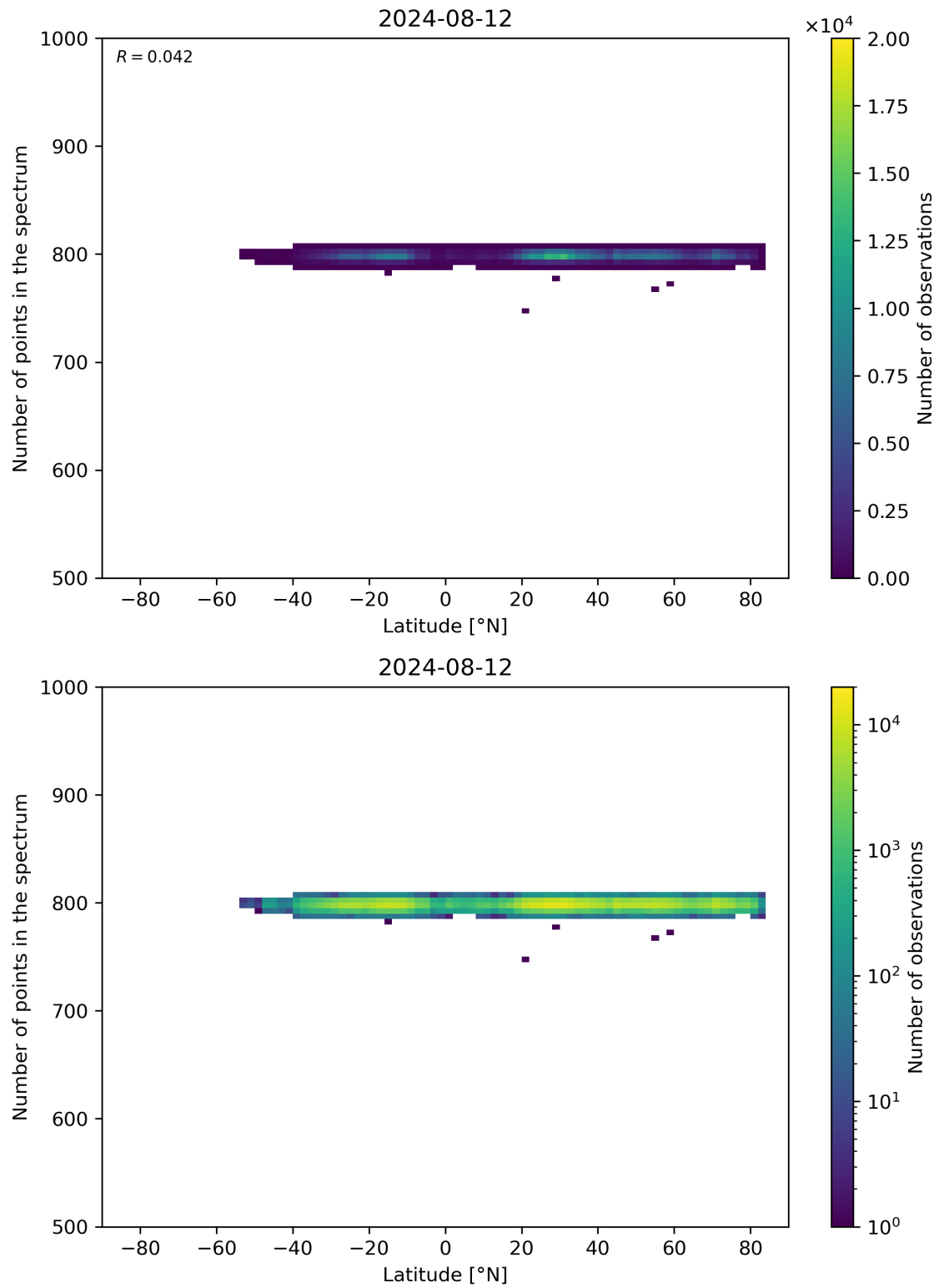
Figure 61: Scatter density plot of “Latitude” against “Number of points in the spectrum” for 2024-08-12 to 2024-08-13.
