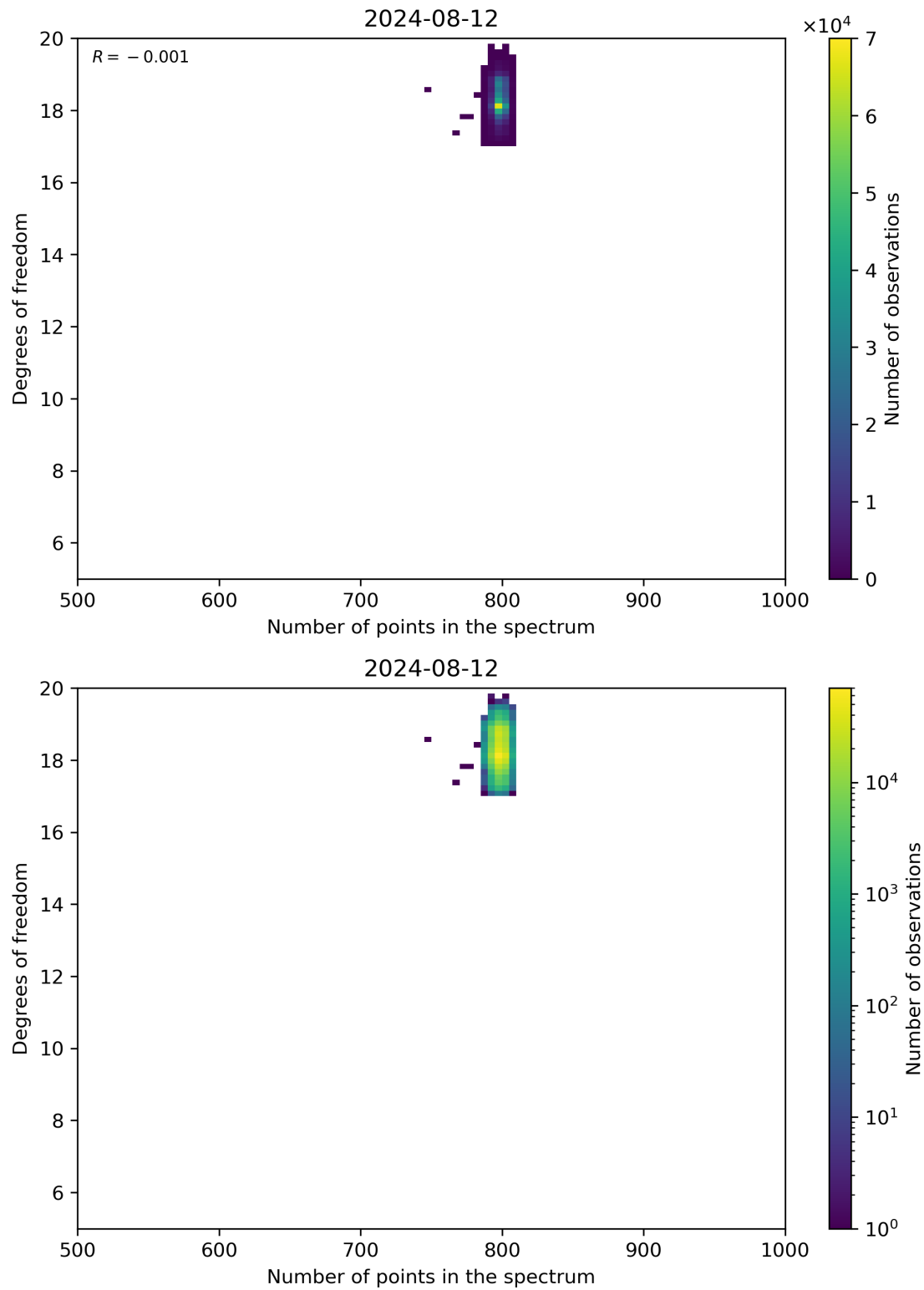
Figure 90: Scatter density plot of “Number of points in the spectrum” against “Degrees of freedom” for 2024-08-12 to 2024-08-13.
