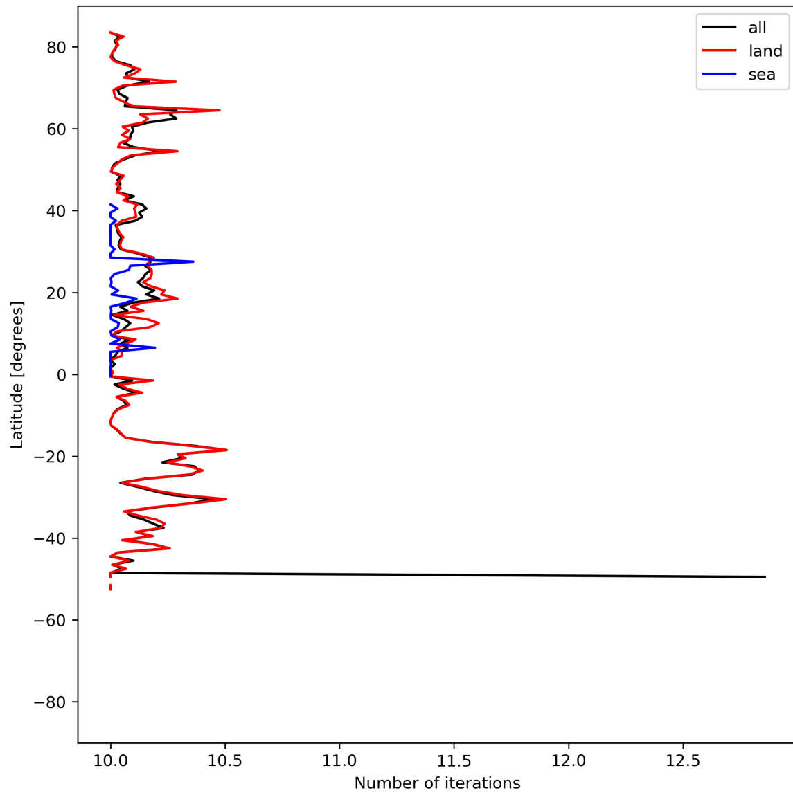
Figure 20: Zonal average of “Number of iterations” for 2024-08-12 to 2024-08-13.
