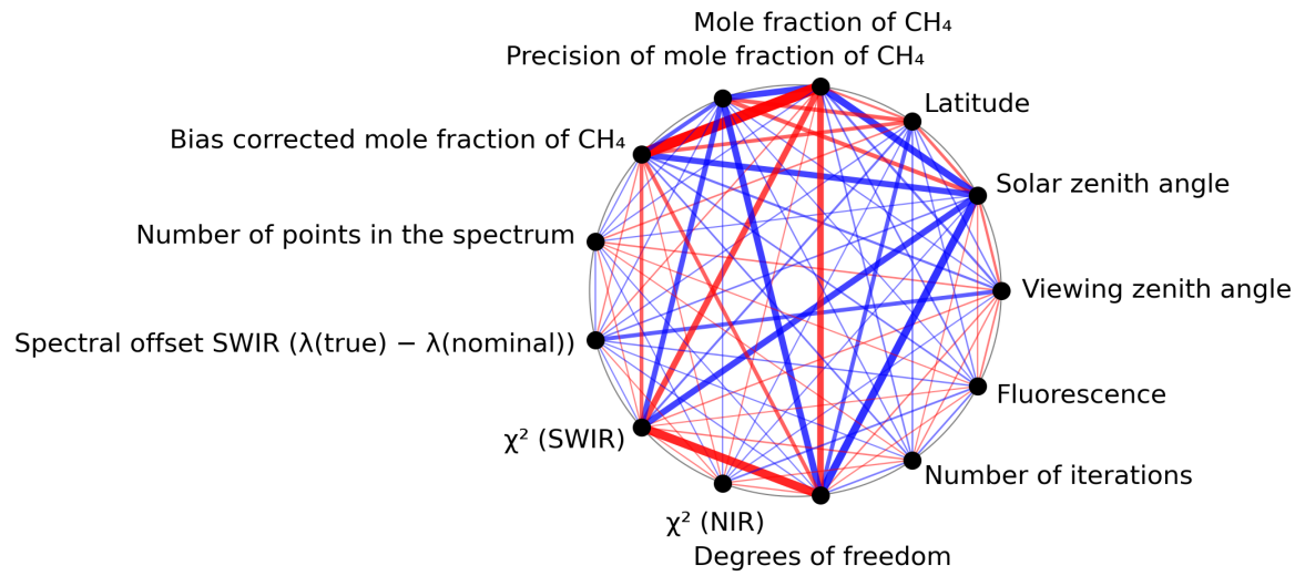
Figure 1: Map of correlation graph for 2024-08-12 to 2024-08-13.
