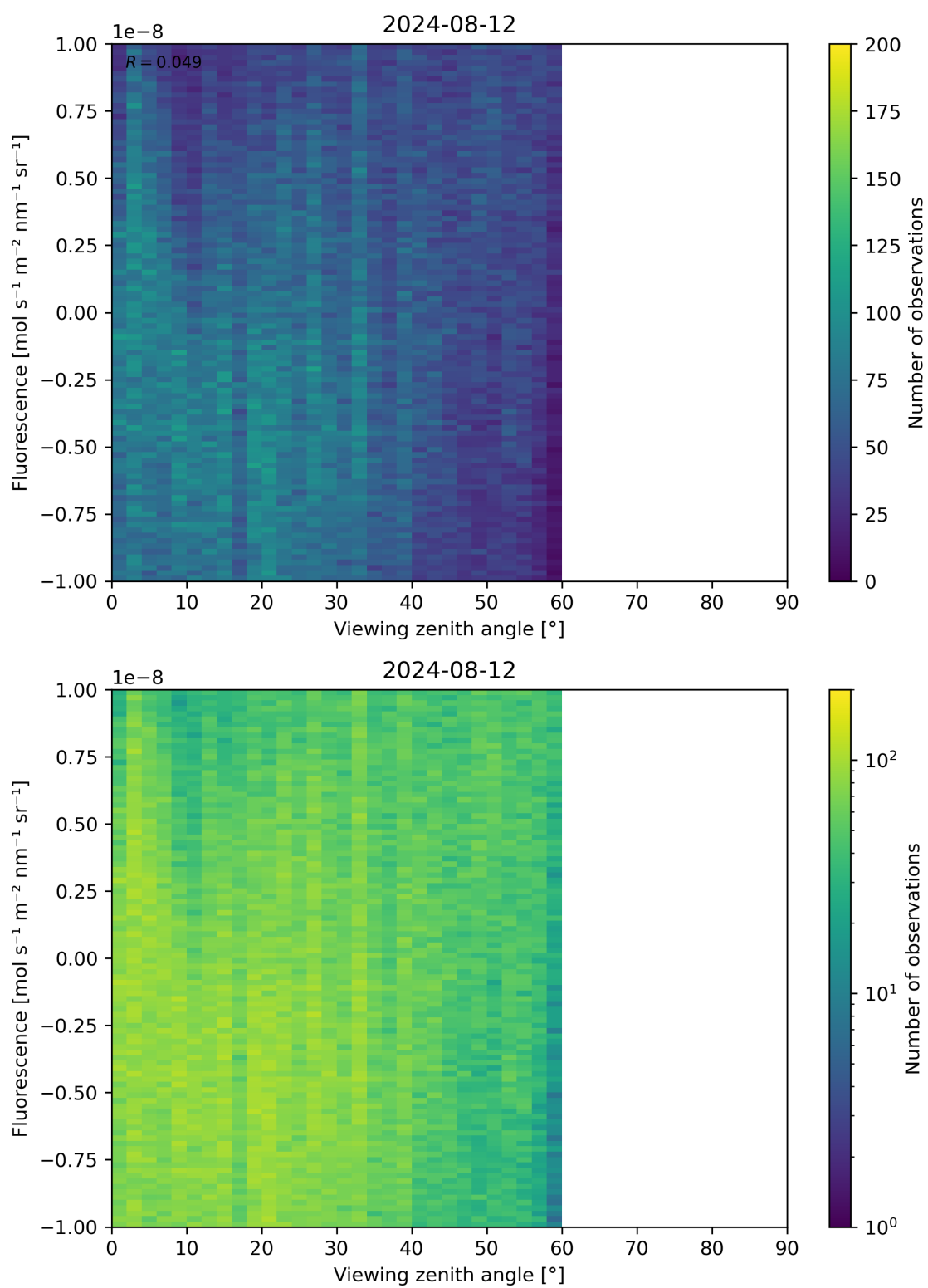
Figure 108: Scatter density plot of “Viewing zenith angle” against “Fluorescence” for 2024-08-12 to 2024-08-13.
