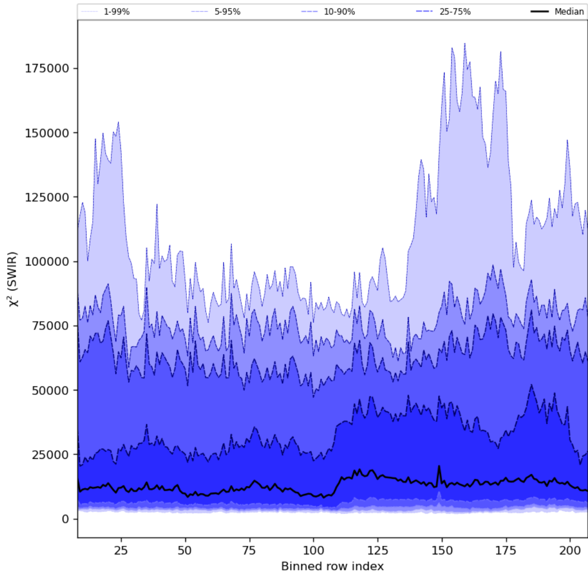
Figure 39: Along track statistics of “ \chi^2 (SWIR)” for 2024-08-12 to 2024-08-13
