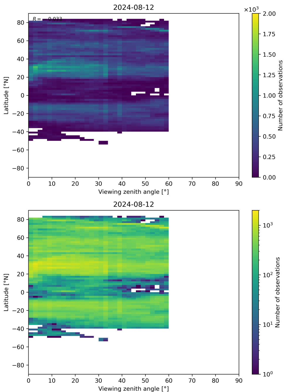
Figure 109: Scatter density plot of “Viewing zenith angle” against “Latitude” for 2024-08-12 to 2024-08-13.
