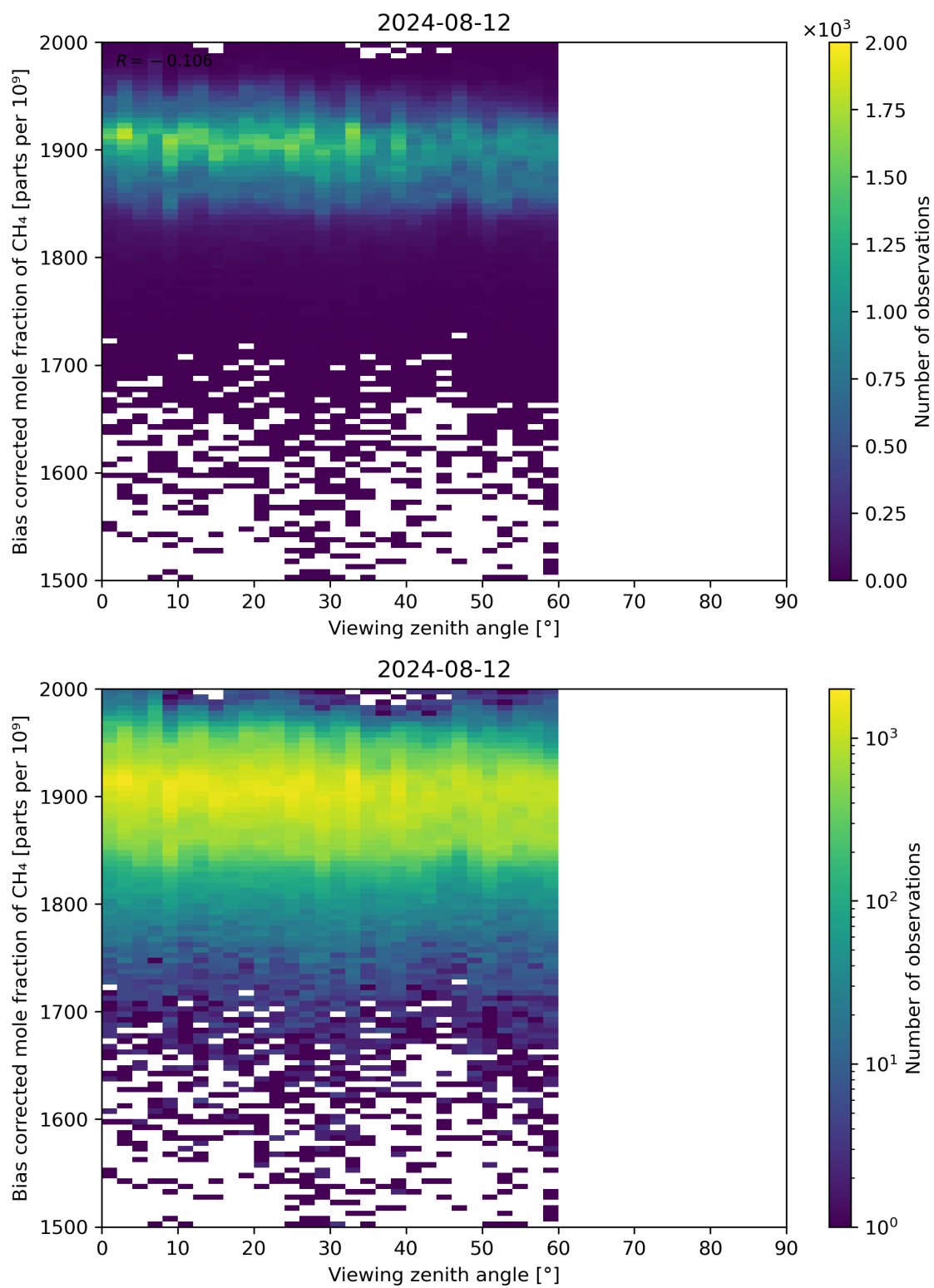
Figure 111: Scatter density plot of “Viewing zenith angle” against “Bias corrected mole fraction of CH 4 ” for 2024-08-12 to 2024-08-13.
