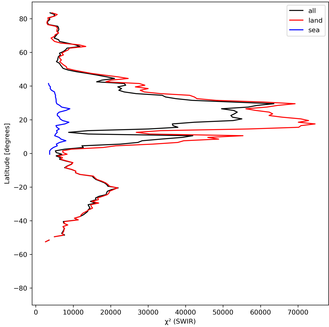
Figure 17: Zonal average of “ \chi^2 (SWIR)” for 2024-08-12 to 2024-08-13.
