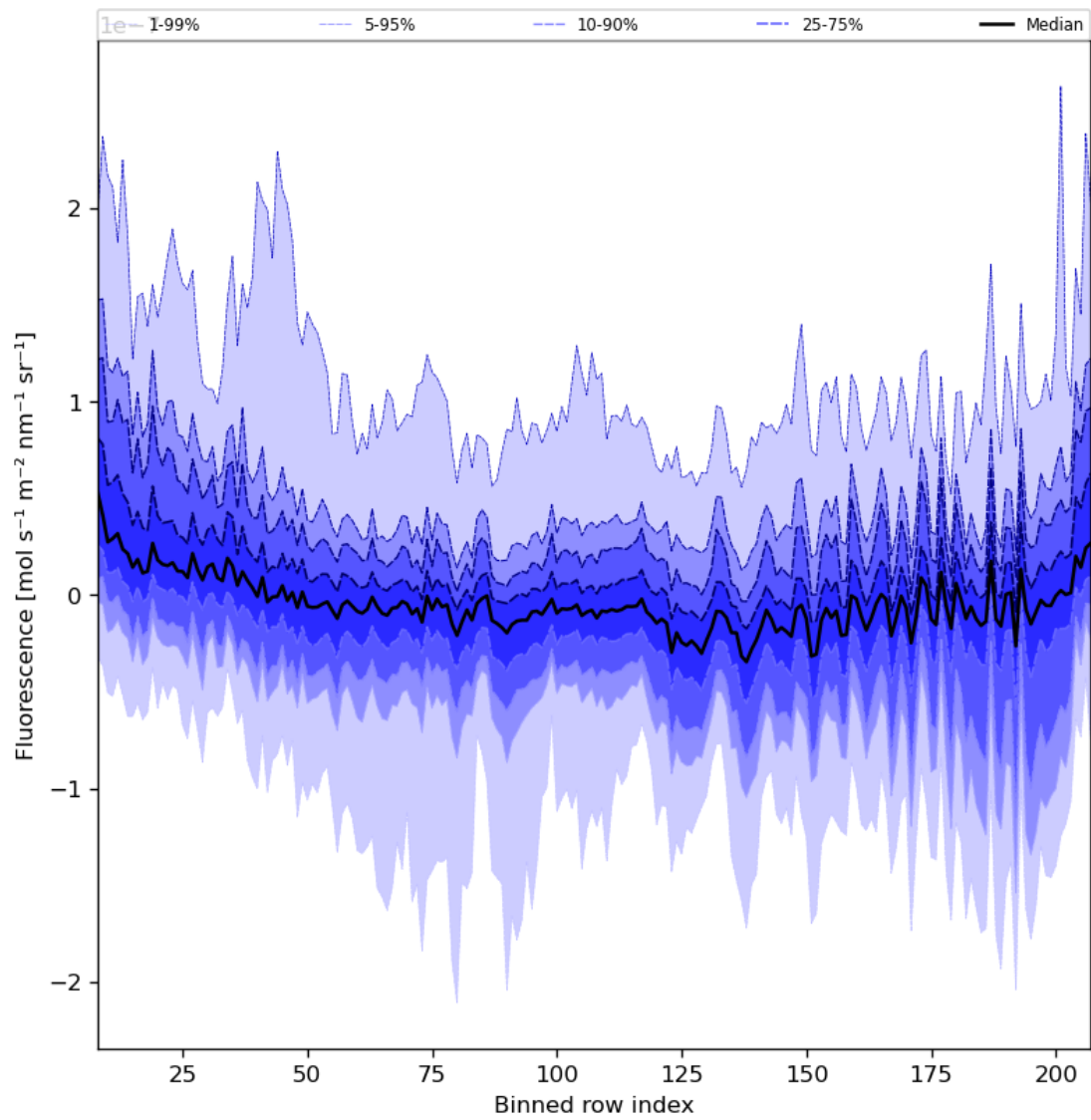
Figure 43: Along track statistics of “Fluorescence” for 2024-08-12 to 2024-08-13
