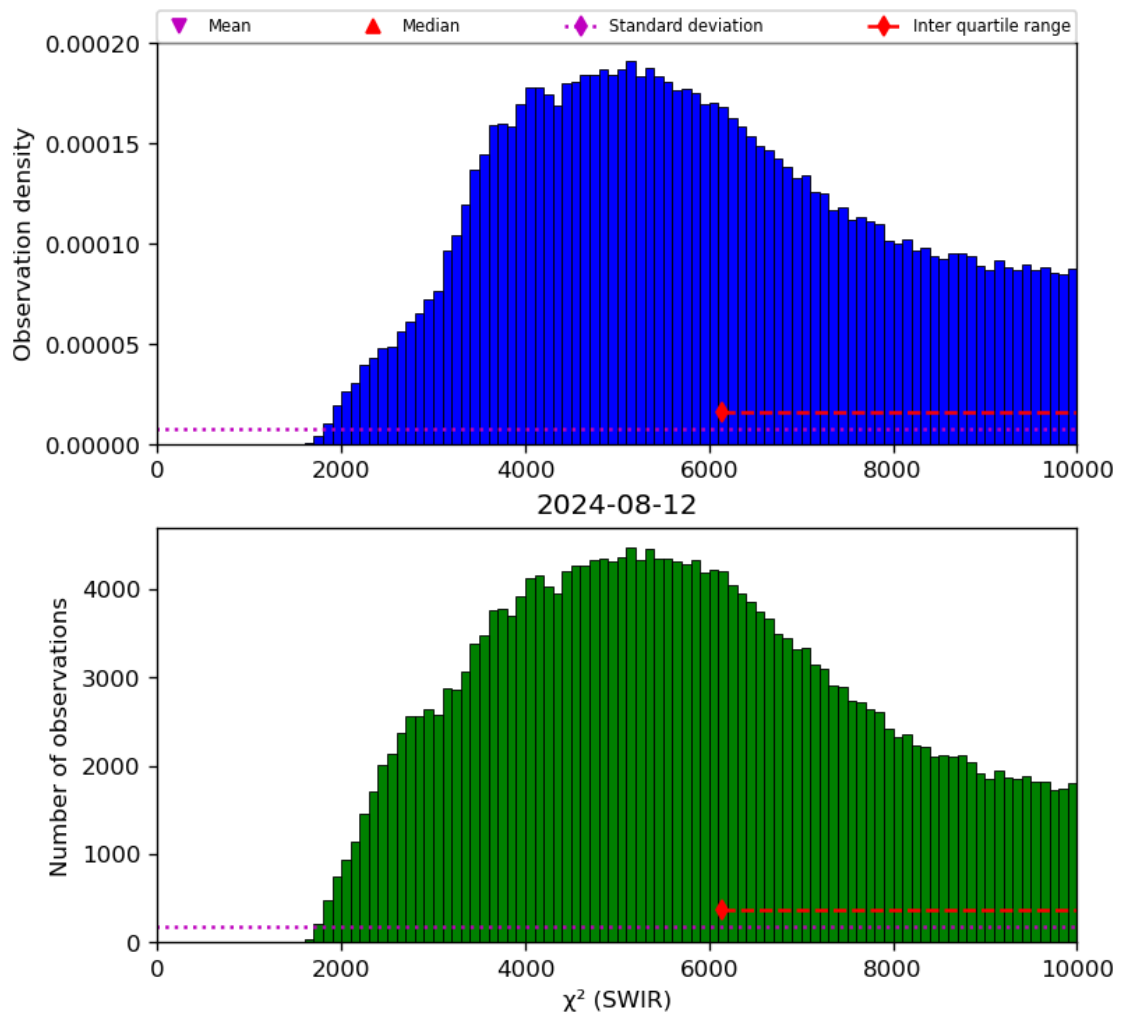
Figure 28: Histogram of “ \chi^2 (SWIR)” for 2024-08-12 to 2024-08-13
