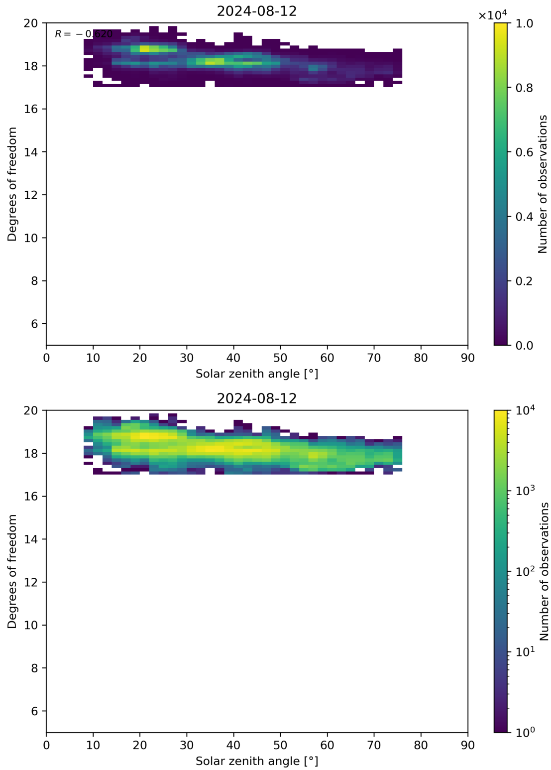
Figure 96: Scatter density plot of “Solar zenith angle” against “Degrees of freedom” for 2024-08-12 to 2024-08-13.
