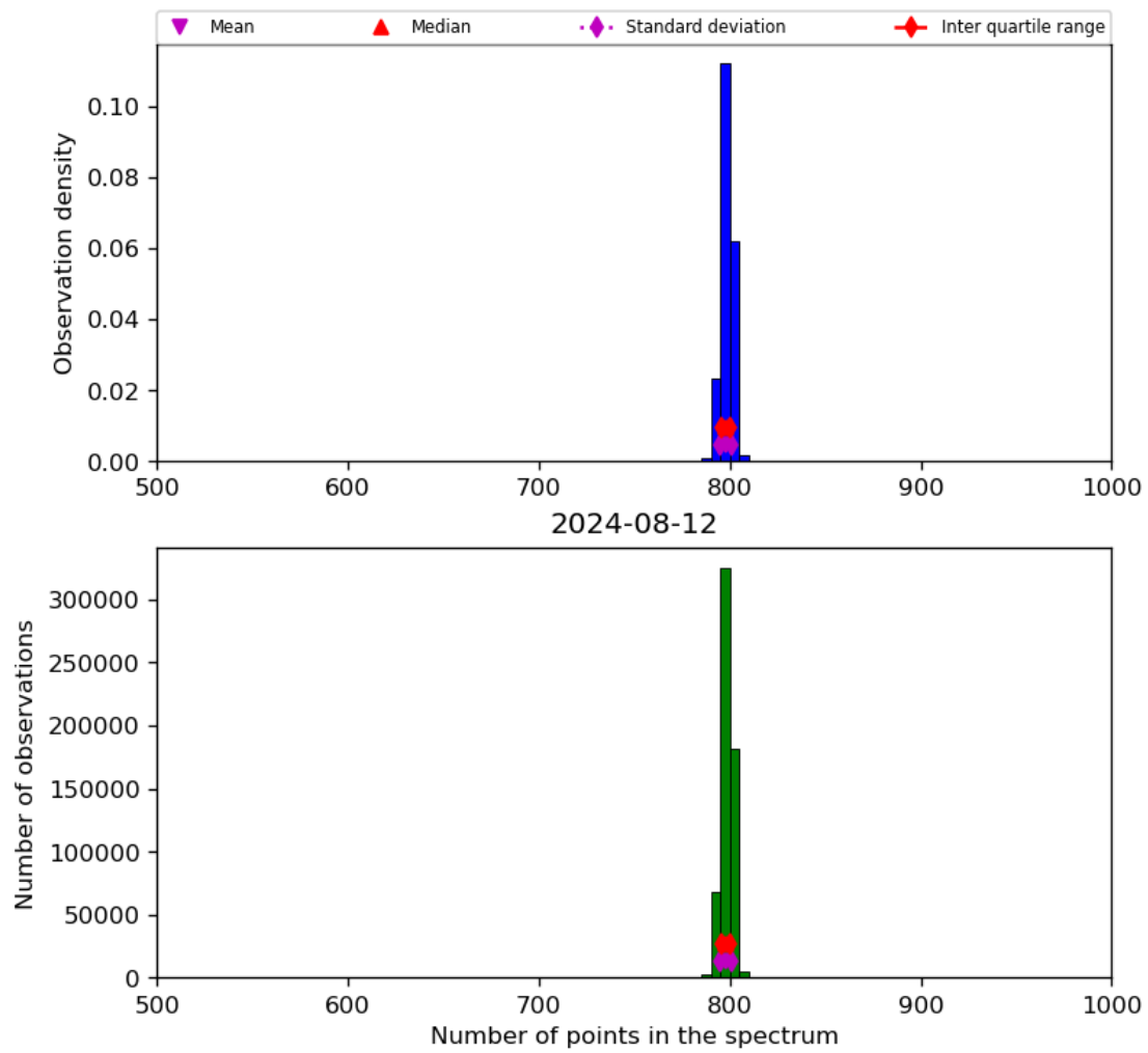
Figure 26: Histogram of “Number of points in the spectrum” for 2024-08-12 to 2024-08-13
