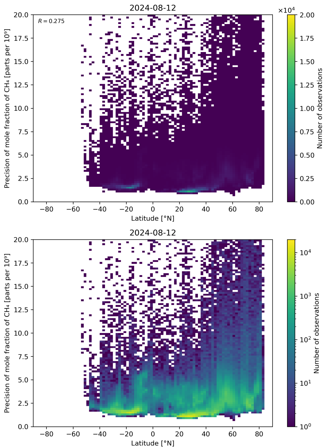
Figure 59: Scatter density plot of “Latitude” against “Precision of mole fraction of \text{CH}_4 ” for 2024-08-12 to 2024-08-13.
