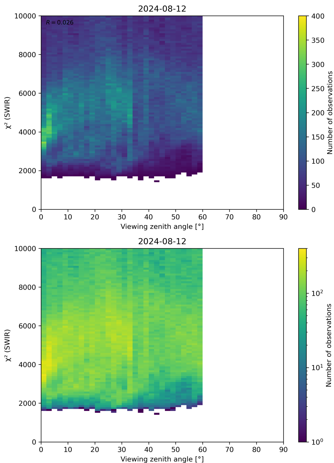
Figure 106: Scatter density plot of “Viewing zenith angle” against “ \chi^2 (SWIR)” for 2024-08-12 to 2024-08-13.
