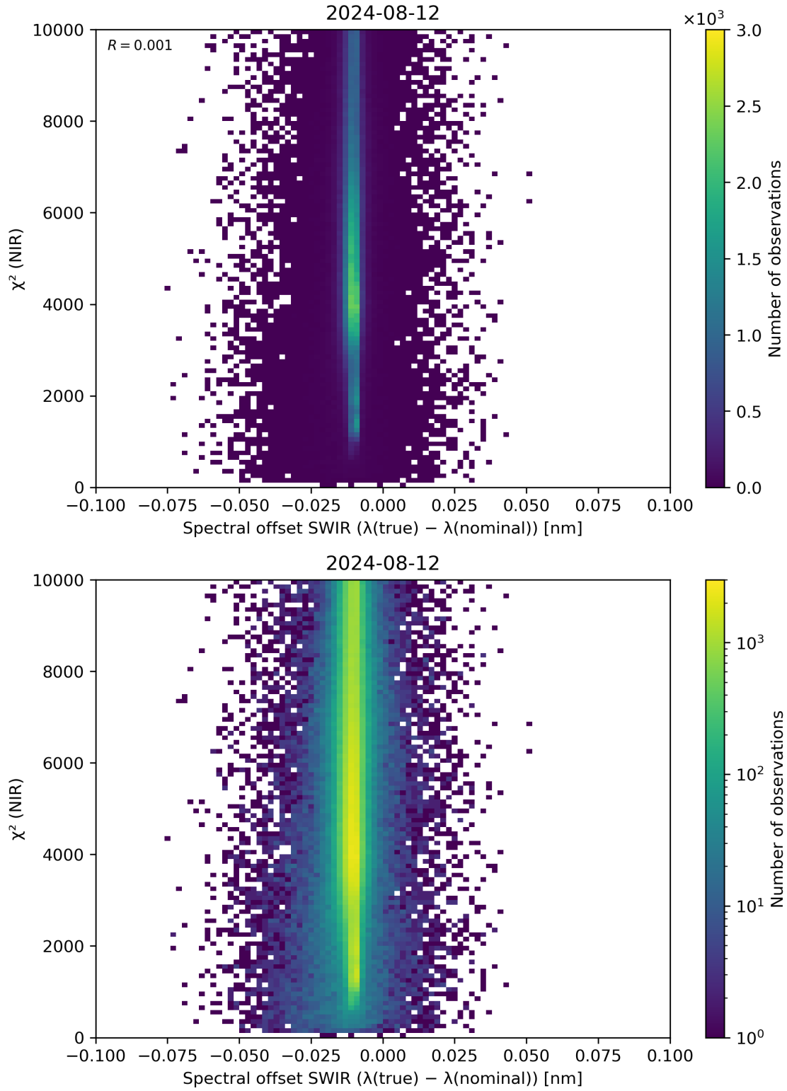
Figure 117: Scatter density plot of “Spectral offset SWIR ( \lambda(\text{true}) - \lambda(\text{nominal}) )” against “ \chi^2 (NIR)” for 2024-08-12 to 2024-08-13.
