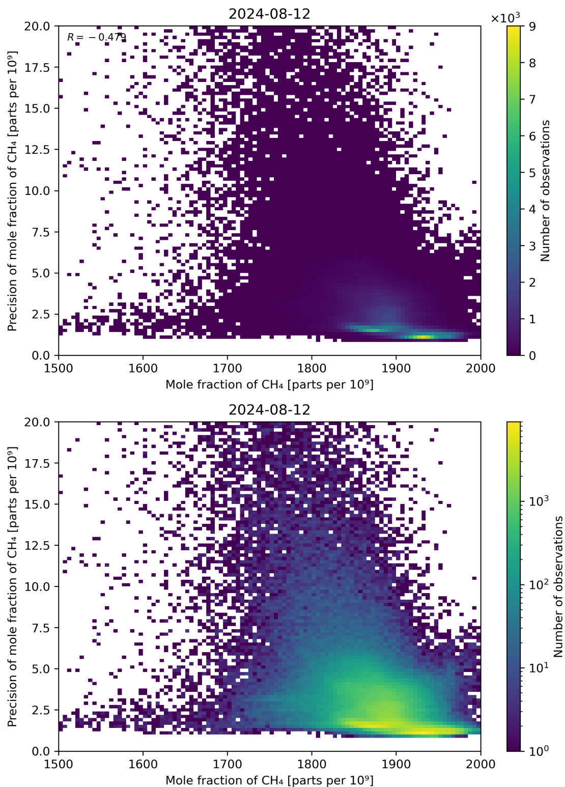
Figure 75: Scatter density plot of “Mole fraction of CH 4 ” against “Precision of mole fraction of CH 4 ” for 2024-08-12 to 2024-08-13.
