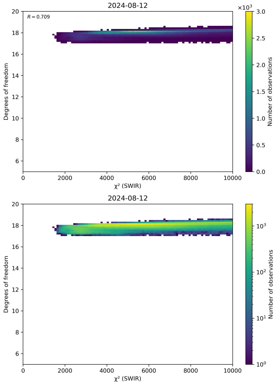
Figure 48: Scatter density plot of “ \chi^2 (SWIR)” against “Degrees of freedom” for 2024-08-12 to 2024-08-13.
