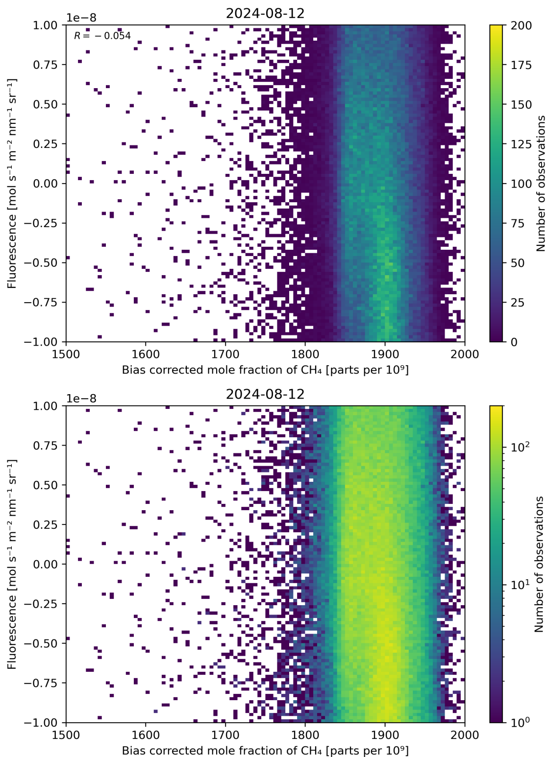
Figure 66: Scatter density plot of “Bias corrected mole fraction of \text{CH}_4 ” against “Fluorescence” for 2024-08-12 to 2024-08-13.
