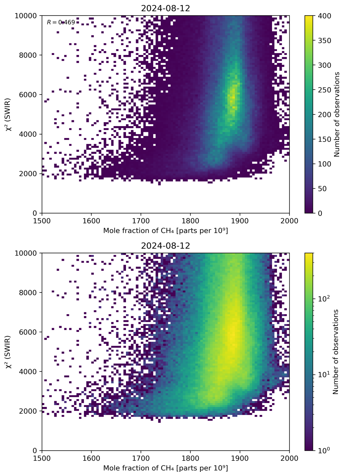
Figure 71: Scatter density plot of “Mole fraction of \text{CH}_4 ” against “ \chi^2 (SWIR)” for 2024-08-12 to 2024-08-13.
