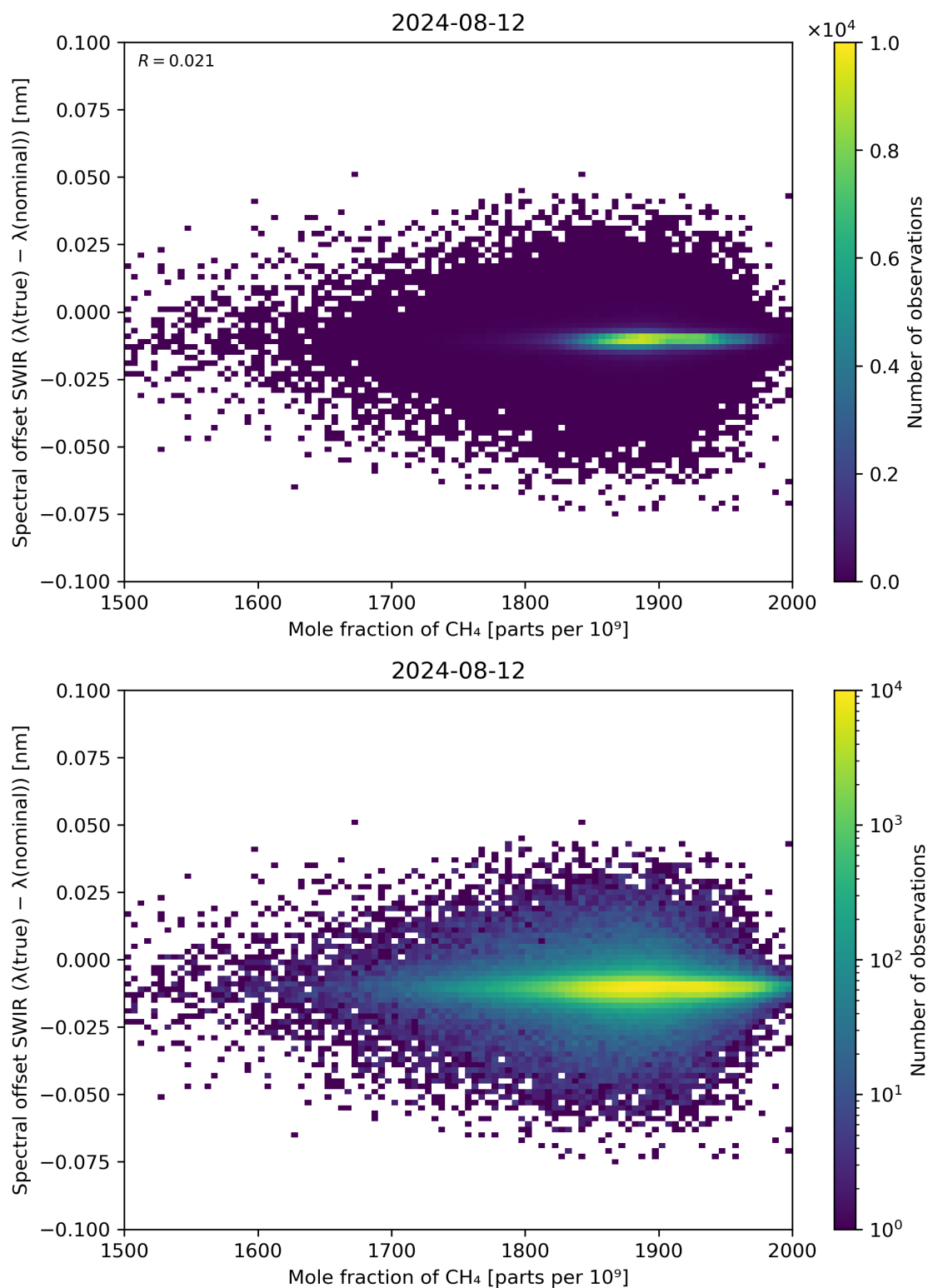
Figure 86: Scatter density plot of “Mole fraction of CH 4 ” against “Spectral offset SWIR ( \lambda(\text{true}) - \lambda(\text{nominal}) )” for 2024-08-12 to 2024-08-13.
