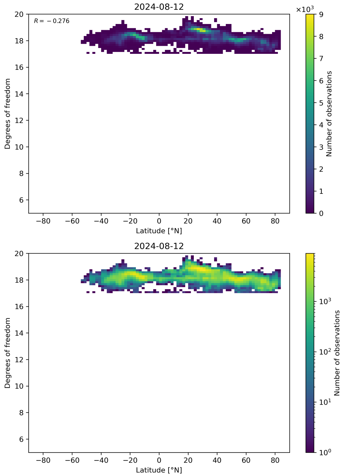
Figure 55: Scatter density plot of “Latitude” against “Degrees of freedom” for 2024-08-12 to 2024-08-13.
