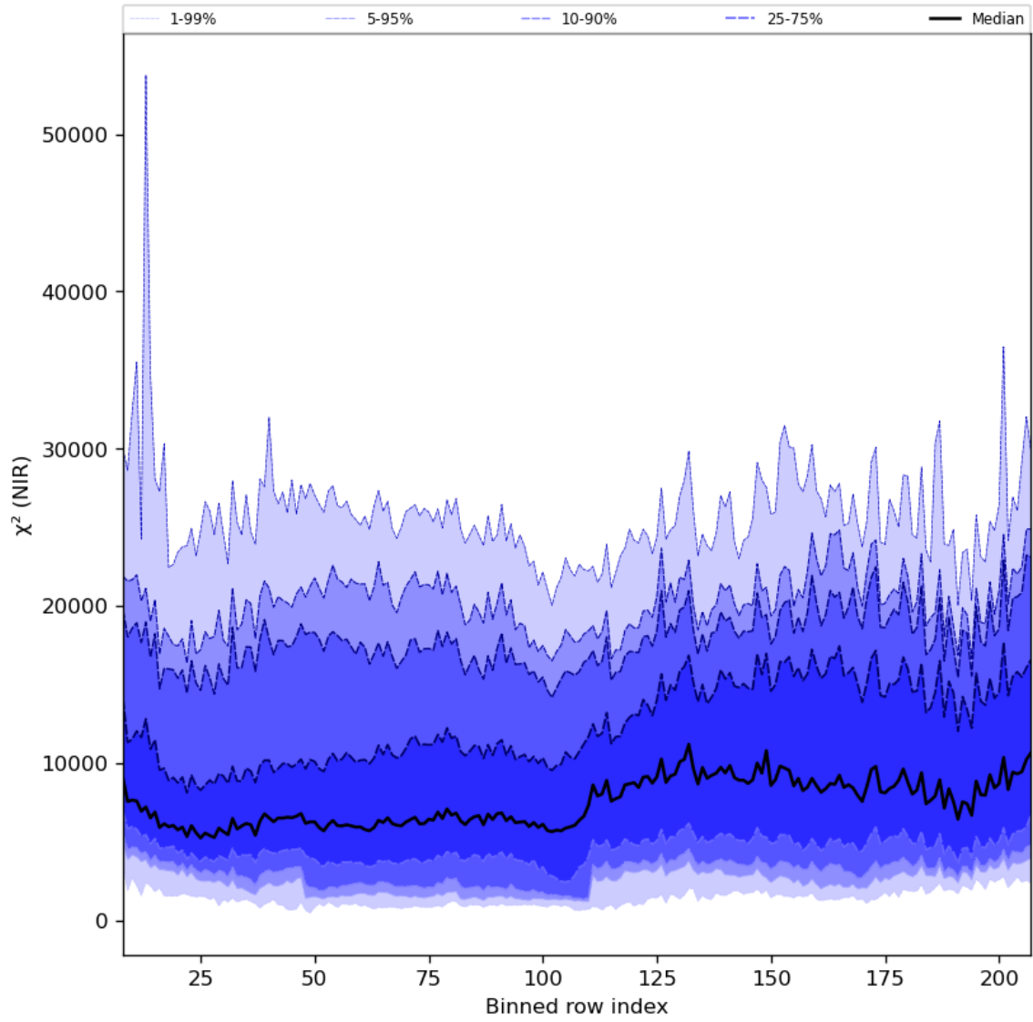
Figure 40: Along track statistics of “ \chi^2 (NIR)” for 2024-08-12 to 2024-08-13
