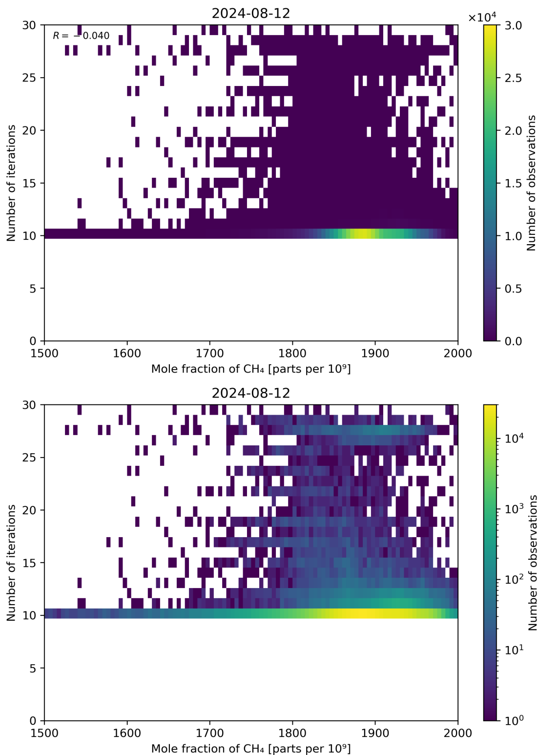
Figure 76: Scatter density plot of “Mole fraction of CH 4 ” against “Number of iterations” for 2024-08-12 to 2024-08-13.
