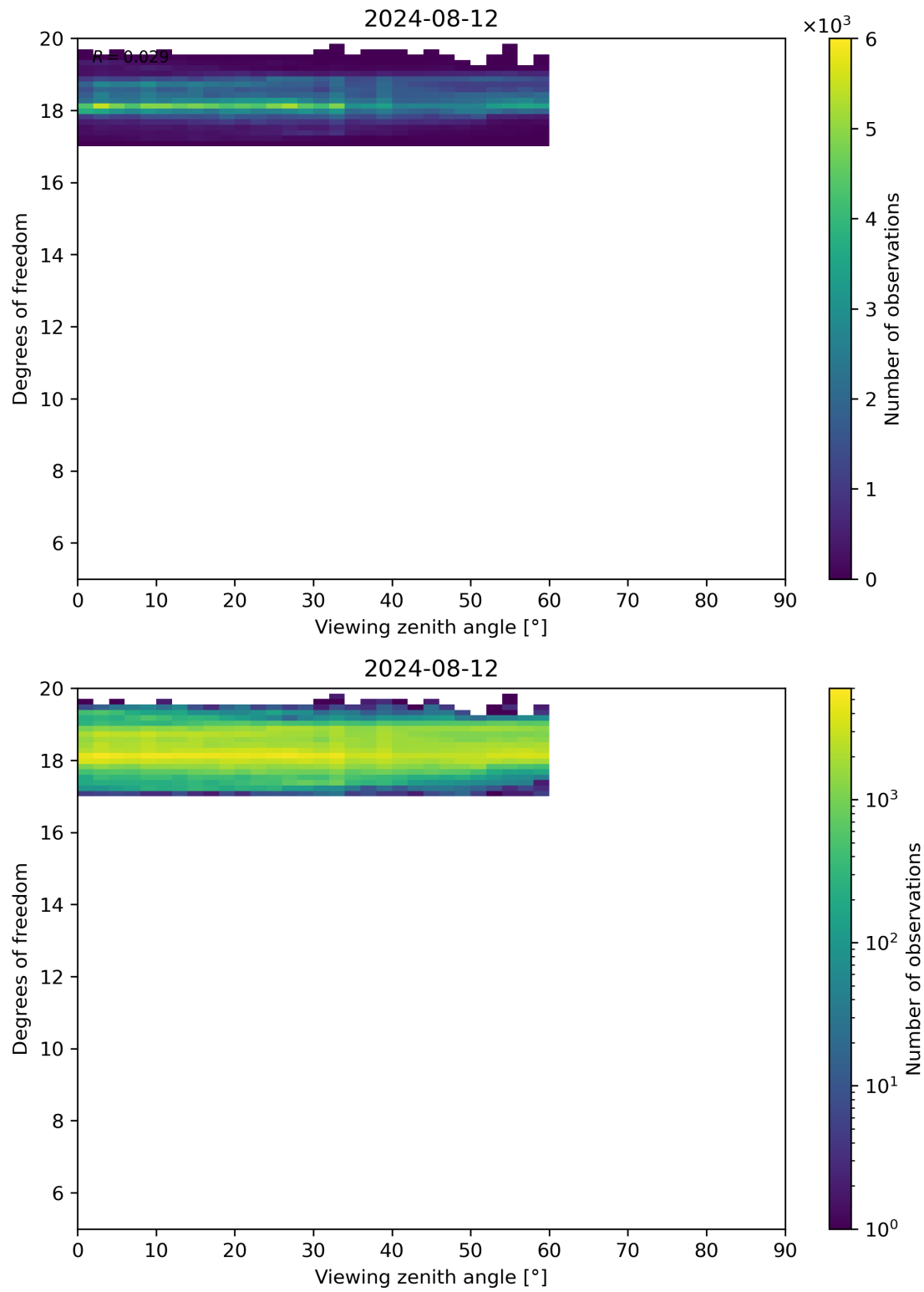
Figure 107: Scatter density plot of “Viewing zenith angle” against “Degrees of freedom” for 2024-08-12 to 2024-08-13.
