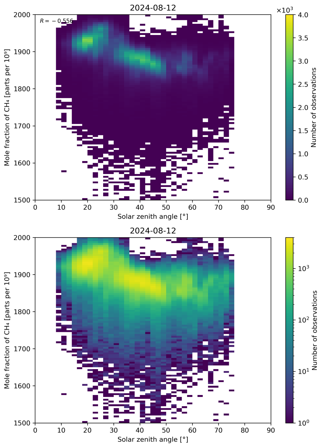
Figure 99: Scatter density plot of “Solar zenith angle” against “Mole fraction of CH 4 ” for 2024-08-12 to 2024-08-13.
