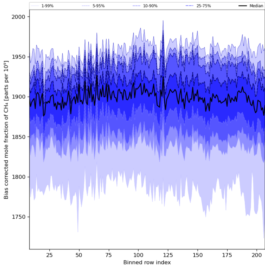
Figure 36: Along track statistics of “Bias corrected mole fraction of CH 4 ” for 2024-08-12 to 2024-08-13
