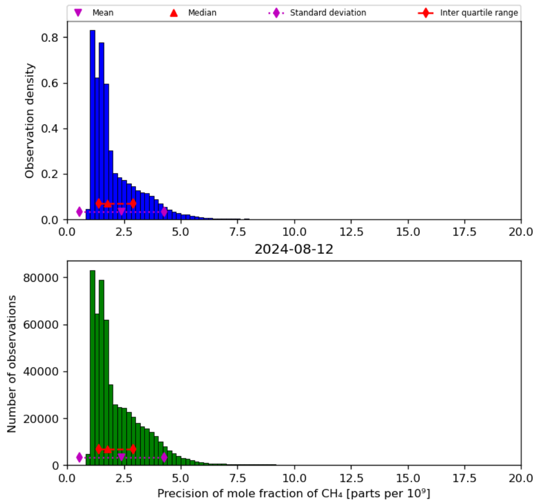
Figure 24: Histogram of “Precision of mole fraction of CH 4 ” for 2024-08-12 to 2024-08-13
