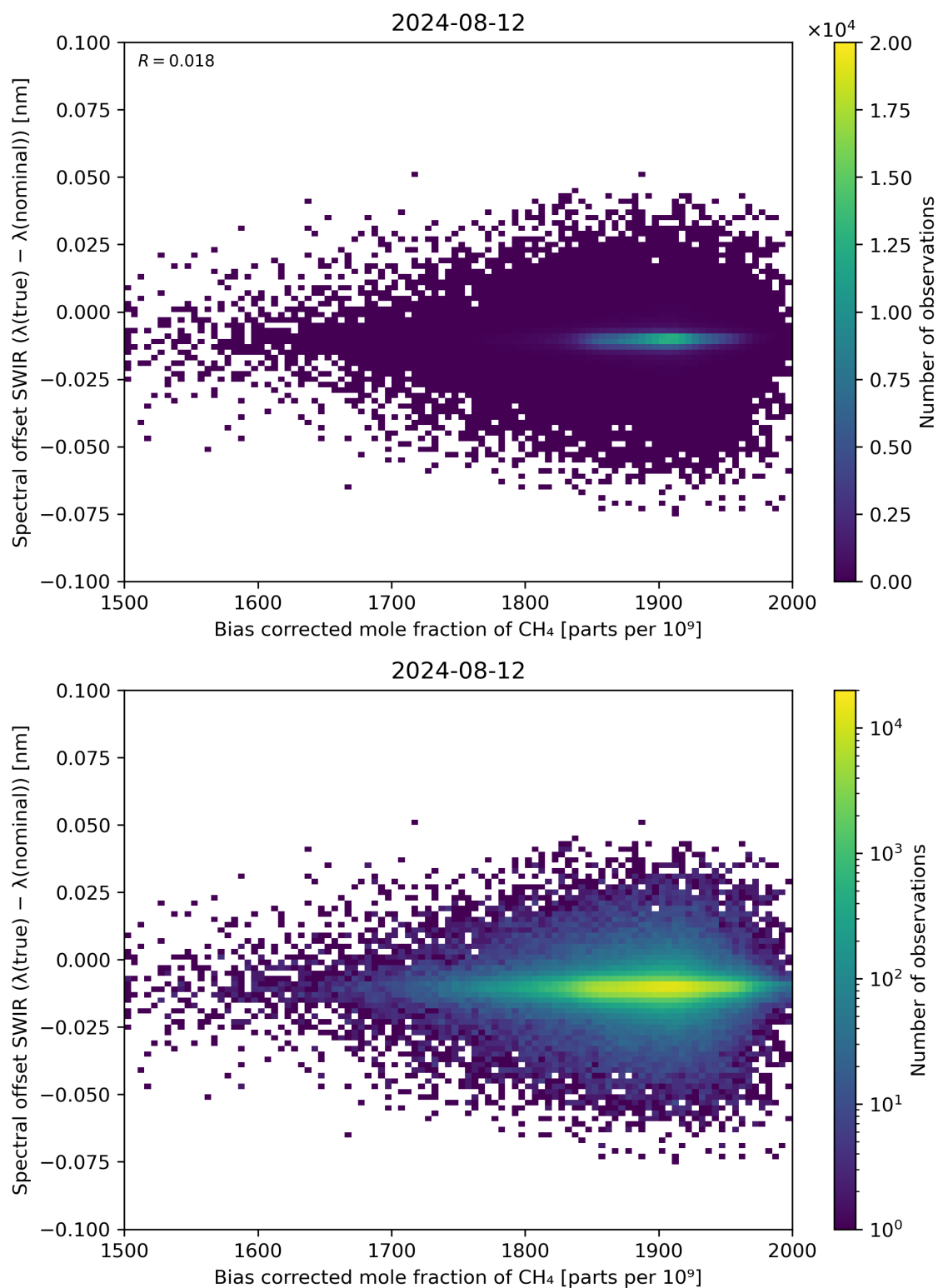
Figure 69: Scatter density plot of “Bias corrected mole fraction of \text{CH}_4 ” against “Spectral offset SWIR ( \lambda(\text{true}) - \lambda(\text{nominal}) )” for 2024-08-12 to 2024-08-13.
