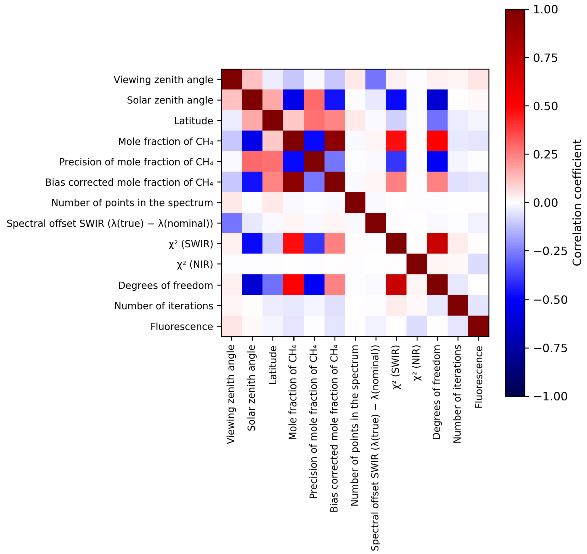
Figure 2: Map of correlation matrix for 2024-08-12 to 2024-08-13.
