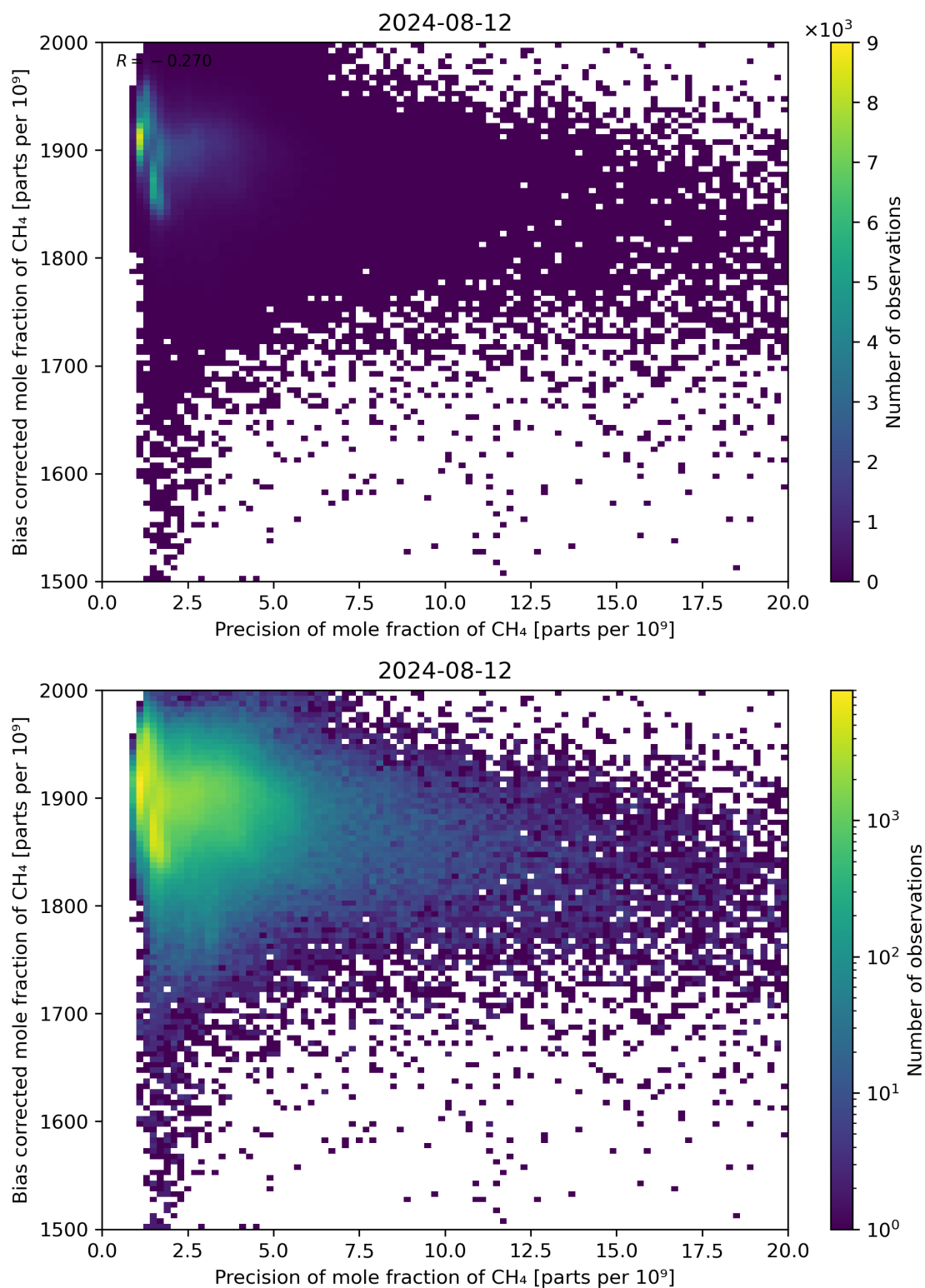
Figure 82: Scatter density plot of “Precision of mole fraction of CH 4 ” against “Bias corrected mole fraction of CH 4 ” for 2024-08-12 to 2024-08-13.
