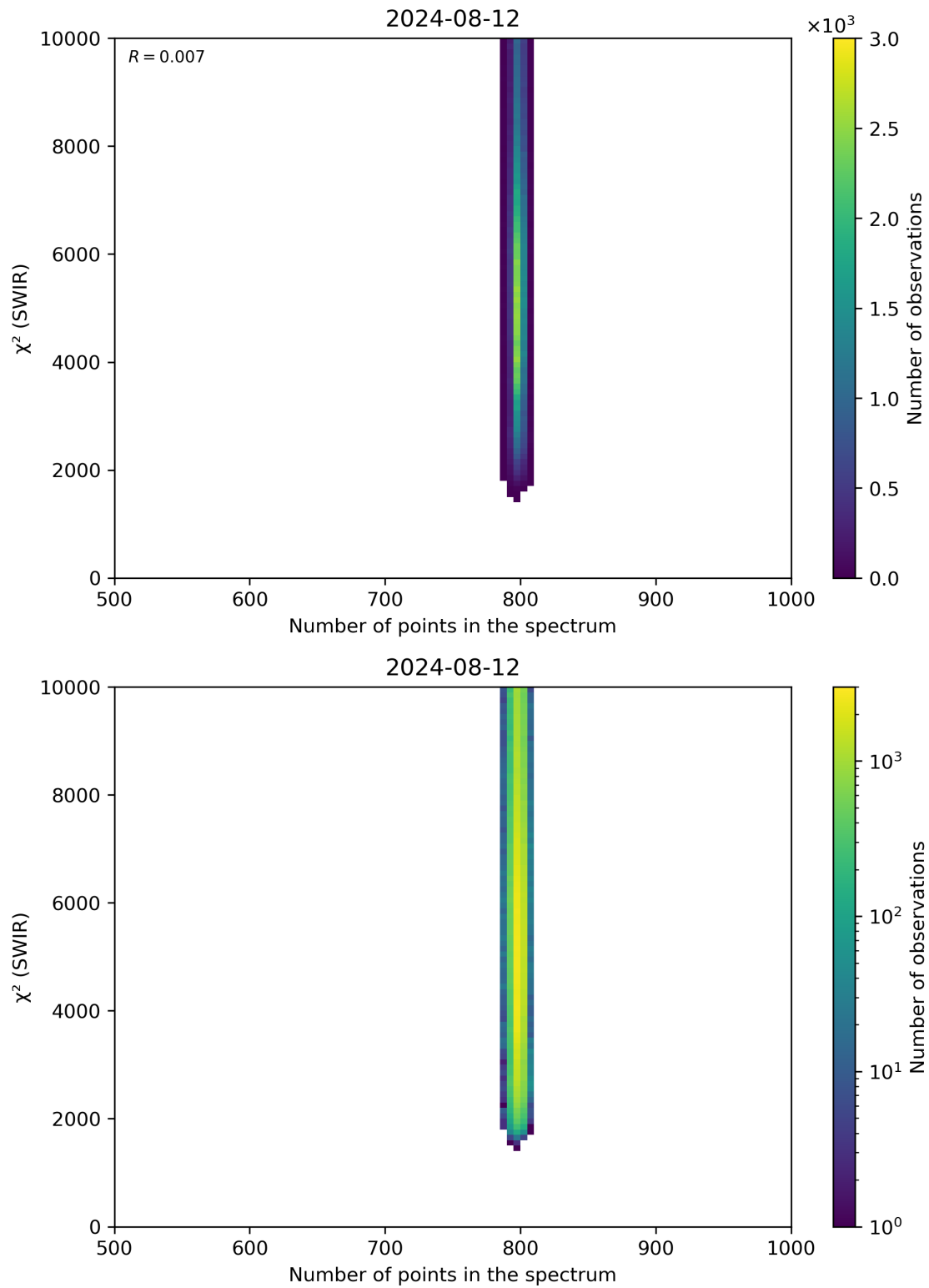
Figure 89: Scatter density plot of “Number of points in the spectrum” against “ \chi^2 (SWIR)” for 2024-08-12 to 2024-08-13.
