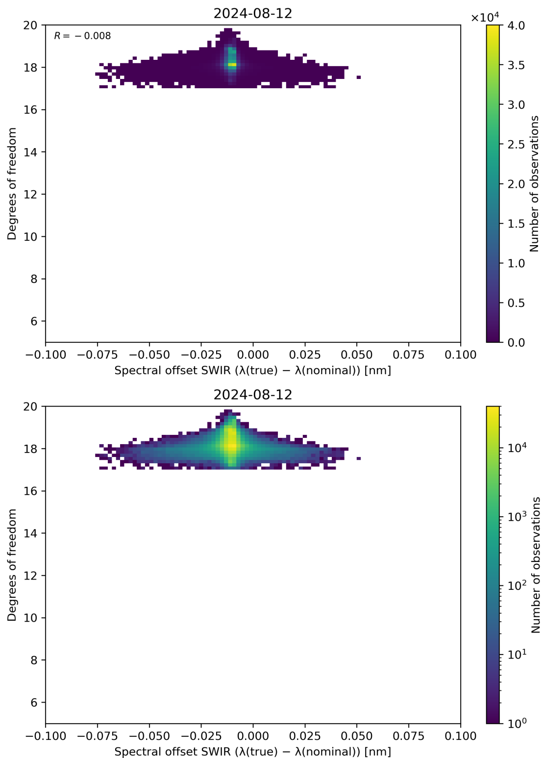
Figure 119: Scatter density plot of “Spectral offset SWIR ( \lambda(\text{true}) - \lambda(\text{nominal}) )” against “Degrees of freedom” for 2024-08-12 to 2024-08-13.
