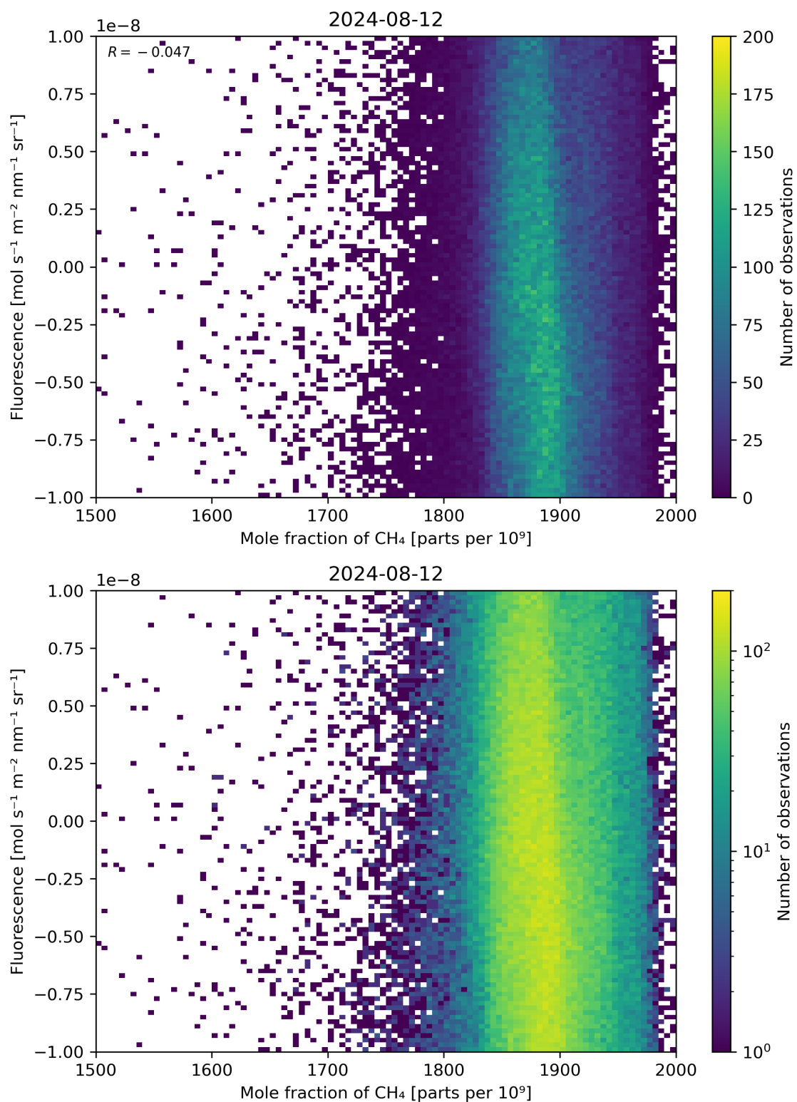
Figure 73: Scatter density plot of “Mole fraction of \text{CH}_4 ” against “Fluorescence” for 2024-08-12 to 2024-08-13.
