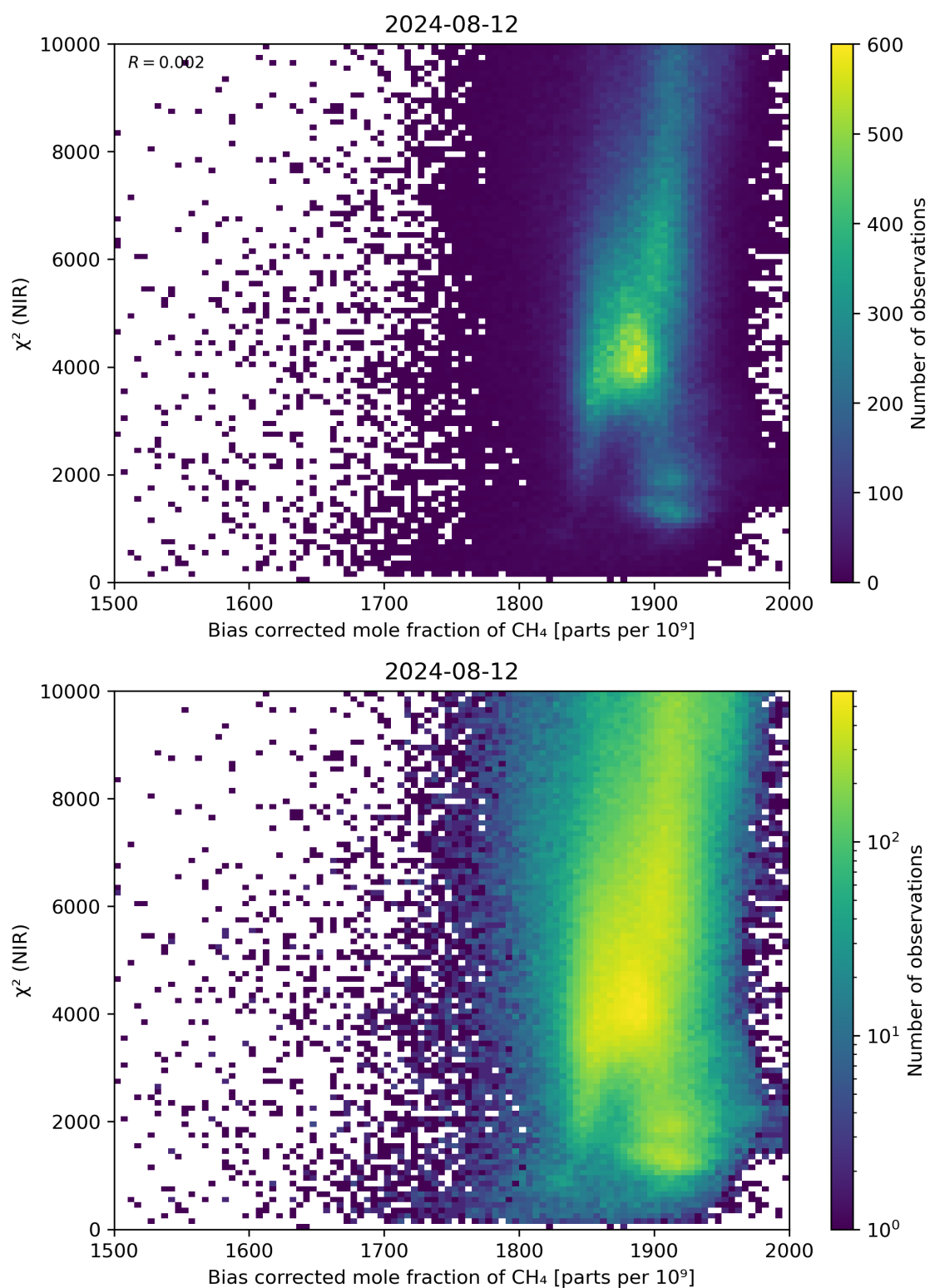
Figure 63: Scatter density plot of “Bias corrected mole fraction of \text{CH}_4 ” against “ \chi^2 (NIR)” for 2024-08-12 to 2024-08-13.
