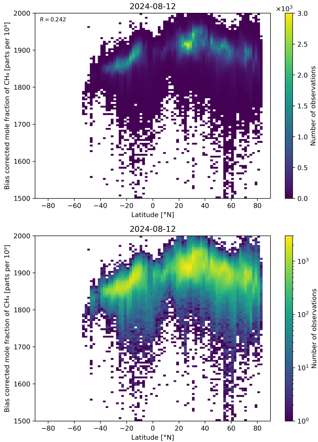
Figure 58: Scatter density plot of “Latitude” against “Bias corrected mole fraction of CH 4 ” for 2024-08-12 to 2024-08-13.
