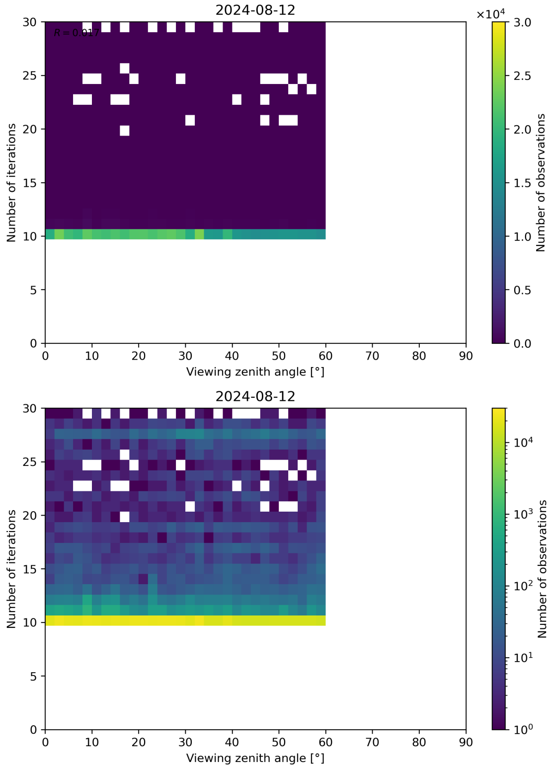
Figure 113: Scatter density plot of “Viewing zenith angle” against “Number of iterations” for 2024-08-12 to 2024-08-13.
