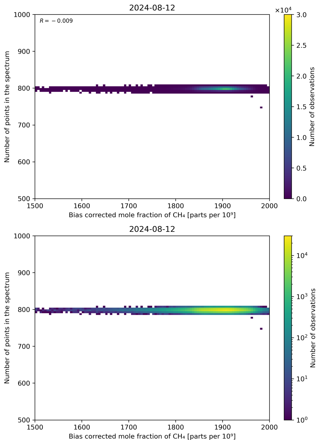
Figure 68: Scatter density plot of “Bias corrected mole fraction of CH 4 ” against “Number of points in the spectrum” for 2024-08-12 to 2024-08-13.
