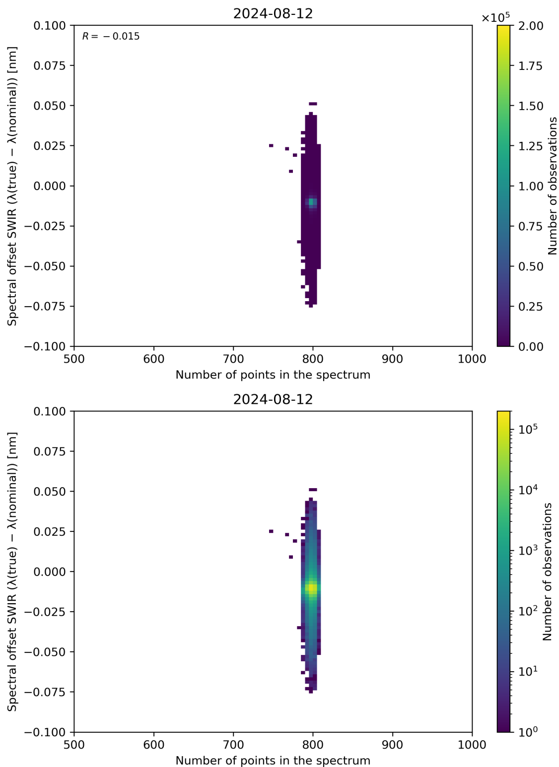
Figure 93: Scatter density plot of “Number of points in the spectrum” against “Spectral offset SWIR ( \lambda(\text{true}) - \lambda(\text{nominal}) )” for 2024-08-12 to 2024-08-13.
