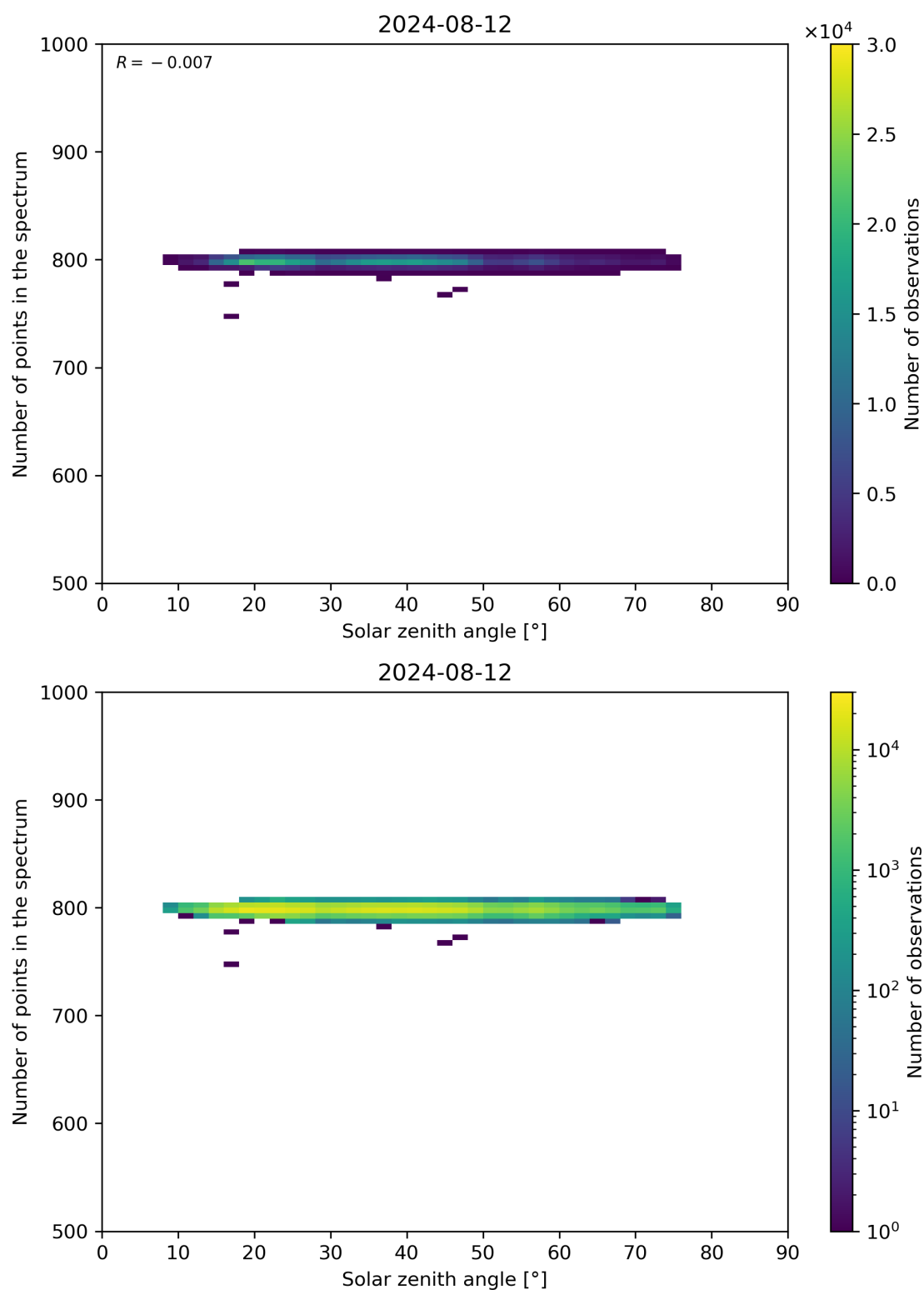
Figure 103: Scatter density plot of “Solar zenith angle” against “Number of points in the spectrum” for 2024-08-12 to 2024-08-13.
