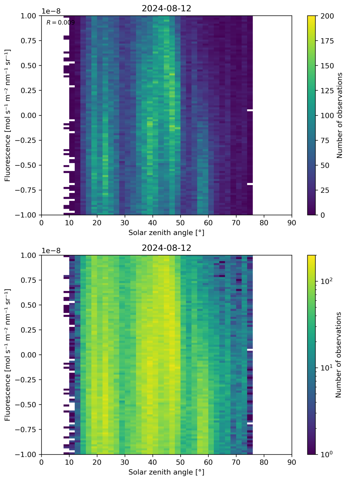
Figure 97: Scatter density plot of “Solar zenith angle” against “Fluorescence” for 2024-08-12 to 2024-08-13.
