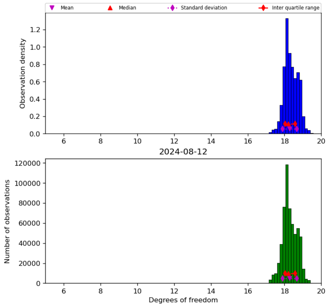
Figure 30: Histogram of “Degrees of freedom” for 2024-08-12 to 2024-08-13
