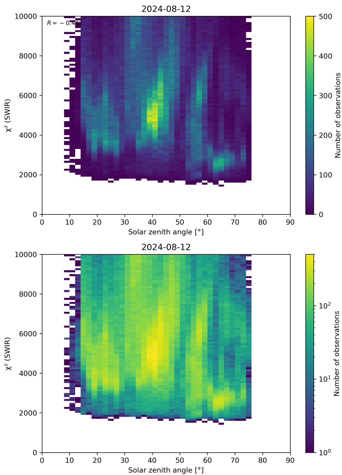
Figure 95: Scatter density plot of “Solar zenith angle” against “ \chi^2 (SWIR)” for 2024-08-12 to 2024-08-13.
