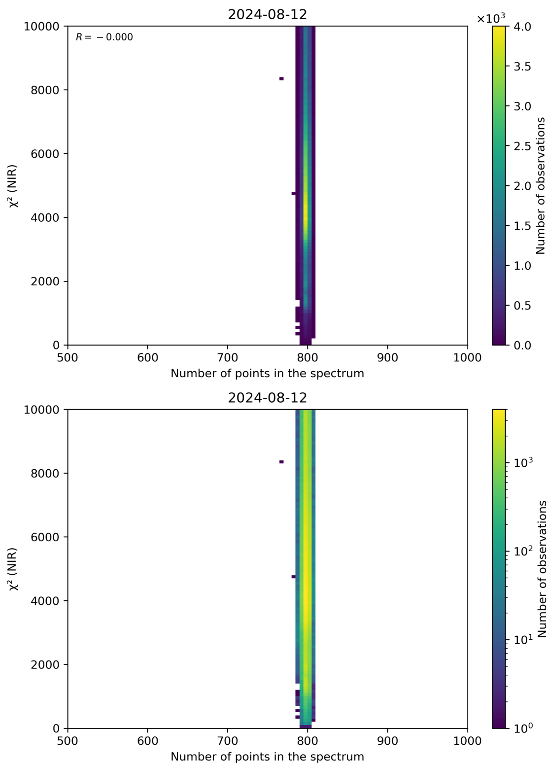
Figure 88: Scatter density plot of “Number of points in the spectrum” against “ \chi^2 (NIR)” for 2024-08-12 to 2024-08-13.
