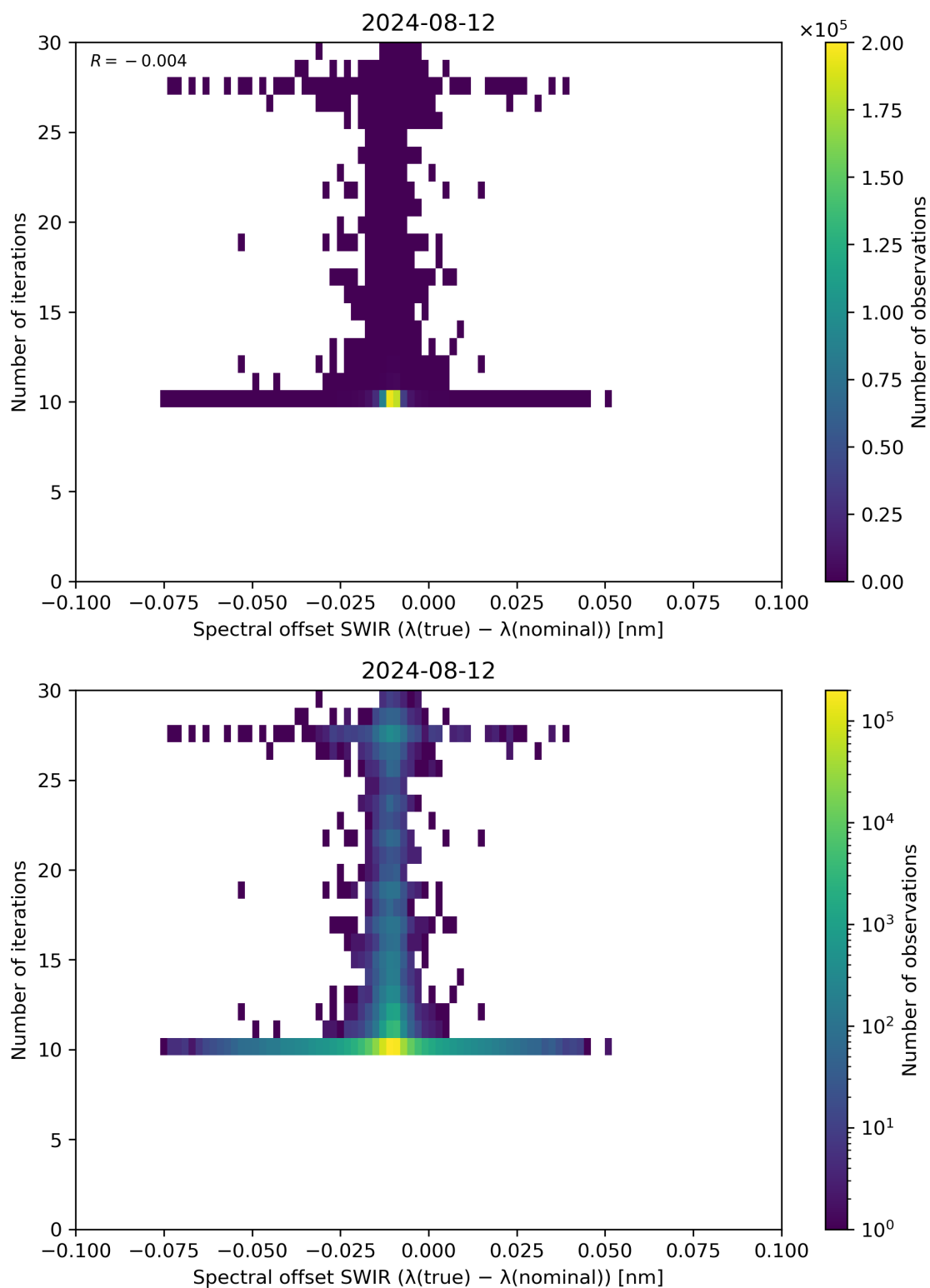
Figure 121: Scatter density plot of “Spectral offset SWIR ( \lambda(\text{true}) - \lambda(\text{nominal}) )” against “Number of iterations” for 2024-08-12 to 2024-08-13.
