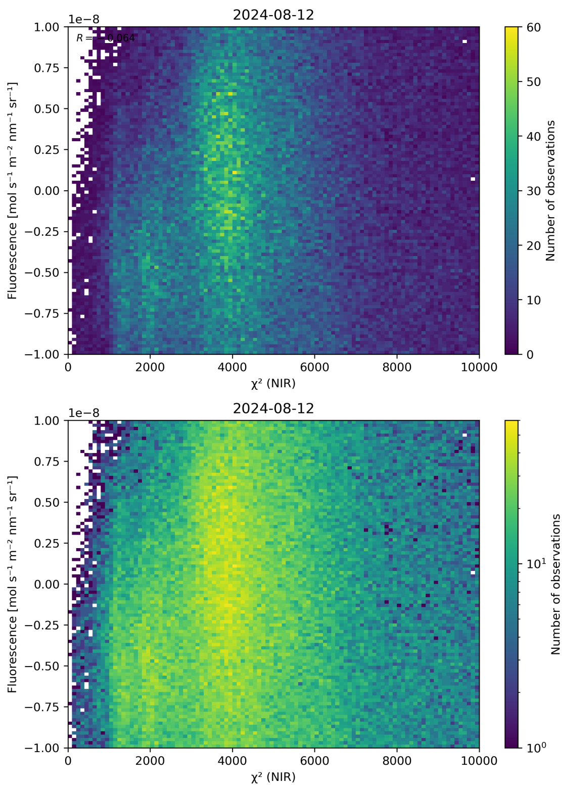
Figure 45: Scatter density plot of “ \chi^2 (NIR)” against “Fluorescence” for 2024-08-12 to 2024-08-13.
