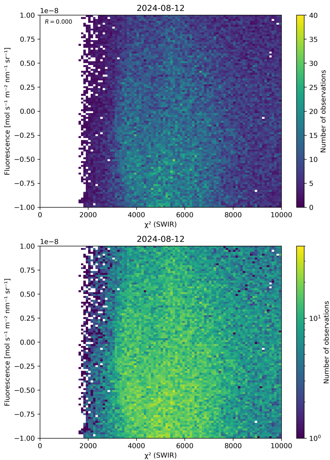
Figure 49: Scatter density plot of “ \chi^2 (SWIR)” against “Fluorescence” for 2024-08-12 to 2024-08-13.
