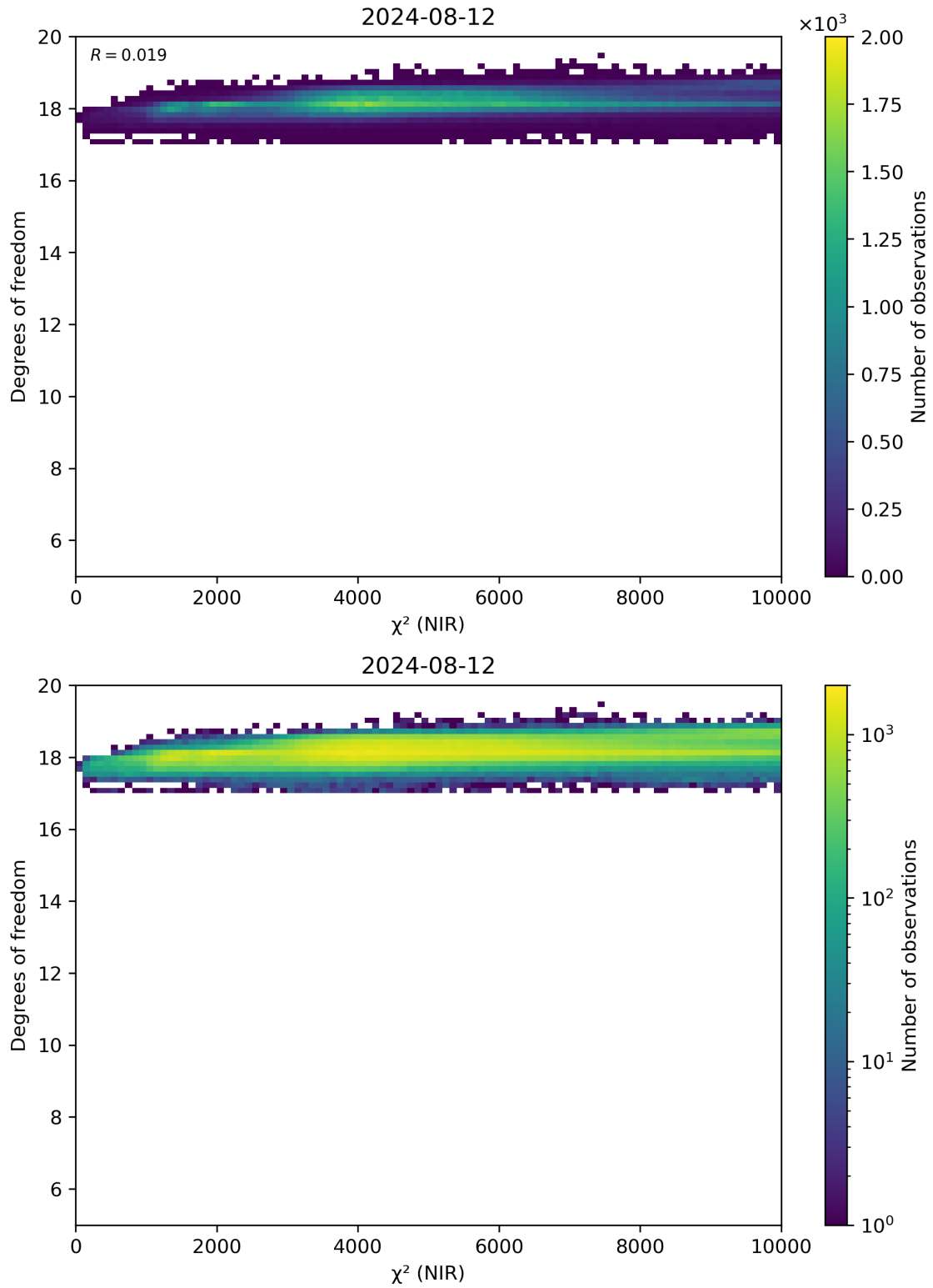
Figure 44: Scatter density plot of “ \chi^2 (NIR)” against “Degrees of freedom” for 2024-08-12 to 2024-08-13.
