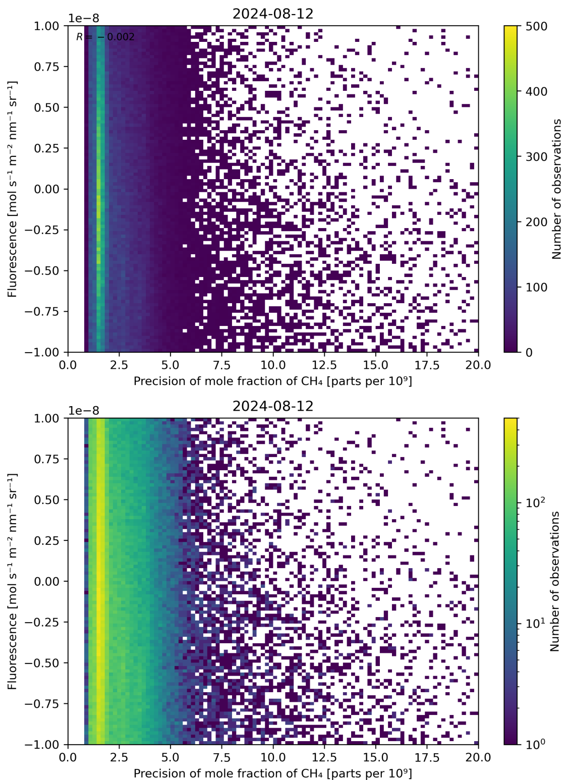
Figure 81: Scatter density plot of “Precision of mole fraction of \text{CH}_4 ” against “Fluorescence” for 2024-08-12 to 2024-08-13.
