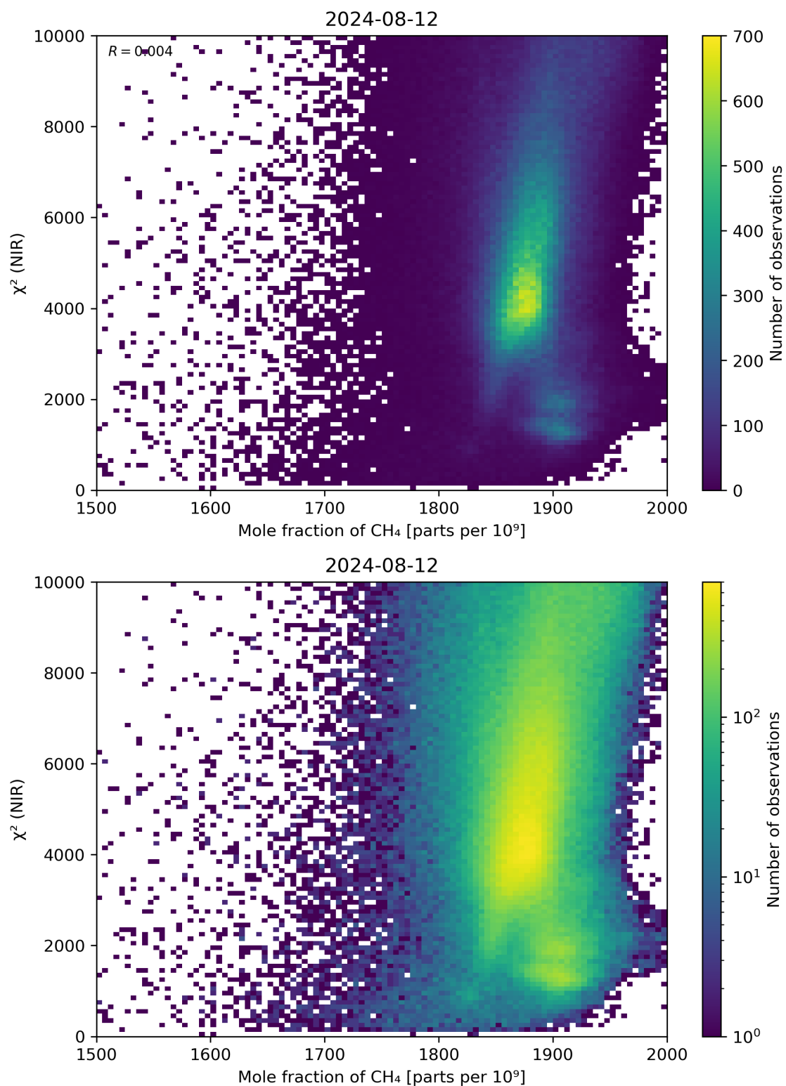
Figure 70: Scatter density plot of “Mole fraction of \text{CH}_4 ” against “ \chi^2 (NIR)” for 2024-08-12 to 2024-08-13.
