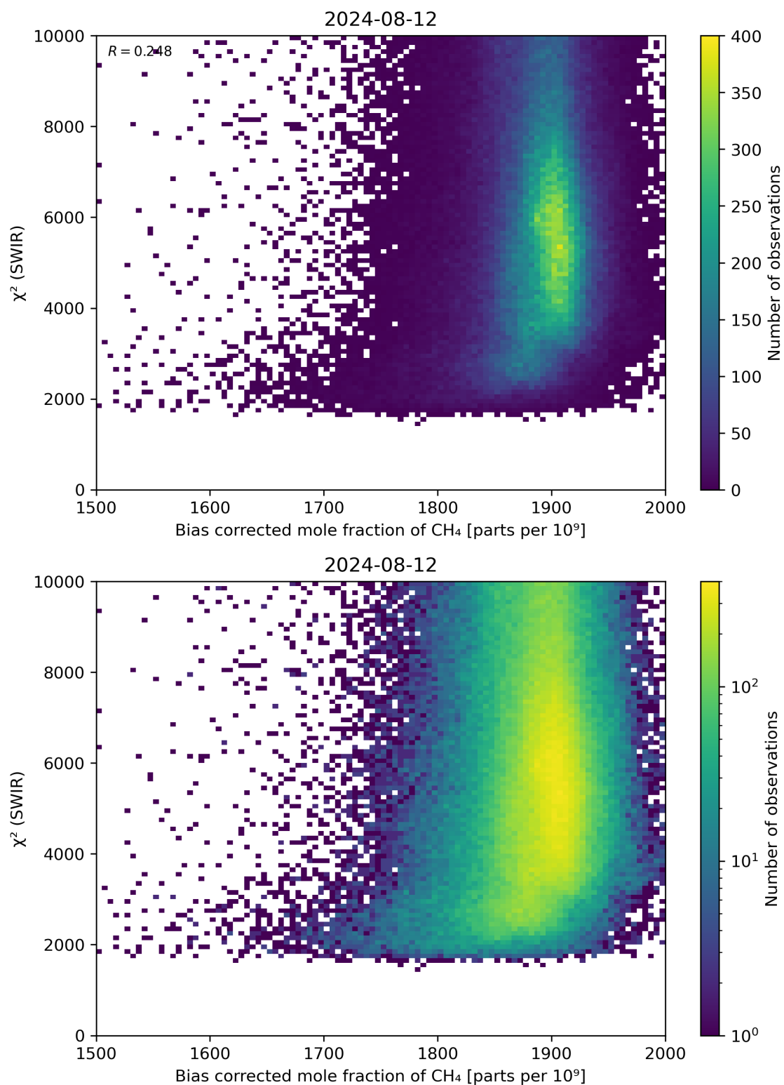
Figure 64: Scatter density plot of “Bias corrected mole fraction of \text{CH}_4 ” against “ \chi^2 (SWIR)” for 2024-08-12 to 2024-08-13.
