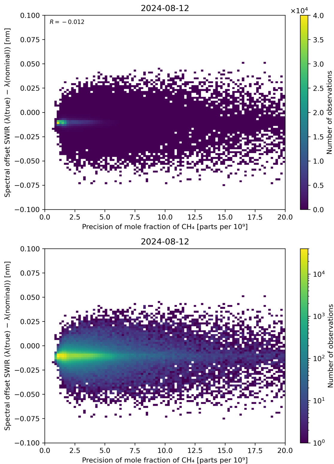
Figure 85: Scatter density plot of “Precision of mole fraction of \text{CH}_4 ” against “Spectral offset SWIR ( \lambda(\text{true}) - \lambda(\text{nominal}) )” for 2024-08-12 to 2024-08-13.
