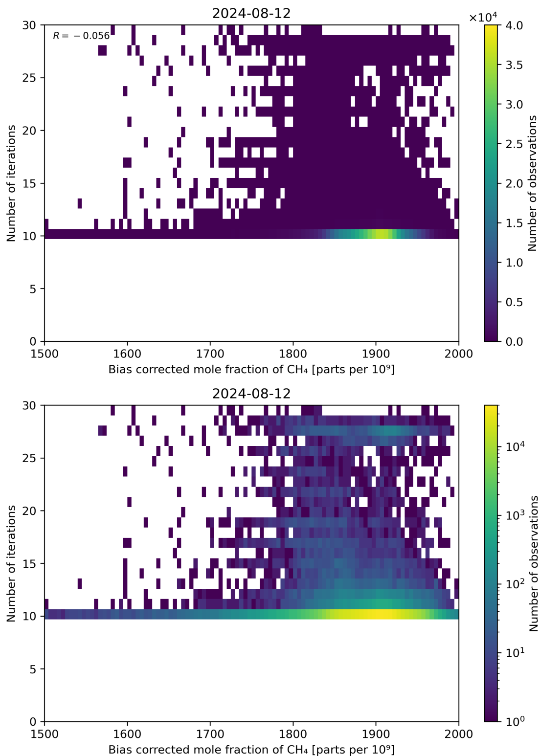
Figure 67: Scatter density plot of “Bias corrected mole fraction of \text{CH}_4 ” against “Number of iterations” for 2024-08-12 to 2024-08-13.
