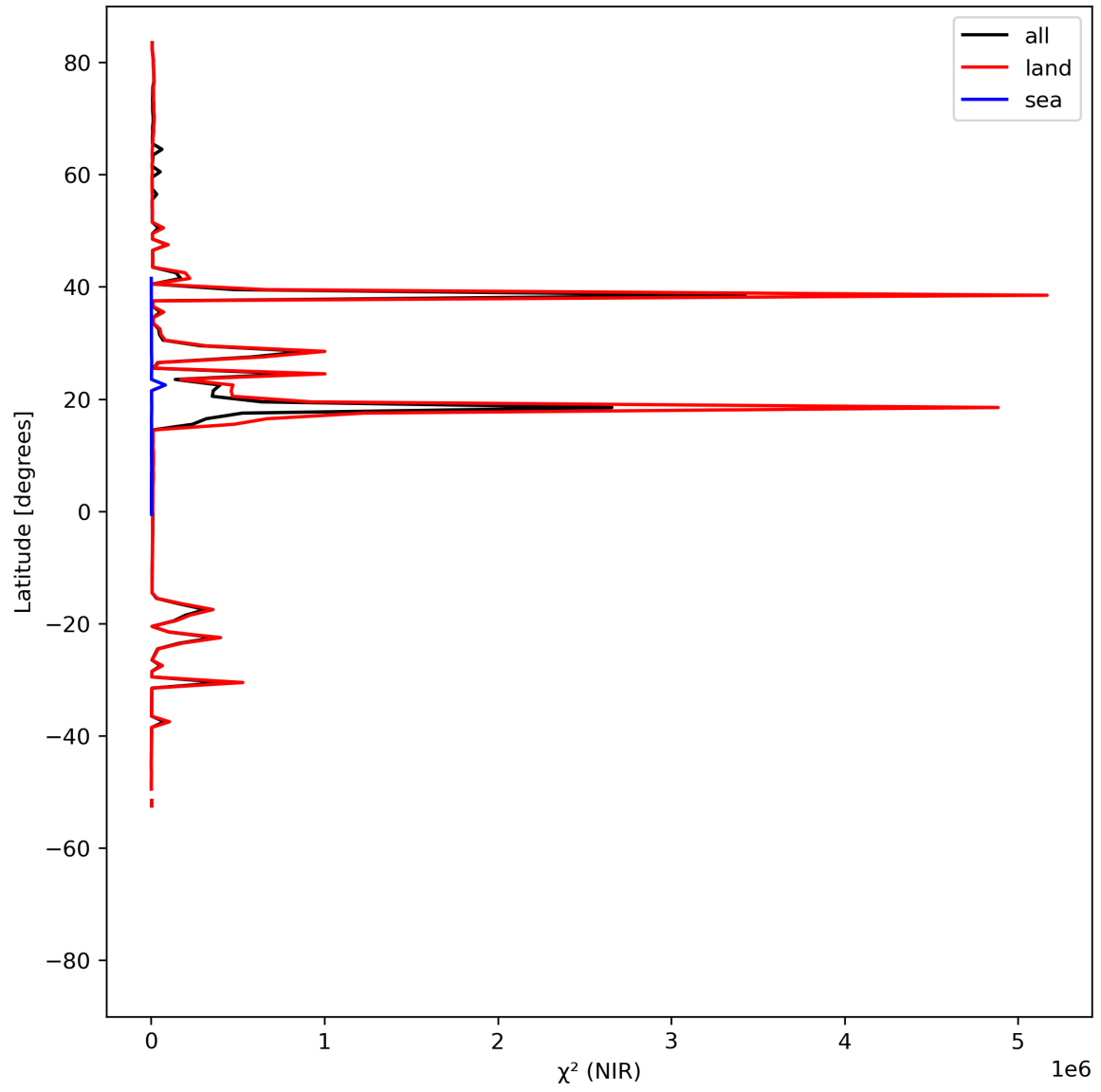
Figure 18: Zonal average of “ \chi^2 (NIR)” for 2024-08-12 to 2024-08-13.
