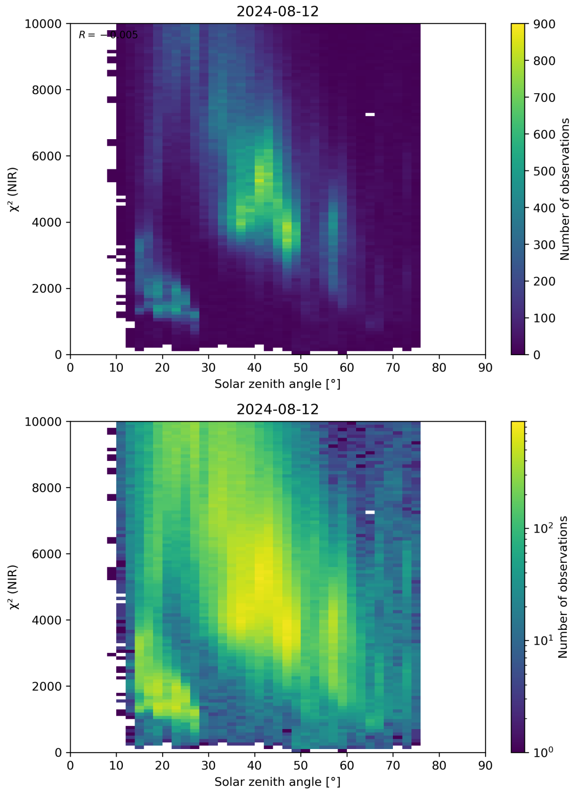
Figure 94: Scatter density plot of “Solar zenith angle” against “ \chi^2 (NIR)” for 2024-08-12 to 2024-08-13.
