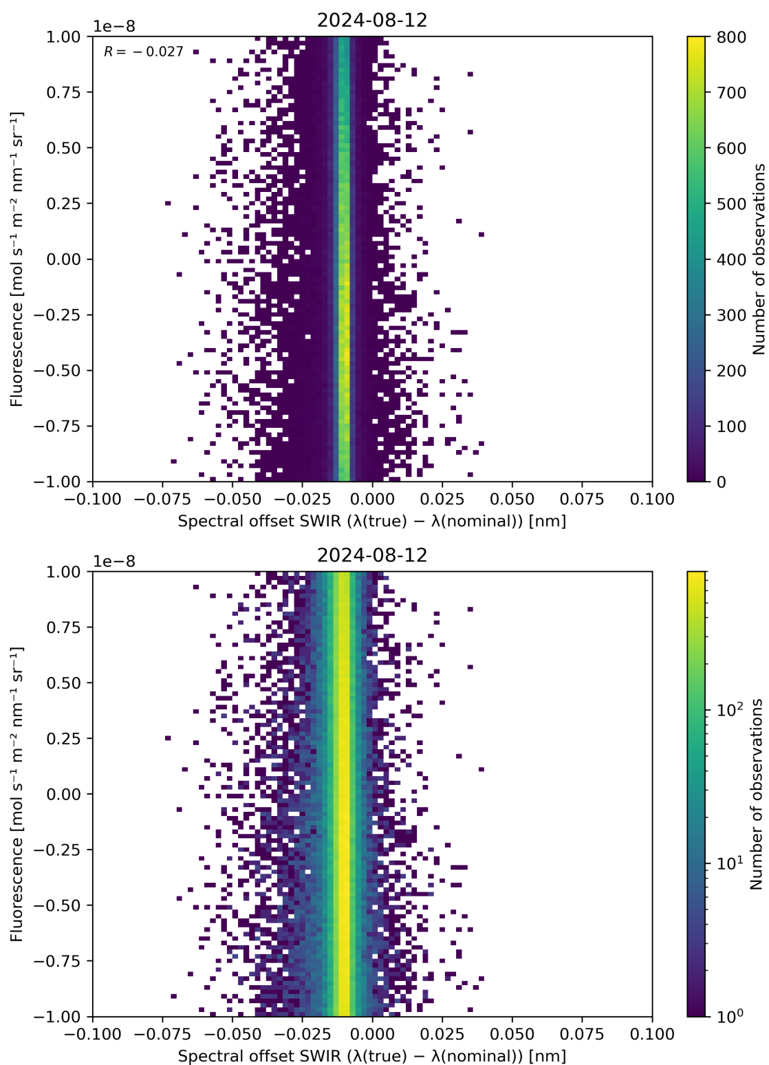
Figure 120: Scatter density plot of “Spectral offset SWIR ( \lambda(\text{true}) - \lambda(\text{nominal}) )” against “Fluorescence” for 2024-08-12 to 2024-08-13.
