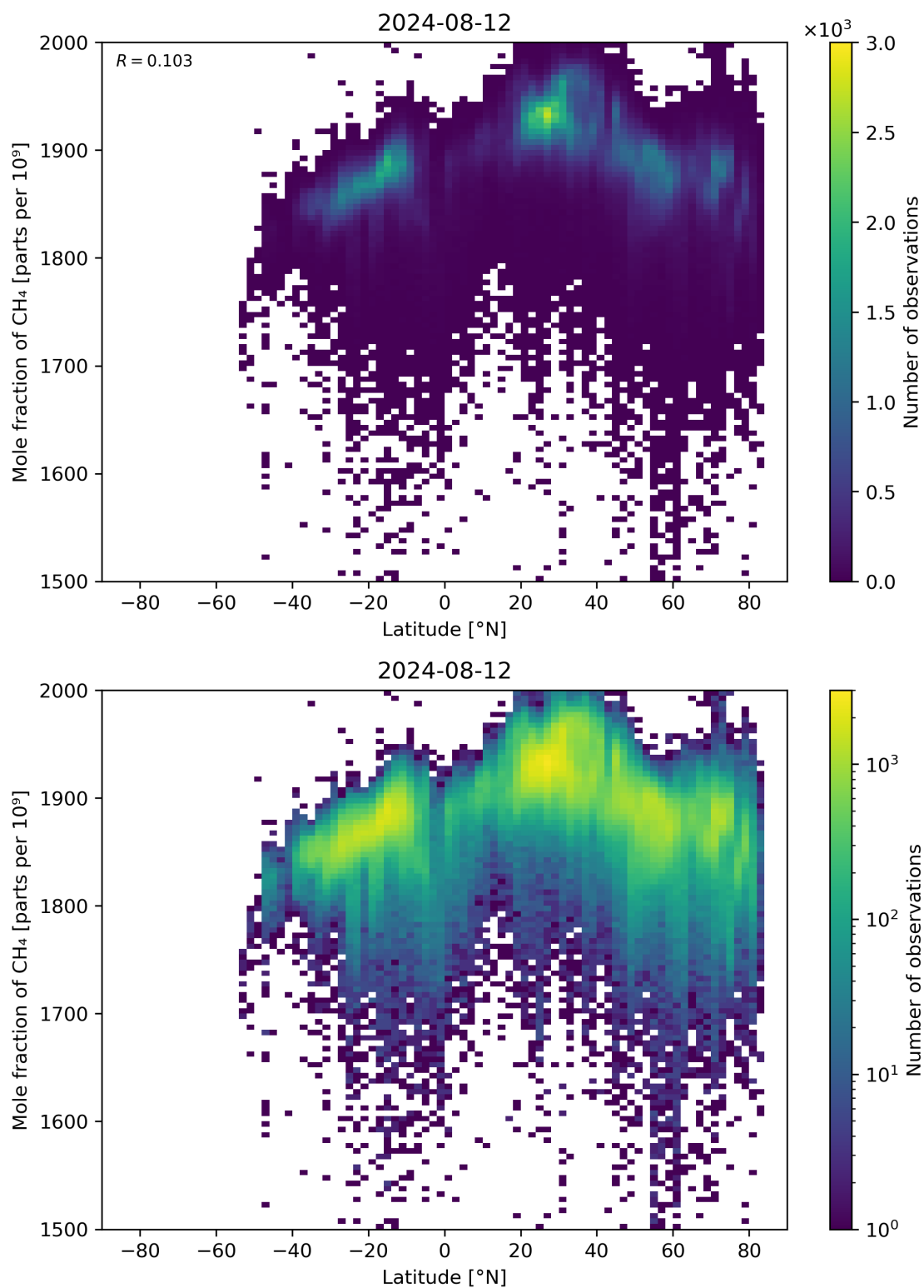
Figure 57: Scatter density plot of “Latitude” against “Mole fraction of \text{CH}_4 ” for 2024-08-12 to 2024-08-13.
