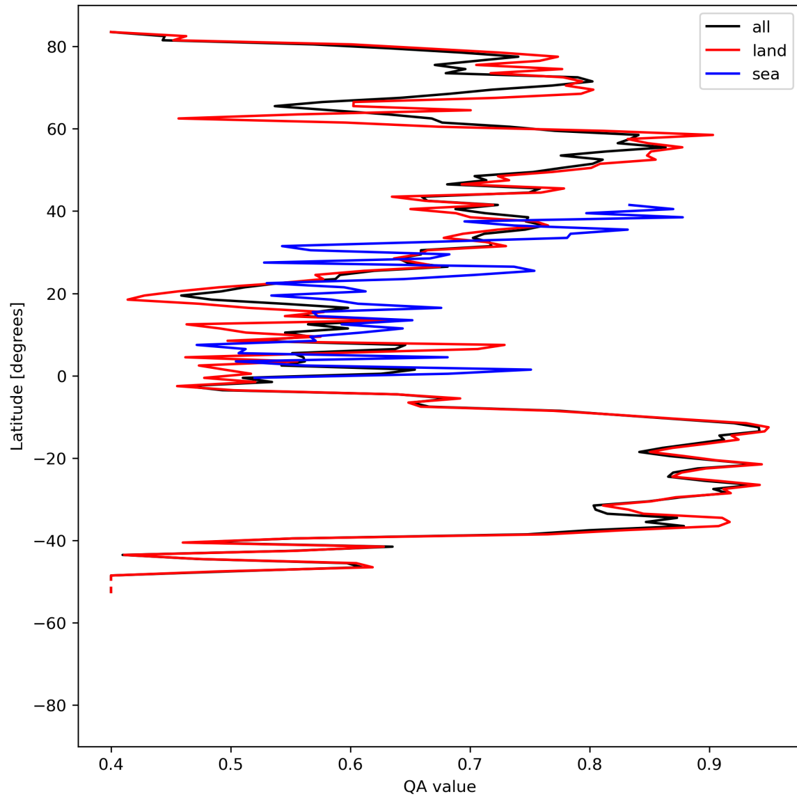
Figure 11: Zonal average of “QA value” for 2024-08-12 to 2024-08-13.
