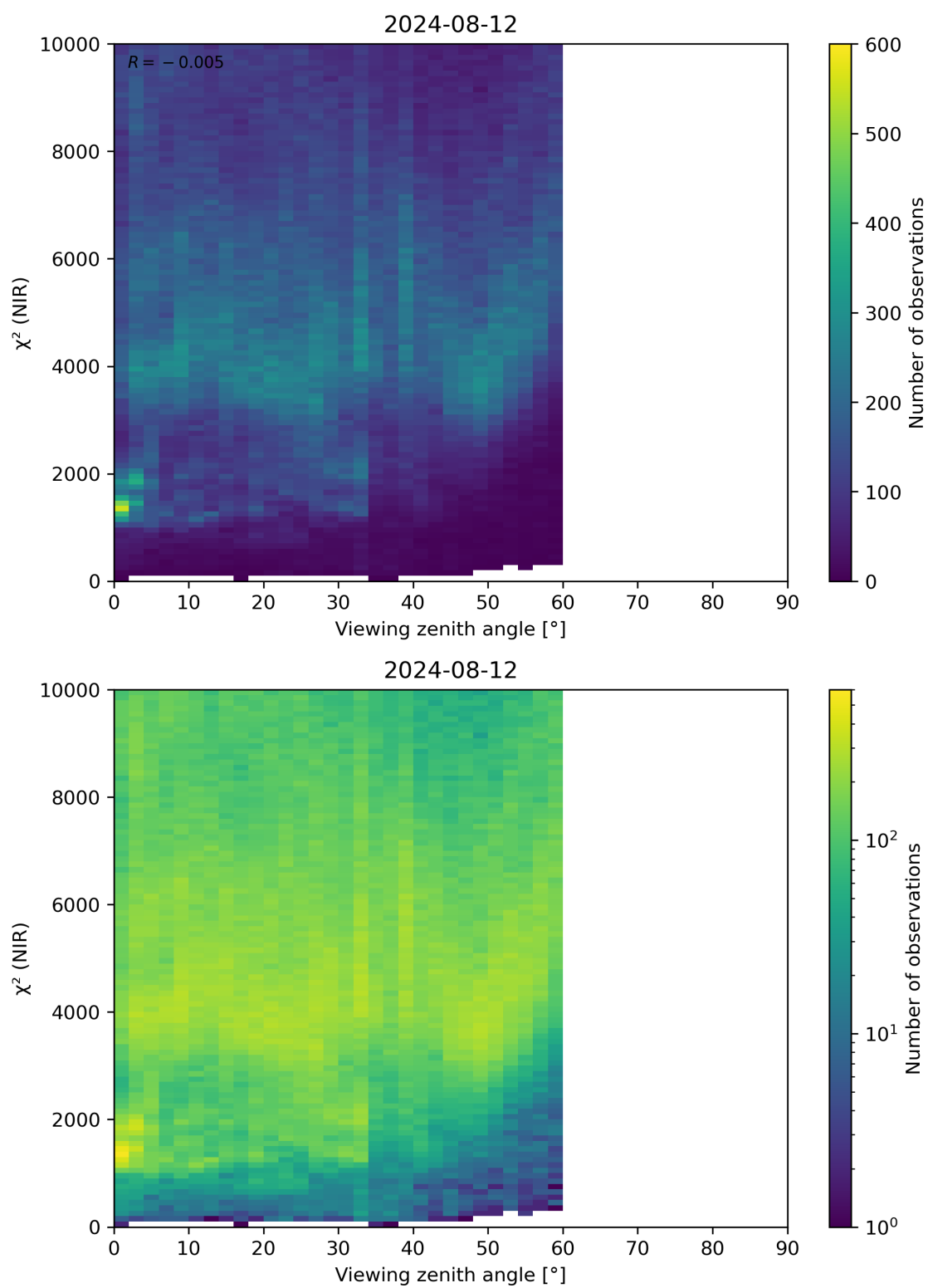
Figure 105: Scatter density plot of “Viewing zenith angle” against “ \chi^2 (NIR)” for 2024-08-12 to 2024-08-13.
