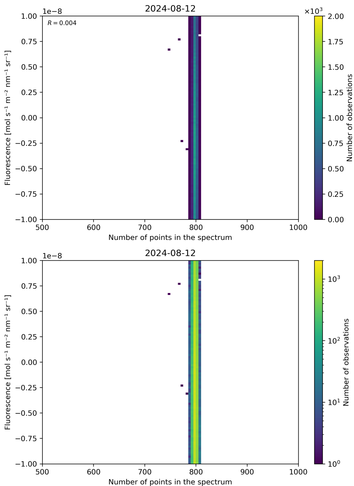
Figure 91: Scatter density plot of “Number of points in the spectrum” against “Fluorescence” for 2024-08-12 to 2024-08-13.
