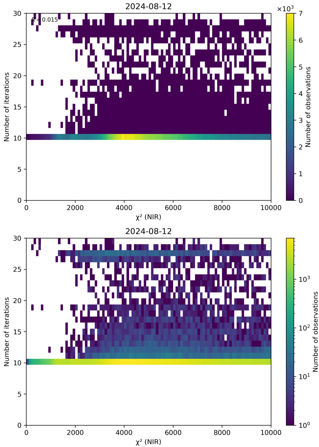
Figure 46: Scatter density plot of “ \chi^2 (NIR)” against “Number of iterations” for 2024-08-12 to 2024-08-13.
