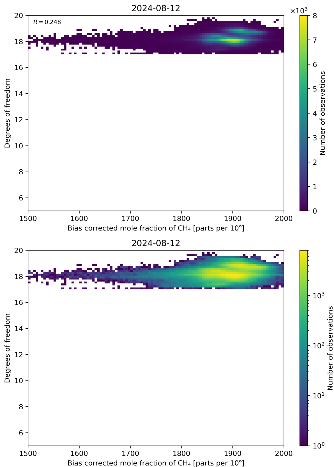
Figure 65: Scatter density plot of “Bias corrected mole fraction of CH 4 ” against “Degrees of freedom” for 2024-08-12 to 2024-08-13.
