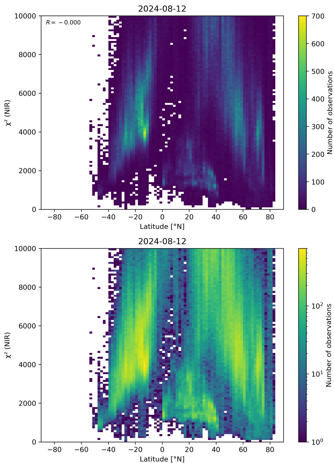
Figure 53: Scatter density plot of “Latitude” against “ \chi^2 (NIR)” for 2024-08-12 to 2024-08-13.
