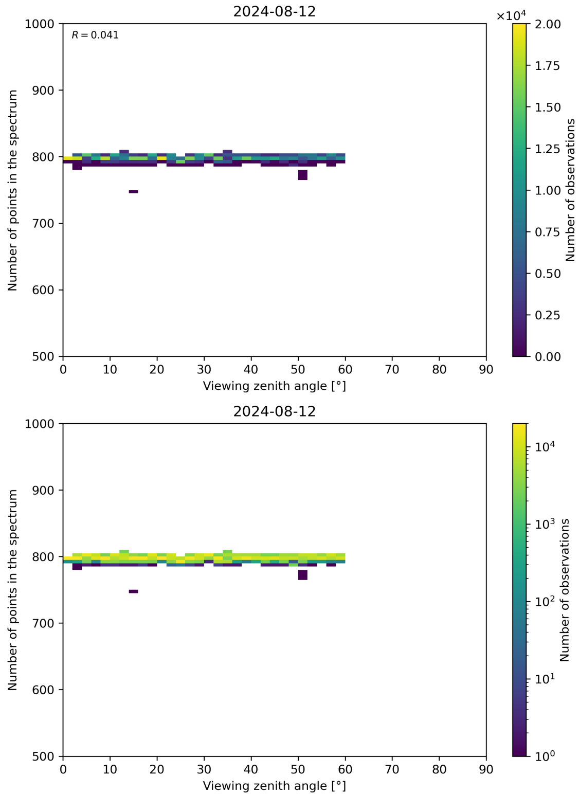
Figure 114: Scatter density plot of “Viewing zenith angle” against “Number of points in the spectrum” for 2024-08-12 to 2024-08-13.
