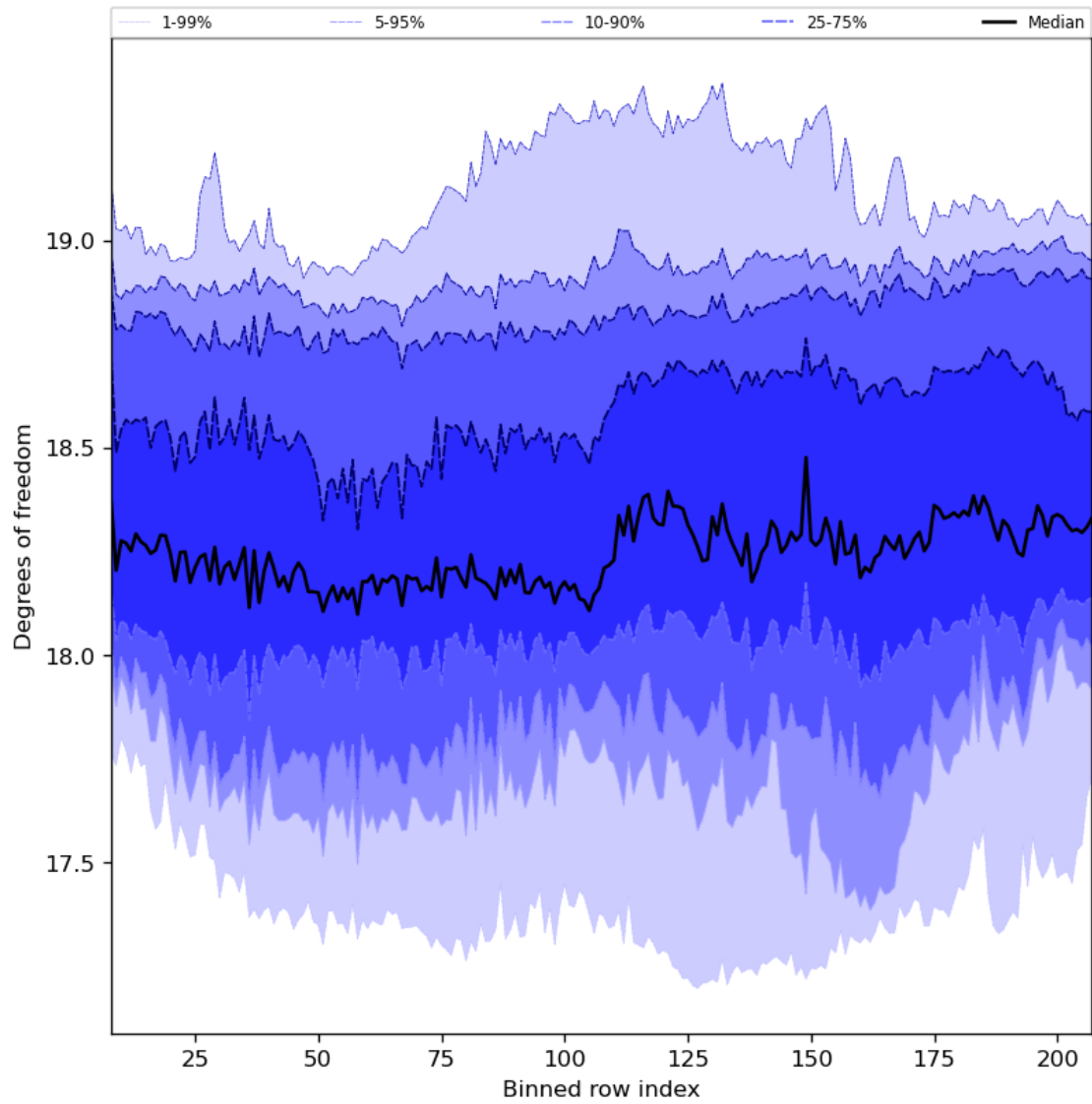
Figure 41: Along track statistics of “Degrees of freedom” for 2024-08-12 to 2024-08-13
