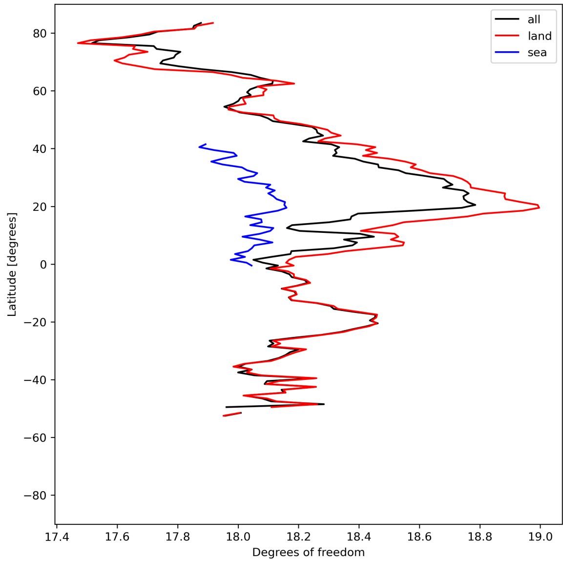
Figure 19: Zonal average of “Degrees of freedom” for 2024-08-12 to 2024-08-13.
