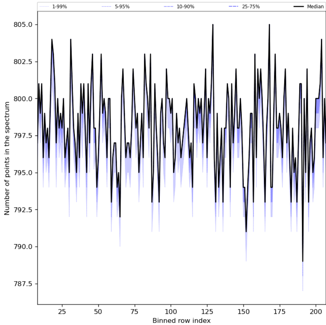
Figure 37: Along track statistics of “Number of points in the spectrum” for 2024-08-12 to 2024-08-13
