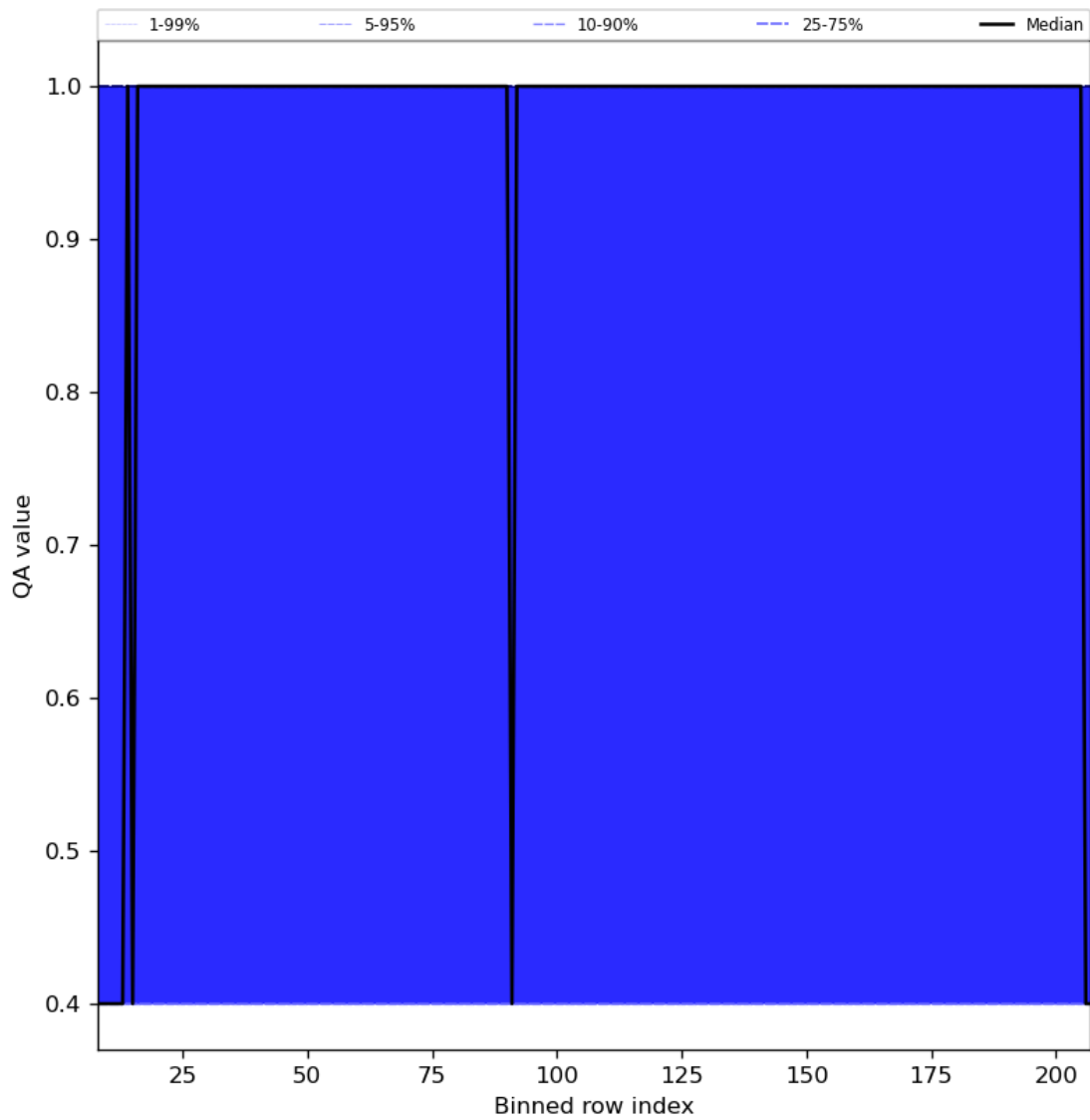
Figure 33: Along track statistics of “QA value” for 2024-08-12 to 2024-08-13
