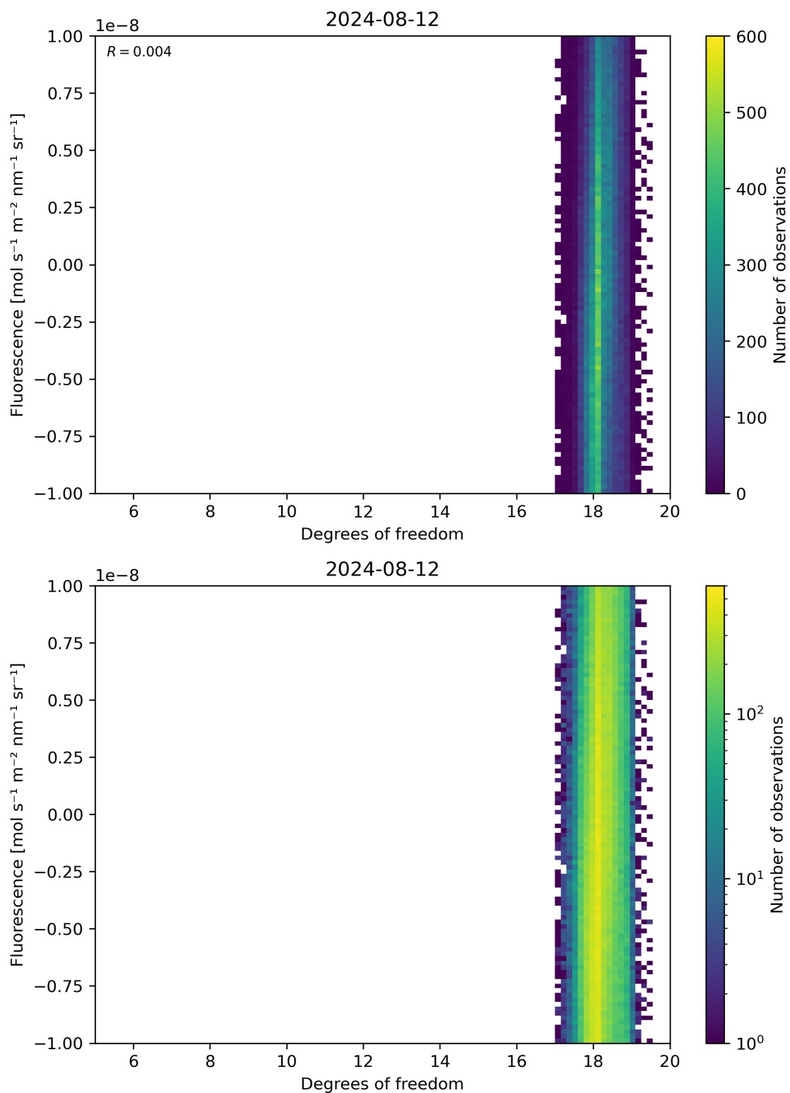
Figure 51: Scatter density plot of “Degrees of freedom” against “Fluorescence” for 2024-08-12 to 2024-08-13.
