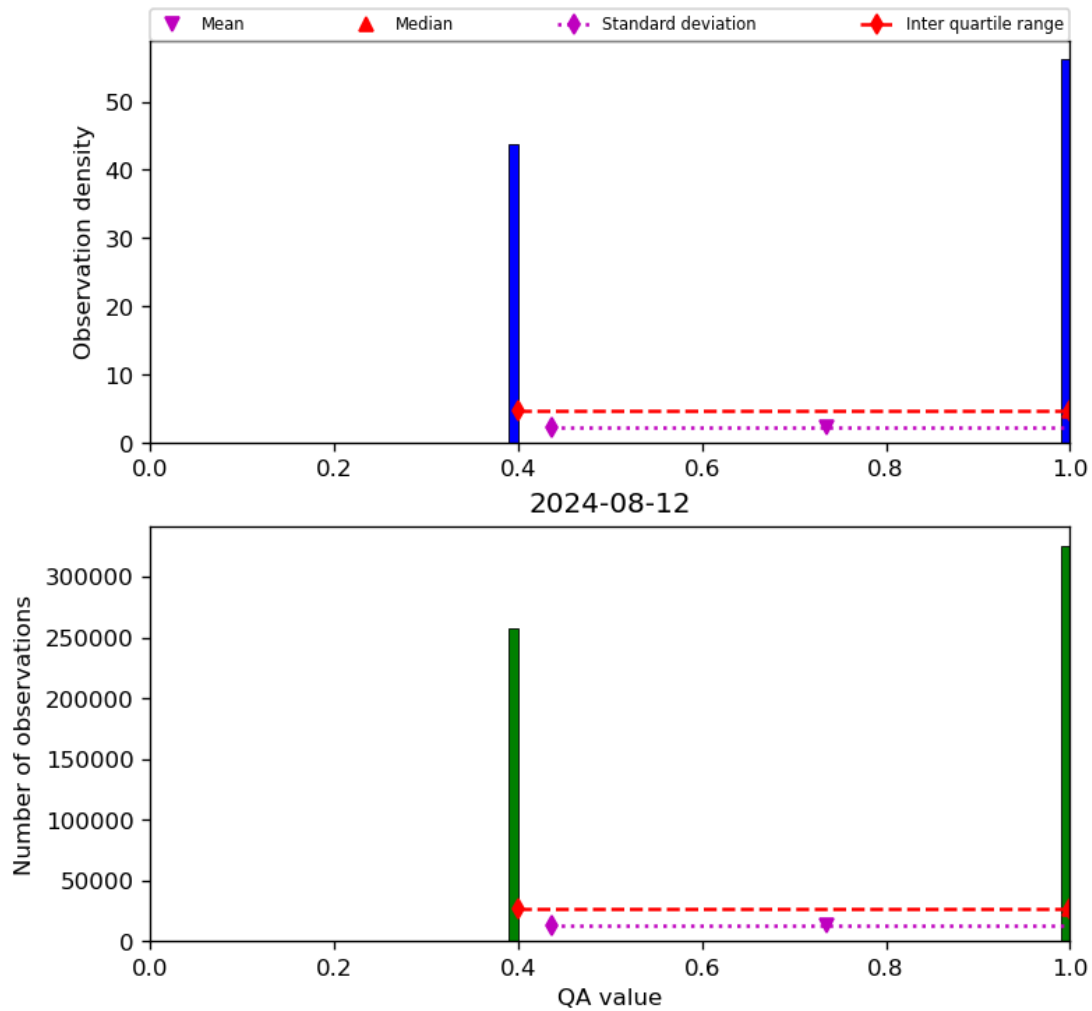
Figure 22: Histogram of “QA value” for 2024-08-12 to 2024-08-13
