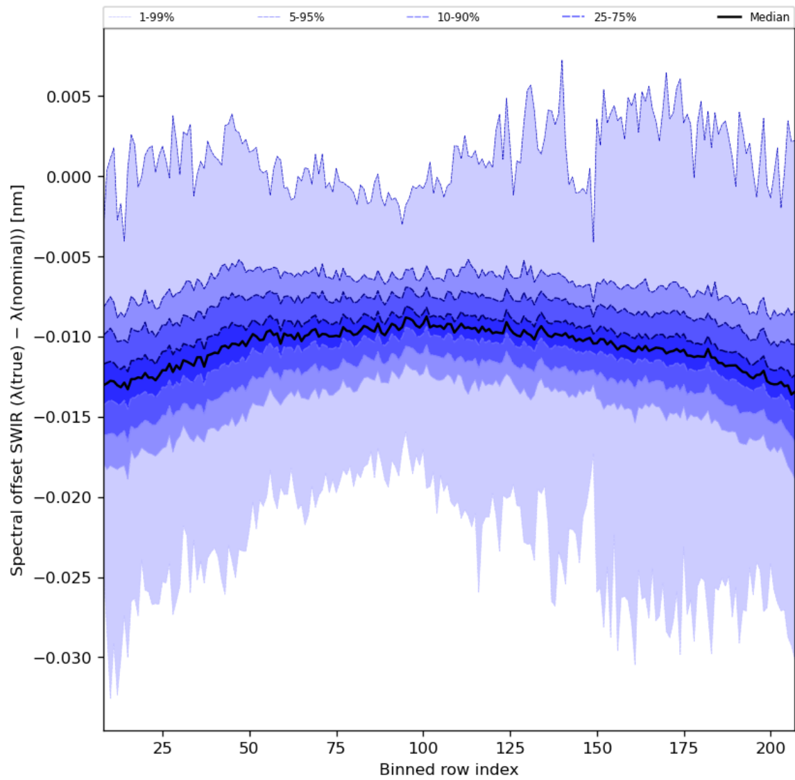
Figure 38: Along track statistics of “Spectral offset SWIR ( \lambda(\text{true}) - \lambda(\text{nominal}) )” for 2024-08-12 to 2024-08-13
