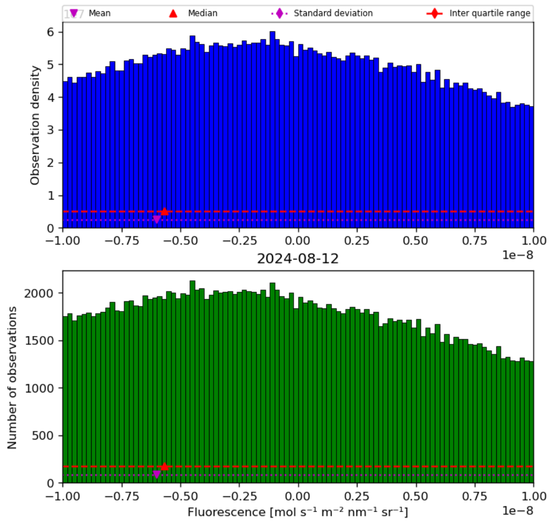
Figure 32: Histogram of “Fluorescence” for 2024-08-12 to 2024-08-13
