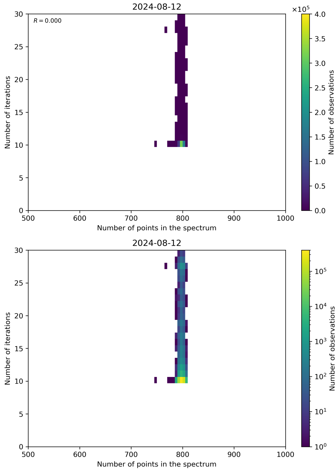
Figure 92: Scatter density plot of “Number of points in the spectrum” against “Number of iterations” for 2024-08-12 to 2024-08-13.
