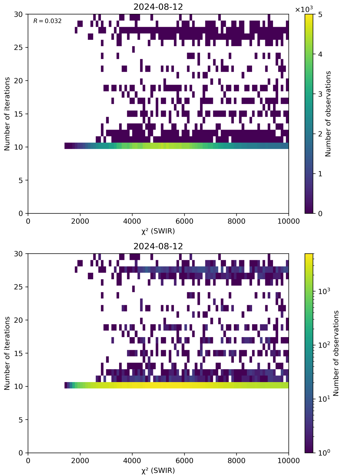
Figure 50: Scatter density plot of “ \chi^2 (SWIR)” against “Number of iterations” for 2024-08-12 to 2024-08-13.
