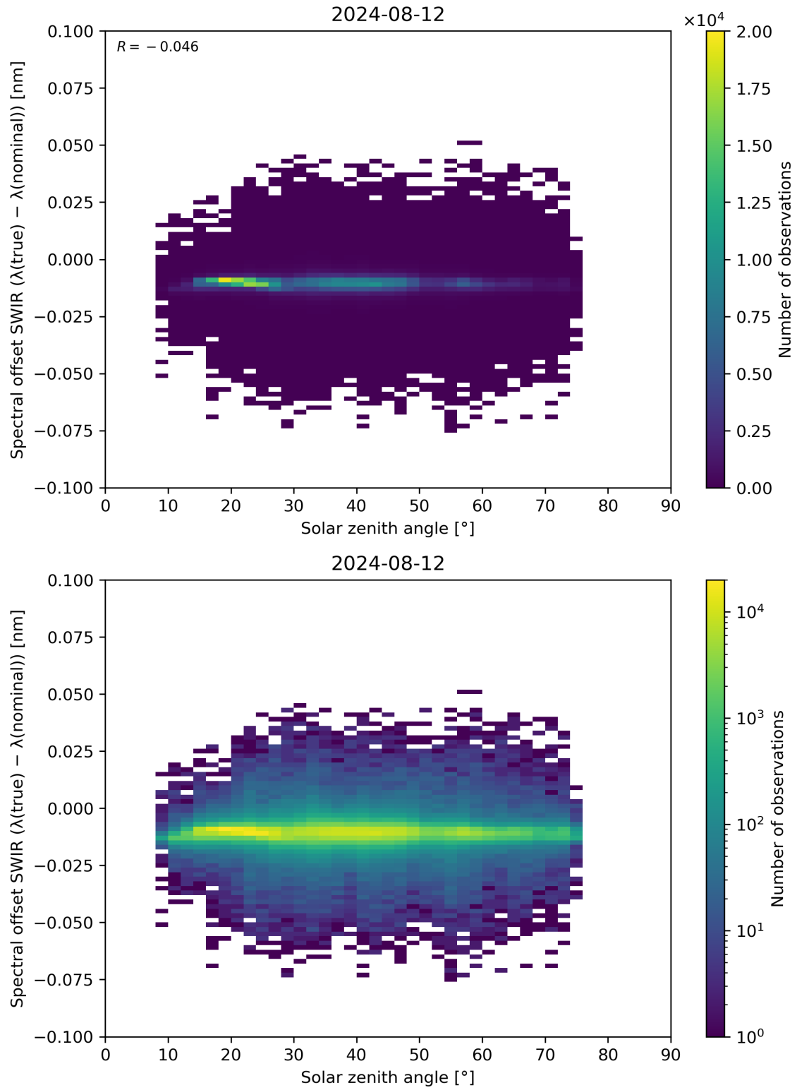
Figure 104: Scatter density plot of “Solar zenith angle” against “Spectral offset SWIR ( \lambda(\text{true}) - \lambda(\text{nominal}) )” for 2024-08-12 to 2024-08-13.
