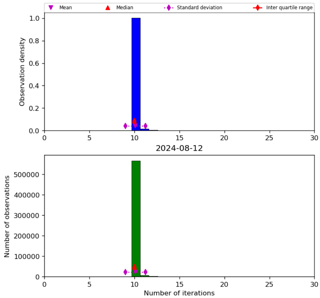
Figure 31: Histogram of “Number of iterations” for 2024-08-12 to 2024-08-13
