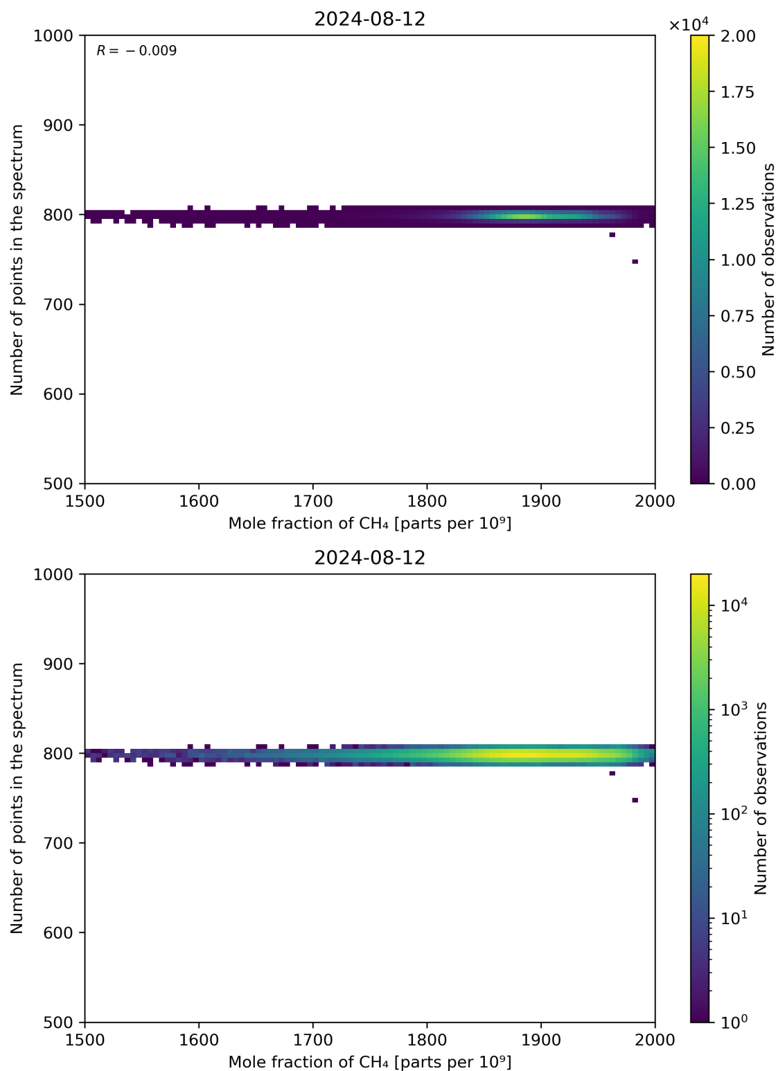
Figure 77: Scatter density plot of “Mole fraction of CH 4 ” against “Number of points in the spectrum” for 2024-08-12 to 2024-08-13.
