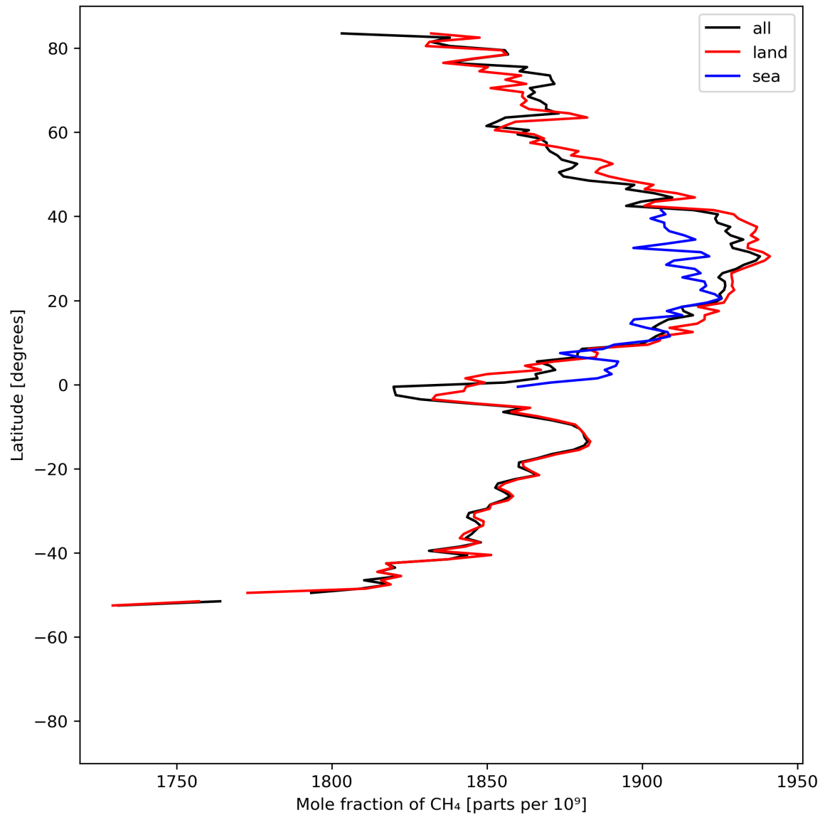
Figure 12: Zonal average of “Mole fraction of \text{CH}_4 ” for 2024-08-12 to 2024-08-13.
