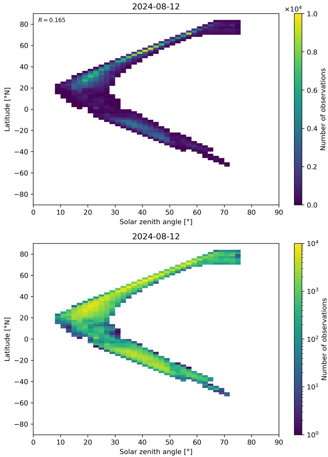
Figure 98: Scatter density plot of “Solar zenith angle” against “Latitude” for 2024-08-12 to 2024-08-13.
