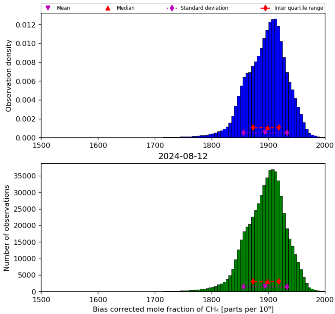
Figure 25: Histogram of “Bias corrected mole fraction of CH 4 ” for 2024-08-12 to 2024-08-13
