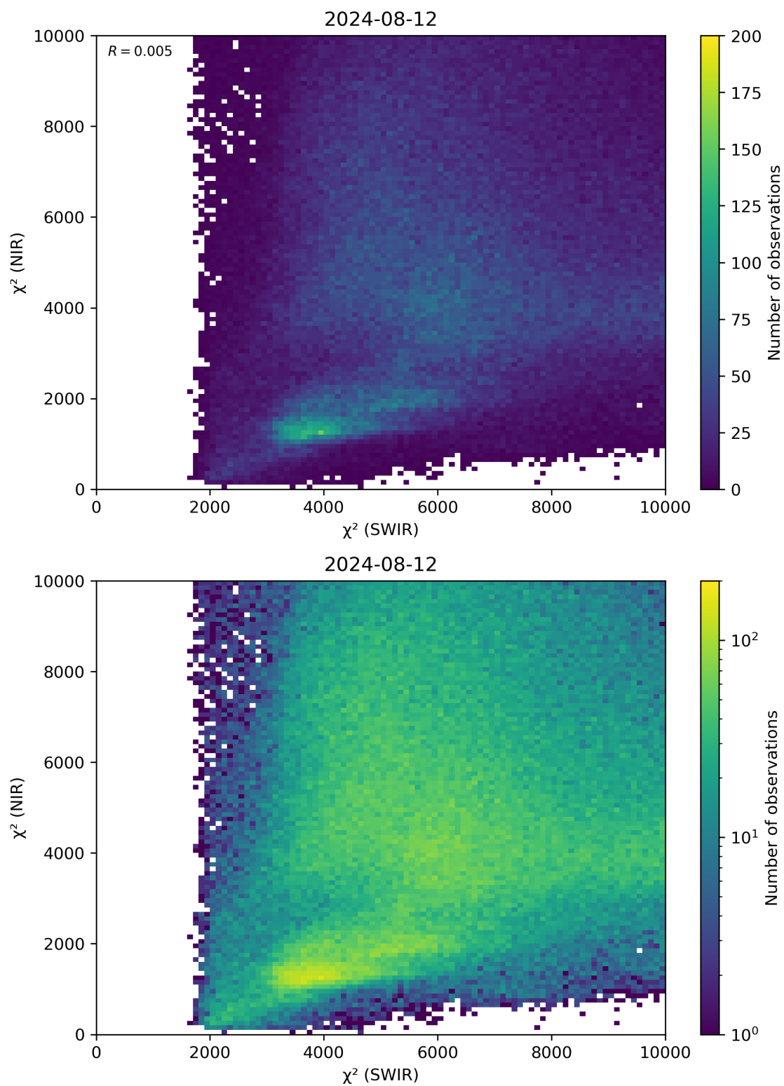
Figure 47: Scatter density plot of “ \chi^2 (SWIR)” against “ \chi^2 (NIR)” for 2024-08-12 to 2024-08-13.
