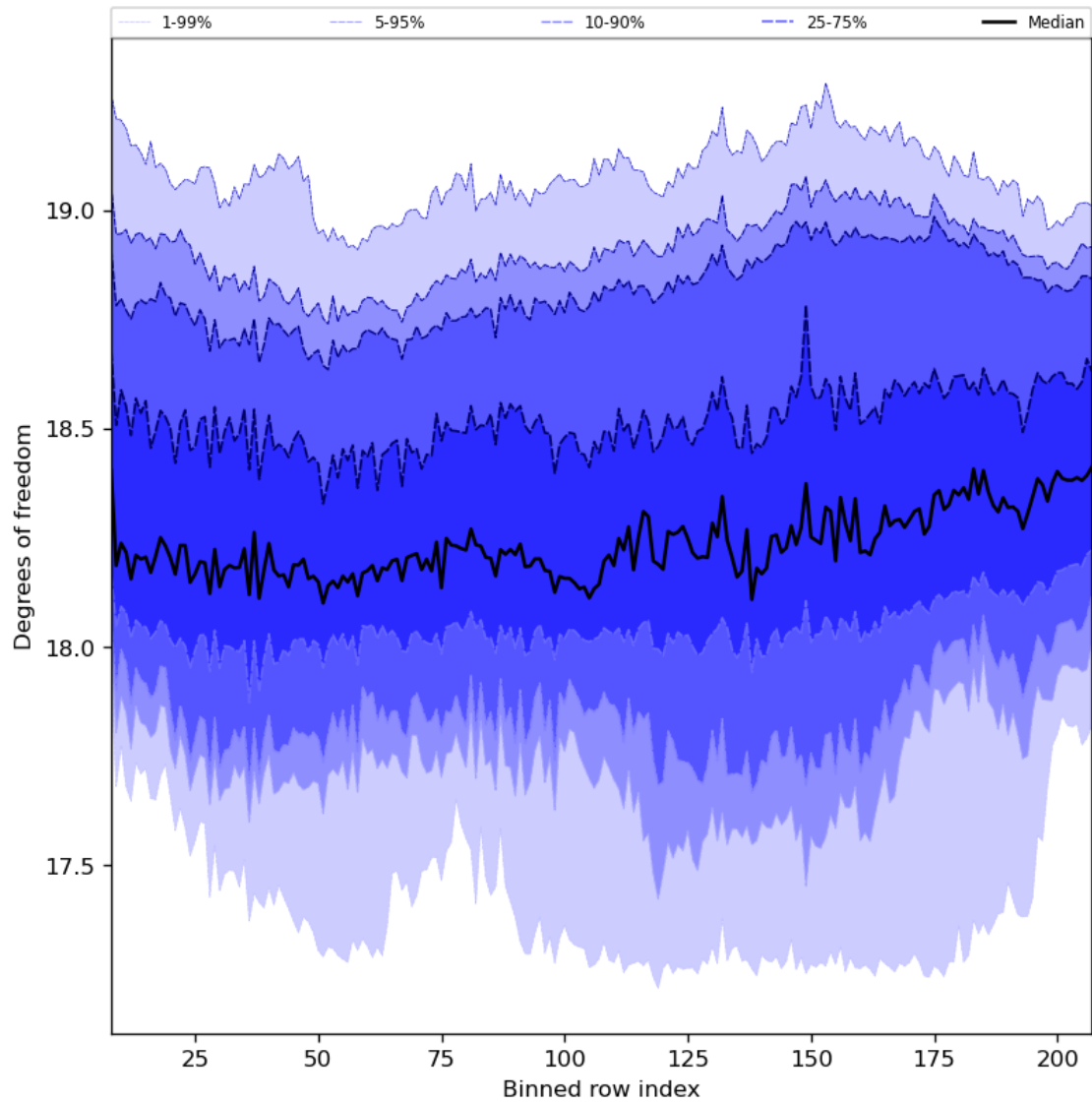
Figure 41: Along track statistics of “Degrees of freedom” for 2024-08-12 to 2024-08-14
