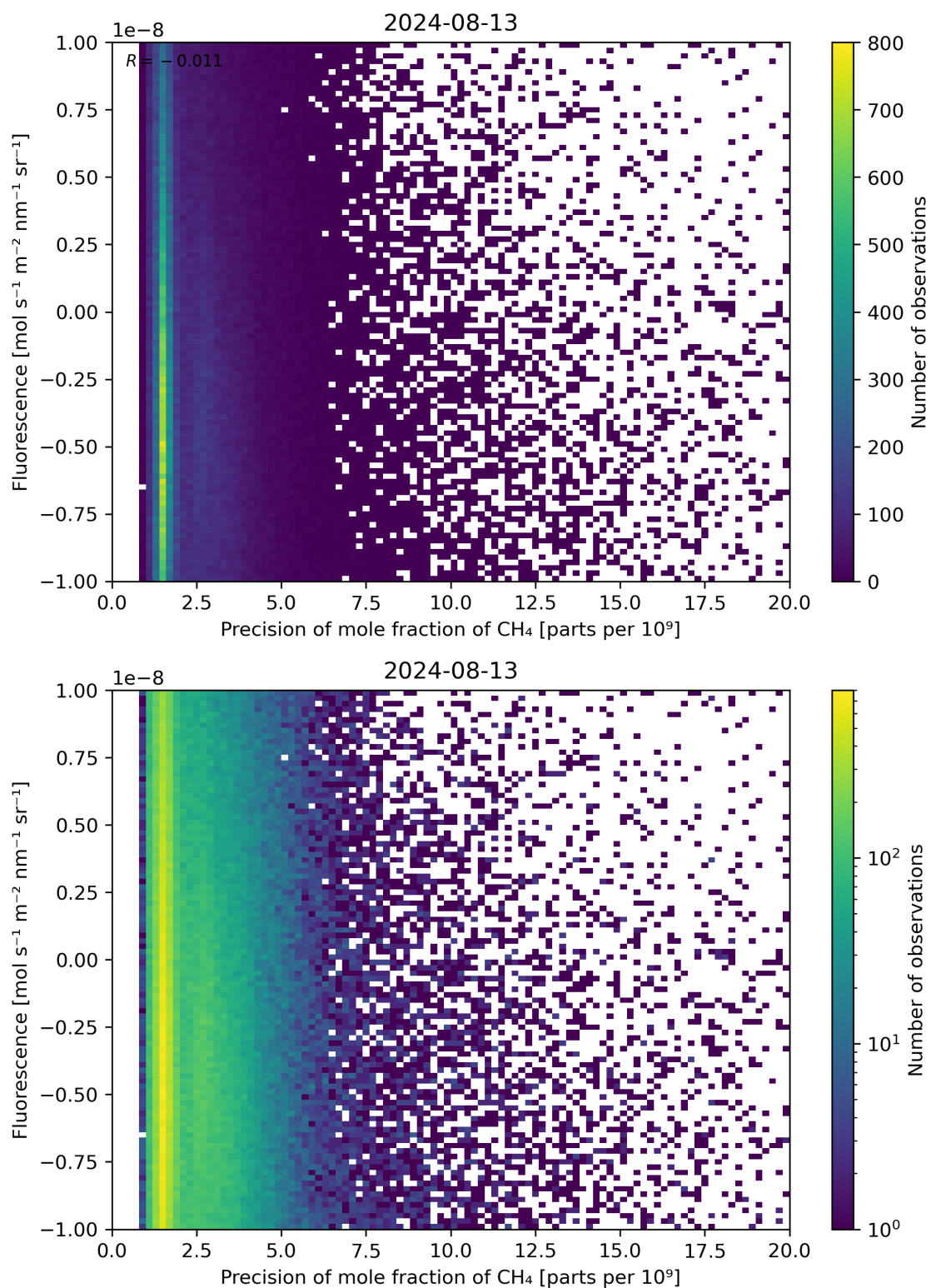
Figure 81: Scatter density plot of “Precision of mole fraction of \text{CH}_4 ” against “Fluorescence” for 2024-08-12 to 2024-08-14.
