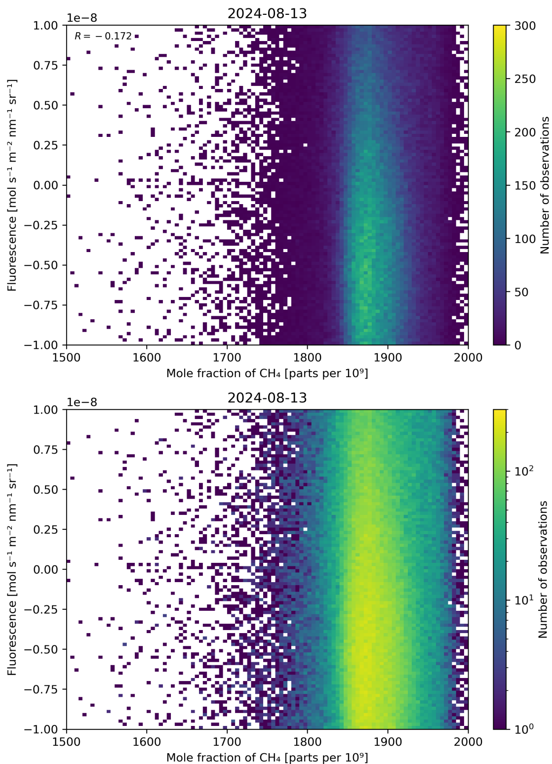
Figure 73: Scatter density plot of “Mole fraction of \text{CH}_4 ” against “Fluorescence” for 2024-08-12 to 2024-08-14.
