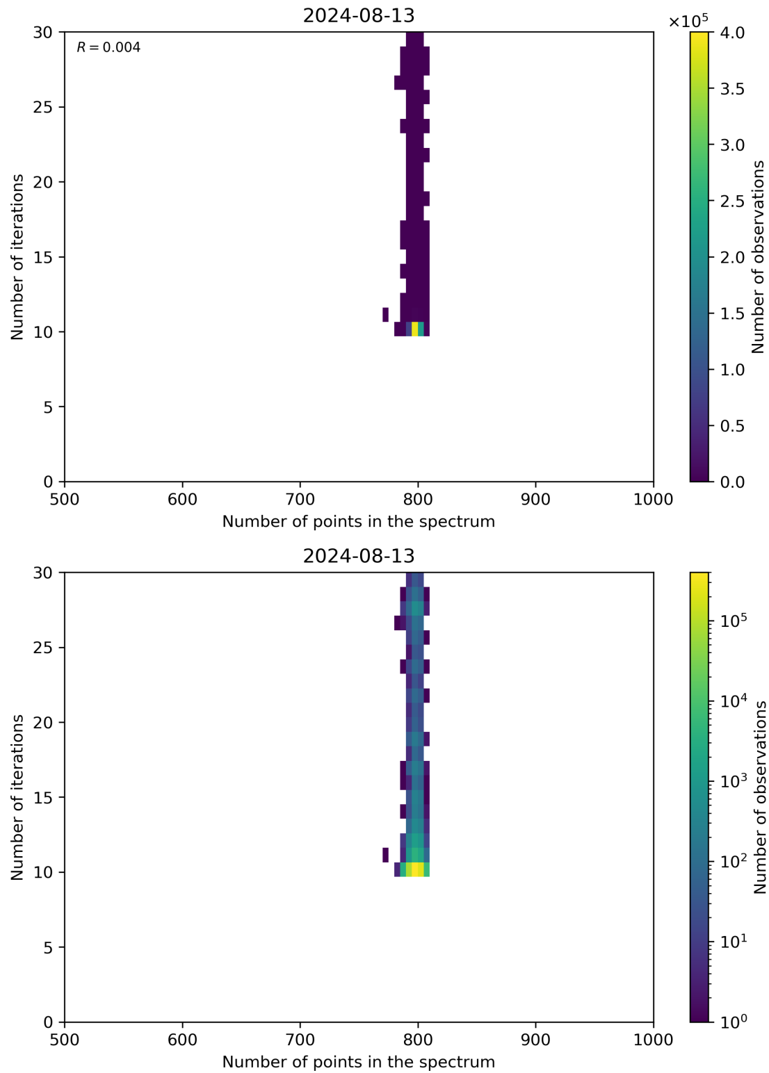
Figure 92: Scatter density plot of “Number of points in the spectrum” against “Number of iterations” for 2024-08-12 to 2024-08-14.
