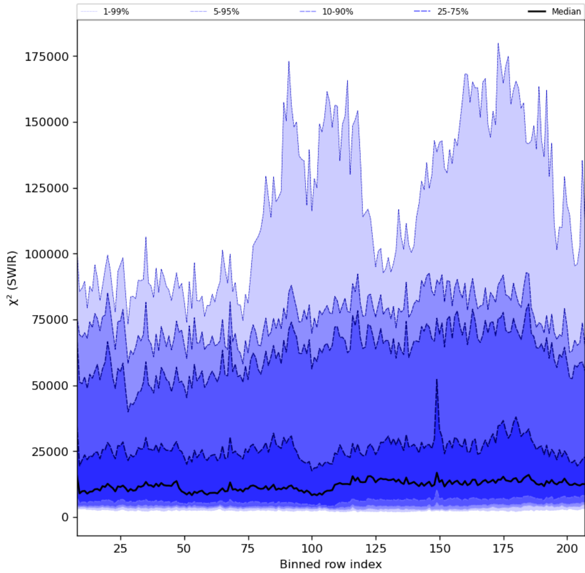
Figure 39: Along track statistics of “ \chi^2 (SWIR)” for 2024-08-12 to 2024-08-14
