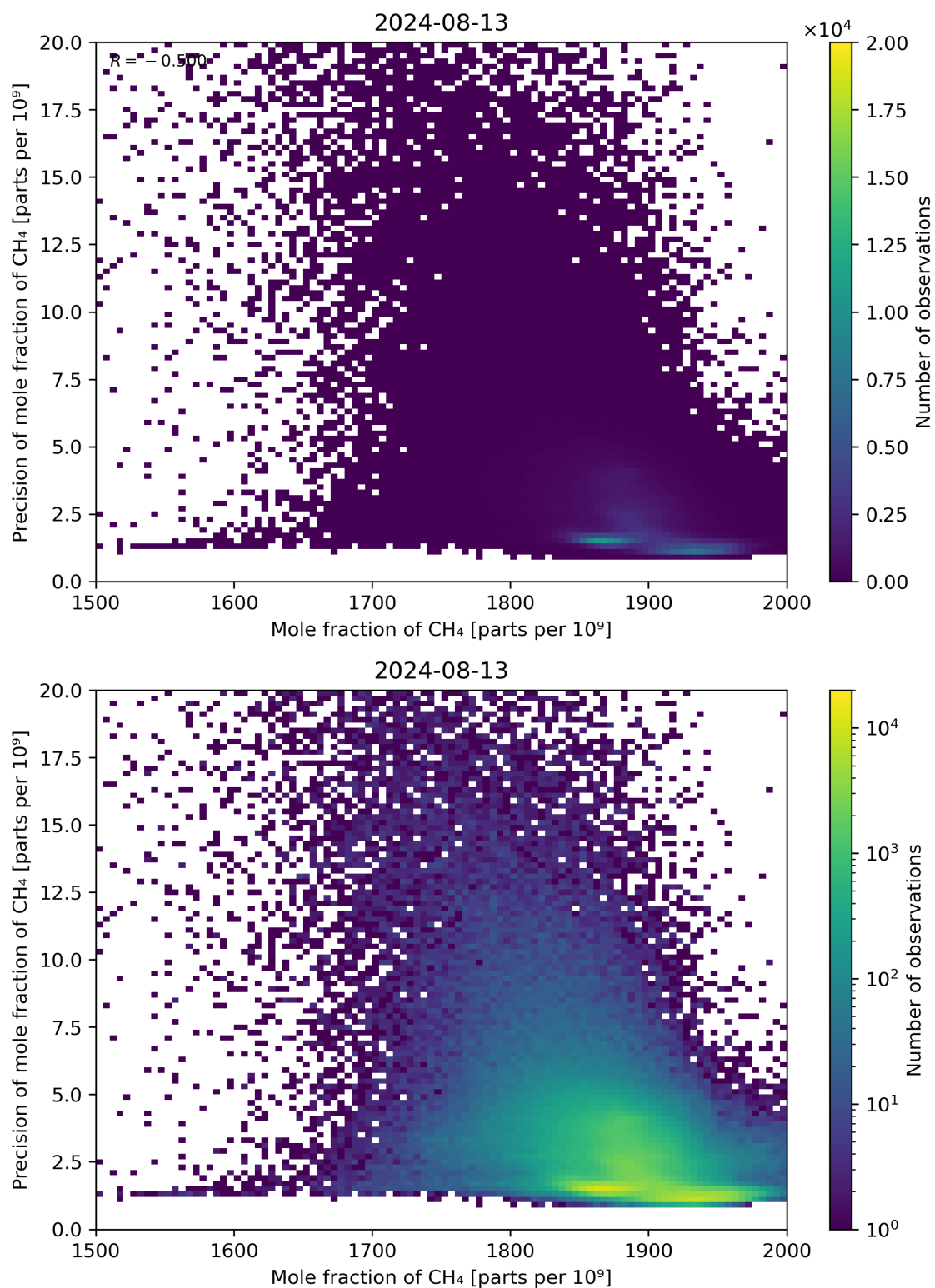
Figure 75: Scatter density plot of “Mole fraction of CH 4 ” against “Precision of mole fraction of CH 4 ” for 2024-08-12 to 2024-08-14.
