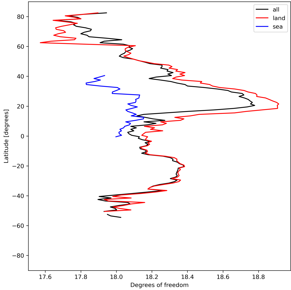
Figure 19: Zonal average of “Degrees of freedom” for 2024-08-12 to 2024-08-14.
