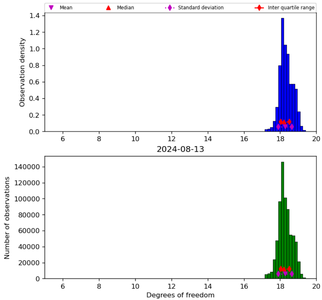
Figure 30: Histogram of “Degrees of freedom” for 2024-08-12 to 2024-08-14
