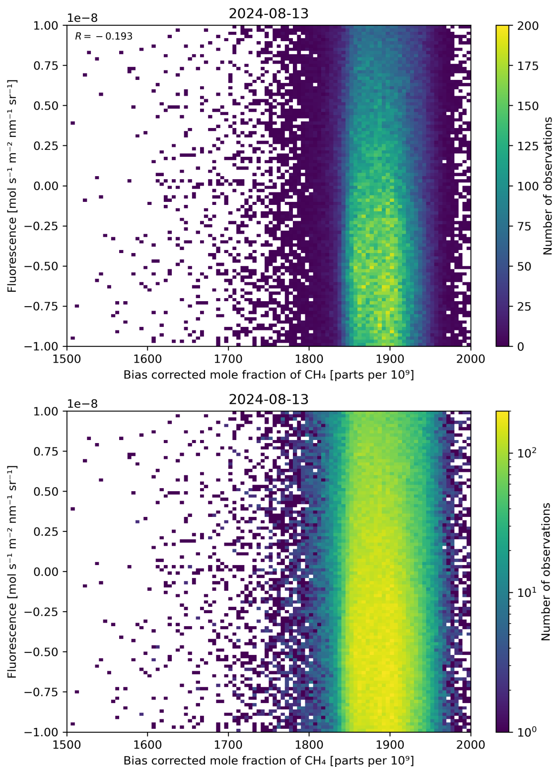
Figure 66: Scatter density plot of “Bias corrected mole fraction of \text{CH}_4 ” against “Fluorescence” for 2024-08-12 to 2024-08-14.
