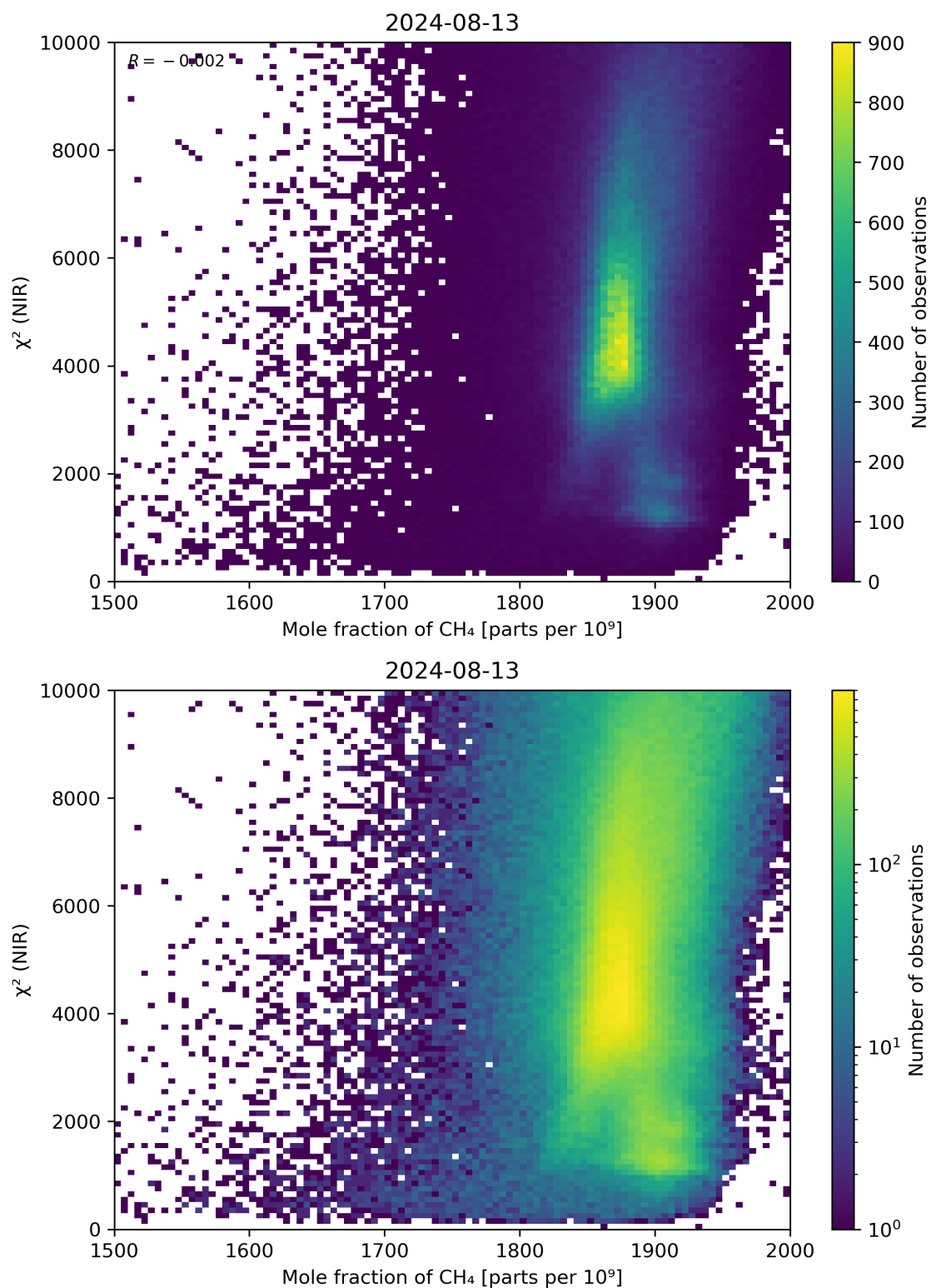
Figure 70: Scatter density plot of “Mole fraction of CH 4 ” against “ \chi^2 (NIR)” for 2024-08-12 to 2024-08-14.
