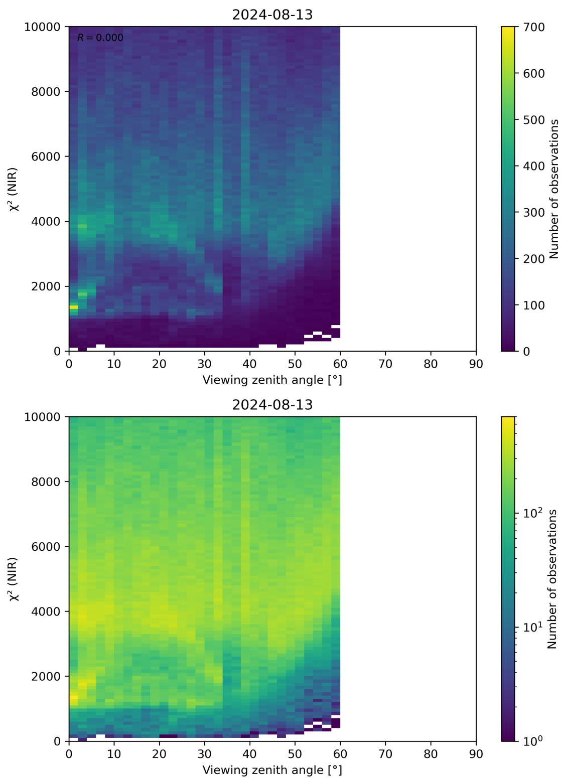
Figure 105: Scatter density plot of “Viewing zenith angle” against “ \chi^2 (NIR)” for 2024-08-12 to 2024-08-14.
