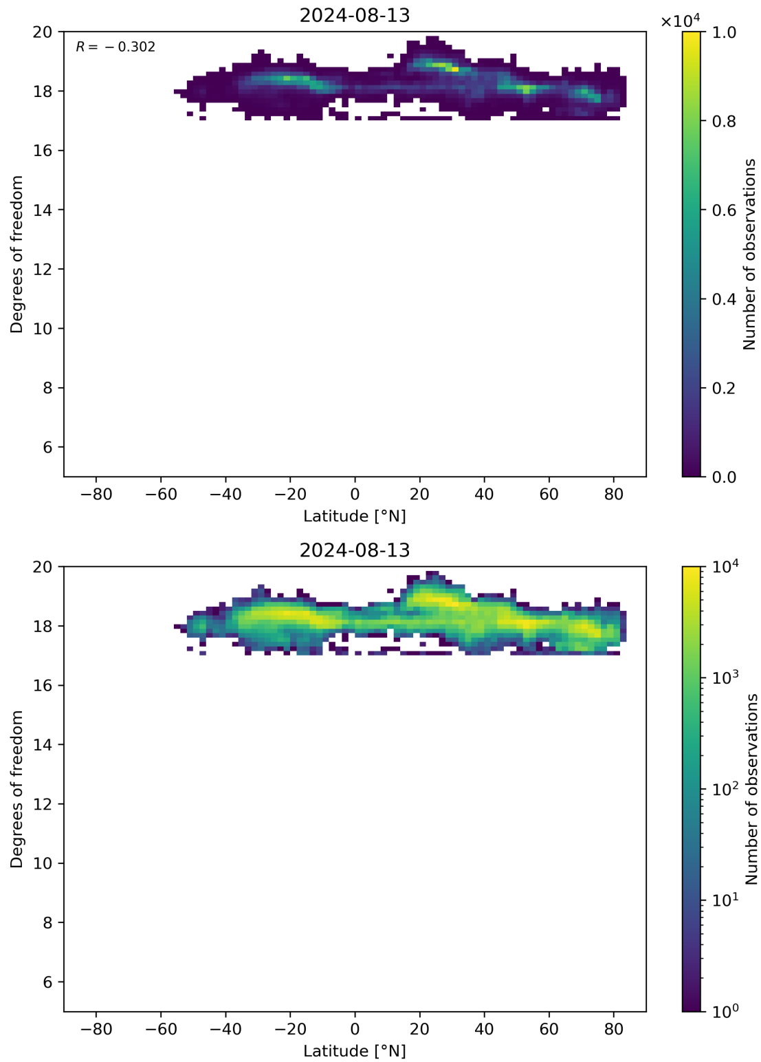
Figure 55: Scatter density plot of “Latitude” against “Degrees of freedom” for 2024-08-12 to 2024-08-14.
