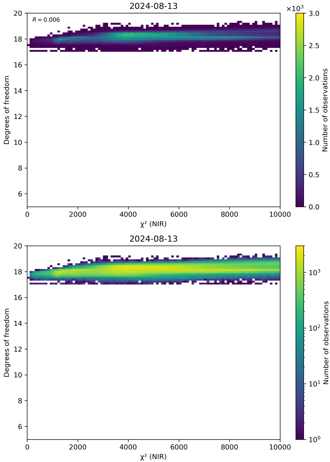
Figure 44: Scatter density plot of “ \chi^2 (NIR)” against “Degrees of freedom” for 2024-08-12 to 2024-08-14.
