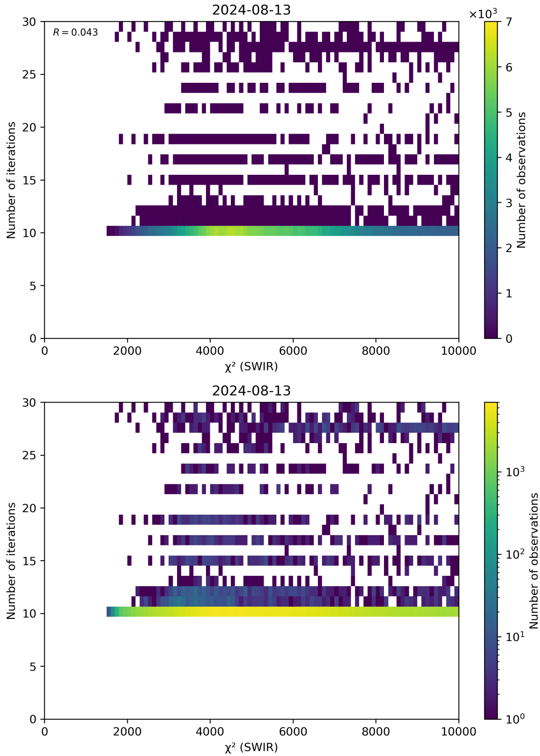
Figure 50: Scatter density plot of “ \chi^2 (SWIR)” against “Number of iterations” for 2024-08-12 to 2024-08-14.
