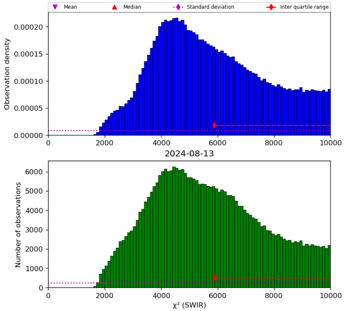
Figure 28: Histogram of “ \chi^2 (SWIR)” for 2024-08-12 to 2024-08-14
