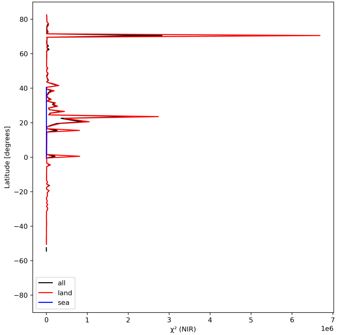
Figure 18: Zonal average of “ \chi^2 (NIR)” for 2024-08-12 to 2024-08-14.
