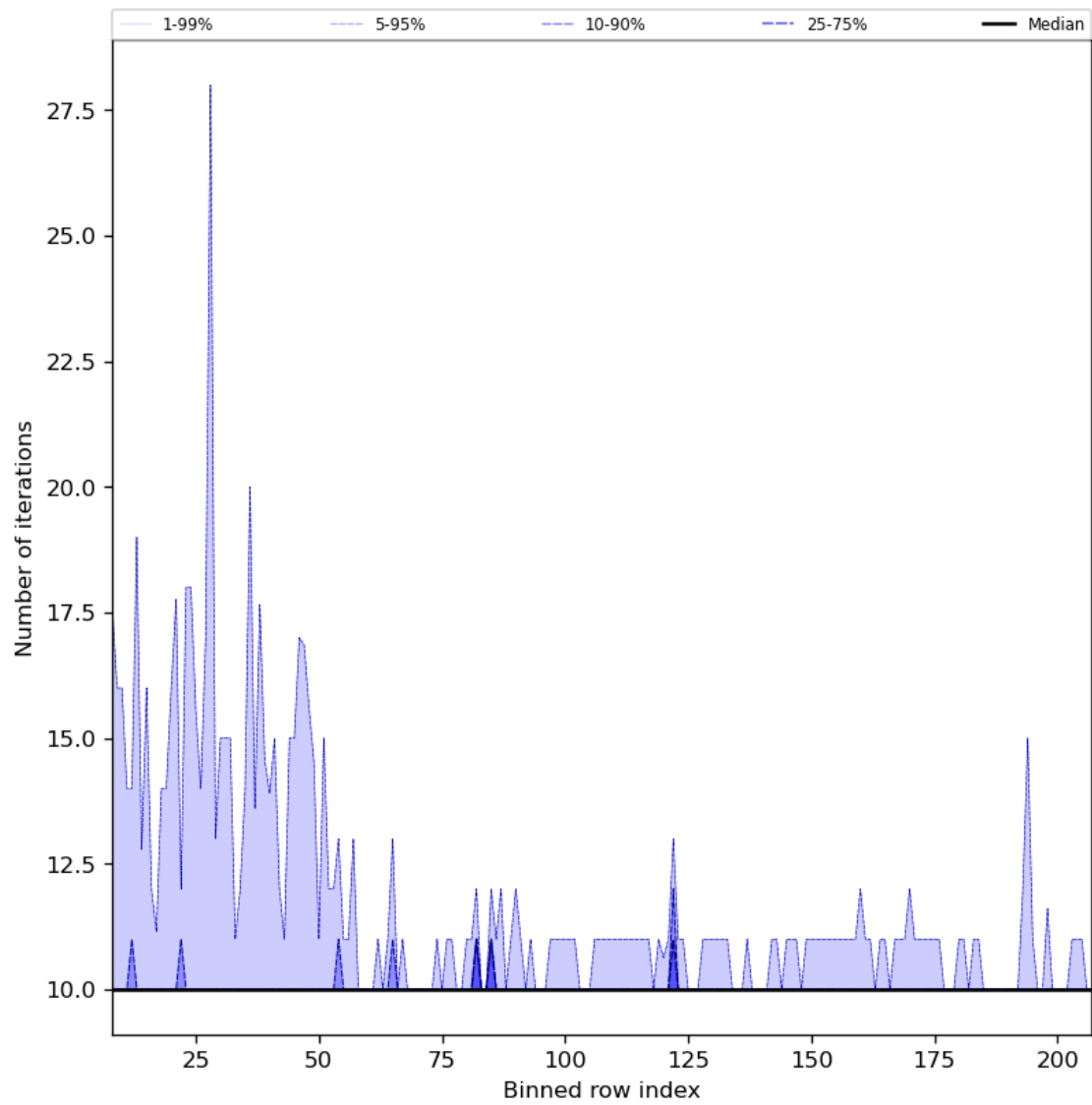
Figure 42: Along track statistics of “Number of iterations” for 2024-08-12 to 2024-08-14
