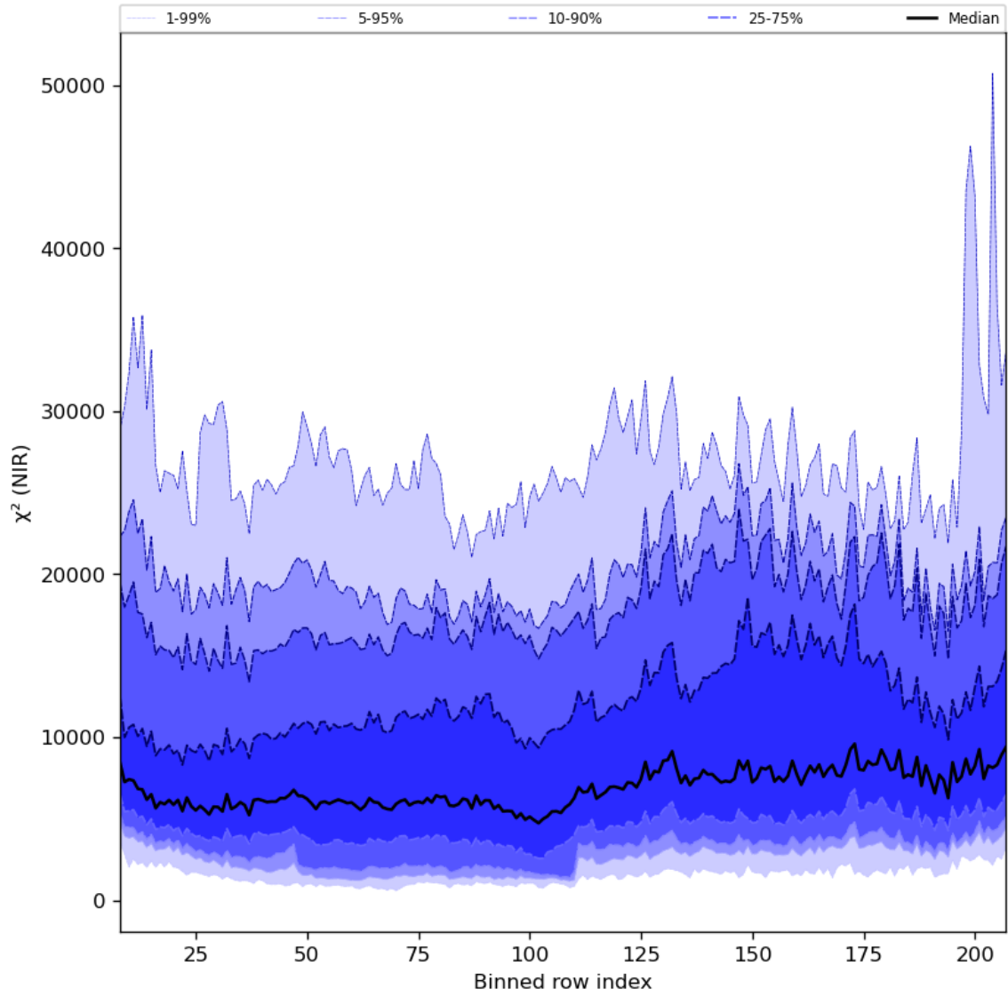
Figure 40: Along track statistics of “ \chi^2 (NIR)” for 2024-08-12 to 2024-08-14
