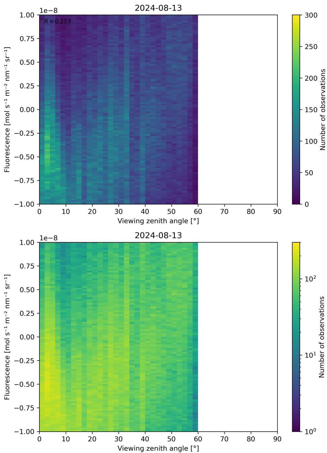
Figure 108: Scatter density plot of “Viewing zenith angle” against “Fluorescence” for 2024-08-12 to 2024-08-14.
