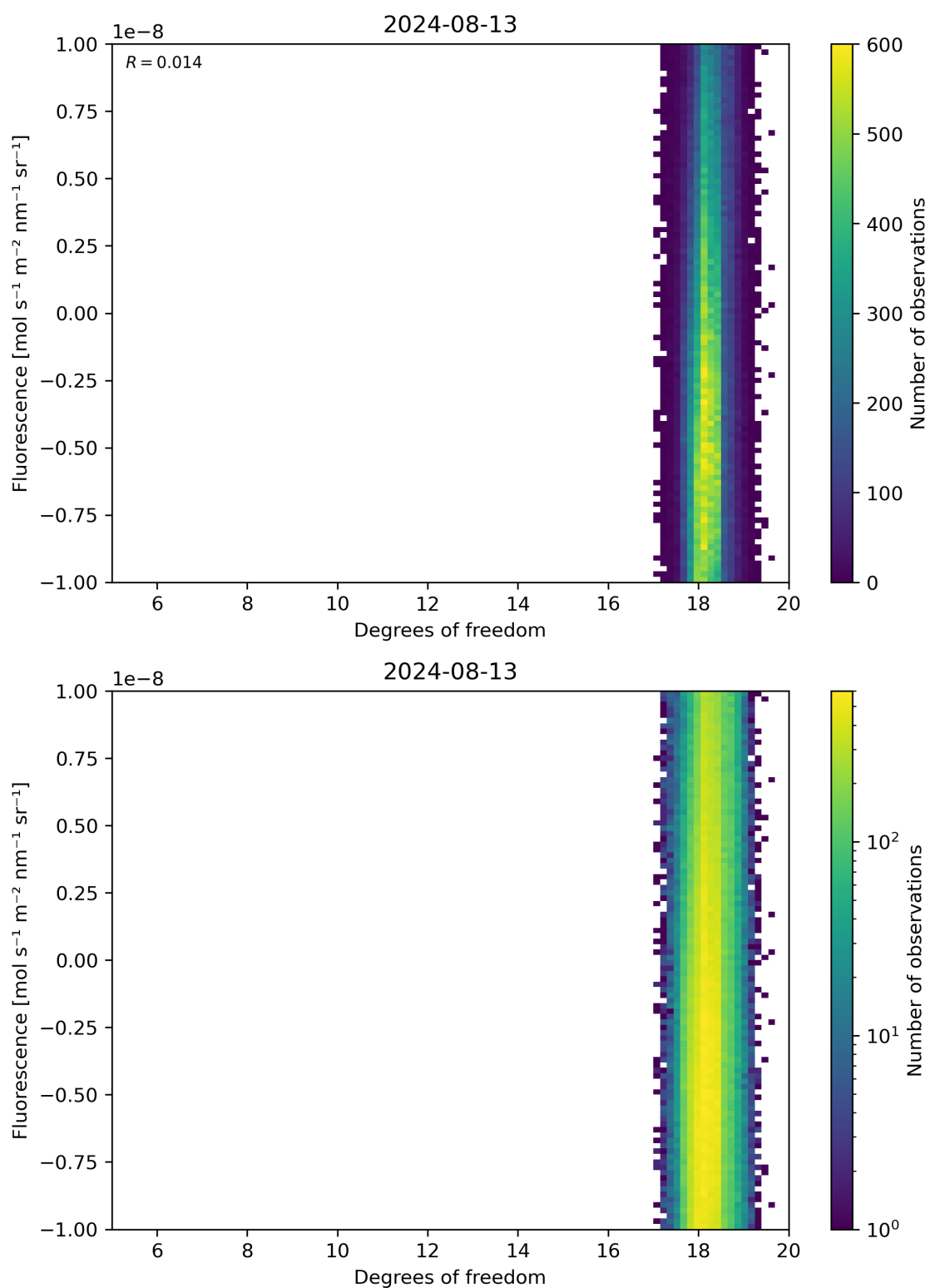
Figure 51: Scatter density plot of “Degrees of freedom” against “Fluorescence” for 2024-08-12 to 2024-08-14.
