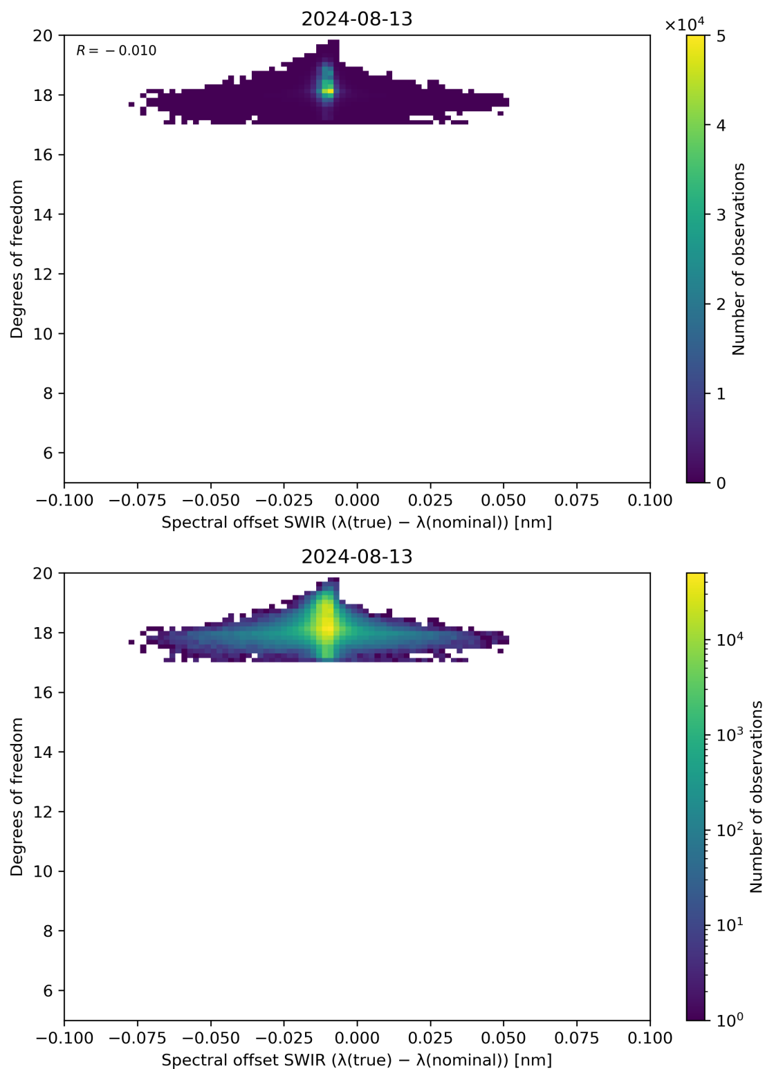
Figure 119: Scatter density plot of “Spectral offset SWIR ( \lambda(\text{true}) - \lambda(\text{nominal}) )” against “Degrees of freedom” for 2024-08-12 to 2024-08-14.
