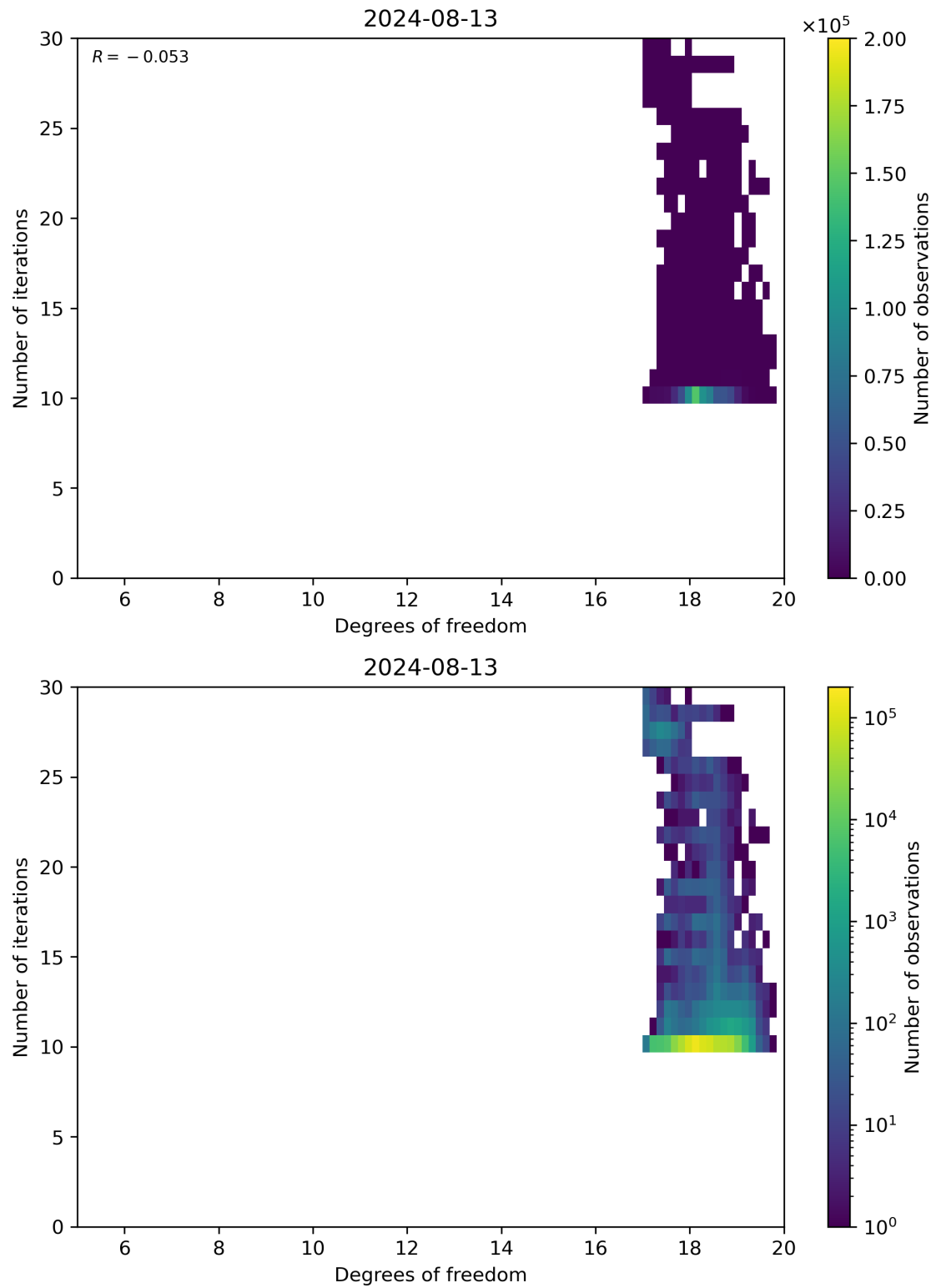
Figure 52: Scatter density plot of “Degrees of freedom” against “Number of iterations” for 2024-08-12 to 2024-08-14.
