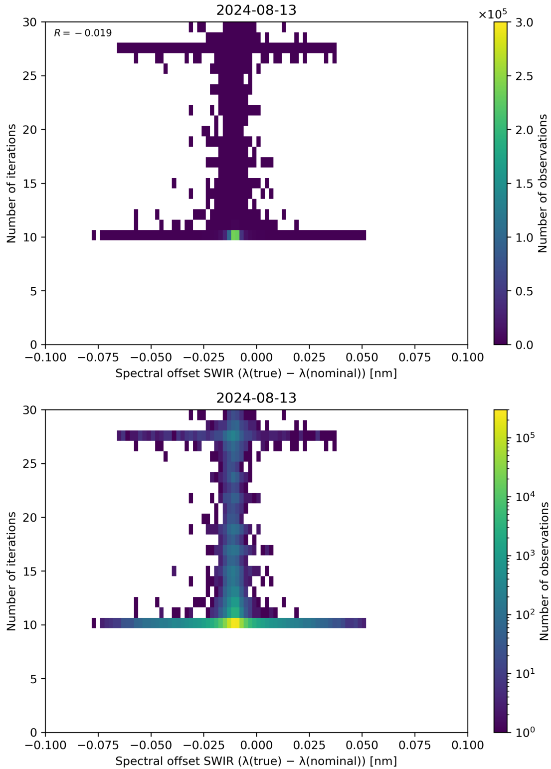
Figure 121: Scatter density plot of “Spectral offset SWIR ( \lambda(\text{true}) - \lambda(\text{nominal}) )” against “Number of iterations” for 2024-08-12 to 2024-08-14.
