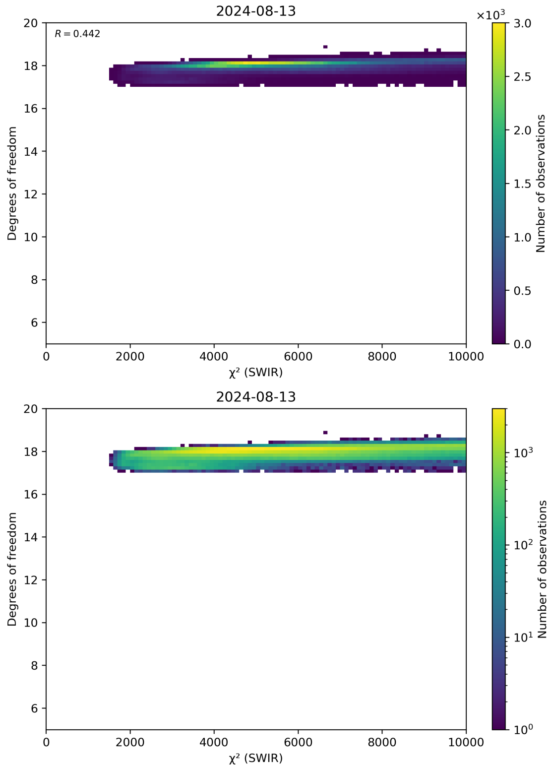
Figure 48: Scatter density plot of “ \chi^2 (SWIR)” against “Degrees of freedom” for 2024-08-12 to 2024-08-14.
