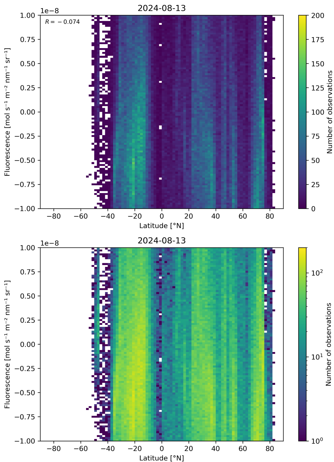
Figure 56: Scatter density plot of “Latitude” against “Fluorescence” for 2024-08-12 to 2024-08-14.
