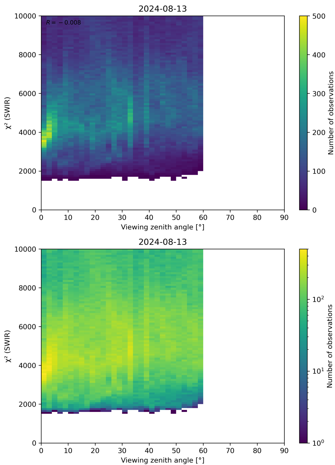
Figure 106: Scatter density plot of “Viewing zenith angle” against “ \chi^2 (SWIR)” for 2024-08-12 to 2024-08-14.
