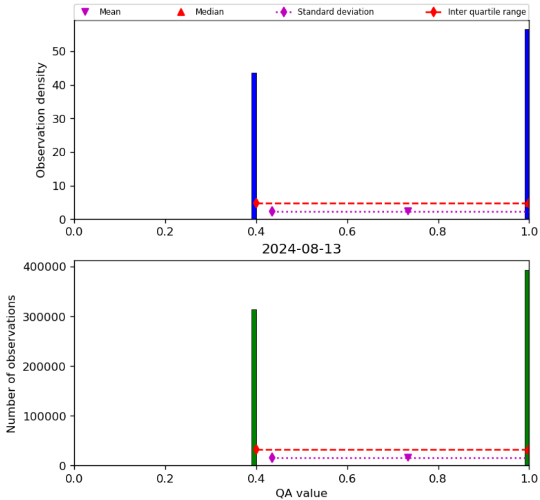
Figure 22: Histogram of “QA value” for 2024-08-12 to 2024-08-14
