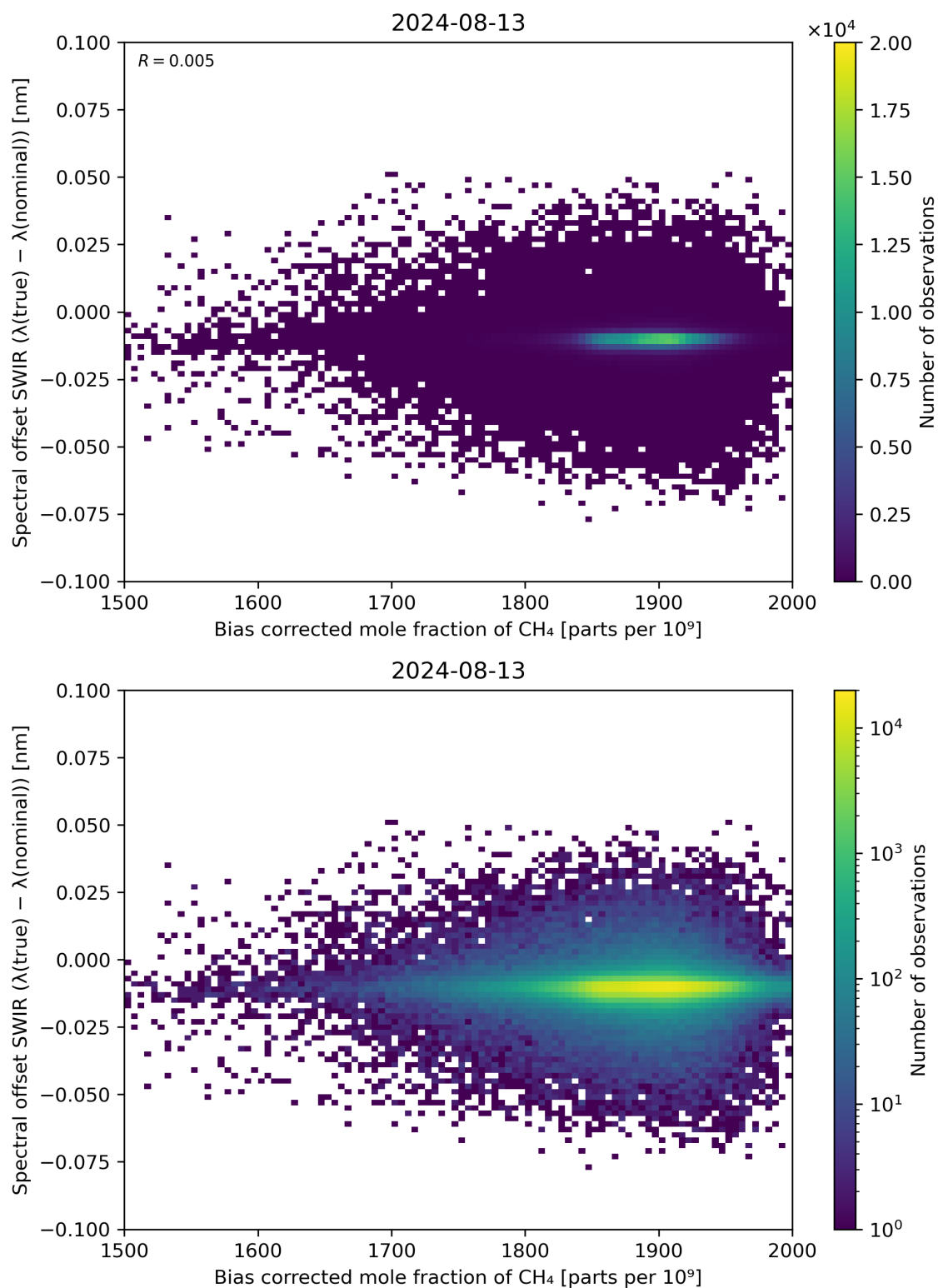
Figure 69: Scatter density plot of “Bias corrected mole fraction of \text{CH}_4 ” against “Spectral offset SWIR ( \lambda(\text{true}) - \lambda(\text{nominal}) )” for 2024-08-12 to 2024-08-14.
