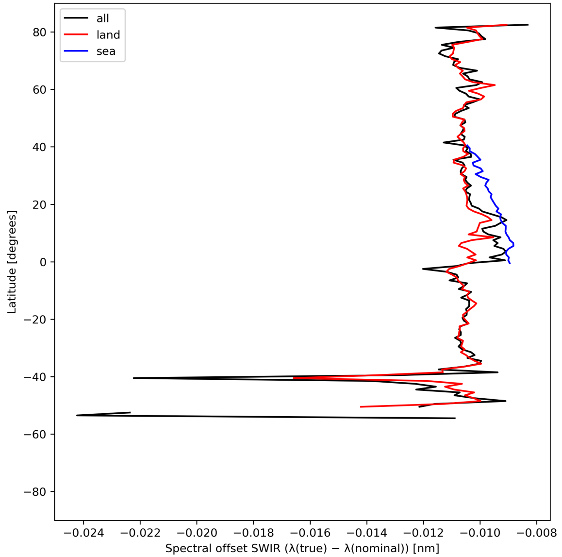
Figure 16: Zonal average of “Spectral offset SWIR ( \lambda(\text{true}) - \lambda(\text{nominal}) )” for 2024-08-12 to 2024-08-14.
