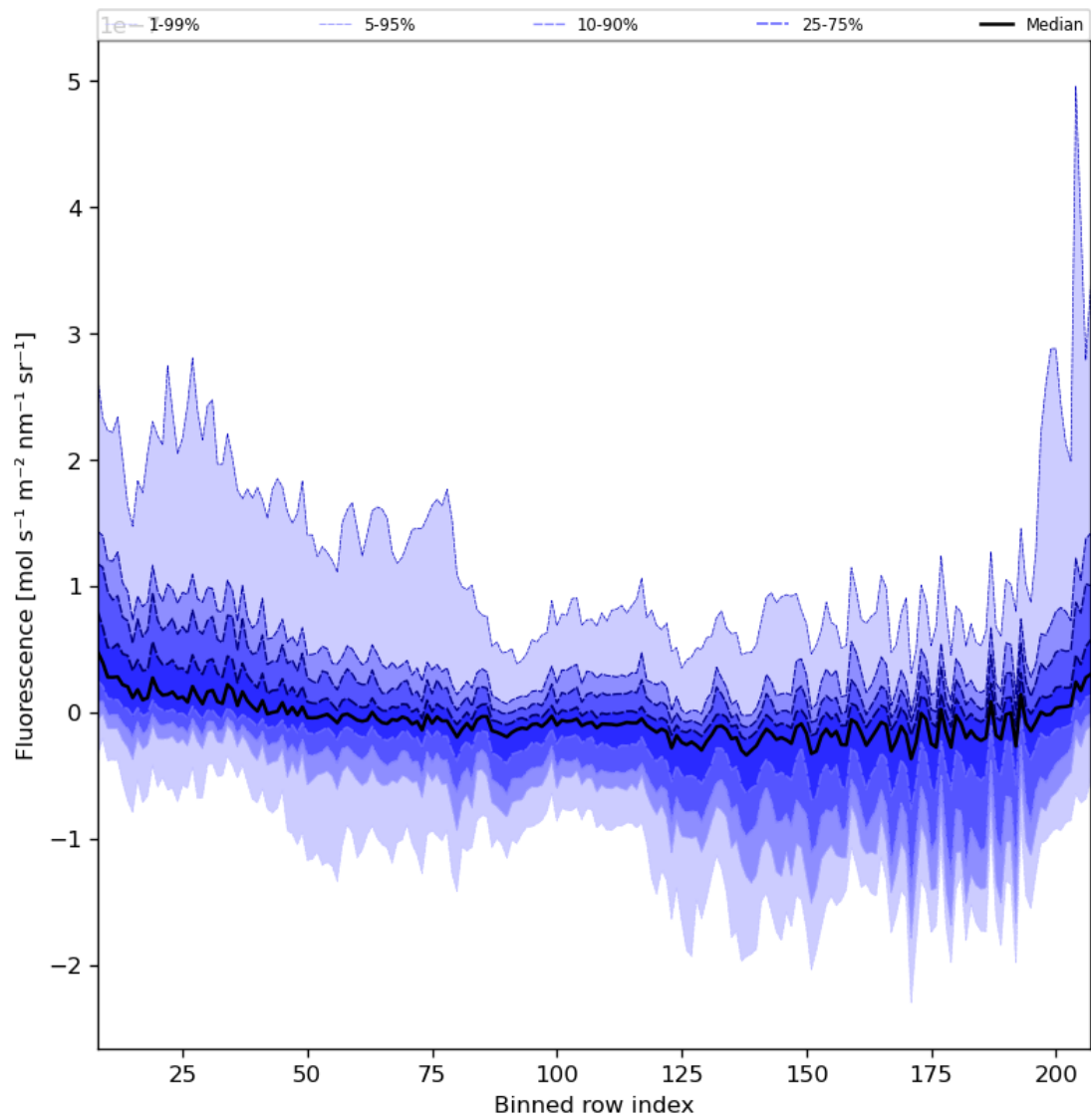
Figure 43: Along track statistics of “Fluorescence” for 2024-08-12 to 2024-08-14
