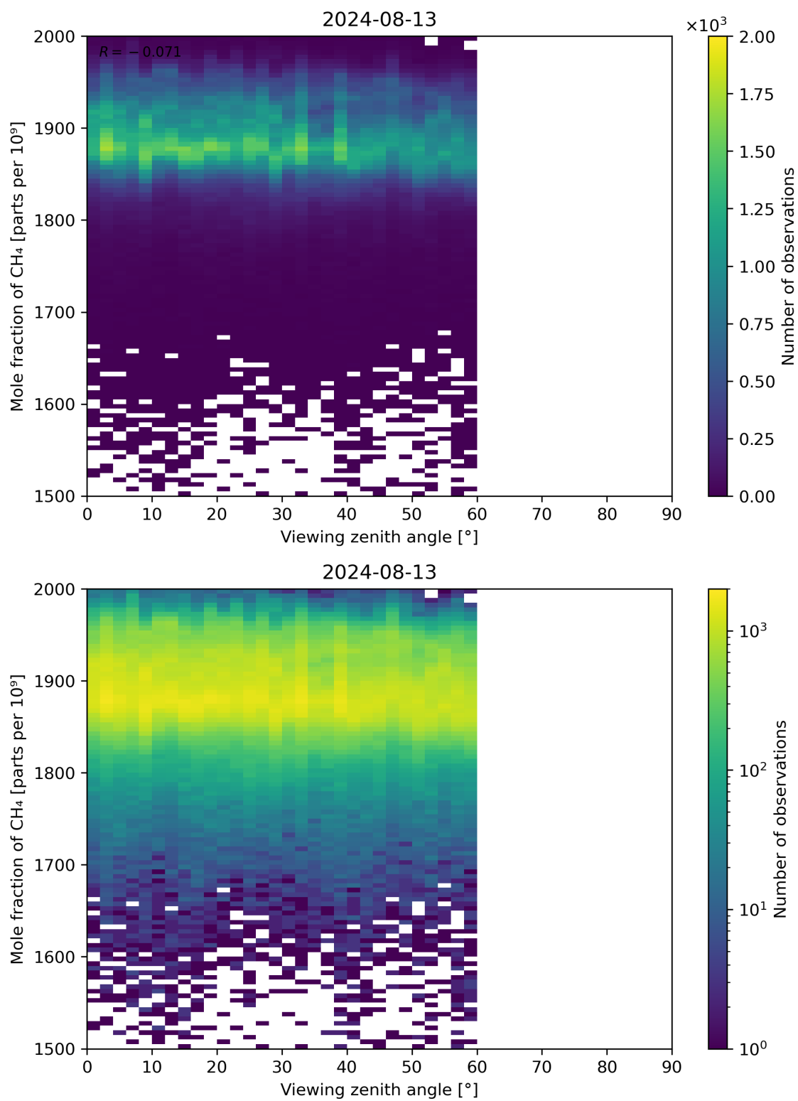
Figure 110: Scatter density plot of “Viewing zenith angle” against “Mole fraction of CH 4 ” for 2024-08-12 to 2024-08-14.
