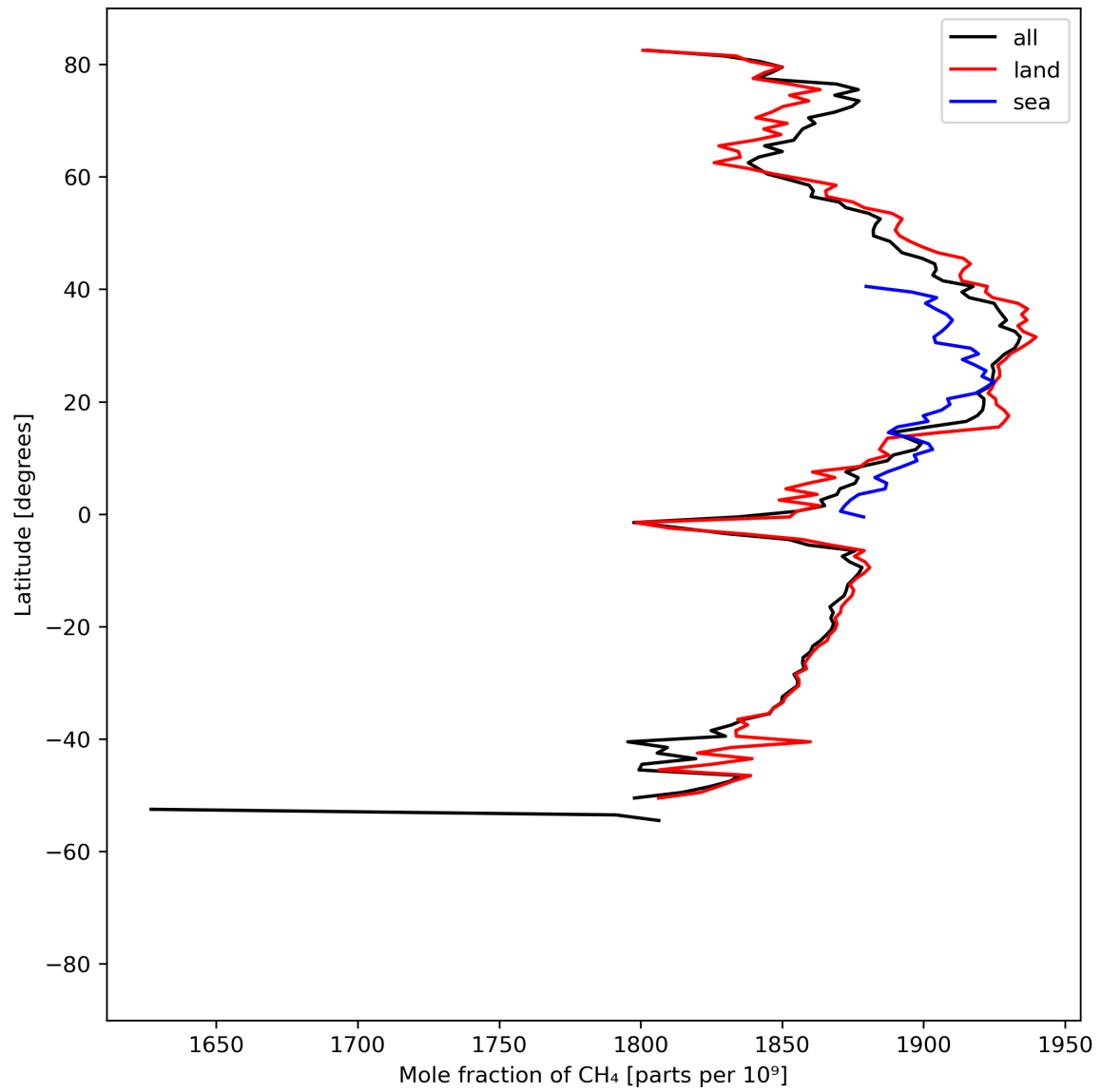
Figure 12: Zonal average of “Mole fraction of CH 4 ” for 2024-08-12 to 2024-08-14.
