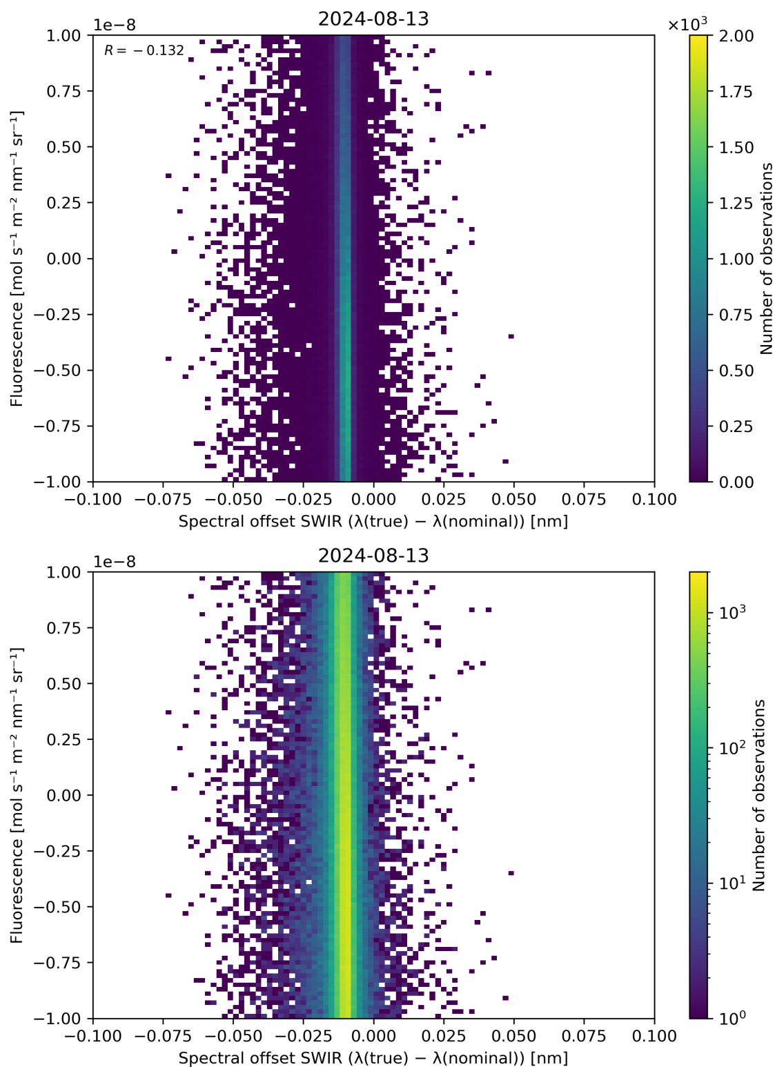
Figure 120: Scatter density plot of “Spectral offset SWIR ( \lambda(\text{true}) - \lambda(\text{nominal}) )” against “Fluorescence” for 2024-08-12 to 2024-08-14.
