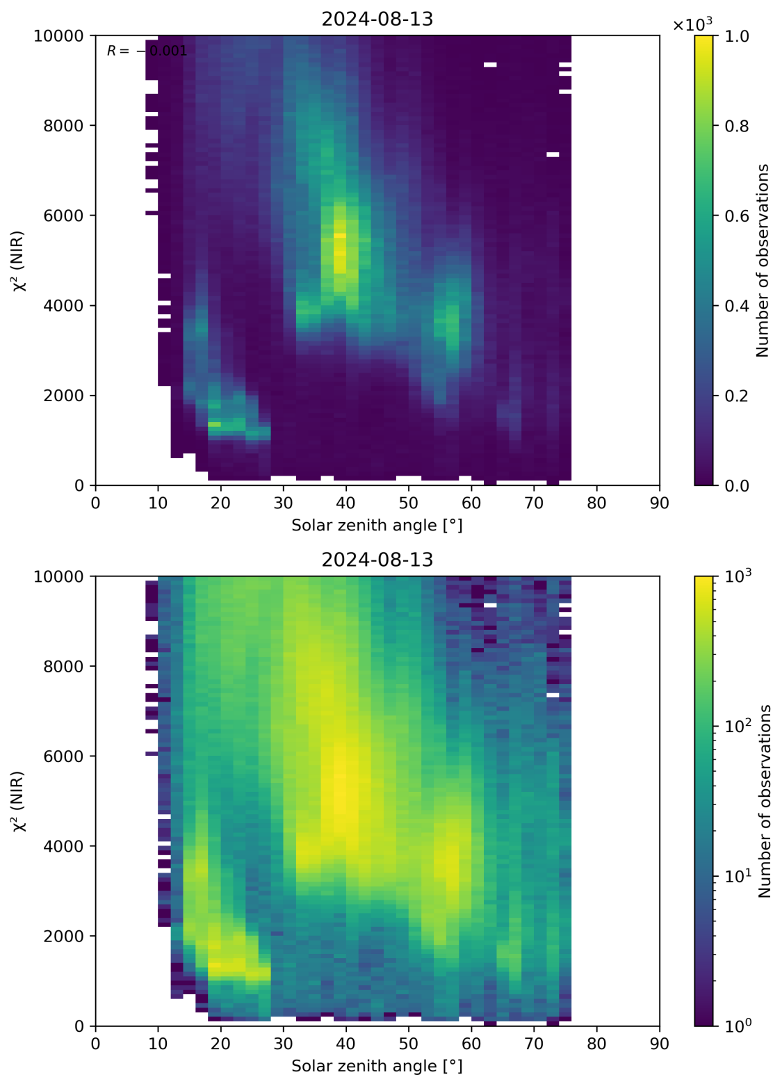
Figure 94: Scatter density plot of “Solar zenith angle” against “ \chi^2 (NIR)” for 2024-08-12 to 2024-08-14.
