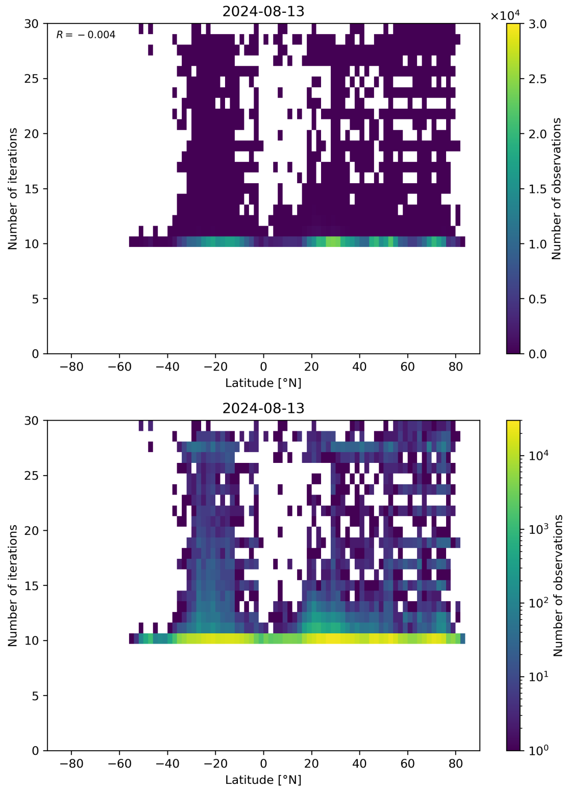
Figure 60: Scatter density plot of “Latitude” against “Number of iterations” for 2024-08-12 to 2024-08-14.
