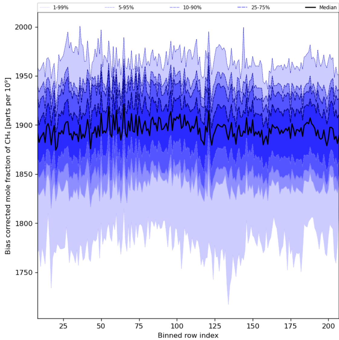
Figure 36: Along track statistics of “Bias corrected mole fraction of CH 4 ” for 2024-08-12 to 2024-08-14
