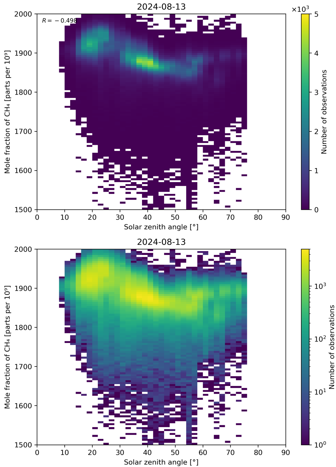
Figure 99: Scatter density plot of “Solar zenith angle” against “Mole fraction of CH 4 ” for 2024-08-12 to 2024-08-14.
