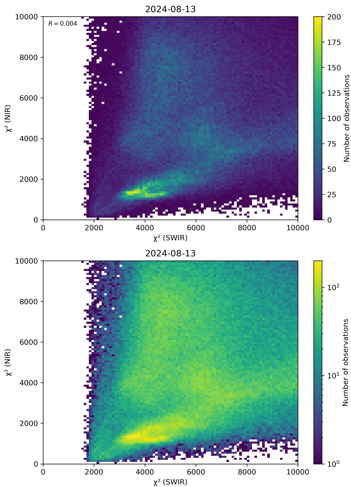
Figure 47: Scatter density plot of “ \chi^2 (SWIR)” against “ \chi^2 (NIR)” for 2024-08-12 to 2024-08-14.
