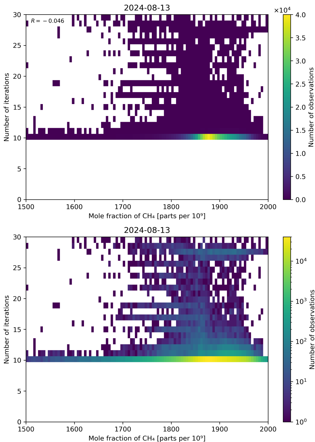
Figure 76: Scatter density plot of “Mole fraction of CH 4 ” against “Number of iterations” for 2024-08-12 to 2024-08-14.
