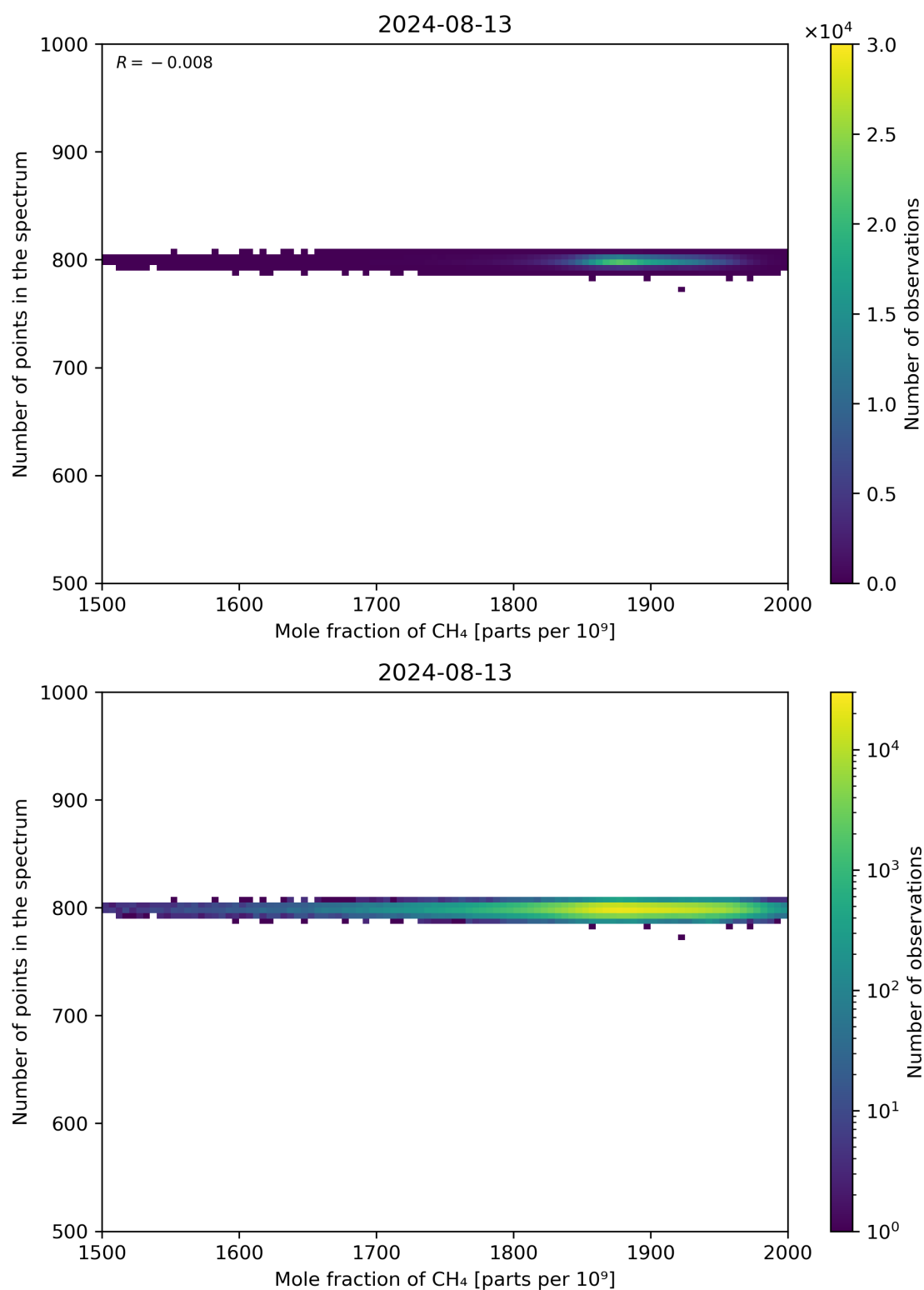
Figure 77: Scatter density plot of “Mole fraction of CH 4 ” against “Number of points in the spectrum” for 2024-08-12 to 2024-08-14.
