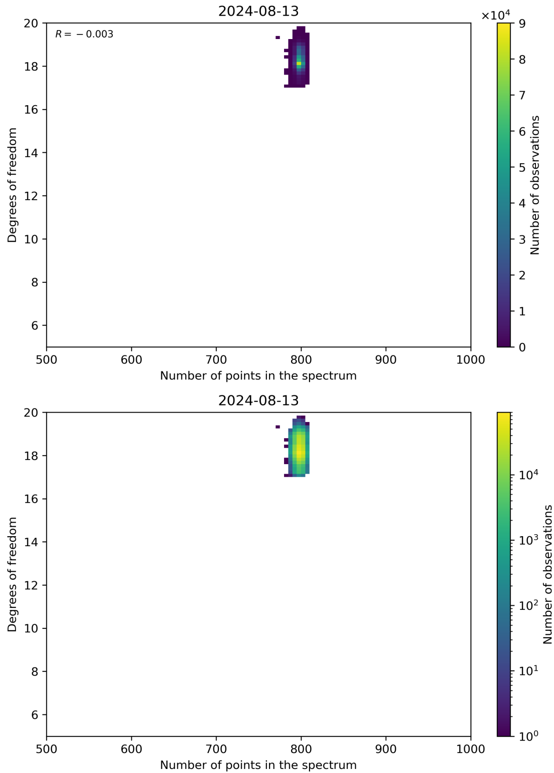
Figure 90: Scatter density plot of “Number of points in the spectrum” against “Degrees of freedom” for 2024-08-12 to 2024-08-14.
