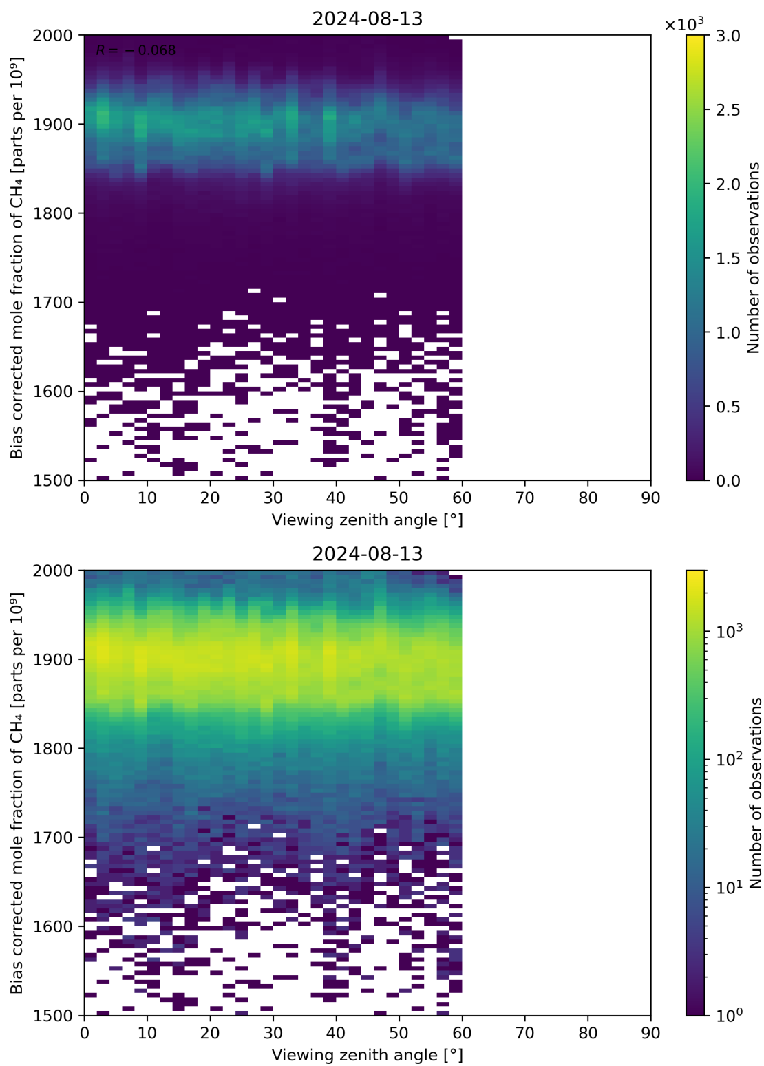
Figure 111: Scatter density plot of “Viewing zenith angle” against “Bias corrected mole fraction of CH 4 ” for 2024-08-12 to 2024-08-14.
