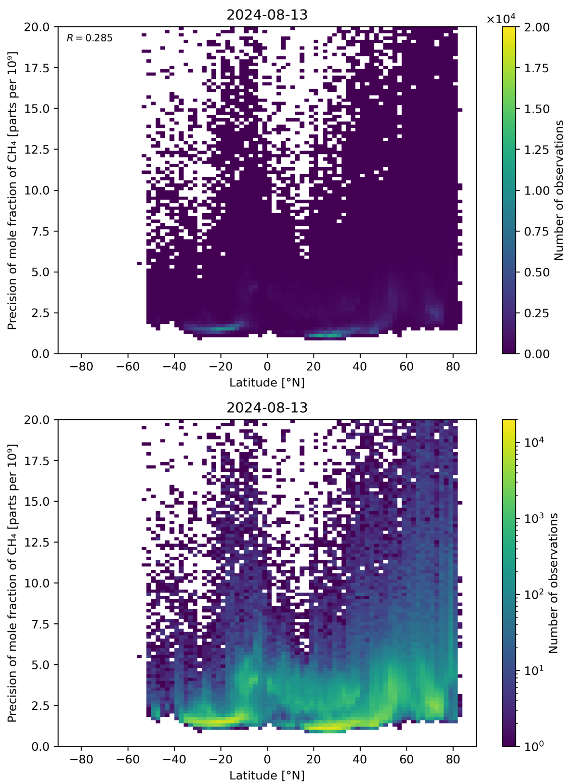
Figure 59: Scatter density plot of “Latitude” against “Precision of mole fraction of \text{CH}_4 ” for 2024-08-12 to 2024-08-14.
