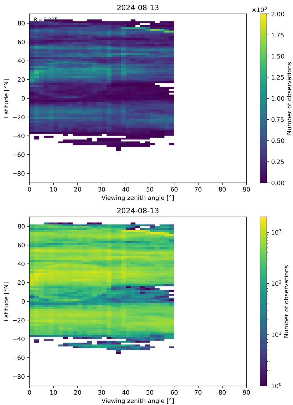
Figure 109: Scatter density plot of “Viewing zenith angle” against “Latitude” for 2024-08-12 to 2024-08-14.
