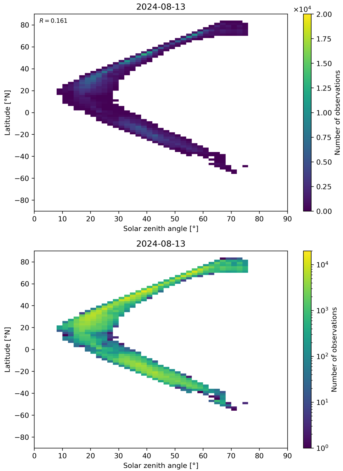
Figure 98: Scatter density plot of “Solar zenith angle” against “Latitude” for 2024-08-12 to 2024-08-14.
