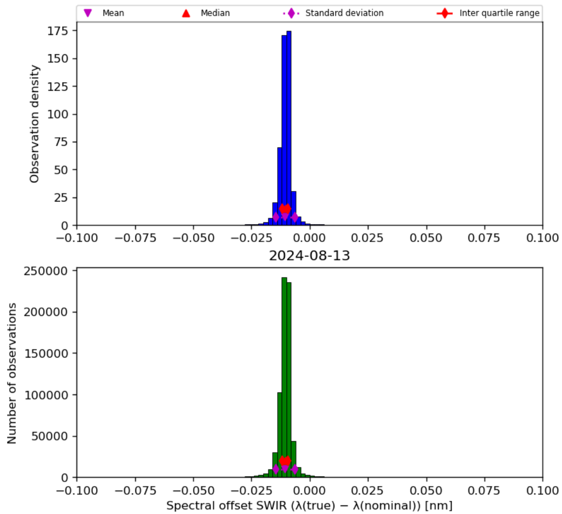
Figure 27: Histogram of “Spectral offset SWIR ( \lambda(\text{true}) - \lambda(\text{nominal}) )” for 2024-08-12 to 2024-08-14
