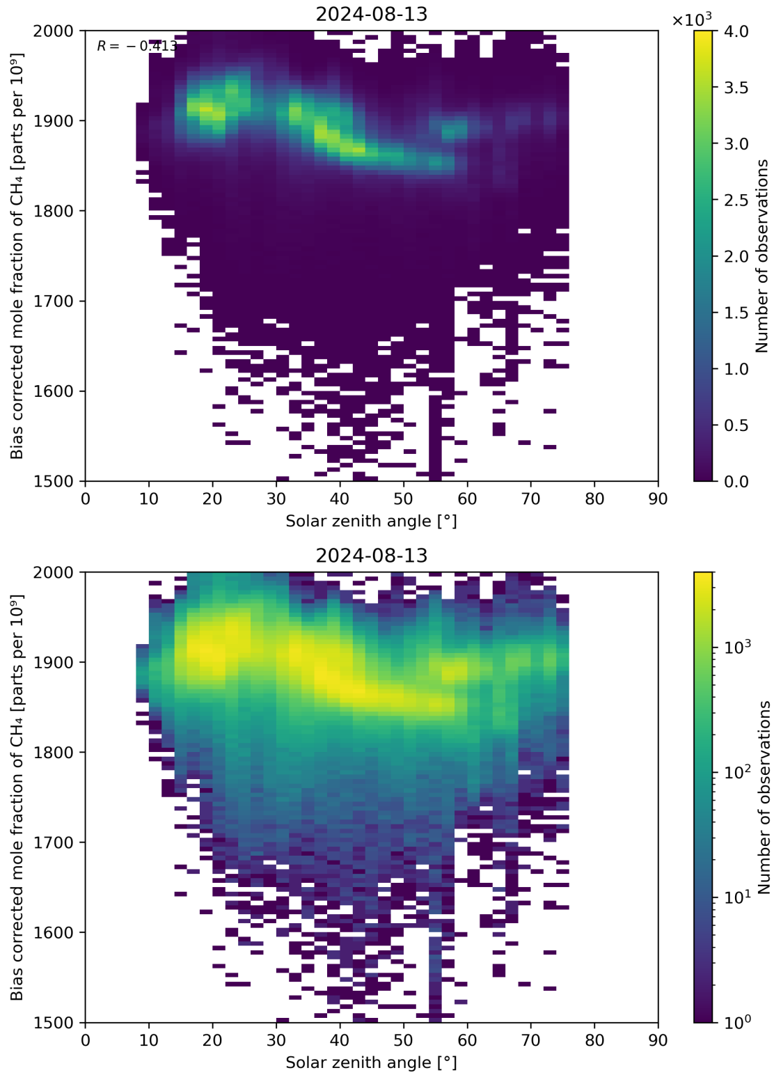
Figure 100: Scatter density plot of “Solar zenith angle” against “Bias corrected mole fraction of CH 4 ” for 2024-08-12 to 2024-08-14.
