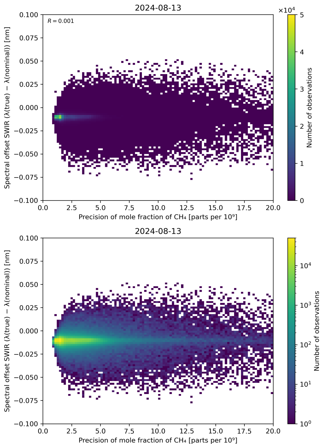
Figure 85: Scatter density plot of “Precision of mole fraction of CH 4 ” against “Spectral offset SWIR ( \lambda(\text{true}) - \lambda(\text{nominal}) )” for 2024-08-12 to 2024-08-14.
