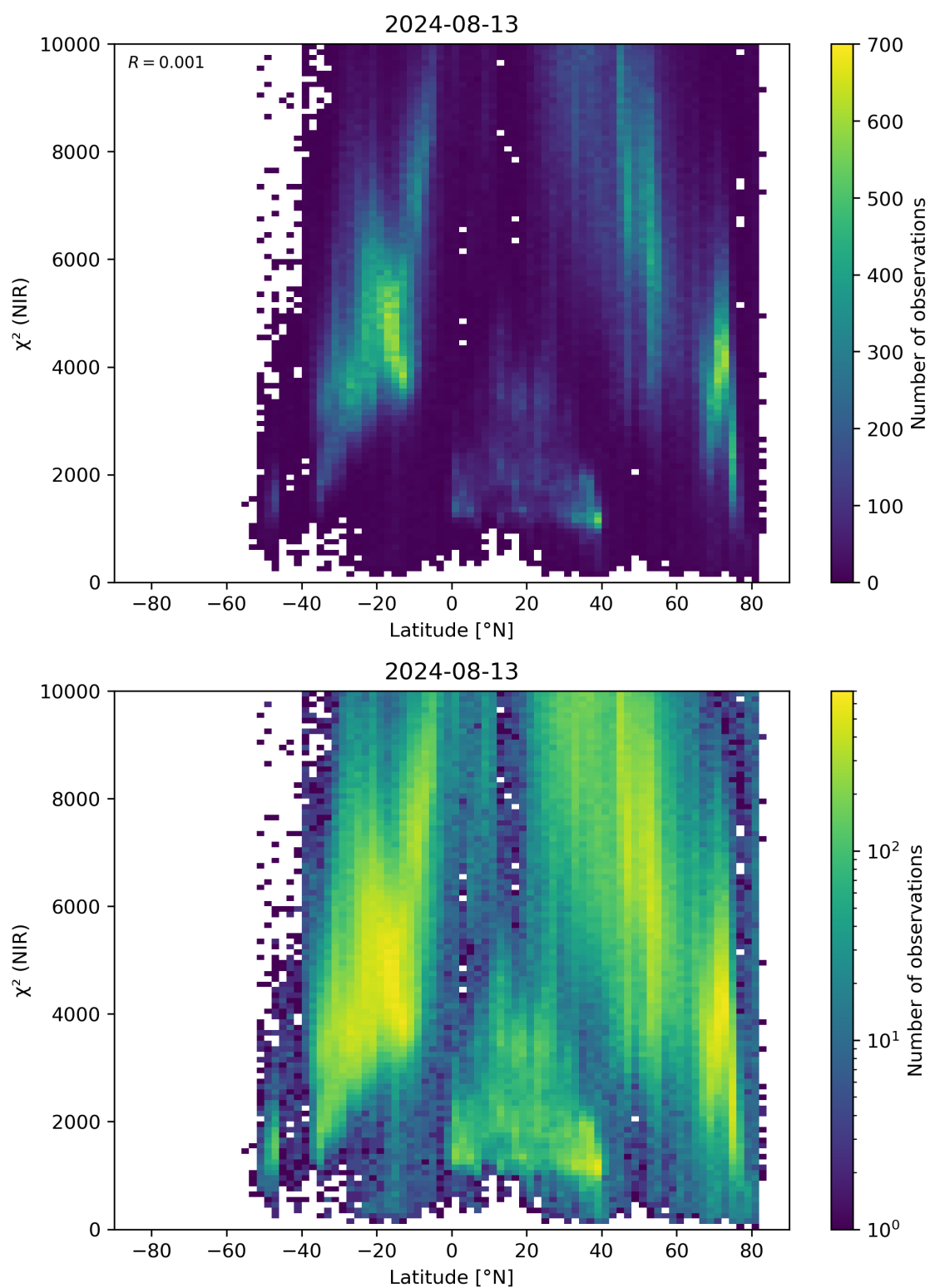
Figure 53: Scatter density plot of “Latitude” against “ \chi^2 (NIR)” for 2024-08-12 to 2024-08-14.
