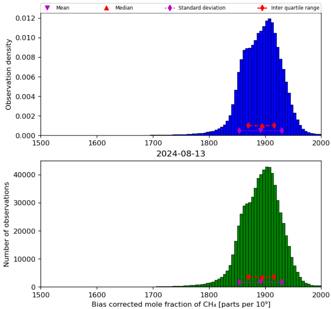
Figure 25: Histogram of “Bias corrected mole fraction of CH 4 ” for 2024-08-12 to 2024-08-14
