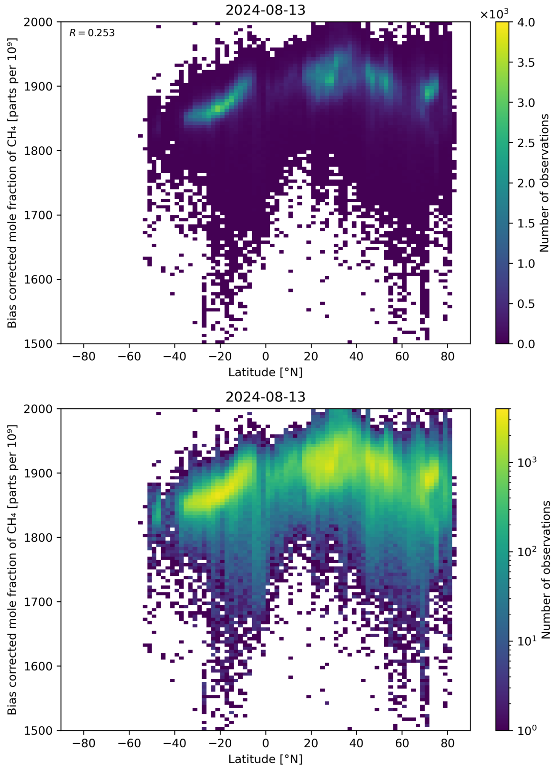
Figure 58: Scatter density plot of “Latitude” against “Bias corrected mole fraction of \text{CH}_4 ” for 2024-08-12 to 2024-08-14.
