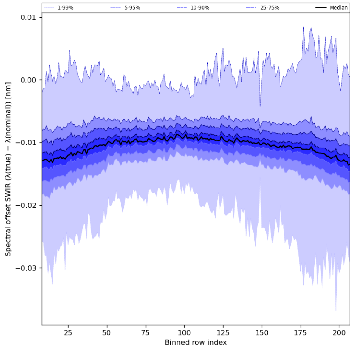
Figure 38: Along track statistics of “Spectral offset SWIR ( \lambda(\text{true}) - \lambda(\text{nominal}) )” for 2024-08-12 to 2024-08-14
