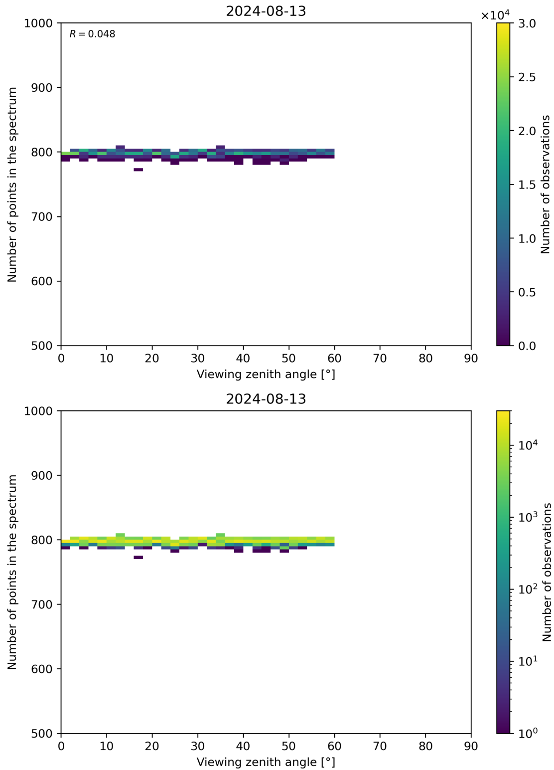
Figure 114: Scatter density plot of “Viewing zenith angle” against “Number of points in the spectrum” for 2024-08-12 to 2024-08-14.
