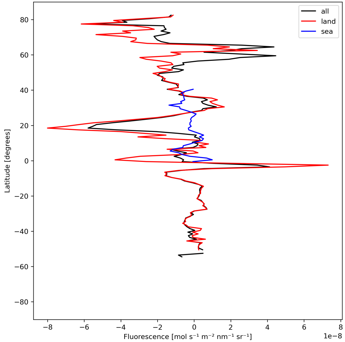
Figure 21: Zonal average of “Fluorescence” for 2024-08-12 to 2024-08-14.
