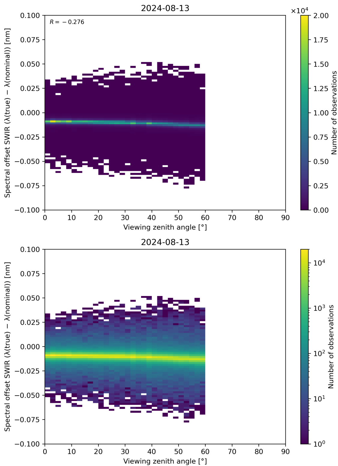
Figure 116: Scatter density plot of “Viewing zenith angle” against “Spectral offset SWIR ( \lambda(\text{true}) - \lambda(\text{nominal}) )” for 2024-08-12 to 2024-08-14.
