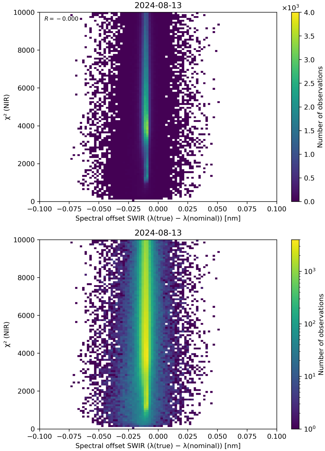
Figure 117: Scatter density plot of “Spectral offset SWIR ( \lambda(\text{true}) - \lambda(\text{nominal}) )” against “ \chi^2 (NIR)” for 2024-08-12 to 2024-08-14.
