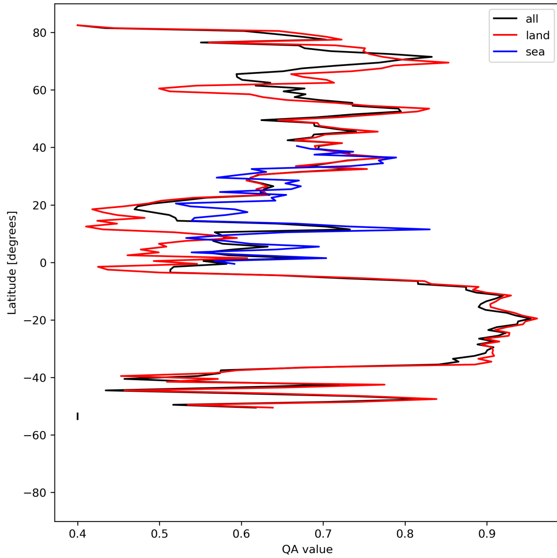
Figure 11: Zonal average of “QA value” for 2024-08-12 to 2024-08-14.
