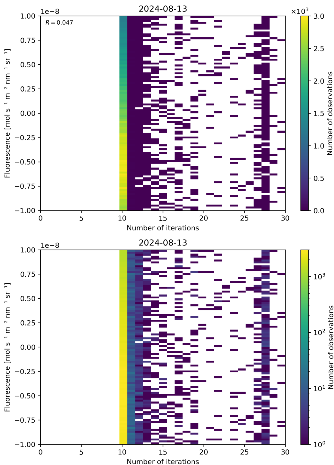
Figure 87: Scatter density plot of “Number of iterations” against “Fluorescence” for 2024-08-12 to 2024-08-14.
