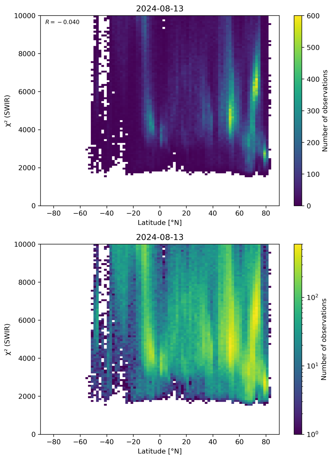
Figure 54: Scatter density plot of “Latitude” against “ \chi^2 (SWIR)” for 2024-08-12 to 2024-08-14.
