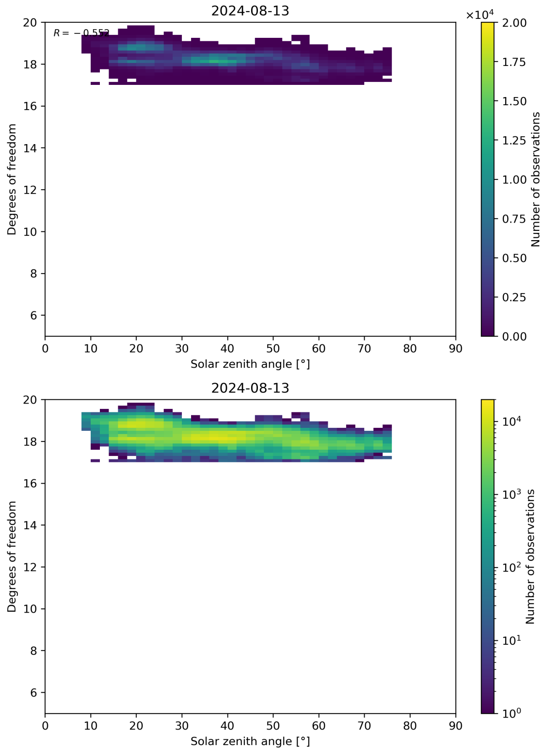
Figure 96: Scatter density plot of “Solar zenith angle” against “Degrees of freedom” for 2024-08-12 to 2024-08-14.
