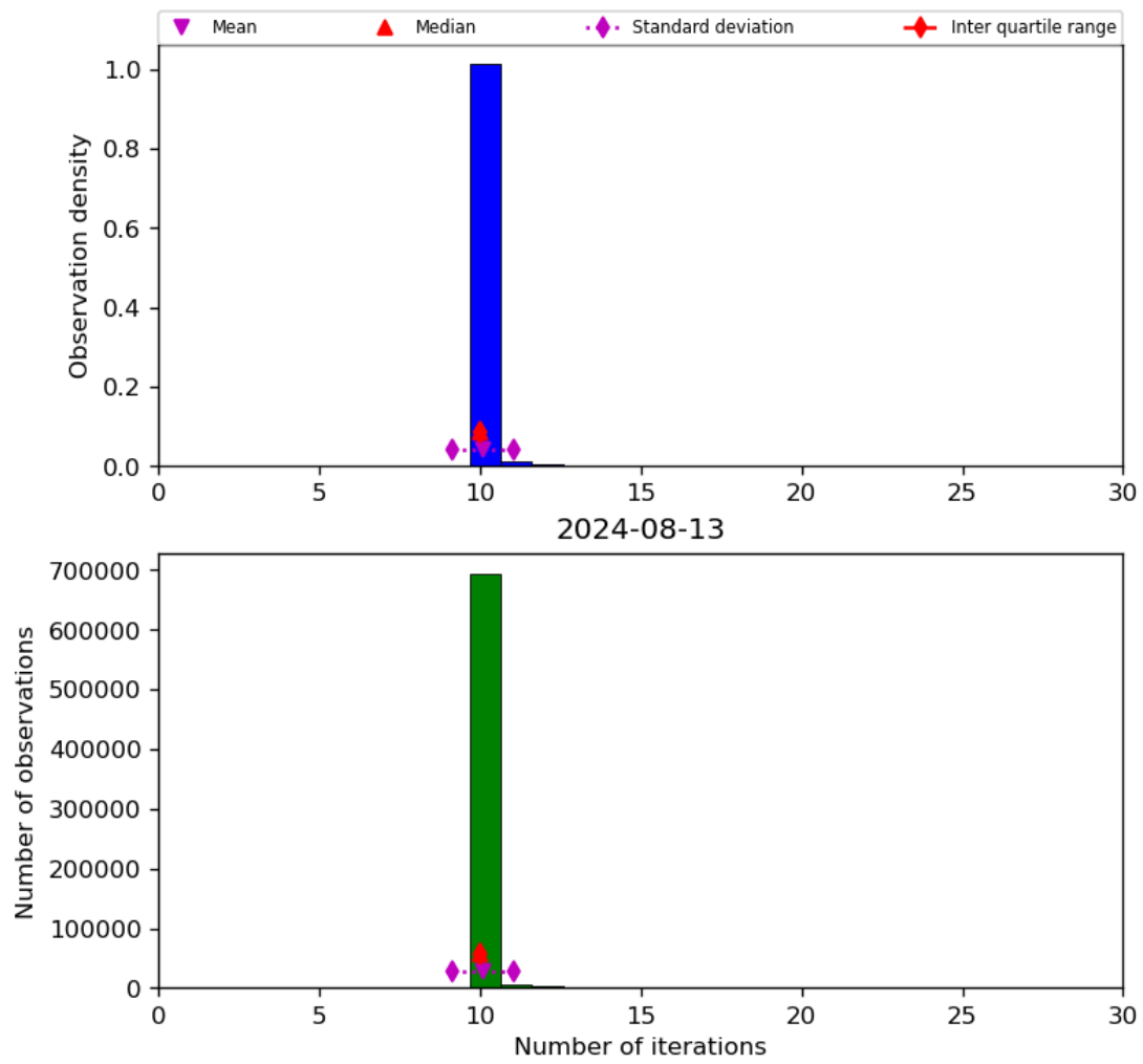
Figure 31: Histogram of “Number of iterations” for 2024-08-12 to 2024-08-14
