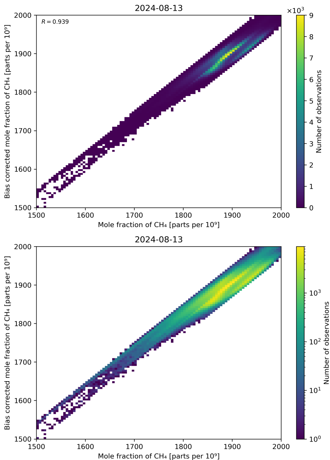
Figure 74: Scatter density plot of “Mole fraction of CH 4 ” against “Bias corrected mole fraction of CH 4 ” for 2024-08-12 to 2024-08-14.
