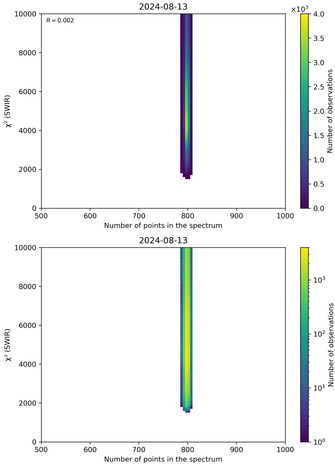
Figure 89: Scatter density plot of “Number of points in the spectrum” against “ \chi^2 (SWIR)” for 2024-08-12 to 2024-08-14.
