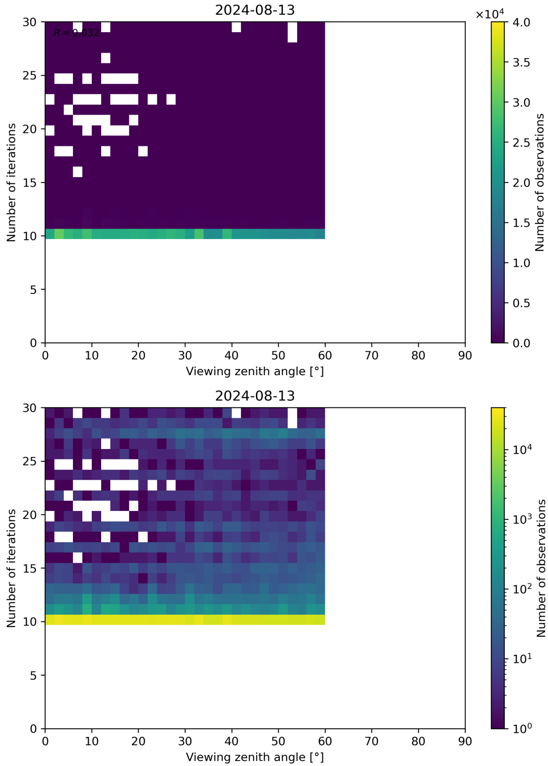
Figure 113: Scatter density plot of “Viewing zenith angle” against “Number of iterations” for 2024-08-12 to 2024-08-14.
