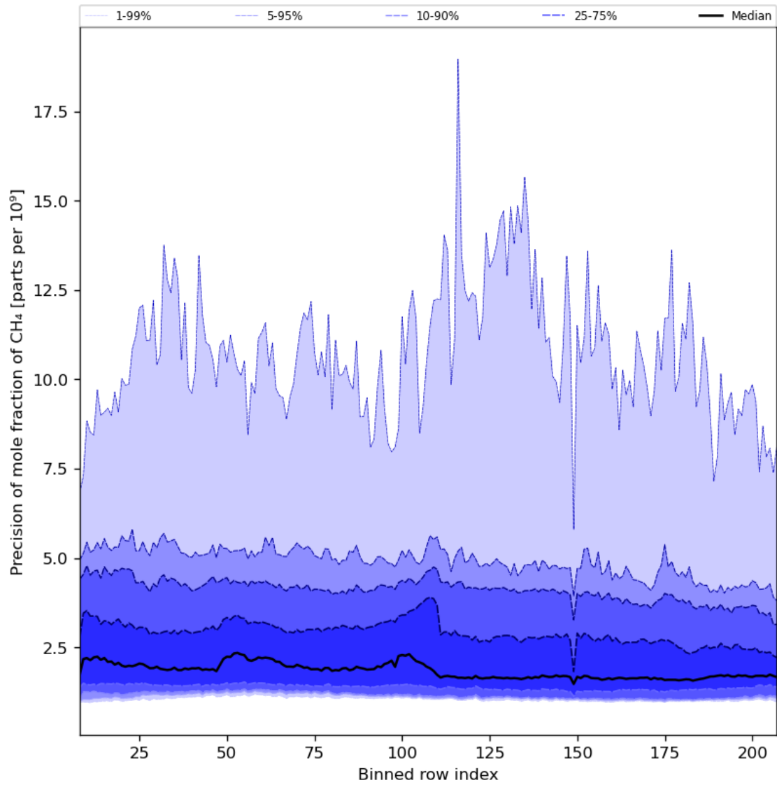
Figure 35: Along track statistics of “Precision of mole fraction of CH 4 ” for 2024-08-12 to 2024-08-14
