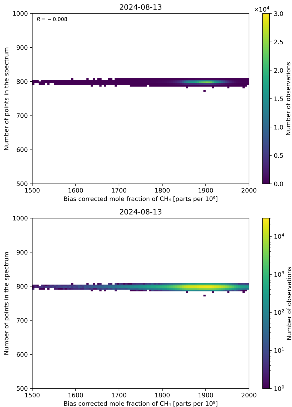
Figure 68: Scatter density plot of “Bias corrected mole fraction of CH 4 ” against “Number of points in the spectrum” for 2024-08-12 to 2024-08-14.
