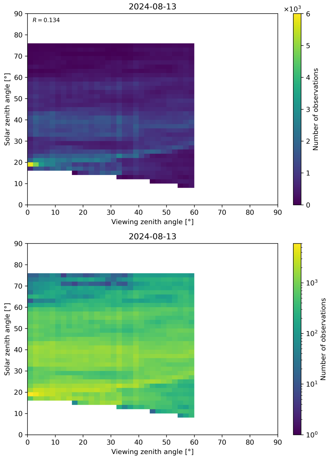
Figure 115: Scatter density plot of “Viewing zenith angle” against “Solar zenith angle” for 2024-08-12 to 2024-08-14.
