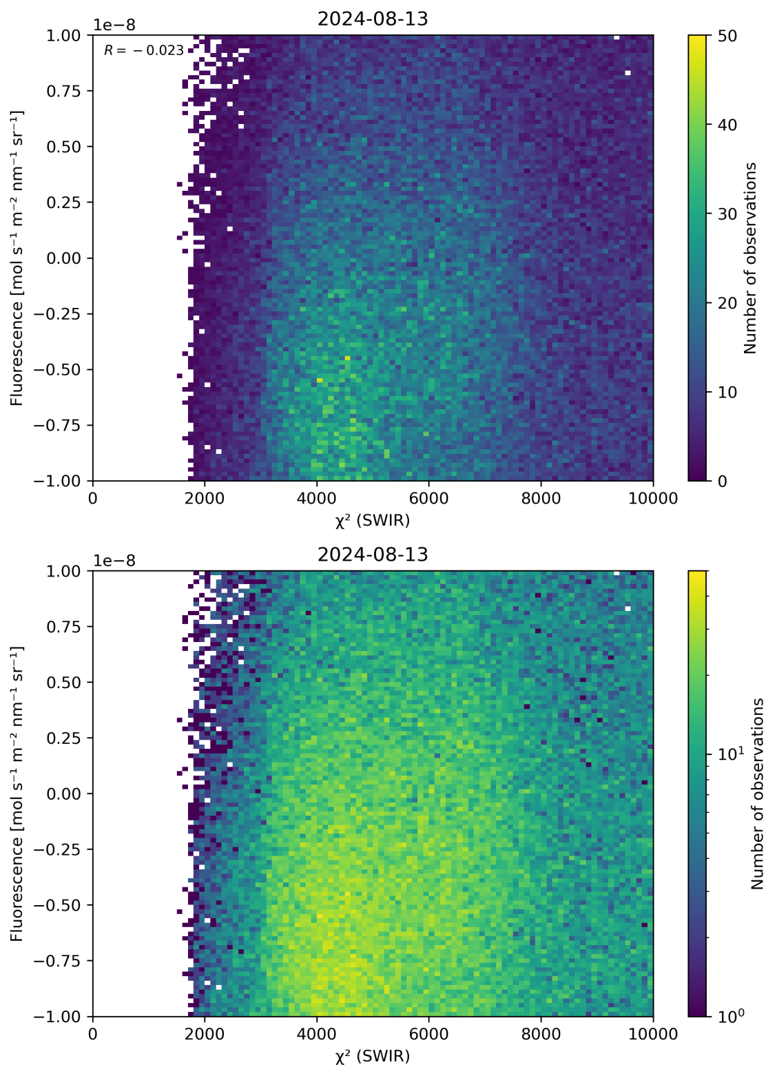
Figure 49: Scatter density plot of “ \chi^2 (SWIR)” against “Fluorescence” for 2024-08-12 to 2024-08-14.
