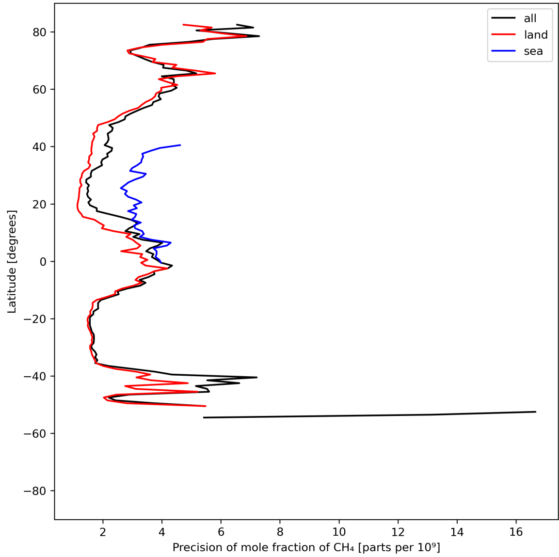
Figure 13: Zonal average of “Precision of mole fraction of CH 4 ” for 2024-08-12 to 2024-08-14.
