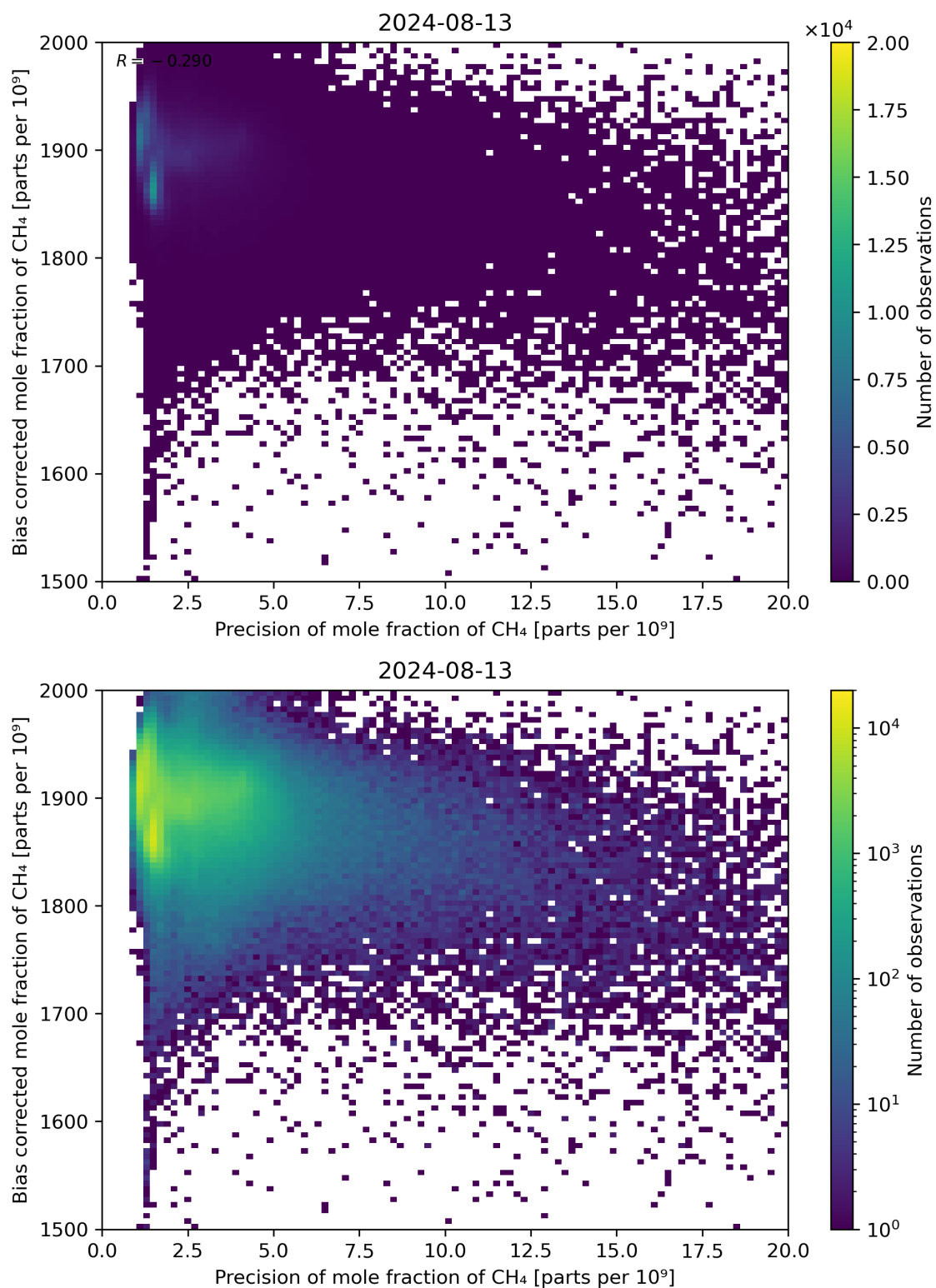
Figure 82: Scatter density plot of “Precision of mole fraction of \text{CH}_4 ” against “Bias corrected mole fraction of \text{CH}_4 ” for 2024-08-12 to 2024-08-14.
