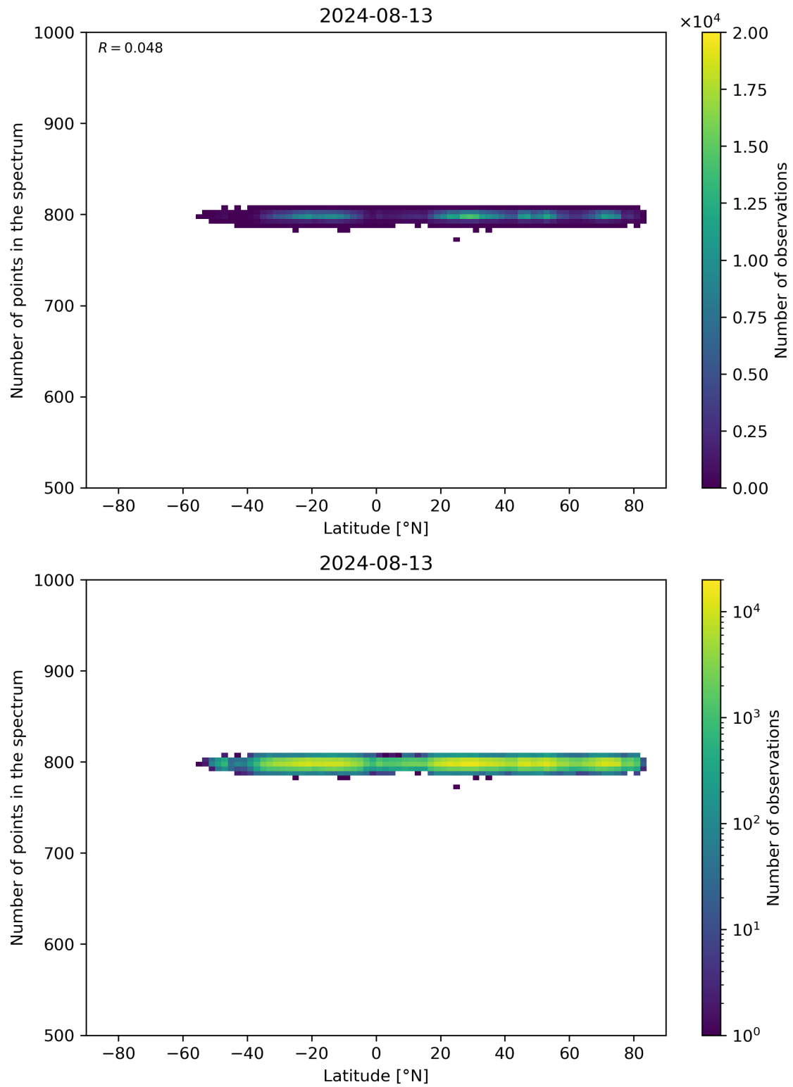
Figure 61: Scatter density plot of “Latitude” against “Number of points in the spectrum” for 2024-08-12 to 2024-08-14.
