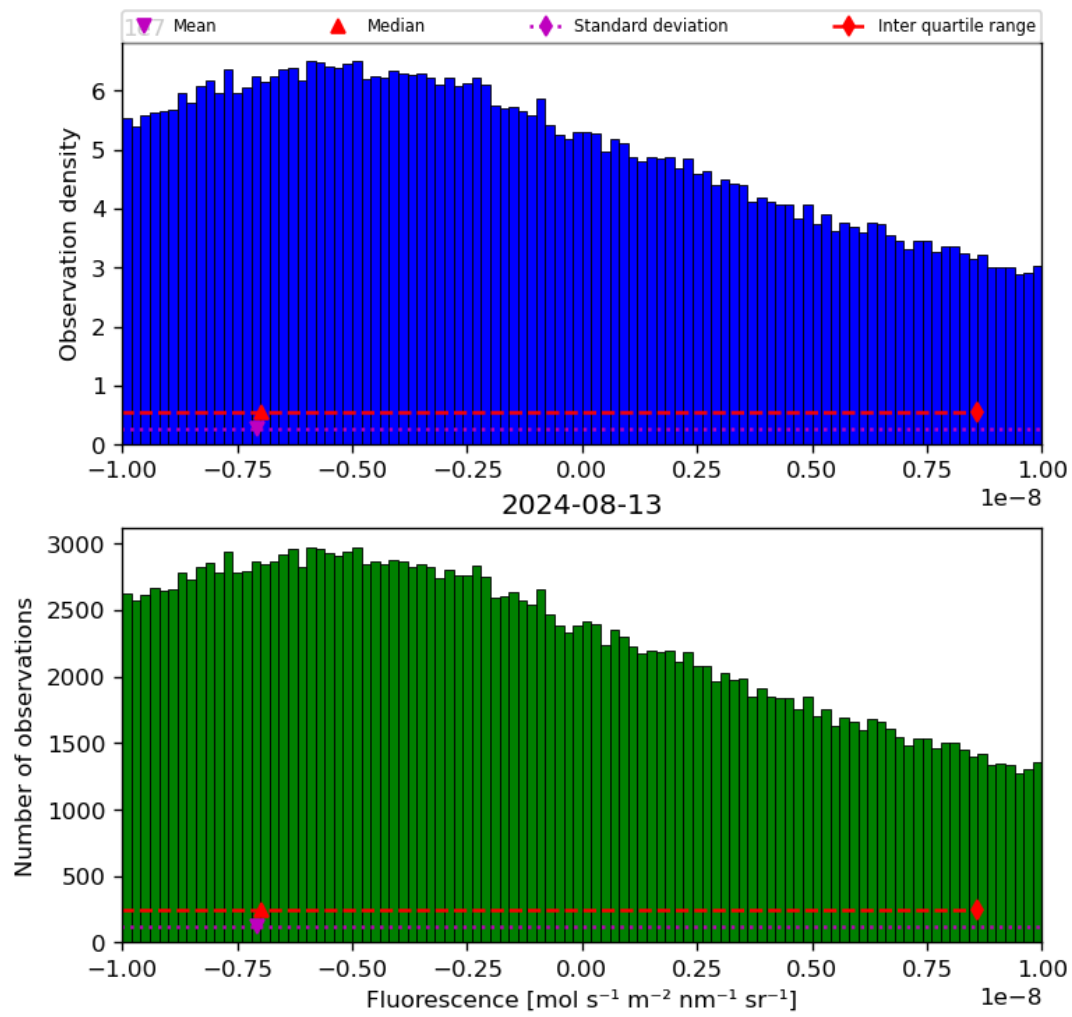
Figure 32: Histogram of “Fluorescence” for 2024-08-12 to 2024-08-14
