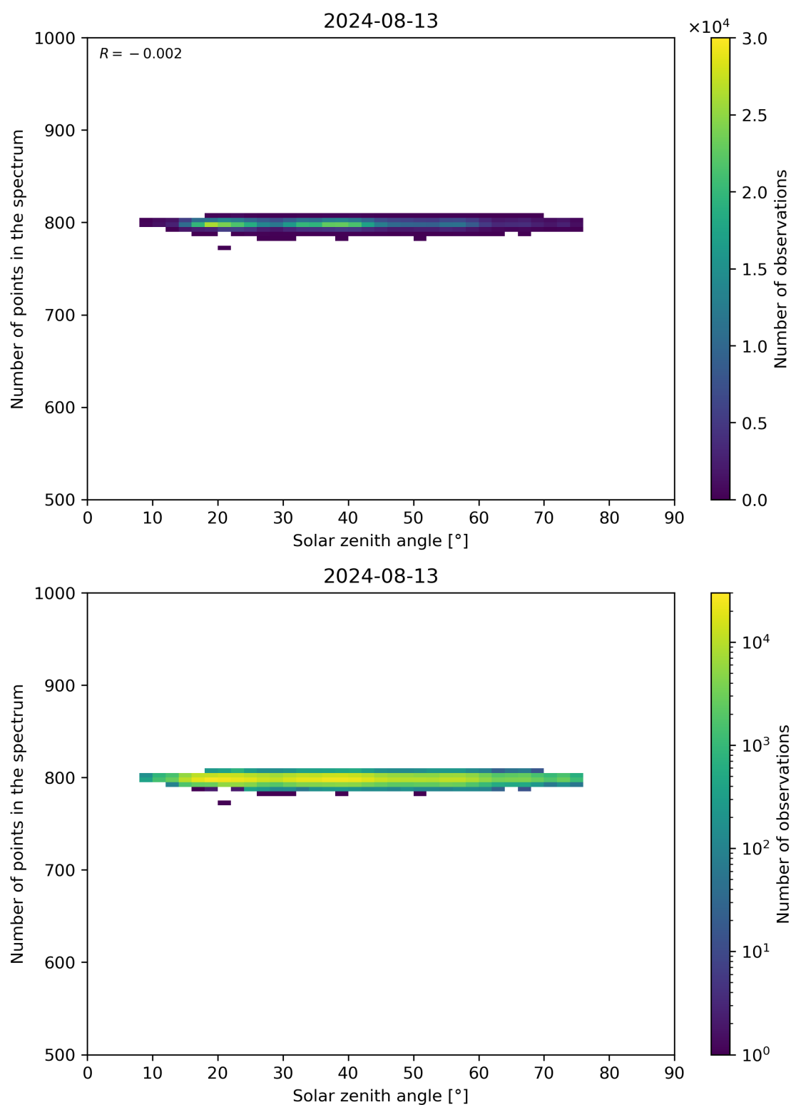
Figure 103: Scatter density plot of “Solar zenith angle” against “Number of points in the spectrum” for 2024-08-12 to 2024-08-14.
