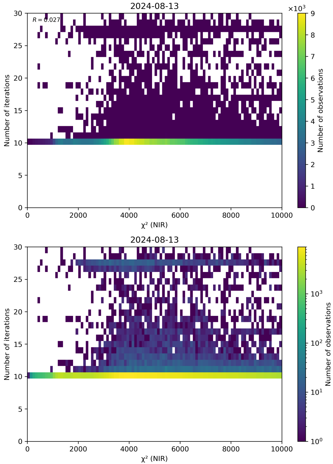
Figure 46: Scatter density plot of “ \chi^2 (NIR)” against “Number of iterations” for 2024-08-12 to 2024-08-14.
