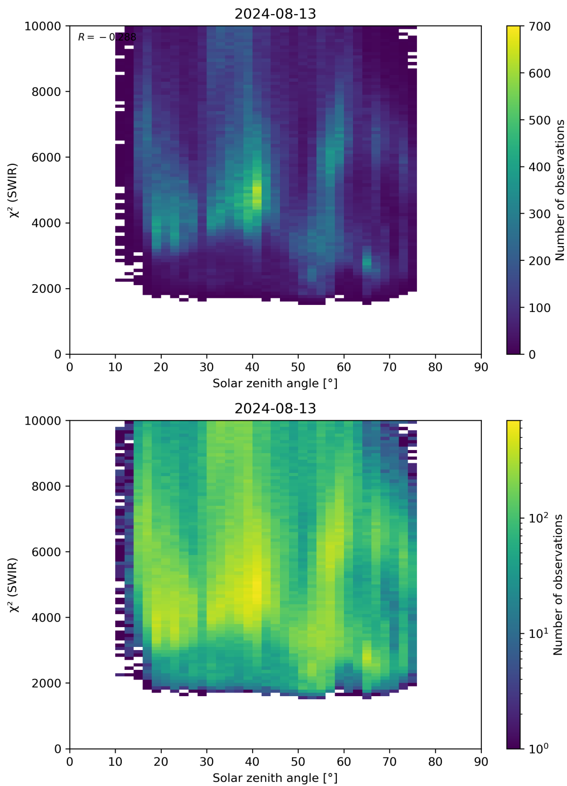
Figure 95: Scatter density plot of “Solar zenith angle” against “ \chi^2 (SWIR)” for 2024-08-12 to 2024-08-14.
