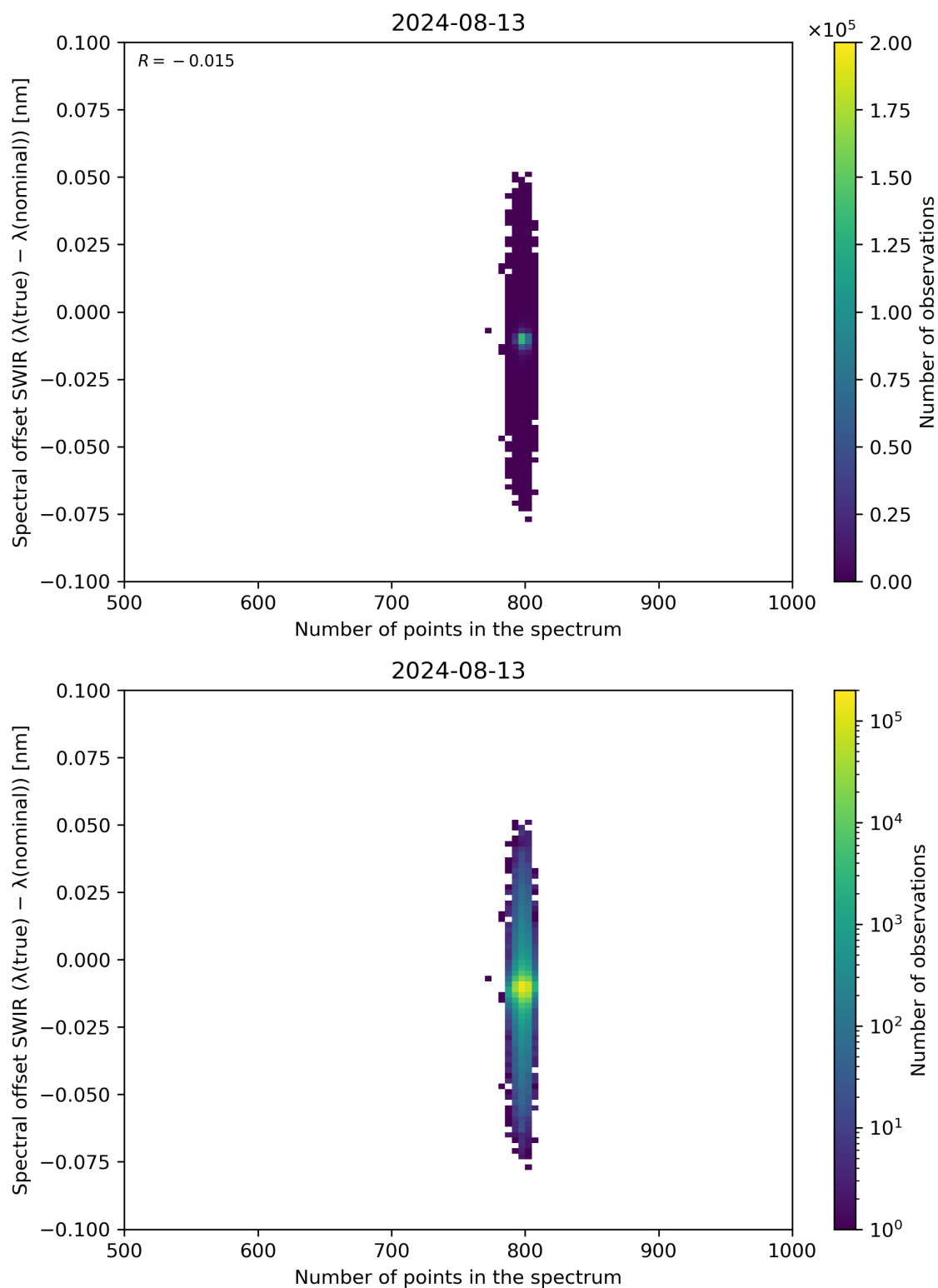
Figure 93: Scatter density plot of “Number of points in the spectrum” against “Spectral offset SWIR ( \lambda(\text{true}) - \lambda(\text{nominal}) )” for 2024-08-12 to 2024-08-14.
