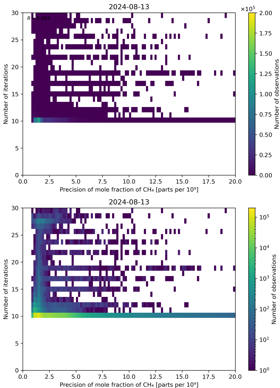
Figure 83: Scatter density plot of “Precision of mole fraction of \text{CH}_4 ” against “Number of iterations” for 2024-08-12 to 2024-08-14.
