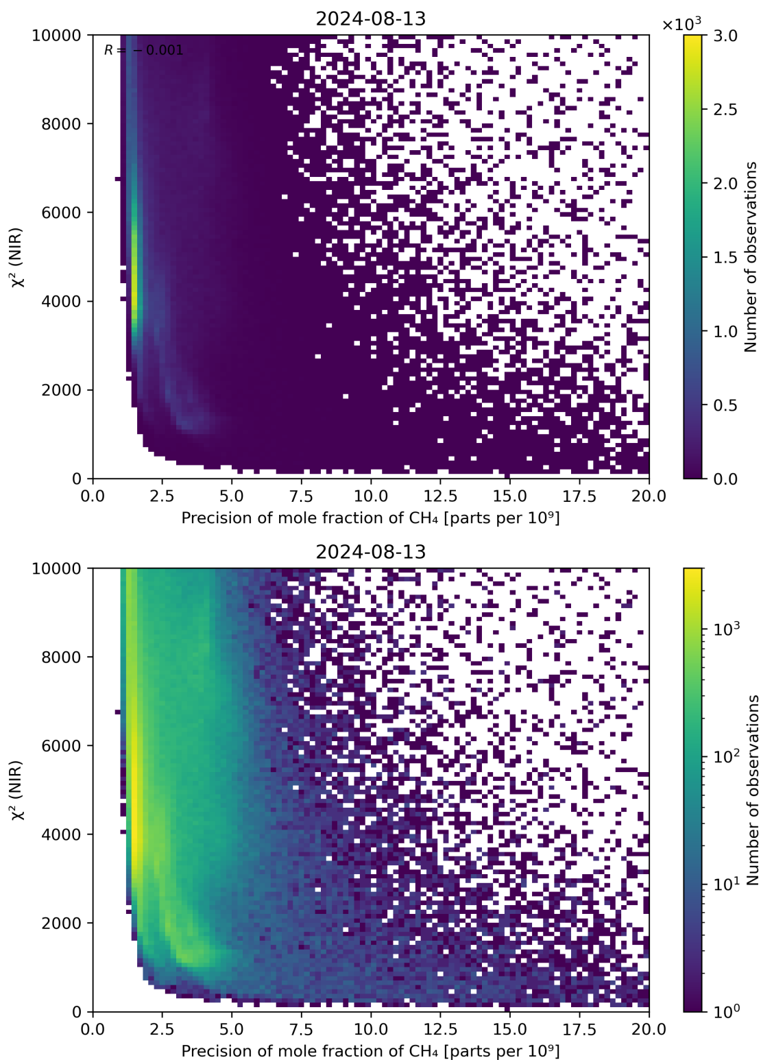
Figure 78: Scatter density plot of “Precision of mole fraction of CH 4 ” against “ \chi^2 (NIR)” for 2024-08-12 to 2024-08-14.
