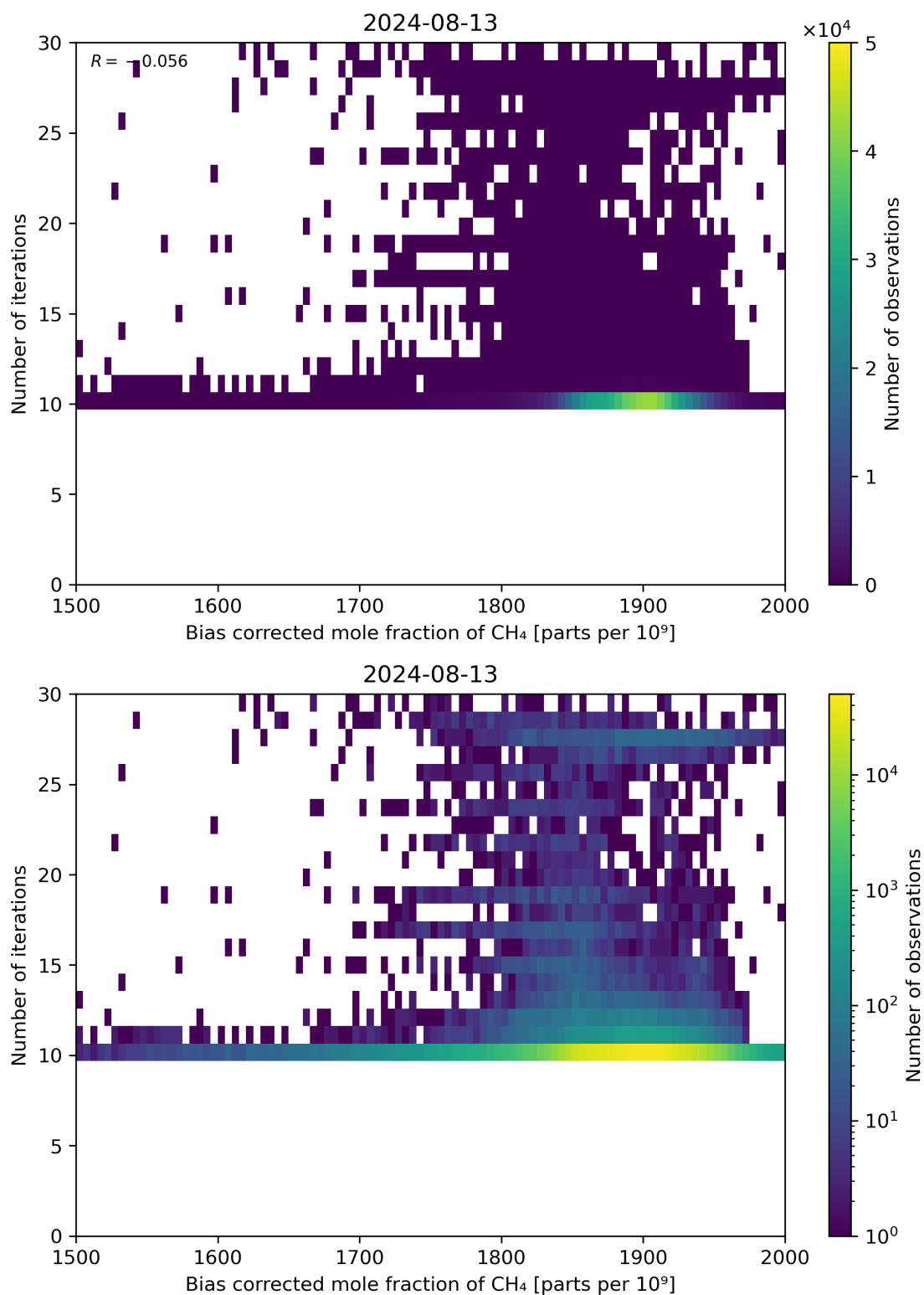
Figure 67: Scatter density plot of “Bias corrected mole fraction of \text{CH}_4 ” against “Number of iterations” for 2024-08-12 to 2024-08-14.
