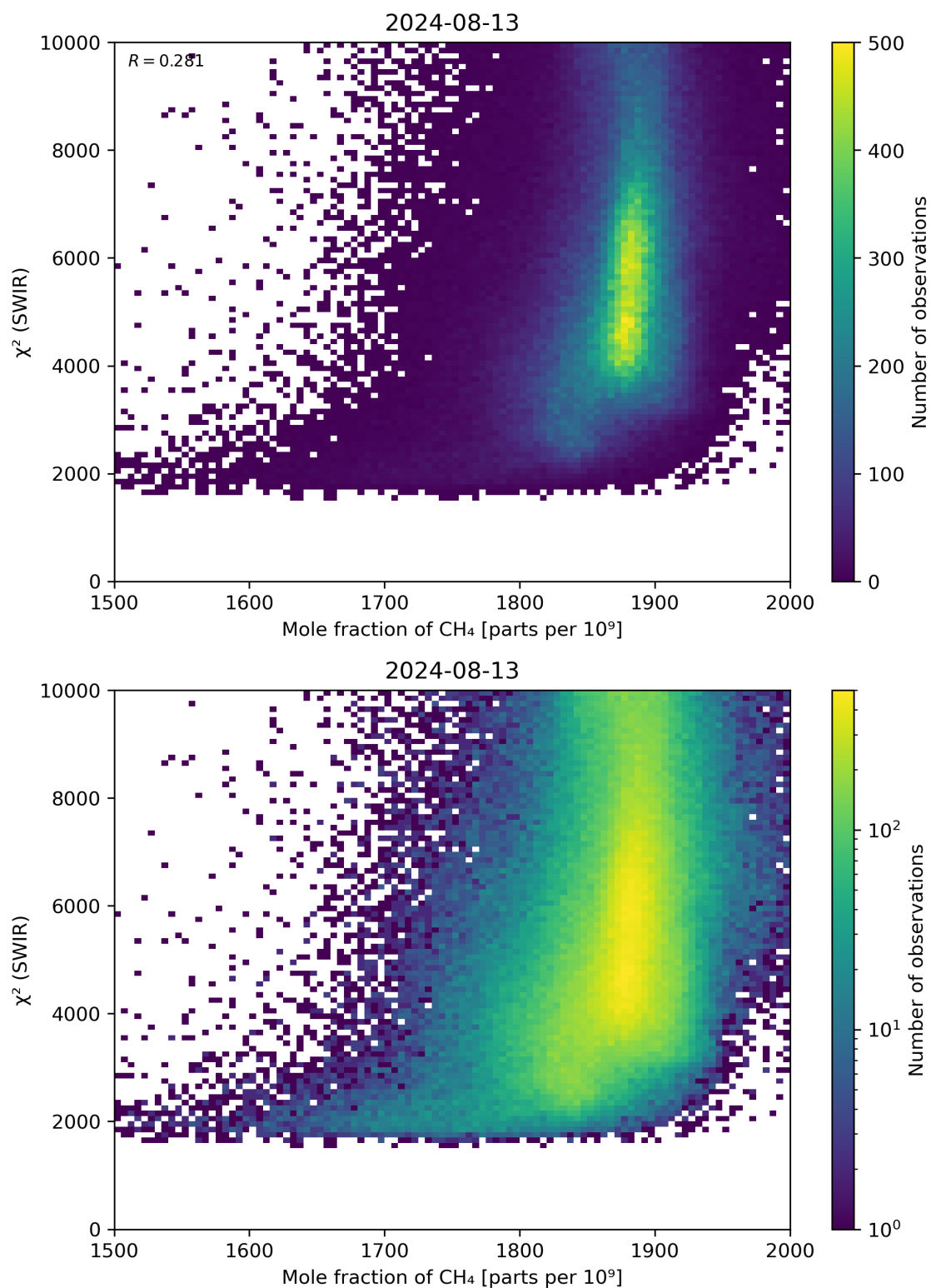
Figure 71: Scatter density plot of “Mole fraction of \text{CH}_4 ” against “ \chi^2 (SWIR)” for 2024-08-12 to 2024-08-14.
