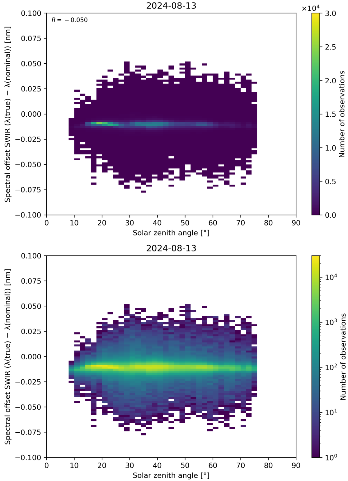
Figure 104: Scatter density plot of “Solar zenith angle” against “Spectral offset SWIR ( \lambda(\text{true}) - \lambda(\text{nominal}) )” for 2024-08-12 to 2024-08-14.
