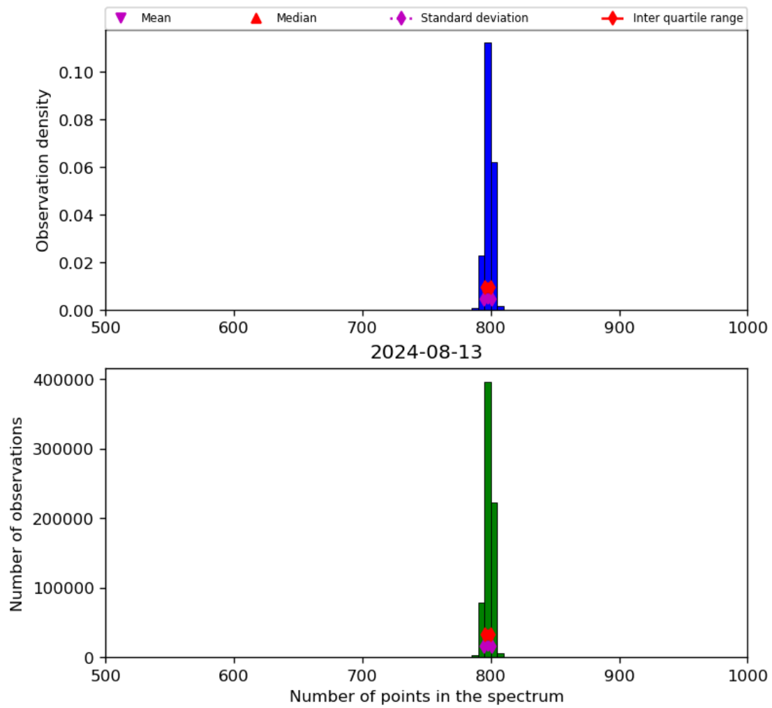
Figure 26: Histogram of “Number of points in the spectrum” for 2024-08-12 to 2024-08-14
