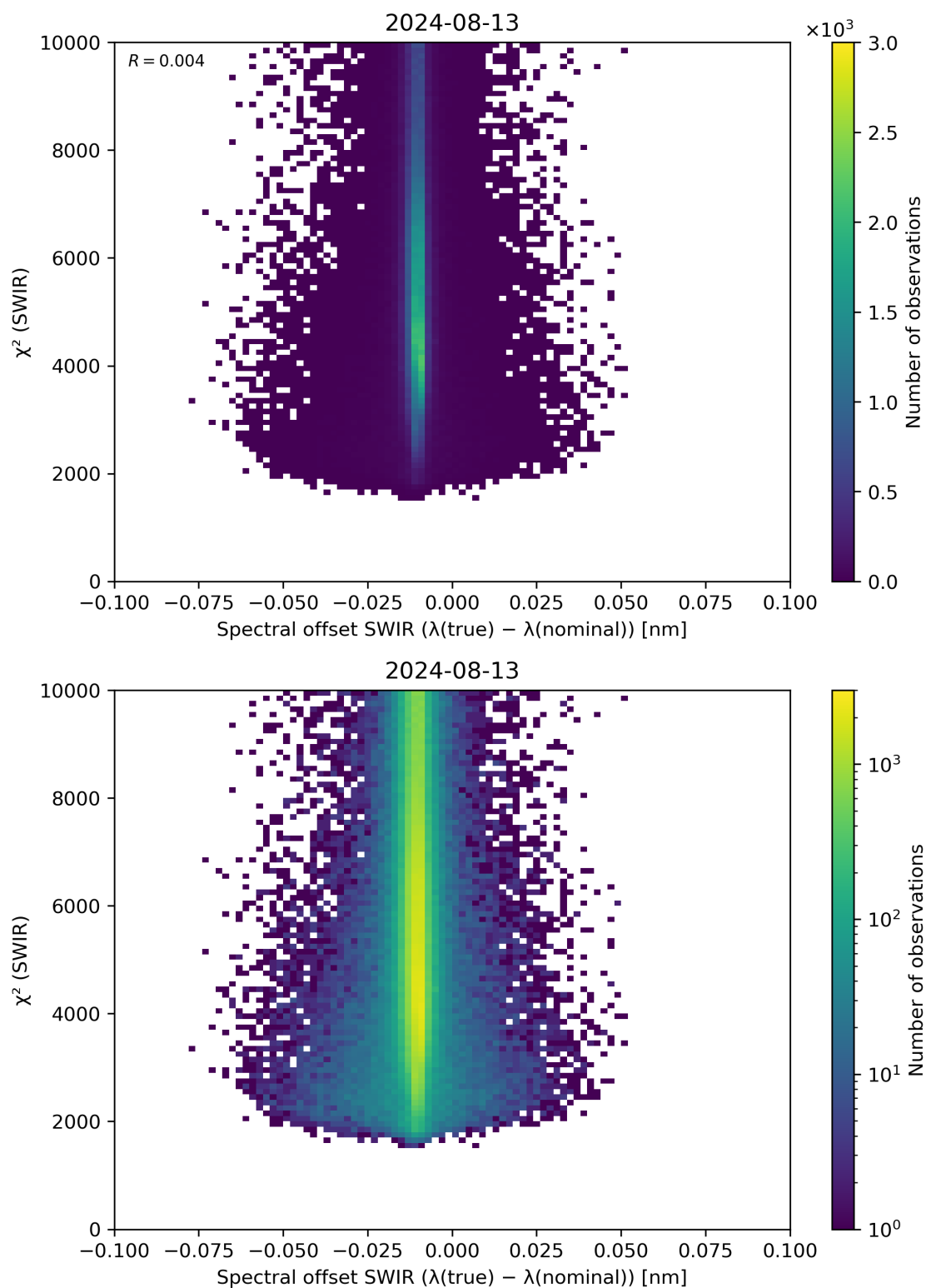
Figure 118: Scatter density plot of “Spectral offset SWIR ( \lambda(\text{true}) - \lambda(\text{nominal}) )” against “ \chi^2 (SWIR)” for 2024-08-12 to 2024-08-14.
