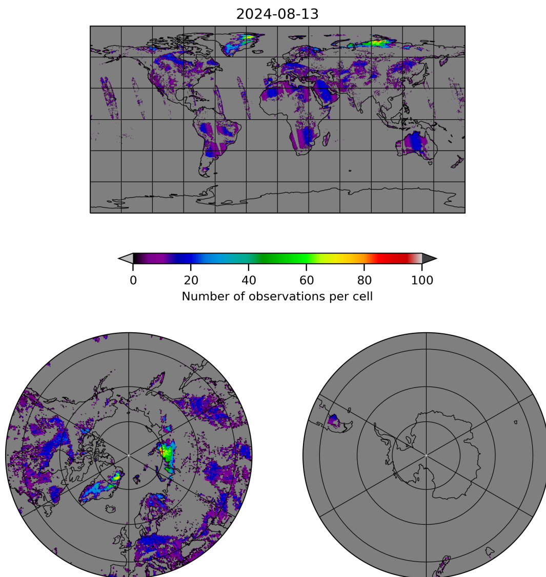
Figure 10: Map of the number of observations for 2024-08-12 to 2024-08-14
