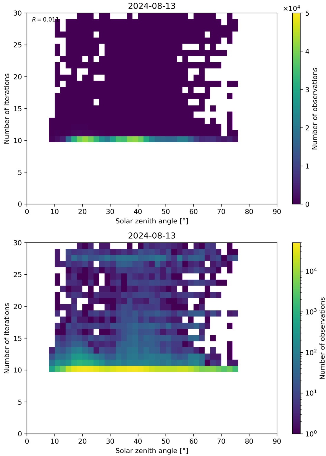
Figure 102: Scatter density plot of “Solar zenith angle” against “Number of iterations” for 2024-08-12 to 2024-08-14.
