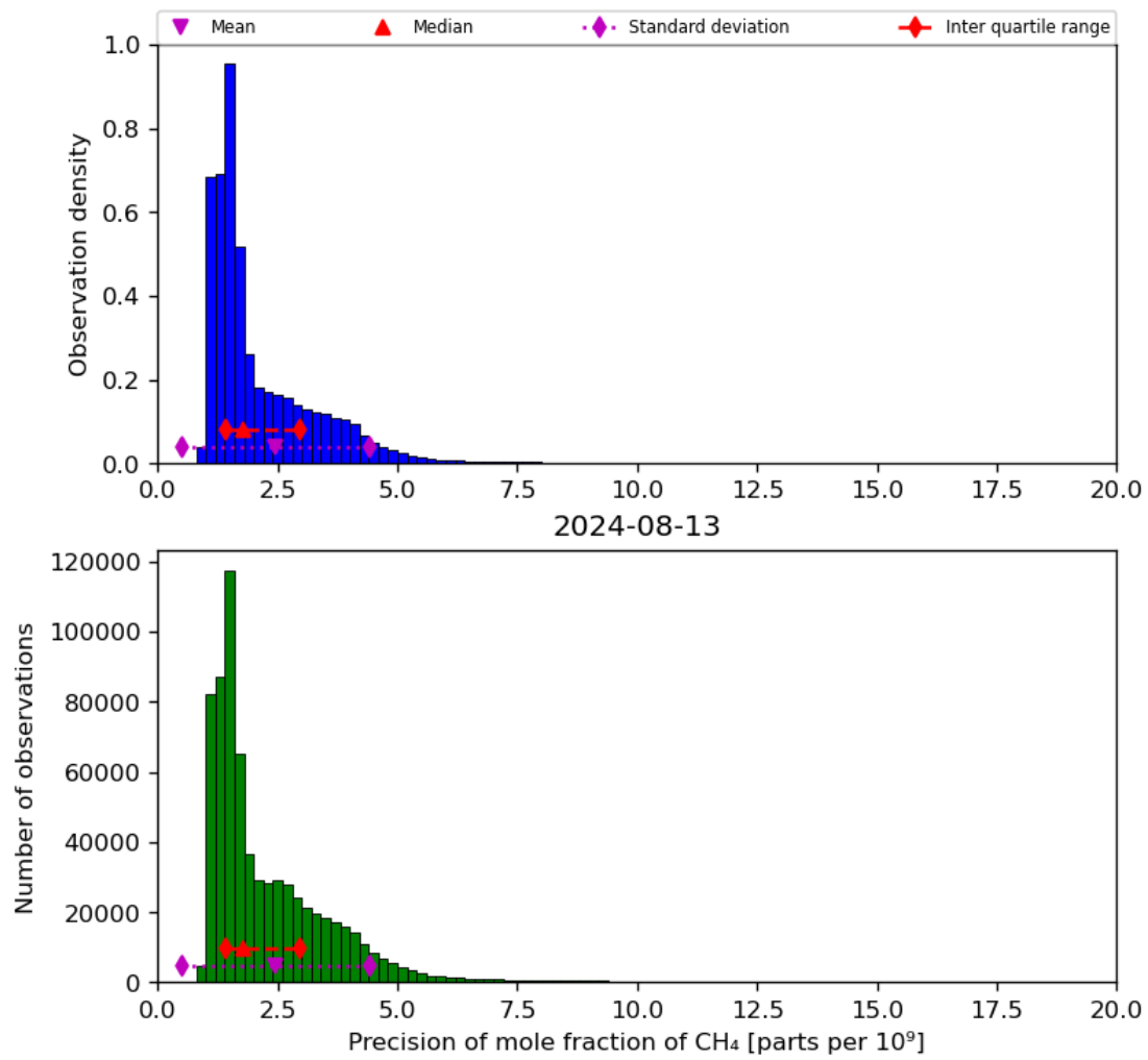
Figure 24: Histogram of “Precision of mole fraction of CH 4 ” for 2024-08-12 to 2024-08-14
