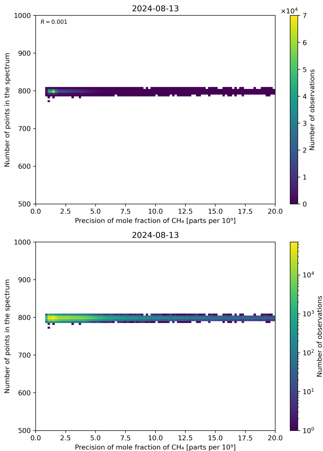
Figure 84: Scatter density plot of “Precision of mole fraction of CH 4 ” against “Number of points in the spectrum” for 2024-08-12 to 2024-08-14.
