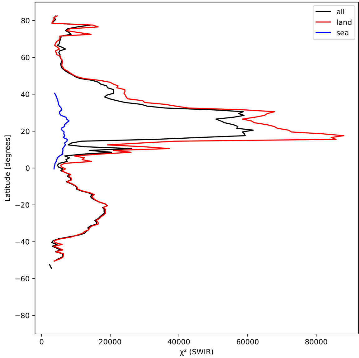
Figure 17: Zonal average of “ \chi^2 (SWIR)” for 2024-08-12 to 2024-08-14.
