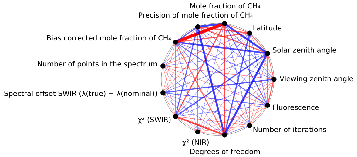
Figure 1: Map of correlation graph for 2024-08-12 to 2024-08-14.
