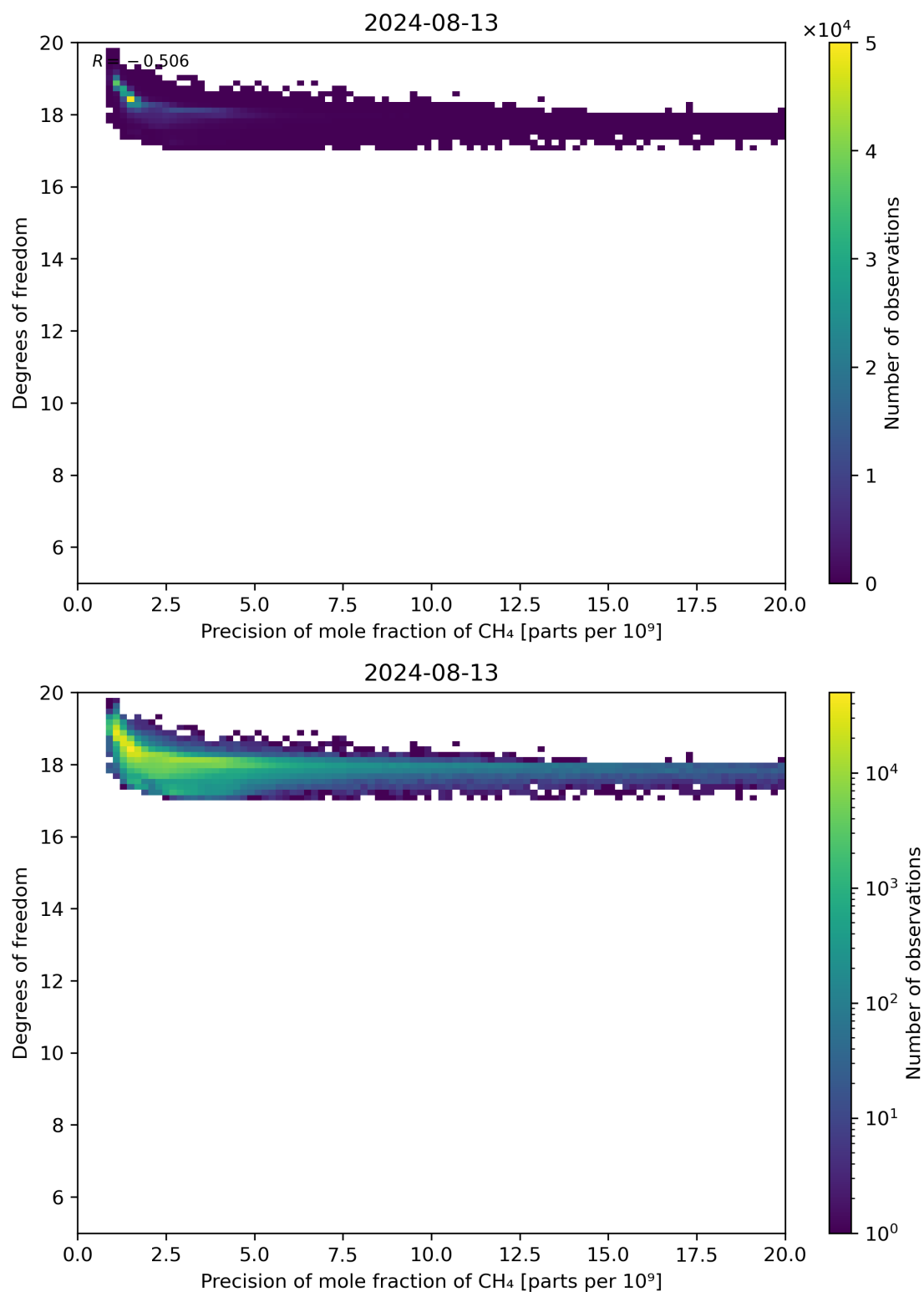
Figure 80: Scatter density plot of “Precision of mole fraction of CH 4 ” against “Degrees of freedom” for 2024-08-12 to 2024-08-14.
