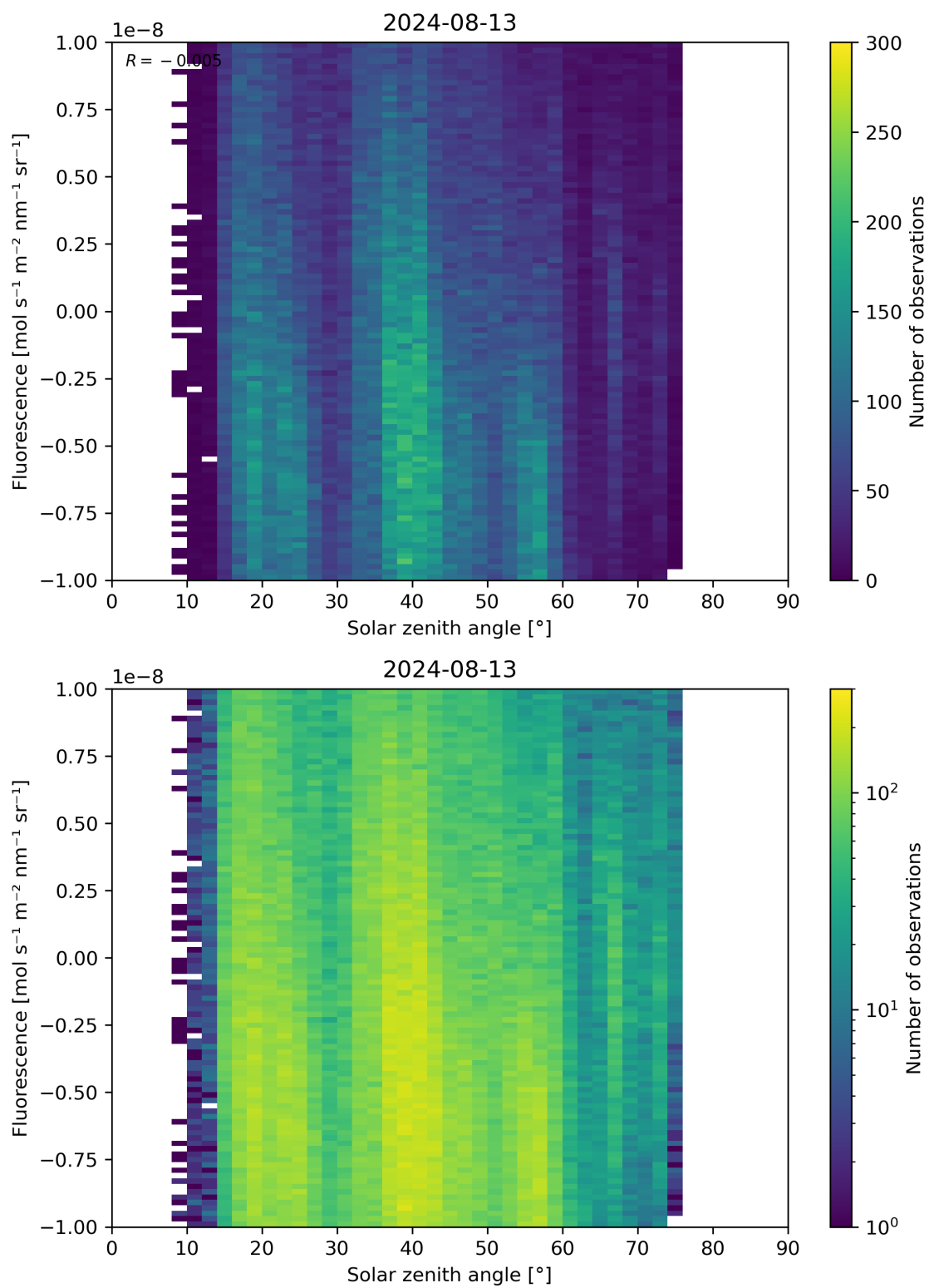
Figure 97: Scatter density plot of “Solar zenith angle” against “Fluorescence” for 2024-08-12 to 2024-08-14.
