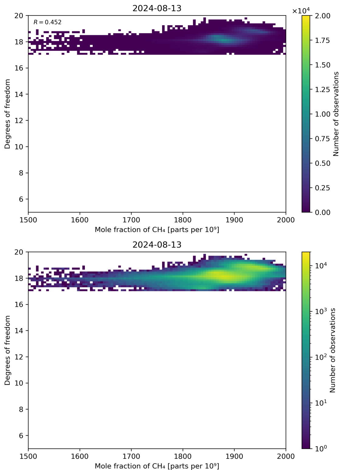
Figure 72: Scatter density plot of “Mole fraction of CH 4 ” against “Degrees of freedom” for 2024-08-12 to 2024-08-14.
