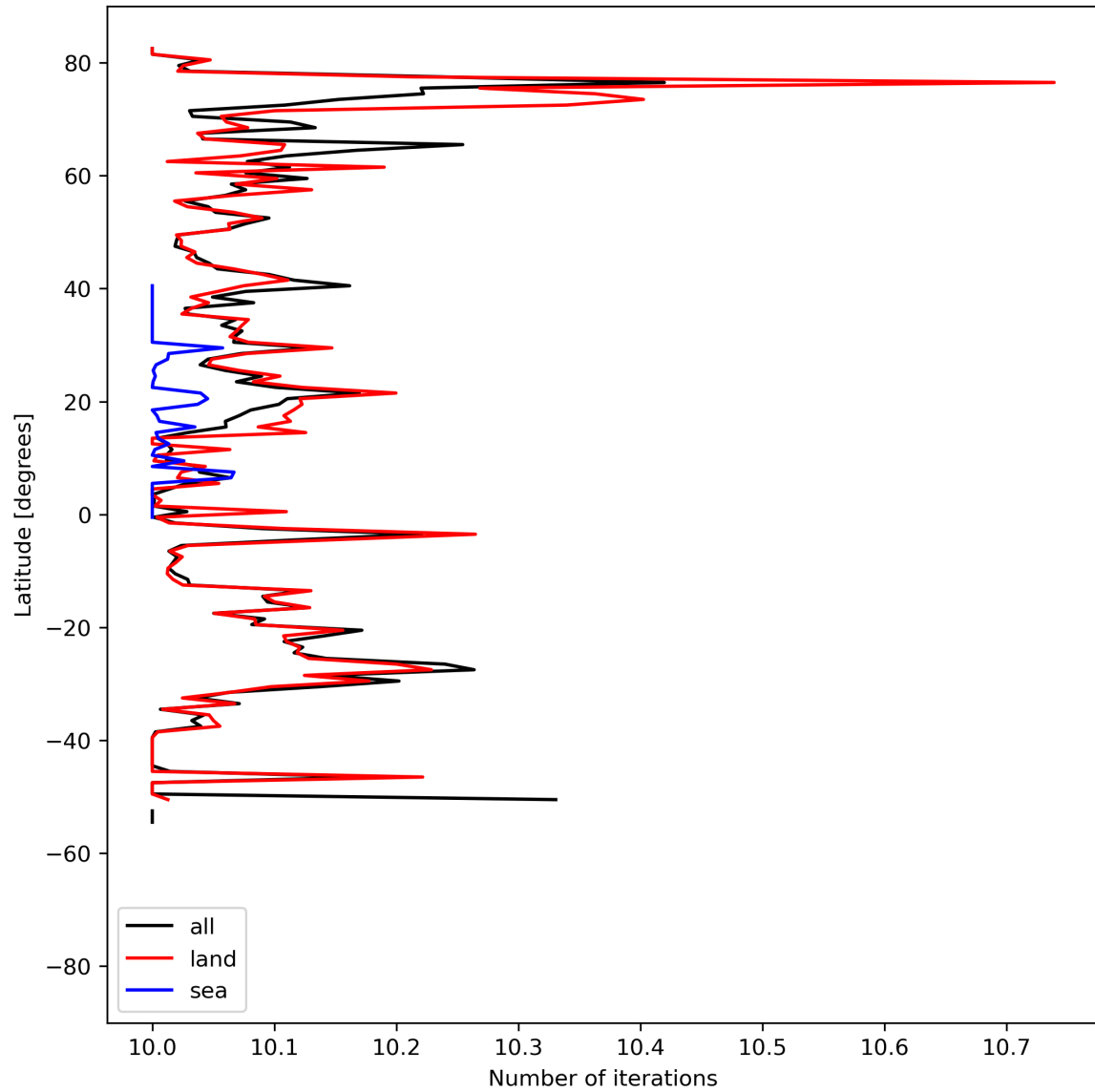
Figure 20: Zonal average of “Number of iterations” for 2024-08-12 to 2024-08-14.
