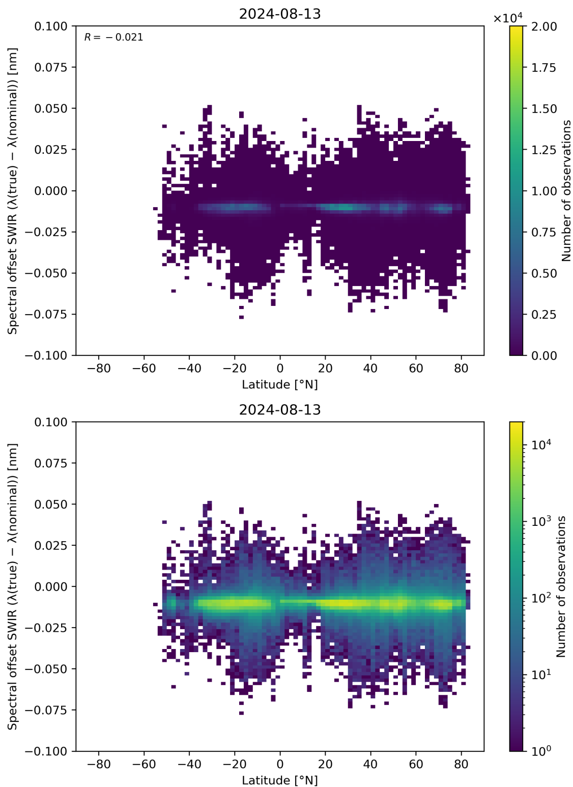
Figure 62: Scatter density plot of “Latitude” against “Spectral offset SWIR ( \lambda(\text{true}) - \lambda(\text{nominal}) )” for 2024-08-12 to 2024-08-14.
