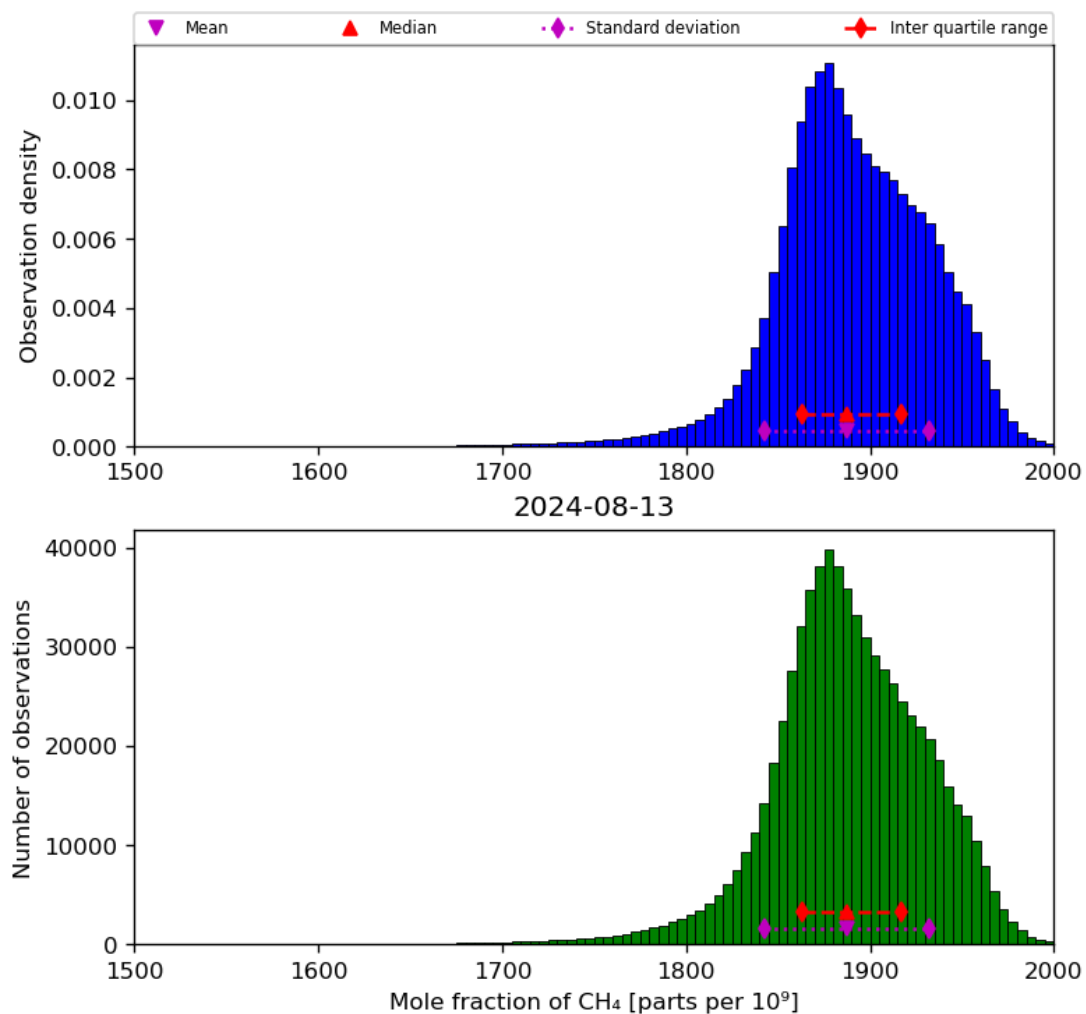
Figure 23: Histogram of “Mole fraction of CH 4 ” for 2024-08-12 to 2024-08-14
