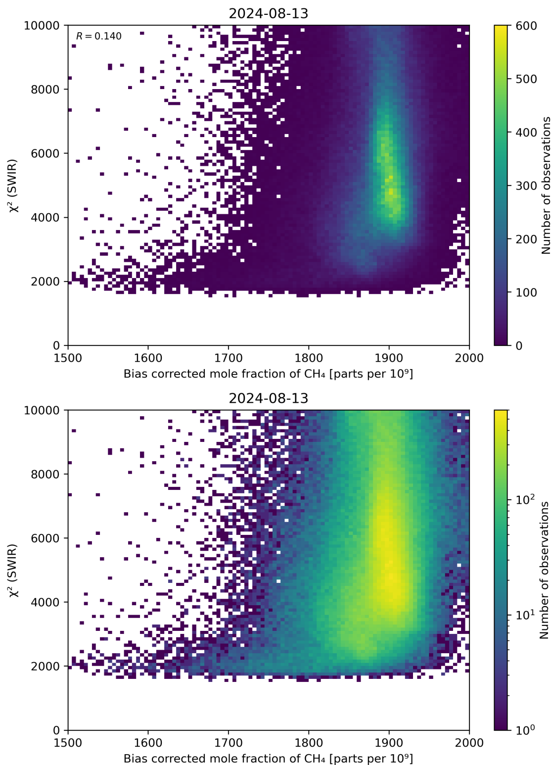
Figure 64: Scatter density plot of “Bias corrected mole fraction of CH 4 ” against “ \chi^2 (SWIR)” for 2024-08-12 to 2024-08-14.
