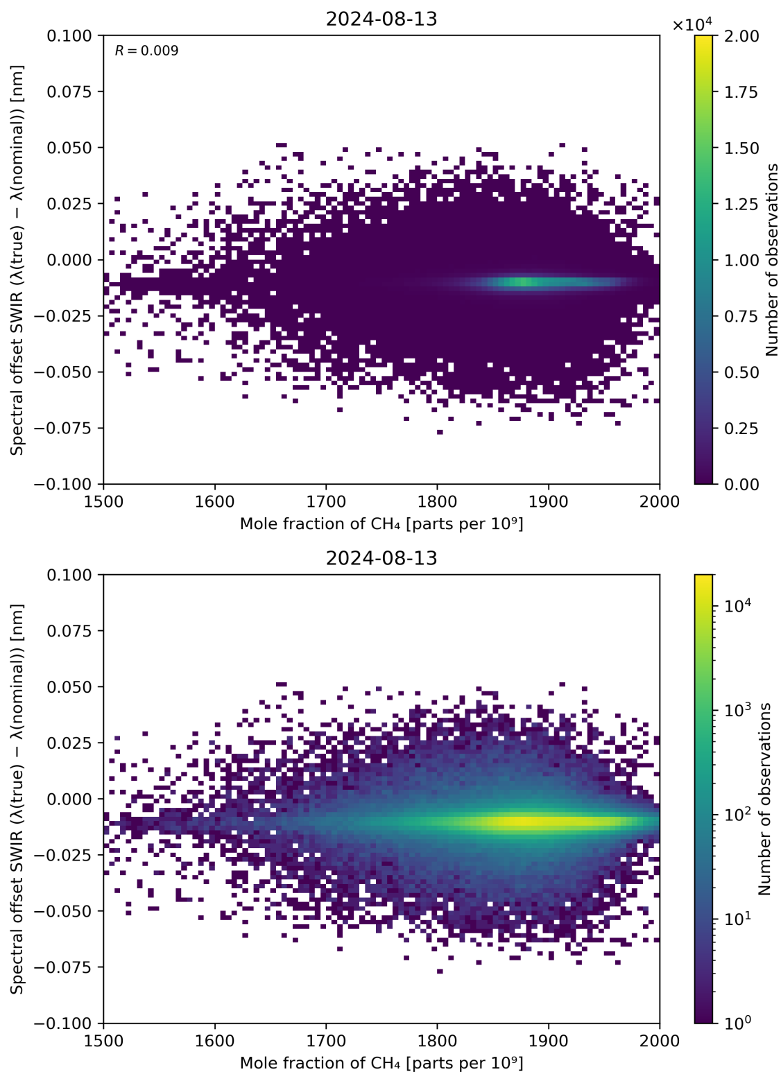
Figure 86: Scatter density plot of “Mole fraction of CH 4 ” against “Spectral offset SWIR ( \lambda(\text{true}) - \lambda(\text{nominal}) )” for 2024-08-12 to 2024-08-14.
