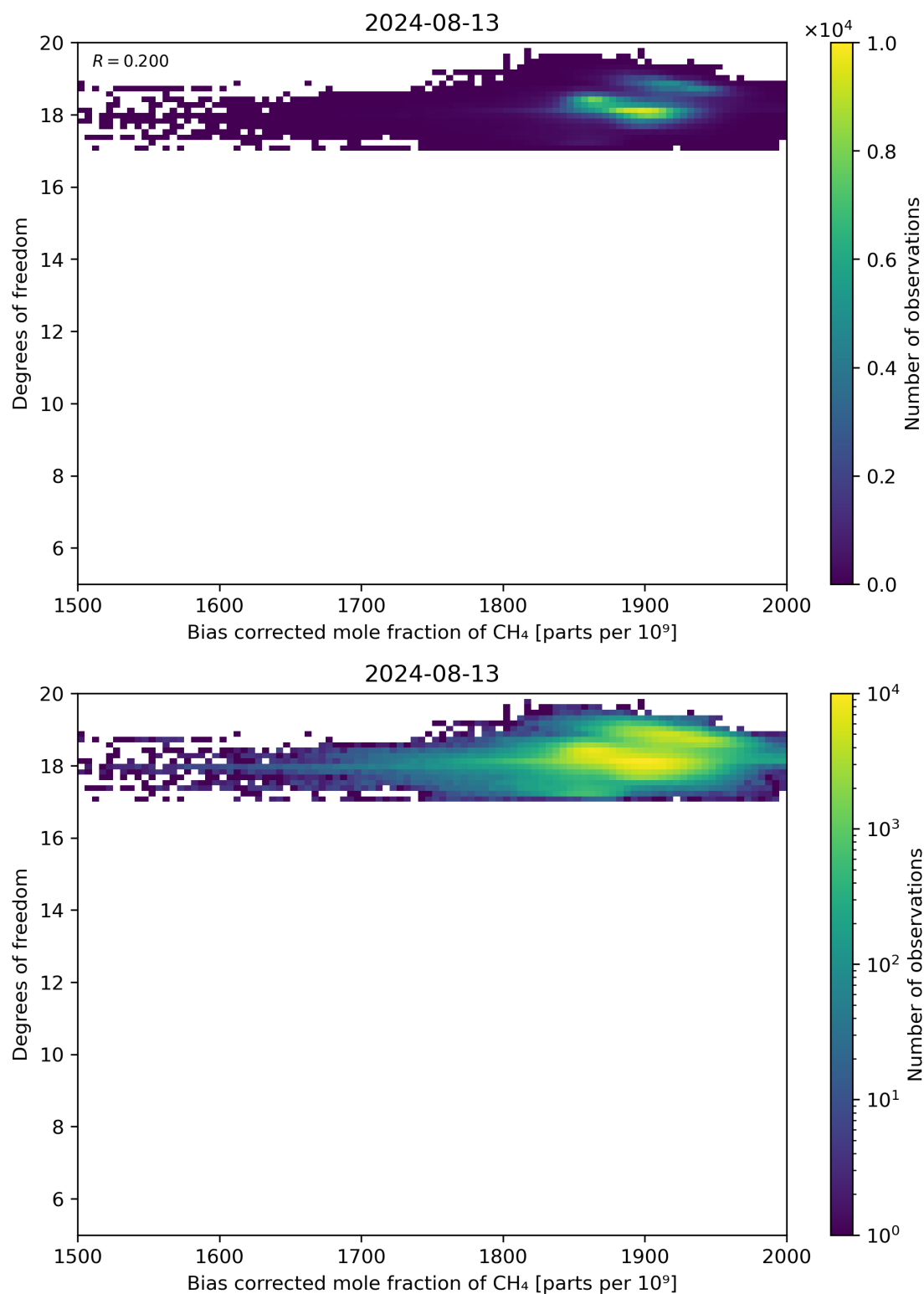
Figure 65: Scatter density plot of “Bias corrected mole fraction of CH 4 ” against “Degrees of freedom” for 2024-08-12 to 2024-08-14.
