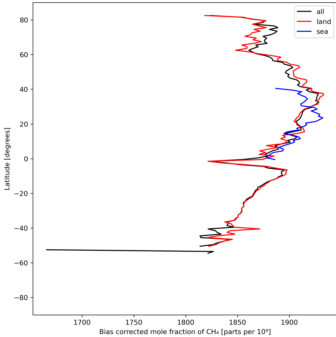
Figure 14: Zonal average of “Bias corrected mole fraction of CH 4 ” for 2024-08-12 to 2024-08-14.
