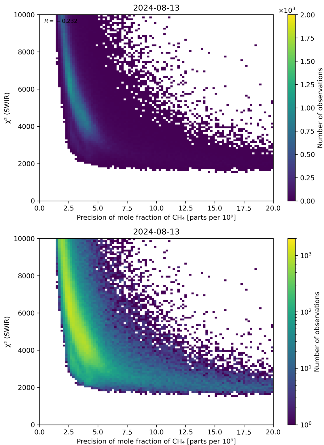
Figure 79: Scatter density plot of “Precision of mole fraction of \text{CH}_4 ” against “ \chi^2 (SWIR)” for 2024-08-12 to 2024-08-14.
