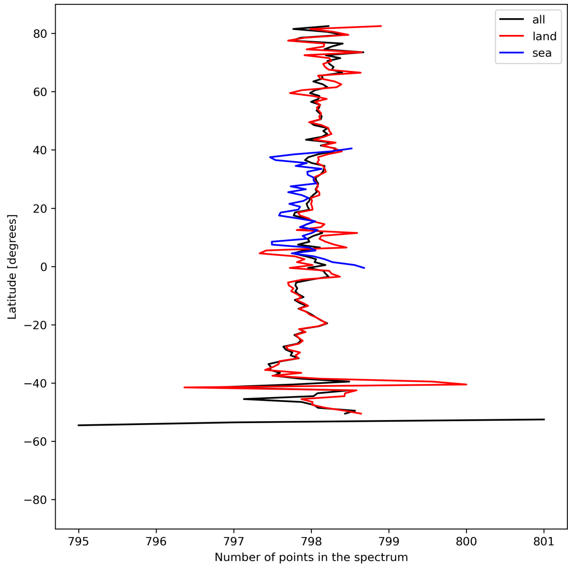
Figure 15: Zonal average of “Number of points in the spectrum” for 2024-08-12 to 2024-08-14.
