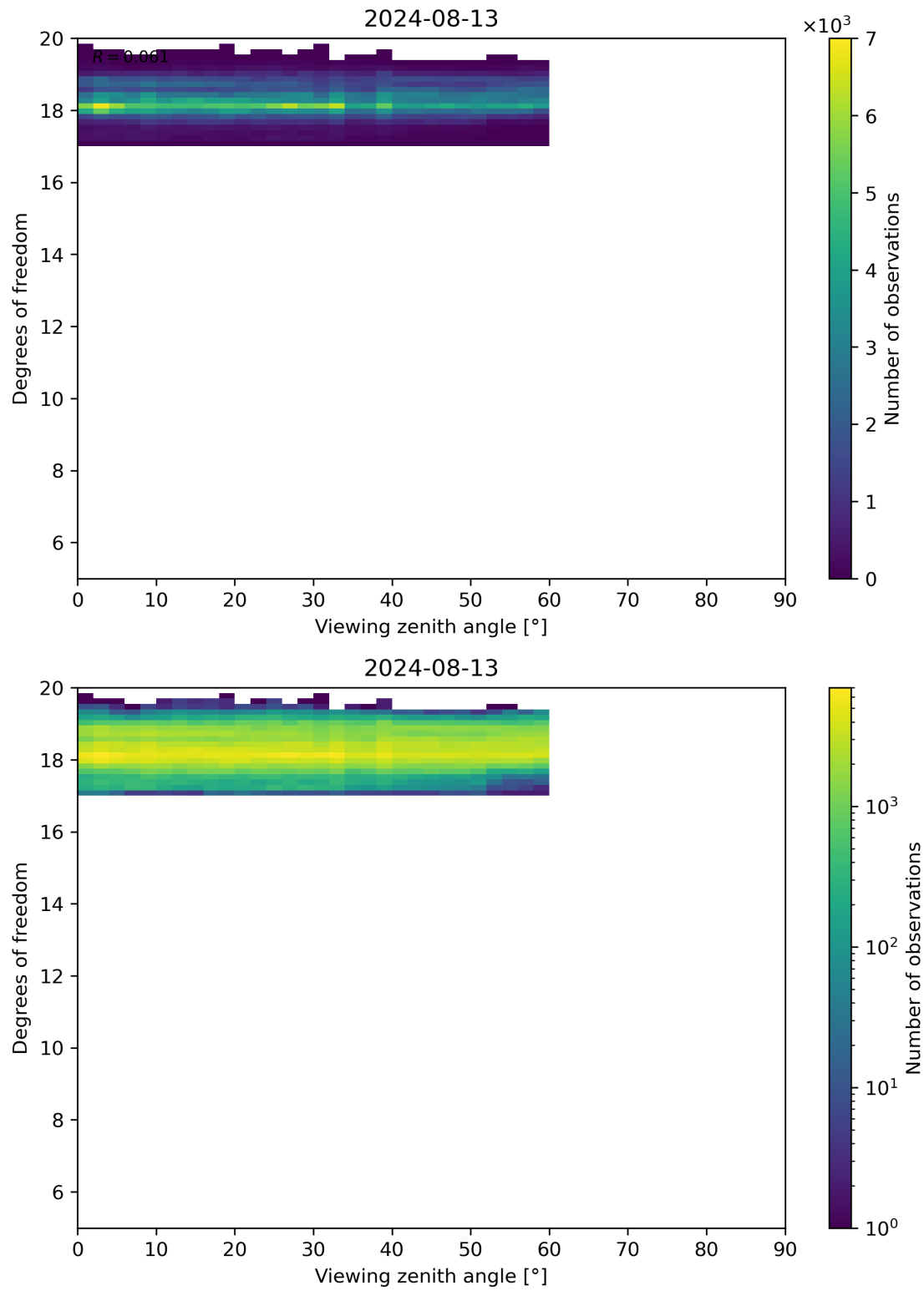
Figure 107: Scatter density plot of “Viewing zenith angle” against “Degrees of freedom” for 2024-08-12 to 2024-08-14.
