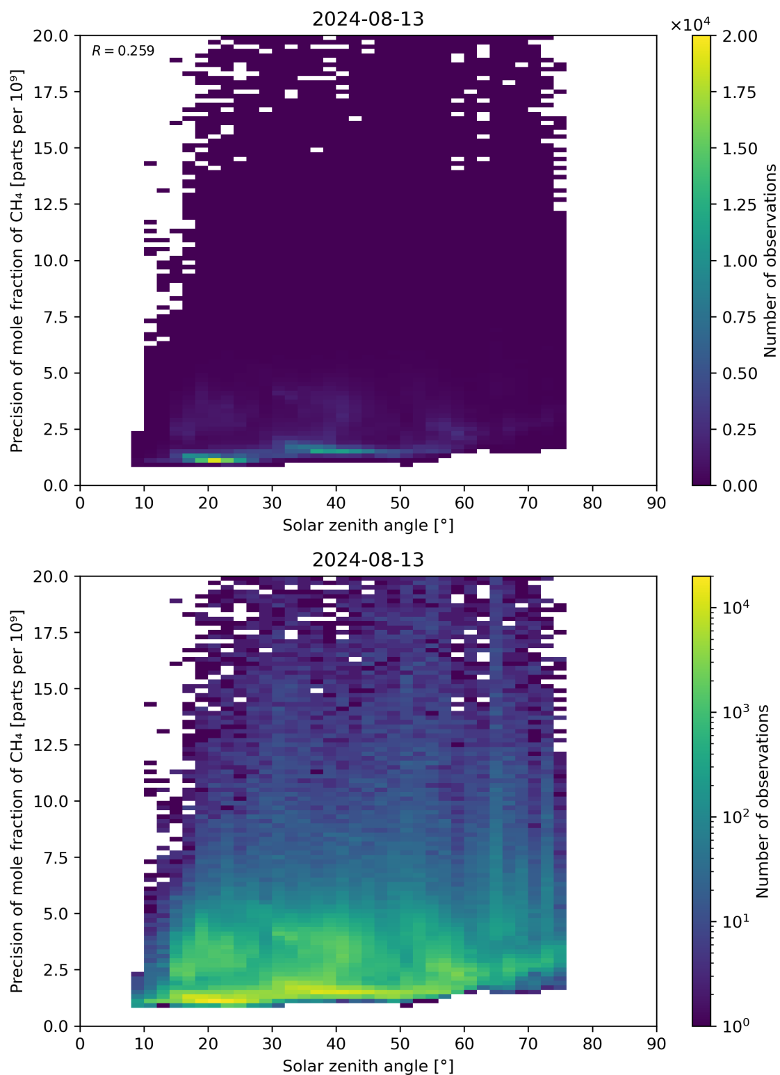
Figure 101: Scatter density plot of “Solar zenith angle” against “Precision of mole fraction of CH 4 ” for 2024-08-12 to 2024-08-14.
