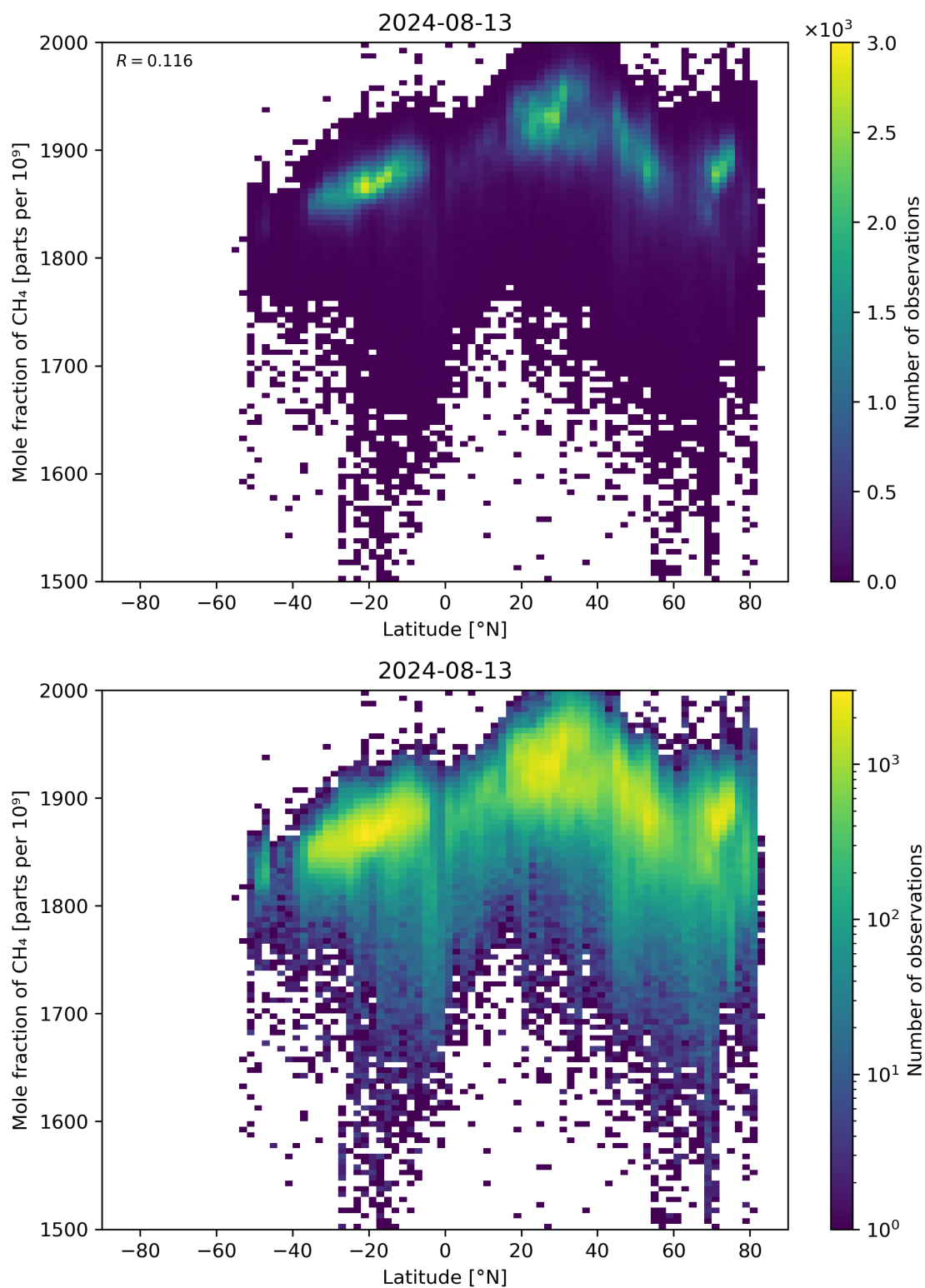
Figure 57: Scatter density plot of “Latitude” against “Mole fraction of CH 4 ” for 2024-08-12 to 2024-08-14.
