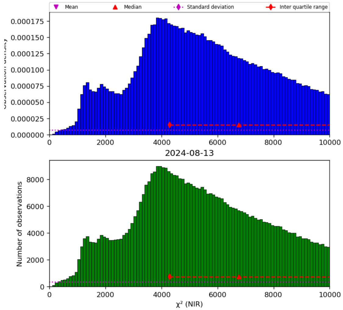
Figure 29: Histogram of “ \chi^2 (NIR)” for 2024-08-12 to 2024-08-14
