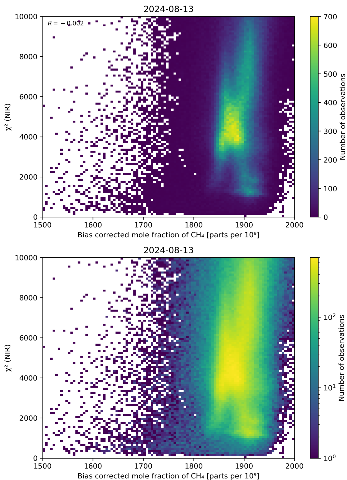
Figure 63: Scatter density plot of “Bias corrected mole fraction of \text{CH}_4 ” against “ \chi^2 (NIR)” for 2024-08-12 to 2024-08-14.
