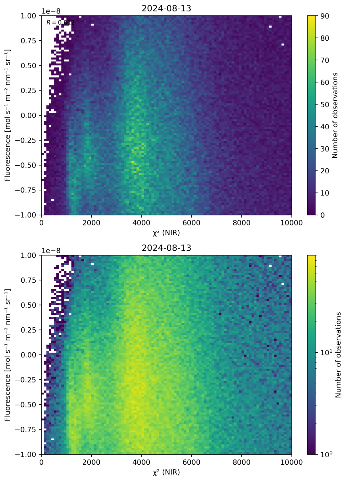
Figure 45: Scatter density plot of “ \chi^2 (NIR)” against “Fluorescence” for 2024-08-12 to 2024-08-14.
