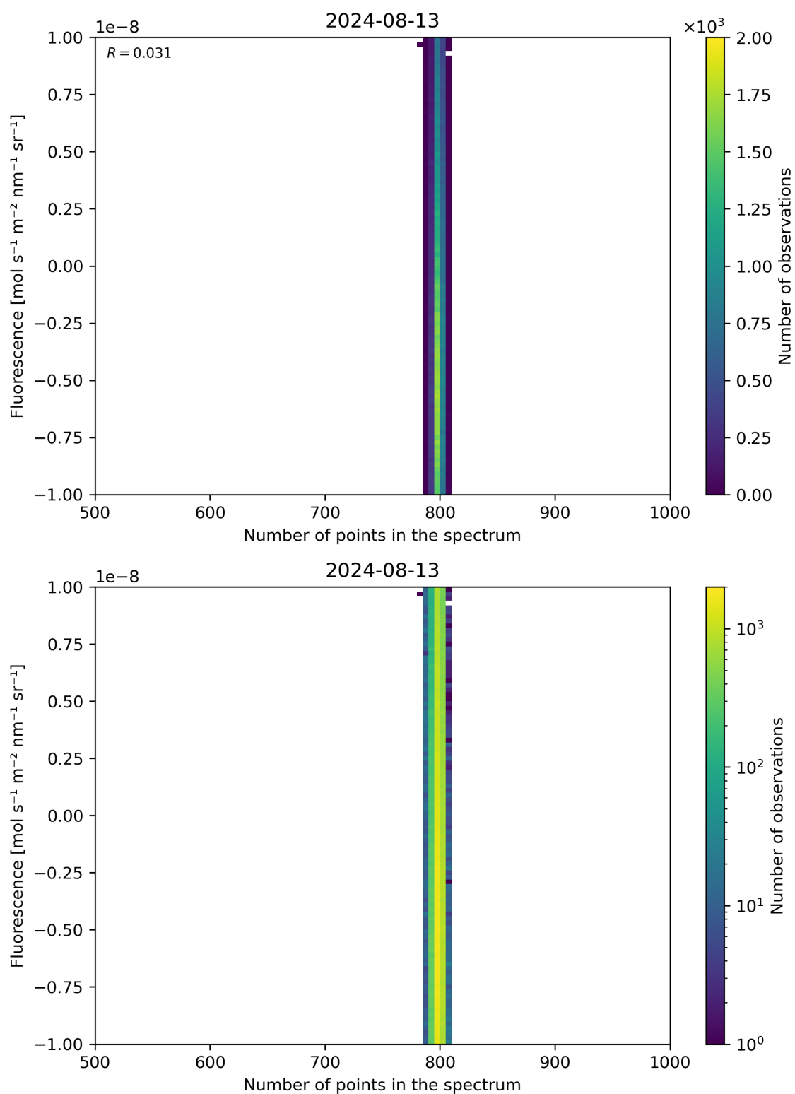
Figure 91: Scatter density plot of “Number of points in the spectrum” against “Fluorescence” for 2024-08-12 to 2024-08-14.
