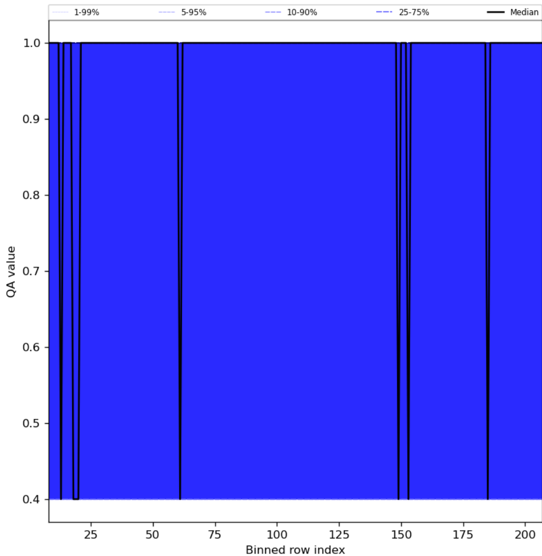
Figure 33: Along track statistics of “QA value” for 2024-08-12 to 2024-08-14
