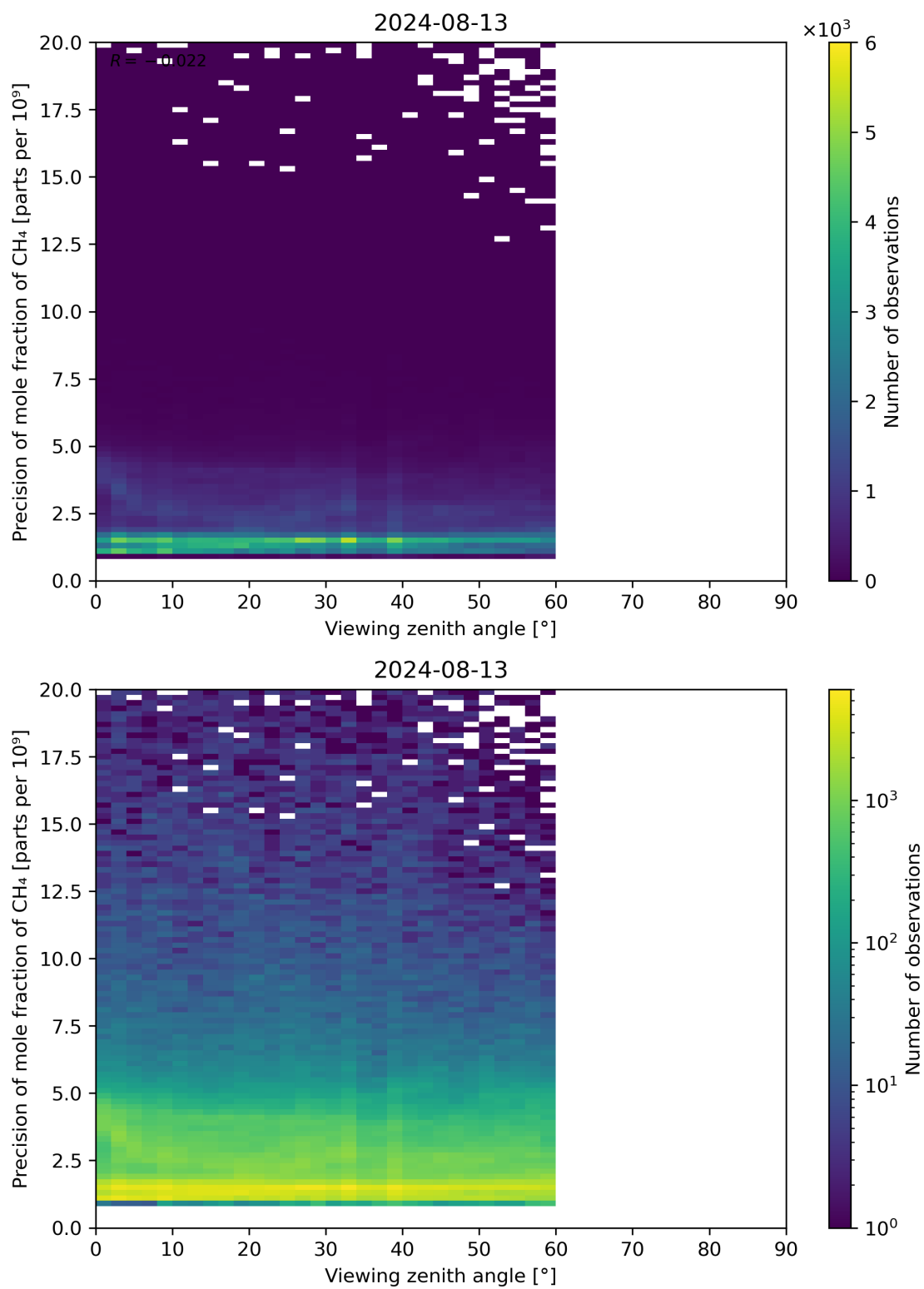
Figure 112: Scatter density plot of “Viewing zenith angle” against “Precision of mole fraction of \text{CH}_4 ” for 2024-08-12 to 2024-08-14.
