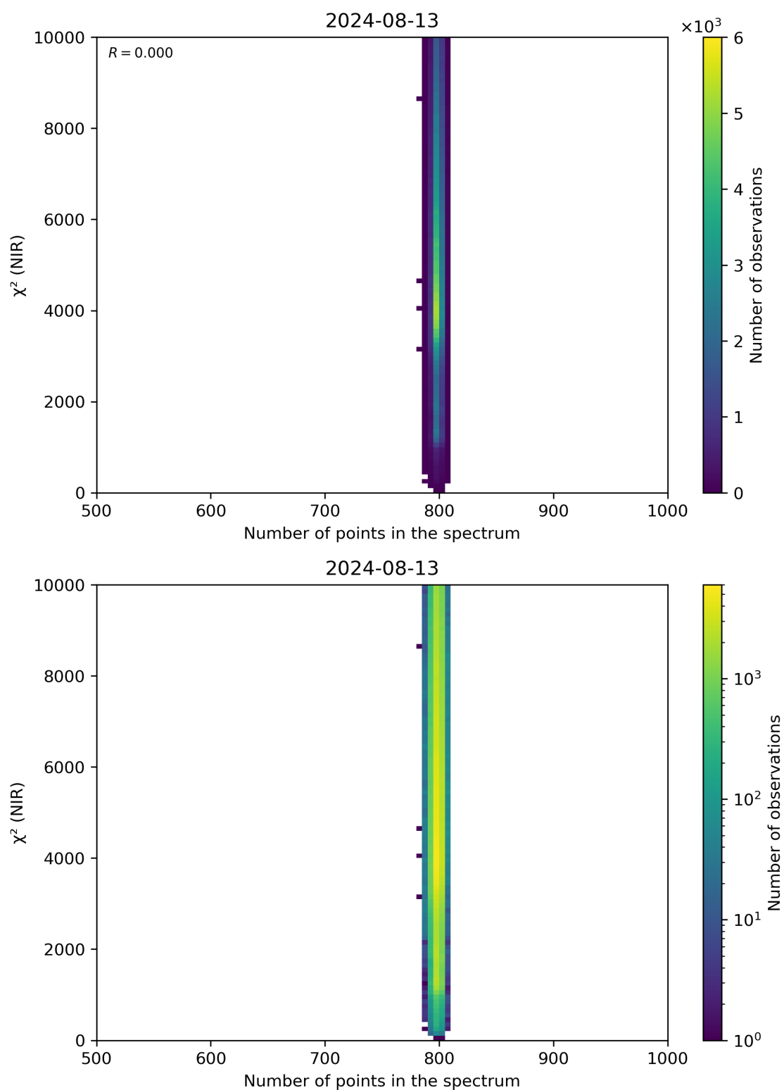
Figure 88: Scatter density plot of “Number of points in the spectrum” against “ \chi^2 (NIR)” for 2024-08-12 to 2024-08-14.
