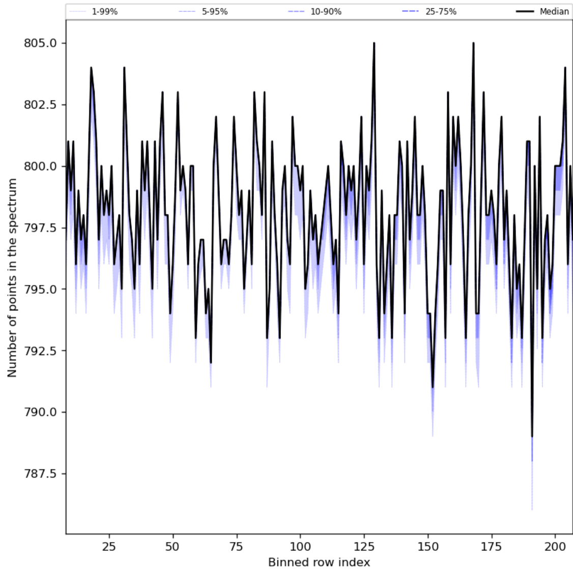
Figure 37: Along track statistics of “Number of points in the spectrum” for 2024-08-12 to 2024-08-14
