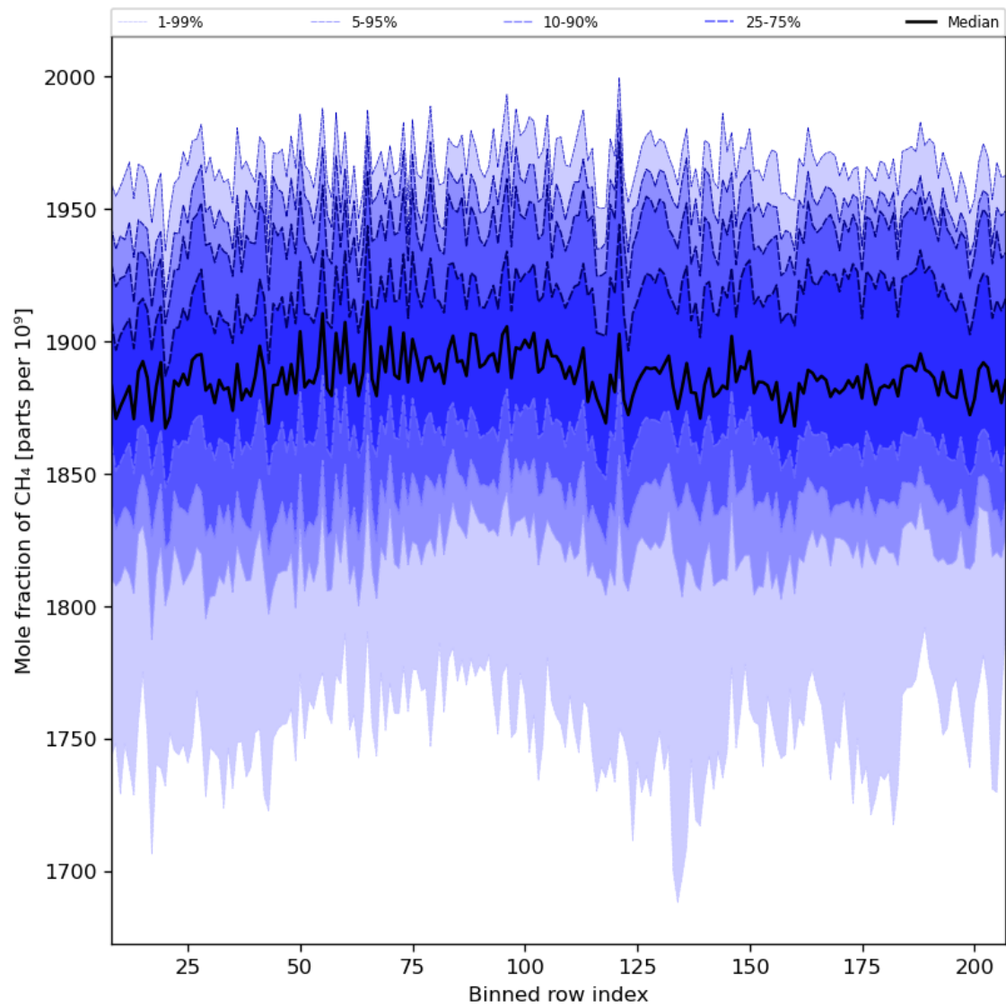
Figure 34: Along track statistics of “Mole fraction of CH 4 ” for 2024-08-12 to 2024-08-14
