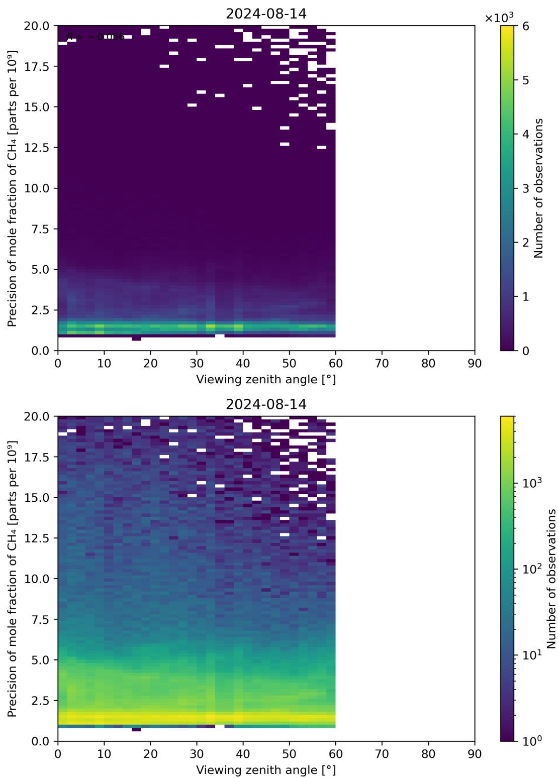
Figure 112: Scatter density plot of “Viewing zenith angle” against “Precision of mole fraction of CH 4 ” for 2024-08-13 to 2024-08-15.
