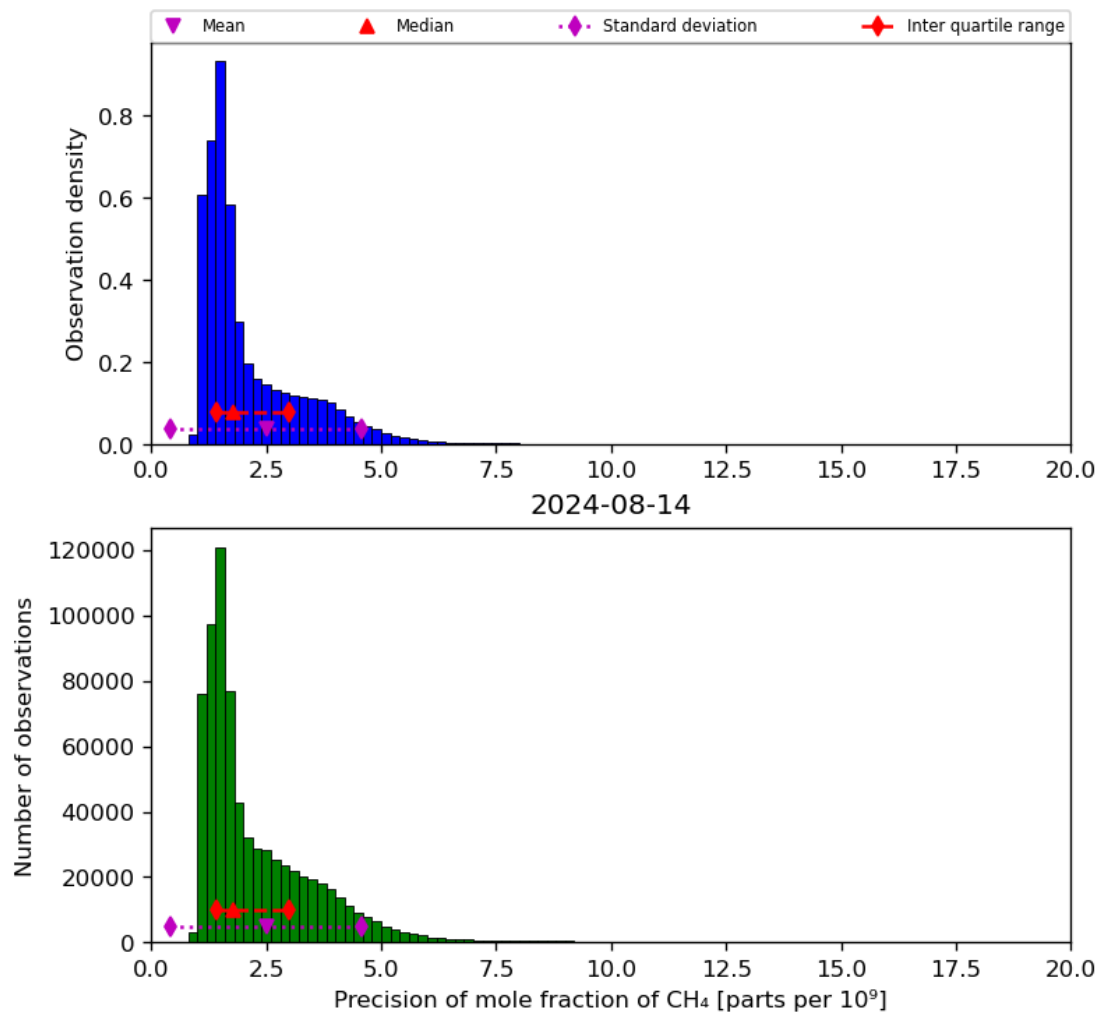
Figure 24: Histogram of “Precision of mole fraction of CH 4 ” for 2024-08-13 to 2024-08-15
