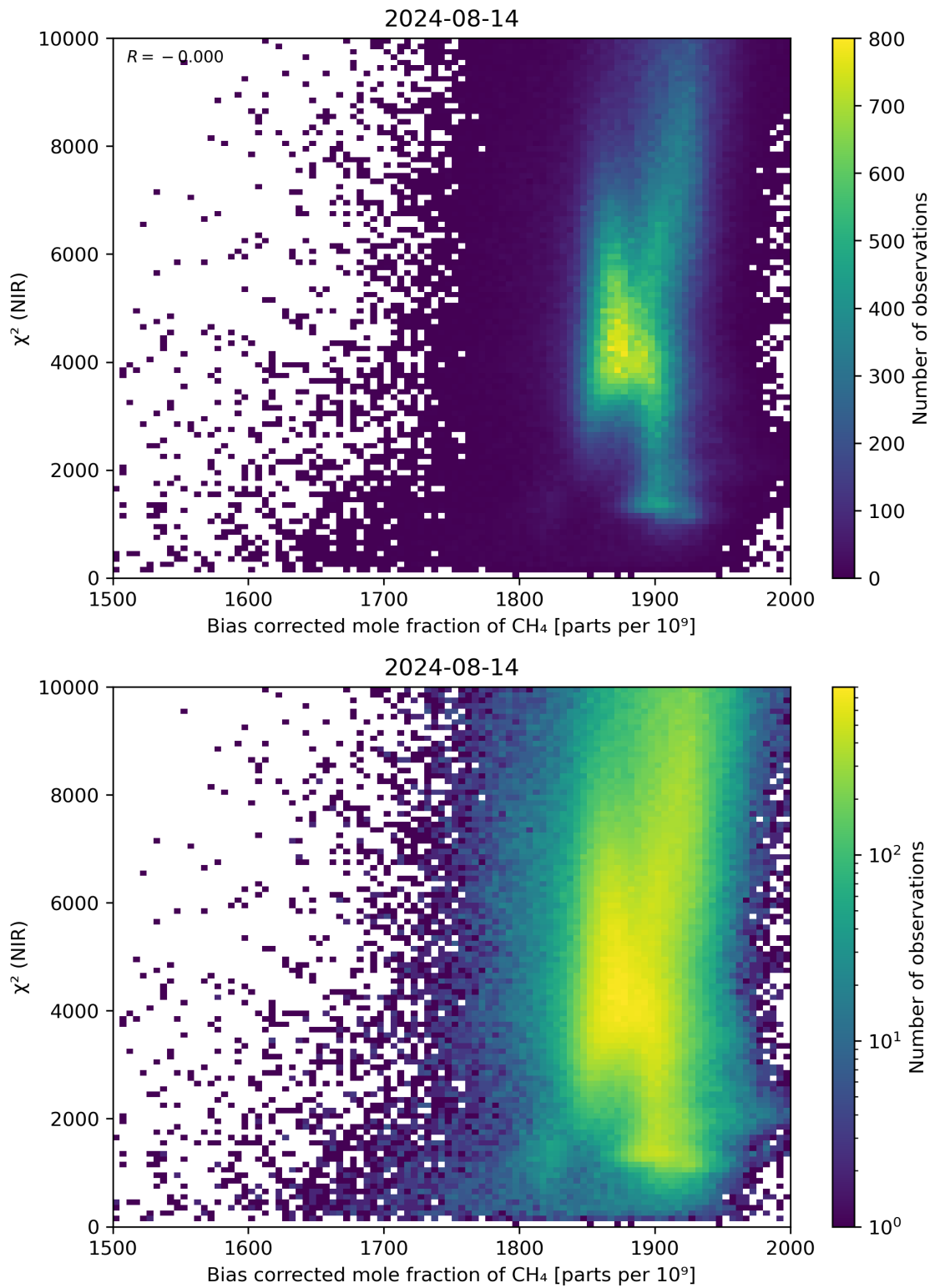
Figure 63: Scatter density plot of “Bias corrected mole fraction of CH 4 ” against “ \chi^2 (NIR)” for 2024-08-13 to 2024-08-15.
