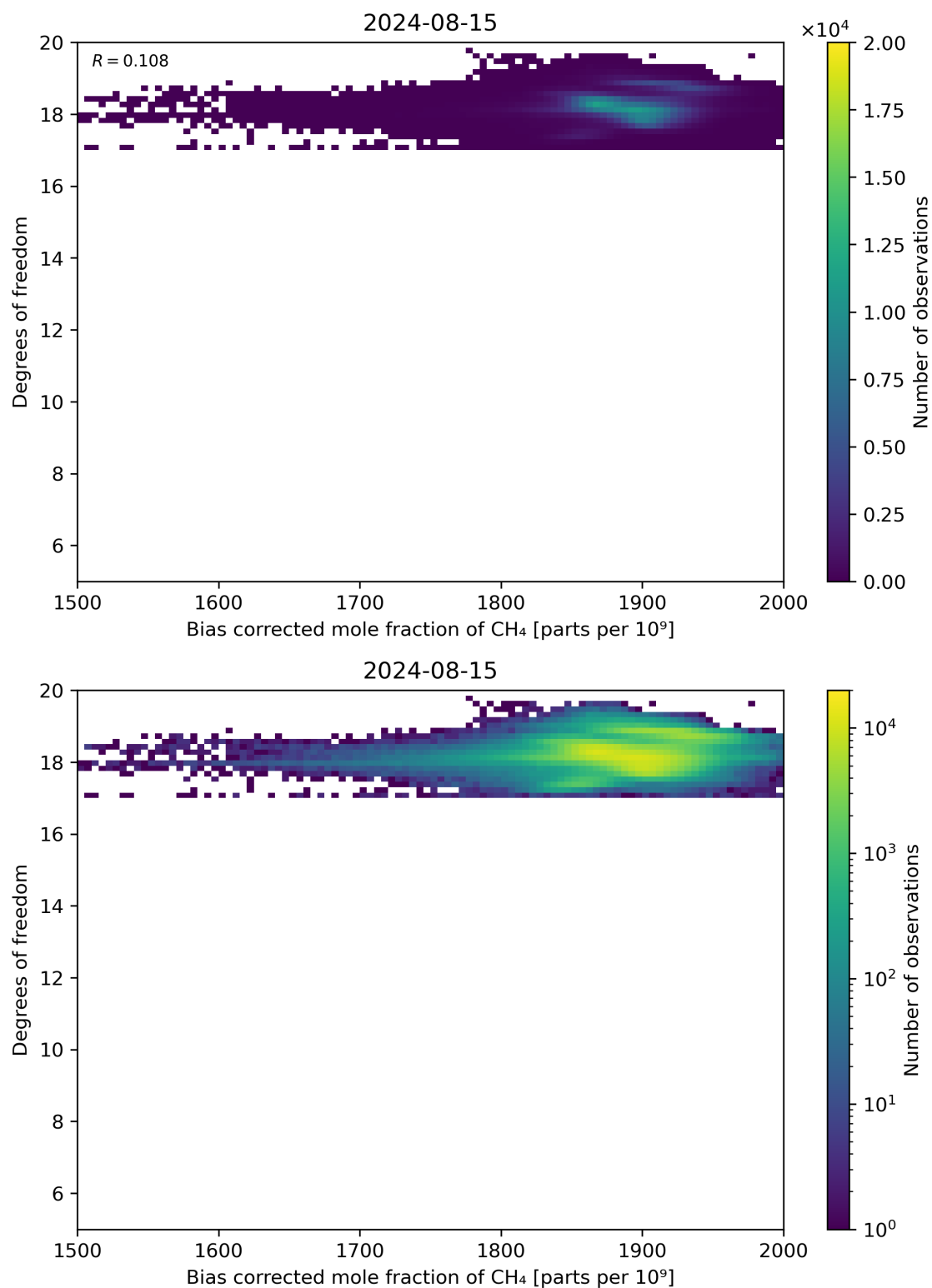
Figure 65: Scatter density plot of “Bias corrected mole fraction of CH 4 ” against “Degrees of freedom” for 2024-08-14 to 2024-08-16.
