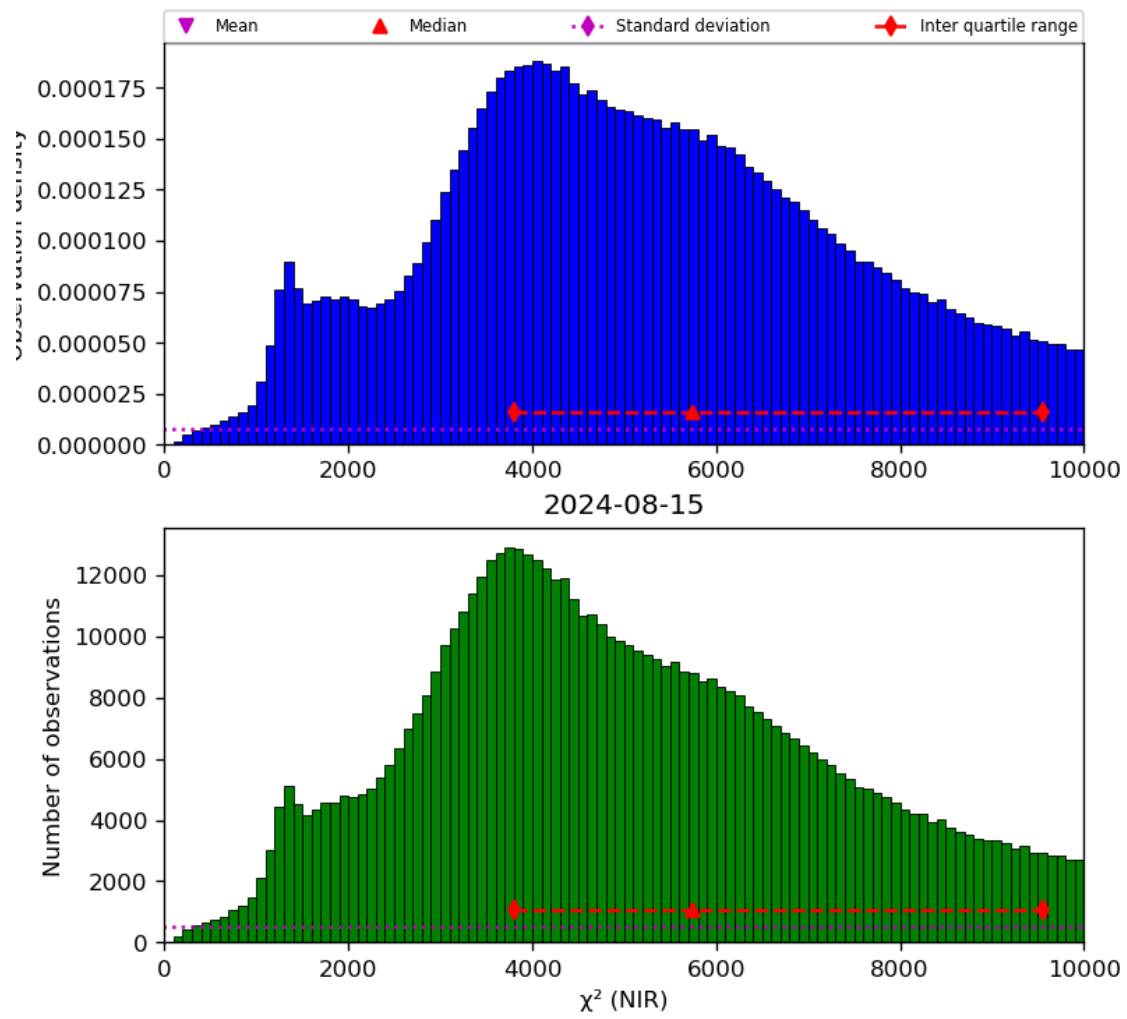
Figure 29: Histogram of “ \chi^2 (NIR)” for 2024-08-14 to 2024-08-16
