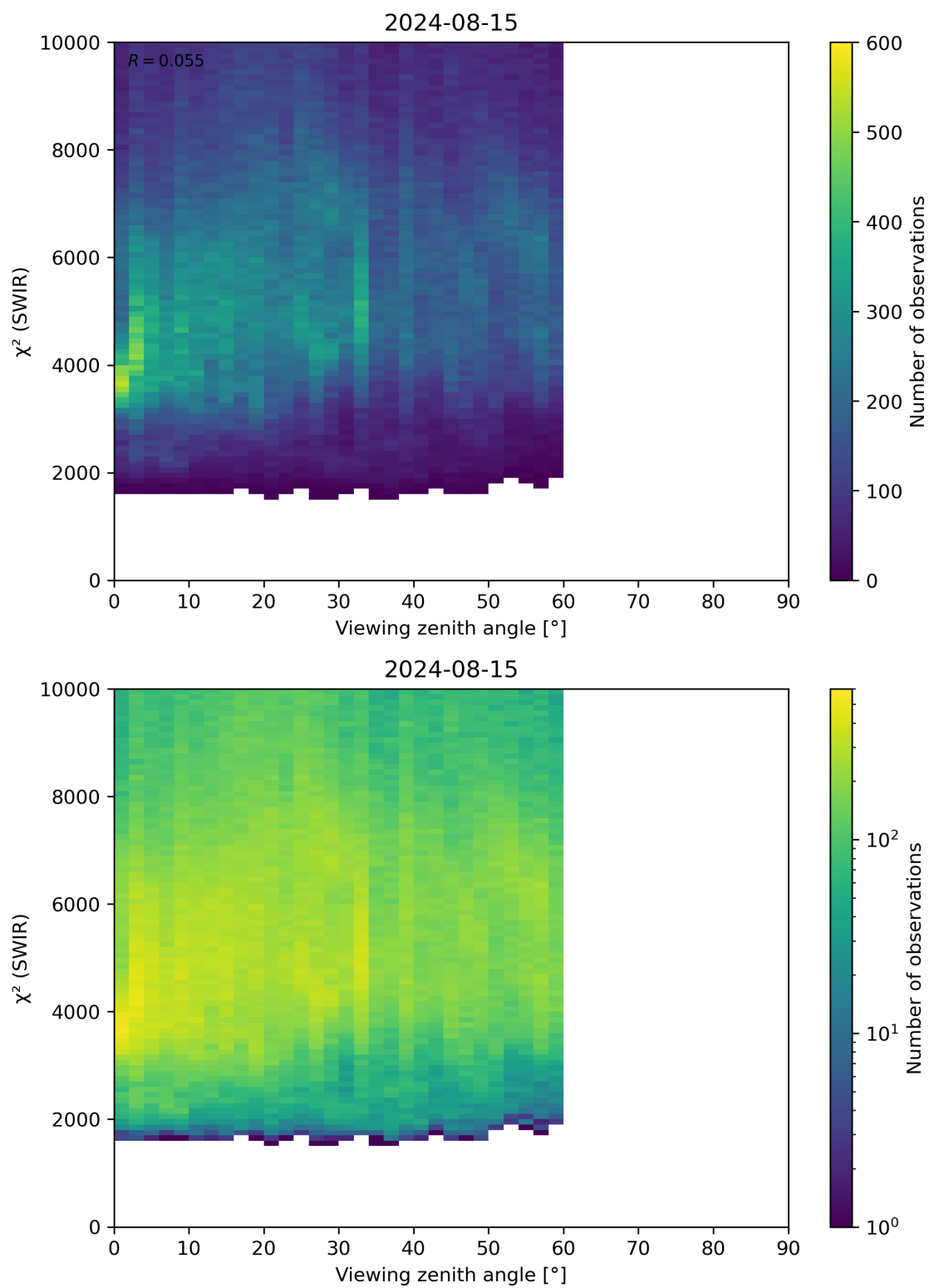
Figure 106: Scatter density plot of “Viewing zenith angle” against “ \chi^2 (SWIR)” for 2024-08-14 to 2024-08-16.
