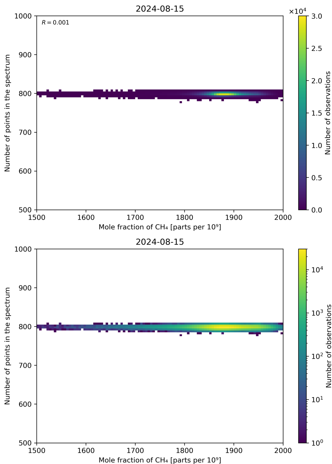
Figure 77: Scatter density plot of “Mole fraction of CH 4 ” against “Number of points in the spectrum” for 2024-08-14 to 2024-08-16.
