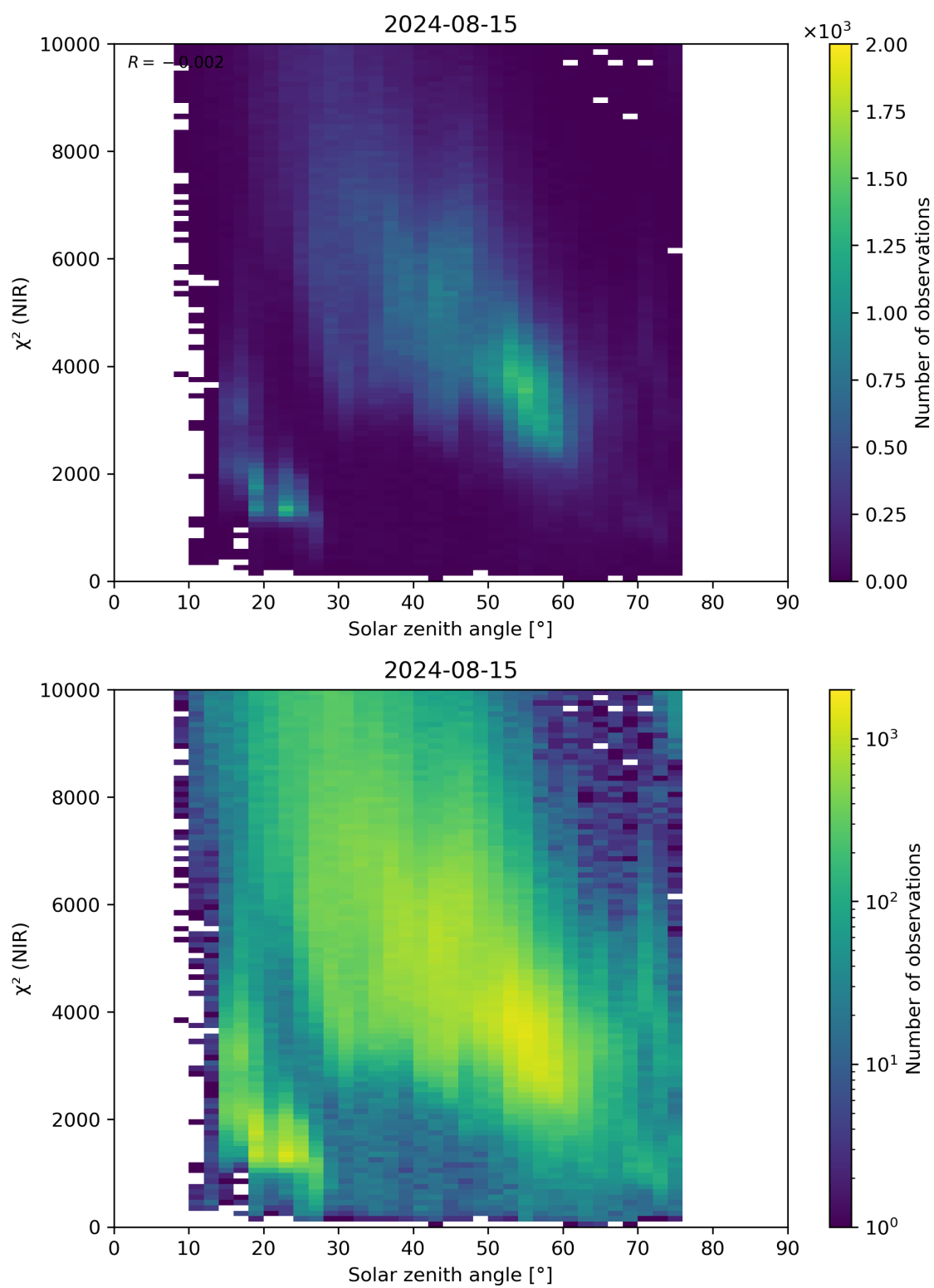
Figure 94: Scatter density plot of “Solar zenith angle” against “ \chi^2 (NIR)” for 2024-08-14 to 2024-08-16.
