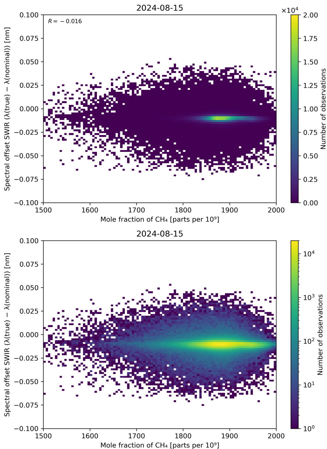
Figure 86: Scatter density plot of “Mole fraction of CH 4 ” against “Spectral offset SWIR ( \lambda(\text{true}) - \lambda(\text{nominal}) )” for 2024-08-14 to 2024-08-16.
