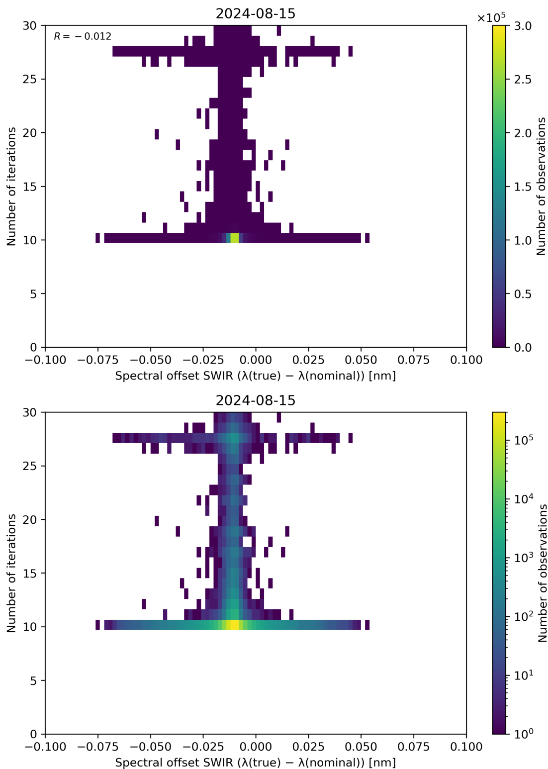
Figure 121: Scatter density plot of “Spectral offset SWIR ( \lambda(\text{true}) - \lambda(\text{nominal}) )” against “Number of iterations” for 2024-08-14 to 2024-08-16.
