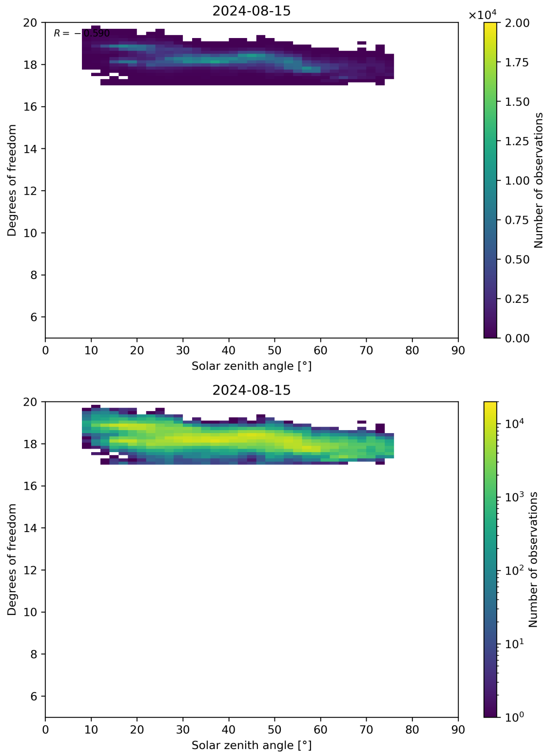
Figure 96: Scatter density plot of “Solar zenith angle” against “Degrees of freedom” for 2024-08-14 to 2024-08-16.
