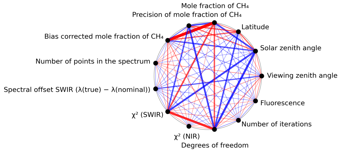
Figure 1: Map of correlation graph for 2024-08-14 to 2024-08-16.
