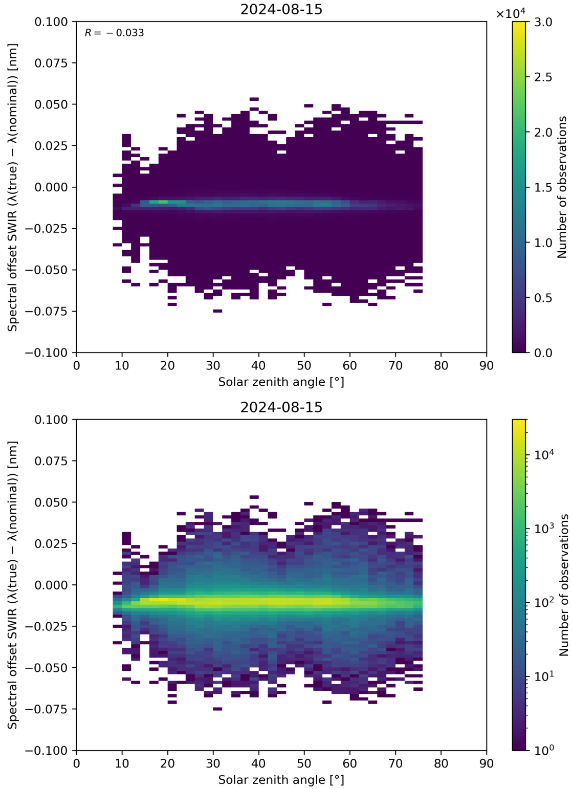
Figure 104: Scatter density plot of “Solar zenith angle” against “Spectral offset SWIR ( \lambda(\text{true}) - \lambda(\text{nominal}) )” for 2024-08-14 to 2024-08-16.
