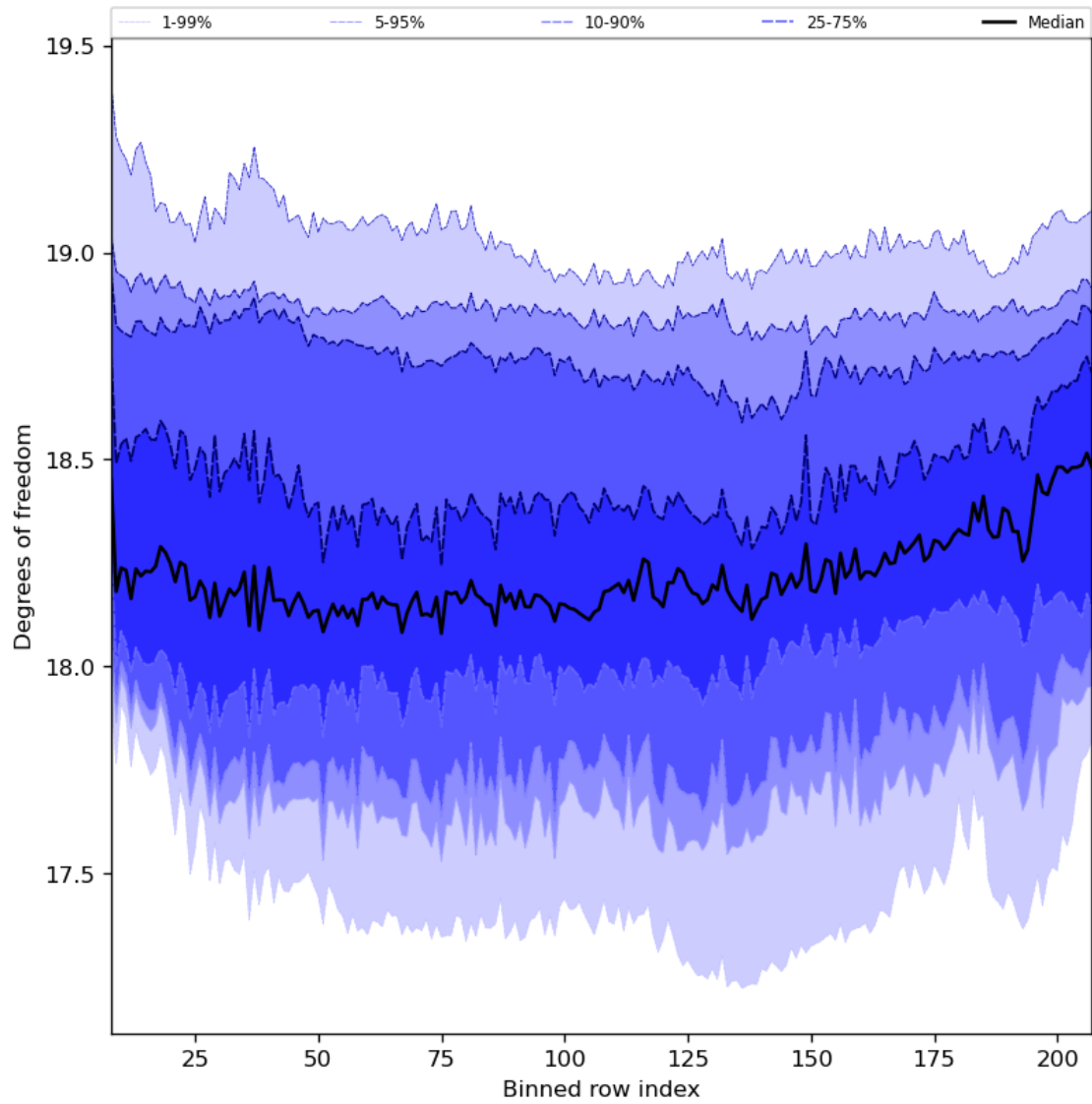
Figure 41: Along track statistics of “Degrees of freedom” for 2024-08-14 to 2024-08-16
