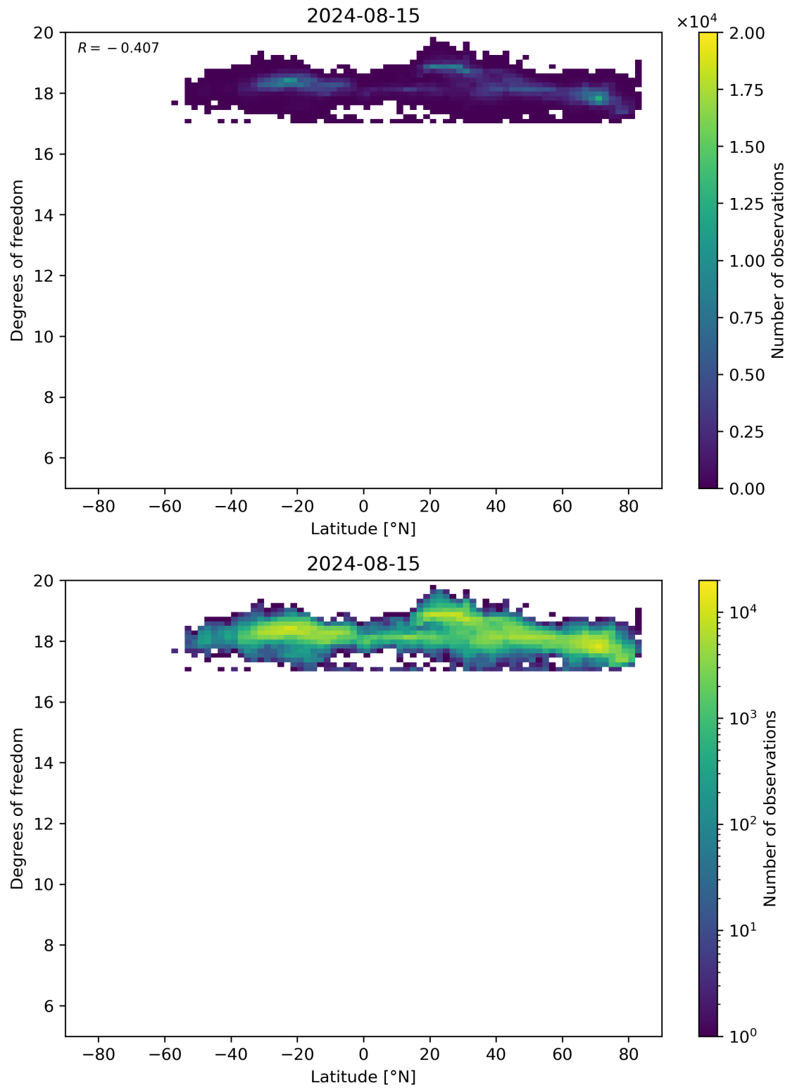
Figure 55: Scatter density plot of “Latitude” against “Degrees of freedom” for 2024-08-14 to 2024-08-16.
