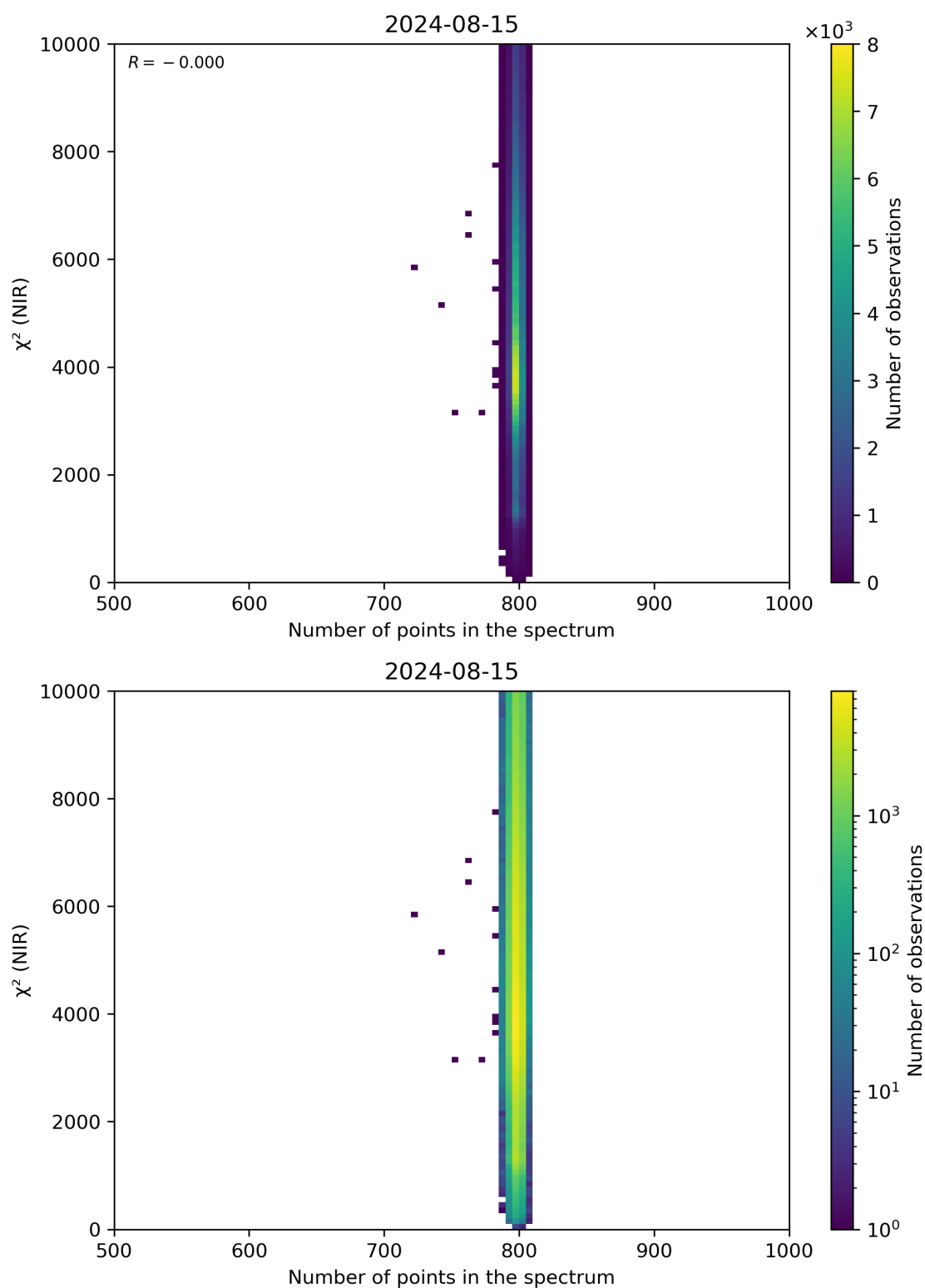
Figure 88: Scatter density plot of “Number of points in the spectrum” against “ \chi^2 (NIR)” for 2024-08-14 to 2024-08-16.
