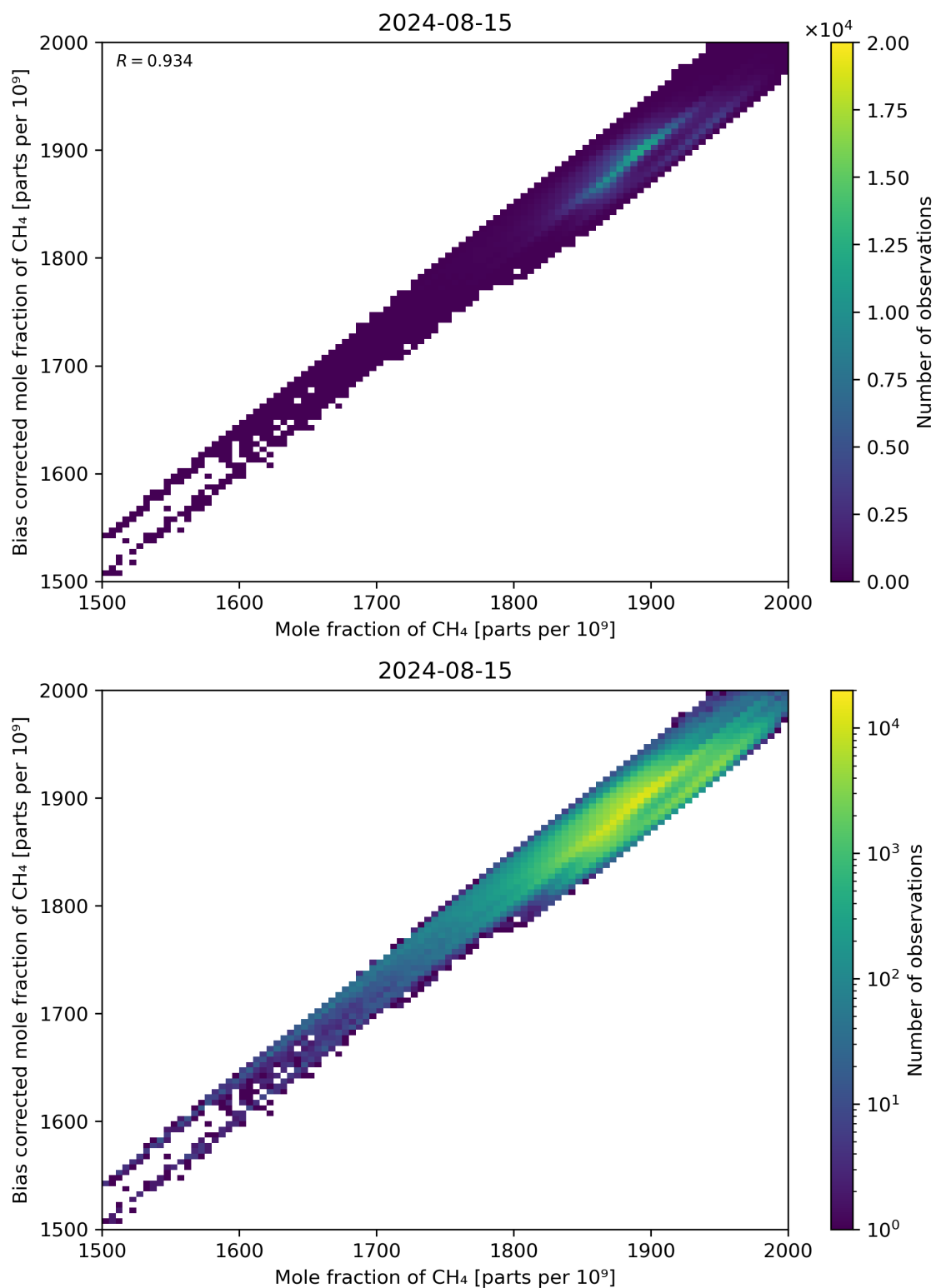
Figure 74: Scatter density plot of “Mole fraction of CH 4 ” against “Bias corrected mole fraction of CH 4 ” for 2024-08-14 to 2024-08-16.
