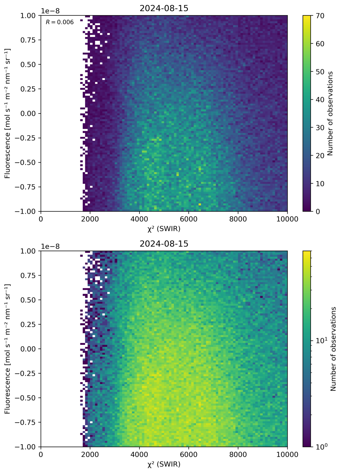
Figure 49: Scatter density plot of “ \chi^2 (SWIR)” against “Fluorescence” for 2024-08-14 to 2024-08-16.
