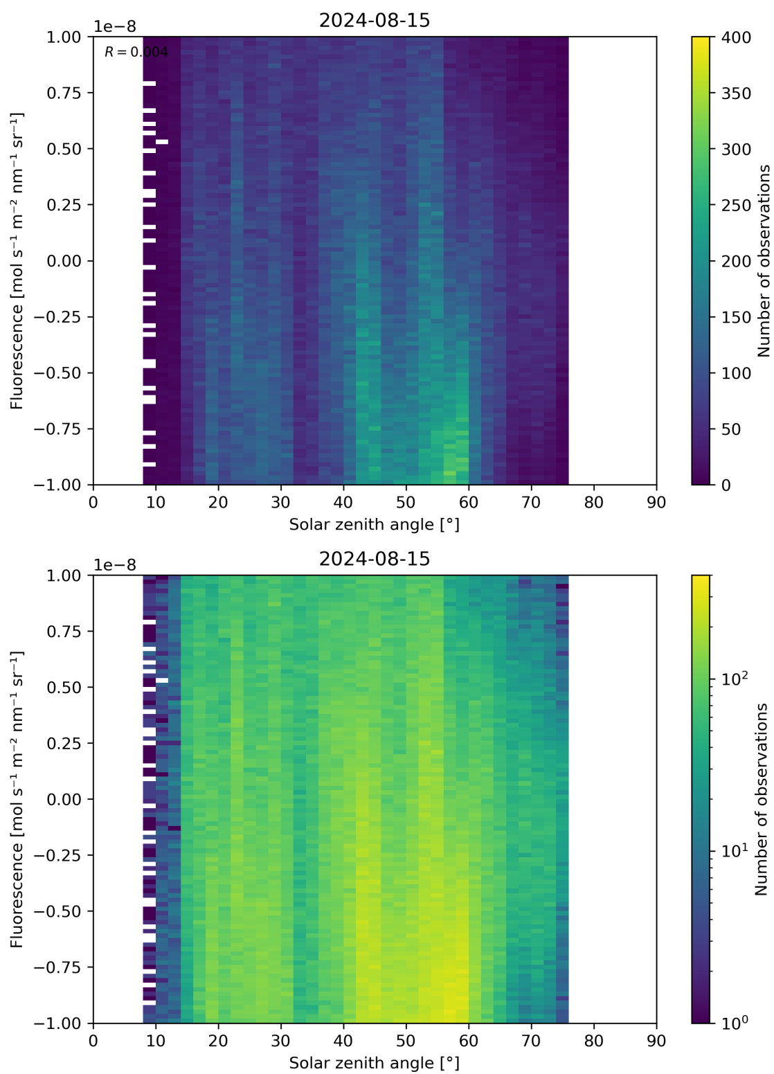
Figure 97: Scatter density plot of “Solar zenith angle” against “Fluorescence” for 2024-08-14 to 2024-08-16.
