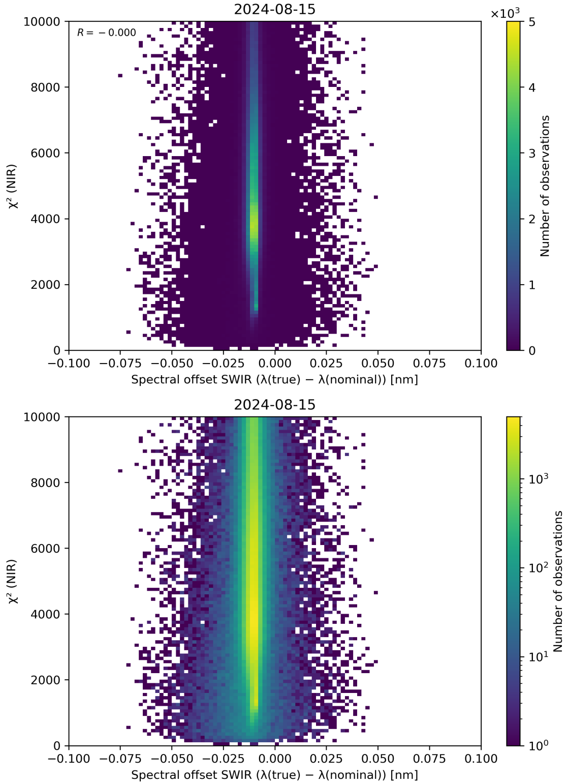
Figure 117: Scatter density plot of “Spectral offset SWIR ( \lambda(\text{true}) - \lambda(\text{nominal}) )” against “ \chi^2 (NIR)” for 2024-08-14 to 2024-08-16.
