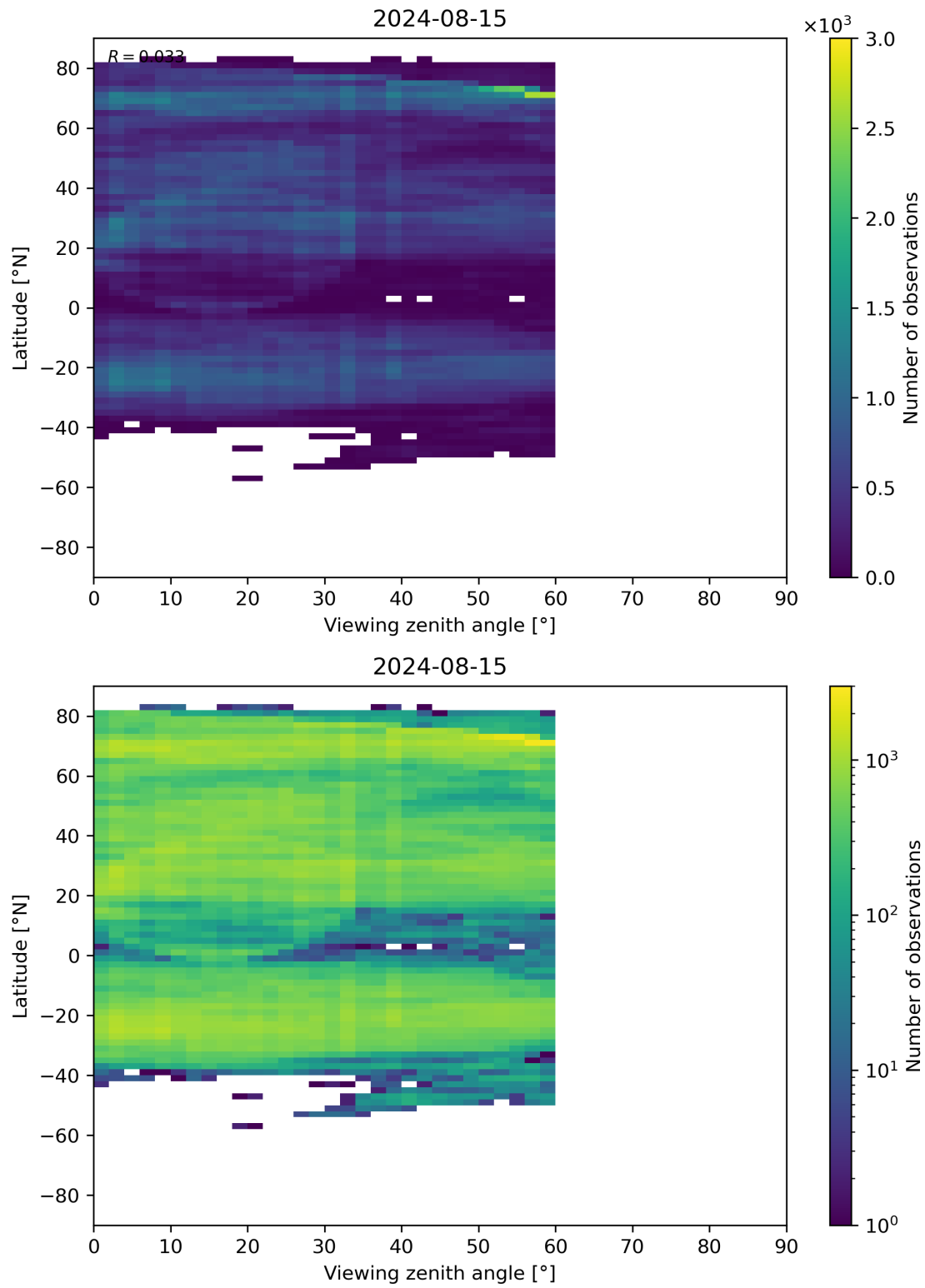
Figure 109: Scatter density plot of “Viewing zenith angle” against “Latitude” for 2024-08-14 to 2024-08-16.
