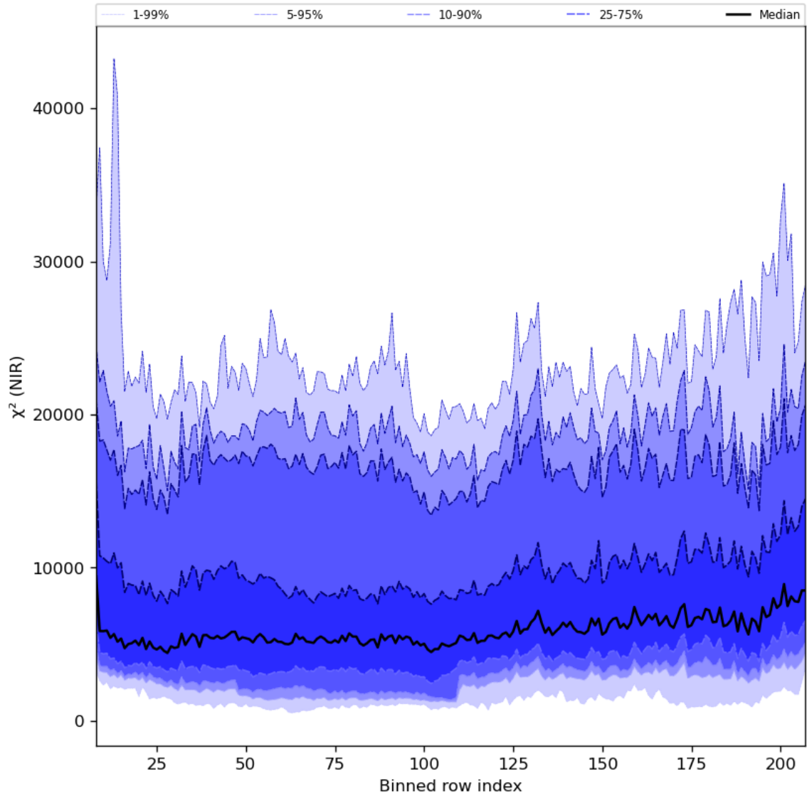
Figure 40: Along track statistics of " \chi^2 (NIR)" for 2024-08-14 to 2024-08-16
