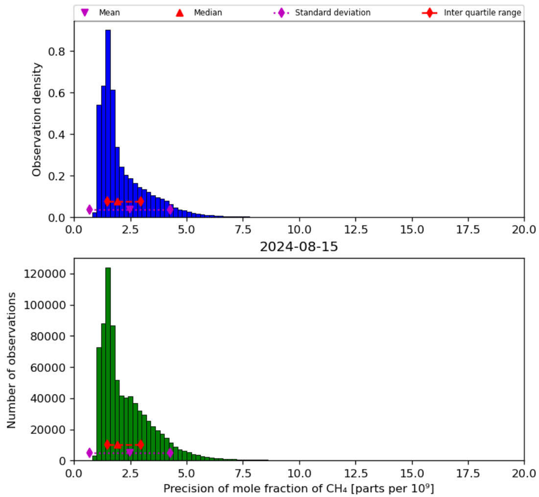
Figure 24: Histogram of “Precision of mole fraction of CH 4 ” for 2024-08-14 to 2024-08-16
