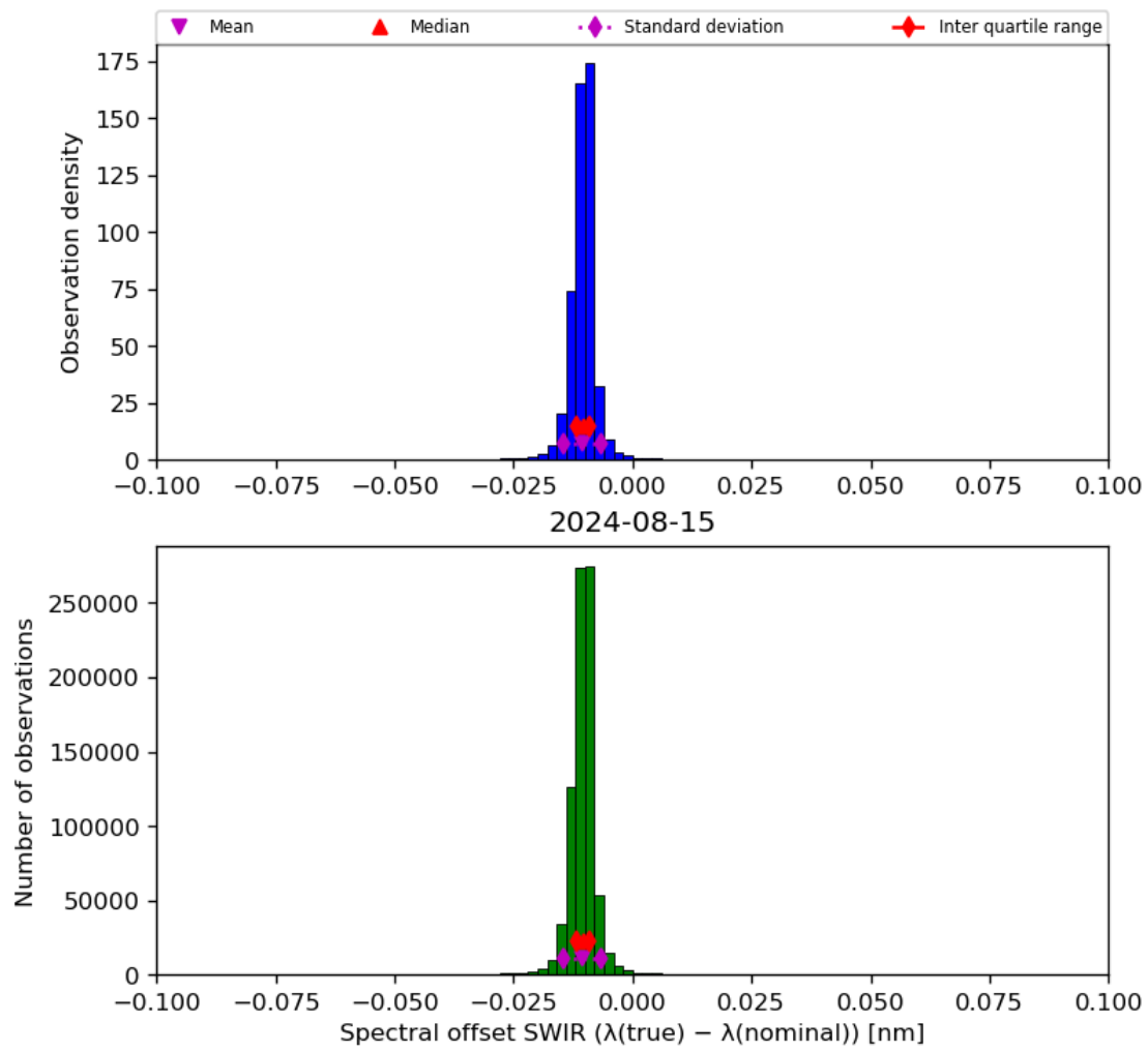
Figure 27: Histogram of “Spectral offset SWIR ( \lambda(\text{true}) - \lambda(\text{nominal}) )” for 2024-08-14 to 2024-08-16
