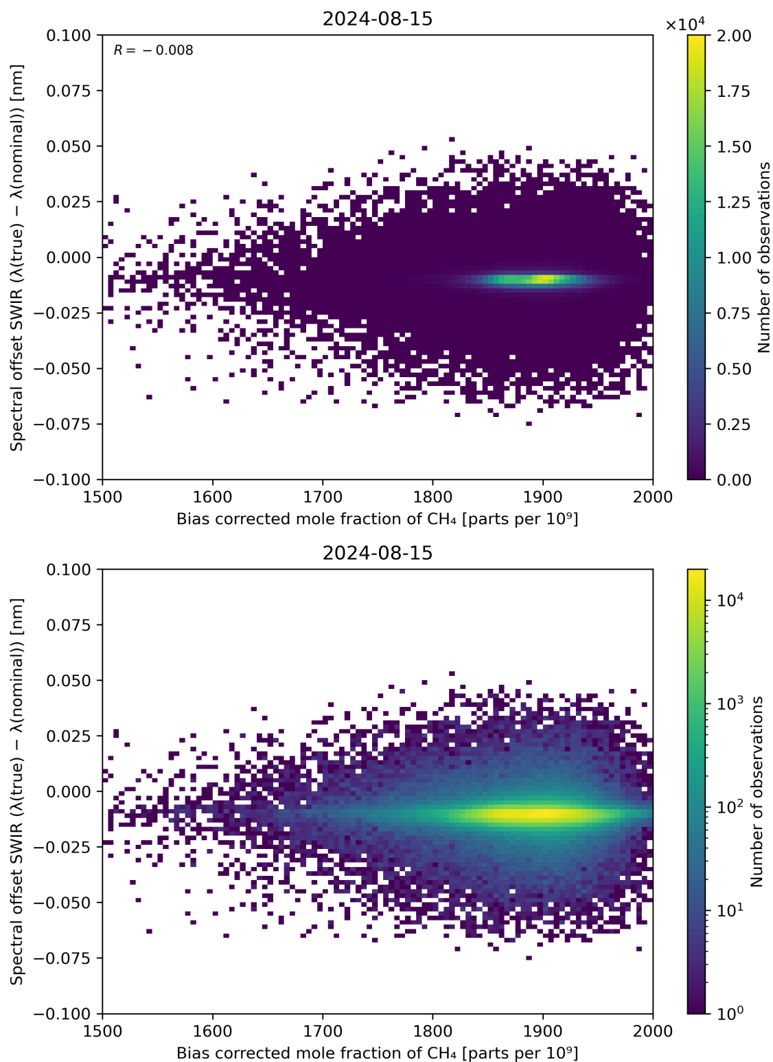
Figure 69: Scatter density plot of “Bias corrected mole fraction of \text{CH}_4 ” against “Spectral offset SWIR ( \lambda(\text{true}) - \lambda(\text{nominal}) )” for 2024-08-14 to 2024-08-16.
