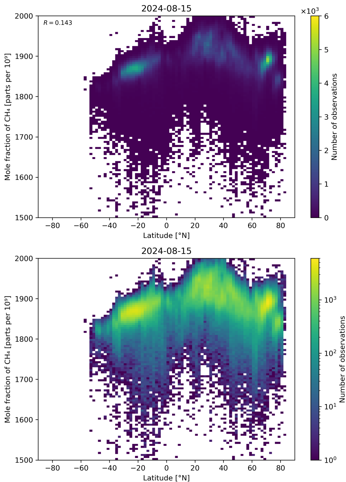
Figure 57: Scatter density plot of “Latitude” against “Mole fraction of CH 4 ” for 2024-08-14 to 2024-08-16.
