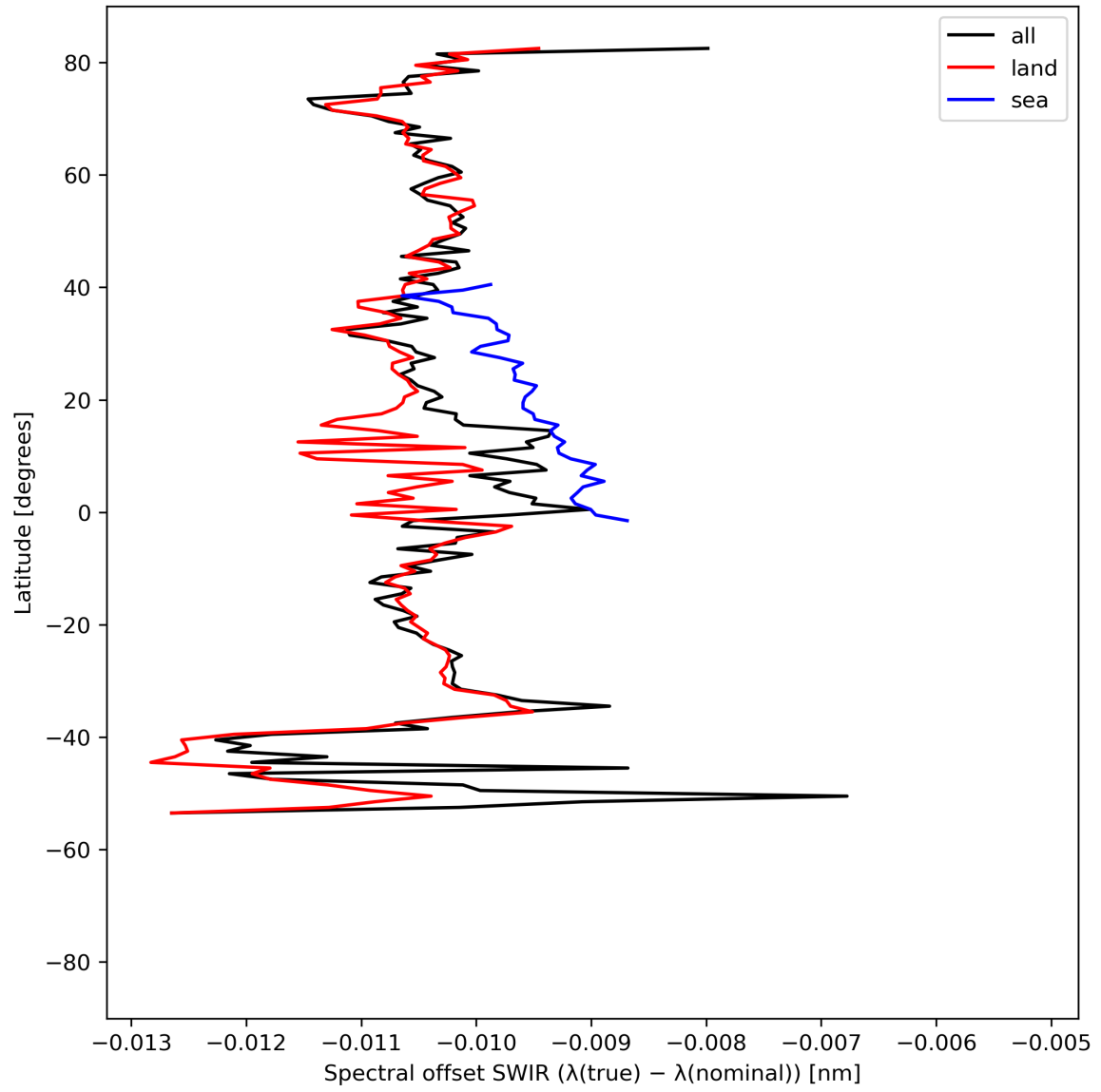
Figure 16: Zonal average of “Spectral offset SWIR ( \lambda(\text{true}) - \lambda(\text{nominal}) )” for 2024-08-14 to 2024-08-16.
