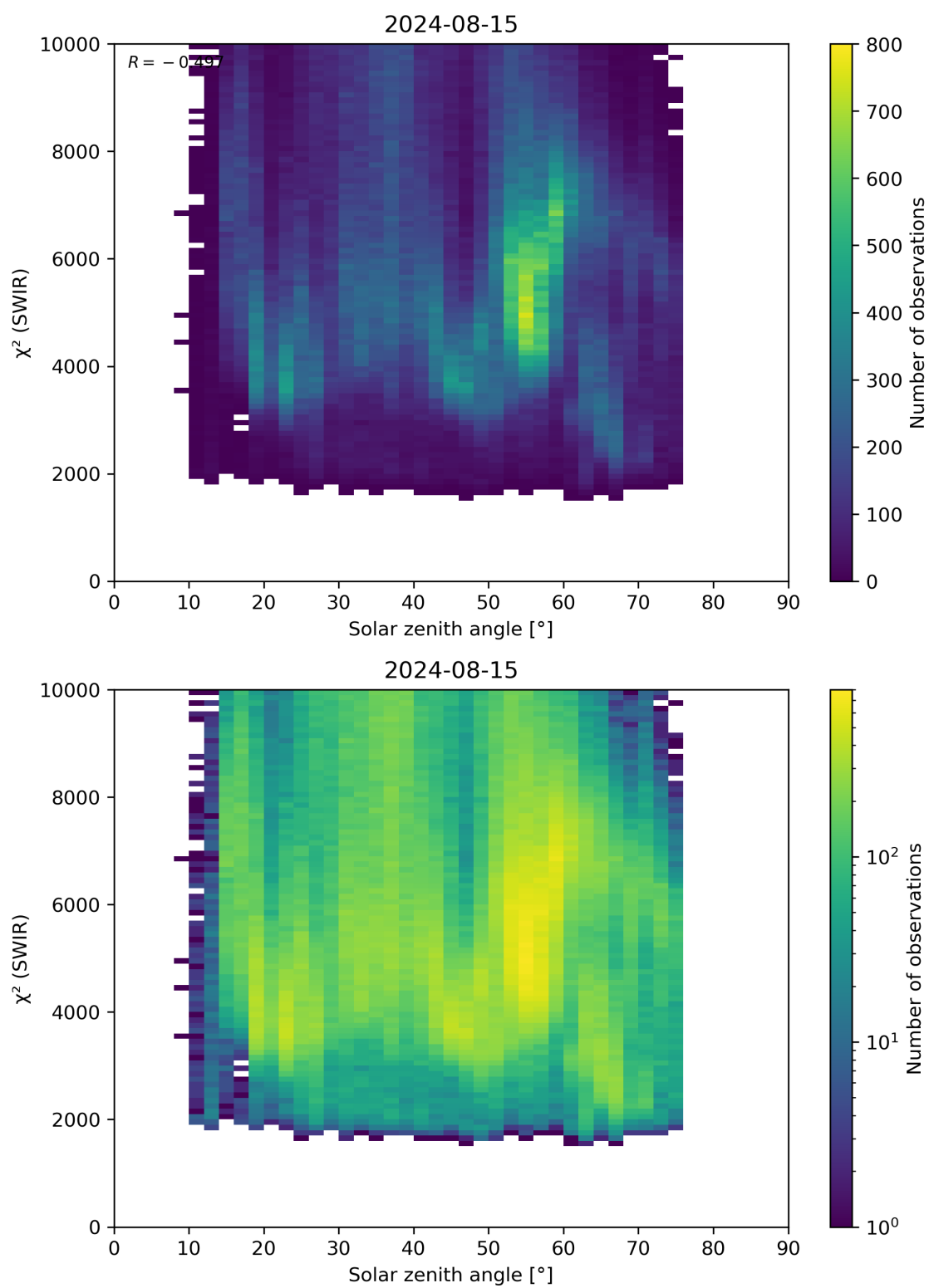
Figure 95: Scatter density plot of “Solar zenith angle” against “ \chi^2 (SWIR)” for 2024-08-14 to 2024-08-16.
