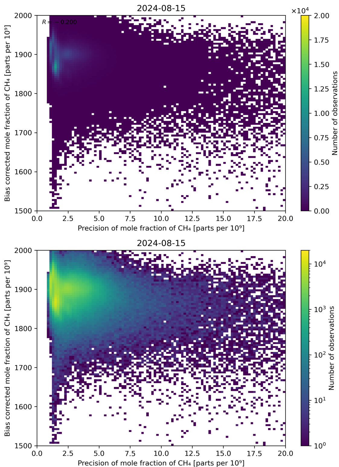
Figure 82: Scatter density plot of “Precision of mole fraction of CH 4 ” against “Bias corrected mole fraction of CH 4 ” for 2024-08-14 to 2024-08-16.
