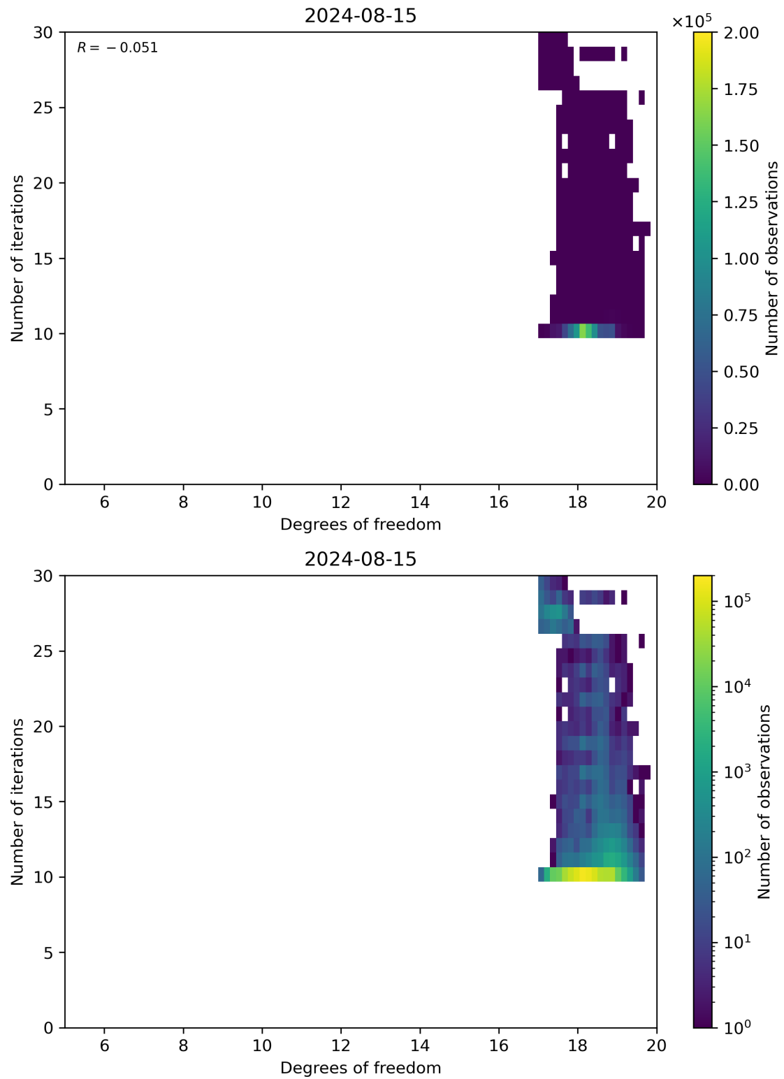
Figure 52: Scatter density plot of “Degrees of freedom” against “Number of iterations” for 2024-08-14 to 2024-08-16.
