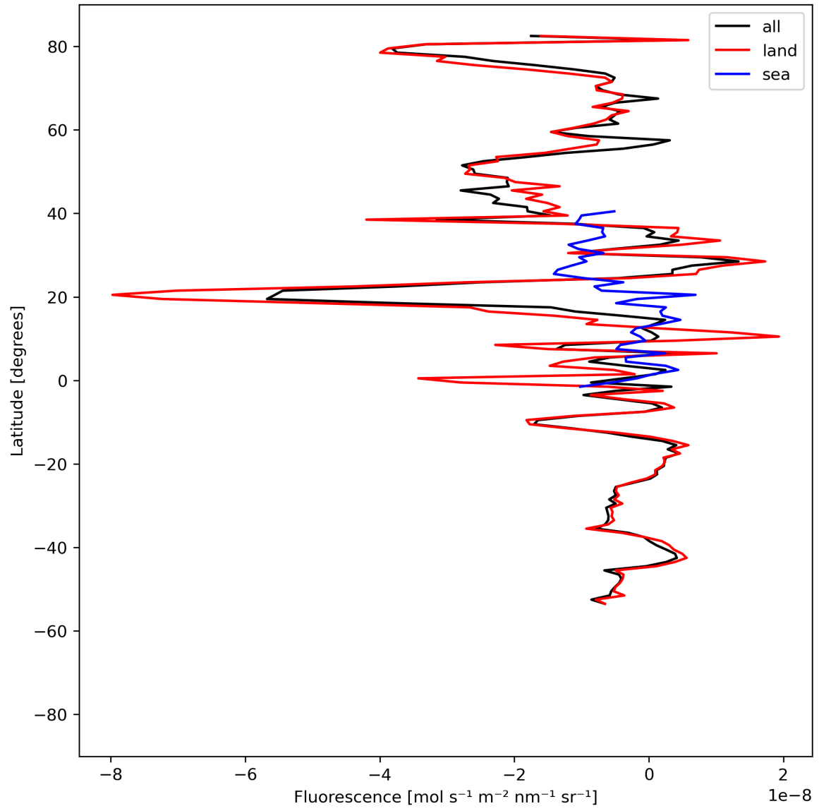
Figure 21: Zonal average of “Fluorescence” for 2024-08-14 to 2024-08-16.
