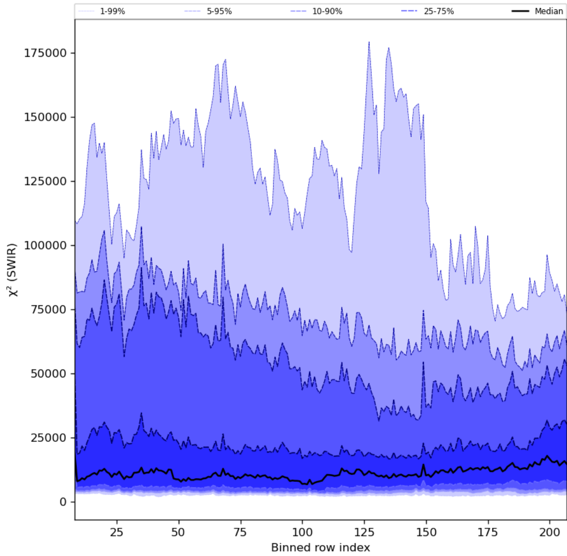
Figure 39: Along track statistics of “ \chi^2 (SWIR)” for 2024-08-14 to 2024-08-16
