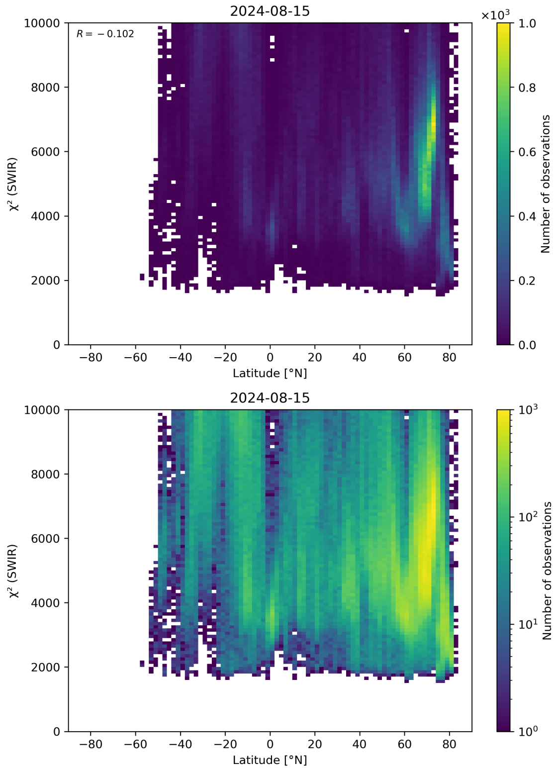
Figure 54: Scatter density plot of “Latitude” against “ \chi^2 (SWIR)” for 2024-08-14 to 2024-08-16.
