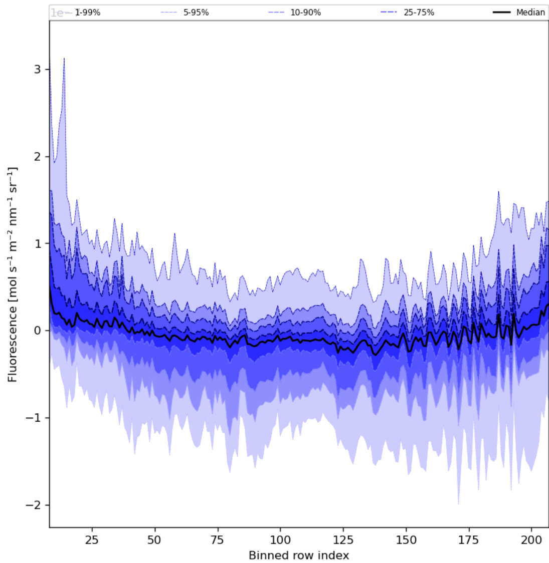
Figure 43: Along track statistics of “Fluorescence” for 2024-08-14 to 2024-08-16
