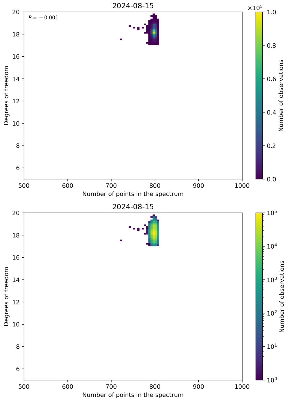
Figure 90: Scatter density plot of “Number of points in the spectrum” against “Degrees of freedom” for 2024-08-14 to 2024-08-16.
