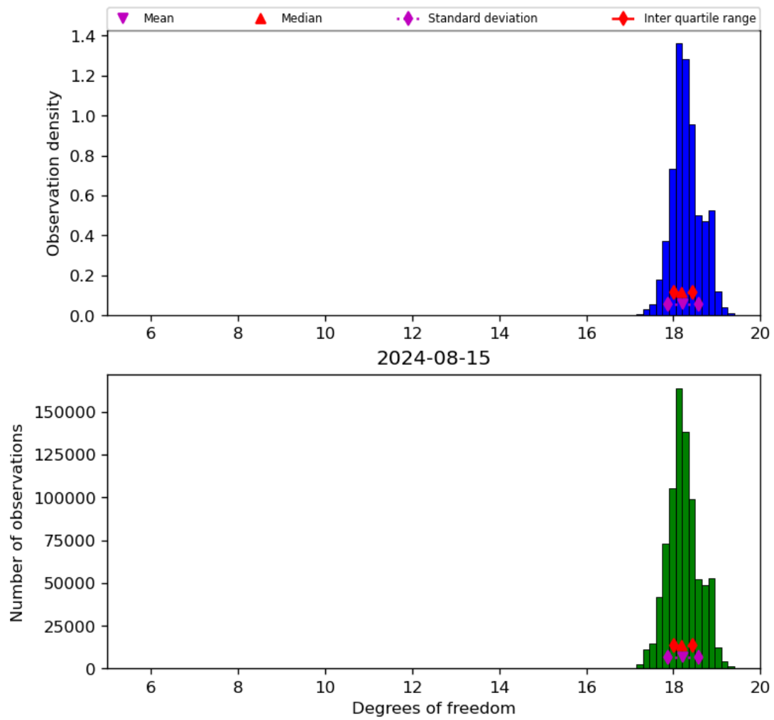
Figure 30: Histogram of “Degrees of freedom” for 2024-08-14 to 2024-08-16
