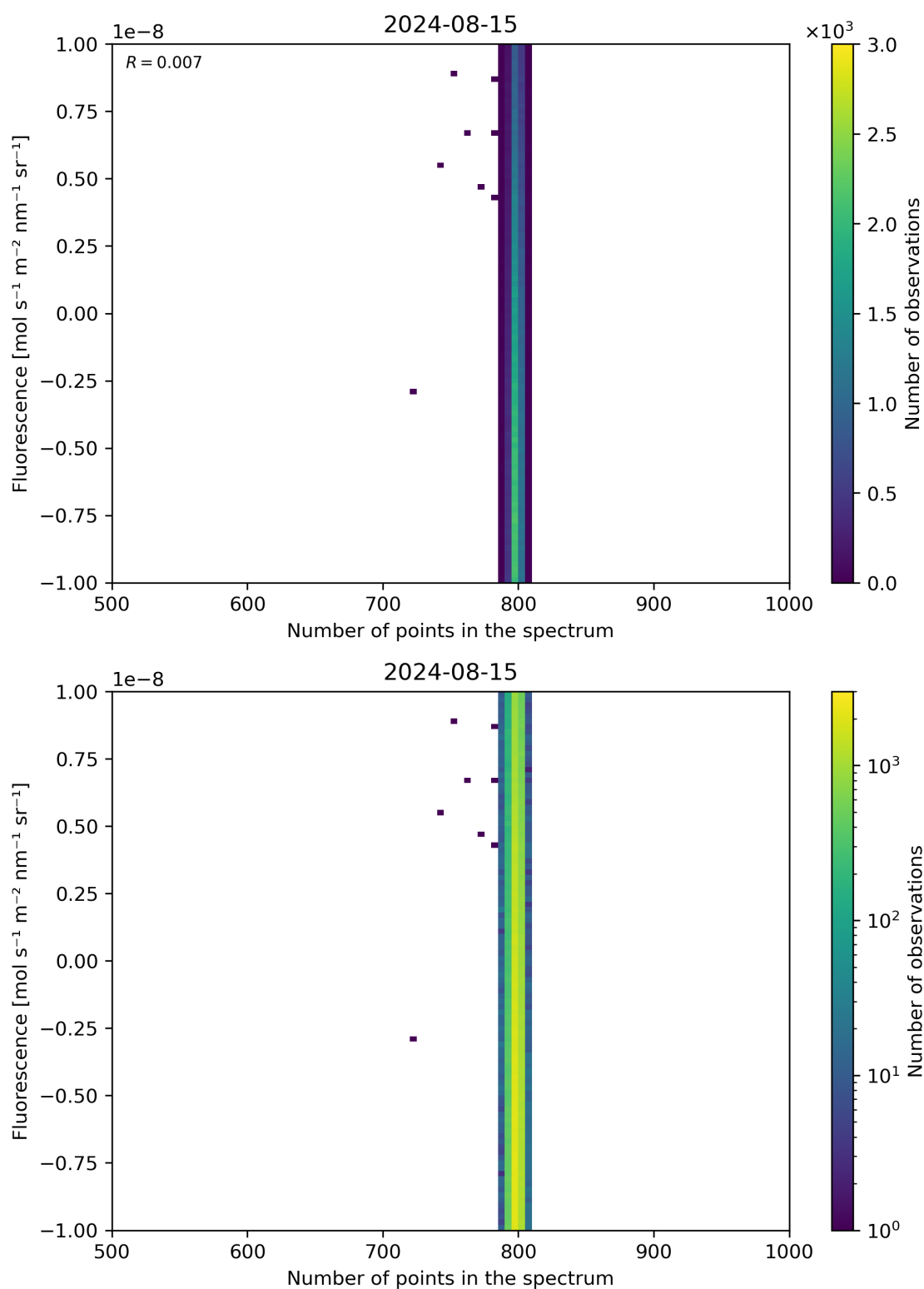
Figure 91: Scatter density plot of “Number of points in the spectrum” against “Fluorescence” for 2024-08-14 to 2024-08-16.
