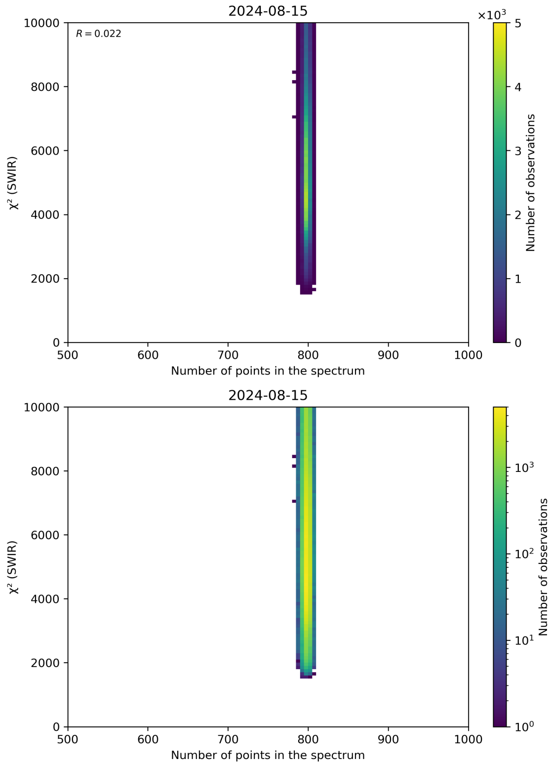
Figure 89: Scatter density plot of “Number of points in the spectrum” against “ \chi^2 (SWIR)” for 2024-08-14 to 2024-08-16.
