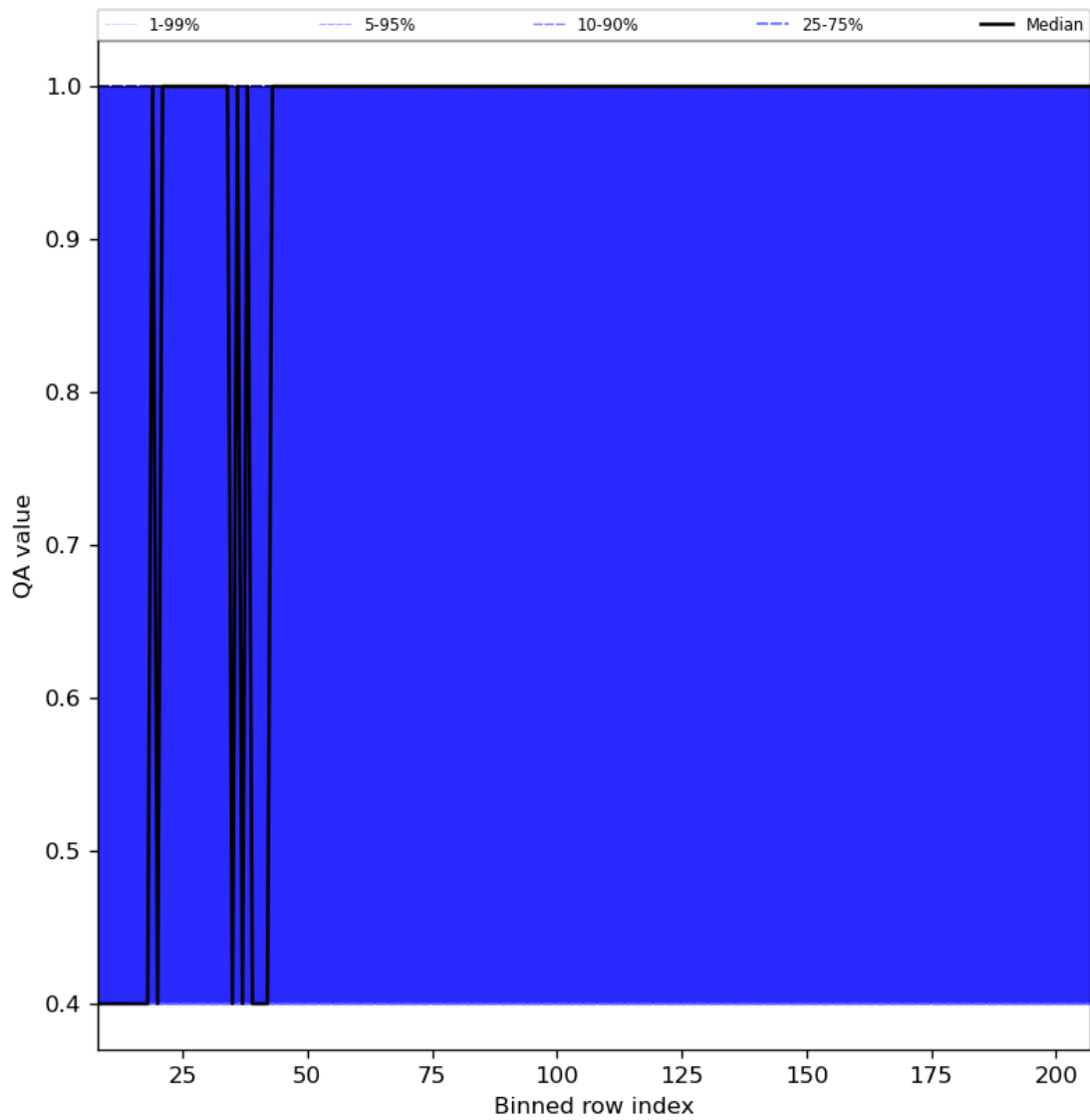
Figure 33: Along track statistics of “QA value” for 2024-08-14 to 2024-08-16
