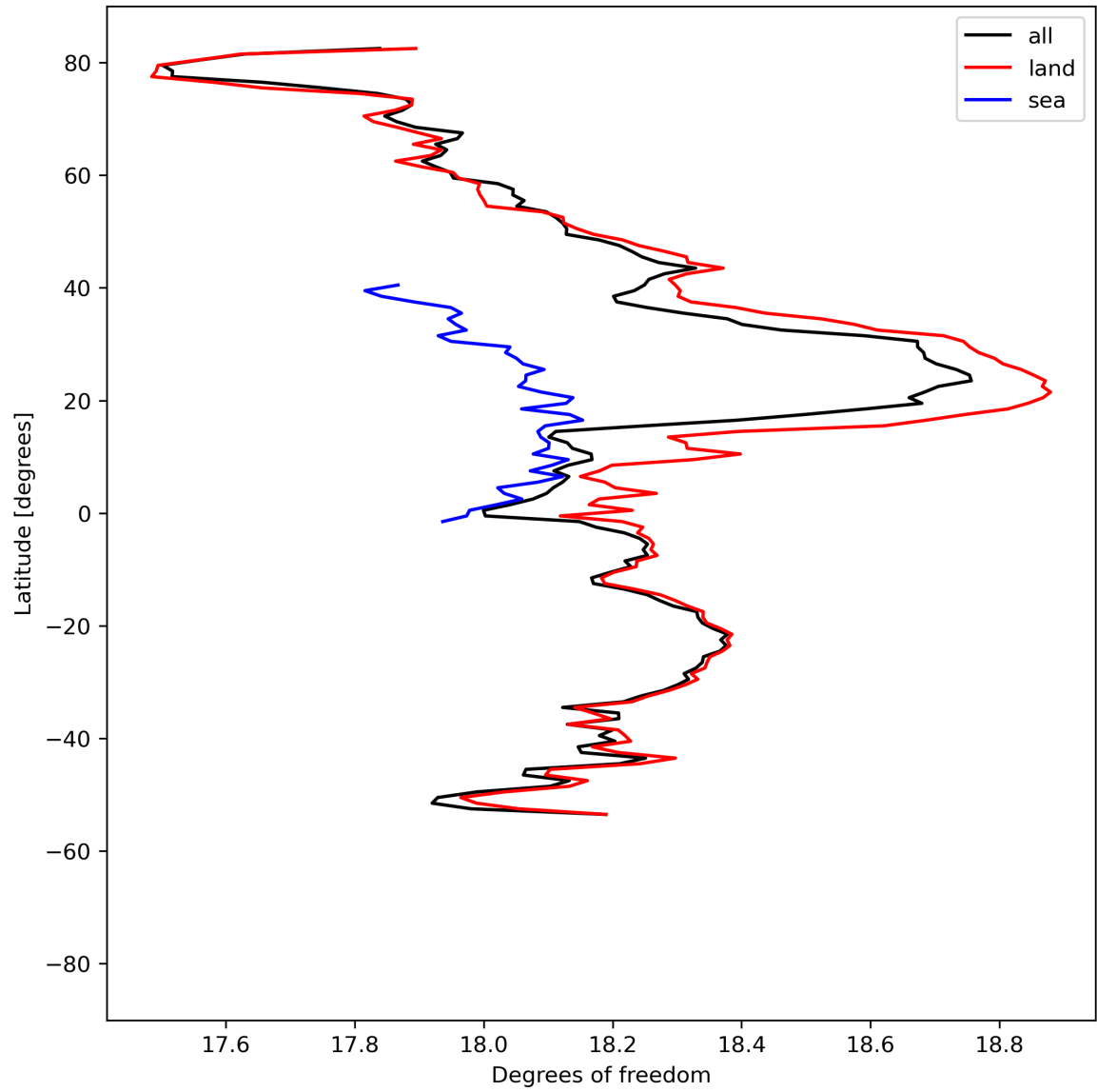
Figure 19: Zonal average of “Degrees of freedom” for 2024-08-14 to 2024-08-16.
