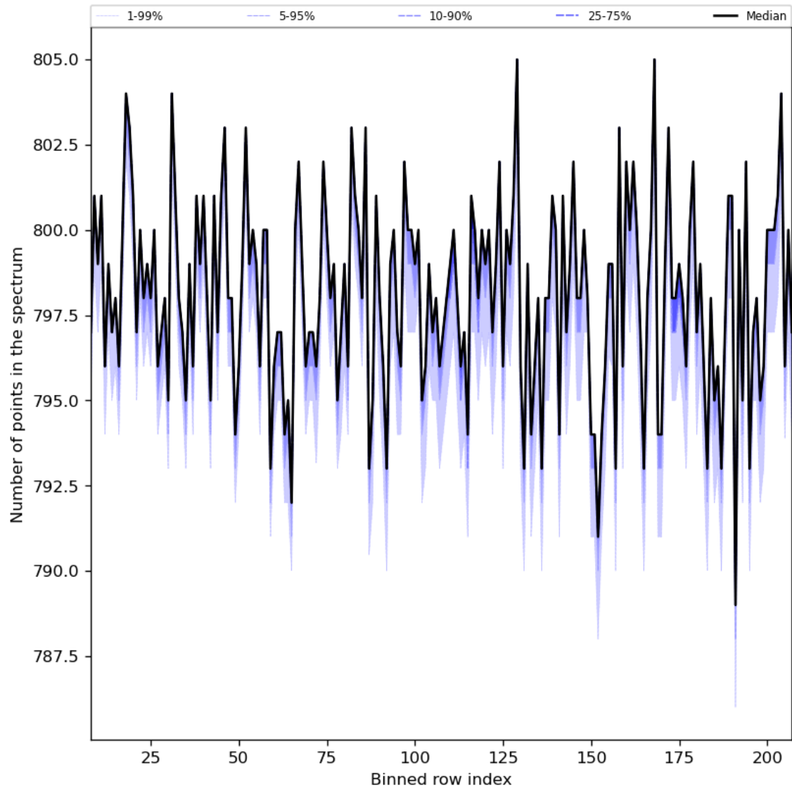
Figure 37: Along track statistics of “Number of points in the spectrum” for 2024-08-14 to 2024-08-16
