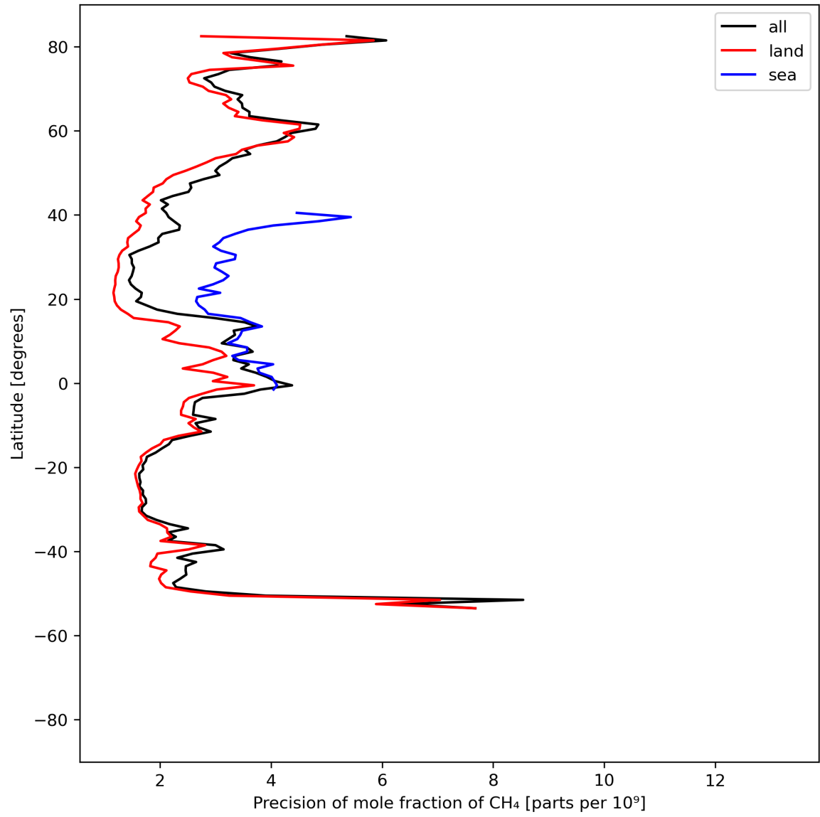
Figure 13: Zonal average of “Precision of mole fraction of CH 4 ” for 2024-08-14 to 2024-08-16.
