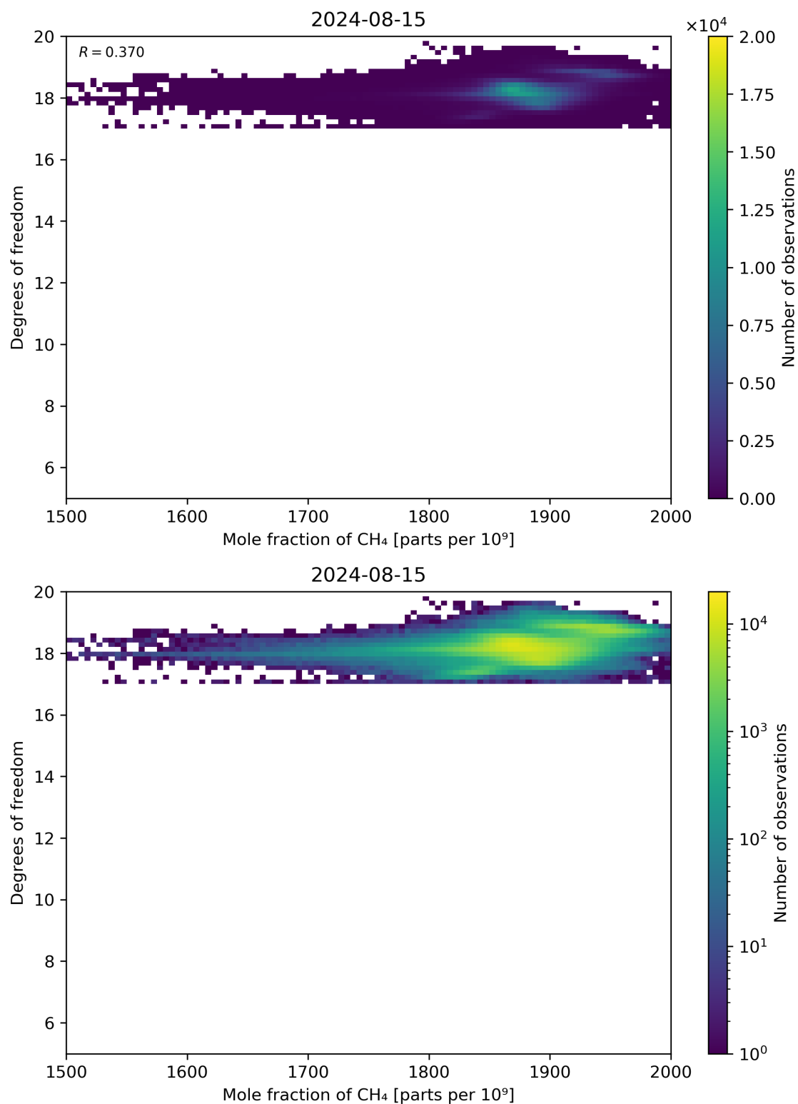
Figure 72: Scatter density plot of “Mole fraction of CH 4 ” against “Degrees of freedom” for 2024-08-14 to 2024-08-16.
