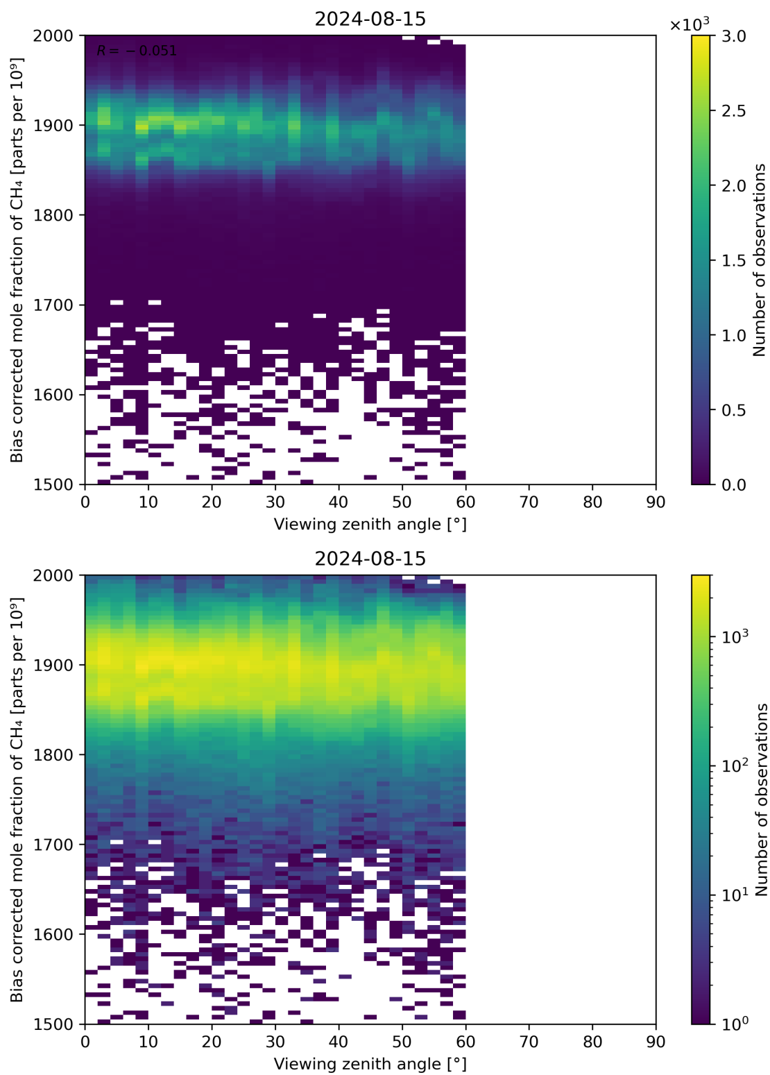
Figure 111: Scatter density plot of “Viewing zenith angle” against “Bias corrected mole fraction of CH 4 ” for 2024-08-14 to 2024-08-16.
