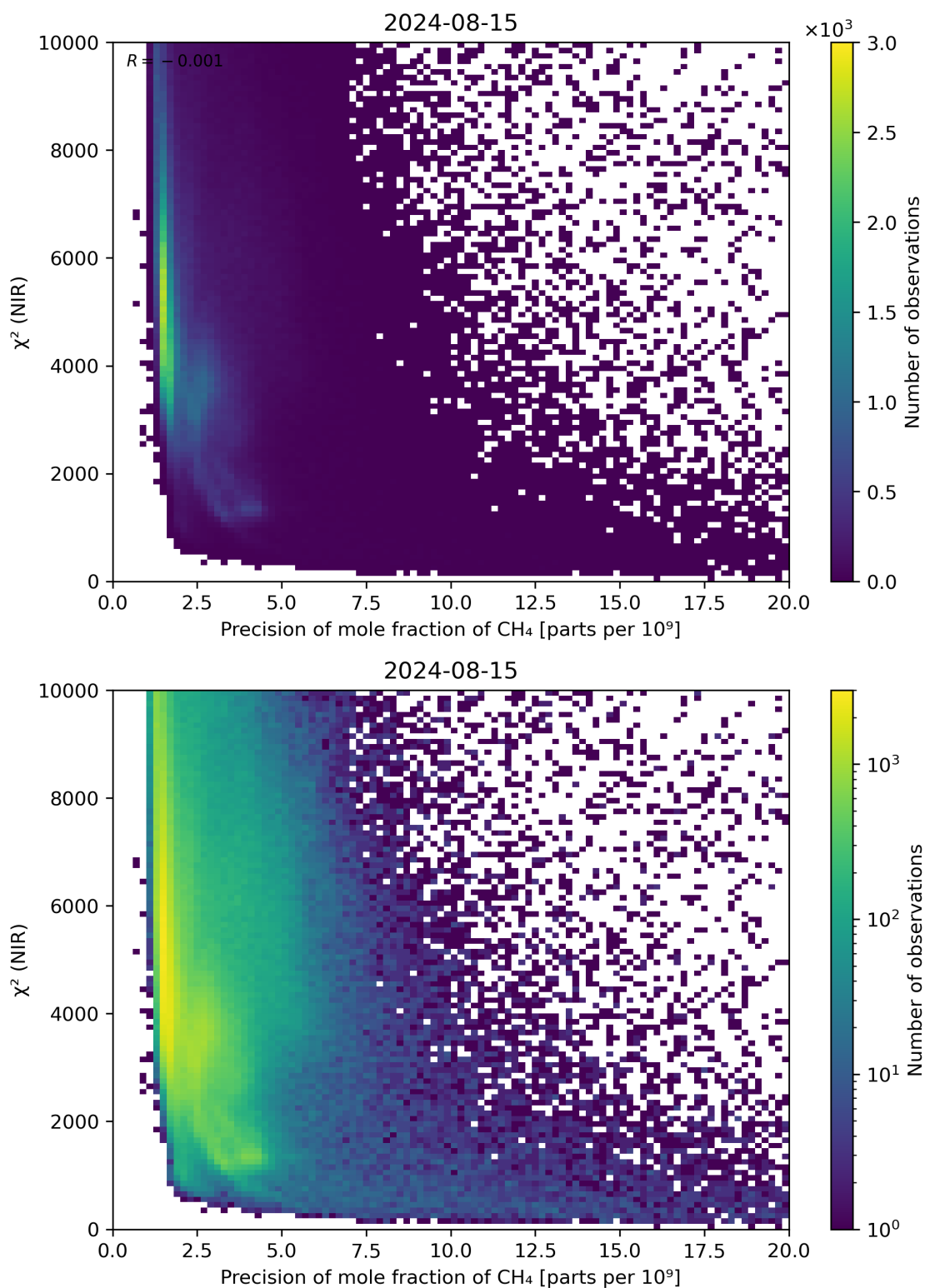
Figure 78: Scatter density plot of “Precision of mole fraction of CH 4 ” against “ \chi^2 (NIR)” for 2024-08-14 to 2024-08-16.
