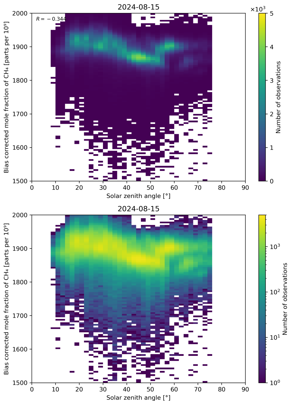
Figure 100: Scatter density plot of “Solar zenith angle” against “Bias corrected mole fraction of CH 4 ” for 2024-08-14 to 2024-08-16.
