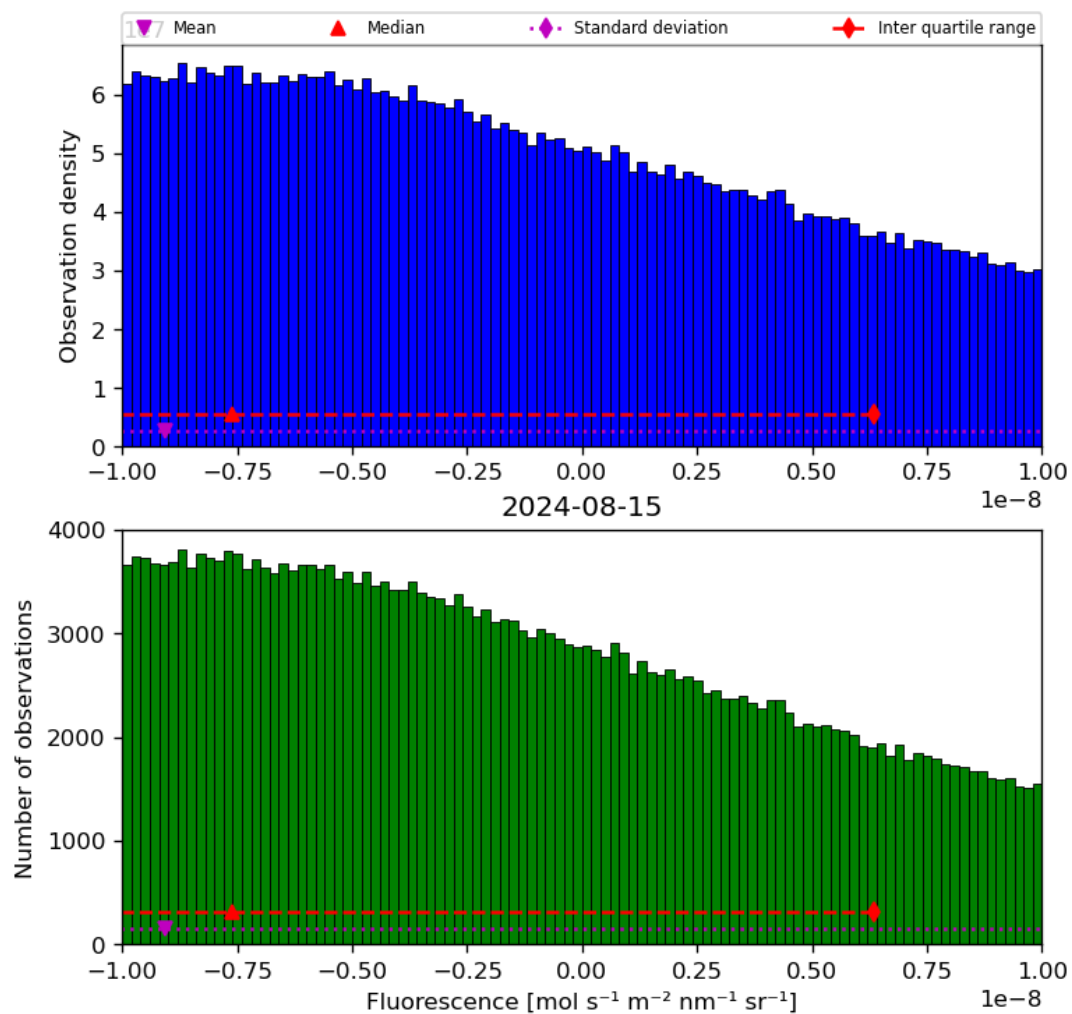
Figure 32: Histogram of “Fluorescence” for 2024-08-14 to 2024-08-16
