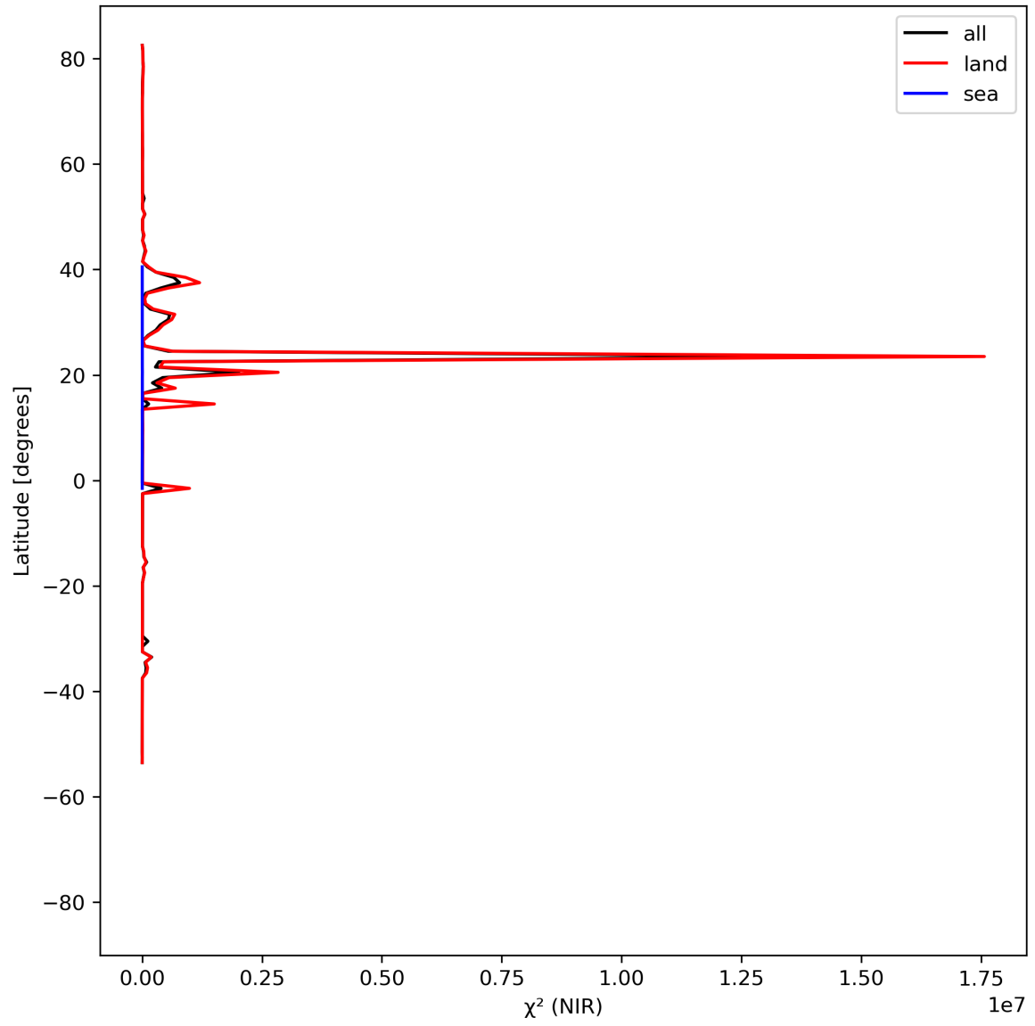
Figure 18: Zonal average of “ \chi^2 (NIR)” for 2024-08-14 to 2024-08-16.
