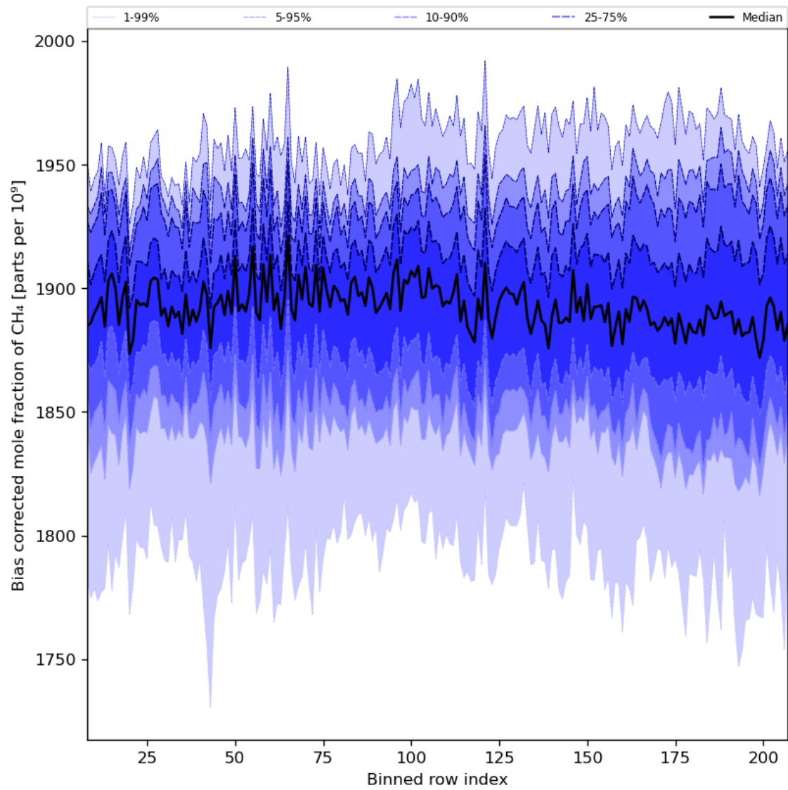
Figure 36: Along track statistics of “Bias corrected mole fraction of CH 4 ” for 2024-08-14 to 2024-08-16
