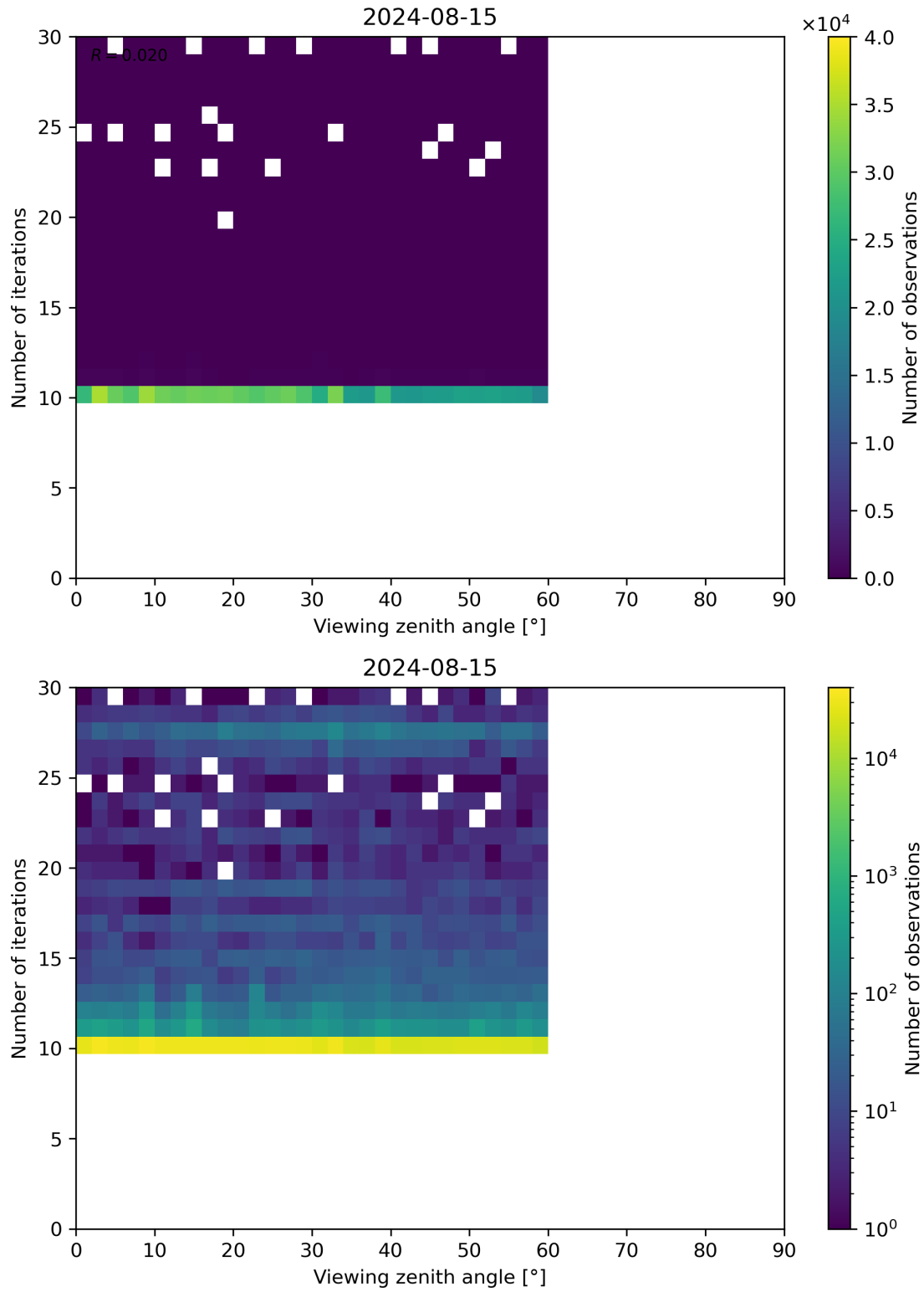
Figure 113: Scatter density plot of “Viewing zenith angle” against “Number of iterations” for 2024-08-14 to 2024-08-16.
