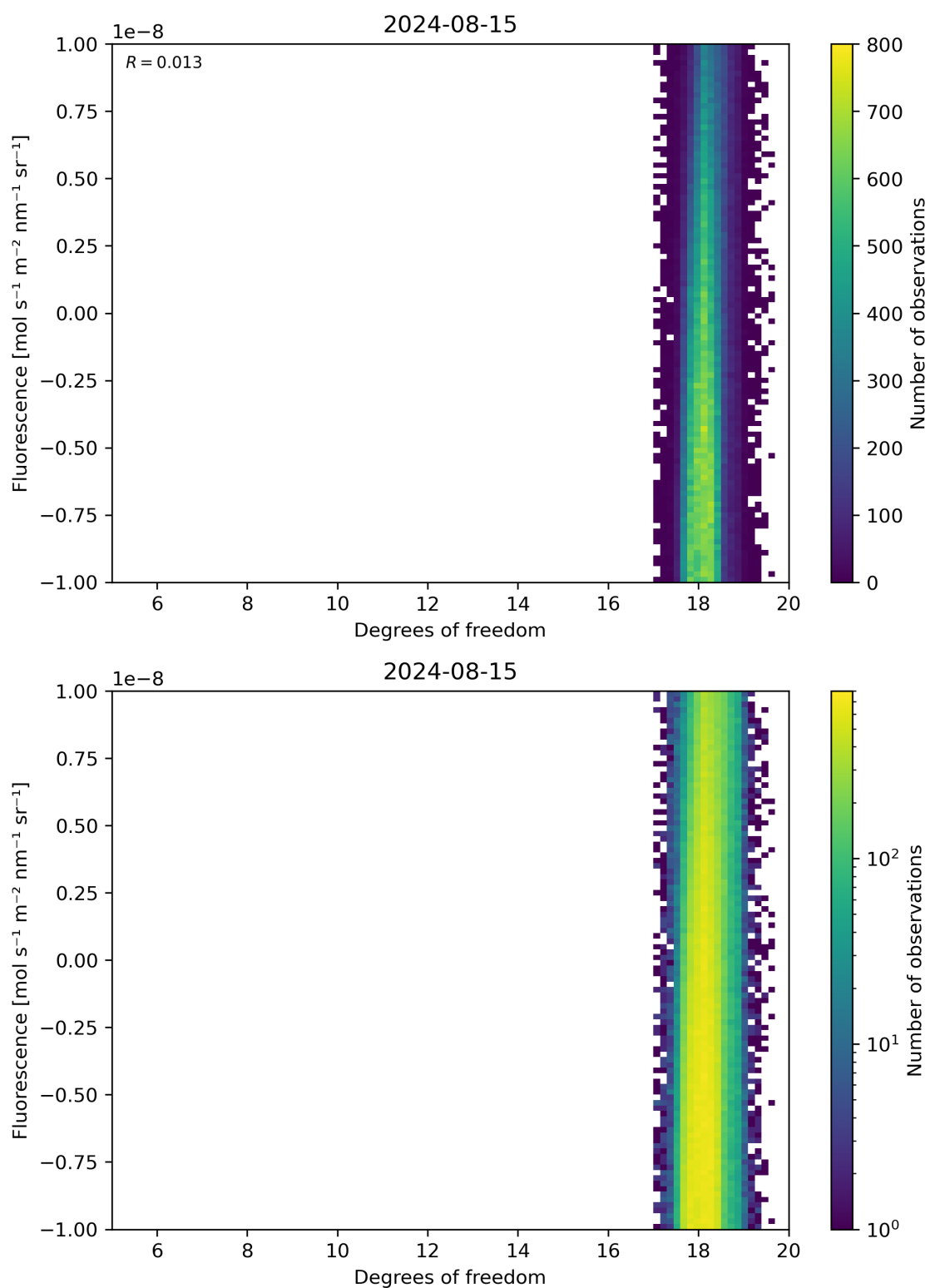
Figure 51: Scatter density plot of “Degrees of freedom” against “Fluorescence” for 2024-08-14 to 2024-08-16.
