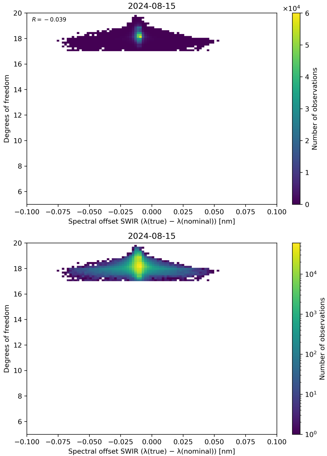
Figure 119: Scatter density plot of “Spectral offset SWIR ( \lambda(\text{true}) - \lambda(\text{nominal}) )” against “Degrees of freedom” for 2024-08-14 to 2024-08-16.
