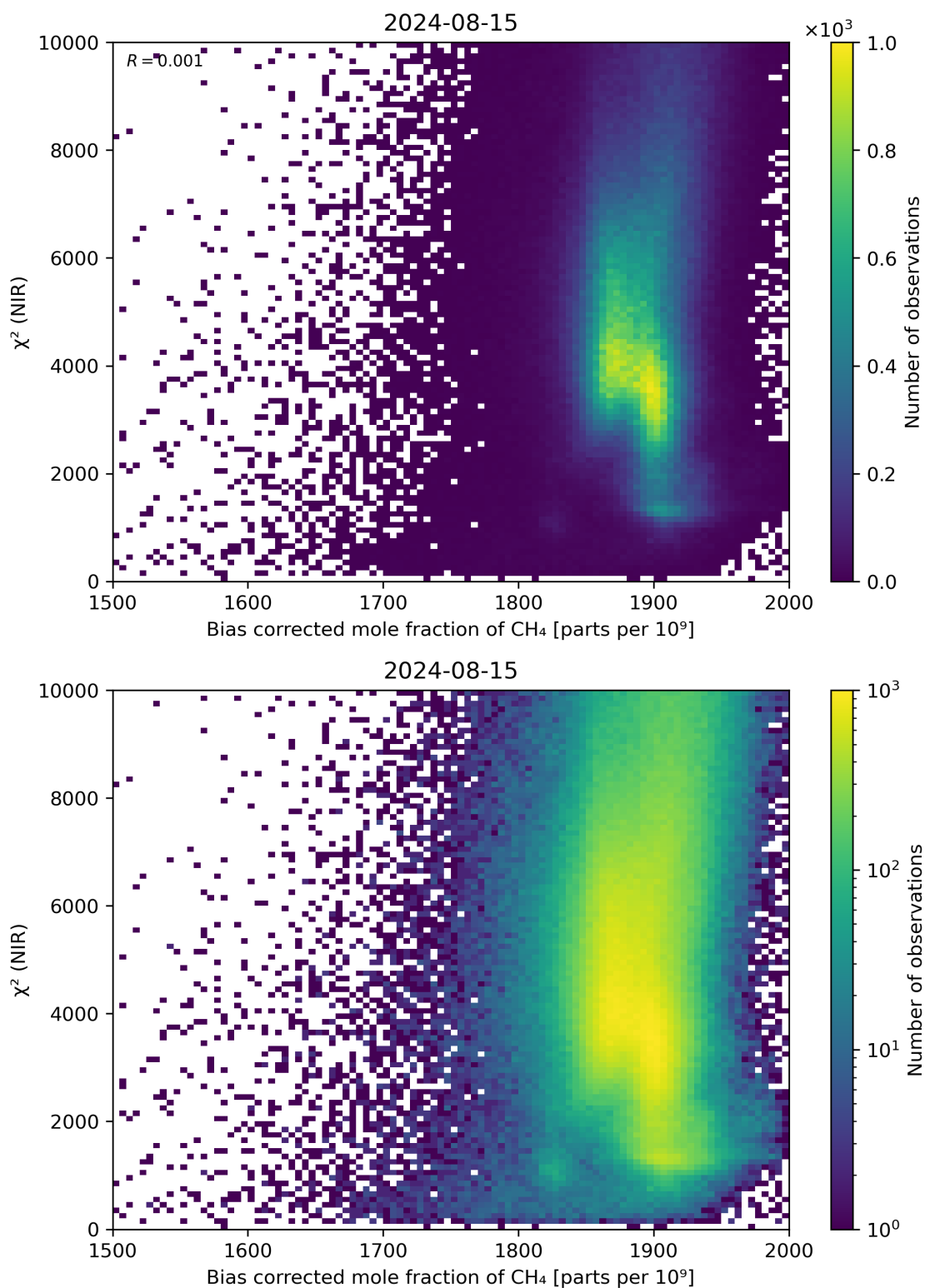
Figure 63: Scatter density plot of “Bias corrected mole fraction of CH 4 ” against “ \chi^2 (NIR)” for 2024-08-14 to 2024-08-16.
