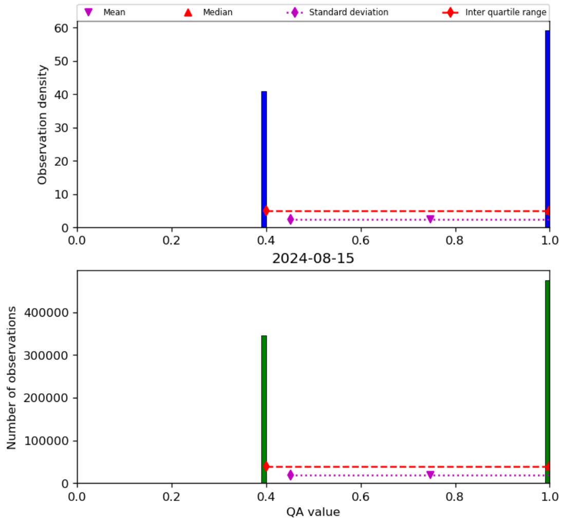
Figure 22: Histogram of “QA value” for 2024-08-14 to 2024-08-16
