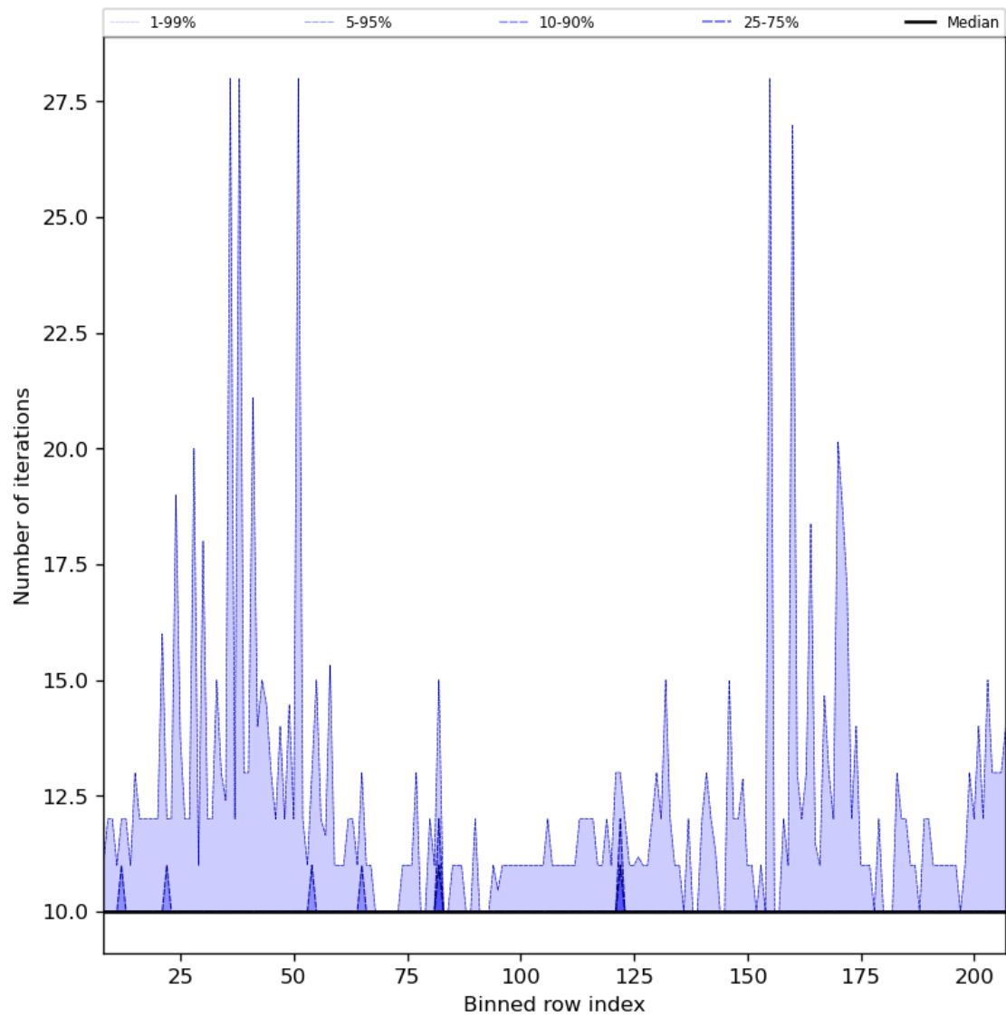
Figure 42: Along track statistics of “Number of iterations” for 2024-08-14 to 2024-08-16
