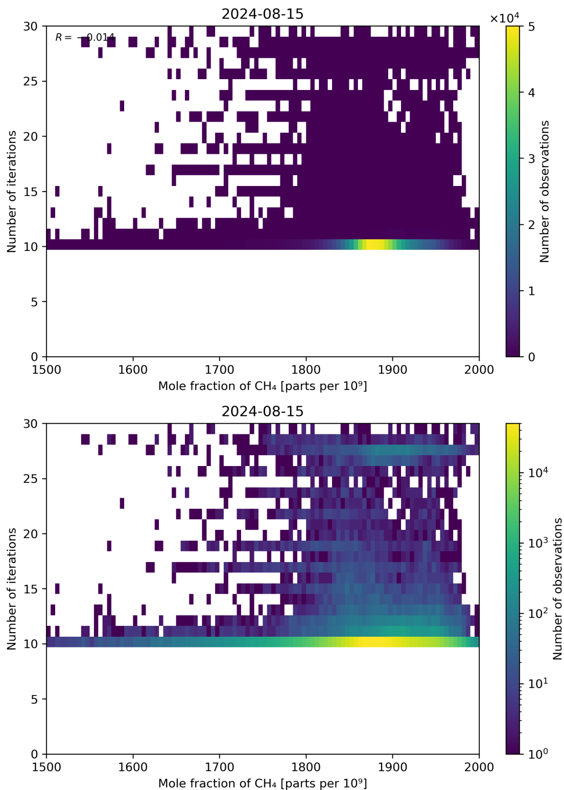
Figure 76: Scatter density plot of “Mole fraction of CH 4 ” against “Number of iterations” for 2024-08-14 to 2024-08-16.
