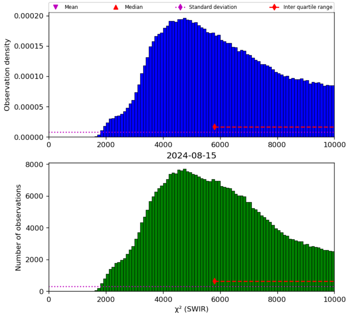
Figure 28: Histogram of “ \chi^2 (SWIR)” for 2024-08-14 to 2024-08-16
