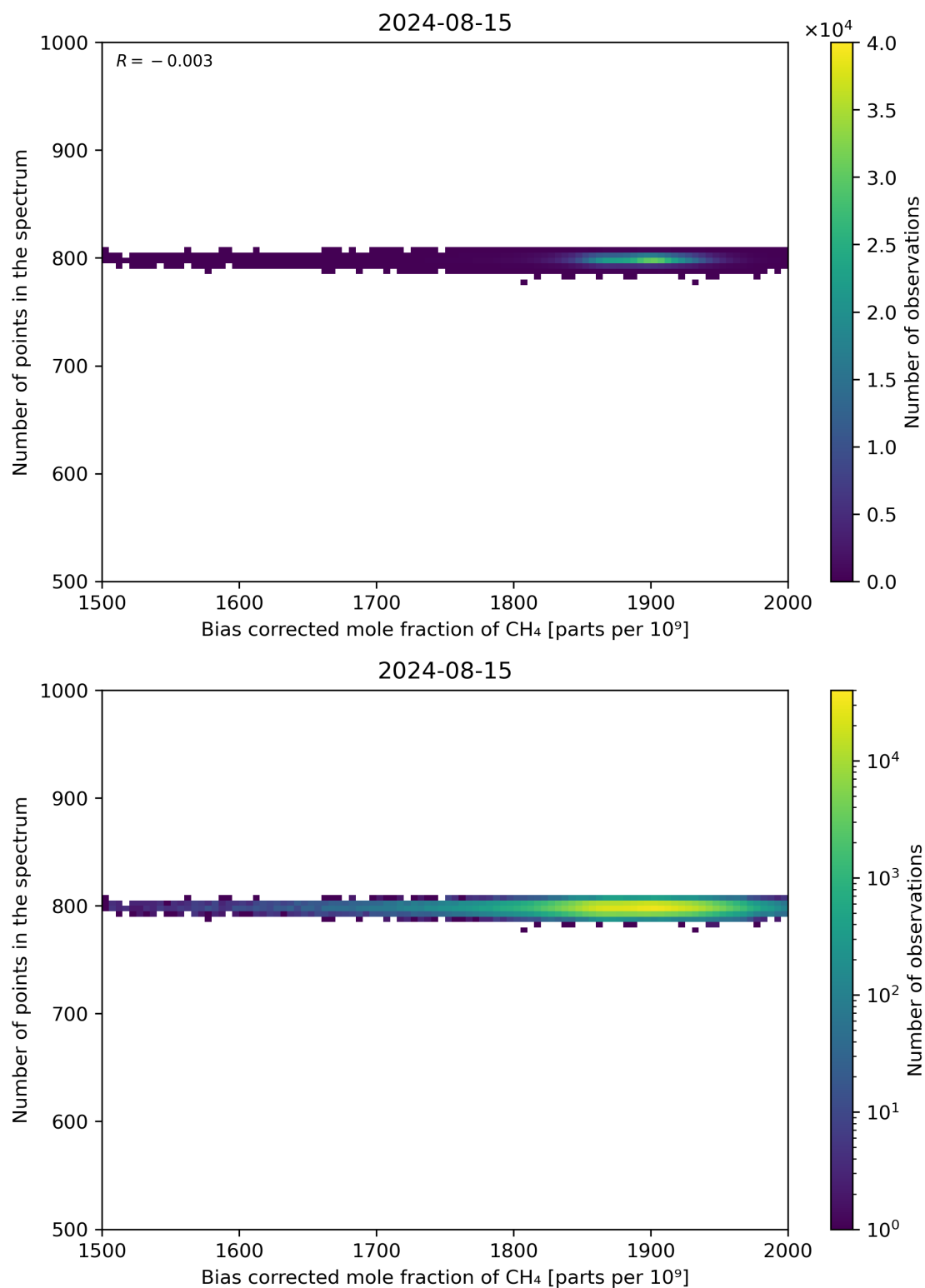
Figure 68: Scatter density plot of “Bias corrected mole fraction of CH 4 ” against “Number of points in the spectrum” for 2024-08-14 to 2024-08-16.
