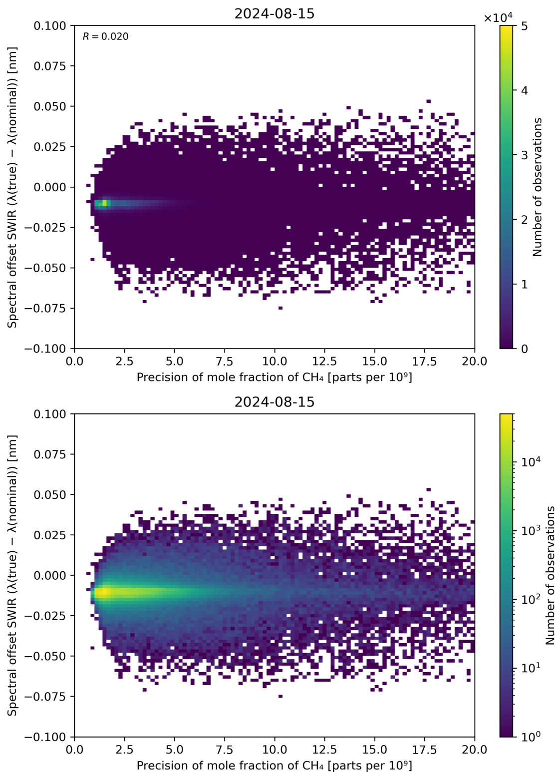
Figure 85: Scatter density plot of “Precision of mole fraction of CH 4 ” against “Spectral offset SWIR ( \lambda(\text{true}) - \lambda(\text{nominal}) )” for 2024-08-14 to 2024-08-16.
