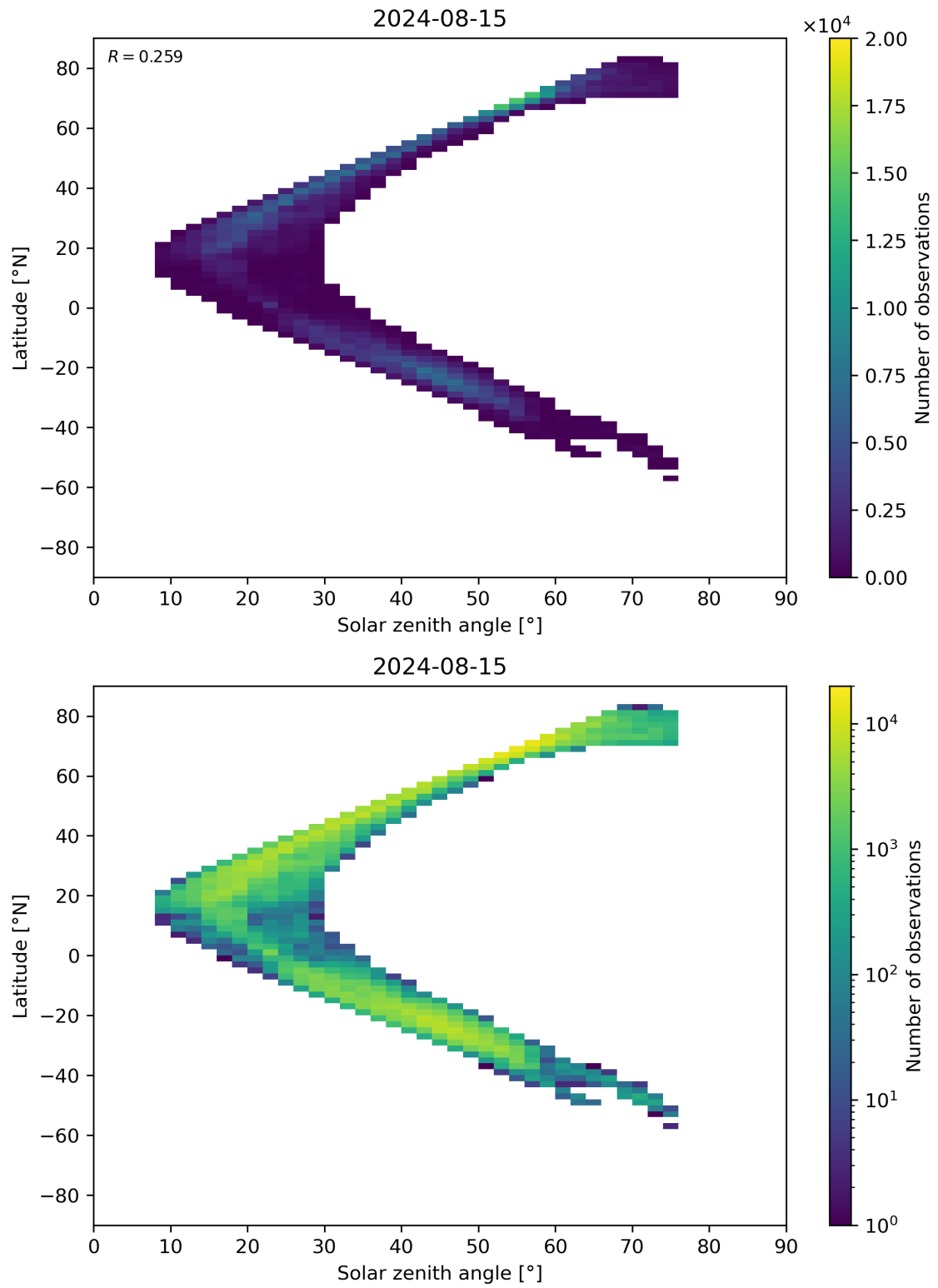
Figure 98: Scatter density plot of “Solar zenith angle” against “Latitude” for 2024-08-14 to 2024-08-16.
