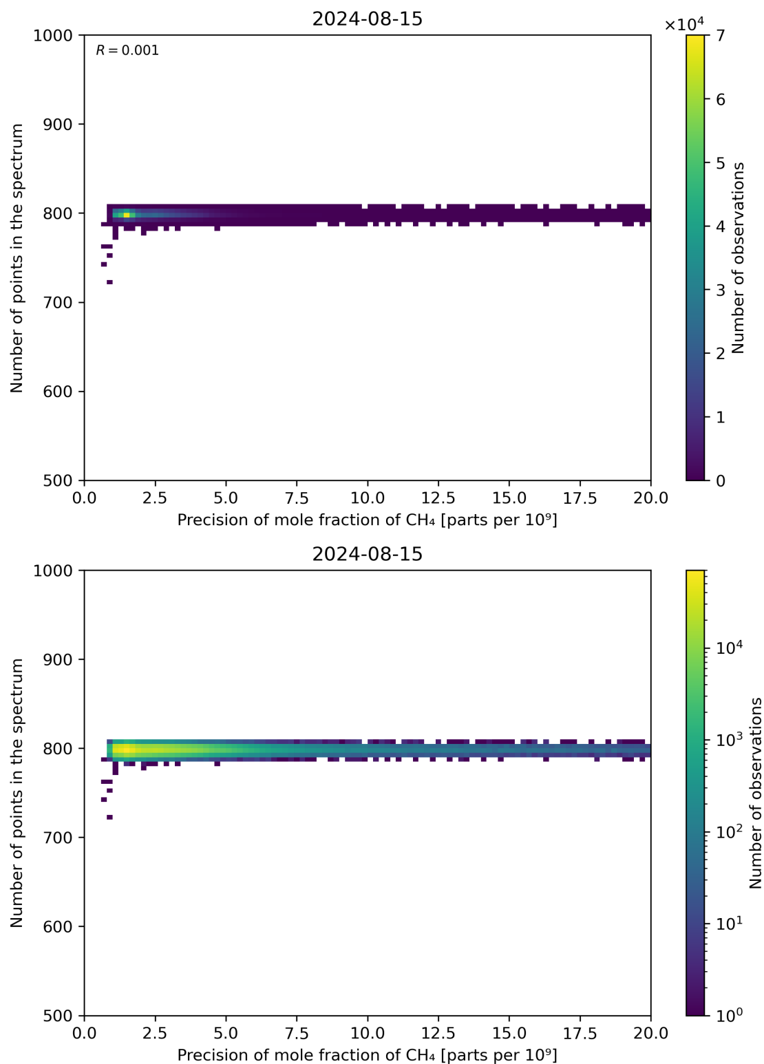
Figure 84: Scatter density plot of “Precision of mole fraction of CH 4 ” against “Number of points in the spectrum” for 2024-08-14 to 2024-08-16.
