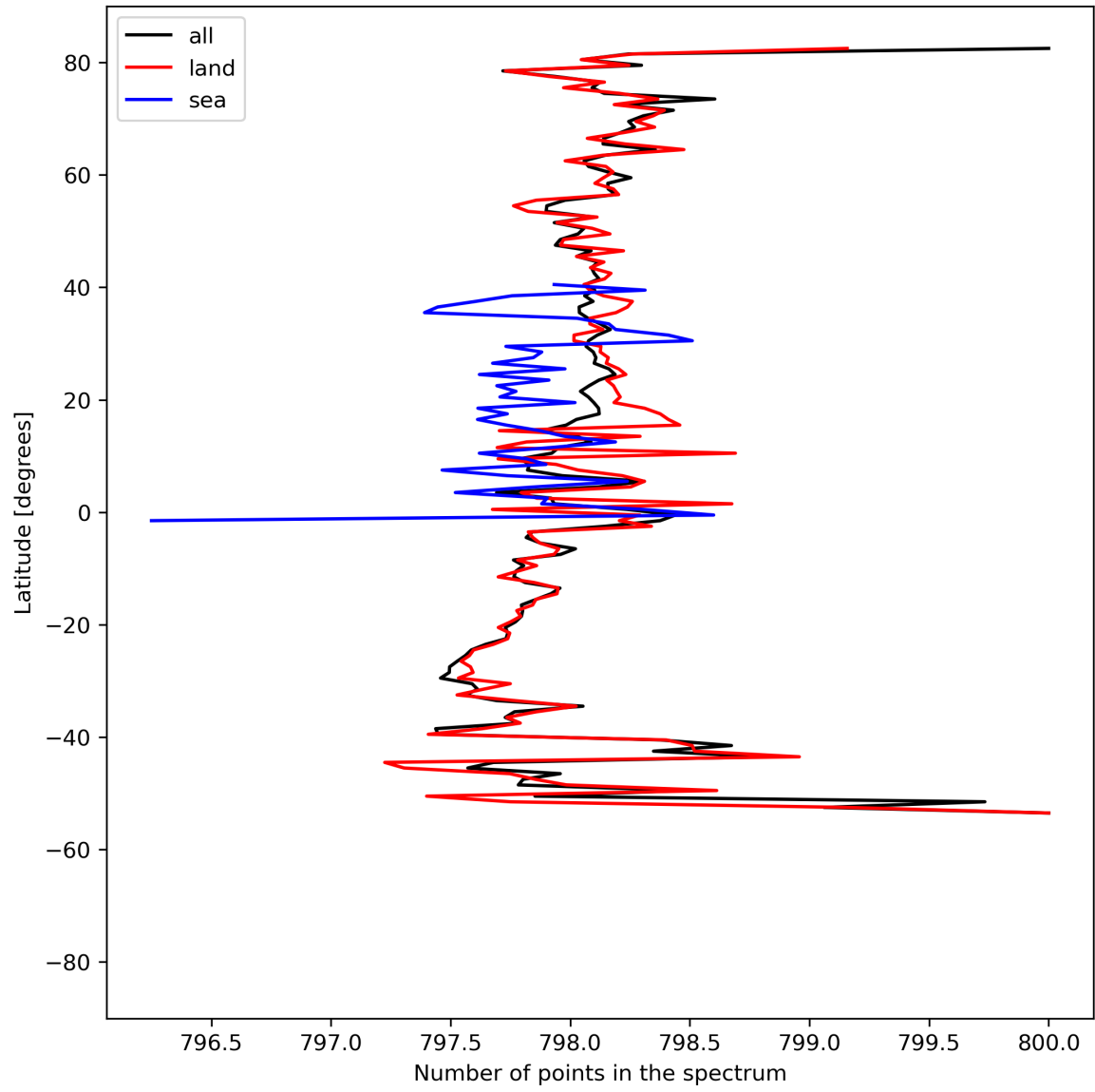
Figure 15: Zonal average of “Number of points in the spectrum” for 2024-08-14 to 2024-08-16.
