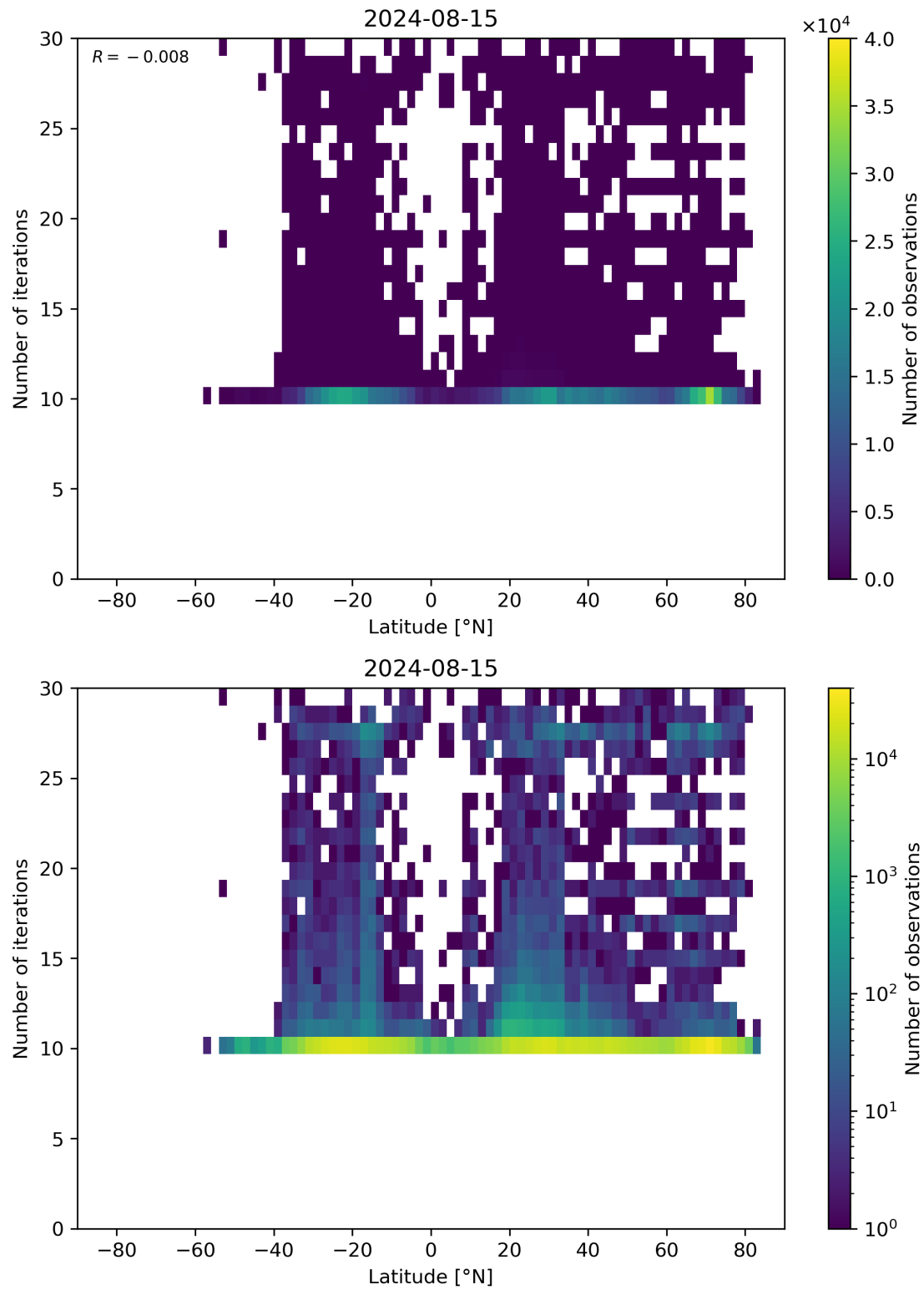
Figure 60: Scatter density plot of “Latitude” against “Number of iterations” for 2024-08-14 to 2024-08-16.
