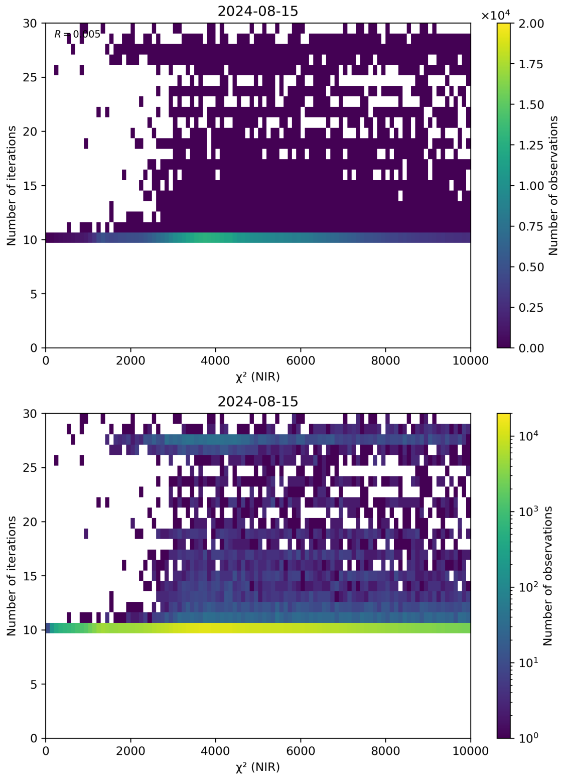
Figure 46: Scatter density plot of “ \chi^2 (NIR)” against “Number of iterations” for 2024-08-14 to 2024-08-16.
