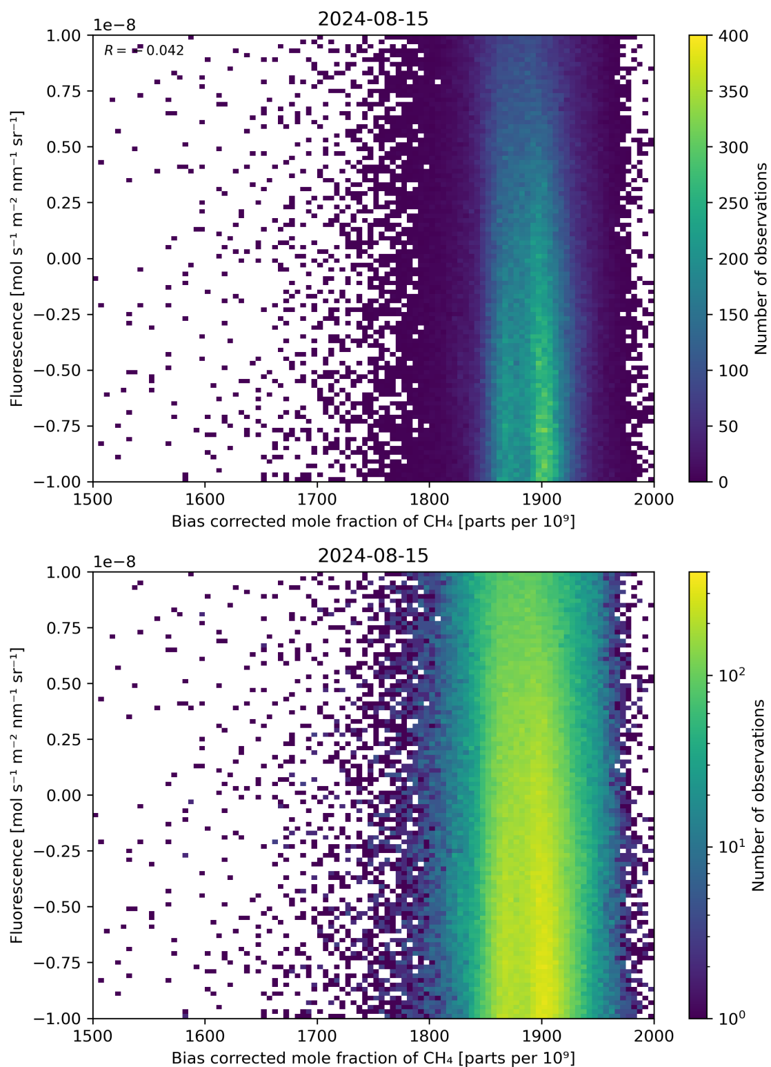
Figure 66: Scatter density plot of “Bias corrected mole fraction of CH 4 ” against “Fluorescence” for 2024-08-14 to 2024-08-16.
