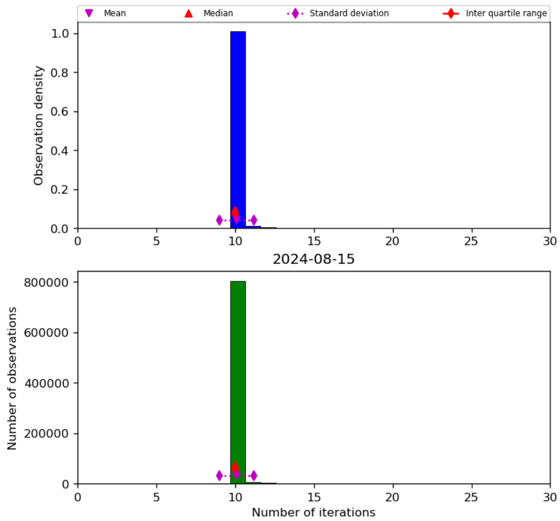
Figure 31: Histogram of “Number of iterations” for 2024-08-14 to 2024-08-16
