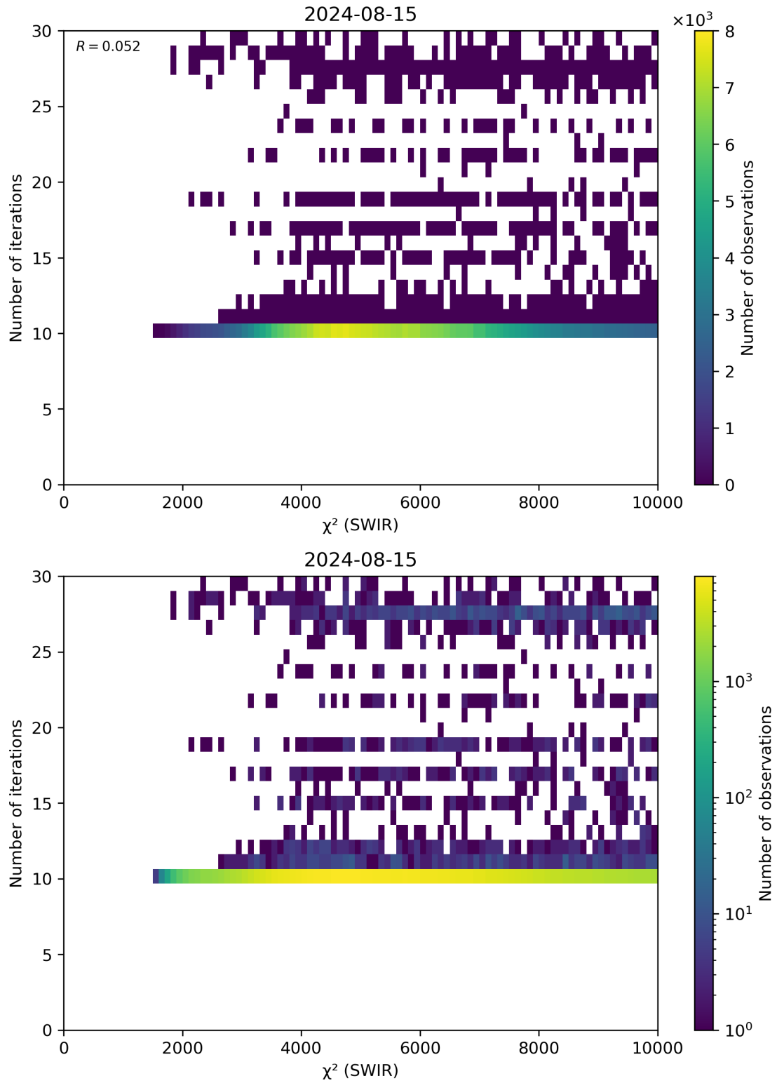
Figure 50: Scatter density plot of “ \chi^2 (SWIR)” against “Number of iterations” for 2024-08-14 to 2024-08-16.
