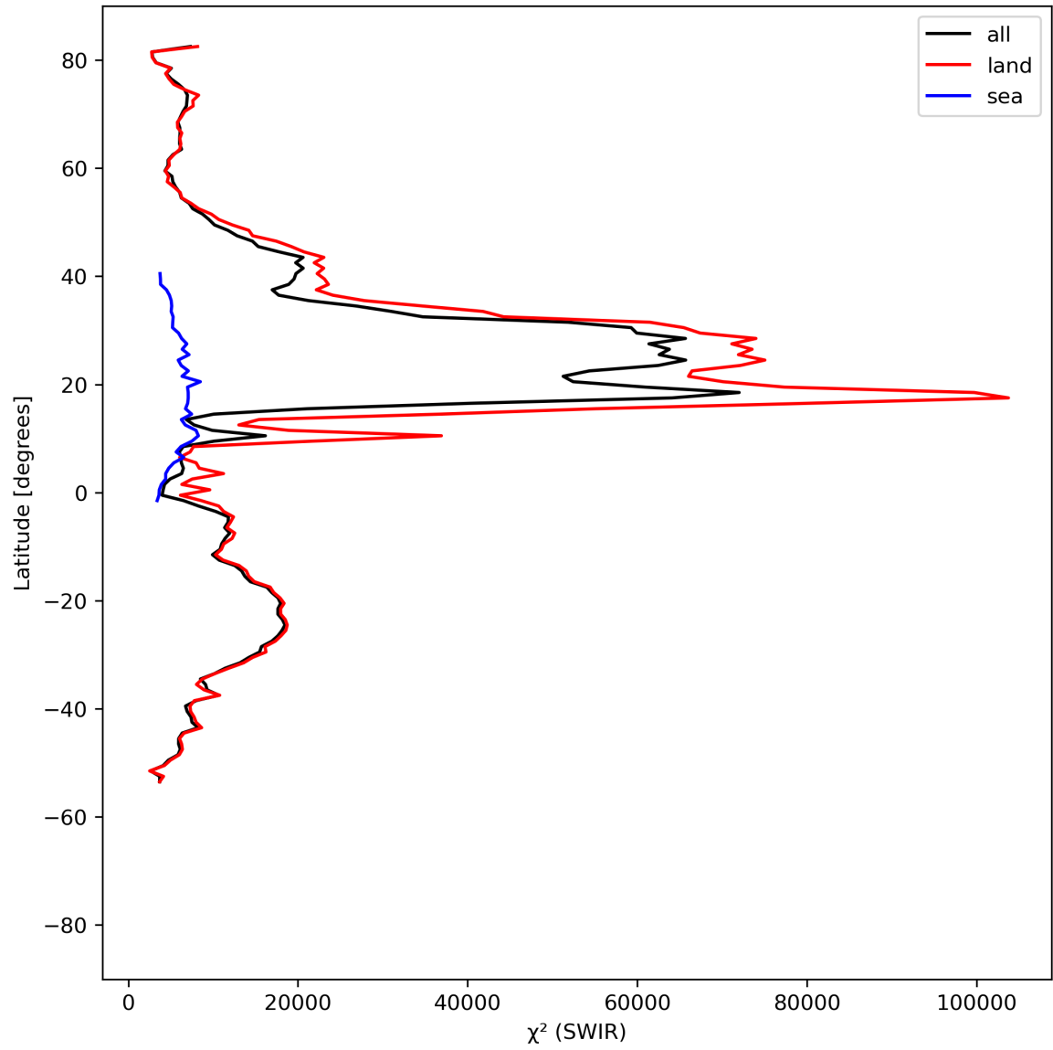
Figure 17: Zonal average of “ \chi^2 (SWIR)” for 2024-08-14 to 2024-08-16.
