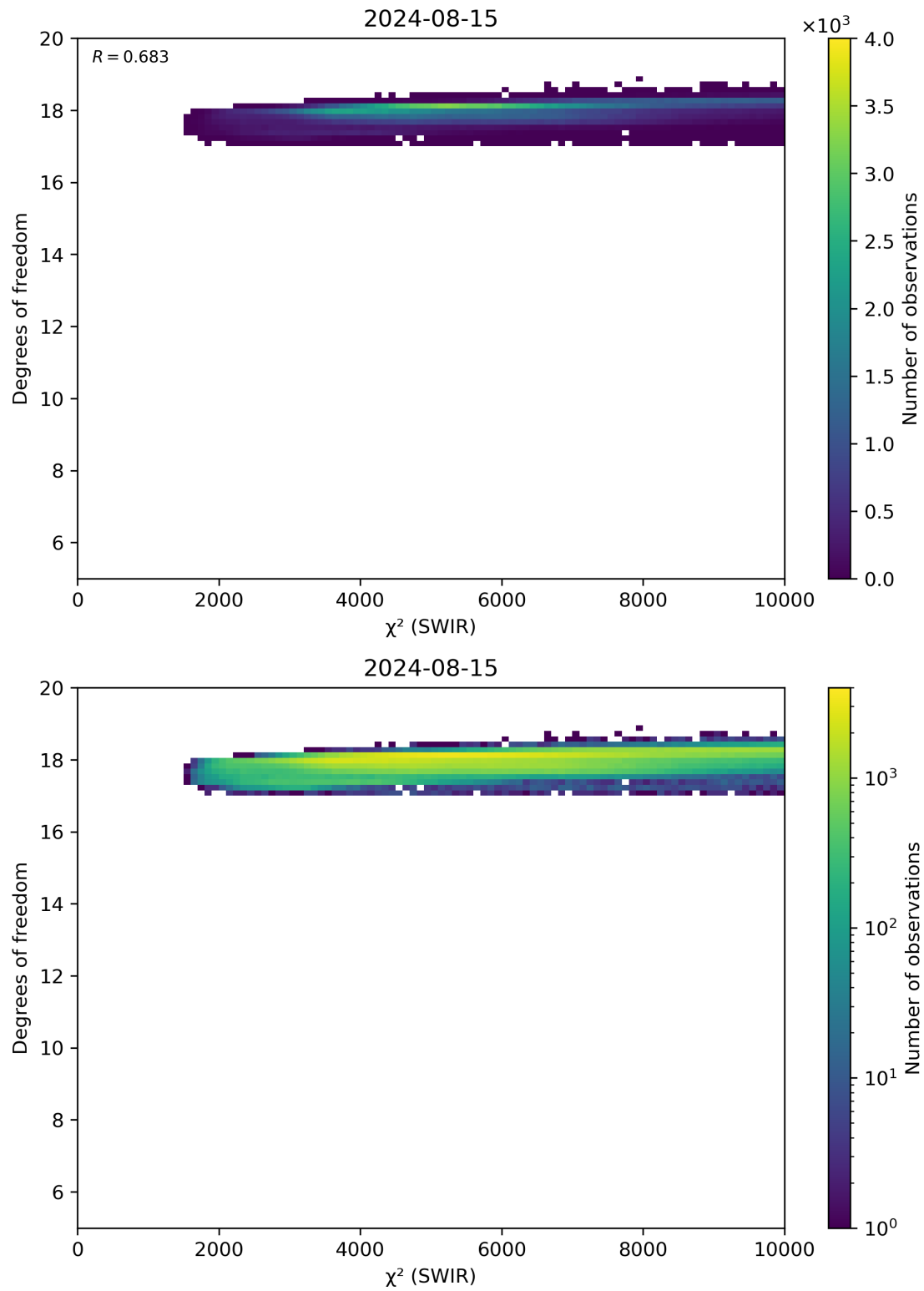
Figure 48: Scatter density plot of “ \chi^2 (SWIR)” against “Degrees of freedom” for 2024-08-14 to 2024-08-16.
