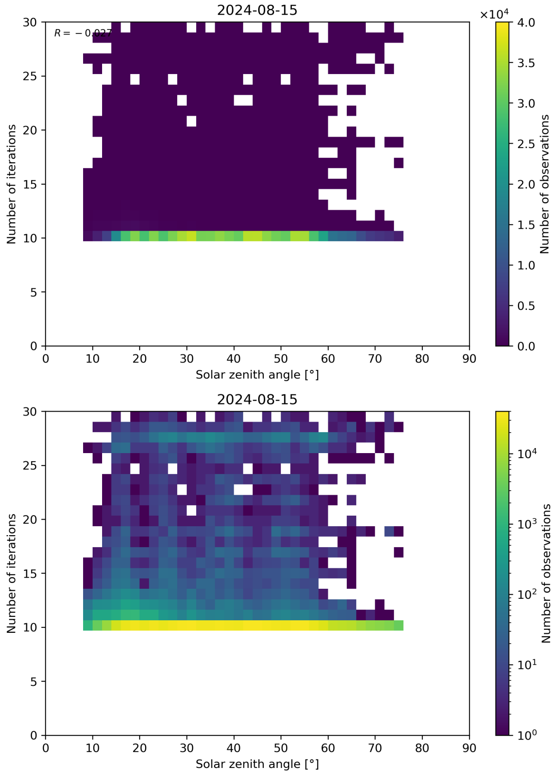
Figure 102: Scatter density plot of “Solar zenith angle” against “Number of iterations” for 2024-08-14 to 2024-08-16.
