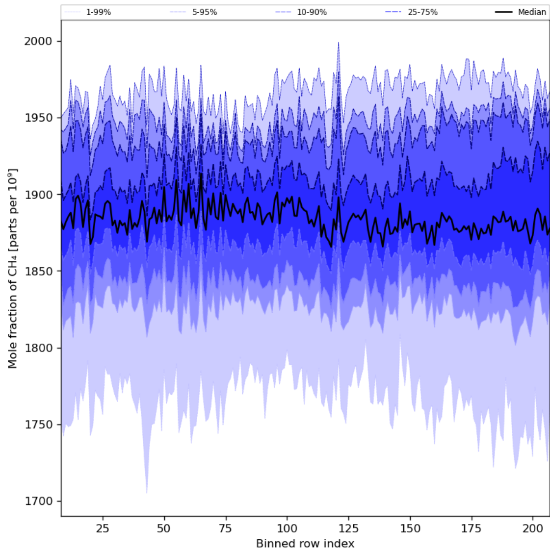
Figure 34: Along track statistics of “Mole fraction of CH 4 ” for 2024-08-14 to 2024-08-16
