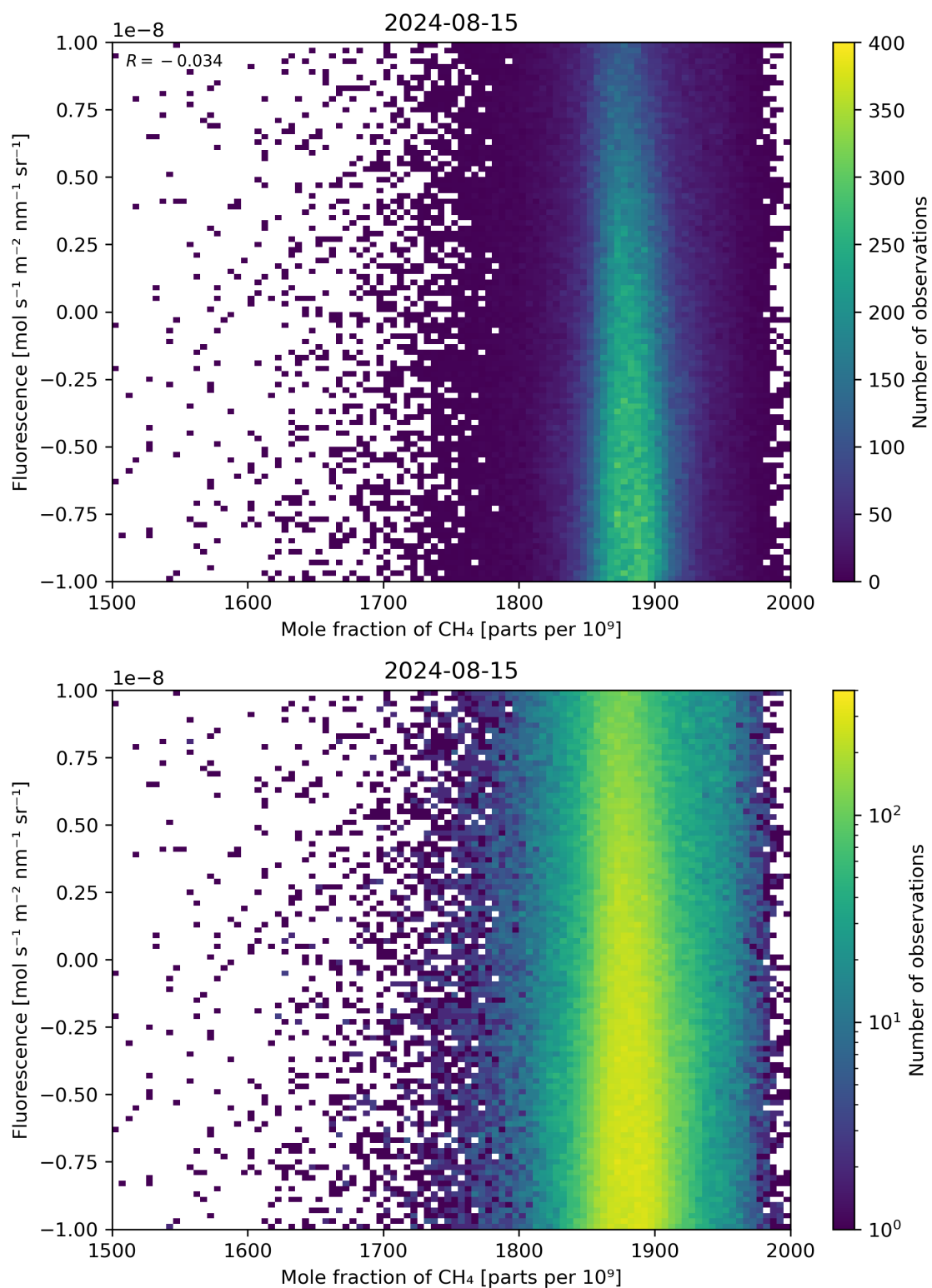
Figure 73: Scatter density plot of “Mole fraction of \text{CH}_4 ” against “Fluorescence” for 2024-08-14 to 2024-08-16.
