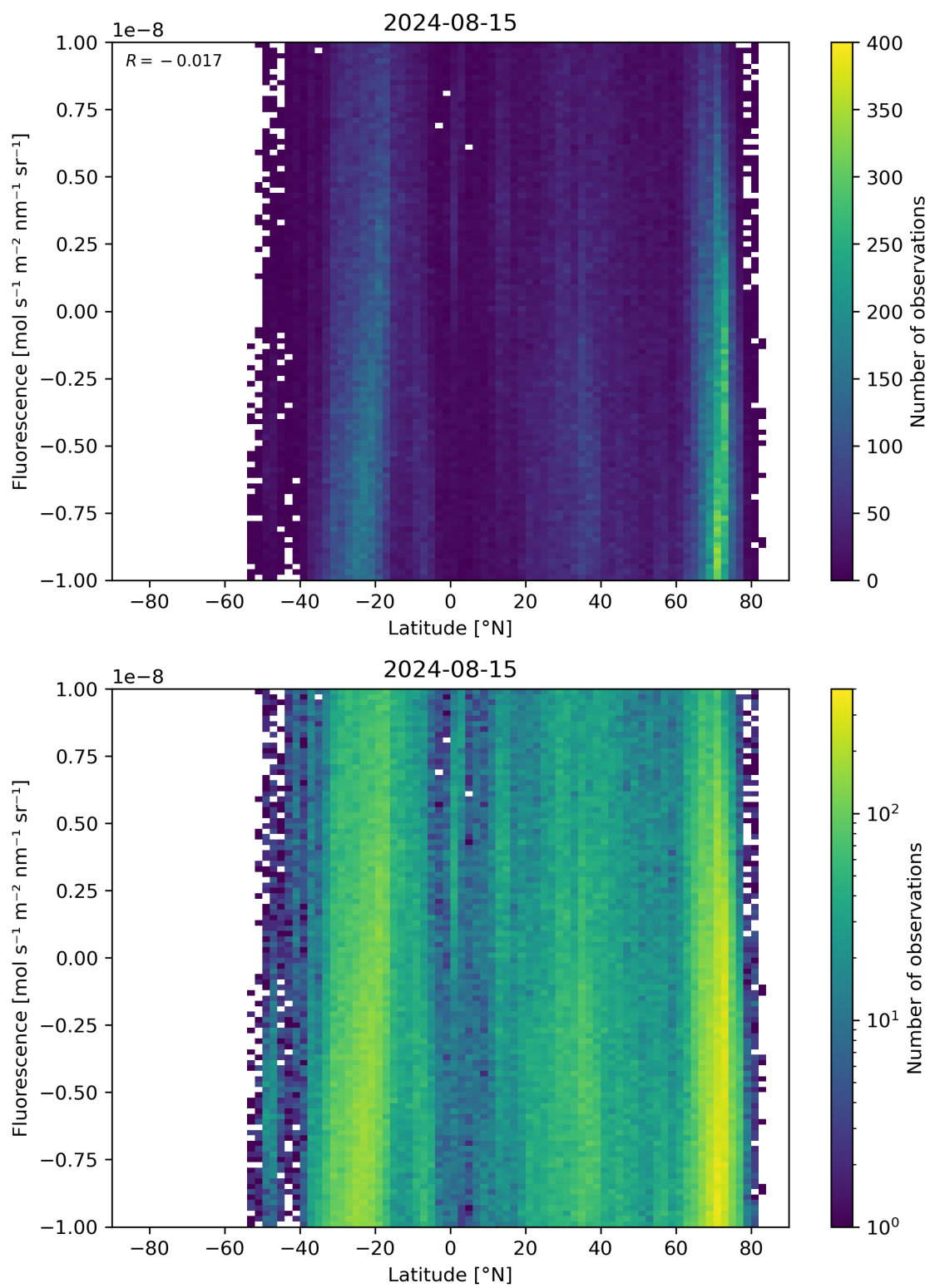
Figure 56: Scatter density plot of “Latitude” against “Fluorescence” for 2024-08-14 to 2024-08-16.
