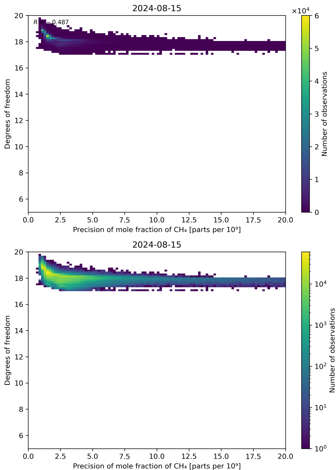
Figure 80: Scatter density plot of “Precision of mole fraction of CH 4 ” against “Degrees of freedom” for 2024-08-14 to 2024-08-16.
