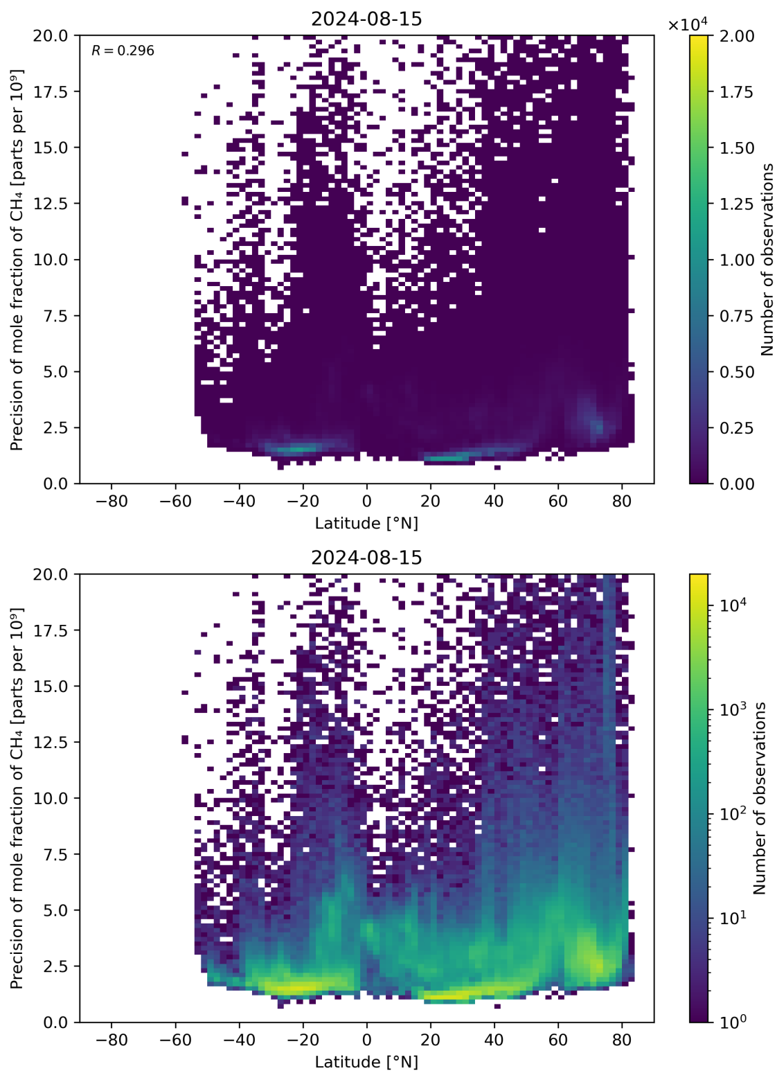
Figure 59: Scatter density plot of “Latitude” against “Precision of mole fraction of \text{CH}_4 ” for 2024-08-14 to 2024-08-16.
