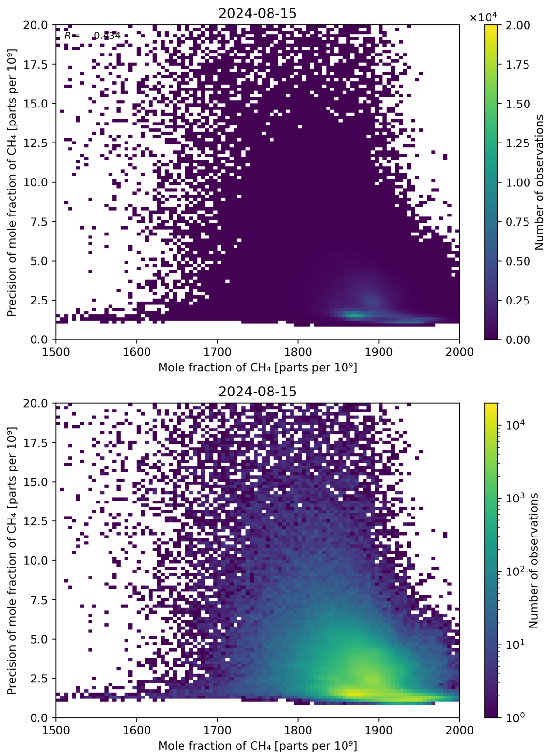
Figure 75: Scatter density plot of “Mole fraction of CH 4 ” against “Precision of mole fraction of CH 4 ” for 2024-08-14 to 2024-08-16.
