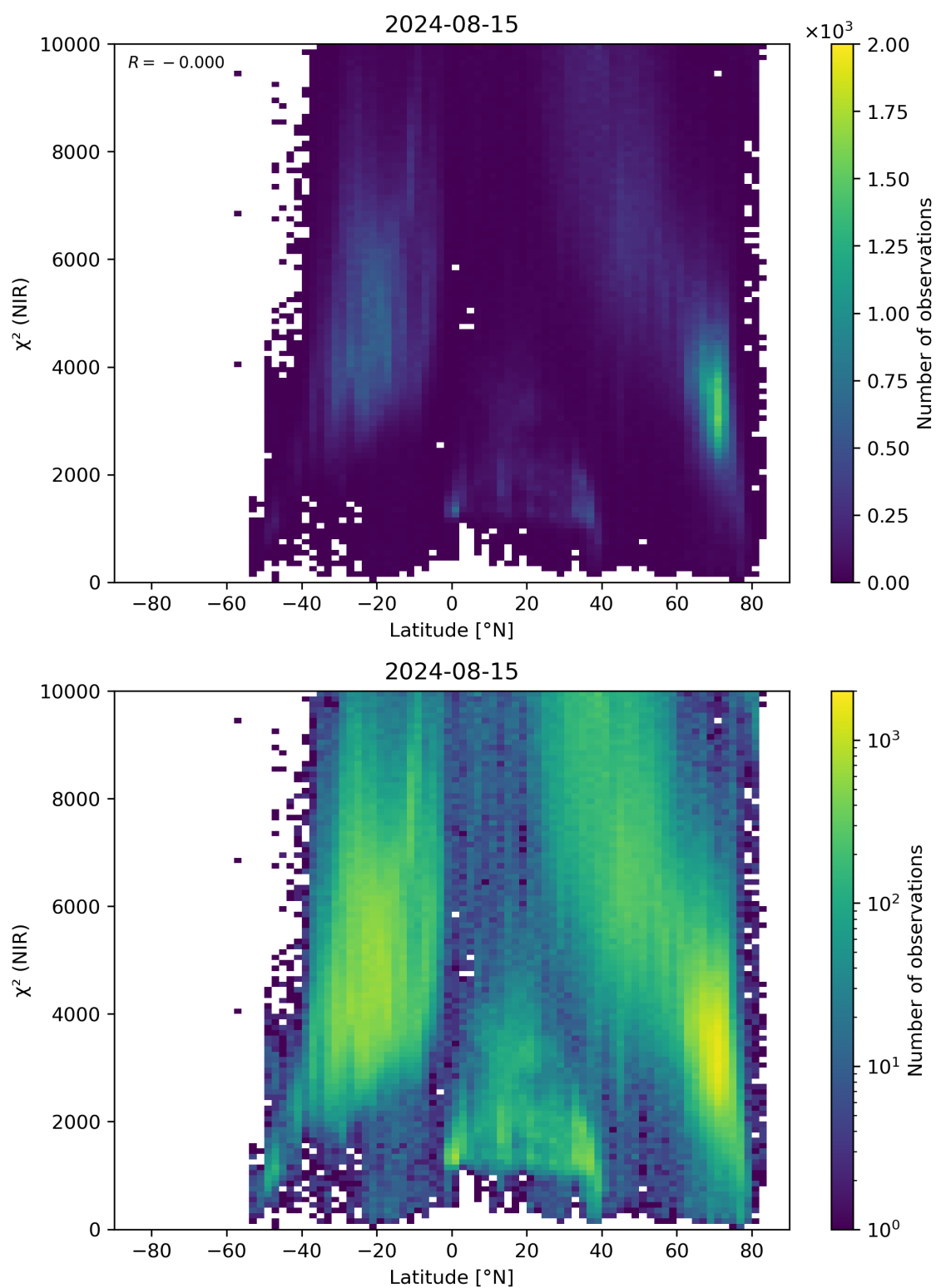
Figure 53: Scatter density plot of “Latitude” against “ \chi^2 (NIR)” for 2024-08-14 to 2024-08-16.
