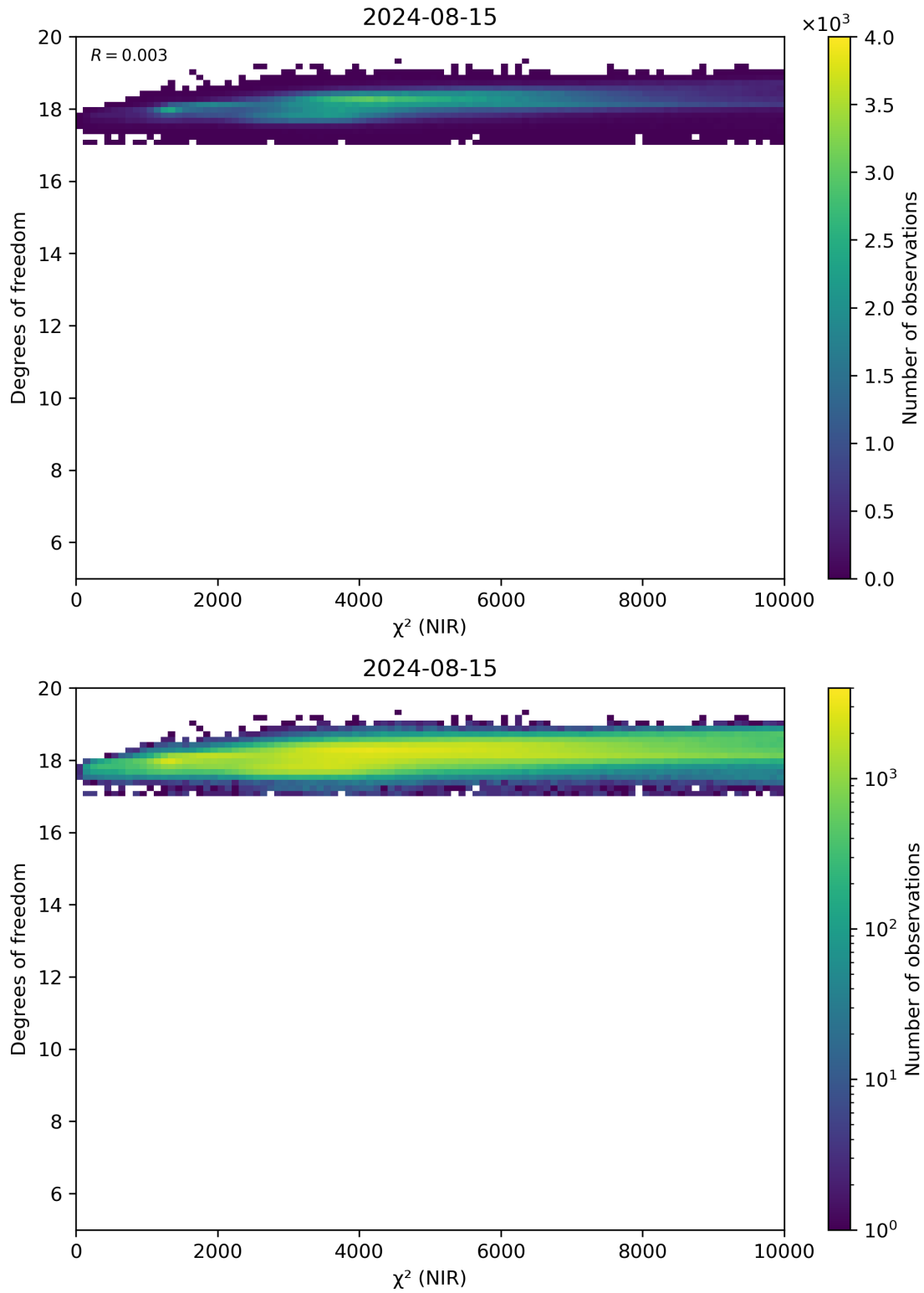
Figure 44: Scatter density plot of “ \chi^2 (NIR)” against “Degrees of freedom” for 2024-08-14 to 2024-08-16.
