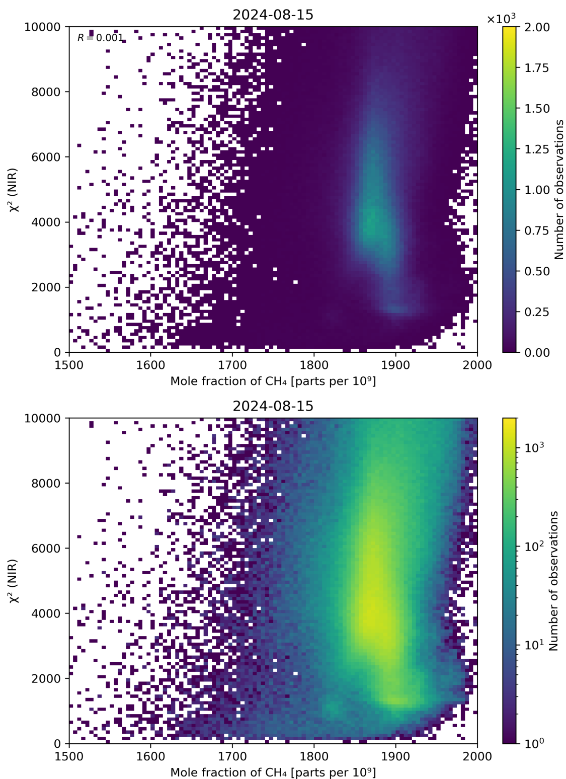
Figure 70: Scatter density plot of “Mole fraction of \text{CH}_4 ” against “ \chi^2 (NIR)” for 2024-08-14 to 2024-08-16.
