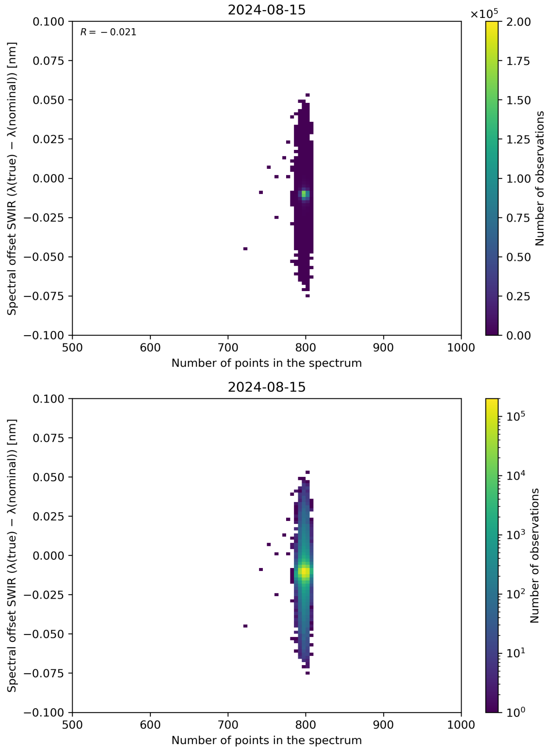
Figure 93: Scatter density plot of “Number of points in the spectrum” against “Spectral offset SWIR ( \lambda(\text{true}) - \lambda(\text{nominal}) )” for 2024-08-14 to 2024-08-16.
