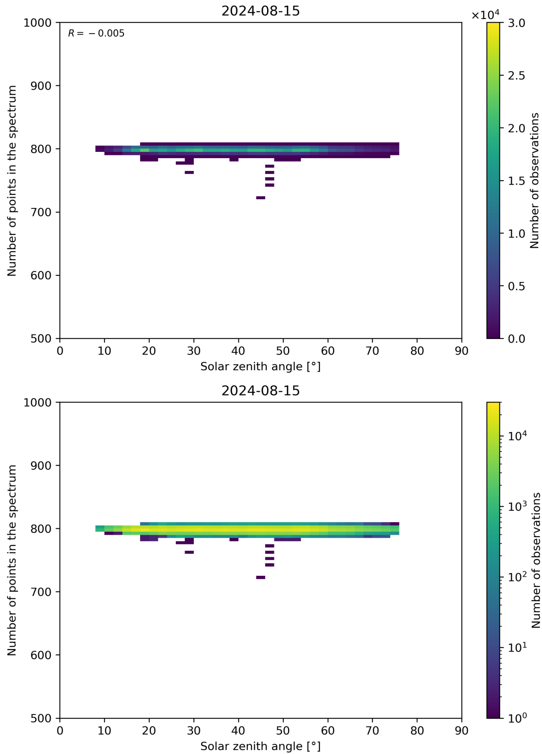
Figure 103: Scatter density plot of “Solar zenith angle” against “Number of points in the spectrum” for 2024-08-14 to 2024-08-16.
