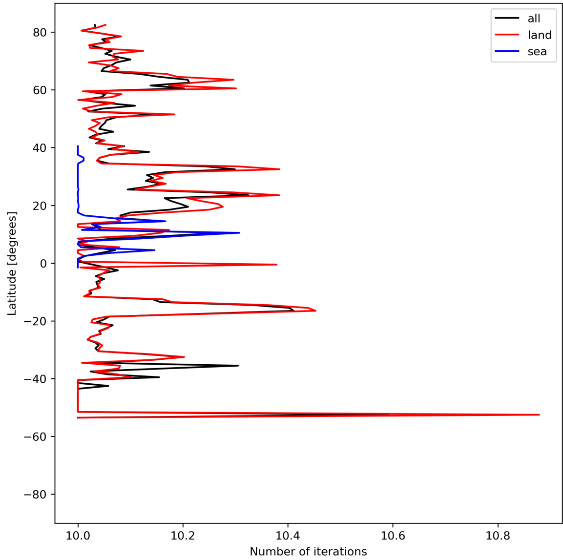
Figure 20: Zonal average of “Number of iterations” for 2024-08-14 to 2024-08-16.
