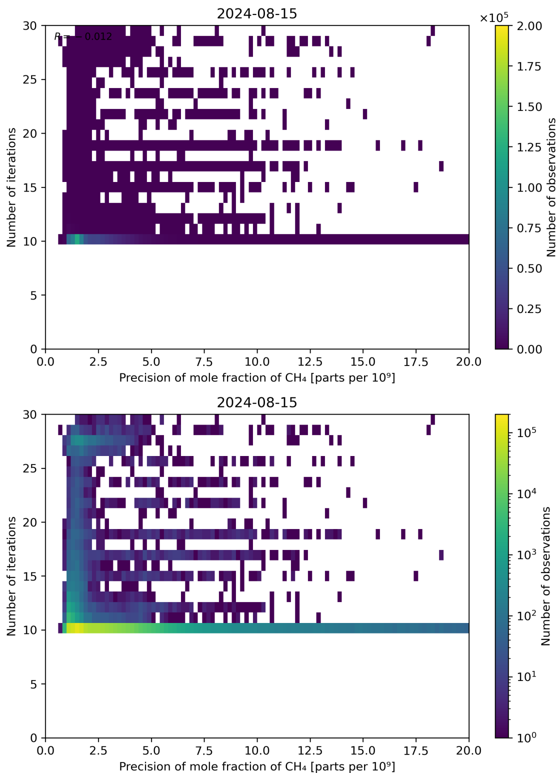
Figure 83: Scatter density plot of “Precision of mole fraction of CH 4 ” against “Number of iterations” for 2024-08-14 to 2024-08-16.
