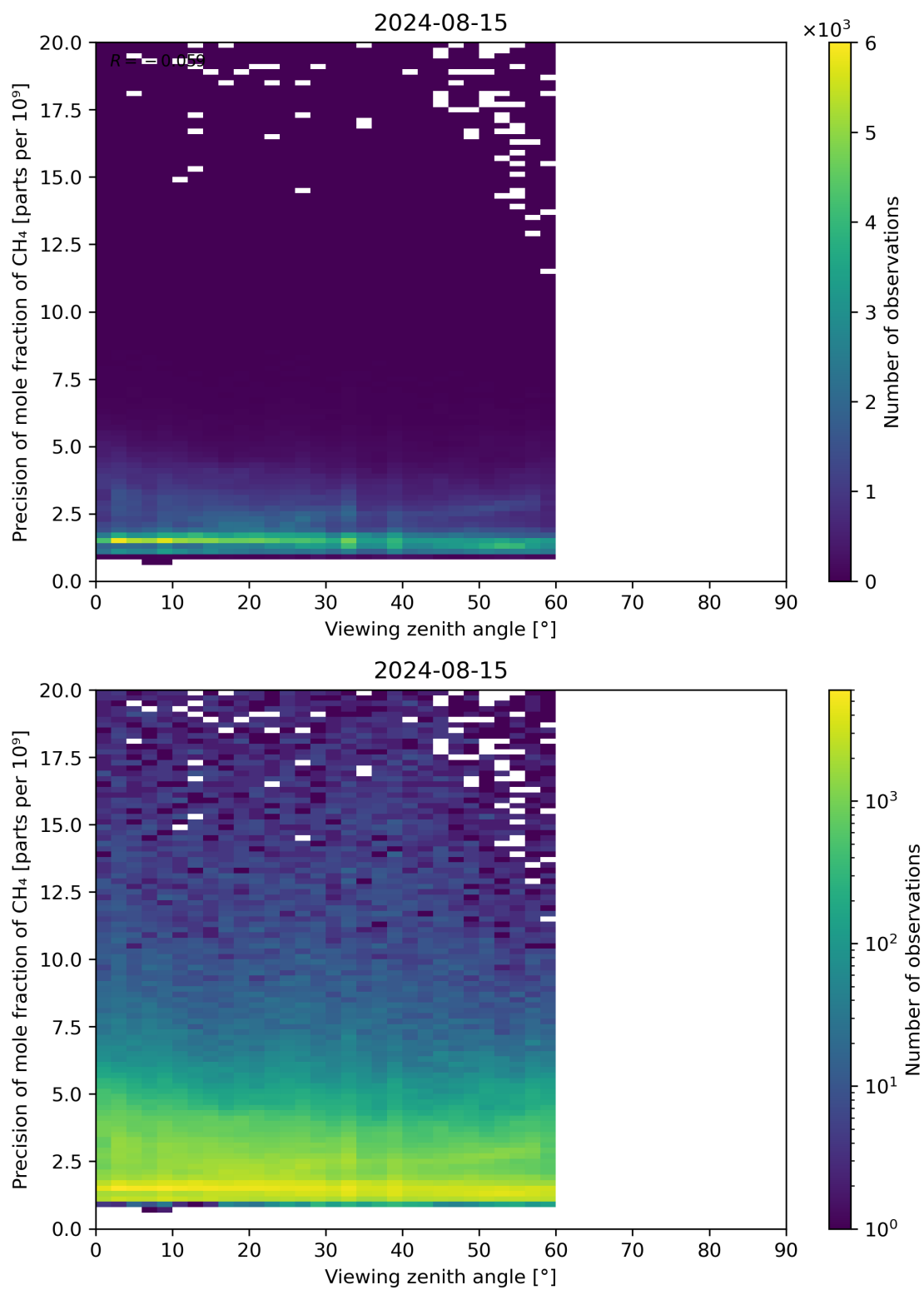
Figure 112: Scatter density plot of “Viewing zenith angle” against “Precision of mole fraction of CH 4 ” for 2024-08-14 to 2024-08-16.
