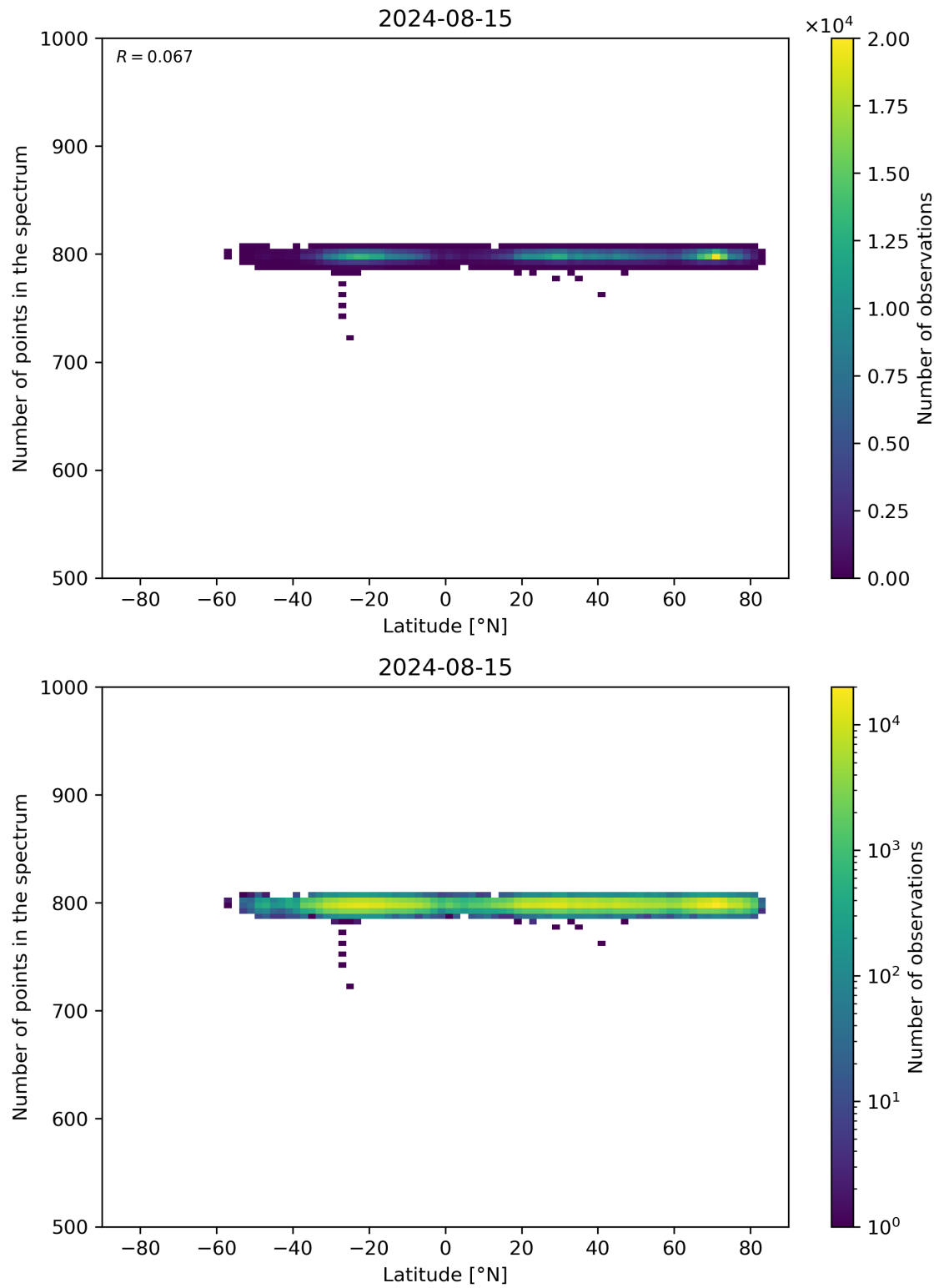
Figure 61: Scatter density plot of “Latitude” against “Number of points in the spectrum” for 2024-08-14 to 2024-08-16.
