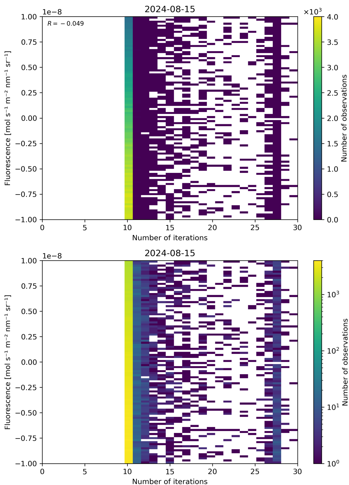
Figure 87: Scatter density plot of “Number of iterations” against “Fluorescence” for 2024-08-14 to 2024-08-16.
