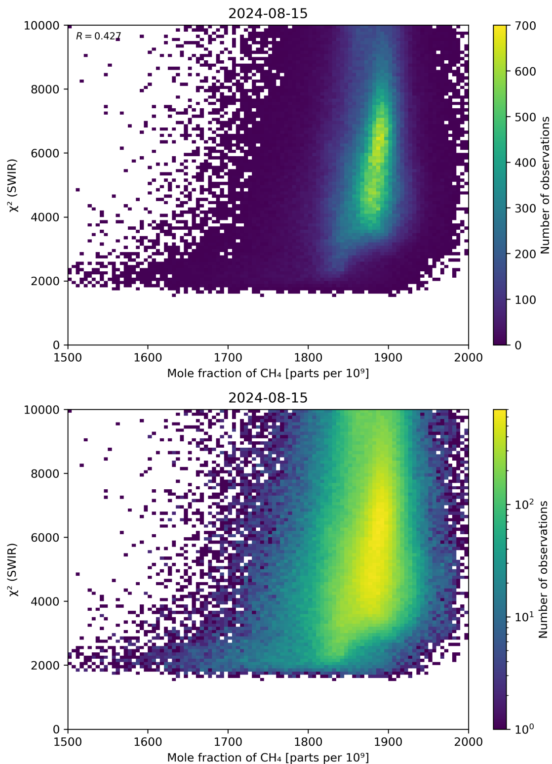
Figure 71: Scatter density plot of “Mole fraction of CH 4 ” against “ \chi^2 (SWIR)” for 2024-08-14 to 2024-08-16.
