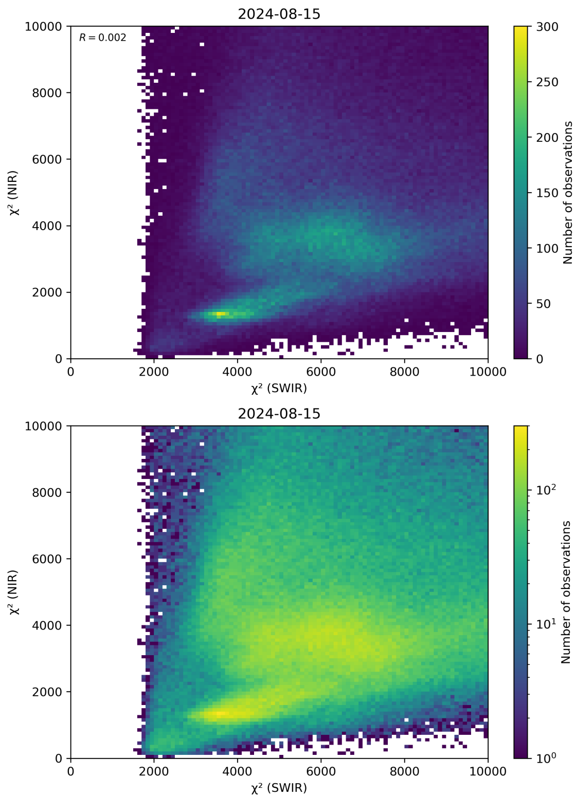
Figure 47: Scatter density plot of “ \chi^2 (SWIR)” against “ \chi^2 (NIR)” for 2024-08-14 to 2024-08-16.
