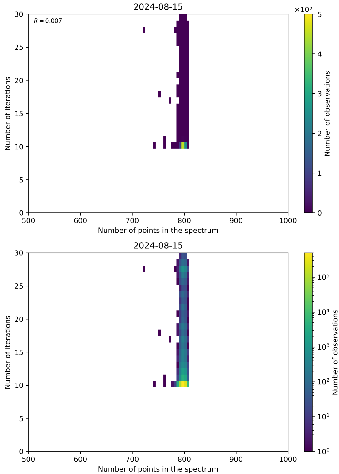
Figure 92: Scatter density plot of “Number of points in the spectrum” against “Number of iterations” for 2024-08-14 to 2024-08-16.
