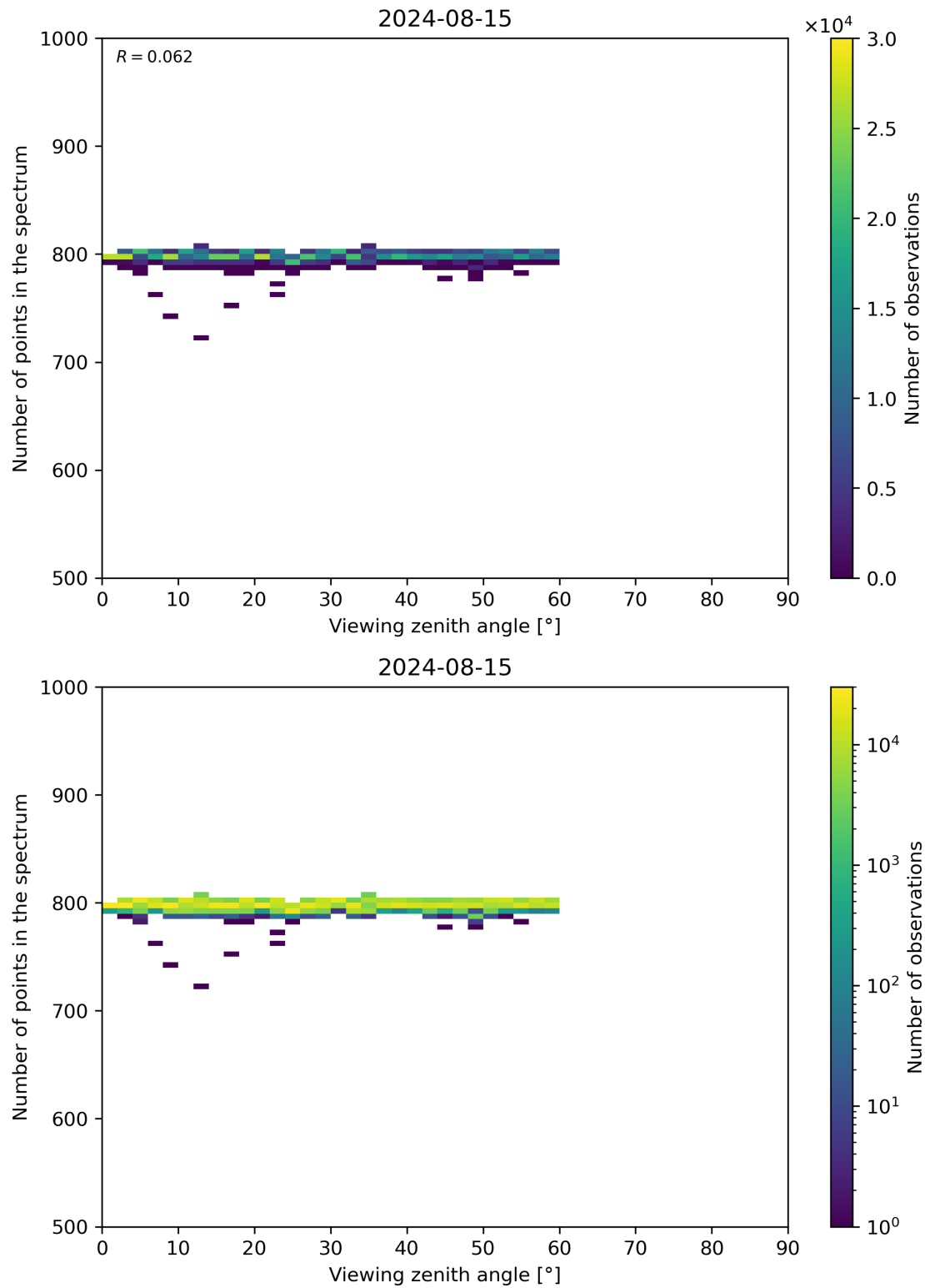
Figure 114: Scatter density plot of “Viewing zenith angle” against “Number of points in the spectrum” for 2024-08-14 to 2024-08-16.
