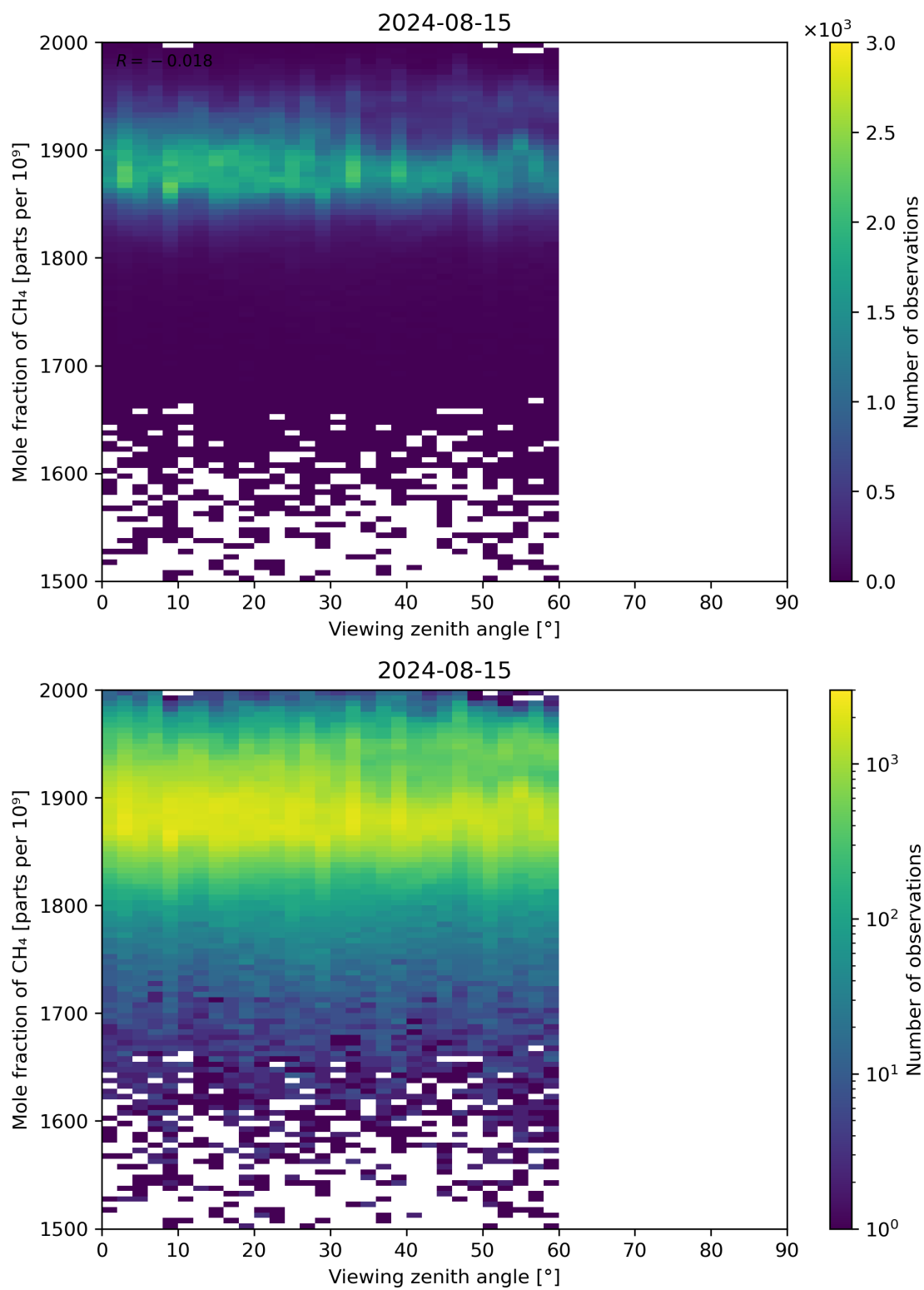
Figure 110: Scatter density plot of “Viewing zenith angle” against “Mole fraction of CH 4 ” for 2024-08-14 to 2024-08-16.
