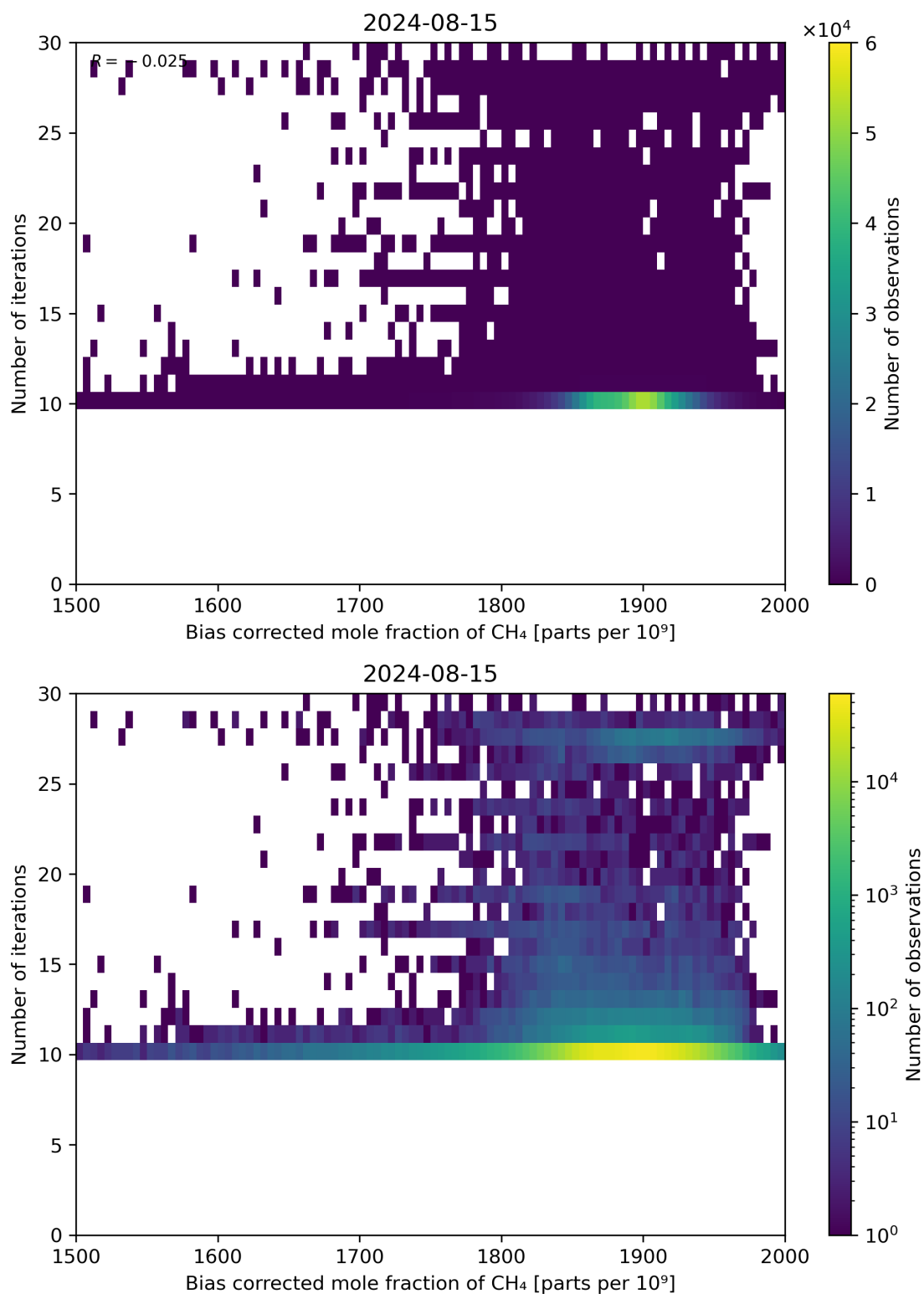
Figure 67: Scatter density plot of “Bias corrected mole fraction of CH 4 ” against “Number of iterations” for 2024-08-14 to 2024-08-16.
