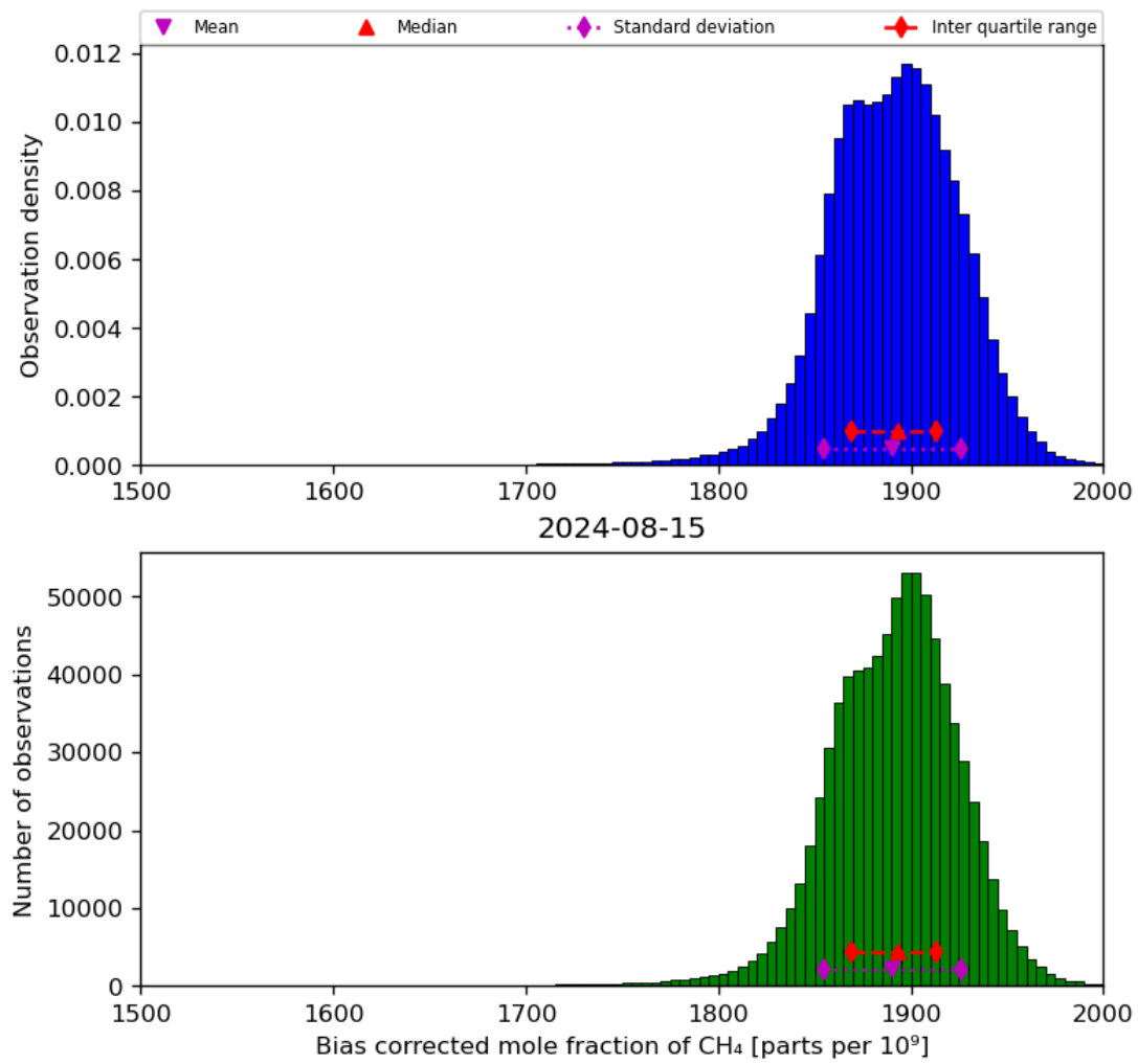
Figure 25: Histogram of “Bias corrected mole fraction of CH 4 ” for 2024-08-14 to 2024-08-16
