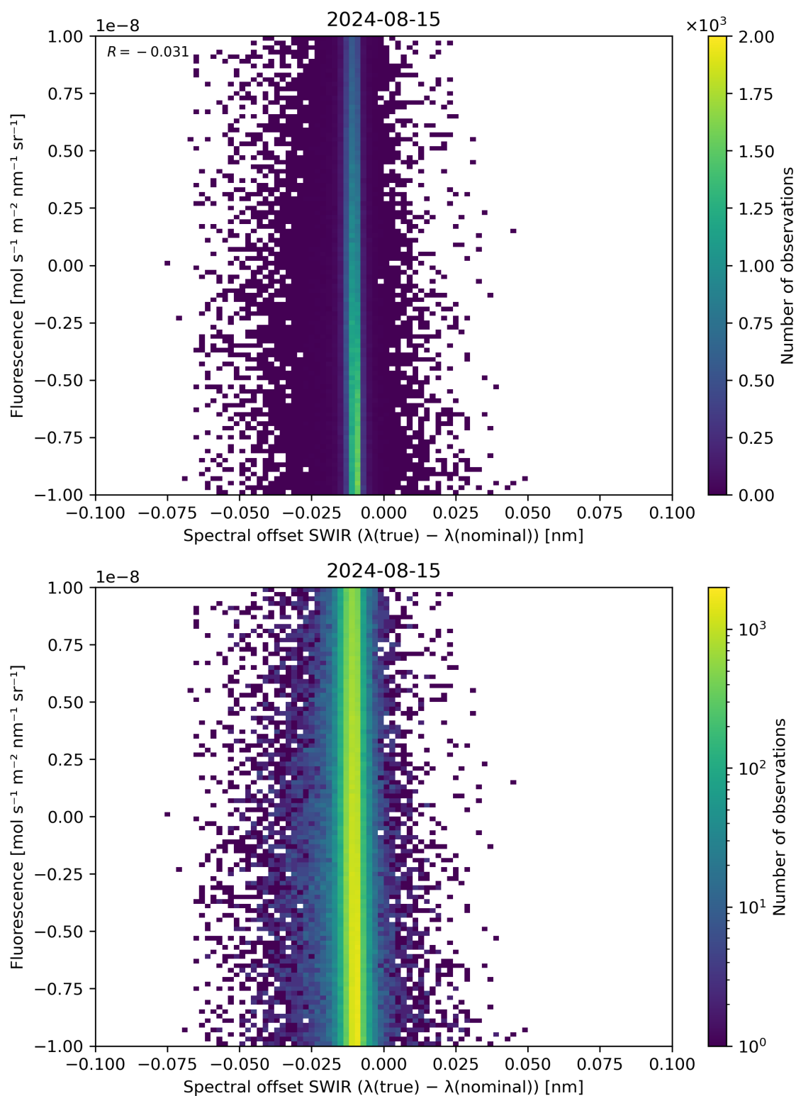
Figure 120: Scatter density plot of “Spectral offset SWIR ( \lambda(\text{true}) - \lambda(\text{nominal}) )” against “Fluorescence” for 2024-08-14 to 2024-08-16.
