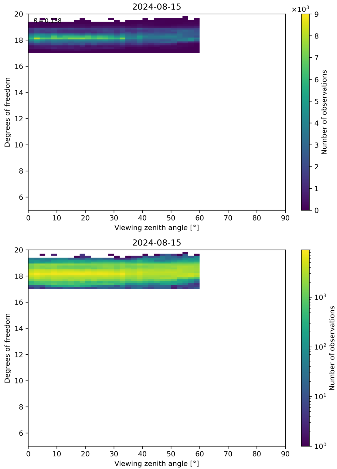
Figure 107: Scatter density plot of “Viewing zenith angle” against “Degrees of freedom” for 2024-08-14 to 2024-08-16.
