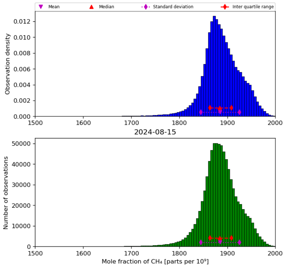
Figure 23: Histogram of “Mole fraction of CH 4 ” for 2024-08-14 to 2024-08-16
