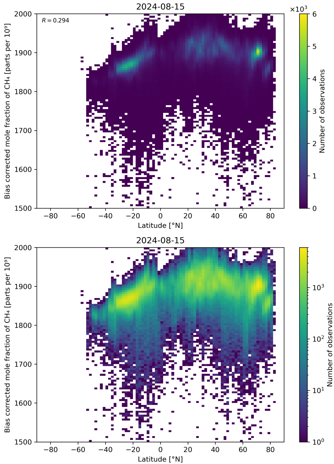
Figure 58: Scatter density plot of “Latitude” against “Bias corrected mole fraction of \text{CH}_4 ” for 2024-08-14 to 2024-08-16.
