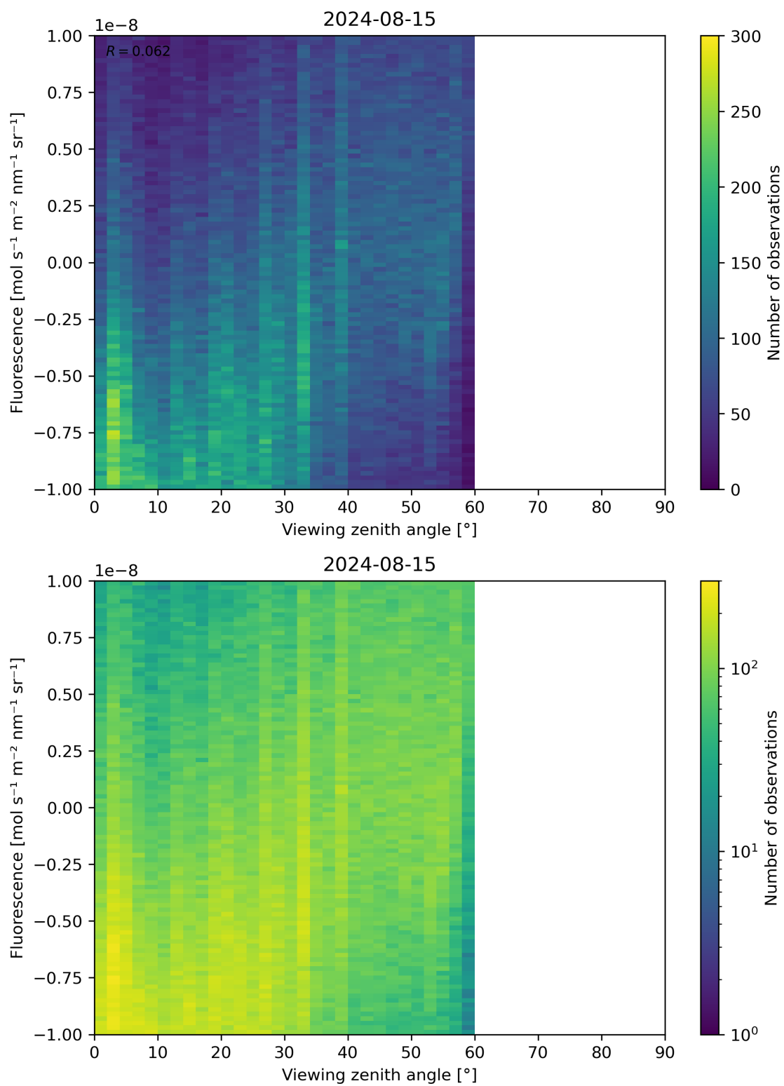
Figure 108: Scatter density plot of “Viewing zenith angle” against “Fluorescence” for 2024-08-14 to 2024-08-16.
