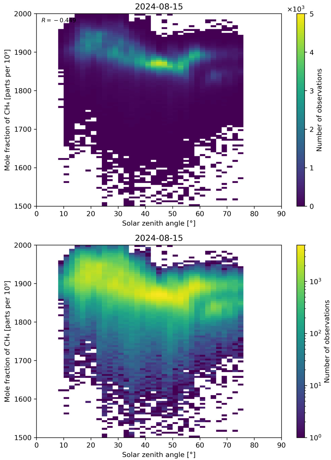
Figure 99: Scatter density plot of “Solar zenith angle” against “Mole fraction of \text{CH}_4 ” for 2024-08-14 to 2024-08-16.
