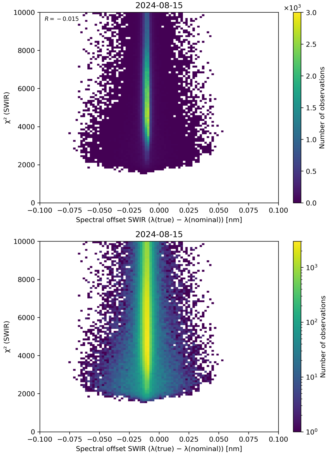
Figure 118: Scatter density plot of “Spectral offset SWIR ( \lambda(\text{true}) - \lambda(\text{nominal}) )” against “ \chi^2 (SWIR)” for 2024-08-14 to 2024-08-16.
