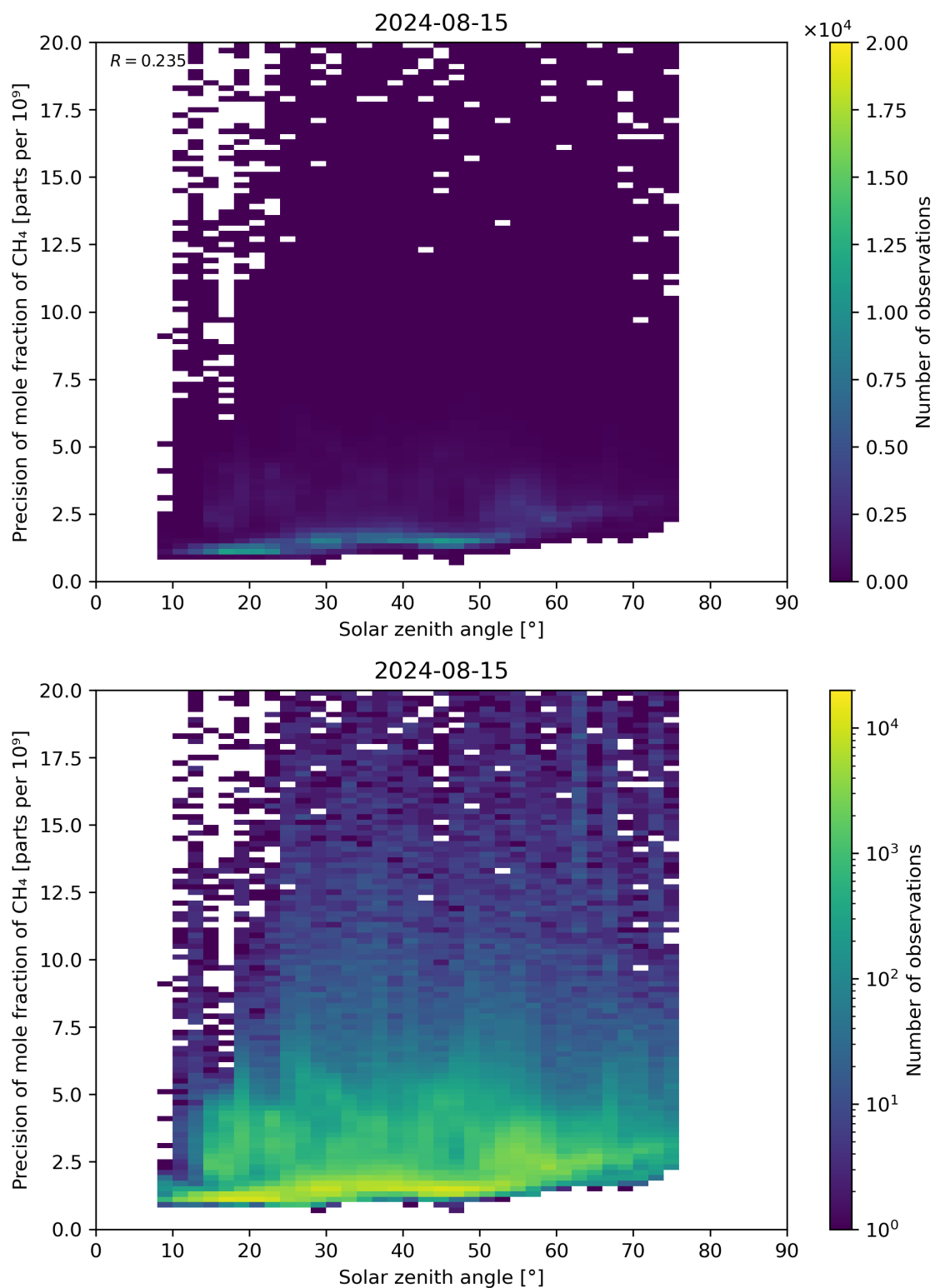
Figure 101: Scatter density plot of “Solar zenith angle” against “Precision of mole fraction of CH 4 ” for 2024-08-14 to 2024-08-16.
