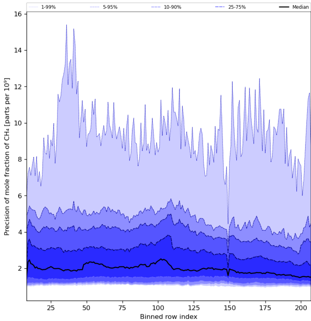
Figure 35: Along track statistics of “Precision of mole fraction of CH 4 ” for 2024-08-14 to 2024-08-16
