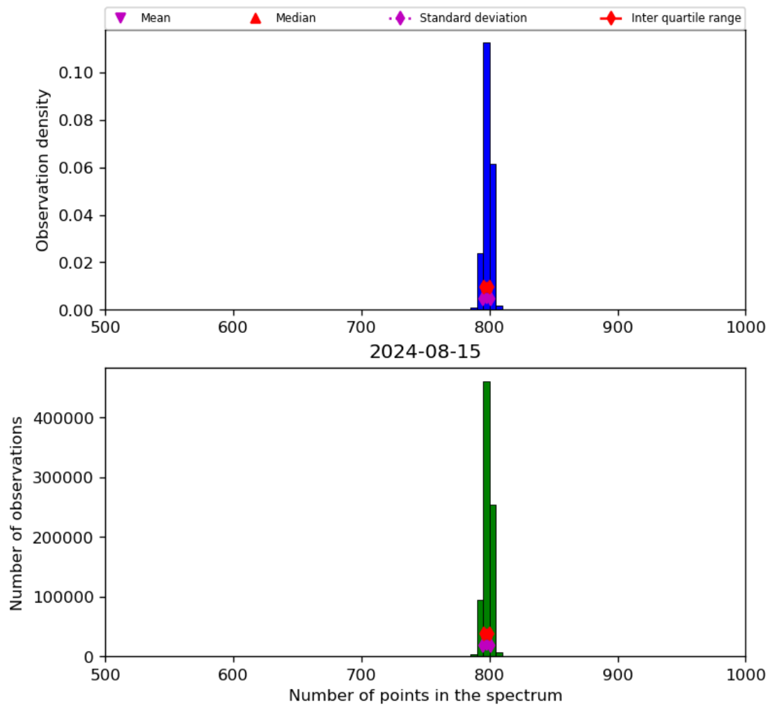
Figure 26: Histogram of “Number of points in the spectrum” for 2024-08-14 to 2024-08-16
