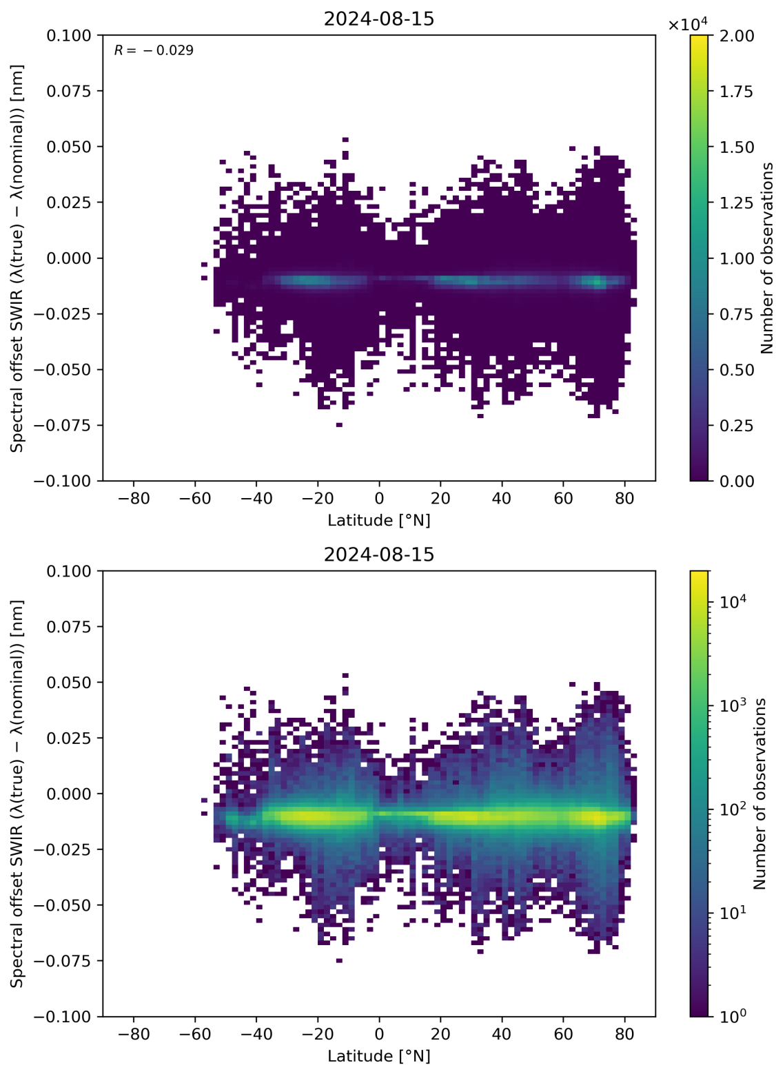
Figure 62: Scatter density plot of “Latitude” against “Spectral offset SWIR ( \lambda(\text{true}) - \lambda(\text{nominal}) )” for 2024-08-14 to 2024-08-16.
