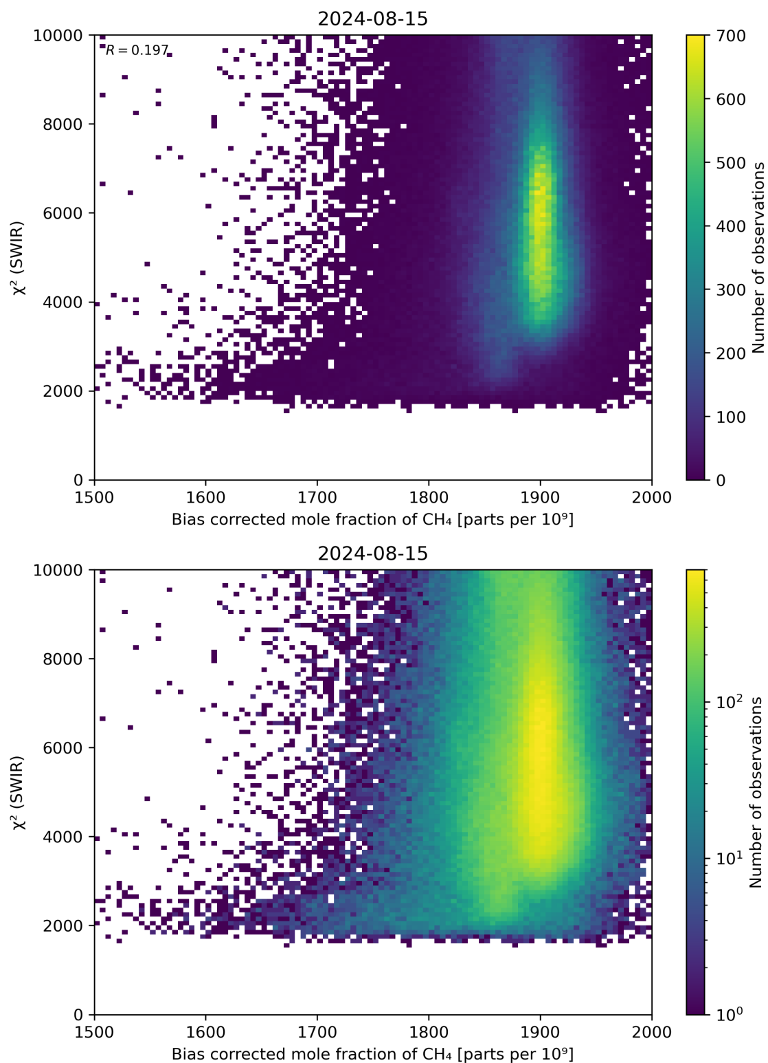
Figure 64: Scatter density plot of “Bias corrected mole fraction of CH 4 ” against “ \chi^2 (SWIR)” for 2024-08-14 to 2024-08-16.
