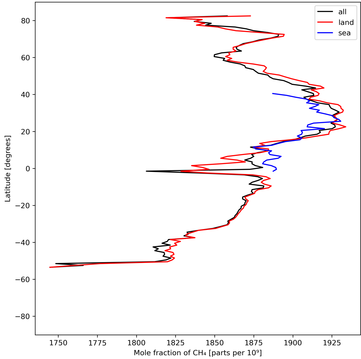
Figure 12: Zonal average of “Mole fraction of \text{CH}_4 ” for 2024-08-14 to 2024-08-16.
