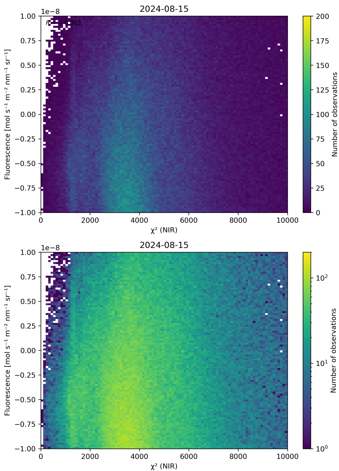
Figure 45: Scatter density plot of “ \chi^2 (NIR)” against “Fluorescence” for 2024-08-14 to 2024-08-16.
