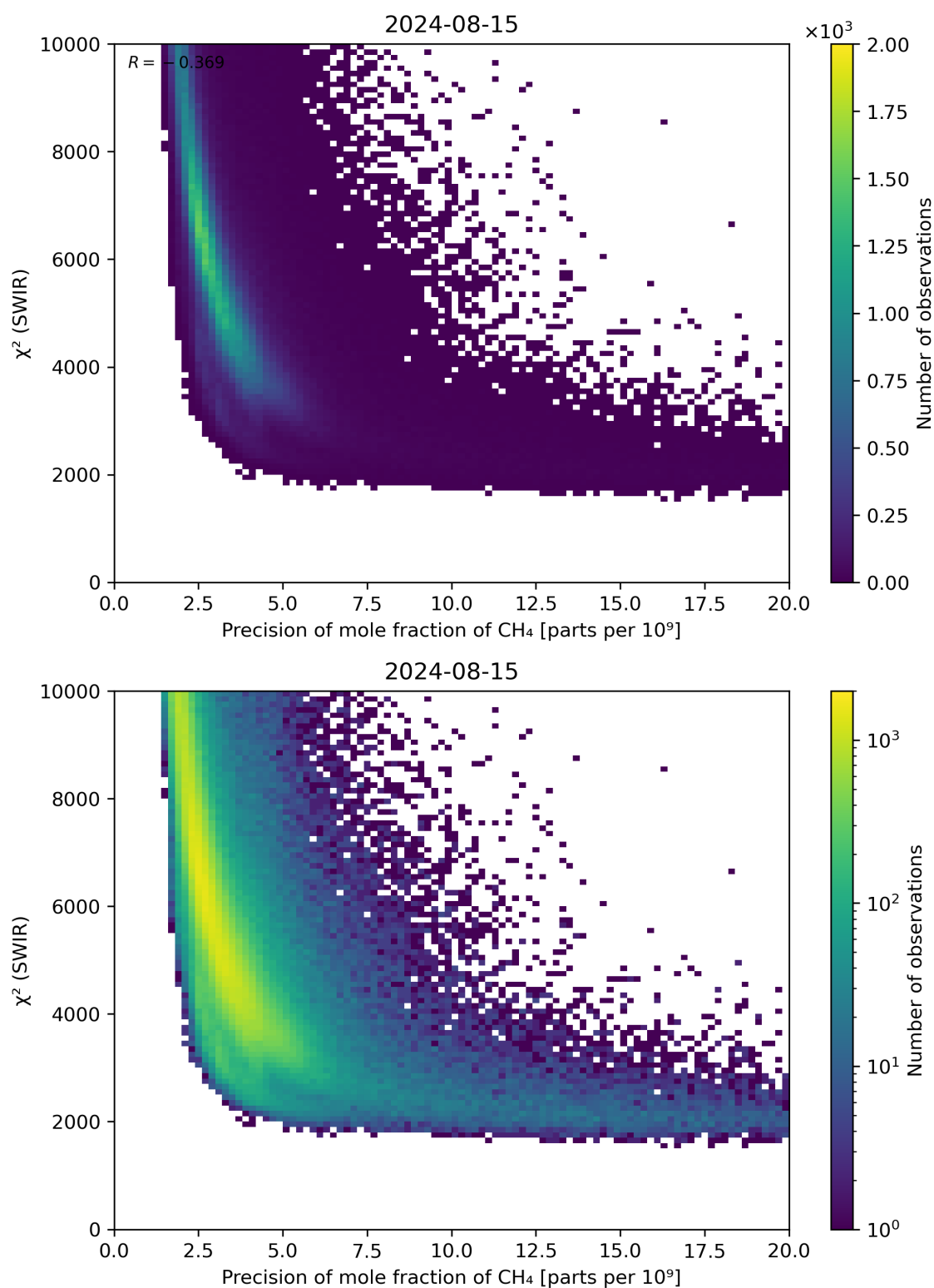
Figure 79: Scatter density plot of “Precision of mole fraction of \text{CH}_4 ” against “ \chi^2 (SWIR)” for 2024-08-14 to 2024-08-16.
