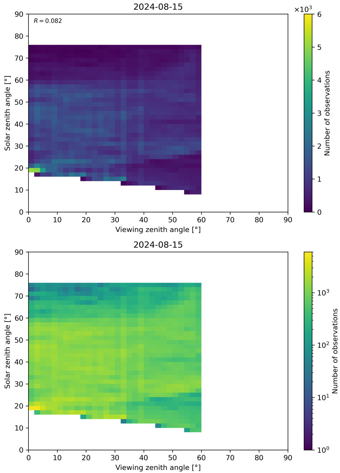
Figure 115: Scatter density plot of “Viewing zenith angle” against “Solar zenith angle” for 2024-08-14 to 2024-08-16.
