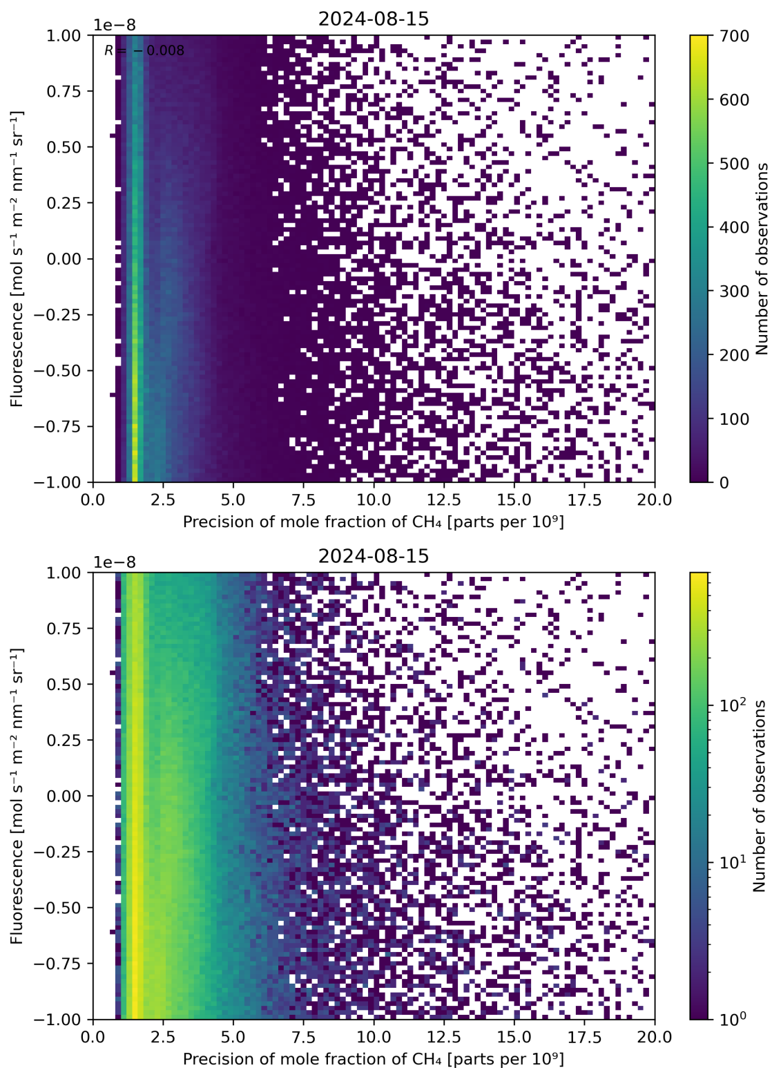
Figure 81: Scatter density plot of “Precision of mole fraction of \text{CH}_4 ” against “Fluorescence” for 2024-08-14 to 2024-08-16.
