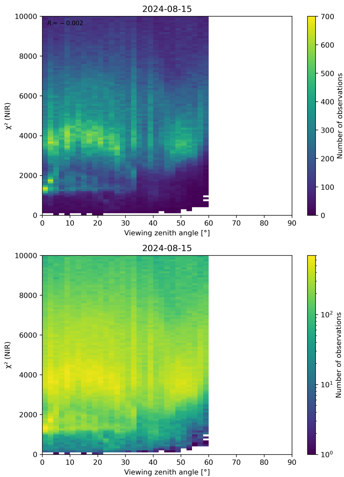
Figure 105: Scatter density plot of “Viewing zenith angle” against “ \chi^2 (NIR)” for 2024-08-14 to 2024-08-16.
