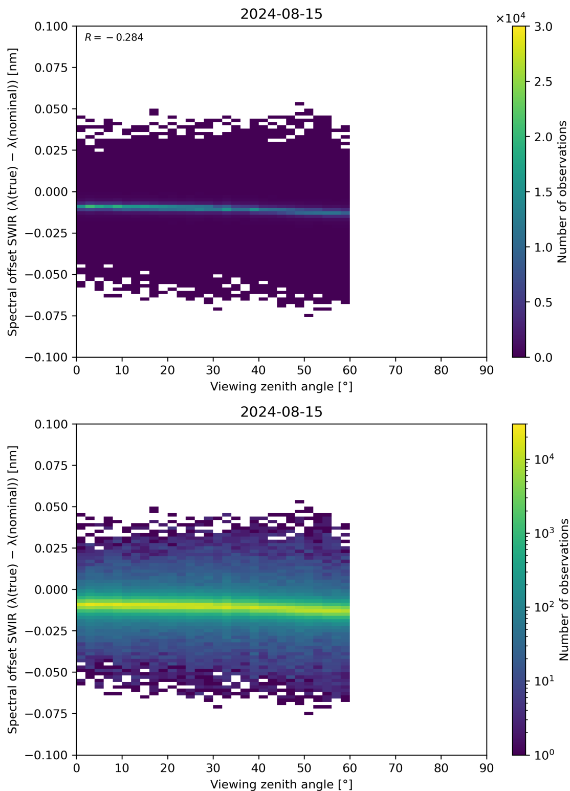
Figure 116: Scatter density plot of “Viewing zenith angle” against “Spectral offset SWIR ( \lambda(\text{true}) - \lambda(\text{nominal}) )” for 2024-08-14 to 2024-08-16.
