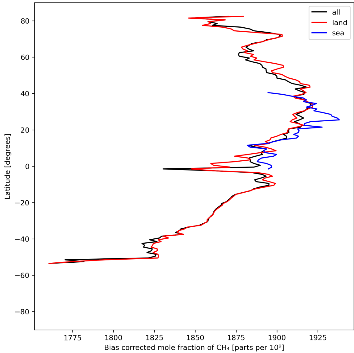
Figure 14: Zonal average of “Bias corrected mole fraction of CH 4 ” for 2024-08-14 to 2024-08-16.
