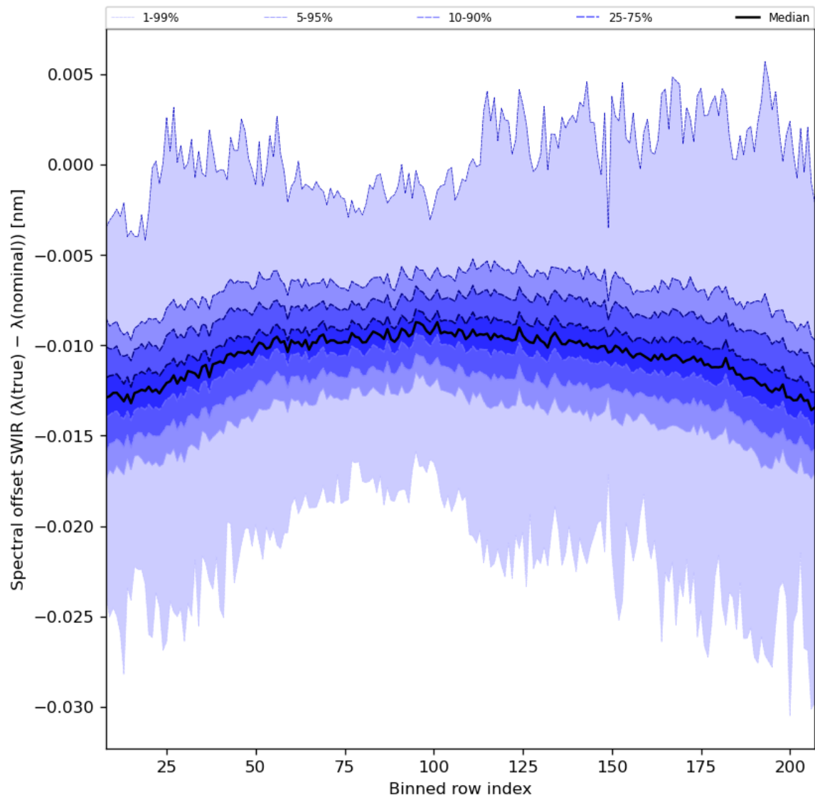
Figure 38: Along track statistics of “Spectral offset SWIR ( \lambda(\text{true}) - \lambda(\text{nominal}) )” for 2024-08-14 to 2024-08-16
