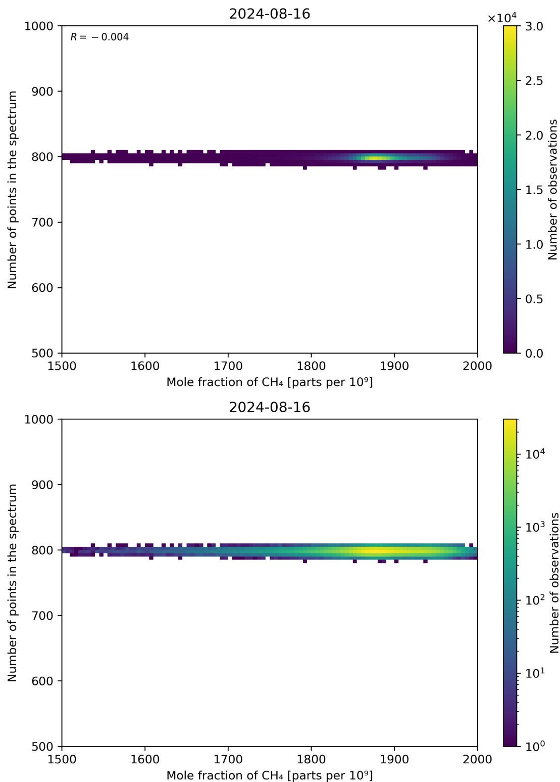
Figure 77: Scatter density plot of “Mole fraction of CH 4 ” against “Number of points in the spectrum” for 2024-08-16 to 2024-08-17.
