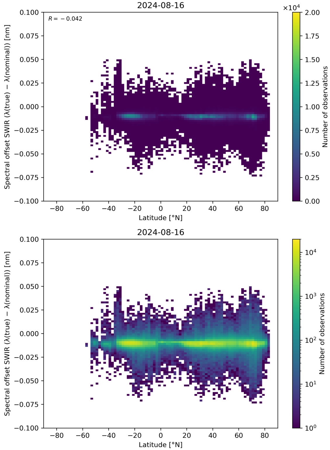
Figure 62: Scatter density plot of “Latitude” against “Spectral offset SWIR ( \lambda(\text{true}) - \lambda(\text{nominal}) )” for 2024-08-16 to 2024-08-17.
