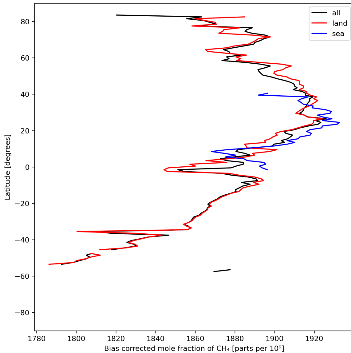
Figure 14: Zonal average of “Bias corrected mole fraction of CH 4 ” for 2024-08-16 to 2024-08-17.
