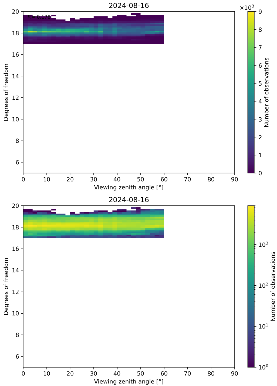
Figure 107: Scatter density plot of “Viewing zenith angle” against “Degrees of freedom” for 2024-08-16 to 2024-08-17.
