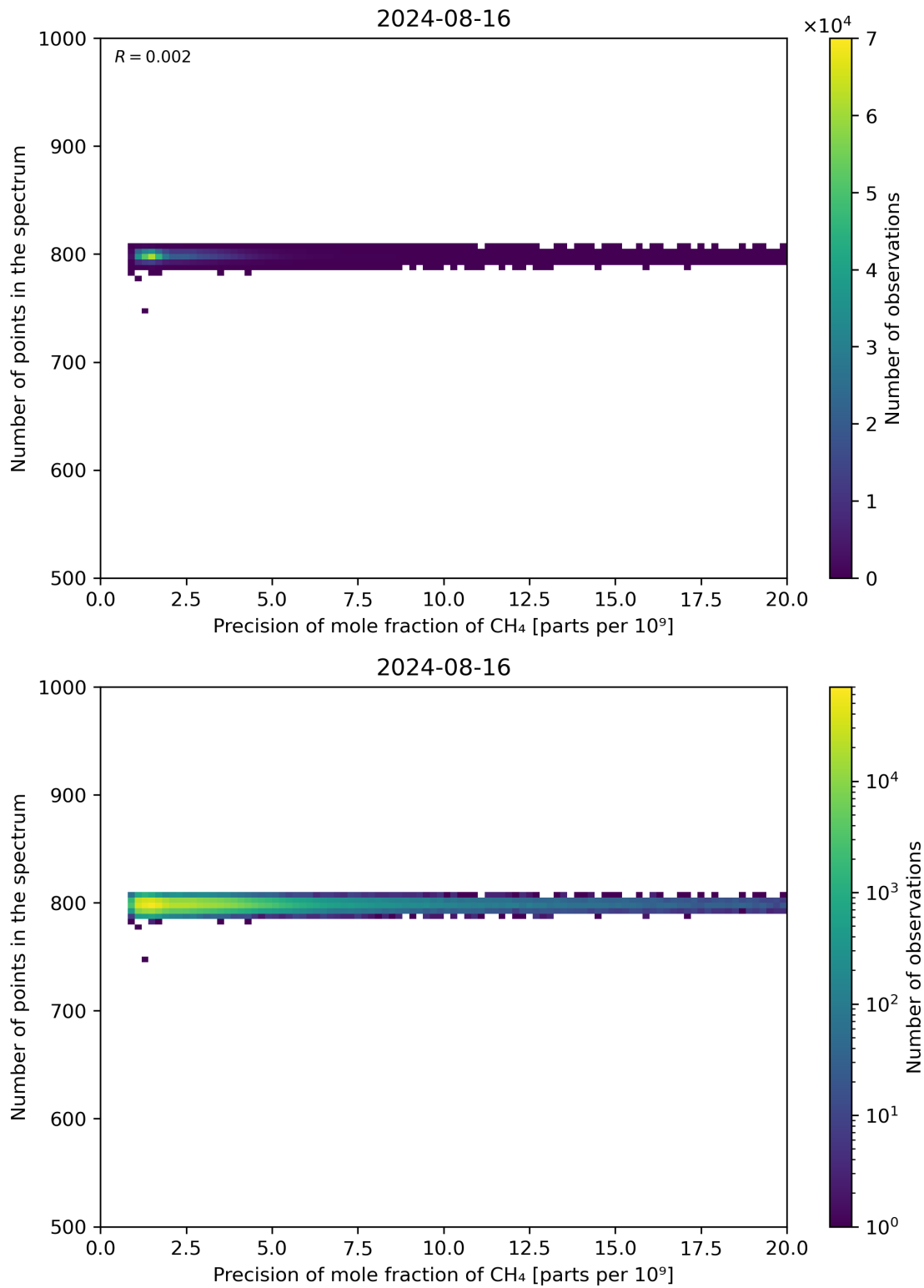
Figure 84: Scatter density plot of “Precision of mole fraction of CH 4 ” against “Number of points in the spectrum” for 2024-08-16 to 2024-08-17.
