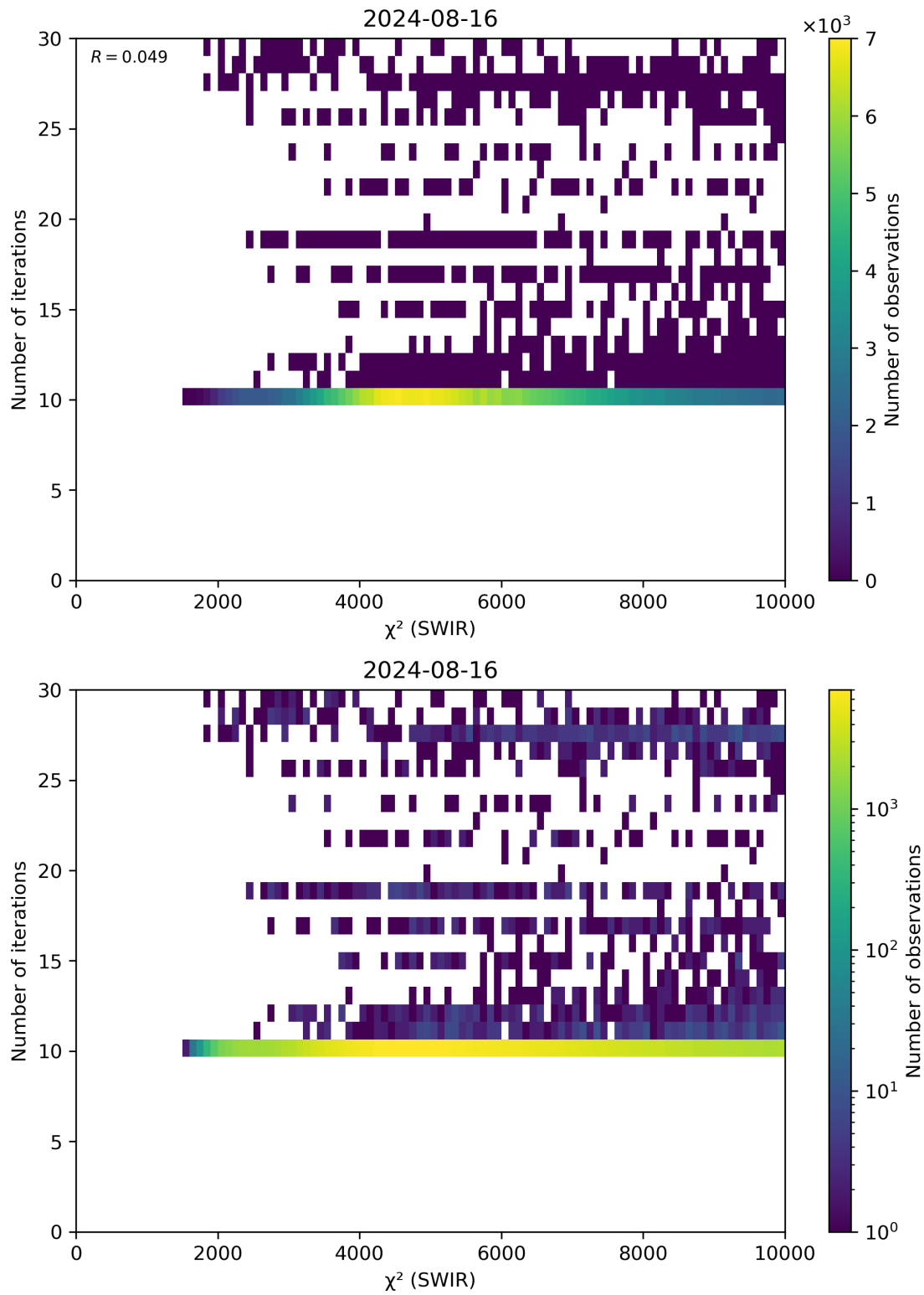
Figure 50: Scatter density plot of “ \chi^2 (SWIR)” against “Number of iterations” for 2024-08-16 to 2024-08-17.
