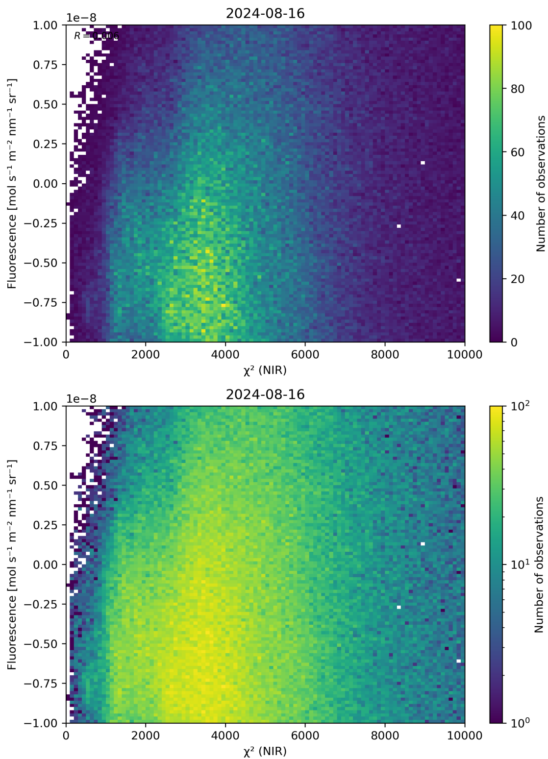
Figure 45: Scatter density plot of “ \chi^2 (NIR)” against “Fluorescence” for 2024-08-16 to 2024-08-17.
