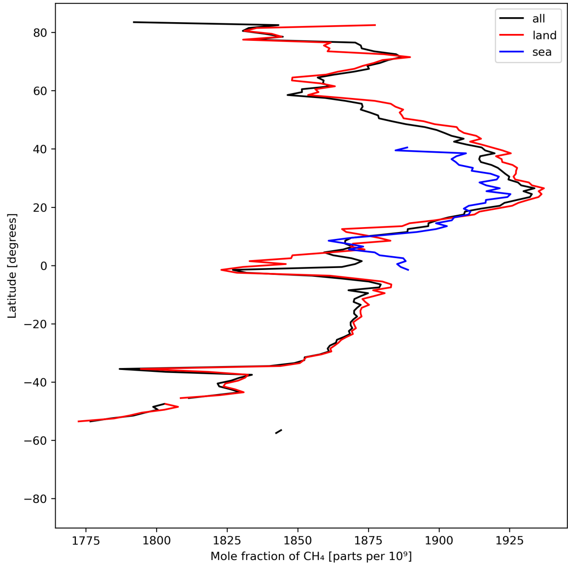
Figure 12: Zonal average of “Mole fraction of \text{CH}_4 ” for 2024-08-16 to 2024-08-17.
