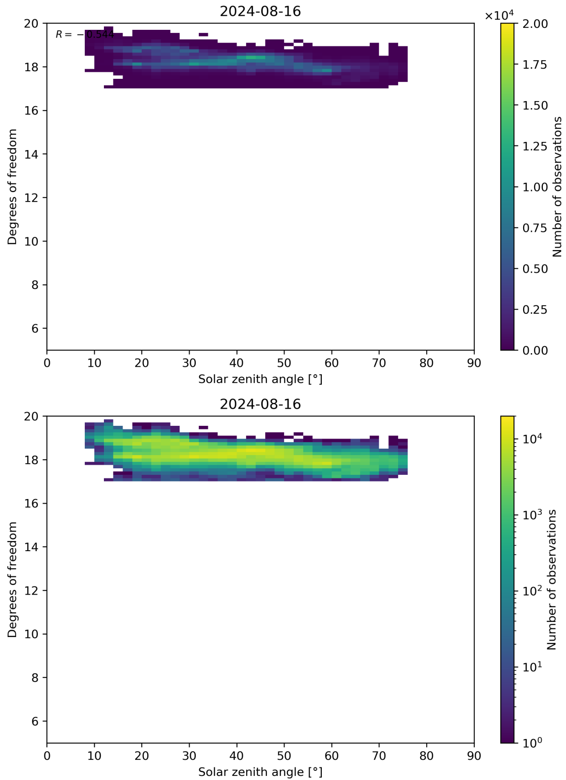
Figure 96: Scatter density plot of “Solar zenith angle” against “Degrees of freedom” for 2024-08-16 to 2024-08-17.
