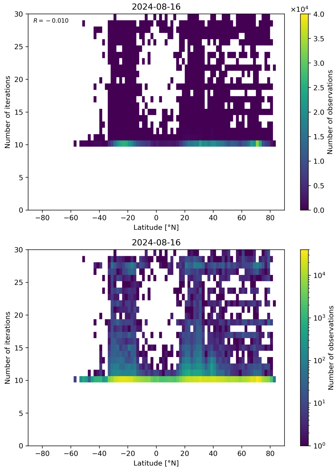
Figure 60: Scatter density plot of “Latitude” against “Number of iterations” for 2024-08-16 to 2024-08-17.
