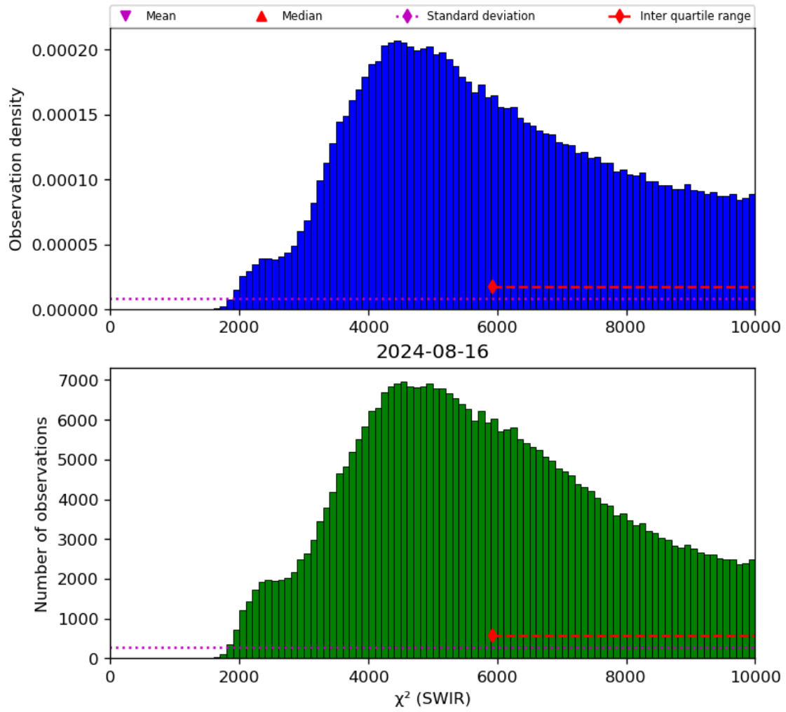
Figure 28: Histogram of “ \chi^2 (SWIR)” for 2024-08-16 to 2024-08-17
