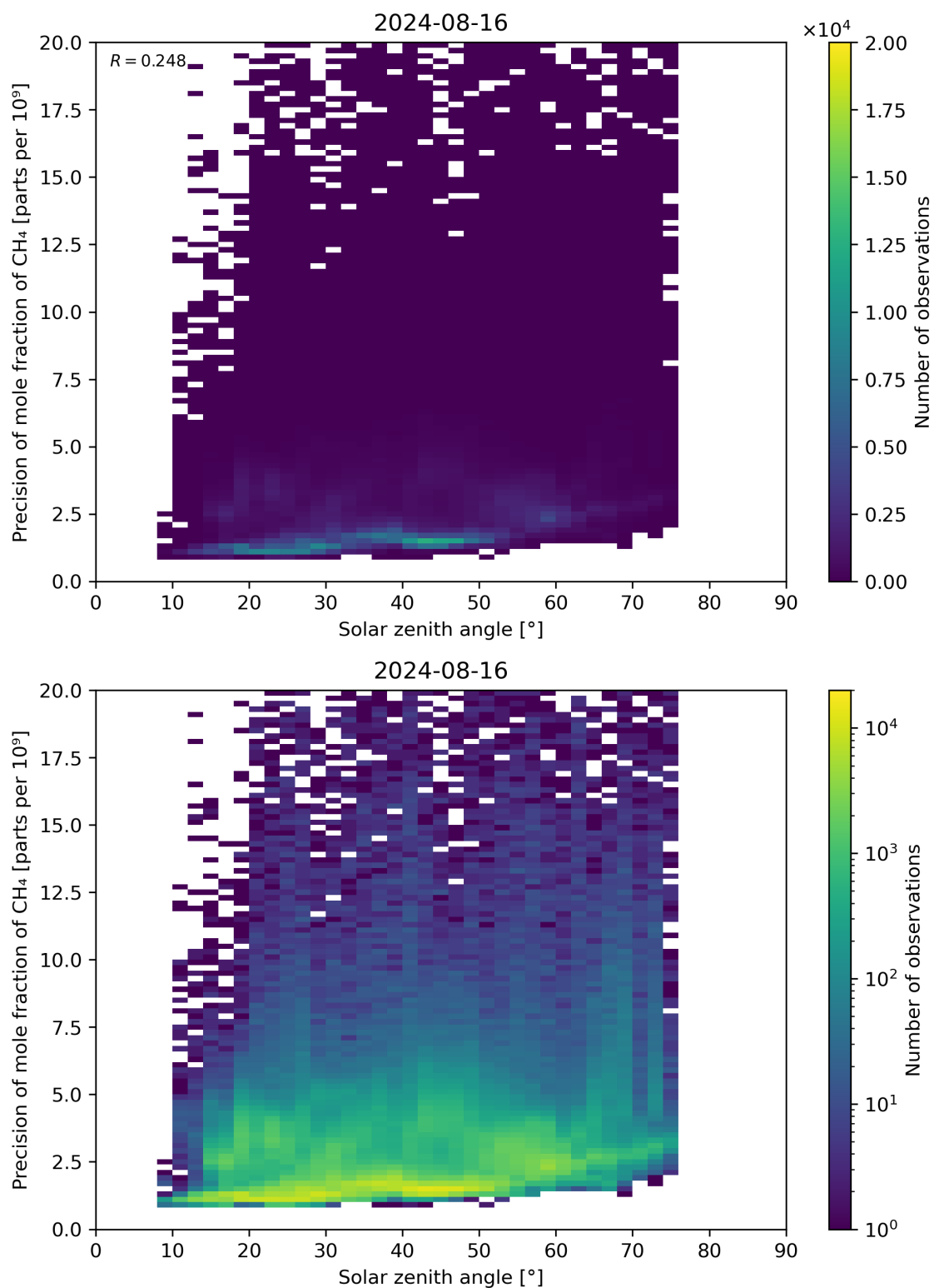
Figure 101: Scatter density plot of “Solar zenith angle” against “Precision of mole fraction of CH 4 ” for 2024-08-16 to 2024-08-17.
