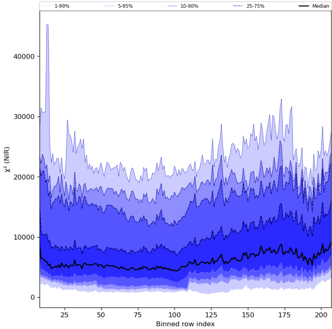
Figure 40: Along track statistics of “ \chi^2 (NIR)” for 2024-08-16 to 2024-08-17
