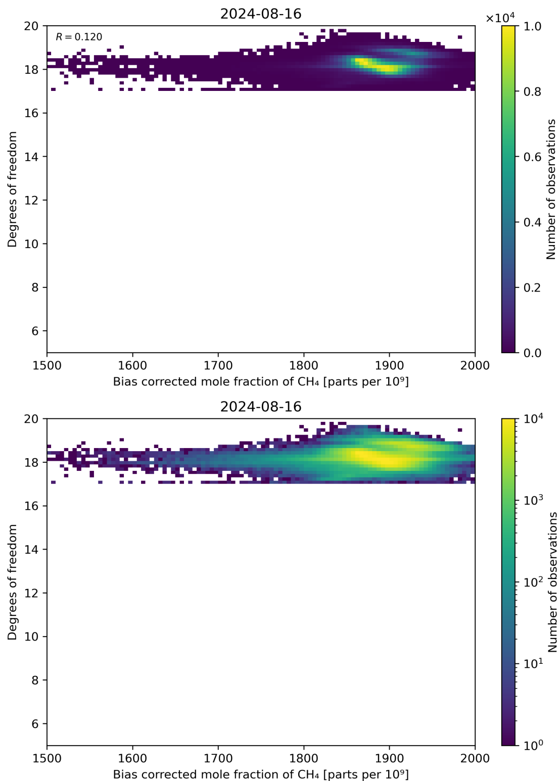
Figure 65: Scatter density plot of “Bias corrected mole fraction of CH 4 ” against “Degrees of freedom” for 2024-08-16 to 2024-08-17.
