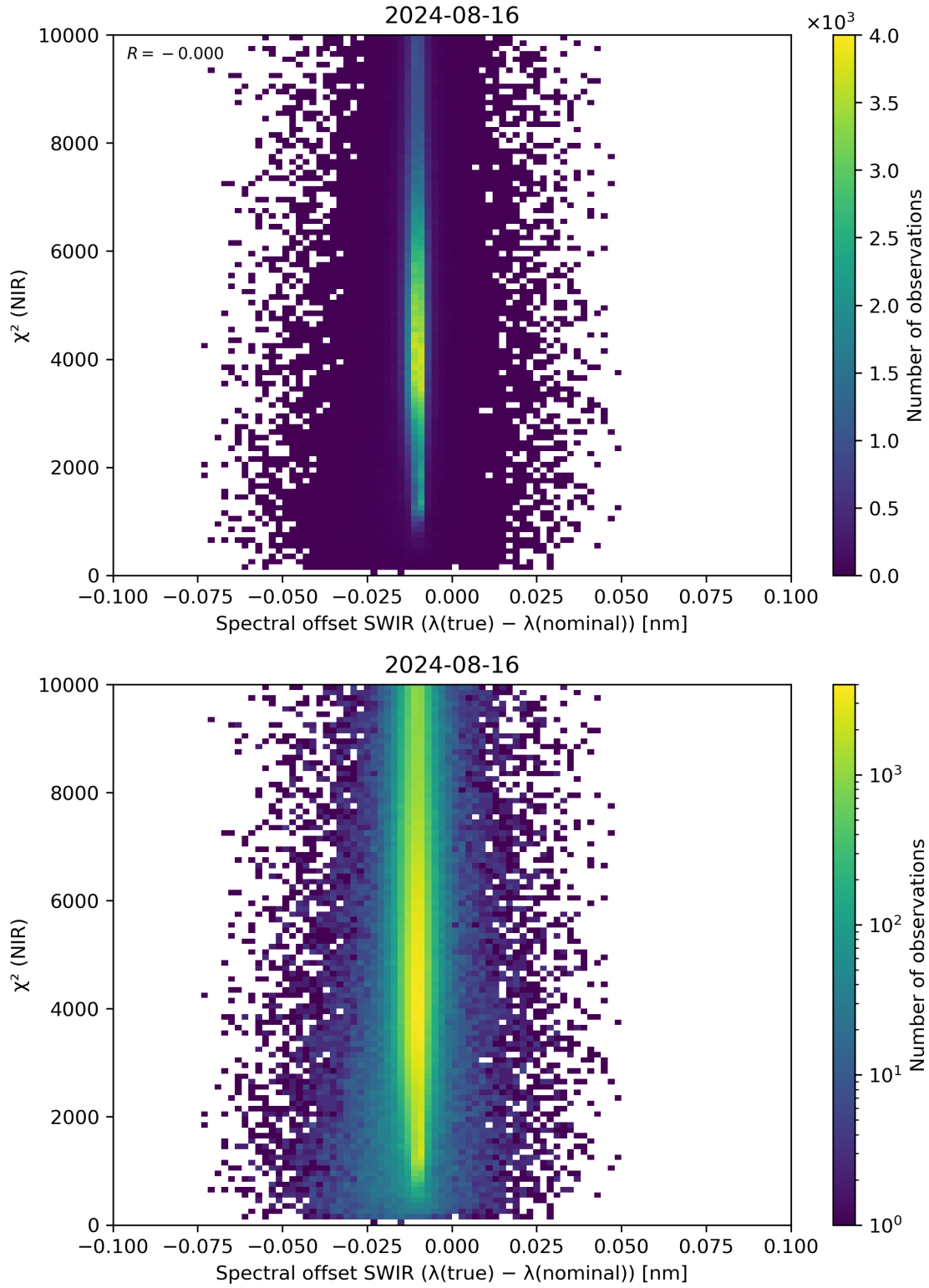
Figure 117: Scatter density plot of “Spectral offset SWIR ( \lambda(\text{true}) - \lambda(\text{nominal}) )” against “ \chi^2 (NIR)” for 2024-08-16 to 2024-08-17.
