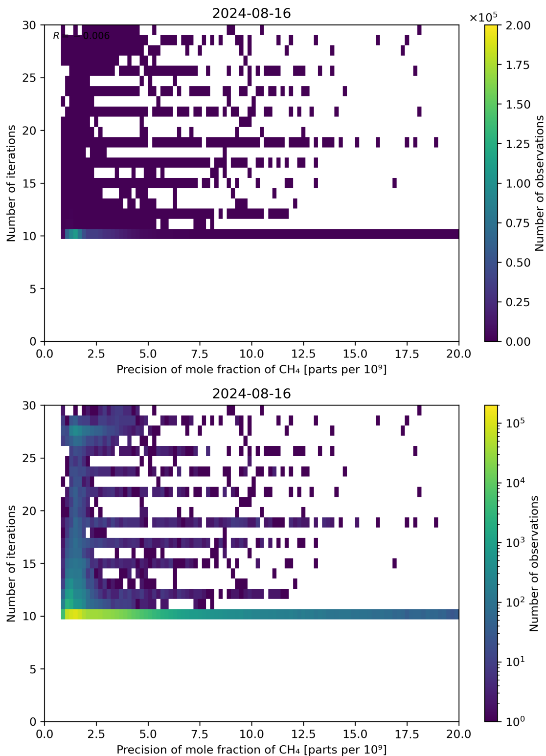
Figure 83: Scatter density plot of “Precision of mole fraction of CH 4 ” against “Number of iterations” for 2024-08-16 to 2024-08-17.
