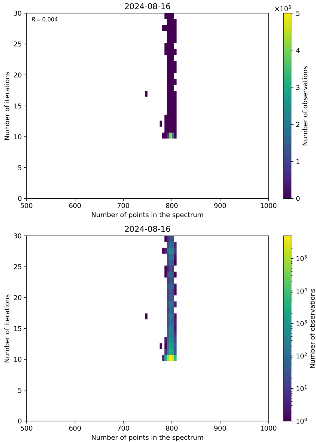
Figure 92: Scatter density plot of “Number of points in the spectrum” against “Number of iterations” for 2024-08-16 to 2024-08-17.
