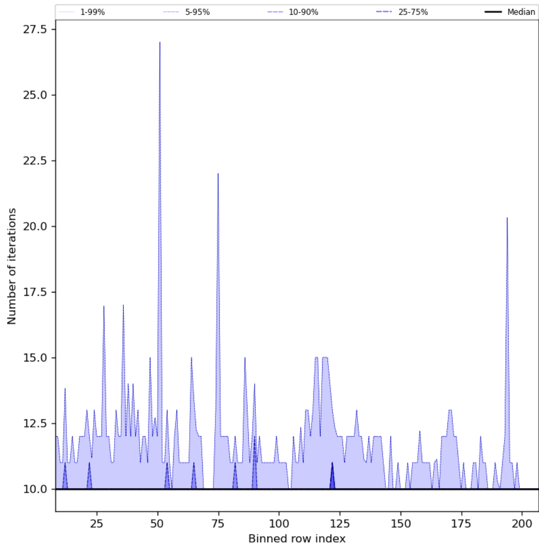
Figure 42: Along track statistics of “Number of iterations” for 2024-08-16 to 2024-08-17
