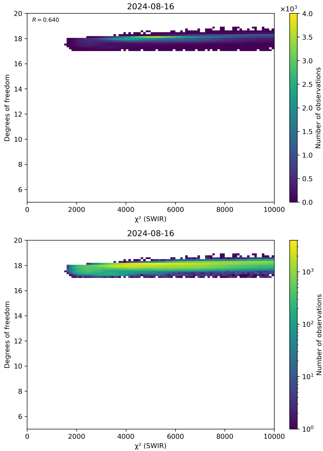
Figure 48: Scatter density plot of “ \chi^2 (SWIR)” against “Degrees of freedom” for 2024-08-16 to 2024-08-17.
