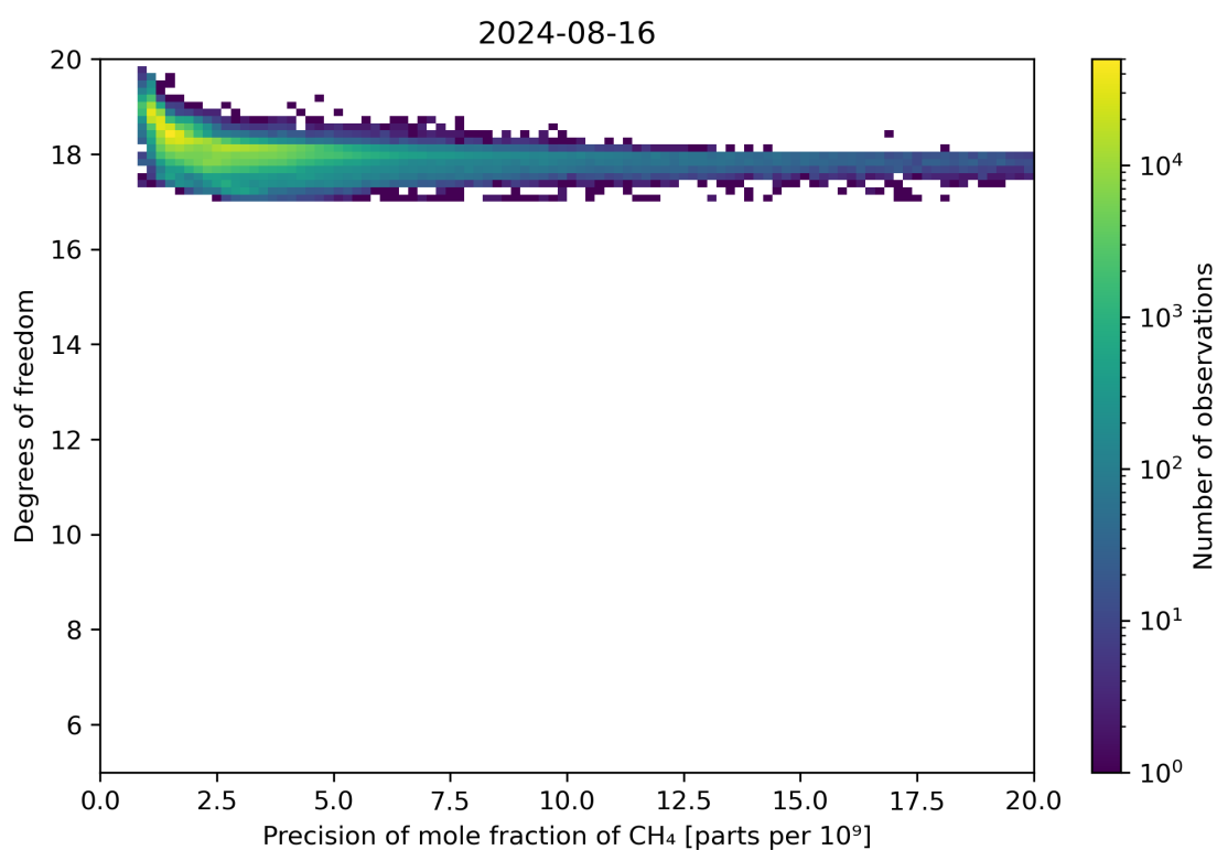
Figure 80: Scatter density plot of “Precision of mole fraction of CH 4 ” against “Degrees of freedom” for 2024-08-16 to 2024-08-17.
