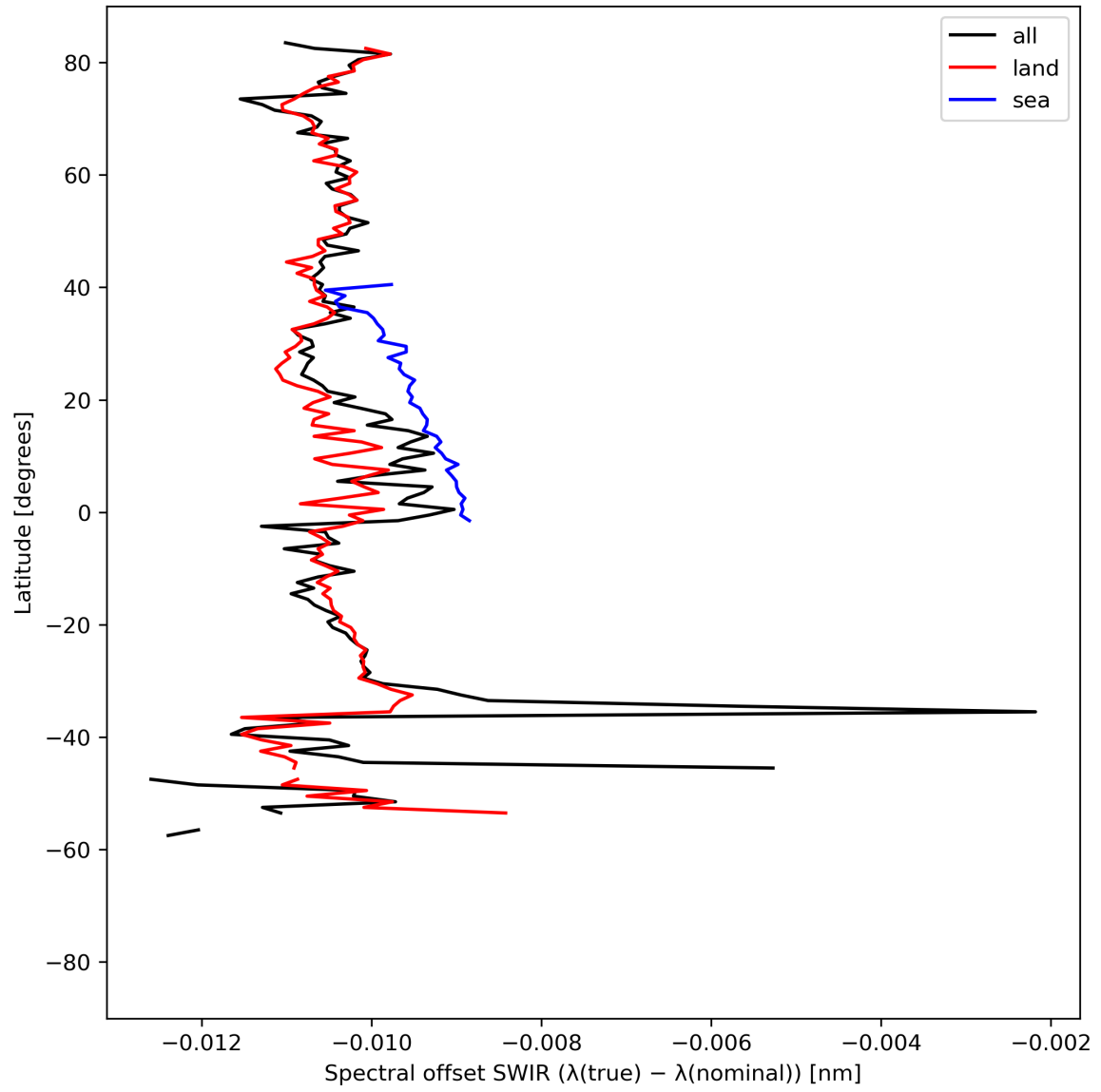
Figure 16: Zonal average of “Spectral offset SWIR ( \lambda(\text{true}) - \lambda(\text{nominal}) )” for 2024-08-16 to 2024-08-17.
