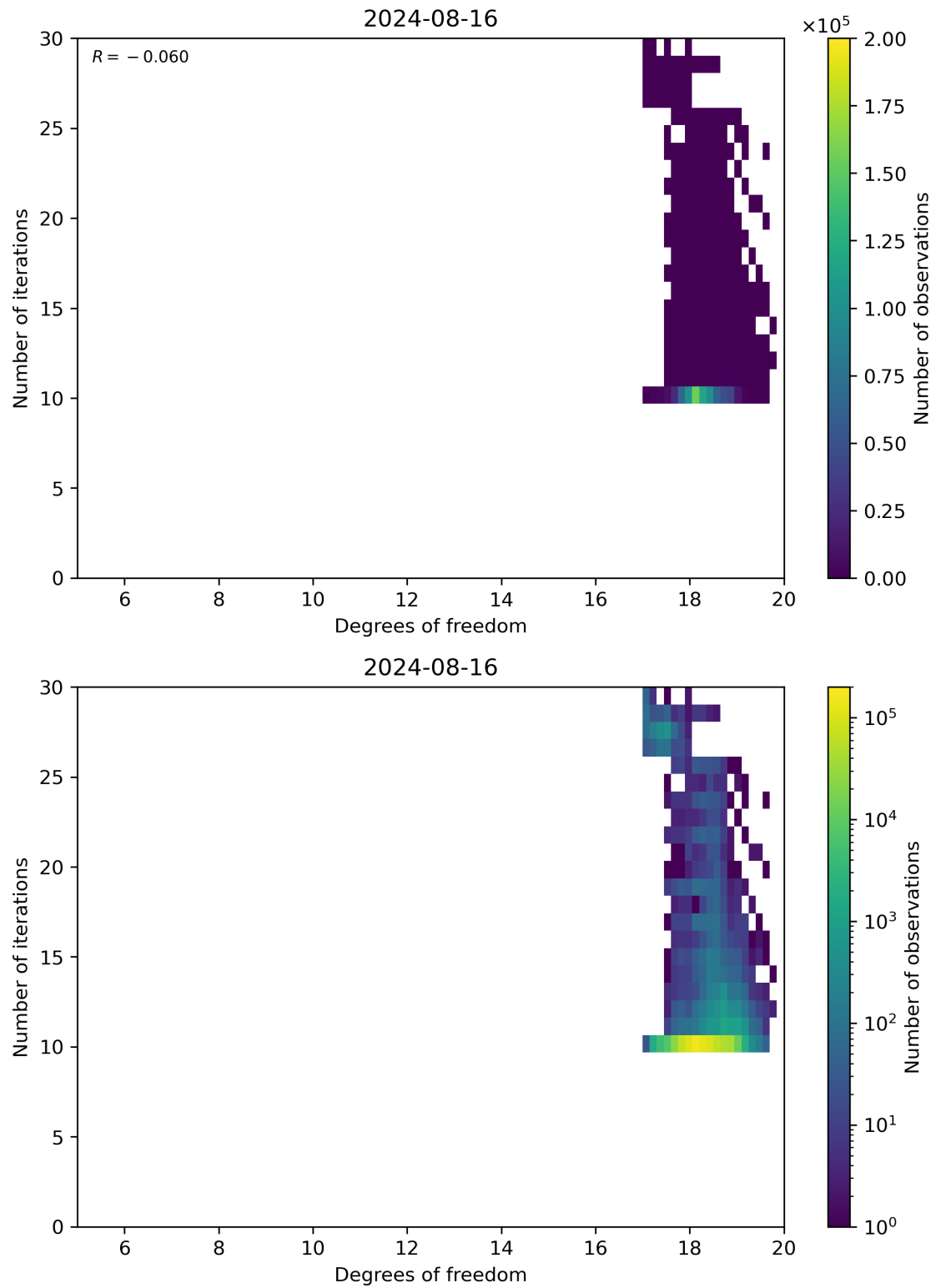
Figure 52: Scatter density plot of “Degrees of freedom” against “Number of iterations” for 2024-08-16 to 2024-08-17.
