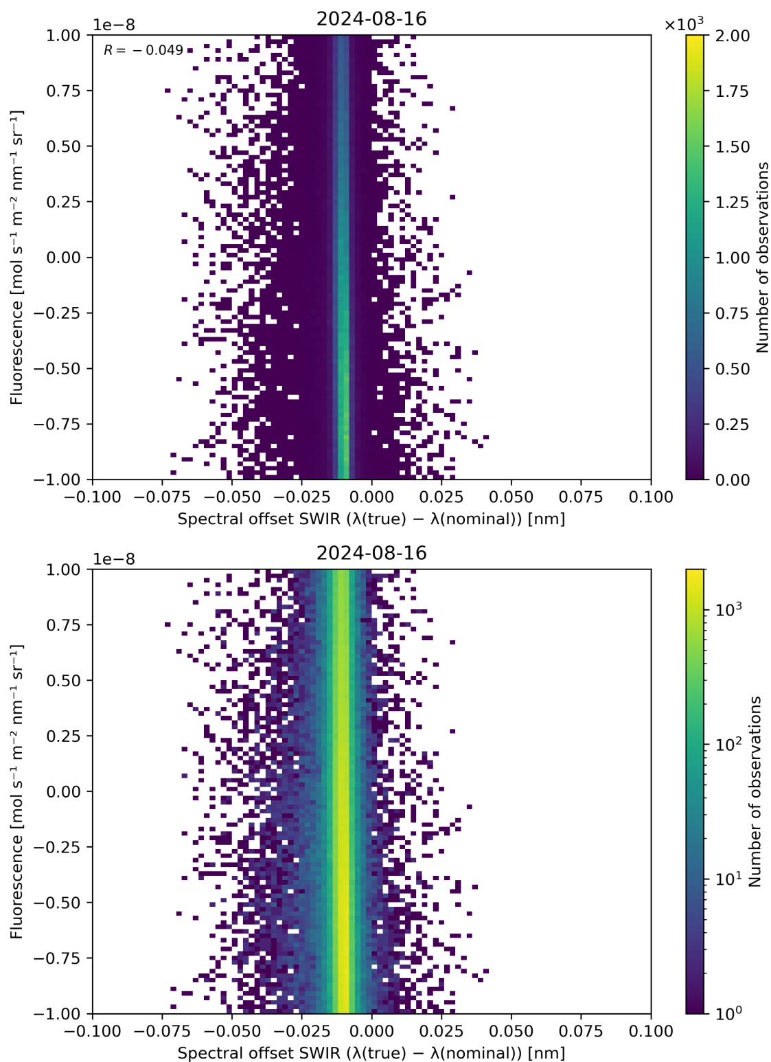
Figure 120: Scatter density plot of “Spectral offset SWIR ( \lambda(\text{true}) - \lambda(\text{nominal}) )” against “Fluorescence” for 2024-08-16 to 2024-08-17.
