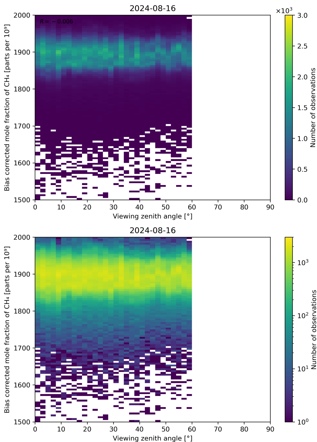
Figure 111: Scatter density plot of “Viewing zenith angle” against “Bias corrected mole fraction of CH 4 ” for 2024-08-16 to 2024-08-17.
