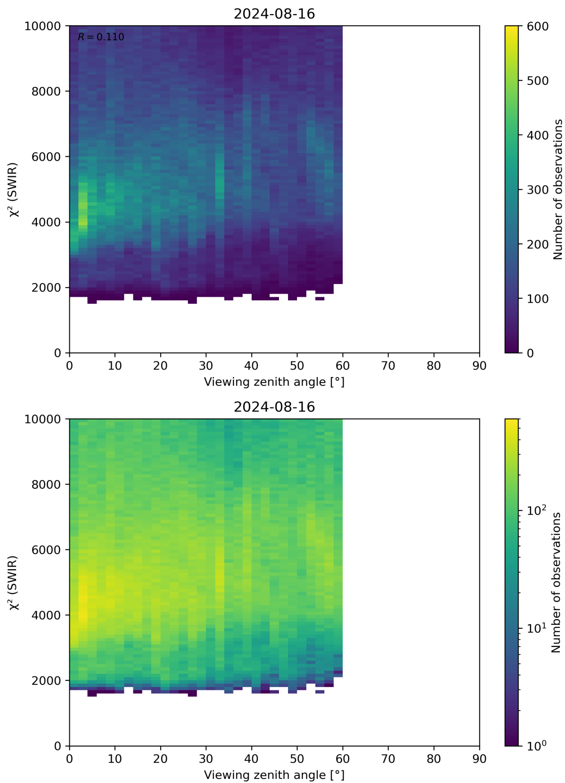
Figure 106: Scatter density plot of “Viewing zenith angle” against “ \chi^2 (SWIR)” for 2024-08-16 to 2024-08-17.
