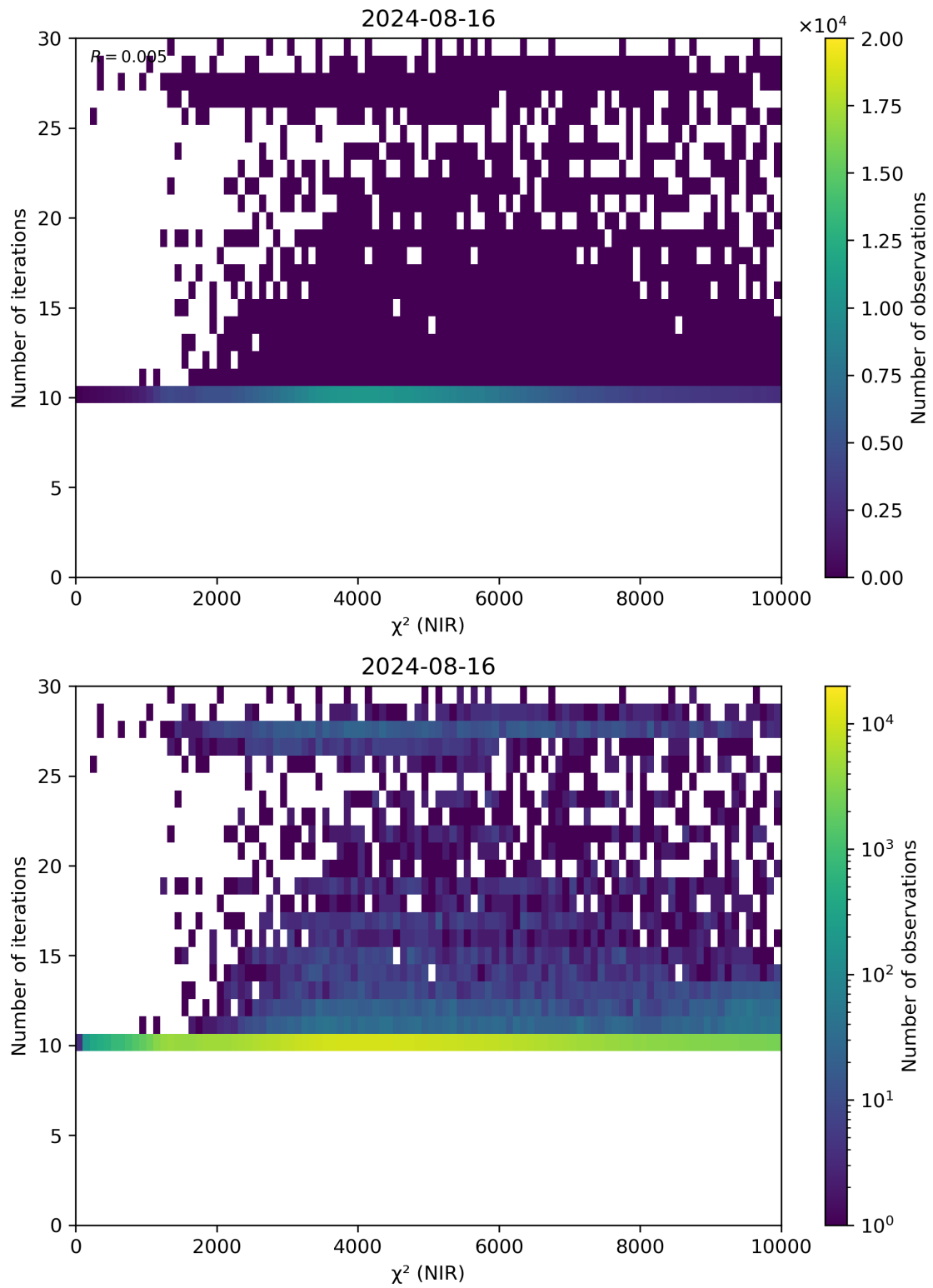
Figure 46: Scatter density plot of “ \chi^2 (NIR)” against “Number of iterations” for 2024-08-16 to 2024-08-17.
