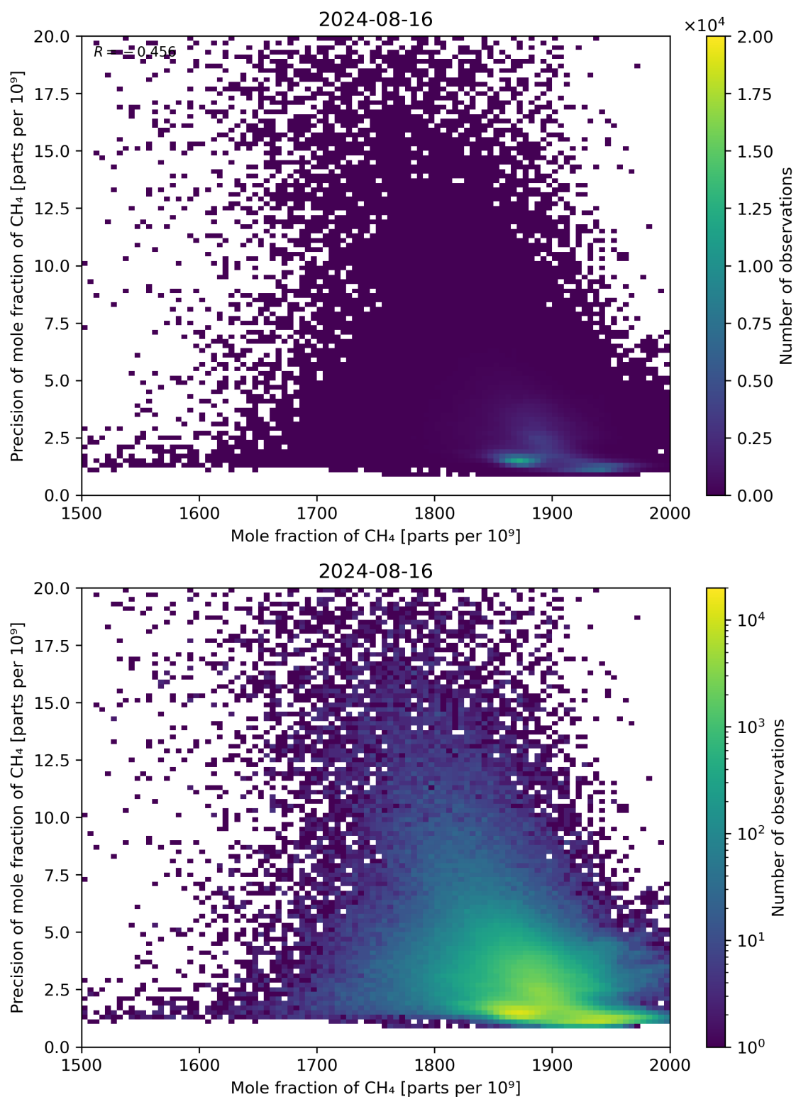
Figure 75: Scatter density plot of “Mole fraction of CH 4 ” against “Precision of mole fraction of CH 4 ” for 2024-08-16 to 2024-08-17.
