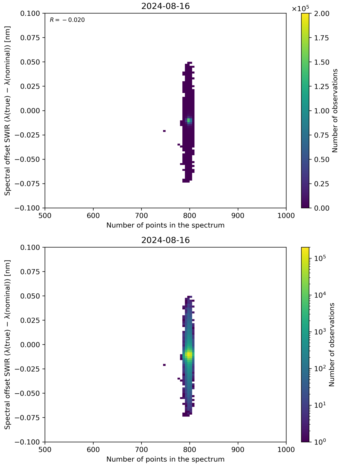
Figure 93: Scatter density plot of “Number of points in the spectrum” against “Spectral offset SWIR ( \lambda(\text{true}) - \lambda(\text{nominal}) )” for 2024-08-16 to 2024-08-17.
