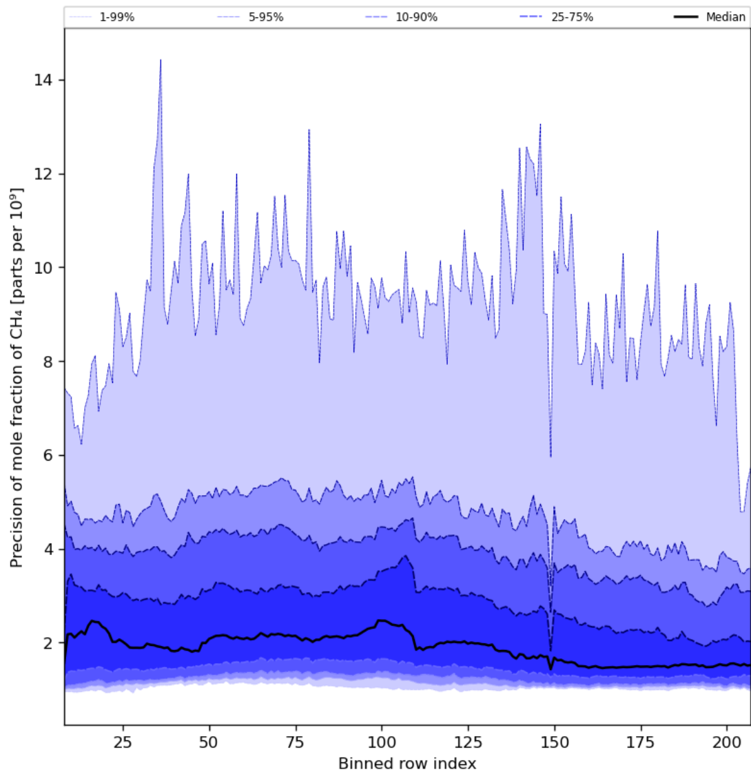
Figure 35: Along track statistics of “Precision of mole fraction of CH 4 ” for 2024-08-16 to 2024-08-17
