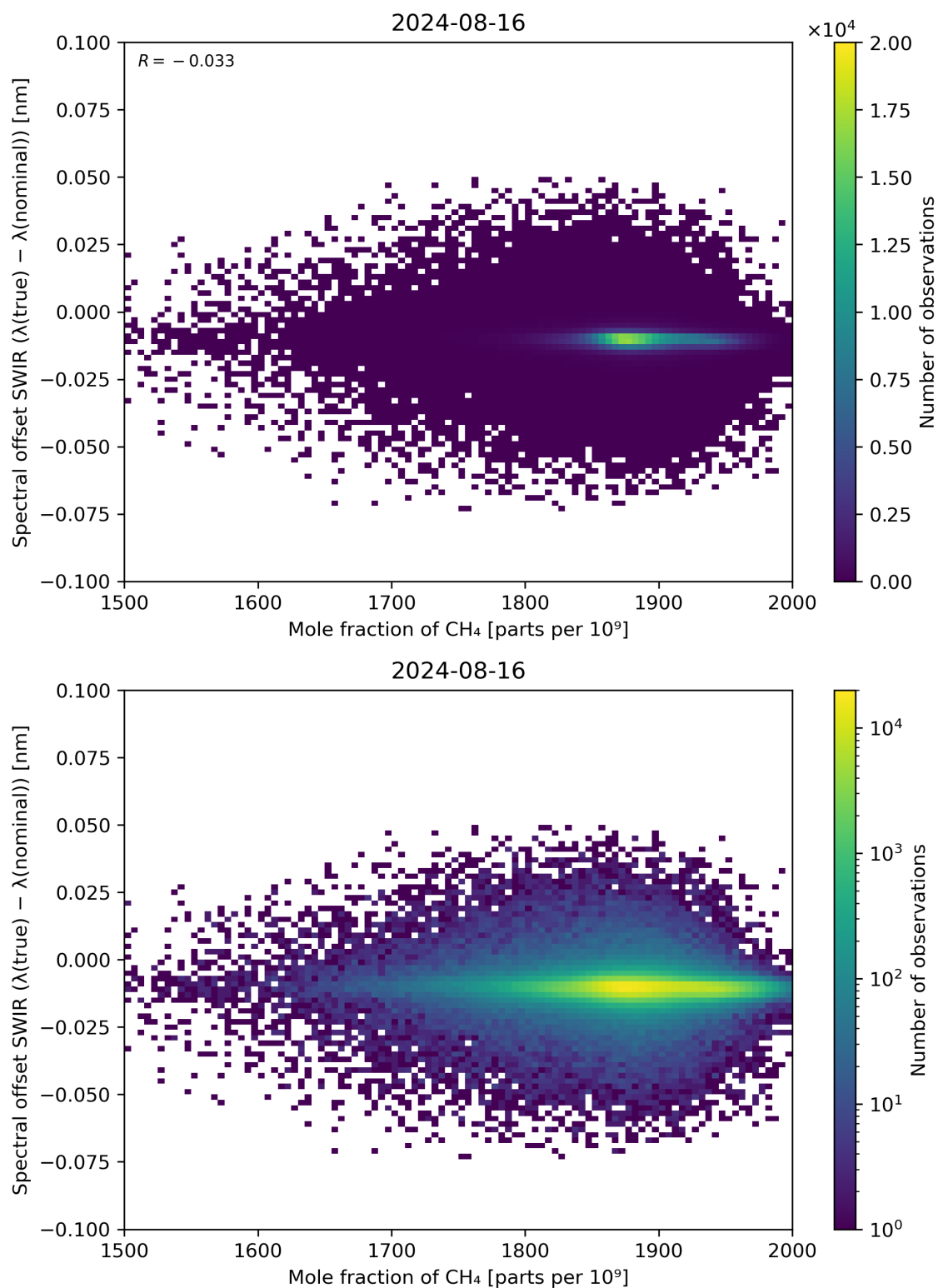
Figure 86: Scatter density plot of “Mole fraction of CH 4 ” against “Spectral offset SWIR ( \lambda(\text{true}) - \lambda(\text{nominal}) )” for 2024-08-16 to 2024-08-17.
