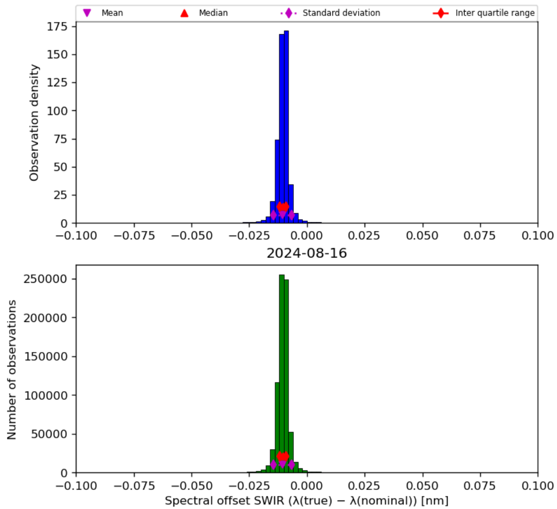
Figure 27: Histogram of “Spectral offset SWIR ( \lambda(\text{true}) - \lambda(\text{nominal}) )” for 2024-08-16 to 2024-08-17
