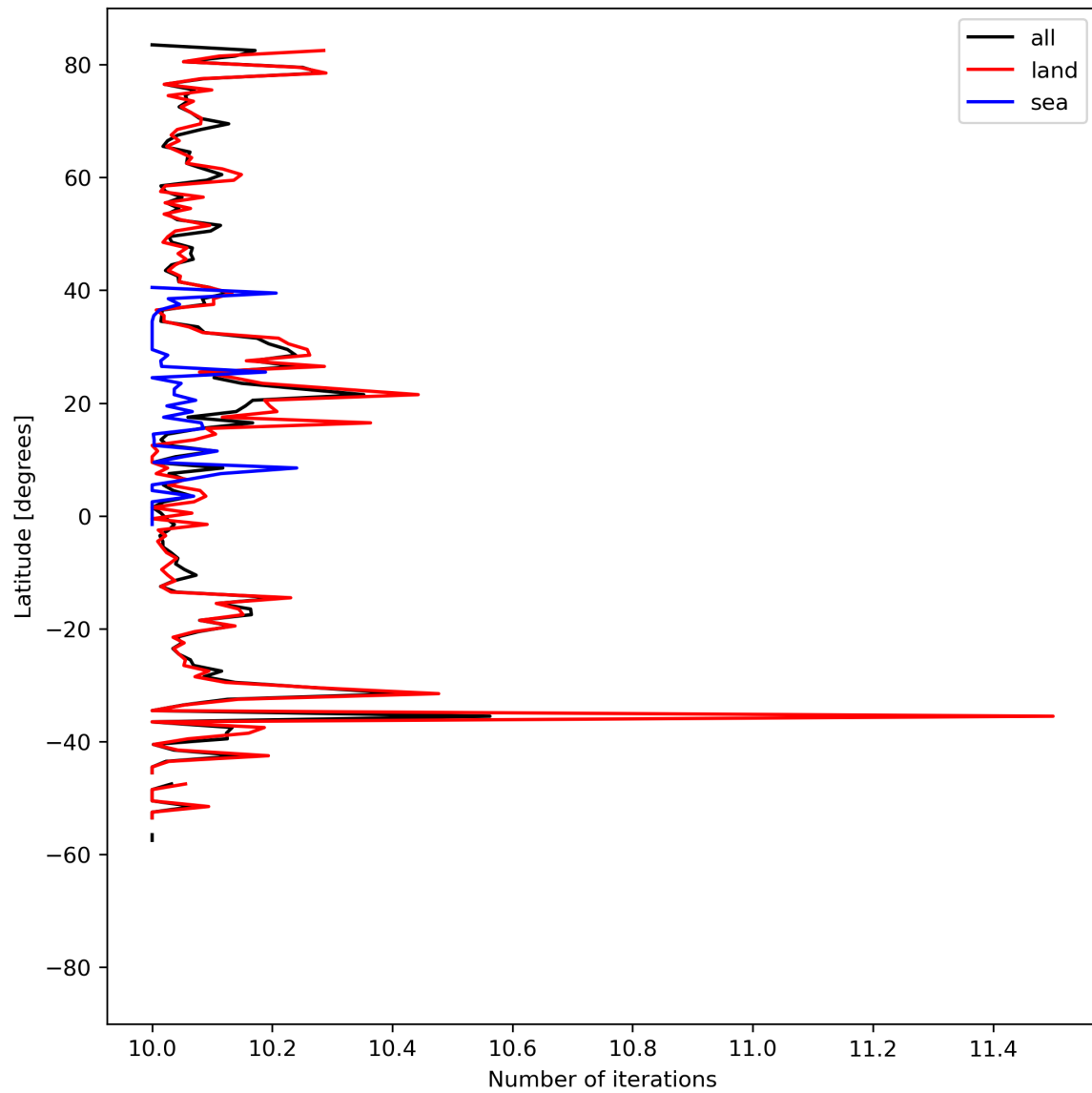
Figure 20: Zonal average of “Number of iterations” for 2024-08-16 to 2024-08-17.
