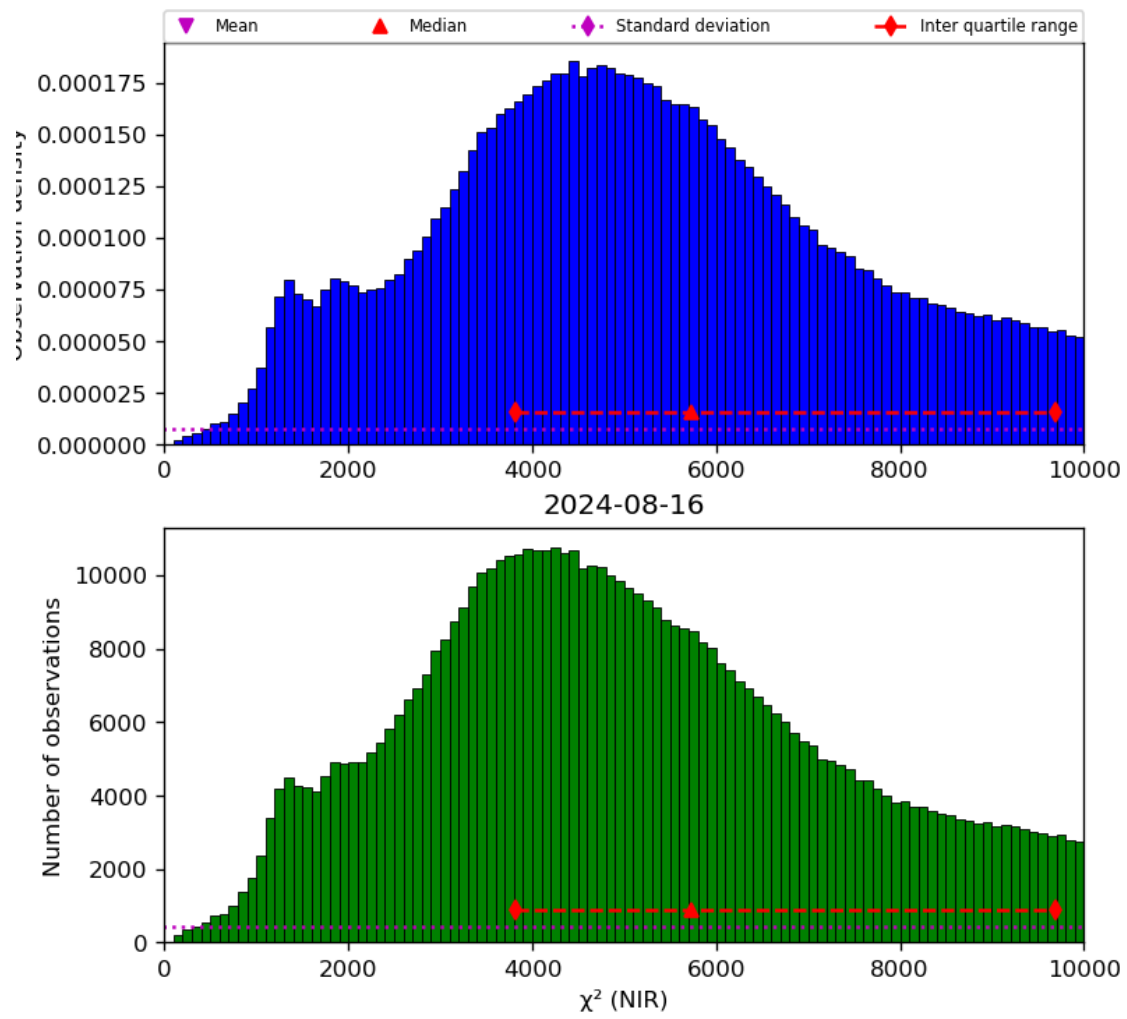
Figure 29: Histogram of " \chi^2 (NIR)" for 2024-08-16 to 2024-08-17
