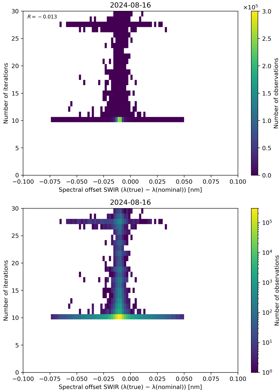
Figure 121: Scatter density plot of “Spectral offset SWIR ( \lambda(\text{true}) - \lambda(\text{nominal}) )” against “Number of iterations” for 2024-08-16 to 2024-08-17.
