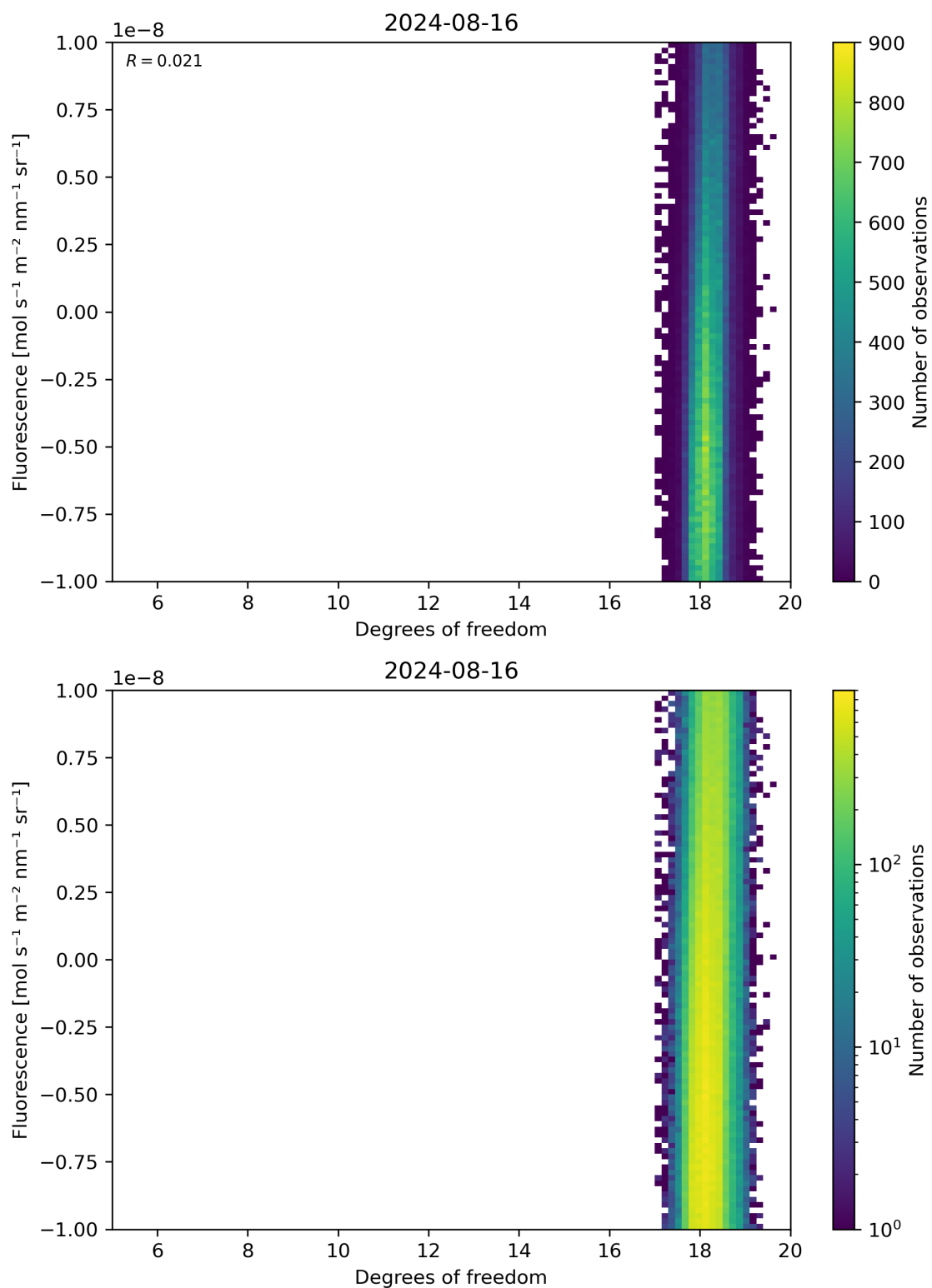
Figure 51: Scatter density plot of “Degrees of freedom” against “Fluorescence” for 2024-08-16 to 2024-08-17.
