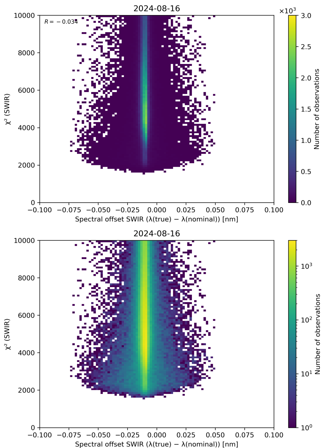
Figure 118: Scatter density plot of “Spectral offset SWIR ( \lambda(\text{true}) - \lambda(\text{nominal}) )” against “ \chi^2 (SWIR)” for 2024-08-16 to 2024-08-17.
