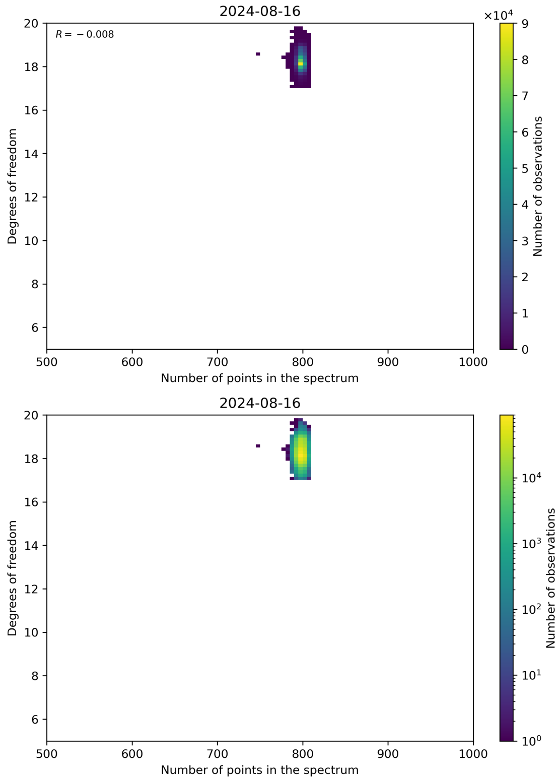
Figure 90: Scatter density plot of “Number of points in the spectrum” against “Degrees of freedom” for 2024-08-16 to 2024-08-17.
