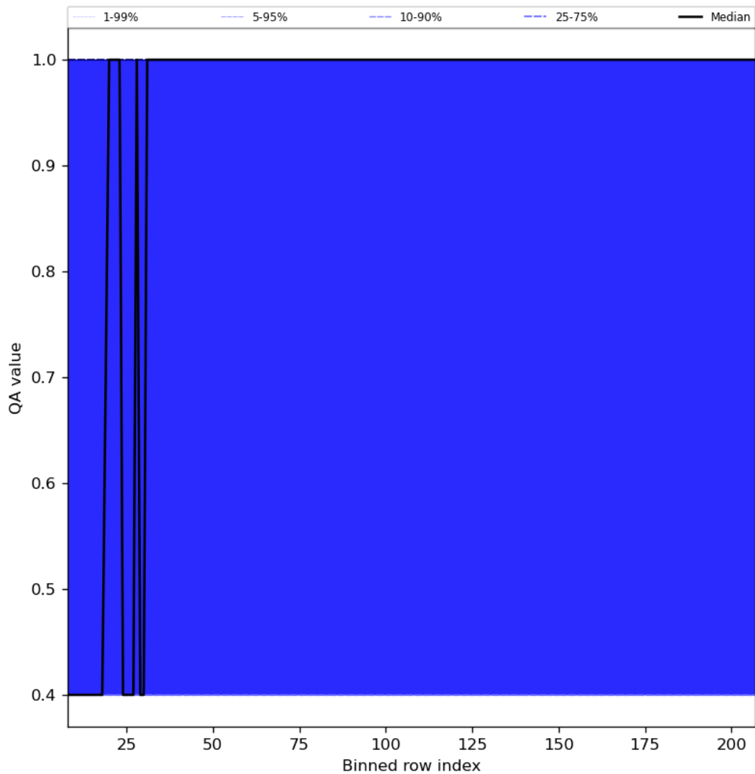
Figure 33: Along track statistics of “QA value” for 2024-08-16 to 2024-08-17
