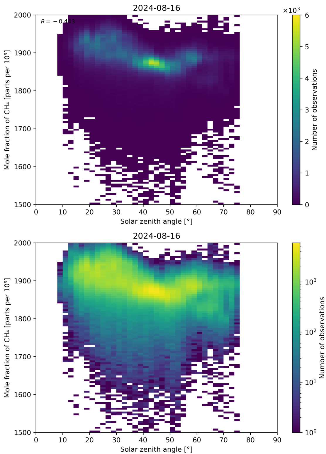
Figure 99: Scatter density plot of “Solar zenith angle” against “Mole fraction of CH 4 ” for 2024-08-16 to 2024-08-17.
