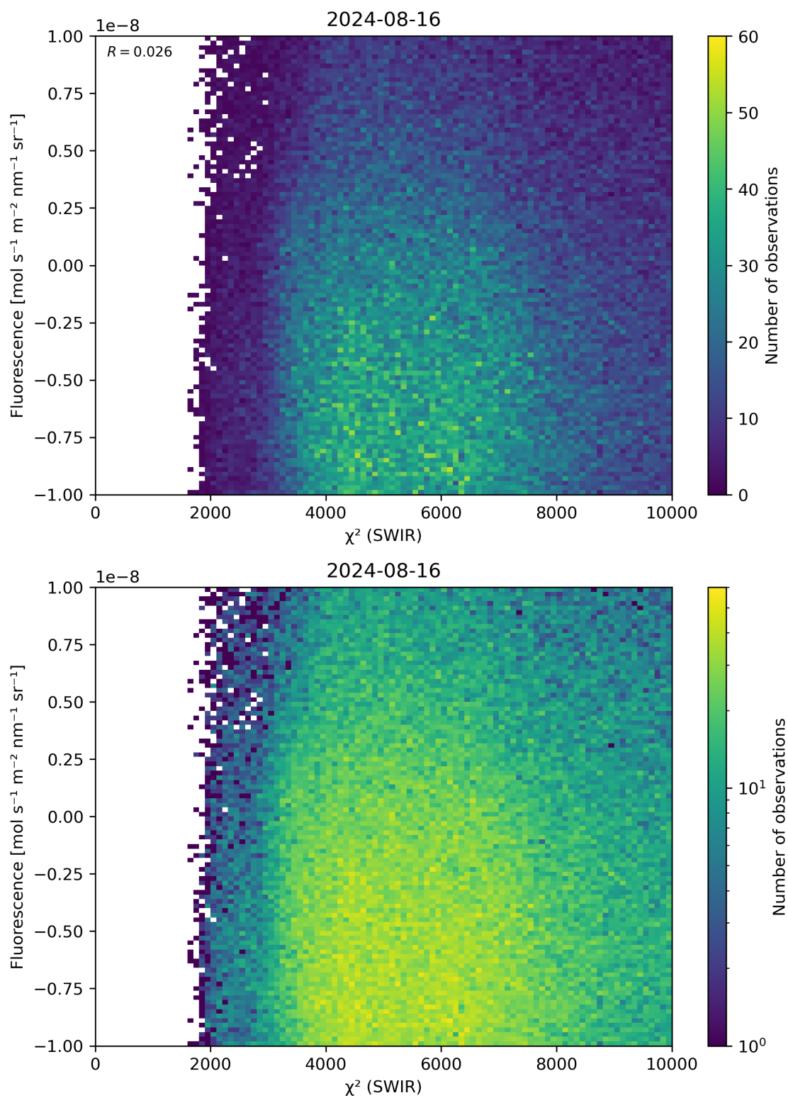
Figure 49: Scatter density plot of “ \chi^2 (SWIR)” against “Fluorescence” for 2024-08-16 to 2024-08-17.
