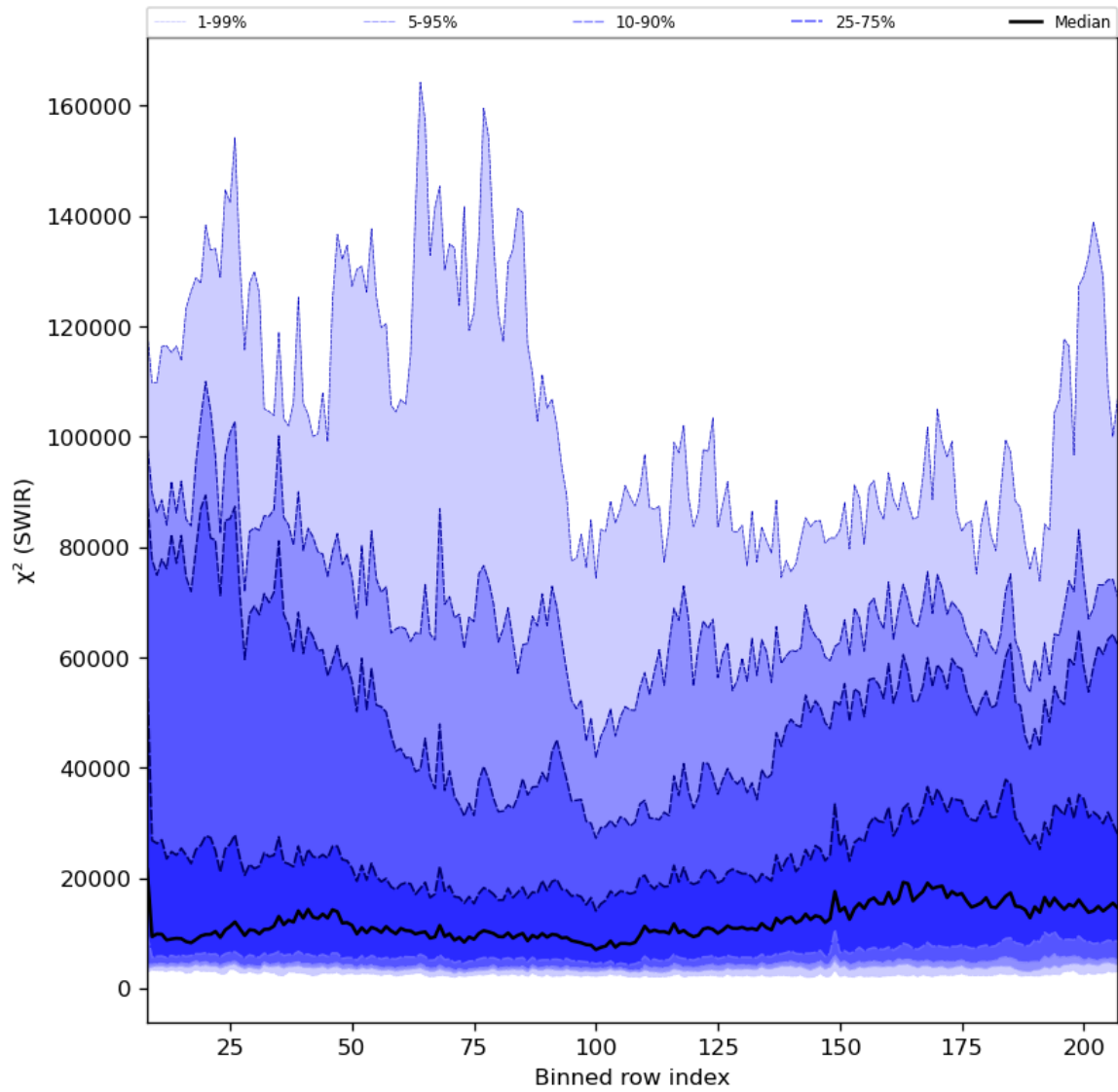
Figure 39: Along track statistics of “ \chi^2 (SWIR)” for 2024-08-16 to 2024-08-17
