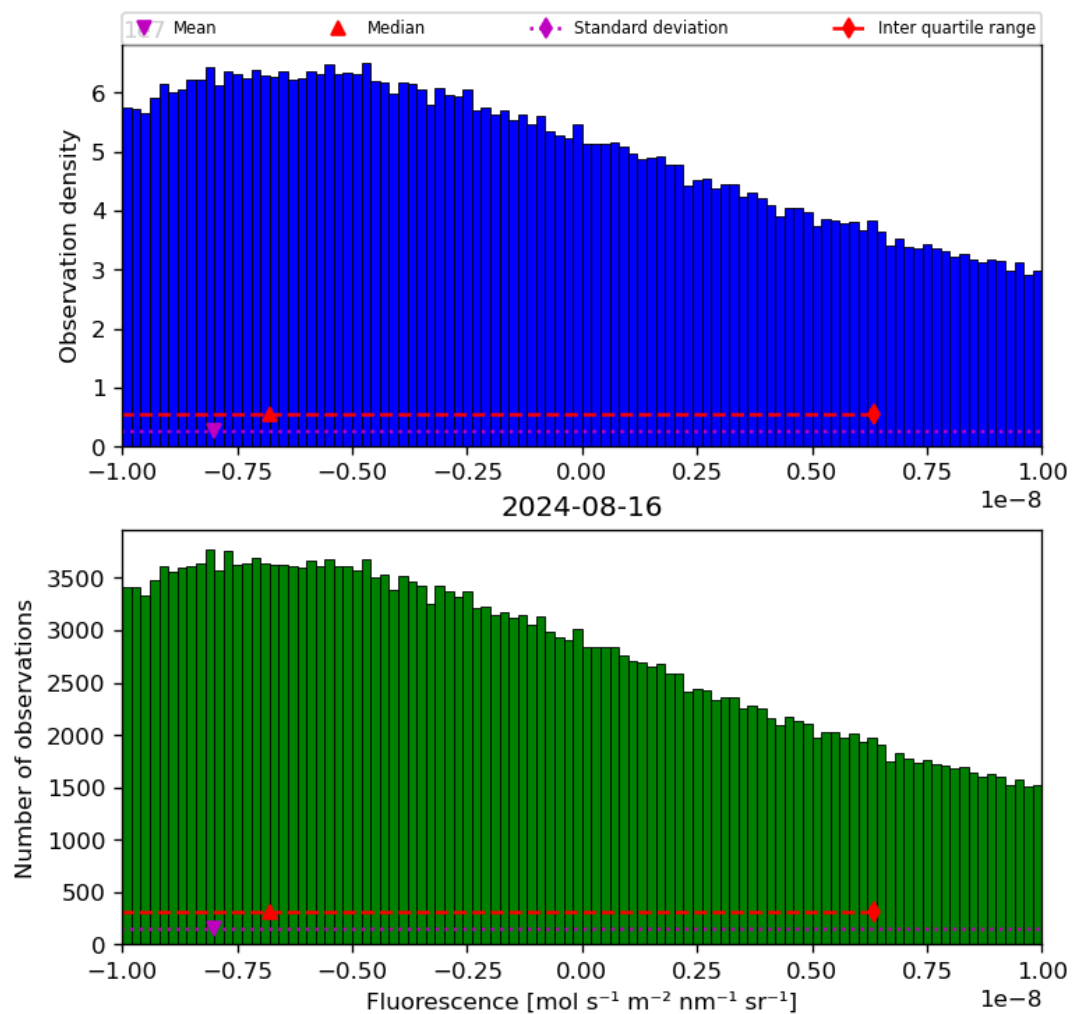
Figure 32: Histogram of “Fluorescence” for 2024-08-16 to 2024-08-17
