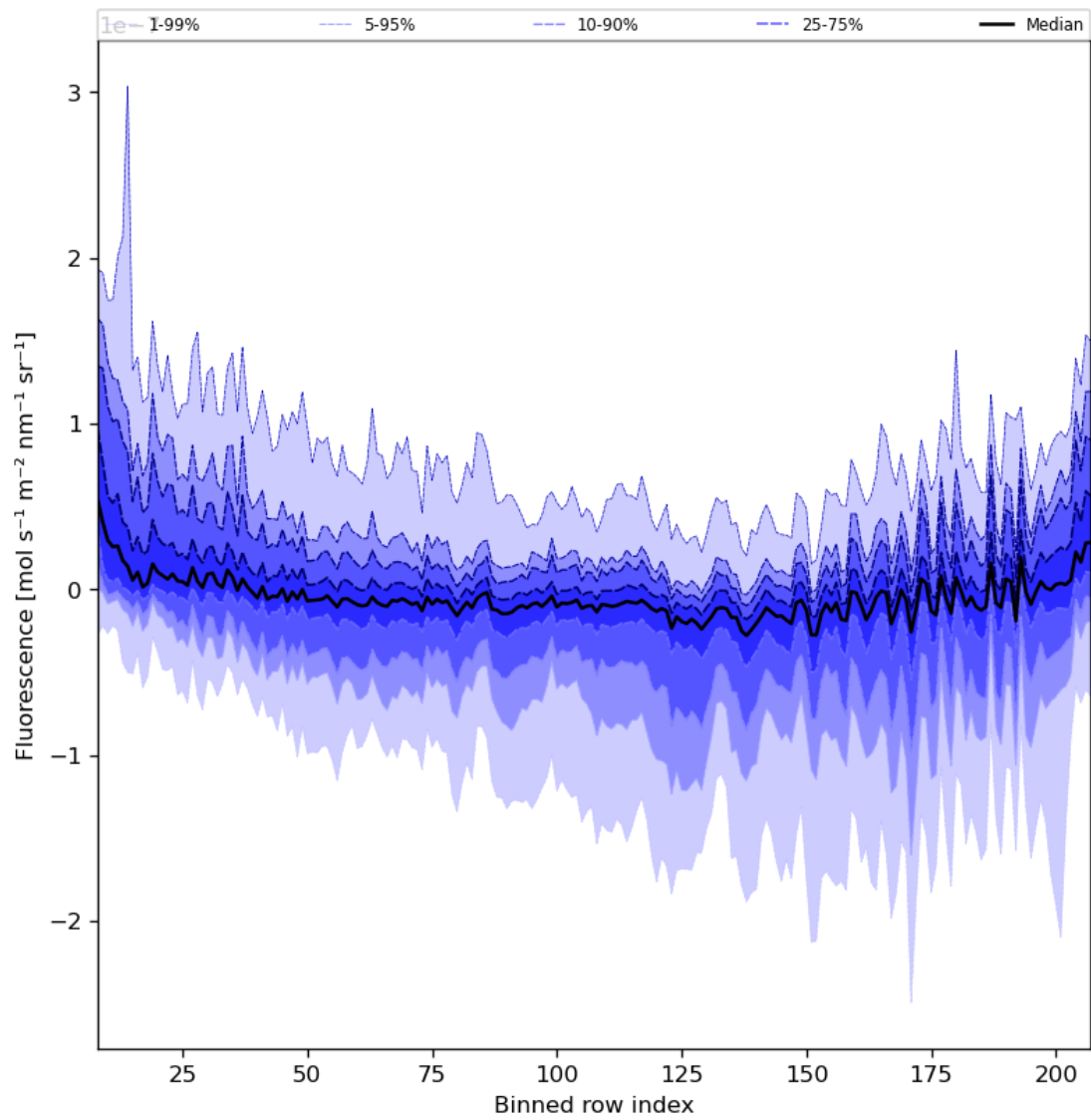
Figure 43: Along track statistics of “Fluorescence” for 2024-08-16 to 2024-08-17
