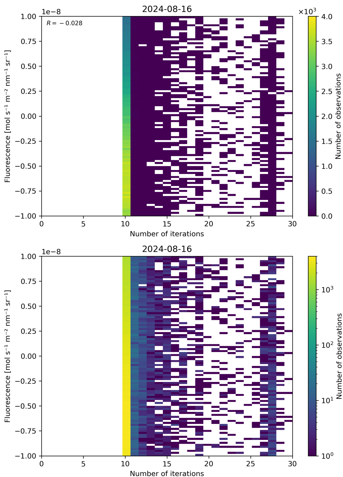
Figure 87: Scatter density plot of “Number of iterations” against “Fluorescence” for 2024-08-16 to 2024-08-17.
