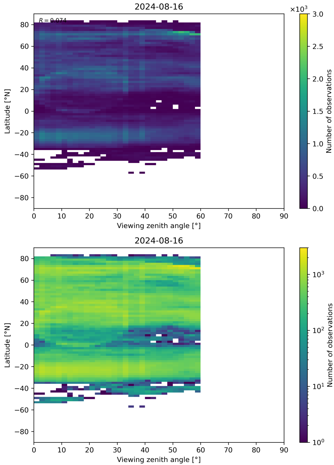
Figure 109: Scatter density plot of “Viewing zenith angle” against “Latitude” for 2024-08-16 to 2024-08-17.
