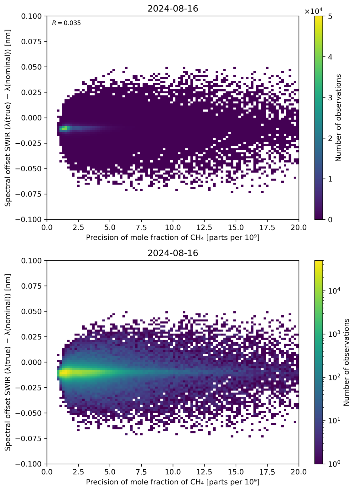
Figure 85: Scatter density plot of “Precision of mole fraction of \text{CH}_4 ” against “Spectral offset SWIR ( \lambda(\text{true}) - \lambda(\text{nominal}) )” for 2024-08-16 to 2024-08-17.
