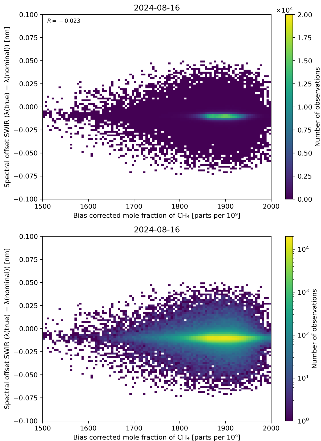
Figure 69: Scatter density plot of “Bias corrected mole fraction of \text{CH}_4 ” against “Spectral offset SWIR ( \lambda(\text{true}) - \lambda(\text{nominal}) )” for 2024-08-16 to 2024-08-17.
