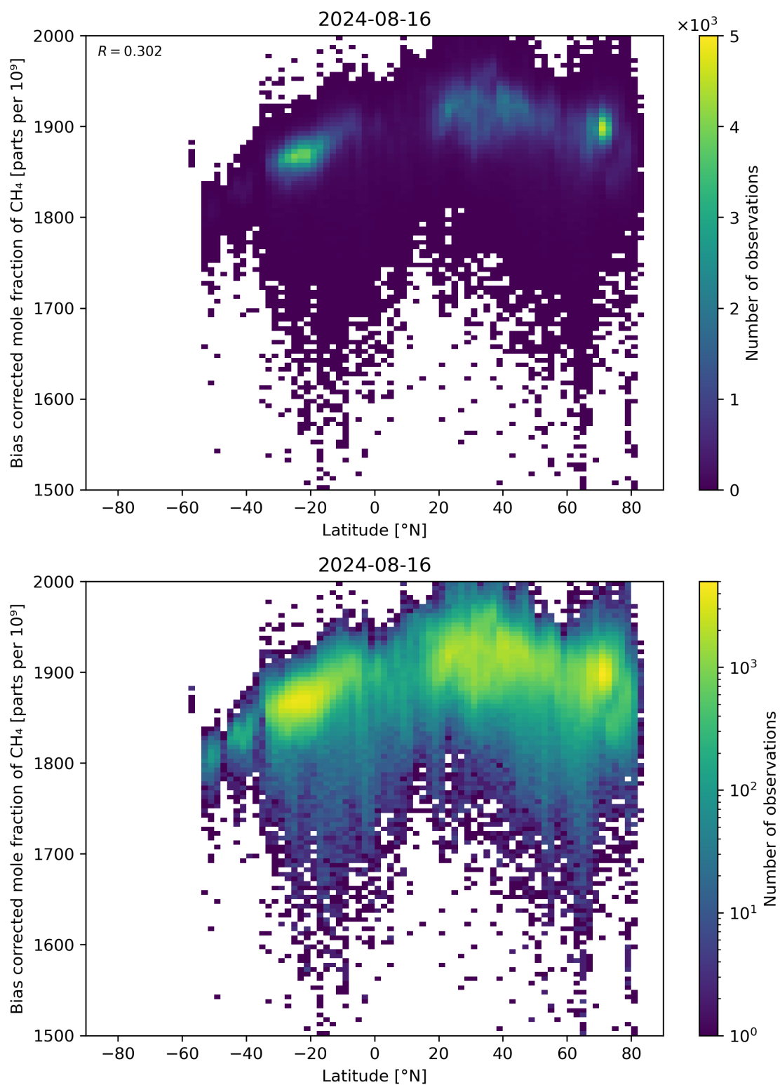
Figure 58: Scatter density plot of “Latitude” against “Bias corrected mole fraction of \text{CH}_4 ” for 2024-08-16 to 2024-08-17.
