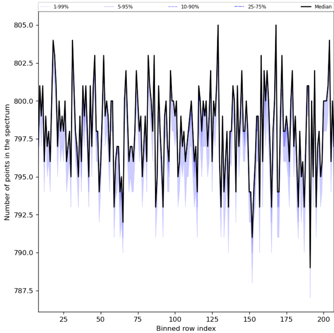
Figure 37: Along track statistics of “Number of points in the spectrum” for 2024-08-16 to 2024-08-17
