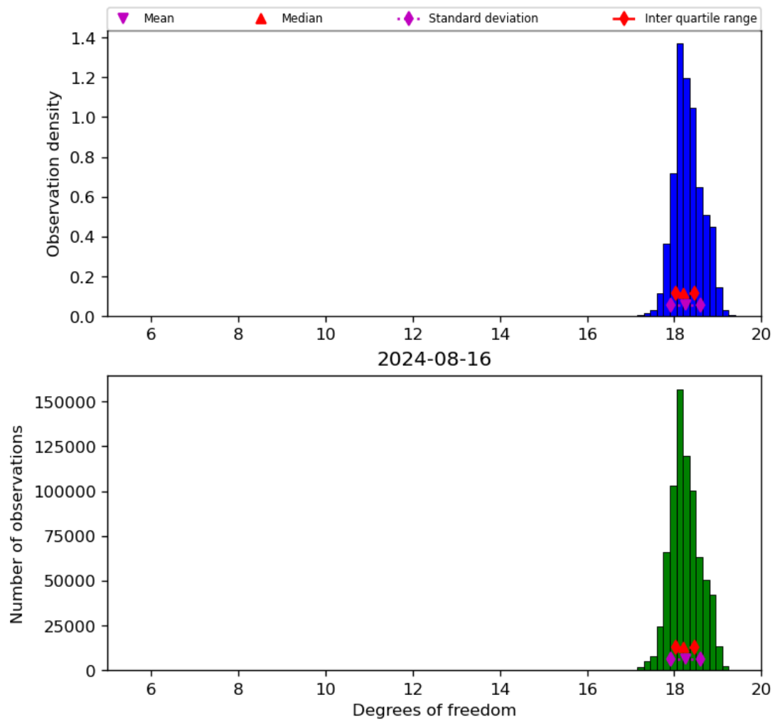
Figure 30: Histogram of “Degrees of freedom” for 2024-08-16 to 2024-08-17
