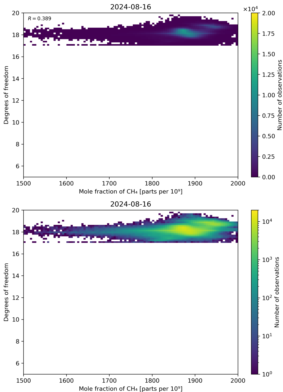
Figure 72: Scatter density plot of “Mole fraction of CH 4 ” against “Degrees of freedom” for 2024-08-16 to 2024-08-17.
