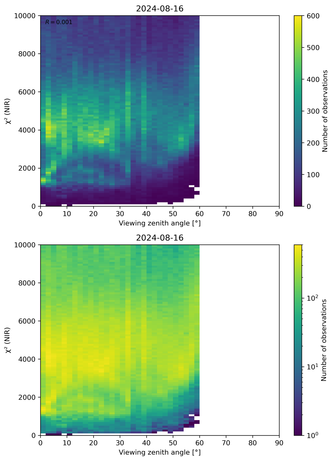
Figure 105: Scatter density plot of “Viewing zenith angle” against “ \chi^2 (NIR)” for 2024-08-16 to 2024-08-17.
