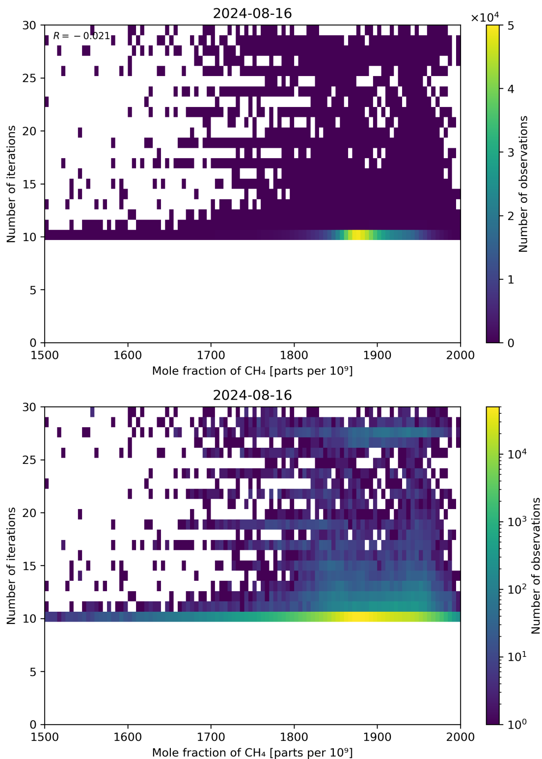
Figure 76: Scatter density plot of “Mole fraction of CH 4 ” against “Number of iterations” for 2024-08-16 to 2024-08-17.
