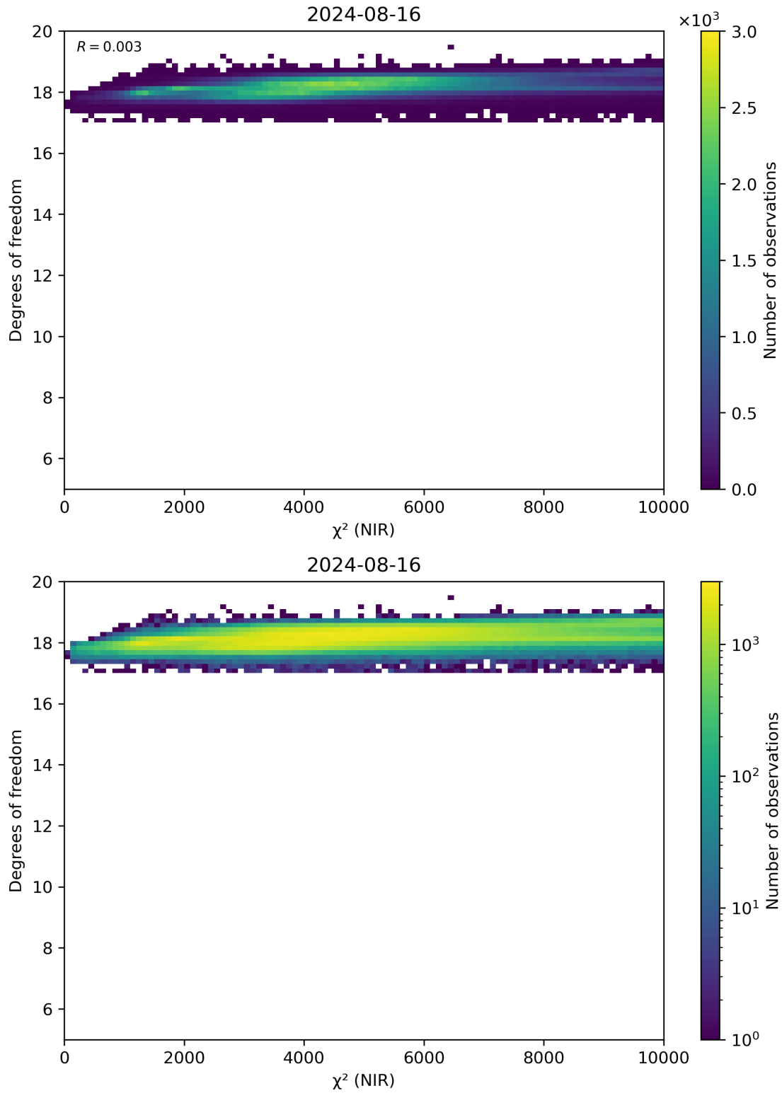
Figure 44: Scatter density plot of “ \chi^2 (NIR)” against “Degrees of freedom” for 2024-08-16 to 2024-08-17.
