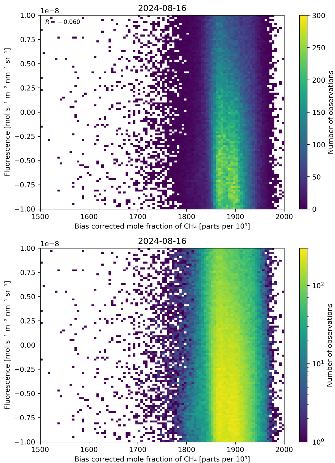
Figure 66: Scatter density plot of “Bias corrected mole fraction of \text{CH}_4 ” against “Fluorescence” for 2024-08-16 to 2024-08-17.
