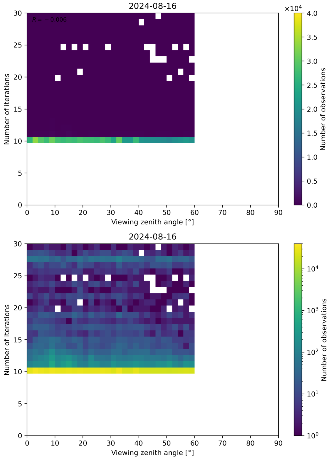
Figure 113: Scatter density plot of “Viewing zenith angle” against “Number of iterations” for 2024-08-16 to 2024-08-17.
