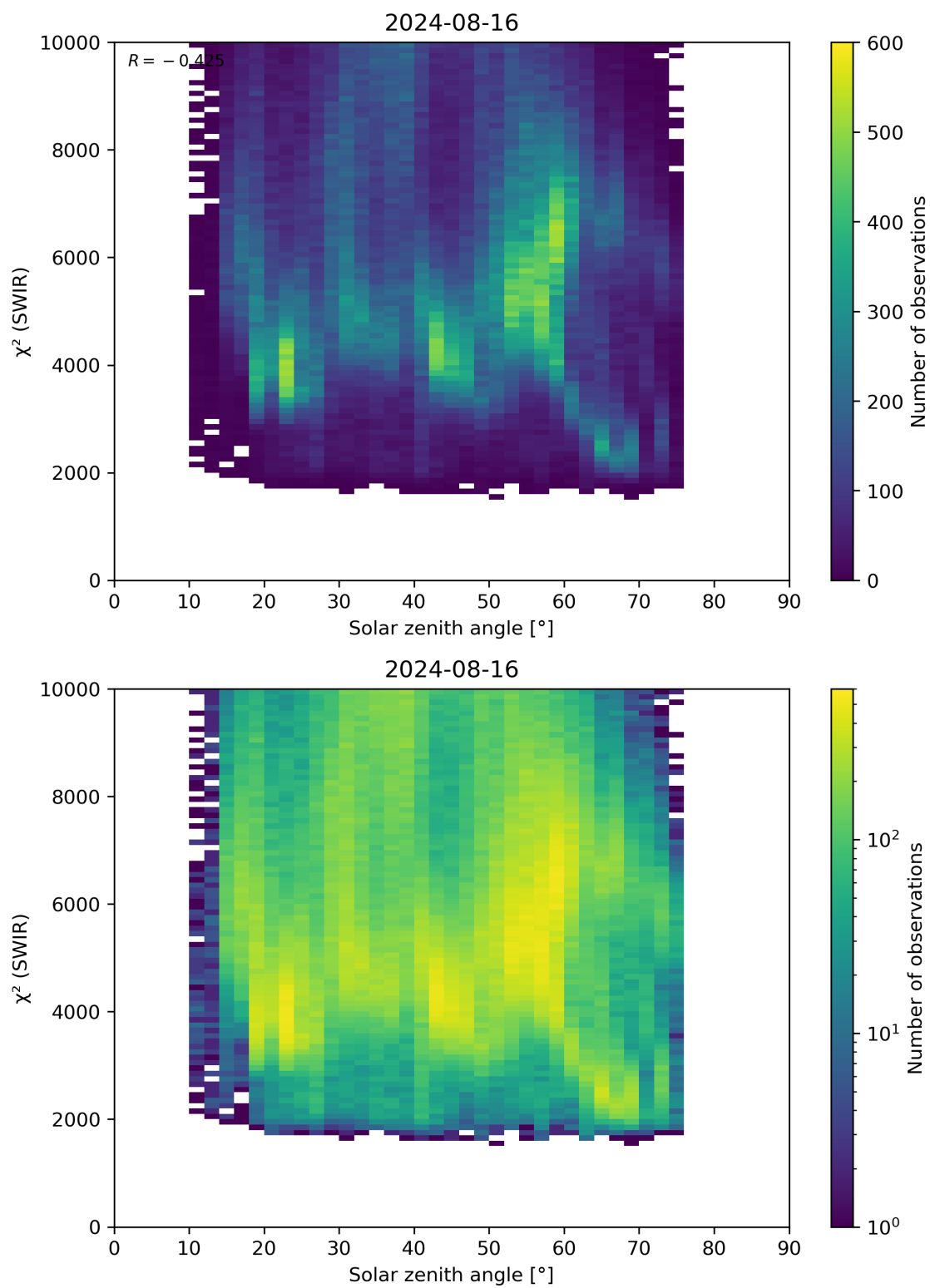
Figure 95: Scatter density plot of “Solar zenith angle” against “ \chi^2 (SWIR)” for 2024-08-16 to 2024-08-17.
