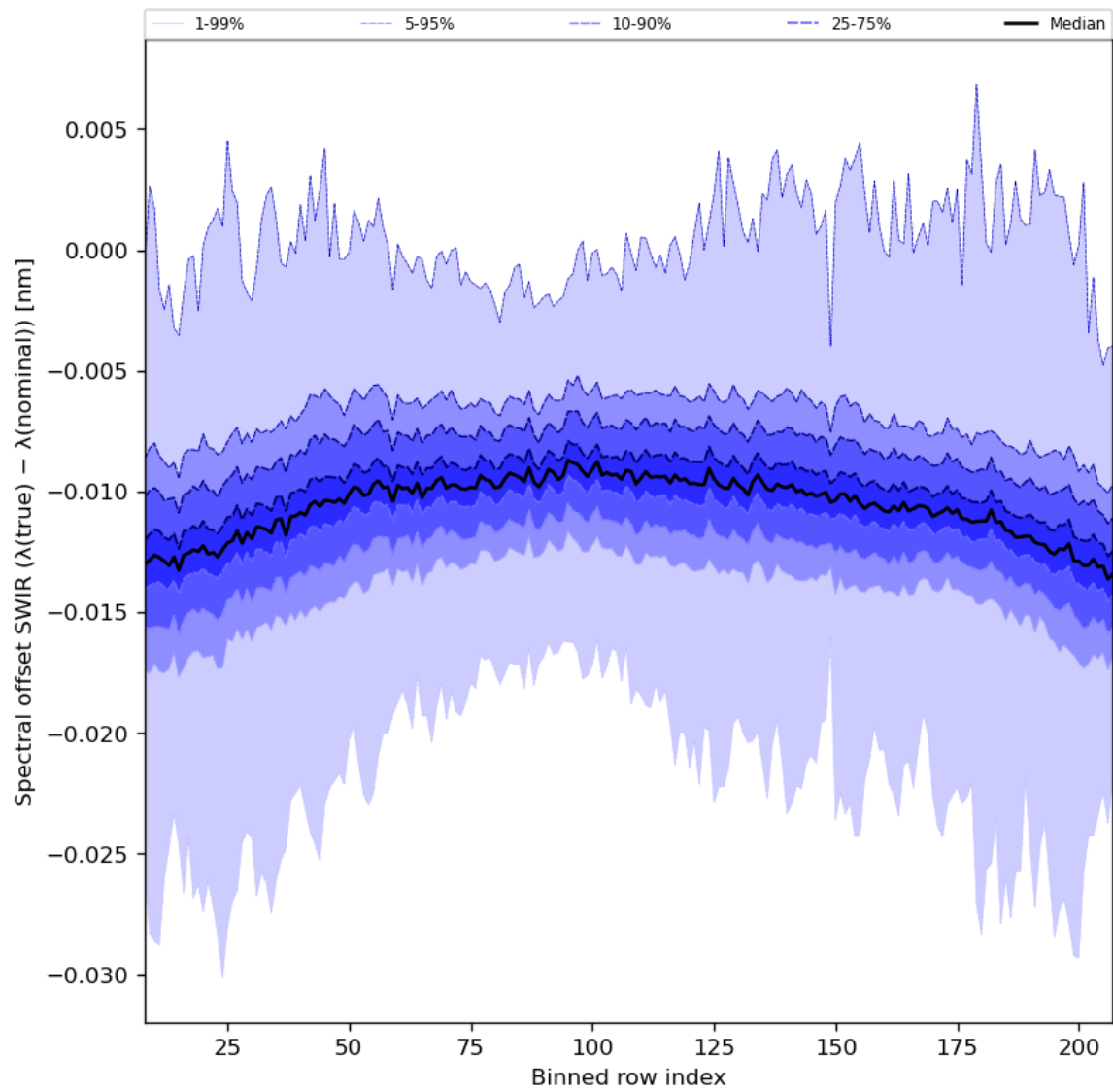
Figure 38: Along track statistics of “Spectral offset SWIR ( \lambda(\text{true}) - \lambda(\text{nominal}) )” for 2024-08-16 to 2024-08-17
