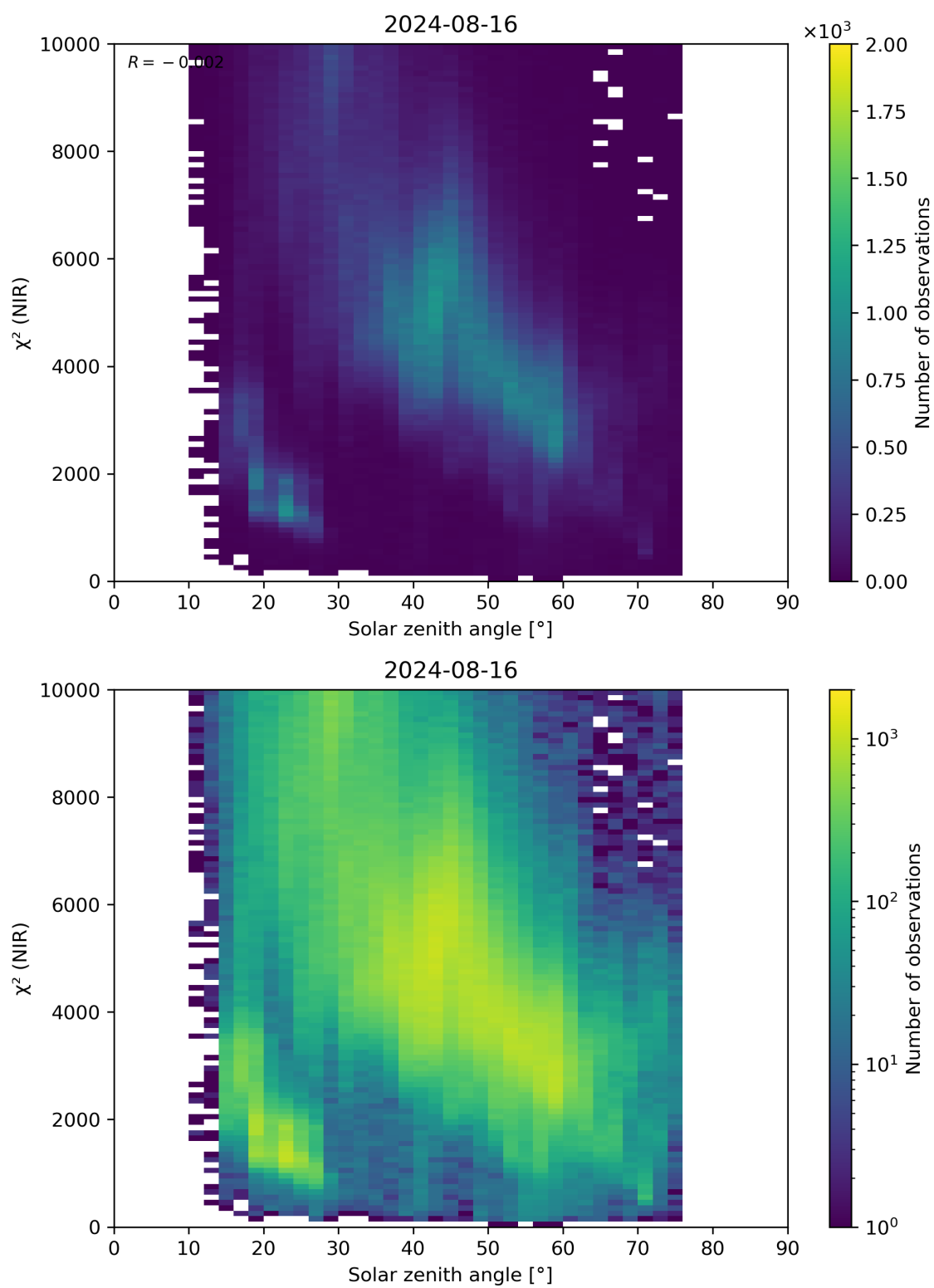
Figure 94: Scatter density plot of “Solar zenith angle” against “ \chi^2 (NIR)” for 2024-08-16 to 2024-08-17.
