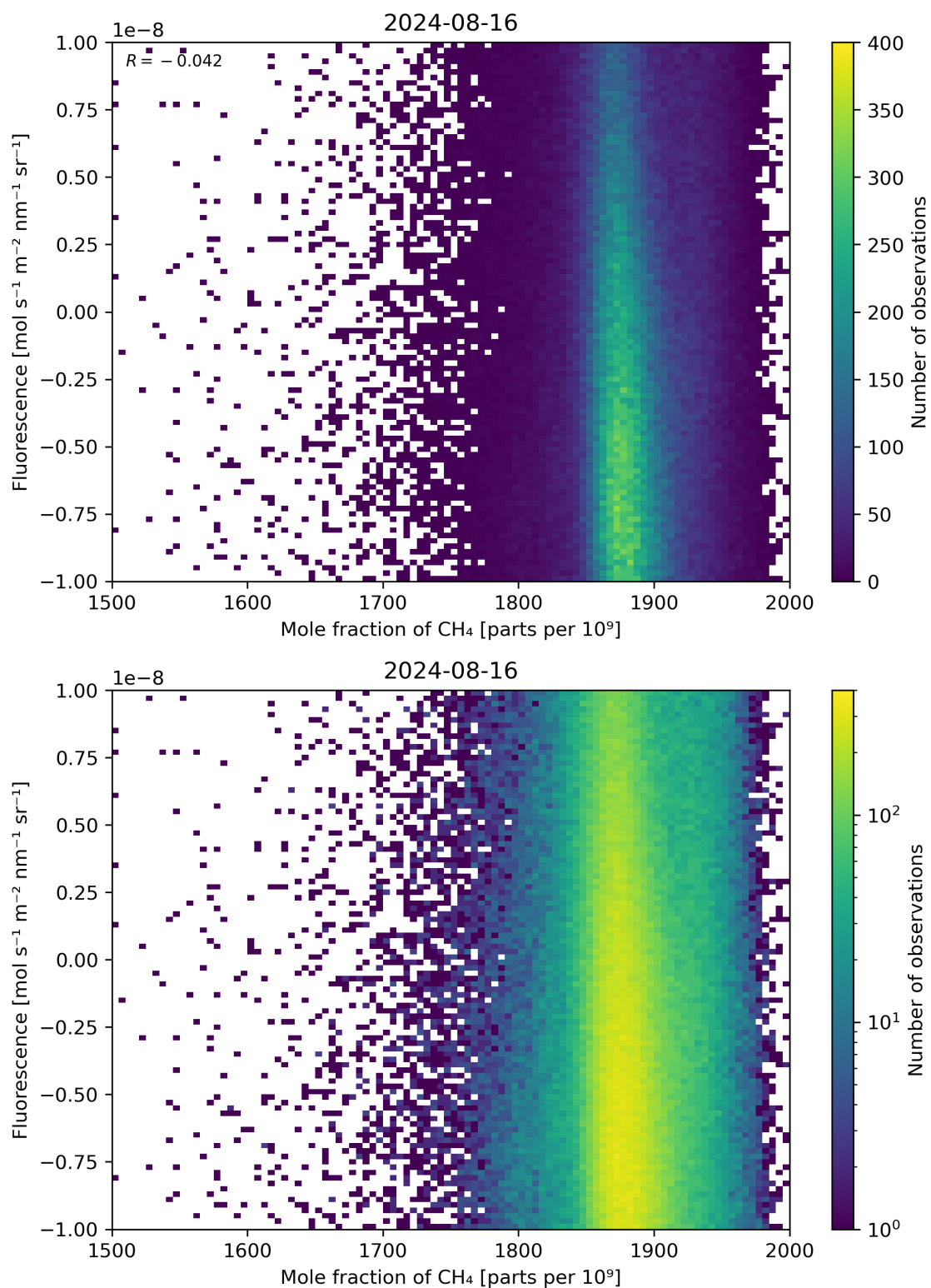
Figure 73: Scatter density plot of “Mole fraction of \text{CH}_4 ” against “Fluorescence” for 2024-08-16 to 2024-08-17.
