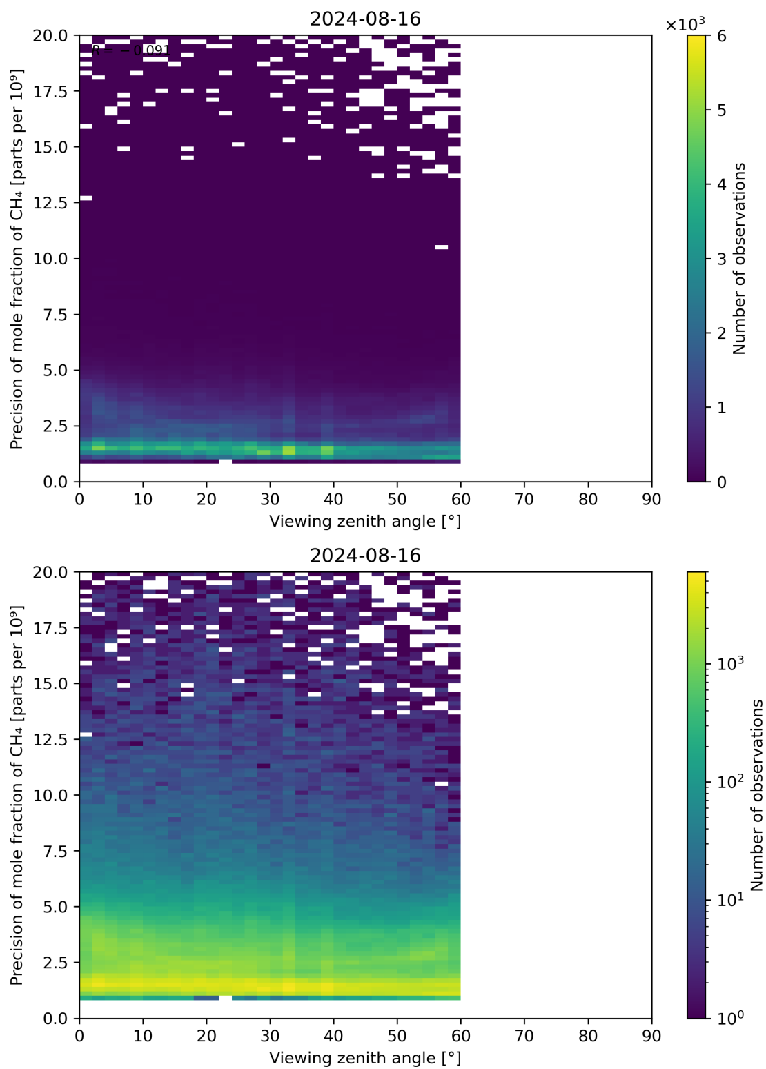
Figure 112: Scatter density plot of “Viewing zenith angle” against “Precision of mole fraction of CH 4 ” for 2024-08-16 to 2024-08-17.
