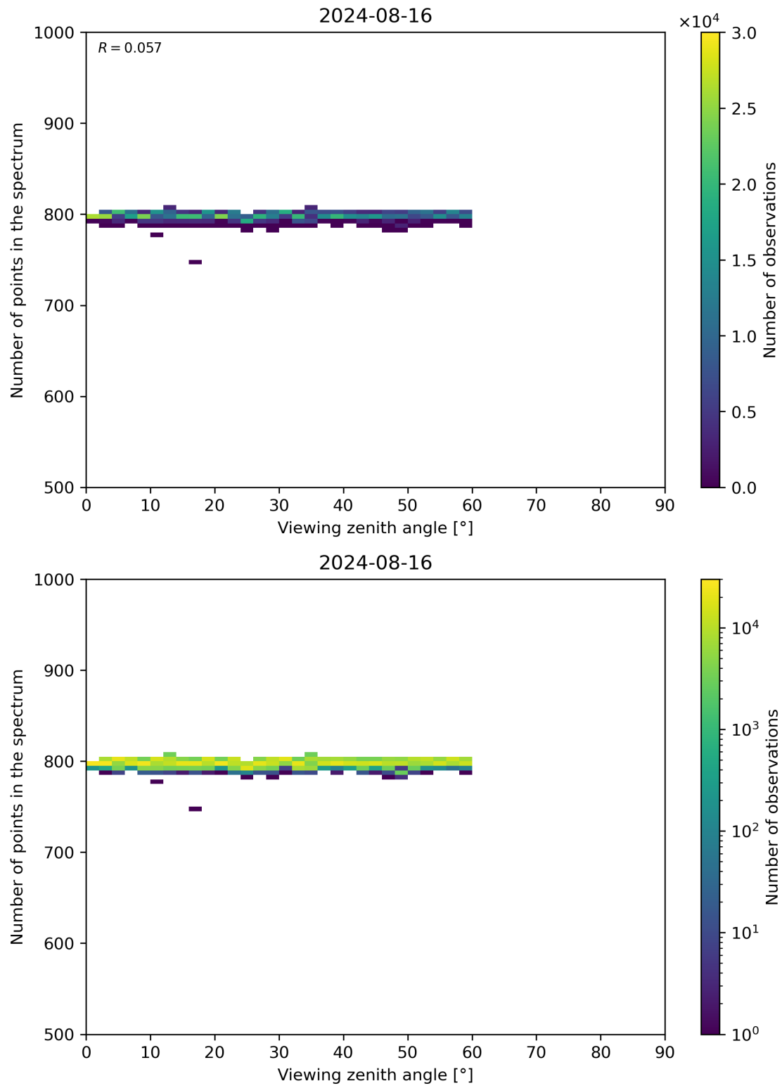
Figure 114: Scatter density plot of “Viewing zenith angle” against “Number of points in the spectrum” for 2024-08-16 to 2024-08-17.
