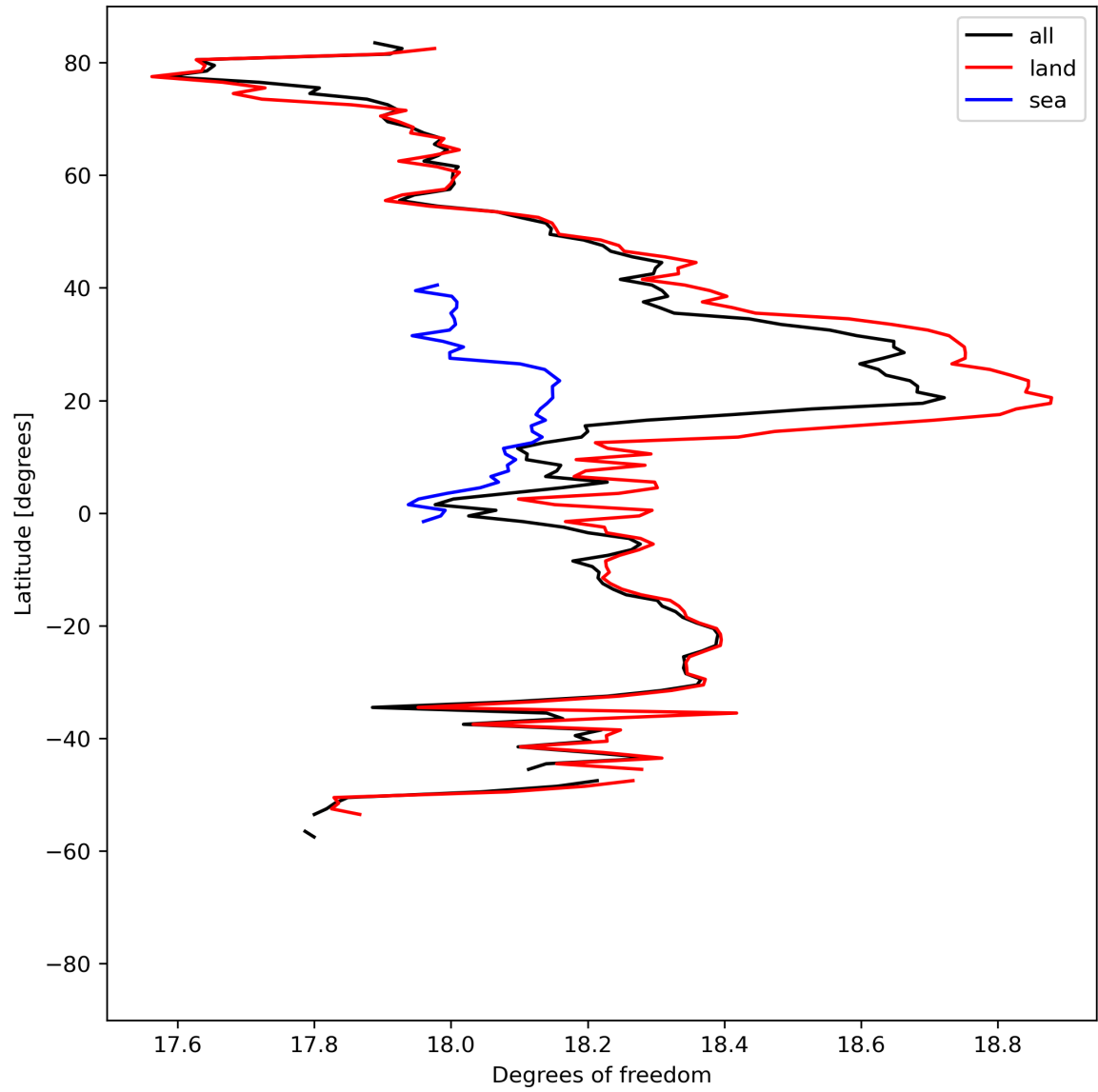
Figure 19: Zonal average of “Degrees of freedom” for 2024-08-16 to 2024-08-17.
