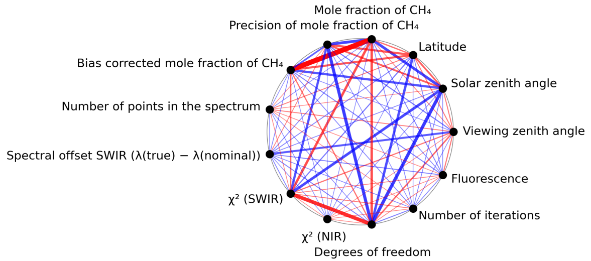
Figure 1: Map of correlation graph for 2024-08-16 to 2024-08-17.
