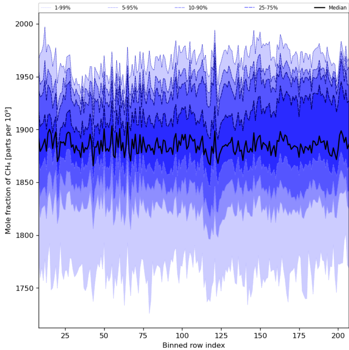
Figure 34: Along track statistics of “Mole fraction of CH 4 ” for 2024-08-16 to 2024-08-17
