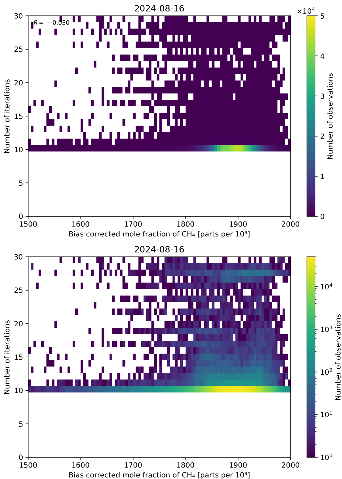
Figure 67: Scatter density plot of “Bias corrected mole fraction of CH 4 ” against “Number of iterations” for 2024-08-16 to 2024-08-17.
