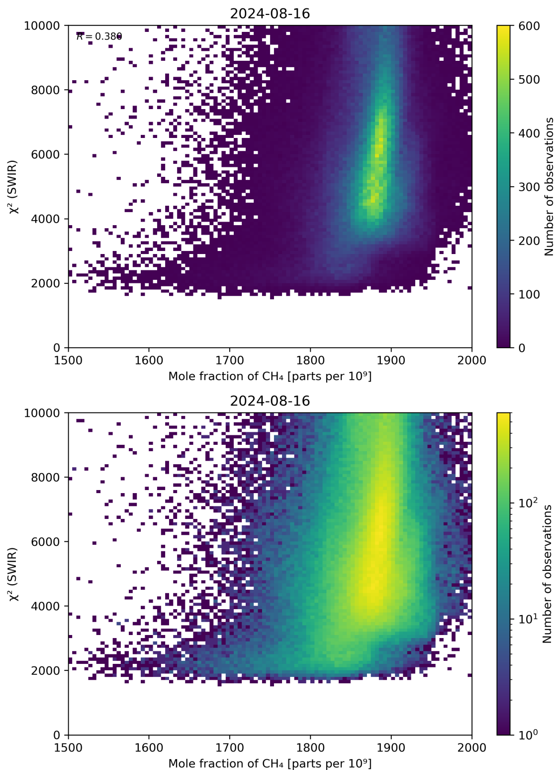
Figure 71: Scatter density plot of “Mole fraction of \text{CH}_4 ” against “ \chi^2 (SWIR)” for 2024-08-16 to 2024-08-17.
