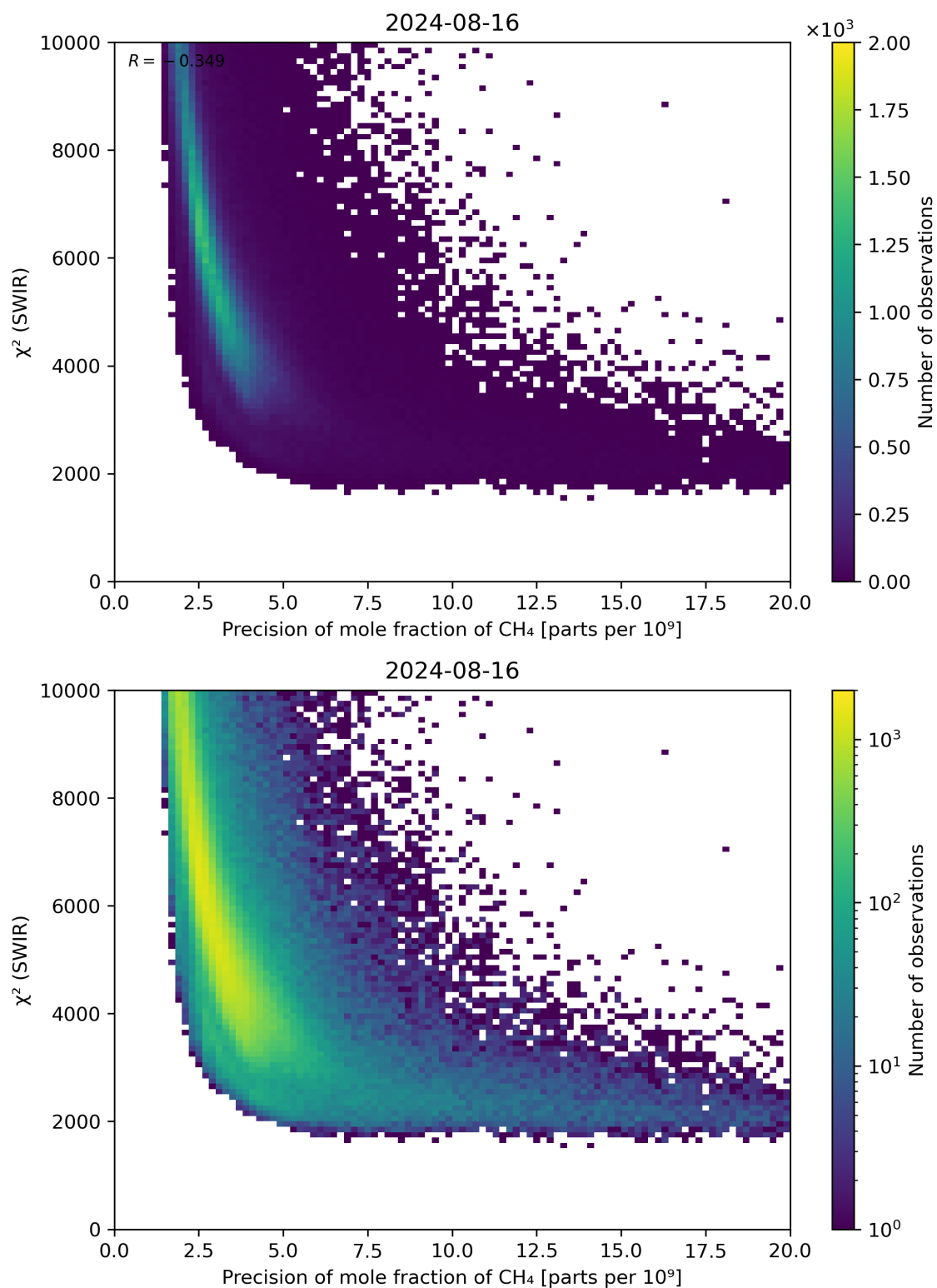
Figure 79: Scatter density plot of “Precision of mole fraction of CH 4 ” against “ \chi^2 (SWIR)” for 2024-08-16 to 2024-08-17.
