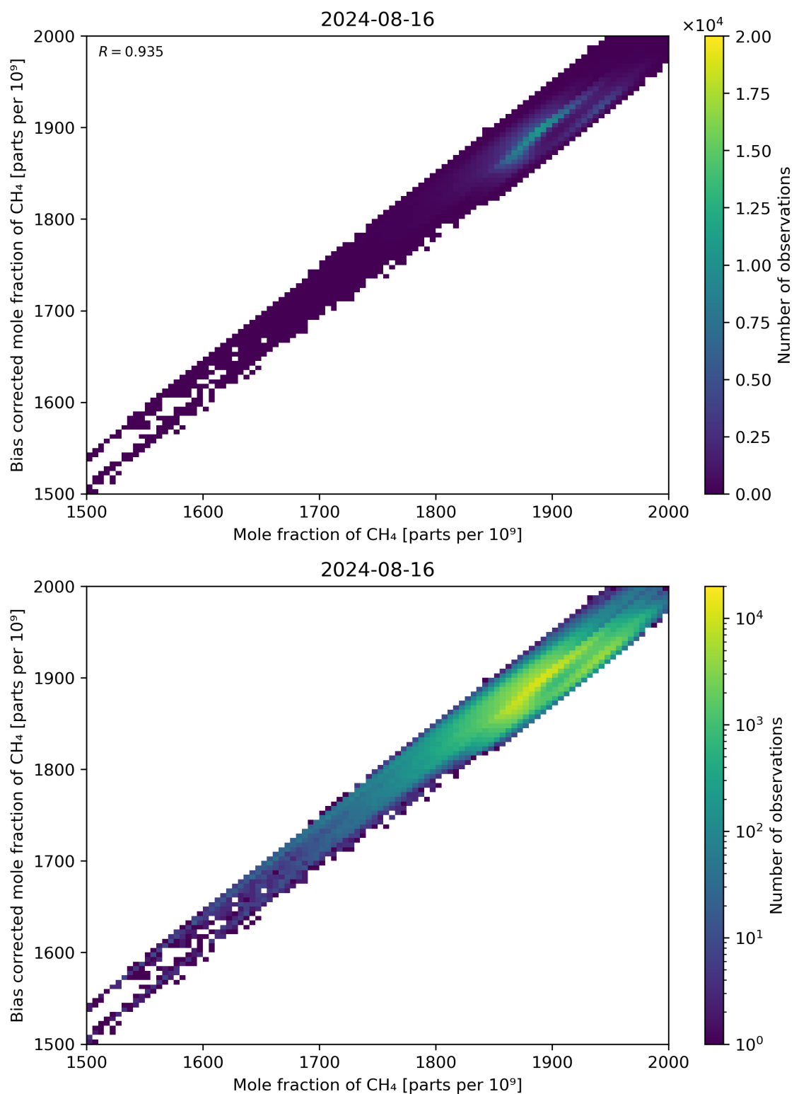
Figure 74: Scatter density plot of “Mole fraction of CH 4 ” against “Bias corrected mole fraction of CH 4 ” for 2024-08-16 to 2024-08-17.
