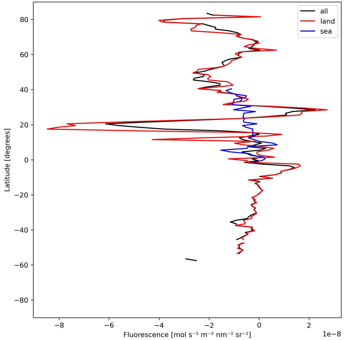
Figure 21: Zonal average of “Fluorescence” for 2024-08-16 to 2024-08-17.
