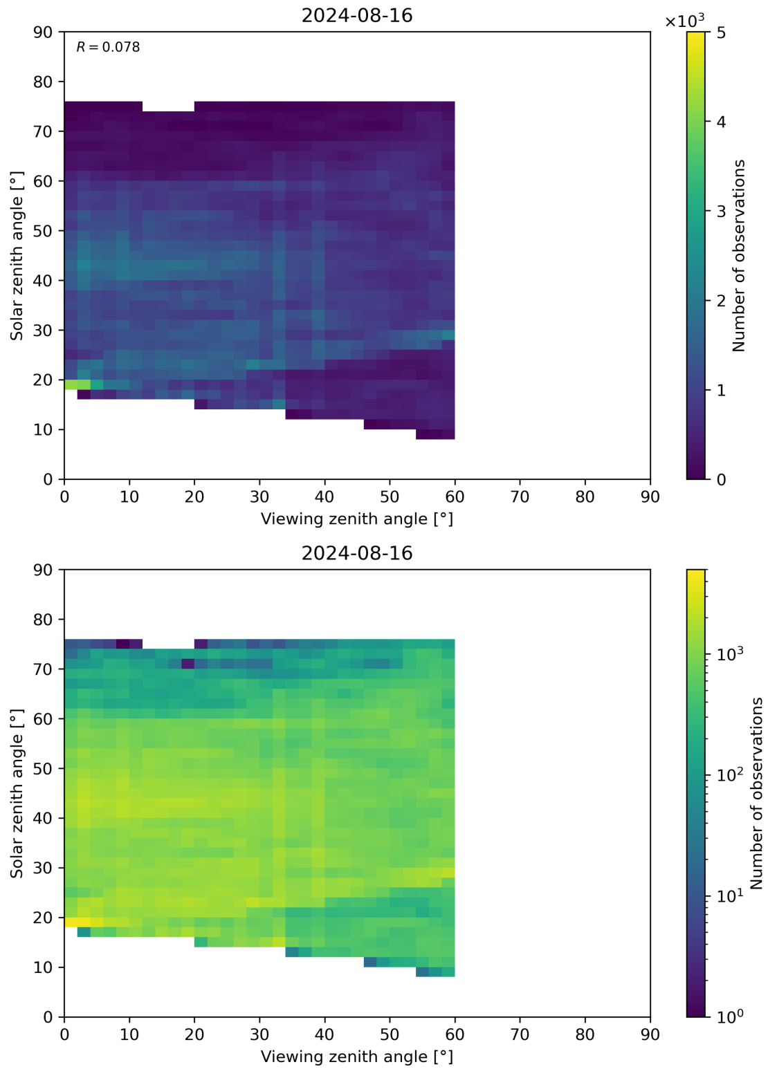
Figure 115: Scatter density plot of “Viewing zenith angle” against “Solar zenith angle” for 2024-08-16 to 2024-08-17.
