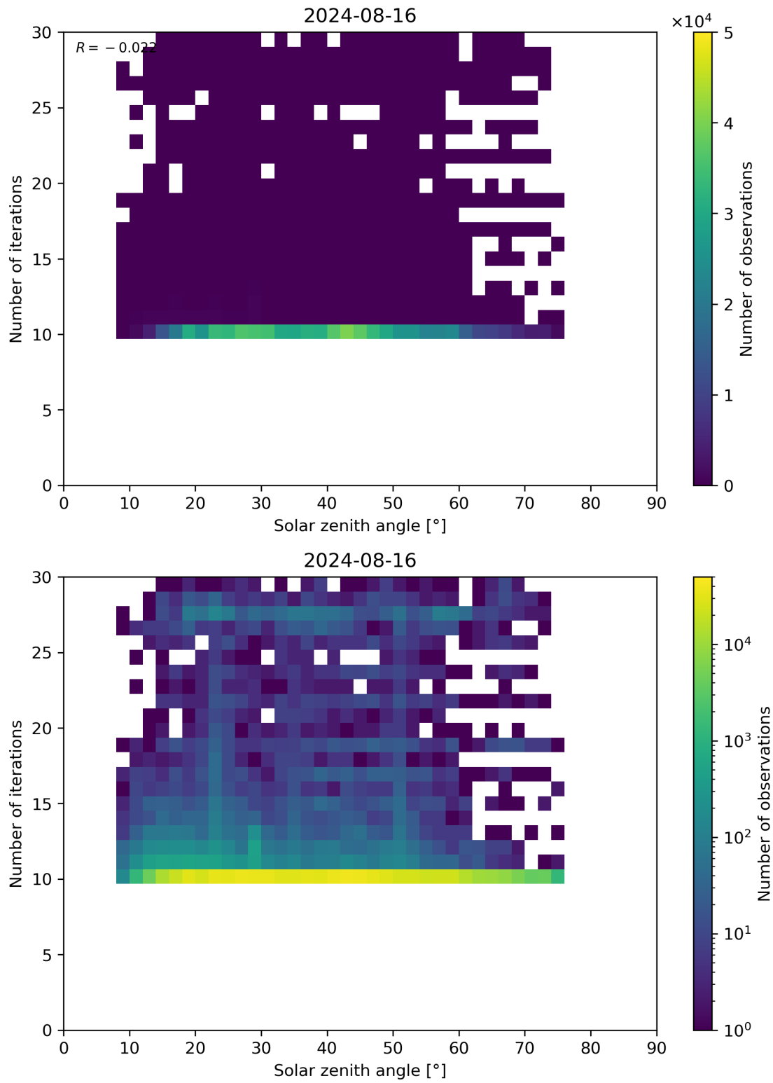
Figure 102: Scatter density plot of “Solar zenith angle” against “Number of iterations” for 2024-08-16 to 2024-08-17.
