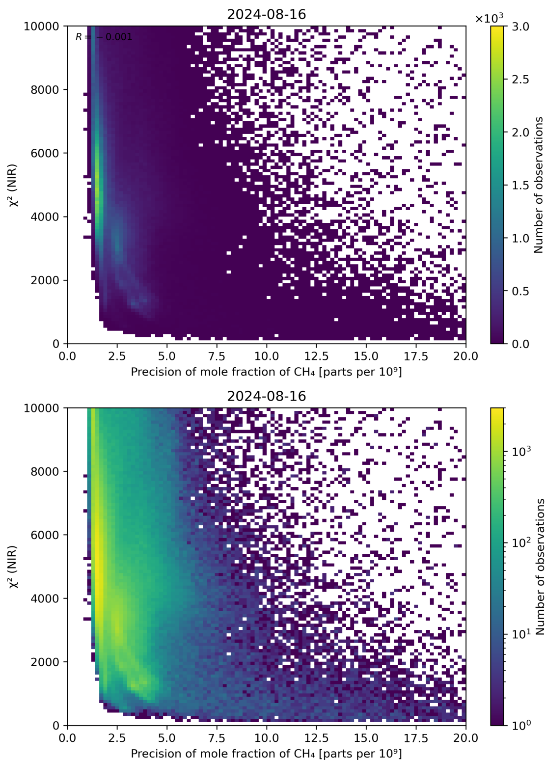
Figure 78: Scatter density plot of “Precision of mole fraction of \text{CH}_4 ” against “ \chi^2 (NIR)” for 2024-08-16 to 2024-08-17.
