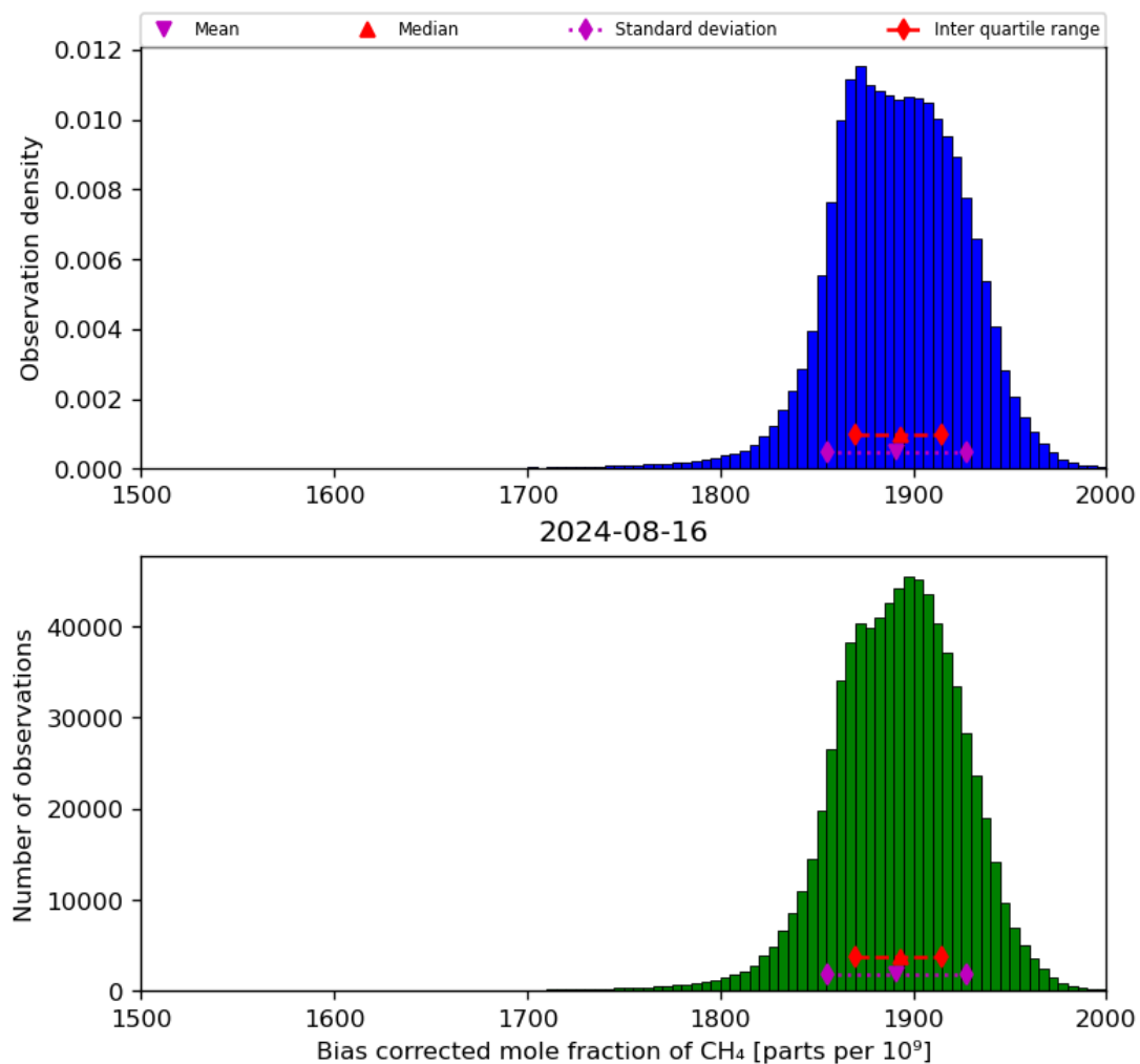
Figure 25: Histogram of “Bias corrected mole fraction of CH 4 ” for 2024-08-16 to 2024-08-17
