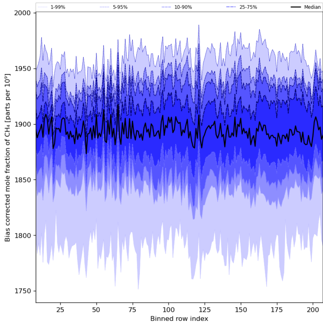
Figure 36: Along track statistics of “Bias corrected mole fraction of CH 4 ” for 2024-08-16 to 2024-08-17
