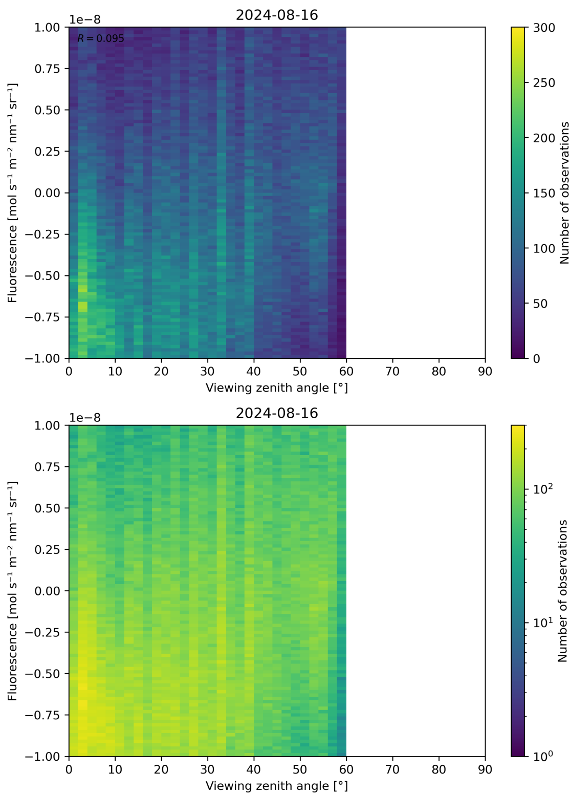
Figure 108: Scatter density plot of “Viewing zenith angle” against “Fluorescence” for 2024-08-16 to 2024-08-17.
