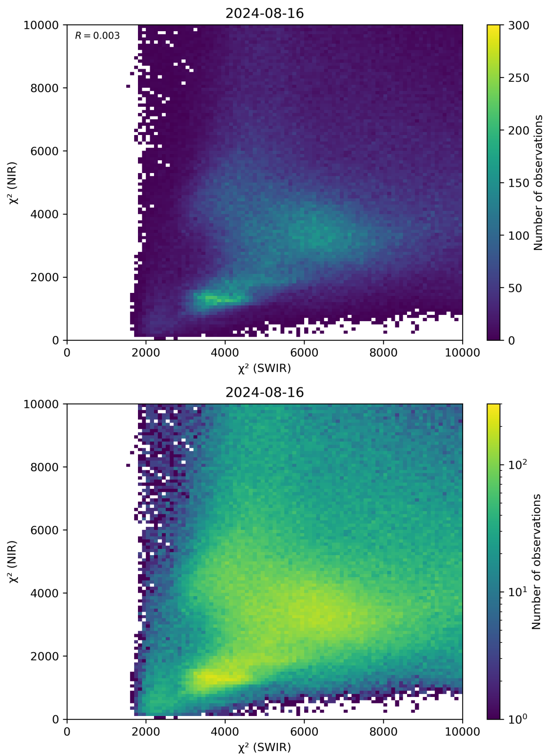
Figure 47: Scatter density plot of “ \chi^2 (SWIR)” against “ \chi^2 (NIR)” for 2024-08-16 to 2024-08-17.
