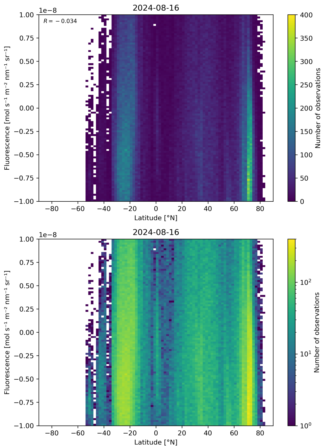
Figure 56: Scatter density plot of “Latitude” against “Fluorescence” for 2024-08-16 to 2024-08-17.
