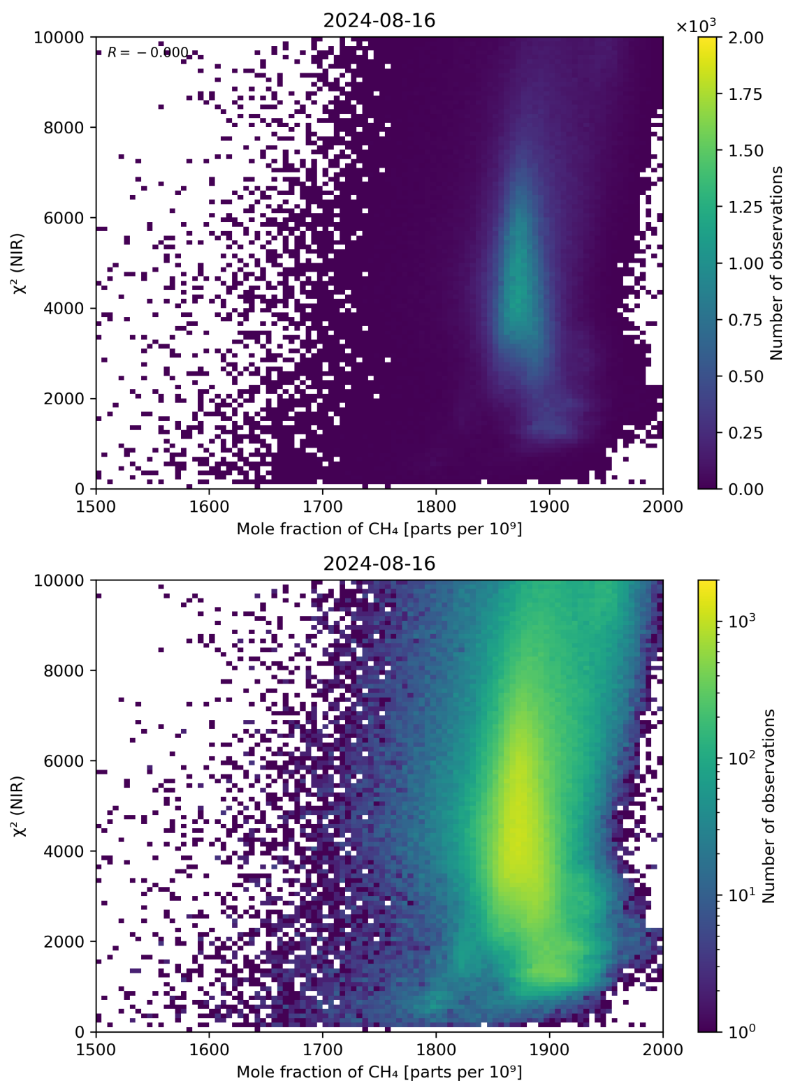
Figure 70: Scatter density plot of “Mole fraction of \text{CH}_4 ” against “ \chi^2 (NIR)” for 2024-08-16 to 2024-08-17.
