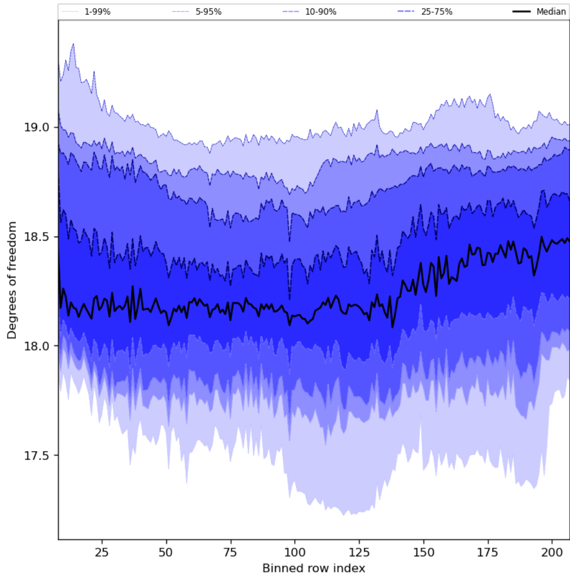
Figure 41: Along track statistics of “Degrees of freedom” for 2024-08-16 to 2024-08-17
