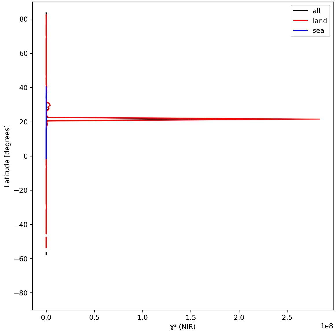
Figure 18: Zonal average of “ \chi^2 (NIR)” for 2024-08-16 to 2024-08-17.
