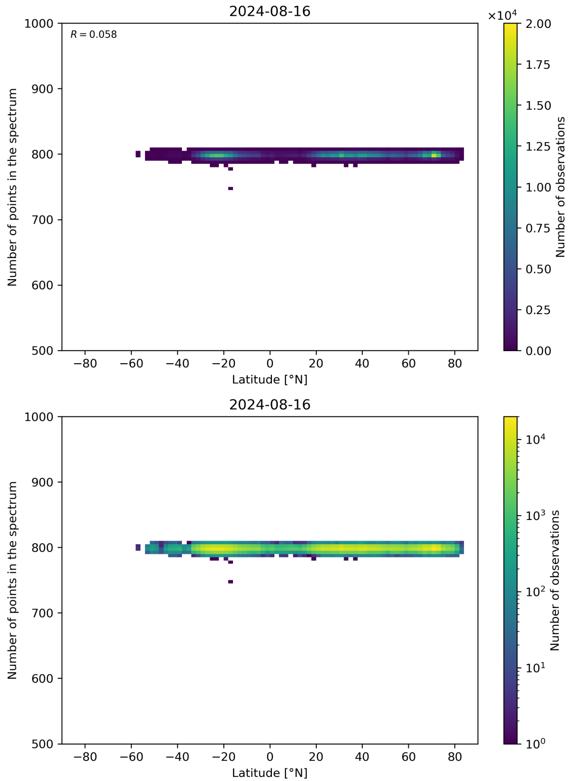
Figure 61: Scatter density plot of “Latitude” against “Number of points in the spectrum” for 2024-08-16 to 2024-08-17.
