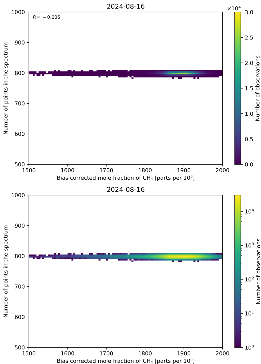
Figure 68: Scatter density plot of “Bias corrected mole fraction of CH 4 ” against “Number of points in the spectrum” for 2024-08-16 to 2024-08-17.
