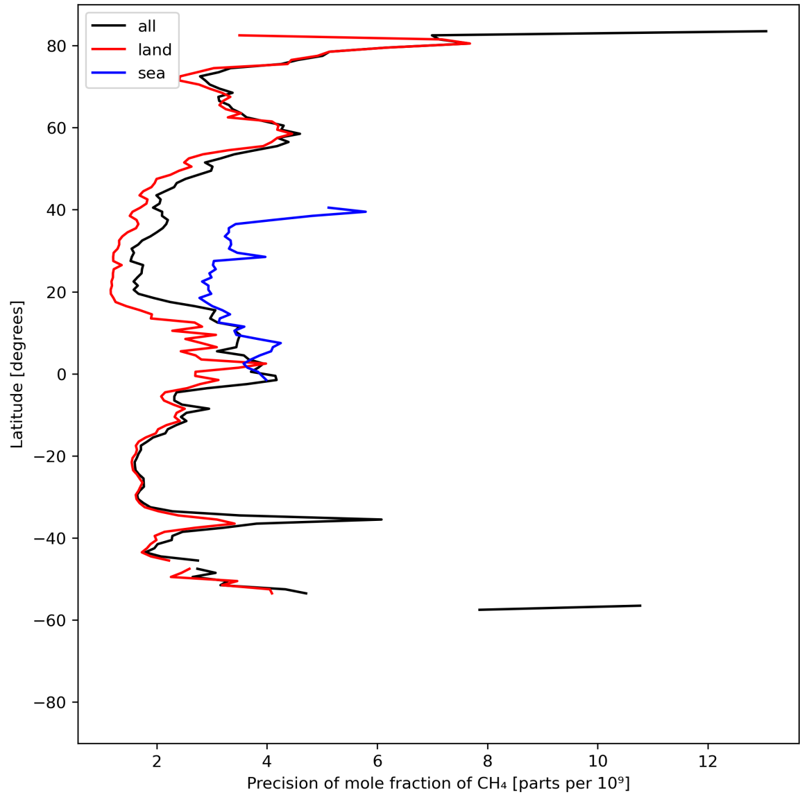
Figure 13: Zonal average of “Precision of mole fraction of \text{CH}_4 ” for 2024-08-16 to 2024-08-17.
