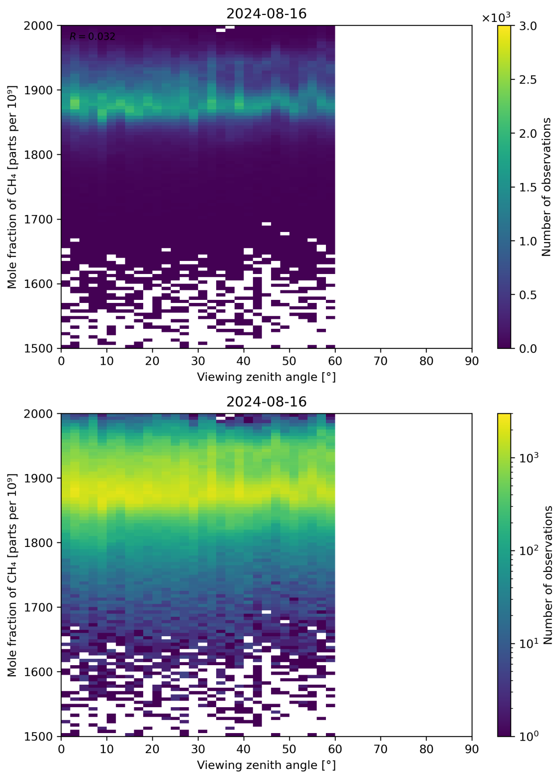
Figure 110: Scatter density plot of “Viewing zenith angle” against “Mole fraction of CH 4 ” for 2024-08-16 to 2024-08-17.
