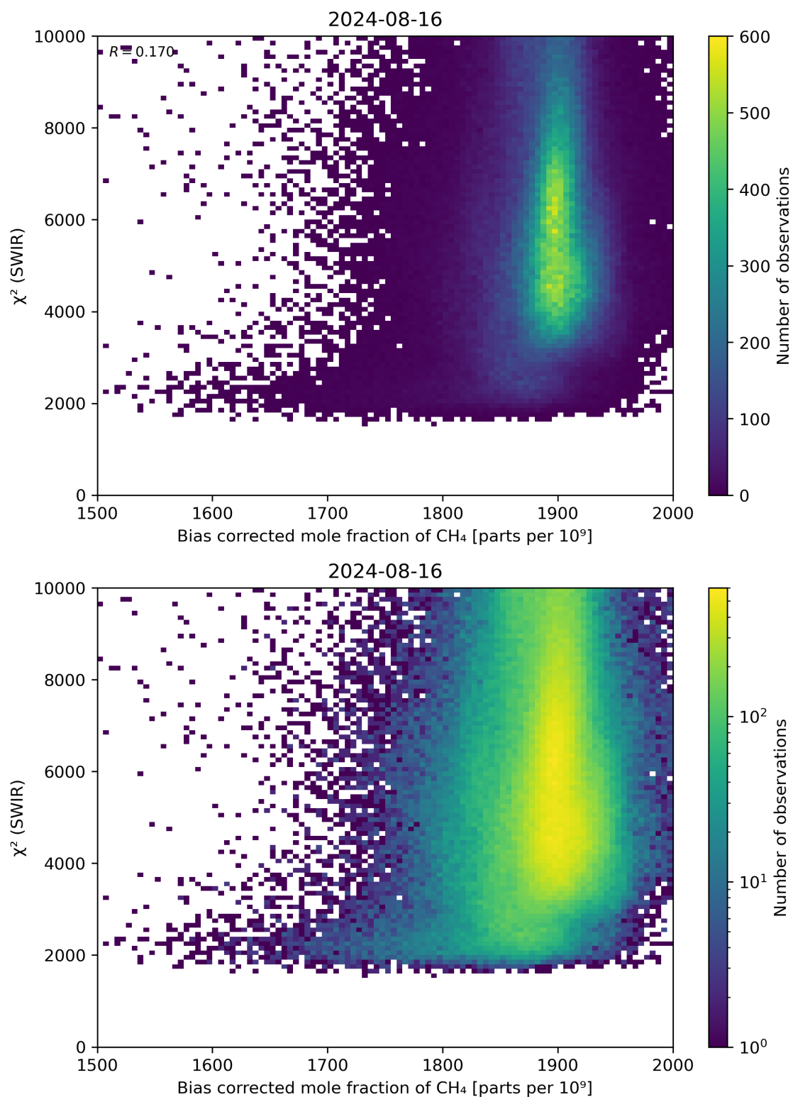
Figure 64: Scatter density plot of “Bias corrected mole fraction of \text{CH}_4 ” against “ \chi^2 (SWIR)” for 2024-08-16 to 2024-08-17.
