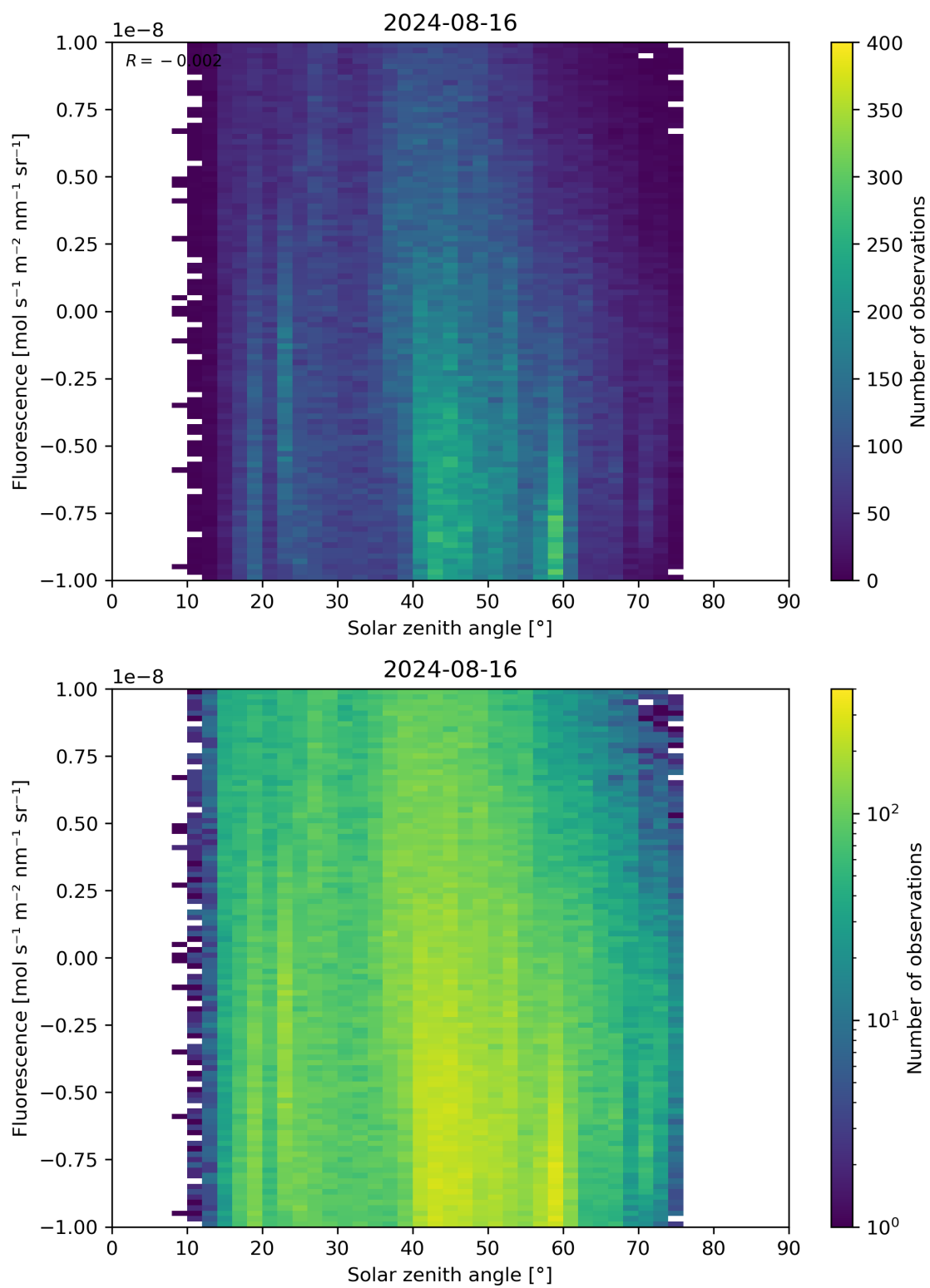
Figure 97: Scatter density plot of “Solar zenith angle” against “Fluorescence” for 2024-08-16 to 2024-08-17.
