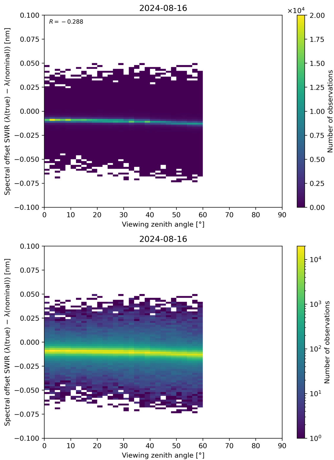
Figure 116: Scatter density plot of “Viewing zenith angle” against “Spectral offset SWIR ( \lambda(\text{true}) - \lambda(\text{nominal}) )” for 2024-08-16 to 2024-08-17.
