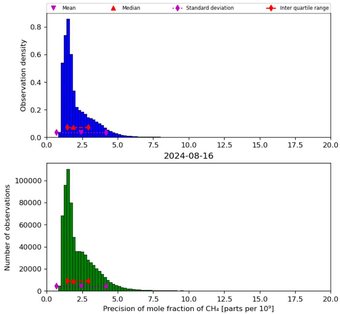
Figure 24: Histogram of “Precision of mole fraction of CH 4 ” for 2024-08-16 to 2024-08-17
