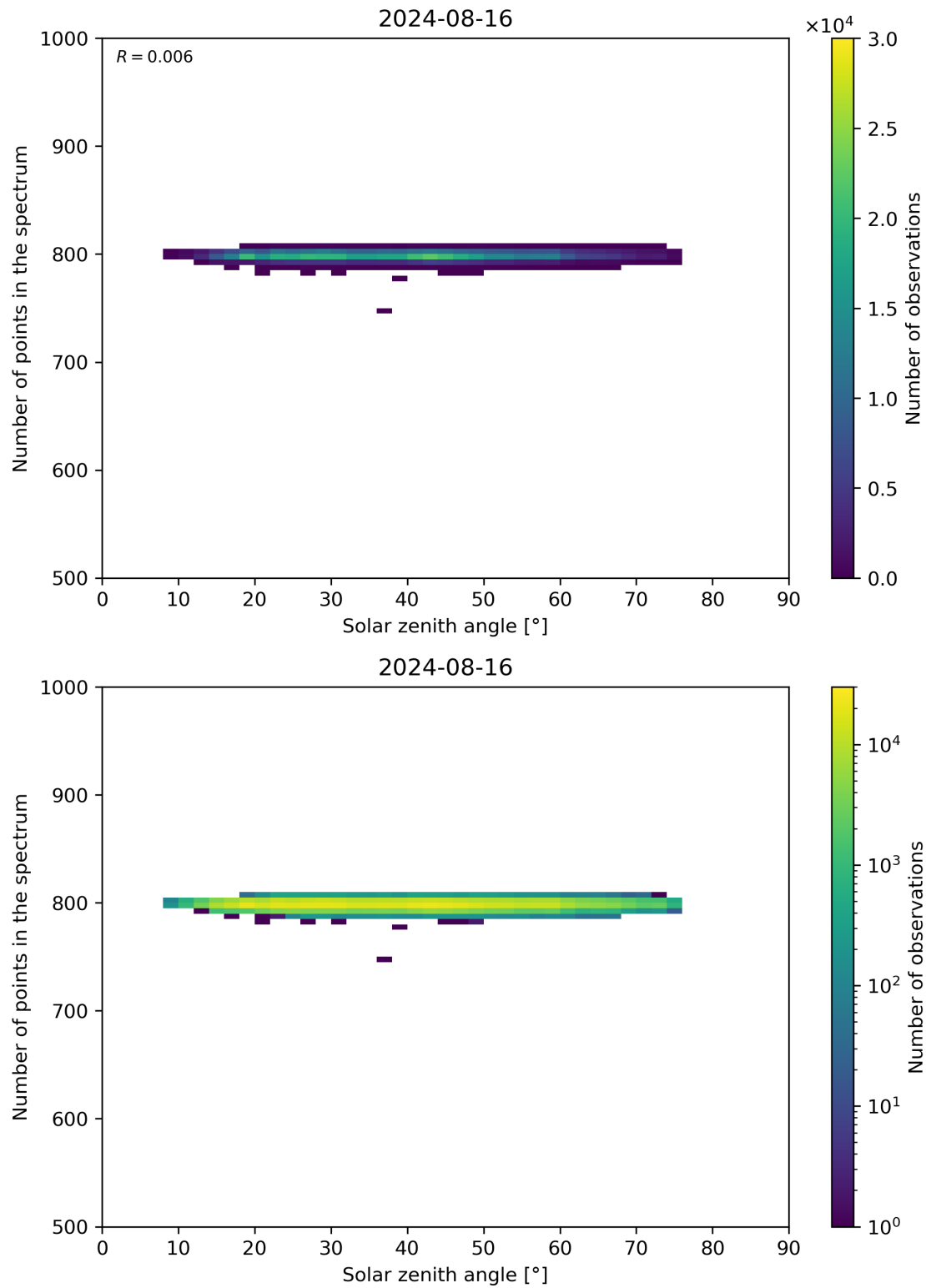
Figure 103: Scatter density plot of “Solar zenith angle” against “Number of points in the spectrum” for 2024-08-16 to 2024-08-17.
