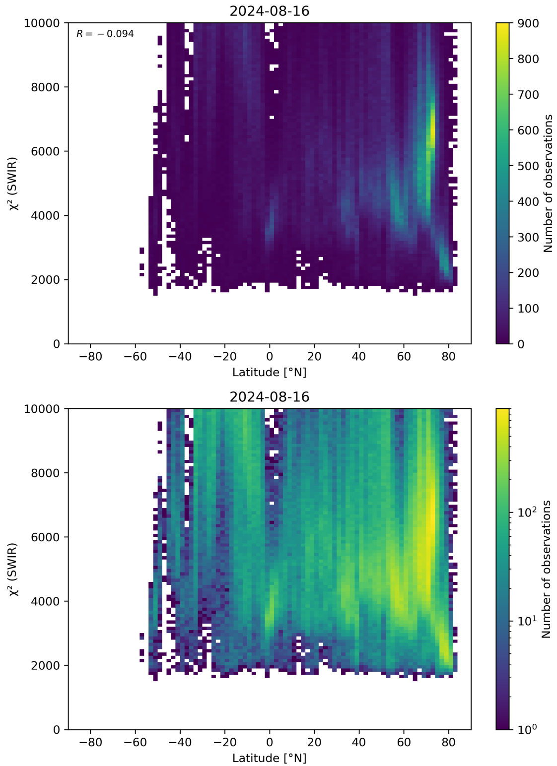
Figure 54: Scatter density plot of “Latitude” against “ \chi^2 (SWIR)” for 2024-08-16 to 2024-08-17.
