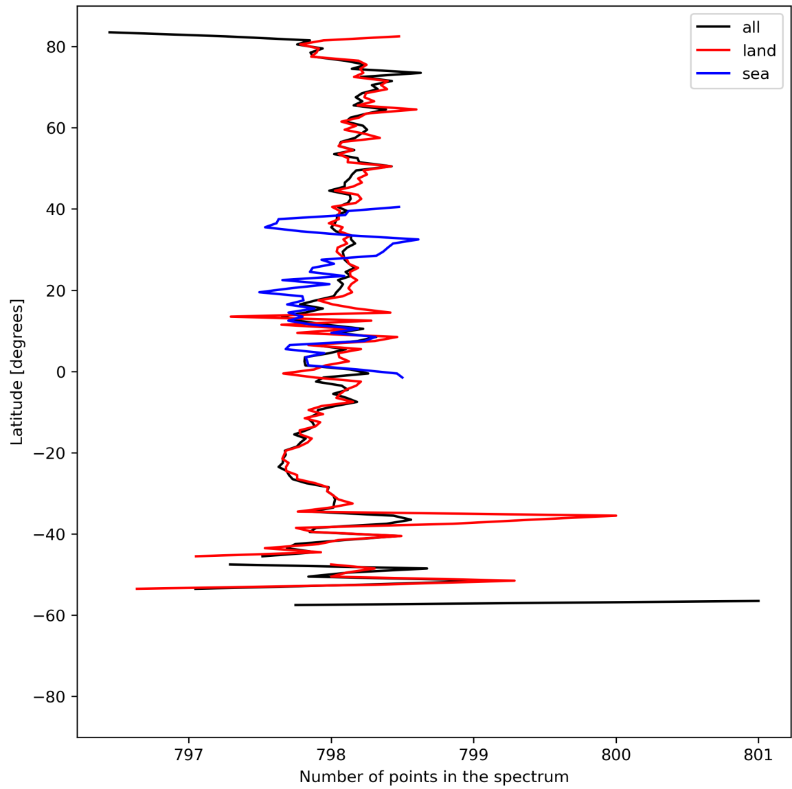
Figure 15: Zonal average of “Number of points in the spectrum” for 2024-08-16 to 2024-08-17.
