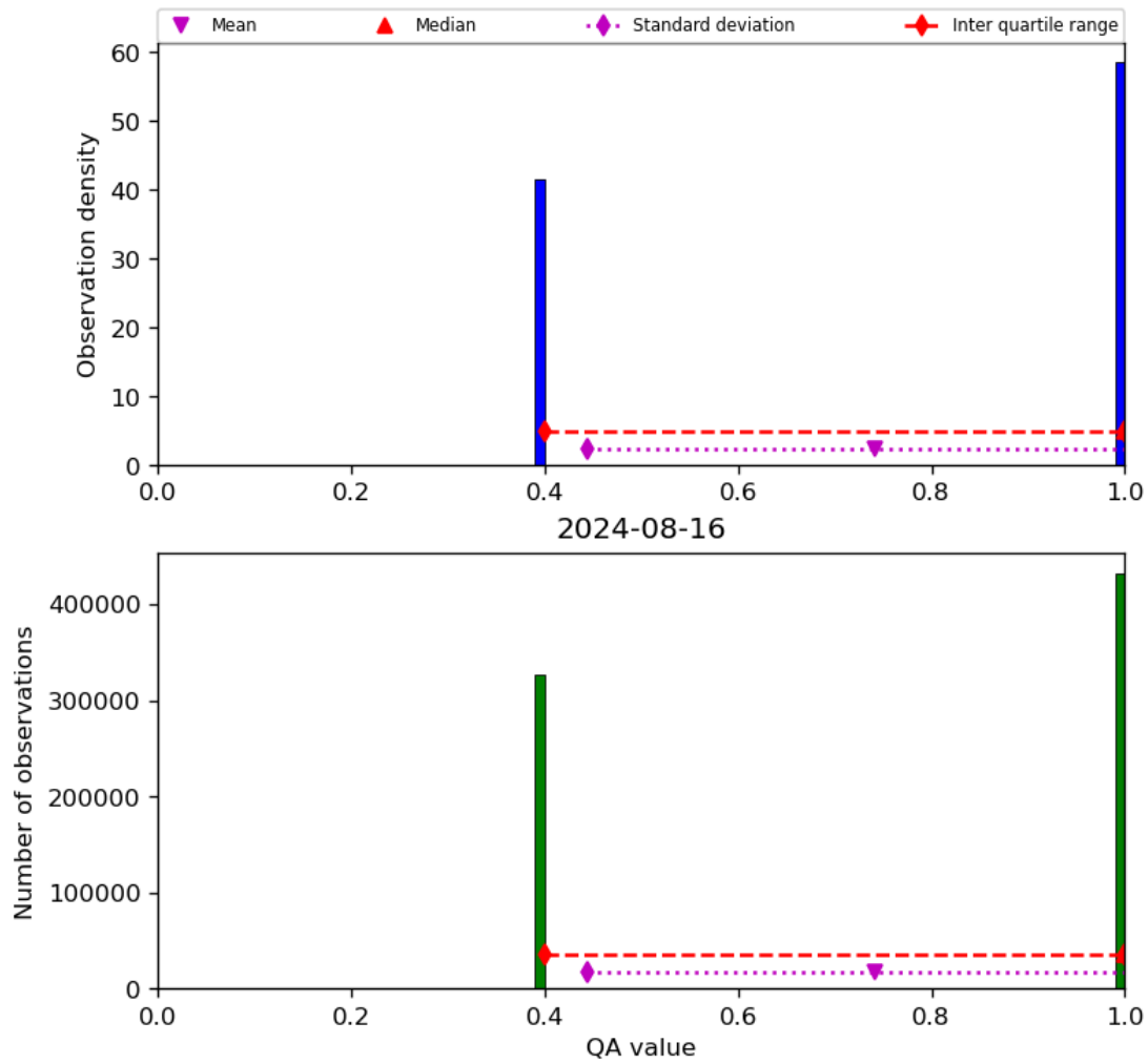
Figure 22: Histogram of “QA value” for 2024-08-16 to 2024-08-17
