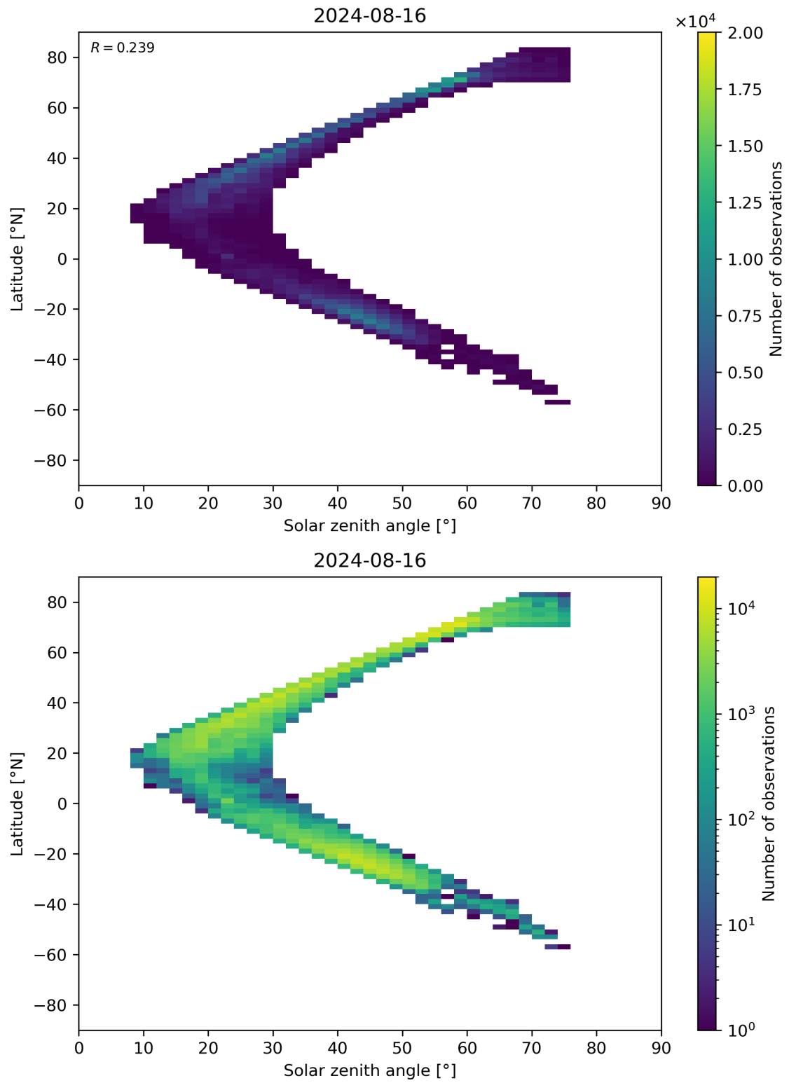
Figure 98: Scatter density plot of “Solar zenith angle” against “Latitude” for 2024-08-16 to 2024-08-17.
