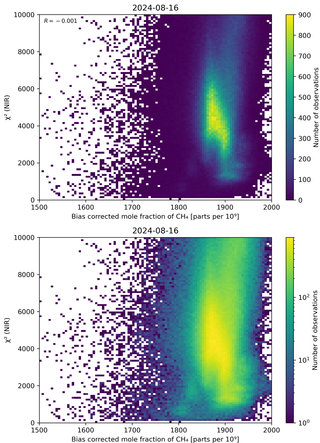
Figure 63: Scatter density plot of “Bias corrected mole fraction of CH 4 ” against “ \chi^2 (NIR)” for 2024-08-16 to 2024-08-17.
