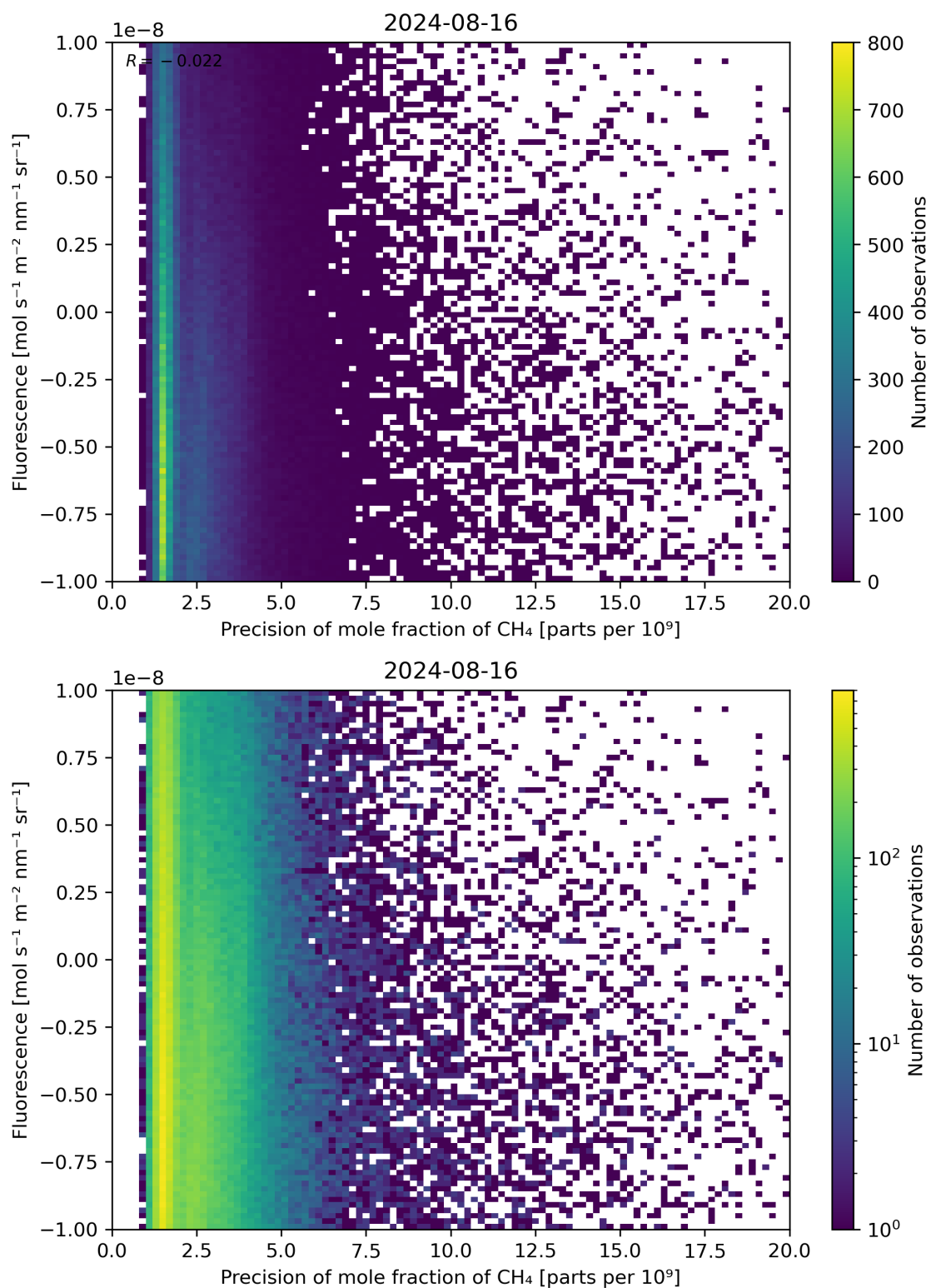
Figure 81: Scatter density plot of “Precision of mole fraction of \text{CH}_4 ” against “Fluorescence” for 2024-08-16 to 2024-08-17.
