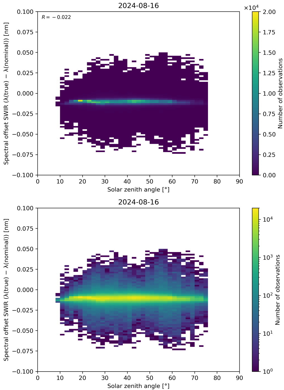
Figure 104: Scatter density plot of “Solar zenith angle” against “Spectral offset SWIR ( \lambda(\text{true}) - \lambda(\text{nominal}) )” for 2024-08-16 to 2024-08-17.
