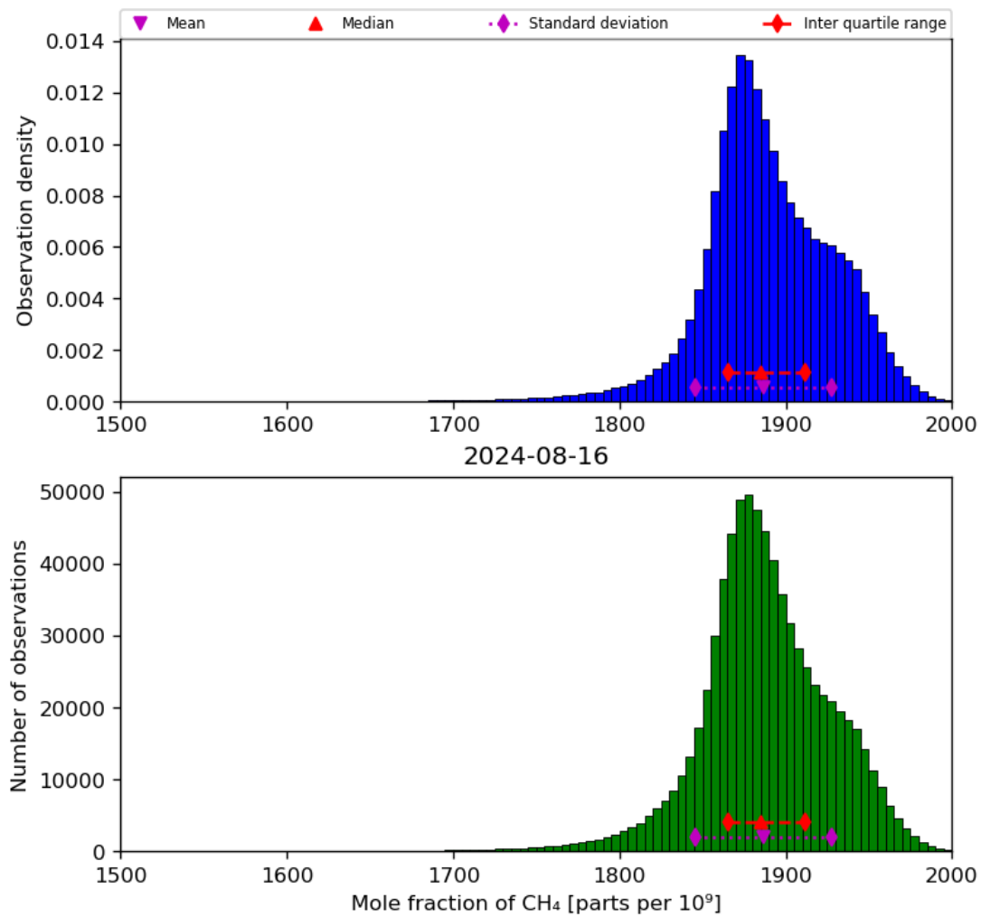
Figure 23: Histogram of “Mole fraction of CH 4 ” for 2024-08-16 to 2024-08-17
