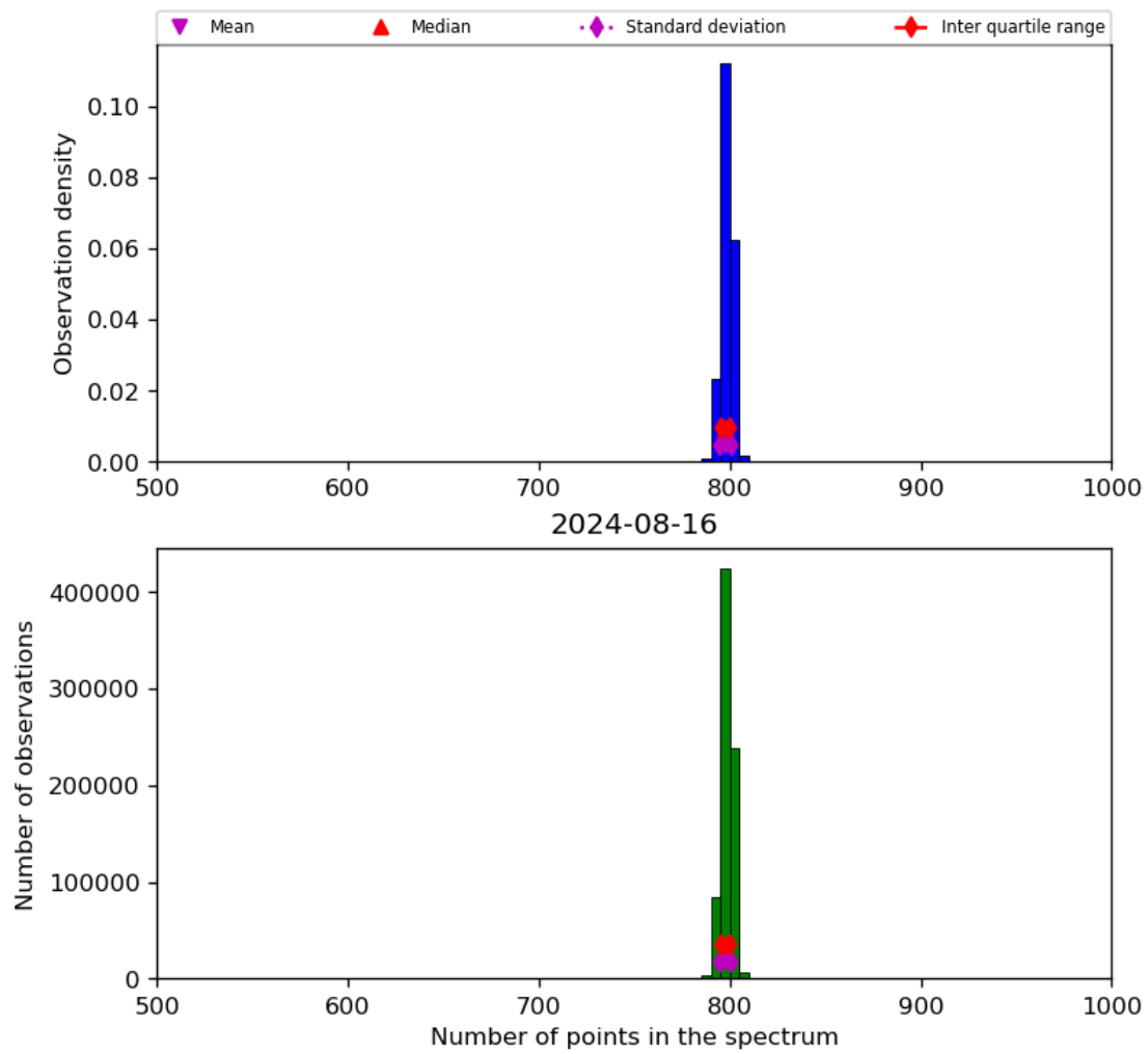
Figure 26: Histogram of “Number of points in the spectrum” for 2024-08-16 to 2024-08-17
