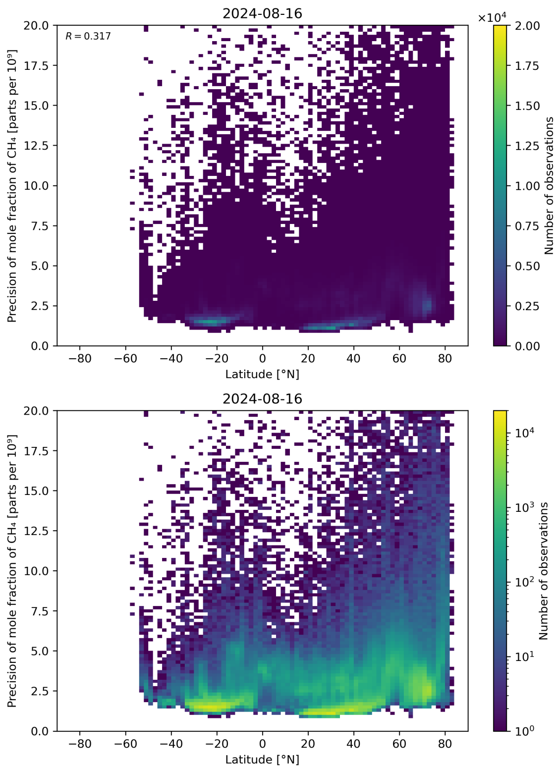
Figure 59: Scatter density plot of “Latitude” against “Precision of mole fraction of CH 4 ” for 2024-08-16 to 2024-08-17.
