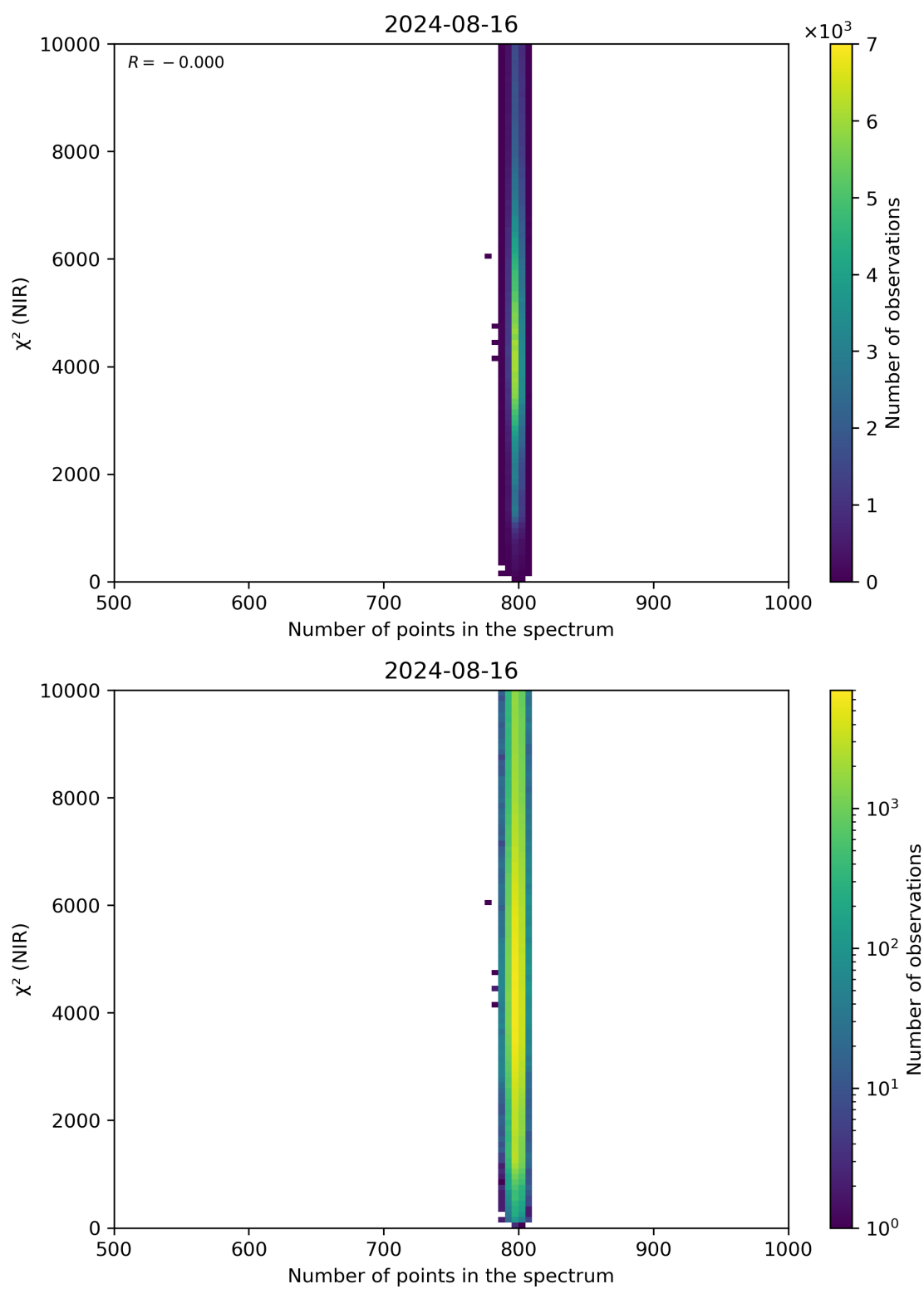
Figure 88: Scatter density plot of “Number of points in the spectrum” against “ \chi^2 (NIR)” for 2024-08-16 to 2024-08-17.
