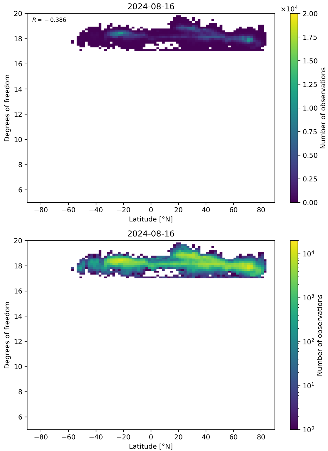
Figure 55: Scatter density plot of “Latitude” against “Degrees of freedom” for 2024-08-16 to 2024-08-17.
