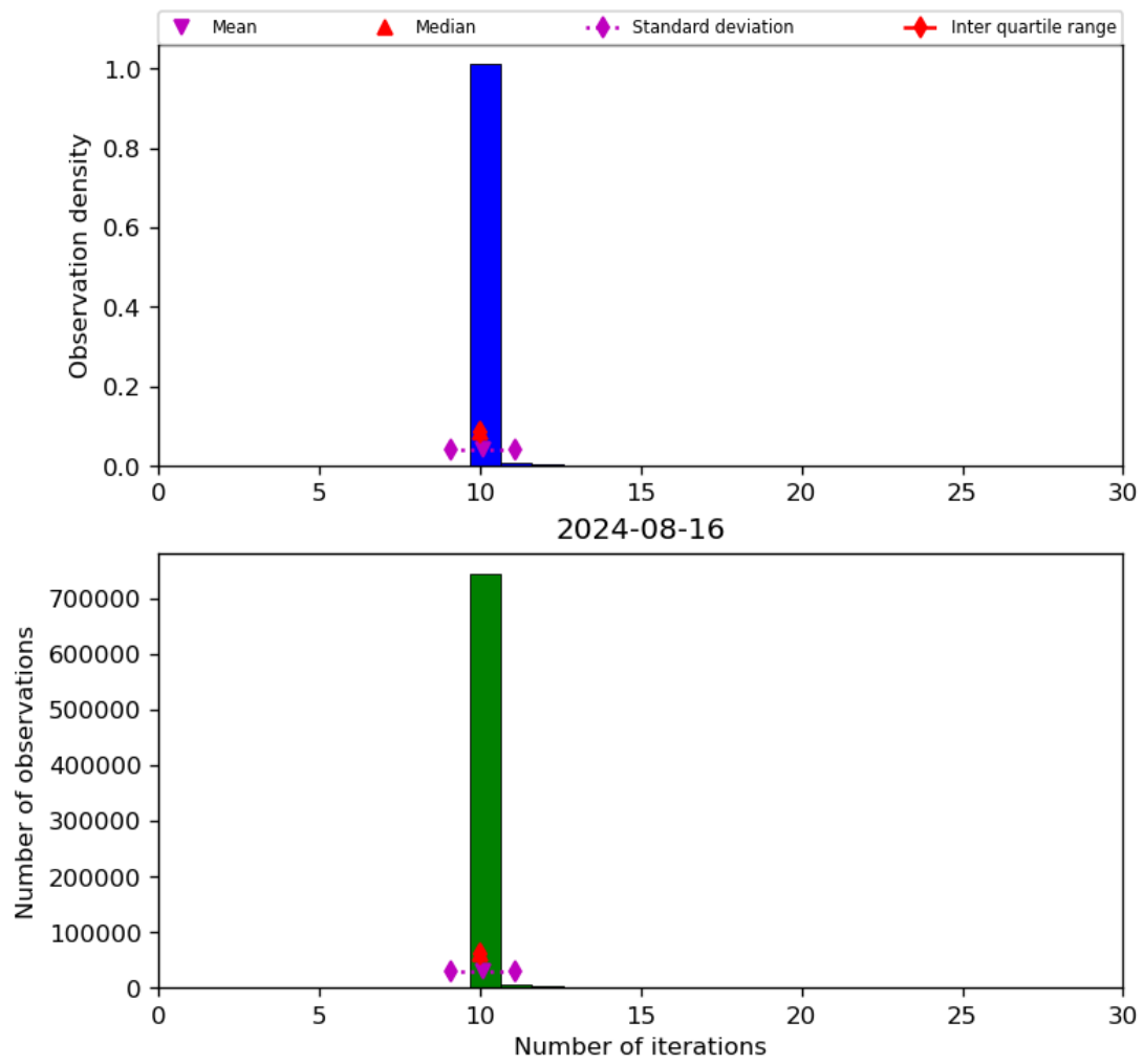
Figure 31: Histogram of “Number of iterations” for 2024-08-16 to 2024-08-17
