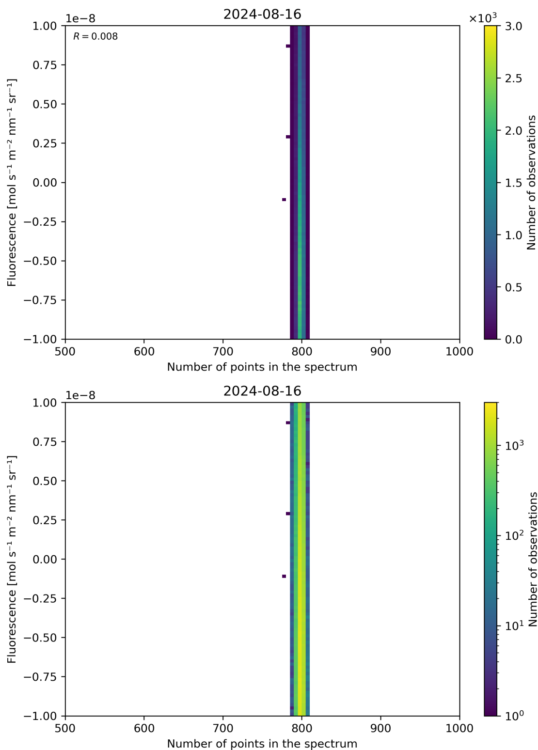
Figure 91: Scatter density plot of “Number of points in the spectrum” against “Fluorescence” for 2024-08-16 to 2024-08-17.
