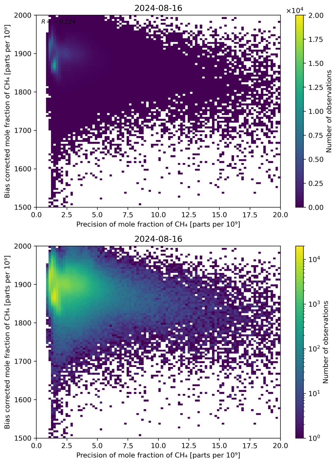
Figure 82: Scatter density plot of “Precision of mole fraction of CH 4 ” against “Bias corrected mole fraction of CH 4 ” for 2024-08-16 to 2024-08-17.
