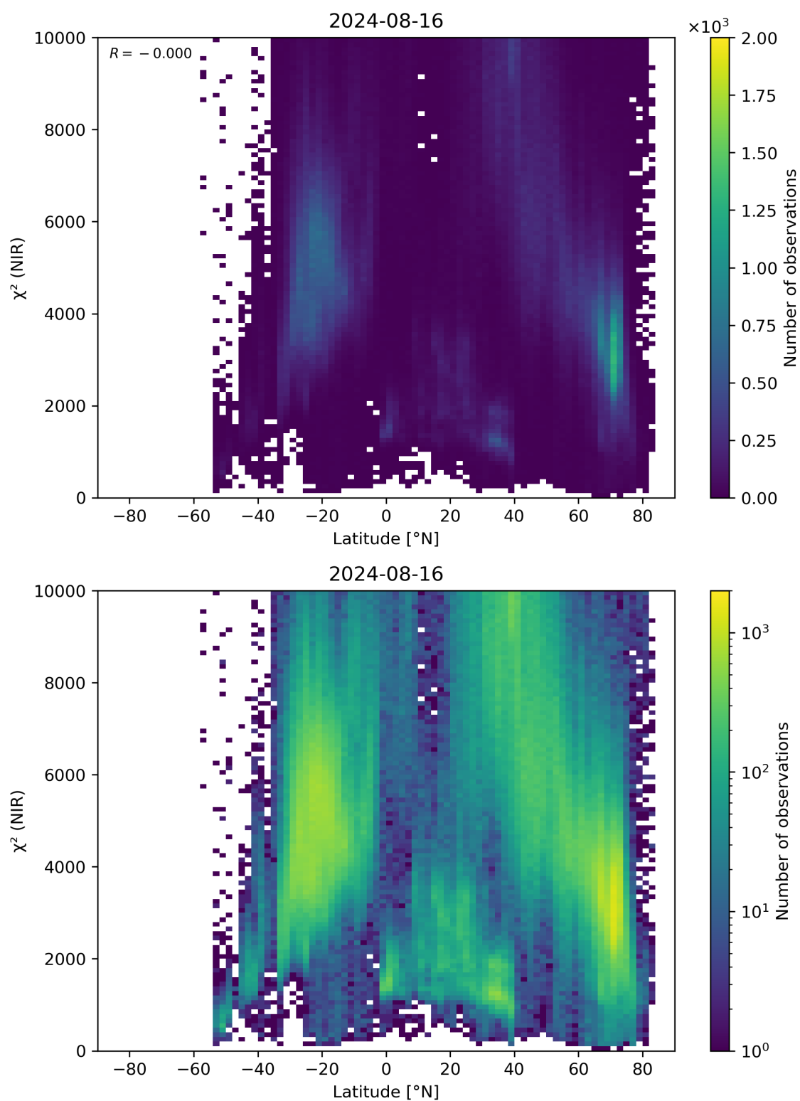
Figure 53: Scatter density plot of “Latitude” against “ \chi^2 (NIR)” for 2024-08-16 to 2024-08-17.
