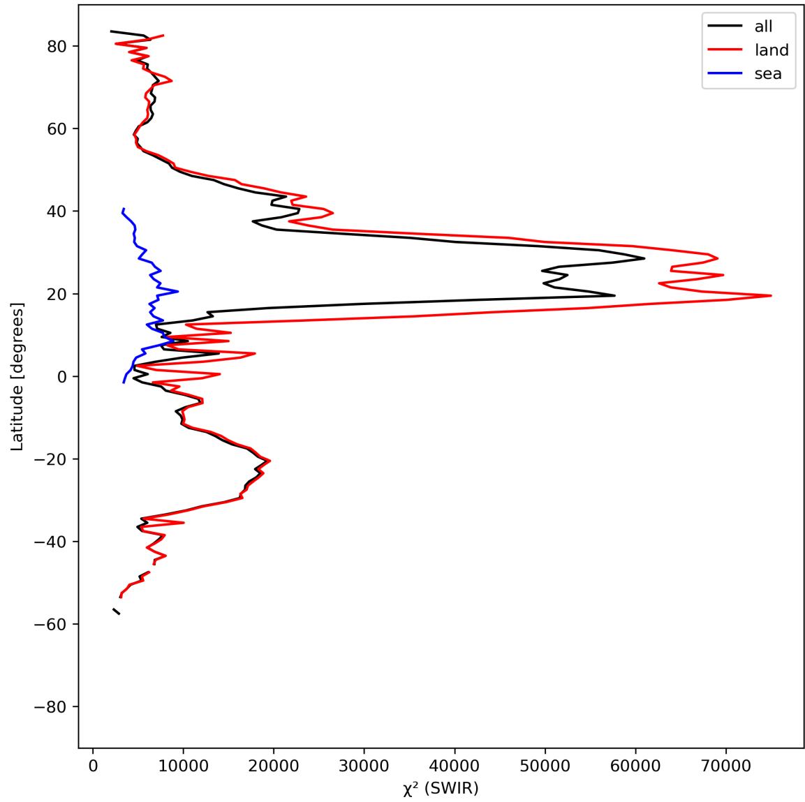
Figure 17: Zonal average of “ \chi^2 (SWIR)” for 2024-08-16 to 2024-08-17.
