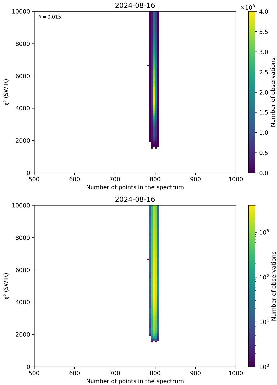
Figure 89: Scatter density plot of “Number of points in the spectrum” against “ \chi^2 (SWIR)” for 2024-08-16 to 2024-08-17.
