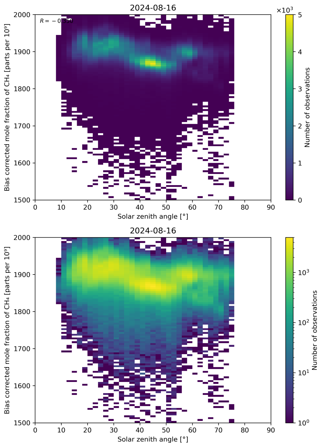
Figure 100: Scatter density plot of “Solar zenith angle” against “Bias corrected mole fraction of CH 4 ” for 2024-08-16 to 2024-08-17.
