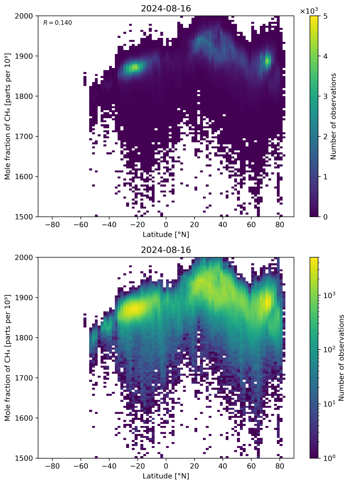
Figure 57: Scatter density plot of “Latitude” against “Mole fraction of CH 4 ” for 2024-08-16 to 2024-08-17.
