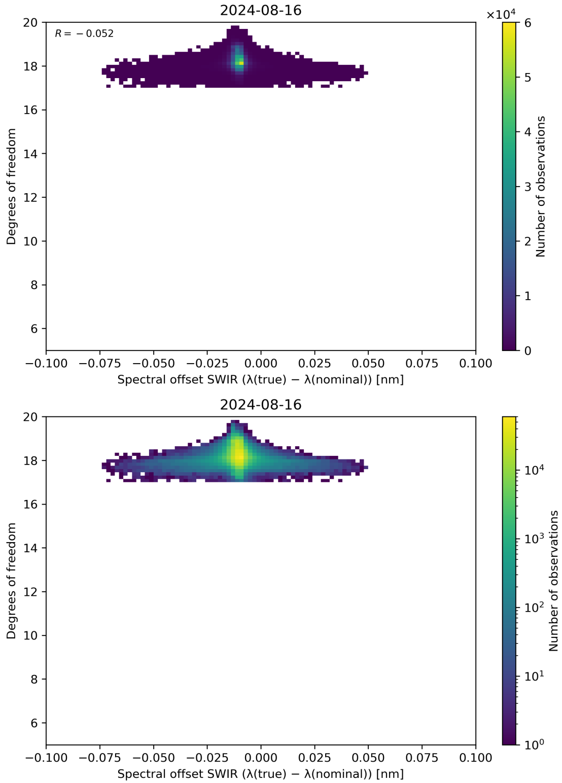
Figure 119: Scatter density plot of “Spectral offset SWIR ( \lambda(\text{true}) - \lambda(\text{nominal}) )” against “Degrees of freedom” for 2024-08-16 to 2024-08-17.
