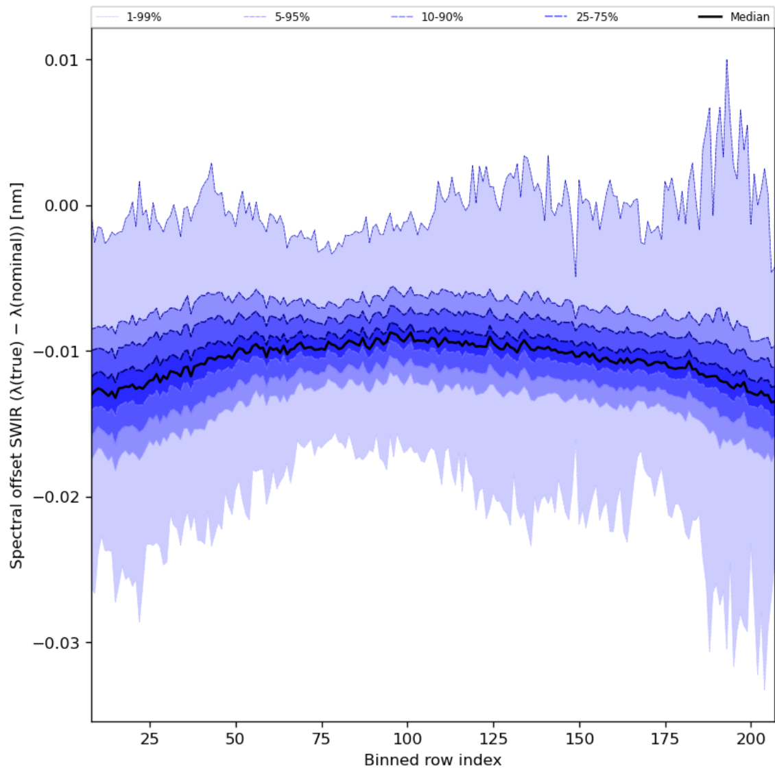
Figure 38: Along track statistics of “Spectral offset SWIR ( \lambda(\text{true}) - \lambda(\text{nominal}) )” for 2024-08-17 to 2024-08-19
