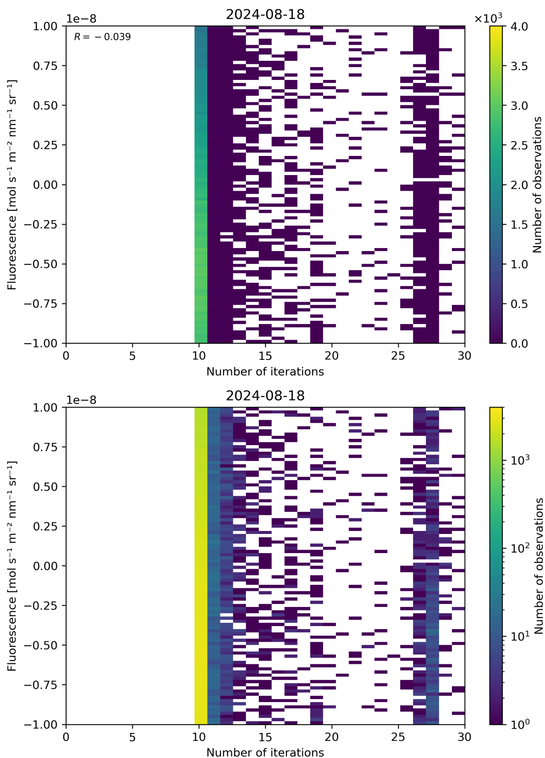
Figure 87: Scatter density plot of “Number of iterations” against “Fluorescence” for 2024-08-17 to 2024-08-19.
