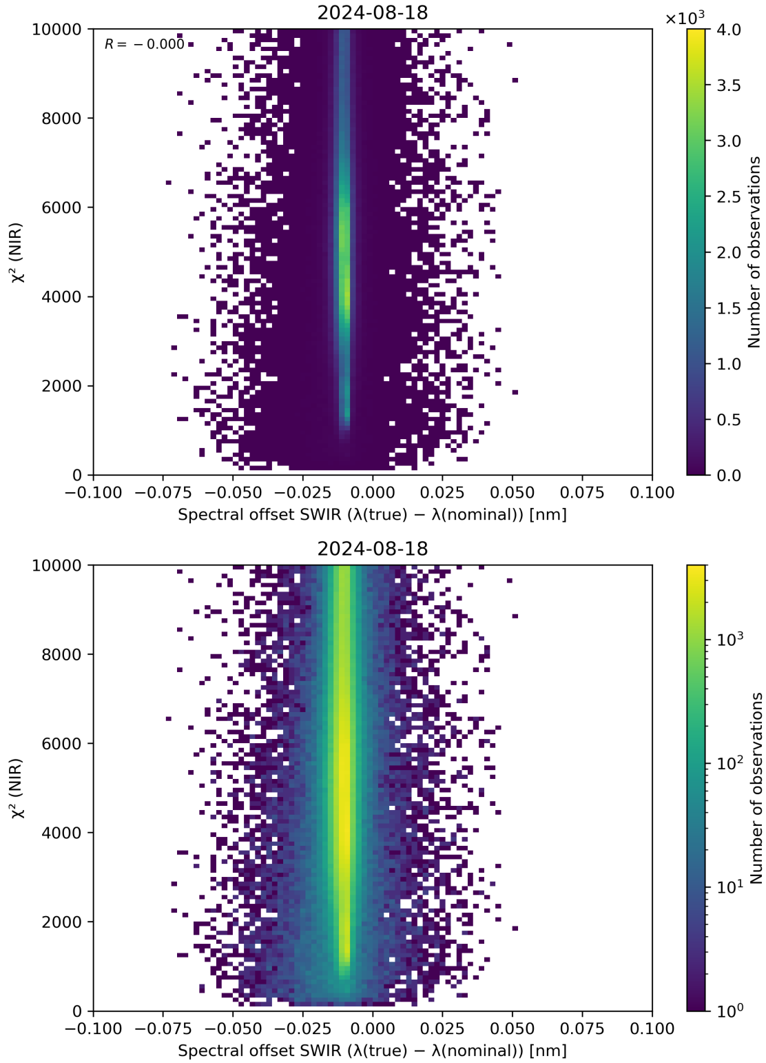
Figure 117: Scatter density plot of “Spectral offset SWIR ( \lambda(\text{true}) - \lambda(\text{nominal}) )” against “ \chi^2 (NIR)” for 2024-08-17 to 2024-08-19.
