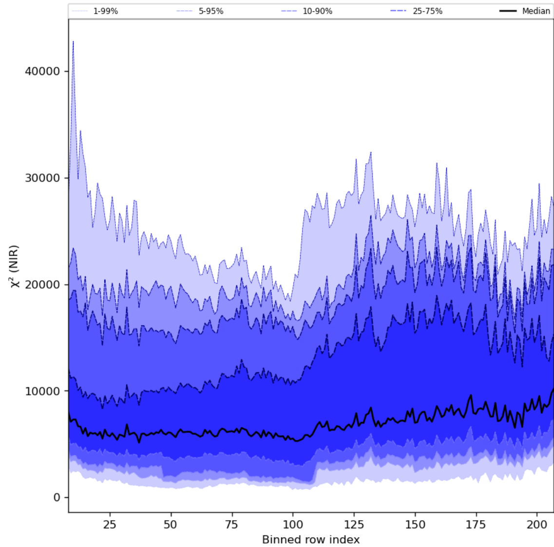
Figure 40: Along track statistics of “ \chi^2 (NIR)” for 2024-08-17 to 2024-08-19
