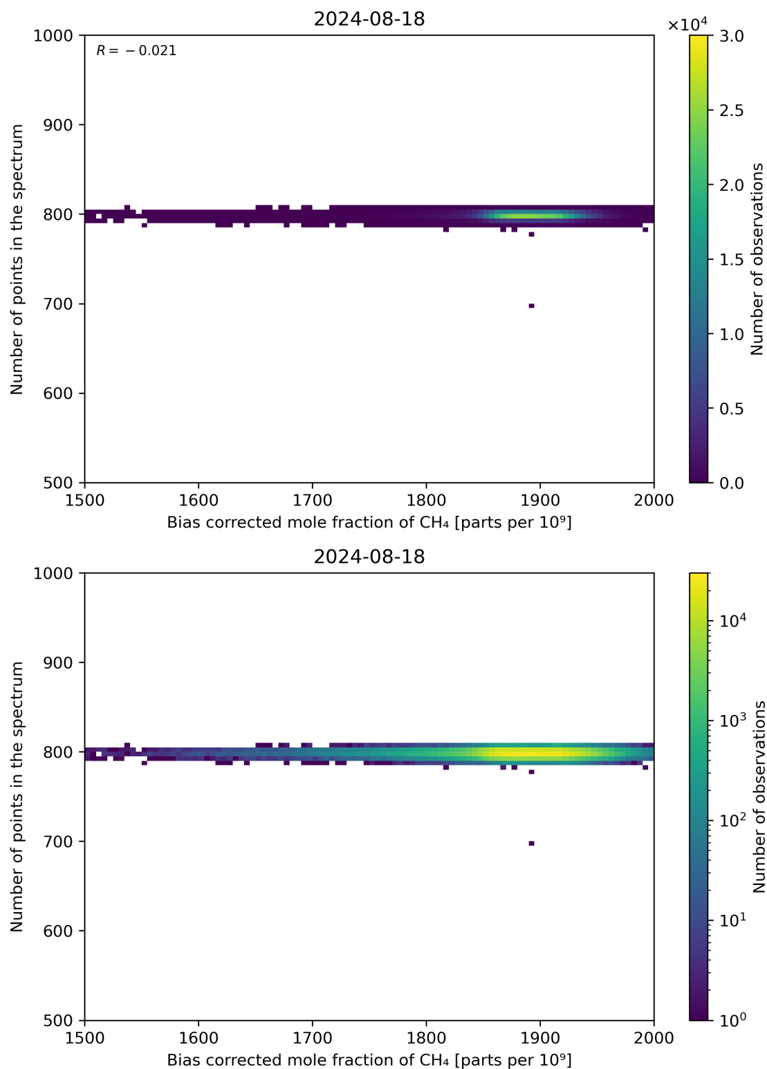
Figure 68: Scatter density plot of “Bias corrected mole fraction of CH 4 ” against “Number of points in the spectrum” for 2024-08-17 to 2024-08-19.
