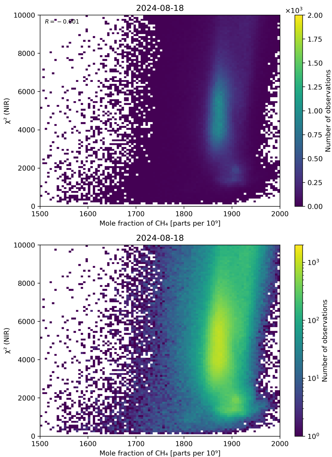
Figure 70: Scatter density plot of “Mole fraction of \text{CH}_4 ” against “ \chi^2 (NIR)” for 2024-08-17 to 2024-08-19.
