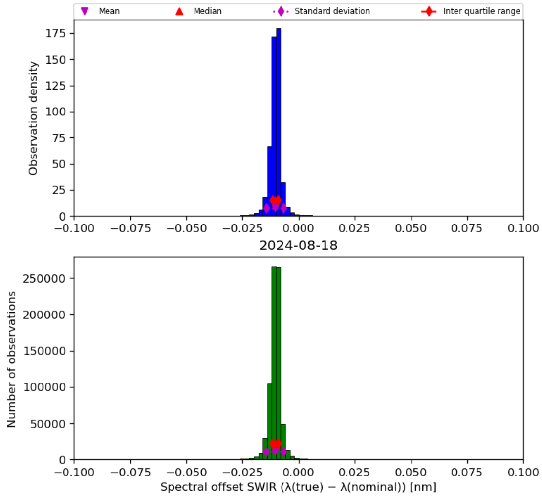
Figure 27: Histogram of “Spectral offset SWIR ( \lambda(\text{true}) - \lambda(\text{nominal}) )” for 2024-08-17 to 2024-08-19
