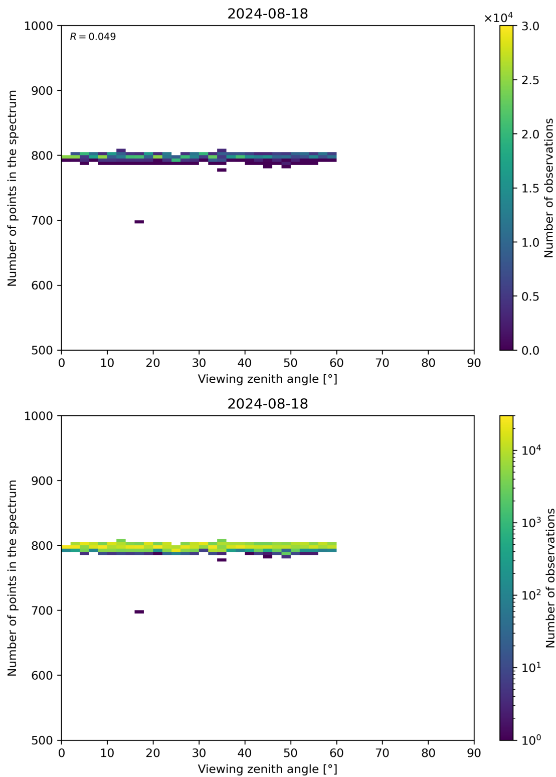
Figure 114: Scatter density plot of “Viewing zenith angle” against “Number of points in the spectrum” for 2024-08-17 to 2024-08-19.
