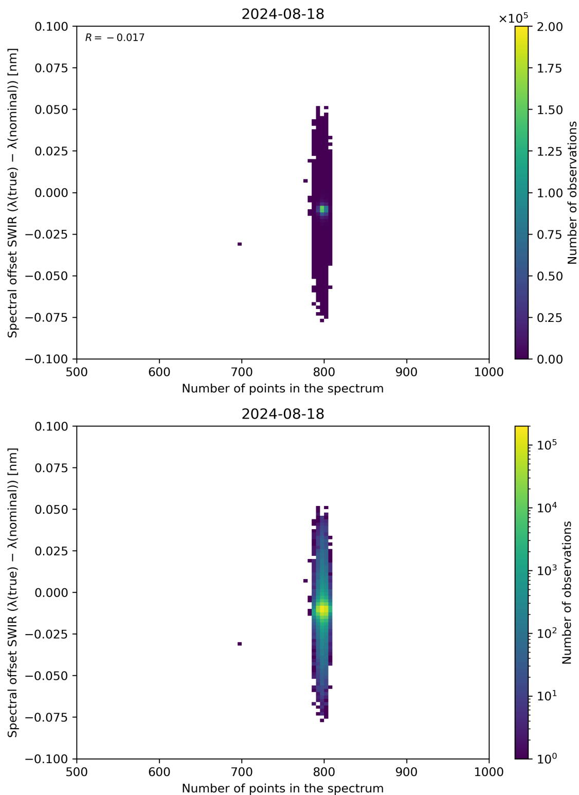
Figure 93: Scatter density plot of “Number of points in the spectrum” against “Spectral offset SWIR ( \lambda(\text{true}) - \lambda(\text{nominal}) )” for 2024-08-17 to 2024-08-19.
