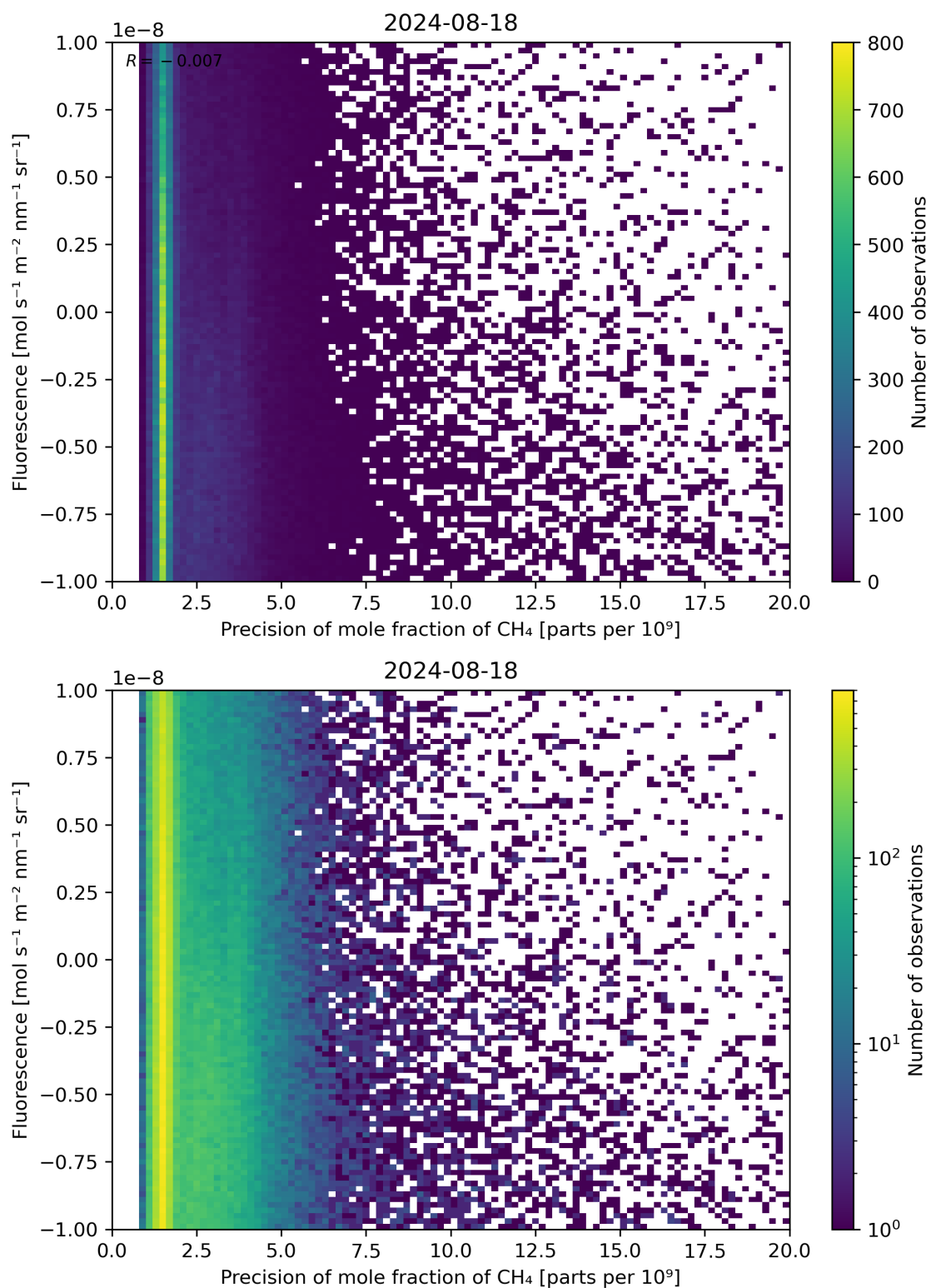
Figure 81: Scatter density plot of “Precision of mole fraction of \text{CH}_4 ” against “Fluorescence” for 2024-08-17 to 2024-08-19.
