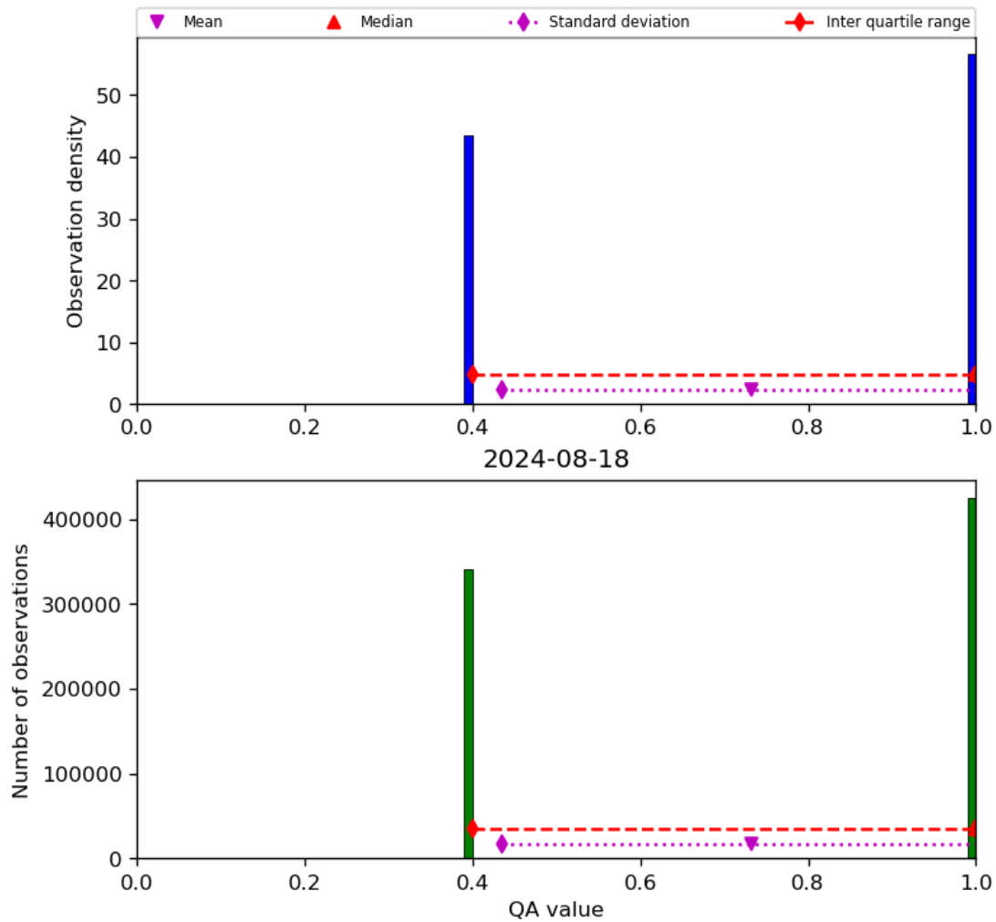
Figure 22: Histogram of “QA value” for 2024-08-17 to 2024-08-19
