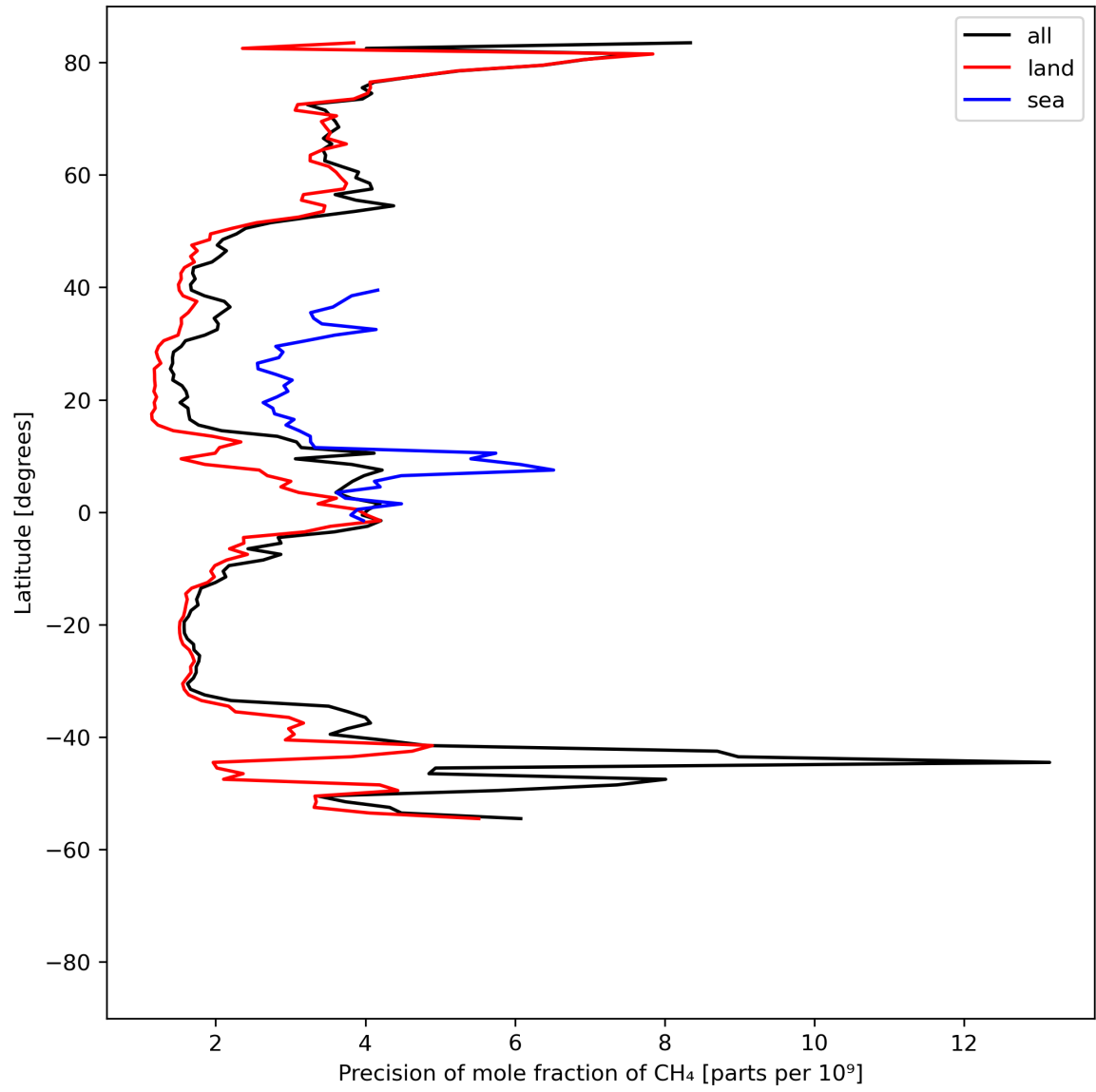
Figure 13: Zonal average of “Precision of mole fraction of CH 4 ” for 2024-08-17 to 2024-08-19.
