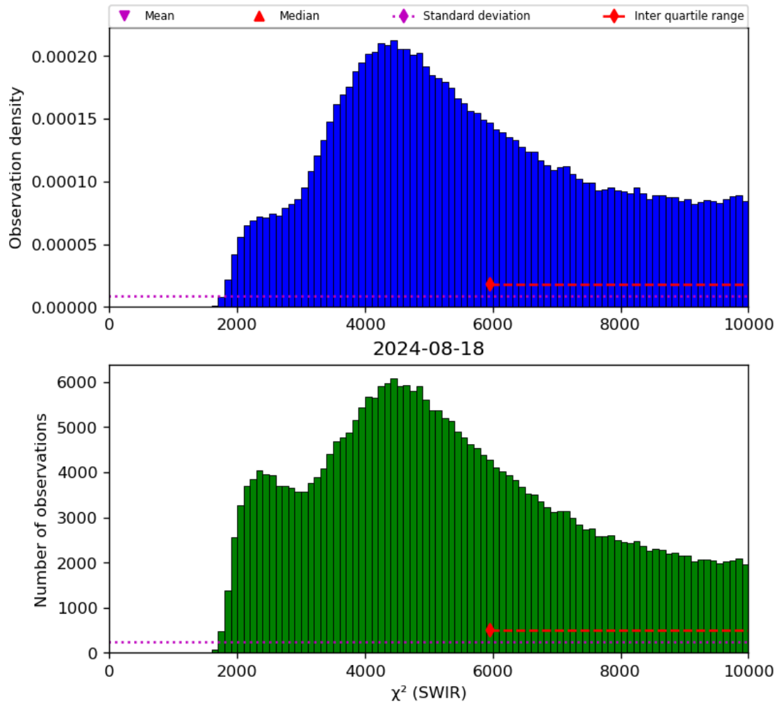
Figure 28: Histogram of “ \chi^2 (SWIR)” for 2024-08-17 to 2024-08-19
