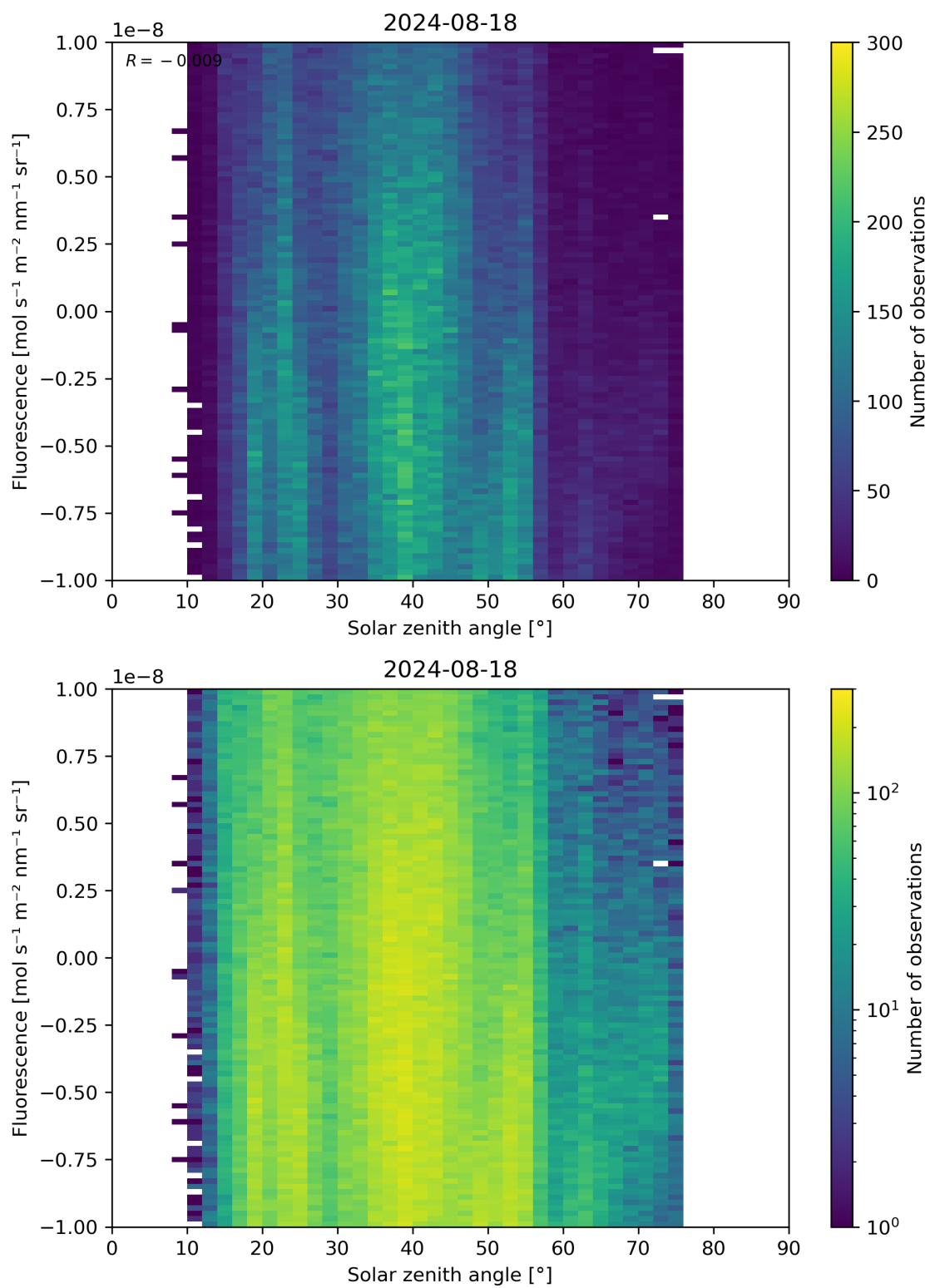
Figure 97: Scatter density plot of “Solar zenith angle” against “Fluorescence” for 2024-08-17 to 2024-08-19.
