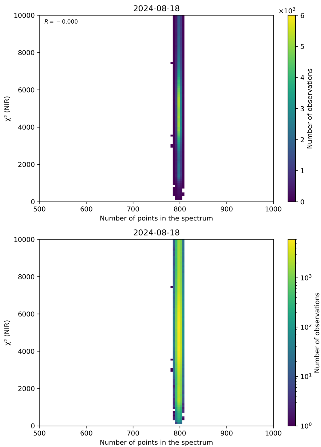
Figure 88: Scatter density plot of “Number of points in the spectrum” against “ \chi^2 (NIR)” for 2024-08-17 to 2024-08-19.
