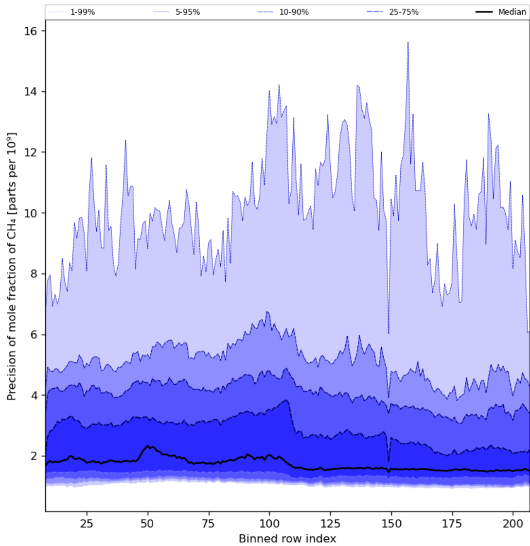
Figure 35: Along track statistics of “Precision of mole fraction of CH 4 ” for 2024-08-17 to 2024-08-19
