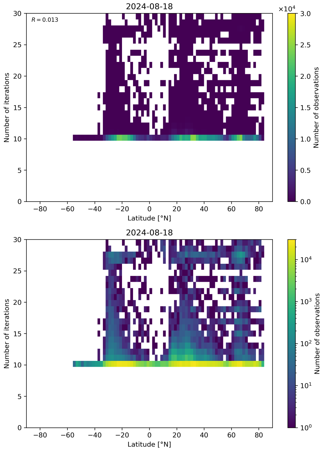
Figure 60: Scatter density plot of “Latitude” against “Number of iterations” for 2024-08-17 to 2024-08-19.
