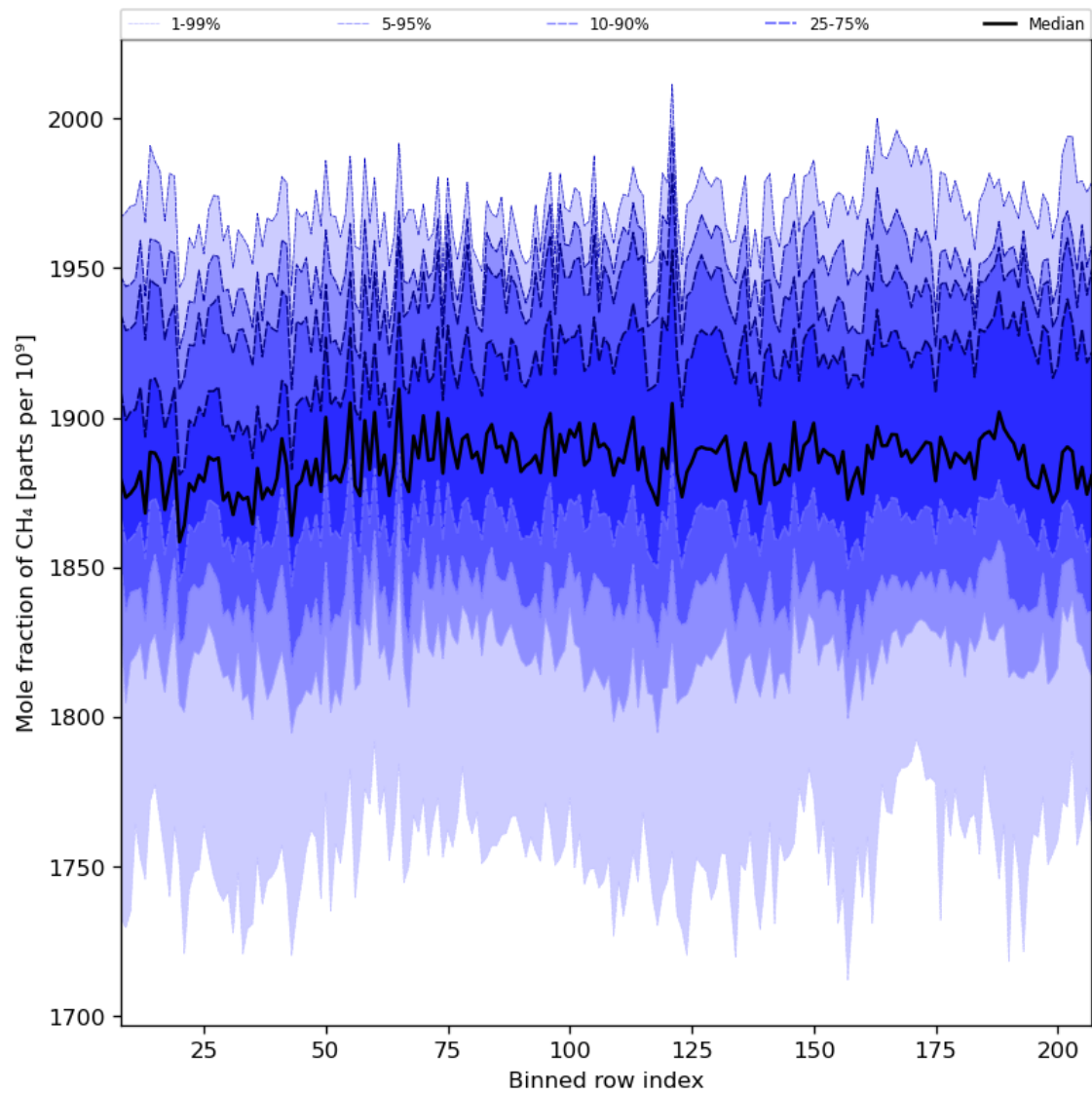
Figure 34: Along track statistics of “Mole fraction of CH 4 ” for 2024-08-17 to 2024-08-19
