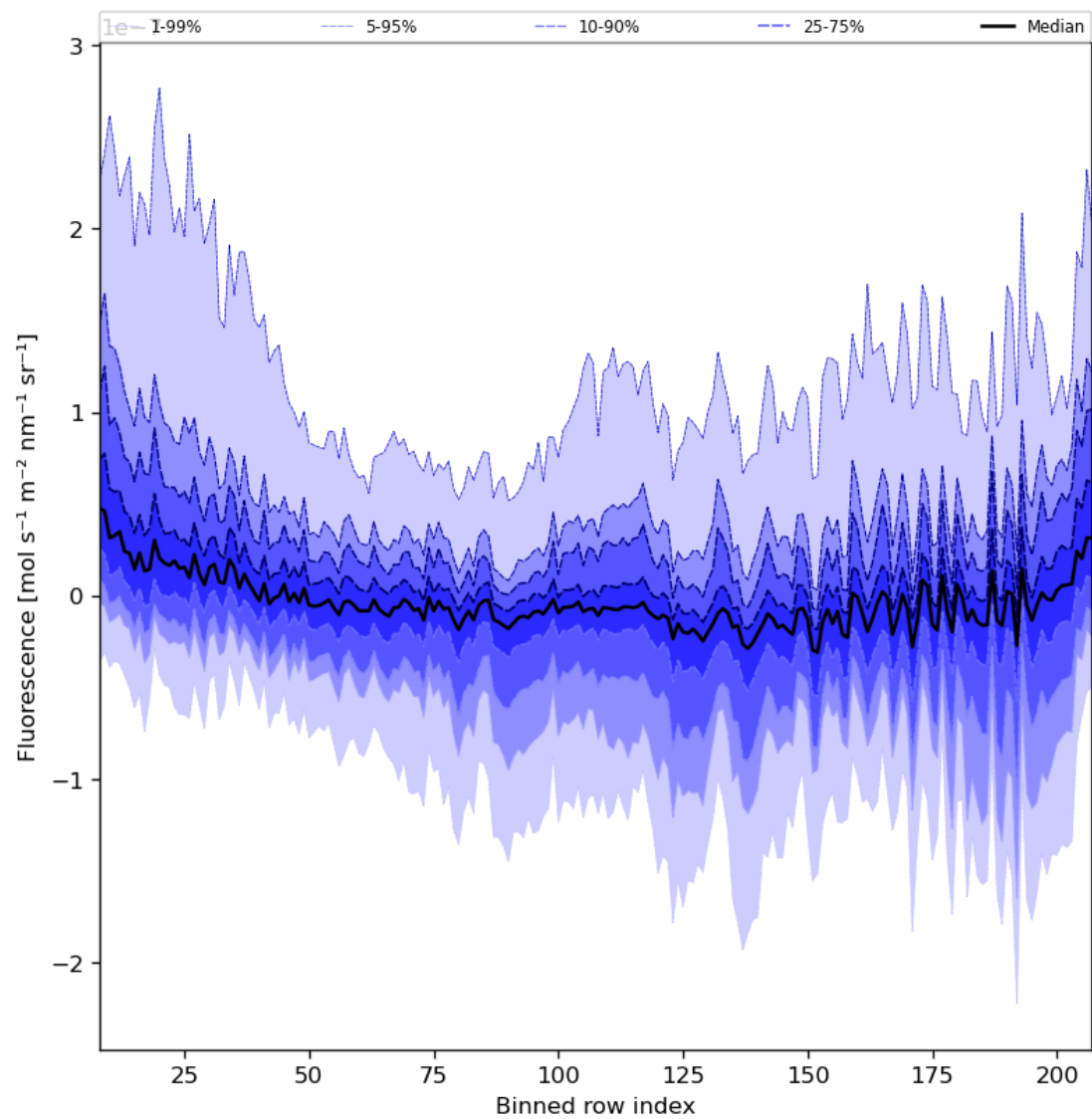
Figure 43: Along track statistics of “Fluorescence” for 2024-08-17 to 2024-08-19
