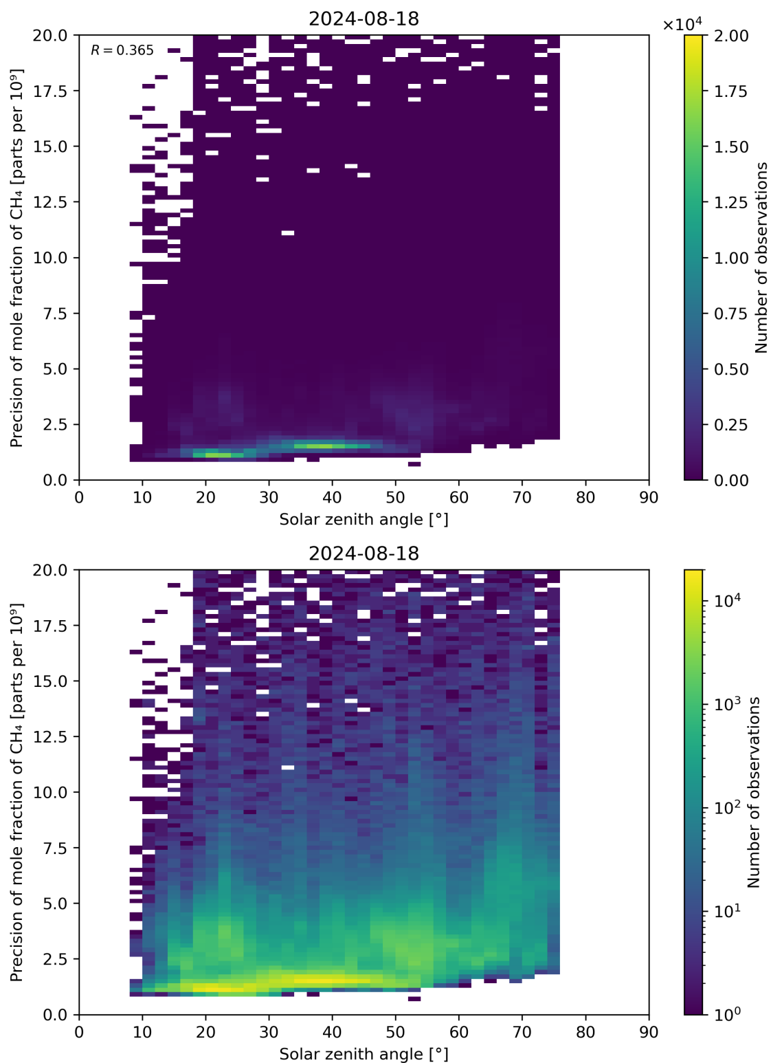
Figure 101: Scatter density plot of “Solar zenith angle” against “Precision of mole fraction of \text{CH}_4 ” for 2024-08-17 to 2024-08-19.
