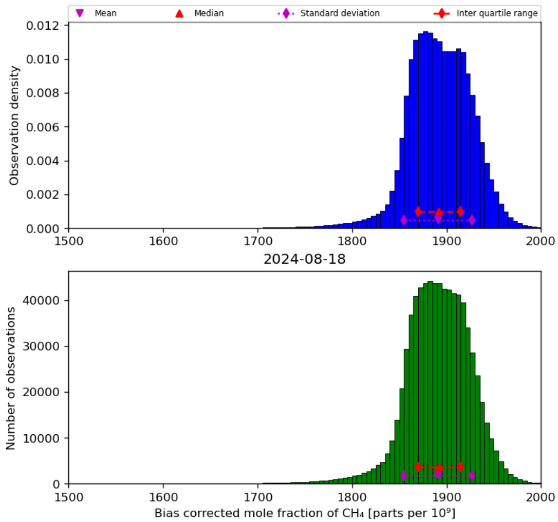
Figure 25: Histogram of “Bias corrected mole fraction of CH 4 ” for 2024-08-17 to 2024-08-19
