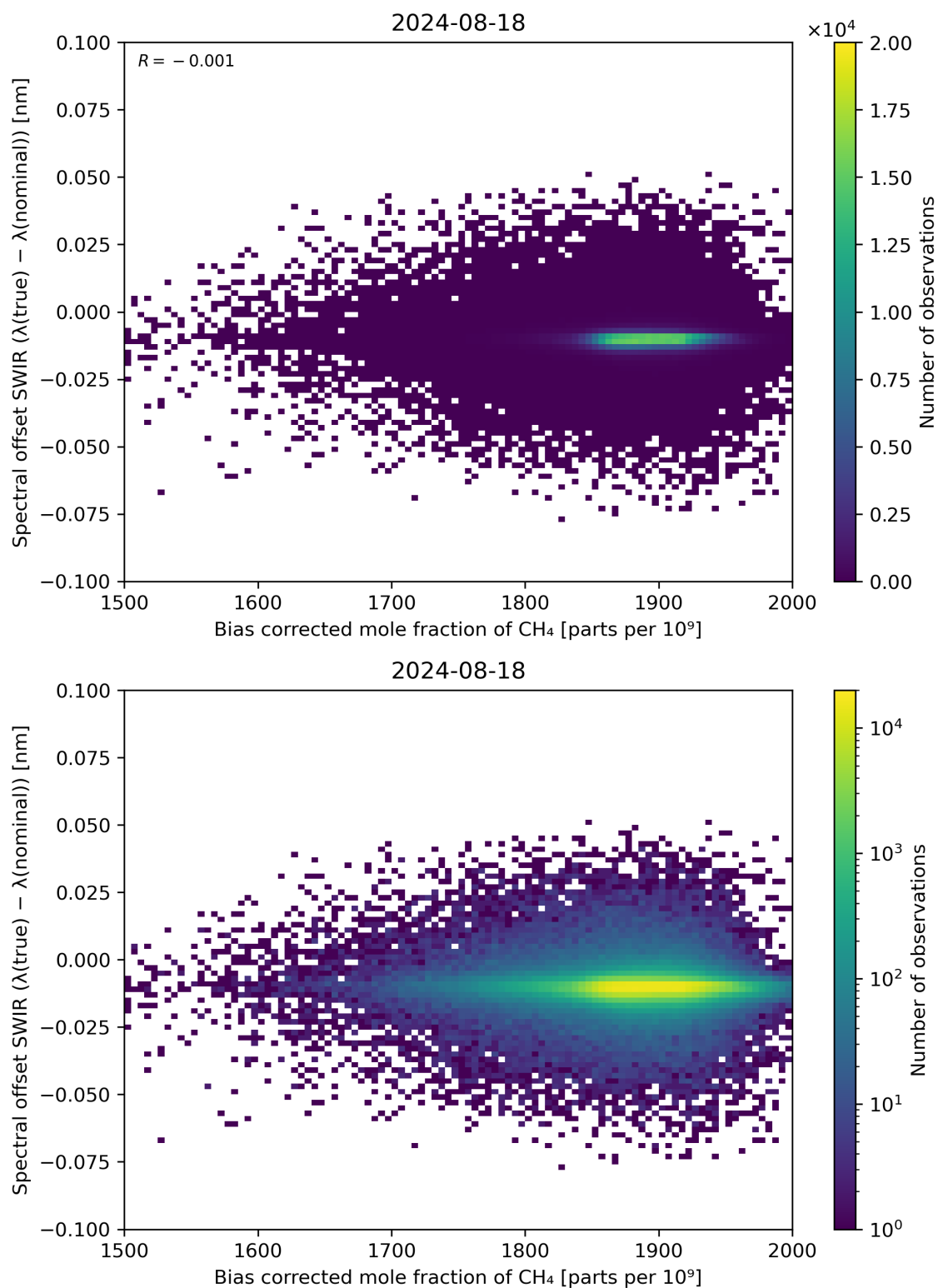
Figure 69: Scatter density plot of “Bias corrected mole fraction of \text{CH}_4 ” against “Spectral offset SWIR ( \lambda(\text{true}) - \lambda(\text{nominal}) )” for 2024-08-17 to 2024-08-19.
