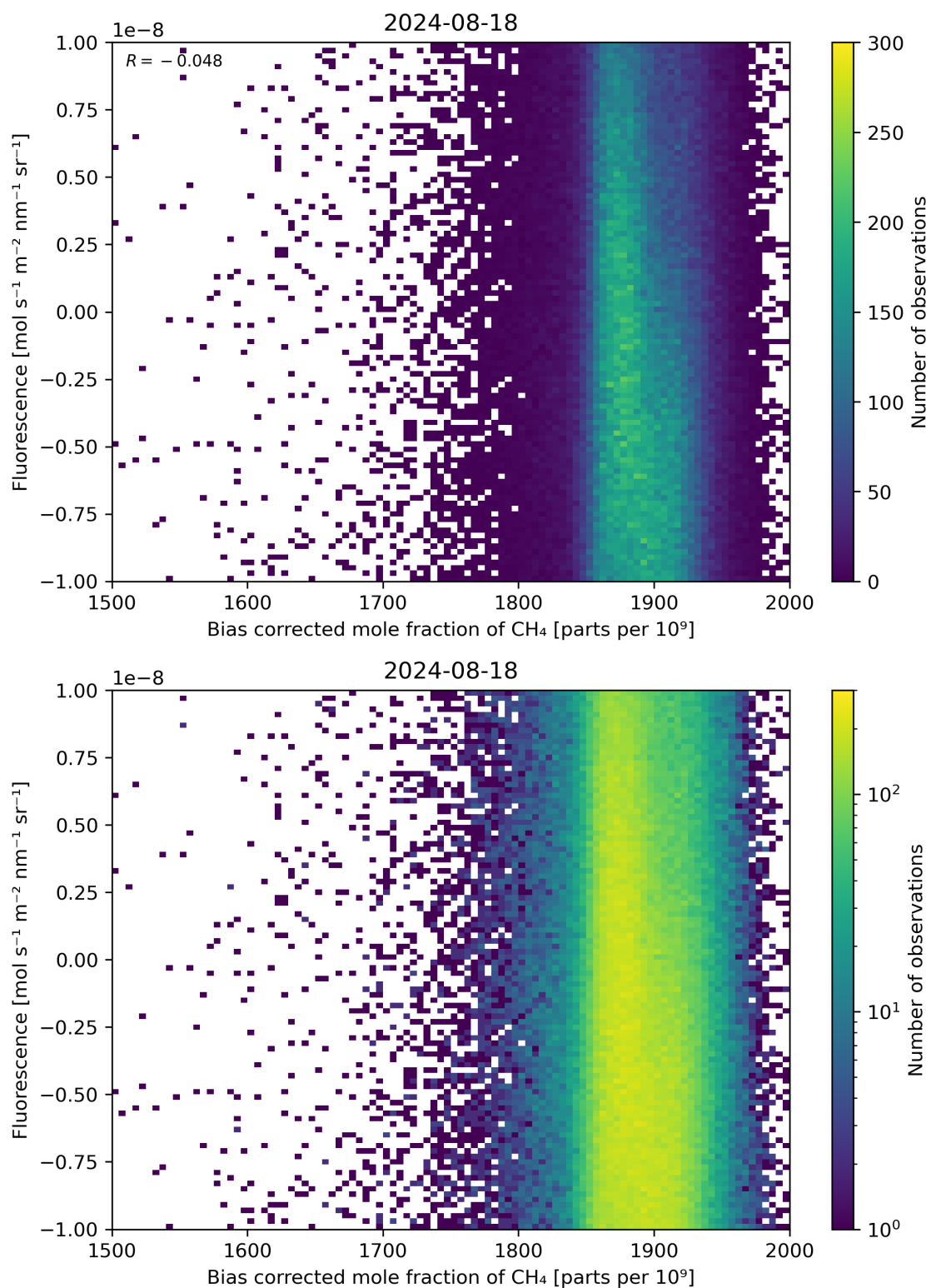
Figure 66: Scatter density plot of “Bias corrected mole fraction of \text{CH}_4 ” against “Fluorescence” for 2024-08-17 to 2024-08-19.
