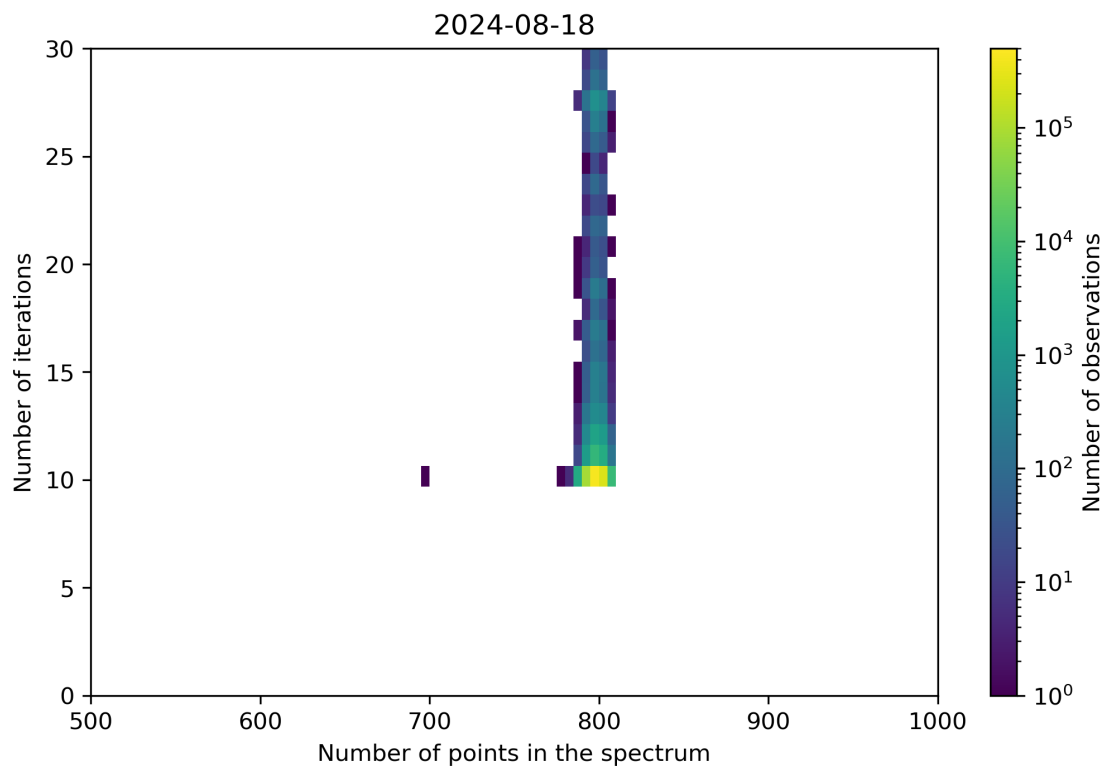
Figure 92: Scatter density plot of “Number of points in the spectrum” against “Number of iterations” for 2024-08-17 to 2024-08-19.
