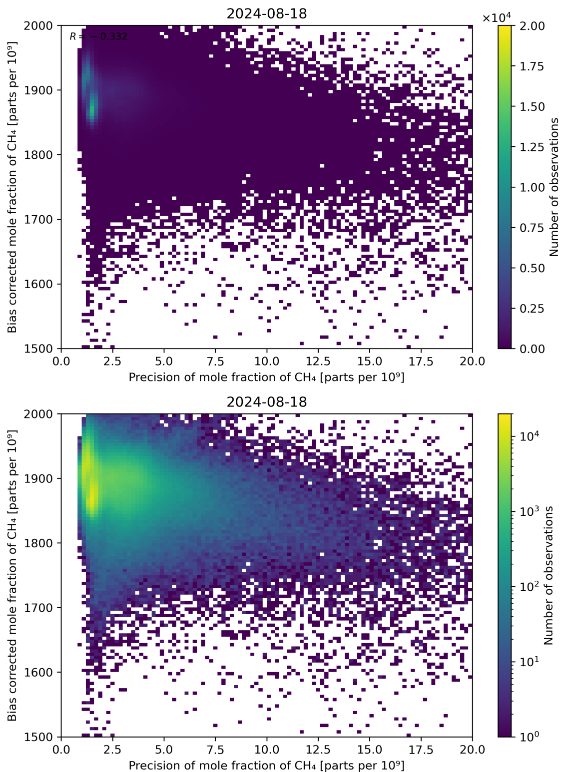
Figure 82: Scatter density plot of “Precision of mole fraction of CH 4 ” against “Bias corrected mole fraction of CH 4 ” for 2024-08-17 to 2024-08-19.
