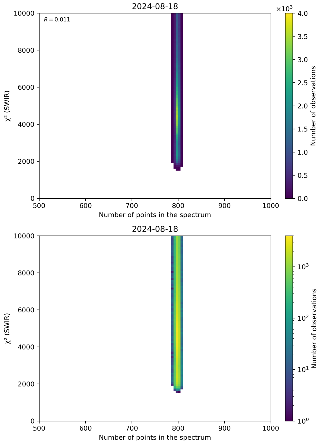
Figure 89: Scatter density plot of “Number of points in the spectrum” against “ \chi^2 (SWIR)” for 2024-08-17 to 2024-08-19.
