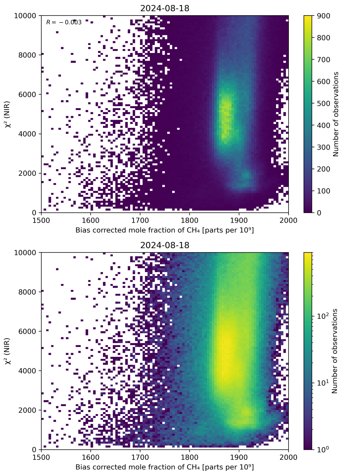
Figure 63: Scatter density plot of “Bias corrected mole fraction of CH 4 ” against “ \chi^2 (NIR)” for 2024-08-17 to 2024-08-19.
