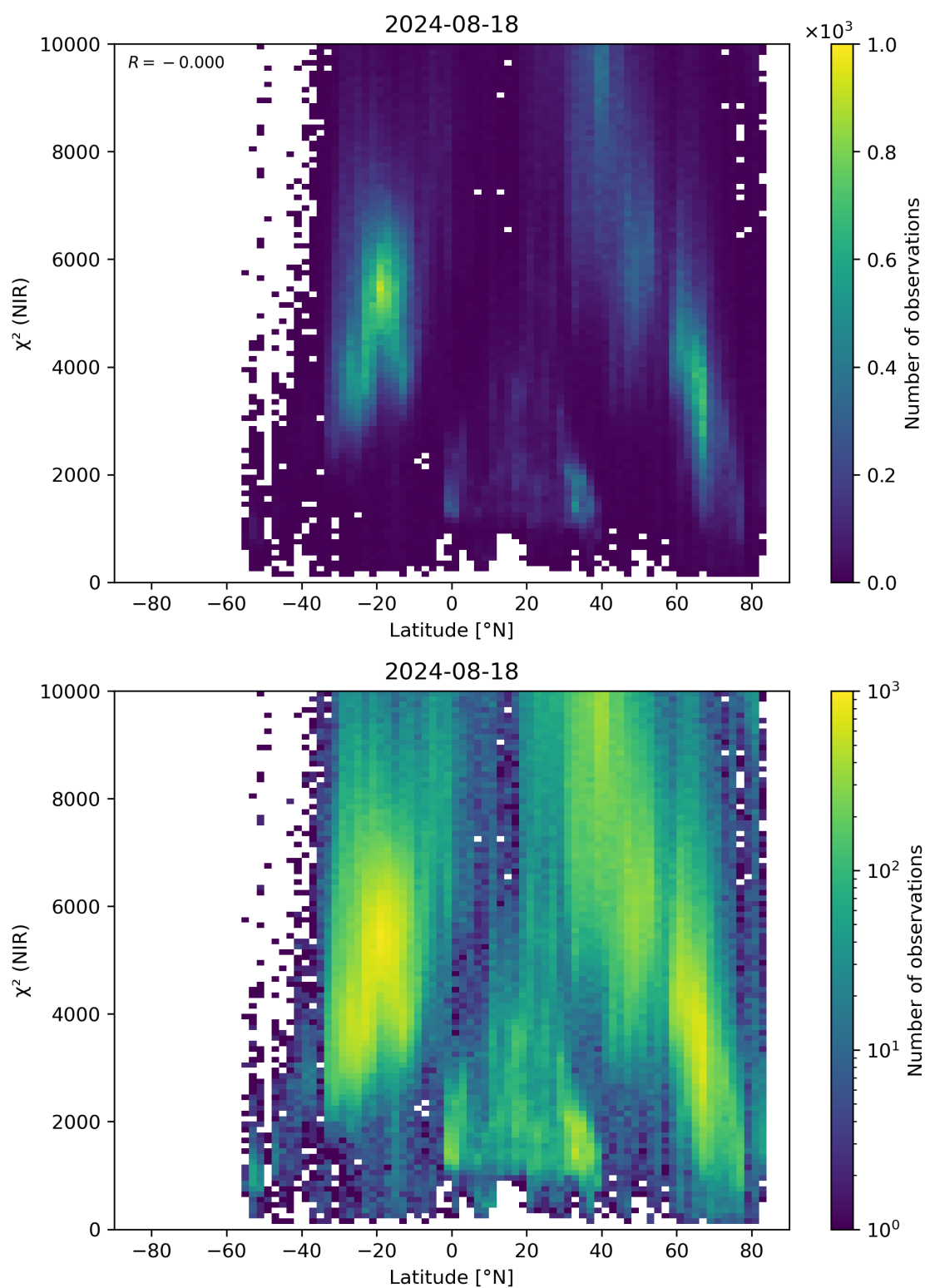
Figure 53: Scatter density plot of “Latitude” against “ \chi^2 (NIR)” for 2024-08-17 to 2024-08-19.
