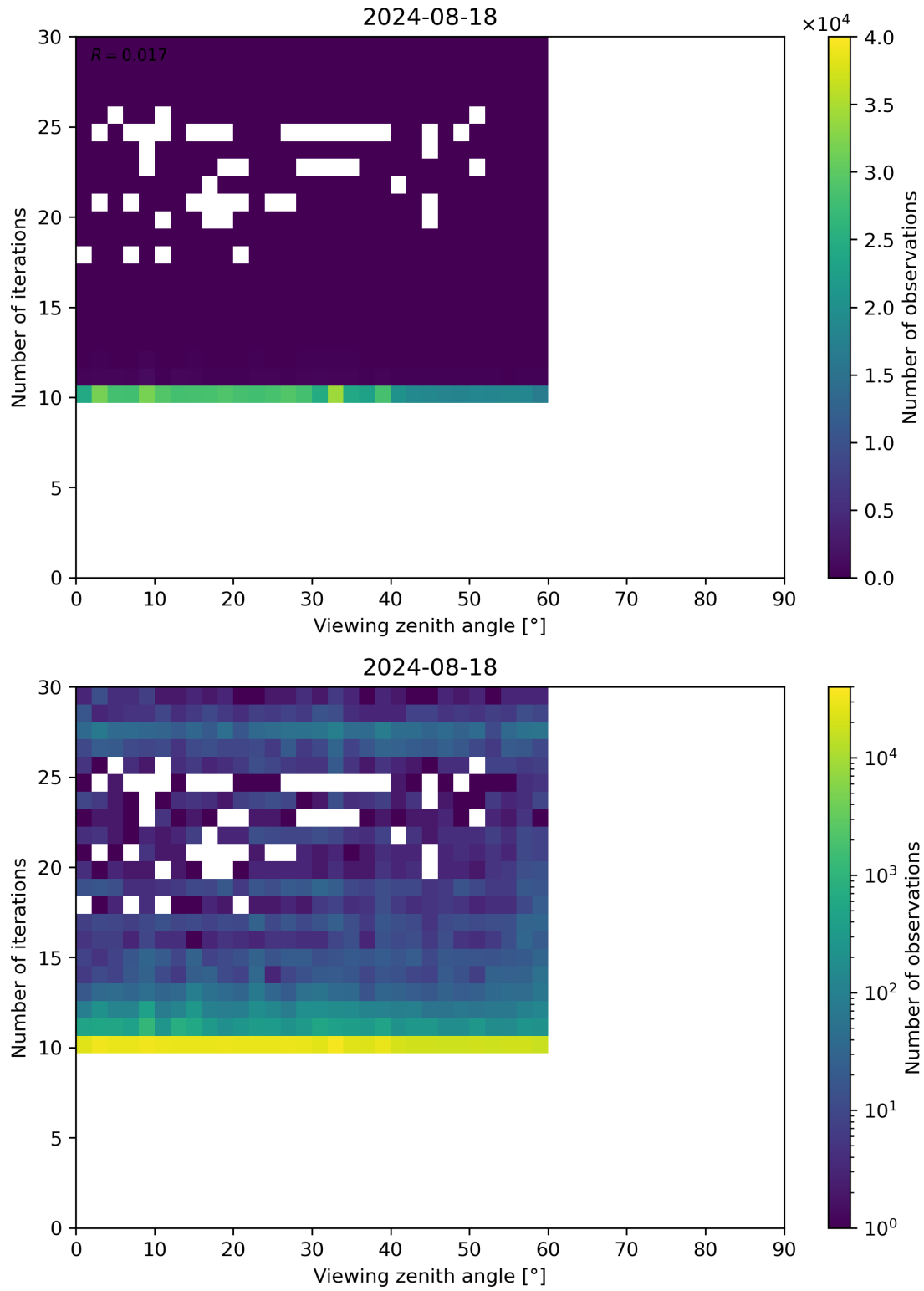
Figure 113: Scatter density plot of “Viewing zenith angle” against “Number of iterations” for 2024-08-17 to 2024-08-19.
