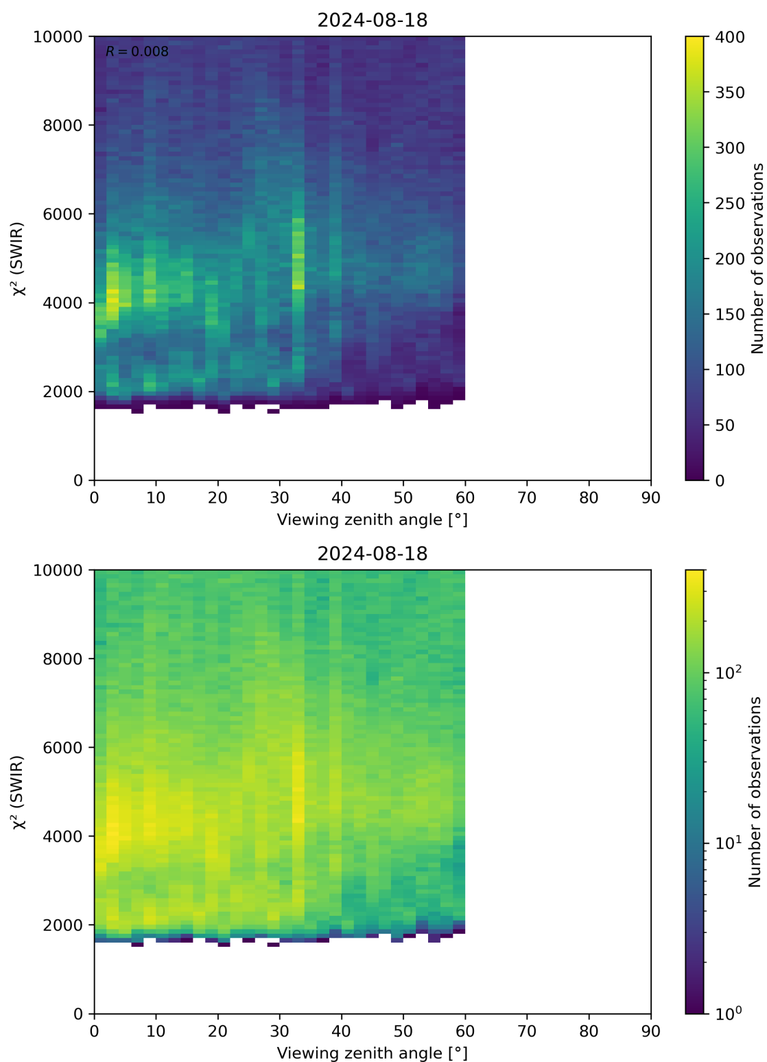
Figure 106: Scatter density plot of “Viewing zenith angle” against “ \chi^2 (SWIR)” for 2024-08-17 to 2024-08-19.
