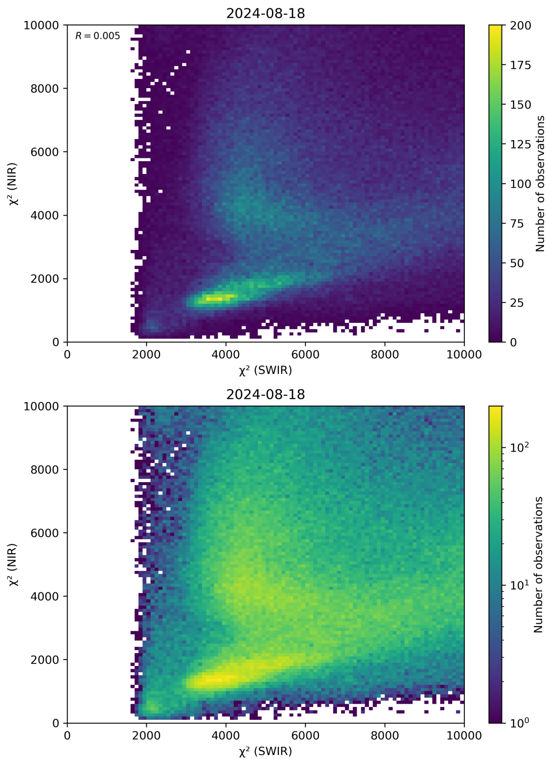
Figure 47: Scatter density plot of “ \chi^2 (SWIR)” against “ \chi^2 (NIR)” for 2024-08-17 to 2024-08-19.
