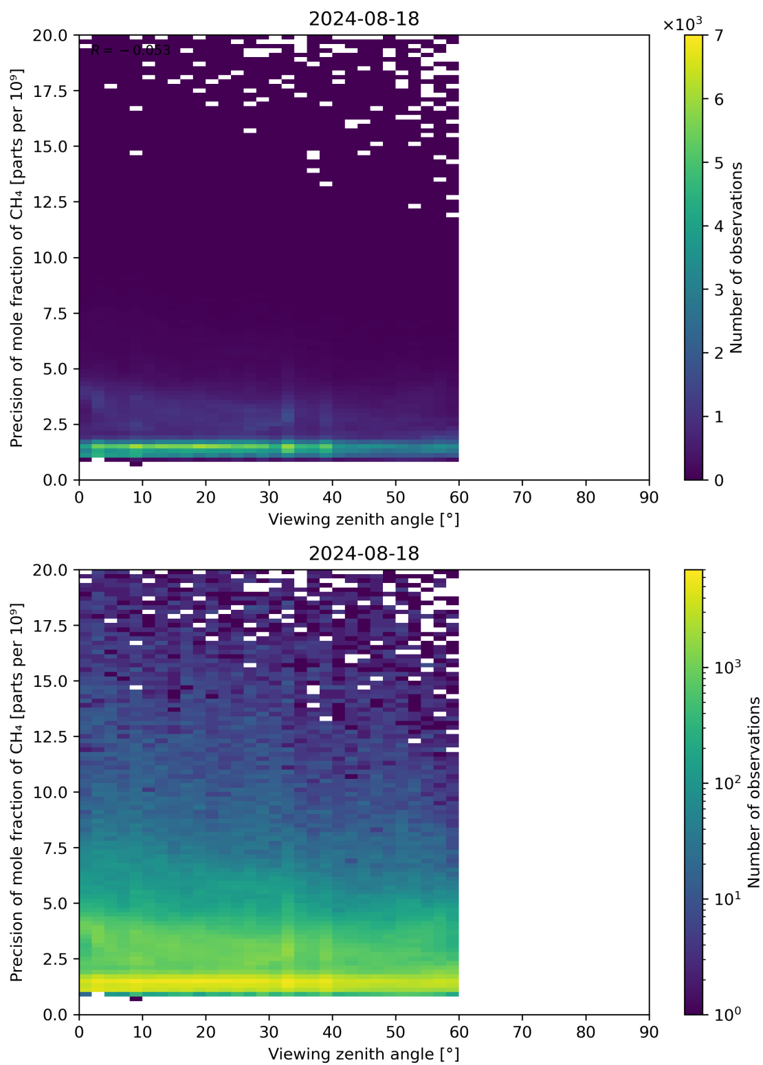
Figure 112: Scatter density plot of “Viewing zenith angle” against “Precision of mole fraction of CH 4 ” for 2024-08-17 to 2024-08-19.
