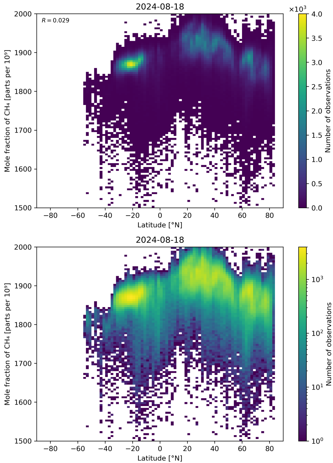
Figure 57: Scatter density plot of “Latitude” against “Mole fraction of \text{CH}_4 ” for 2024-08-17 to 2024-08-19.
