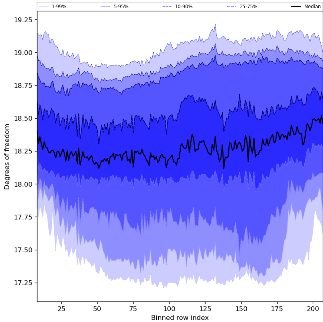
Figure 41: Along track statistics of “Degrees of freedom” for 2024-08-17 to 2024-08-19
