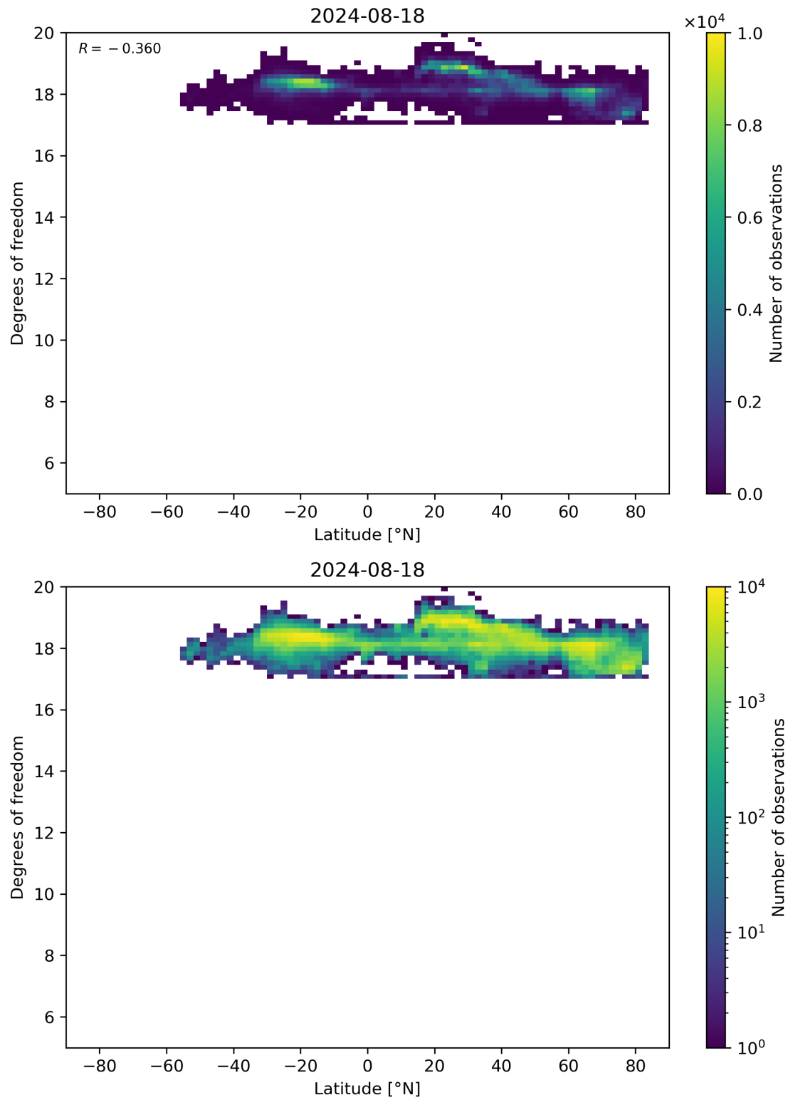
Figure 55: Scatter density plot of “Latitude” against “Degrees of freedom” for 2024-08-17 to 2024-08-19.
