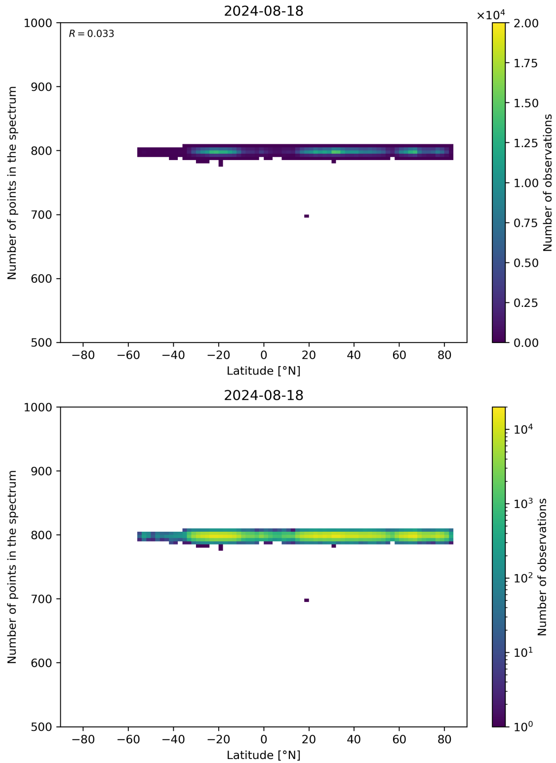
Figure 61: Scatter density plot of “Latitude” against “Number of points in the spectrum” for 2024-08-17 to 2024-08-19.
