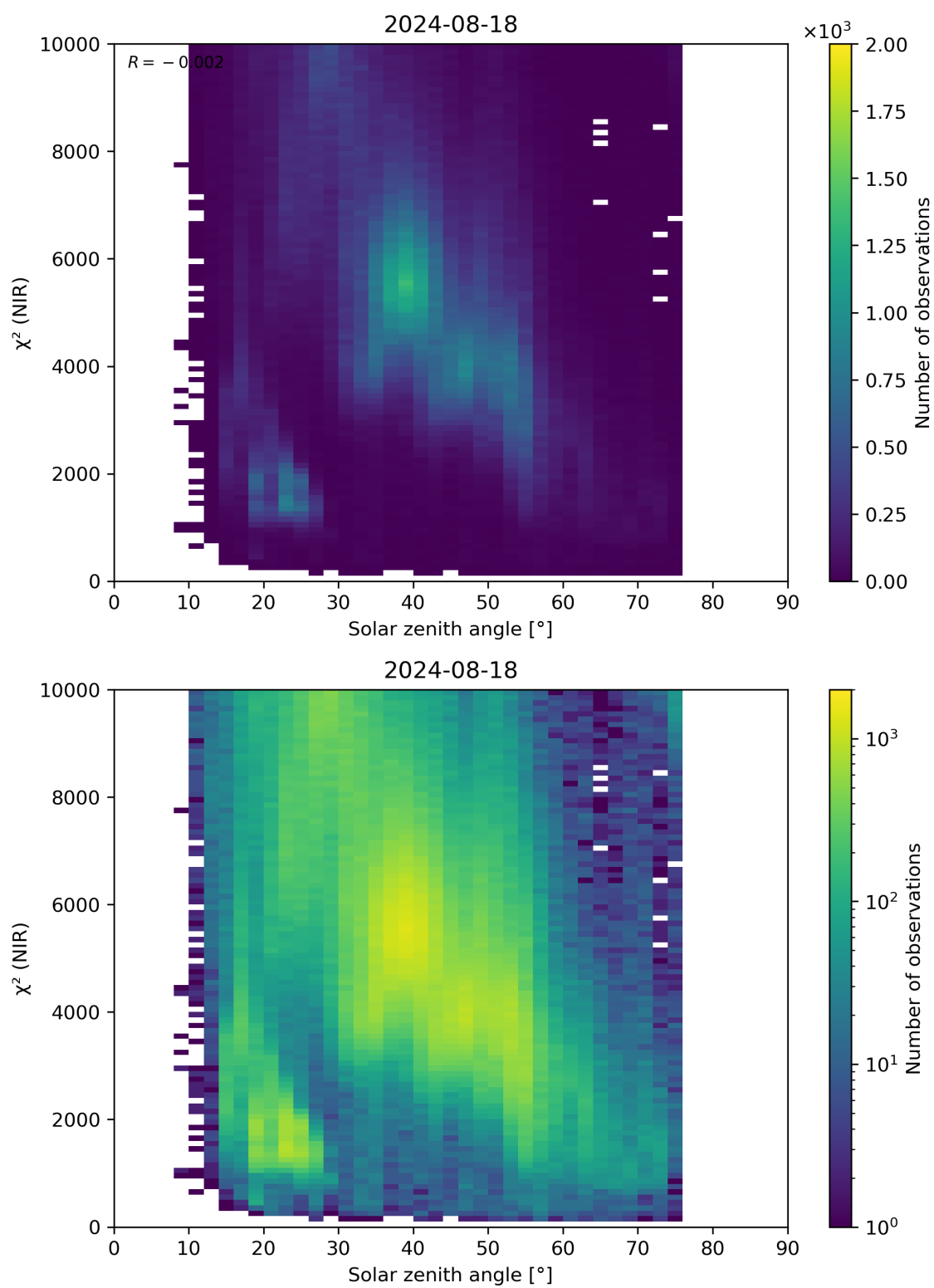
Figure 94: Scatter density plot of “Solar zenith angle” against “ \chi^2 (NIR)” for 2024-08-17 to 2024-08-19.
