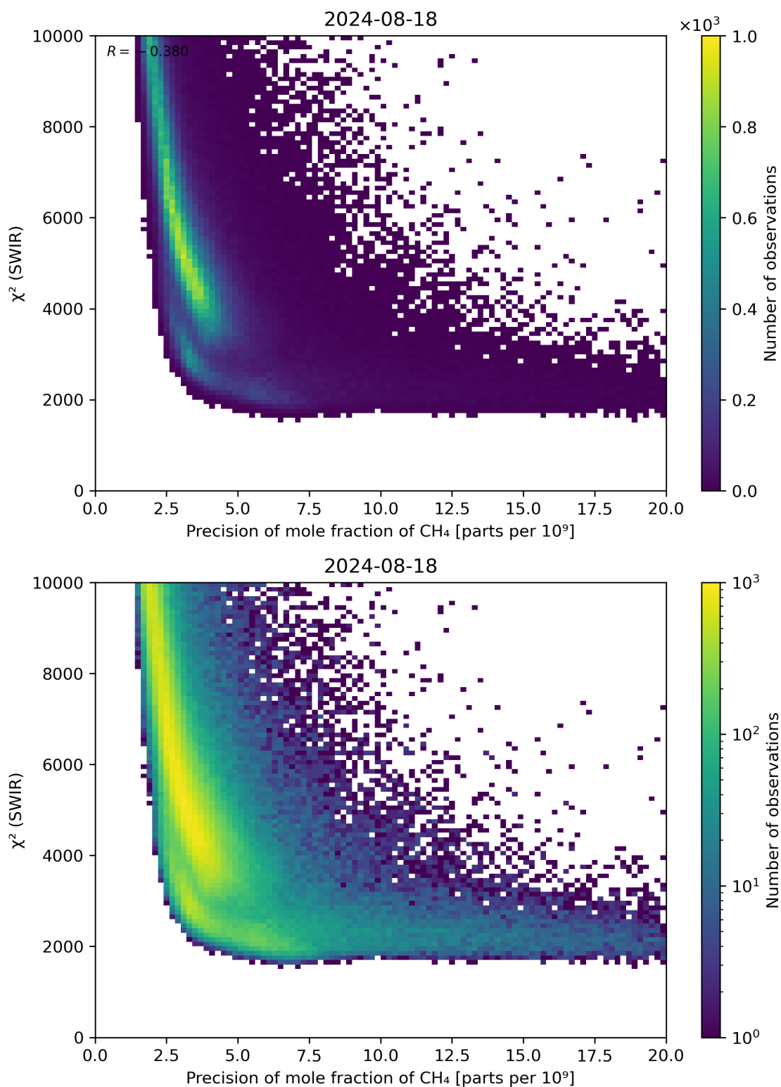
Figure 79: Scatter density plot of “Precision of mole fraction of \text{CH}_4 ” against “ \chi^2 (SWIR)” for 2024-08-17 to 2024-08-19.
