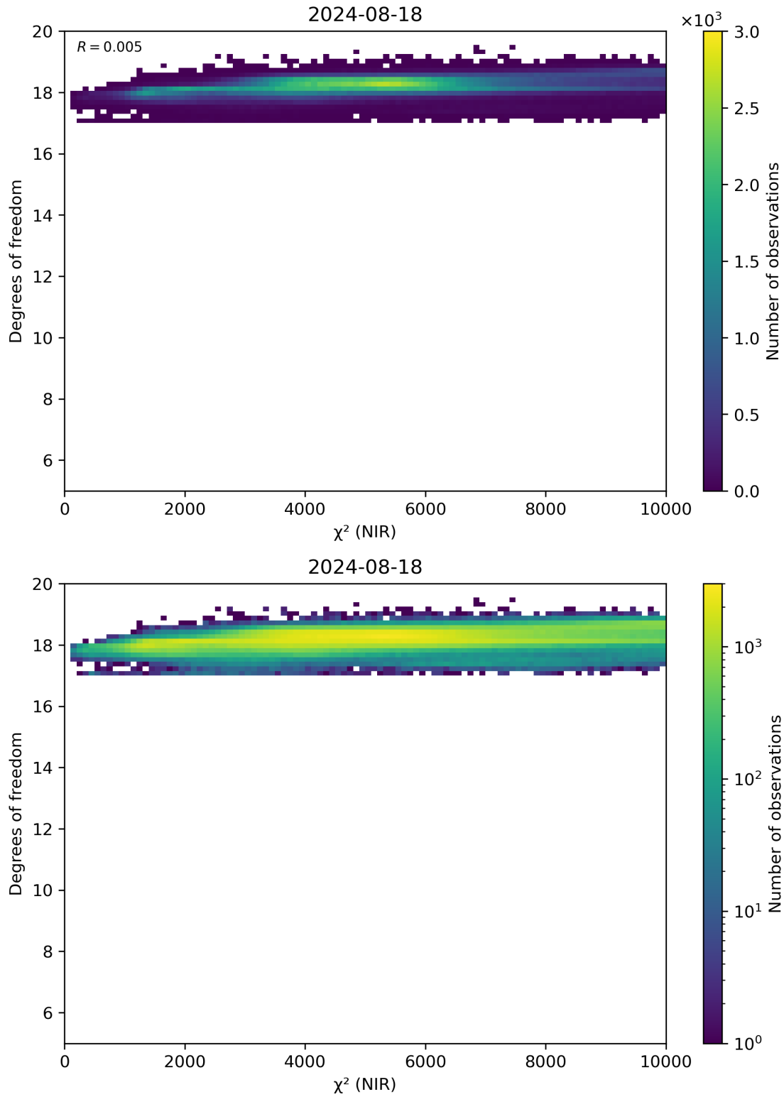
Figure 44: Scatter density plot of “ \chi^2 (NIR)” against “Degrees of freedom” for 2024-08-17 to 2024-08-19.
