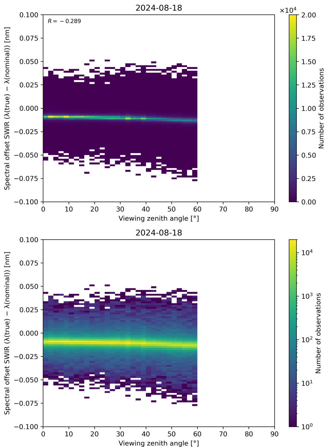
Figure 116: Scatter density plot of “Viewing zenith angle” against “Spectral offset SWIR ( \lambda(\text{true}) - \lambda(\text{nominal}) )” for 2024-08-17 to 2024-08-19.
