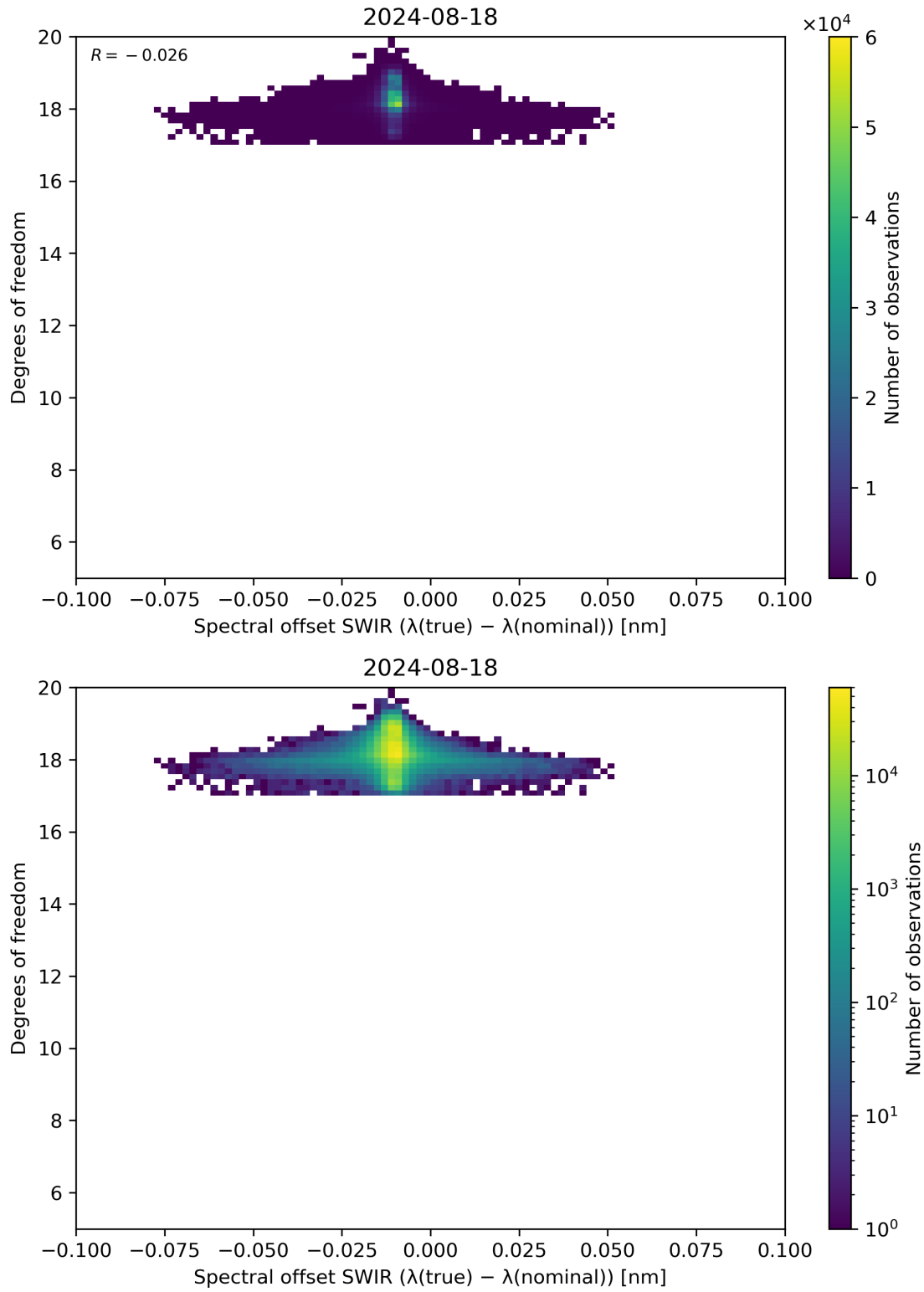
Figure 119: Scatter density plot of “Spectral offset SWIR ( \lambda(\text{true}) - \lambda(\text{nominal}) )” against “Degrees of freedom” for 2024-08-17 to 2024-08-19.
