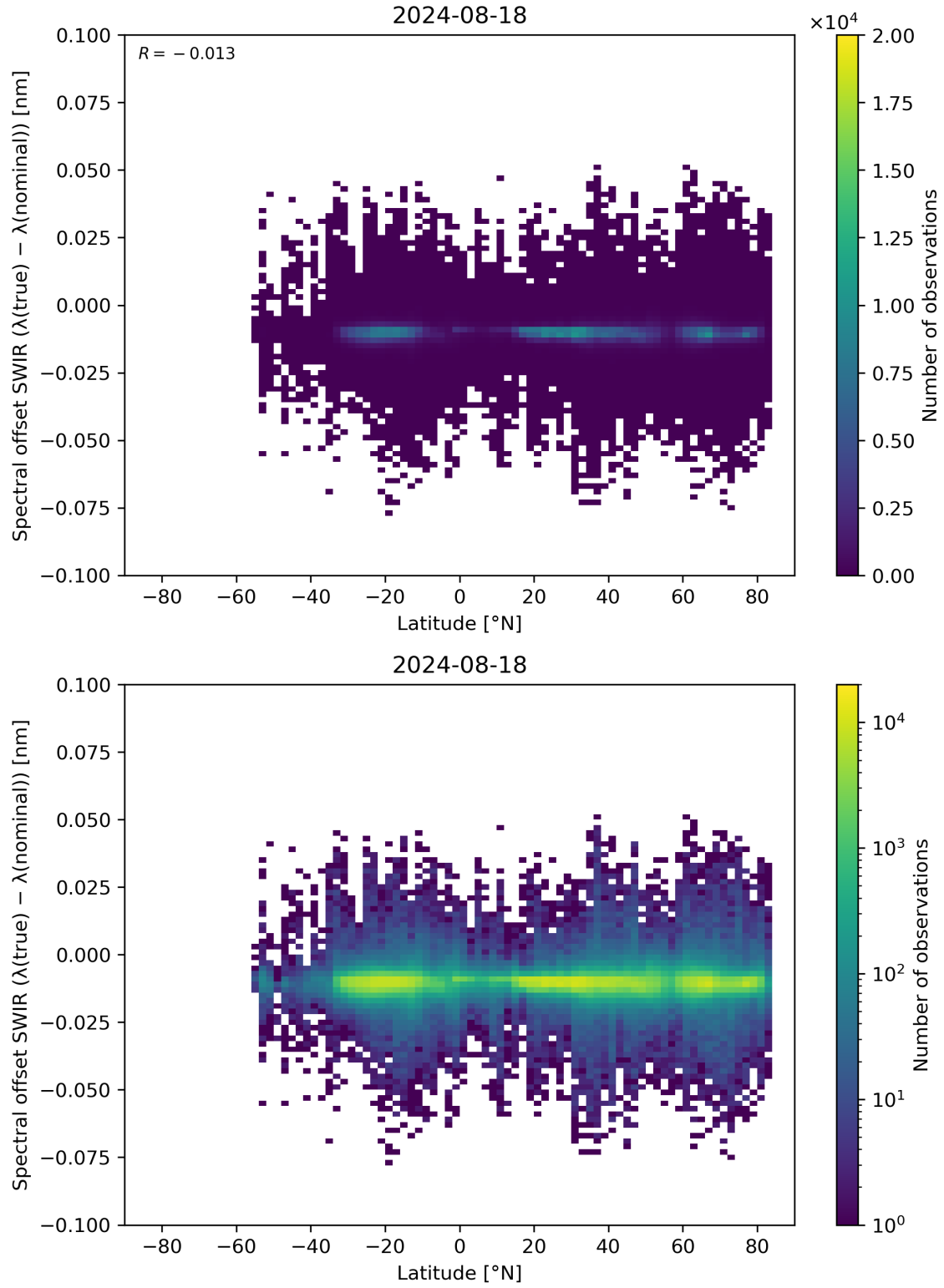
Figure 62: Scatter density plot of “Latitude” against “Spectral offset SWIR ( \lambda(\text{true}) - \lambda(\text{nominal}) )” for 2024-08-17 to 2024-08-19.
