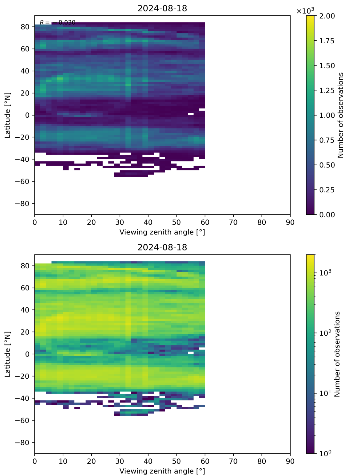
Figure 109: Scatter density plot of “Viewing zenith angle” against “Latitude” for 2024-08-17 to 2024-08-19.
