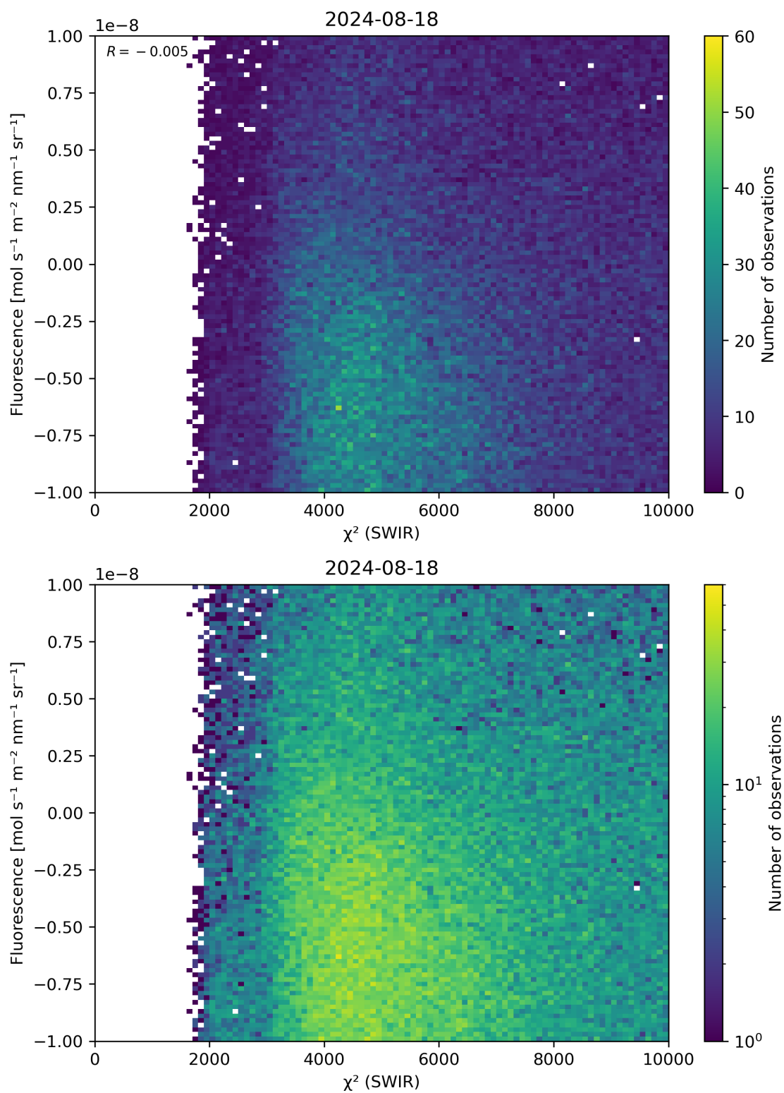
Figure 49: Scatter density plot of “ \chi^2 (SWIR)” against “Fluorescence” for 2024-08-17 to 2024-08-19.
