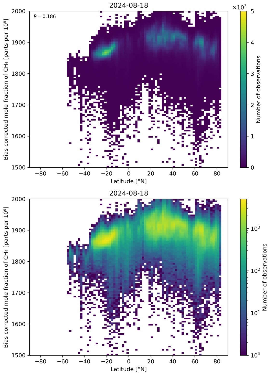
Figure 58: Scatter density plot of “Latitude” against “Bias corrected mole fraction of \text{CH}_4 ” for 2024-08-17 to 2024-08-19.
