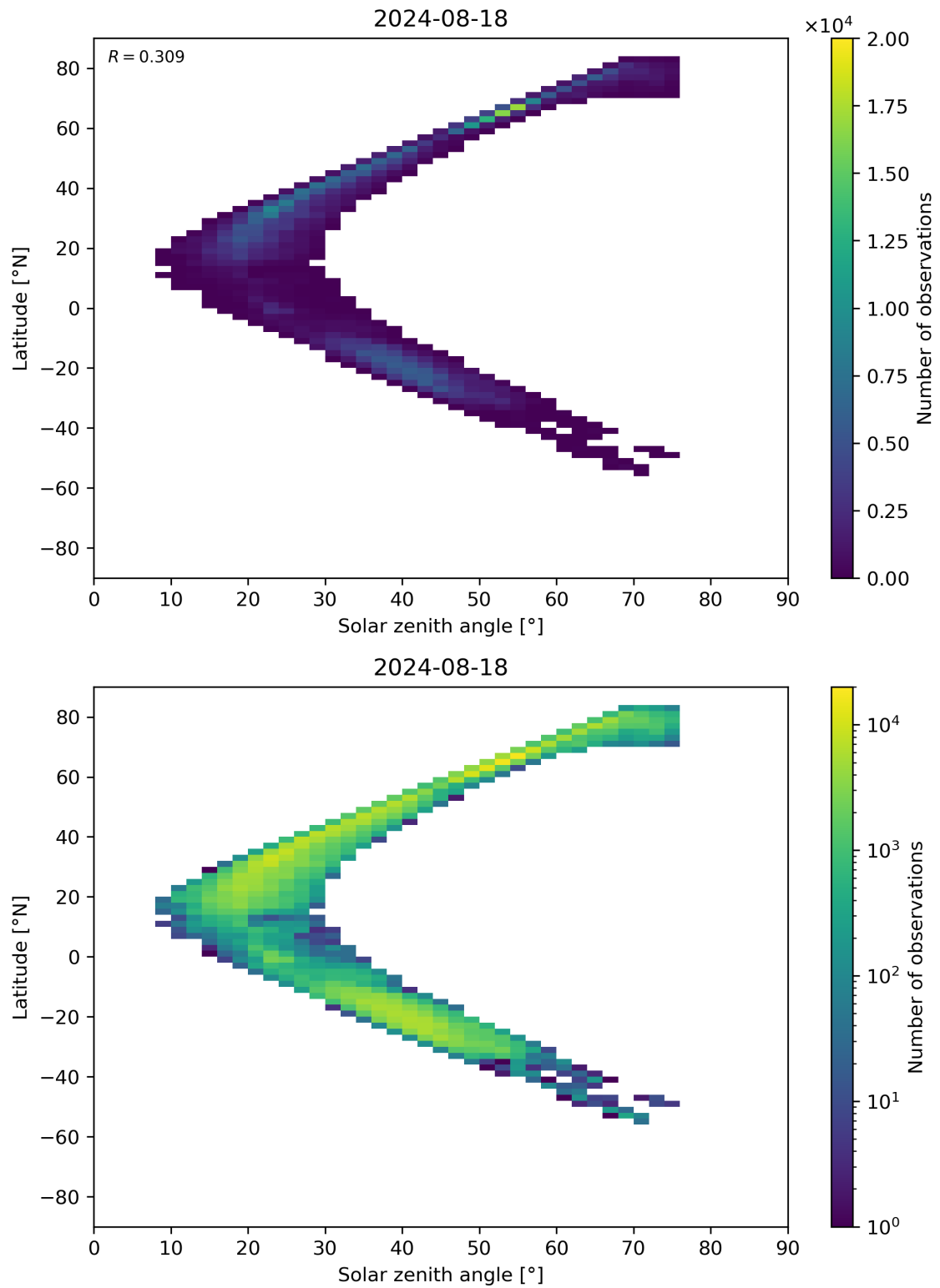
Figure 98: Scatter density plot of “Solar zenith angle” against “Latitude” for 2024-08-17 to 2024-08-19.
