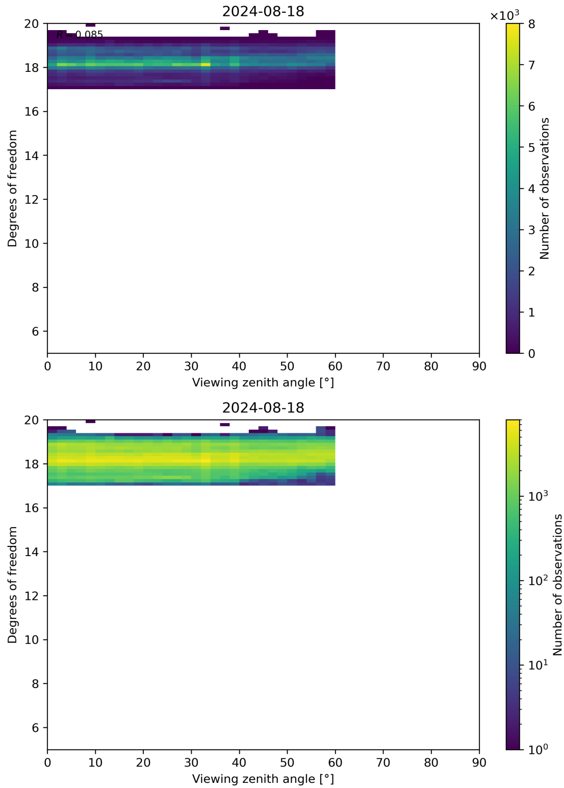
Figure 107: Scatter density plot of “Viewing zenith angle” against “Degrees of freedom” for 2024-08-17 to 2024-08-19.
