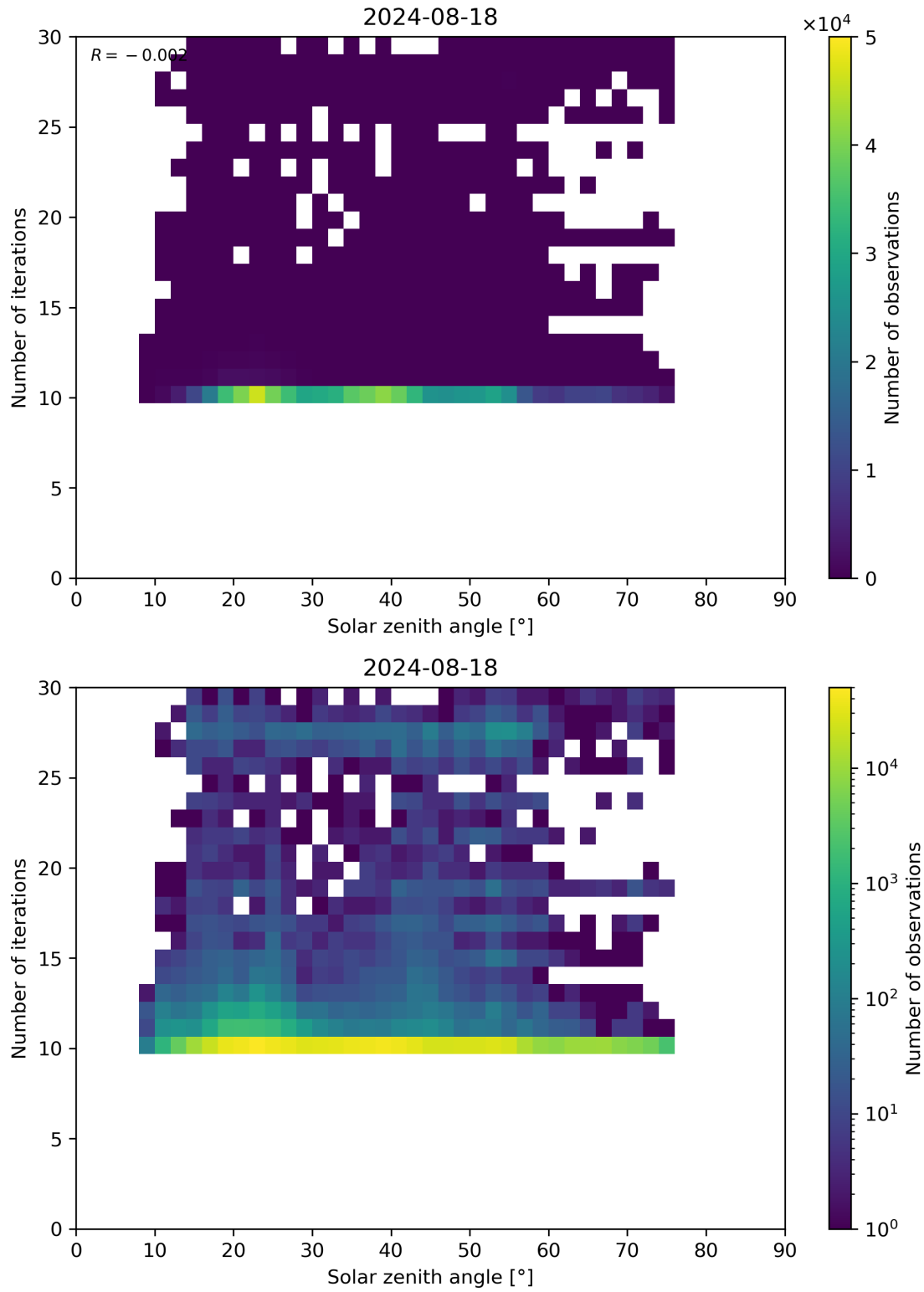
Figure 102: Scatter density plot of “Solar zenith angle” against “Number of iterations” for 2024-08-17 to 2024-08-19.
