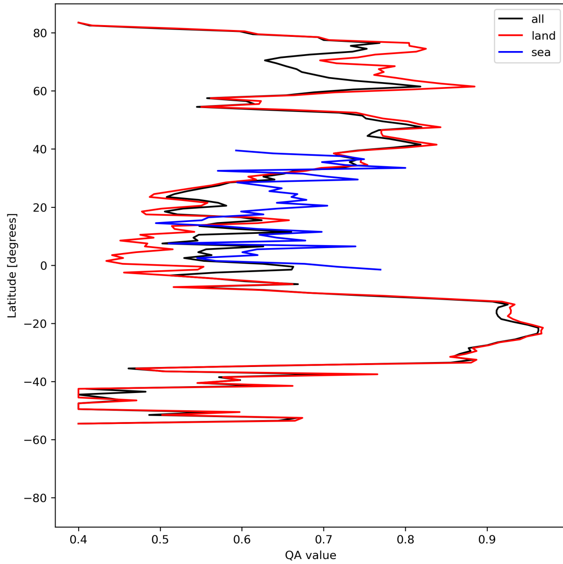
Figure 11: Zonal average of “QA value” for 2024-08-17 to 2024-08-19.
