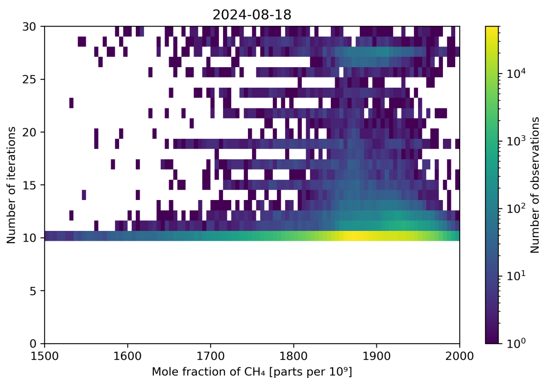
Figure 76: Scatter density plot of “Mole fraction of CH 4 ” against “Number of iterations” for 2024-08-17 to 2024-08-19.
