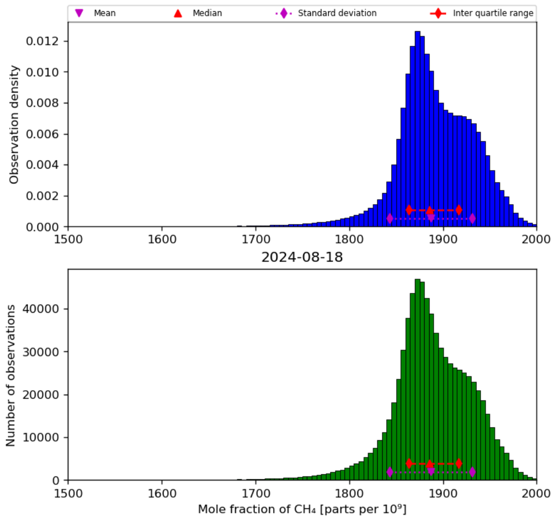
Figure 23: Histogram of “Mole fraction of CH 4 ” for 2024-08-17 to 2024-08-19
