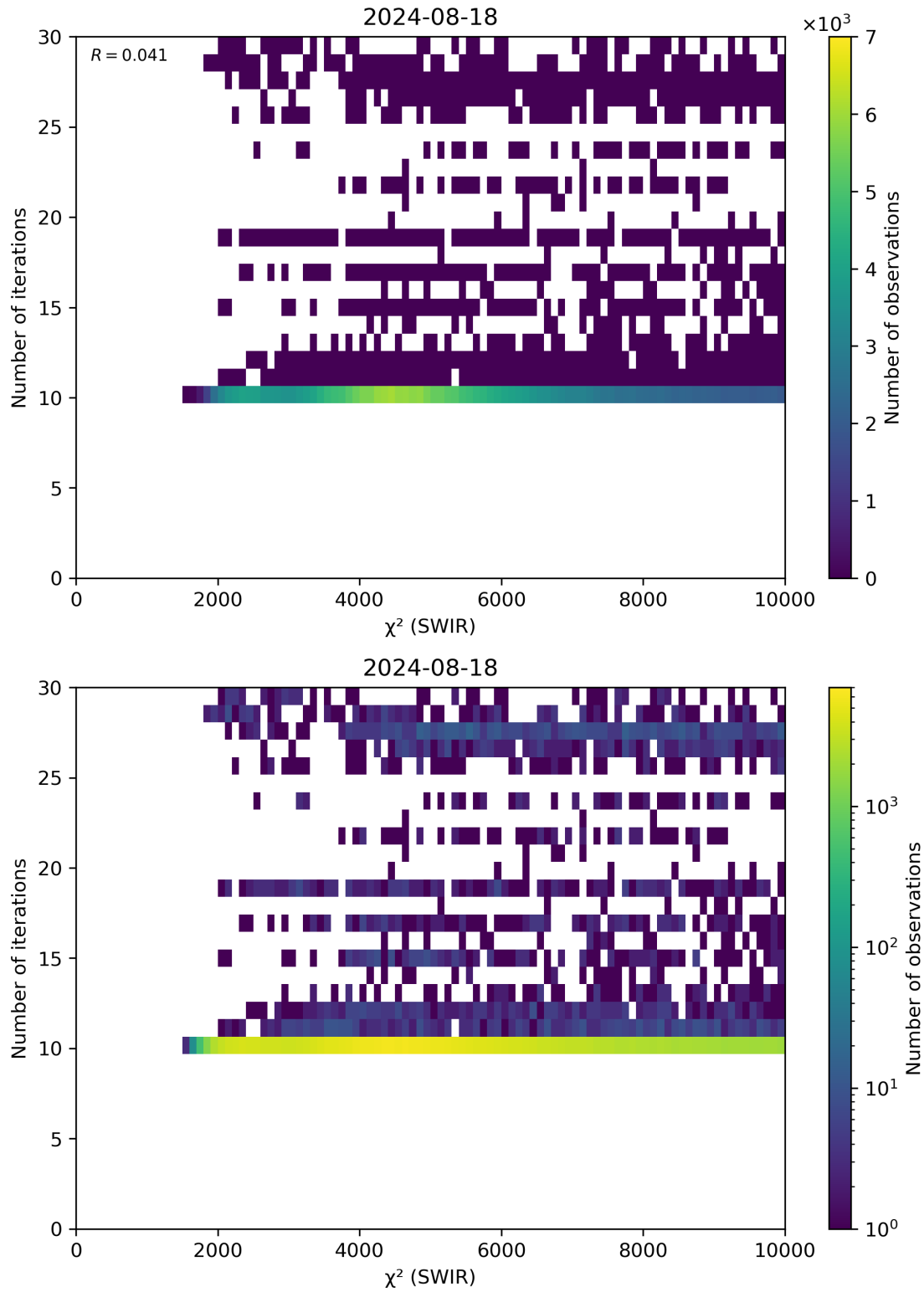
Figure 50: Scatter density plot of “ \chi^2 (SWIR)” against “Number of iterations” for 2024-08-17 to 2024-08-19.
