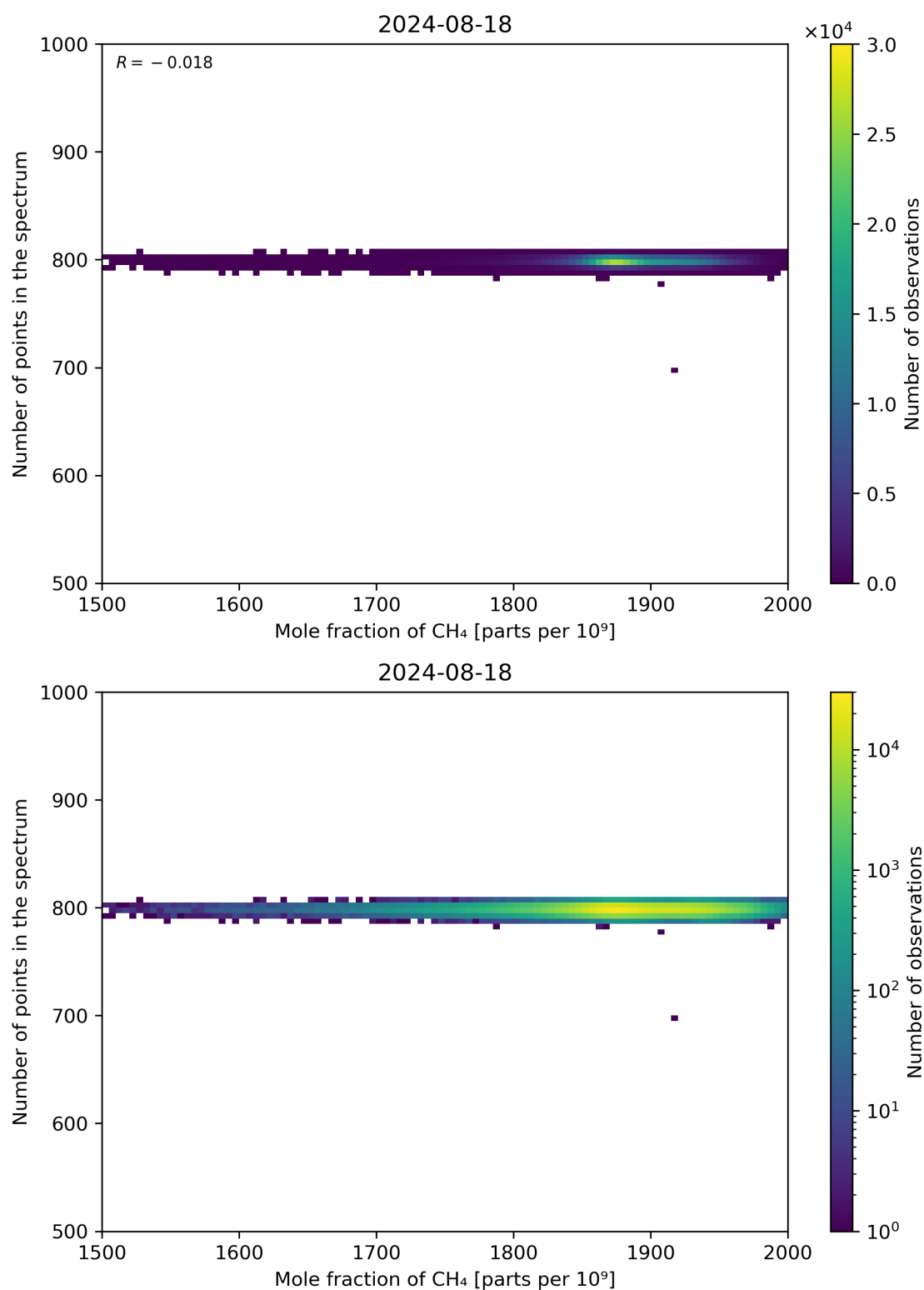
Figure 77: Scatter density plot of “Mole fraction of CH 4 ” against “Number of points in the spectrum” for 2024-08-17 to 2024-08-19.
