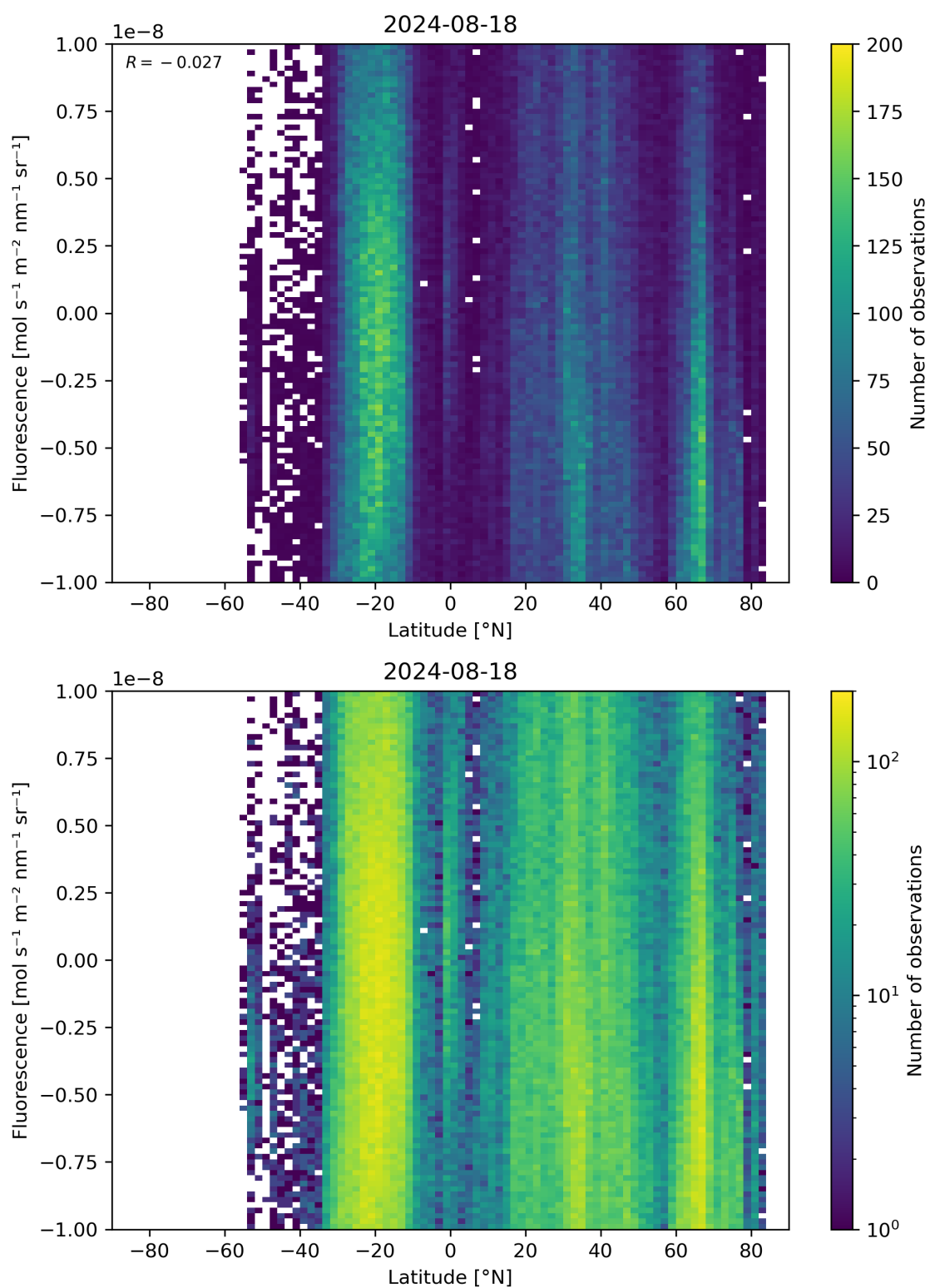
Figure 56: Scatter density plot of “Latitude” against “Fluorescence” for 2024-08-17 to 2024-08-19.
