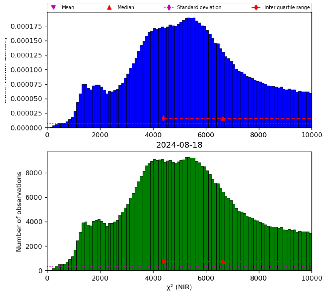
Figure 29: Histogram of “ \chi^2 (NIR)” for 2024-08-17 to 2024-08-19
