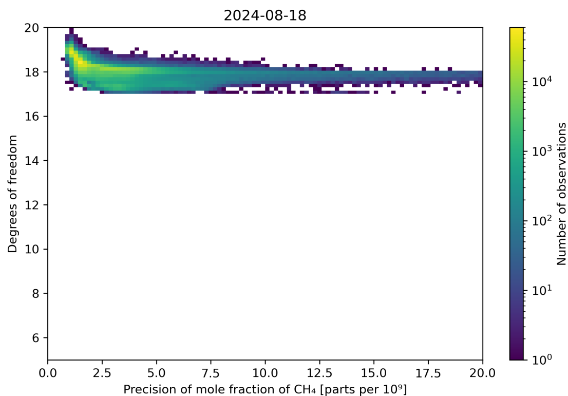
Figure 80: Scatter density plot of “Precision of mole fraction of CH 4 ” against “Degrees of freedom” for 2024-08-17 to 2024-08-19.
