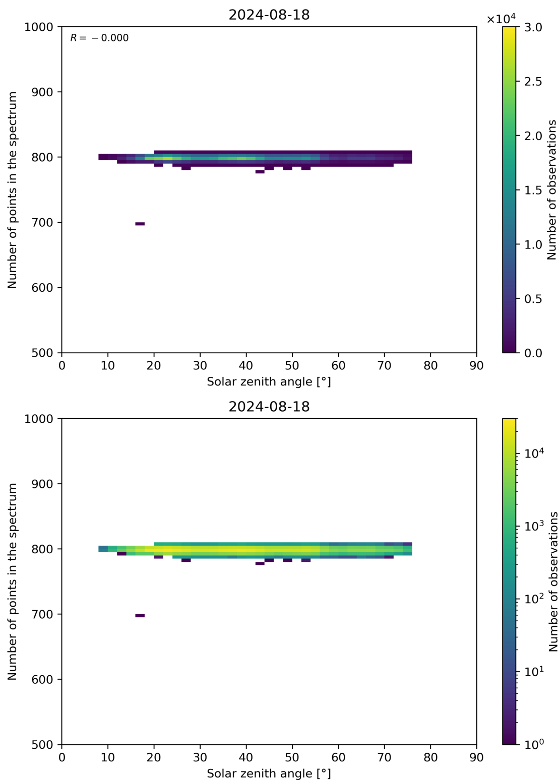
Figure 103: Scatter density plot of “Solar zenith angle” against “Number of points in the spectrum” for 2024-08-17 to 2024-08-19.
