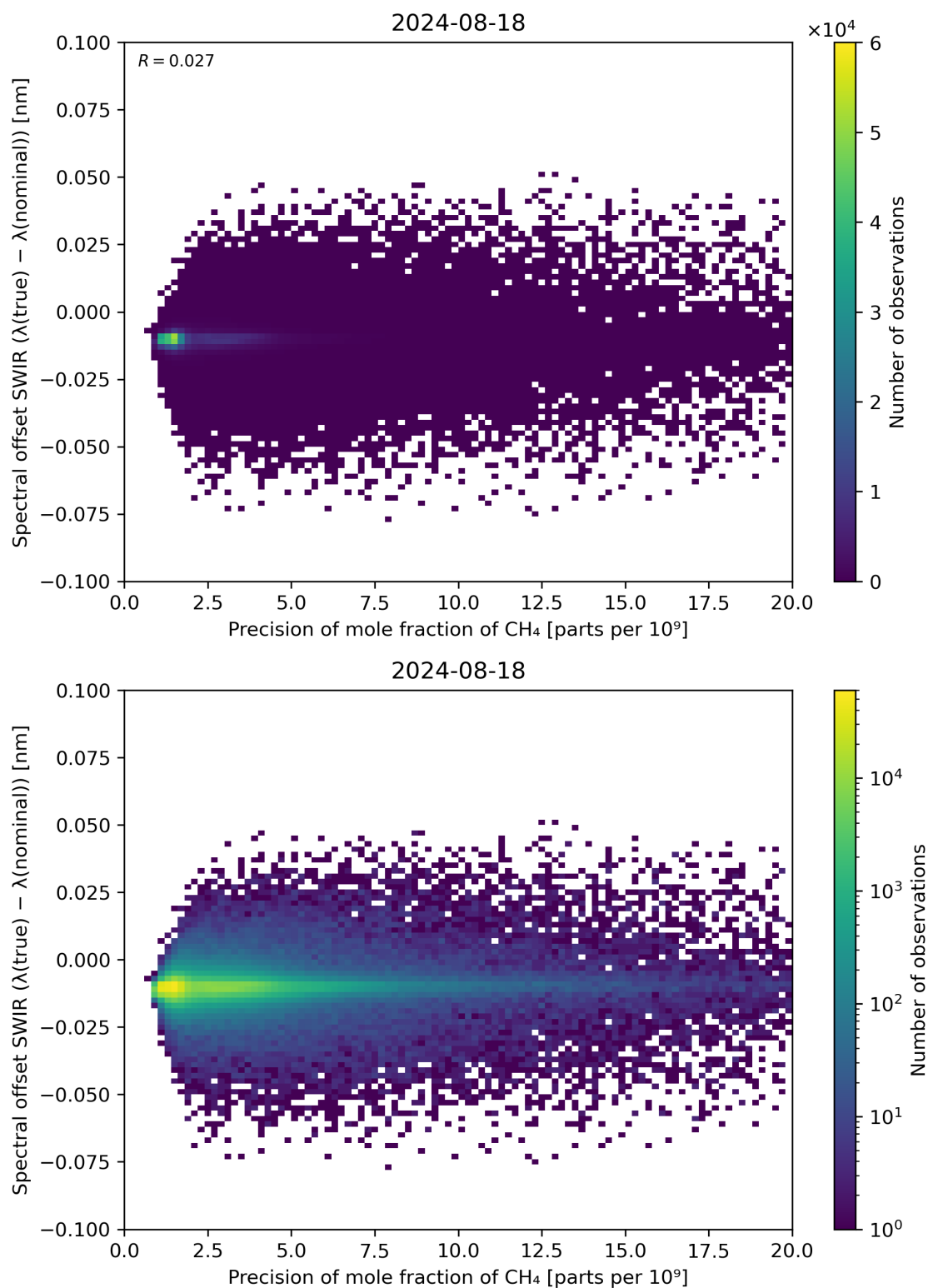
Figure 85: Scatter density plot of “Precision of mole fraction of CH 4 ” against “Spectral offset SWIR ( \lambda(\text{true}) - \lambda(\text{nominal}) )” for 2024-08-17 to 2024-08-19.
