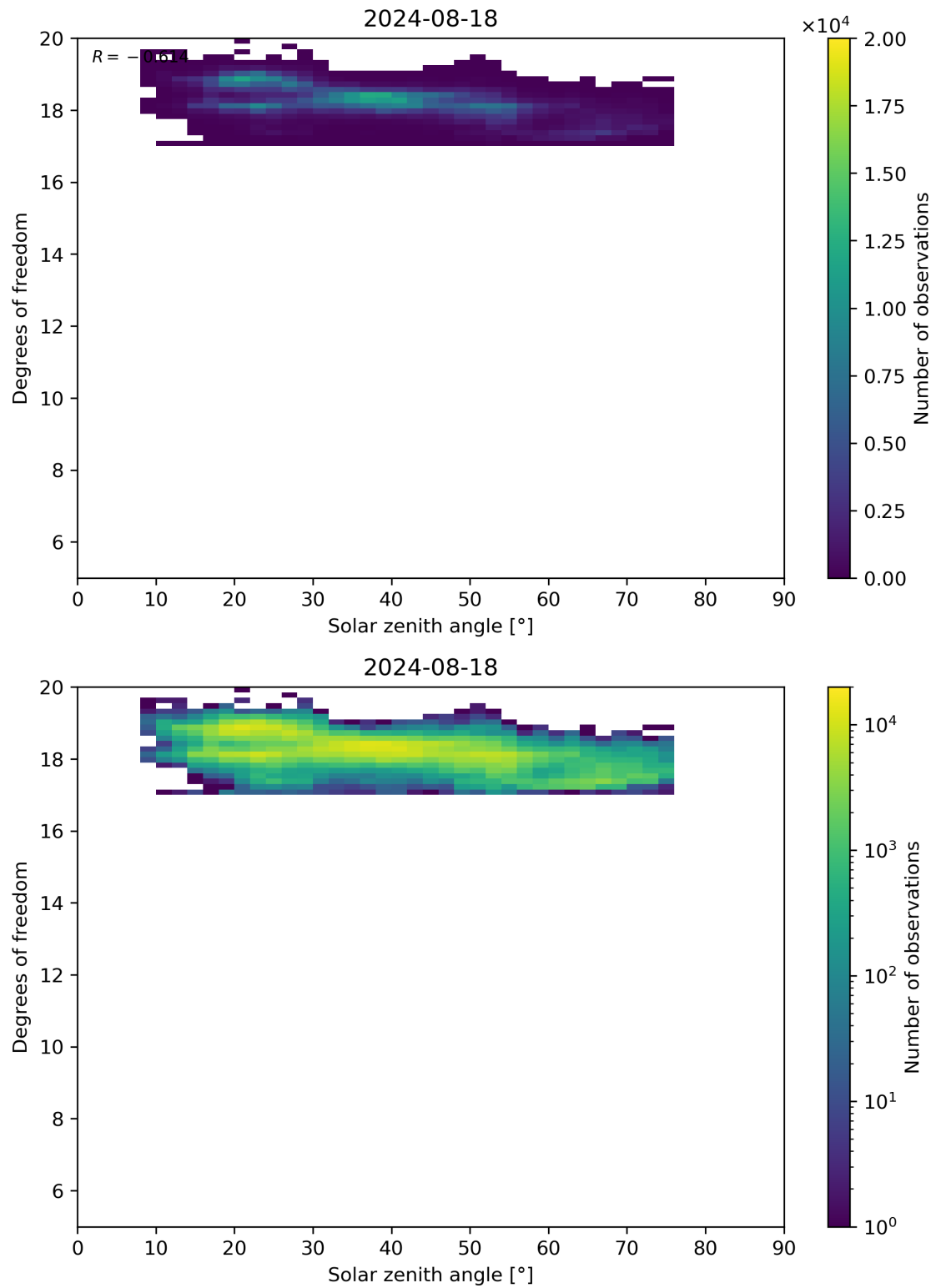
Figure 96: Scatter density plot of “Solar zenith angle” against “Degrees of freedom” for 2024-08-17 to 2024-08-19.
