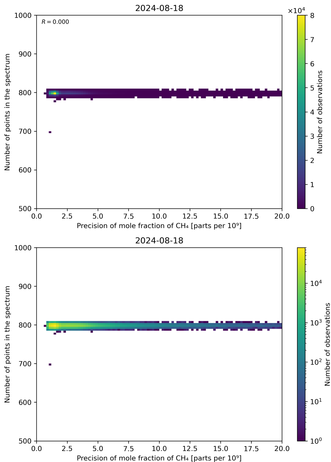
Figure 84: Scatter density plot of “Precision of mole fraction of CH 4 ” against “Number of points in the spectrum” for 2024-08-17 to 2024-08-19.
