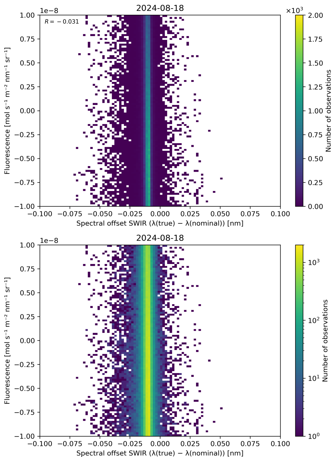
Figure 120: Scatter density plot of “Spectral offset SWIR ( \lambda(\text{true}) - \lambda(\text{nominal}) )” against “Fluorescence” for 2024-08-17 to 2024-08-19.
