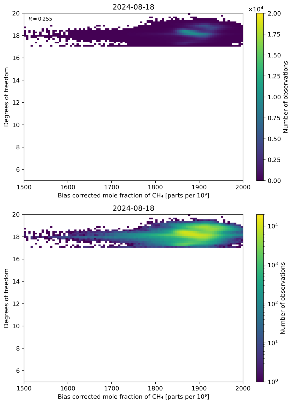
Figure 65: Scatter density plot of “Bias corrected mole fraction of CH 4 ” against “Degrees of freedom” for 2024-08-17 to 2024-08-19.
