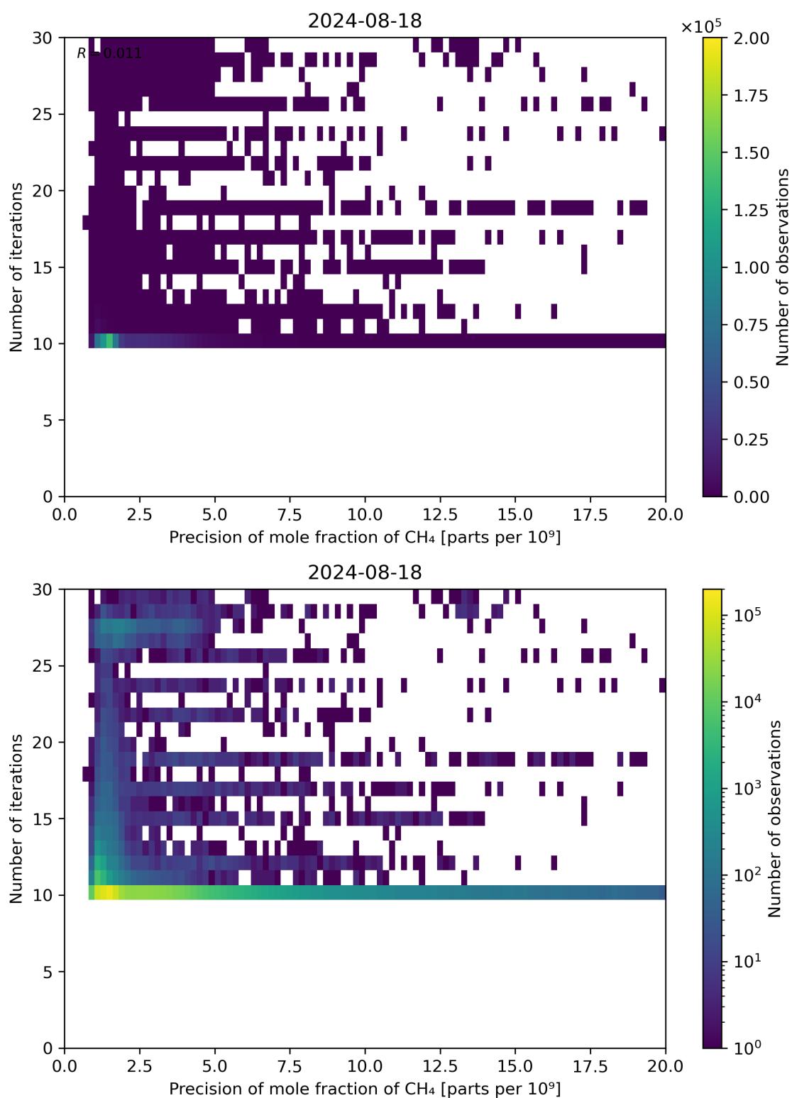
Figure 83: Scatter density plot of “Precision of mole fraction of CH 4 ” against “Number of iterations” for 2024-08-17 to 2024-08-19.
