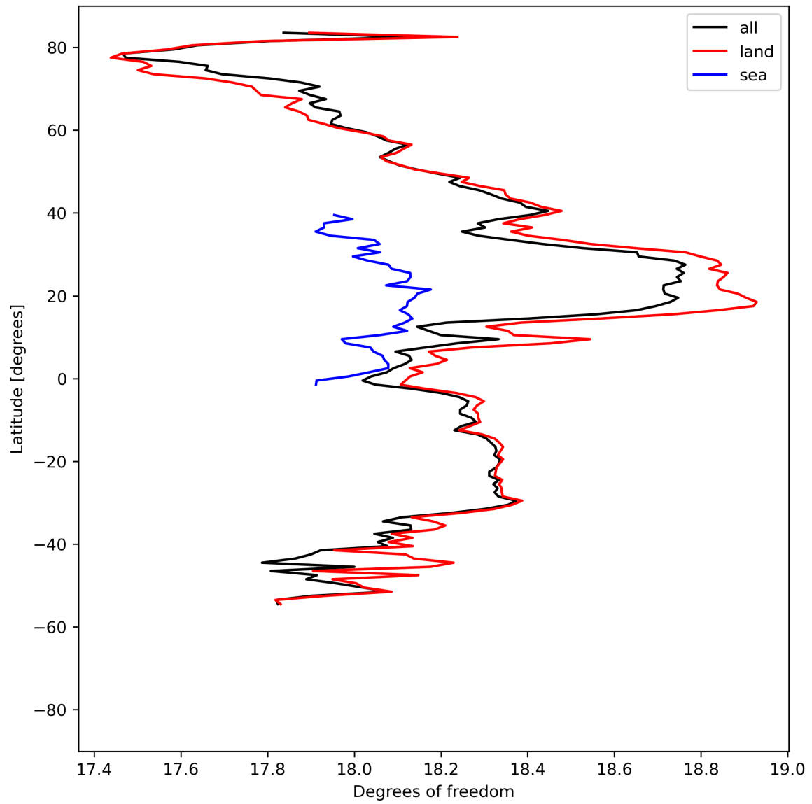
Figure 19: Zonal average of “Degrees of freedom” for 2024-08-17 to 2024-08-19.
