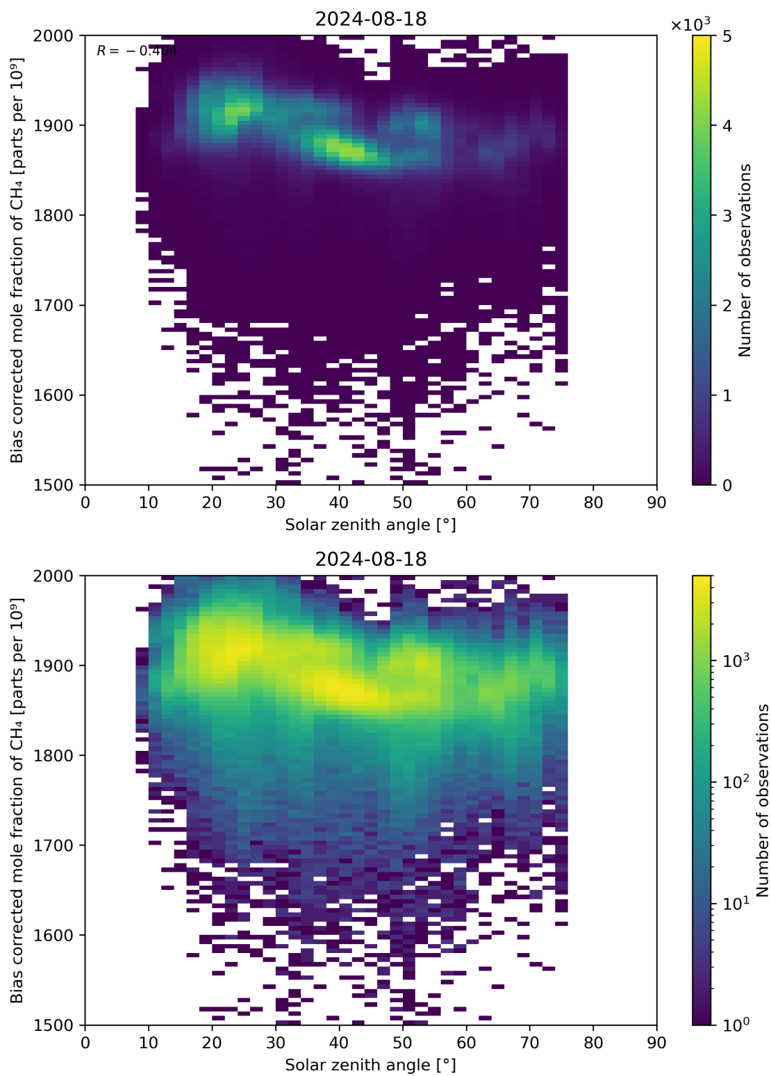
Figure 100: Scatter density plot of “Solar zenith angle” against “Bias corrected mole fraction of CH 4 ” for 2024-08-17 to 2024-08-19.
