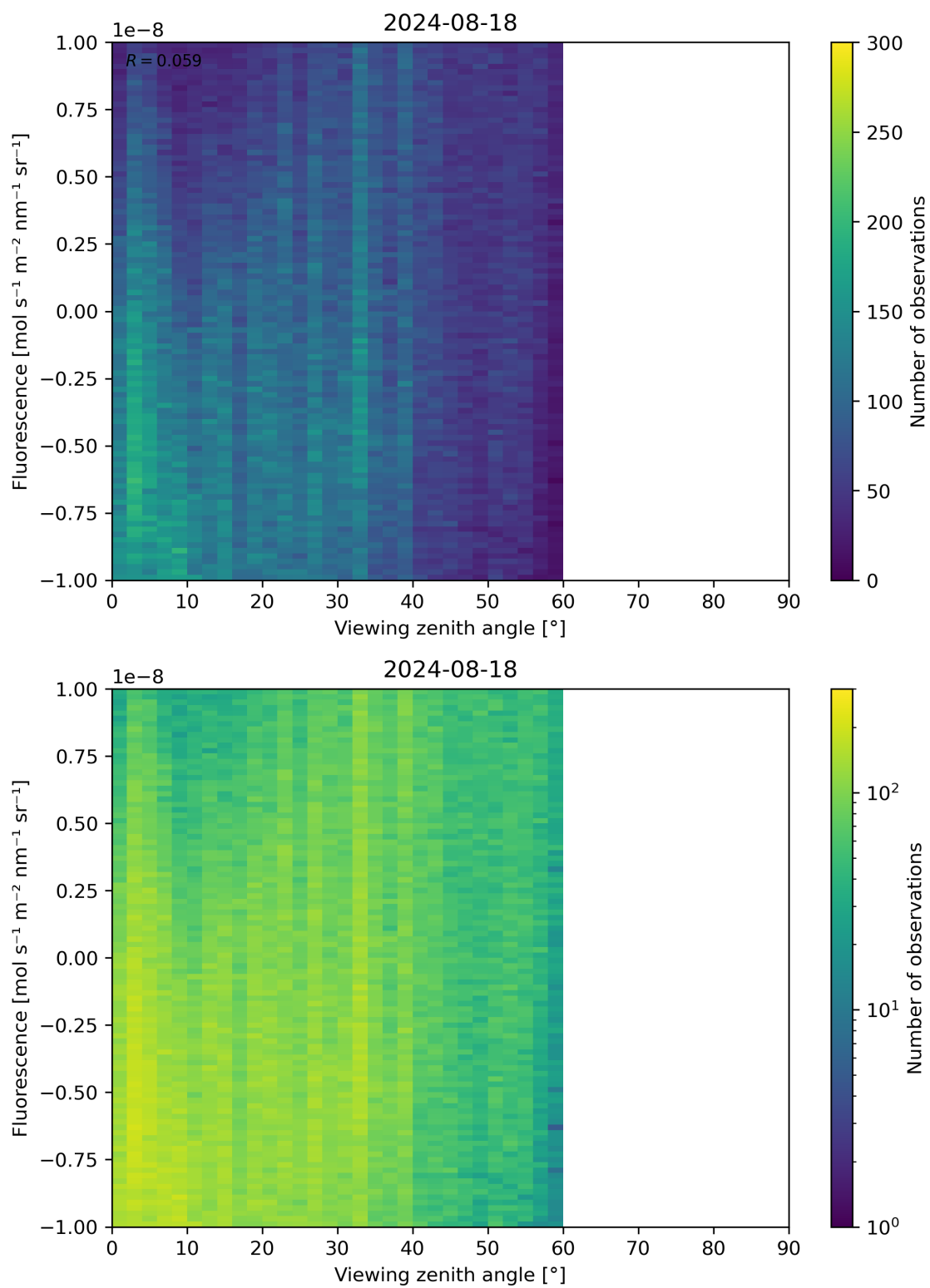
Figure 108: Scatter density plot of “Viewing zenith angle” against “Fluorescence” for 2024-08-17 to 2024-08-19.
