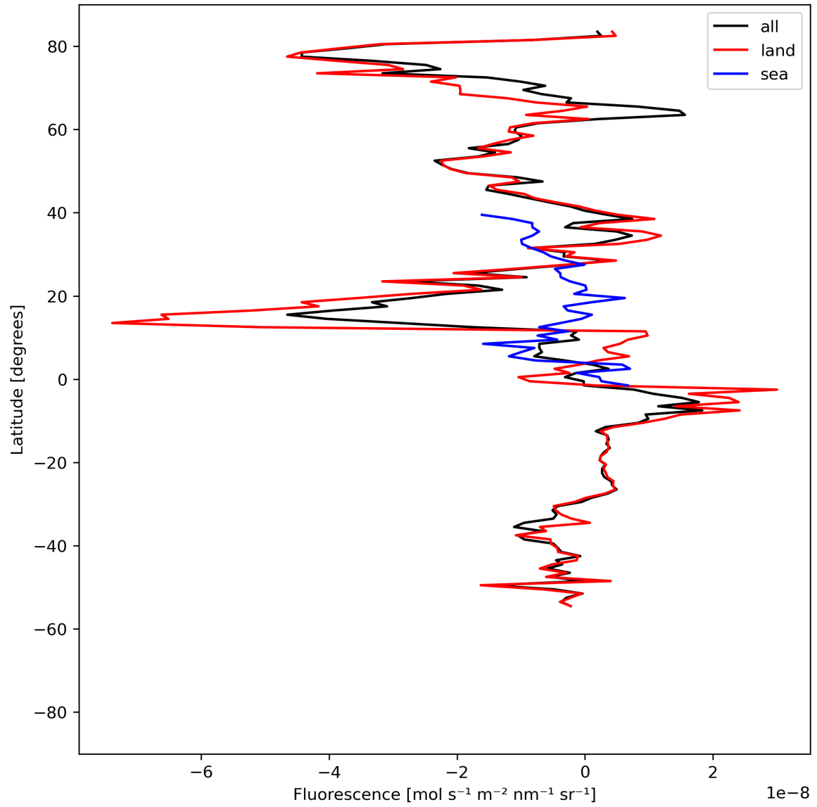
Figure 21: Zonal average of “Fluorescence” for 2024-08-17 to 2024-08-19.
