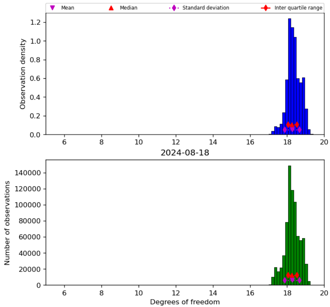
Figure 30: Histogram of “Degrees of freedom” for 2024-08-17 to 2024-08-19
