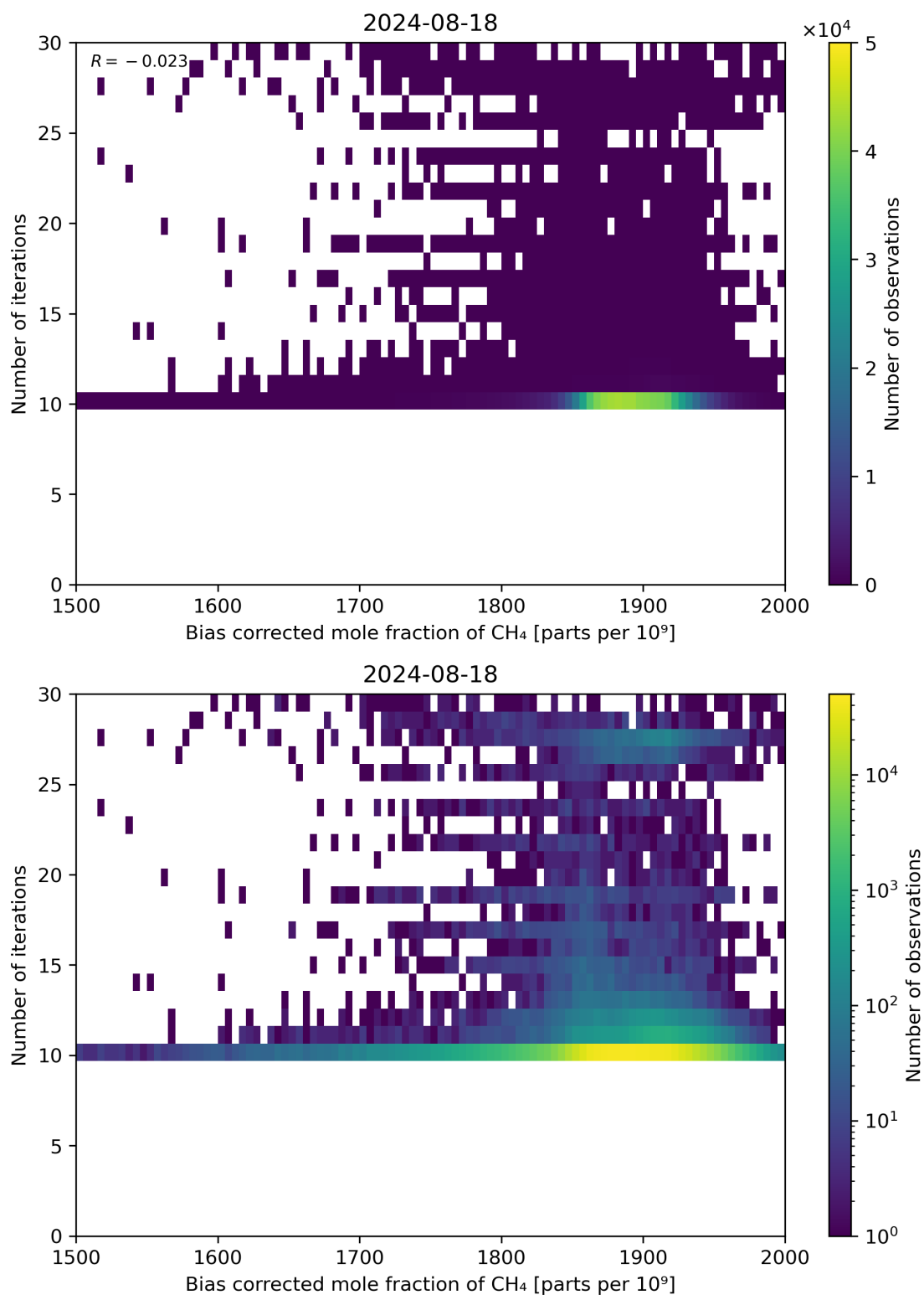
Figure 67: Scatter density plot of “Bias corrected mole fraction of CH 4 ” against “Number of iterations” for 2024-08-17 to 2024-08-19.
