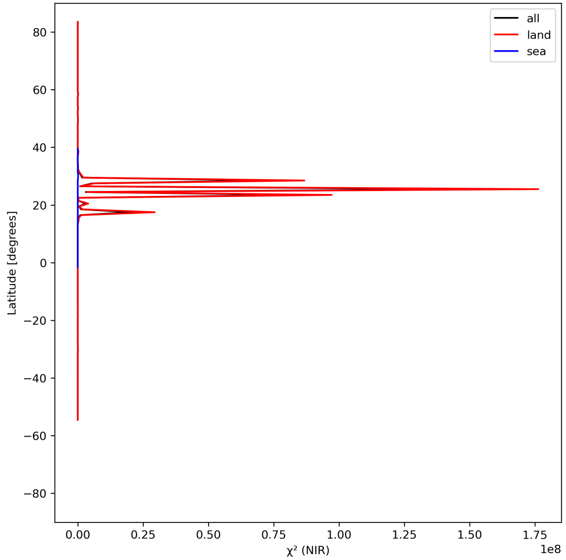
Figure 18: Zonal average of “ \chi^2 (NIR)” for 2024-08-17 to 2024-08-19.
