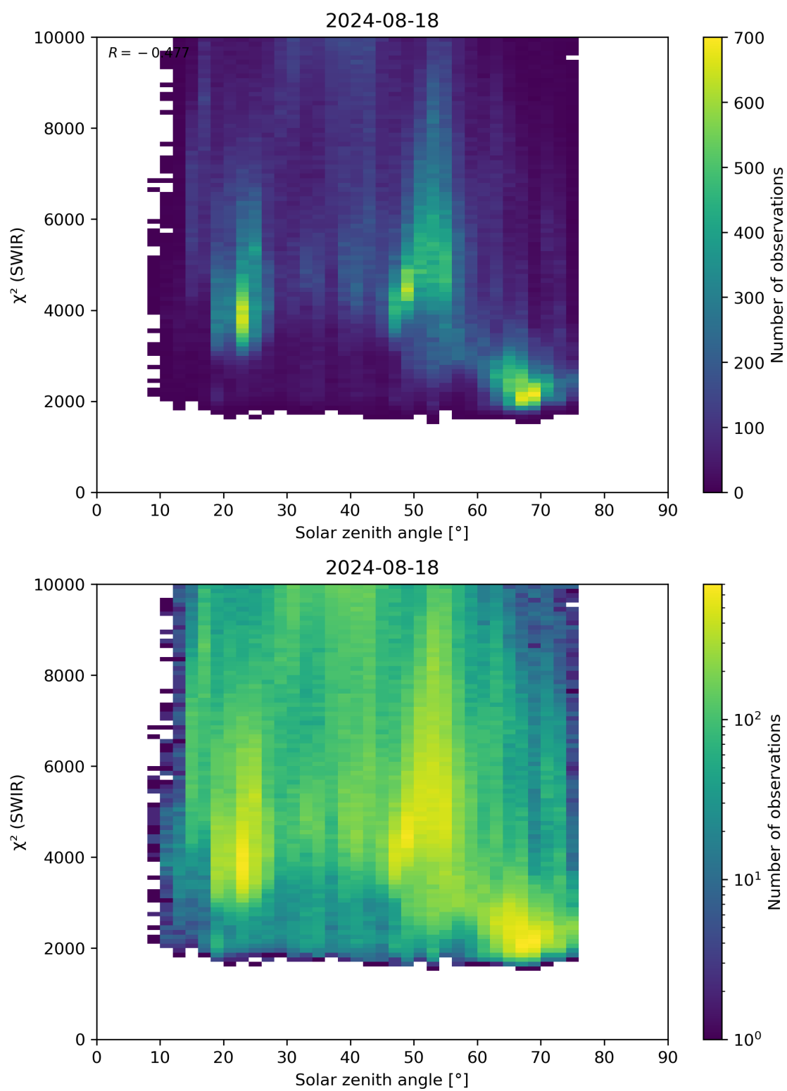
Figure 95: Scatter density plot of “Solar zenith angle” against “ \chi^2 (SWIR)” for 2024-08-17 to 2024-08-19.
