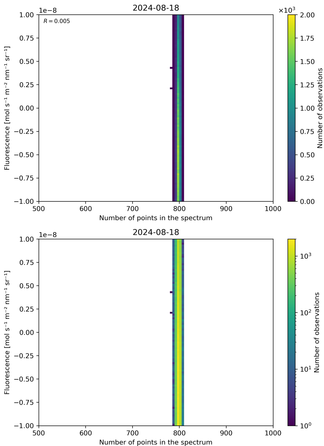
Figure 91: Scatter density plot of “Number of points in the spectrum” against “Fluorescence” for 2024-08-17 to 2024-08-19.
