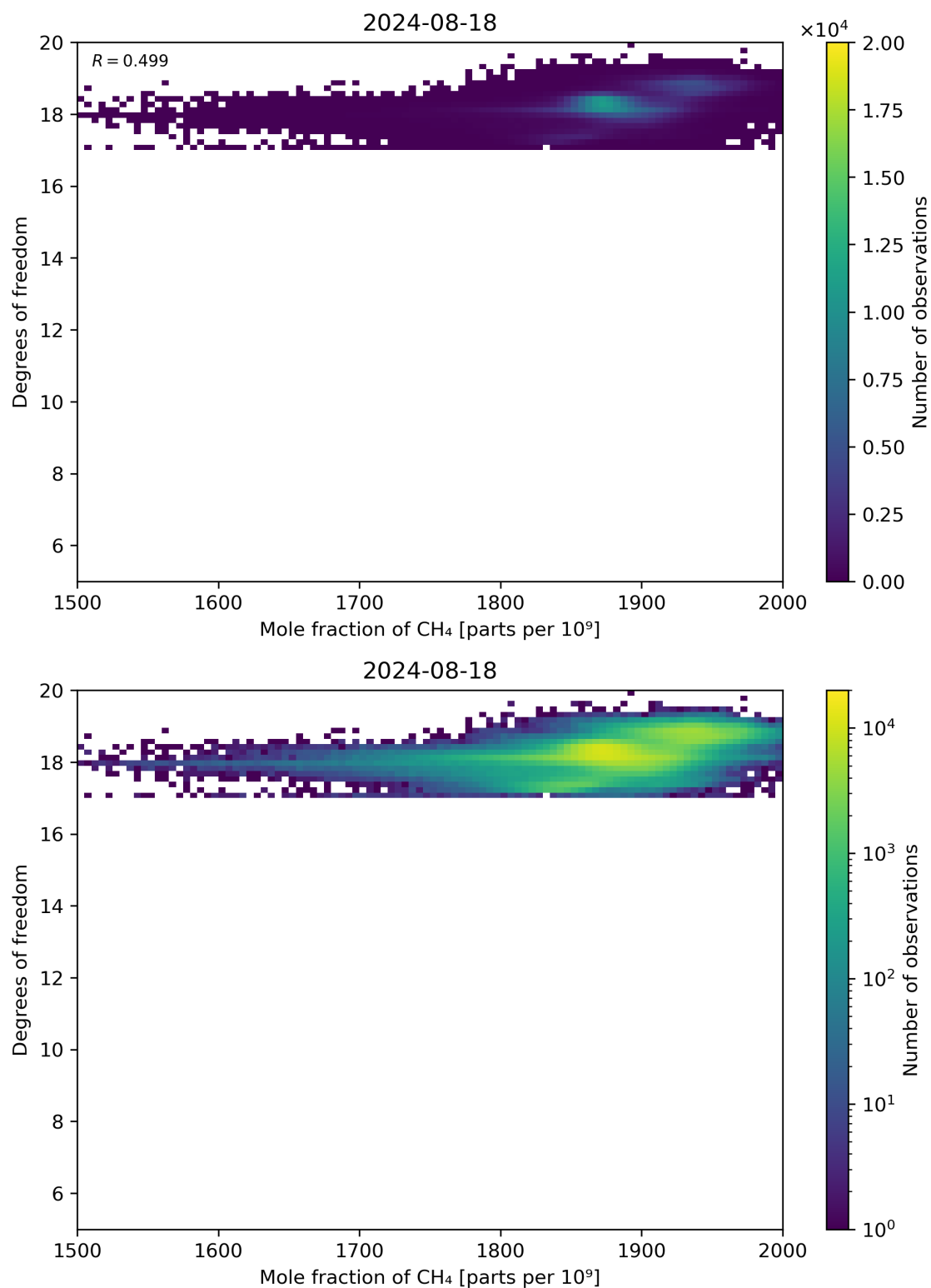
Figure 72: Scatter density plot of “Mole fraction of CH 4 ” against “Degrees of freedom” for 2024-08-17 to 2024-08-19.
