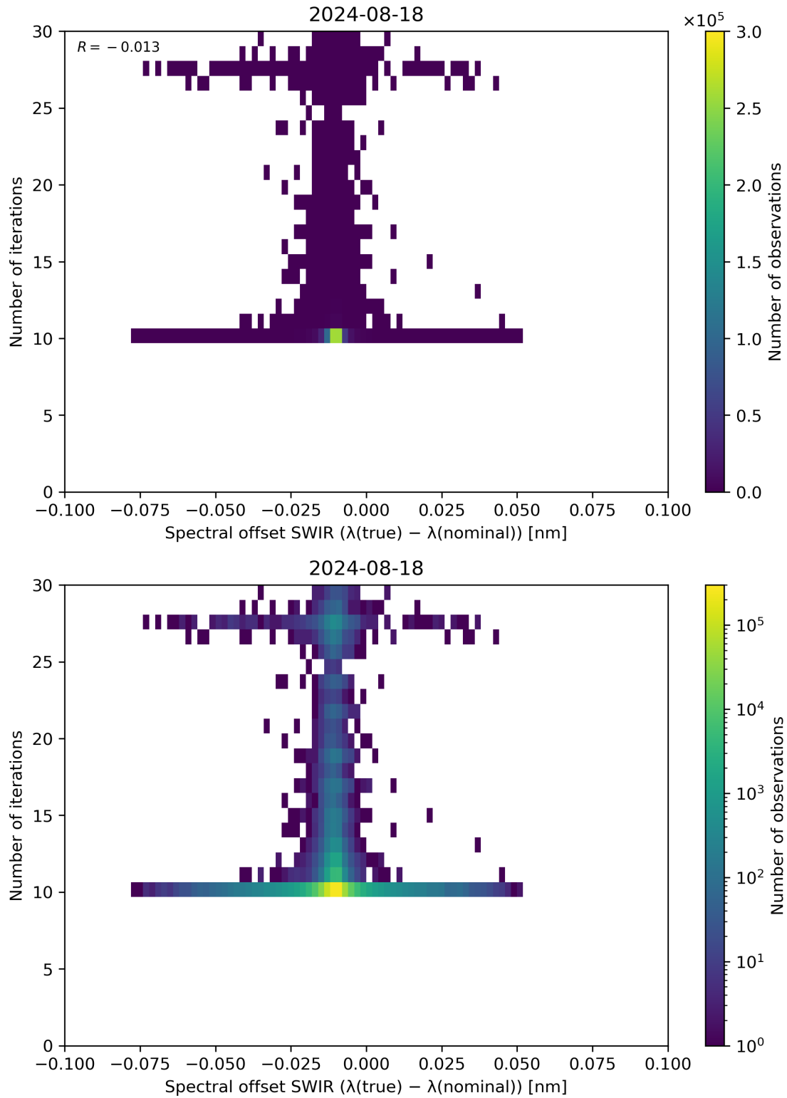
Figure 121: Scatter density plot of “Spectral offset SWIR ( \lambda(\text{true}) - \lambda(\text{nominal}) )” against “Number of iterations” for 2024-08-17 to 2024-08-19.
