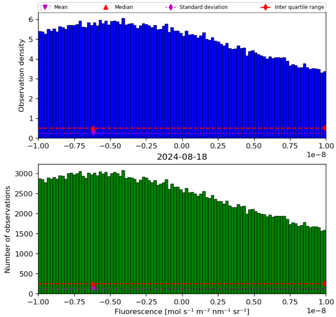
Figure 32: Histogram of “Fluorescence” for 2024-08-17 to 2024-08-19
