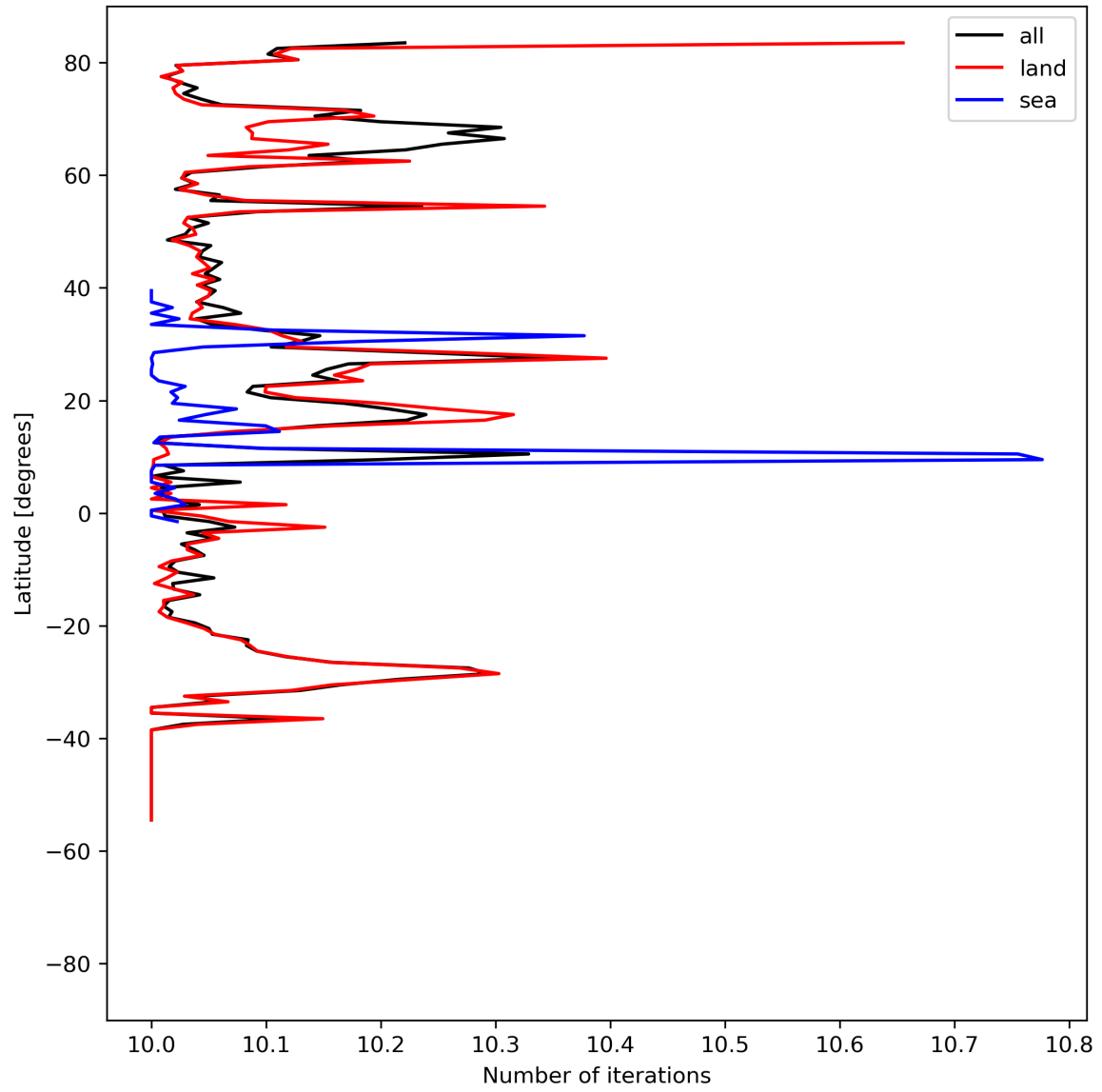
Figure 20: Zonal average of “Number of iterations” for 2024-08-17 to 2024-08-19.
