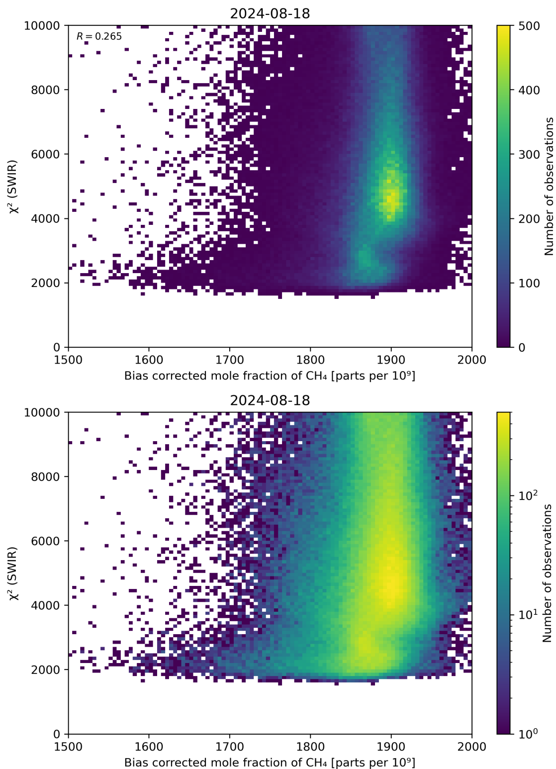
Figure 64: Scatter density plot of “Bias corrected mole fraction of CH 4 ” against “ \chi^2 (SWIR)” for 2024-08-17 to 2024-08-19.
