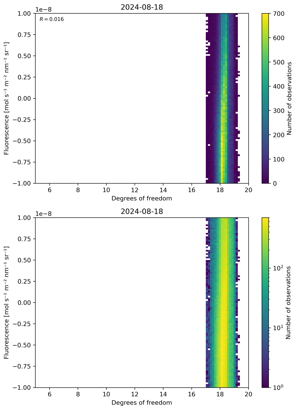
Figure 51: Scatter density plot of “Degrees of freedom” against “Fluorescence” for 2024-08-17 to 2024-08-19.
