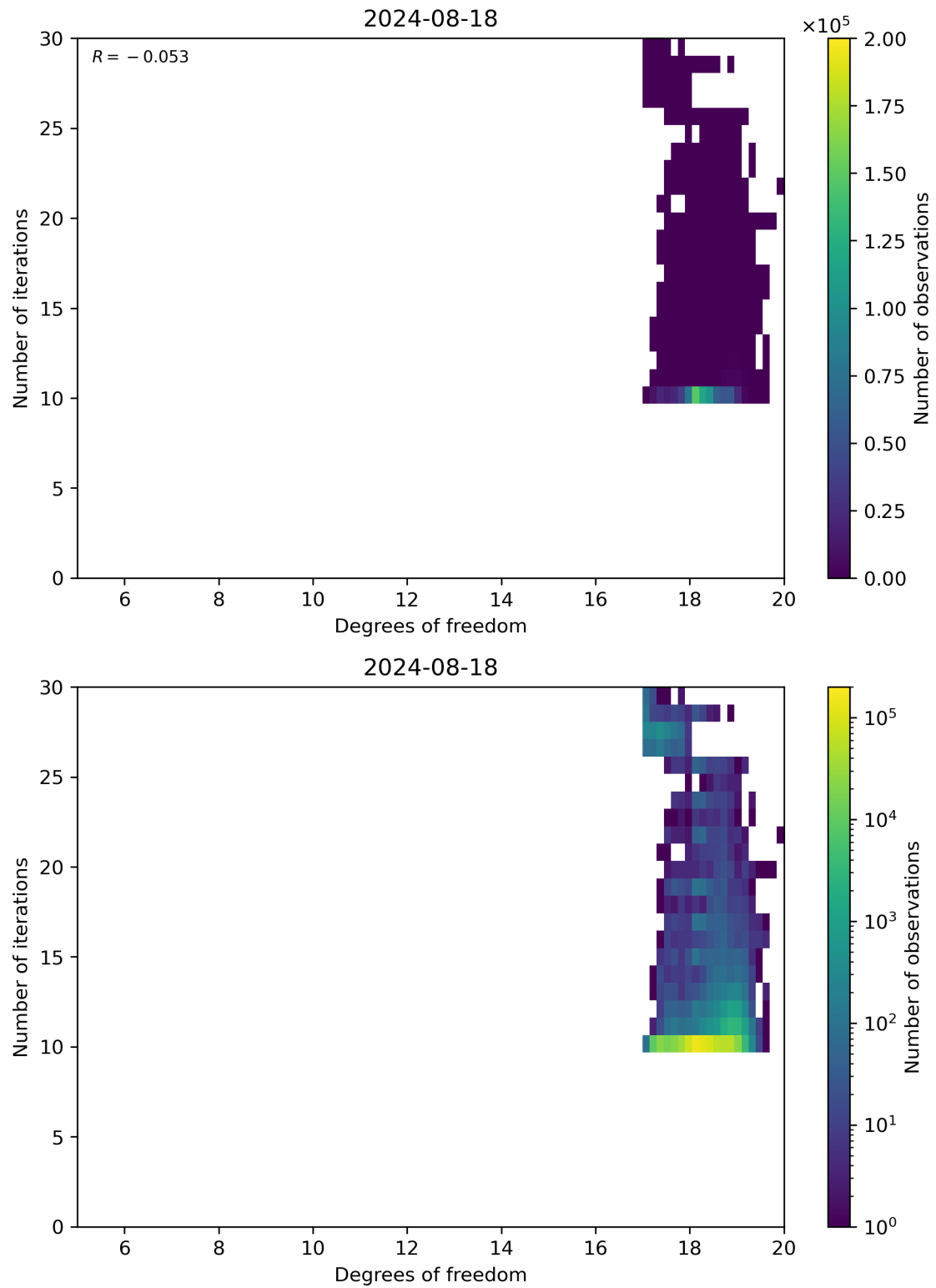
Figure 52: Scatter density plot of “Degrees of freedom” against “Number of iterations” for 2024-08-17 to 2024-08-19.
