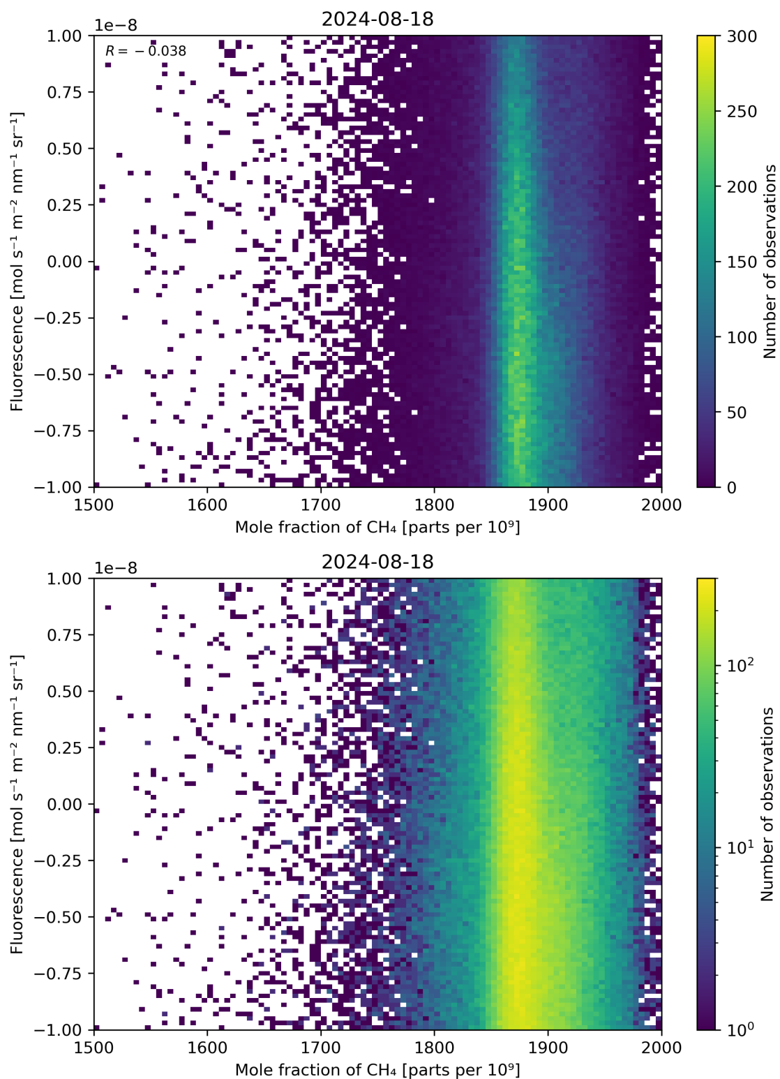
Figure 73: Scatter density plot of “Mole fraction of \text{CH}_4 ” against “Fluorescence” for 2024-08-17 to 2024-08-19.
