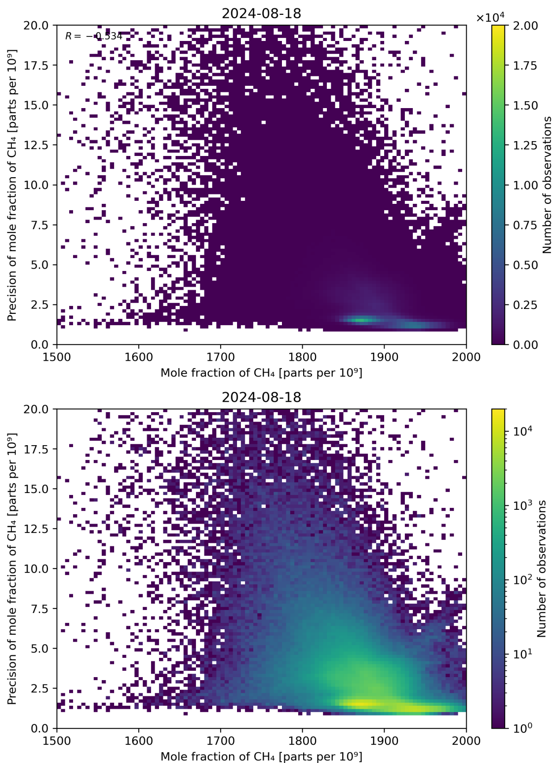
Figure 75: Scatter density plot of “Mole fraction of CH 4 ” against “Precision of mole fraction of CH 4 ” for 2024-08-17 to 2024-08-19.
