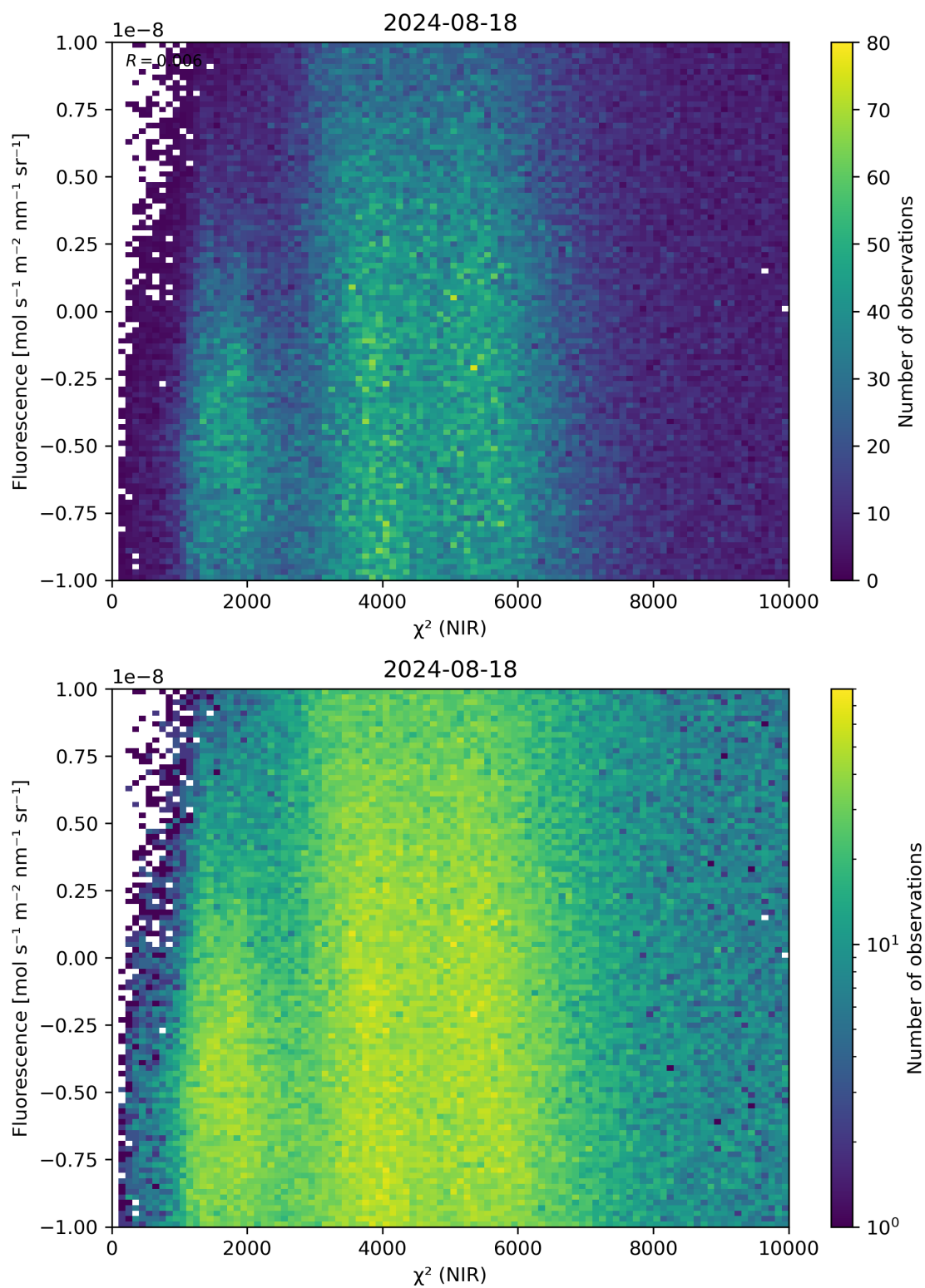
Figure 45: Scatter density plot of “ \chi^2 (NIR)” against “Fluorescence” for 2024-08-17 to 2024-08-19.
