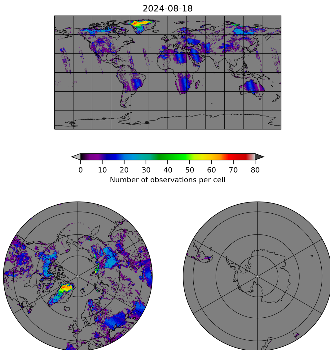
Figure 10: Map of the number of observations for 2024-08-17 to 2024-08-19
