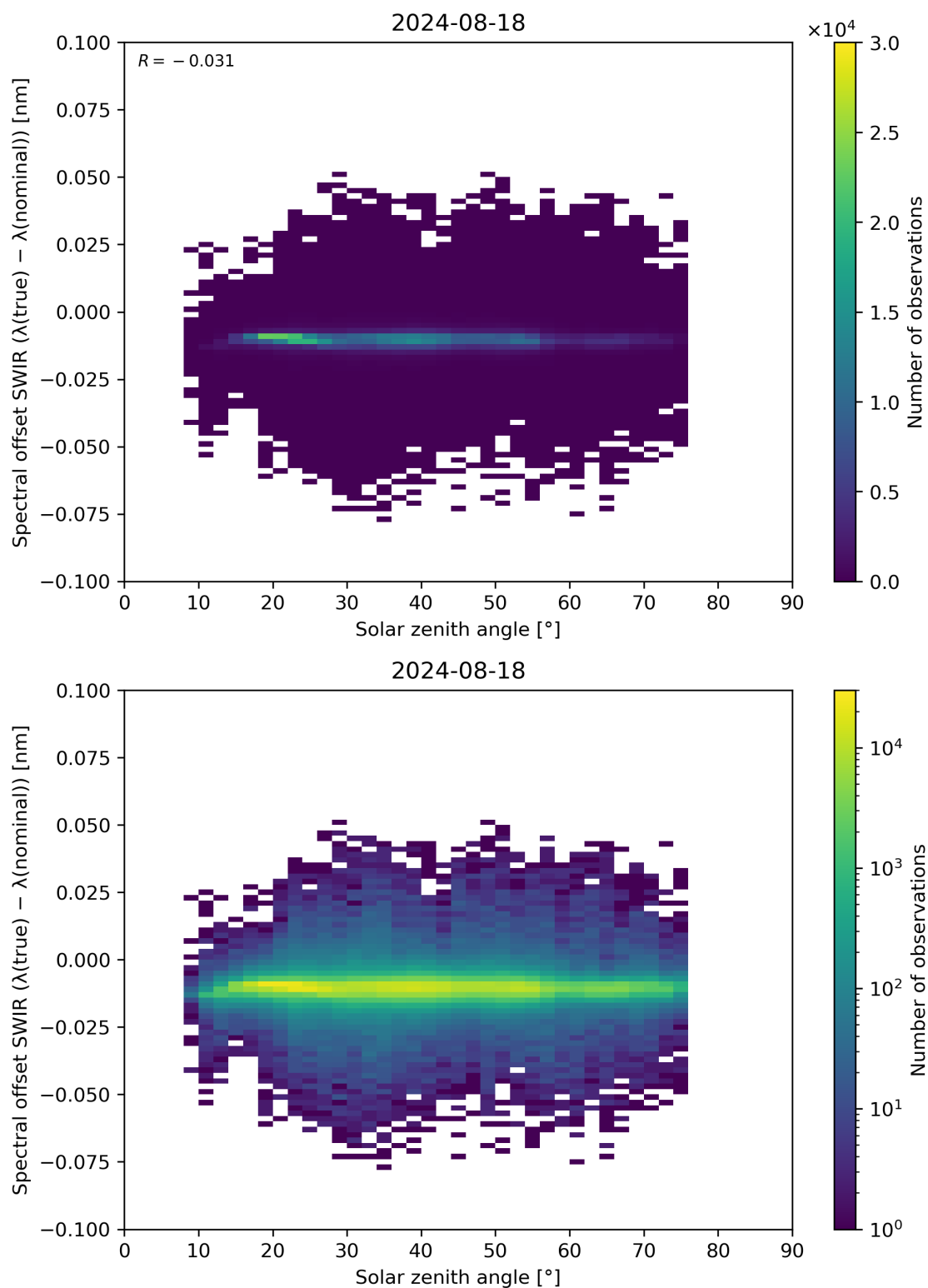
Figure 104: Scatter density plot of “Solar zenith angle” against “Spectral offset SWIR ( \lambda(\text{true}) - \lambda(\text{nominal}) )” for 2024-08-17 to 2024-08-19.
