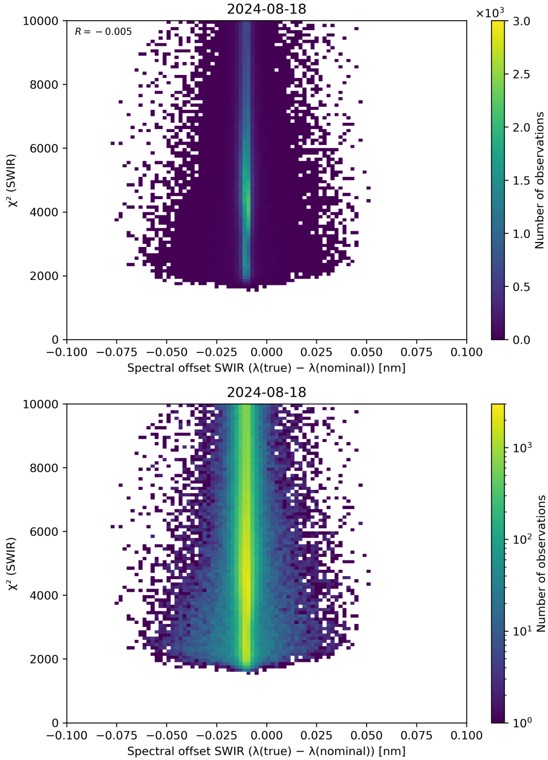
Figure 118: Scatter density plot of “Spectral offset SWIR ( \lambda(\text{true}) - \lambda(\text{nominal}) )” against “ \chi^2 (SWIR)” for 2024-08-17 to 2024-08-19.
