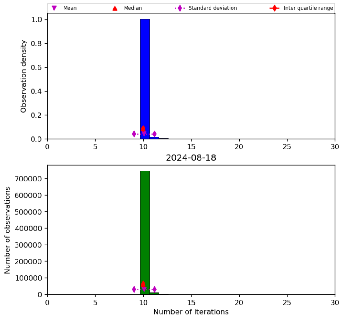
Figure 31: Histogram of “Number of iterations” for 2024-08-17 to 2024-08-19
