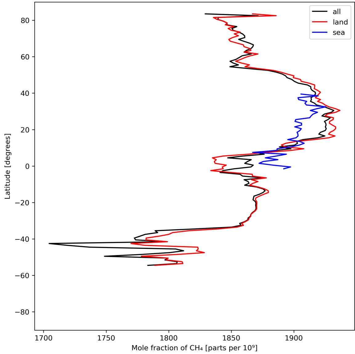
Figure 12: Zonal average of “Mole fraction of \text{CH}_4 ” for 2024-08-17 to 2024-08-19.
