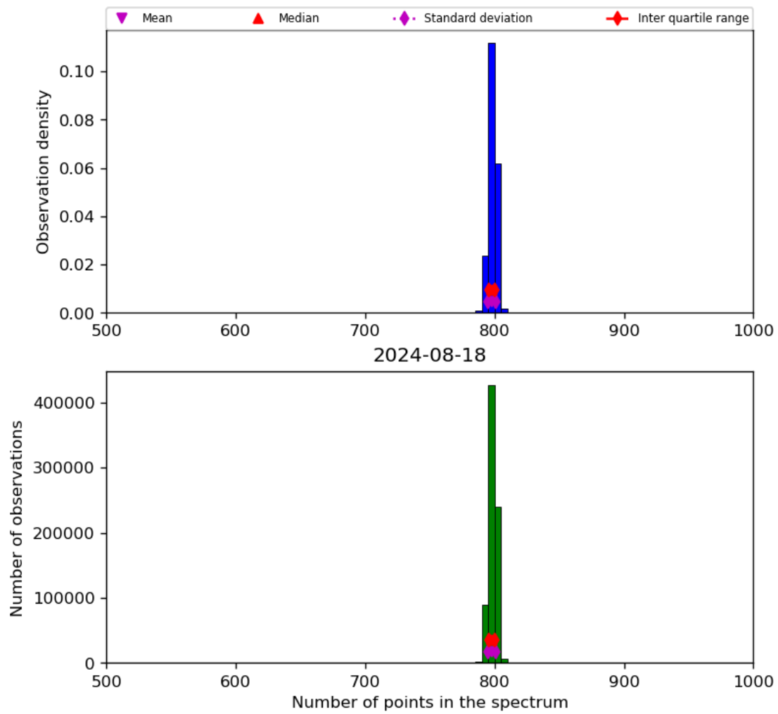
Figure 26: Histogram of “Number of points in the spectrum” for 2024-08-17 to 2024-08-19
