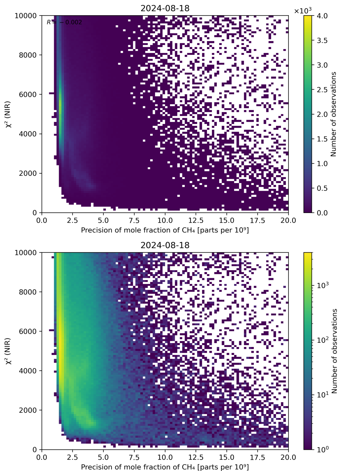
Figure 78: Scatter density plot of “Precision of mole fraction of \text{CH}_4 ” against “ \chi^2 (NIR)” for 2024-08-17 to 2024-08-19.
