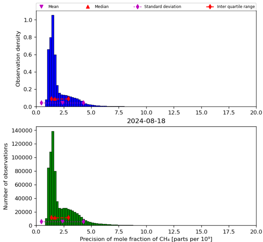
Figure 24: Histogram of “Precision of mole fraction of CH 4 ” for 2024-08-17 to 2024-08-19
