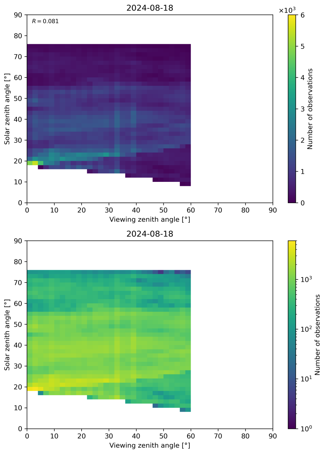
Figure 115: Scatter density plot of “Viewing zenith angle” against “Solar zenith angle” for 2024-08-17 to 2024-08-19.
