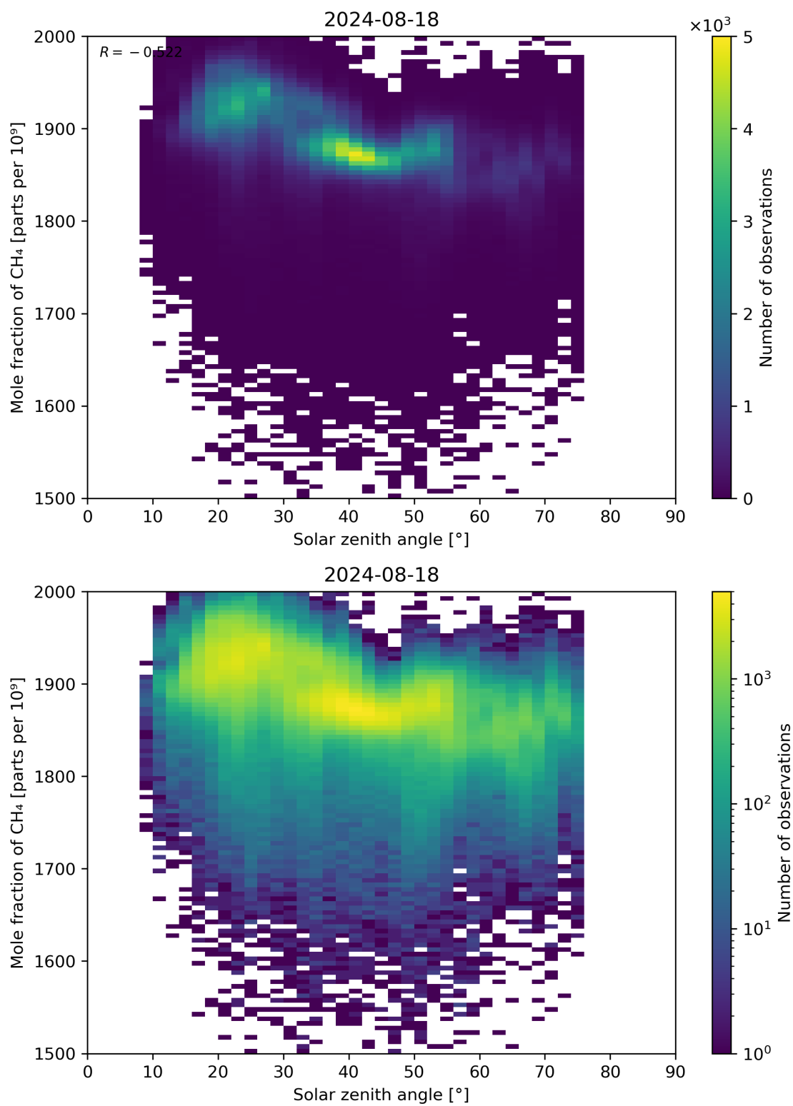
Figure 99: Scatter density plot of “Solar zenith angle” against “Mole fraction of \text{CH}_4 ” for 2024-08-17 to 2024-08-19.
