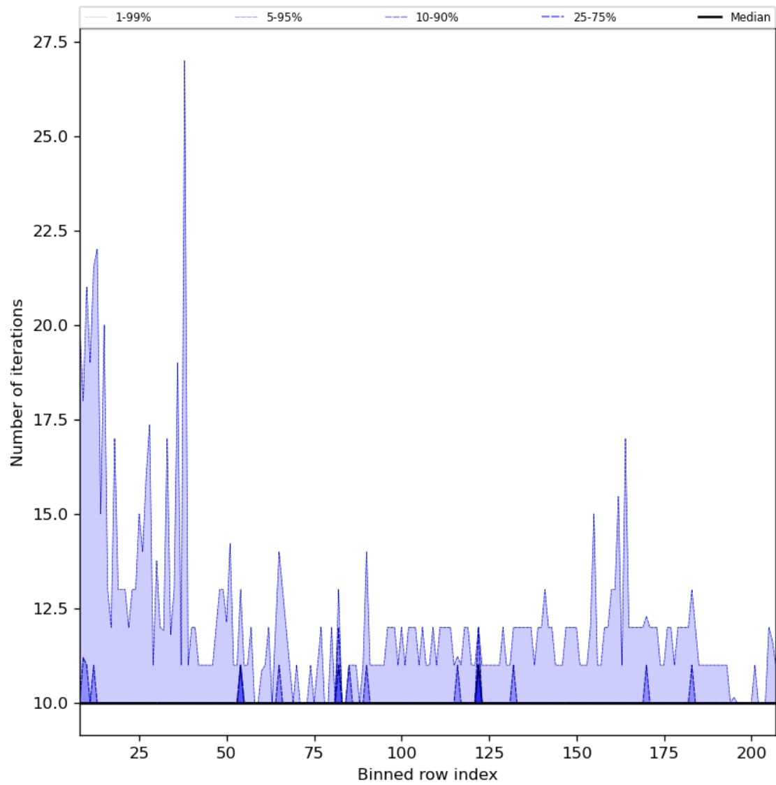
Figure 42: Along track statistics of “Number of iterations” for 2024-08-17 to 2024-08-19
