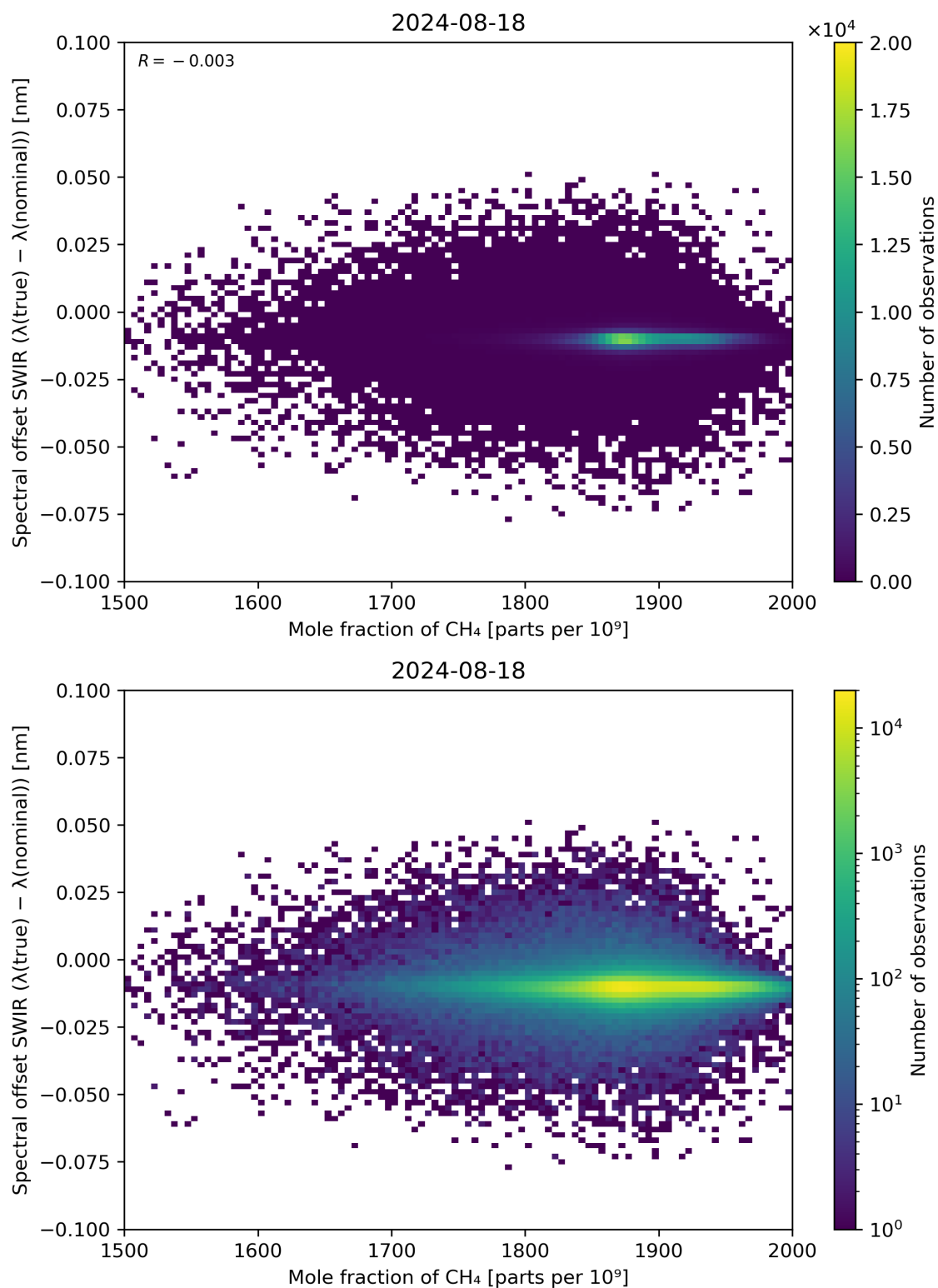
Figure 86: Scatter density plot of “Mole fraction of CH 4 ” against “Spectral offset SWIR ( \lambda(\text{true}) - \lambda(\text{nominal}) )” for 2024-08-17 to 2024-08-19.
