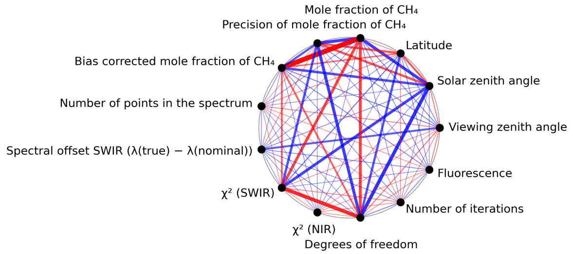
Figure 1: Map of correlation graph for 2024-08-17 to 2024-08-19.
