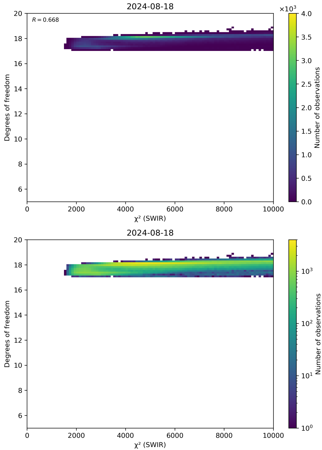
Figure 48: Scatter density plot of “ \chi^2 (SWIR)” against “Degrees of freedom” for 2024-08-17 to 2024-08-19.
