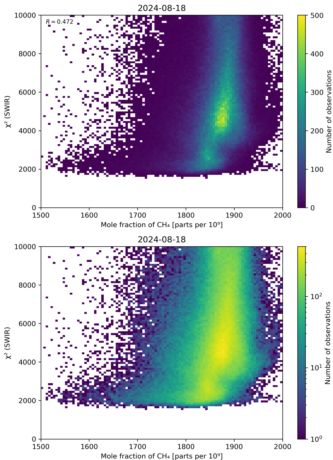
Figure 71: Scatter density plot of “Mole fraction of \text{CH}_4 ” against “ \chi^2 (SWIR)” for 2024-08-17 to 2024-08-19.
