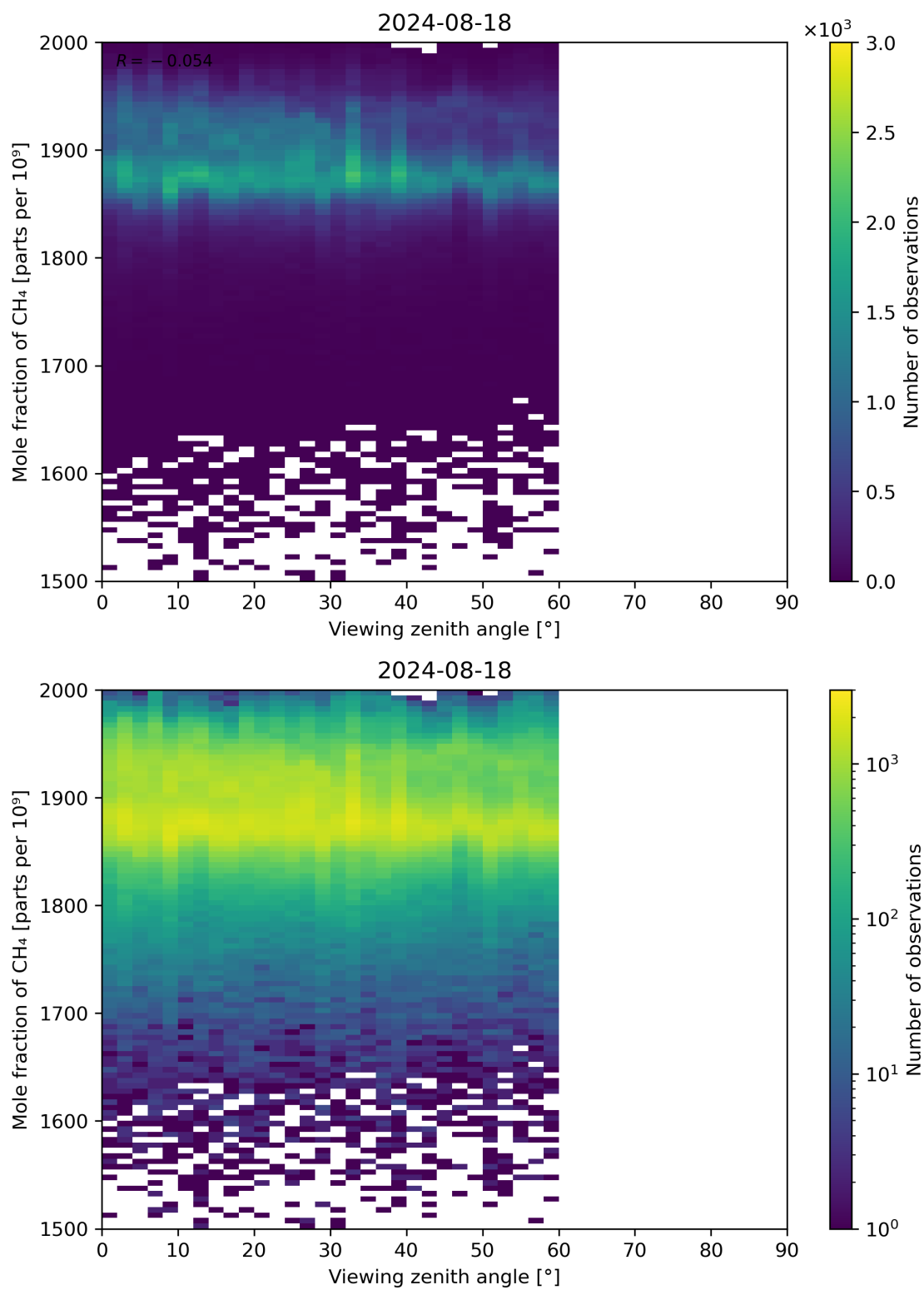
Figure 110: Scatter density plot of “Viewing zenith angle” against “Mole fraction of CH 4 ” for 2024-08-17 to 2024-08-19.
