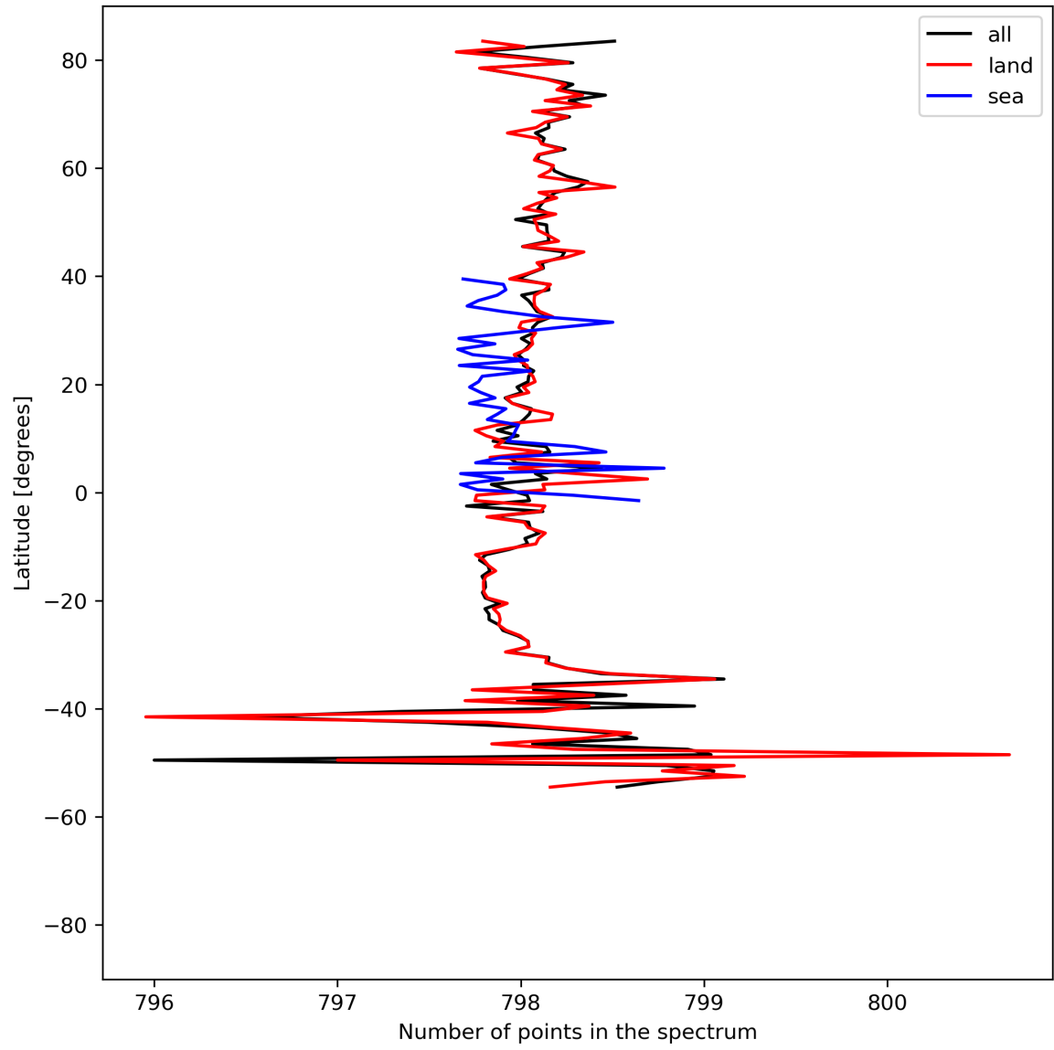
Figure 15: Zonal average of “Number of points in the spectrum” for 2024-08-17 to 2024-08-19.
