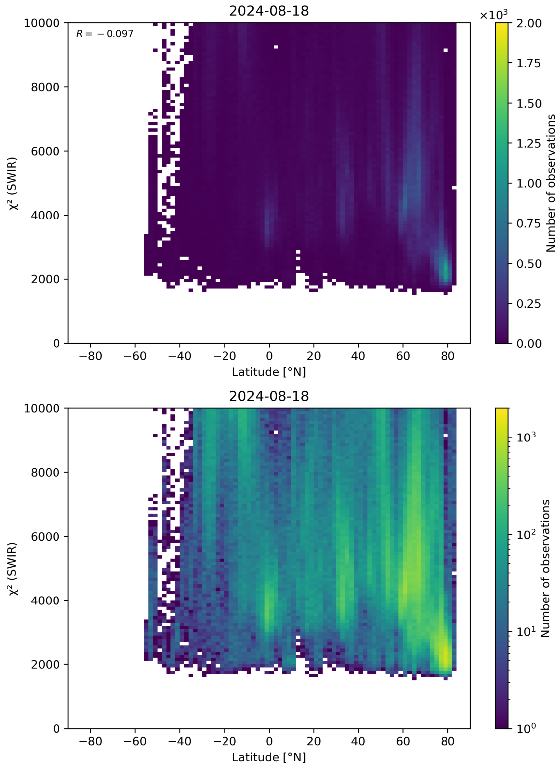
Figure 54: Scatter density plot of “Latitude” against “ \chi^2 (SWIR)” for 2024-08-17 to 2024-08-19.
