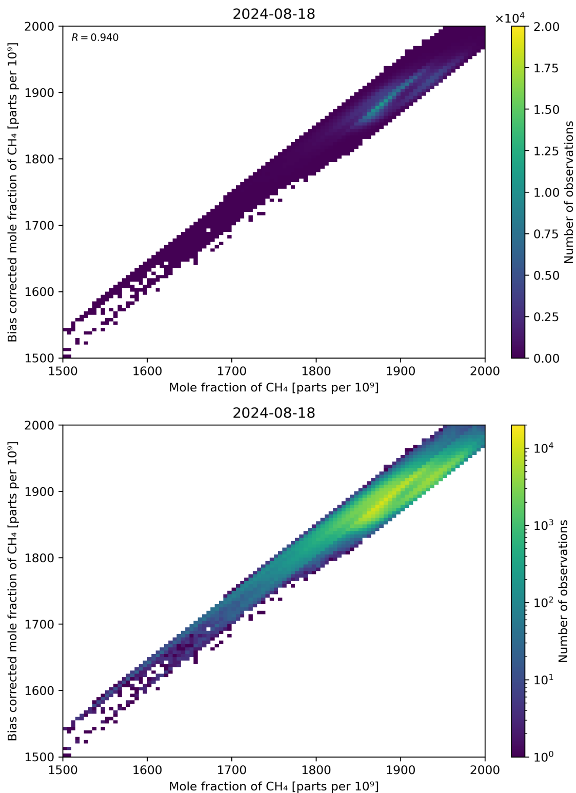
Figure 74: Scatter density plot of “Mole fraction of CH 4 ” against “Bias corrected mole fraction of CH 4 ” for 2024-08-17 to 2024-08-19.
