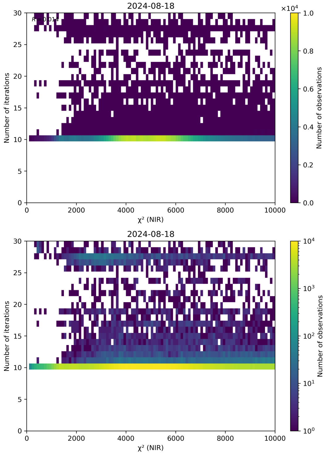
Figure 46: Scatter density plot of “ \chi^2 (NIR)” against “Number of iterations” for 2024-08-17 to 2024-08-19.
