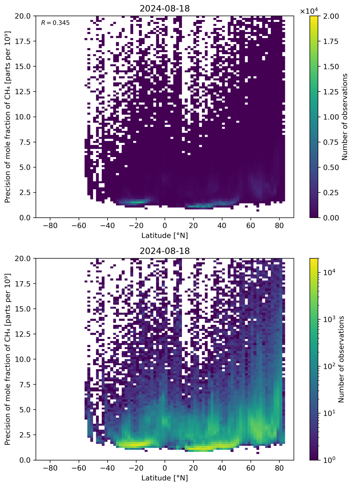
Figure 59: Scatter density plot of “Latitude” against “Precision of mole fraction of \text{CH}_4 ” for 2024-08-17 to 2024-08-19.
