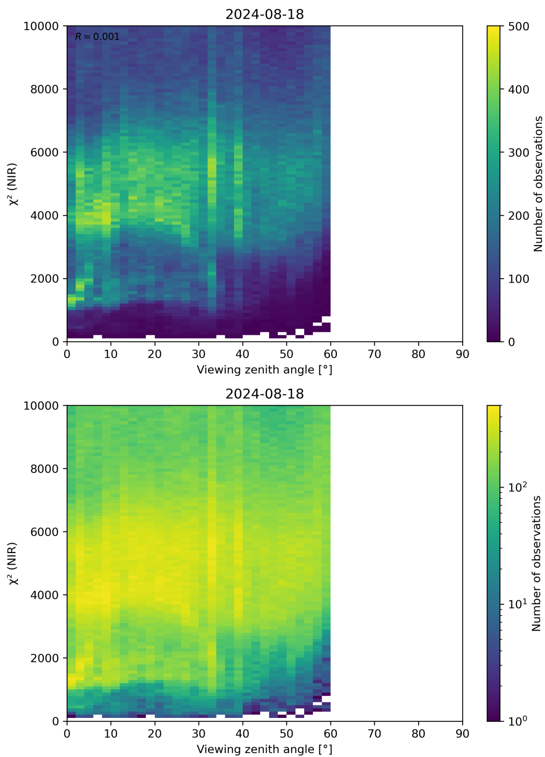
Figure 105: Scatter density plot of “Viewing zenith angle” against “ \chi^2 (NIR)” for 2024-08-17 to 2024-08-19.
