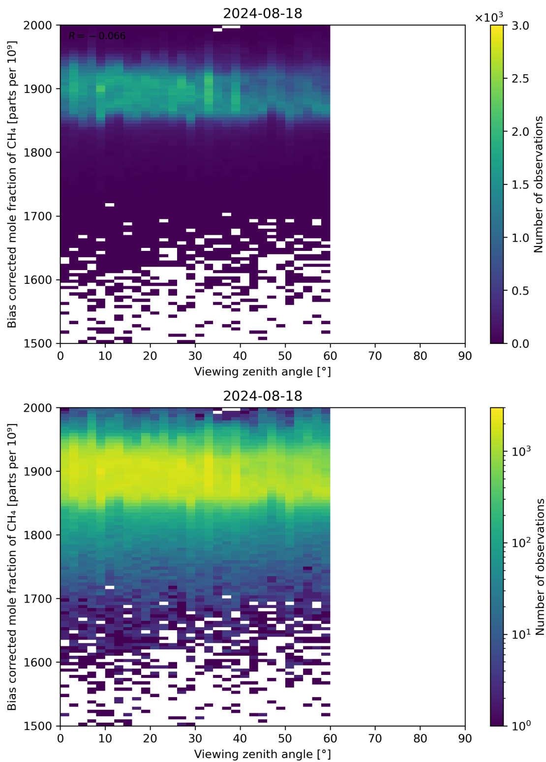
Figure 111: Scatter density plot of “Viewing zenith angle” against “Bias corrected mole fraction of CH 4 ” for 2024-08-17 to 2024-08-19.
