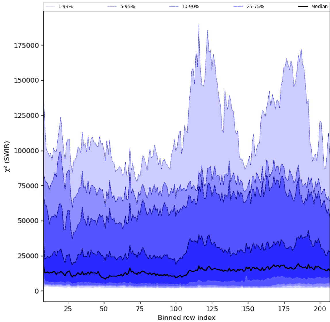
Figure 39: Along track statistics of “ \chi^2 (SWIR)” for 2024-08-17 to 2024-08-19
