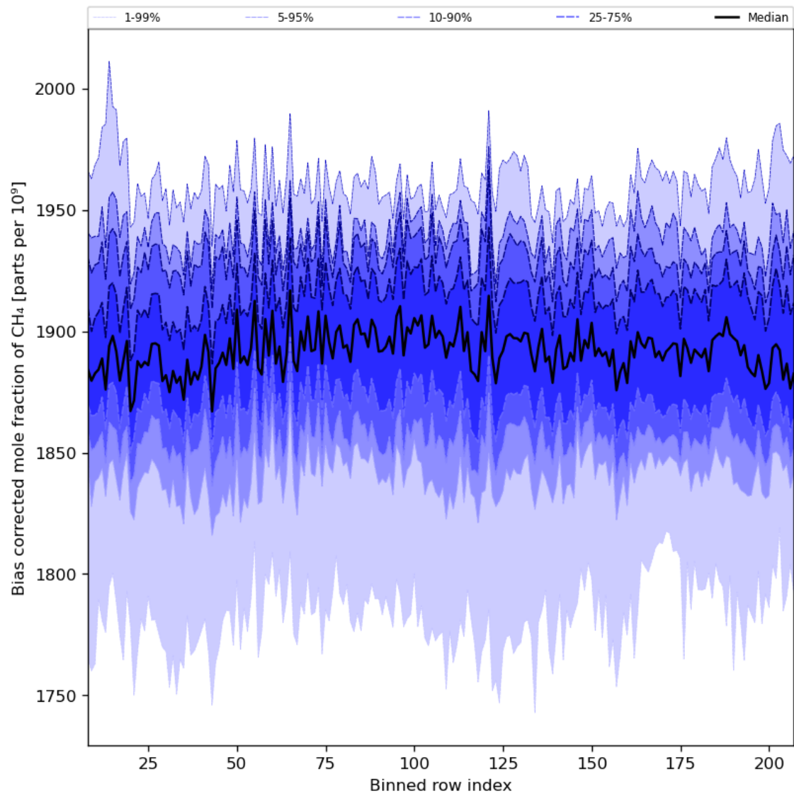
Figure 36: Along track statistics of “Bias corrected mole fraction of CH 4 ” for 2024-08-17 to 2024-08-19
