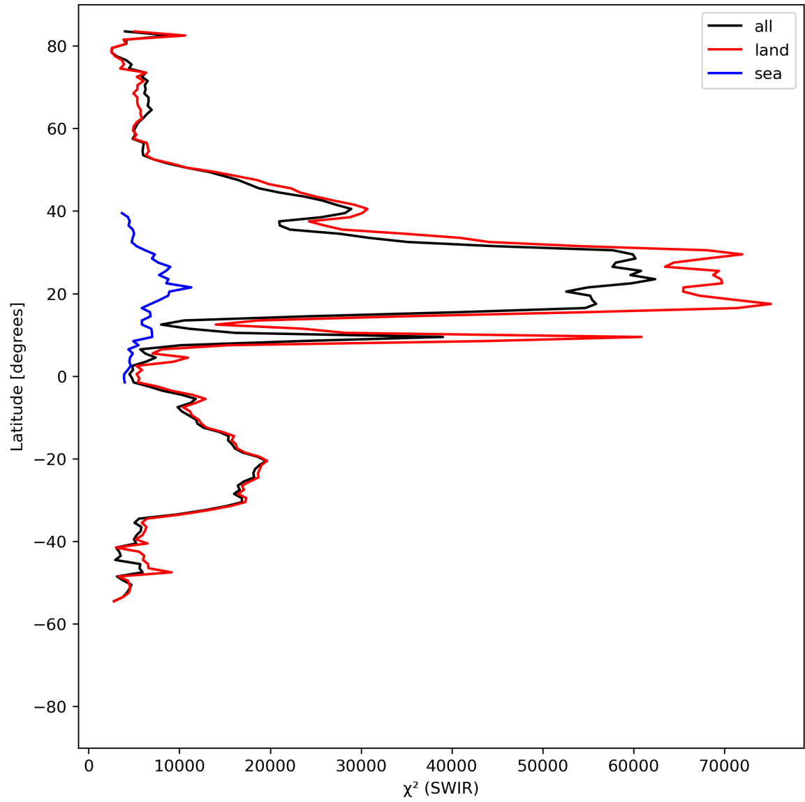
Figure 17: Zonal average of “ \chi^2 (SWIR)” for 2024-08-17 to 2024-08-19.
