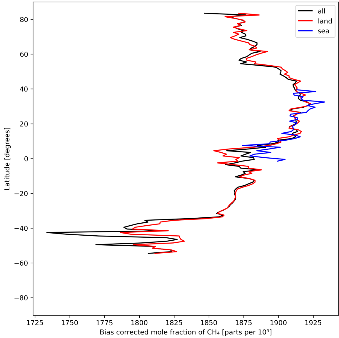
Figure 14: Zonal average of “Bias corrected mole fraction of CH 4 ” for 2024-08-17 to 2024-08-19.
