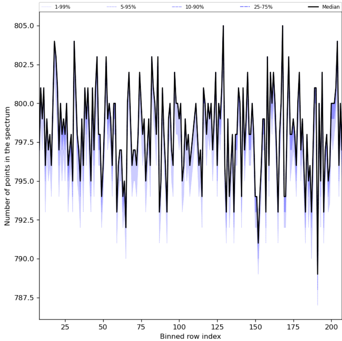
Figure 37: Along track statistics of “Number of points in the spectrum” for 2024-08-17 to 2024-08-19
