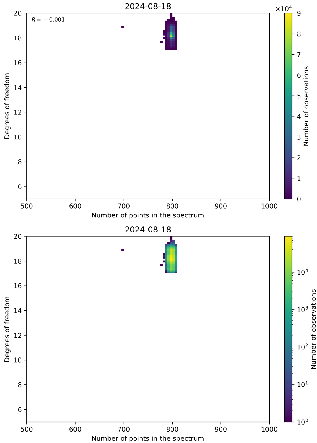
Figure 90: Scatter density plot of “Number of points in the spectrum” against “Degrees of freedom” for 2024-08-17 to 2024-08-19.
