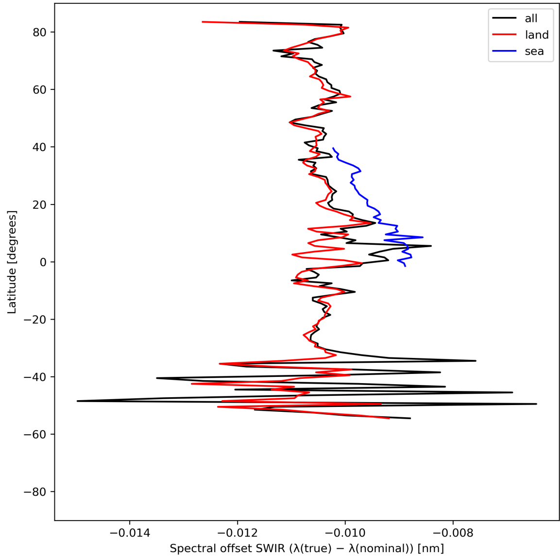
Figure 16: Zonal average of “Spectral offset SWIR ( \lambda(\text{true}) - \lambda(\text{nominal}) )” for 2024-08-17 to 2024-08-19.
