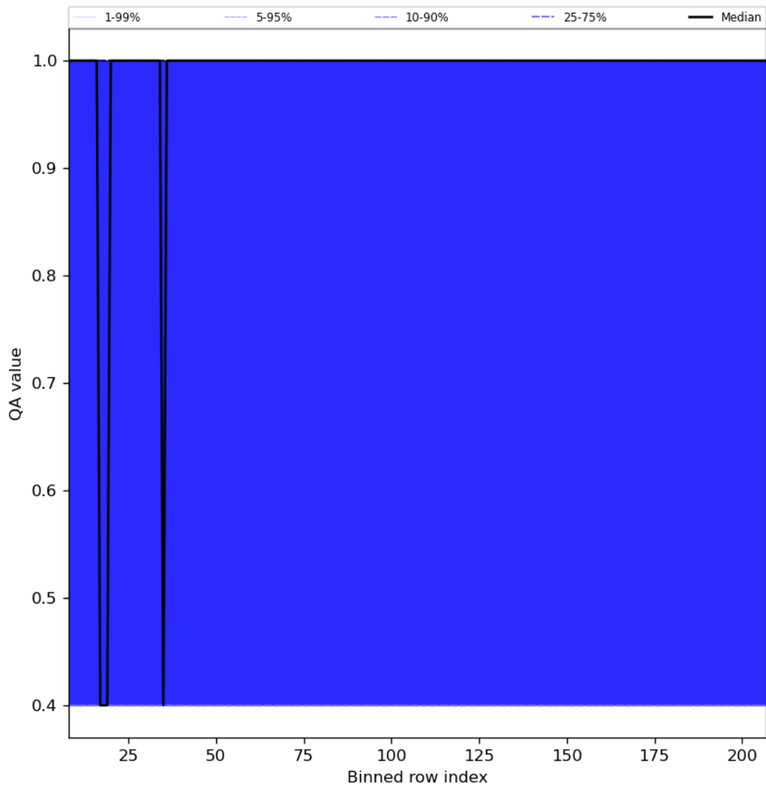
Figure 33: Along track statistics of “QA value” for 2024-08-17 to 2024-08-19
