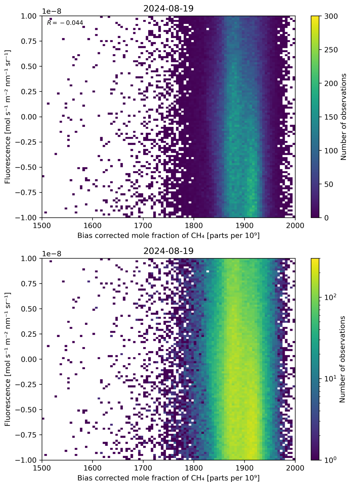
Figure 66: Scatter density plot of “Bias corrected mole fraction of \text{CH}_4 ” against “Fluorescence” for 2024-08-18 to 2024-08-20.
