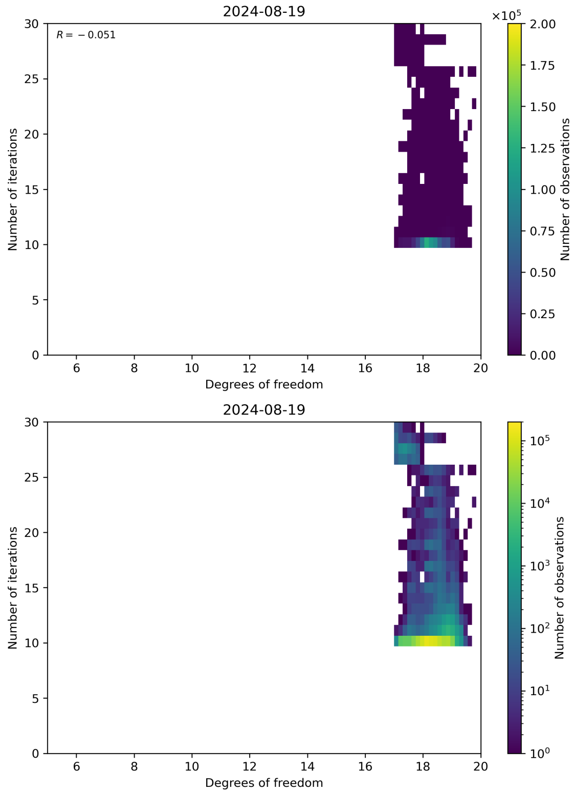
Figure 52: Scatter density plot of “Degrees of freedom” against “Number of iterations” for 2024-08-18 to 2024-08-20.
