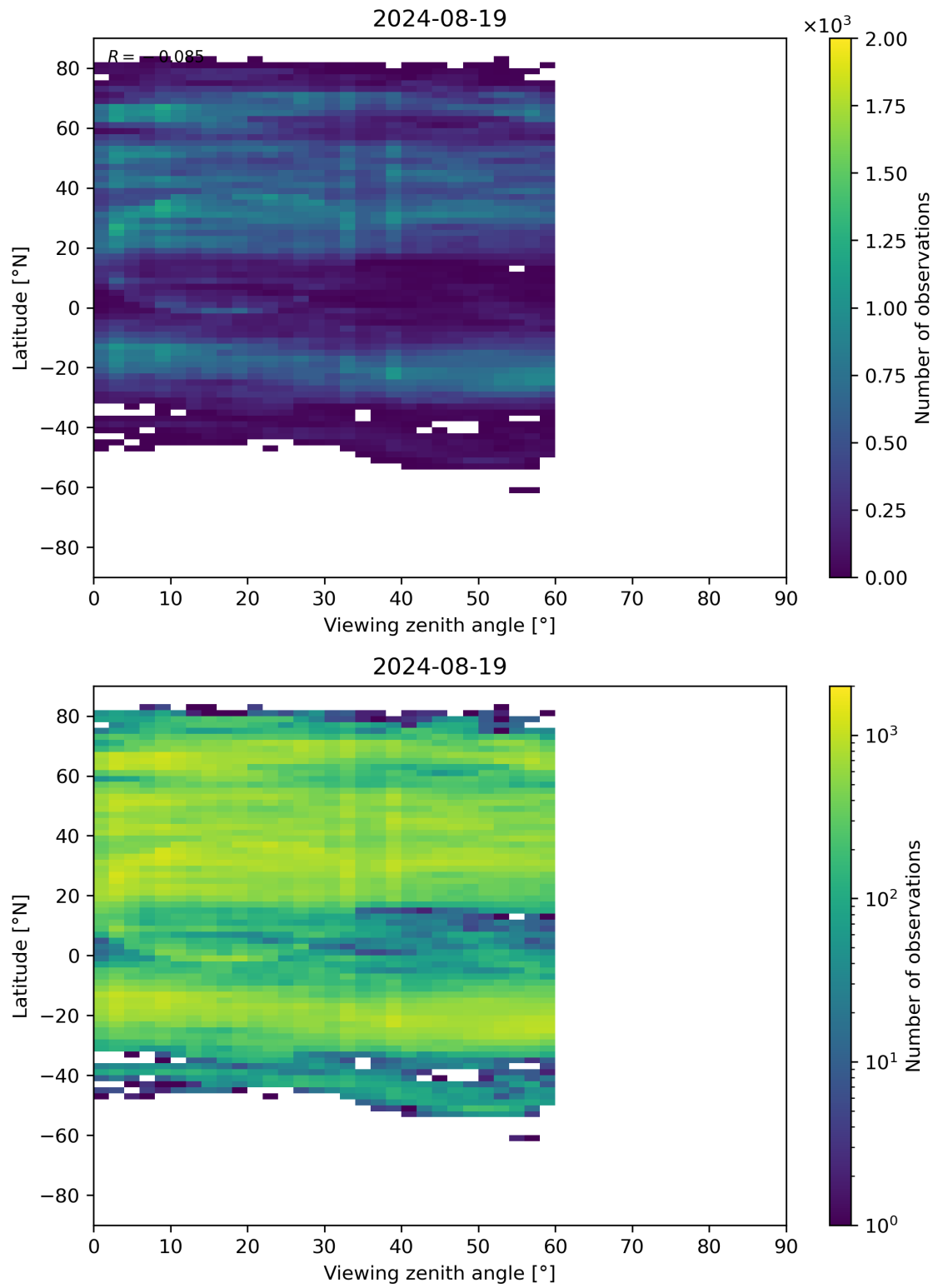
Figure 109: Scatter density plot of “Viewing zenith angle” against “Latitude” for 2024-08-18 to 2024-08-20.
