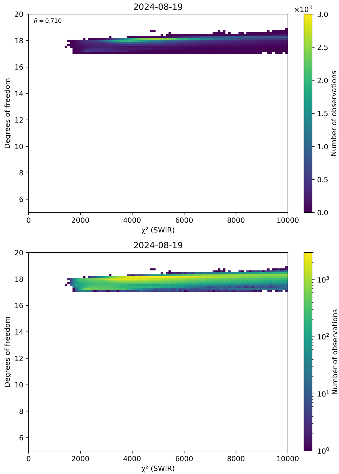
Figure 48: Scatter density plot of “ \chi^2 (SWIR)” against “Degrees of freedom” for 2024-08-18 to 2024-08-20.
