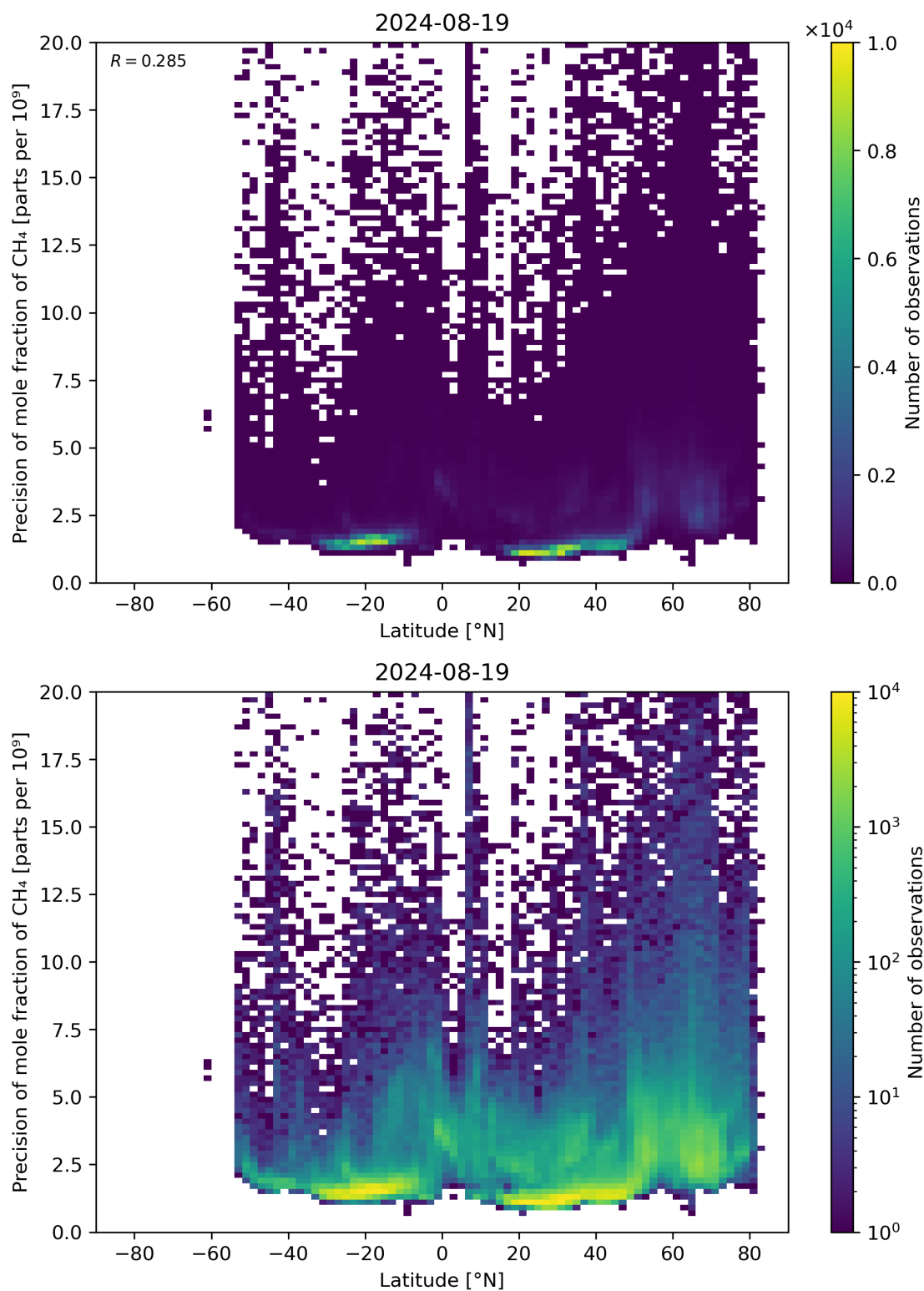
Figure 59: Scatter density plot of “Latitude” against “Precision of mole fraction of \text{CH}_4 ” for 2024-08-18 to 2024-08-20.
