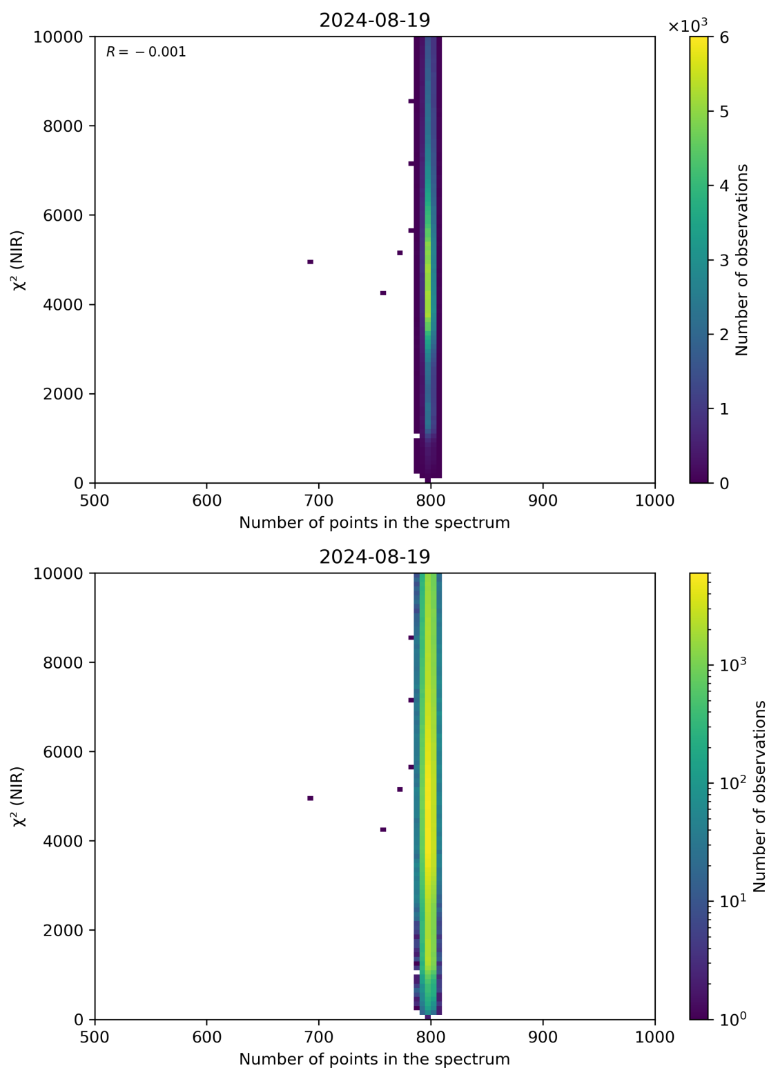
Figure 88: Scatter density plot of “Number of points in the spectrum” against “ \chi^2 (NIR)” for 2024-08-18 to 2024-08-20.
