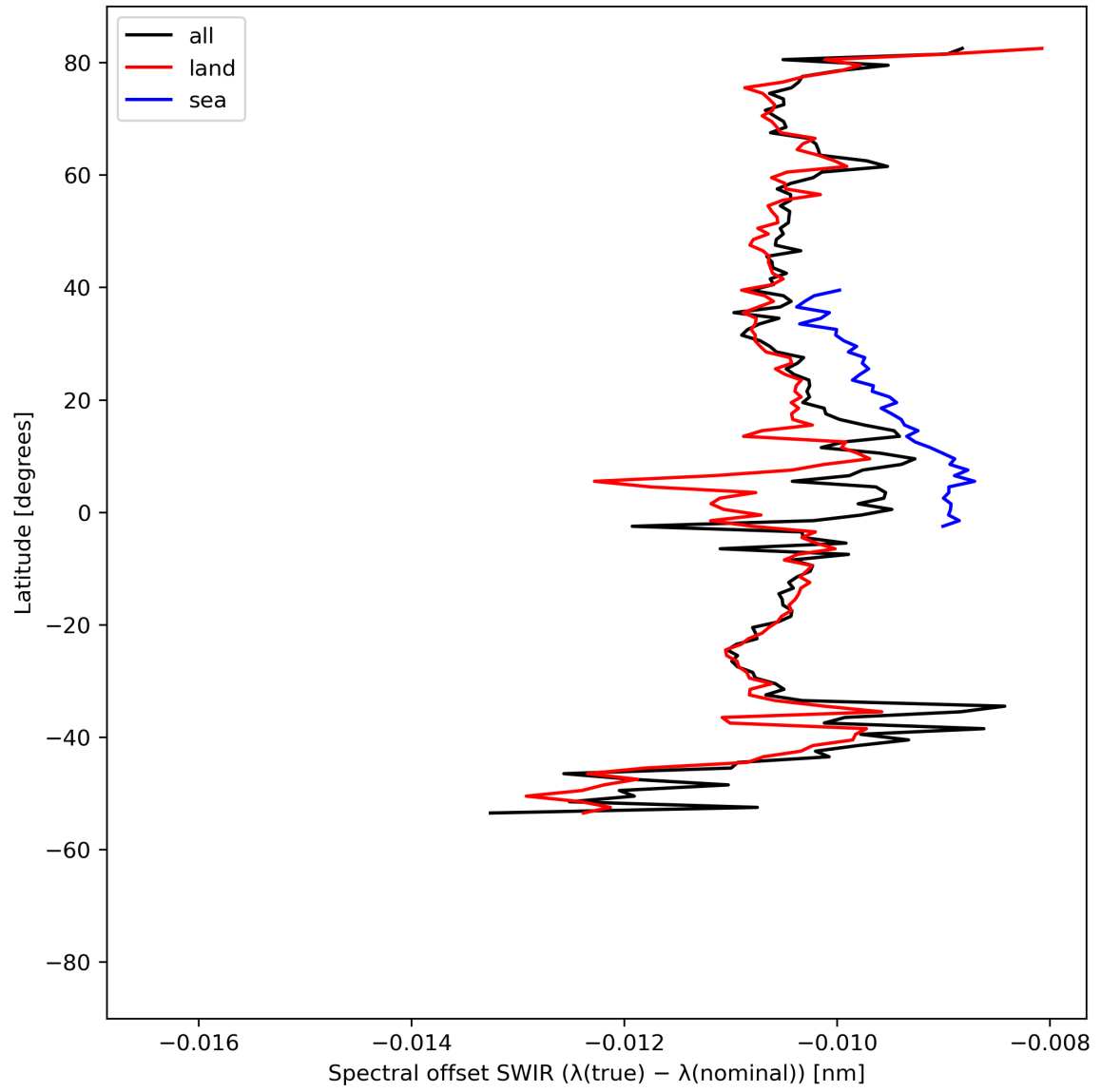
Figure 16: Zonal average of “Spectral offset SWIR ( \lambda(\text{true}) - \lambda(\text{nominal}) )” for 2024-08-18 to 2024-08-20.
