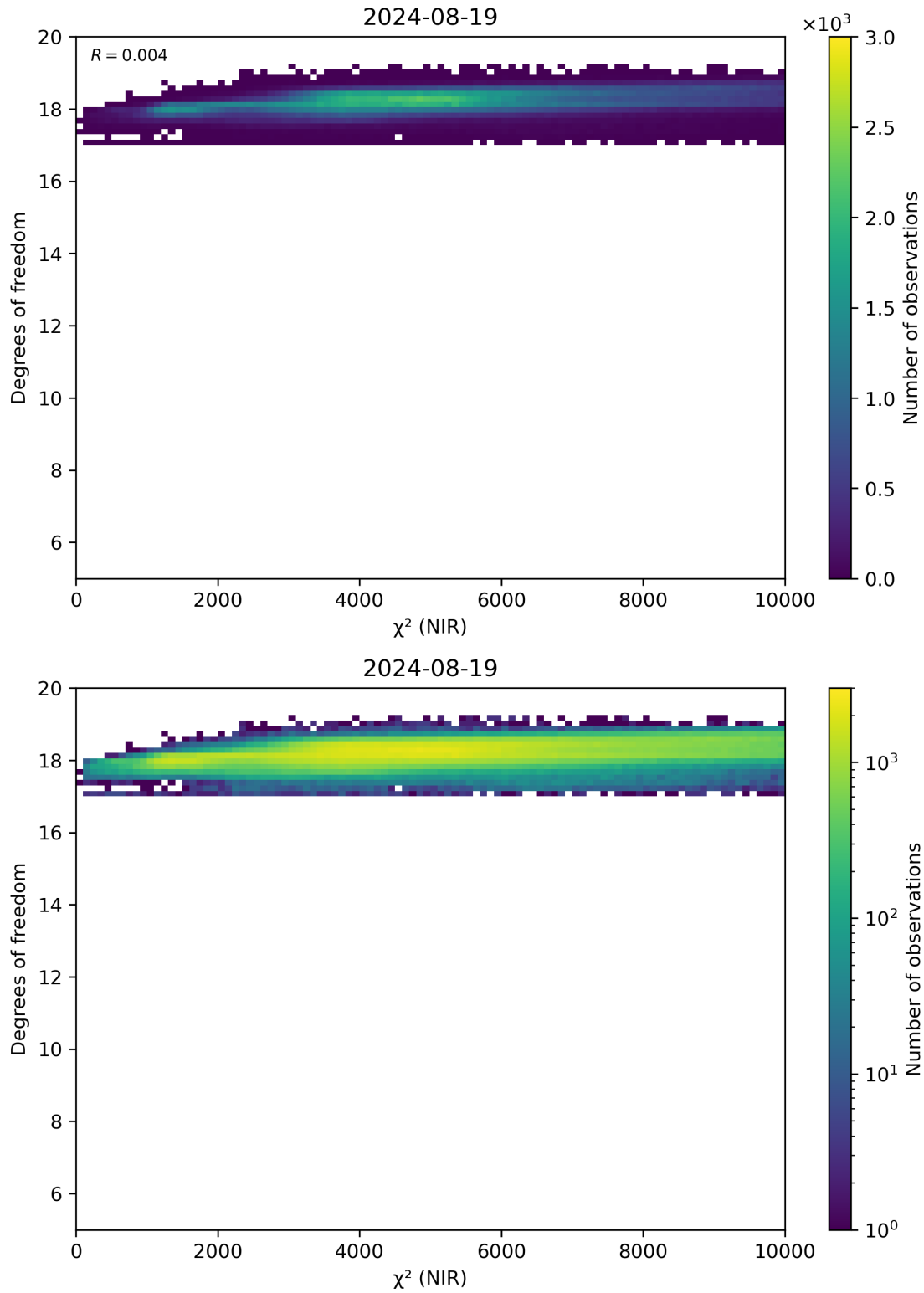
Figure 44: Scatter density plot of “ \chi^2 (NIR)” against “Degrees of freedom” for 2024-08-18 to 2024-08-20.
