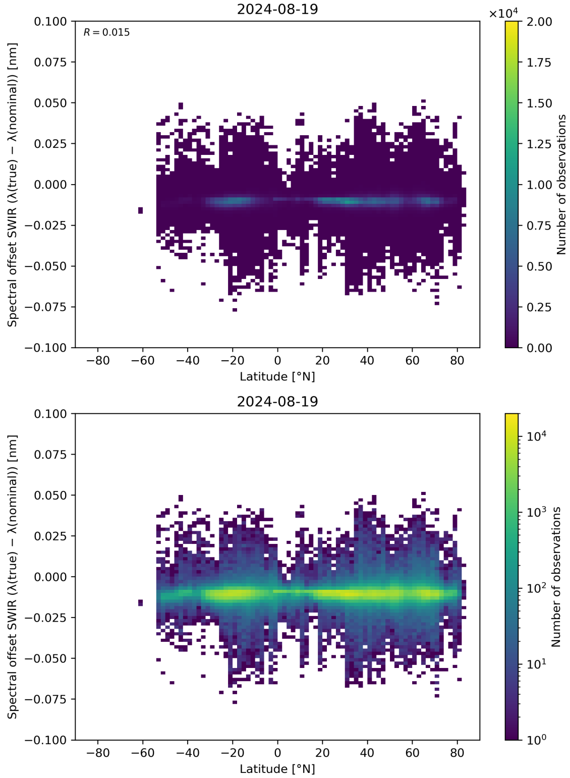
Figure 62: Scatter density plot of “Latitude” against “Spectral offset SWIR ( \lambda(\text{true}) - \lambda(\text{nominal}) )” for 2024-08-18 to 2024-08-20.
