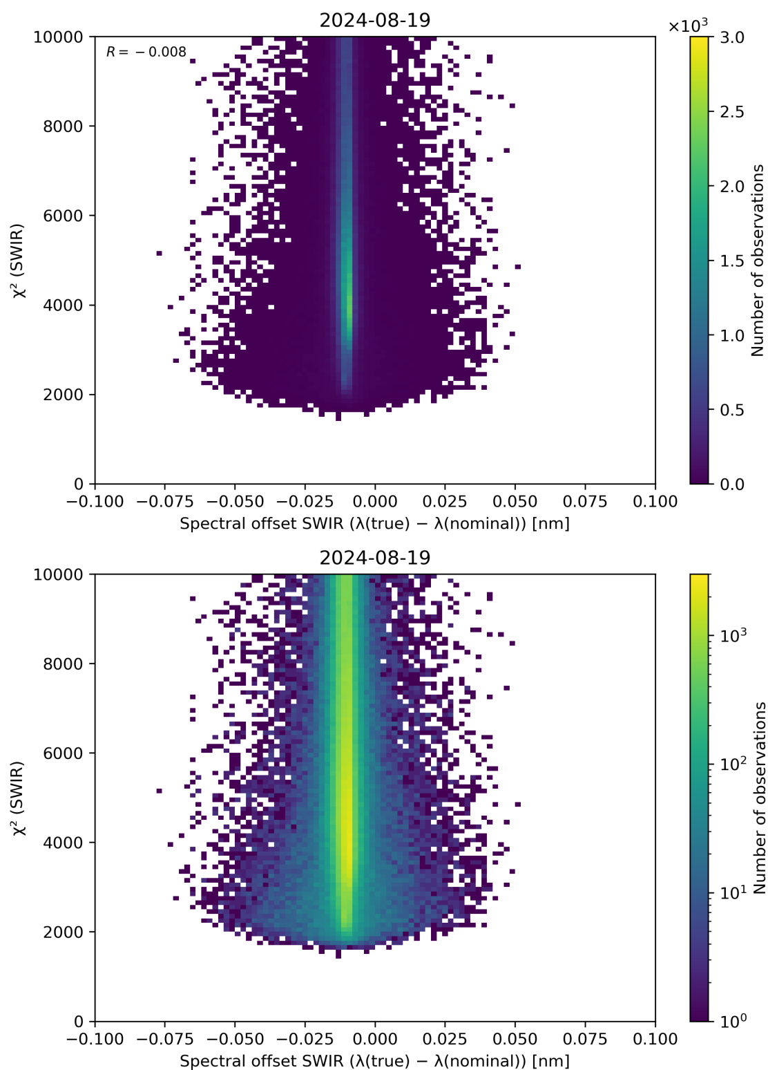
Figure 118: Scatter density plot of “Spectral offset SWIR ( \lambda(\text{true}) - \lambda(\text{nominal}) )” against “ \chi^2 (SWIR)” for 2024-08-18 to 2024-08-20.
