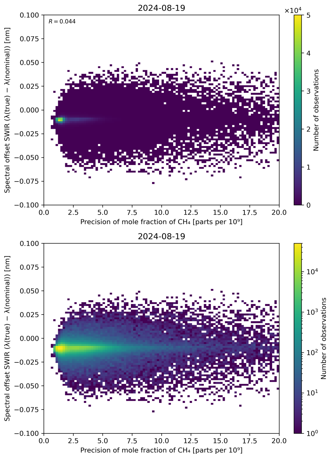
Figure 85: Scatter density plot of “Precision of mole fraction of CH 4 ” against “Spectral offset SWIR ( \lambda(\text{true}) - \lambda(\text{nominal}) )” for 2024-08-18 to 2024-08-20.
