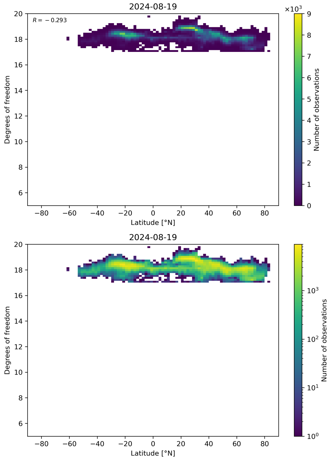
Figure 55: Scatter density plot of “Latitude” against “Degrees of freedom” for 2024-08-18 to 2024-08-20.
