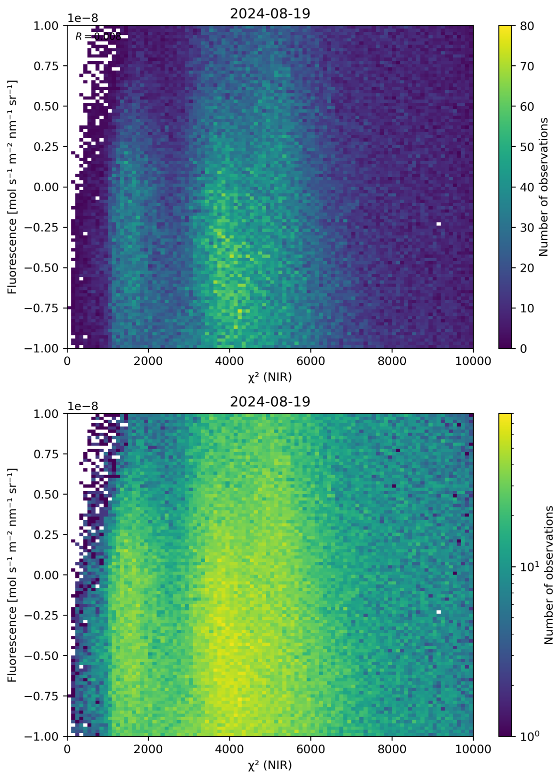
Figure 45: Scatter density plot of “ \chi^2 (NIR)” against “Fluorescence” for 2024-08-18 to 2024-08-20.
