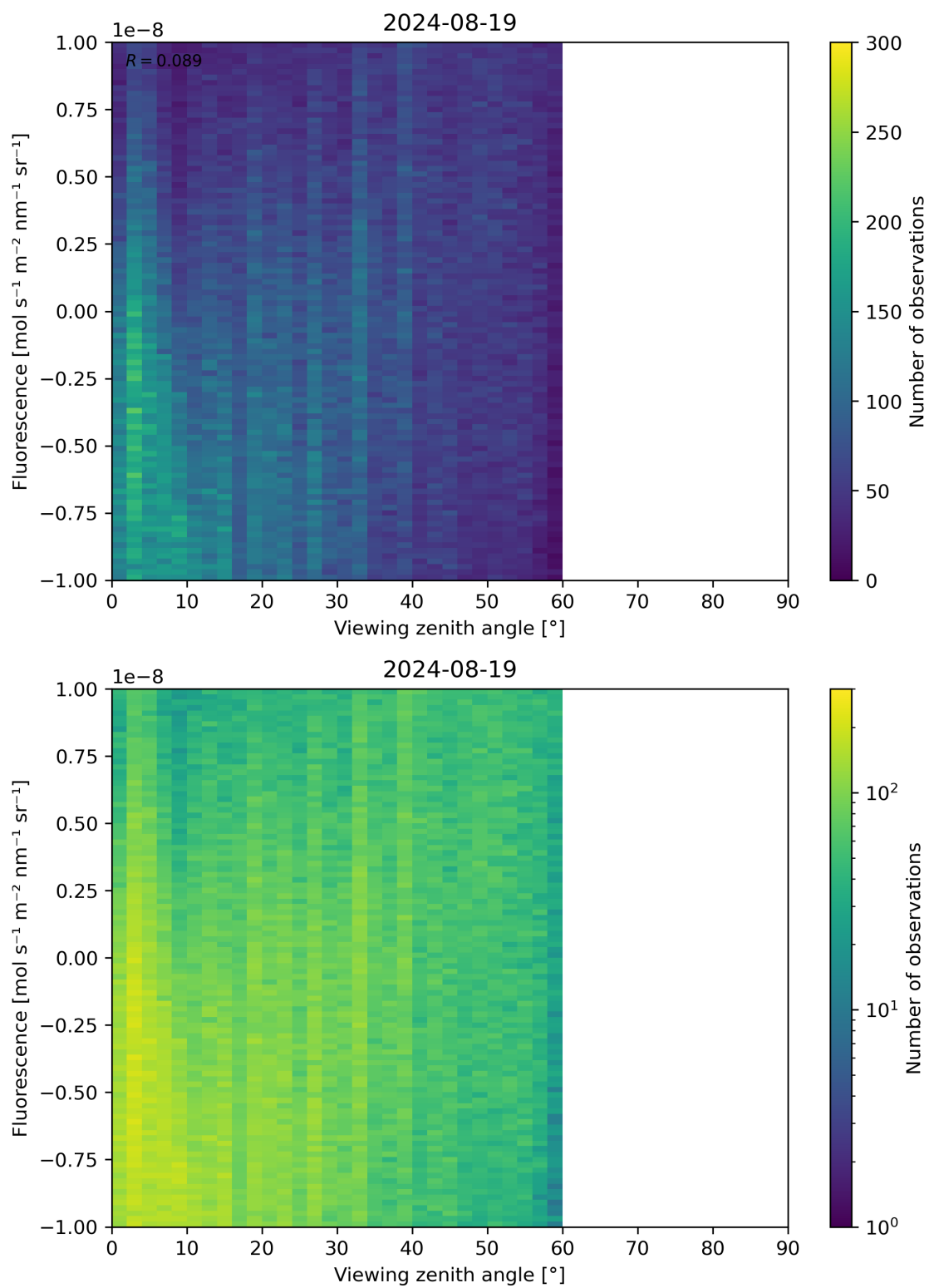
Figure 108: Scatter density plot of “Viewing zenith angle” against “Fluorescence” for 2024-08-18 to 2024-08-20.
