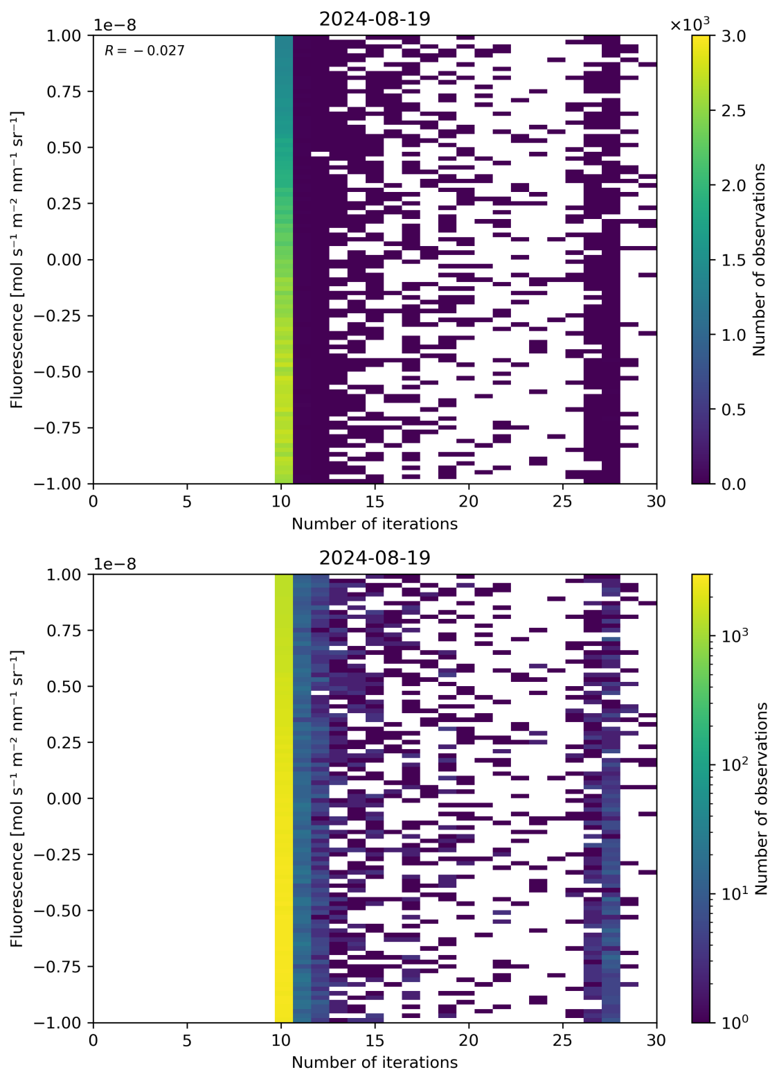
Figure 87: Scatter density plot of “Number of iterations” against “Fluorescence” for 2024-08-18 to 2024-08-20.
