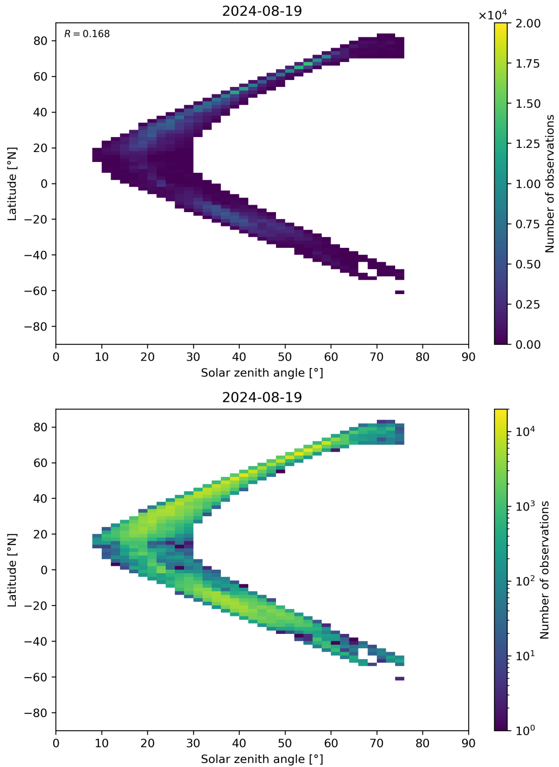
Figure 98: Scatter density plot of “Solar zenith angle” against “Latitude” for 2024-08-18 to 2024-08-20.
