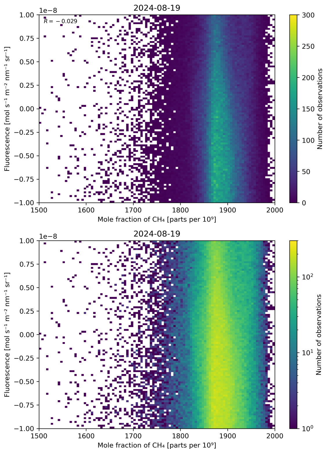
Figure 73: Scatter density plot of “Mole fraction of \text{CH}_4 ” against “Fluorescence” for 2024-08-18 to 2024-08-20.
