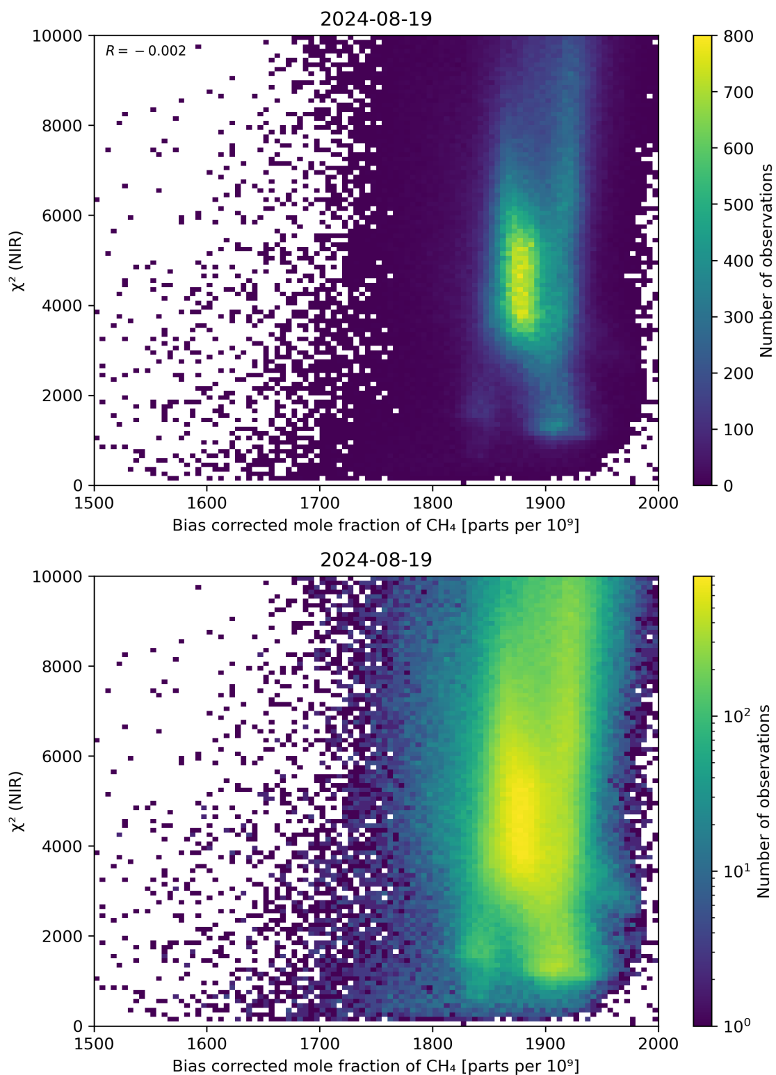
Figure 63: Scatter density plot of “Bias corrected mole fraction of CH 4 ” against “ \chi^2 (NIR)” for 2024-08-18 to 2024-08-20.
