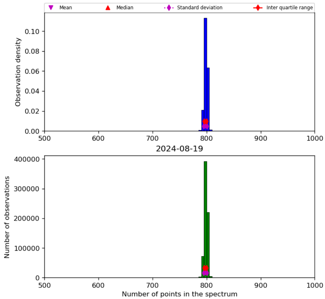
Figure 26: Histogram of “Number of points in the spectrum” for 2024-08-18 to 2024-08-20
