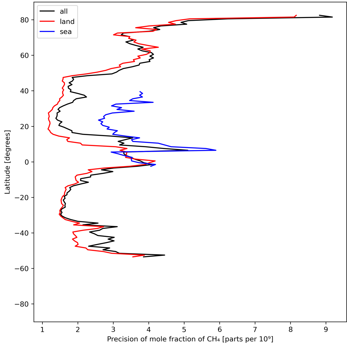
Figure 13: Zonal average of “Precision of mole fraction of CH 4 ” for 2024-08-18 to 2024-08-20.
