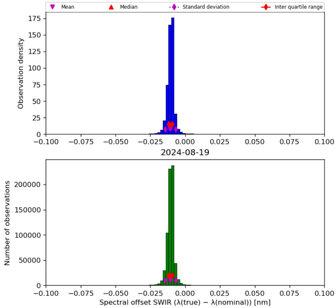
Figure 27: Histogram of “Spectral offset SWIR ( \lambda(\text{true}) - \lambda(\text{nominal}) )” for 2024-08-18 to 2024-08-20
