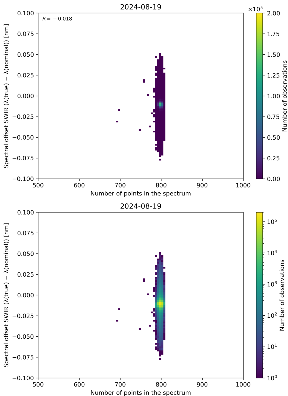
Figure 93: Scatter density plot of “Number of points in the spectrum” against “Spectral offset SWIR ( \lambda(\text{true}) - \lambda(\text{nominal}) )” for 2024-08-18 to 2024-08-20.
