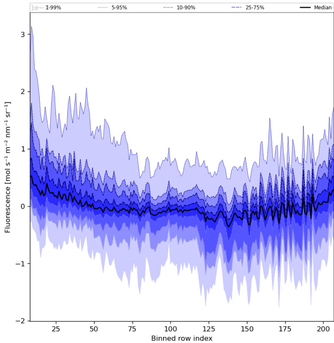
Figure 43: Along track statistics of “Fluorescence” for 2024-08-18 to 2024-08-20
