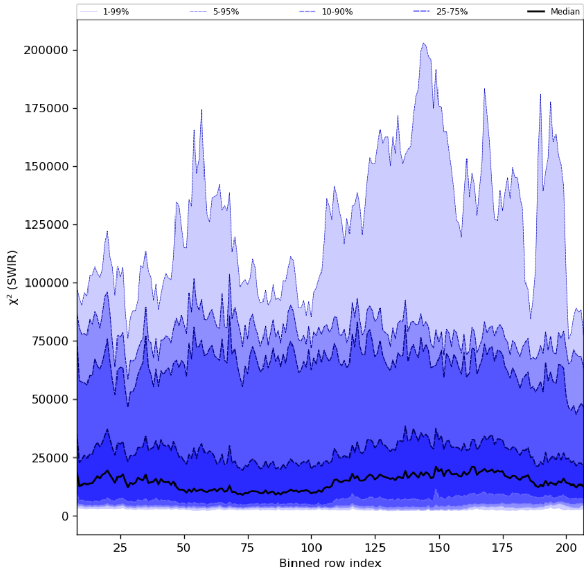
Figure 39: Along track statistics of " \chi^2 (SWIR)" for 2024-08-18 to 2024-08-20
