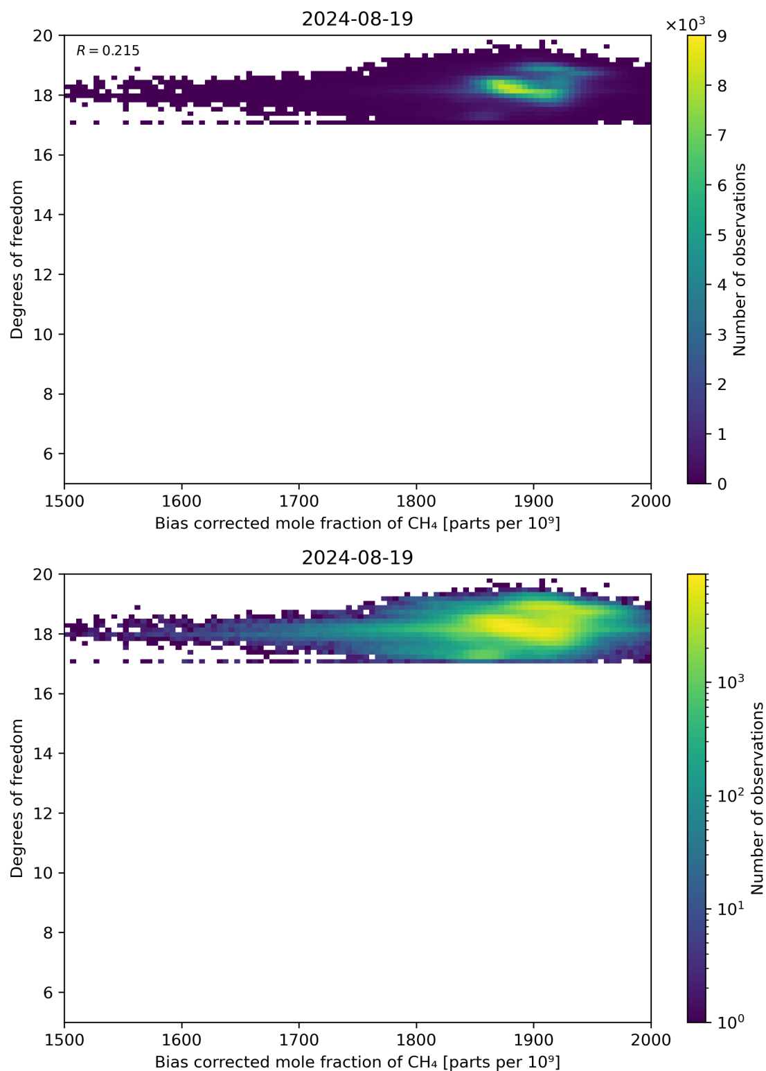
Figure 65: Scatter density plot of “Bias corrected mole fraction of CH 4 ” against “Degrees of freedom” for 2024-08-18 to 2024-08-20.
