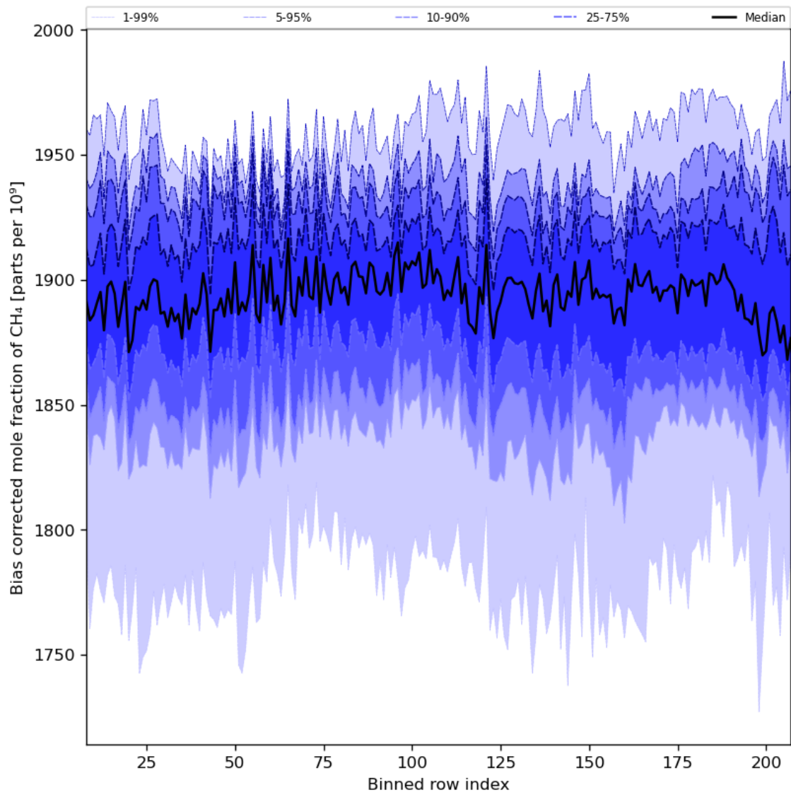
Figure 36: Along track statistics of “Bias corrected mole fraction of CH 4 ” for 2024-08-18 to 2024-08-20
