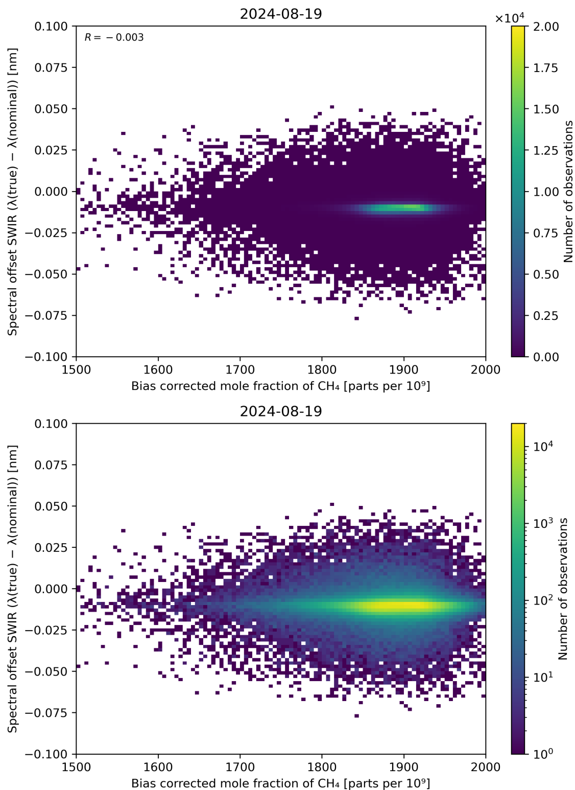
Figure 69: Scatter density plot of “Bias corrected mole fraction of \text{CH}_4 ” against “Spectral offset SWIR ( \lambda(\text{true}) - \lambda(\text{nominal}) )” for 2024-08-18 to 2024-08-20.
