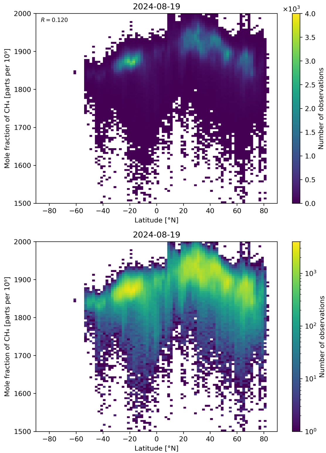
Figure 57: Scatter density plot of “Latitude” against “Mole fraction of \text{CH}_4 ” for 2024-08-18 to 2024-08-20.
