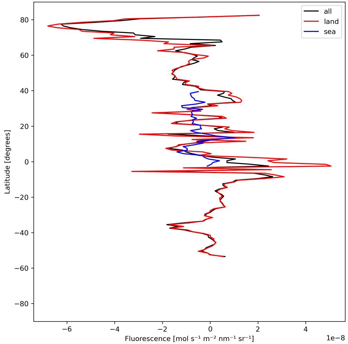
Figure 21: Zonal average of “Fluorescence” for 2024-08-18 to 2024-08-20.
