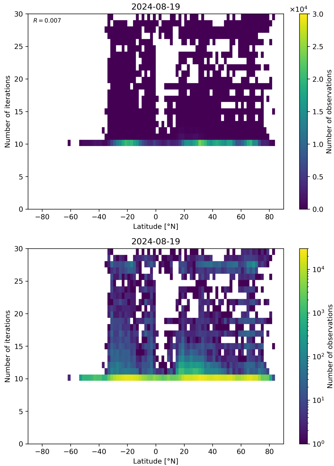
Figure 60: Scatter density plot of “Latitude” against “Number of iterations” for 2024-08-18 to 2024-08-20.
