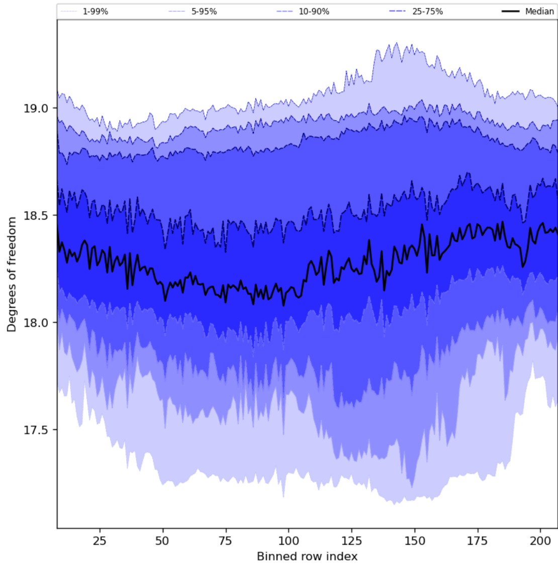
Figure 41: Along track statistics of “Degrees of freedom” for 2024-08-18 to 2024-08-20
