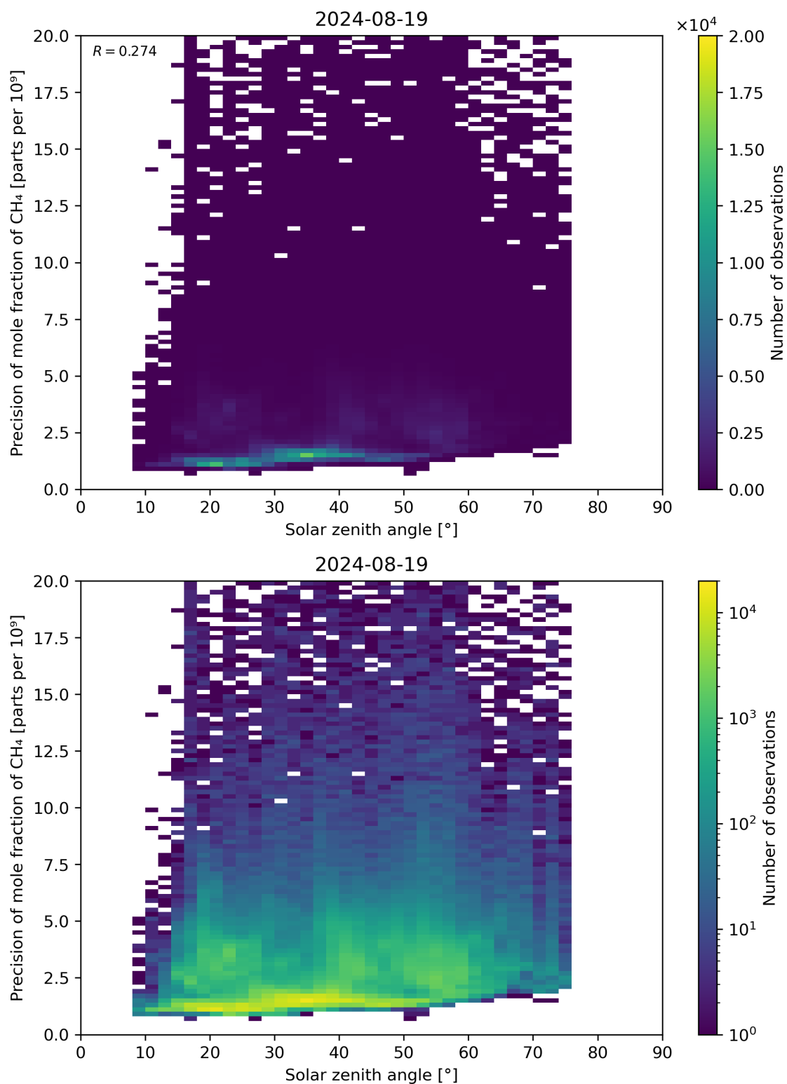
Figure 101: Scatter density plot of “Solar zenith angle” against “Precision of mole fraction of CH 4 ” for 2024-08-18 to 2024-08-20.
