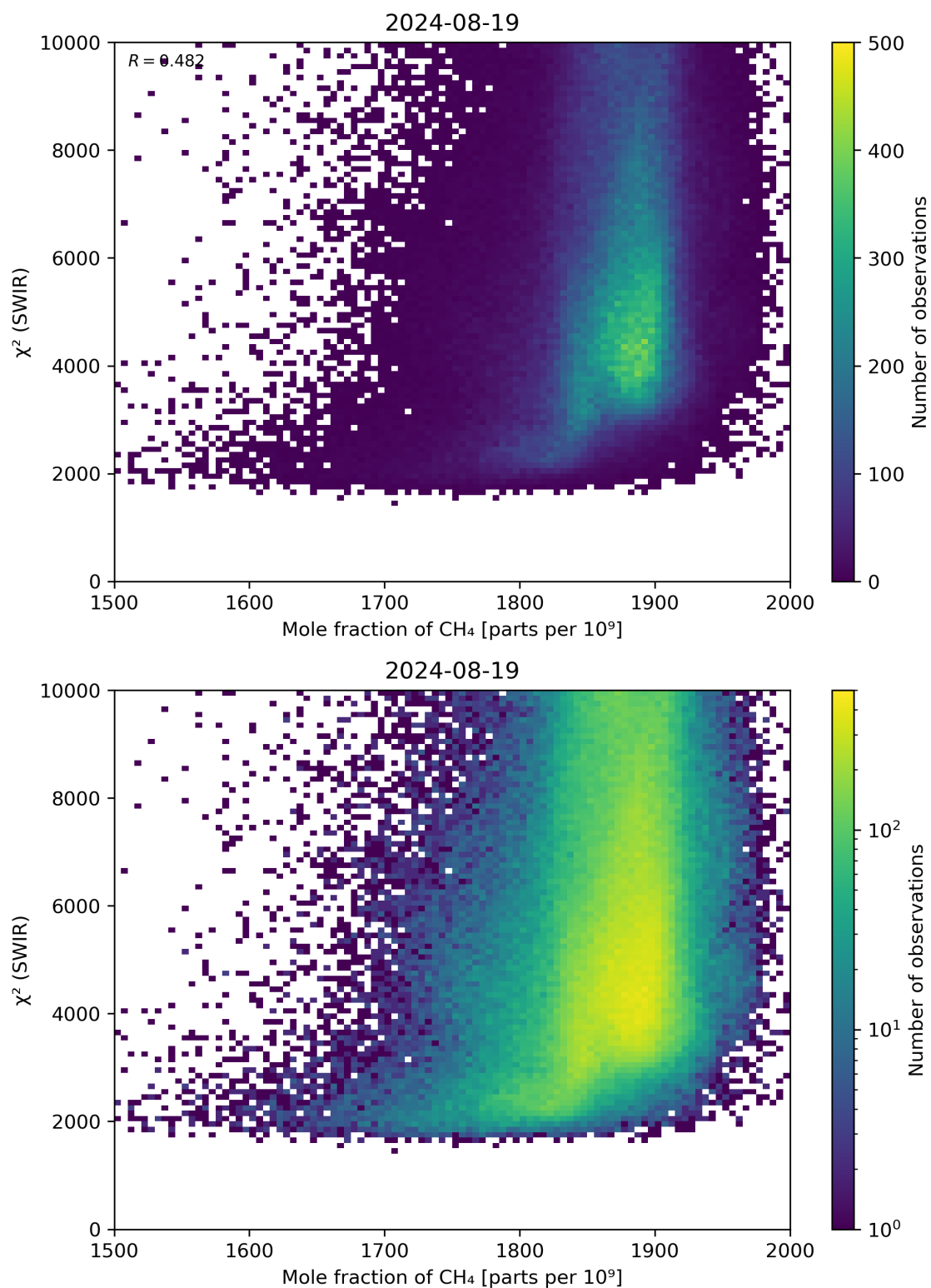
Figure 71: Scatter density plot of “Mole fraction of \text{CH}_4 ” against “ \chi^2 (SWIR)” for 2024-08-18 to 2024-08-20.
