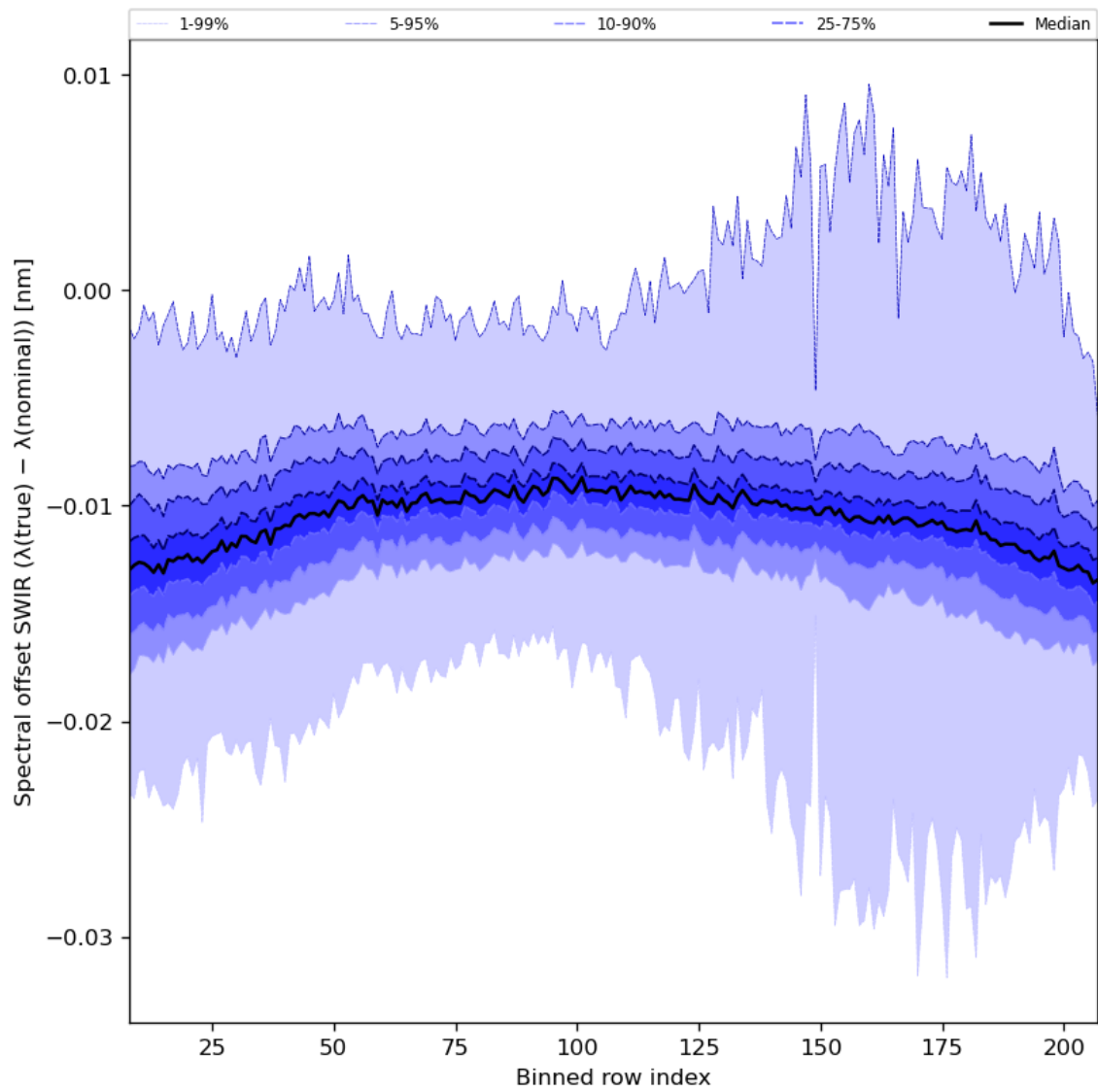
Figure 38: Along track statistics of “Spectral offset SWIR ( \lambda(\text{true}) - \lambda(\text{nominal}) )” for 2024-08-18 to 2024-08-20
