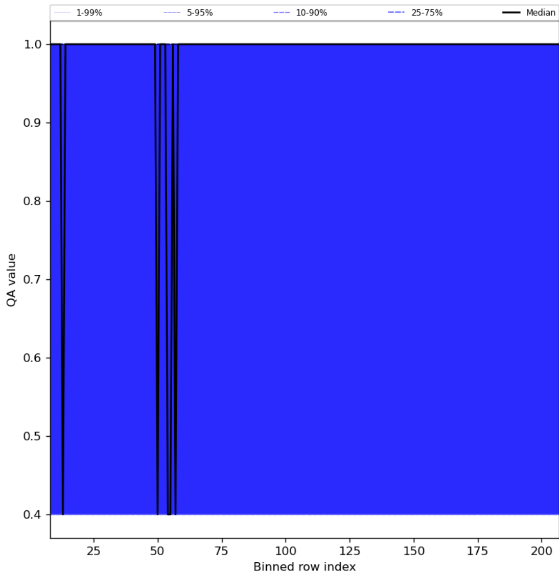
Figure 33: Along track statistics of “QA value” for 2024-08-18 to 2024-08-20
