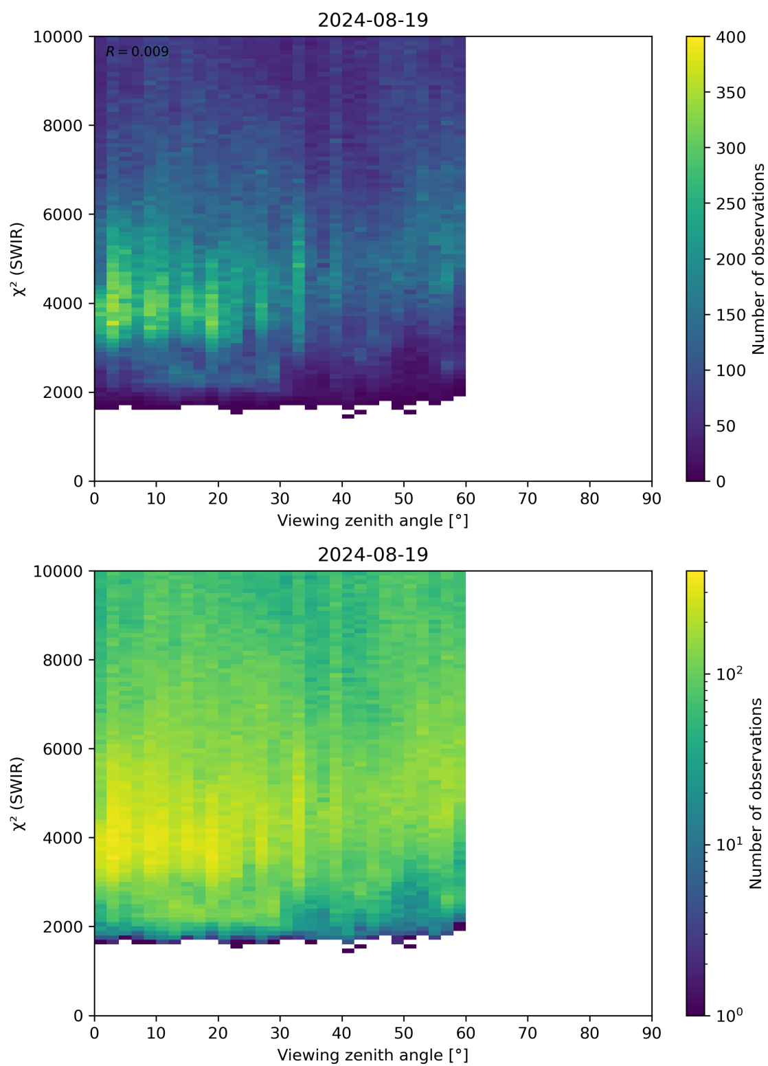
Figure 106: Scatter density plot of “Viewing zenith angle” against “ \chi^2 (SWIR)” for 2024-08-18 to 2024-08-20.
