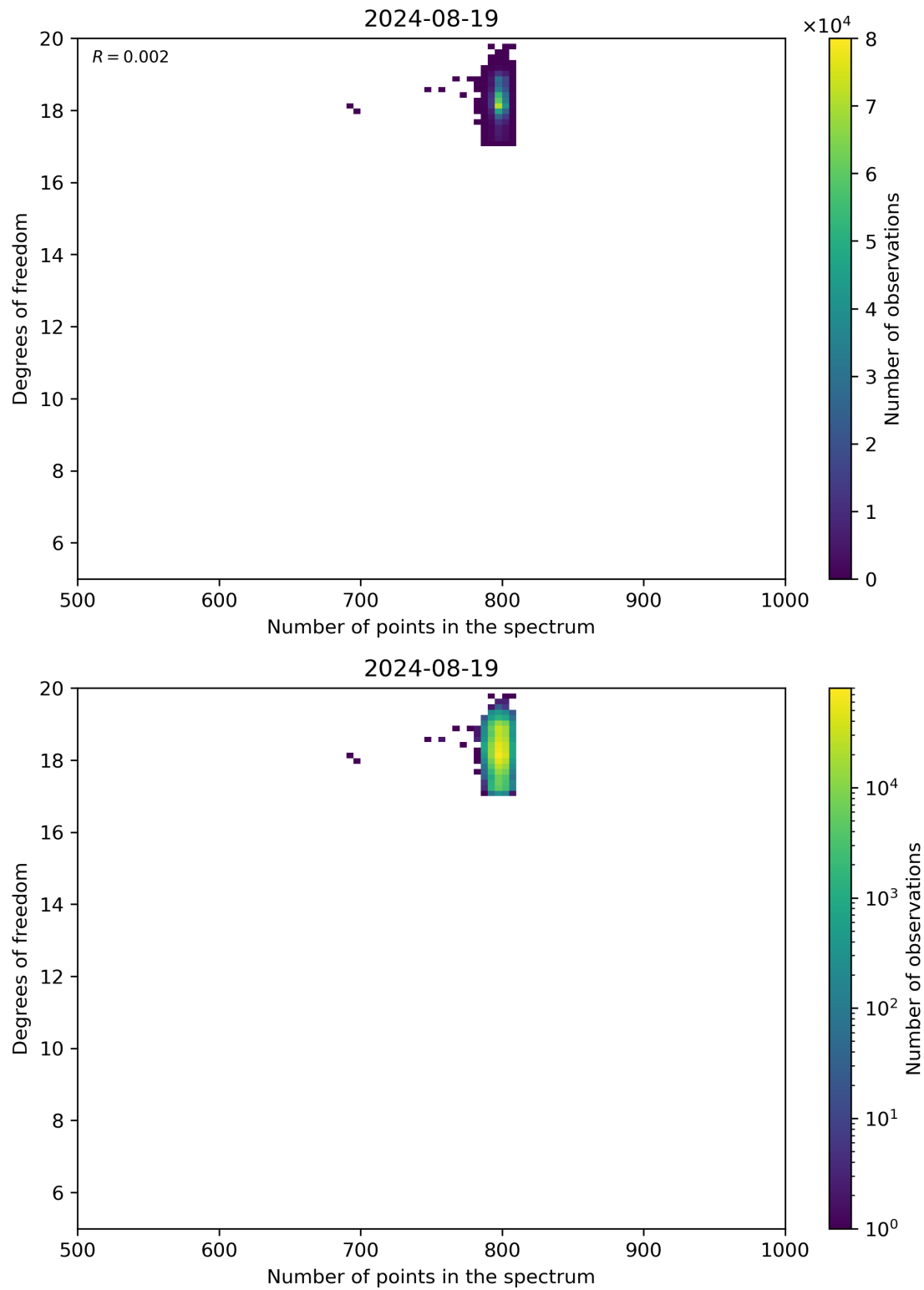
Figure 90: Scatter density plot of “Number of points in the spectrum” against “Degrees of freedom” for 2024-08-18 to 2024-08-20.
