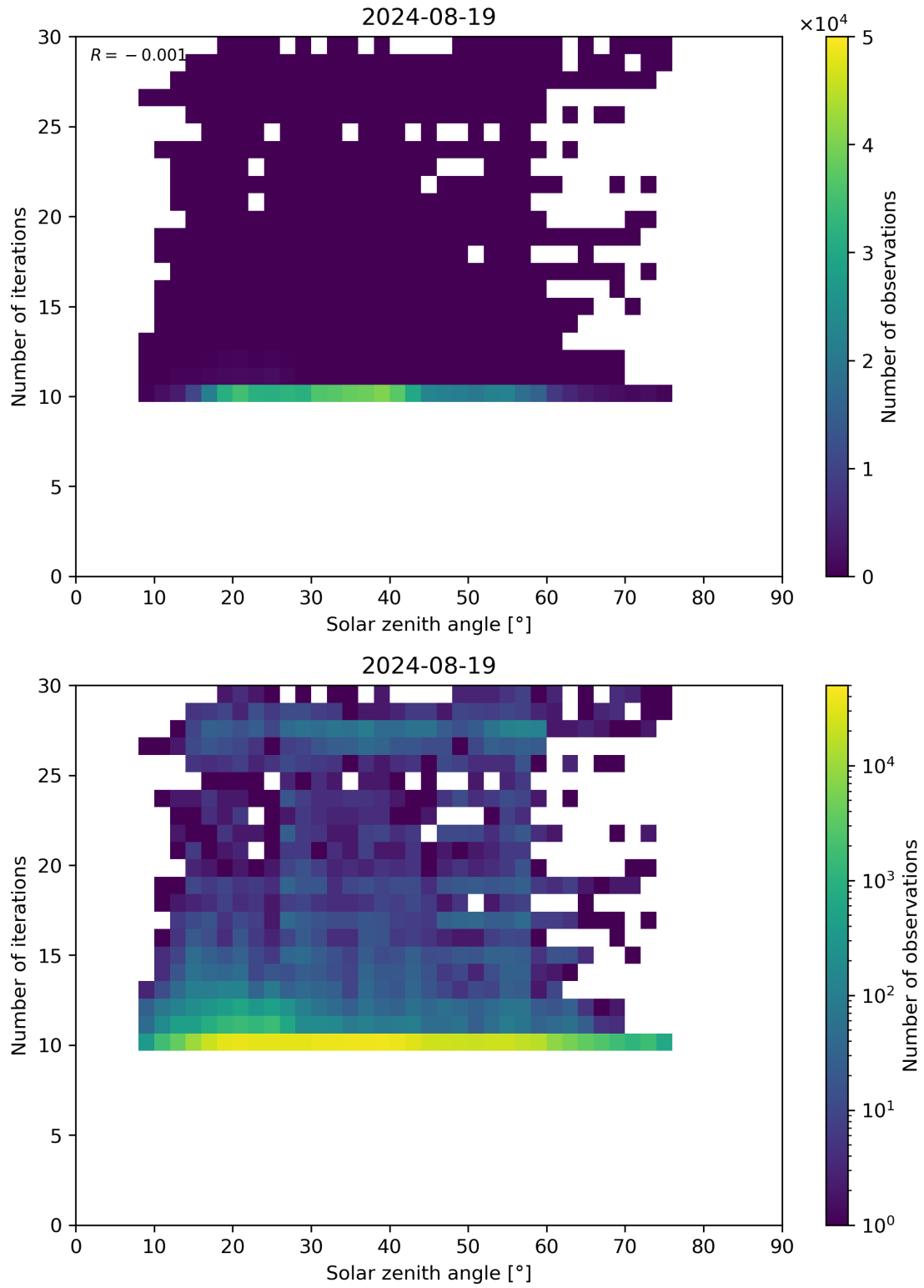
Figure 102: Scatter density plot of “Solar zenith angle” against “Number of iterations” for 2024-08-18 to 2024-08-20.
