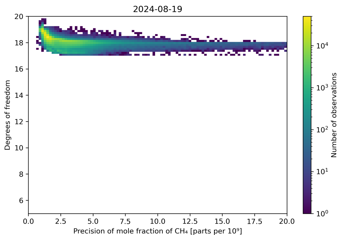
Figure 80: Scatter density plot of “Precision of mole fraction of CH 4 ” against “Degrees of freedom” for 2024-08-18 to 2024-08-20.
