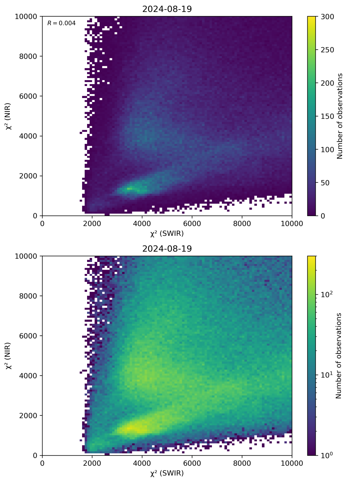
Figure 47: Scatter density plot of “ \chi^2 (SWIR)” against “ \chi^2 (NIR)” for 2024-08-18 to 2024-08-20.
