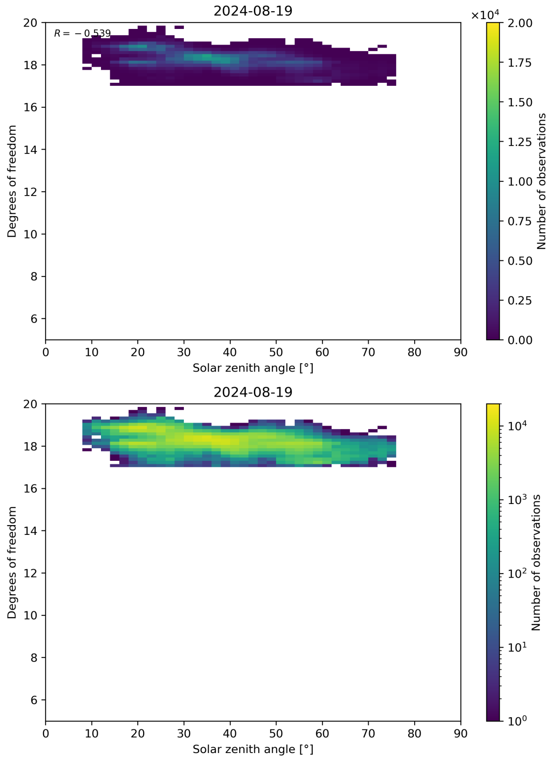
Figure 96: Scatter density plot of “Solar zenith angle” against “Degrees of freedom” for 2024-08-18 to 2024-08-20.
