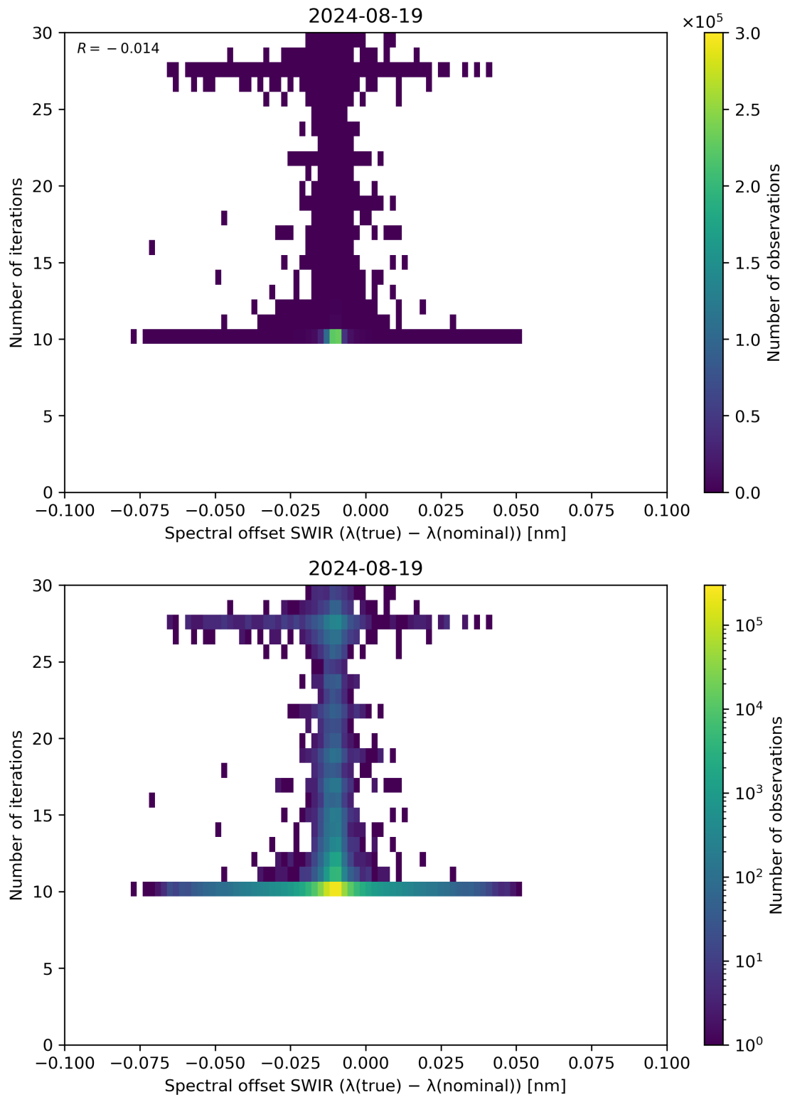
Figure 121: Scatter density plot of “Spectral offset SWIR ( \lambda(\text{true}) - \lambda(\text{nominal}) )” against “Number of iterations” for 2024-08-18 to 2024-08-20.
