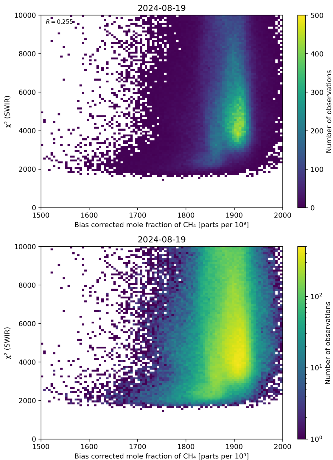
Figure 64: Scatter density plot of “Bias corrected mole fraction of \text{CH}_4 ” against “ \chi^2 (SWIR)” for 2024-08-18 to 2024-08-20.
