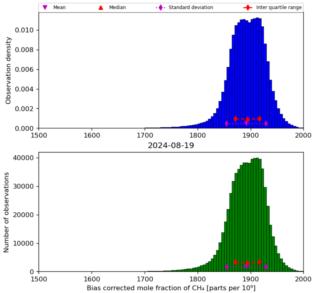
Figure 25: Histogram of “Bias corrected mole fraction of CH 4 ” for 2024-08-18 to 2024-08-20
