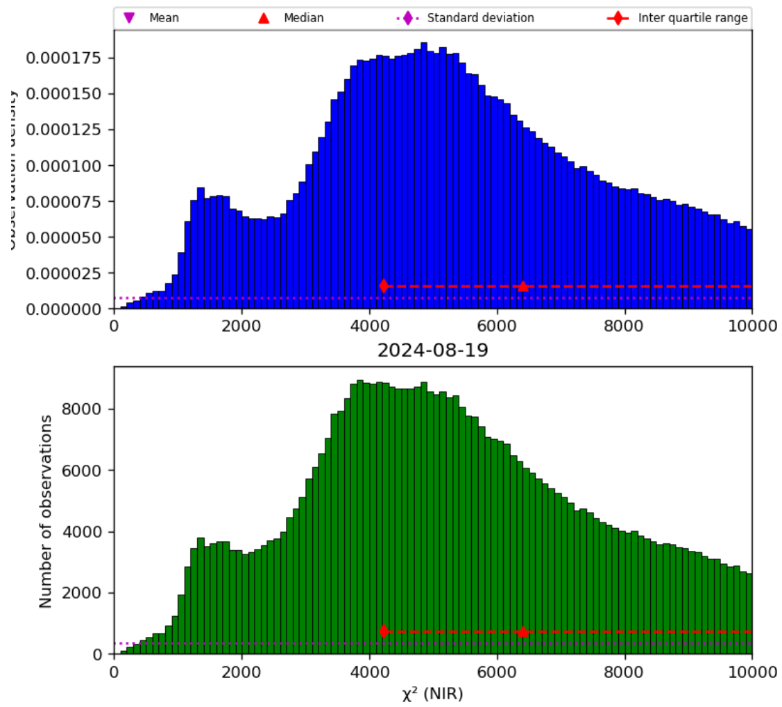
Figure 29: Histogram of “ \chi^2 (NIR)” for 2024-08-18 to 2024-08-20
