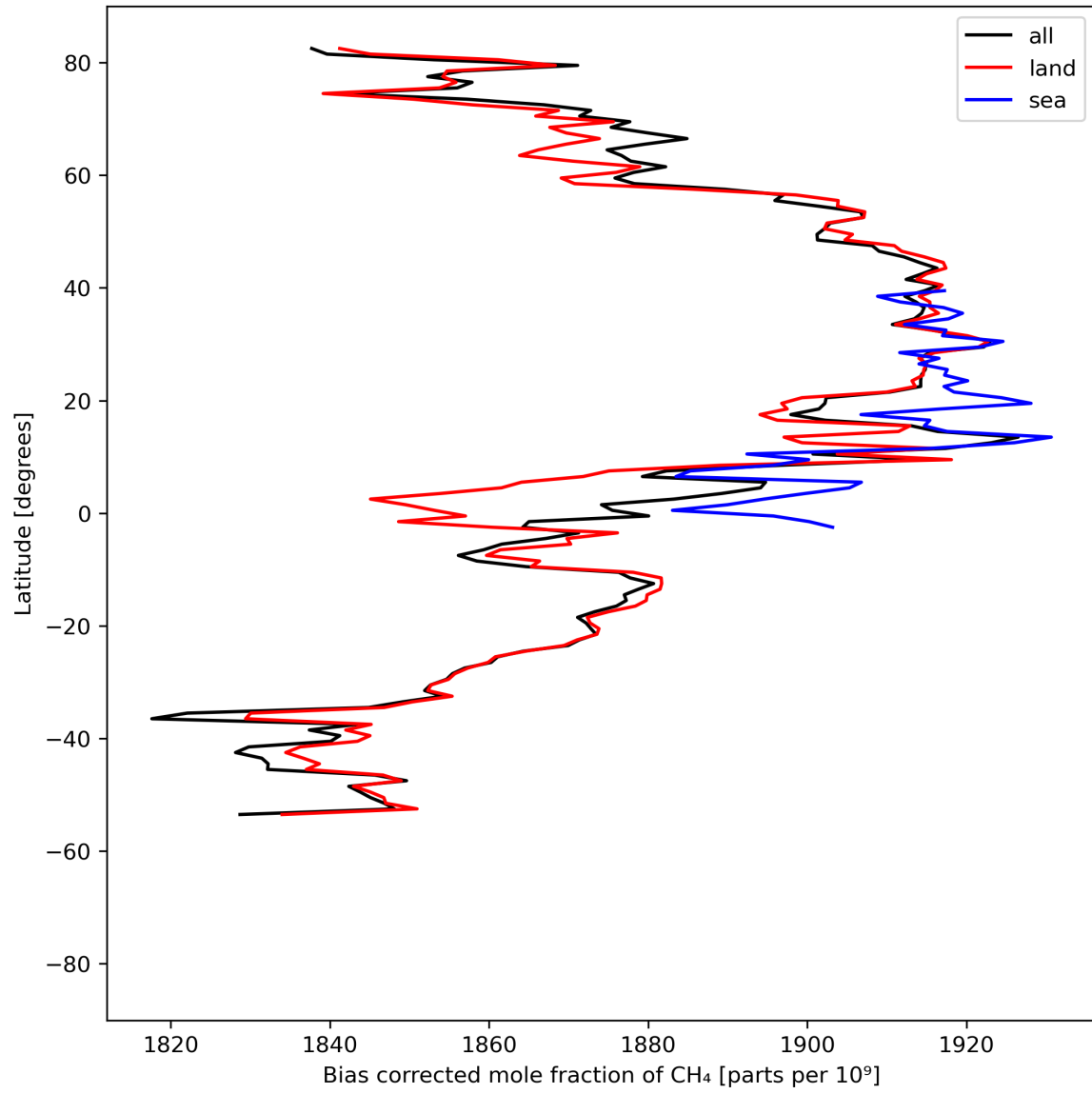
Figure 14: Zonal average of “Bias corrected mole fraction of CH 4 ” for 2024-08-18 to 2024-08-20.
