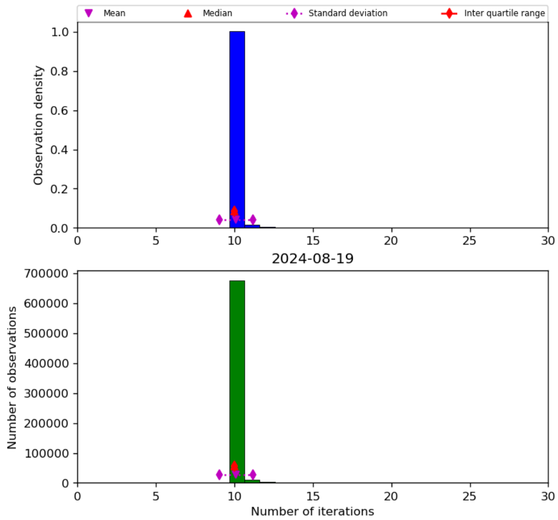
Figure 31: Histogram of “Number of iterations” for 2024-08-18 to 2024-08-20
