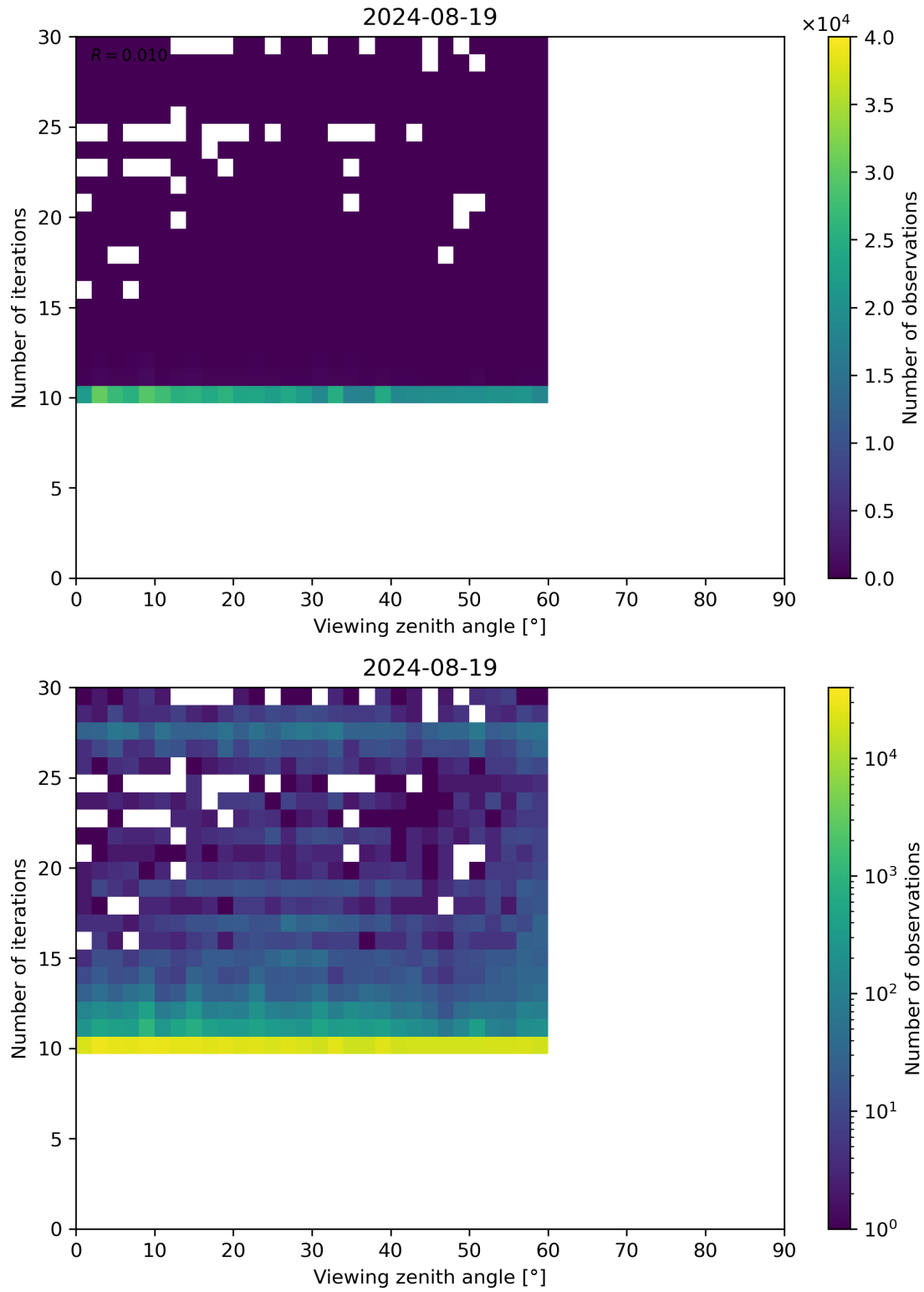
Figure 113: Scatter density plot of “Viewing zenith angle” against “Number of iterations” for 2024-08-18 to 2024-08-20.
