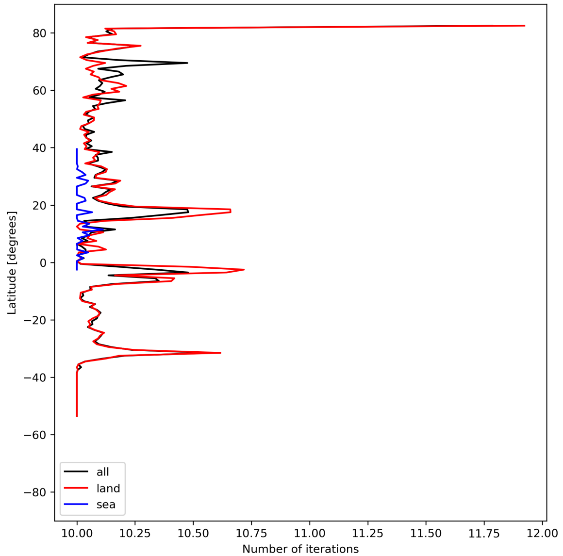
Figure 20: Zonal average of “Number of iterations” for 2024-08-18 to 2024-08-20.
