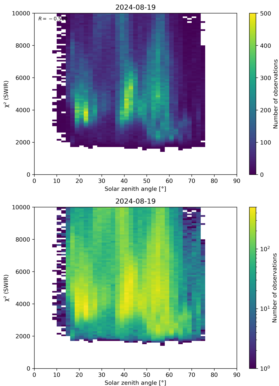
Figure 95: Scatter density plot of “Solar zenith angle” against “ \chi^2 (SWIR)” for 2024-08-18 to 2024-08-20.
