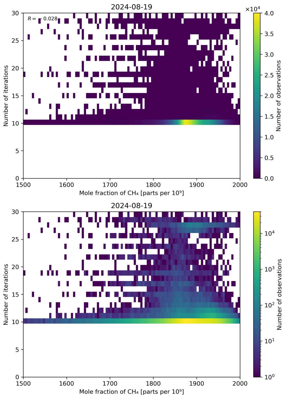
Figure 76: Scatter density plot of “Mole fraction of CH 4 ” against “Number of iterations” for 2024-08-18 to 2024-08-20.
