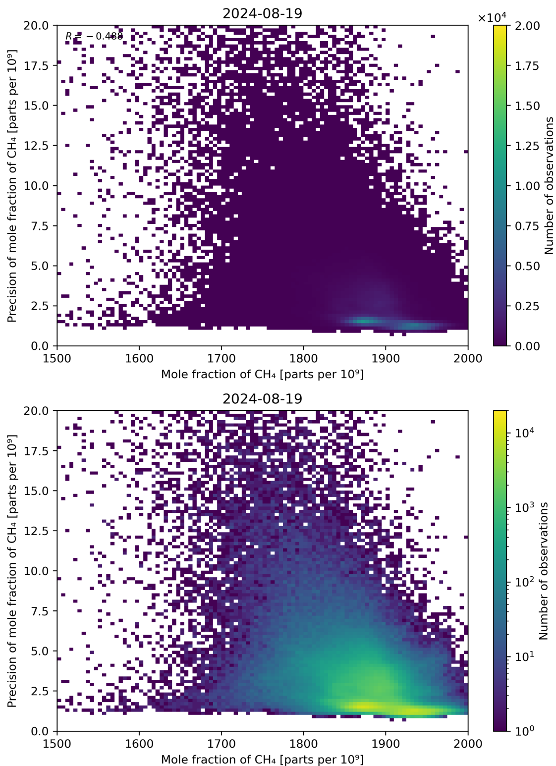
Figure 75: Scatter density plot of “Mole fraction of CH 4 ” against “Precision of mole fraction of CH 4 ” for 2024-08-18 to 2024-08-20.
