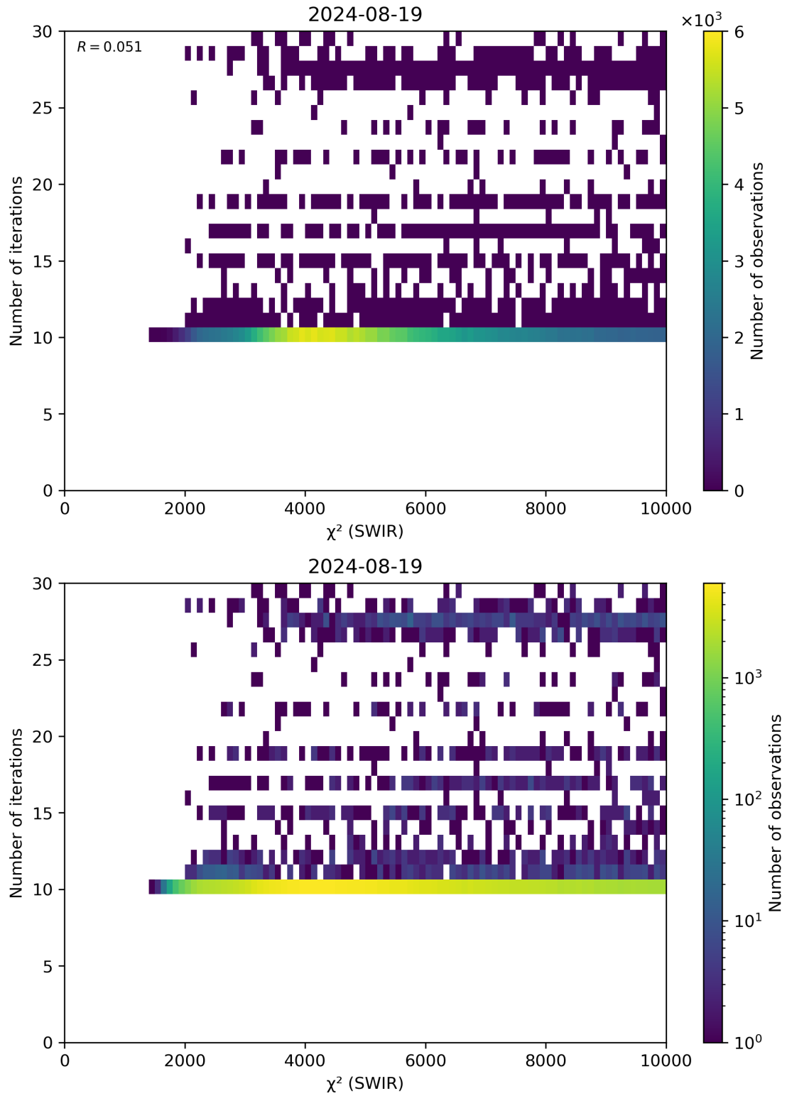
Figure 50: Scatter density plot of “ \chi^2 (SWIR)” against “Number of iterations” for 2024-08-18 to 2024-08-20.
