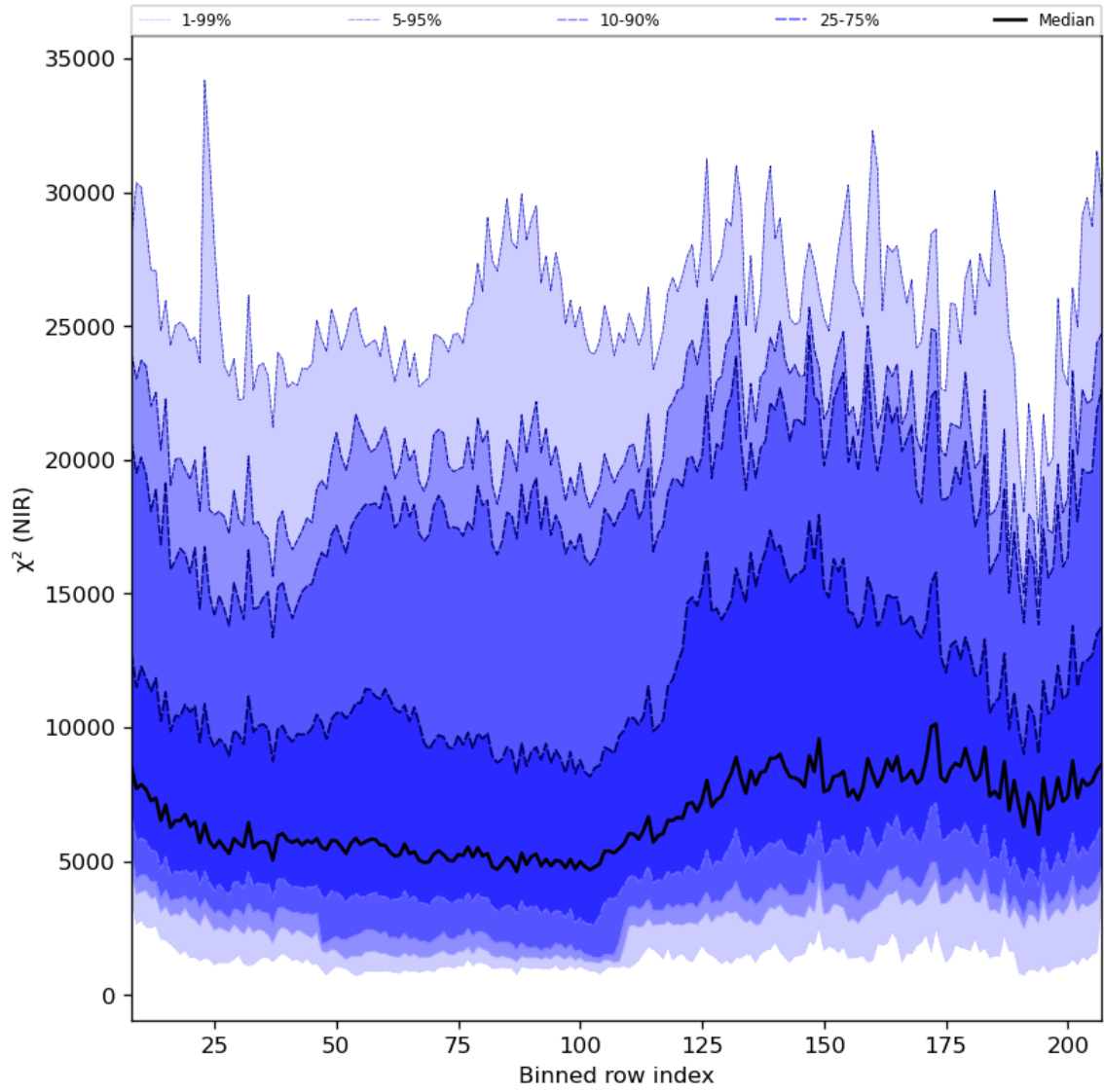
Figure 40: Along track statistics of “ \chi^2 (NIR)” for 2024-08-18 to 2024-08-20
