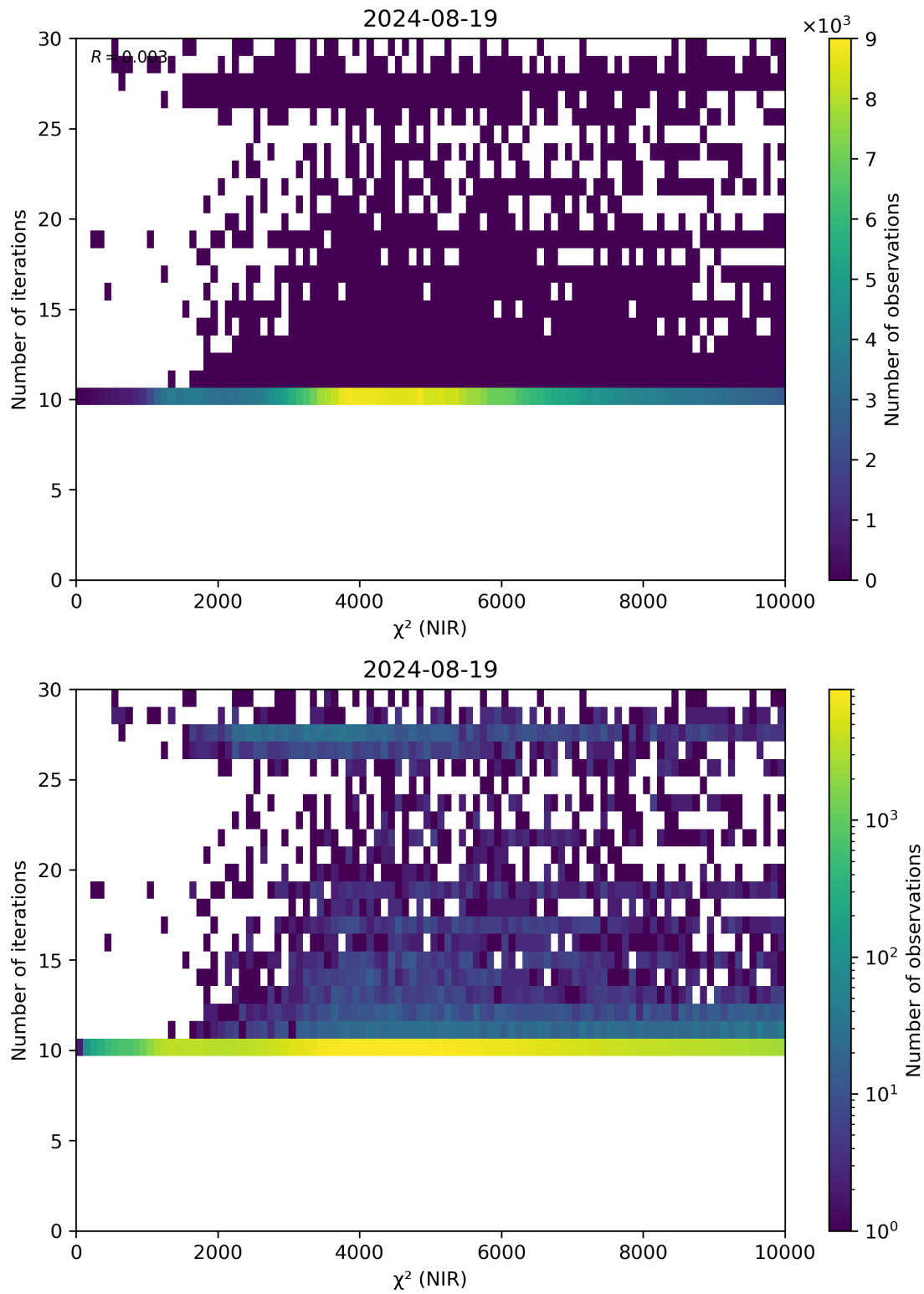
Figure 46: Scatter density plot of “ \chi^2 (NIR)” against “Number of iterations” for 2024-08-18 to 2024-08-20.
