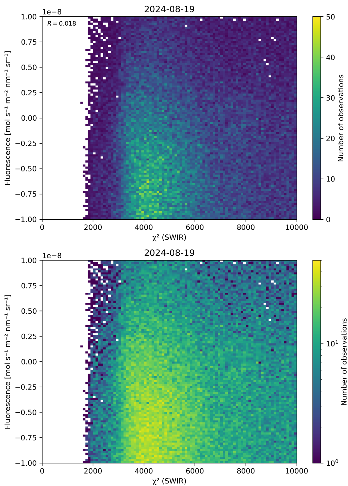
Figure 49: Scatter density plot of “ \chi^2 (SWIR)” against “Fluorescence” for 2024-08-18 to 2024-08-20.
