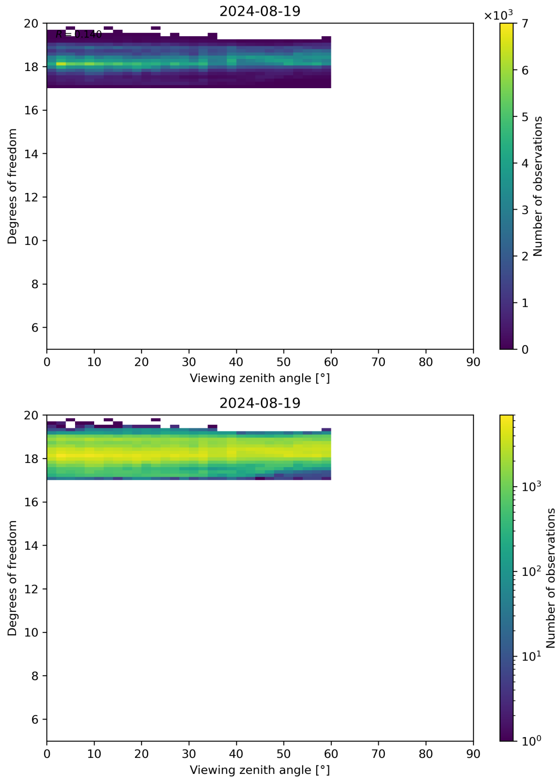
Figure 107: Scatter density plot of “Viewing zenith angle” against “Degrees of freedom” for 2024-08-18 to 2024-08-20.
