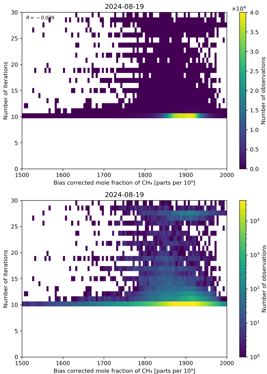
Figure 67: Scatter density plot of “Bias corrected mole fraction of CH 4 ” against “Number of iterations” for 2024-08-18 to 2024-08-20.
