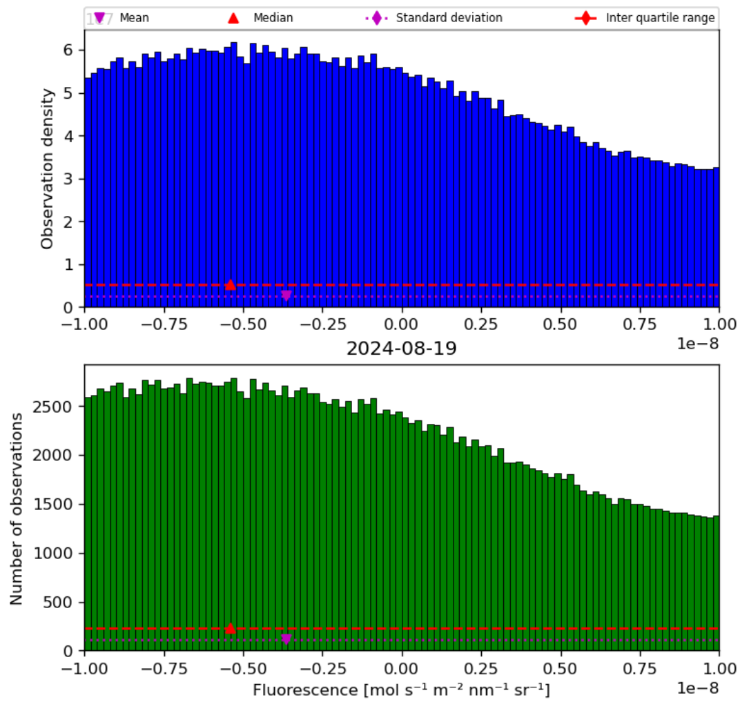
Figure 32: Histogram of “Fluorescence” for 2024-08-18 to 2024-08-20
