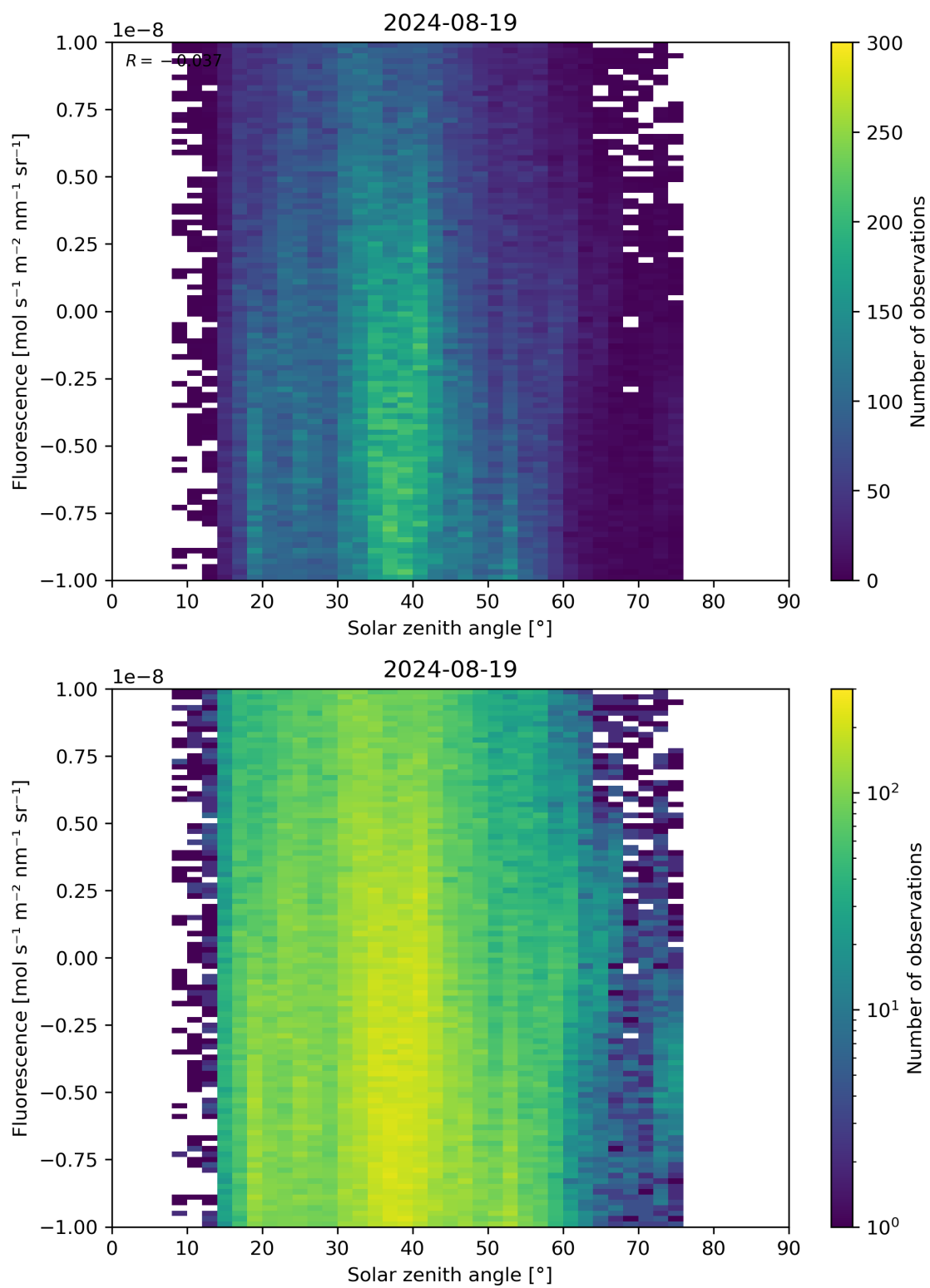
Figure 97: Scatter density plot of “Solar zenith angle” against “Fluorescence” for 2024-08-18 to 2024-08-20.
