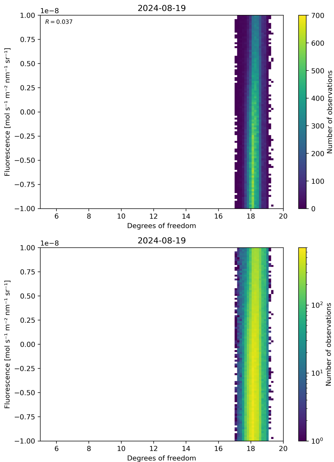
Figure 51: Scatter density plot of “Degrees of freedom” against “Fluorescence” for 2024-08-18 to 2024-08-20.
