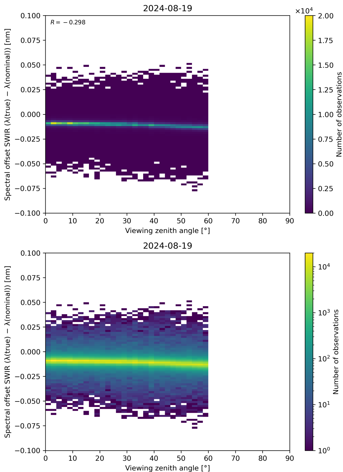
Figure 116: Scatter density plot of “Viewing zenith angle” against “Spectral offset SWIR ( \lambda(\text{true}) - \lambda(\text{nominal}) )” for 2024-08-18 to 2024-08-20.
