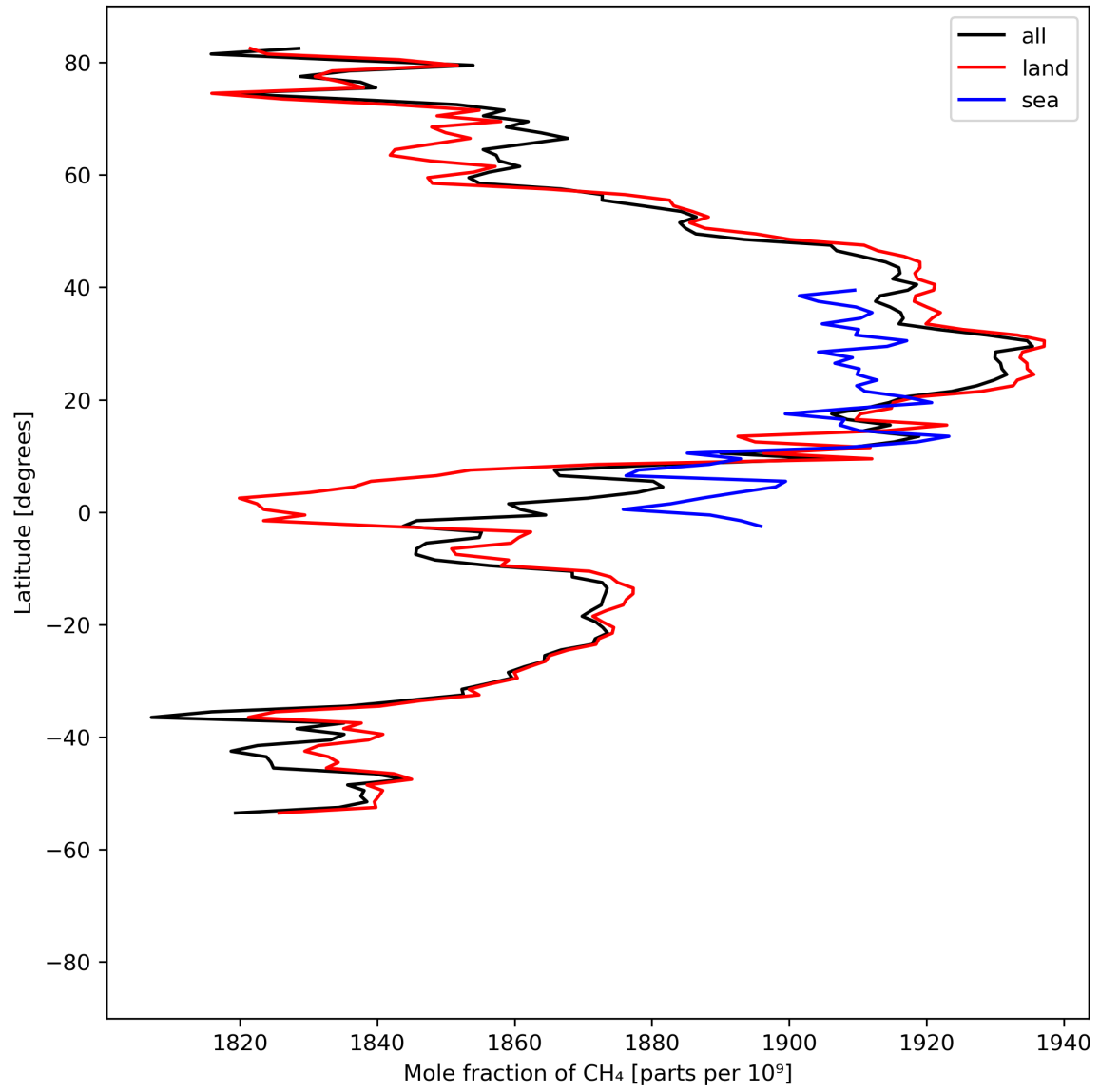
Figure 12: Zonal average of “Mole fraction of \text{CH}_4 ” for 2024-08-18 to 2024-08-20.
