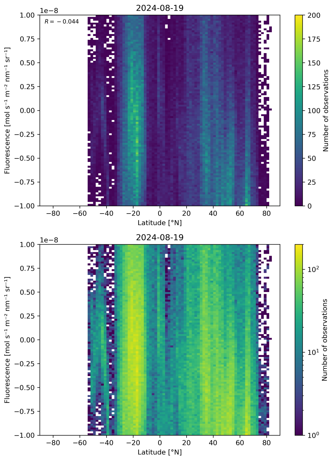
Figure 56: Scatter density plot of “Latitude” against “Fluorescence” for 2024-08-18 to 2024-08-20.
