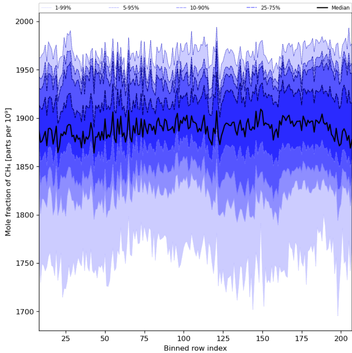
Figure 34: Along track statistics of “Mole fraction of CH 4 ” for 2024-08-18 to 2024-08-20
