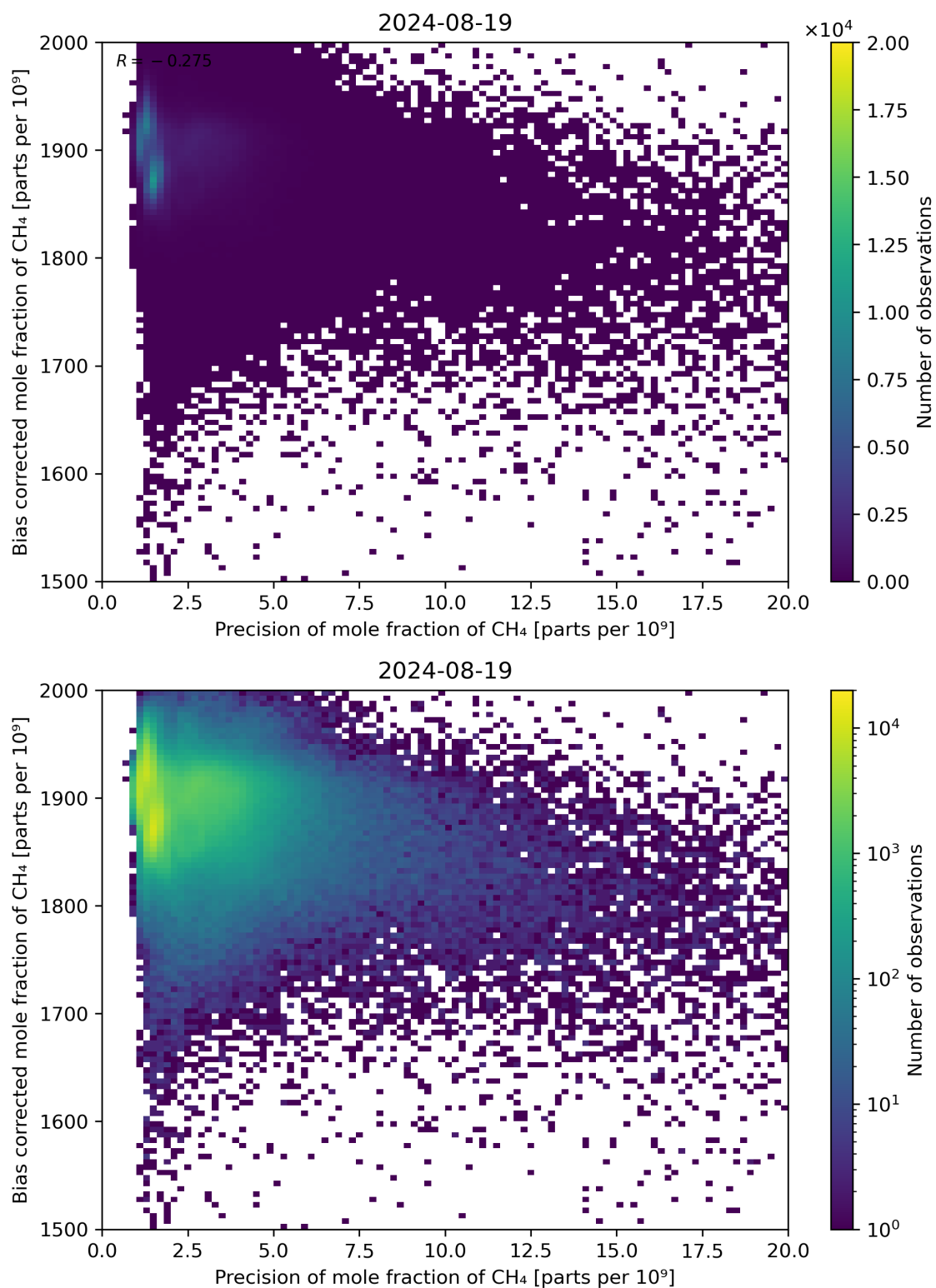
Figure 82: Scatter density plot of “Precision of mole fraction of CH 4 ” against “Bias corrected mole fraction of CH 4 ” for 2024-08-18 to 2024-08-20.
