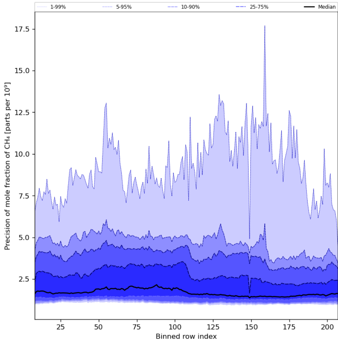
Figure 35: Along track statistics of “Precision of mole fraction of CH 4 ” for 2024-08-18 to 2024-08-20
