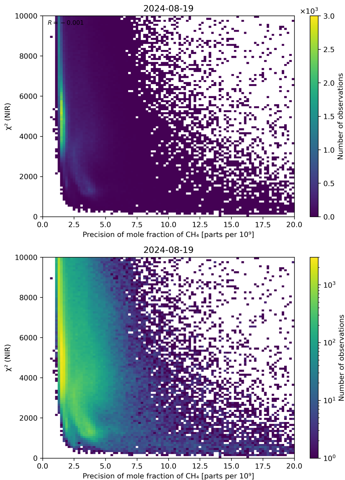
Figure 78: Scatter density plot of “Precision of mole fraction of CH 4 ” against “ \chi^2 (NIR)” for 2024-08-18 to 2024-08-20.
