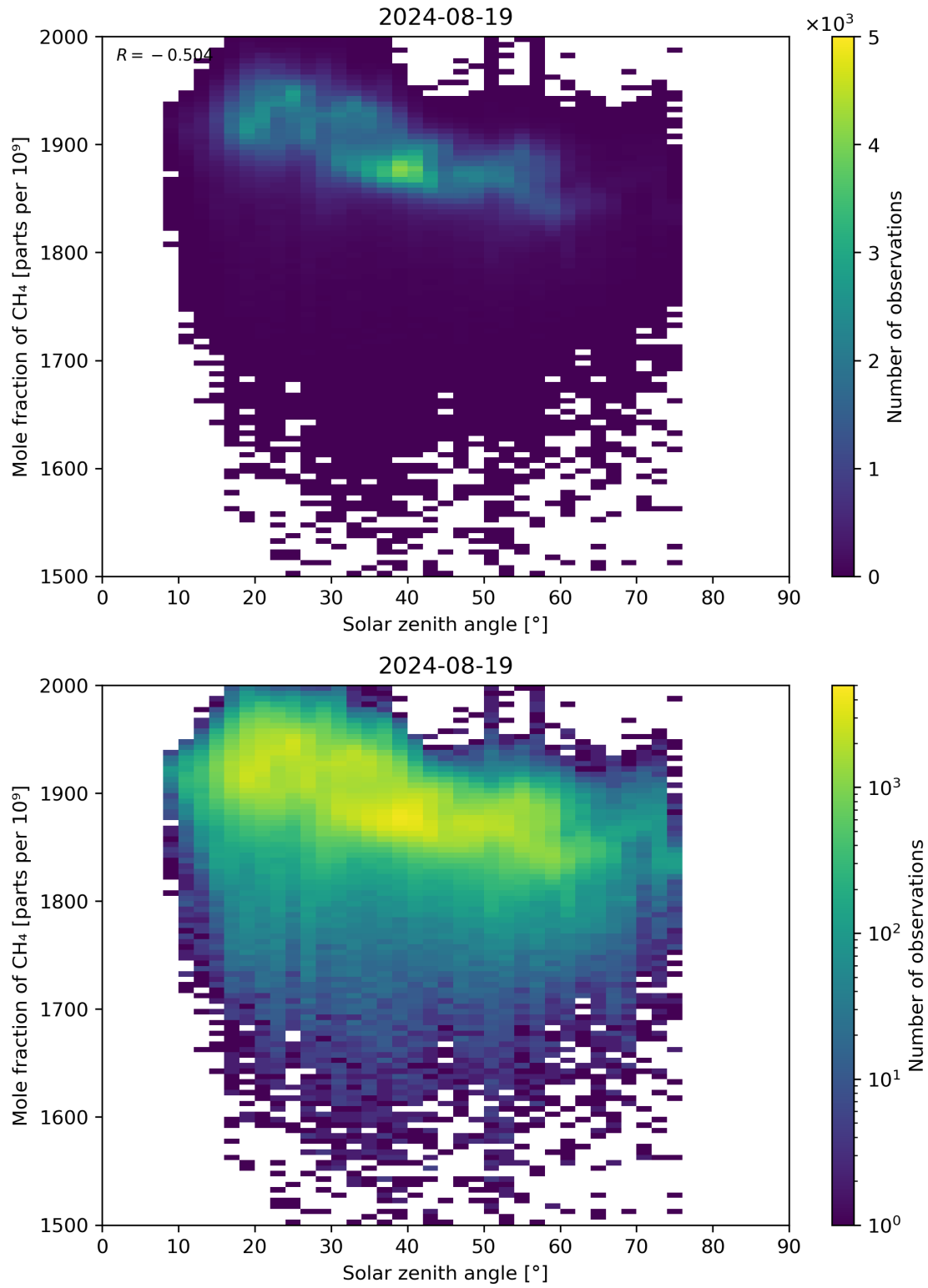
Figure 99: Scatter density plot of “Solar zenith angle” against “Mole fraction of CH 4 ” for 2024-08-18 to 2024-08-20.
