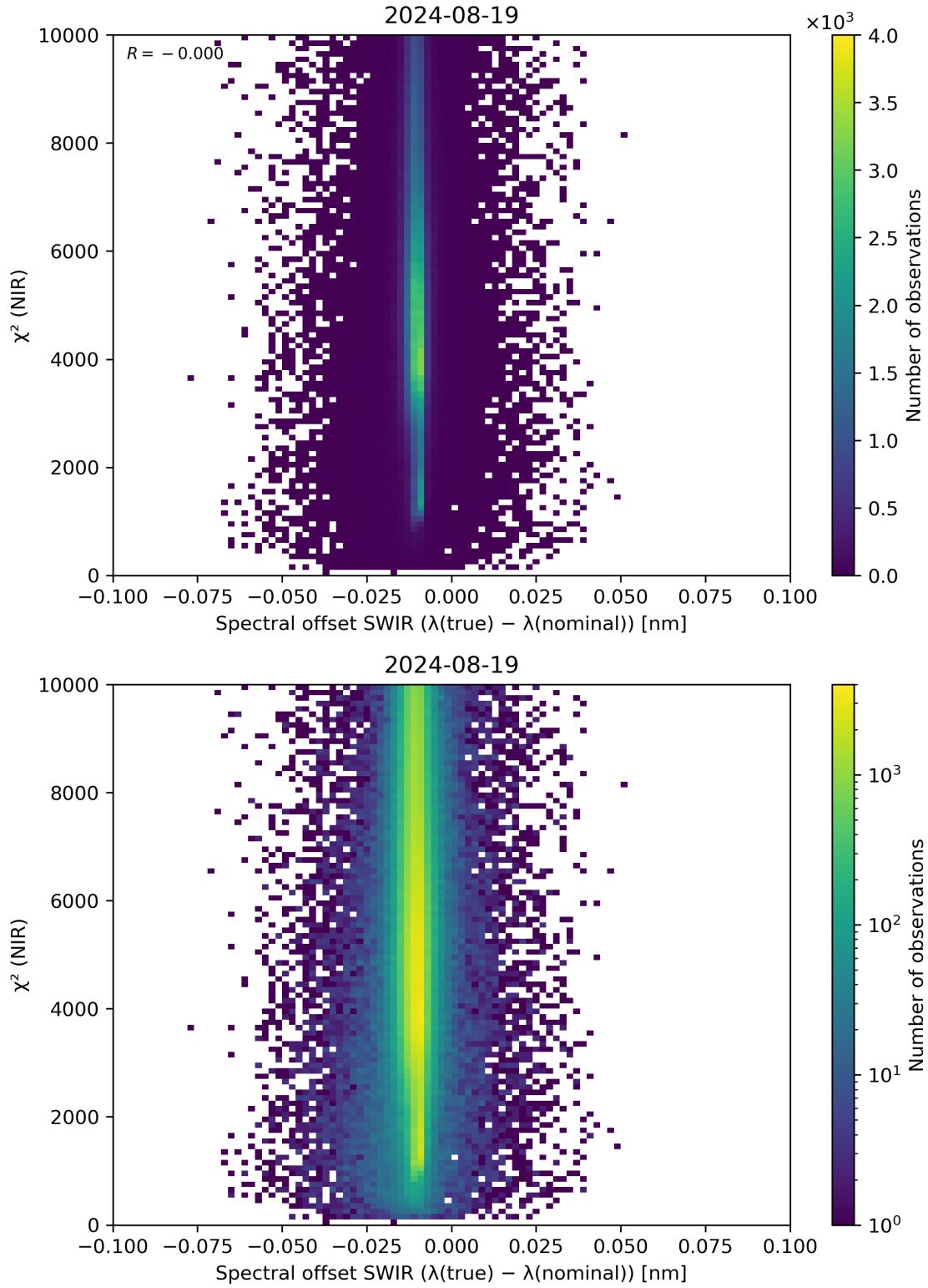
Figure 117: Scatter density plot of “Spectral offset SWIR ( \lambda(\text{true}) - \lambda(\text{nominal}) )” against “ \chi^2 (NIR)” for 2024-08-18 to 2024-08-20.
