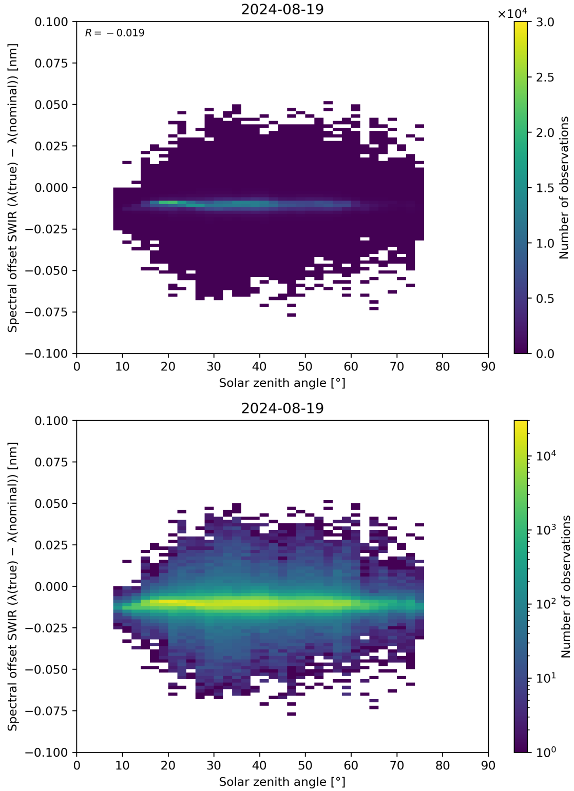
Figure 104: Scatter density plot of “Solar zenith angle” against “Spectral offset SWIR ( \lambda(\text{true}) - \lambda(\text{nominal}) )” for 2024-08-18 to 2024-08-20.
