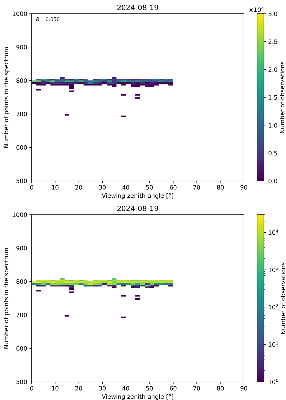
Figure 114: Scatter density plot of “Viewing zenith angle” against “Number of points in the spectrum” for 2024-08-18 to 2024-08-20.
