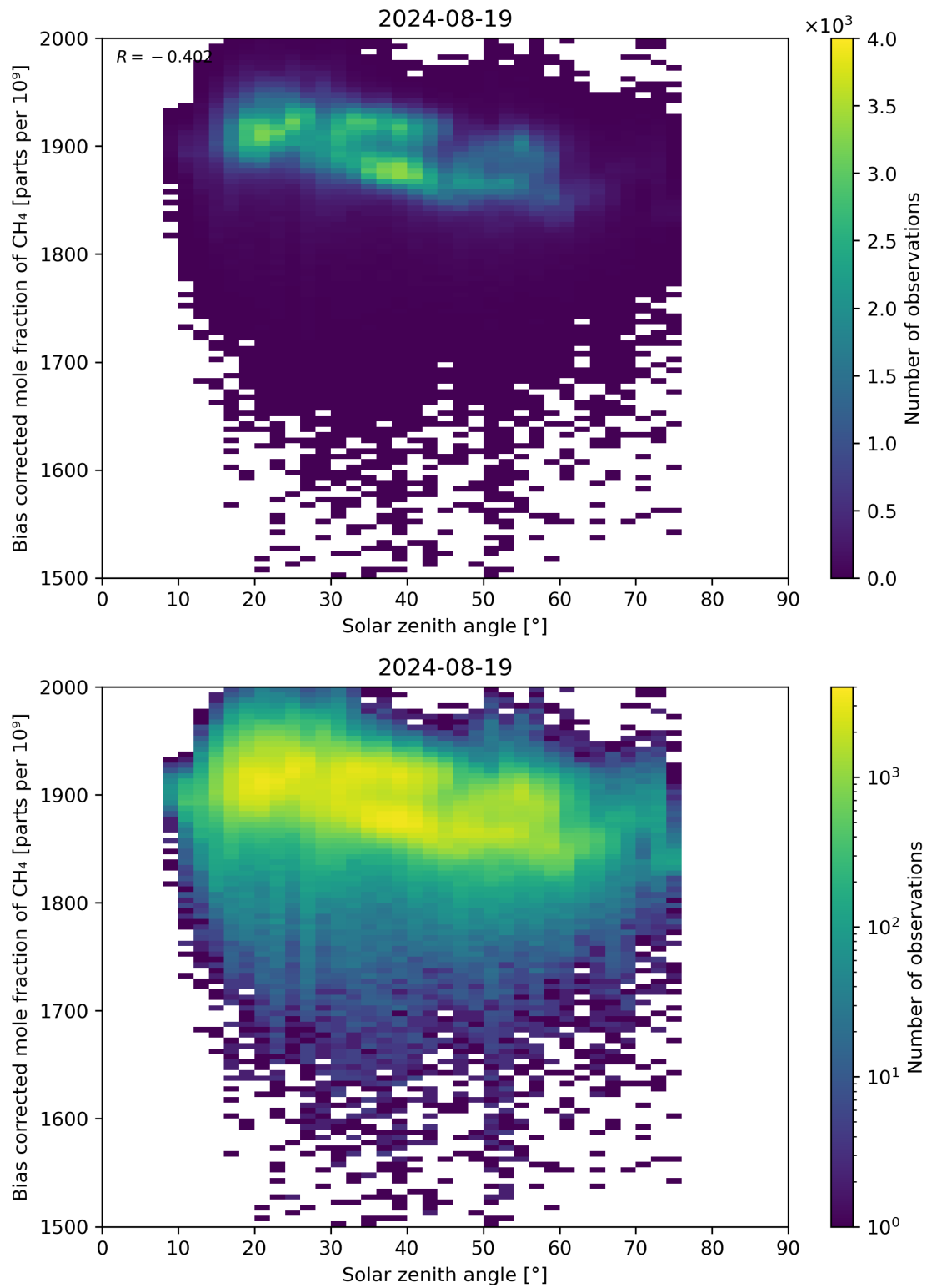
Figure 100: Scatter density plot of “Solar zenith angle” against “Bias corrected mole fraction of CH 4 ” for 2024-08-18 to 2024-08-20.
