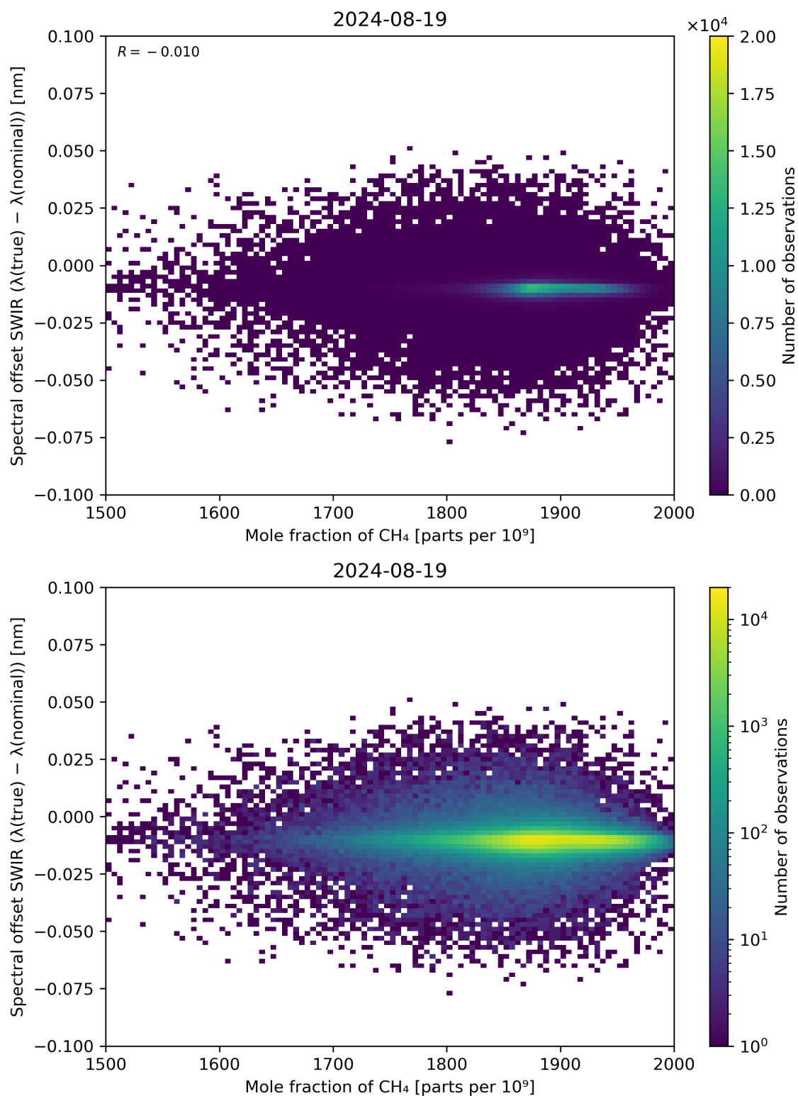
Figure 86: Scatter density plot of “Mole fraction of CH 4 ” against “Spectral offset SWIR ( \lambda(\text{true}) - \lambda(\text{nominal}) )” for 2024-08-18 to 2024-08-20.
