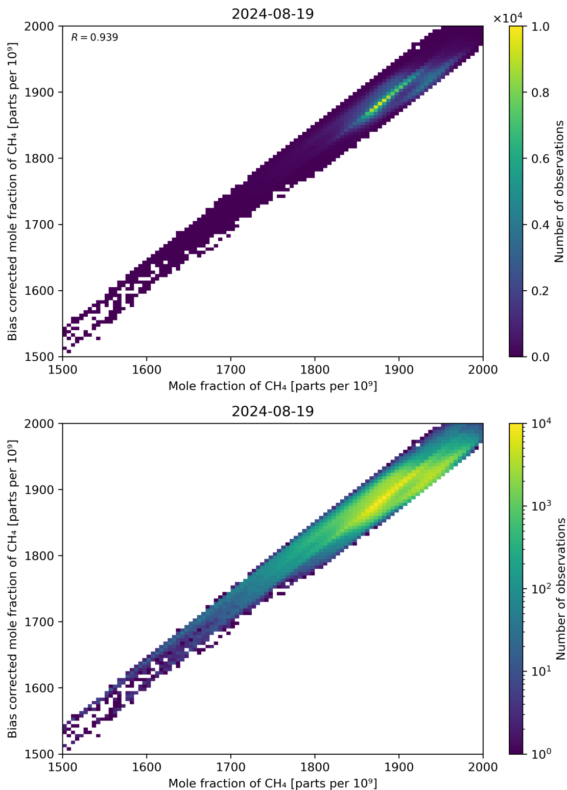
Figure 74: Scatter density plot of “Mole fraction of \text{CH}_4 ” against “Bias corrected mole fraction of \text{CH}_4 ” for 2024-08-18 to 2024-08-20.
