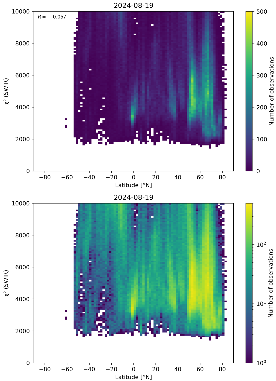
Figure 54: Scatter density plot of “Latitude” against “ \chi^2 (SWIR)” for 2024-08-18 to 2024-08-20.
