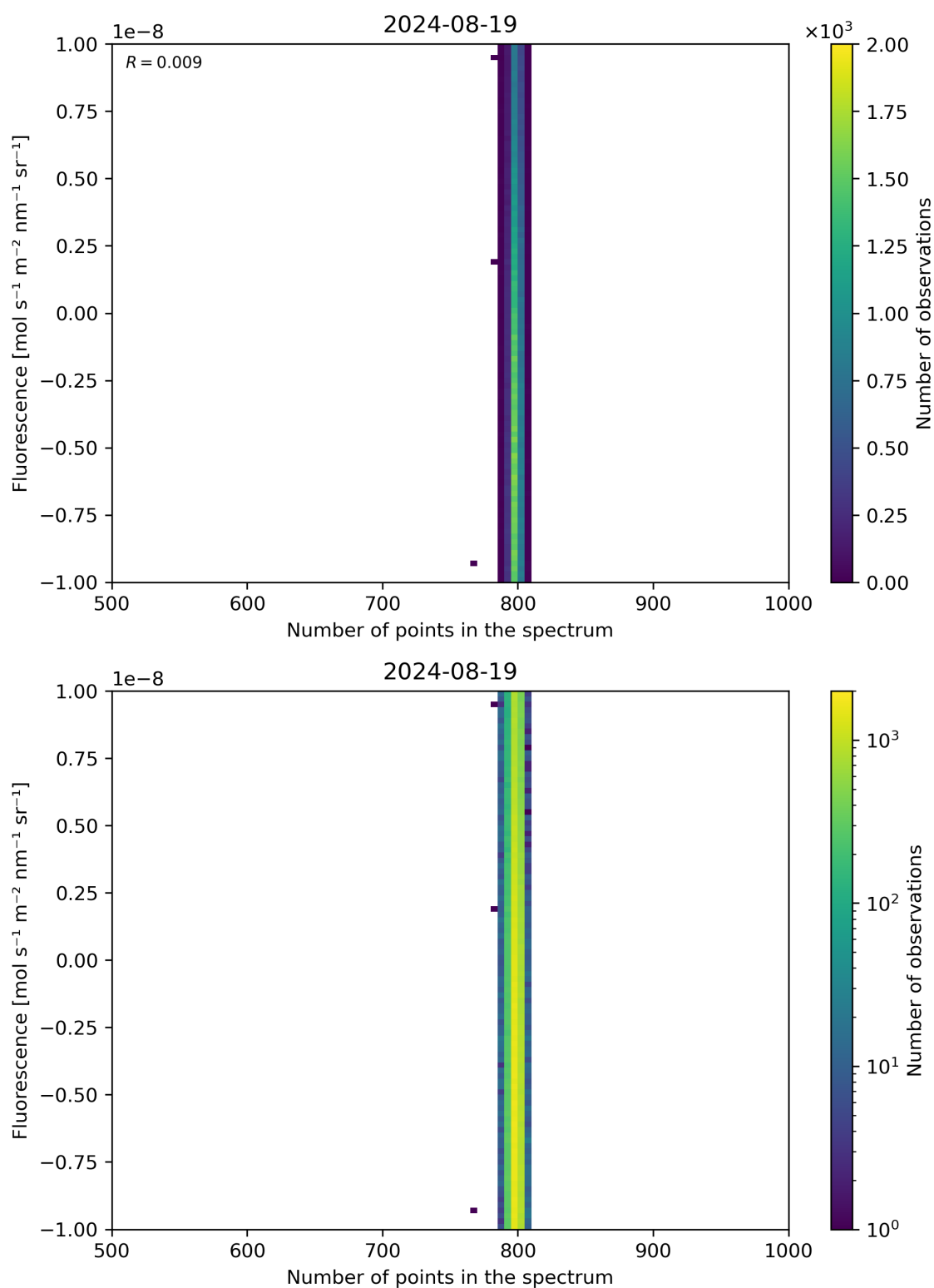
Figure 91: Scatter density plot of “Number of points in the spectrum” against “Fluorescence” for 2024-08-18 to 2024-08-20.
