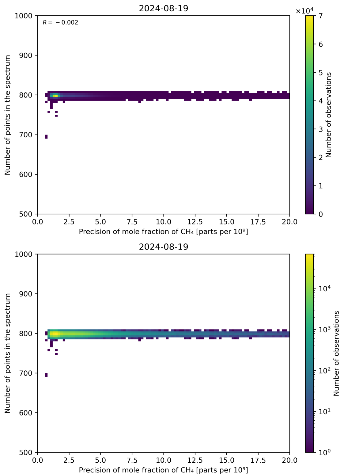
Figure 84: Scatter density plot of “Precision of mole fraction of CH 4 ” against “Number of points in the spectrum” for 2024-08-18 to 2024-08-20.
