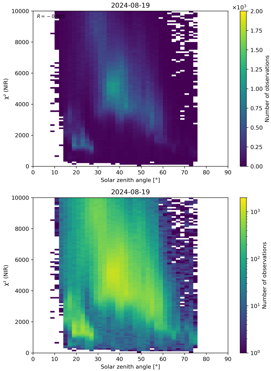
Figure 94: Scatter density plot of “Solar zenith angle” against “ \chi^2 (NIR)” for 2024-08-18 to 2024-08-20.
