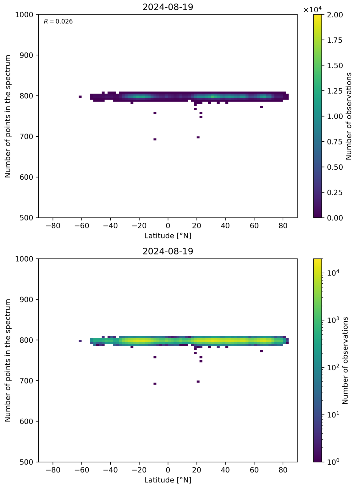
Figure 61: Scatter density plot of “Latitude” against “Number of points in the spectrum” for 2024-08-18 to 2024-08-20.
