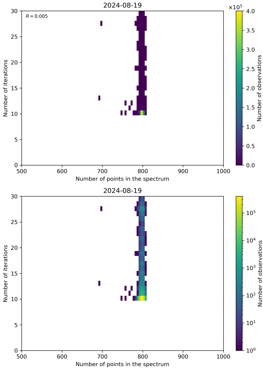
Figure 92: Scatter density plot of “Number of points in the spectrum” against “Number of iterations” for 2024-08-18 to 2024-08-20.
