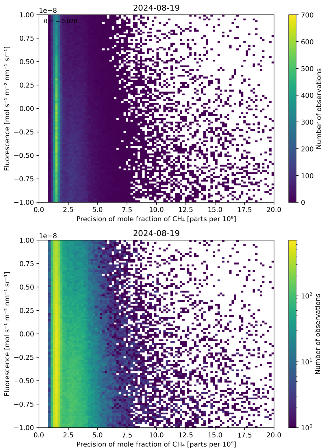
Figure 81: Scatter density plot of “Precision of mole fraction of \text{CH}_4 ” against “Fluorescence” for 2024-08-18 to 2024-08-20.
