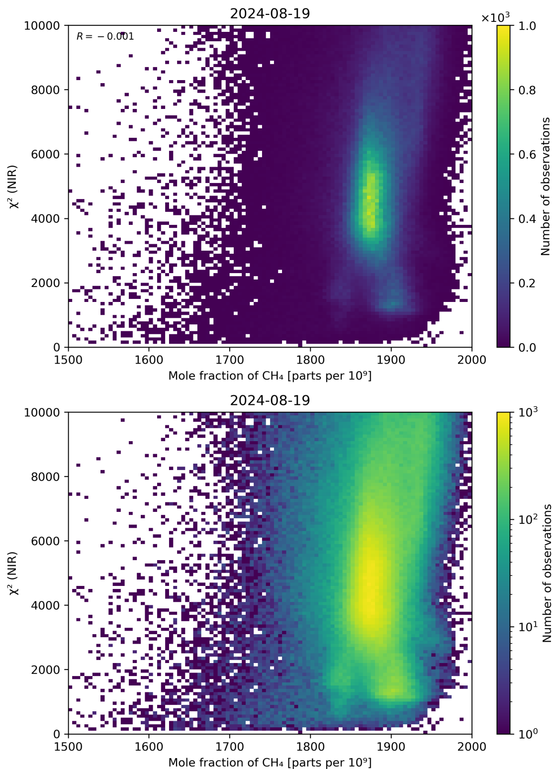
Figure 70: Scatter density plot of “Mole fraction of CH 4 ” against “ \chi^2 (NIR)” for 2024-08-18 to 2024-08-20.
