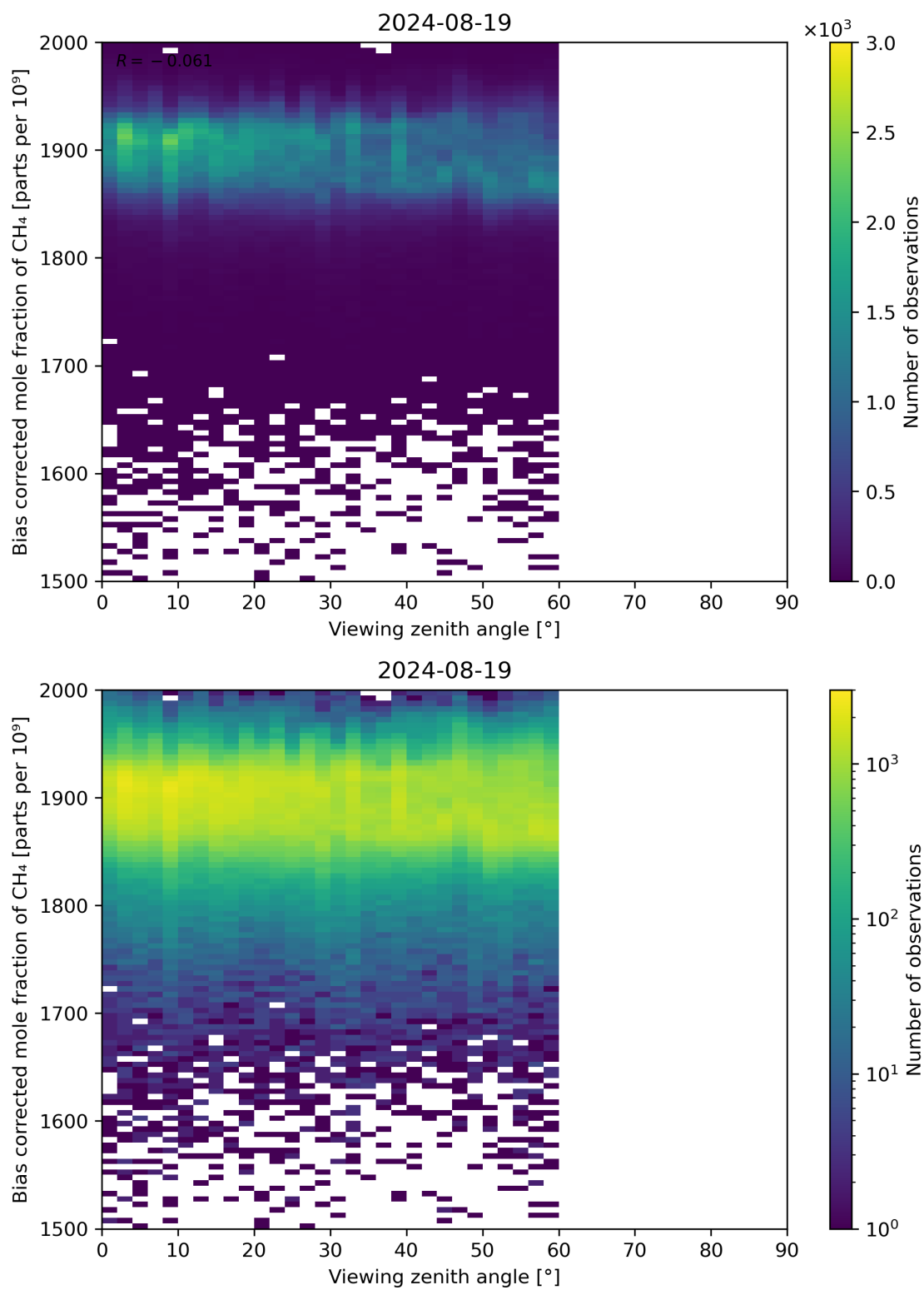
Figure 111: Scatter density plot of “Viewing zenith angle” against “Bias corrected mole fraction of CH 4 ” for 2024-08-18 to 2024-08-20.
