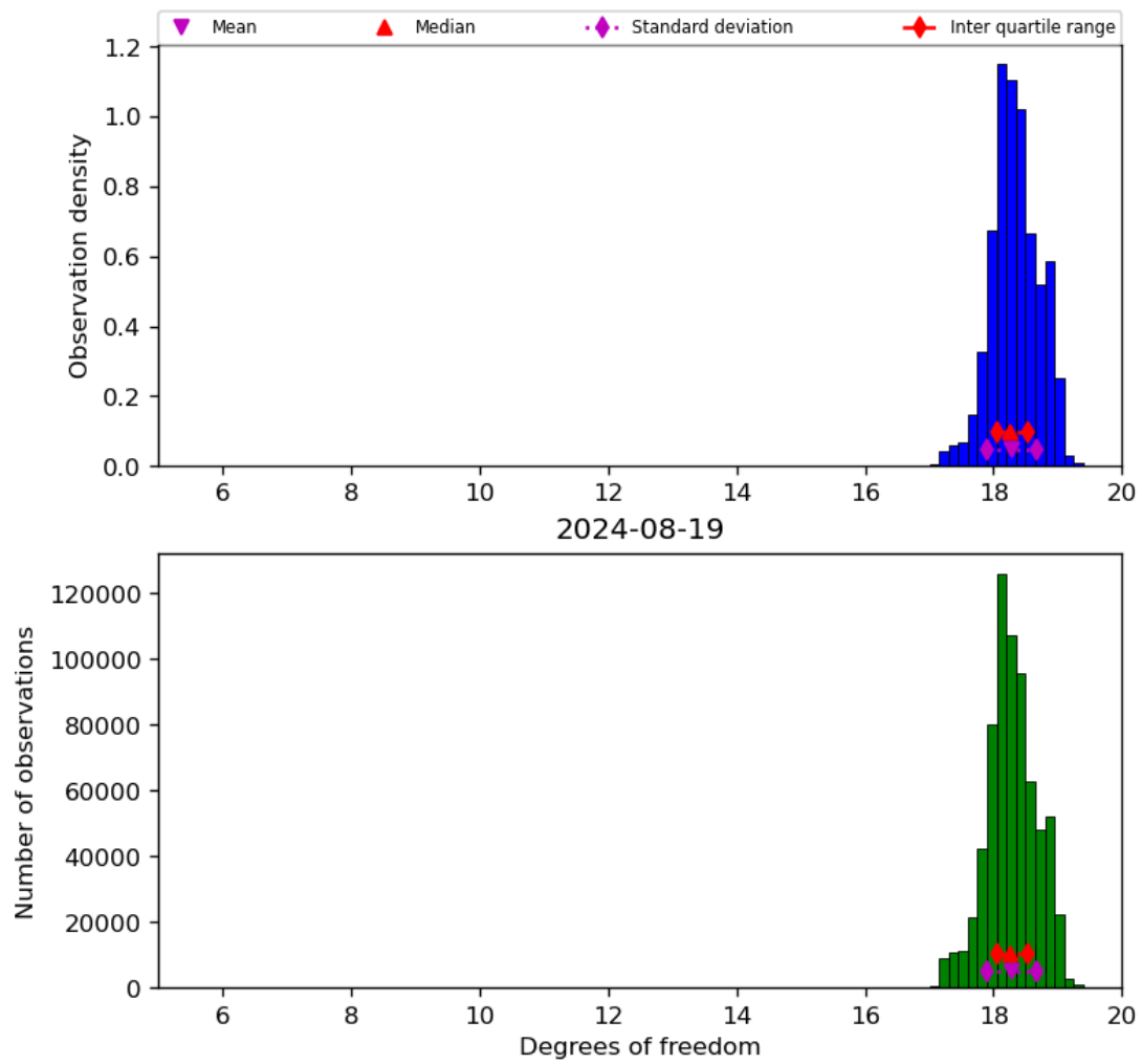
Figure 30: Histogram of “Degrees of freedom” for 2024-08-18 to 2024-08-20
