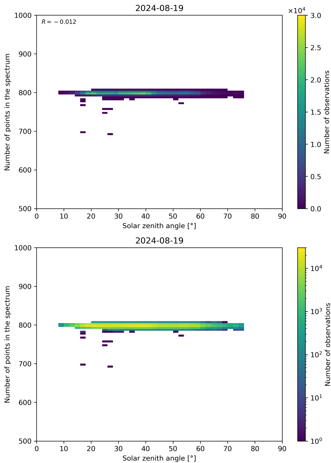
Figure 103: Scatter density plot of “Solar zenith angle” against “Number of points in the spectrum” for 2024-08-18 to 2024-08-20.
