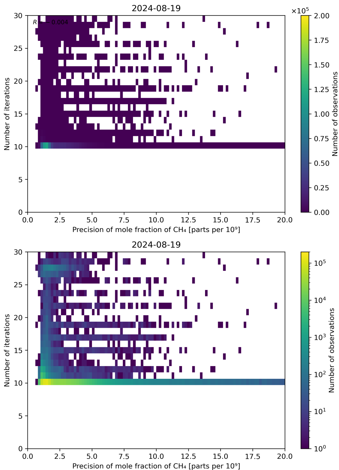
Figure 83: Scatter density plot of “Precision of mole fraction of CH 4 ” against “Number of iterations” for 2024-08-18 to 2024-08-20.
