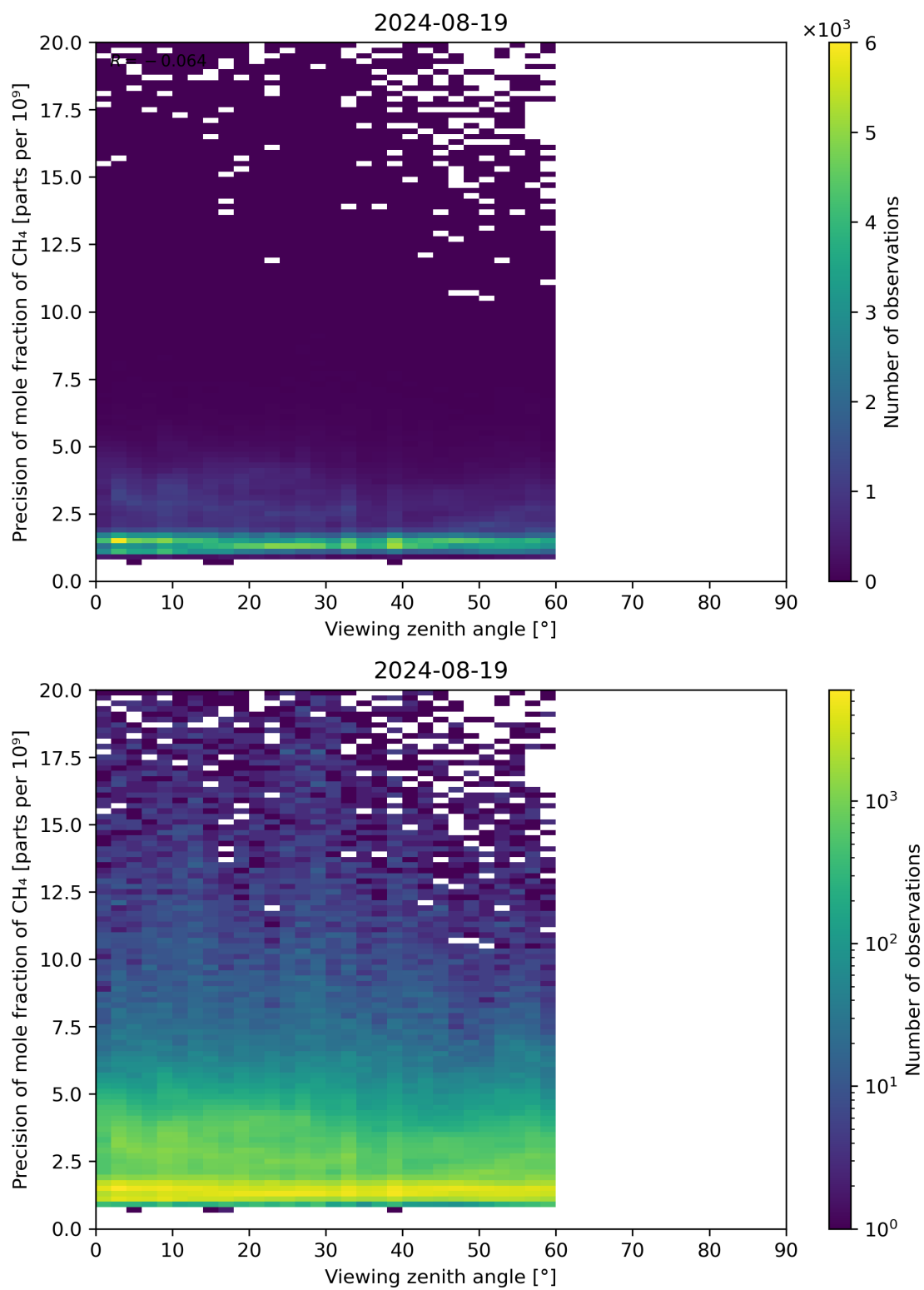
Figure 112: Scatter density plot of “Viewing zenith angle” against “Precision of mole fraction of CH 4 ” for 2024-08-18 to 2024-08-20.
