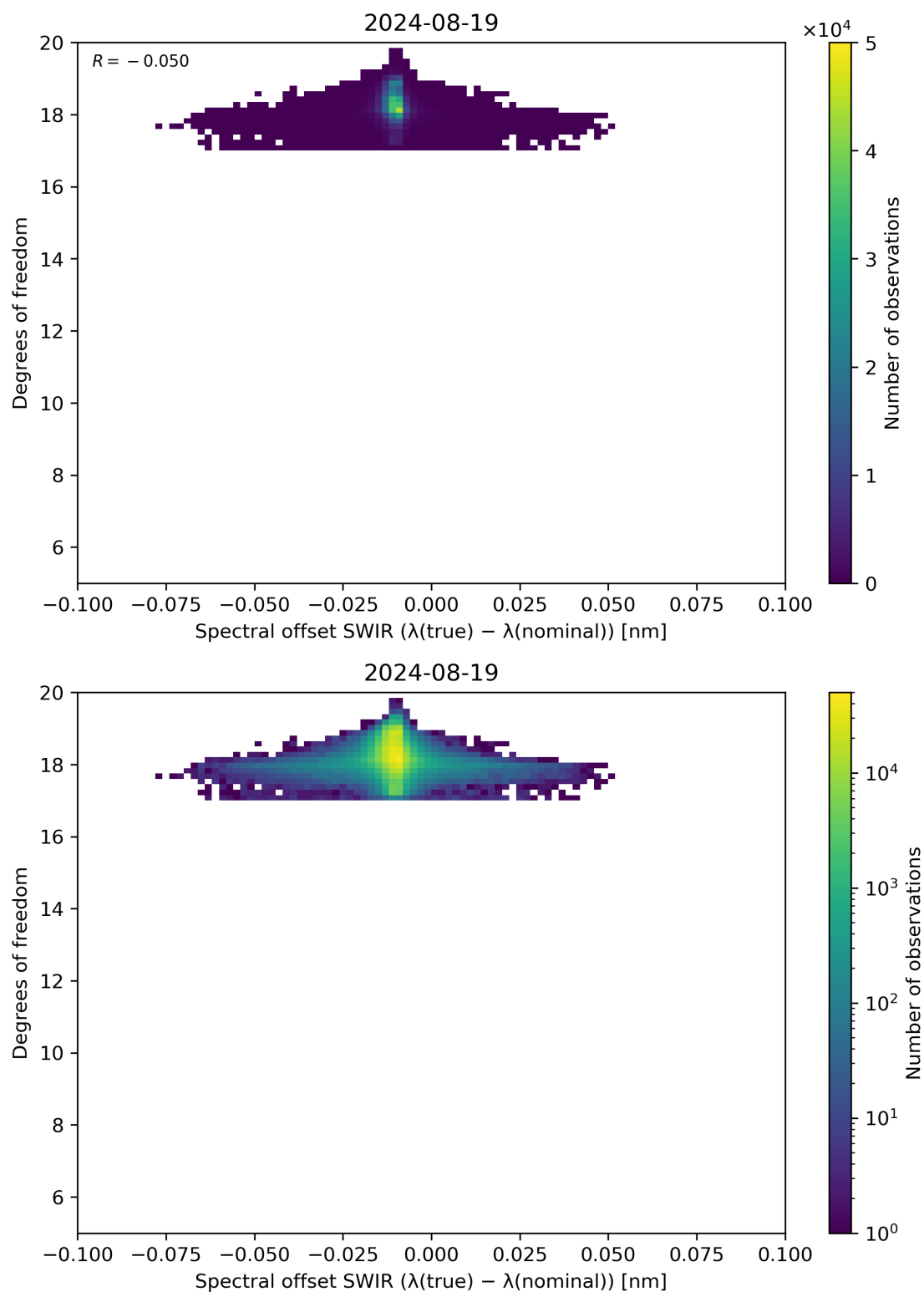
Figure 119: Scatter density plot of “Spectral offset SWIR ( \lambda(\text{true}) - \lambda(\text{nominal}) )” against “Degrees of freedom” for 2024-08-18 to 2024-08-20.
