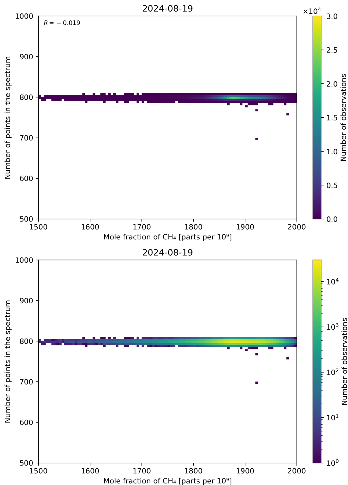
Figure 77: Scatter density plot of “Mole fraction of CH 4 ” against “Number of points in the spectrum” for 2024-08-18 to 2024-08-20.
