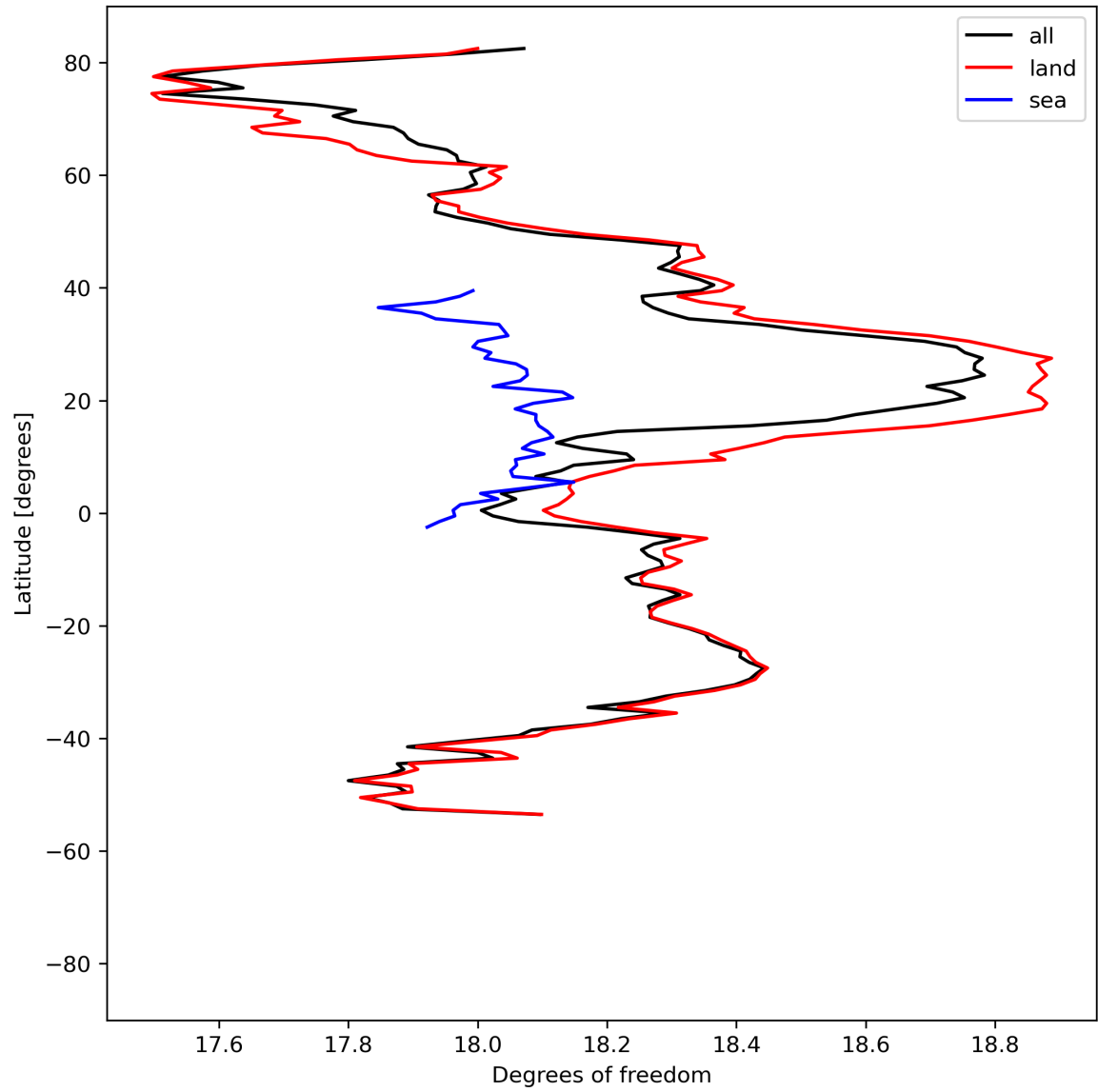
Figure 19: Zonal average of “Degrees of freedom” for 2024-08-18 to 2024-08-20.
