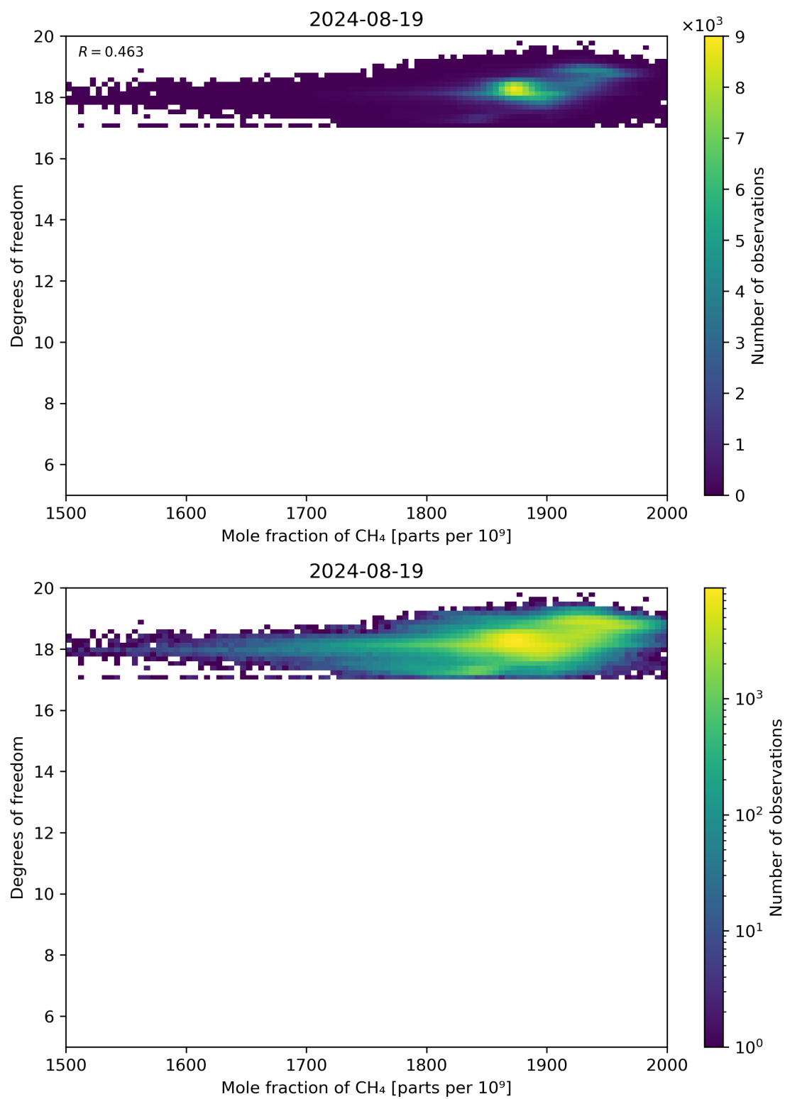
Figure 72: Scatter density plot of “Mole fraction of CH 4 ” against “Degrees of freedom” for 2024-08-18 to 2024-08-20.
