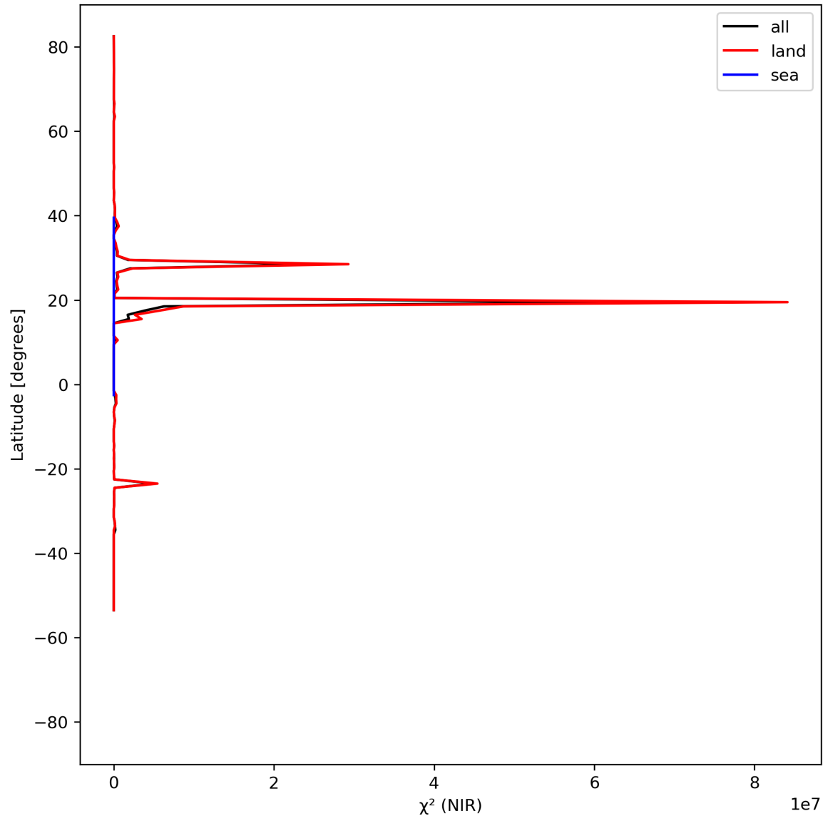
Figure 18: Zonal average of “ \chi^2 (NIR)” for 2024-08-18 to 2024-08-20.
