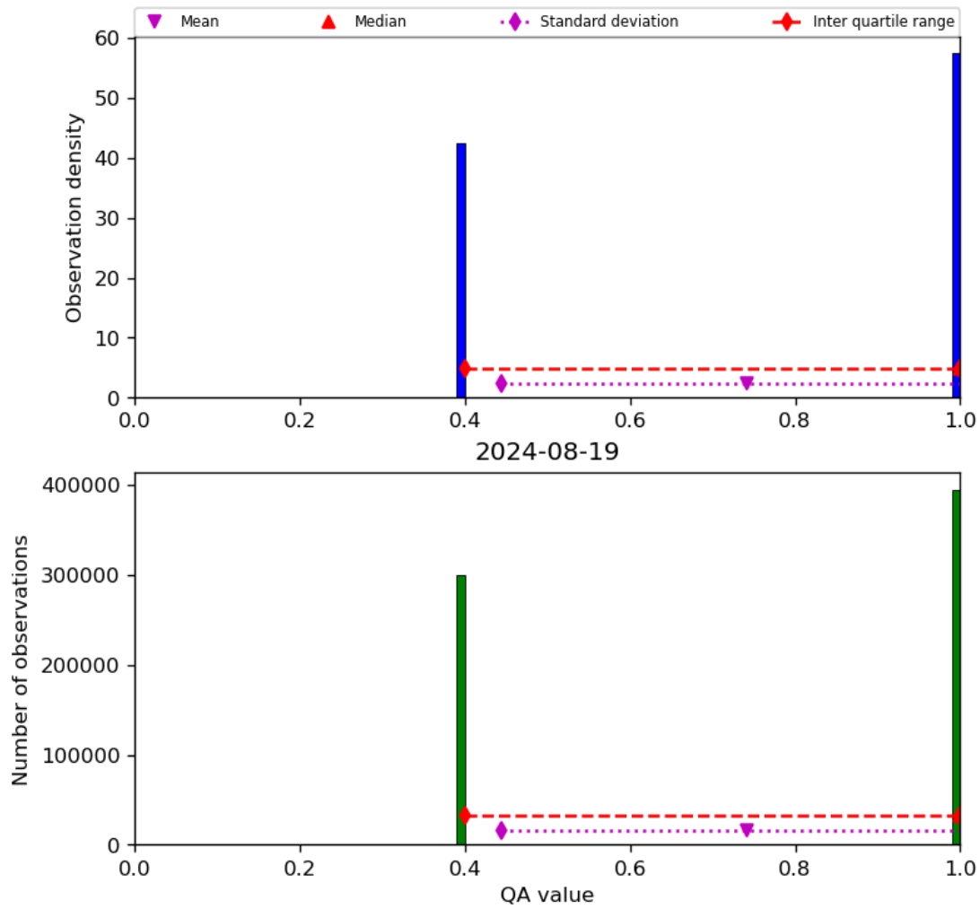
Figure 22: Histogram of “QA value” for 2024-08-18 to 2024-08-20
