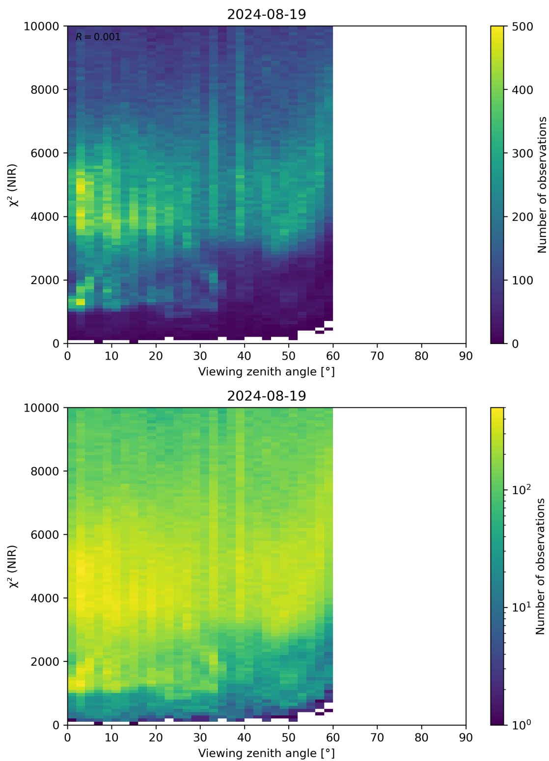
Figure 105: Scatter density plot of “Viewing zenith angle” against “ \chi^2 (NIR)” for 2024-08-18 to 2024-08-20.
