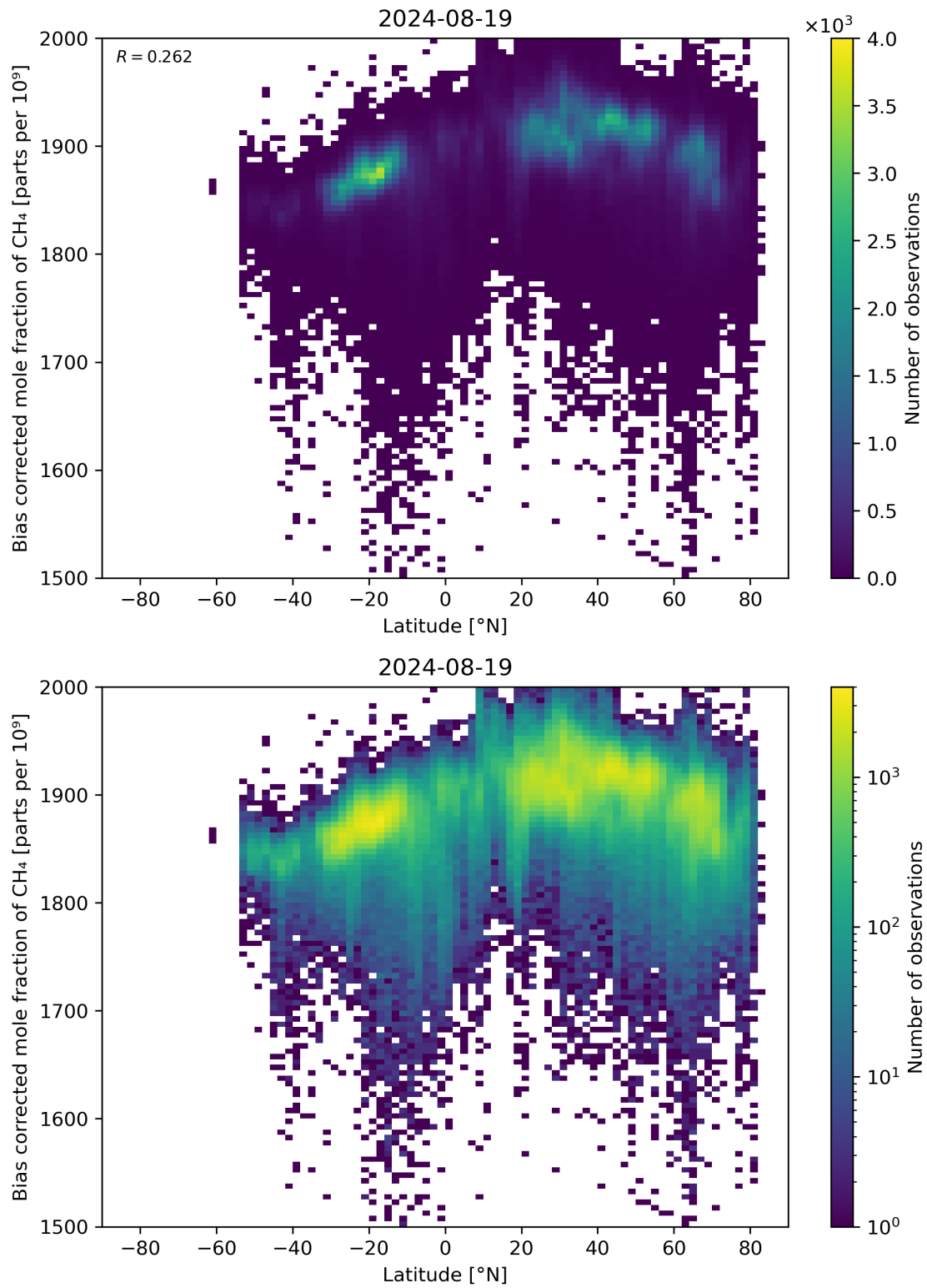
Figure 58: Scatter density plot of “Latitude” against “Bias corrected mole fraction of \text{CH}_4 ” for 2024-08-18 to 2024-08-20.
