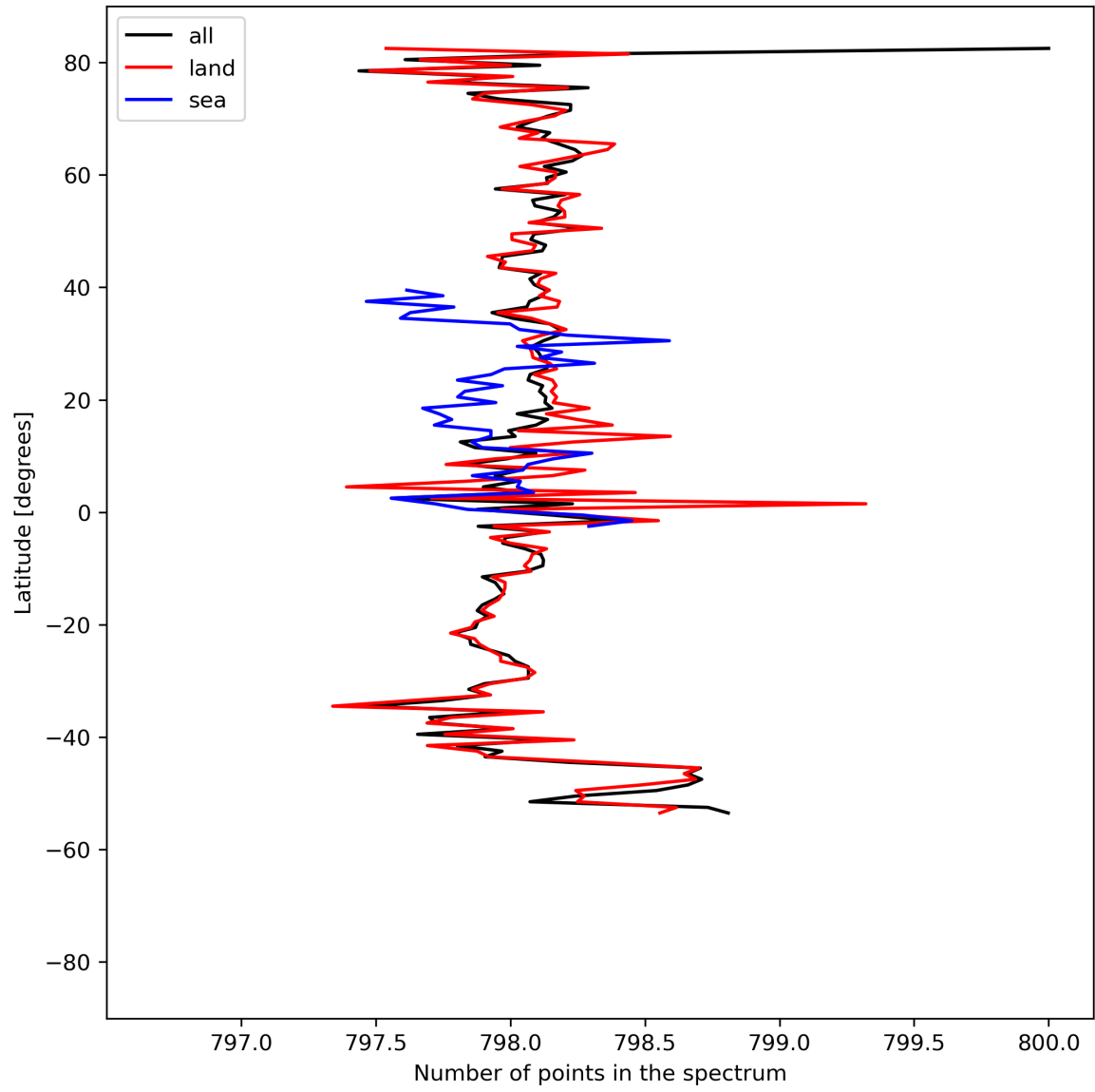
Figure 15: Zonal average of “Number of points in the spectrum” for 2024-08-18 to 2024-08-20.
