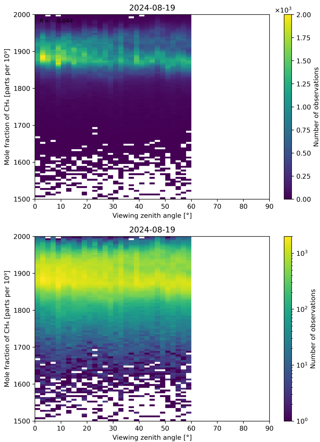
Figure 110: Scatter density plot of “Viewing zenith angle” against “Mole fraction of CH 4 ” for 2024-08-18 to 2024-08-20.
