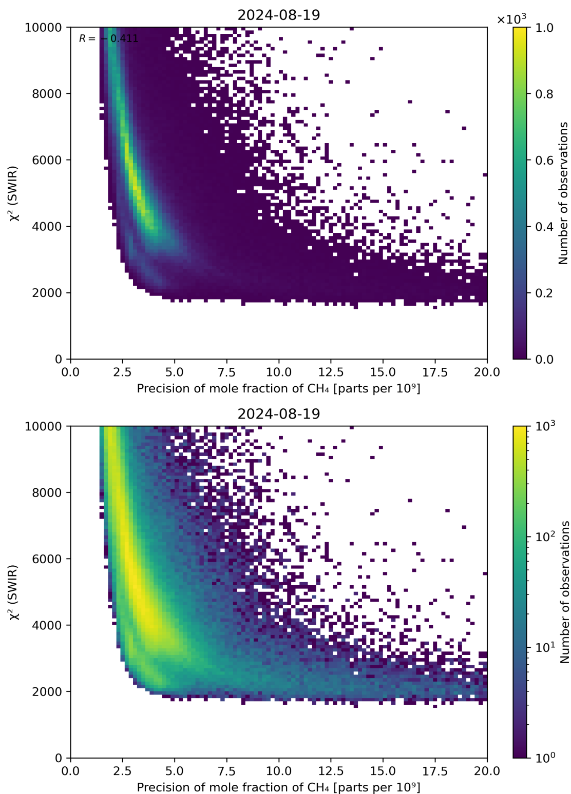
Figure 79: Scatter density plot of “Precision of mole fraction of \text{CH}_4 ” against “ \chi^2 (SWIR)” for 2024-08-18 to 2024-08-20.
