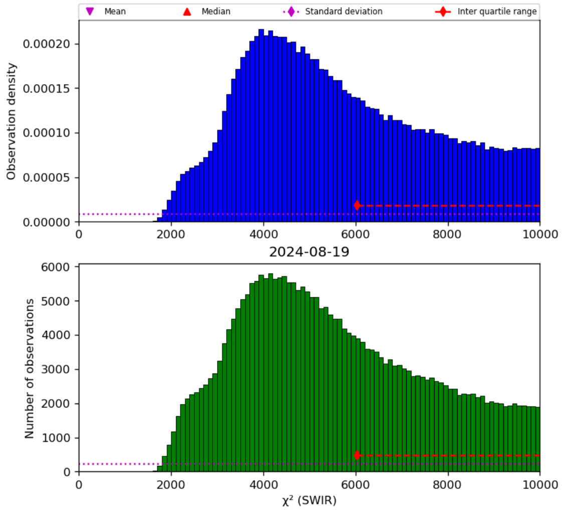
Figure 28: Histogram of “ \chi^2 (SWIR)” for 2024-08-18 to 2024-08-20
