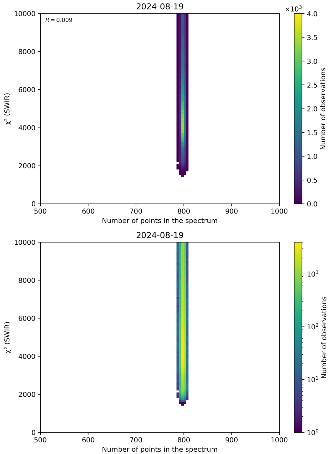
Figure 89: Scatter density plot of “Number of points in the spectrum” against “ \chi^2 (SWIR)” for 2024-08-18 to 2024-08-20.
