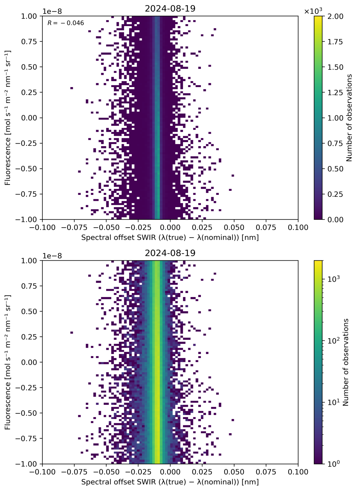
Figure 120: Scatter density plot of “Spectral offset SWIR ( \lambda(\text{true}) - \lambda(\text{nominal}) )” against “Fluorescence” for 2024-08-18 to 2024-08-20.
