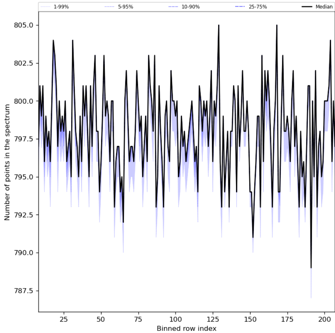
Figure 37: Along track statistics of “Number of points in the spectrum” for 2024-08-18 to 2024-08-20
