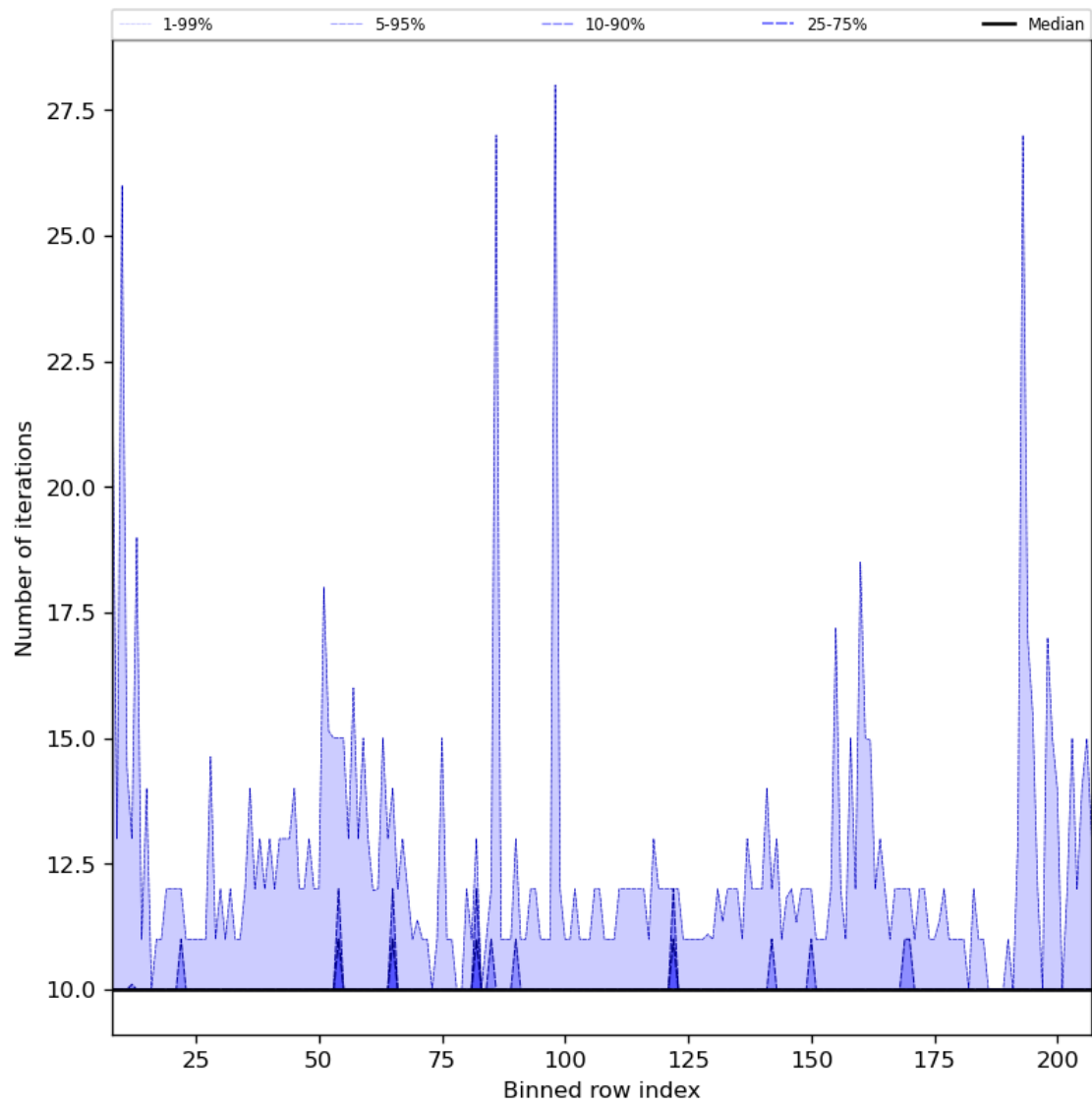
Figure 42: Along track statistics of “Number of iterations” for 2024-08-18 to 2024-08-20
