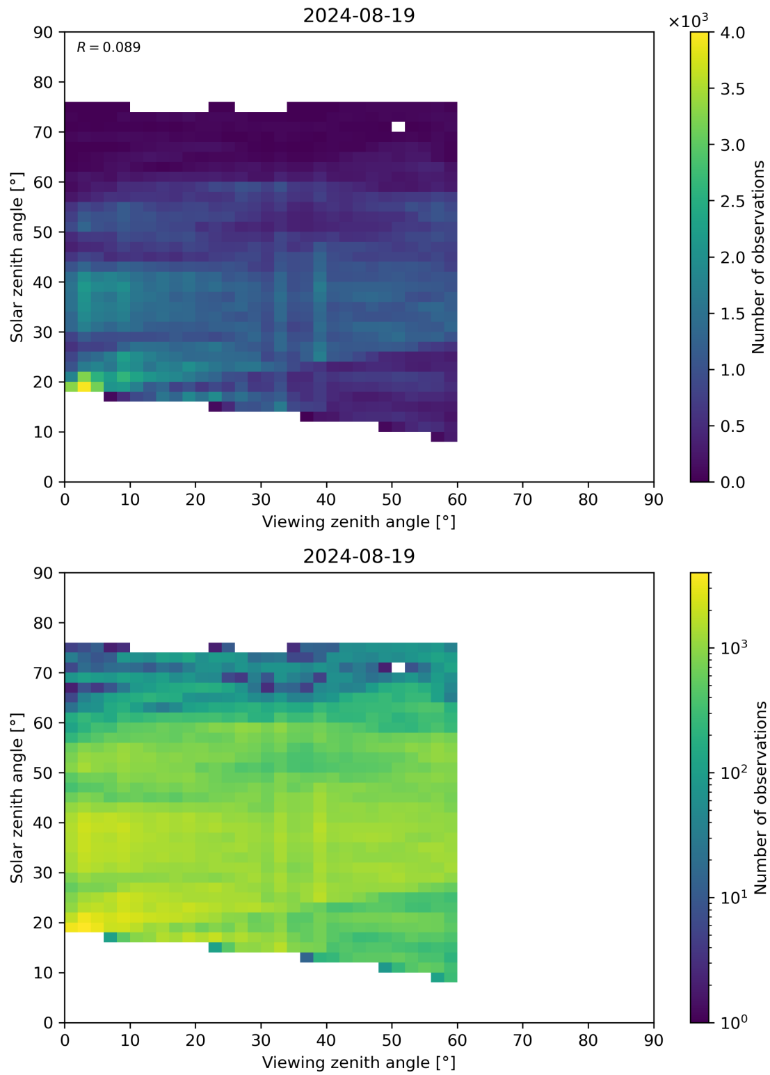
Figure 115: Scatter density plot of “Viewing zenith angle” against “Solar zenith angle” for 2024-08-18 to 2024-08-20.
