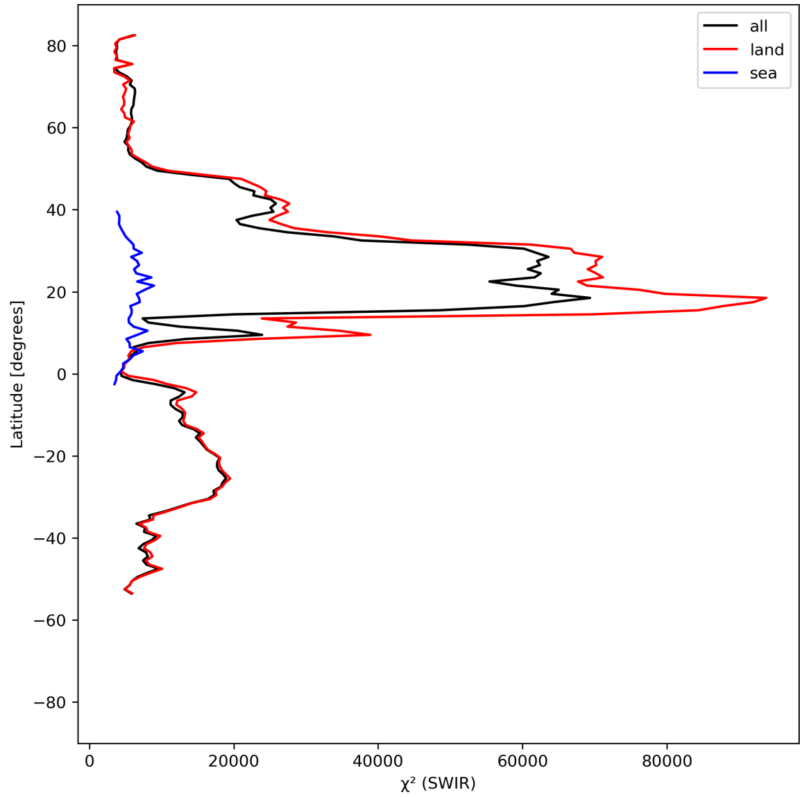
Figure 17: Zonal average of “ \chi^2 (SWIR)” for 2024-08-18 to 2024-08-20.
