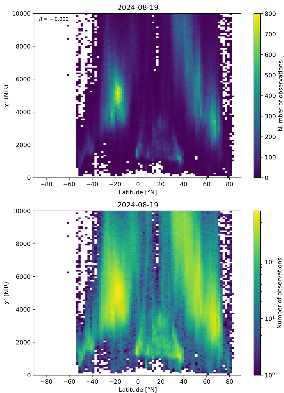
Figure 53: Scatter density plot of “Latitude” against “ \chi^2 (NIR)” for 2024-08-18 to 2024-08-20.
