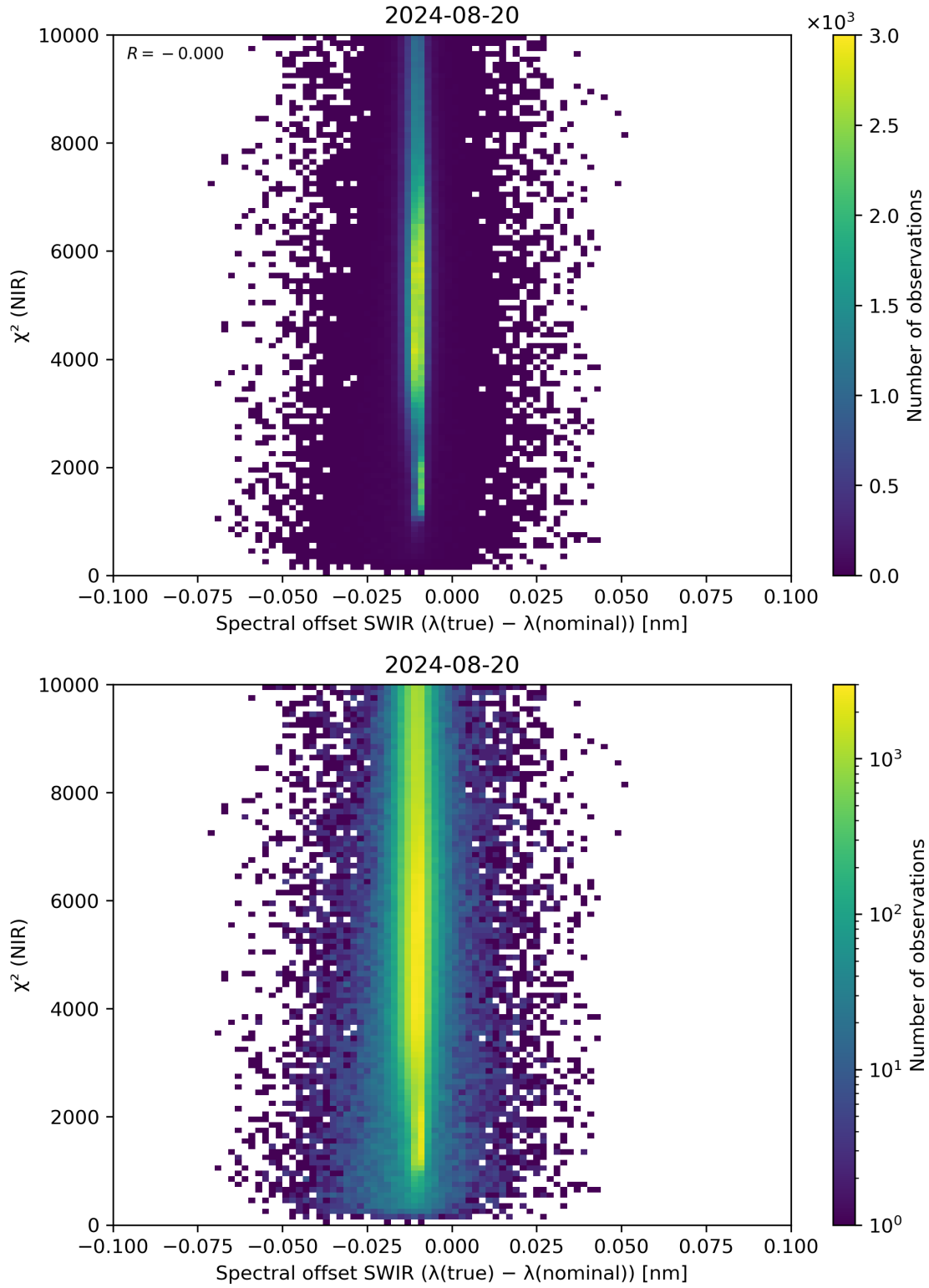
Figure 117: Scatter density plot of “Spectral offset SWIR ( \lambda(\text{true}) - \lambda(\text{nominal}) )” against “ \chi^2 (NIR)” for 2024-08-19 to 2024-08-21.
