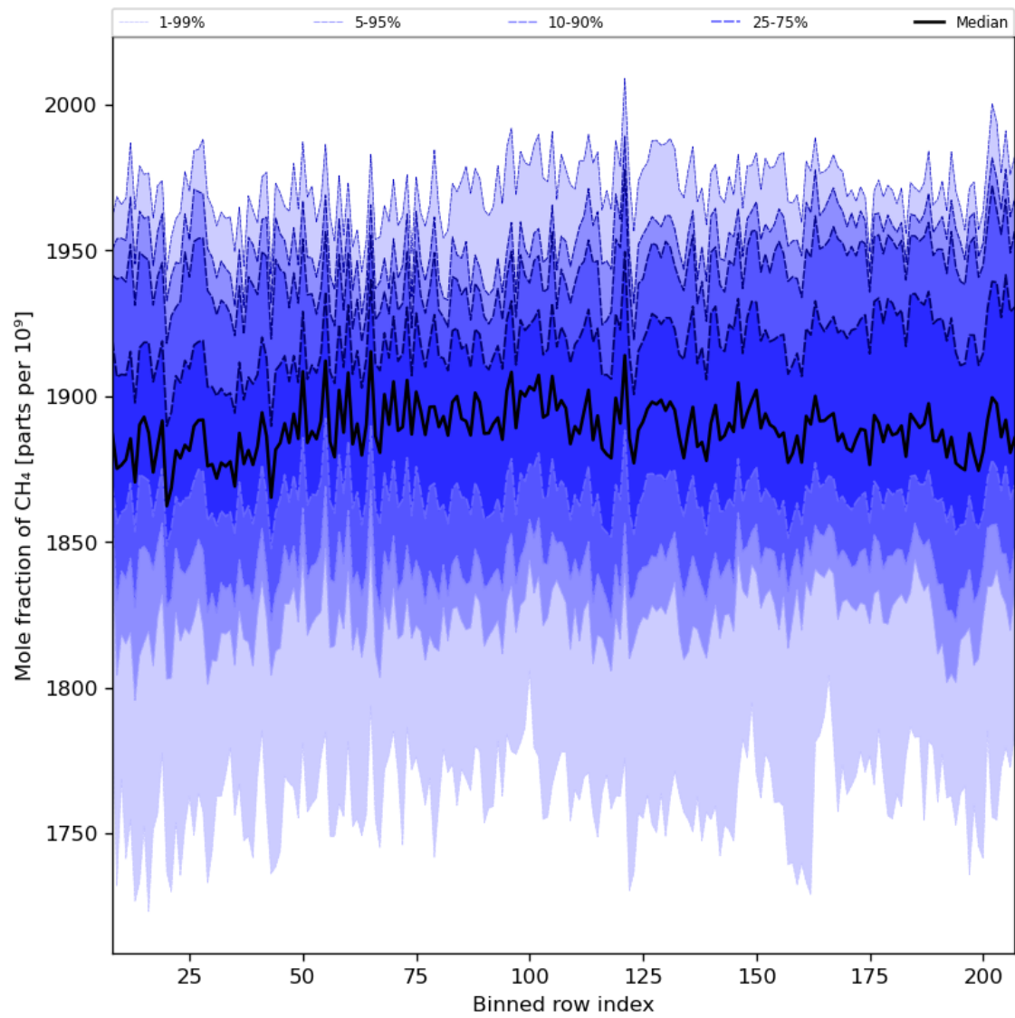
Figure 34: Along track statistics of “Mole fraction of CH 4 ” for 2024-08-19 to 2024-08-21
