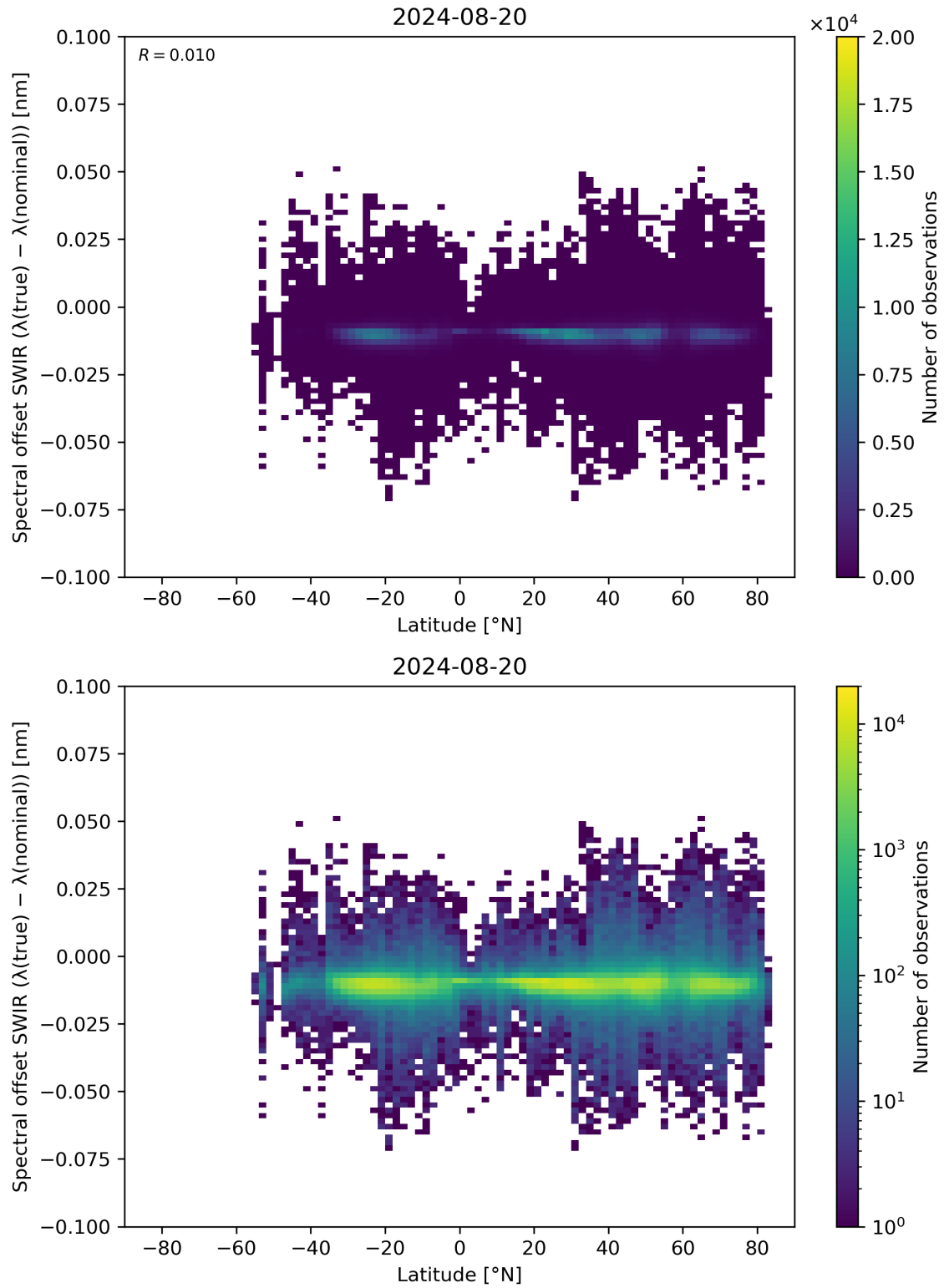
Figure 62: Scatter density plot of “Latitude” against “Spectral offset SWIR ( \lambda(\text{true}) - \lambda(\text{nominal}) )” for 2024-08-19 to 2024-08-21.
