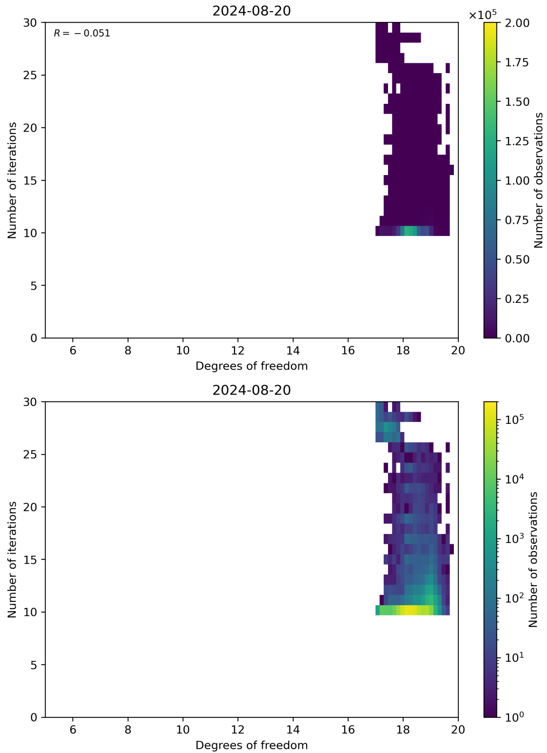
Figure 52: Scatter density plot of “Degrees of freedom” against “Number of iterations” for 2024-08-19 to 2024-08-21.
