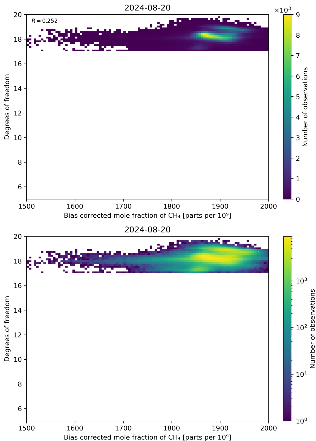
Figure 65: Scatter density plot of “Bias corrected mole fraction of CH 4 ” against “Degrees of freedom” for 2024-08-19 to 2024-08-21.
