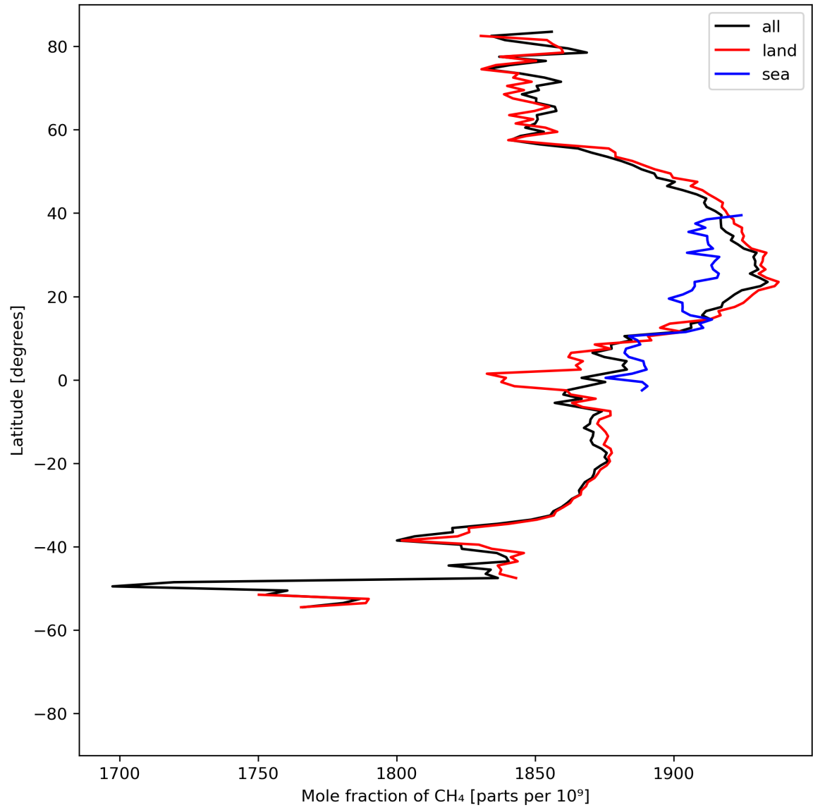
Figure 12: Zonal average of “Mole fraction of \text{CH}_4 ” for 2024-08-19 to 2024-08-21.
