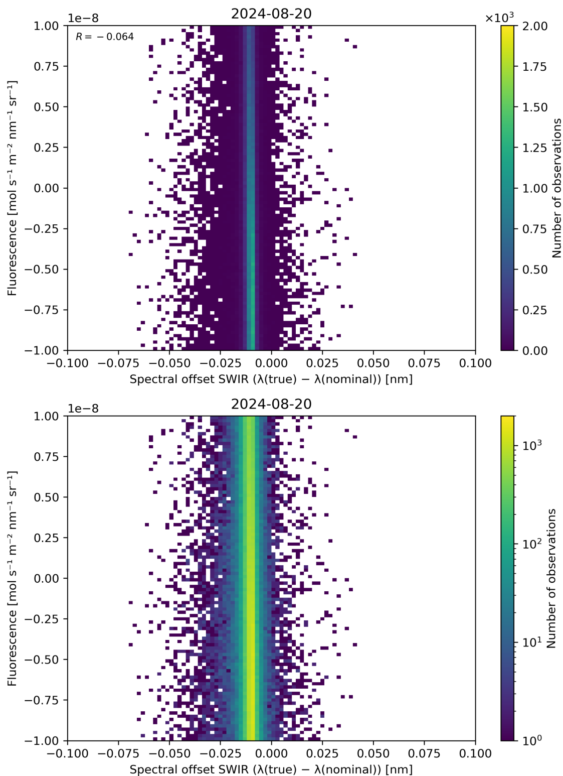
Figure 120: Scatter density plot of “Spectral offset SWIR ( \lambda(\text{true}) - \lambda(\text{nominal}) )” against “Fluorescence” for 2024-08-19 to 2024-08-21.
