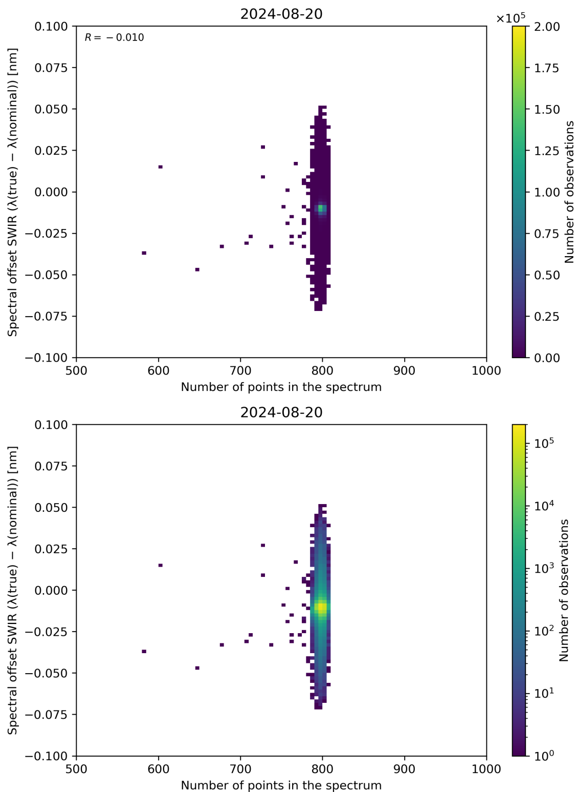
Figure 93: Scatter density plot of “Number of points in the spectrum” against “Spectral offset SWIR ( \lambda(\text{true}) - \lambda(\text{nominal}) )” for 2024-08-19 to 2024-08-21.
