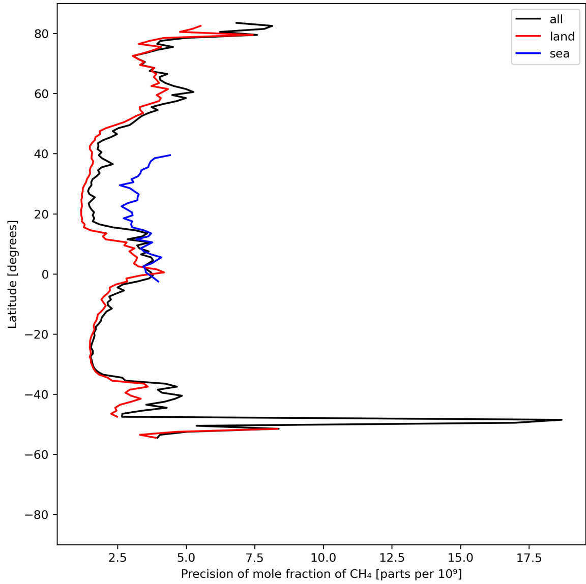
Figure 13: Zonal average of “Precision of mole fraction of CH 4 ” for 2024-08-19 to 2024-08-21.
