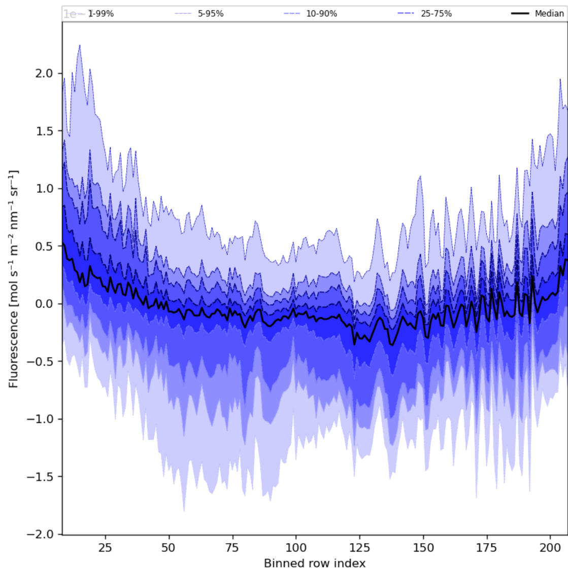
Figure 43: Along track statistics of “Fluorescence” for 2024-08-19 to 2024-08-21
