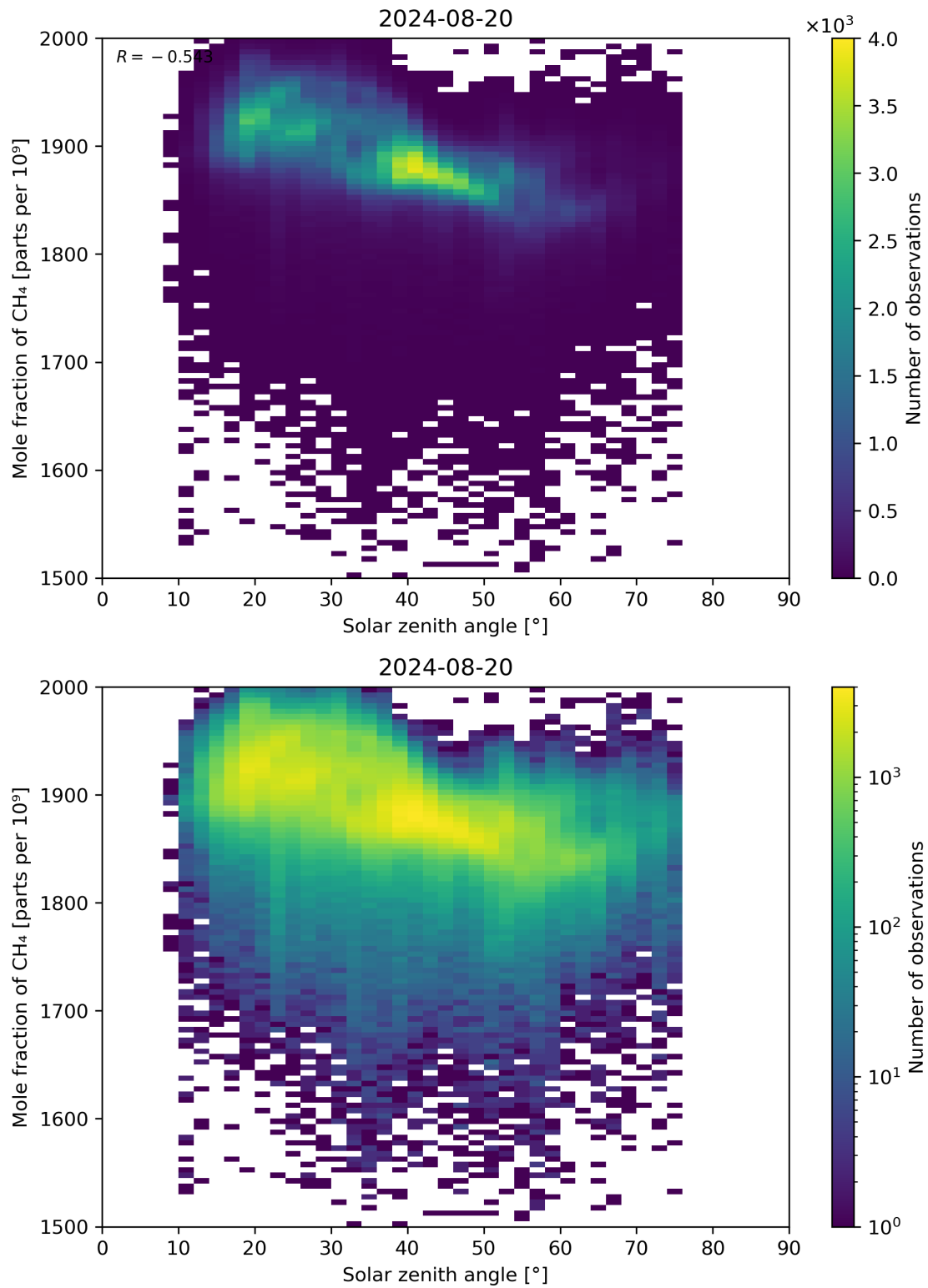
Figure 99: Scatter density plot of “Solar zenith angle” against “Mole fraction of CH 4 ” for 2024-08-19 to 2024-08-21.
