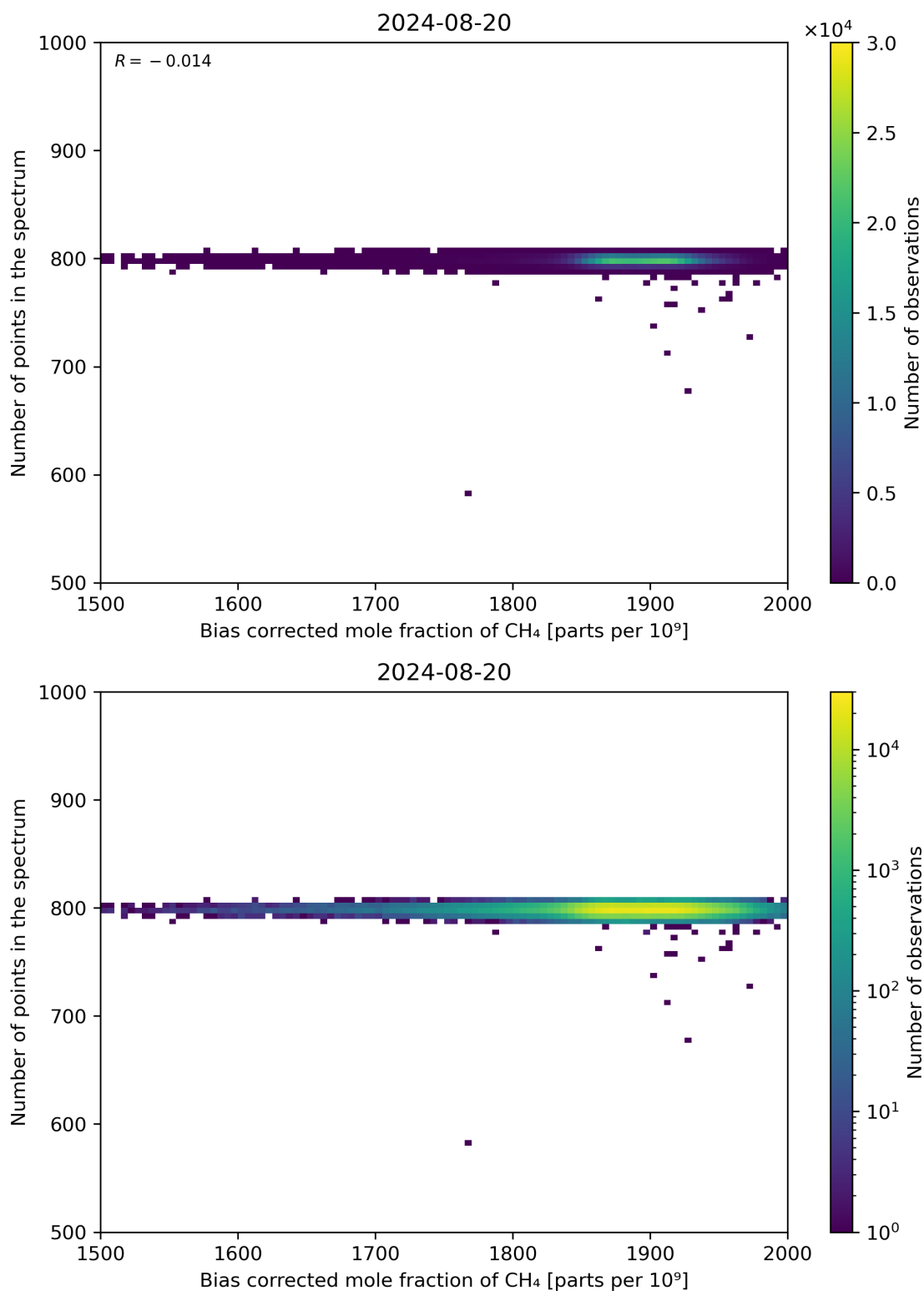
Figure 68: Scatter density plot of “Bias corrected mole fraction of CH 4 ” against “Number of points in the spectrum” for 2024-08-19 to 2024-08-21.
