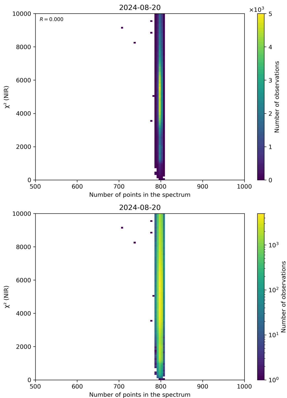
Figure 88: Scatter density plot of “Number of points in the spectrum” against “ \chi^2 (NIR)” for 2024-08-19 to 2024-08-21.
