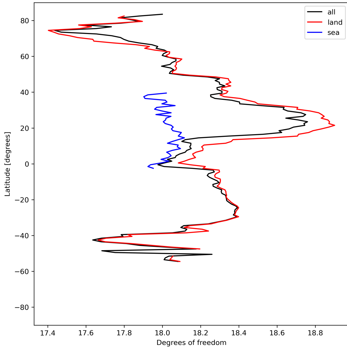
Figure 19: Zonal average of “Degrees of freedom” for 2024-08-19 to 2024-08-21.
