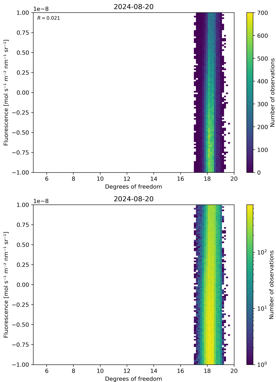
Figure 51: Scatter density plot of “Degrees of freedom” against “Fluorescence” for 2024-08-19 to 2024-08-21.
