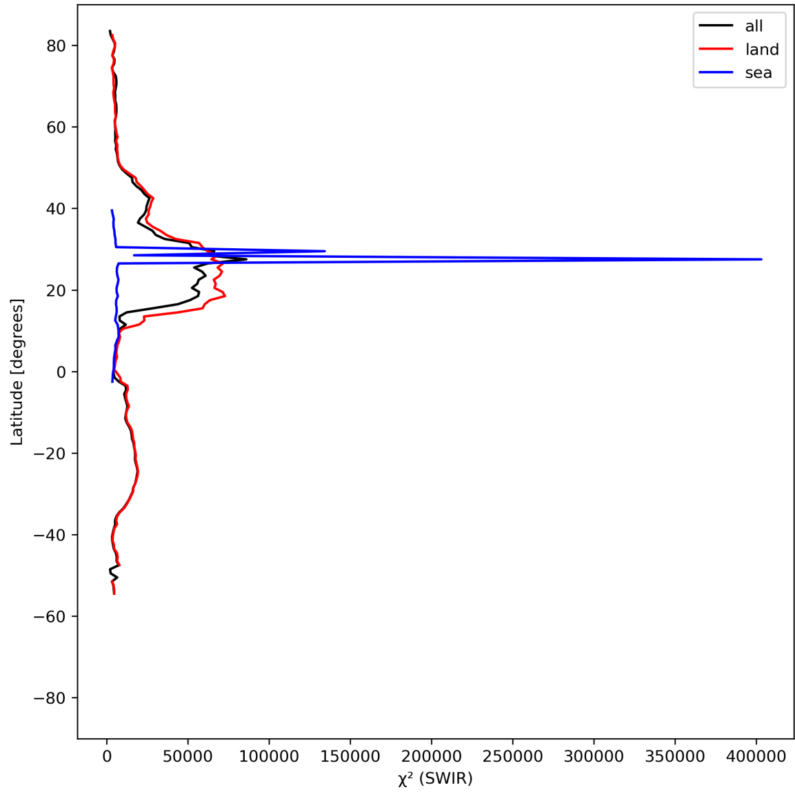
Figure 17: Zonal average of “ \chi^2 (SWIR)” for 2024-08-19 to 2024-08-21.
