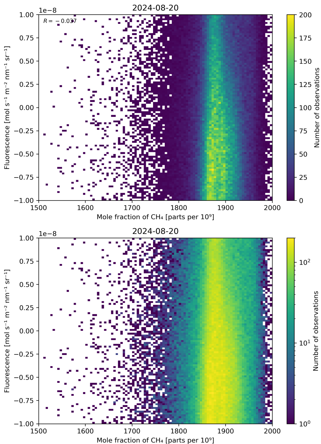
Figure 73: Scatter density plot of “Mole fraction of \text{CH}_4 ” against “Fluorescence” for 2024-08-19 to 2024-08-21.
