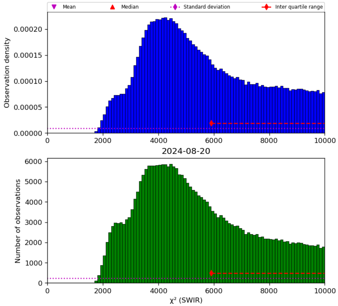
Figure 28: Histogram of " \chi^2 (SWIR)" for 2024-08-19 to 2024-08-21
