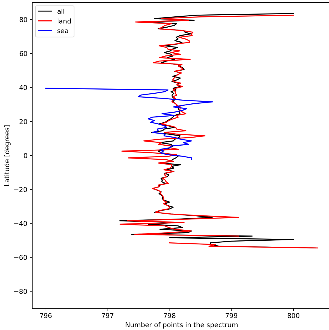
Figure 15: Zonal average of “Number of points in the spectrum” for 2024-08-19 to 2024-08-21.
