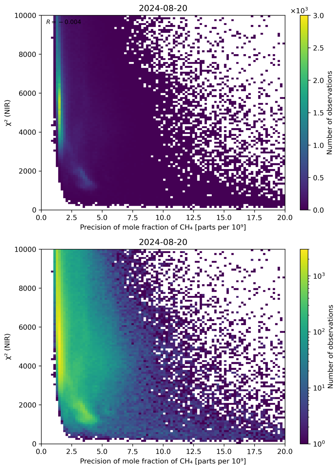
Figure 78: Scatter density plot of “Precision of mole fraction of CH 4 ” against “ \chi^2 (NIR)” for 2024-08-19 to 2024-08-21.
