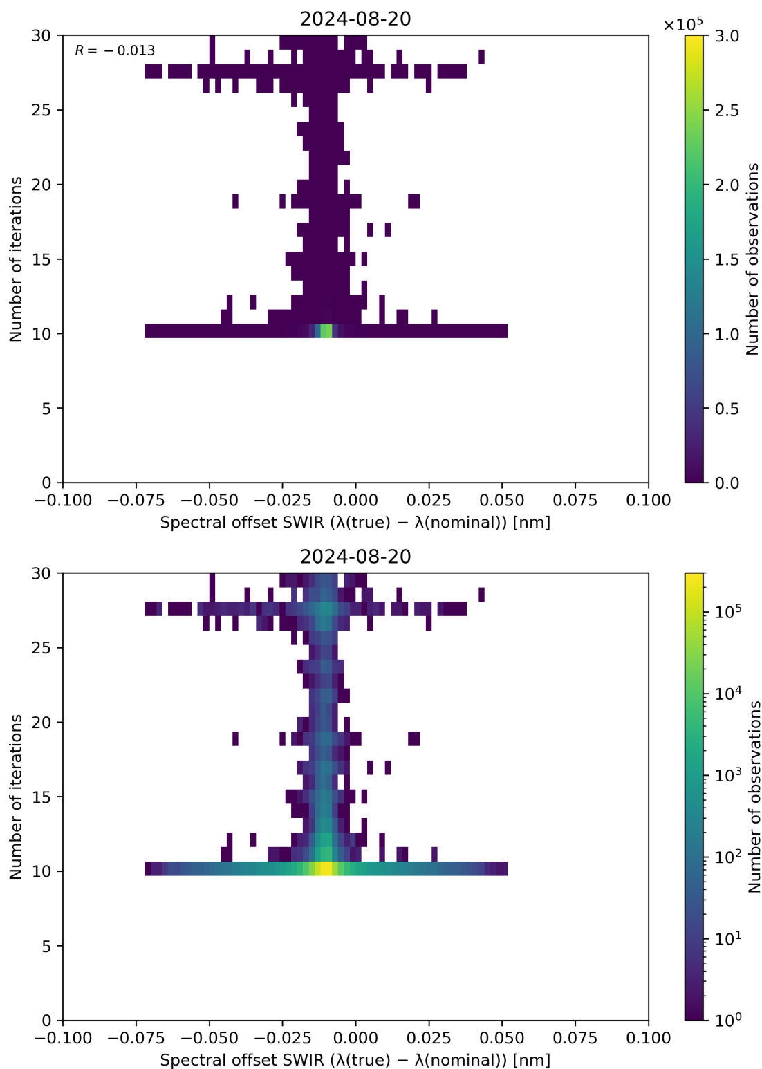
Figure 121: Scatter density plot of “Spectral offset SWIR ( \lambda(\text{true}) - \lambda(\text{nominal}) )” against “Number of iterations” for 2024-08-19 to 2024-08-21.
