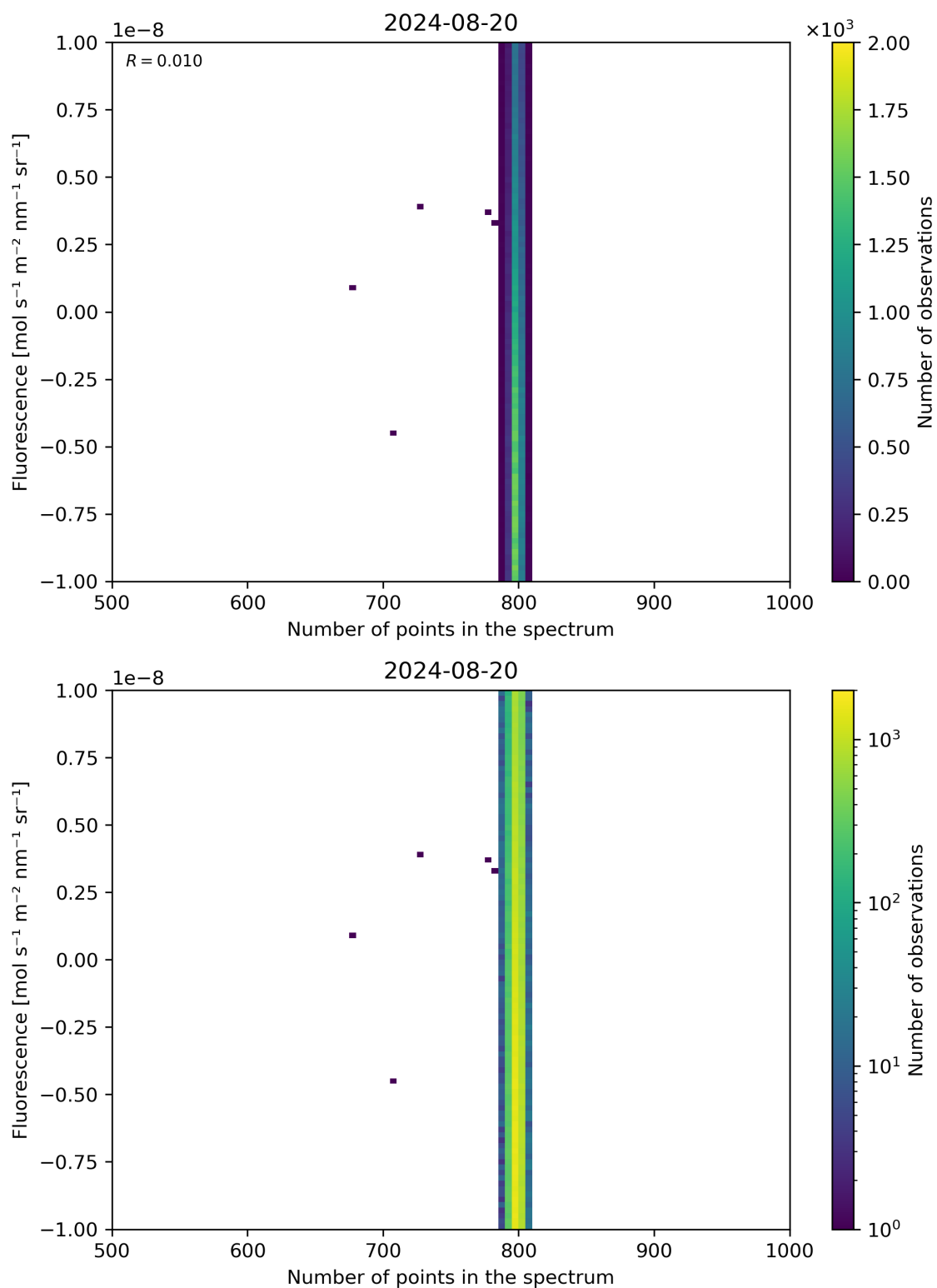
Figure 91: Scatter density plot of “Number of points in the spectrum” against “Fluorescence” for 2024-08-19 to 2024-08-21.
