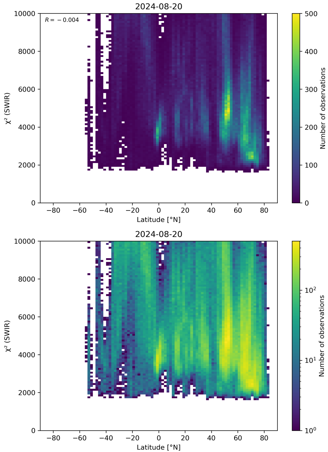
Figure 54: Scatter density plot of “Latitude” against “ \chi^2 (SWIR)” for 2024-08-19 to 2024-08-21.
