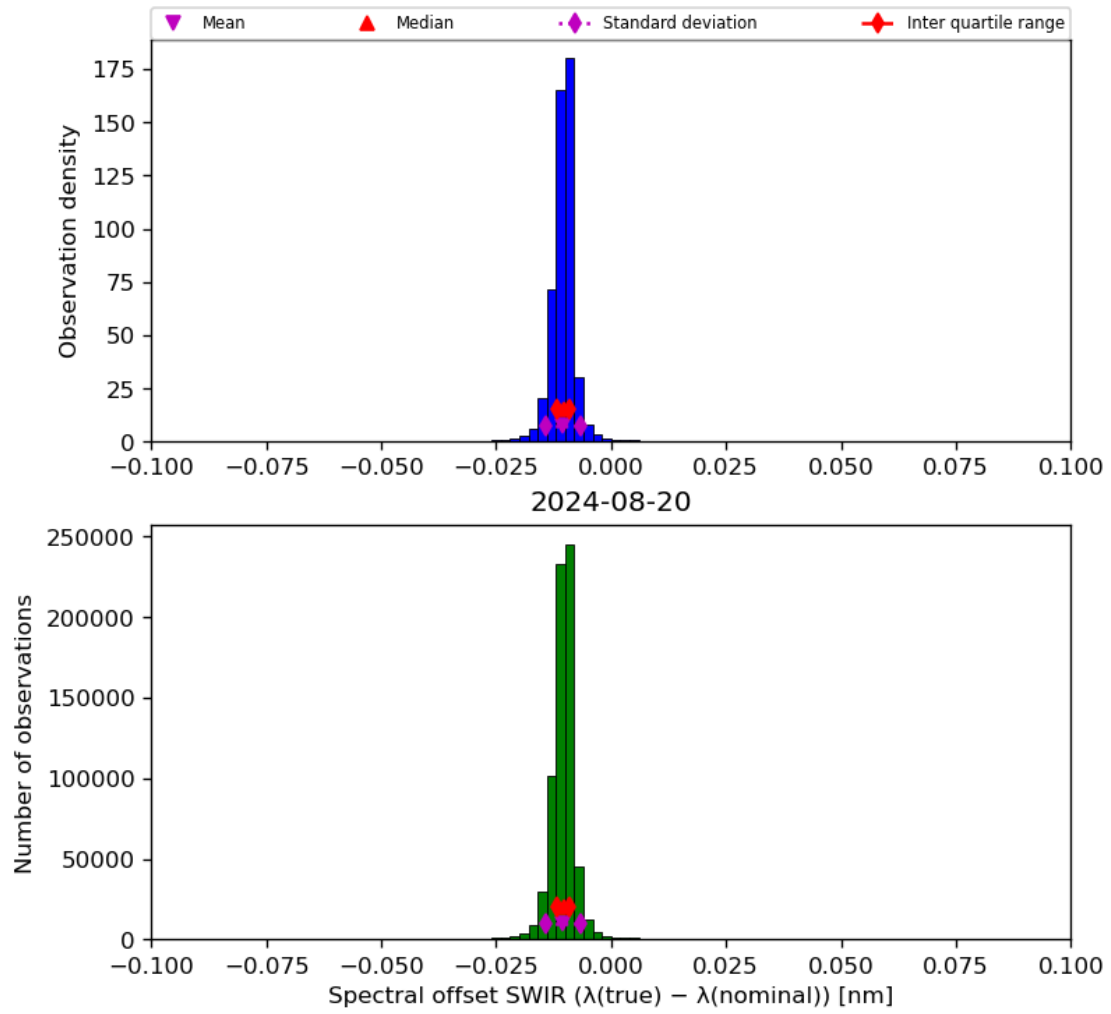
Figure 27: Histogram of “Spectral offset SWIR ( \lambda(\text{true}) - \lambda(\text{nominal}) )” for 2024-08-19 to 2024-08-21
