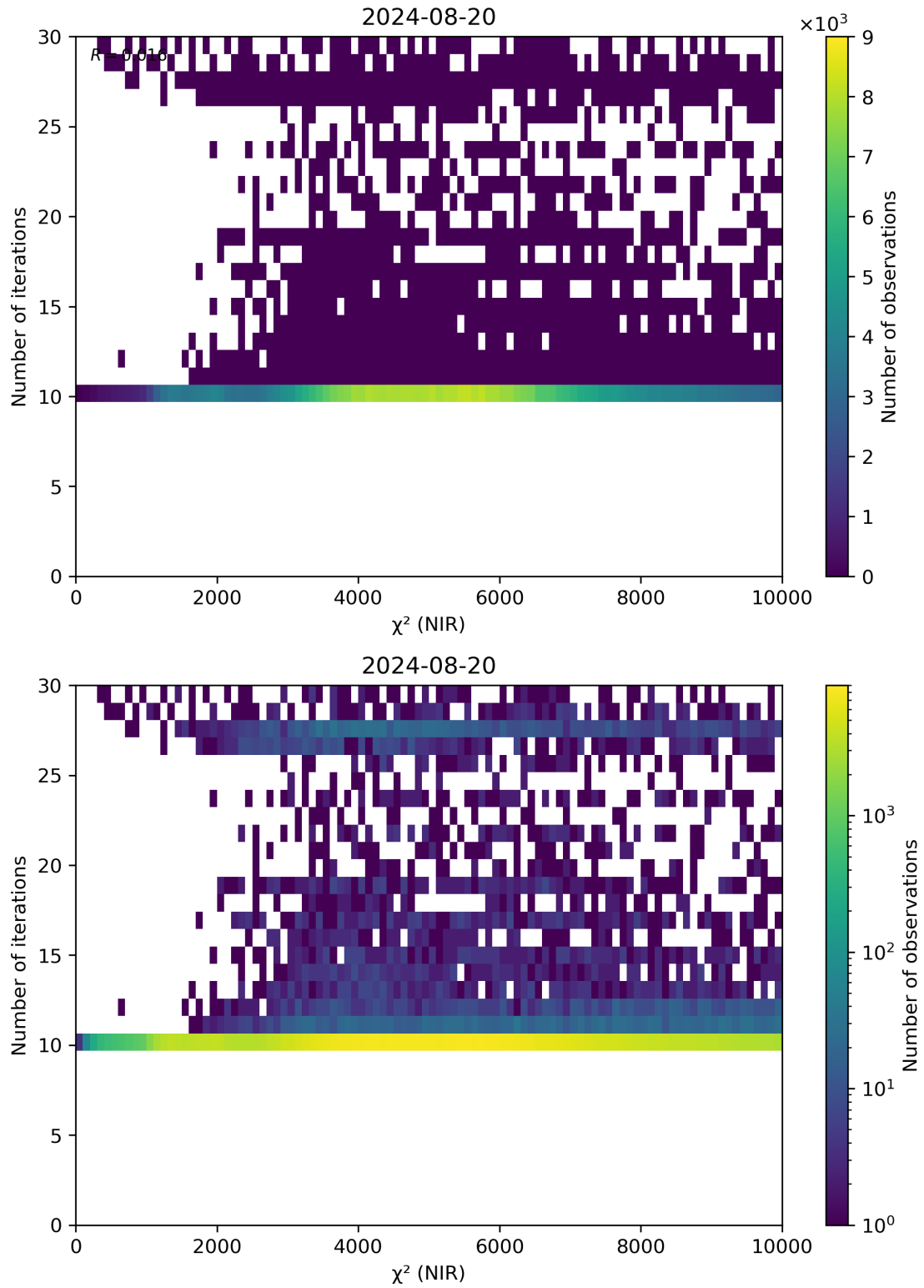
Figure 46: Scatter density plot of “ \chi^2 (NIR)” against “Number of iterations” for 2024-08-19 to 2024-08-21.
