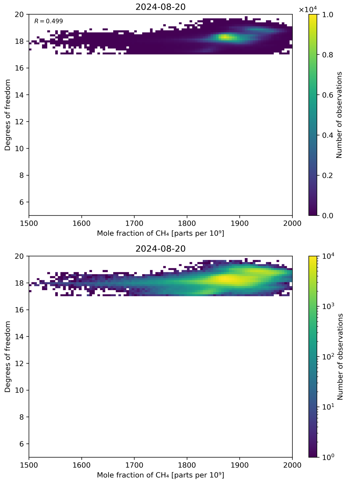
Figure 72: Scatter density plot of “Mole fraction of CH 4 ” against “Degrees of freedom” for 2024-08-19 to 2024-08-21.
