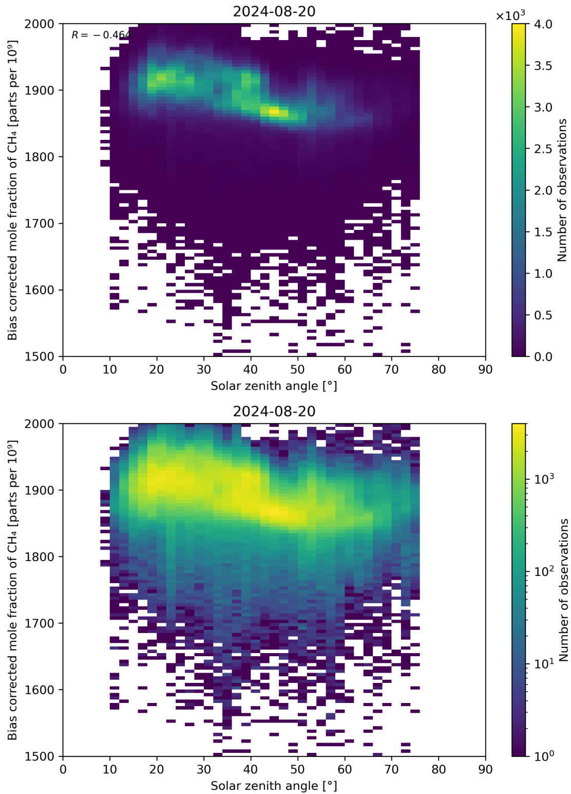
Figure 100: Scatter density plot of “Solar zenith angle” against “Bias corrected mole fraction of CH 4 ” for 2024-08-19 to 2024-08-21.
