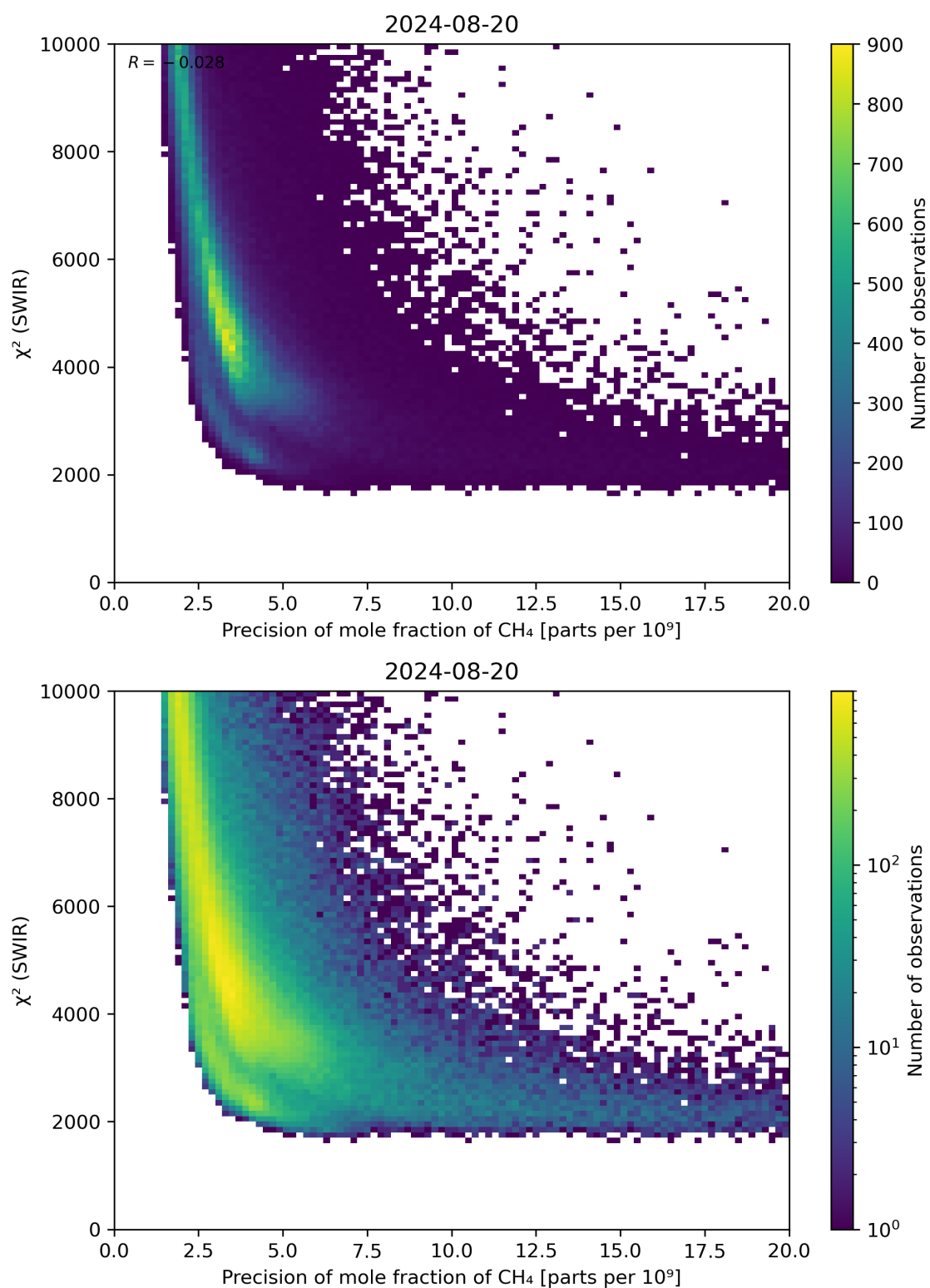
Figure 79: Scatter density plot of “Precision of mole fraction of CH 4 ” against “ \chi^2 (SWIR)” for 2024-08-19 to 2024-08-21.
