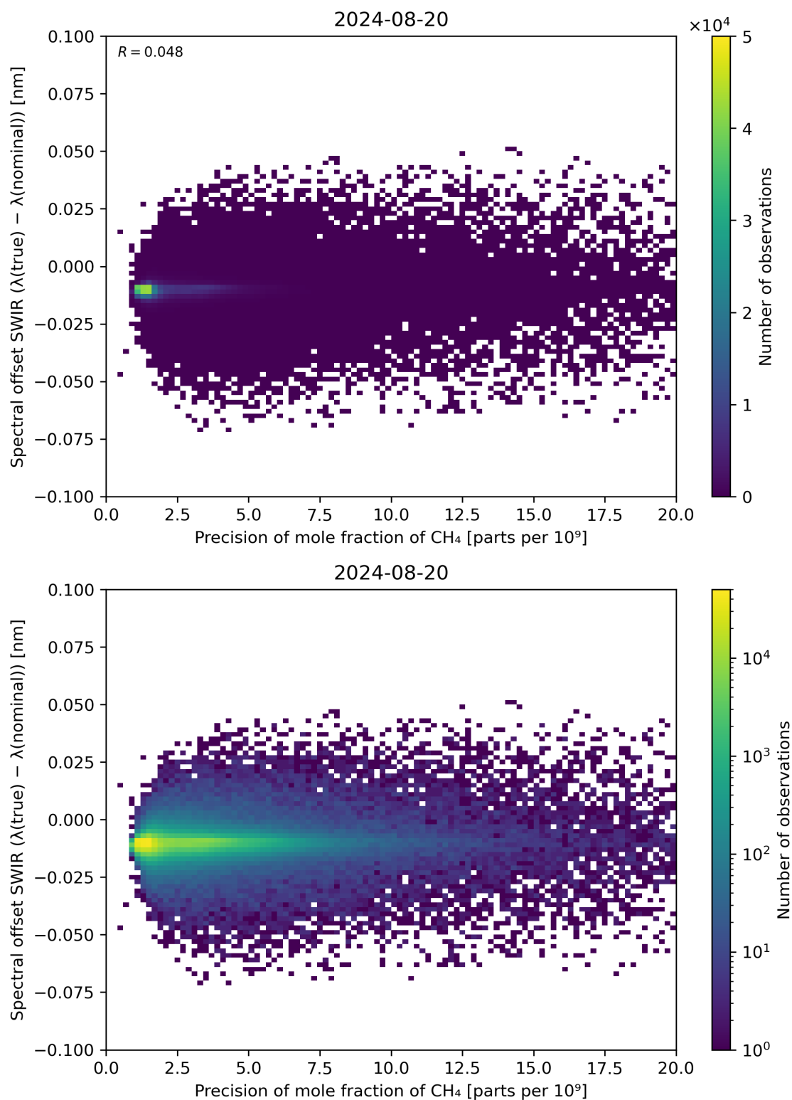
Figure 85: Scatter density plot of “Precision of mole fraction of \text{CH}_4 ” against “Spectral offset SWIR ( \lambda(\text{true}) - \lambda(\text{nominal}) )” for 2024-08-19 to 2024-08-21.
