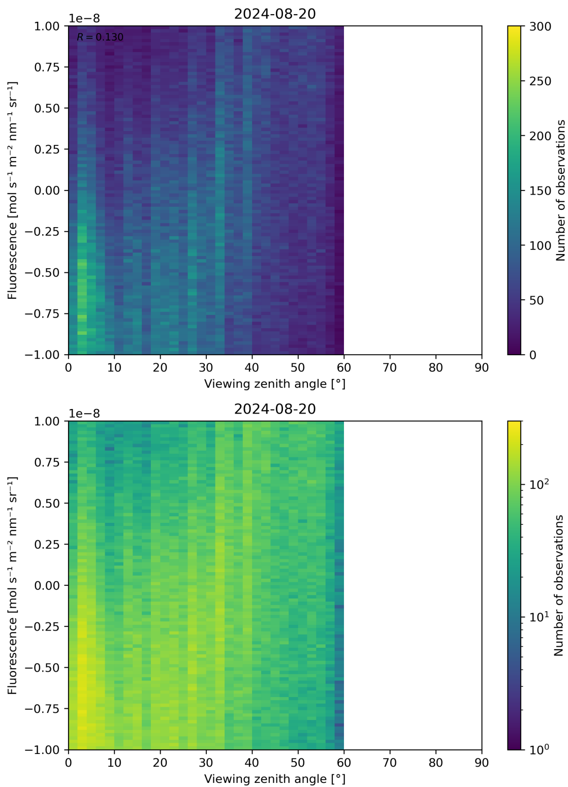
Figure 108: Scatter density plot of “Viewing zenith angle” against “Fluorescence” for 2024-08-19 to 2024-08-21.
