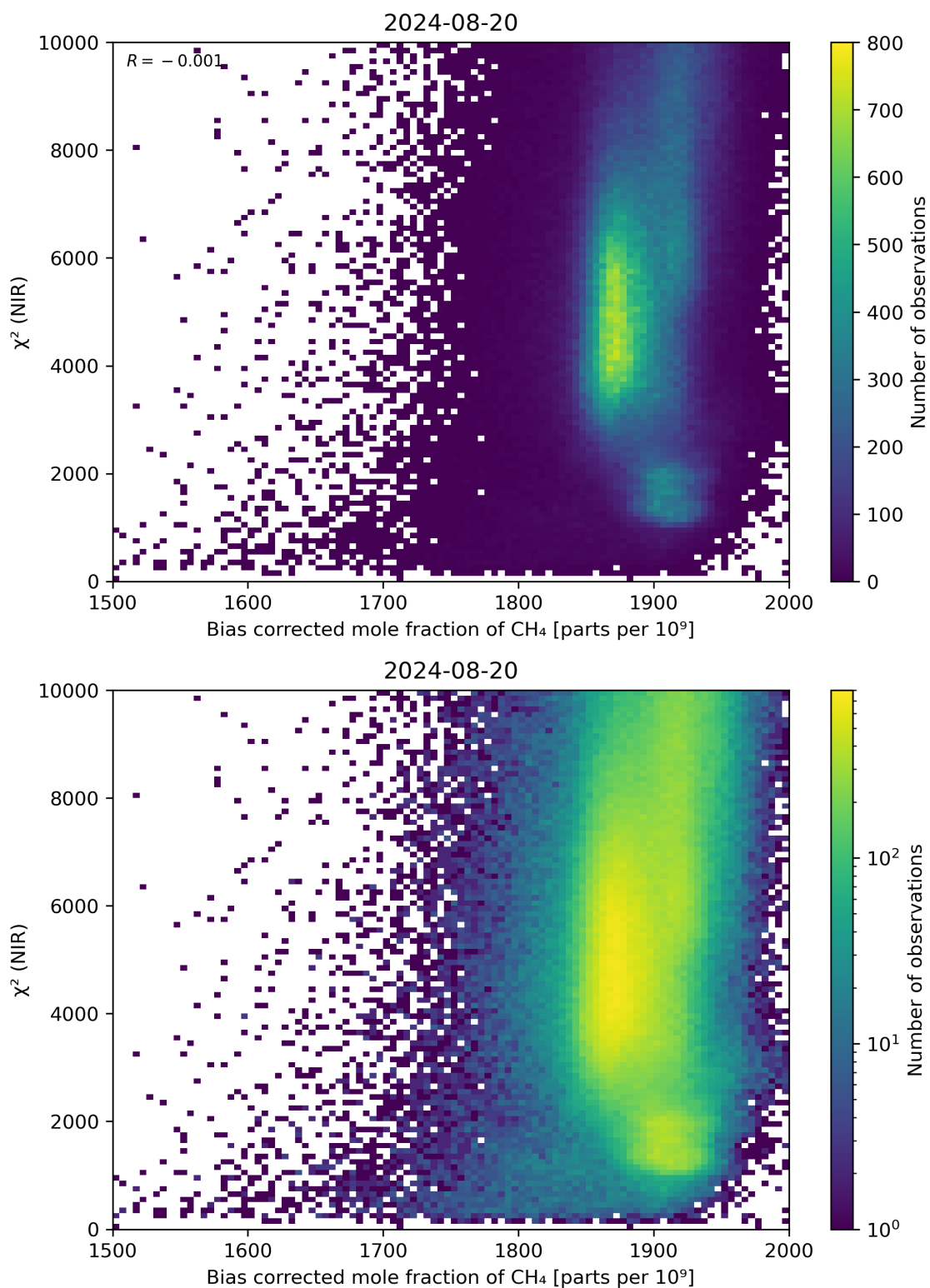
Figure 63: Scatter density plot of “Bias corrected mole fraction of CH 4 ” against “ \chi^2 (NIR)” for 2024-08-19 to 2024-08-21.
