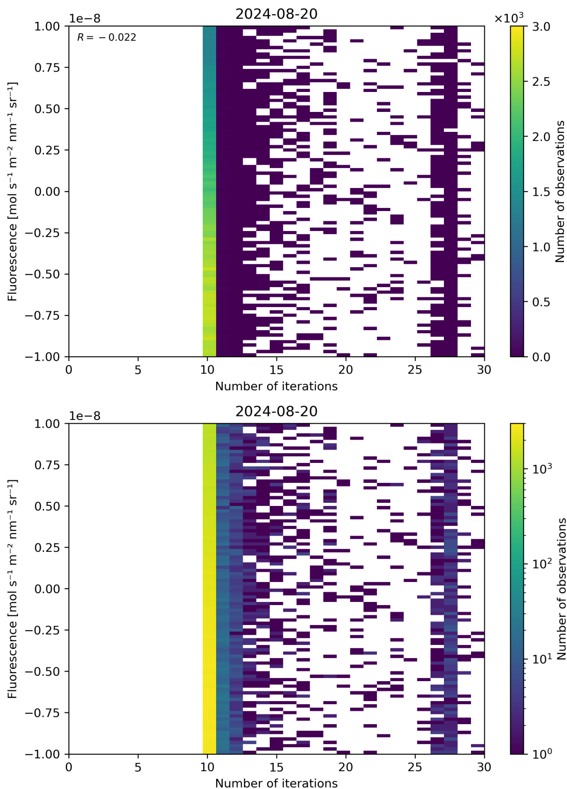
Figure 87: Scatter density plot of “Number of iterations” against “Fluorescence” for 2024-08-19 to 2024-08-21.
