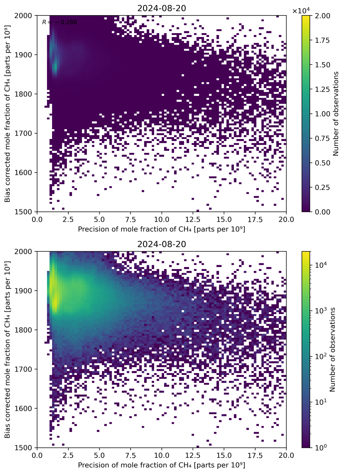
Figure 82: Scatter density plot of “Precision of mole fraction of \text{CH}_4 ” against “Bias corrected mole fraction of \text{CH}_4 ” for 2024-08-19 to 2024-08-21.
