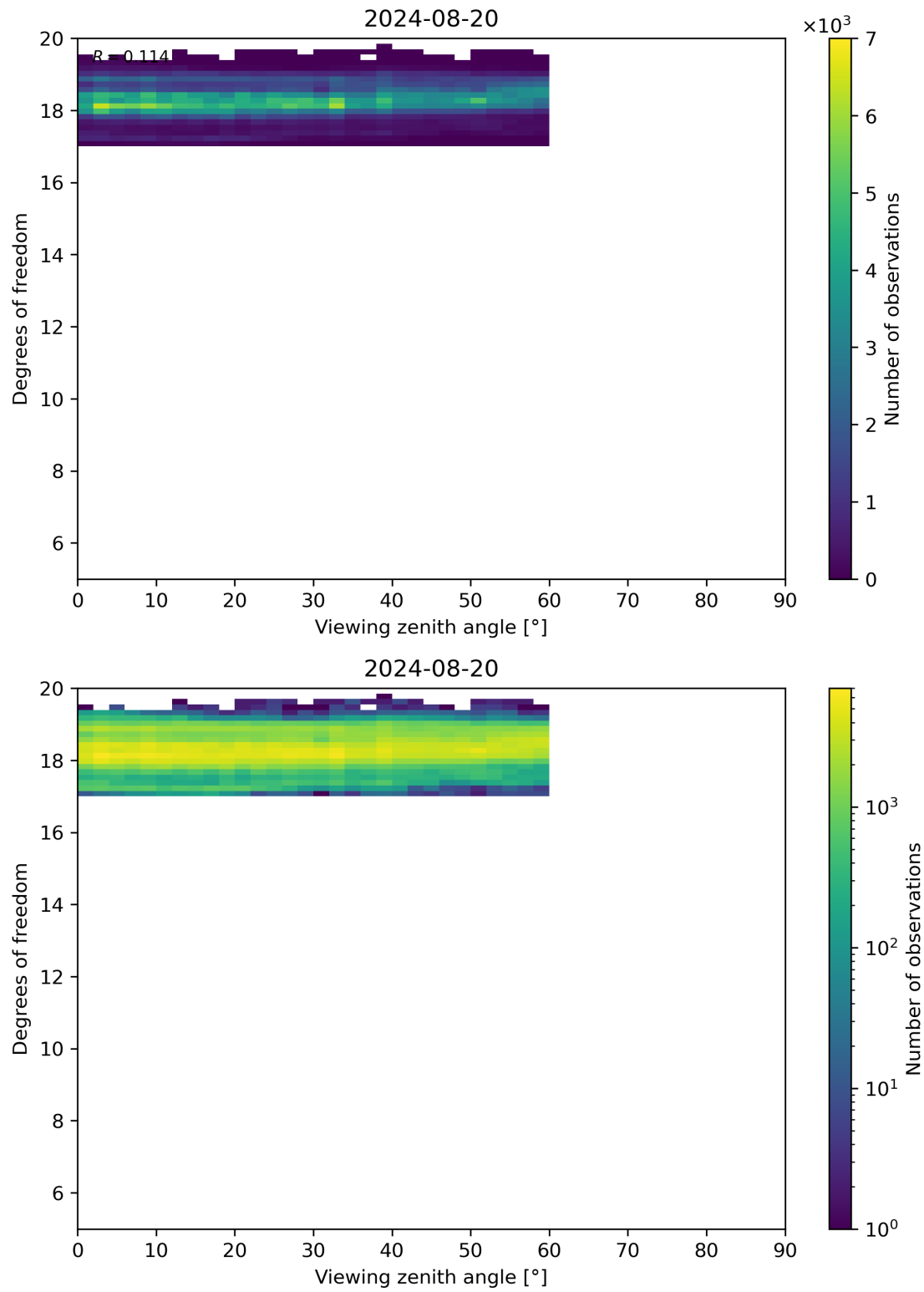
Figure 107: Scatter density plot of “Viewing zenith angle” against “Degrees of freedom” for 2024-08-19 to 2024-08-21.
