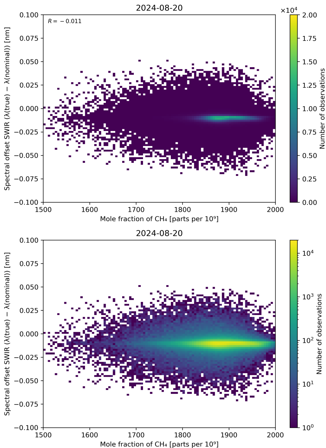
Figure 86: Scatter density plot of “Mole fraction of CH 4 ” against “Spectral offset SWIR ( \lambda(\text{true}) - \lambda(\text{nominal}) )” for 2024-08-19 to 2024-08-21.
