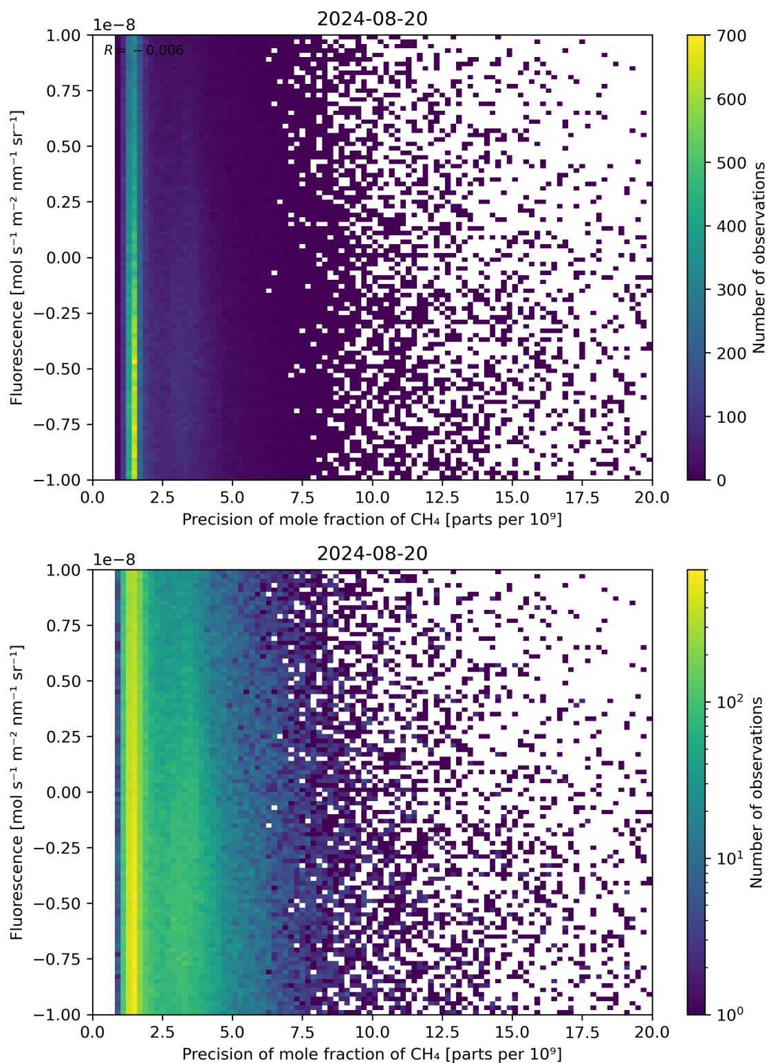
Figure 81: Scatter density plot of “Precision of mole fraction of \text{CH}_4 ” against “Fluorescence” for 2024-08-19 to 2024-08-21.
