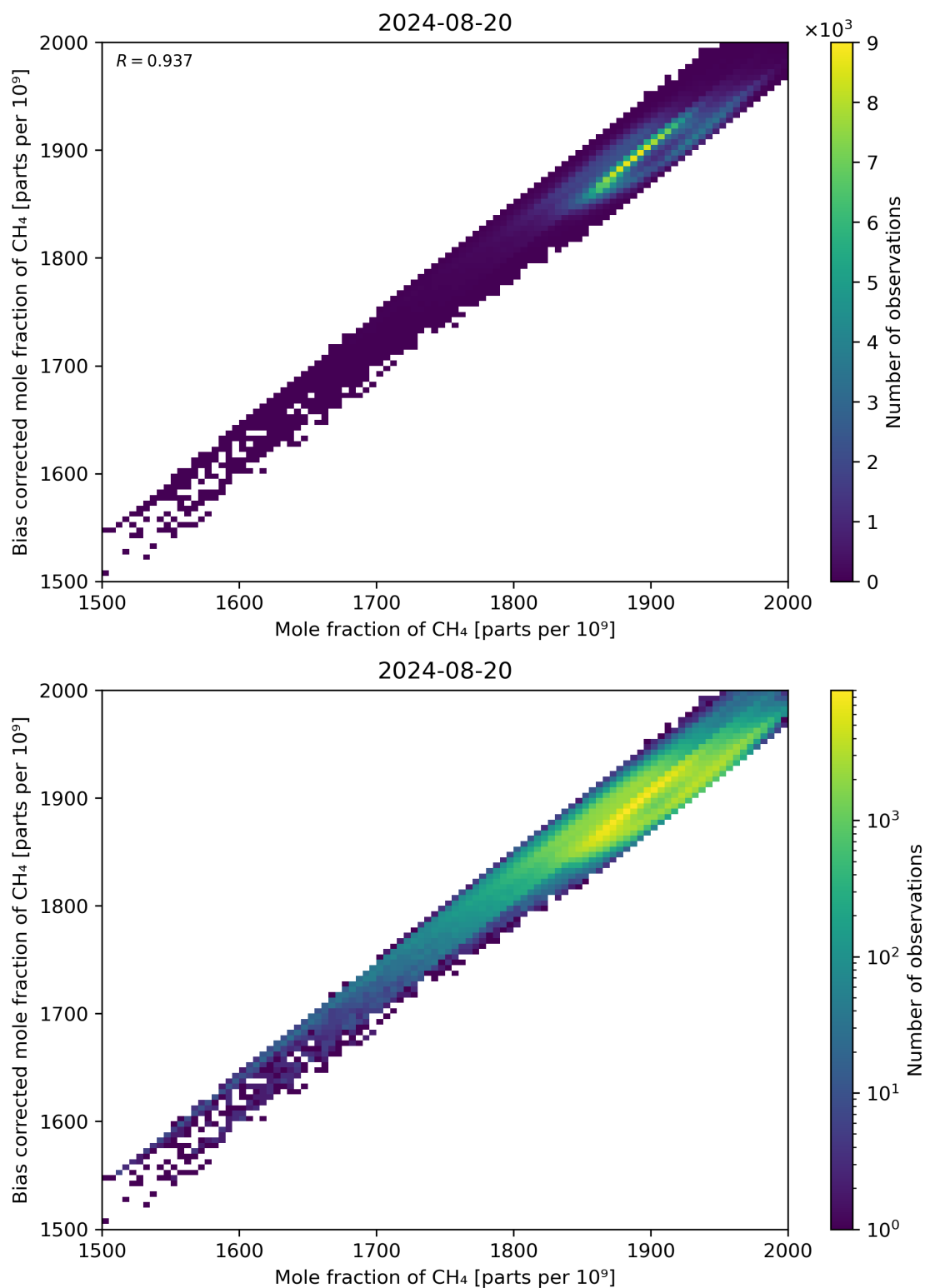
Figure 74: Scatter density plot of “Mole fraction of CH 4 ” against “Bias corrected mole fraction of CH 4 ” for 2024-08-19 to 2024-08-21.
