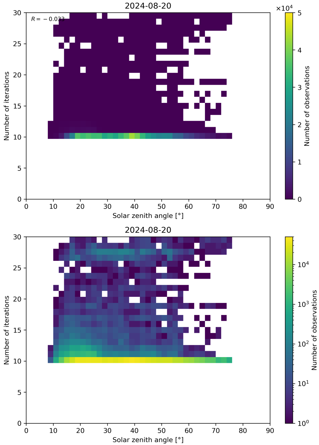
Figure 102: Scatter density plot of “Solar zenith angle” against “Number of iterations” for 2024-08-19 to 2024-08-21.
