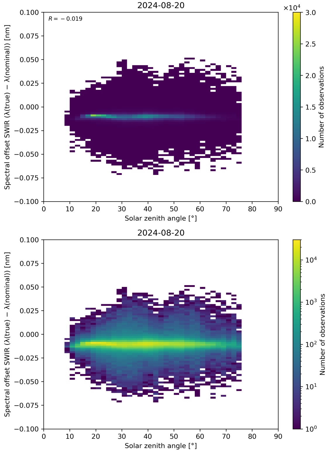
Figure 104: Scatter density plot of “Solar zenith angle” against “Spectral offset SWIR ( \lambda(\text{true}) - \lambda(\text{nominal}) )” for 2024-08-19 to 2024-08-21.
