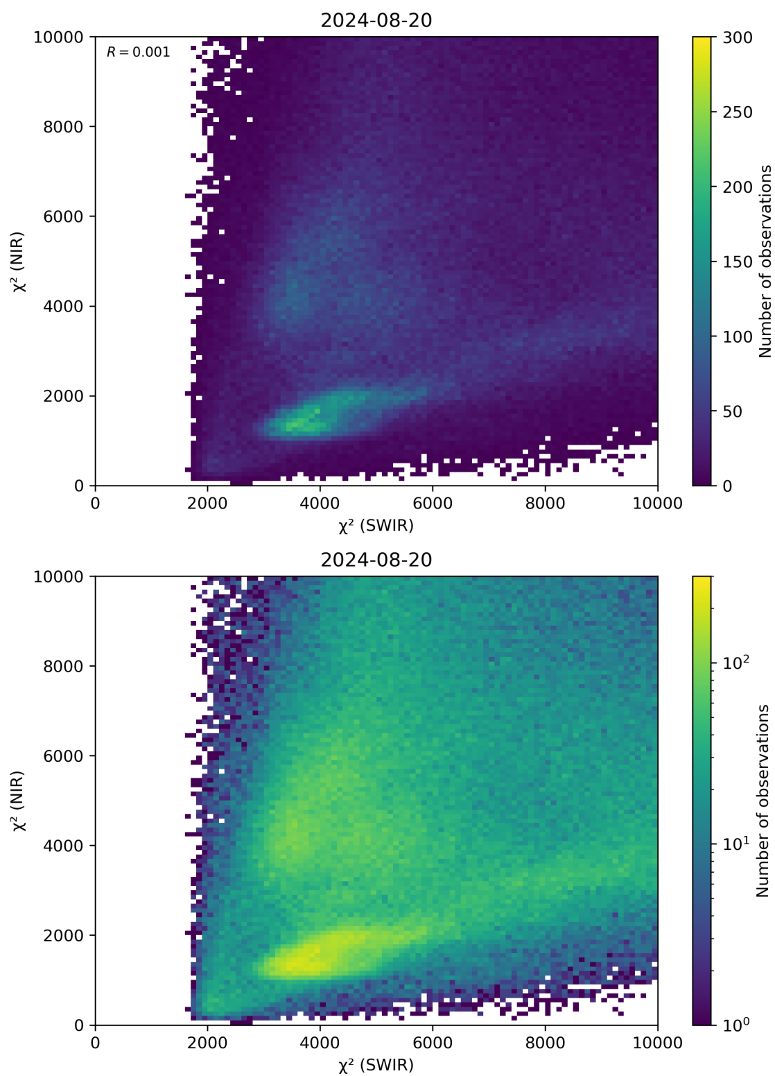
Figure 47: Scatter density plot of “ \chi^2 (SWIR)” against “ \chi^2 (NIR)” for 2024-08-19 to 2024-08-21.
