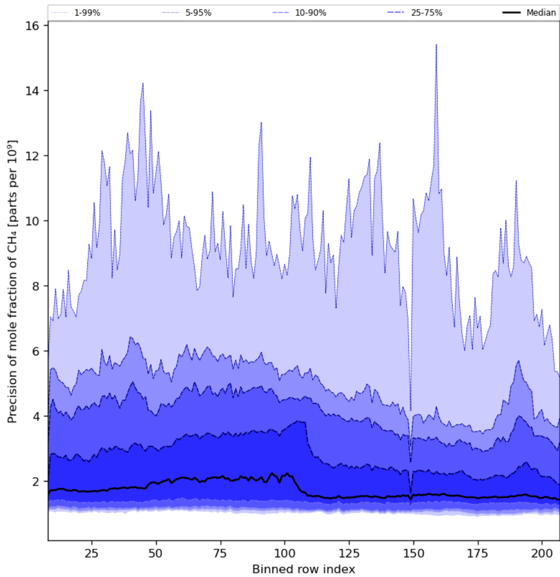
Figure 35: Along track statistics of “Precision of mole fraction of CH 4 ” for 2024-08-19 to 2024-08-21
