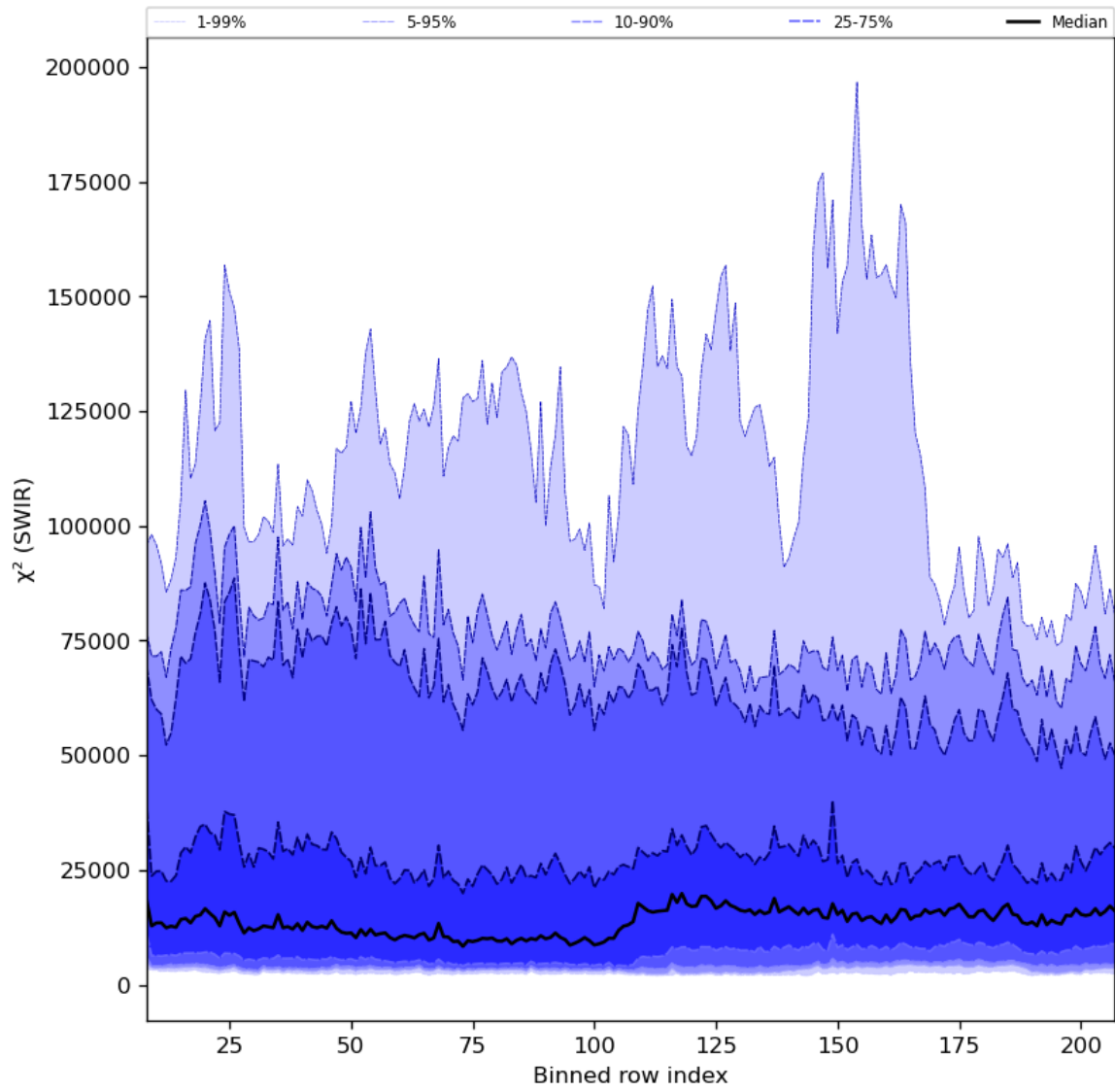
Figure 39: Along track statistics of “ \chi^2 (SWIR)” for 2024-08-19 to 2024-08-21
