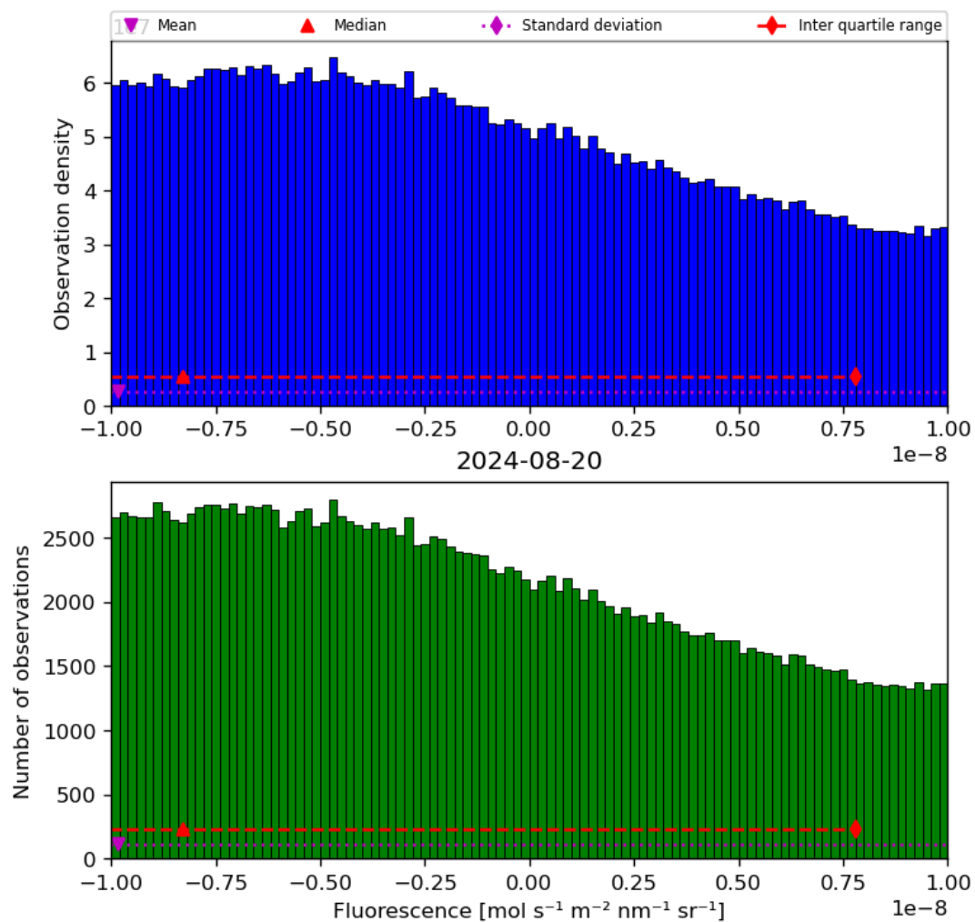
Figure 32: Histogram of “Fluorescence” for 2024-08-19 to 2024-08-21
