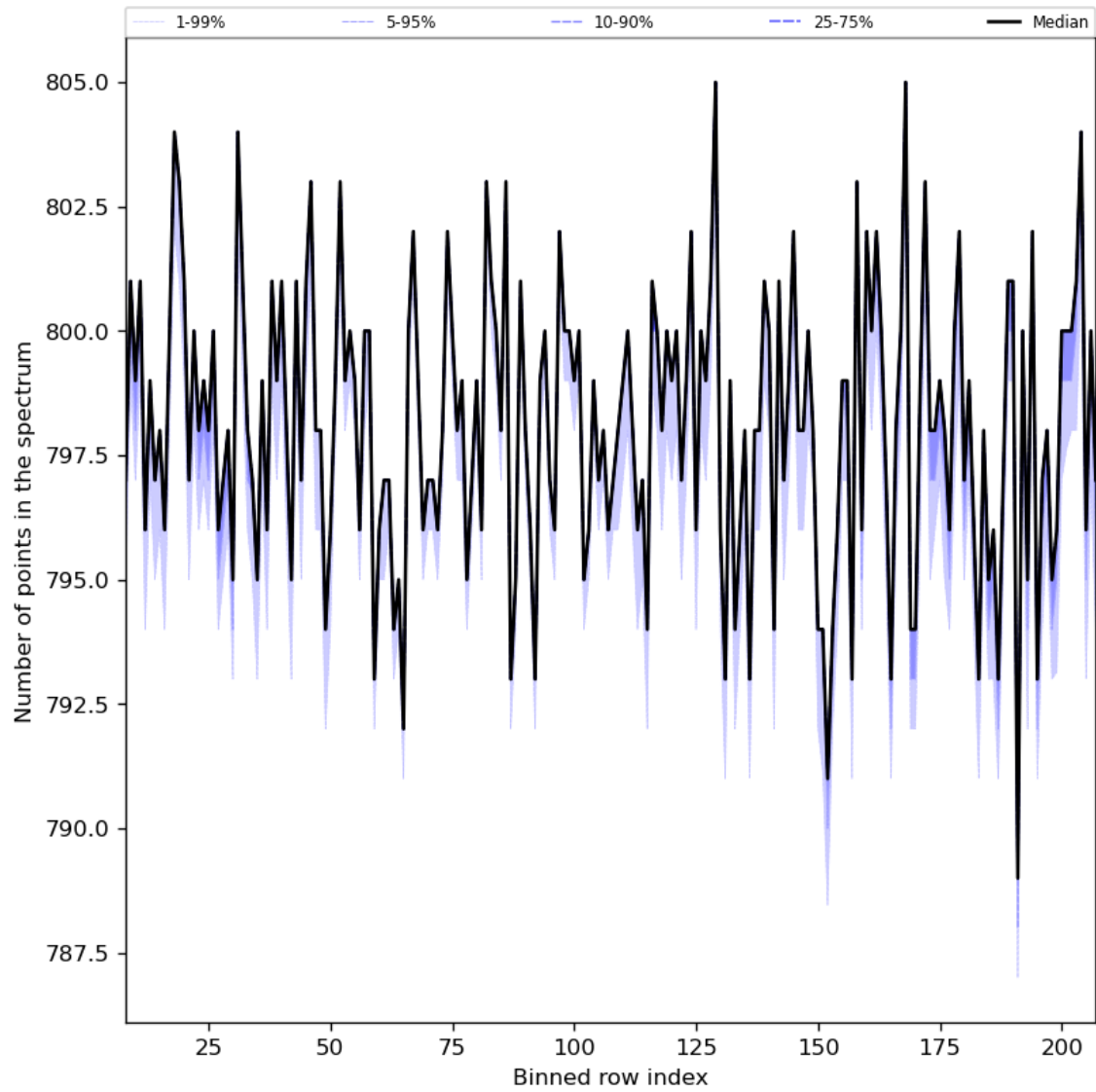
Figure 37: Along track statistics of “Number of points in the spectrum” for 2024-08-19 to 2024-08-21
