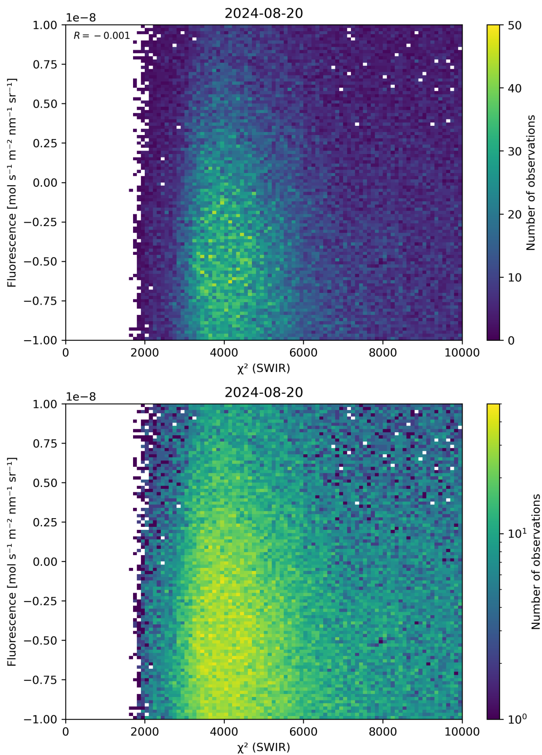
Figure 49: Scatter density plot of “ \chi^2 (SWIR)” against “Fluorescence” for 2024-08-19 to 2024-08-21.
