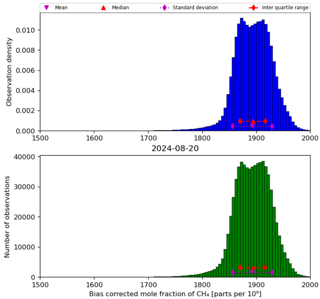
Figure 25: Histogram of “Bias corrected mole fraction of CH 4 ” for 2024-08-19 to 2024-08-21
