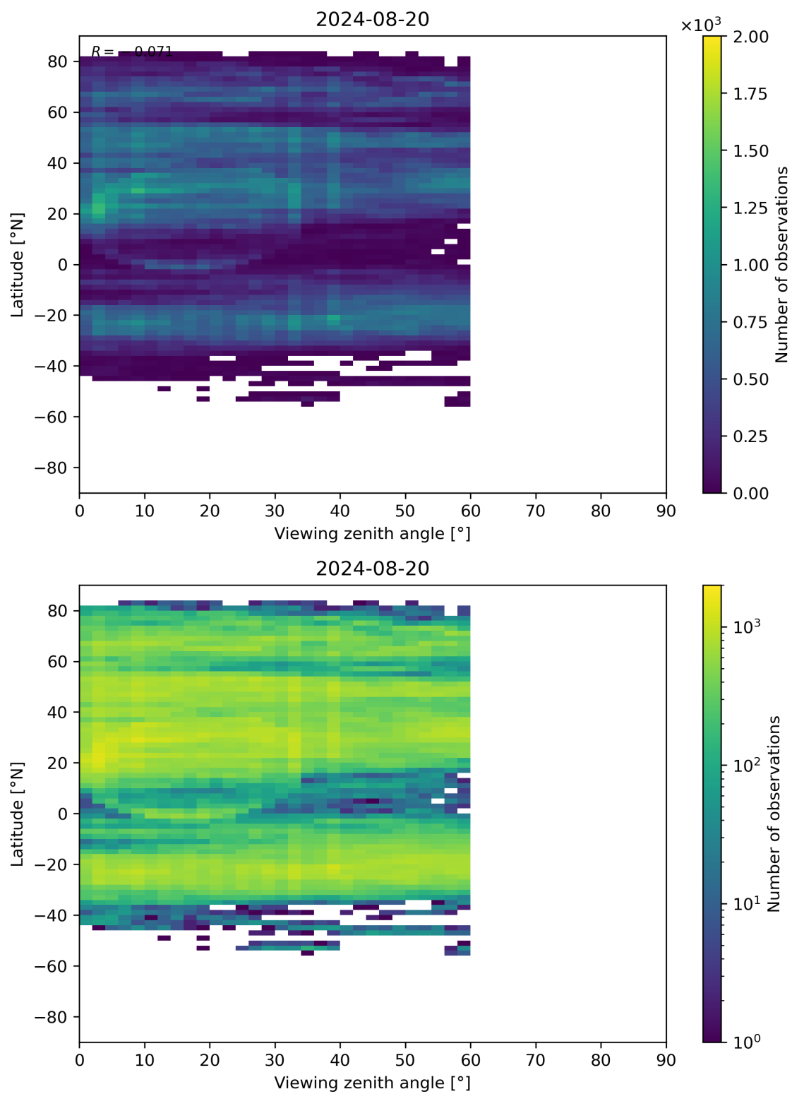
Figure 109: Scatter density plot of “Viewing zenith angle” against “Latitude” for 2024-08-19 to 2024-08-21.
