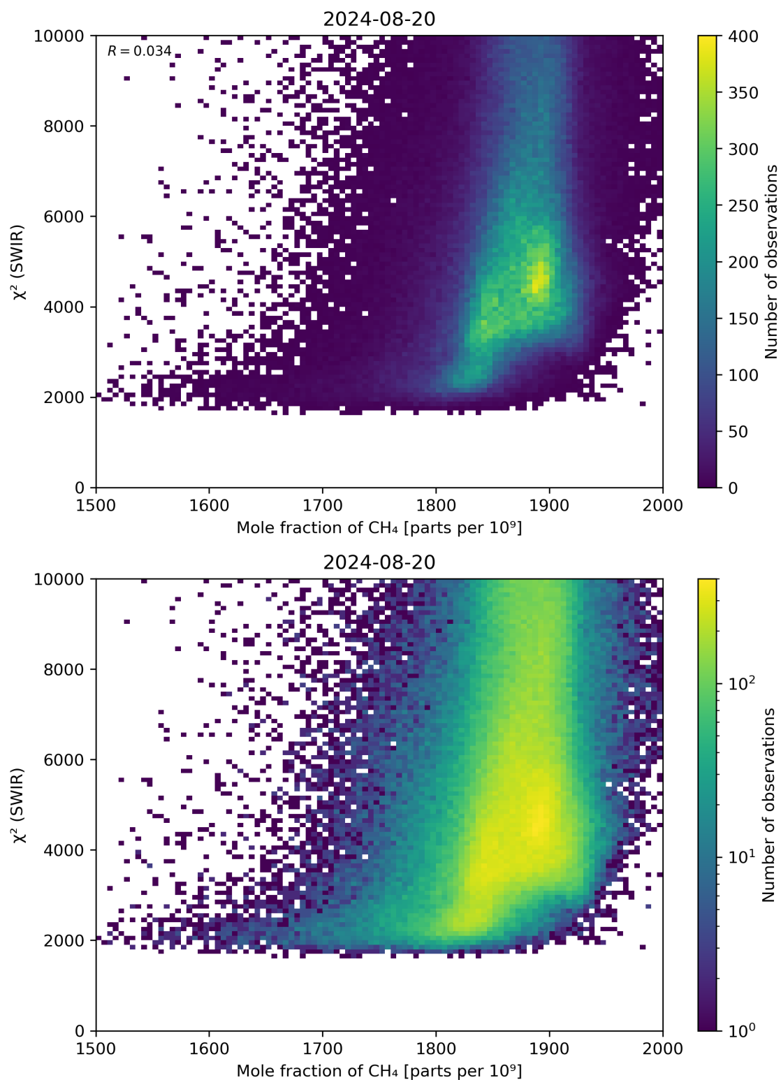
Figure 71: Scatter density plot of “Mole fraction of \text{CH}_4 ” against “ \chi^2 (SWIR)” for 2024-08-19 to 2024-08-21.
