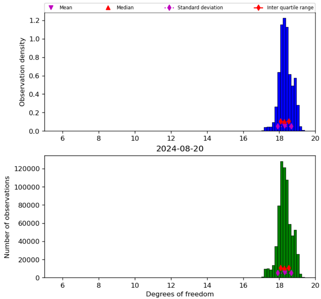
Figure 30: Histogram of “Degrees of freedom” for 2024-08-19 to 2024-08-21
