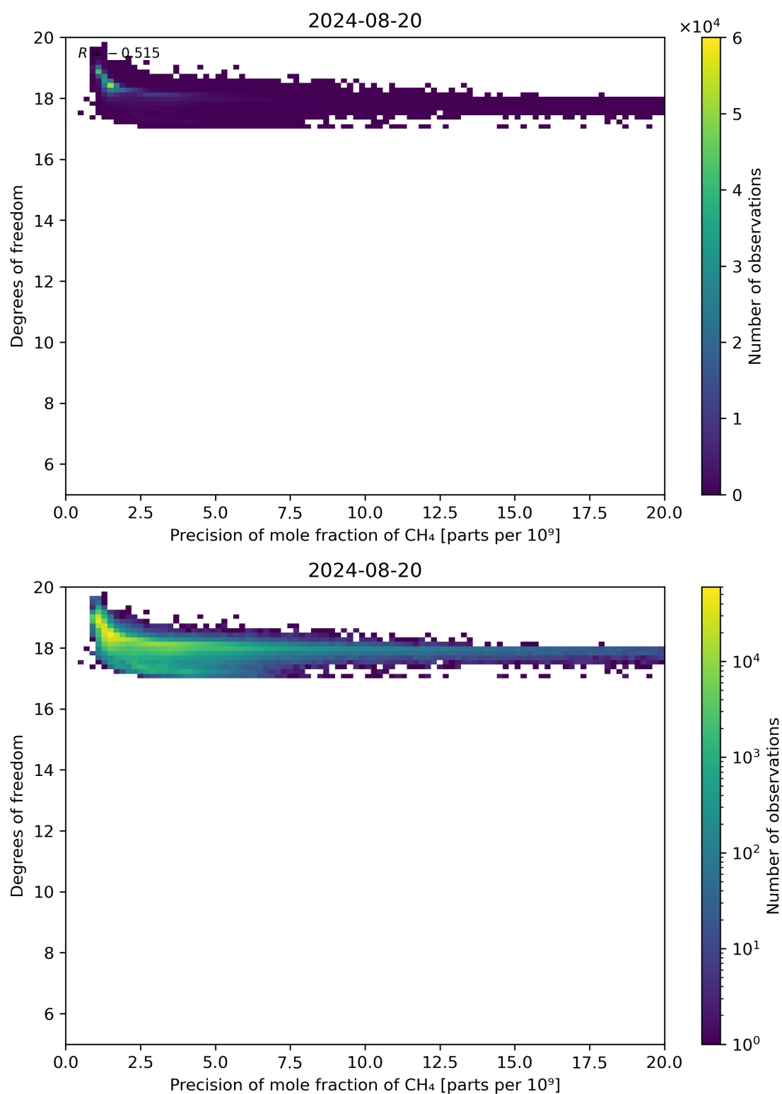
Figure 80: Scatter density plot of “Precision of mole fraction of CH 4 ” against “Degrees of freedom” for 2024-08-19 to 2024-08-21.
