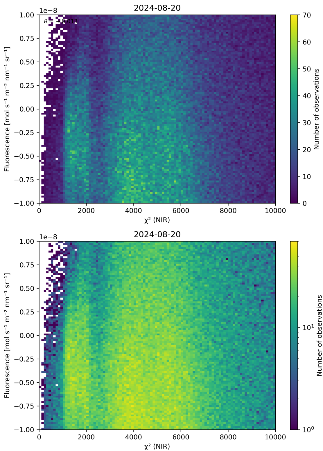
Figure 45: Scatter density plot of “ \chi^2 (NIR)” against “Fluorescence” for 2024-08-19 to 2024-08-21.
