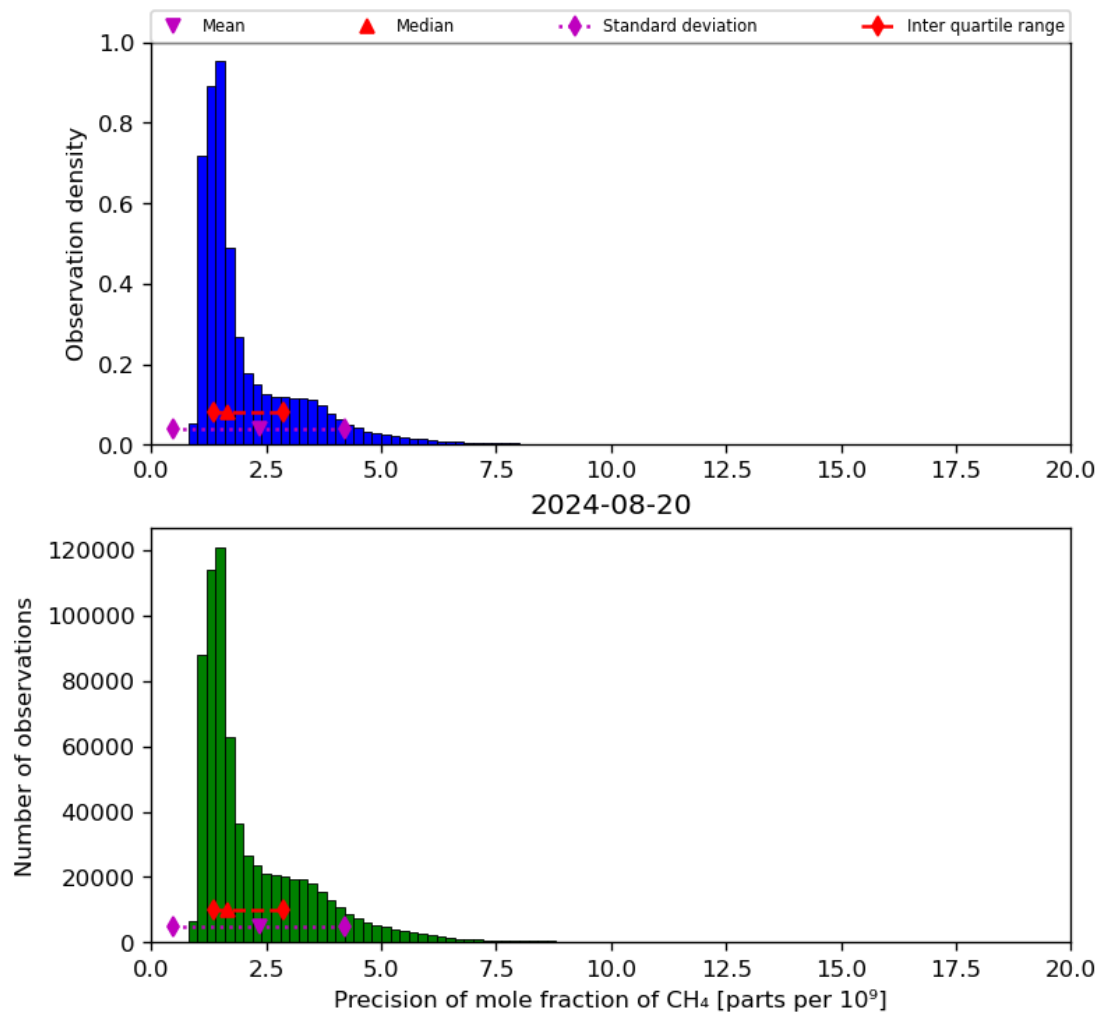
Figure 24: Histogram of “Precision of mole fraction of CH 4 ” for 2024-08-19 to 2024-08-21
