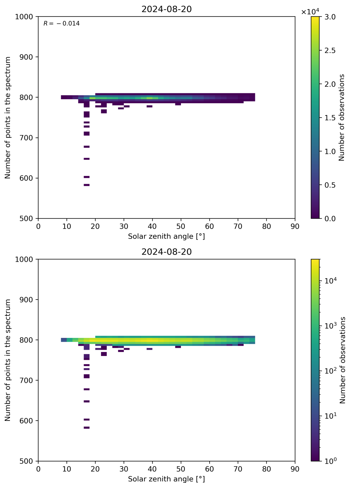
Figure 103: Scatter density plot of “Solar zenith angle” against “Number of points in the spectrum” for 2024-08-19 to 2024-08-21.
