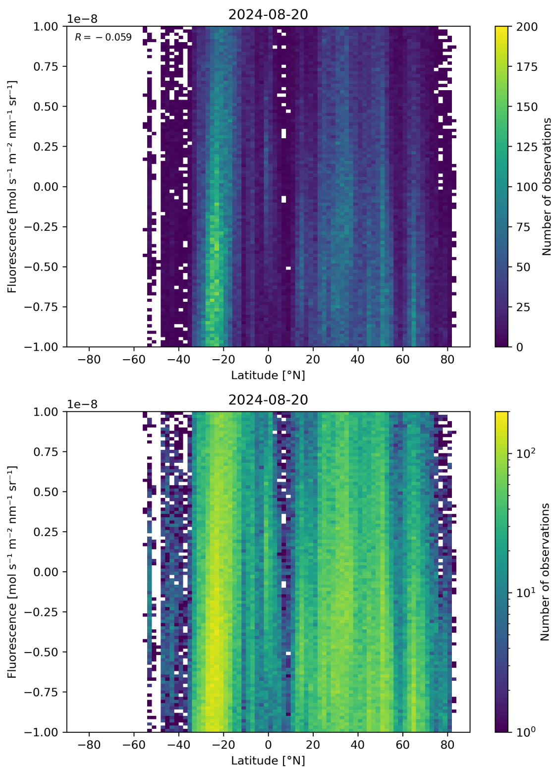
Figure 56: Scatter density plot of “Latitude” against “Fluorescence” for 2024-08-19 to 2024-08-21.
