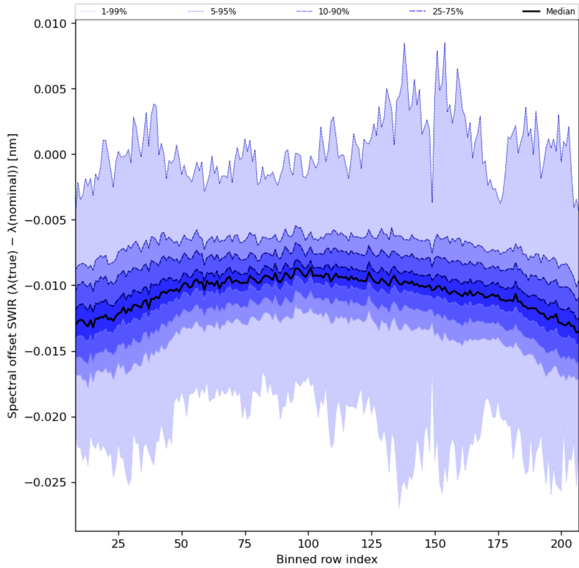
Figure 38: Along track statistics of “Spectral offset SWIR ( \lambda(\text{true}) - \lambda(\text{nominal}) )” for 2024-08-19 to 2024-08-21
