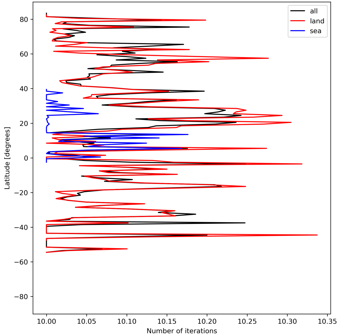
Figure 20: Zonal average of “Number of iterations” for 2024-08-19 to 2024-08-21.
