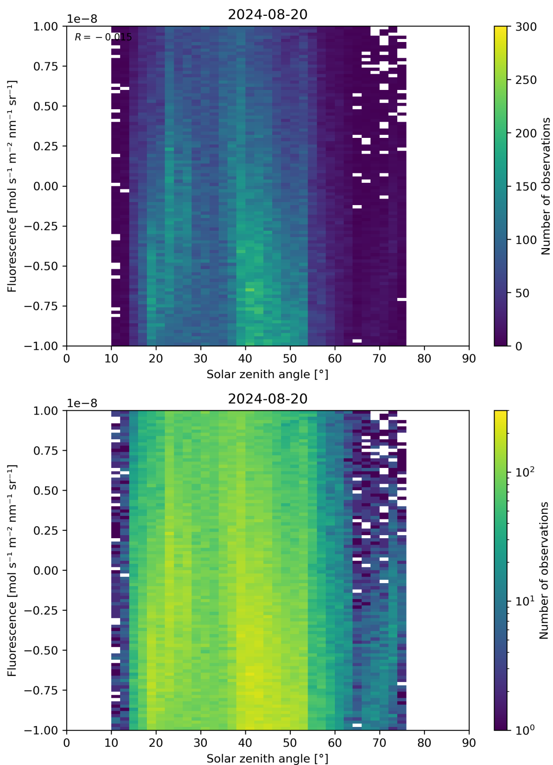
Figure 97: Scatter density plot of “Solar zenith angle” against “Fluorescence” for 2024-08-19 to 2024-08-21.
