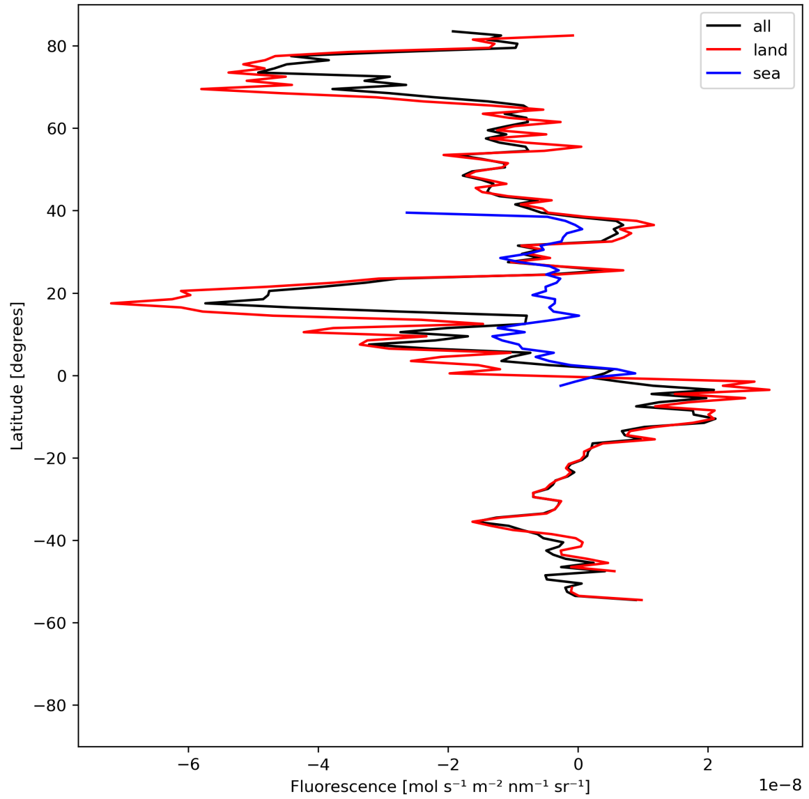
Figure 21: Zonal average of “Fluorescence” for 2024-08-19 to 2024-08-21.
