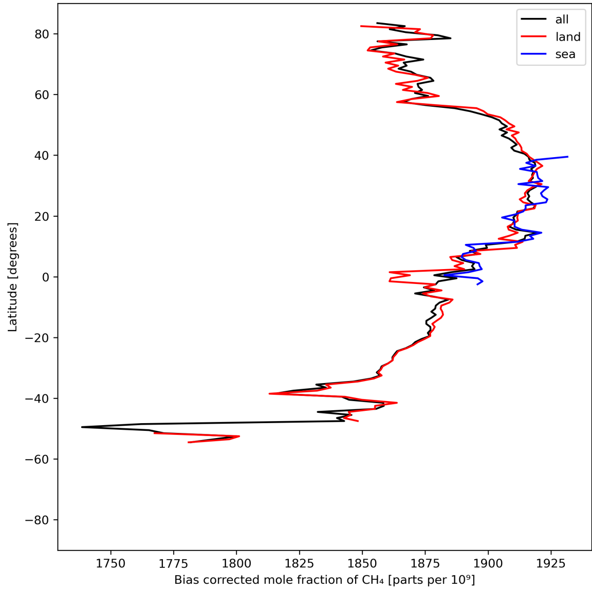
Figure 14: Zonal average of “Bias corrected mole fraction of \text{CH}_4 ” for 2024-08-19 to 2024-08-21.
