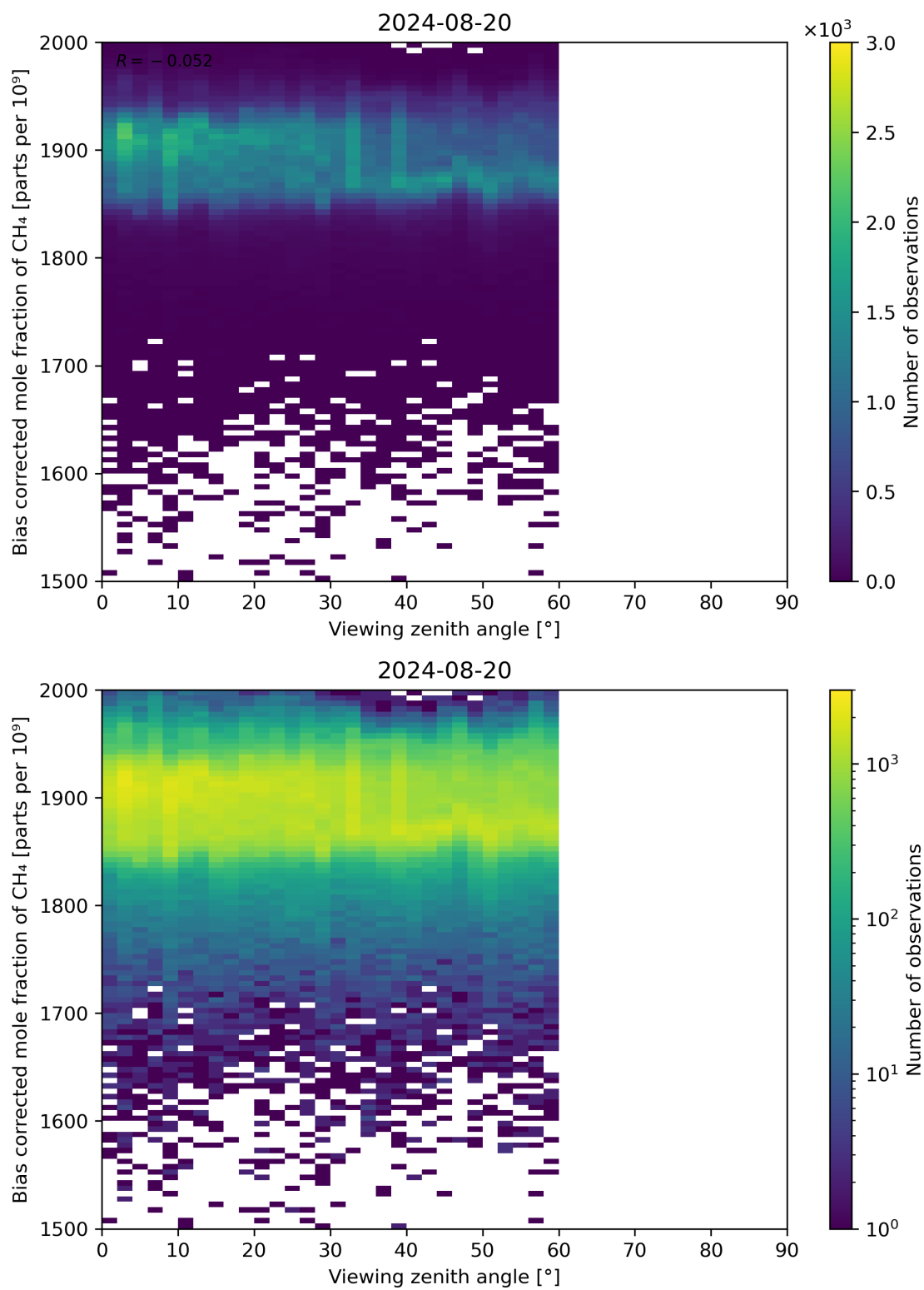
Figure 111: Scatter density plot of “Viewing zenith angle” against “Bias corrected mole fraction of CH 4 ” for 2024-08-19 to 2024-08-21.
