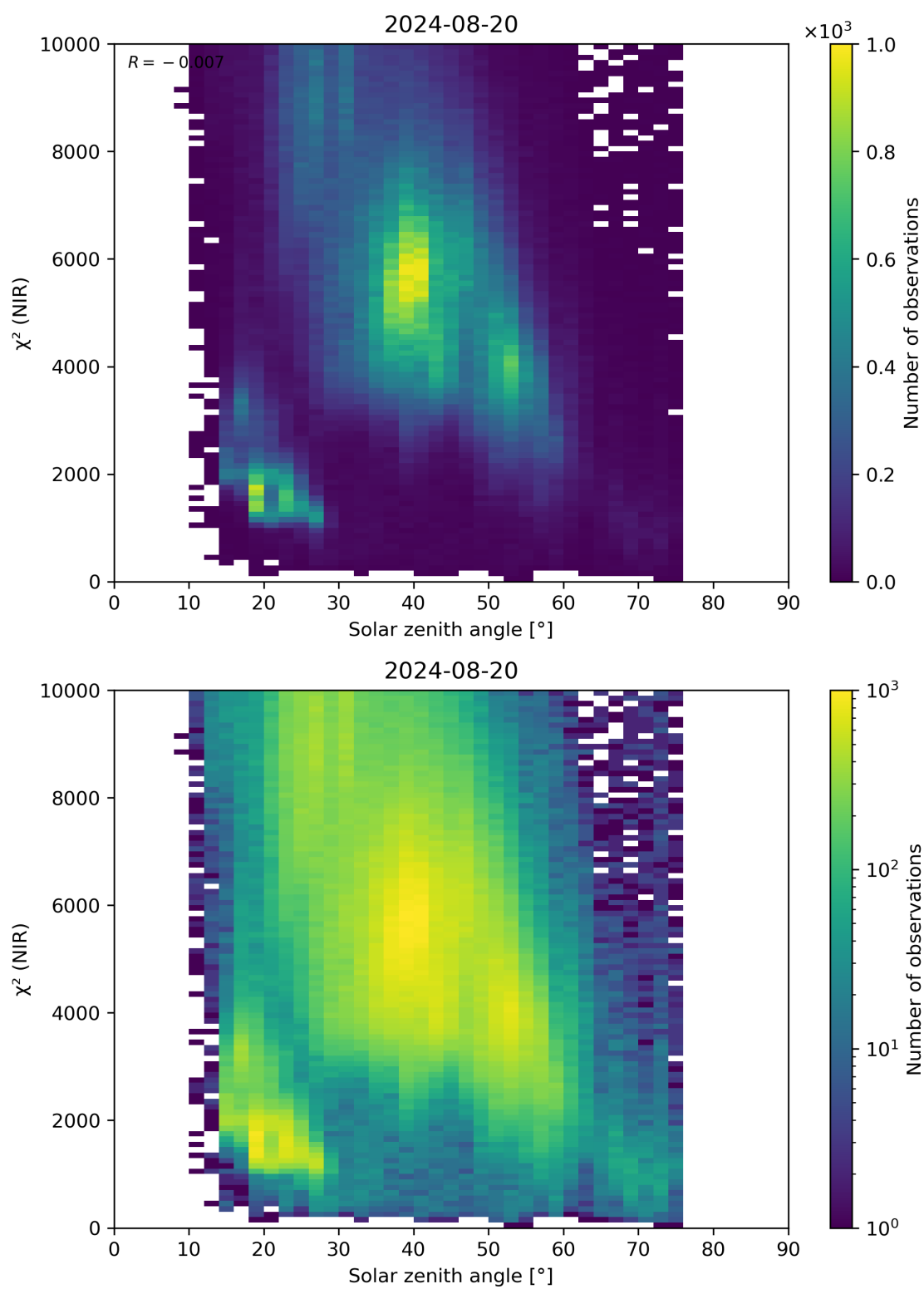
Figure 94: Scatter density plot of “Solar zenith angle” against “ \chi^2 (NIR)” for 2024-08-19 to 2024-08-21.
