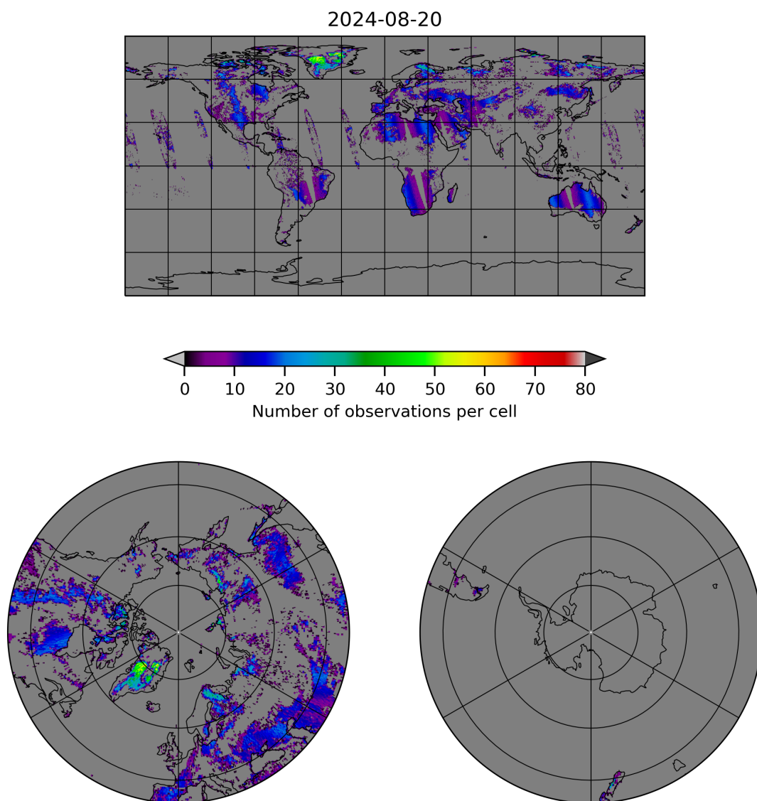
Figure 10: Map of the number of observations for 2024-08-19 to 2024-08-21
