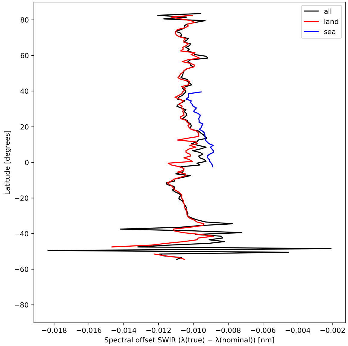
Figure 16: Zonal average of “Spectral offset SWIR ( \lambda(\text{true}) - \lambda(\text{nominal}) )” for 2024-08-19 to 2024-08-21.
