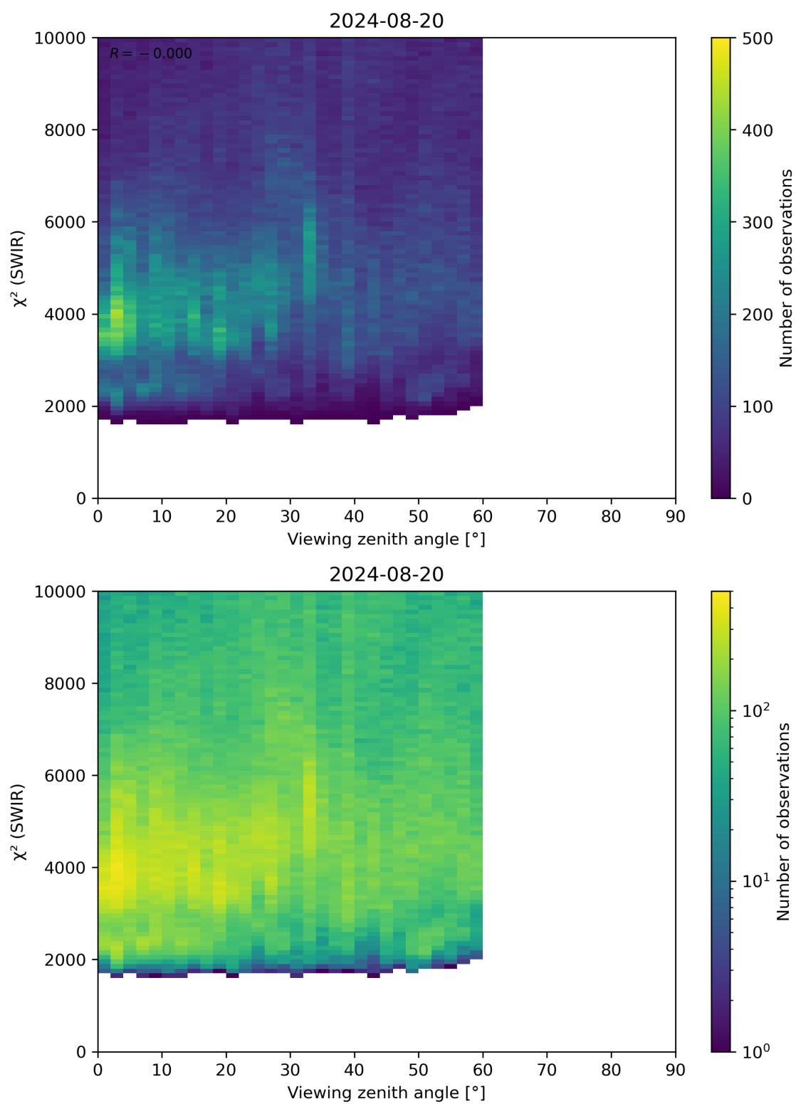
Figure 106: Scatter density plot of “Viewing zenith angle” against “ \chi^2 (SWIR)” for 2024-08-19 to 2024-08-21.
