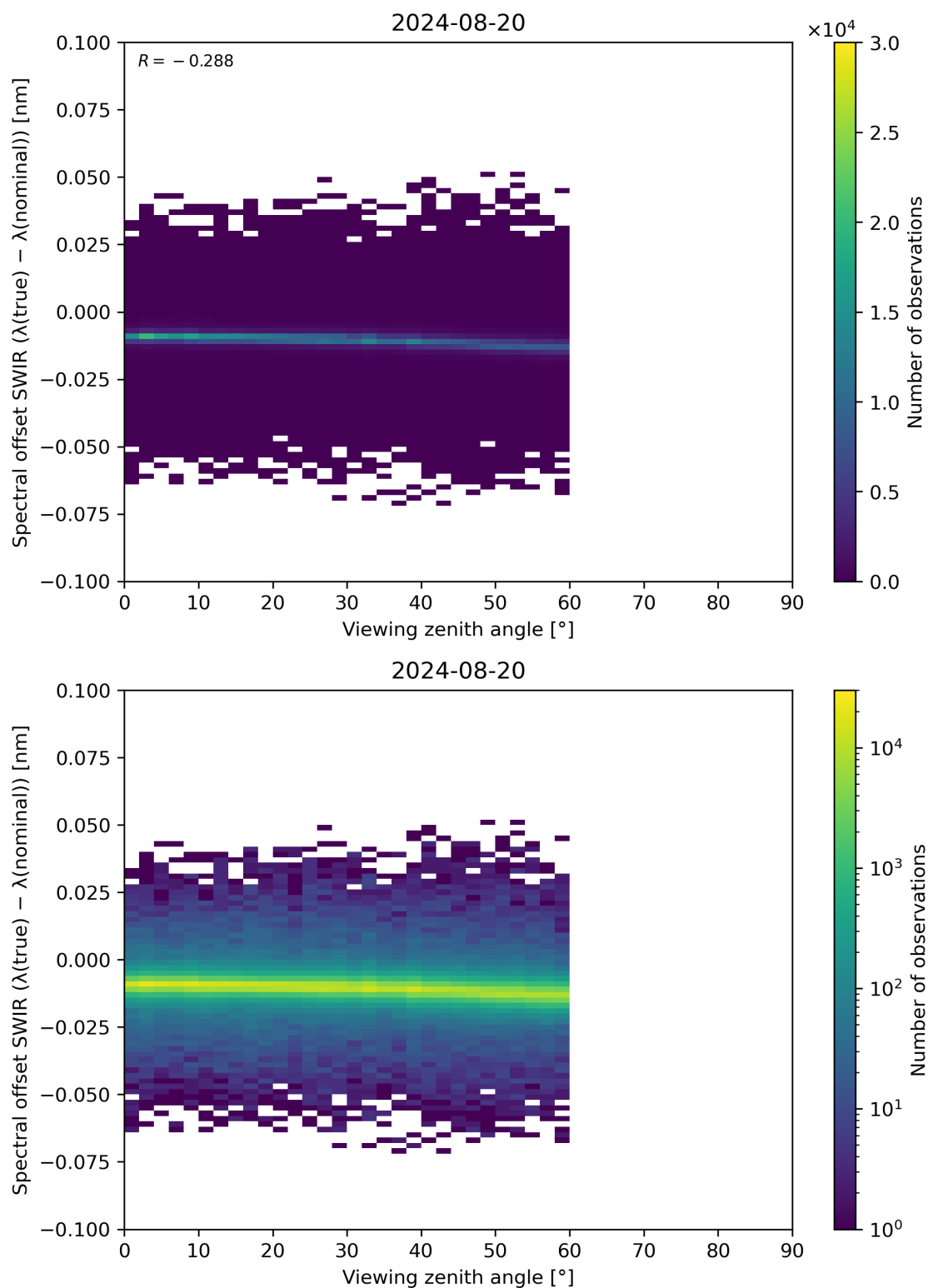
Figure 116: Scatter density plot of “Viewing zenith angle” against “Spectral offset SWIR ( \lambda(\text{true}) - \lambda(\text{nominal}) )” for 2024-08-19 to 2024-08-21.
