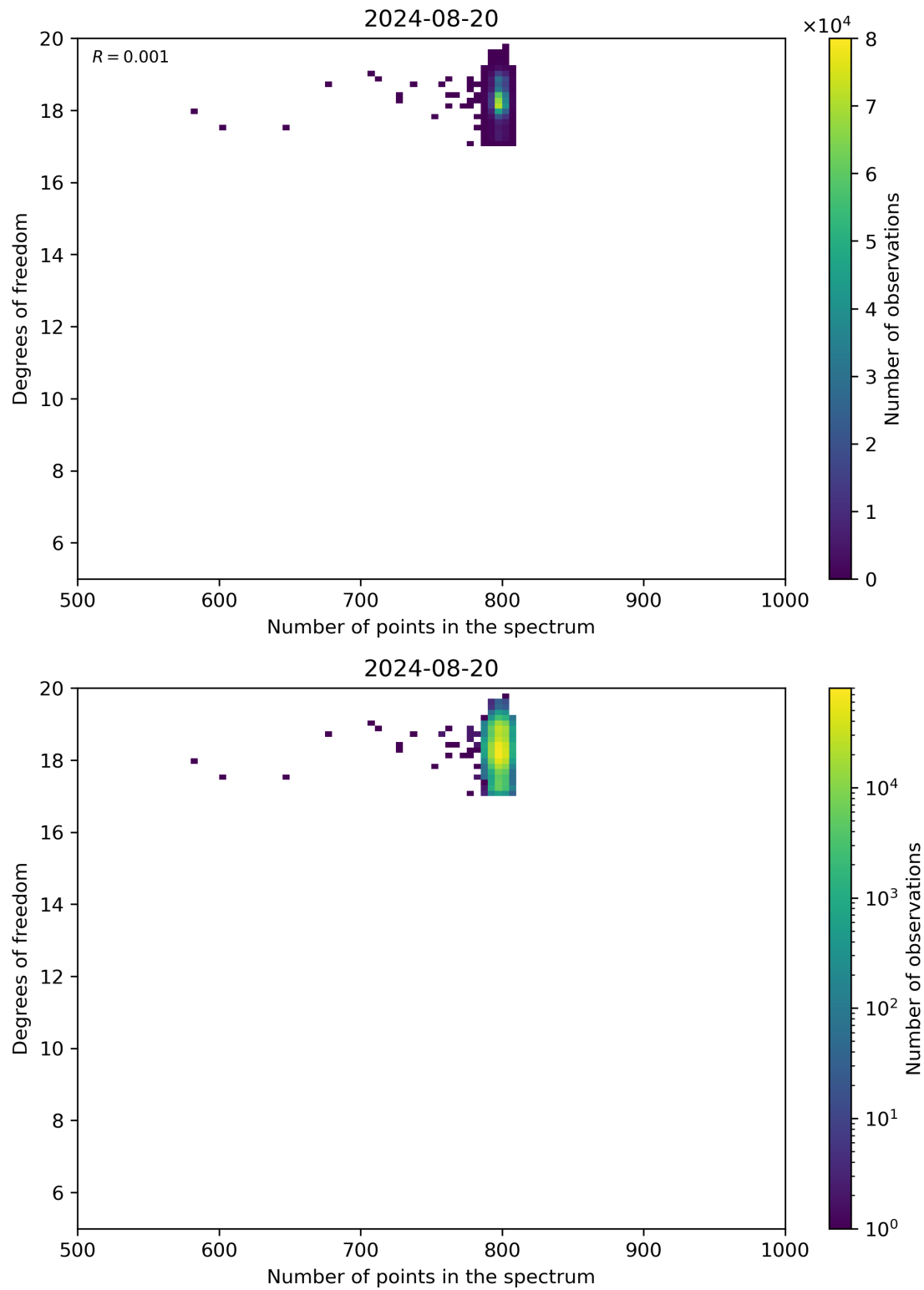
Figure 90: Scatter density plot of “Number of points in the spectrum” against “Degrees of freedom” for 2024-08-19 to 2024-08-21.
