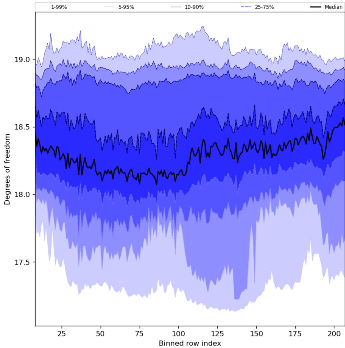
Figure 41: Along track statistics of “Degrees of freedom” for 2024-08-19 to 2024-08-21
