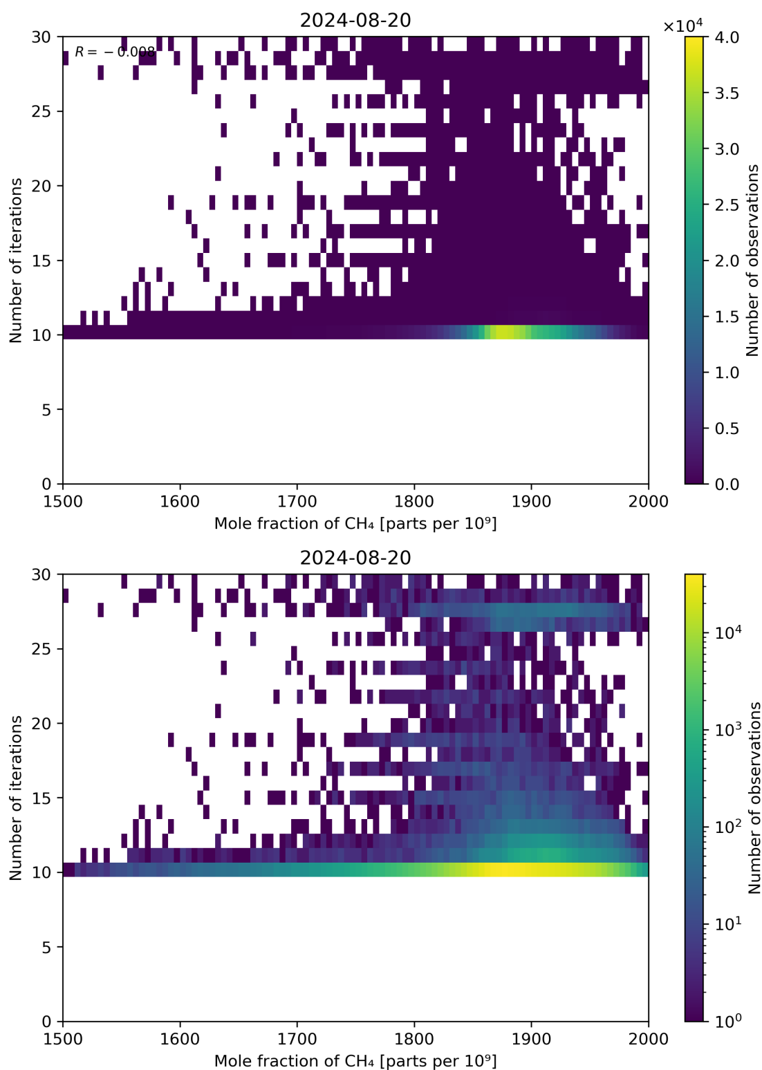
Figure 76: Scatter density plot of “Mole fraction of CH 4 ” against “Number of iterations” for 2024-08-19 to 2024-08-21.
