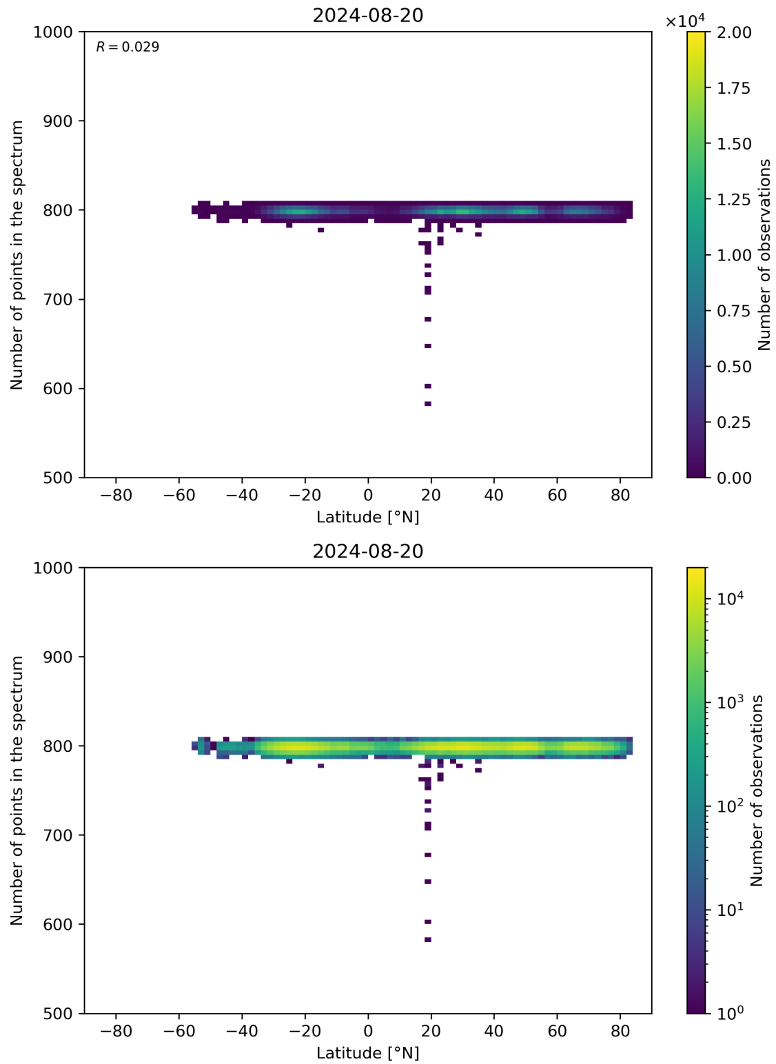
Figure 61: Scatter density plot of “Latitude” against “Number of points in the spectrum” for 2024-08-19 to 2024-08-21.
