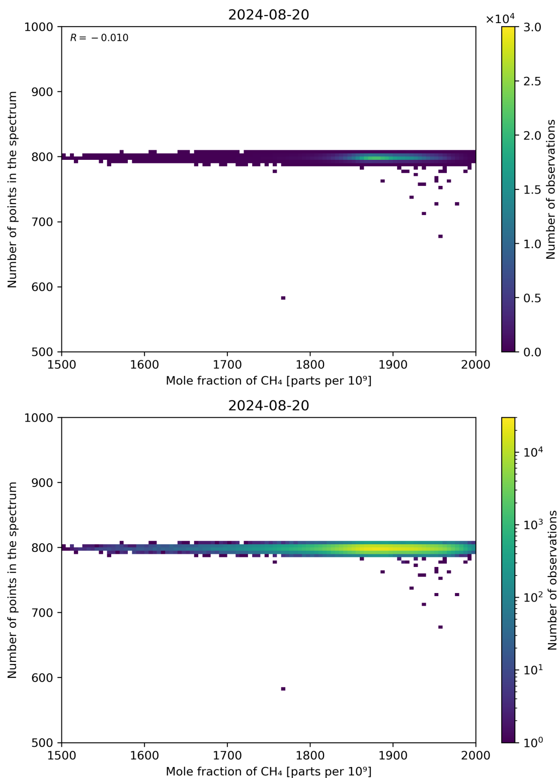
Figure 77: Scatter density plot of “Mole fraction of CH 4 ” against “Number of points in the spectrum” for 2024-08-19 to 2024-08-21.
