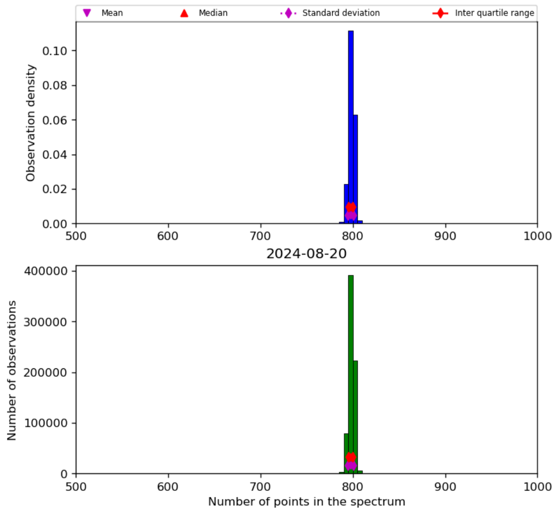
Figure 26: Histogram of “Number of points in the spectrum” for 2024-08-19 to 2024-08-21
