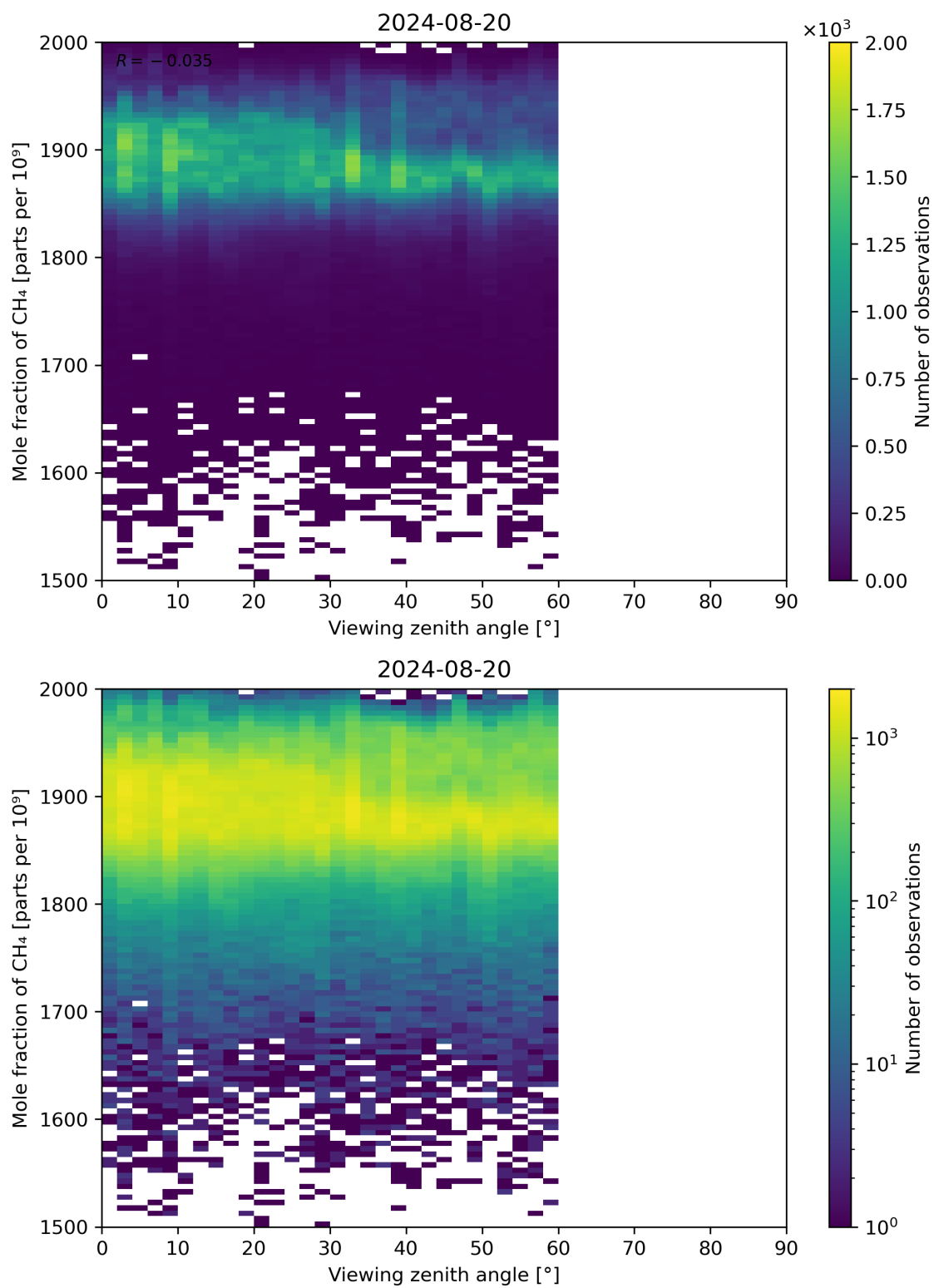
Figure 110: Scatter density plot of “Viewing zenith angle” against “Mole fraction of CH 4 ” for 2024-08-19 to 2024-08-21.
