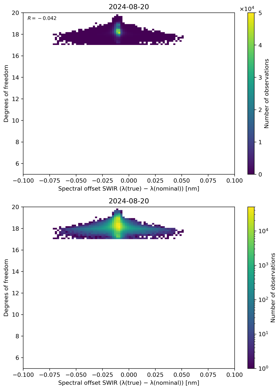
Figure 119: Scatter density plot of “Spectral offset SWIR ( \lambda(\text{true}) - \lambda(\text{nominal}) )” against “Degrees of freedom” for 2024-08-19 to 2024-08-21.
