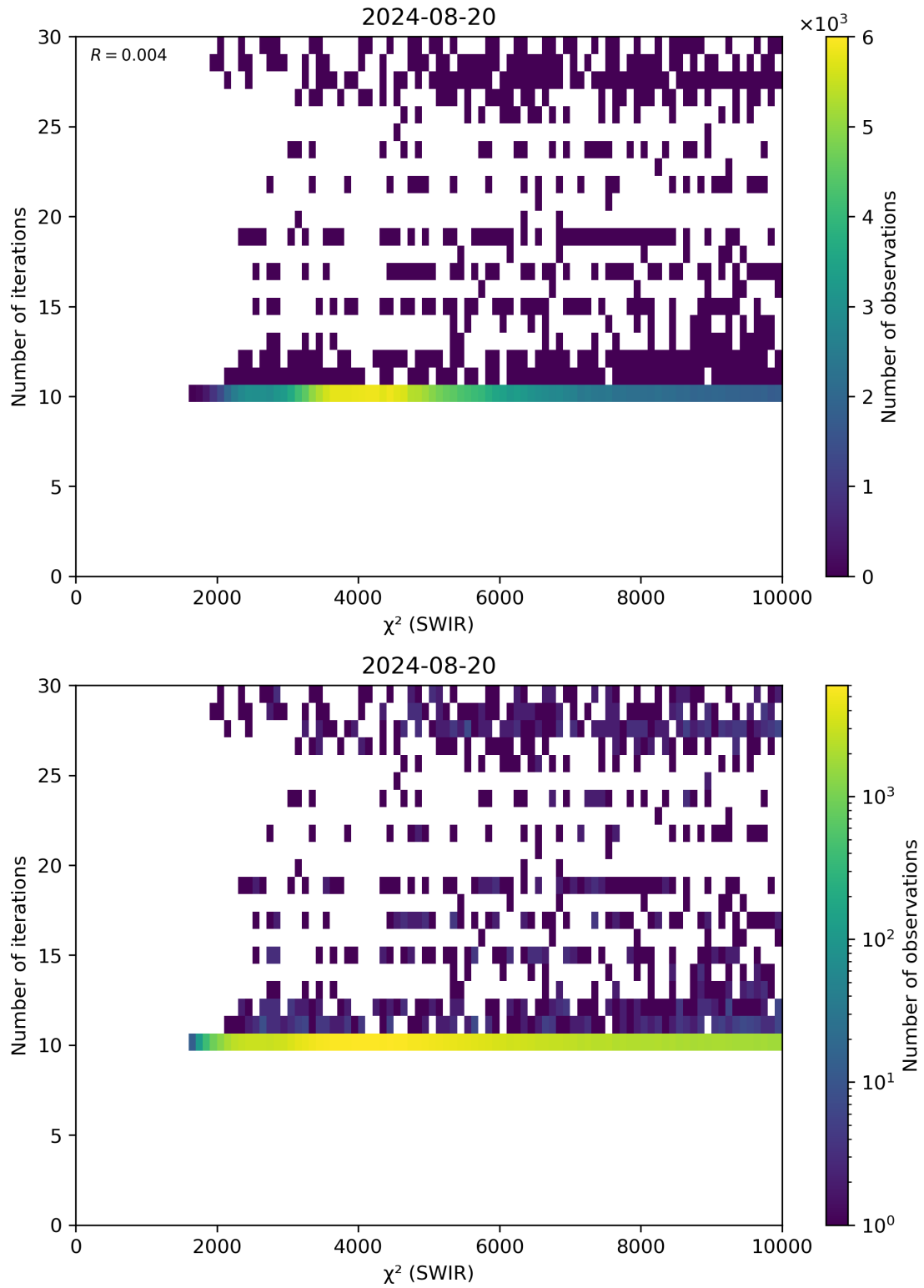
Figure 50: Scatter density plot of “ \chi^2 (SWIR)” against “Number of iterations” for 2024-08-19 to 2024-08-21.
