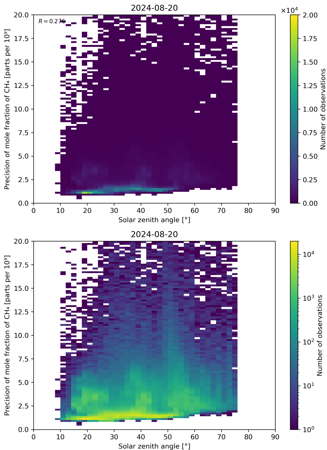
Figure 101: Scatter density plot of “Solar zenith angle” against “Precision of mole fraction of \text{CH}_4 ” for 2024-08-19 to 2024-08-21.
