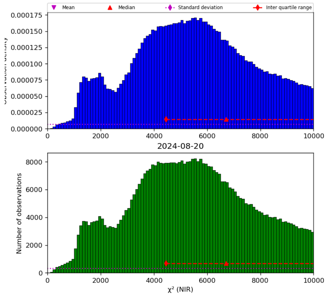
Figure 29: Histogram of “ \chi^2 (NIR)” for 2024-08-19 to 2024-08-21
