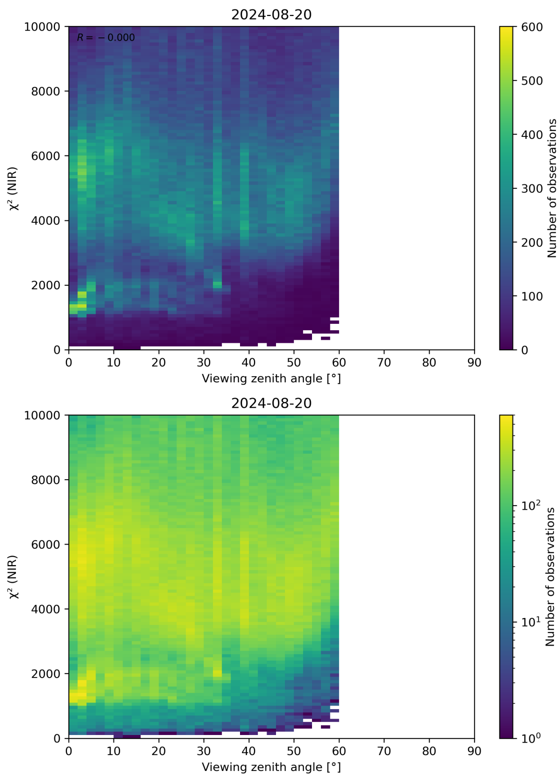
Figure 105: Scatter density plot of “Viewing zenith angle” against “ \chi^2 (NIR)” for 2024-08-19 to 2024-08-21.
