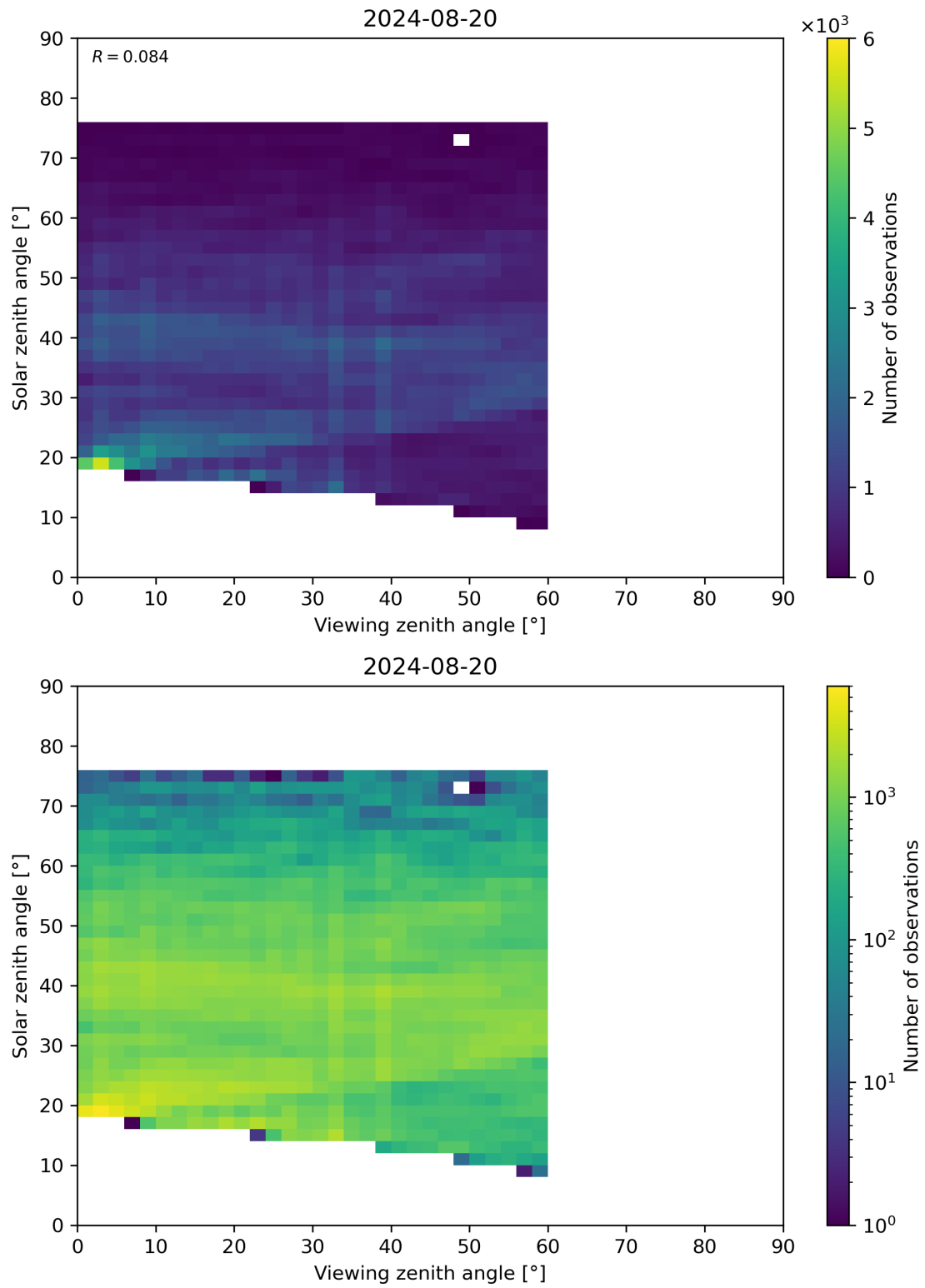
Figure 115: Scatter density plot of “Viewing zenith angle” against “Solar zenith angle” for 2024-08-19 to 2024-08-21.
