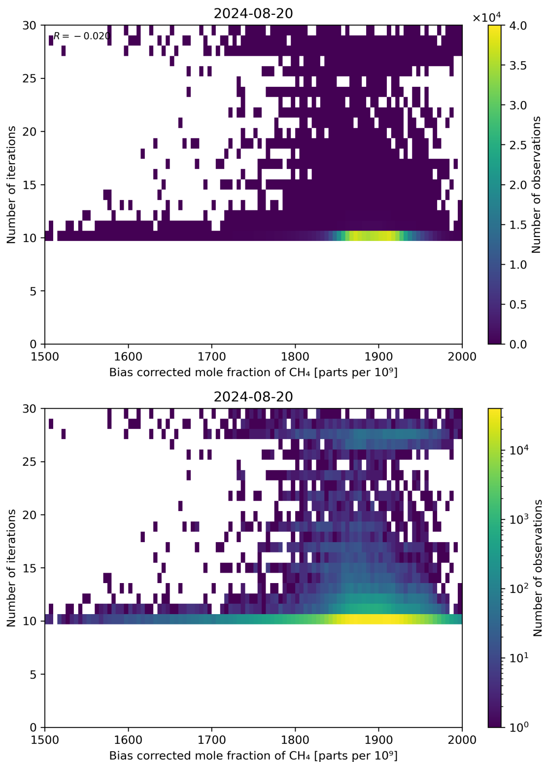
Figure 67: Scatter density plot of “Bias corrected mole fraction of CH 4 ” against “Number of iterations” for 2024-08-19 to 2024-08-21.
