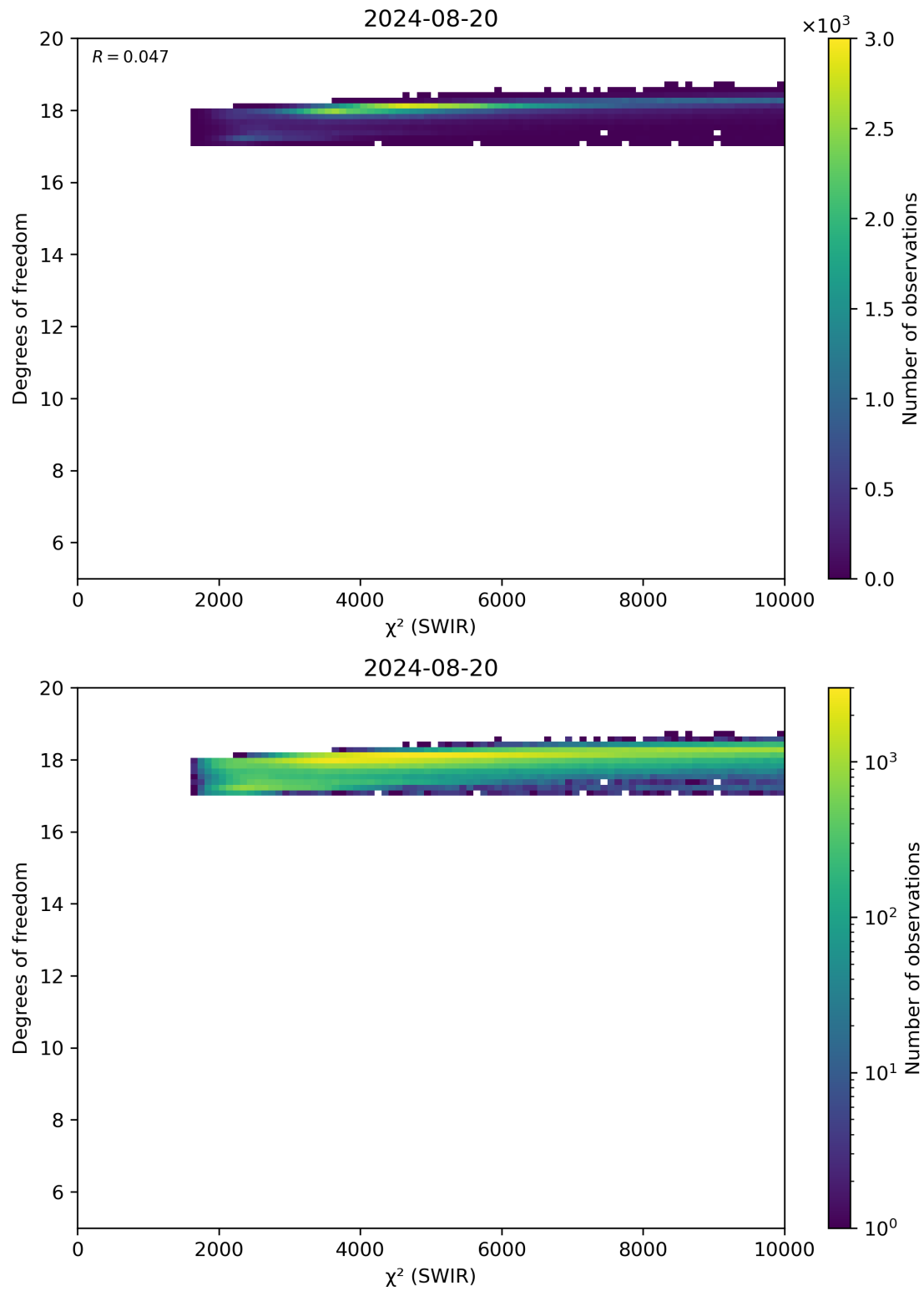
Figure 48: Scatter density plot of “ \chi^2 (SWIR)” against “Degrees of freedom” for 2024-08-19 to 2024-08-21.
