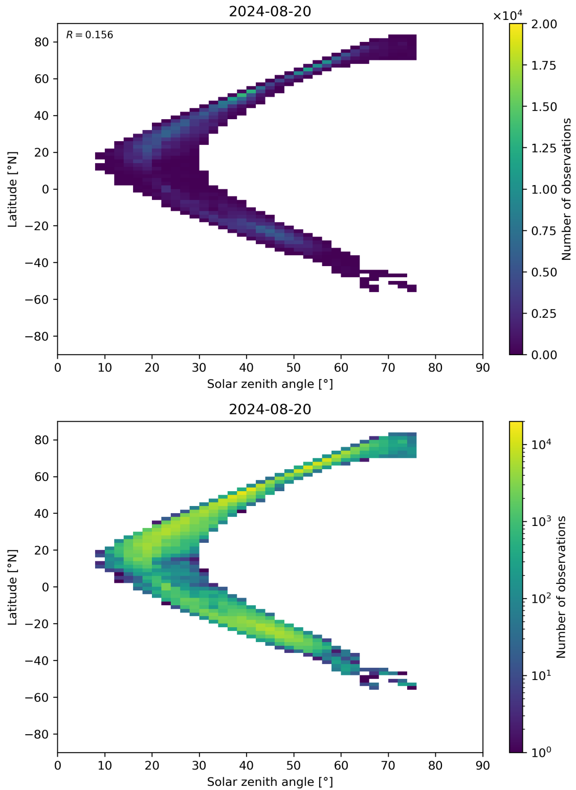
Figure 98: Scatter density plot of “Solar zenith angle” against “Latitude” for 2024-08-19 to 2024-08-21.
