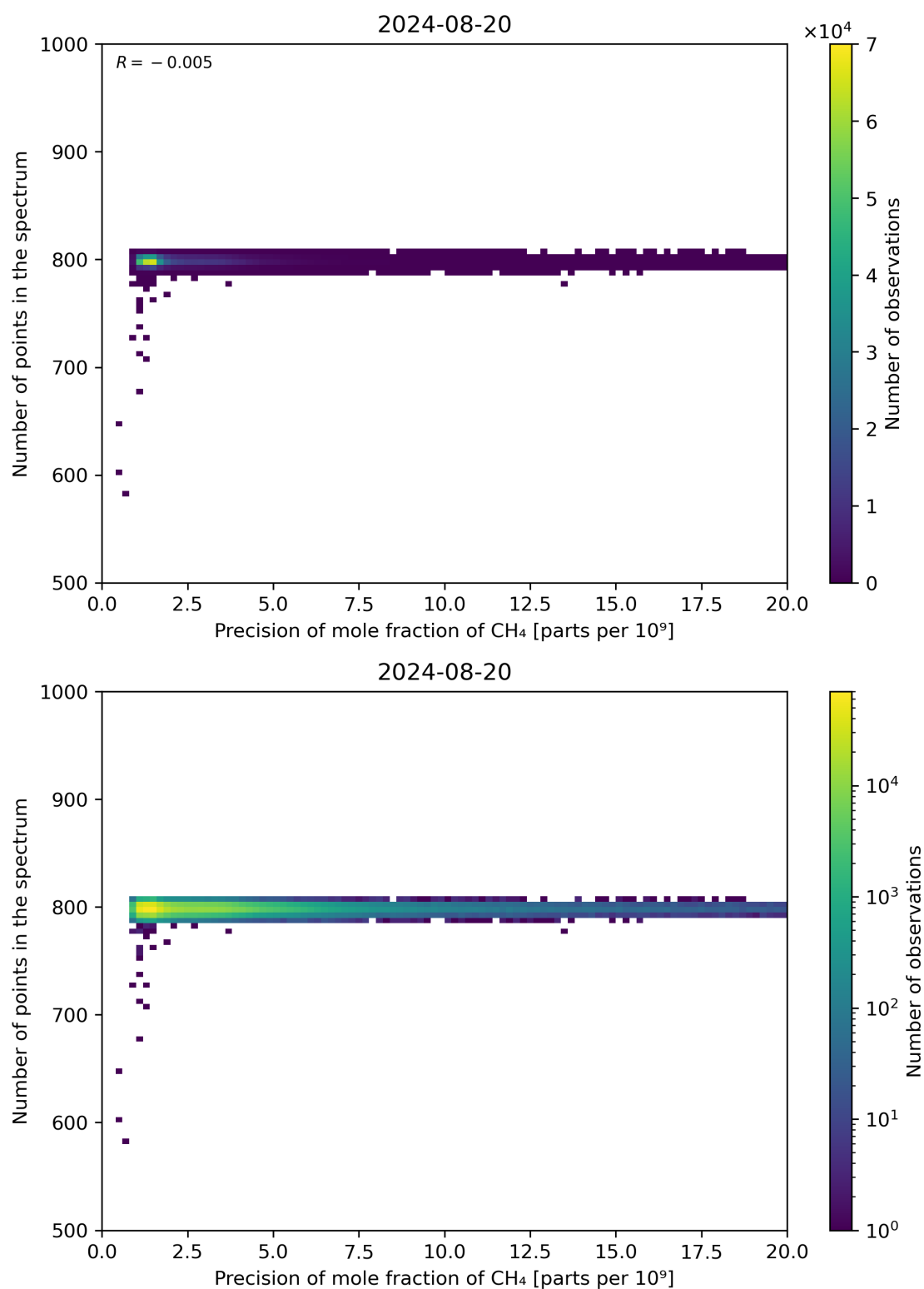
Figure 84: Scatter density plot of “Precision of mole fraction of CH 4 ” against “Number of points in the spectrum” for 2024-08-19 to 2024-08-21.
