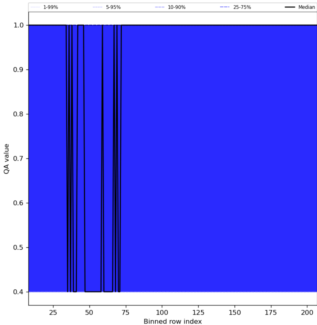
Figure 33: Along track statistics of “QA value” for 2024-08-19 to 2024-08-21
