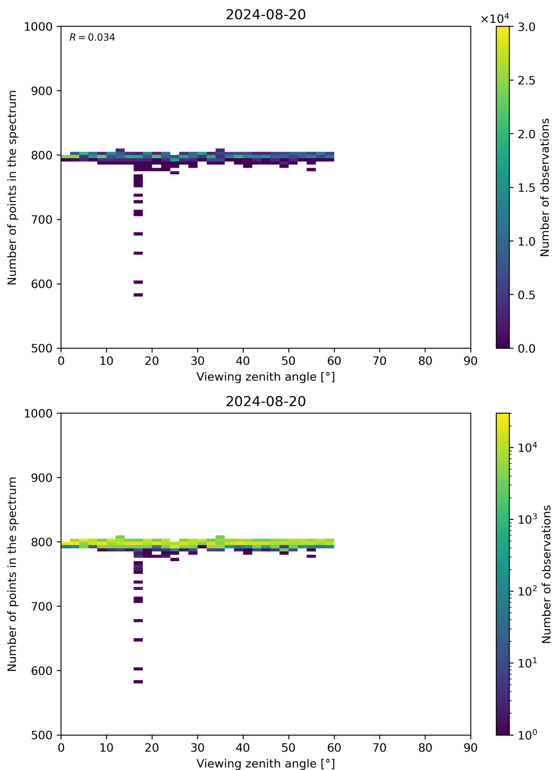
Figure 114: Scatter density plot of “Viewing zenith angle” against “Number of points in the spectrum” for 2024-08-19 to 2024-08-21.
