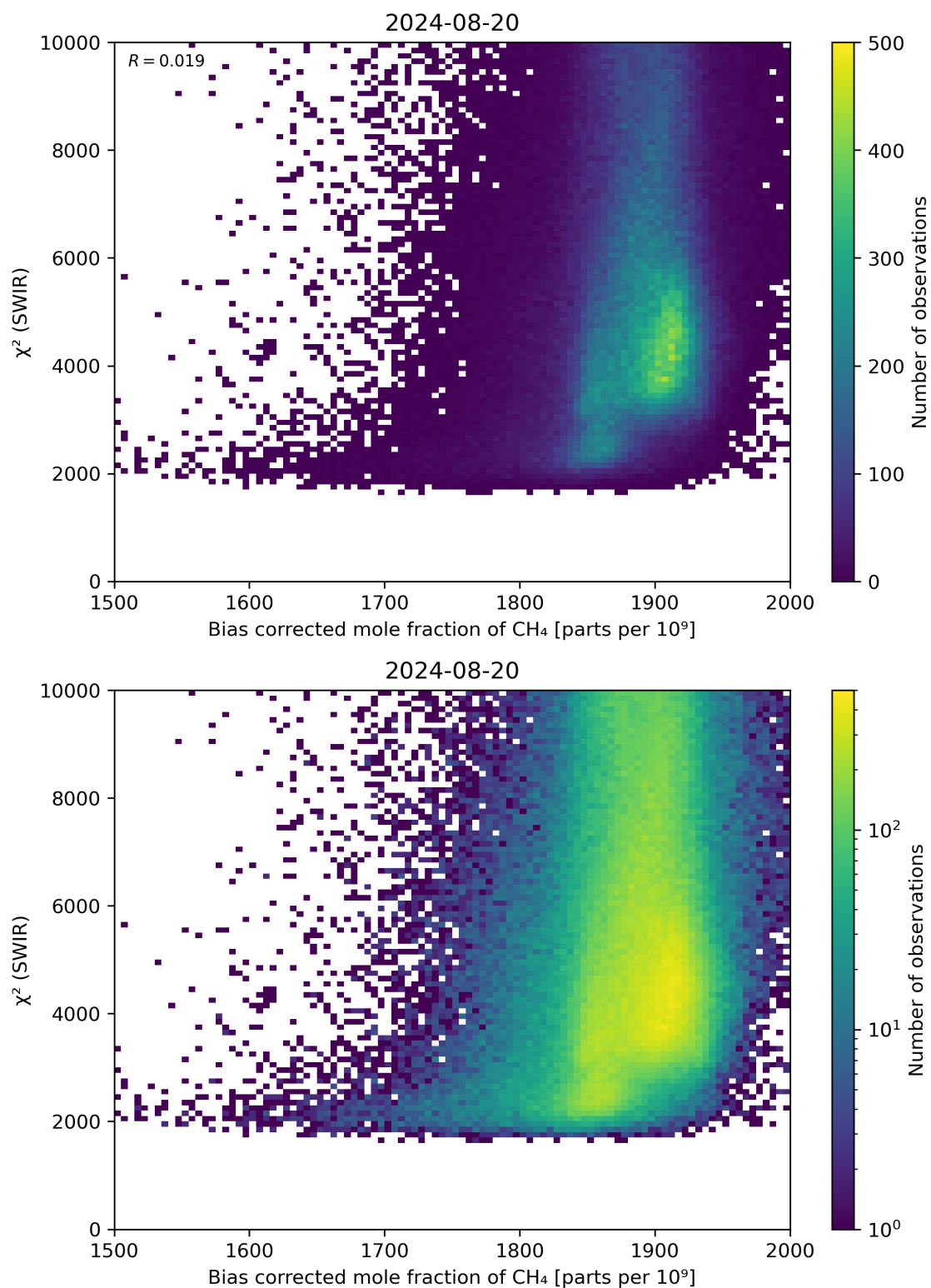
Figure 64: Scatter density plot of “Bias corrected mole fraction of CH 4 ” against “ \chi^2 (SWIR)” for 2024-08-19 to 2024-08-21.
