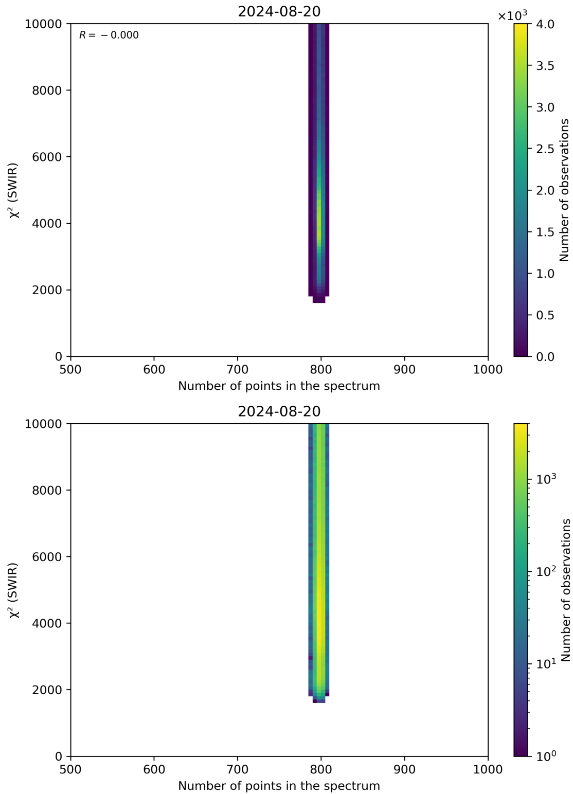
Figure 89: Scatter density plot of “Number of points in the spectrum” against “ \chi^2 (SWIR)” for 2024-08-19 to 2024-08-21.
