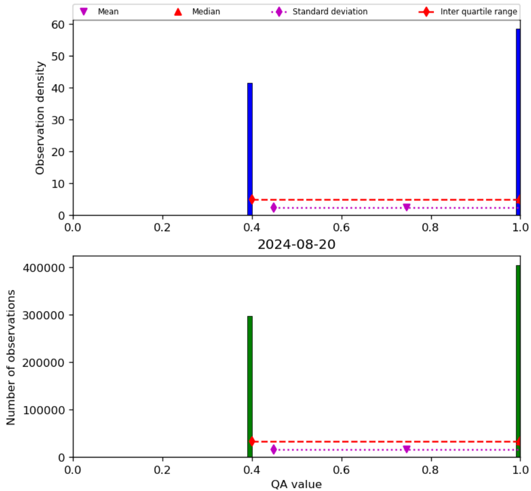
Figure 22: Histogram of “QA value” for 2024-08-19 to 2024-08-21
