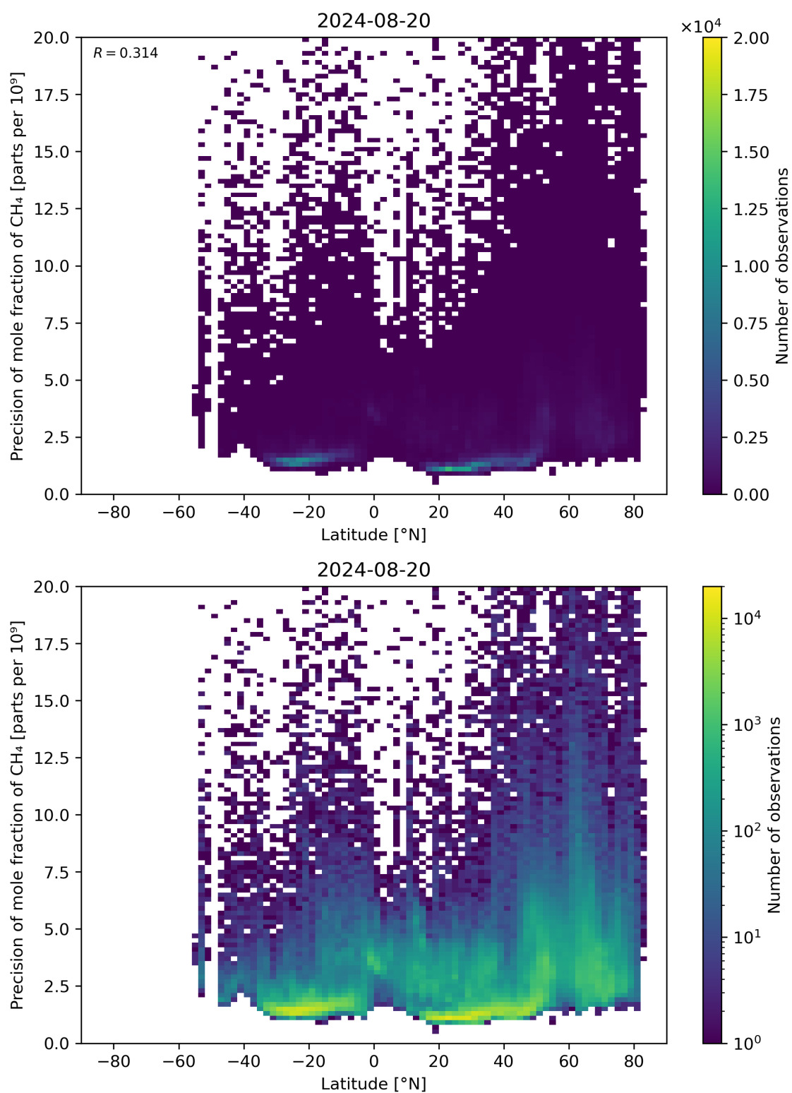
Figure 59: Scatter density plot of “Latitude” against “Precision of mole fraction of \text{CH}_4 ” for 2024-08-19 to 2024-08-21.
