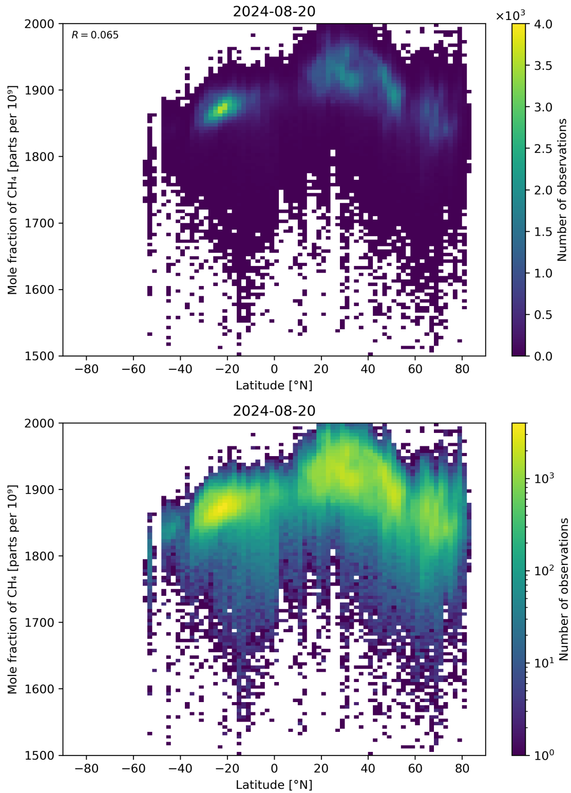
Figure 57: Scatter density plot of “Latitude” against “Mole fraction of CH 4 ” for 2024-08-19 to 2024-08-21.
