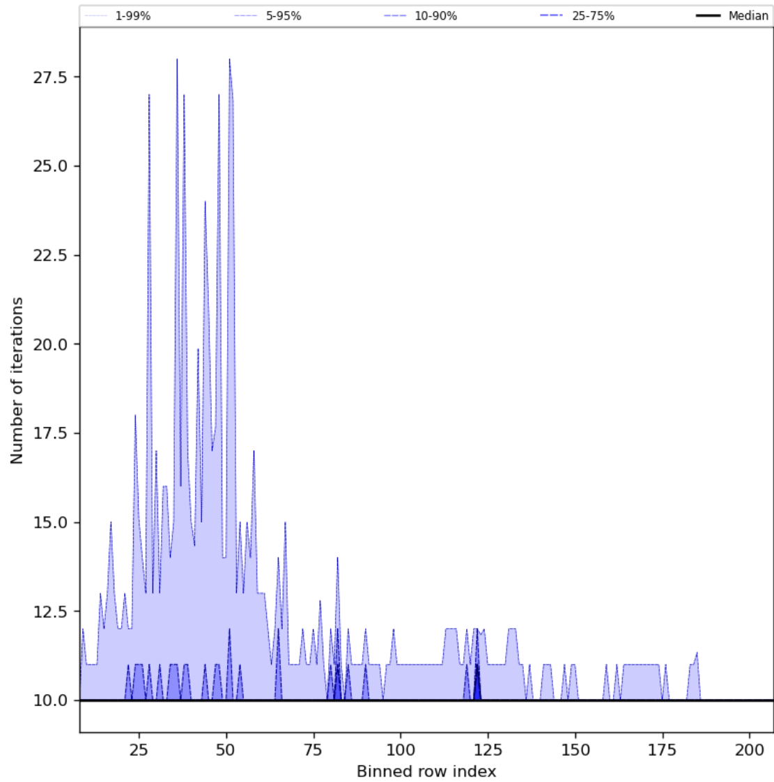
Figure 42: Along track statistics of “Number of iterations” for 2024-08-19 to 2024-08-21
