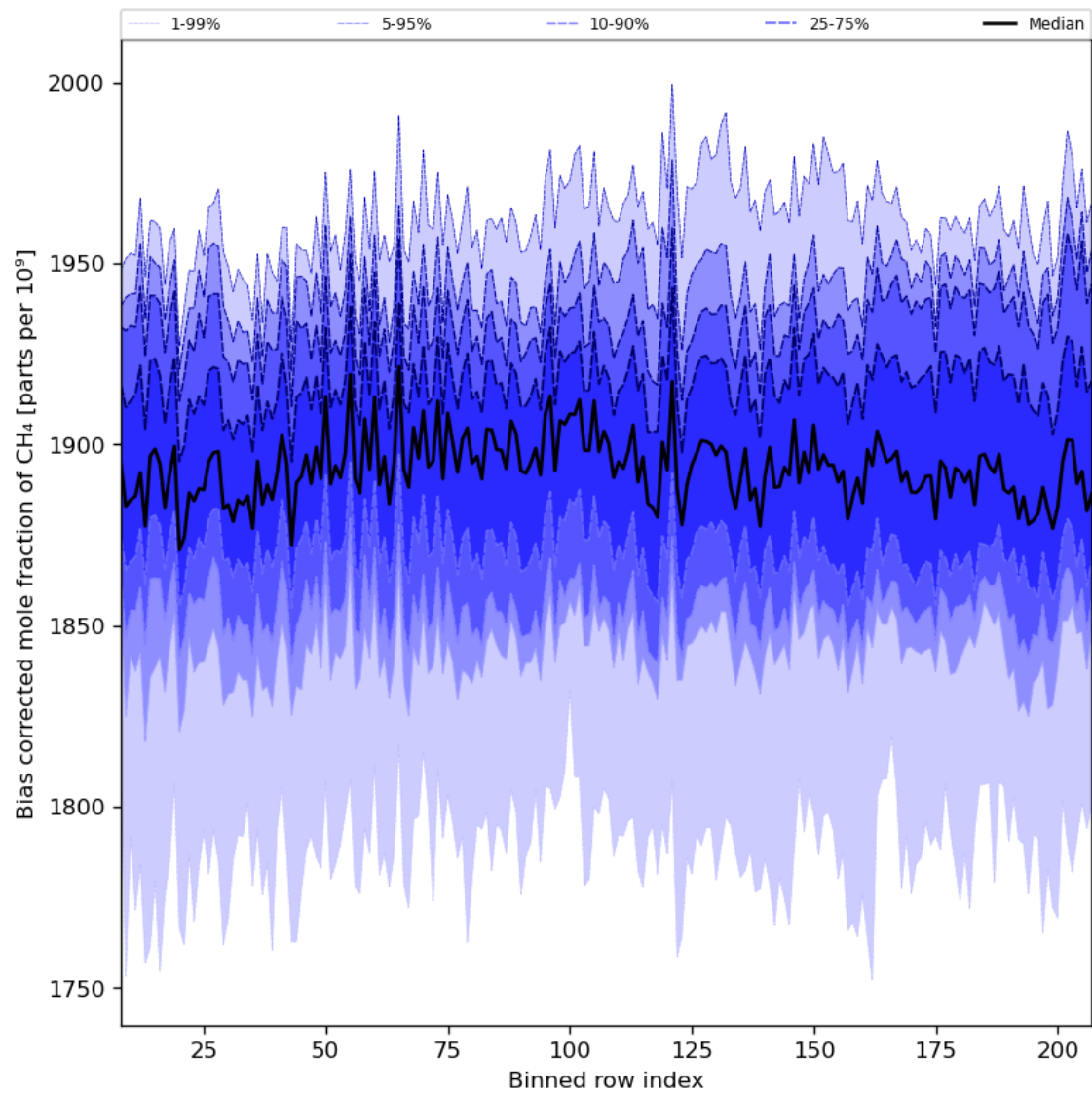
Figure 36: Along track statistics of “Bias corrected mole fraction of CH 4 ” for 2024-08-19 to 2024-08-21
