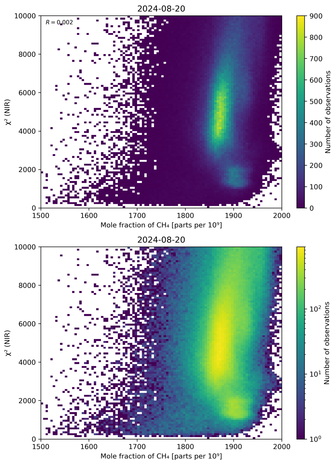
Figure 70: Scatter density plot of “Mole fraction of CH 4 ” against “ \chi^2 (NIR)” for 2024-08-19 to 2024-08-21.
