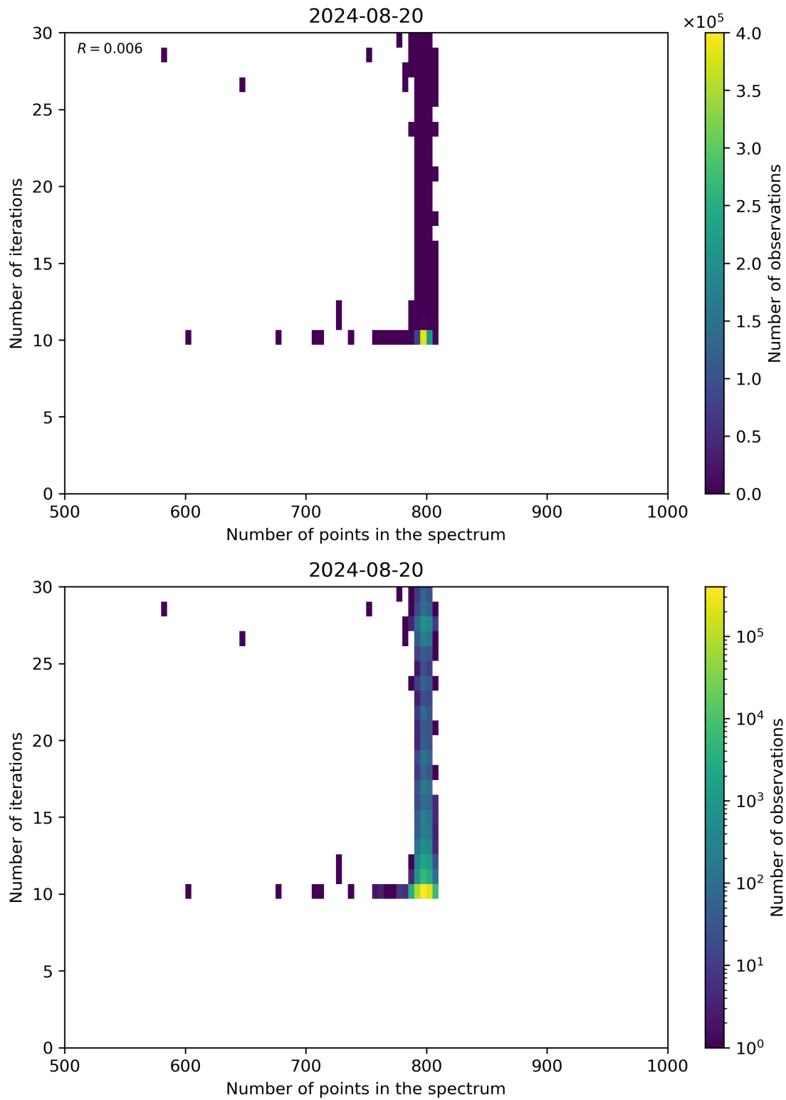
Figure 92: Scatter density plot of “Number of points in the spectrum” against “Number of iterations” for 2024-08-19 to 2024-08-21.
