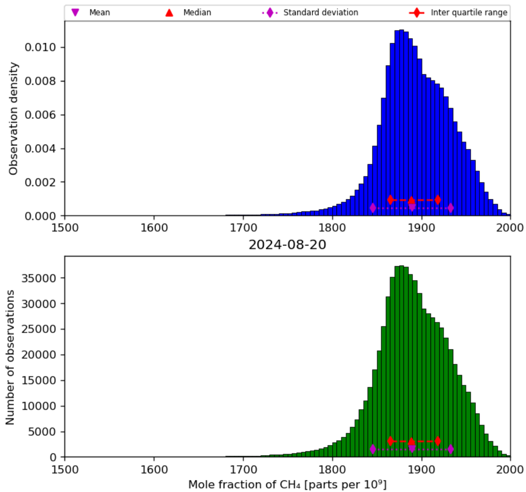
Figure 23: Histogram of “Mole fraction of CH 4 ” for 2024-08-19 to 2024-08-21
