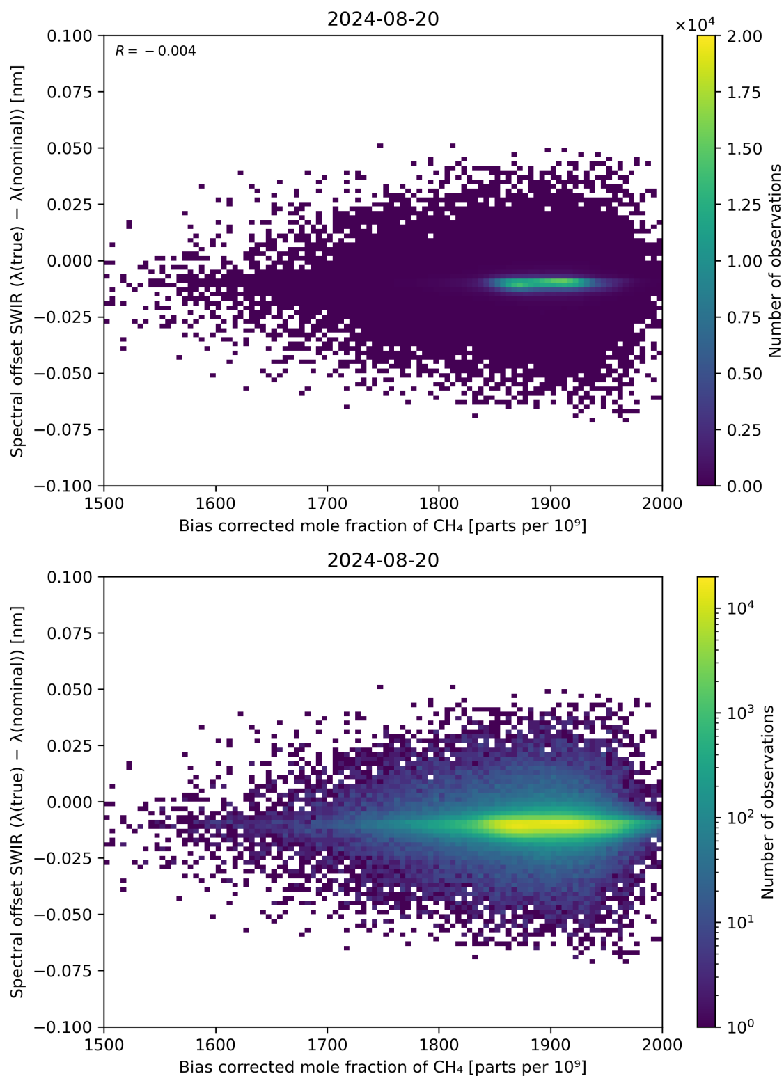
Figure 69: Scatter density plot of “Bias corrected mole fraction of \text{CH}_4 ” against “Spectral offset SWIR ( \lambda(\text{true}) - \lambda(\text{nominal}) )” for 2024-08-19 to 2024-08-21.
