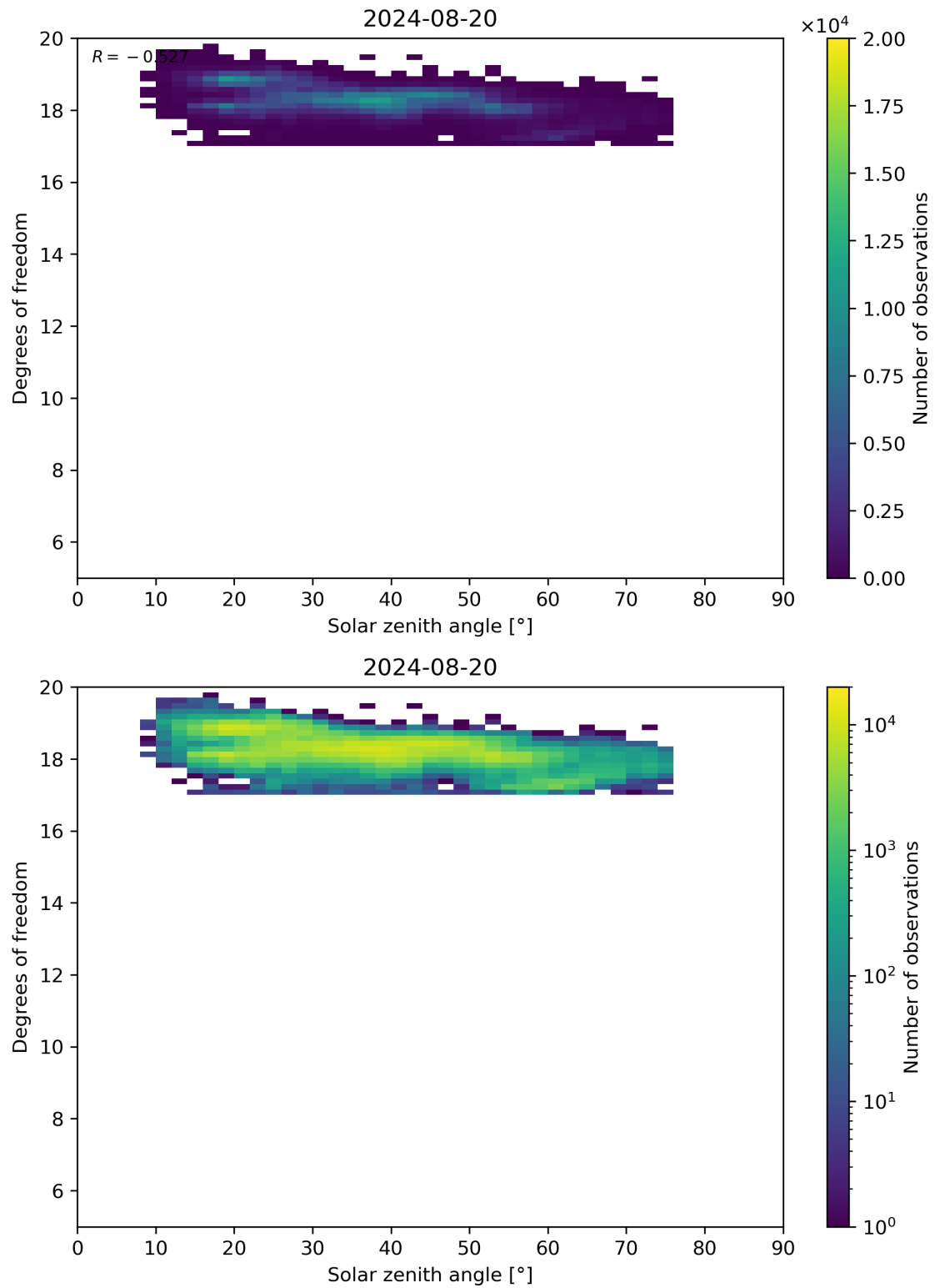
Figure 96: Scatter density plot of “Solar zenith angle” against “Degrees of freedom” for 2024-08-19 to 2024-08-21.
