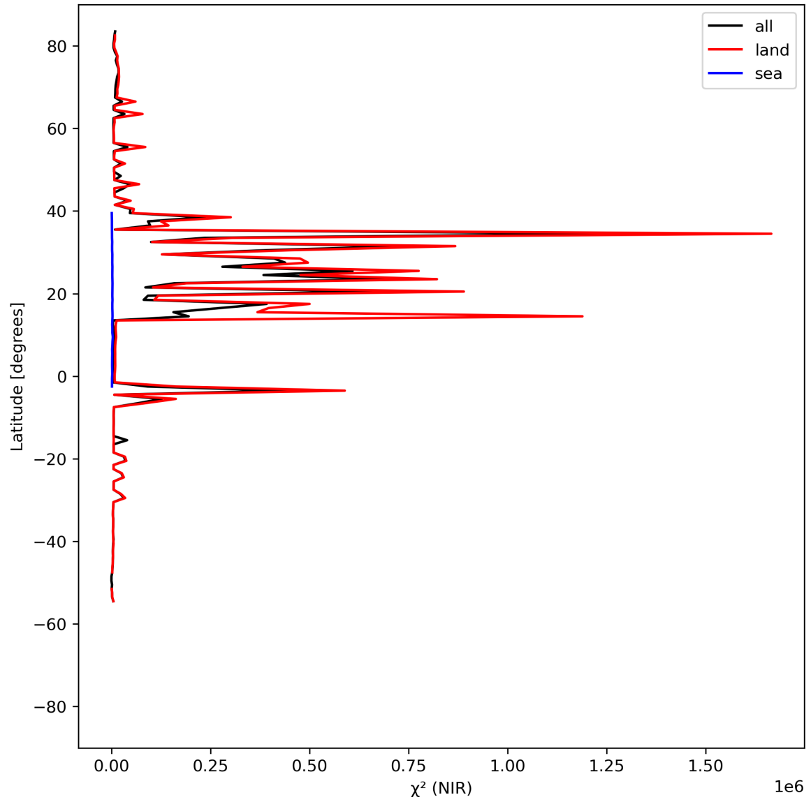
Figure 18: Zonal average of “ \chi^2 (NIR)” for 2024-08-19 to 2024-08-21.
