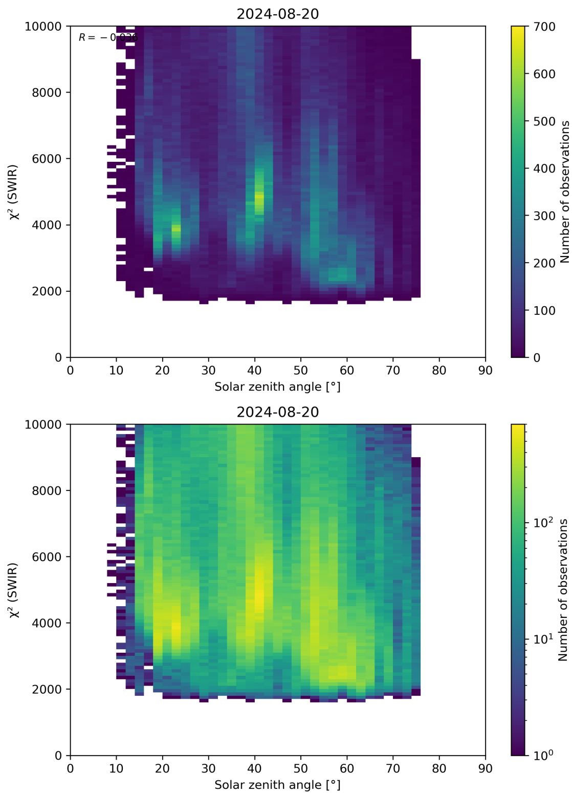
Figure 95: Scatter density plot of “Solar zenith angle” against “ \chi^2 (SWIR)” for 2024-08-19 to 2024-08-21.
