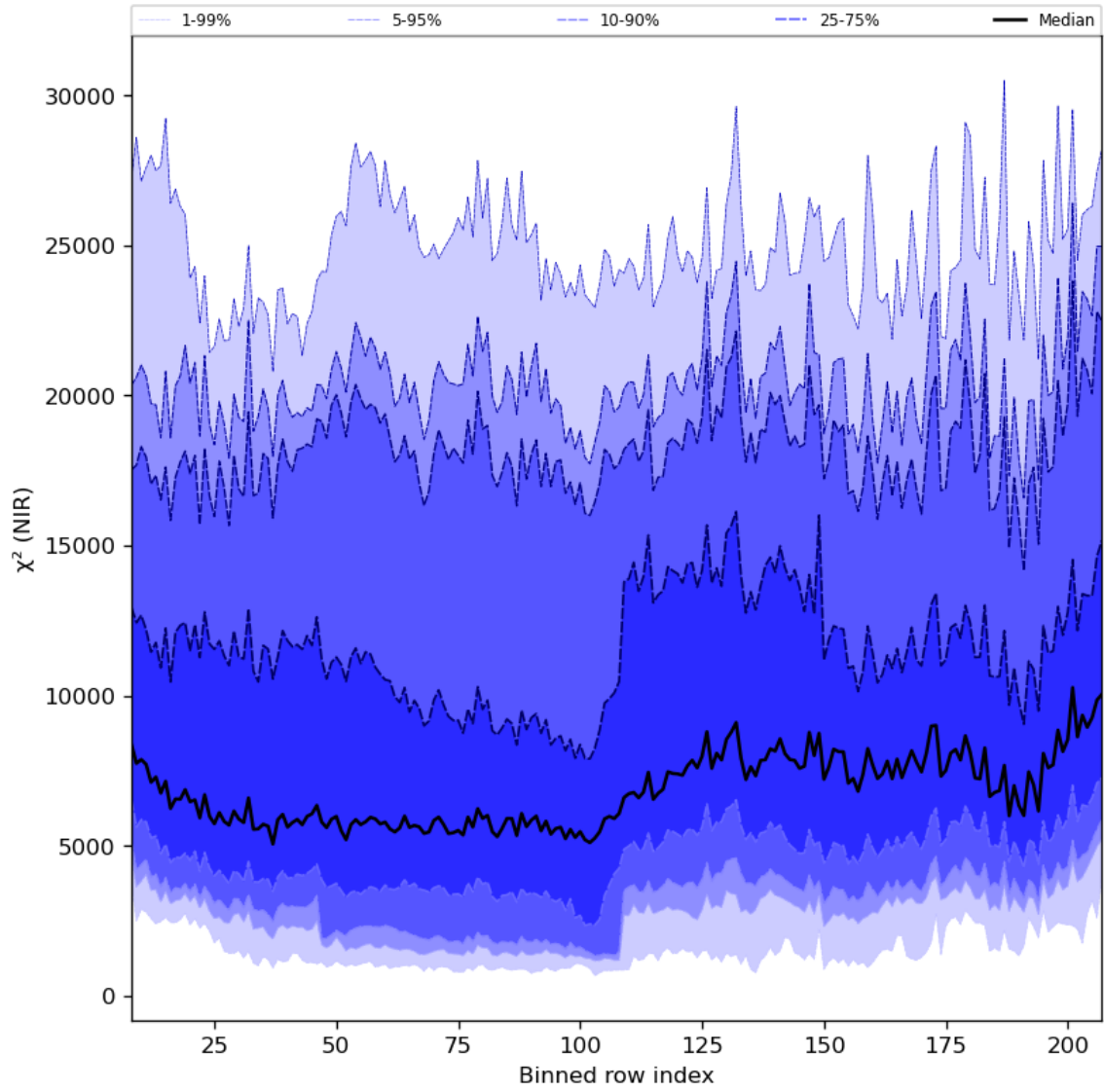
Figure 40: Along track statistics of “ \chi^2 (NIR)” for 2024-08-19 to 2024-08-21
