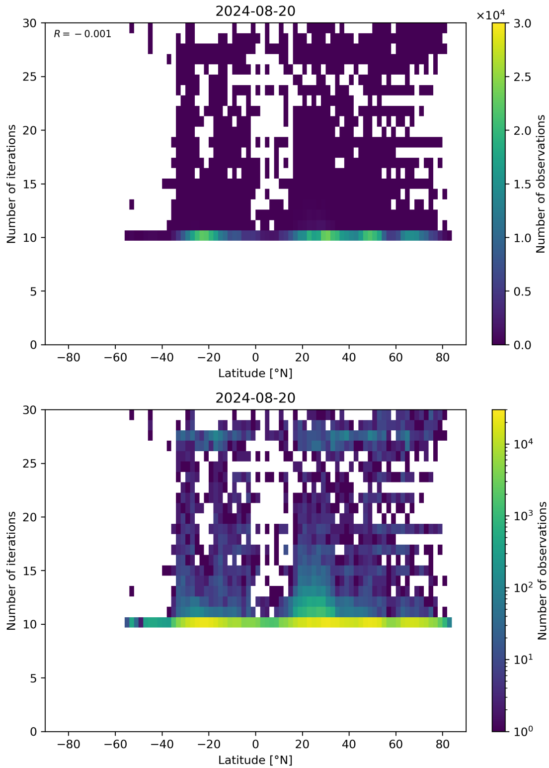
Figure 60: Scatter density plot of “Latitude” against “Number of iterations” for 2024-08-19 to 2024-08-21.
