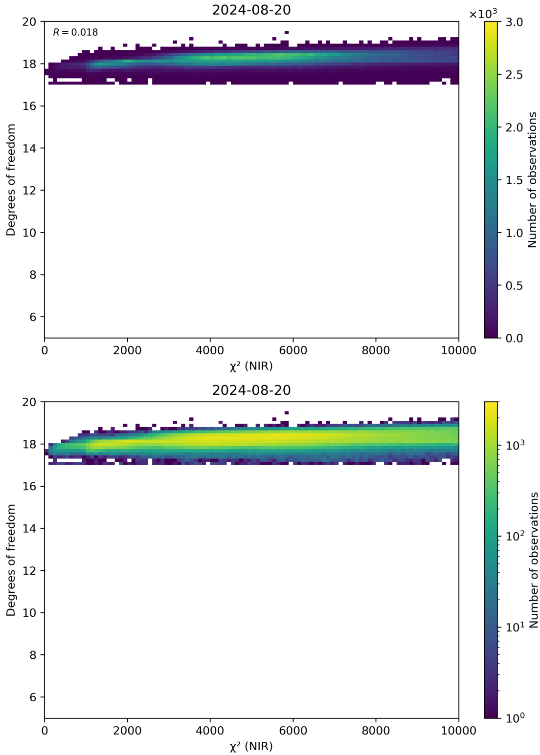
Figure 44: Scatter density plot of “ \chi^2 (NIR)” against “Degrees of freedom” for 2024-08-19 to 2024-08-21.
