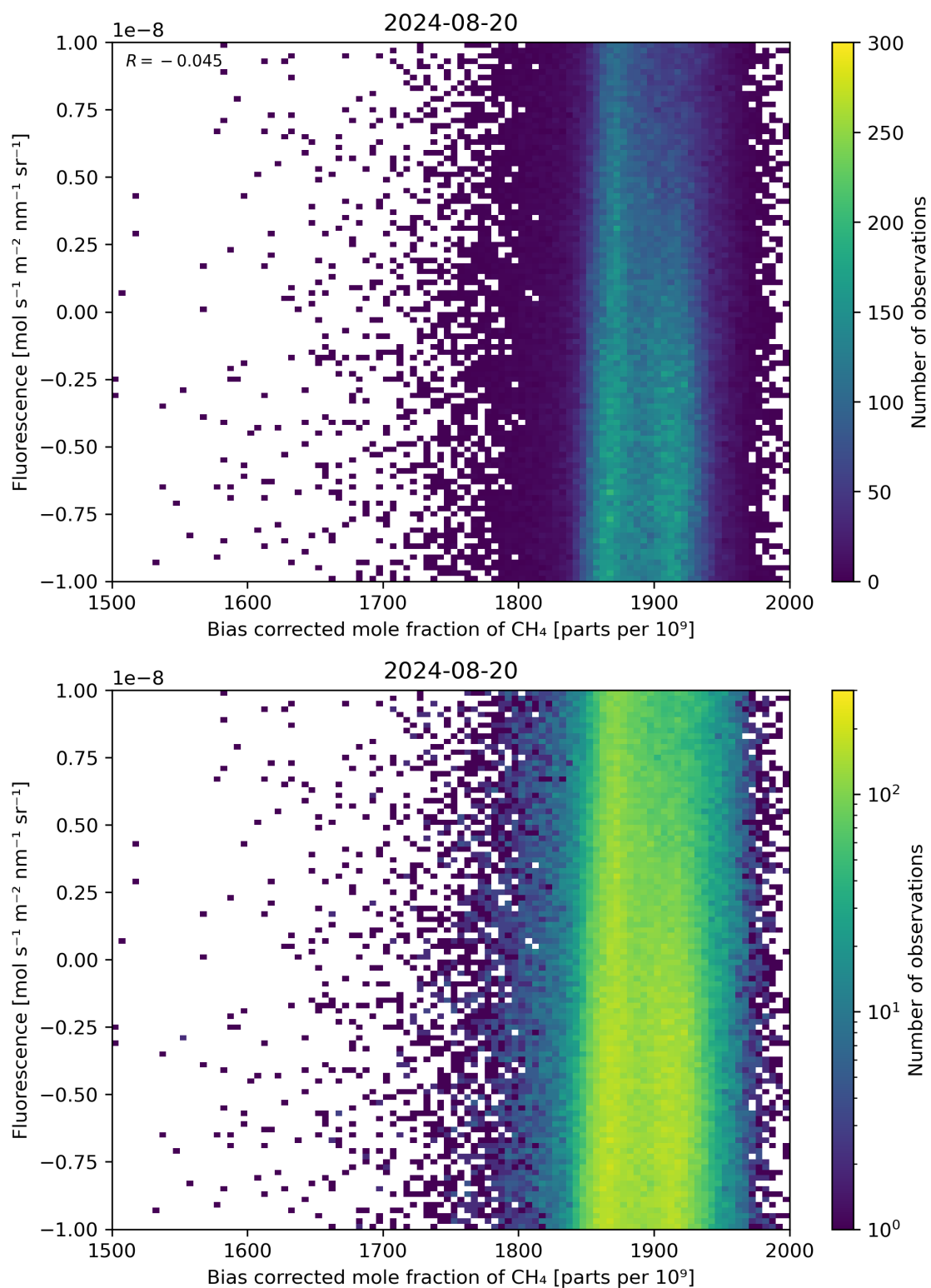
Figure 66: Scatter density plot of “Bias corrected mole fraction of \text{CH}_4 ” against “Fluorescence” for 2024-08-19 to 2024-08-21.
