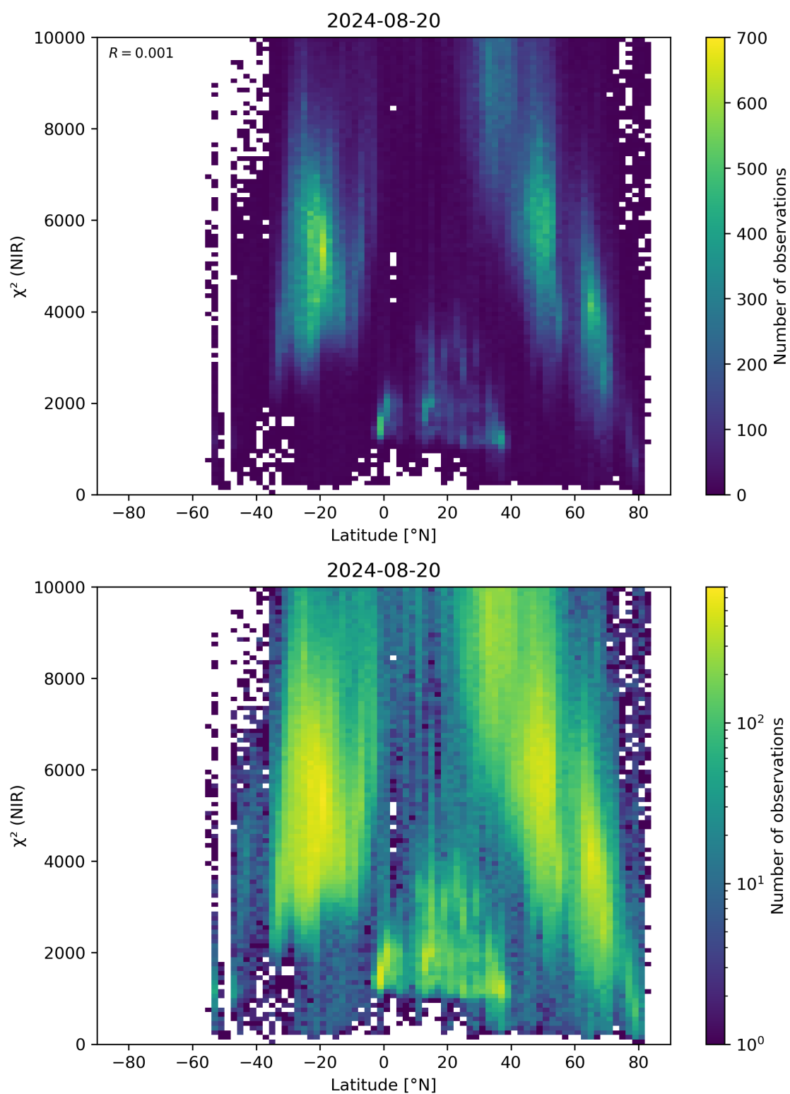
Figure 53: Scatter density plot of “Latitude” against “ \chi^2 (NIR)” for 2024-08-19 to 2024-08-21.
