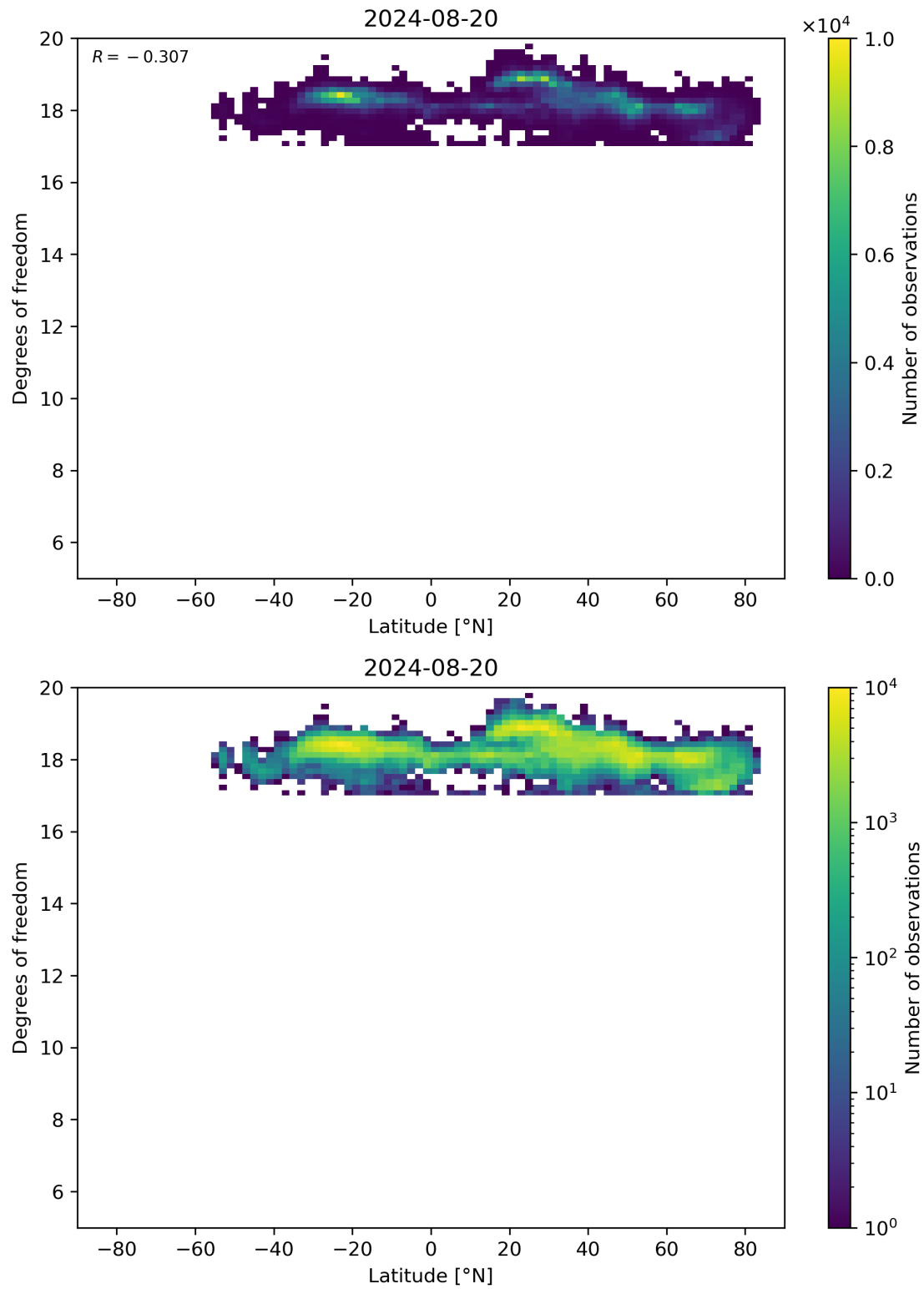
Figure 55: Scatter density plot of “Latitude” against “Degrees of freedom” for 2024-08-19 to 2024-08-21.
