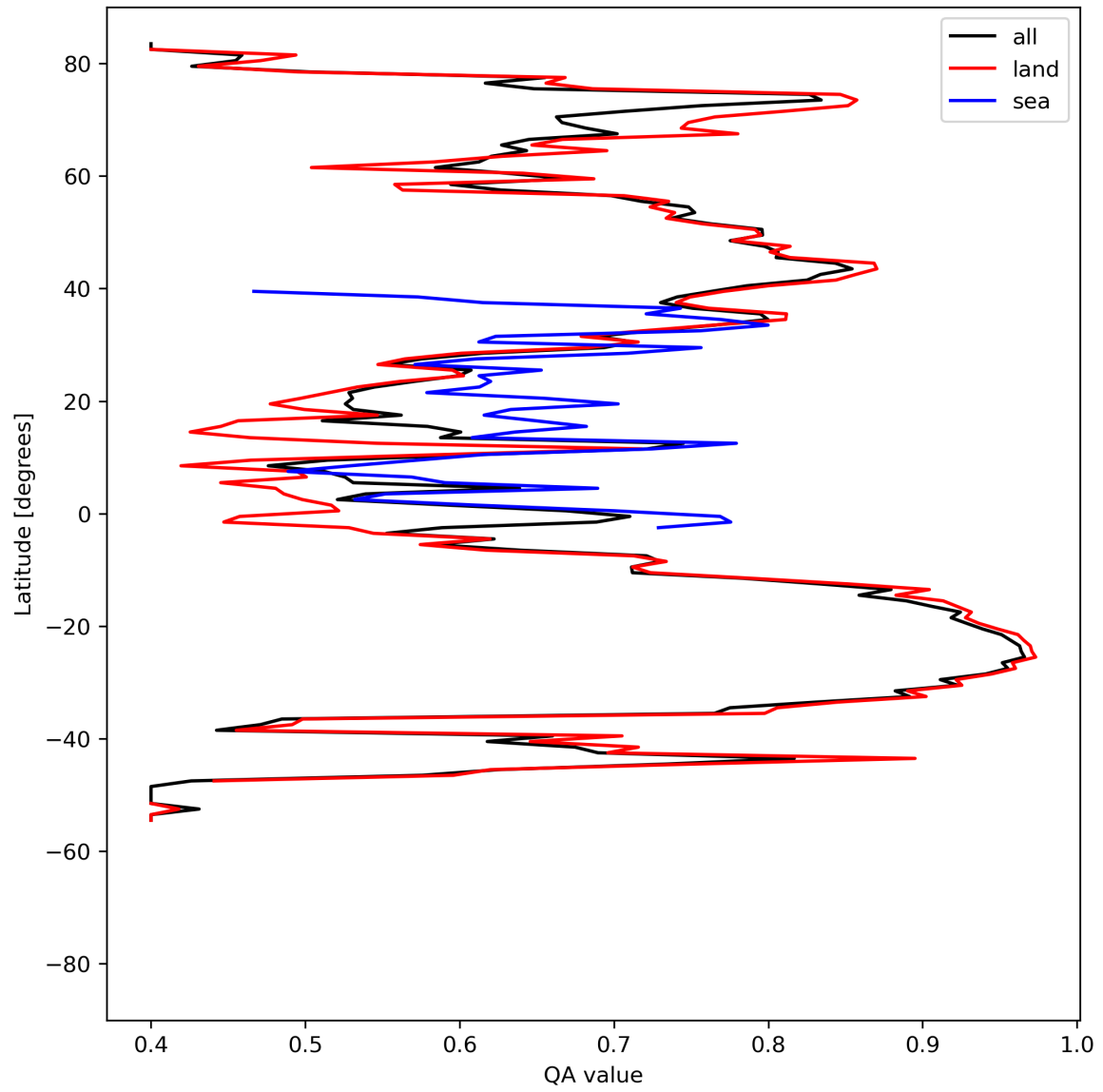
Figure 11: Zonal average of “QA value” for 2024-08-19 to 2024-08-21.
