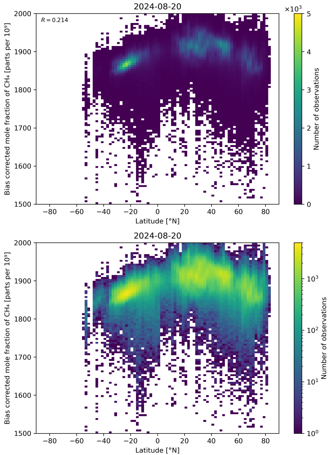
Figure 58: Scatter density plot of “Latitude” against “Bias corrected mole fraction of \text{CH}_4 ” for 2024-08-19 to 2024-08-21.
