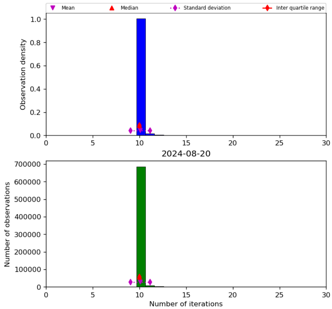
Figure 31: Histogram of “Number of iterations” for 2024-08-19 to 2024-08-21
