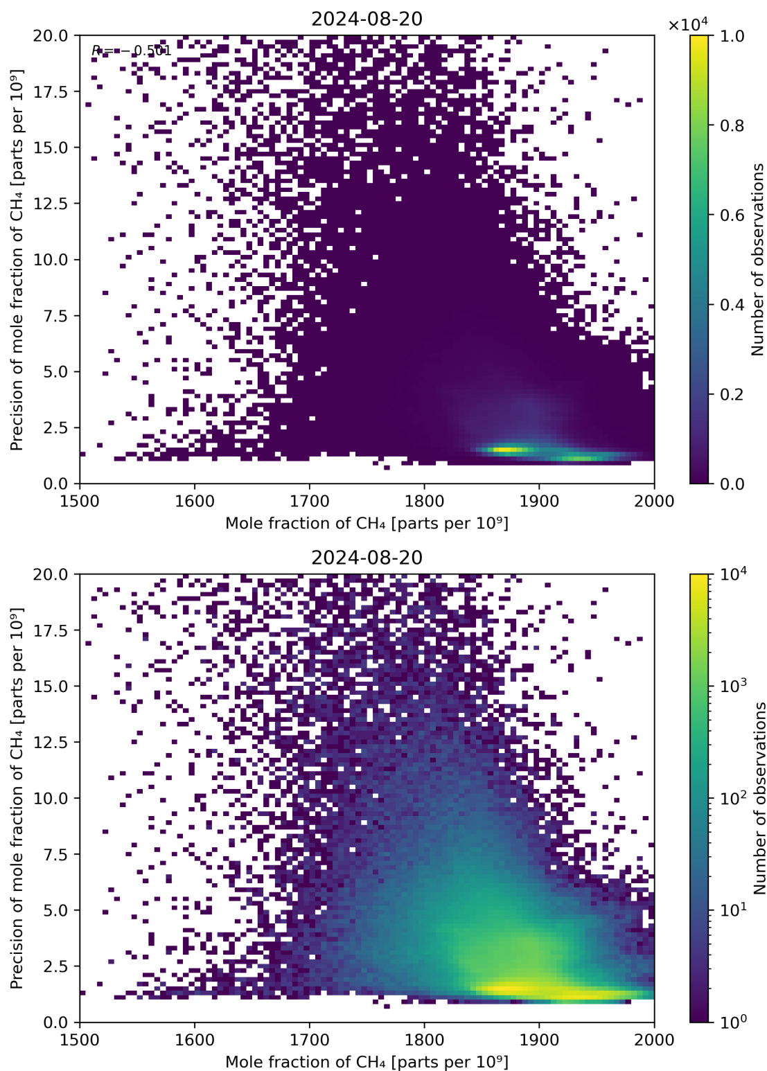
Figure 75: Scatter density plot of “Mole fraction of CH 4 ” against “Precision of mole fraction of CH 4 ” for 2024-08-19 to 2024-08-21.
