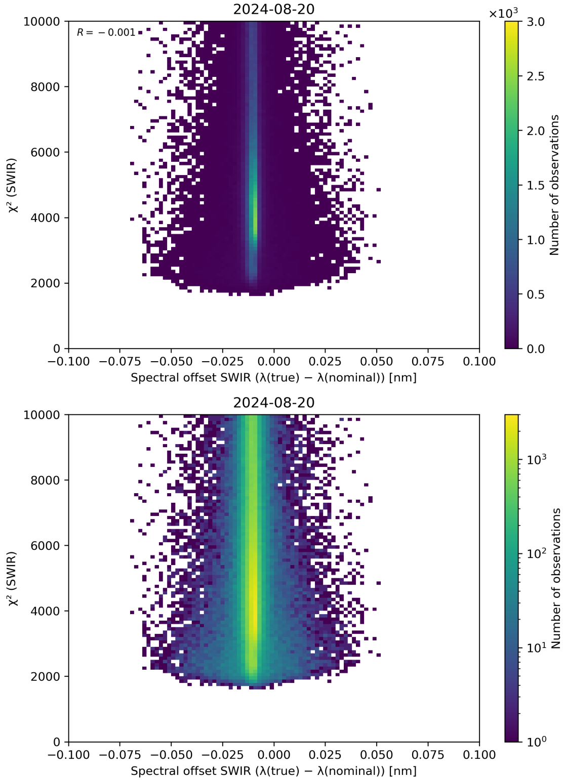
Figure 118: Scatter density plot of “Spectral offset SWIR ( \lambda(\text{true}) - \lambda(\text{nominal}) )” against “ \chi^2 (SWIR)” for 2024-08-19 to 2024-08-21.
