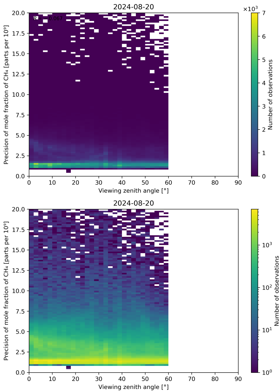
Figure 112: Scatter density plot of “Viewing zenith angle” against “Precision of mole fraction of CH 4 ” for 2024-08-19 to 2024-08-21.
