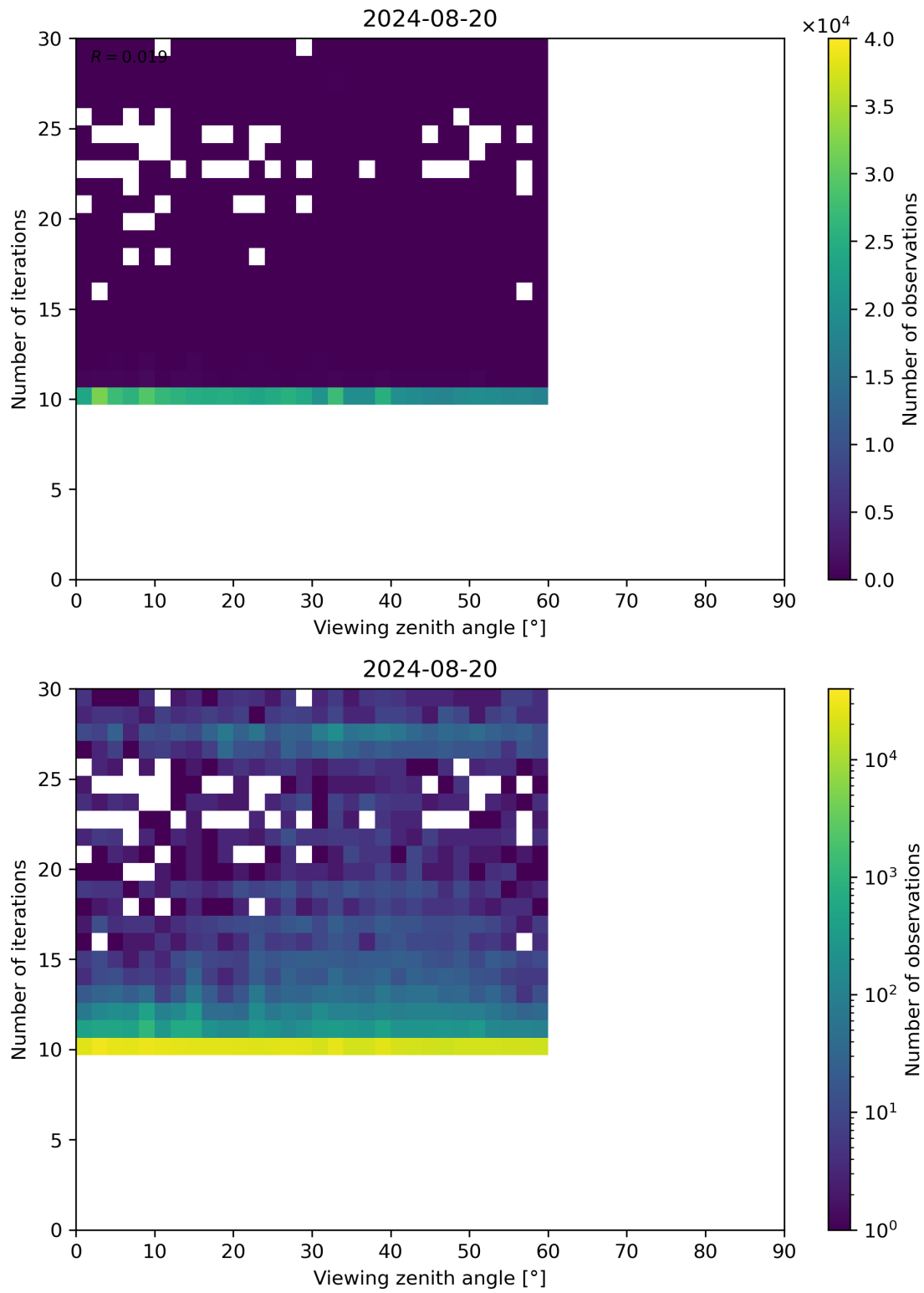
Figure 113: Scatter density plot of “Viewing zenith angle” against “Number of iterations” for 2024-08-19 to 2024-08-21.
