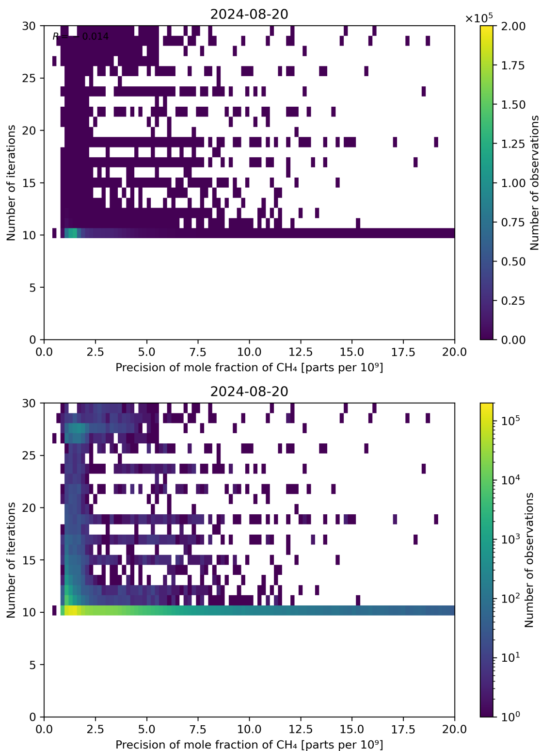
Figure 83: Scatter density plot of “Precision of mole fraction of CH 4 ” against “Number of iterations” for 2024-08-19 to 2024-08-21.
