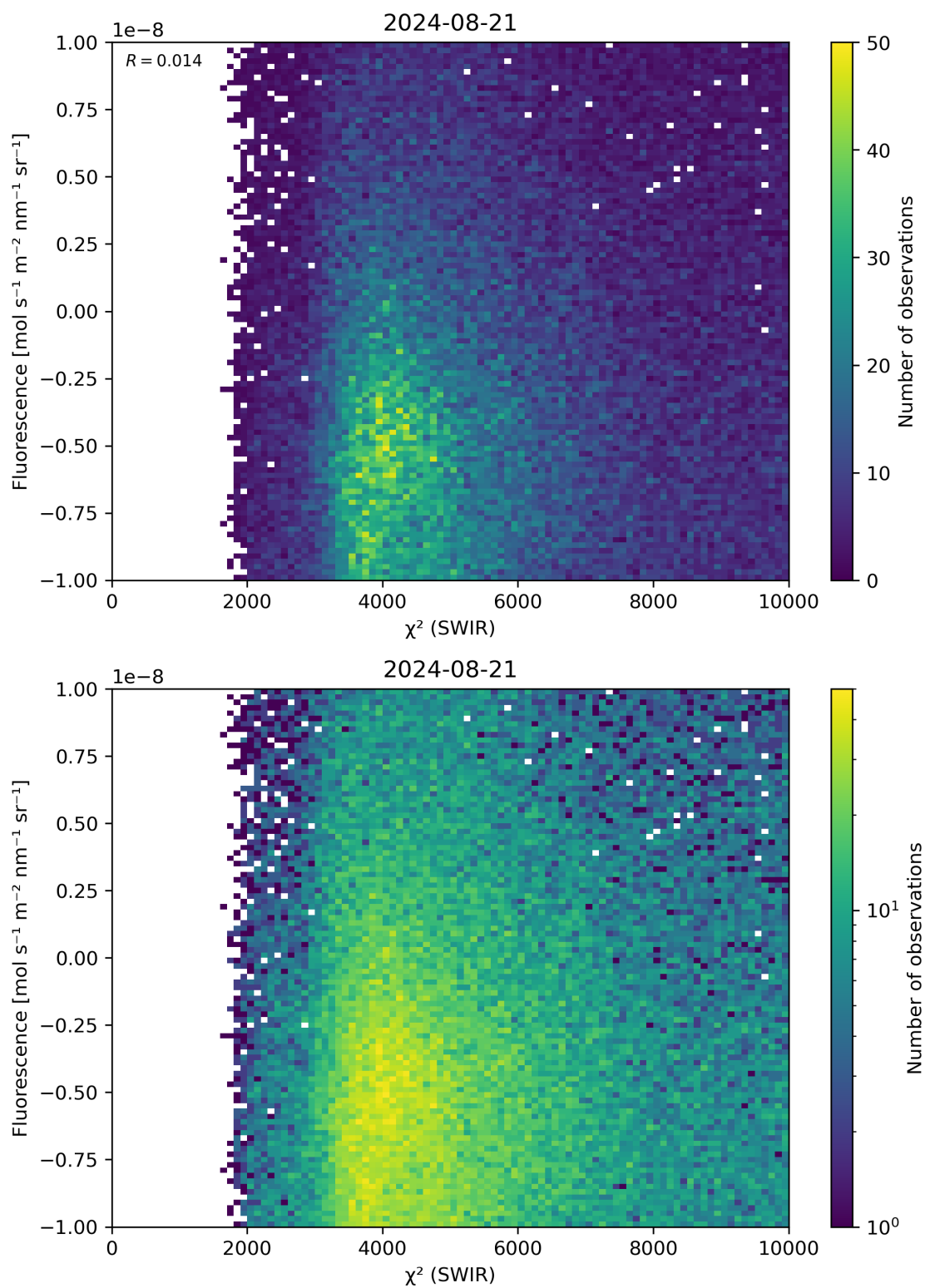
Figure 49: Scatter density plot of “ \chi^2 (SWIR)” against “Fluorescence” for 2024-08-21 to 2024-08-22.
