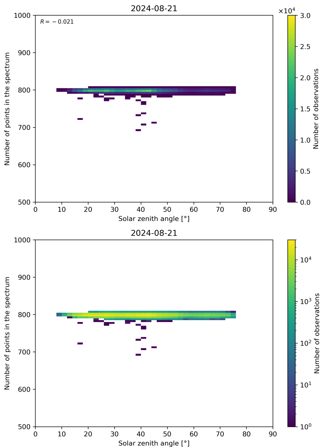
Figure 103: Scatter density plot of “Solar zenith angle” against “Number of points in the spectrum” for 2024-08-21 to 2024-08-22.
