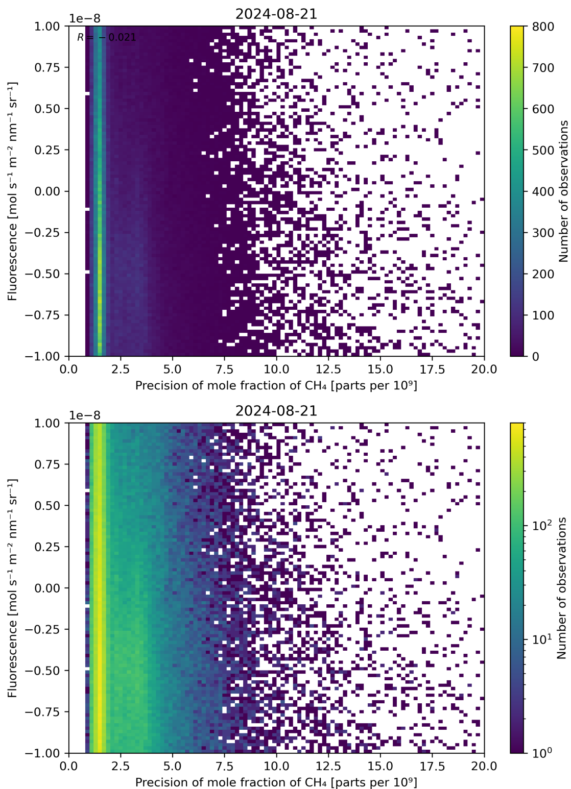
Figure 81: Scatter density plot of “Precision of mole fraction of \text{CH}_4 ” against “Fluorescence” for 2024-08-21 to 2024-08-22.
