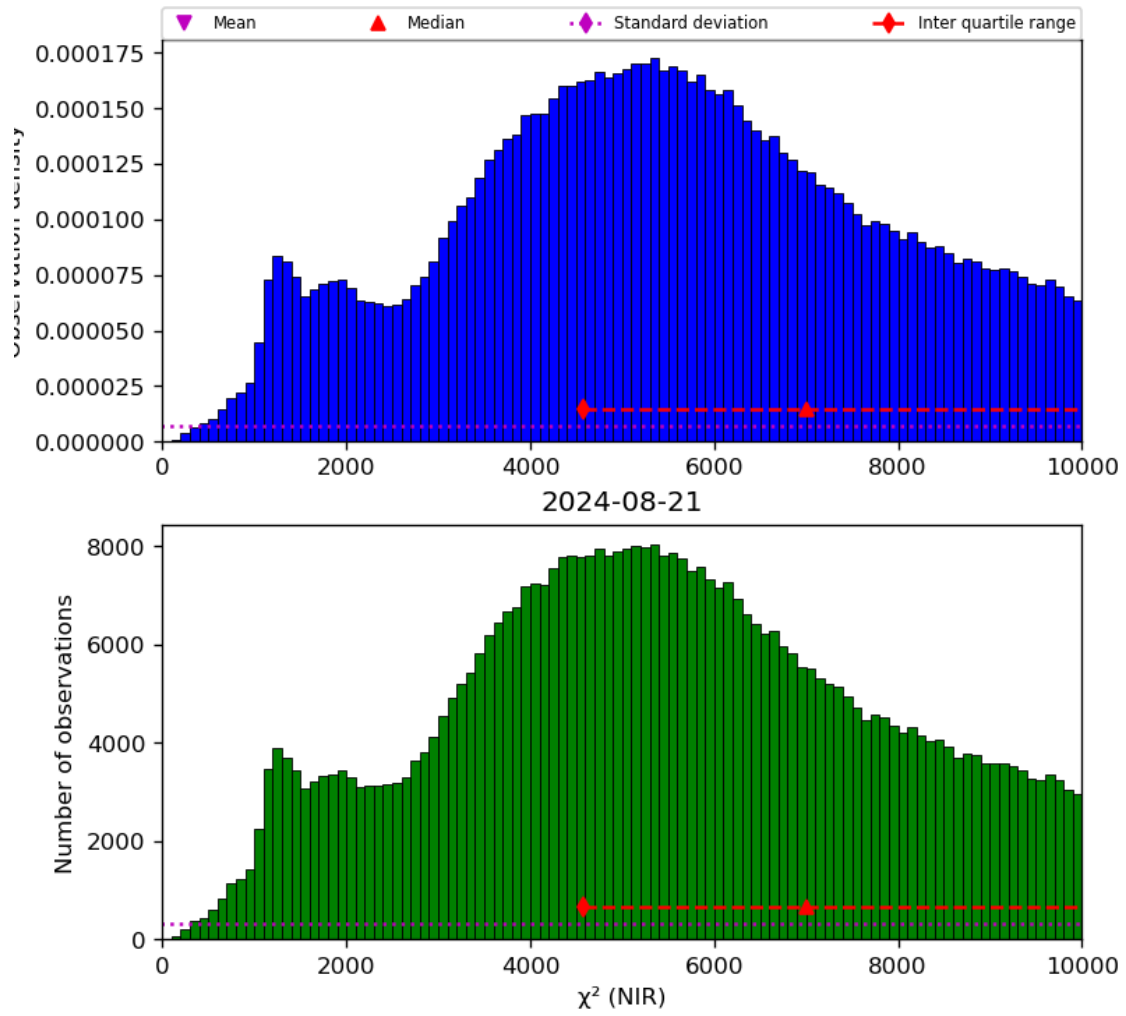
Figure 29: Histogram of “ \chi^2 (NIR)” for 2024-08-21 to 2024-08-22
