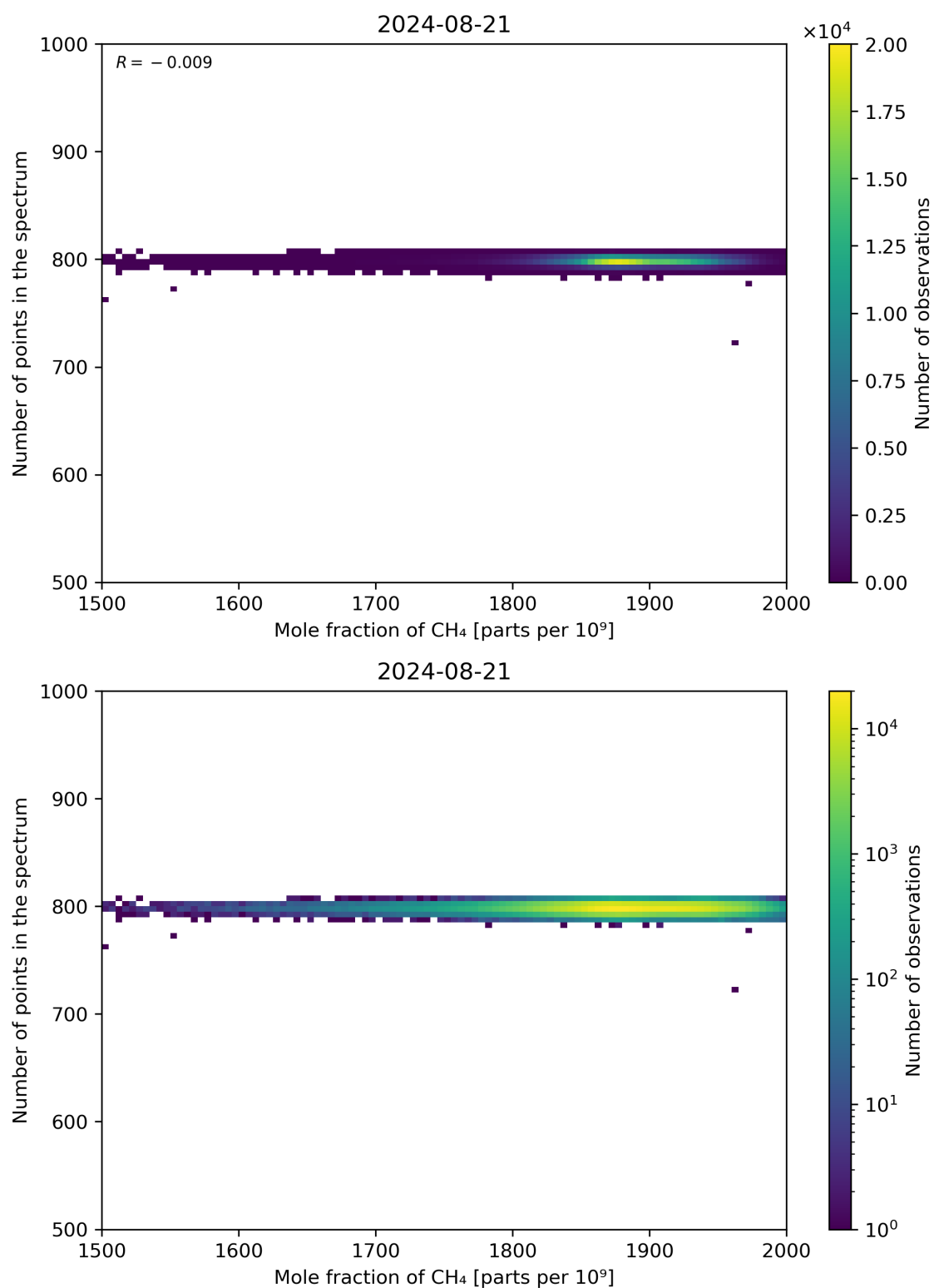
Figure 77: Scatter density plot of “Mole fraction of CH 4 ” against “Number of points in the spectrum” for 2024-08-21 to 2024-08-22.
