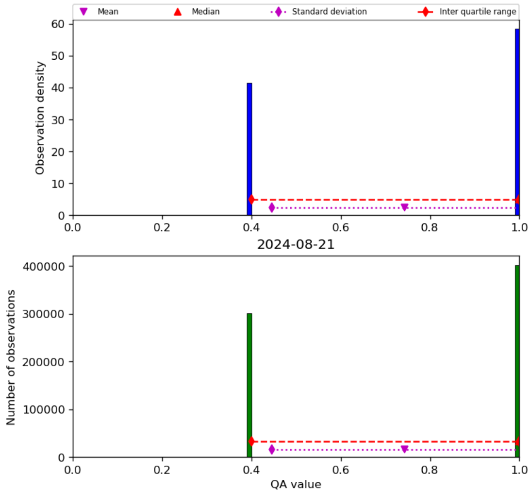
Figure 22: Histogram of “QA value” for 2024-08-21 to 2024-08-22
