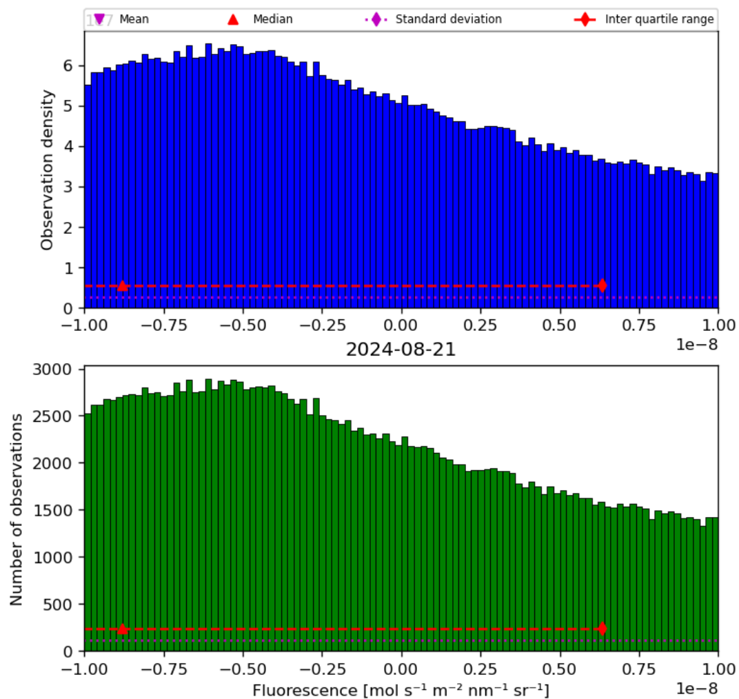
Figure 32: Histogram of “Fluorescence” for 2024-08-21 to 2024-08-22
