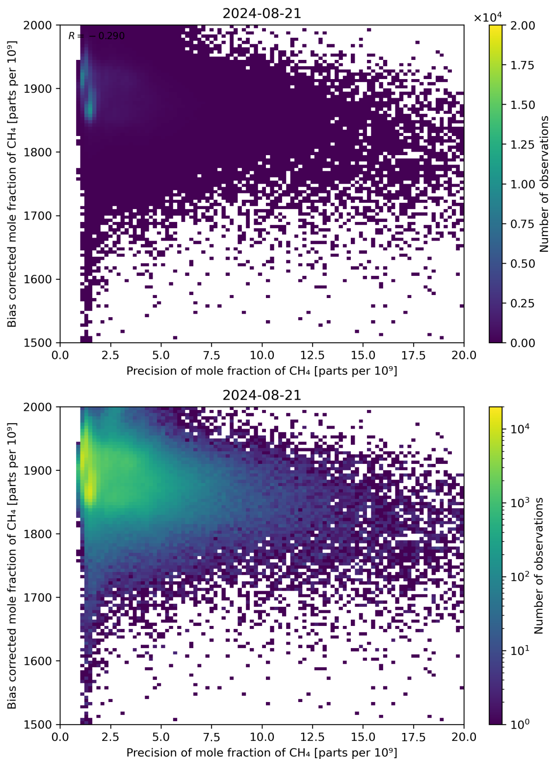
Figure 82: Scatter density plot of “Precision of mole fraction of CH 4 ” against “Bias corrected mole fraction of CH 4 ” for 2024-08-21 to 2024-08-22.
