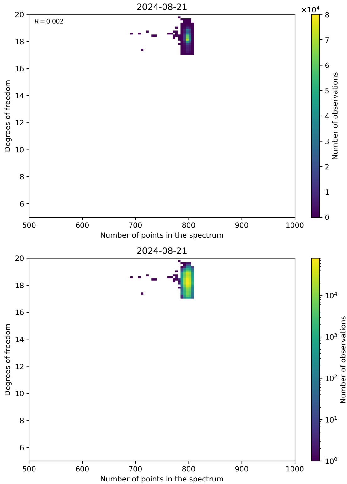
Figure 90: Scatter density plot of “Number of points in the spectrum” against “Degrees of freedom” for 2024-08-21 to 2024-08-22.
