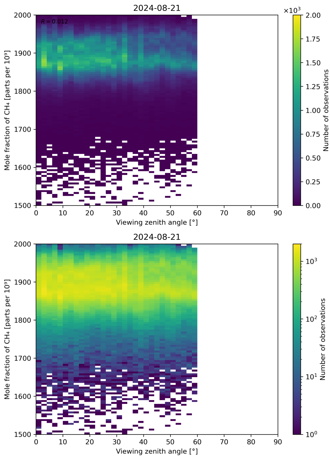
Figure 110: Scatter density plot of “Viewing zenith angle” against “Mole fraction of CH 4 ” for 2024-08-21 to 2024-08-22.
