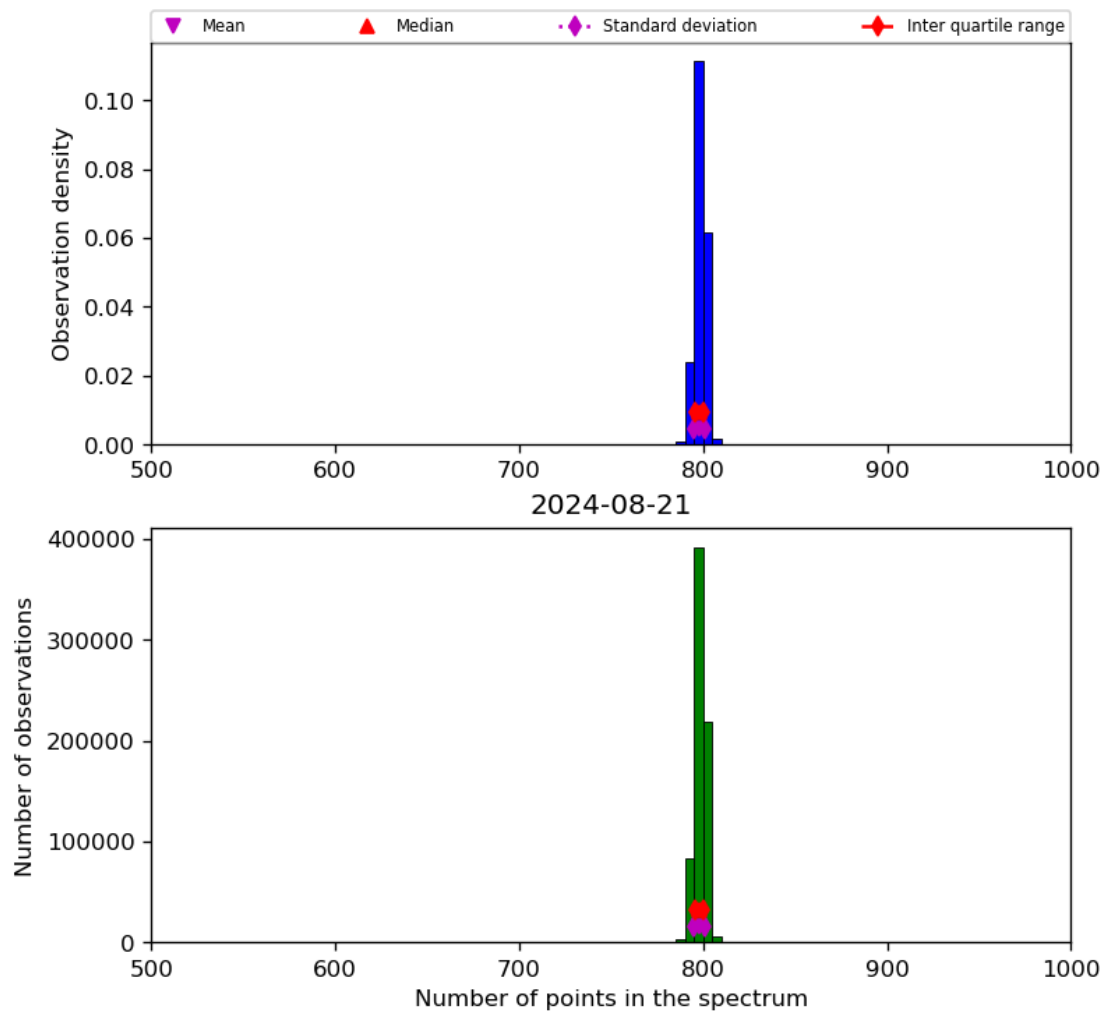
Figure 26: Histogram of “Number of points in the spectrum” for 2024-08-21 to 2024-08-22
