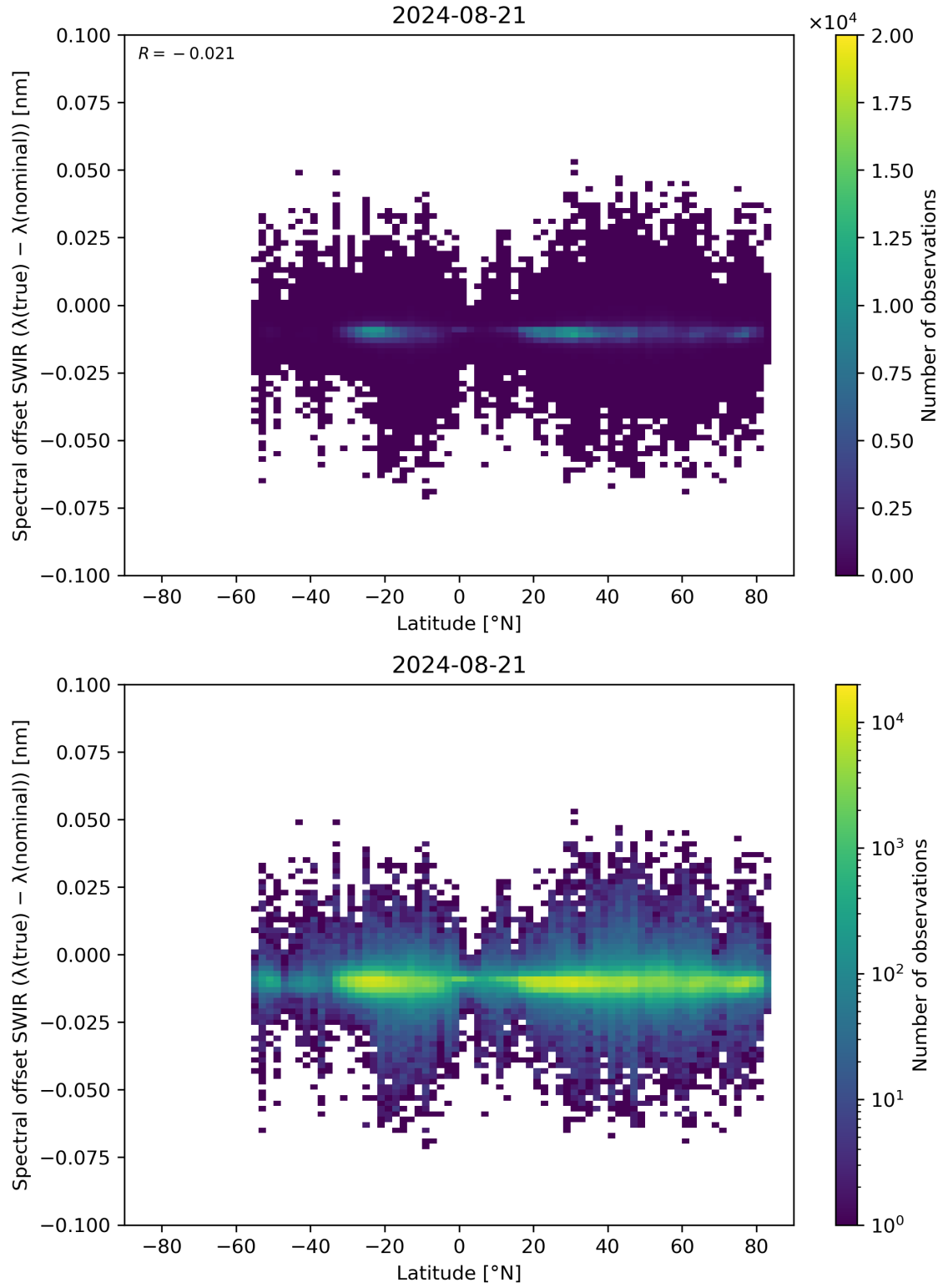
Figure 62: Scatter density plot of “Latitude” against “Spectral offset SWIR ( \lambda(\text{true}) - \lambda(\text{nominal}) )” for 2024-08-21 to 2024-08-22.
