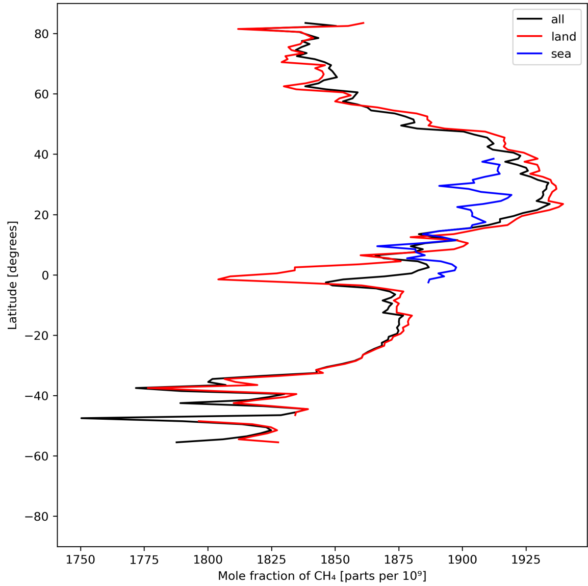
Figure 12: Zonal average of “Mole fraction of \text{CH}_4 ” for 2024-08-21 to 2024-08-22.
