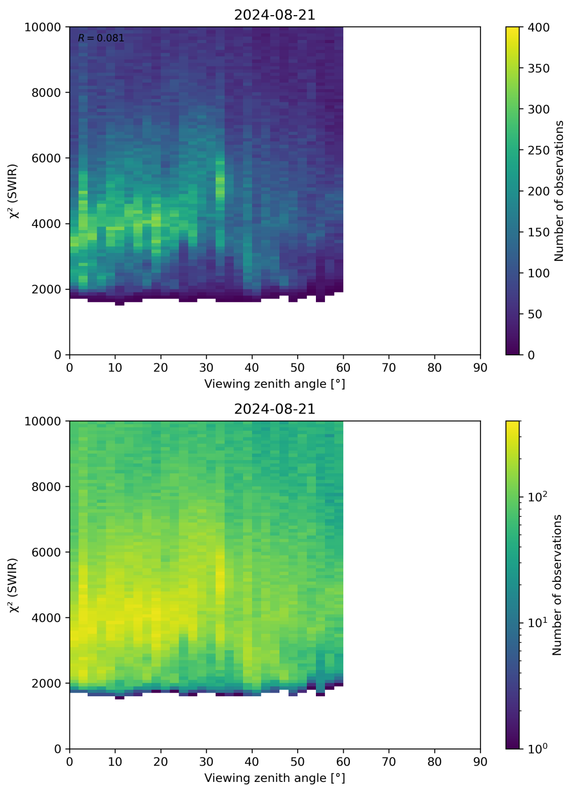
Figure 106: Scatter density plot of “Viewing zenith angle” against “ \chi^2 (SWIR)” for 2024-08-21 to 2024-08-22.
