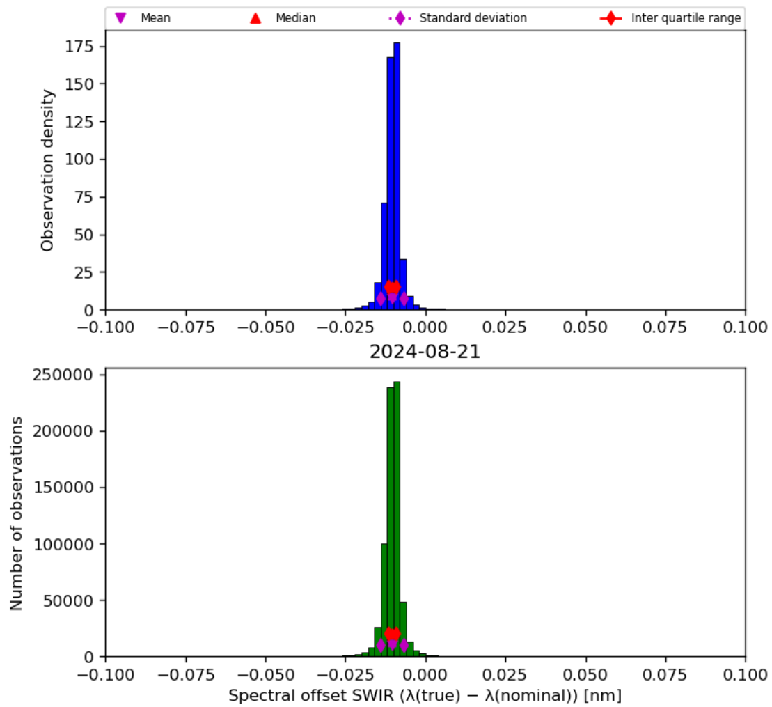
Figure 27: Histogram of “Spectral offset SWIR ( \lambda(\text{true}) - \lambda(\text{nominal}) )” for 2024-08-21 to 2024-08-22
