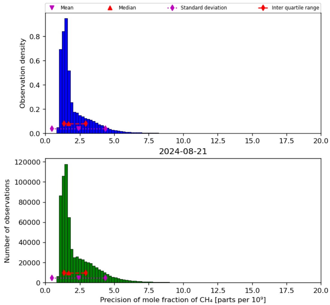
Figure 24: Histogram of “Precision of mole fraction of CH 4 ” for 2024-08-21 to 2024-08-22
