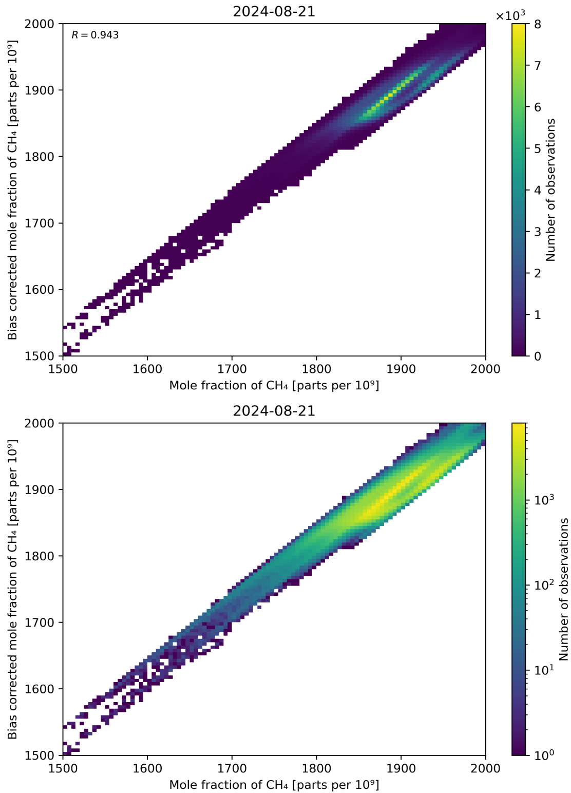
Figure 74: Scatter density plot of “Mole fraction of CH 4 ” against “Bias corrected mole fraction of CH 4 ” for 2024-08-21 to 2024-08-22.
