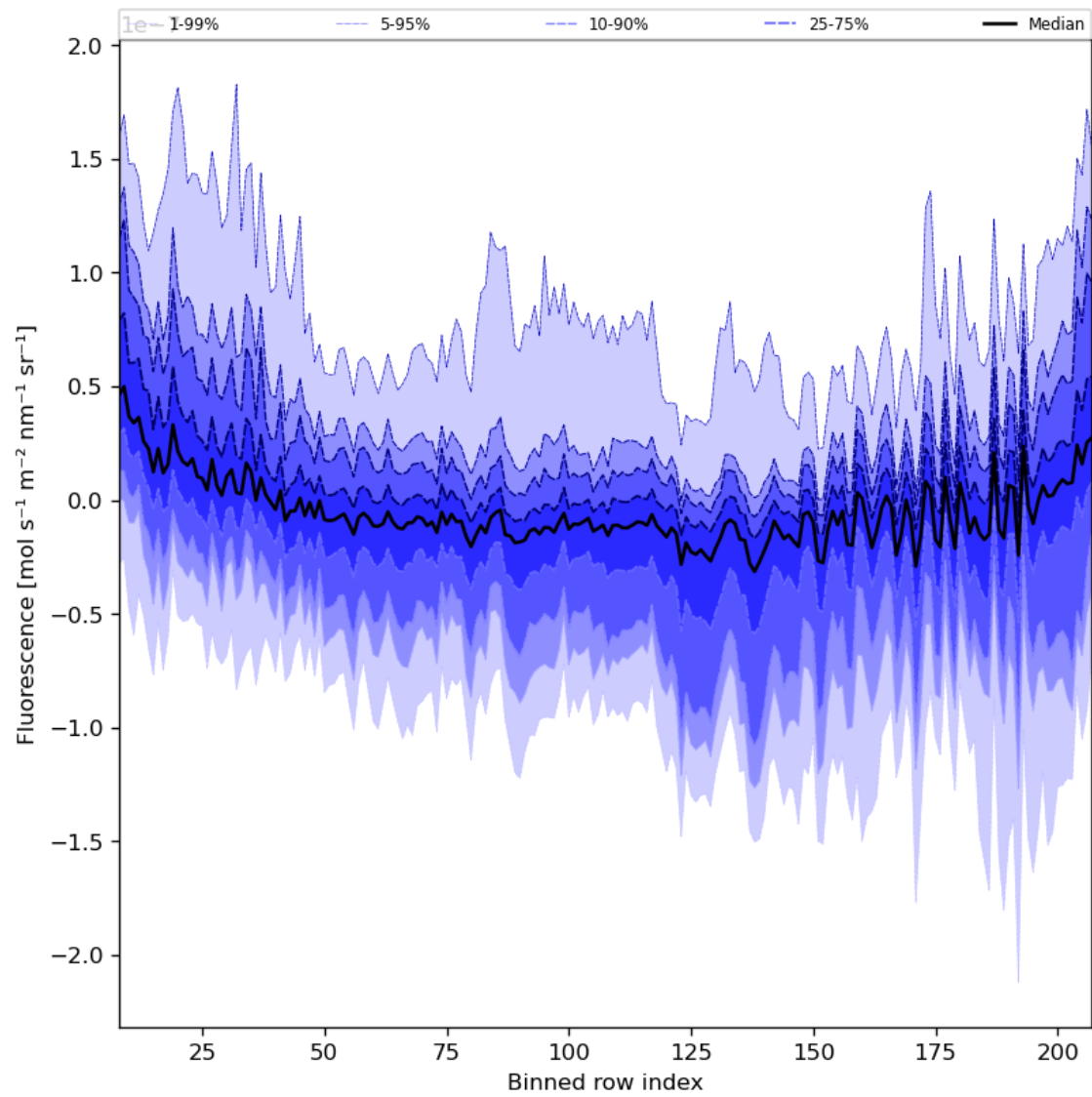
Figure 43: Along track statistics of “Fluorescence” for 2024-08-21 to 2024-08-22
