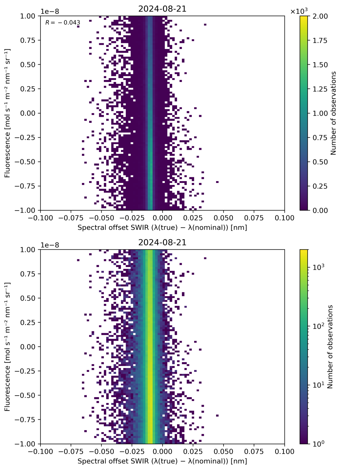
Figure 120: Scatter density plot of “Spectral offset SWIR ( \lambda(\text{true}) - \lambda(\text{nominal}) )” against “Fluorescence” for 2024-08-21 to 2024-08-22.
