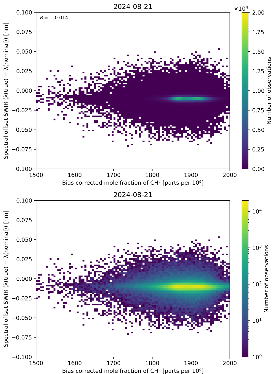
Figure 69: Scatter density plot of “Bias corrected mole fraction of \text{CH}_4 ” against “Spectral offset SWIR ( \lambda(\text{true}) - \lambda(\text{nominal}) )” for 2024-08-21 to 2024-08-22.
