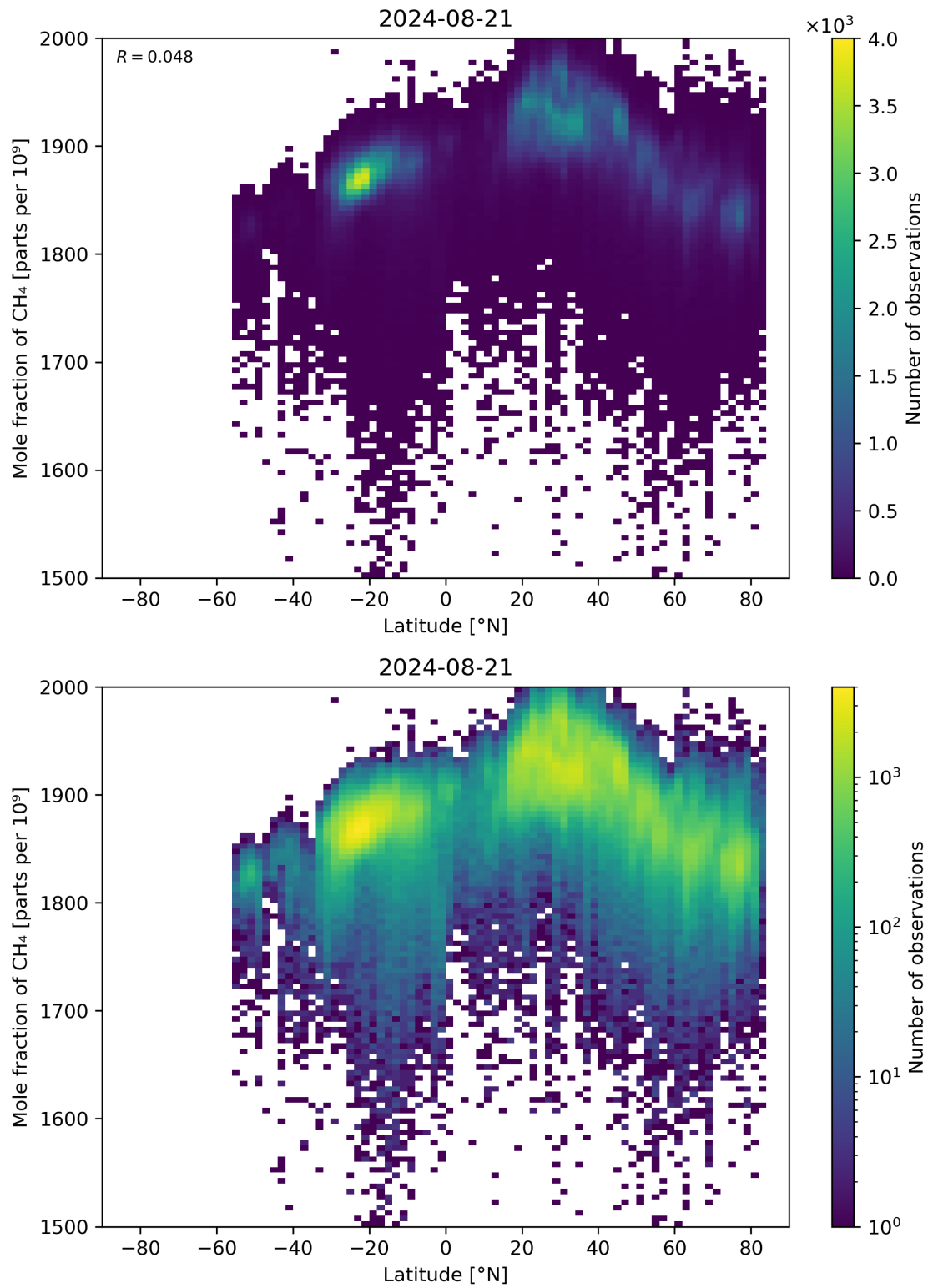
Figure 57: Scatter density plot of “Latitude” against “Mole fraction of \text{CH}_4 ” for 2024-08-21 to 2024-08-22.
