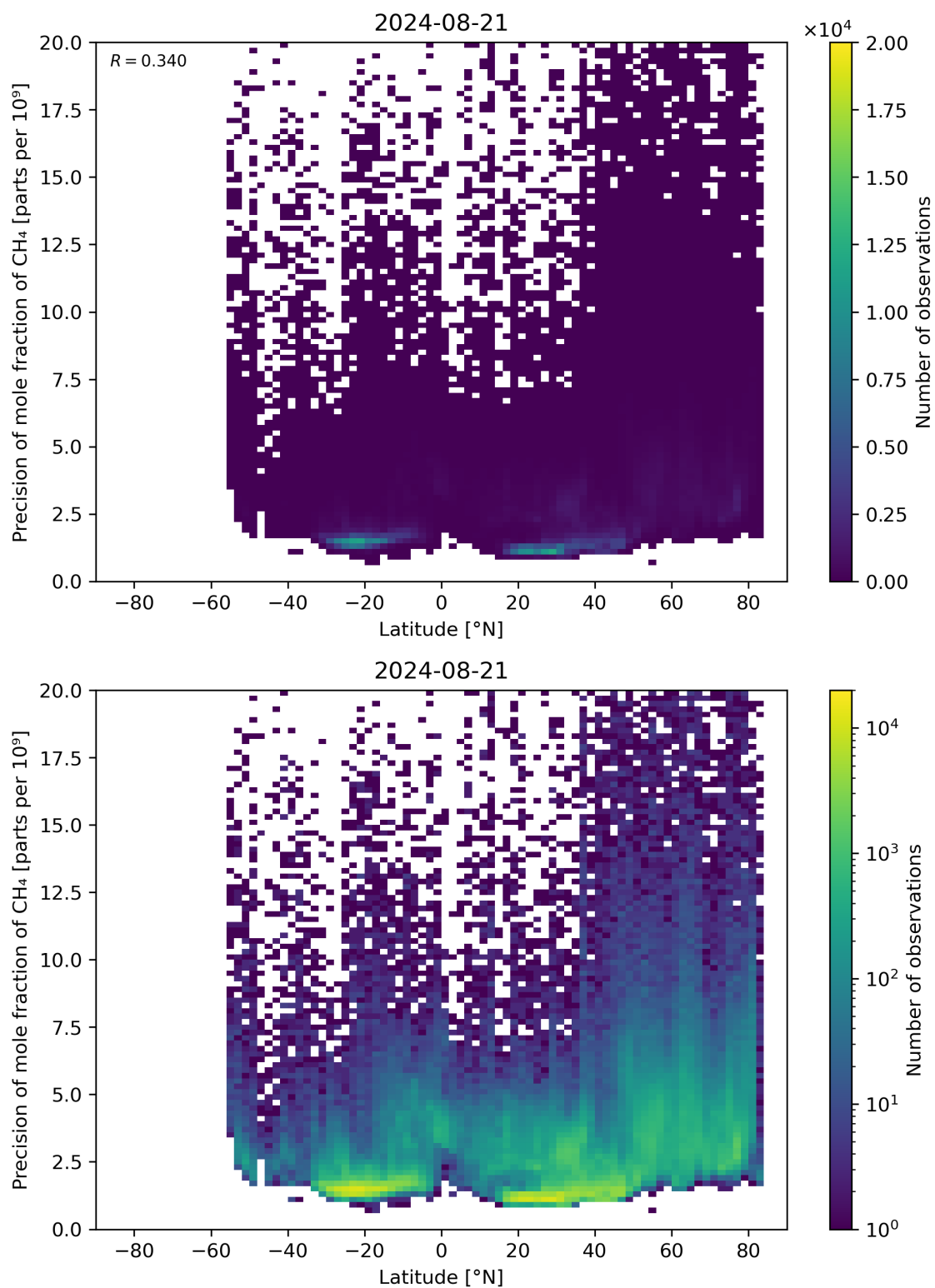
Figure 59: Scatter density plot of “Latitude” against “Precision of mole fraction of CH 4 ” for 2024-08-21 to 2024-08-22.
