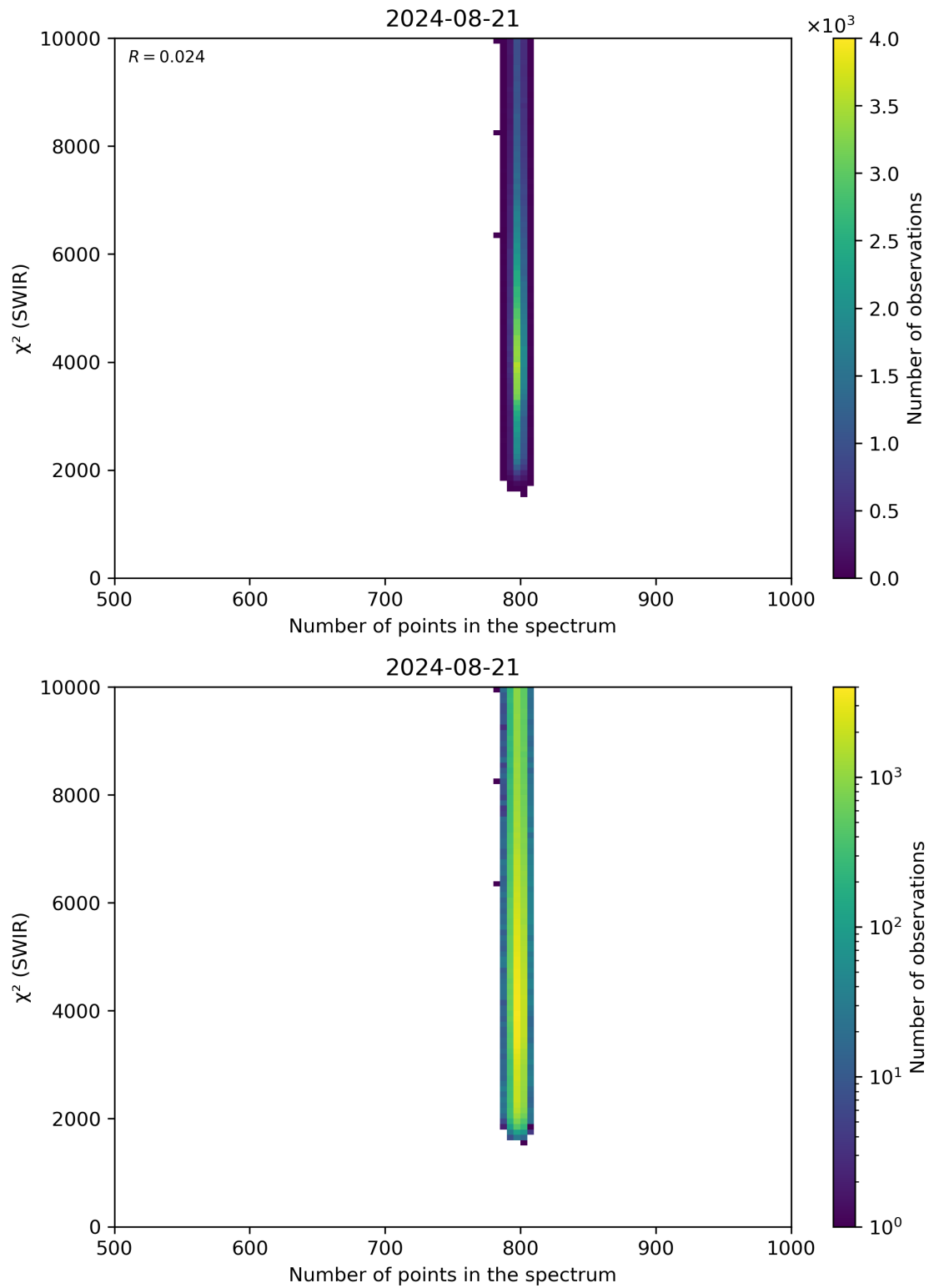
Figure 89: Scatter density plot of “Number of points in the spectrum” against “ \chi^2 (SWIR)” for 2024-08-21 to 2024-08-22.
