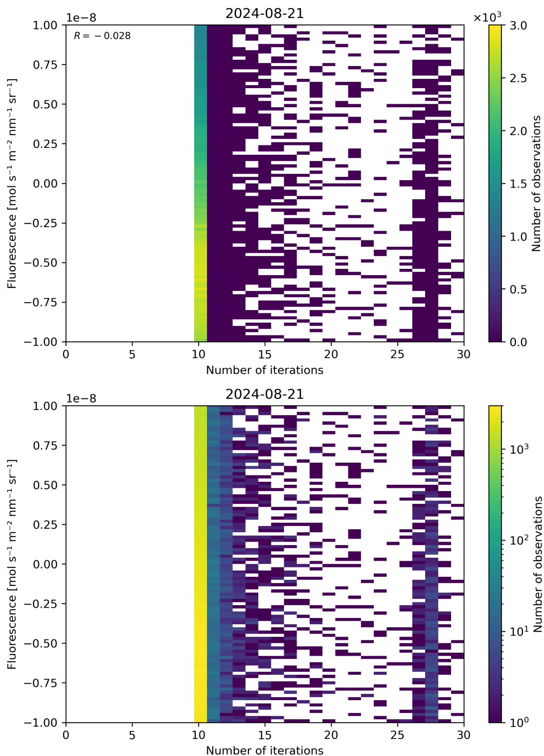
Figure 87: Scatter density plot of “Number of iterations” against “Fluorescence” for 2024-08-21 to 2024-08-22.
