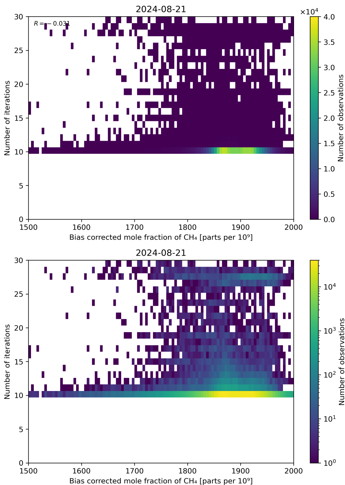
Figure 67: Scatter density plot of “Bias corrected mole fraction of CH 4 ” against “Number of iterations” for 2024-08-21 to 2024-08-22.
