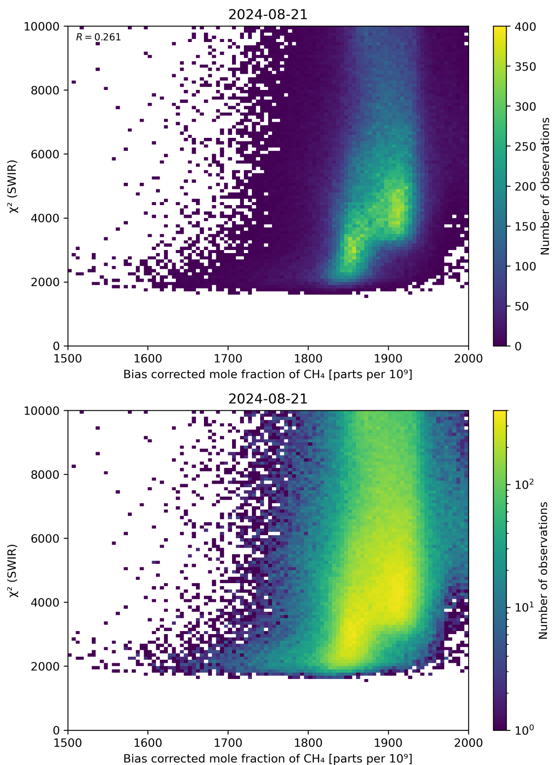
Figure 64: Scatter density plot of “Bias corrected mole fraction of \text{CH}_4 ” against “ \chi^2 (SWIR)” for 2024-08-21 to 2024-08-22.
