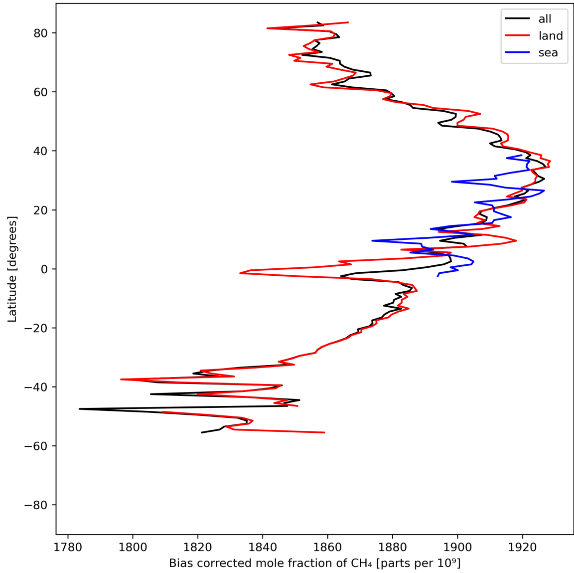
Figure 14: Zonal average of “Bias corrected mole fraction of \text{CH}_4 ” for 2024-08-21 to 2024-08-22.
