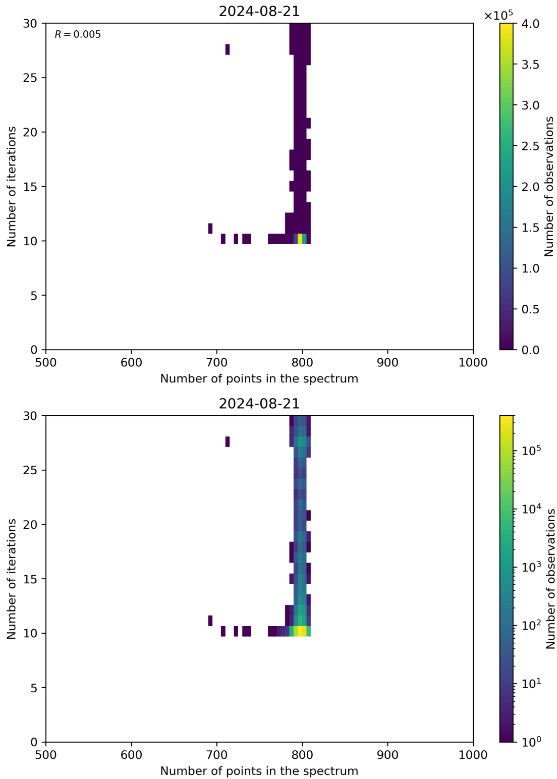
Figure 92: Scatter density plot of “Number of points in the spectrum” against “Number of iterations” for 2024-08-21 to 2024-08-22.
