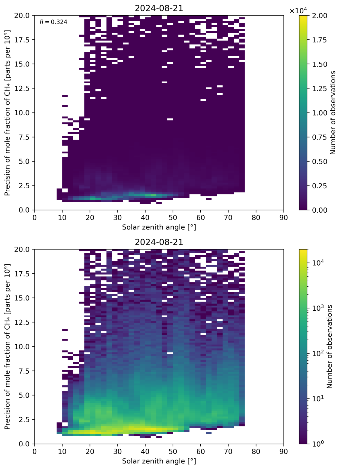
Figure 101: Scatter density plot of “Solar zenith angle” against “Precision of mole fraction of CH 4 ” for 2024-08-21 to 2024-08-22.
