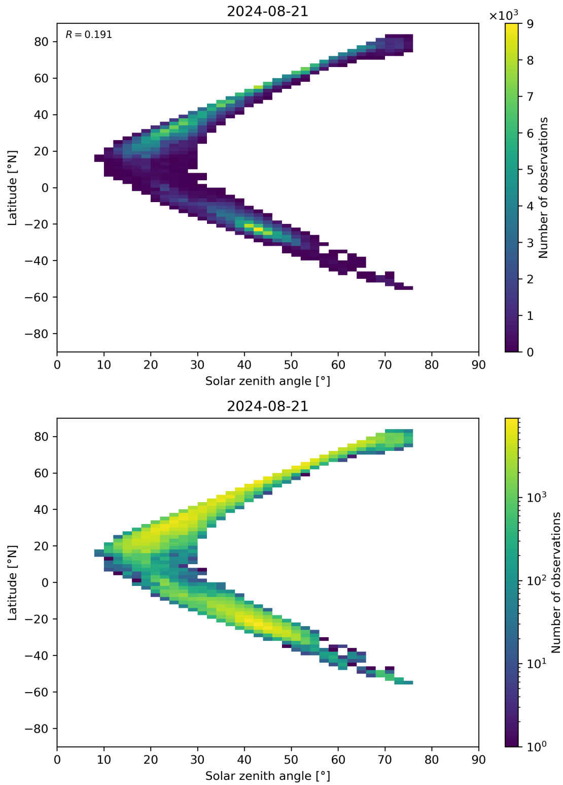
Figure 98: Scatter density plot of “Solar zenith angle” against “Latitude” for 2024-08-21 to 2024-08-22.
