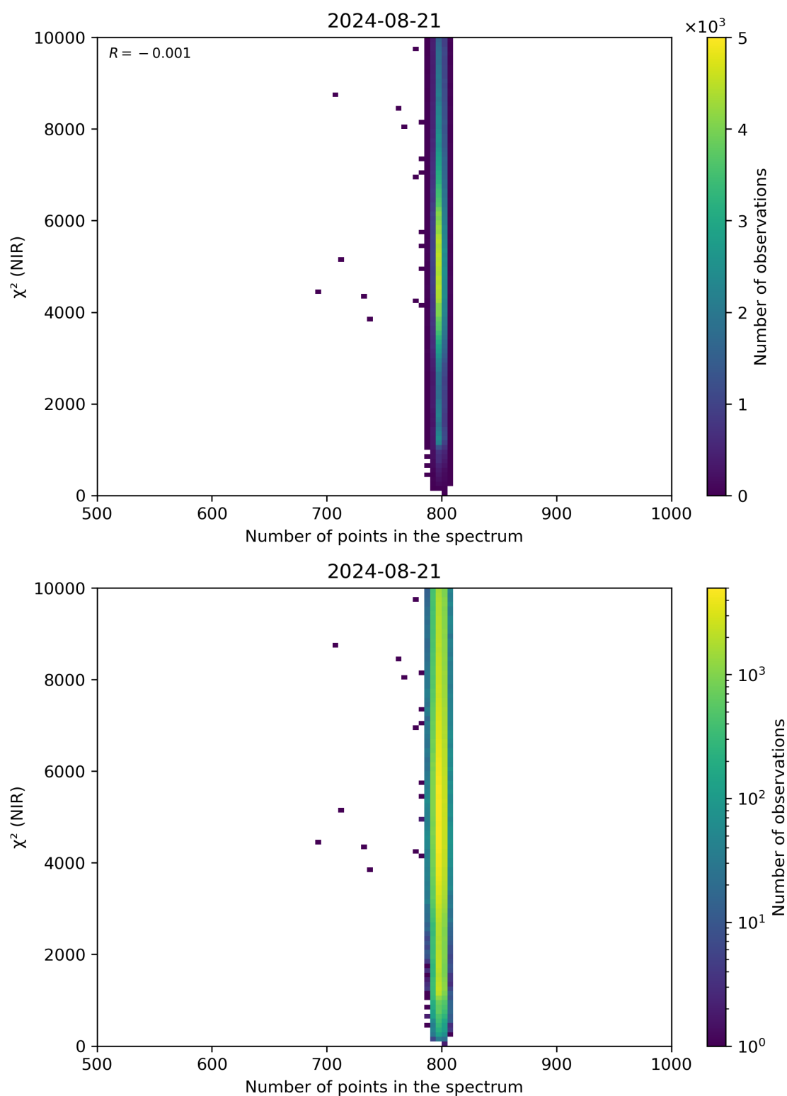
Figure 88: Scatter density plot of “Number of points in the spectrum” against “ \chi^2 (NIR)” for 2024-08-21 to 2024-08-22.
