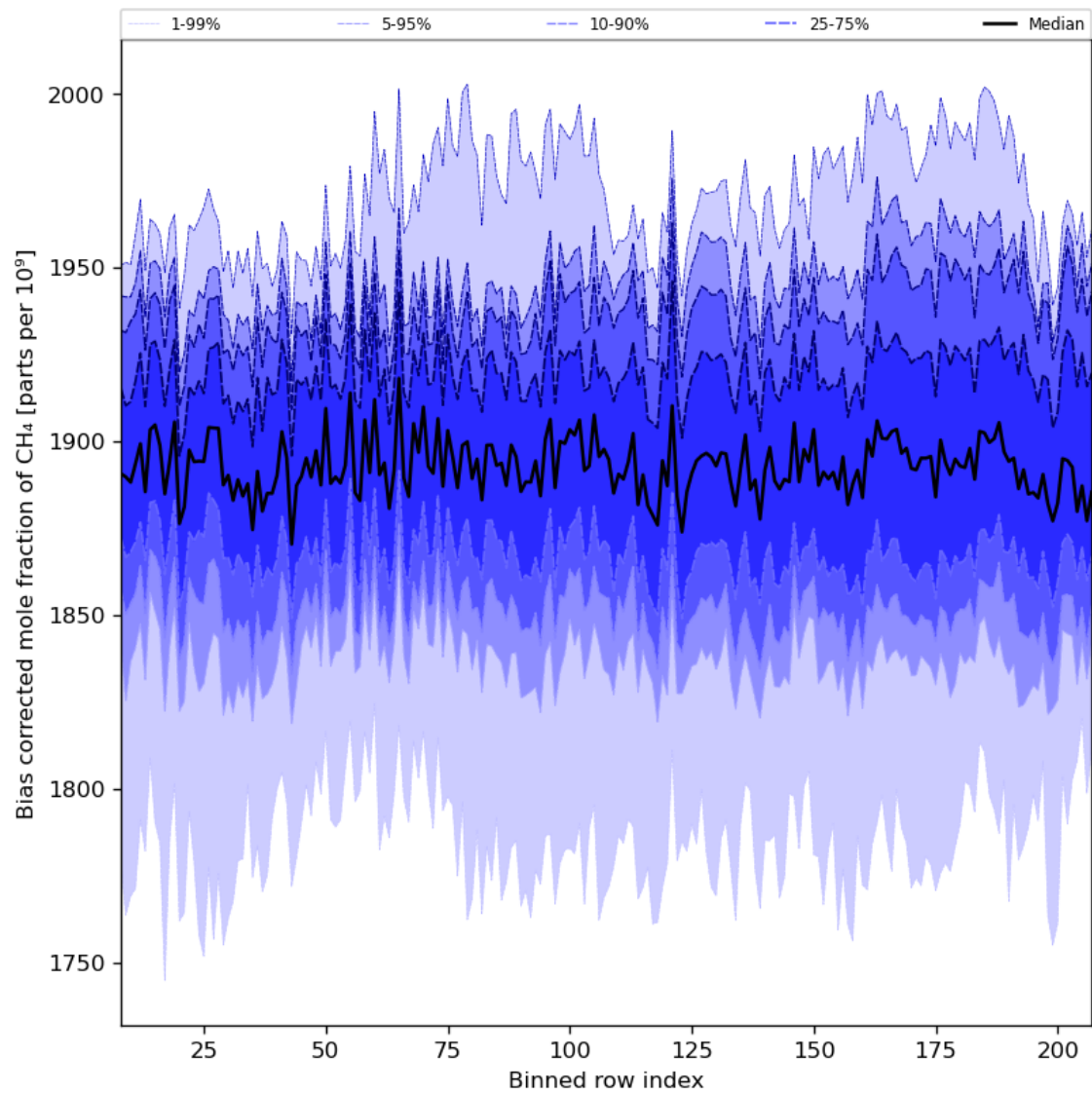
Figure 36: Along track statistics of “Bias corrected mole fraction of CH 4 ” for 2024-08-21 to 2024-08-22
