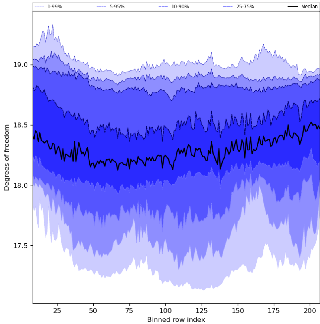
Figure 41: Along track statistics of “Degrees of freedom” for 2024-08-21 to 2024-08-22
