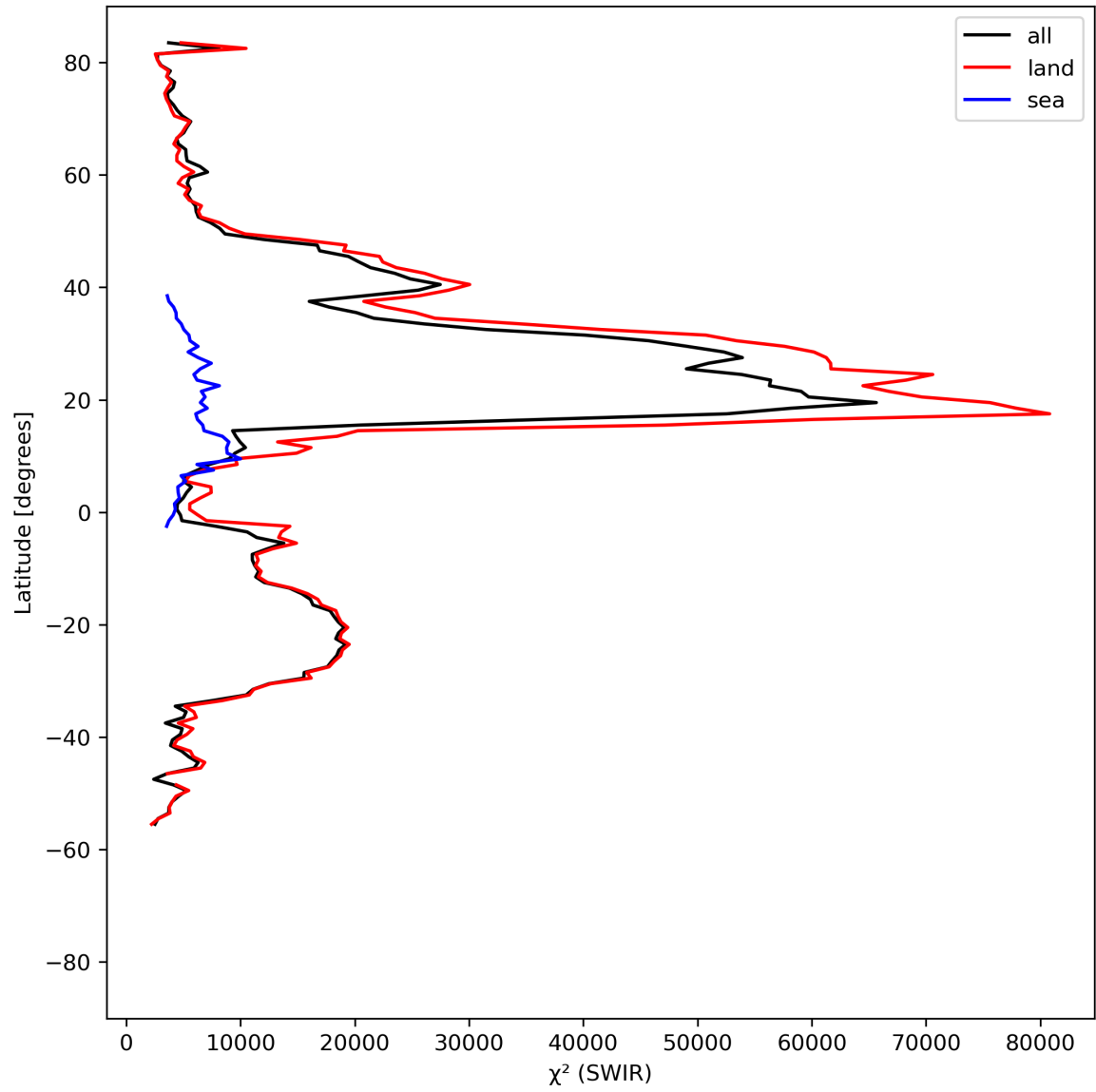
Figure 17: Zonal average of “ \chi^2 (SWIR)” for 2024-08-21 to 2024-08-22.
