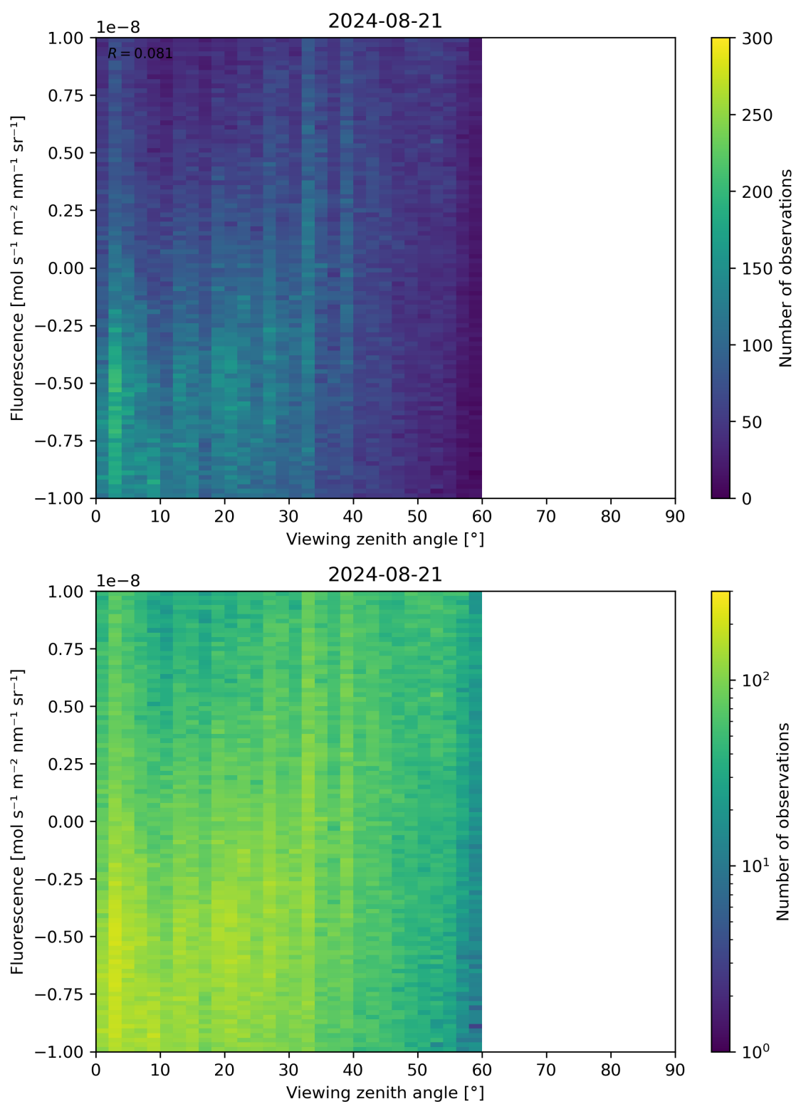
Figure 108: Scatter density plot of “Viewing zenith angle” against “Fluorescence” for 2024-08-21 to 2024-08-22.
