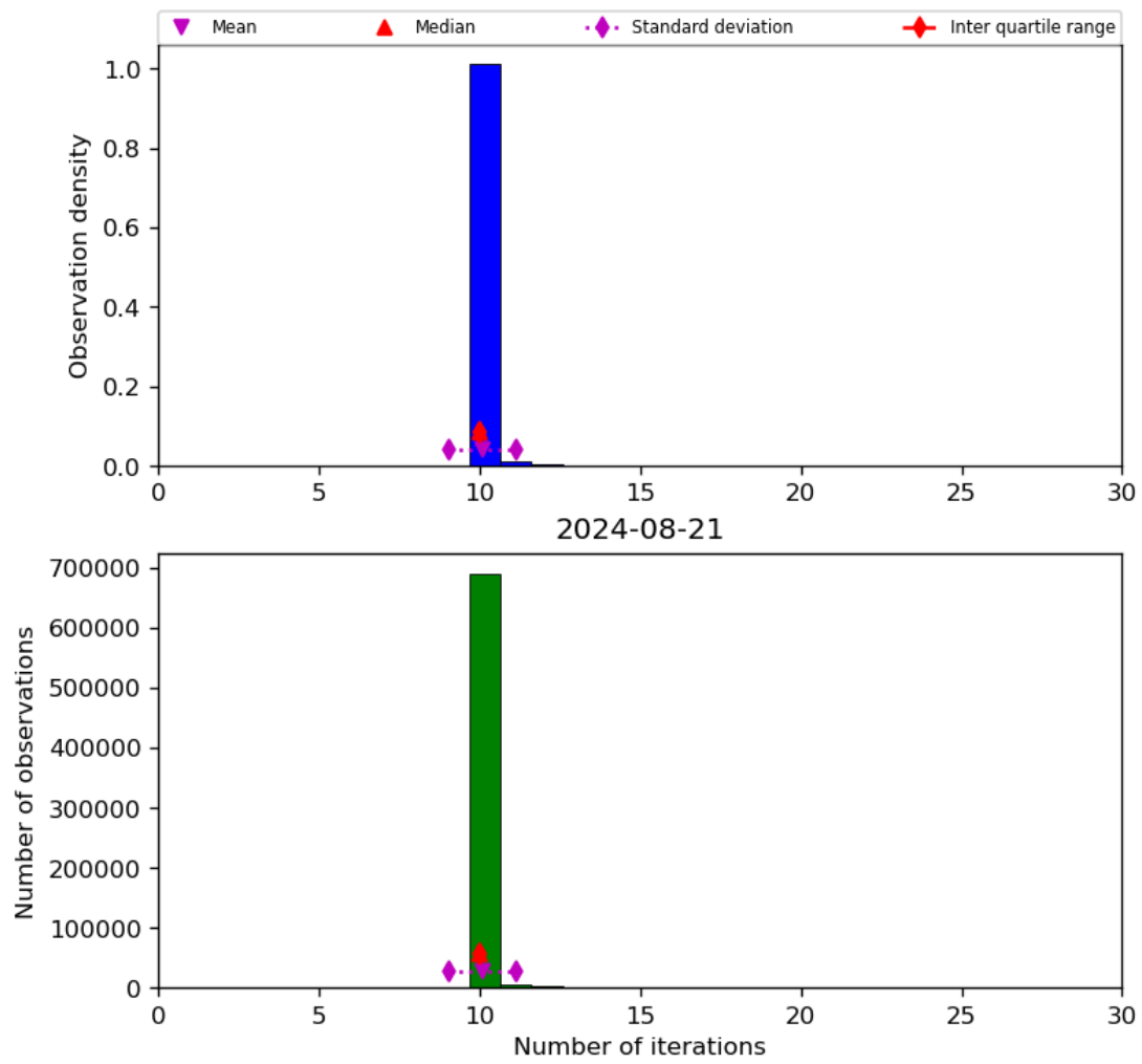
Figure 31: Histogram of “Number of iterations” for 2024-08-21 to 2024-08-22
