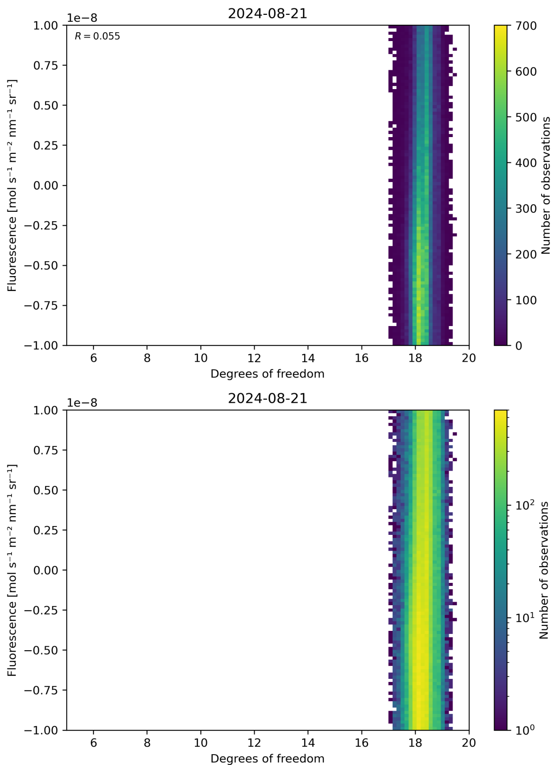
Figure 51: Scatter density plot of “Degrees of freedom” against “Fluorescence” for 2024-08-21 to 2024-08-22.
