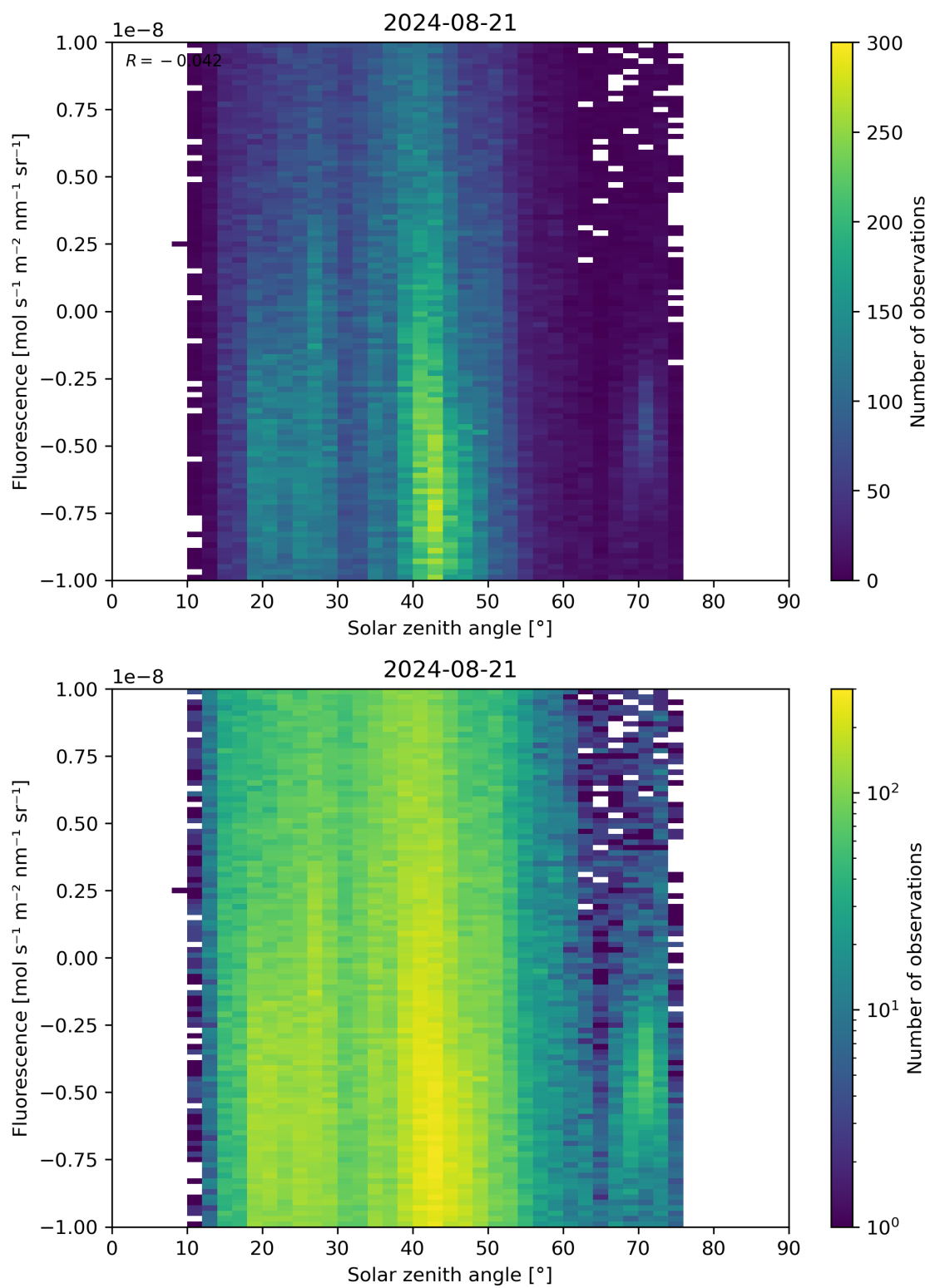
Figure 97: Scatter density plot of “Solar zenith angle” against “Fluorescence” for 2024-08-21 to 2024-08-22.
