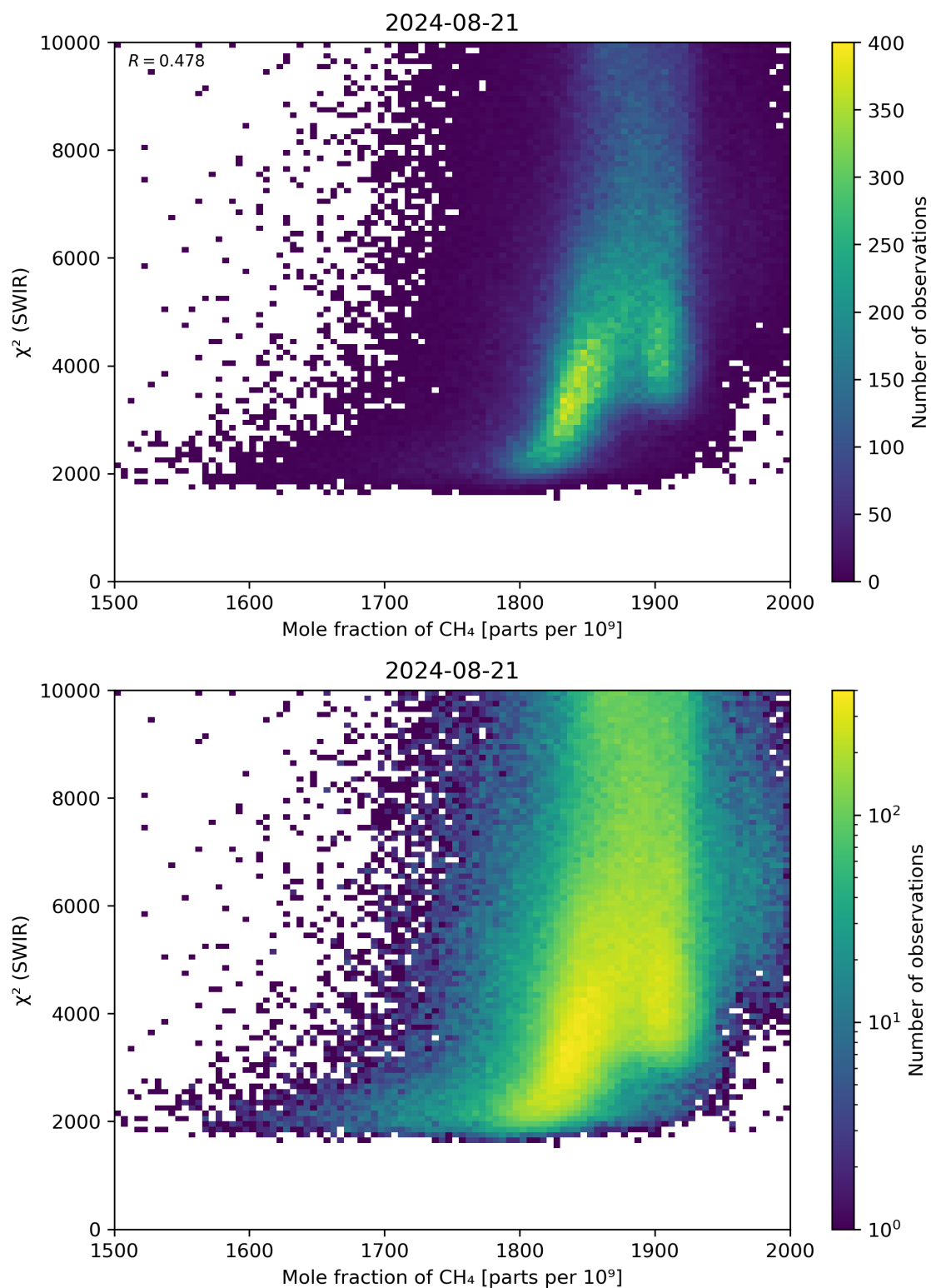
Figure 71: Scatter density plot of “Mole fraction of \text{CH}_4 ” against “ \chi^2 (SWIR)” for 2024-08-21 to 2024-08-22.
