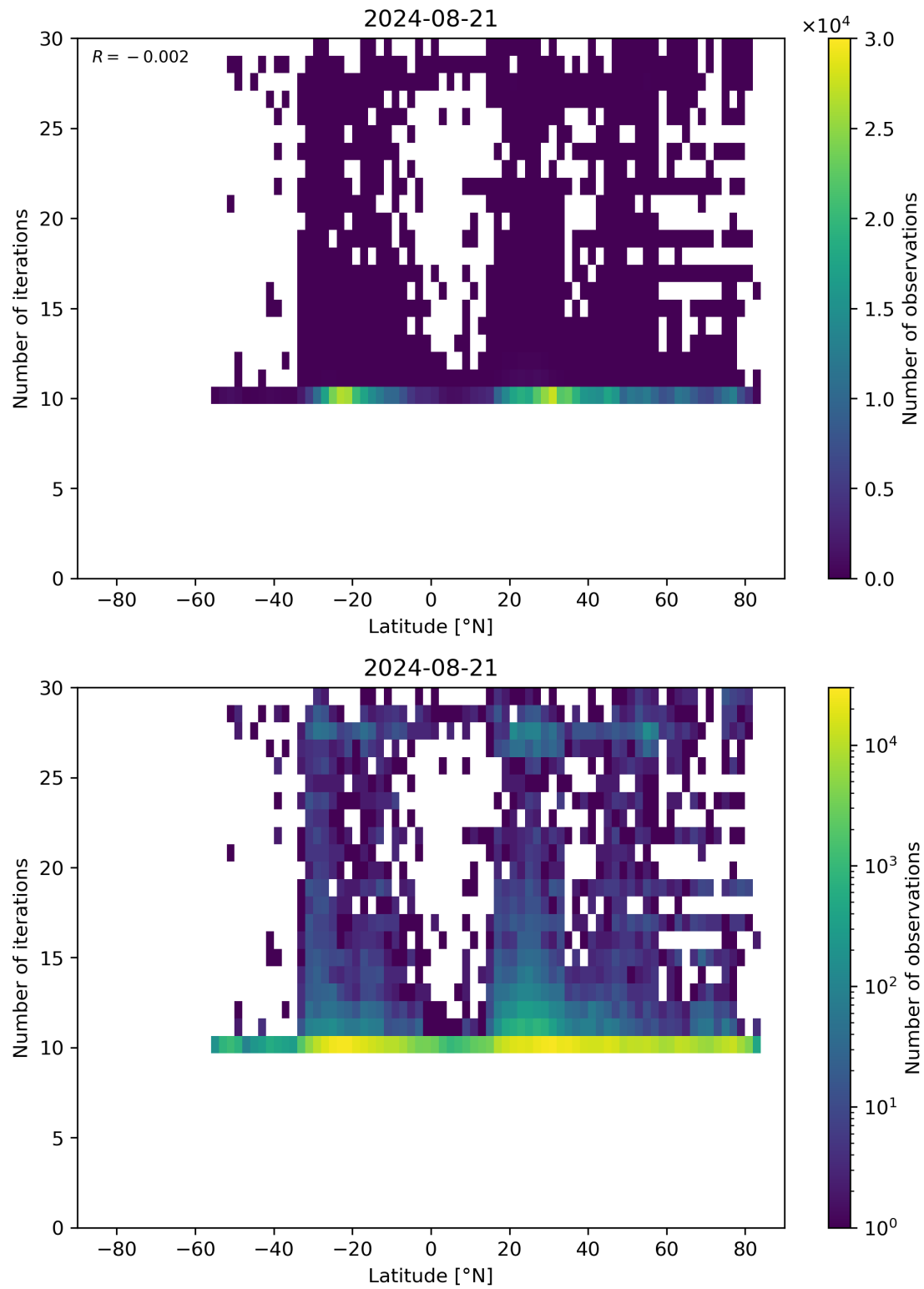
Figure 60: Scatter density plot of “Latitude” against “Number of iterations” for 2024-08-21 to 2024-08-22.
