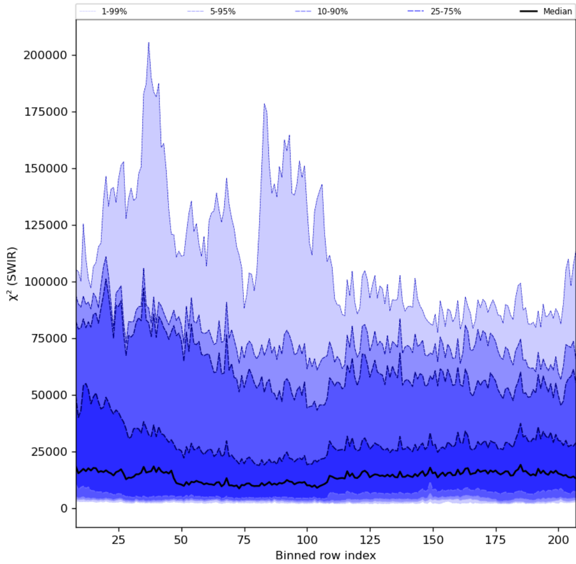
Figure 39: Along track statistics of “ \chi^2 (SWIR)” for 2024-08-21 to 2024-08-22
