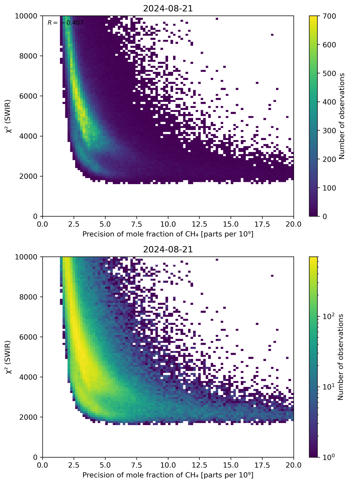
Figure 79: Scatter density plot of “Precision of mole fraction of \text{CH}_4 ” against “ \chi^2 (SWIR)” for 2024-08-21 to 2024-08-22.
