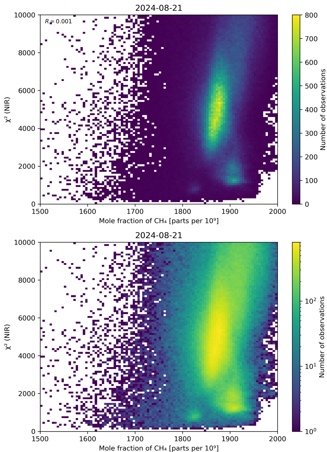
Figure 70: Scatter density plot of “Mole fraction of CH 4 ” against “ \chi^2 (NIR)” for 2024-08-21 to 2024-08-22.
