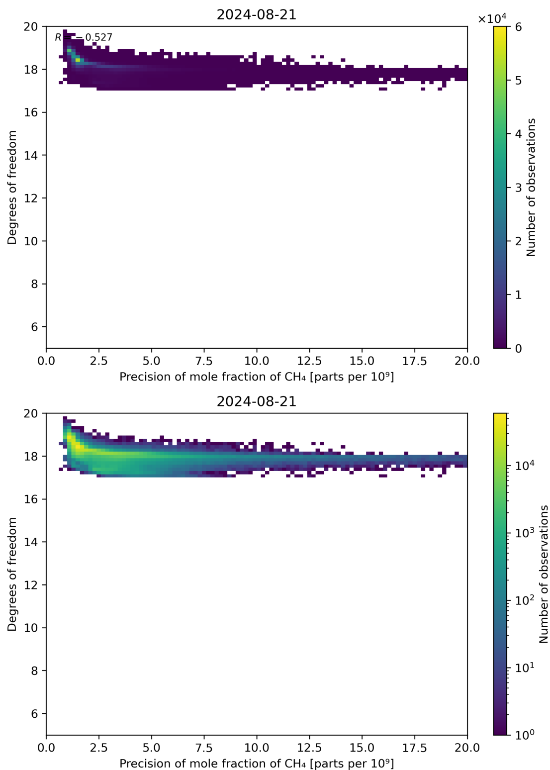
Figure 80: Scatter density plot of “Precision of mole fraction of CH 4 ” against “Degrees of freedom” for 2024-08-21 to 2024-08-22.
