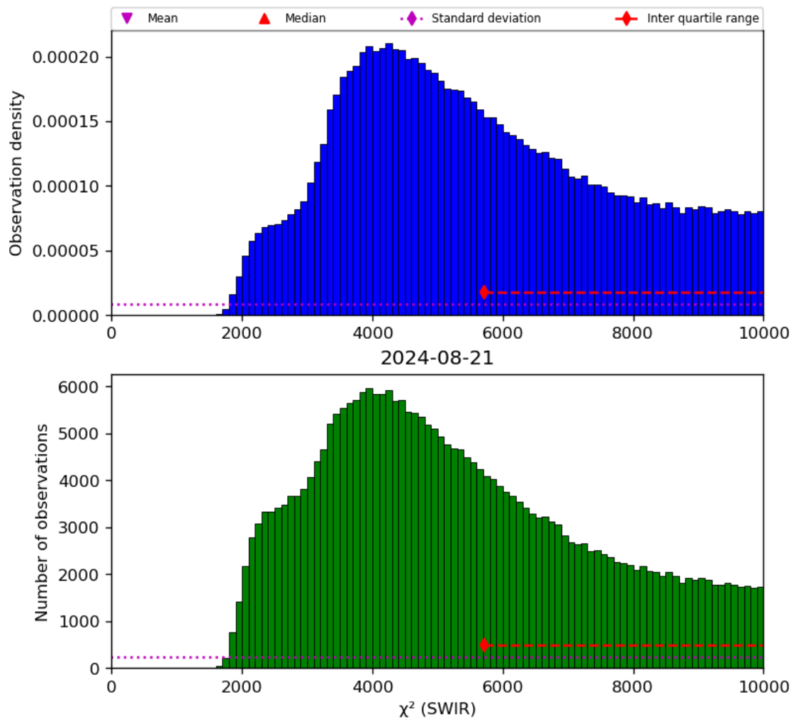
Figure 28: Histogram of “ \chi^2 (SWIR)” for 2024-08-21 to 2024-08-22
