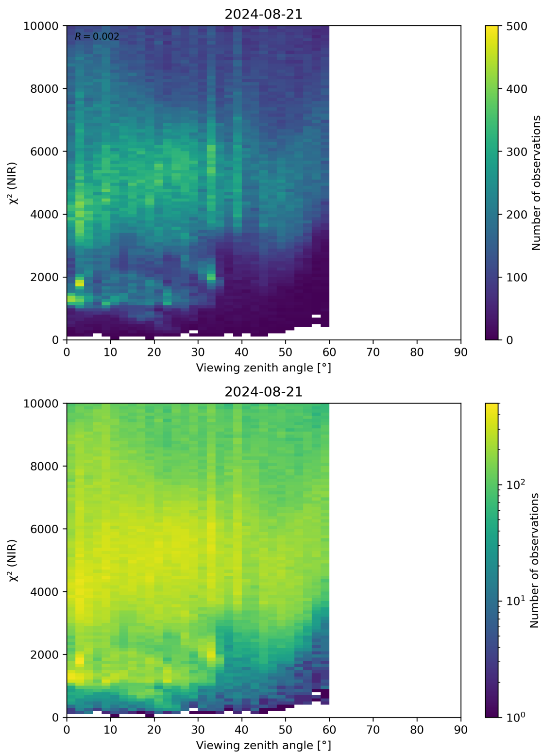
Figure 105: Scatter density plot of “Viewing zenith angle” against “ \chi^2 (NIR)” for 2024-08-21 to 2024-08-22.
