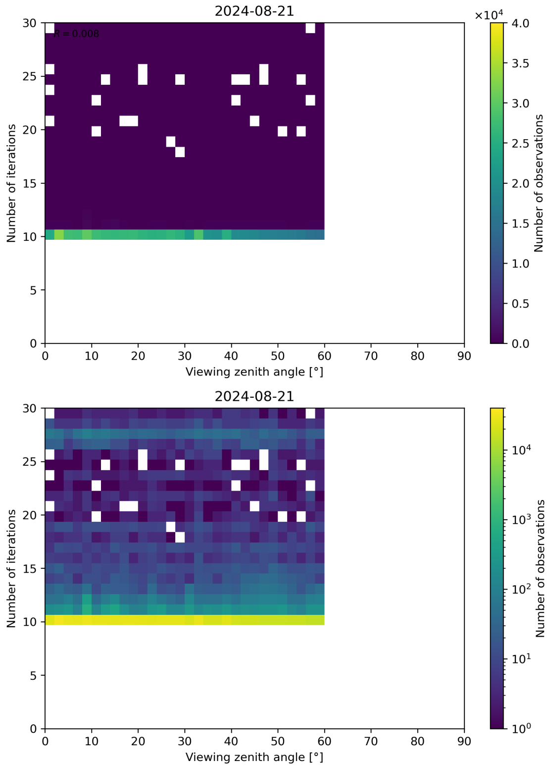
Figure 113: Scatter density plot of “Viewing zenith angle” against “Number of iterations” for 2024-08-21 to 2024-08-22.
