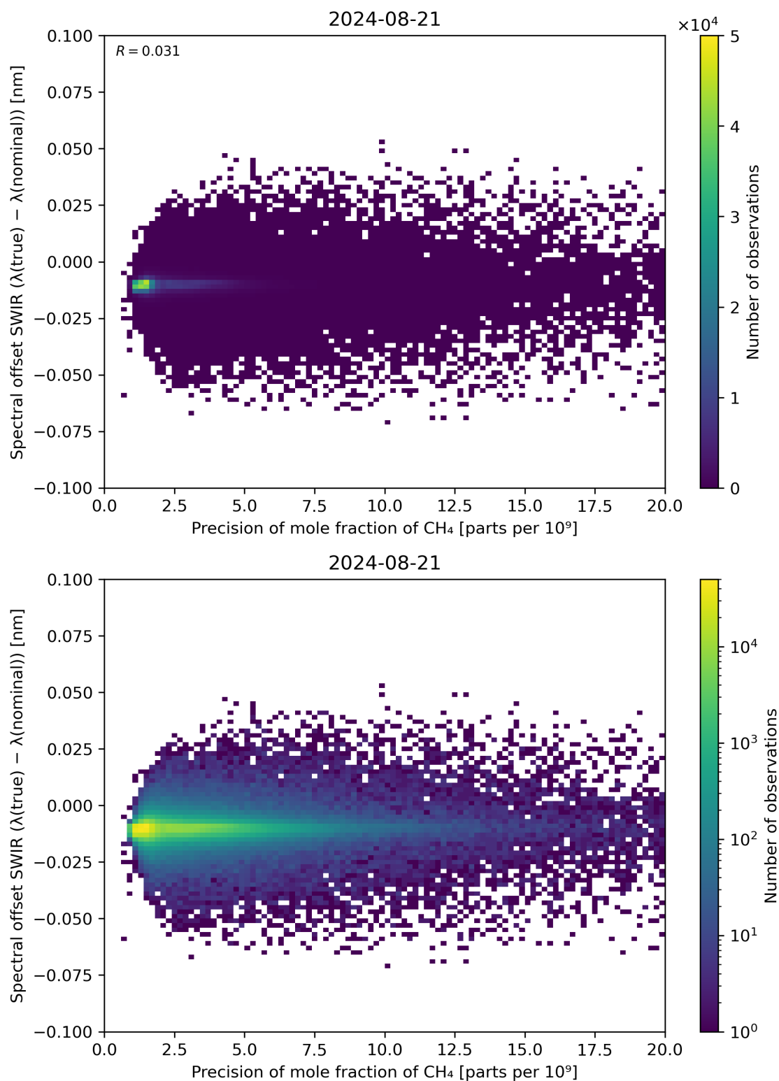
Figure 85: Scatter density plot of “Precision of mole fraction of CH 4 ” against “Spectral offset SWIR ( \lambda(\text{true}) - \lambda(\text{nominal}) )” for 2024-08-21 to 2024-08-22.
