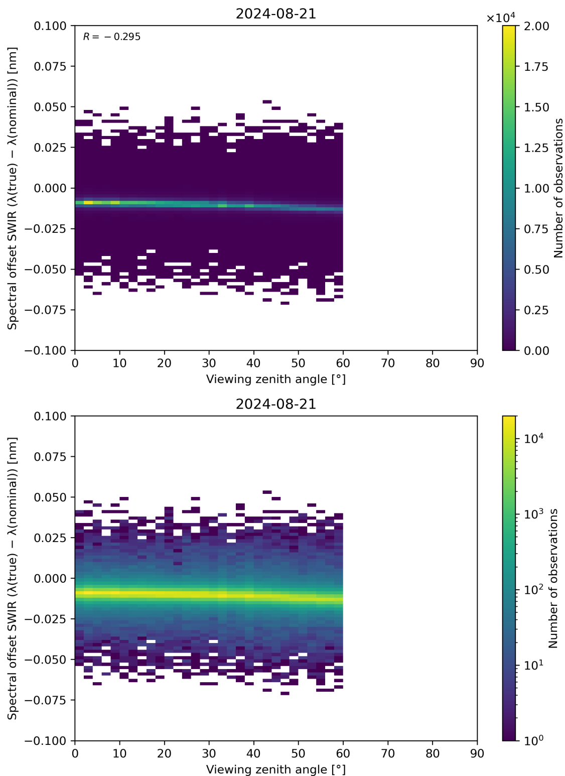
Figure 116: Scatter density plot of “Viewing zenith angle” against “Spectral offset SWIR ( \lambda(\text{true}) - \lambda(\text{nominal}) )” for 2024-08-21 to 2024-08-22.
