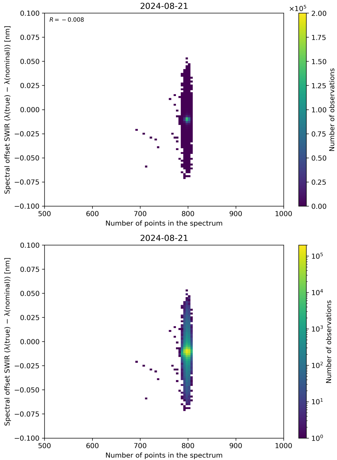
Figure 93: Scatter density plot of “Number of points in the spectrum” against “Spectral offset SWIR ( \lambda(\text{true}) - \lambda(\text{nominal}) )” for 2024-08-21 to 2024-08-22.
