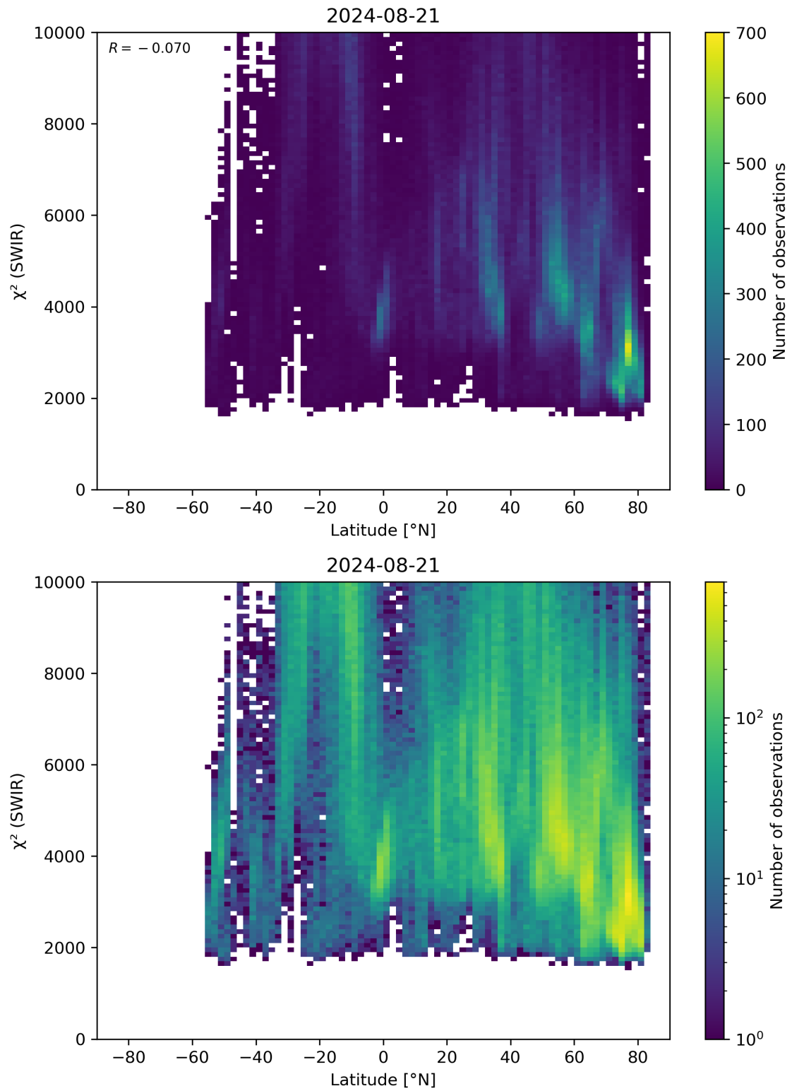
Figure 54: Scatter density plot of “Latitude” against “ \chi^2 (SWIR)” for 2024-08-21 to 2024-08-22.
