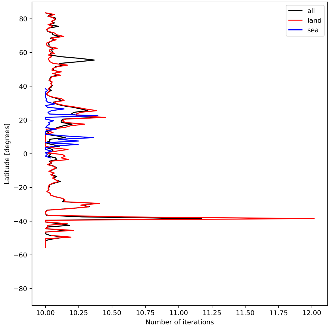
Figure 20: Zonal average of “Number of iterations” for 2024-08-21 to 2024-08-22.
