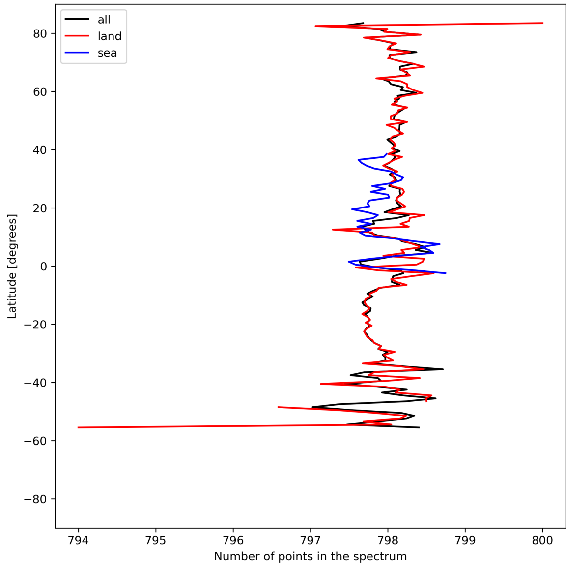
Figure 15: Zonal average of “Number of points in the spectrum” for 2024-08-21 to 2024-08-22.
