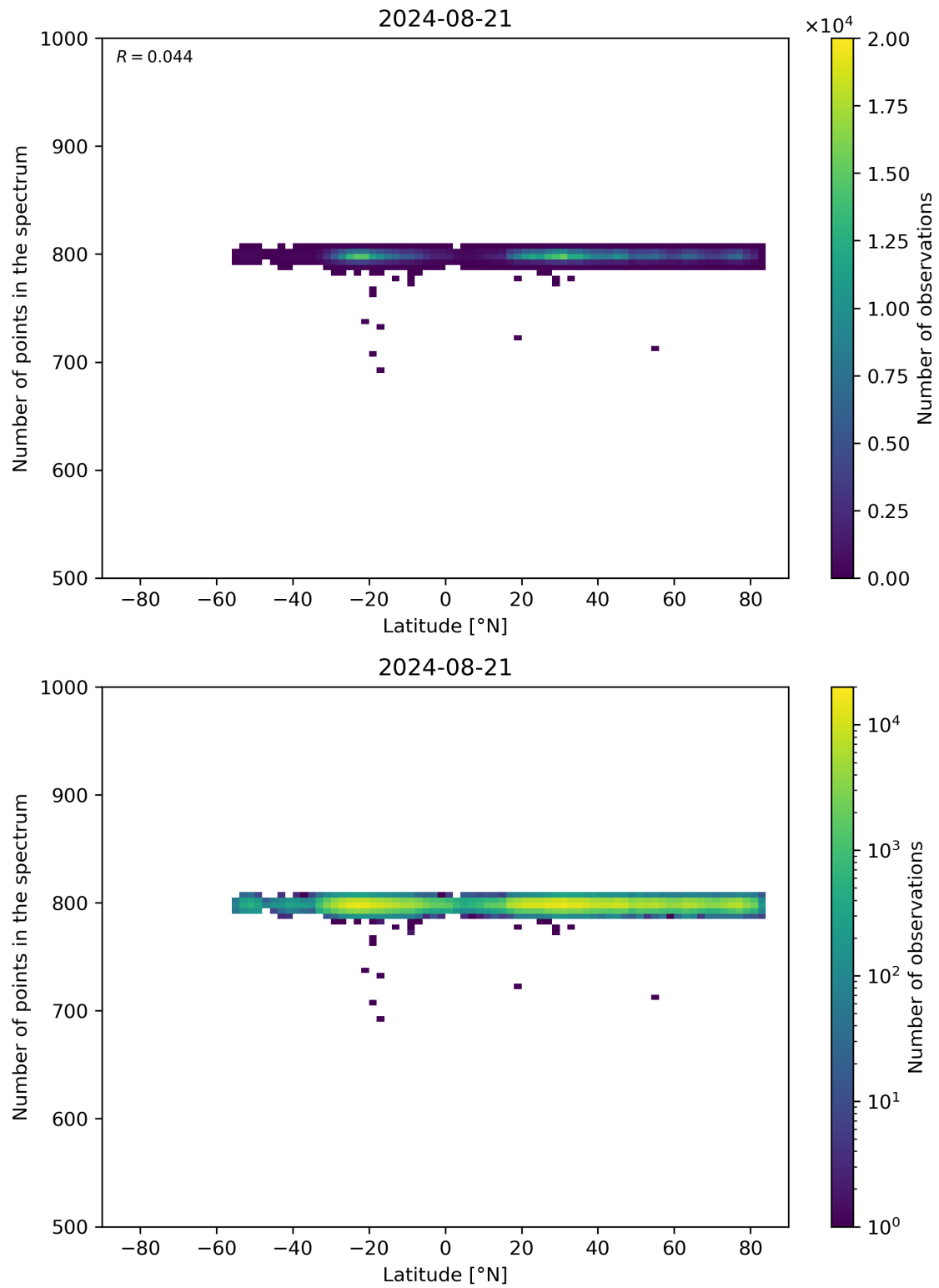
Figure 61: Scatter density plot of “Latitude” against “Number of points in the spectrum” for 2024-08-21 to 2024-08-22.
