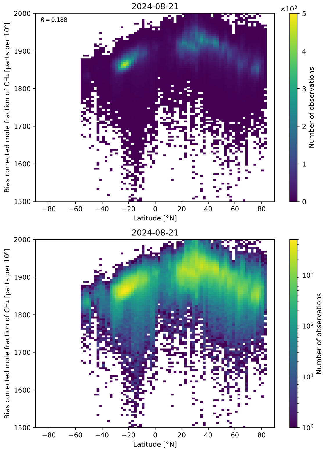
Figure 58: Scatter density plot of “Latitude” against “Bias corrected mole fraction of CH 4 ” for 2024-08-21 to 2024-08-22.
