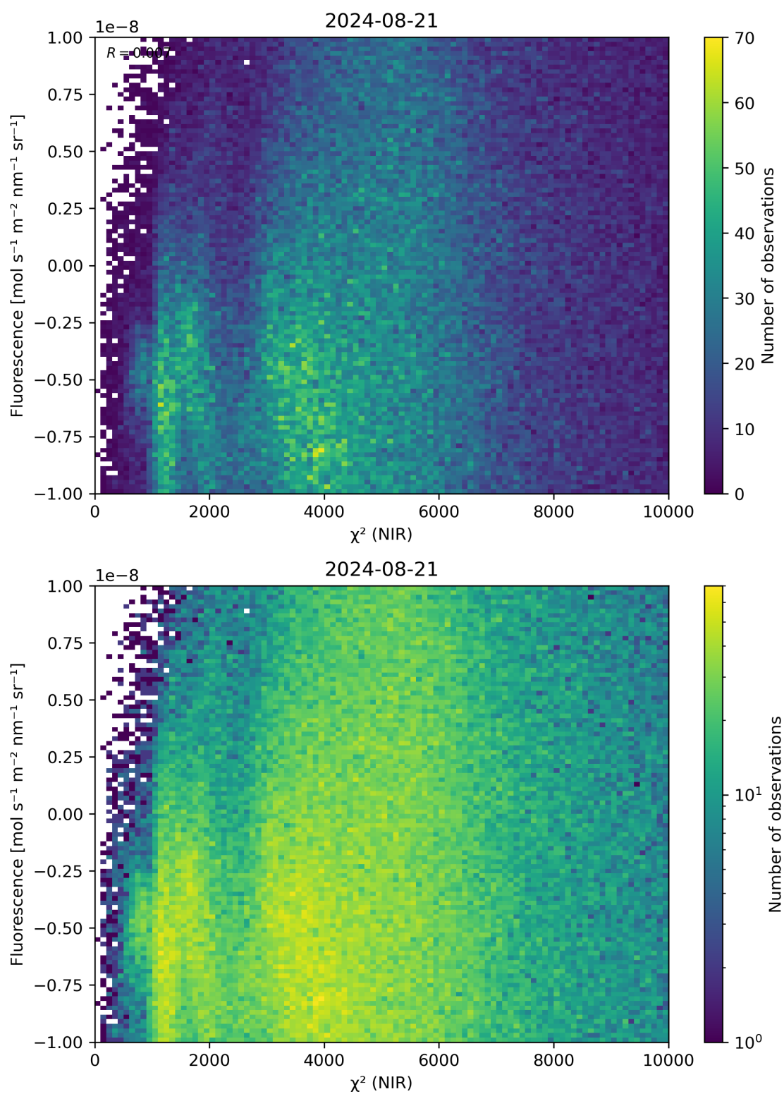
Figure 45: Scatter density plot of “ \chi^2 (NIR)” against “Fluorescence” for 2024-08-21 to 2024-08-22.
