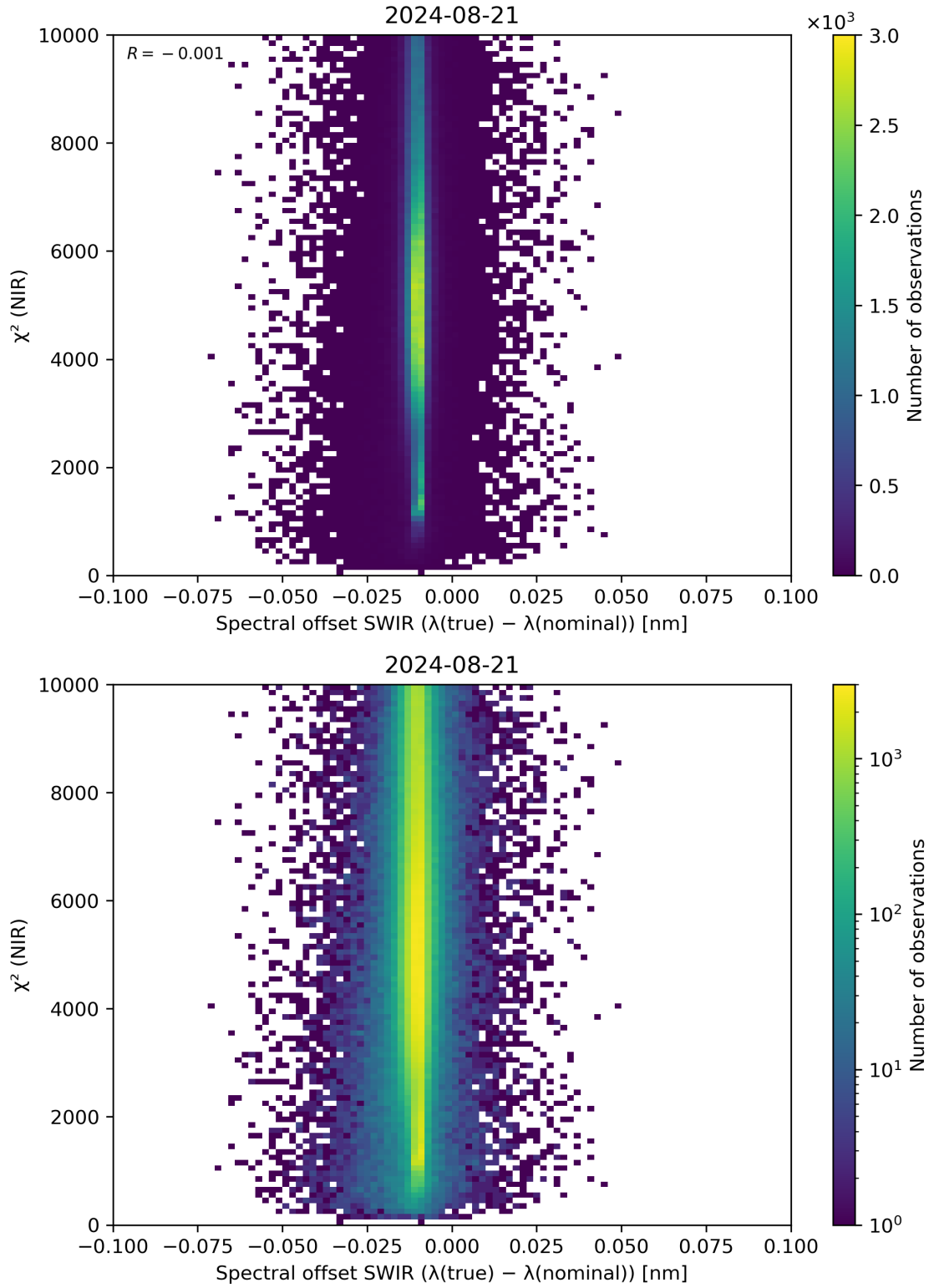
Figure 117: Scatter density plot of “Spectral offset SWIR ( \lambda(\text{true}) - \lambda(\text{nominal}) )” against “ \chi^2 (NIR)” for 2024-08-21 to 2024-08-22.
