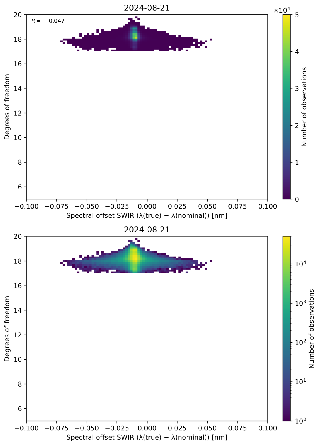
Figure 119: Scatter density plot of “Spectral offset SWIR ( \lambda(\text{true}) - \lambda(\text{nominal}) )” against “Degrees of freedom” for 2024-08-21 to 2024-08-22.
