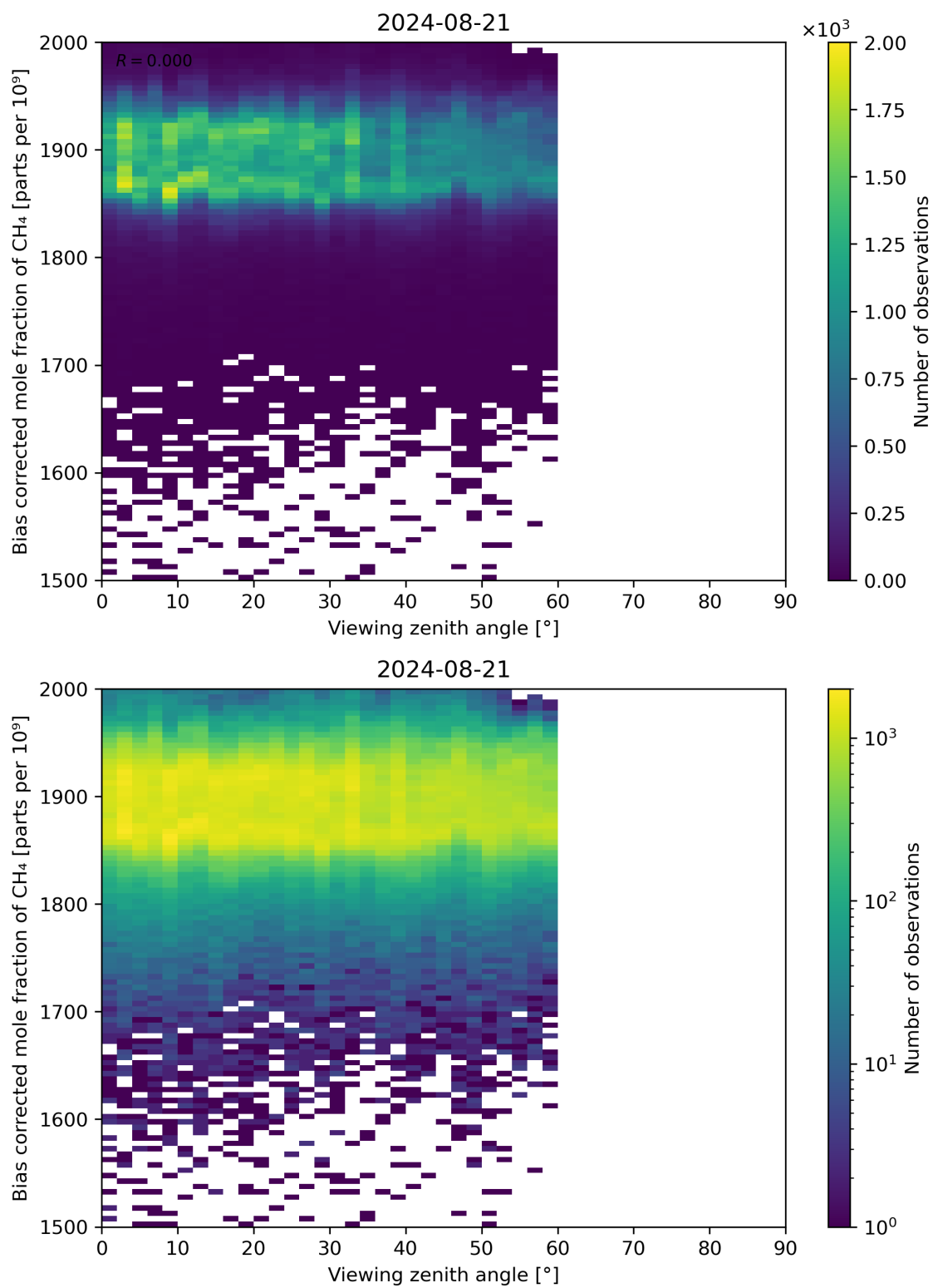
Figure 111: Scatter density plot of “Viewing zenith angle” against “Bias corrected mole fraction of CH 4 ” for 2024-08-21 to 2024-08-22.
