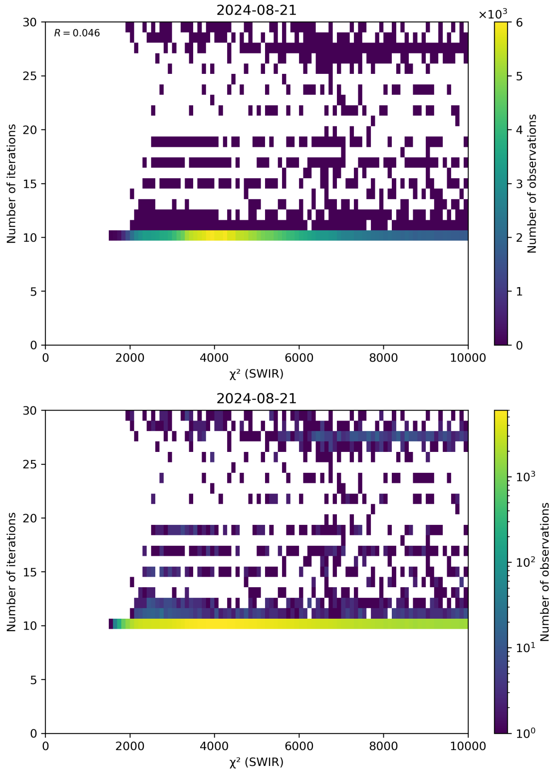
Figure 50: Scatter density plot of “ \chi^2 (SWIR)” against “Number of iterations” for 2024-08-21 to 2024-08-22.
