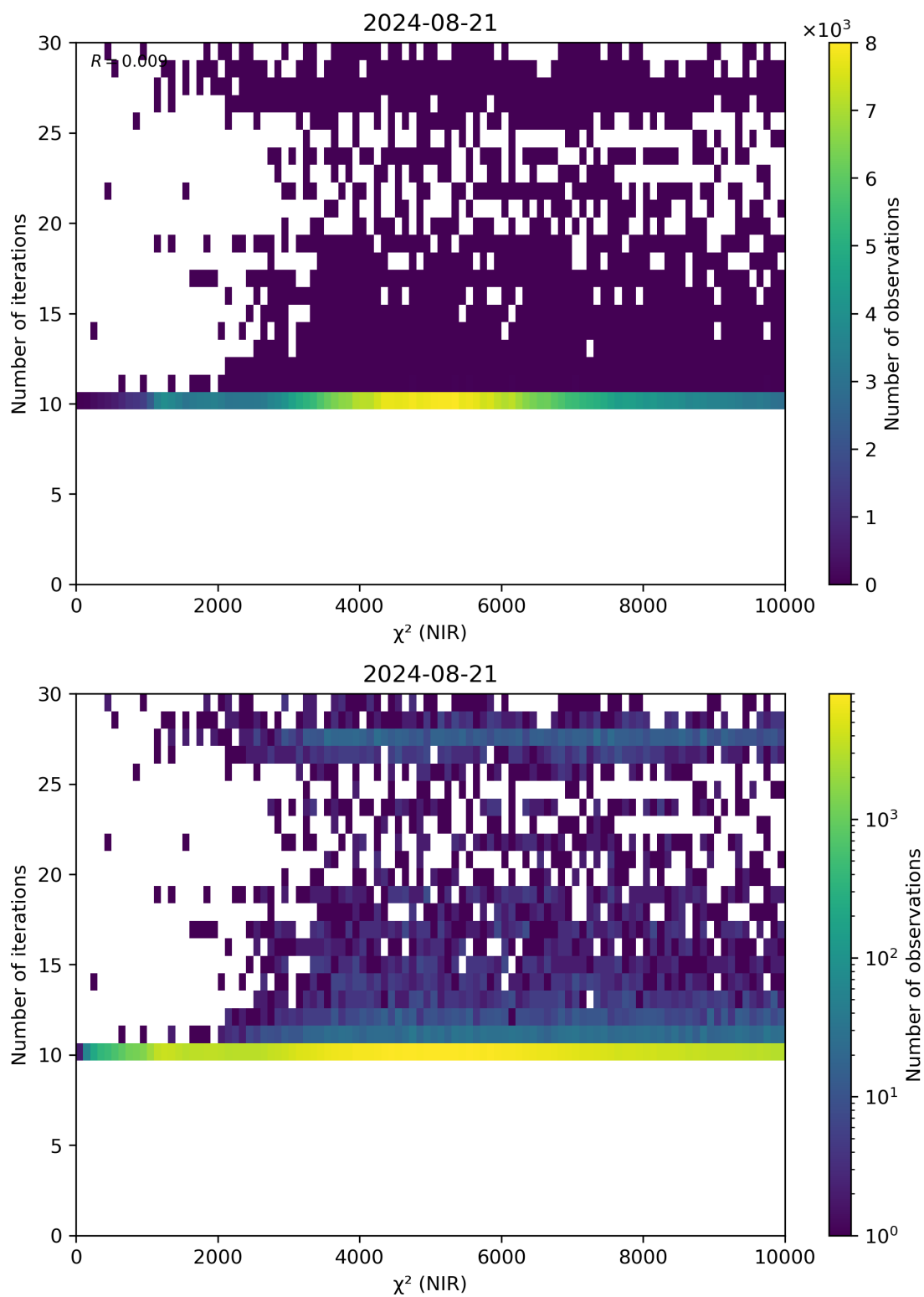
Figure 46: Scatter density plot of “ \chi^2 (NIR)” against “Number of iterations” for 2024-08-21 to 2024-08-22.
