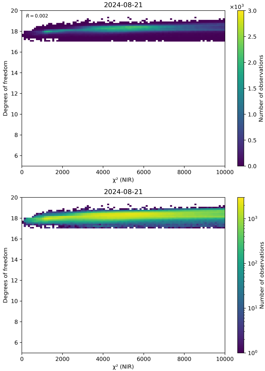
Figure 44: Scatter density plot of “ \chi^2 (NIR)” against “Degrees of freedom” for 2024-08-21 to 2024-08-22.
