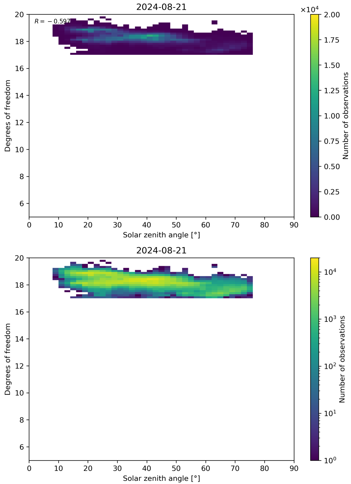
Figure 96: Scatter density plot of “Solar zenith angle” against “Degrees of freedom” for 2024-08-21 to 2024-08-22.
