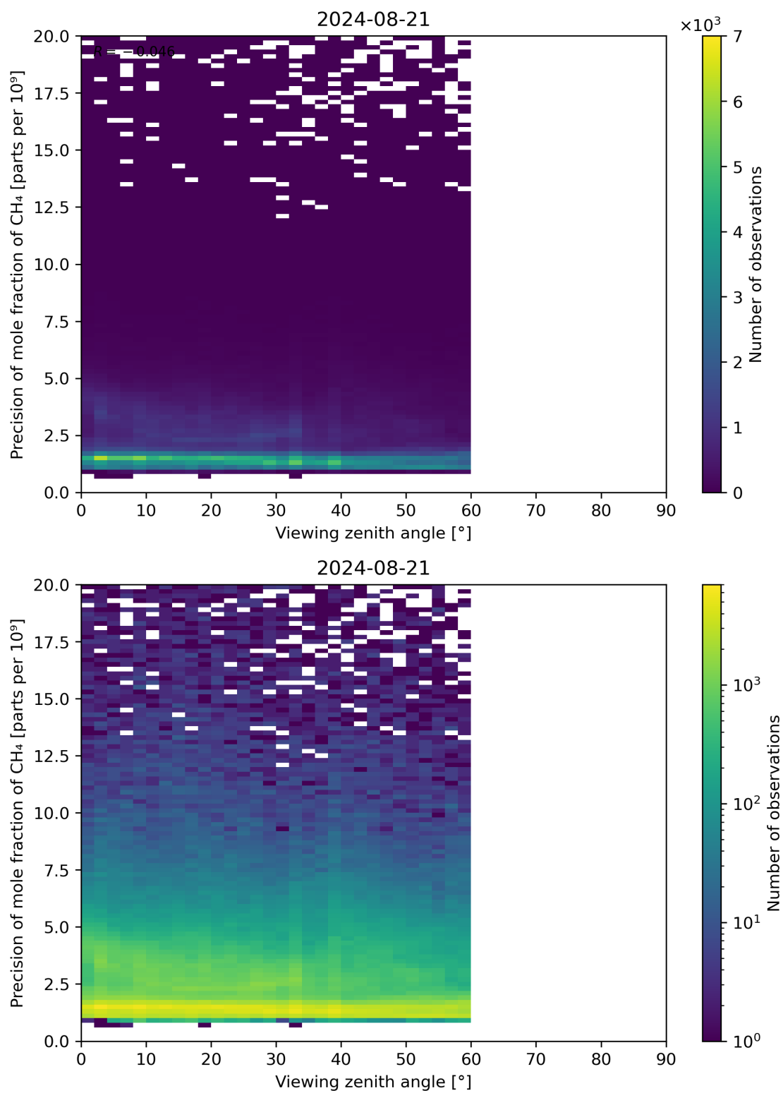
Figure 112: Scatter density plot of “Viewing zenith angle” against “Precision of mole fraction of \text{CH}_4 ” for 2024-08-21 to 2024-08-22.
