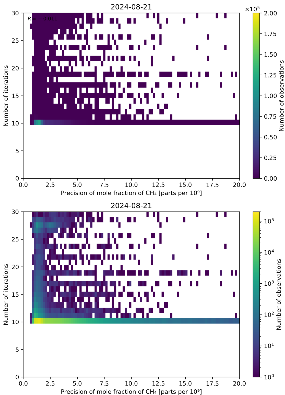
Figure 83: Scatter density plot of “Precision of mole fraction of CH 4 ” against “Number of iterations” for 2024-08-21 to 2024-08-22.
