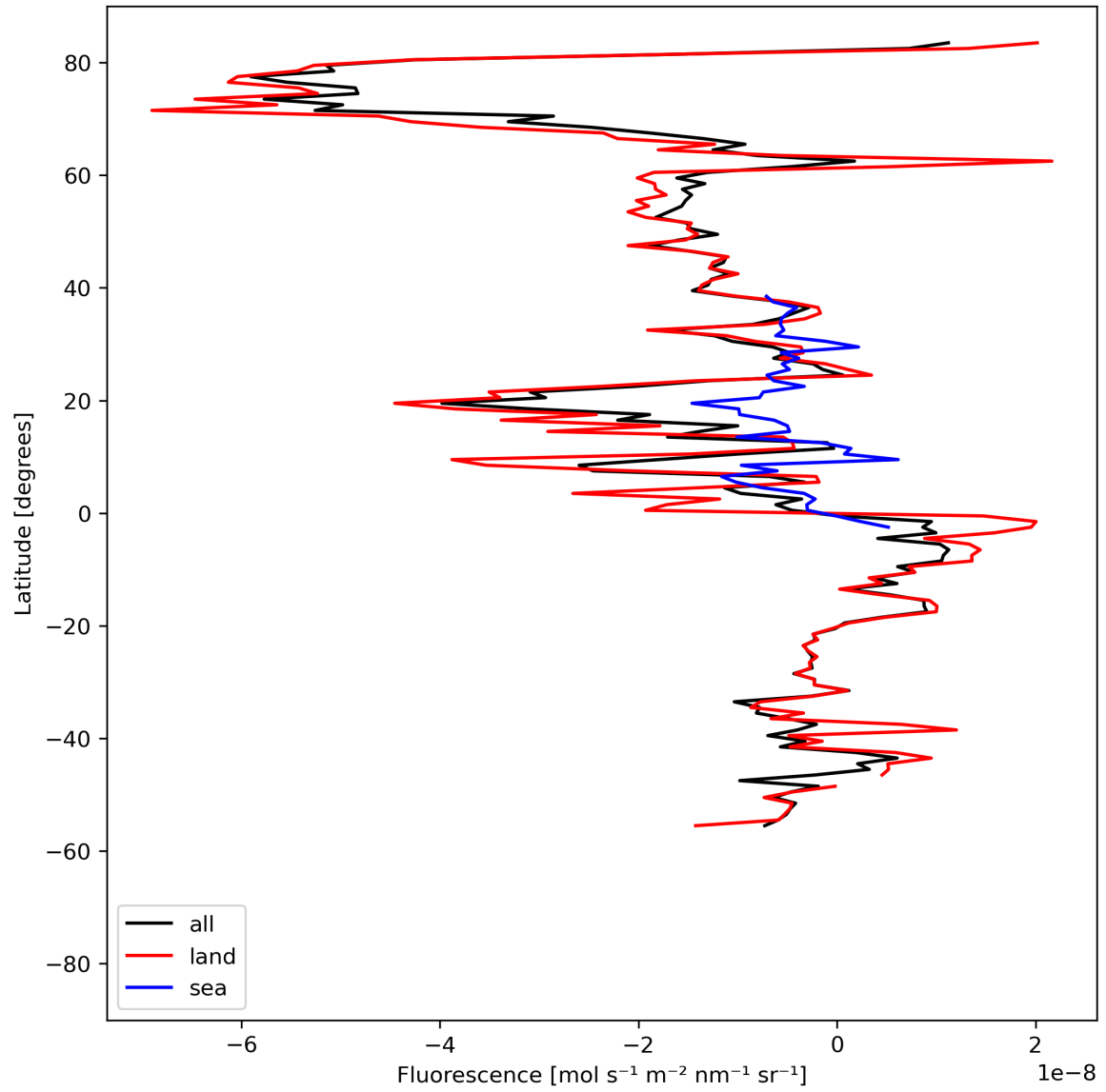
Figure 21: Zonal average of “Fluorescence” for 2024-08-21 to 2024-08-22.
