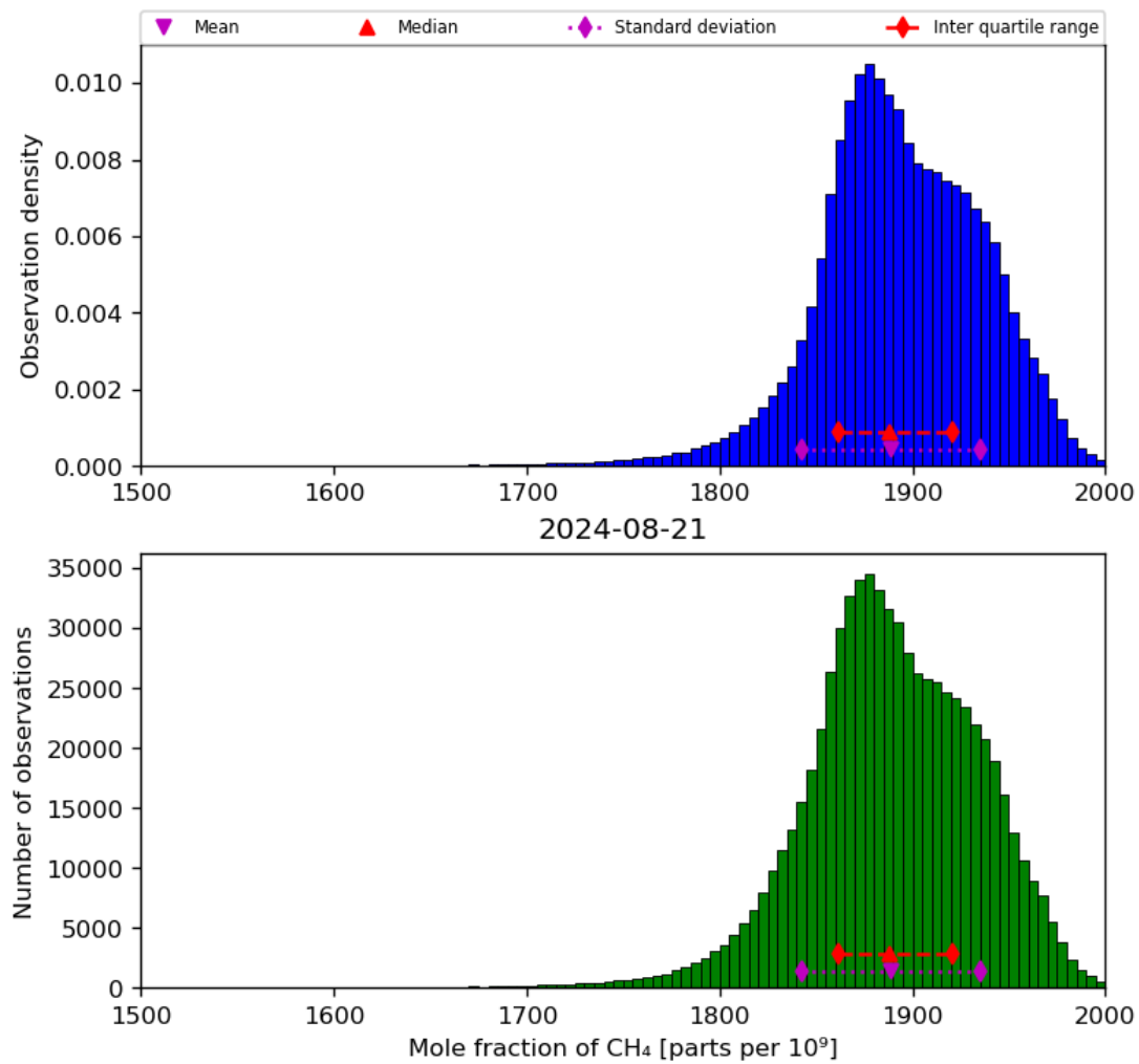
Figure 23: Histogram of “Mole fraction of CH 4 ” for 2024-08-21 to 2024-08-22
