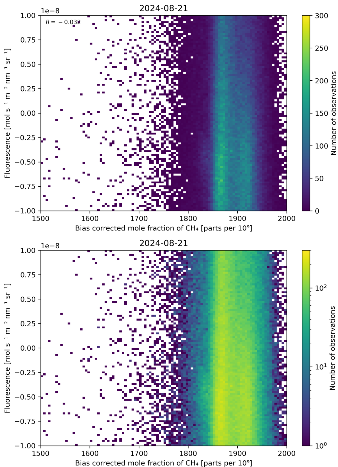
Figure 66: Scatter density plot of “Bias corrected mole fraction of CH 4 ” against “Fluorescence” for 2024-08-21 to 2024-08-22.
