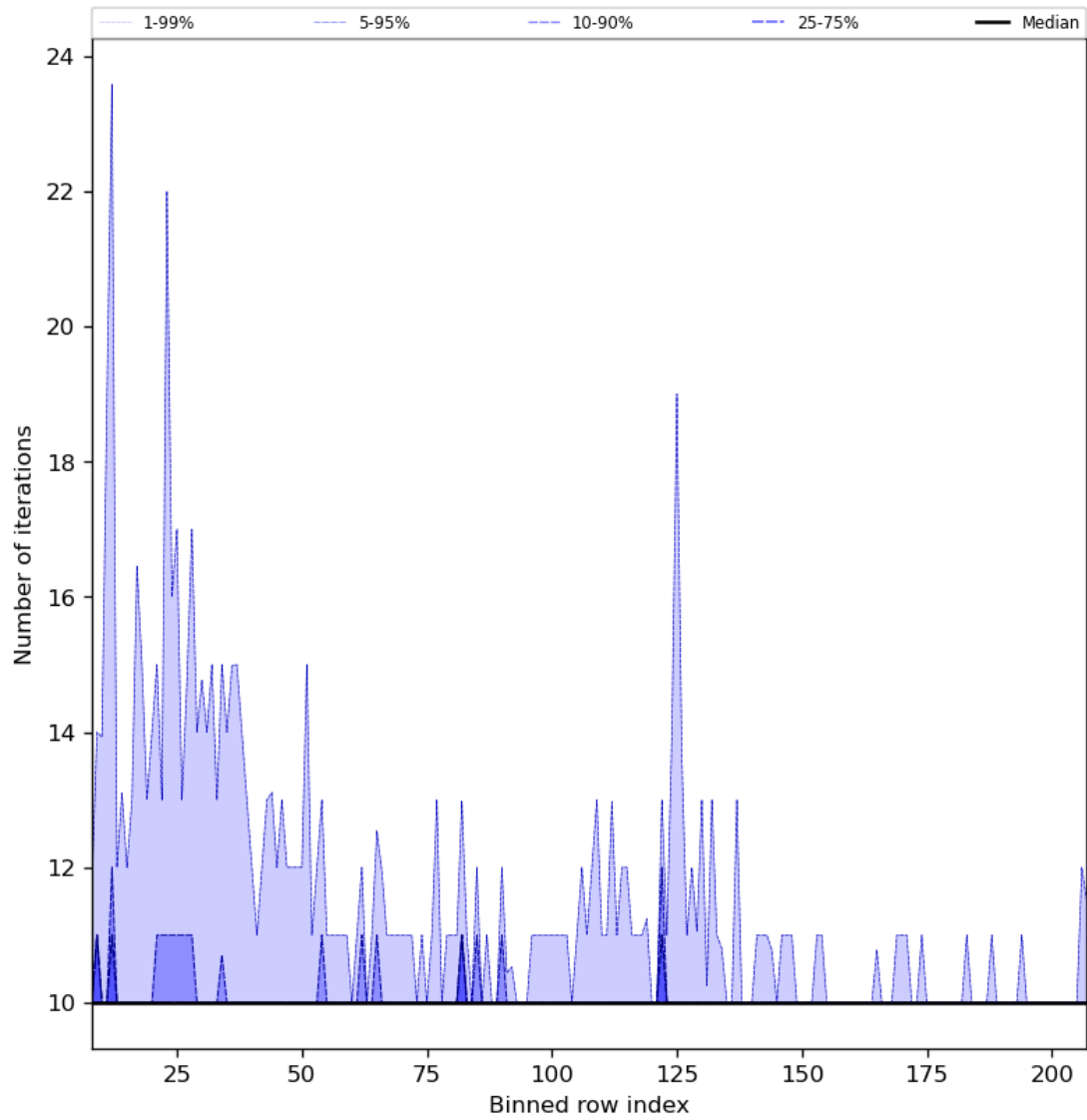
Figure 42: Along track statistics of “Number of iterations” for 2024-08-21 to 2024-08-22
