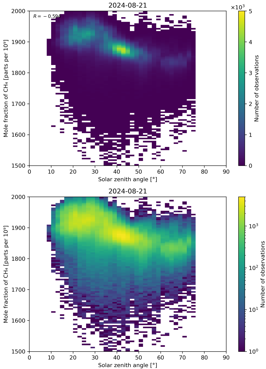
Figure 99: Scatter density plot of “Solar zenith angle” against “Mole fraction of CH 4 ” for 2024-08-21 to 2024-08-22.
