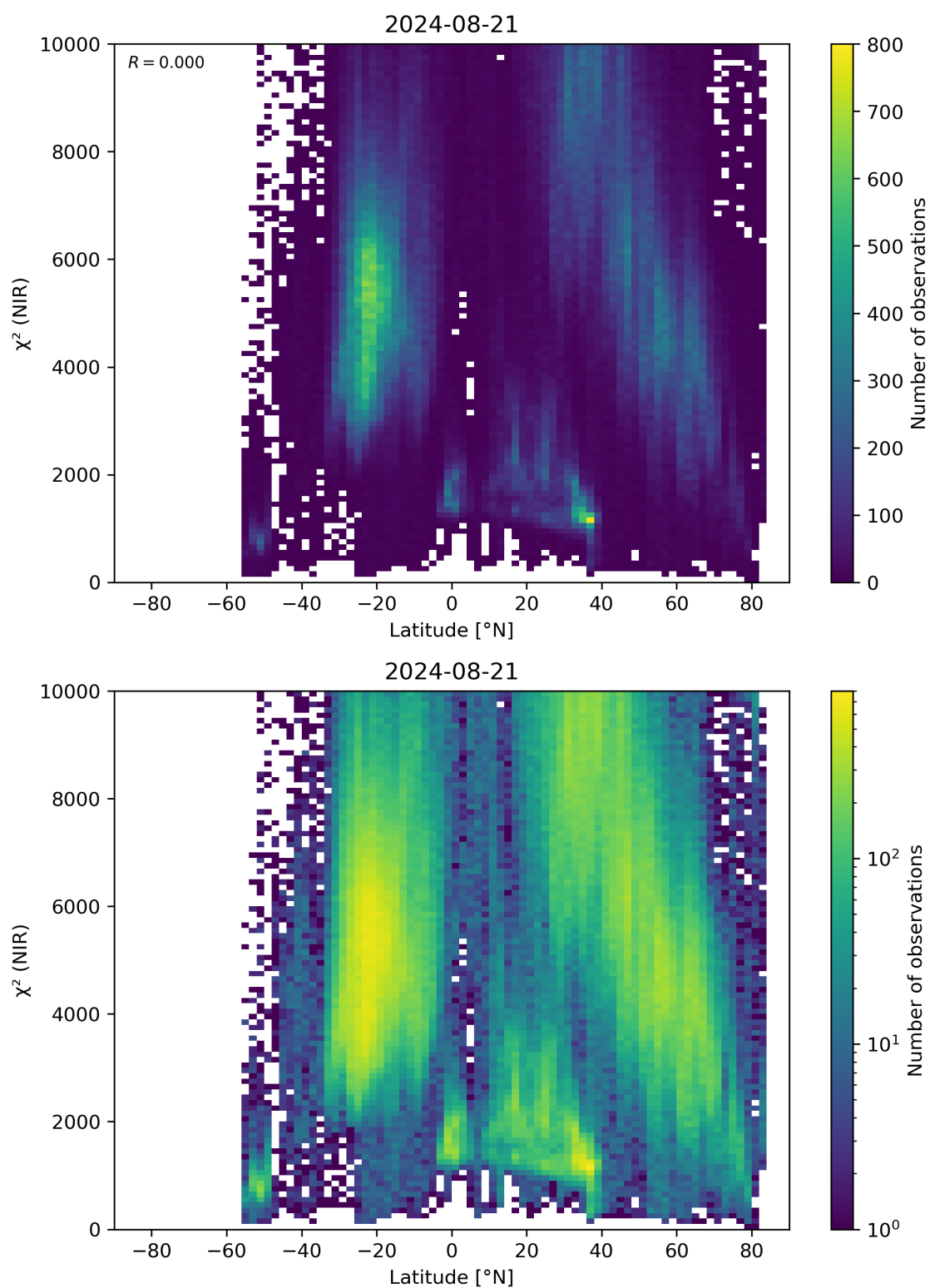
Figure 53: Scatter density plot of “Latitude” against “ \chi^2 (NIR)” for 2024-08-21 to 2024-08-22.
