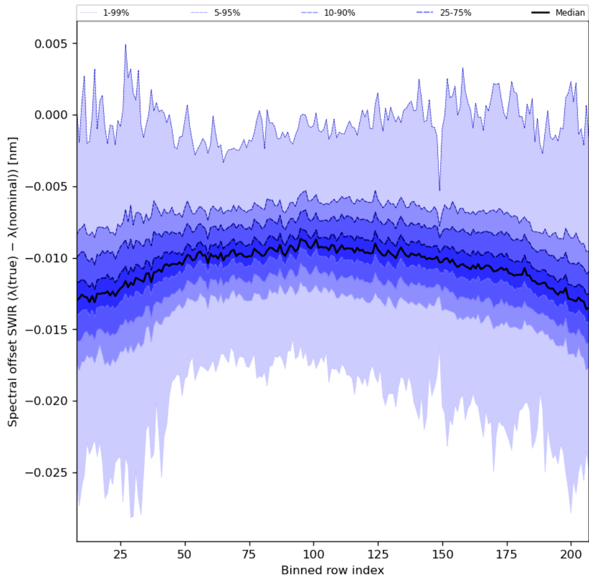
Figure 38: Along track statistics of “Spectral offset SWIR ( \lambda(\text{true}) - \lambda(\text{nominal}) )” for 2024-08-21 to 2024-08-22
