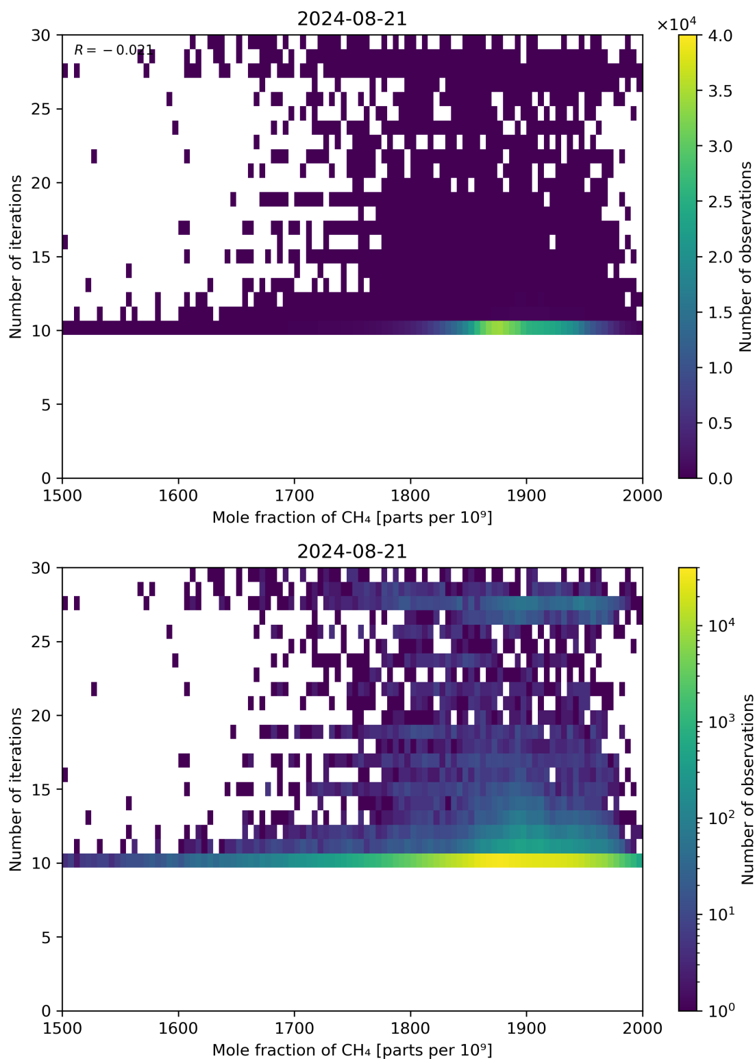
Figure 76: Scatter density plot of “Mole fraction of CH 4 ” against “Number of iterations” for 2024-08-21 to 2024-08-22.
