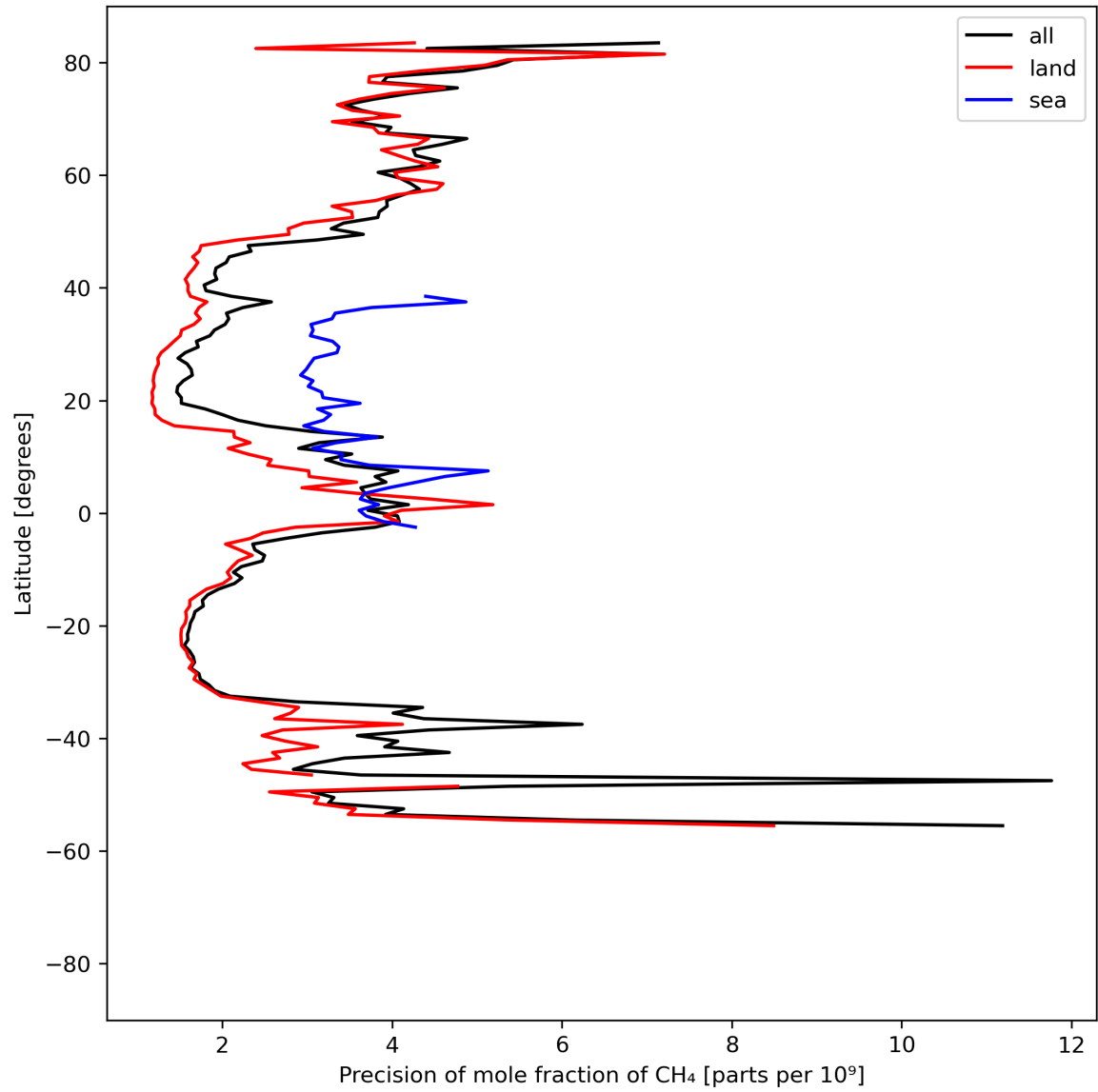
Figure 13: Zonal average of “Precision of mole fraction of \text{CH}_4 ” for 2024-08-21 to 2024-08-22.
