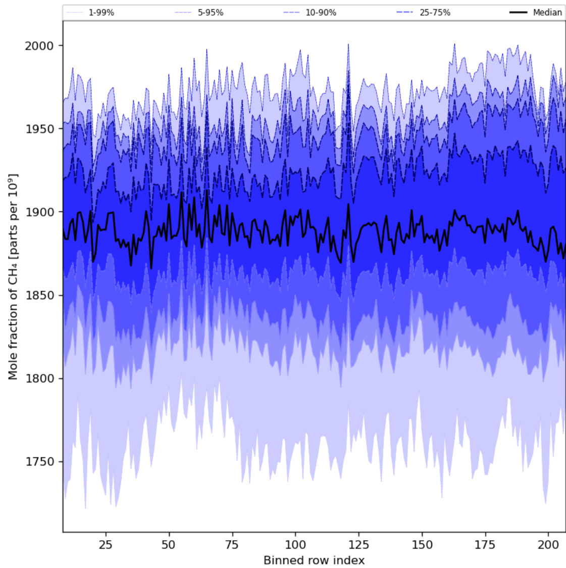
Figure 34: Along track statistics of “Mole fraction of CH 4 ” for 2024-08-21 to 2024-08-22
