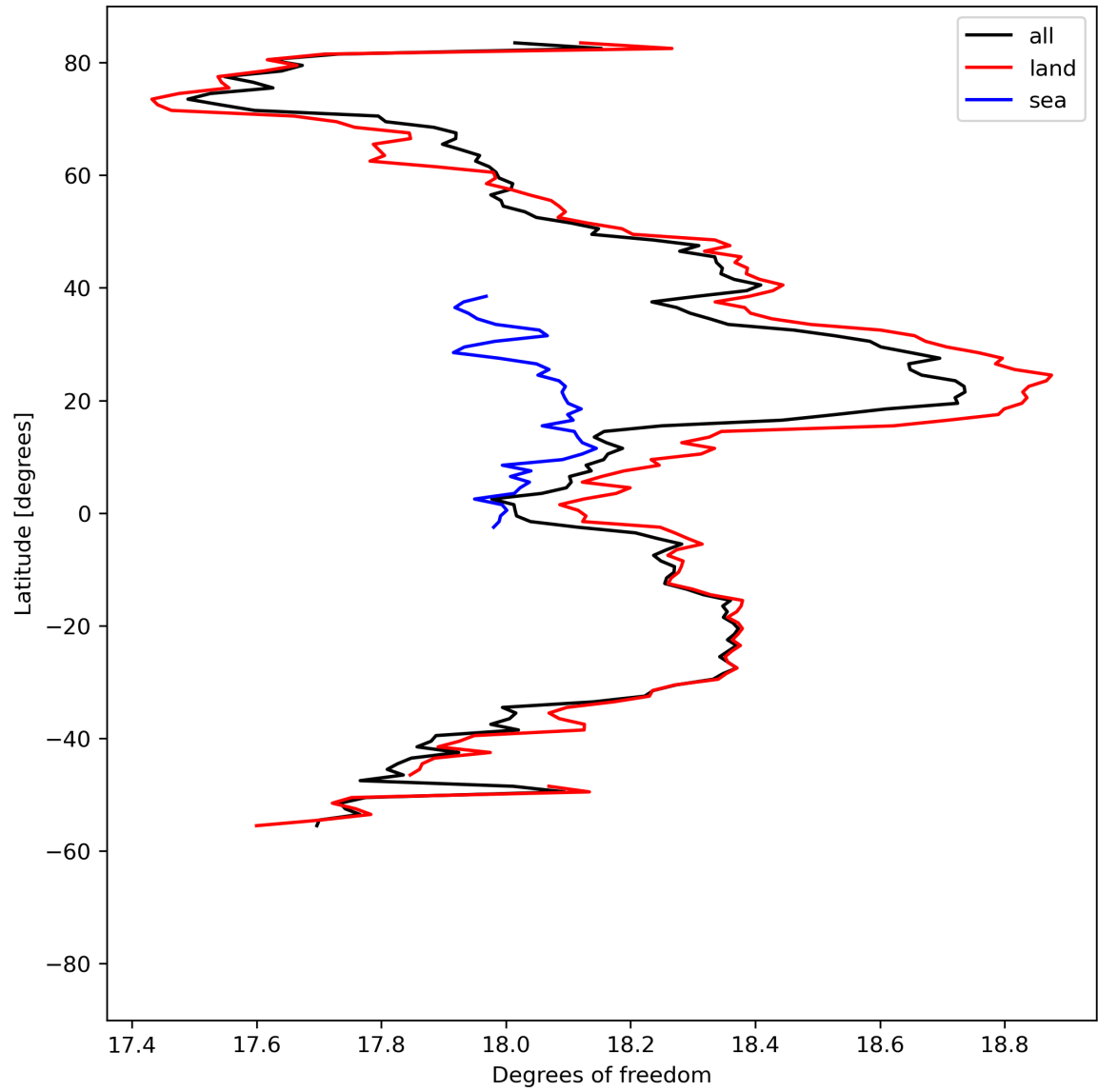
Figure 19: Zonal average of “Degrees of freedom” for 2024-08-21 to 2024-08-22.
