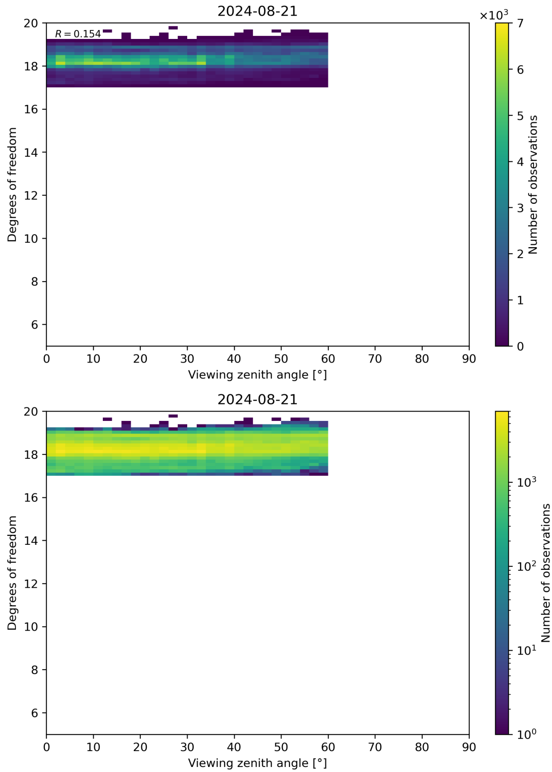
Figure 107: Scatter density plot of “Viewing zenith angle” against “Degrees of freedom” for 2024-08-21 to 2024-08-22.
