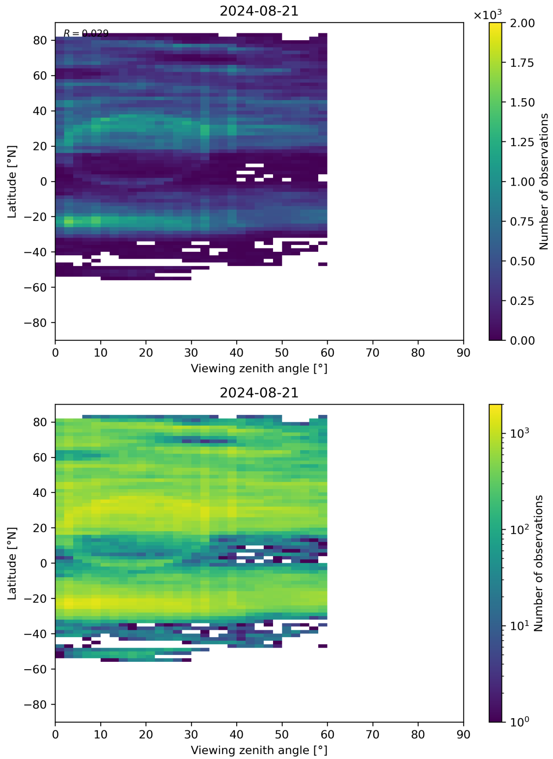
Figure 109: Scatter density plot of “Viewing zenith angle” against “Latitude” for 2024-08-21 to 2024-08-22.
