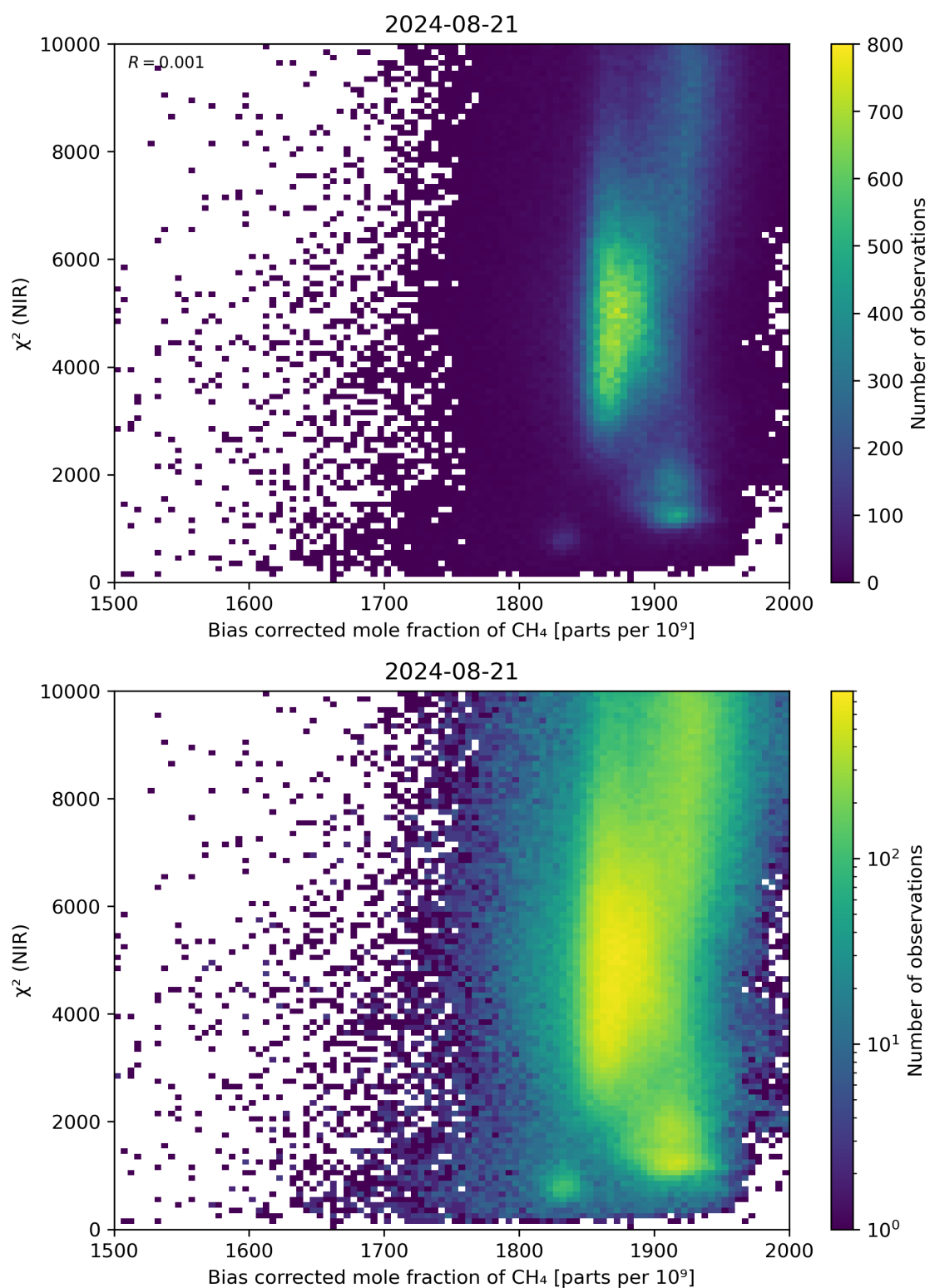
Figure 63: Scatter density plot of “Bias corrected mole fraction of CH 4 ” against “ \chi^2 (NIR)” for 2024-08-21 to 2024-08-22.
