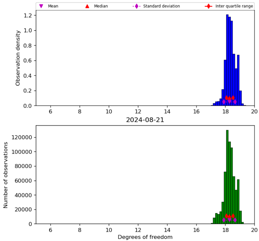
Figure 30: Histogram of “Degrees of freedom” for 2024-08-21 to 2024-08-22
