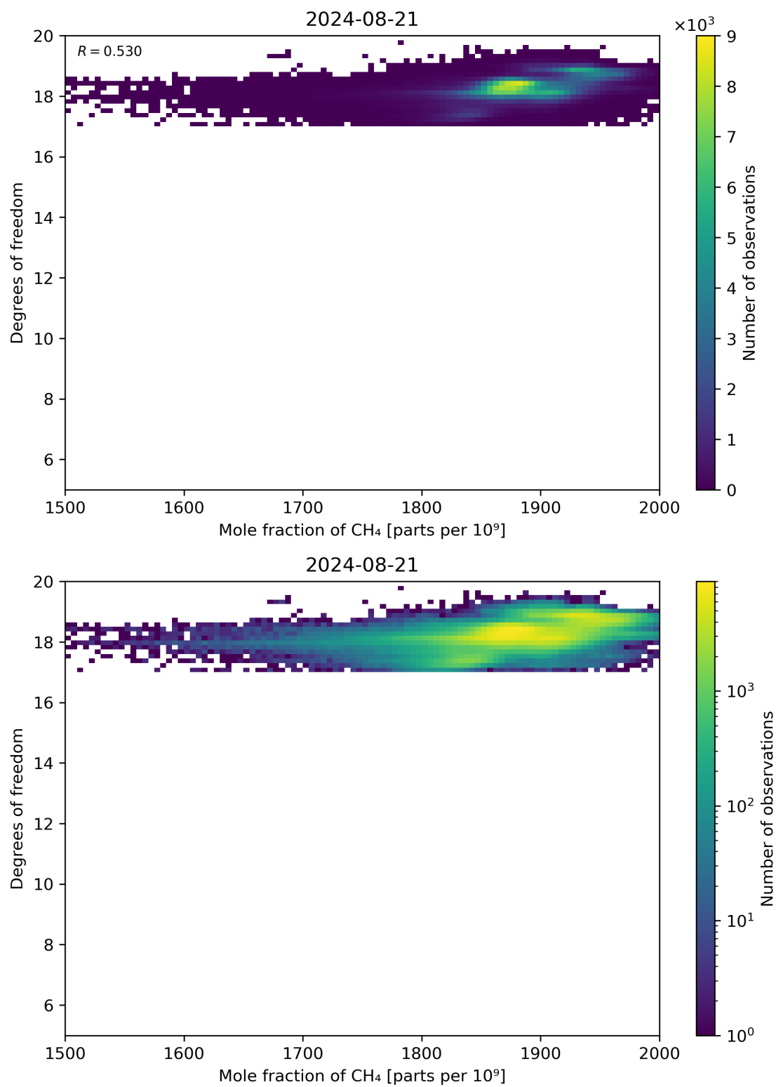
Figure 72: Scatter density plot of “Mole fraction of CH 4 ” against “Degrees of freedom” for 2024-08-21 to 2024-08-22.
