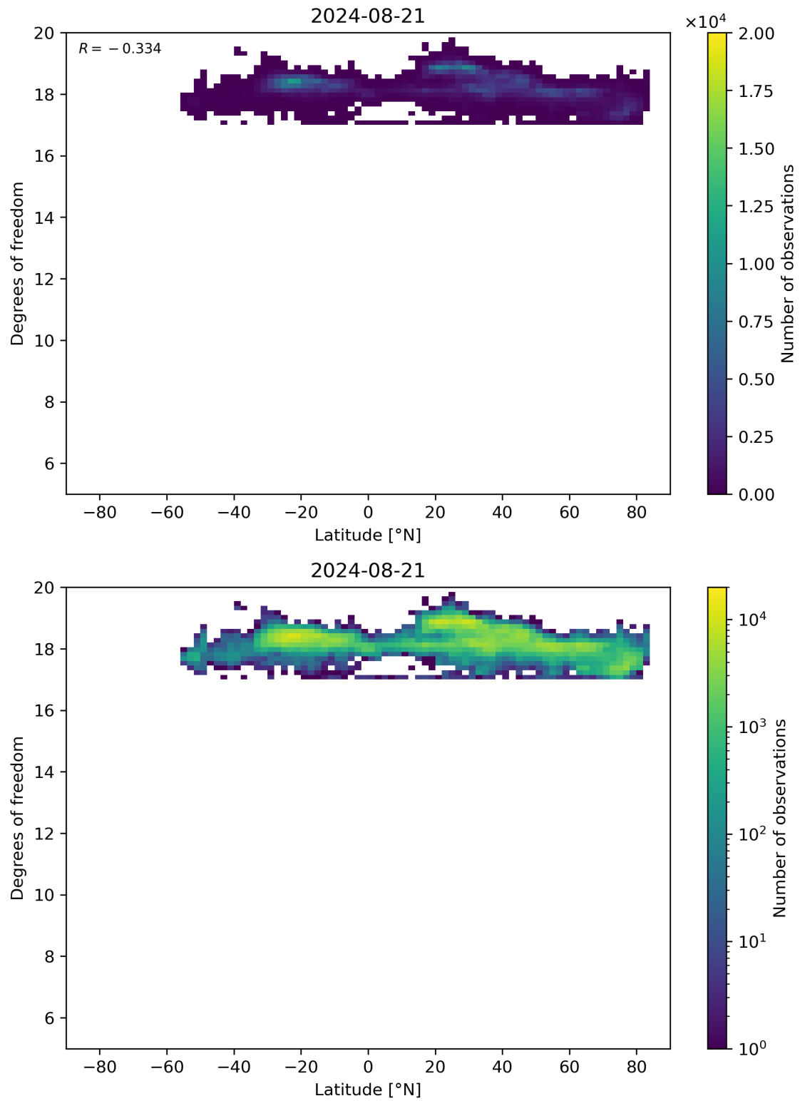
Figure 55: Scatter density plot of “Latitude” against “Degrees of freedom” for 2024-08-21 to 2024-08-22.
