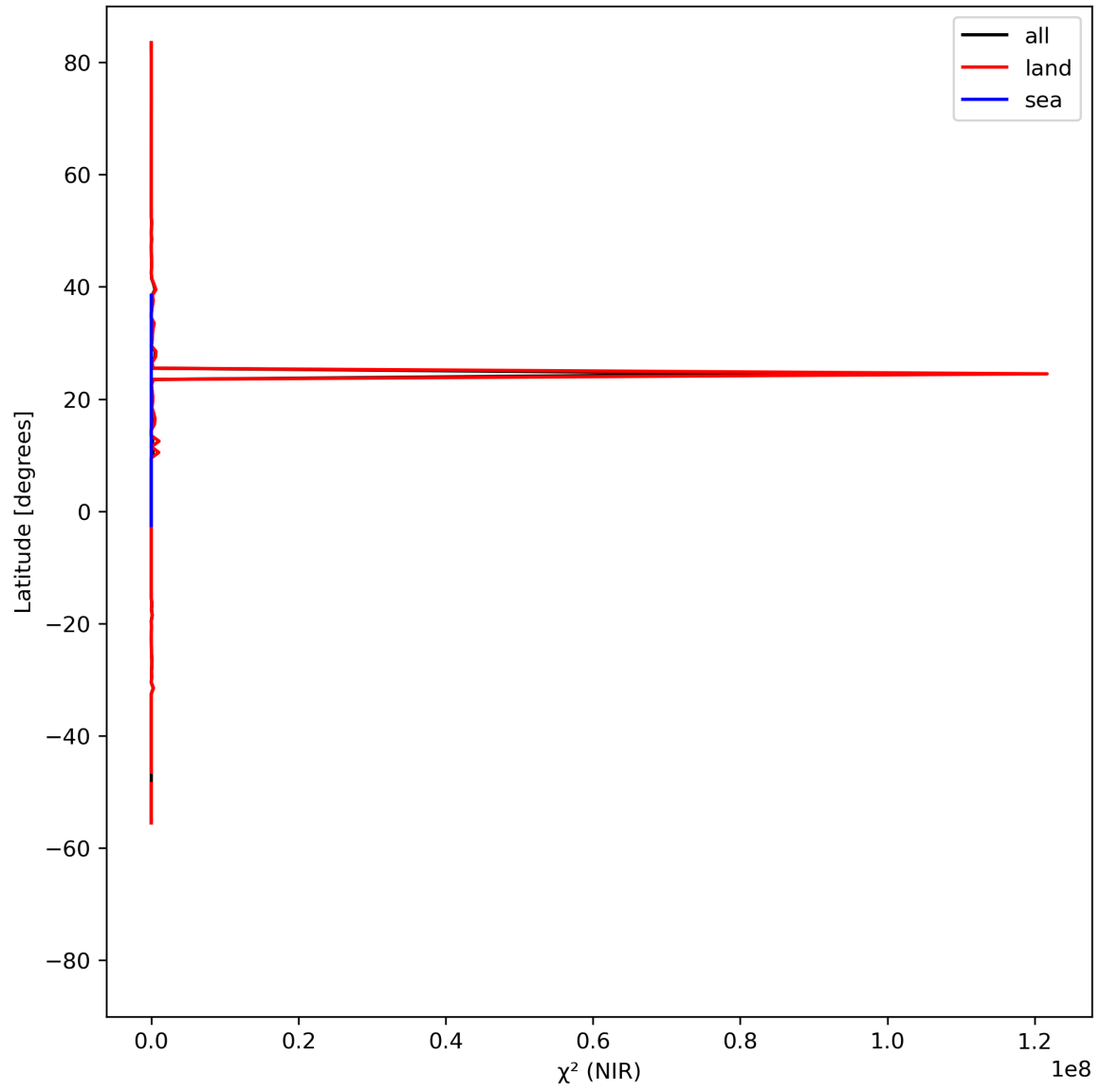
Figure 18: Zonal average of “ \chi^2 (NIR)” for 2024-08-21 to 2024-08-22.
