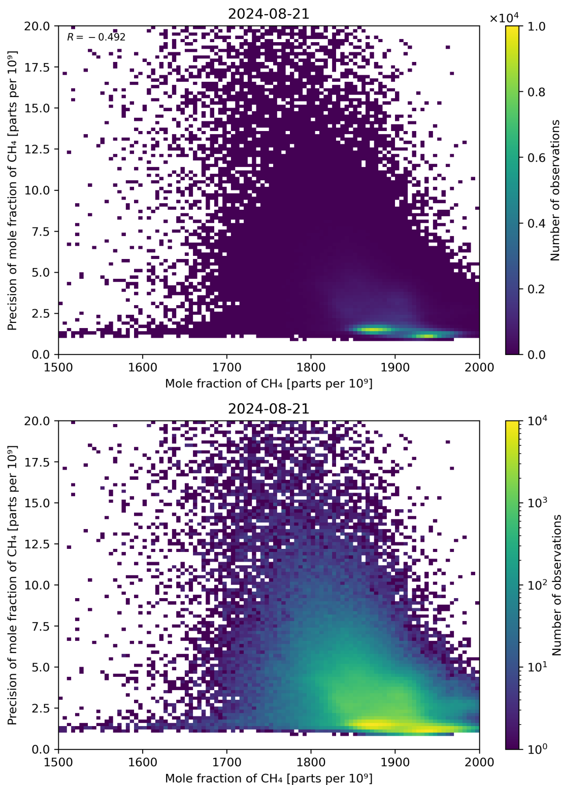
Figure 75: Scatter density plot of “Mole fraction of CH 4 ” against “Precision of mole fraction of CH 4 ” for 2024-08-21 to 2024-08-22.
