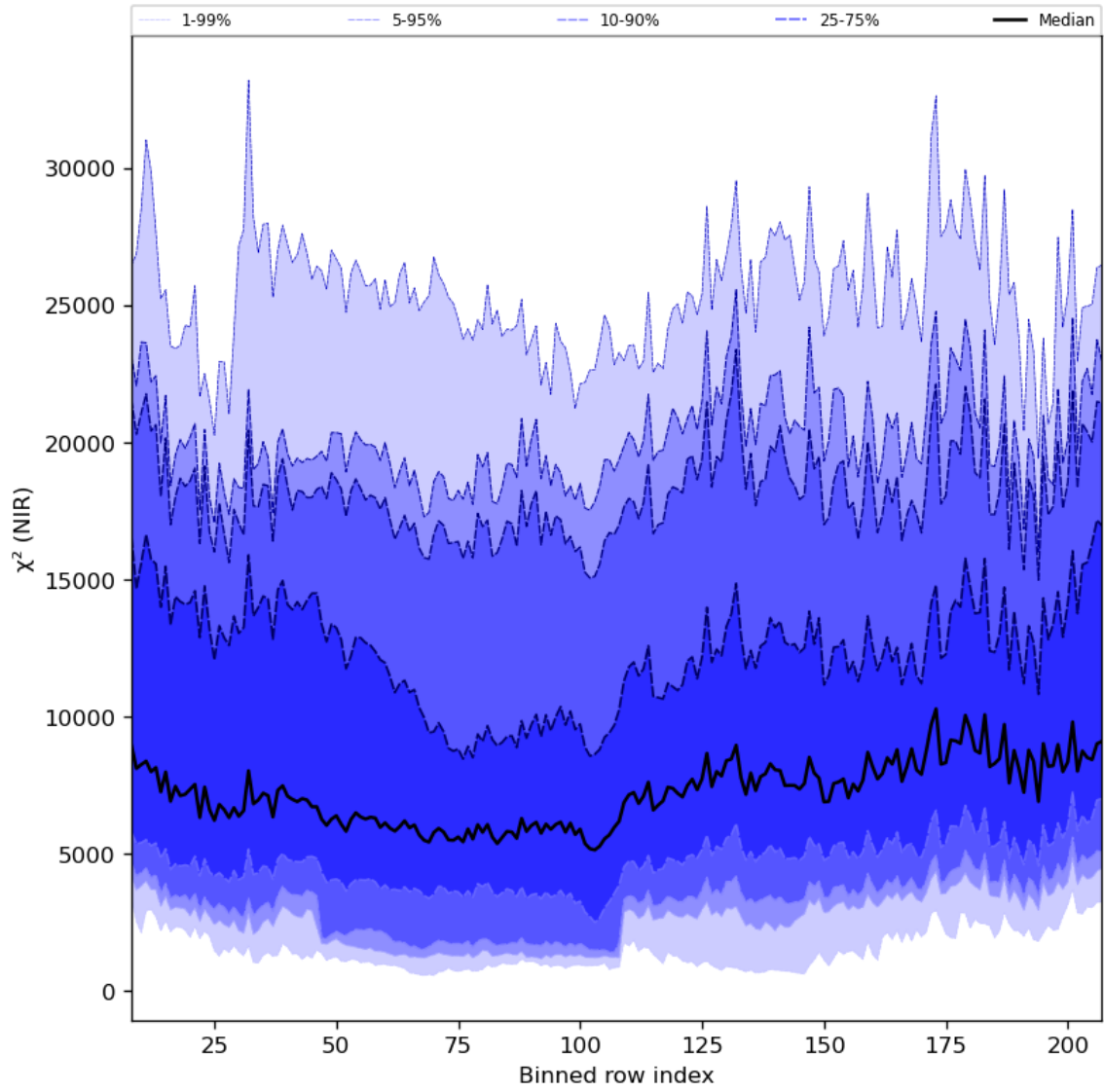
Figure 40: Along track statistics of “ \chi^2 (NIR)” for 2024-08-21 to 2024-08-22
