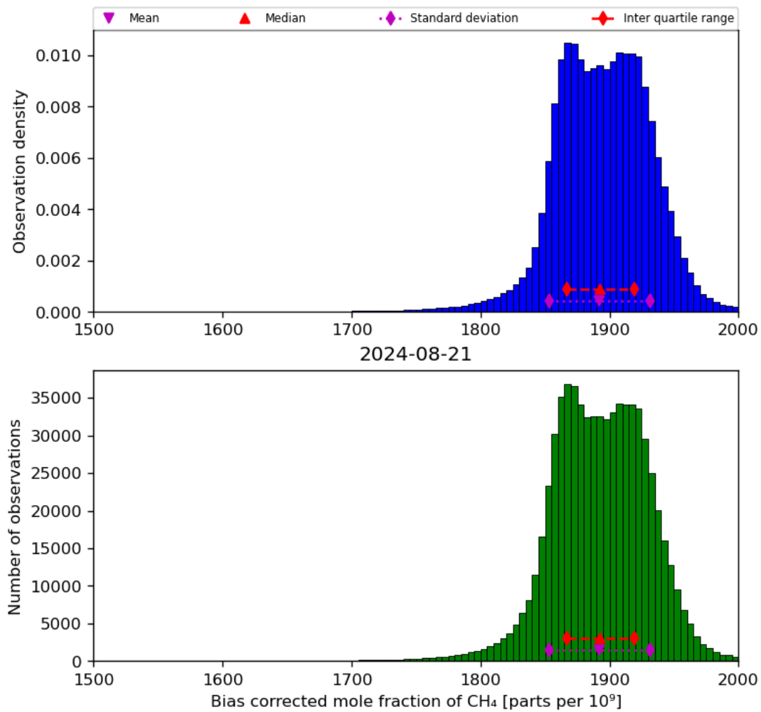
Figure 25: Histogram of “Bias corrected mole fraction of CH 4 ” for 2024-08-21 to 2024-08-22
