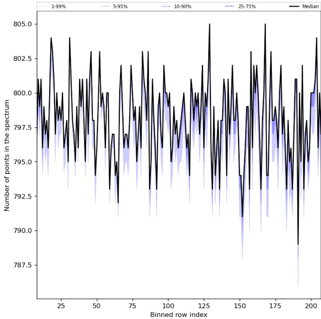
Figure 37: Along track statistics of “Number of points in the spectrum” for 2024-08-21 to 2024-08-22
