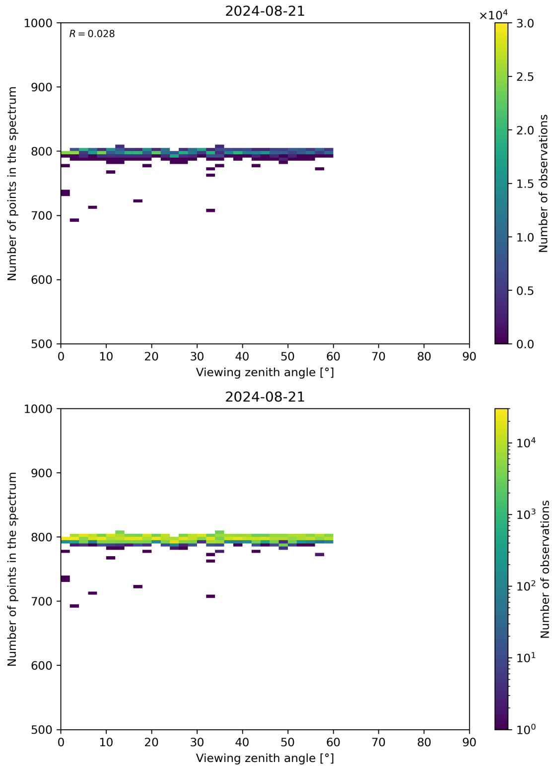
Figure 114: Scatter density plot of “Viewing zenith angle” against “Number of points in the spectrum” for 2024-08-21 to 2024-08-22.
