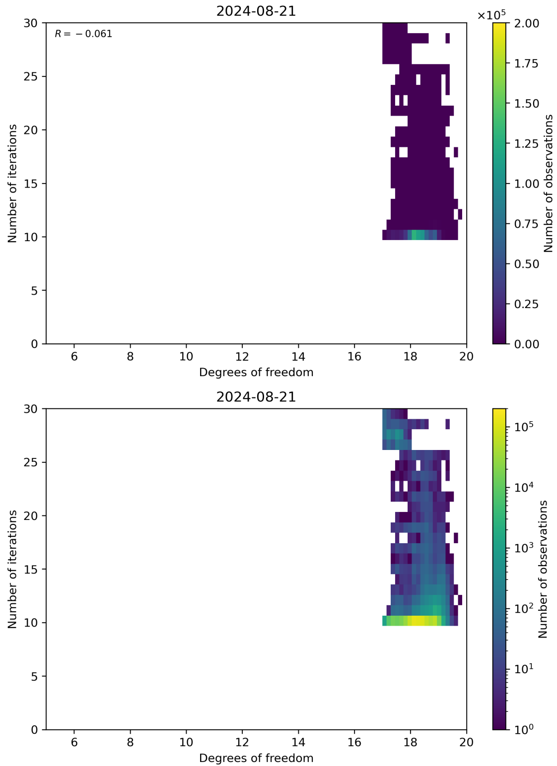
Figure 52: Scatter density plot of “Degrees of freedom” against “Number of iterations” for 2024-08-21 to 2024-08-22.
