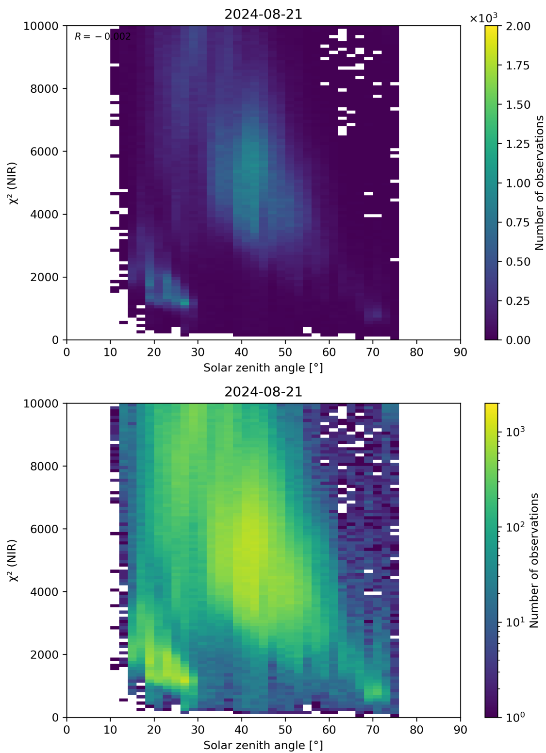
Figure 94: Scatter density plot of “Solar zenith angle” against “ \chi^2 (NIR)” for 2024-08-21 to 2024-08-22.
