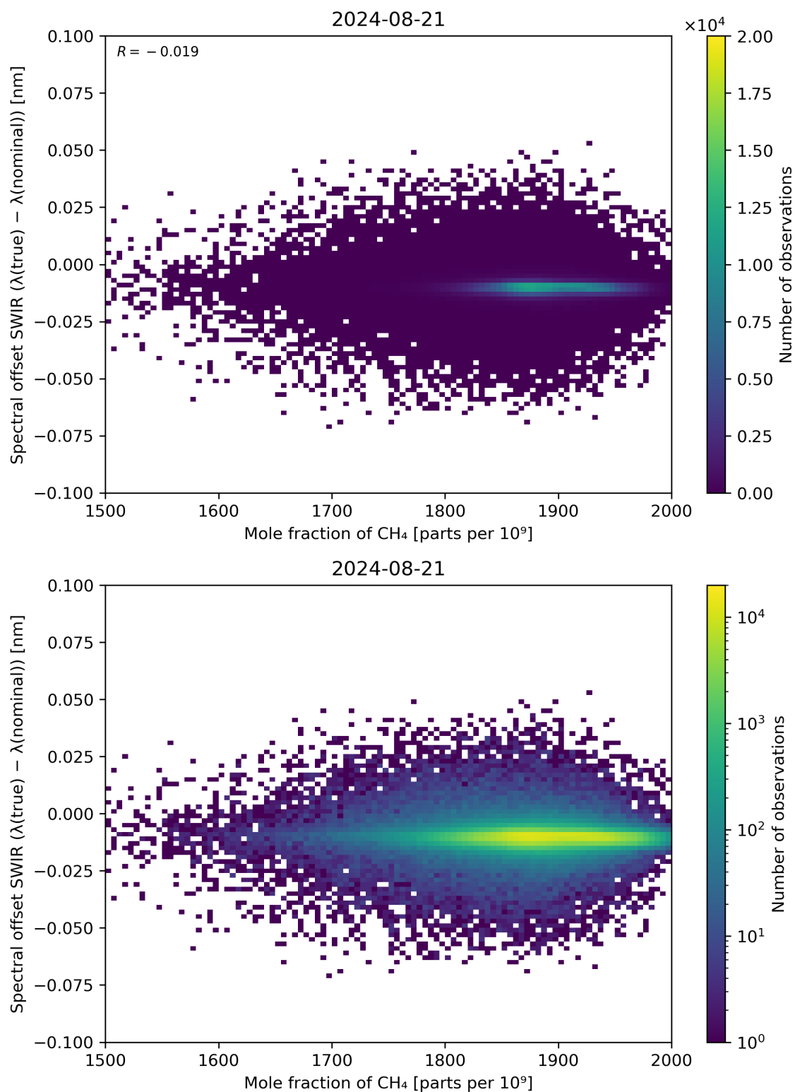
Figure 86: Scatter density plot of “Mole fraction of CH 4 ” against “Spectral offset SWIR ( \lambda(\text{true}) - \lambda(\text{nominal}) )” for 2024-08-21 to 2024-08-22.
