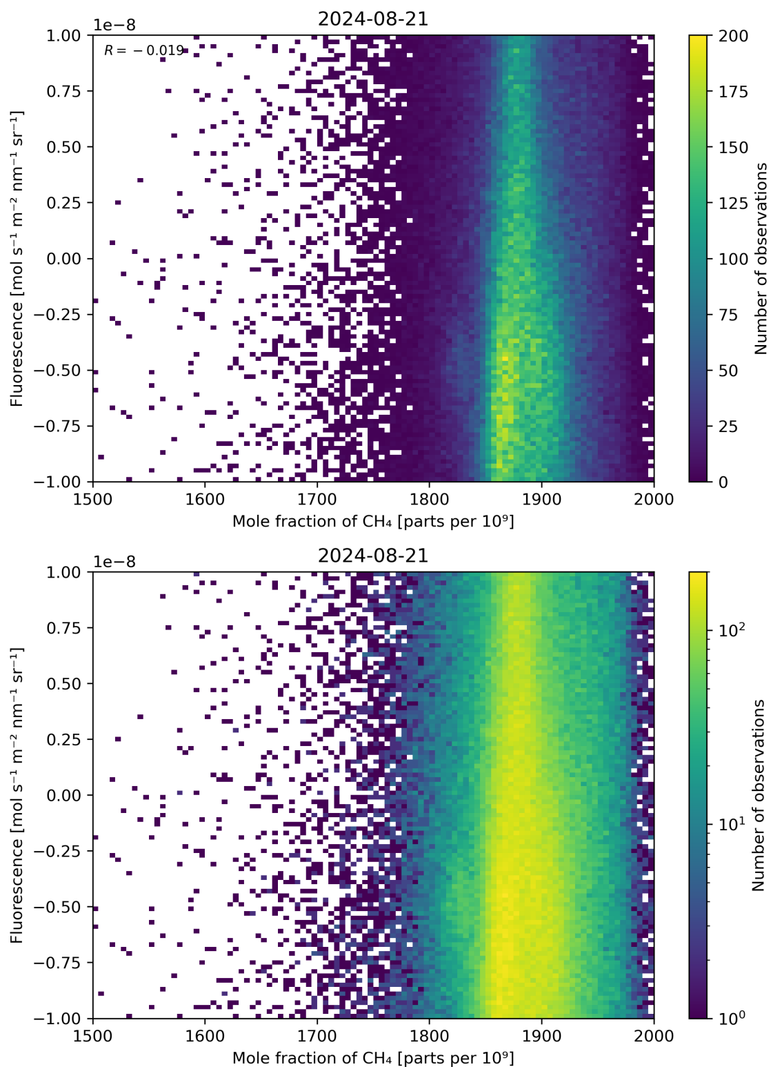
Figure 73: Scatter density plot of “Mole fraction of \text{CH}_4 ” against “Fluorescence” for 2024-08-21 to 2024-08-22.
