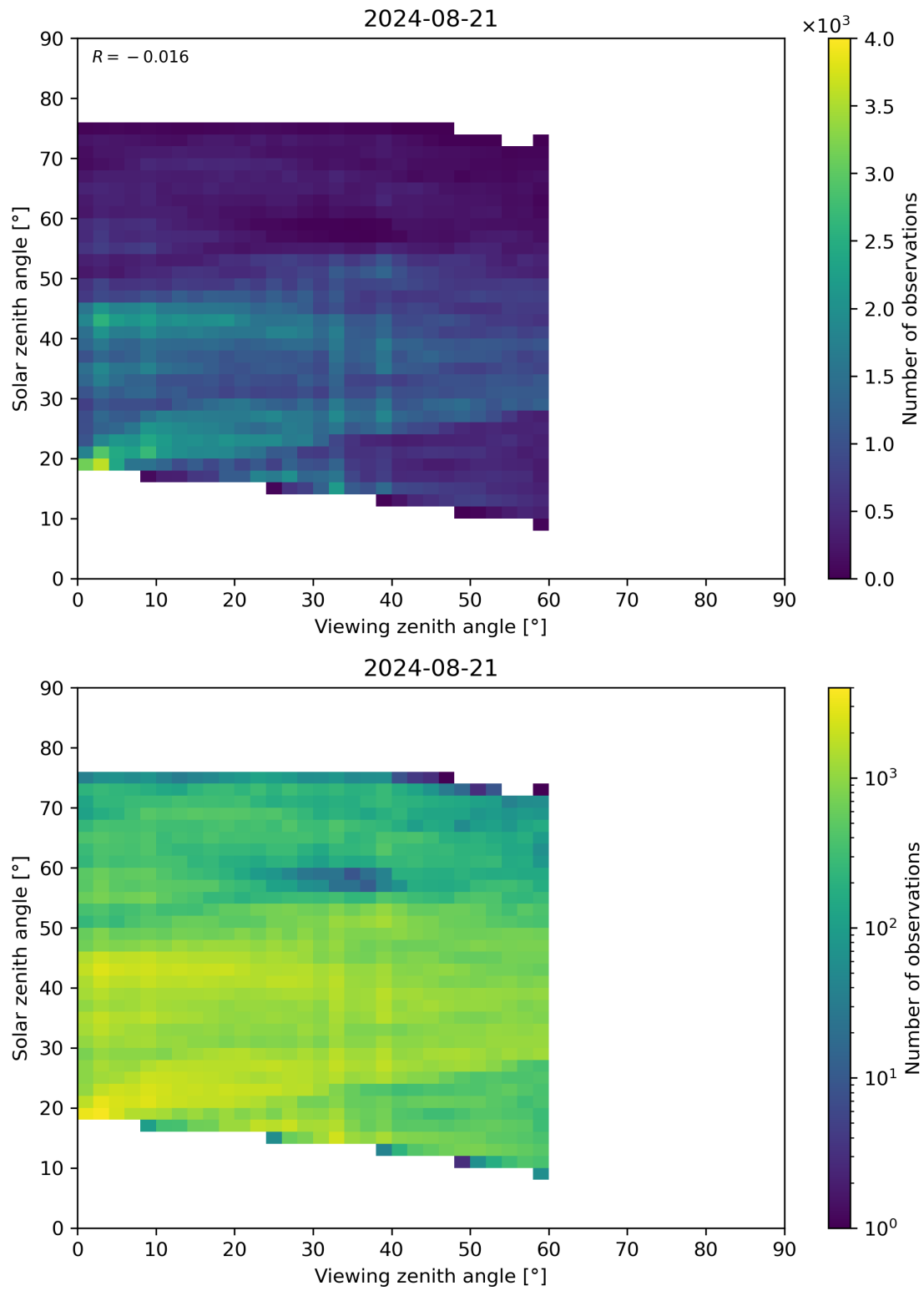
Figure 115: Scatter density plot of “Viewing zenith angle” against “Solar zenith angle” for 2024-08-21 to 2024-08-22.
