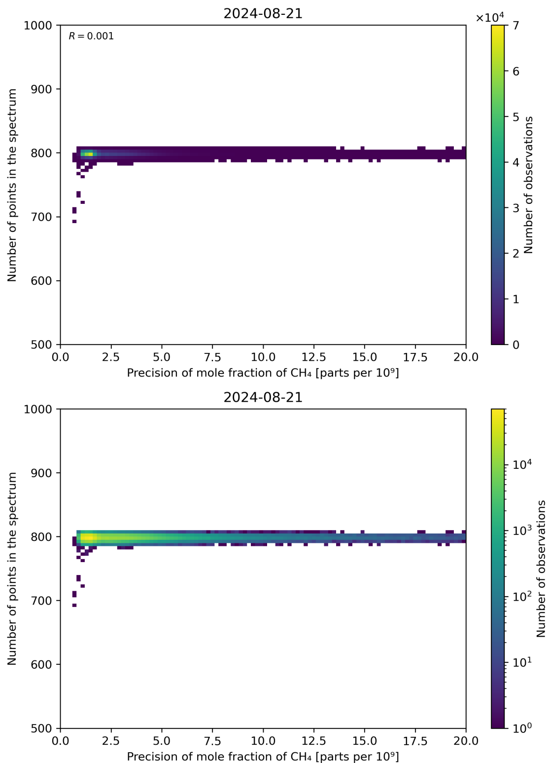
Figure 84: Scatter density plot of “Precision of mole fraction of \text{CH}_4 ” against “Number of points in the spectrum” for 2024-08-21 to 2024-08-22.
