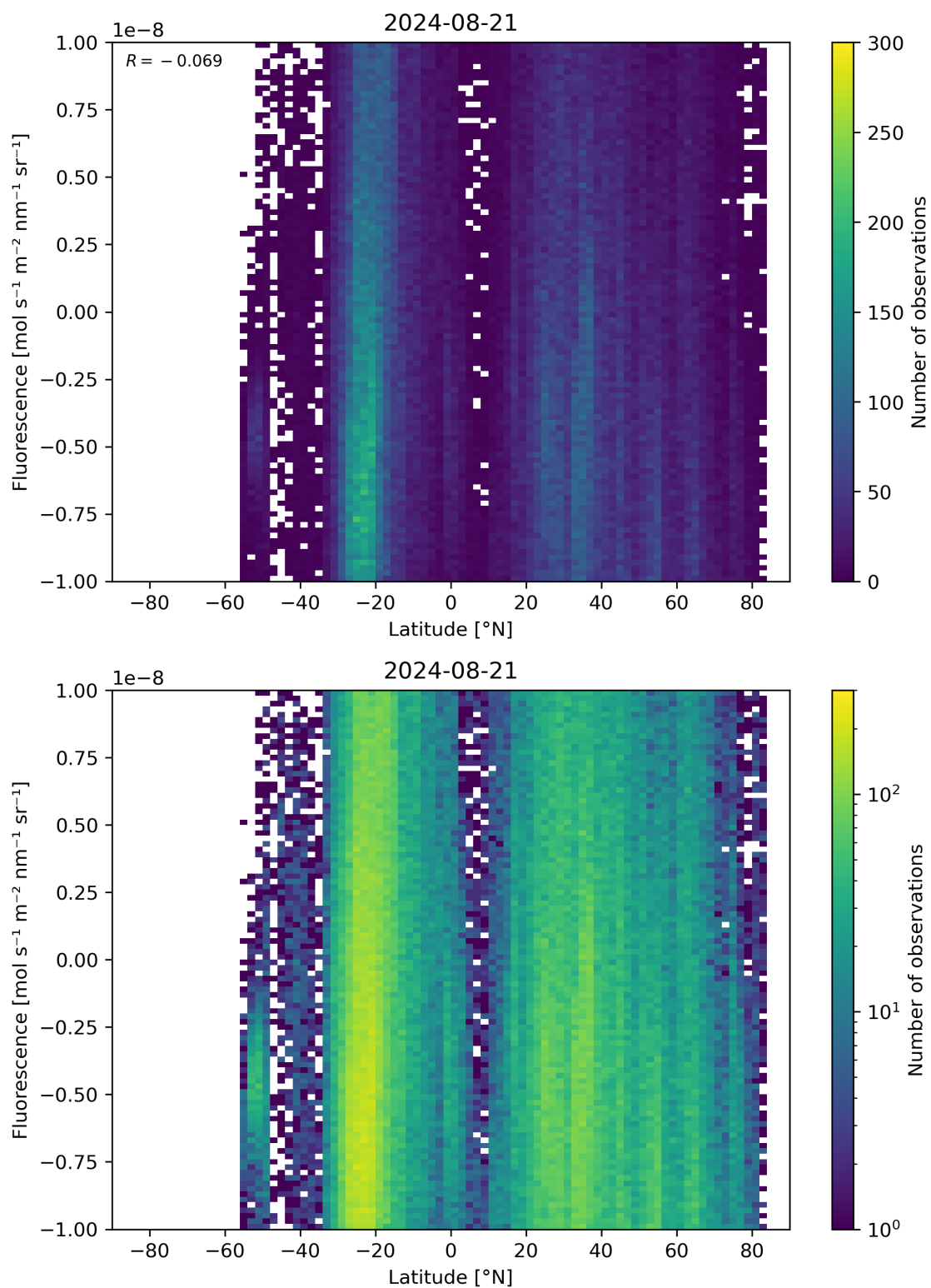
Figure 56: Scatter density plot of “Latitude” against “Fluorescence” for 2024-08-21 to 2024-08-22.
