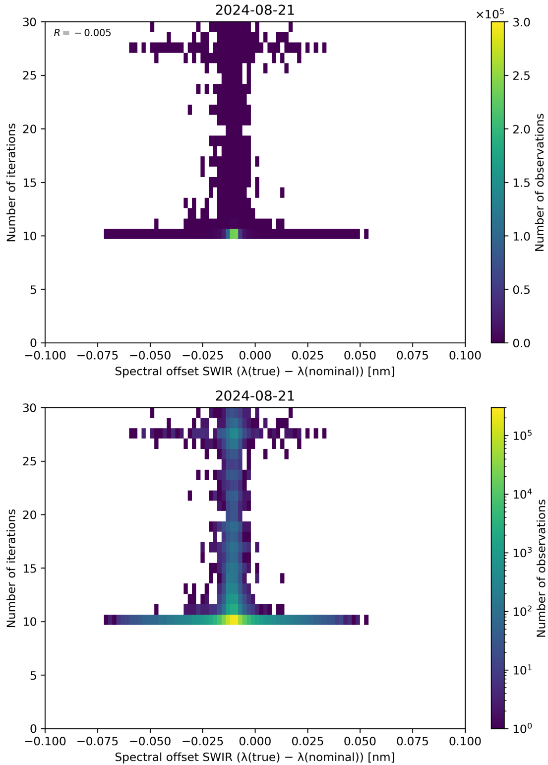
Figure 121: Scatter density plot of “Spectral offset SWIR ( \lambda(\text{true}) - \lambda(\text{nominal}) )” against “Number of iterations” for 2024-08-21 to 2024-08-22.
