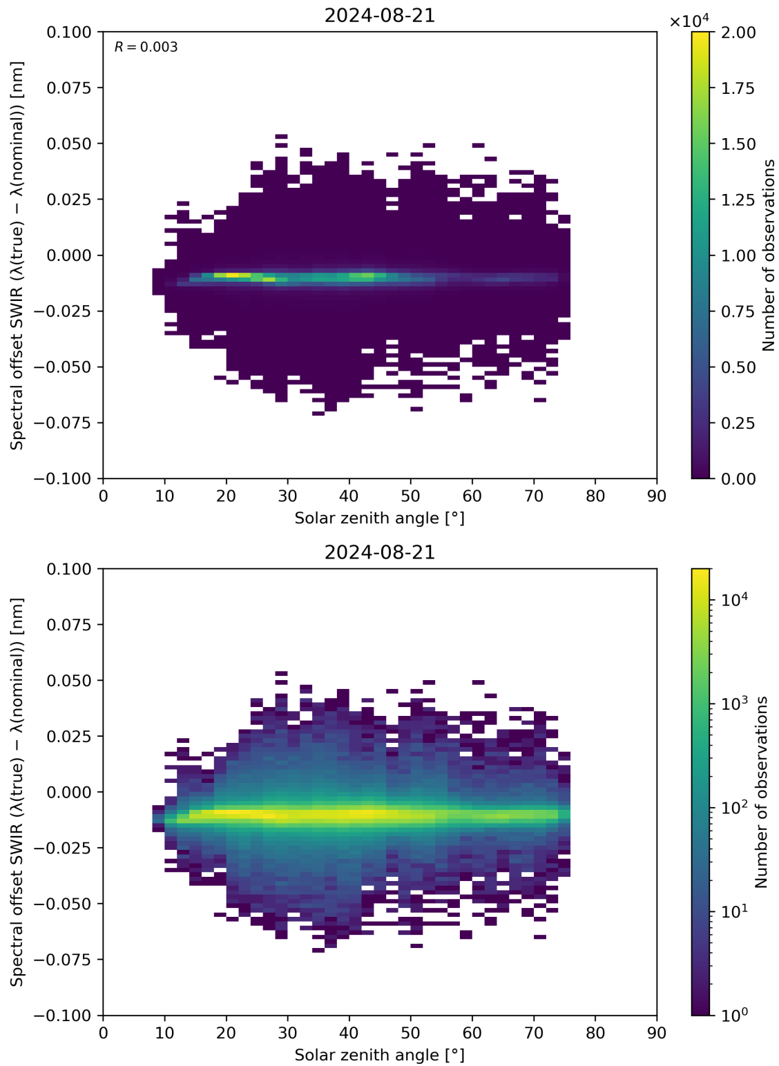
Figure 104: Scatter density plot of “Solar zenith angle” against “Spectral offset SWIR ( \lambda(\text{true}) - \lambda(\text{nominal}) )” for 2024-08-21 to 2024-08-22.
