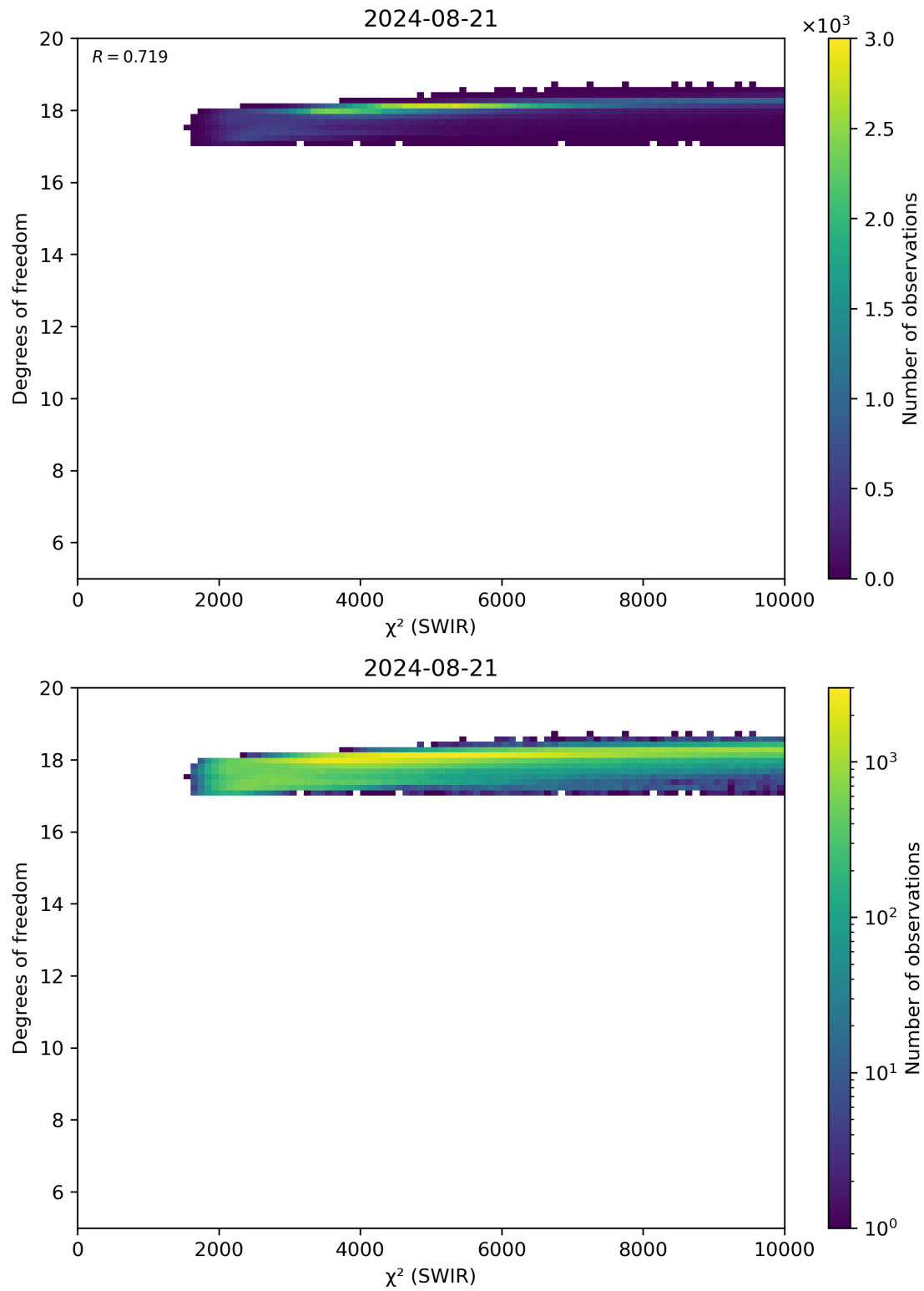
Figure 48: Scatter density plot of " \chi^2 (SWIR)" against "Degrees of freedom" for 2024-08-21 to 2024-08-22.
