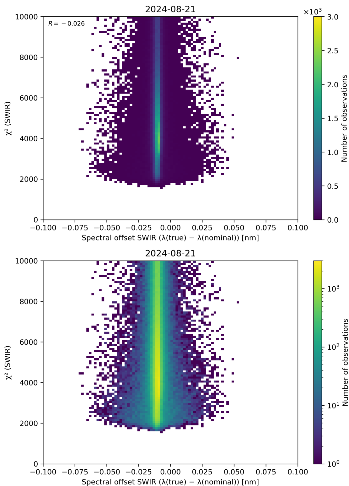
Figure 118: Scatter density plot of “Spectral offset SWIR ( \lambda(\text{true}) - \lambda(\text{nominal}) )” against “ \chi^2 (SWIR)” for 2024-08-21 to 2024-08-22.
