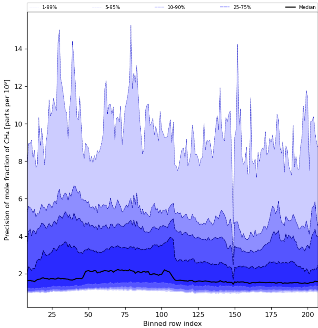
Figure 35: Along track statistics of “Precision of mole fraction of CH 4 ” for 2024-08-21 to 2024-08-22
