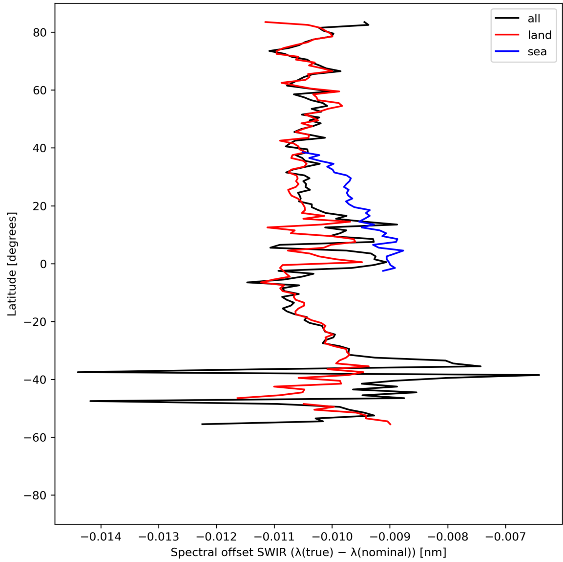
Figure 16: Zonal average of “Spectral offset SWIR ( \lambda(\text{true}) - \lambda(\text{nominal}) )” for 2024-08-21 to 2024-08-22.
