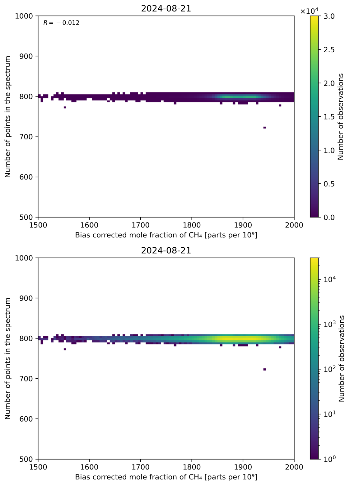
Figure 68: Scatter density plot of “Bias corrected mole fraction of CH 4 ” against “Number of points in the spectrum” for 2024-08-21 to 2024-08-22.
