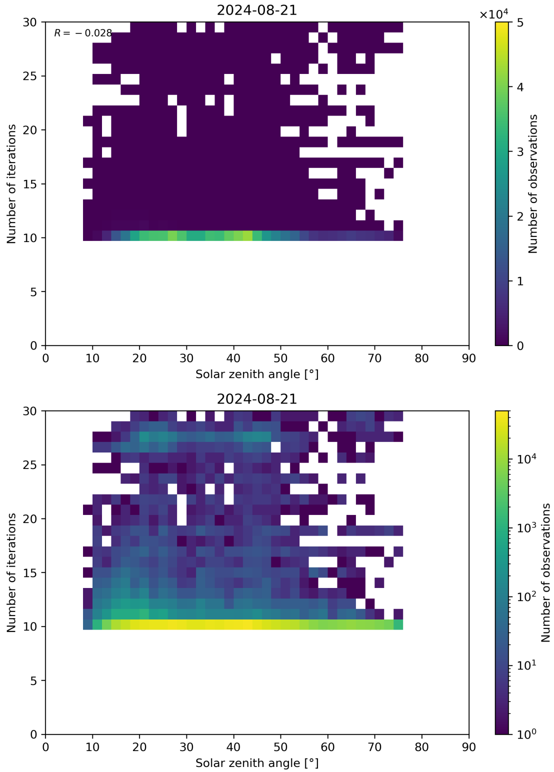
Figure 102: Scatter density plot of “Solar zenith angle” against “Number of iterations” for 2024-08-21 to 2024-08-22.
