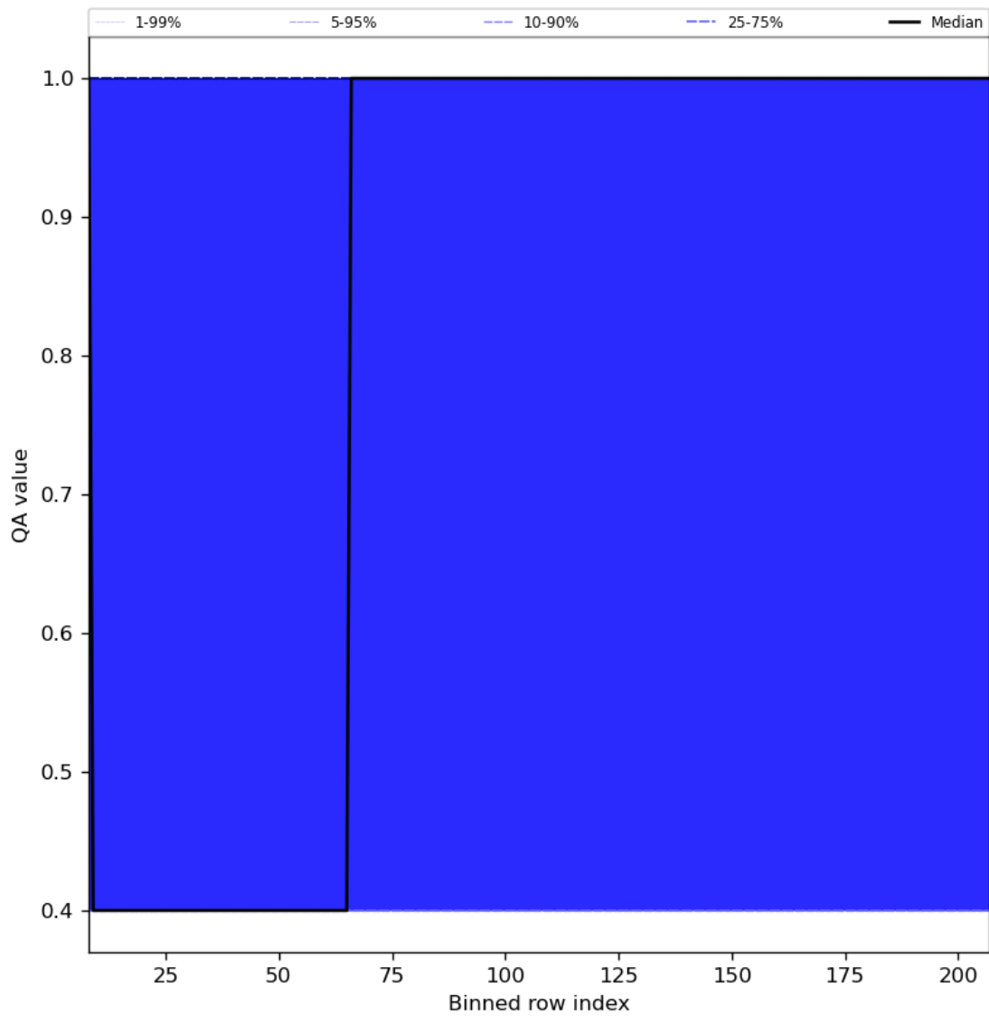
Figure 33: Along track statistics of “QA value” for 2024-08-21 to 2024-08-22
