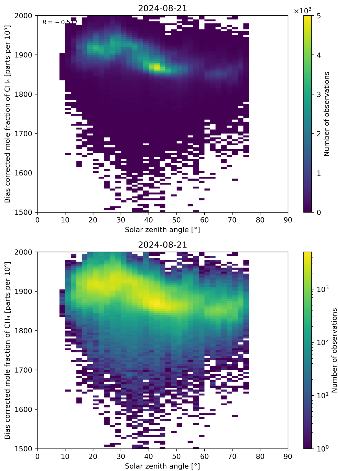
Figure 100: Scatter density plot of “Solar zenith angle” against “Bias corrected mole fraction of CH 4 ” for 2024-08-21 to 2024-08-22.
