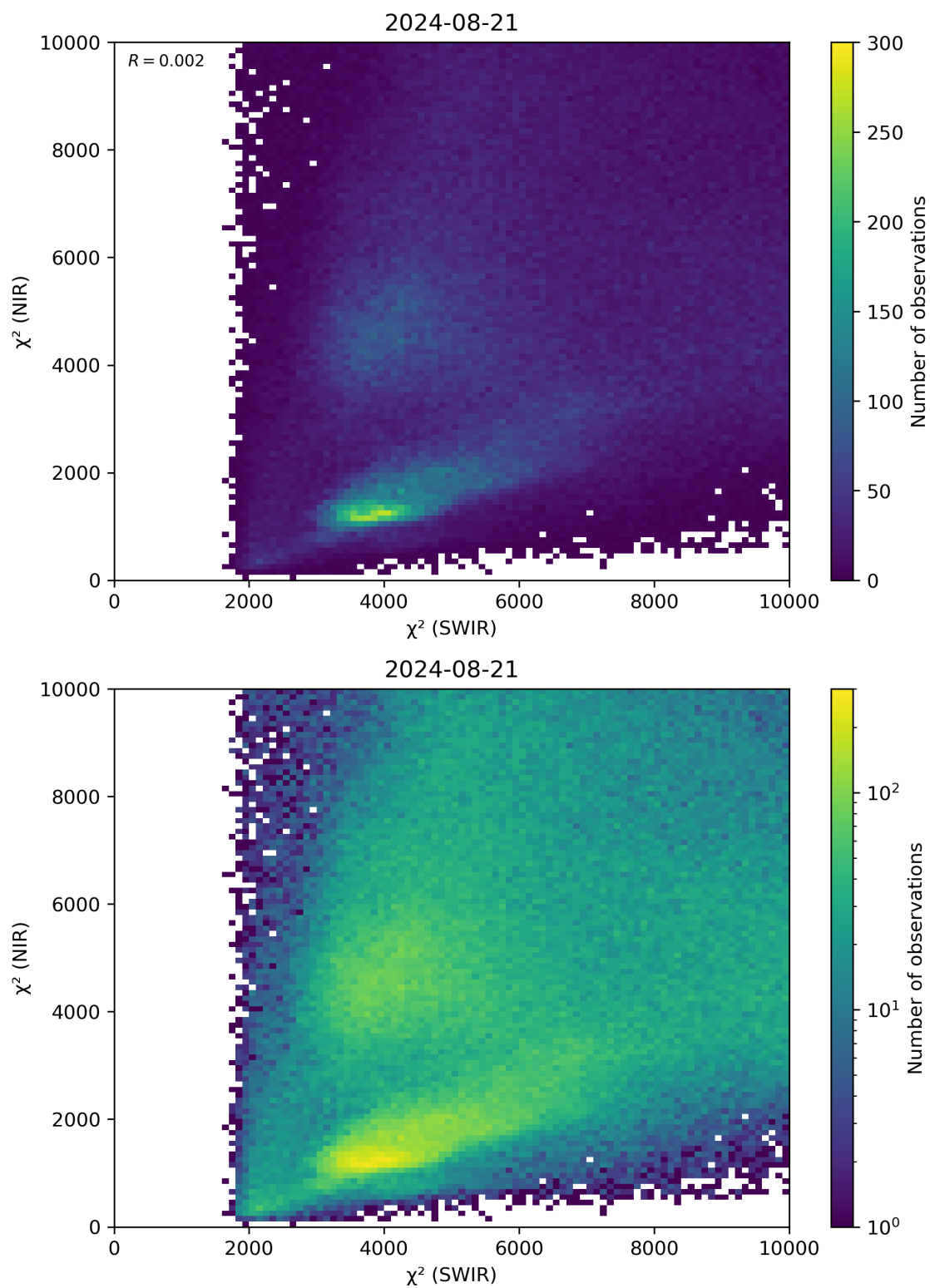
Figure 47: Scatter density plot of “ \chi^2 (SWIR)” against “ \chi^2 (NIR)” for 2024-08-21 to 2024-08-22.
