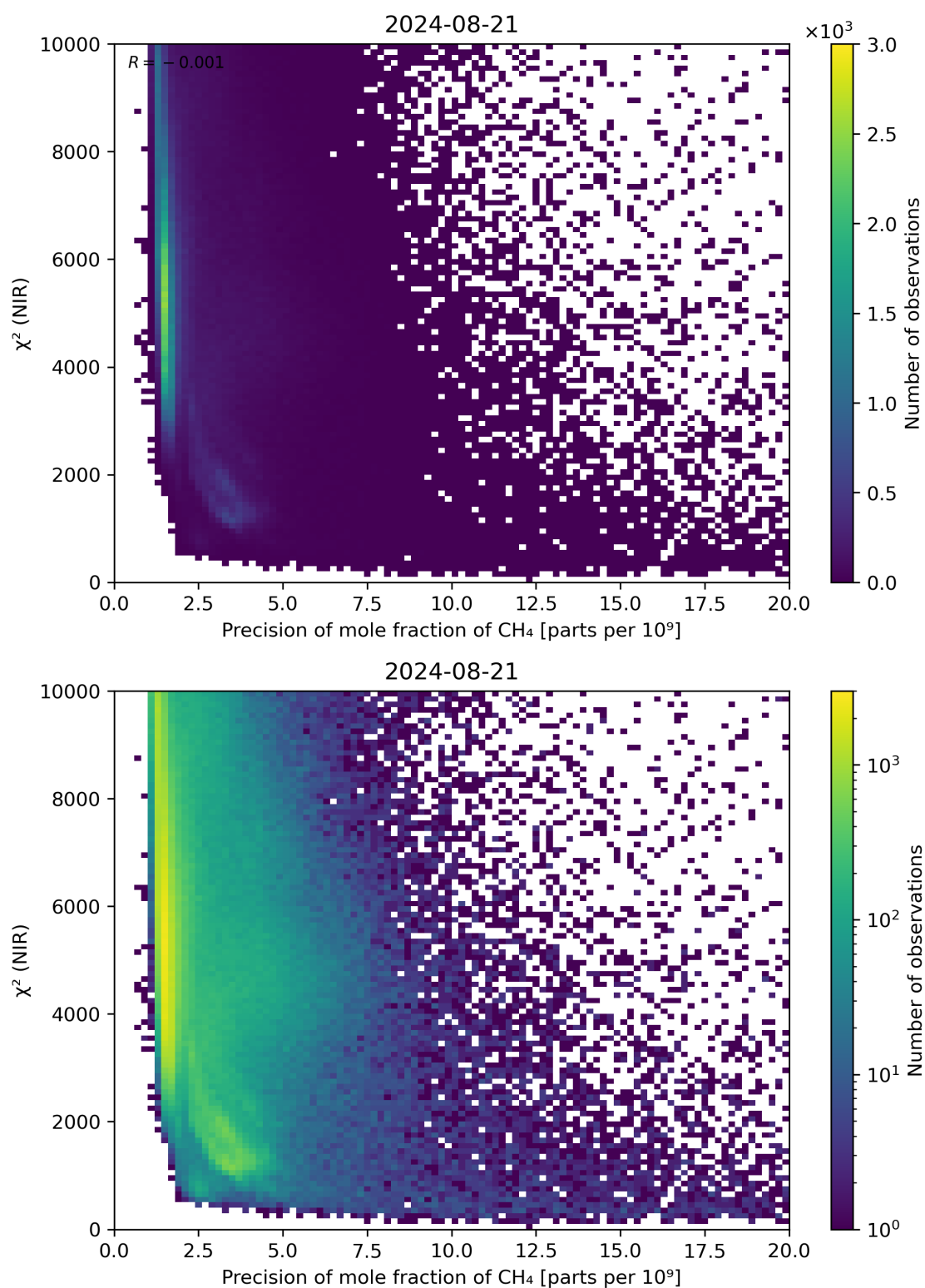
Figure 78: Scatter density plot of “Precision of mole fraction of CH 4 ” against “ \chi^2 (NIR)” for 2024-08-21 to 2024-08-22.
