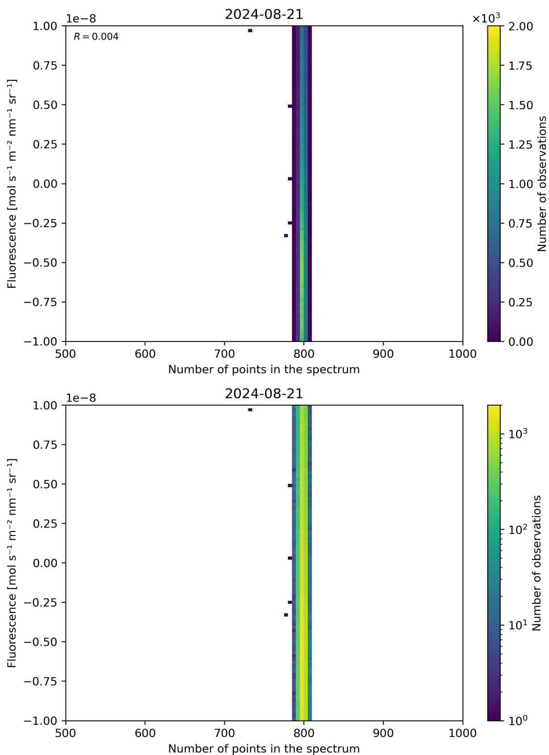
Figure 91: Scatter density plot of “Number of points in the spectrum” against “Fluorescence” for 2024-08-21 to 2024-08-22.
