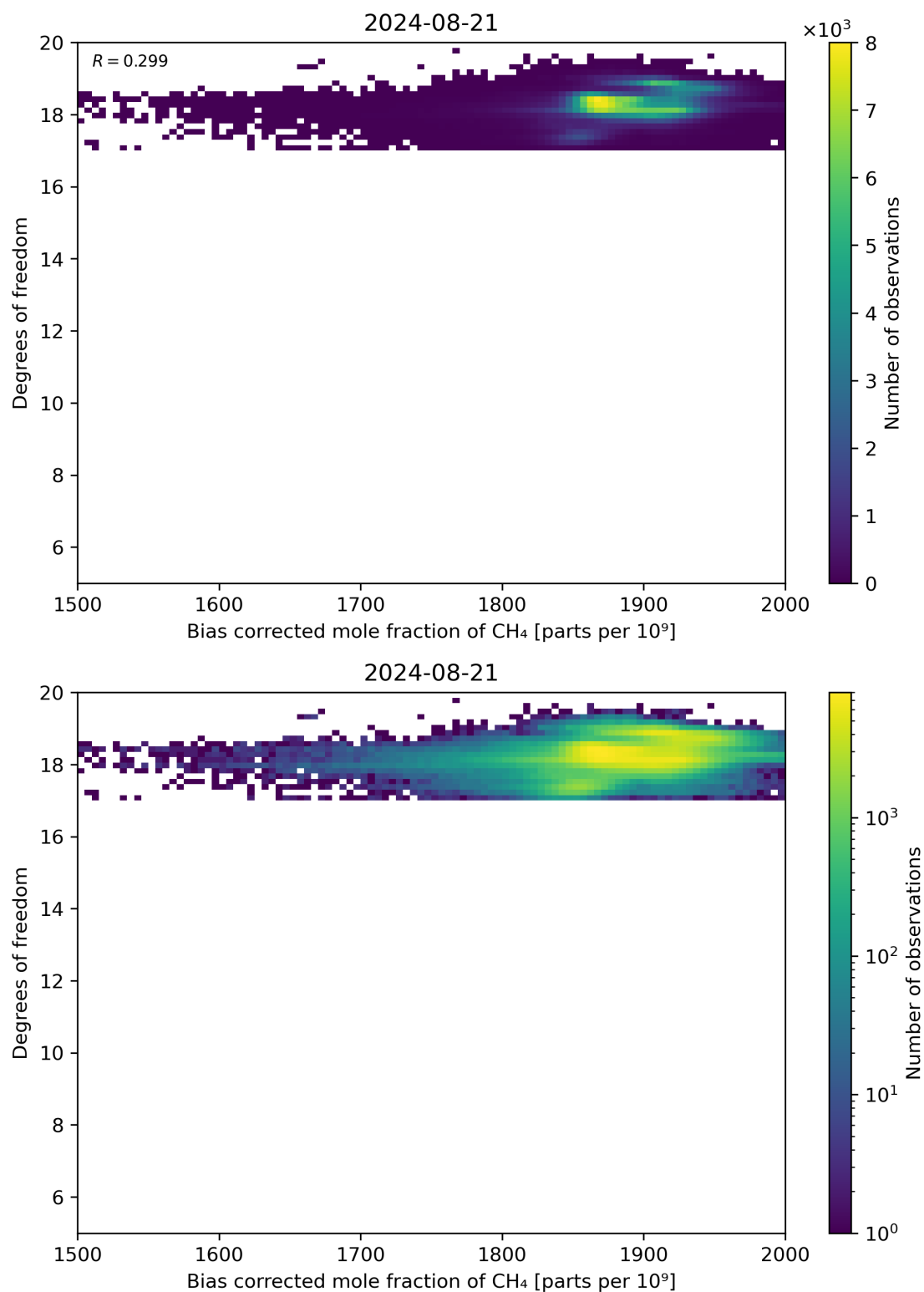
Figure 65: Scatter density plot of “Bias corrected mole fraction of CH 4 ” against “Degrees of freedom” for 2024-08-21 to 2024-08-22.
