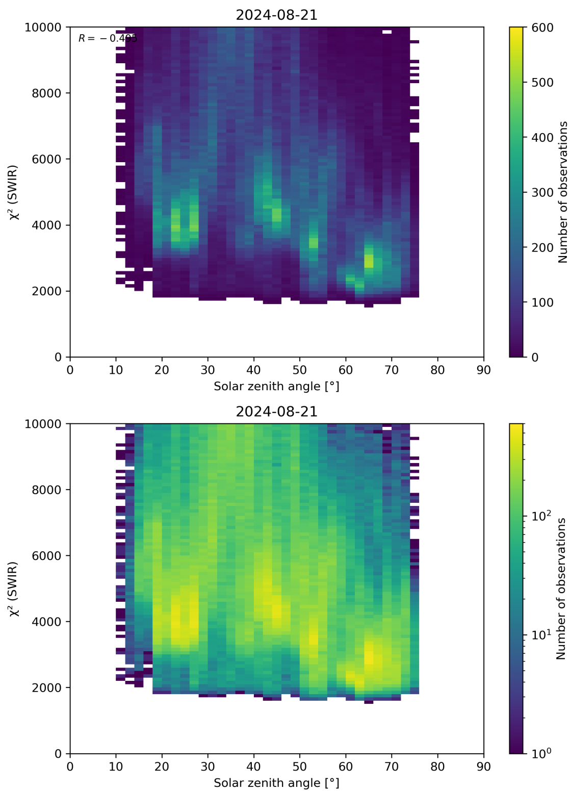
Figure 95: Scatter density plot of “Solar zenith angle” against “ \chi^2 (SWIR)” for 2024-08-21 to 2024-08-22.
