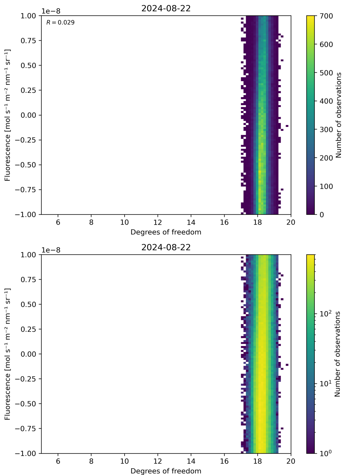
Figure 51: Scatter density plot of “Degrees of freedom” against “Fluorescence” for 2024-08-22 to 2024-08-23.
