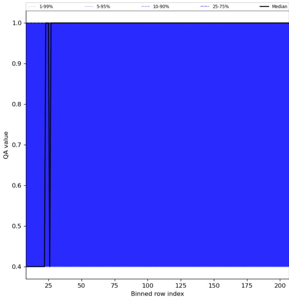
Figure 33: Along track statistics of “QA value” for 2024-08-22 to 2024-08-23
