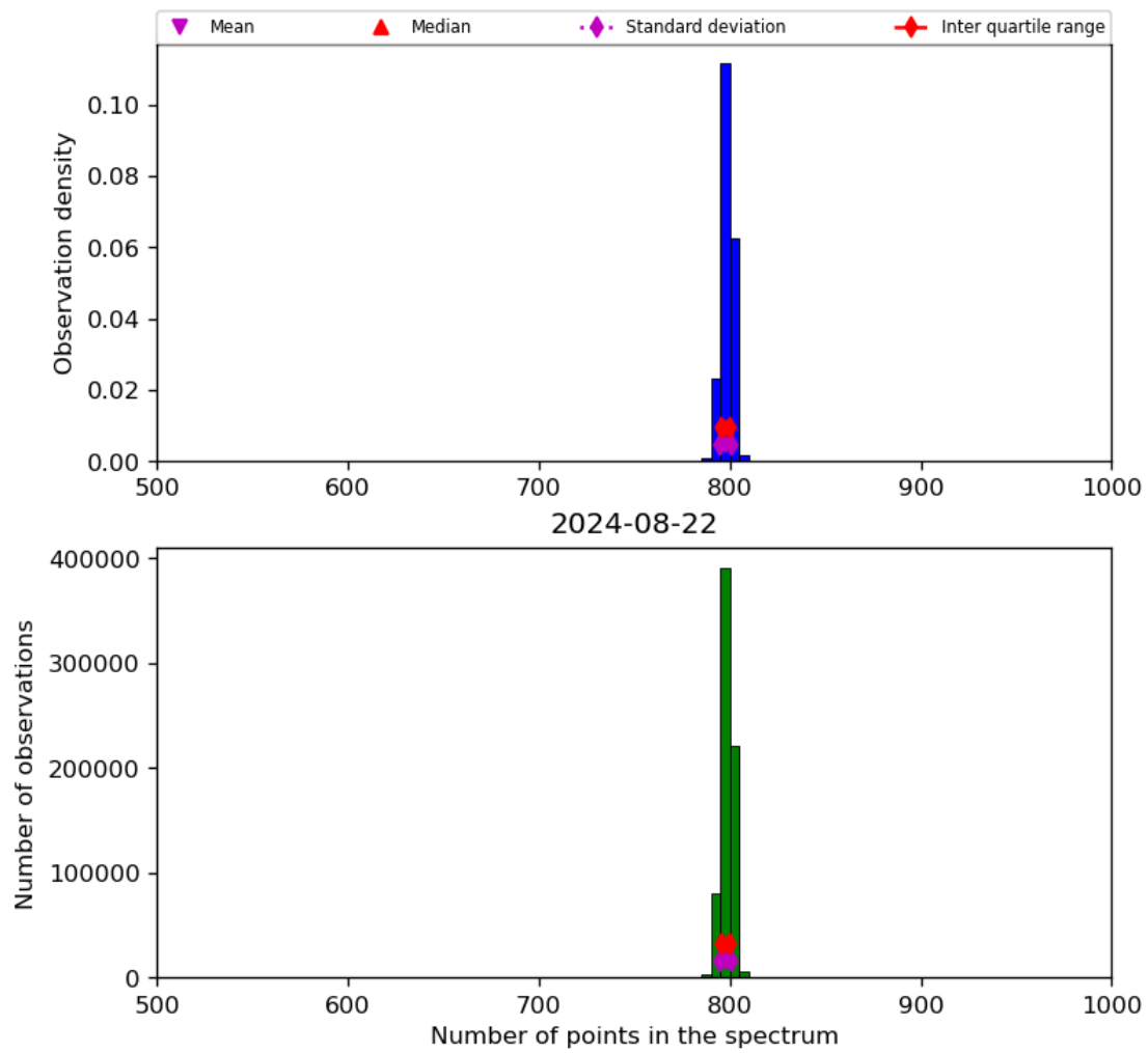
Figure 26: Histogram of “Number of points in the spectrum” for 2024-08-22 to 2024-08-23
