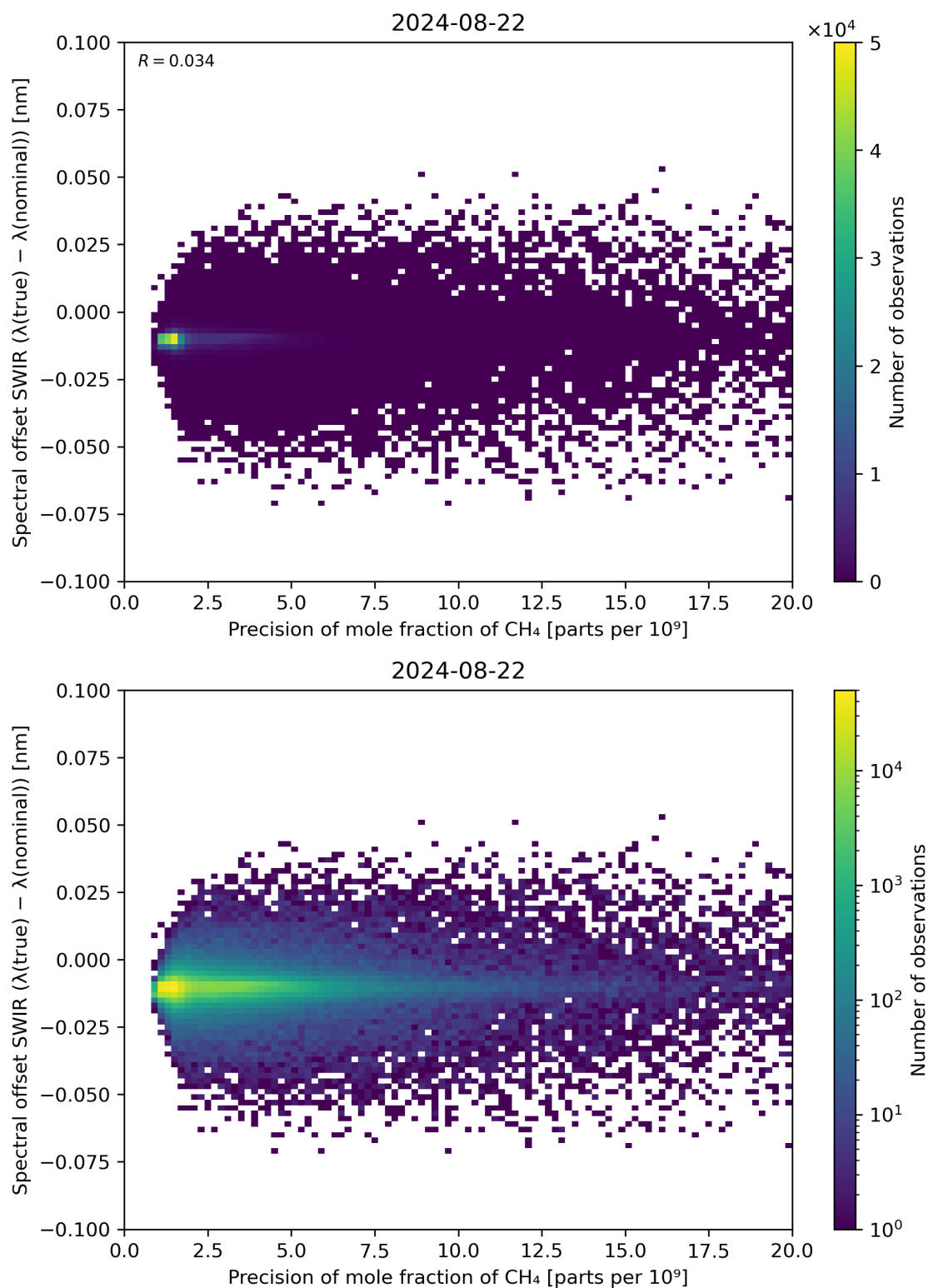
Figure 85: Scatter density plot of “Precision of mole fraction of CH 4 ” against “Spectral offset SWIR ( \lambda(\text{true}) - \lambda(\text{nominal}) )” for 2024-08-22 to 2024-08-23.
