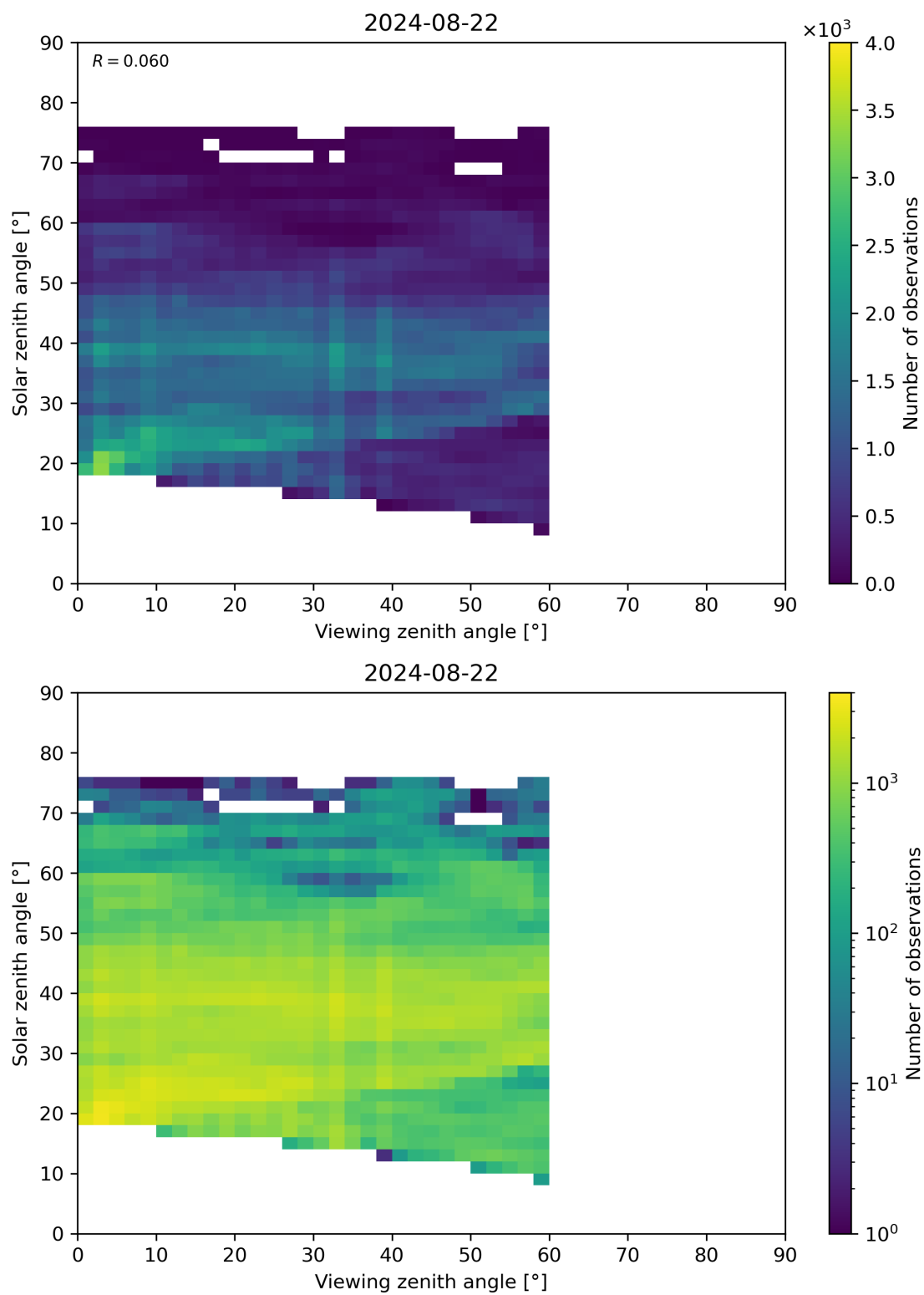
Figure 115: Scatter density plot of “Viewing zenith angle” against “Solar zenith angle” for 2024-08-22 to 2024-08-23.
