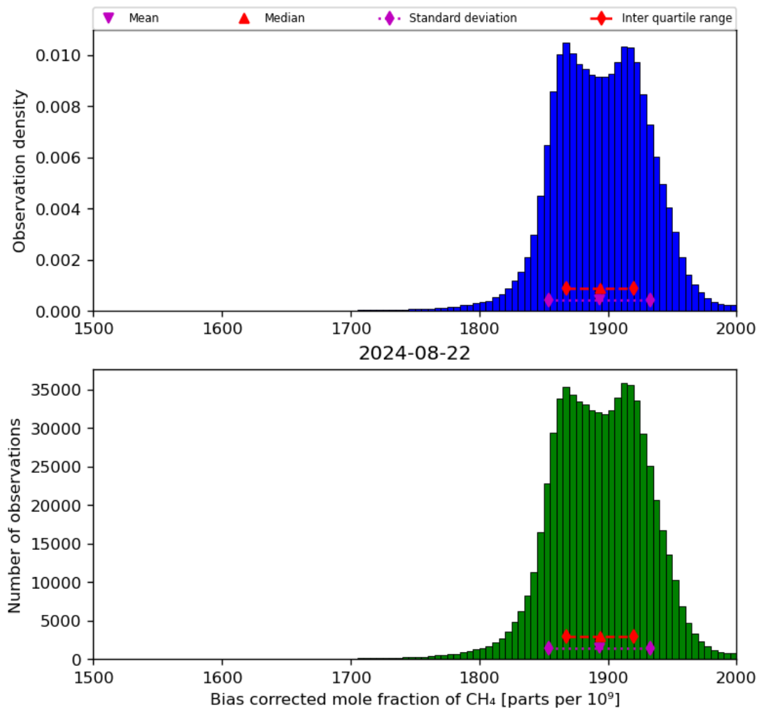
Figure 25: Histogram of “Bias corrected mole fraction of CH 4 ” for 2024-08-22 to 2024-08-23
