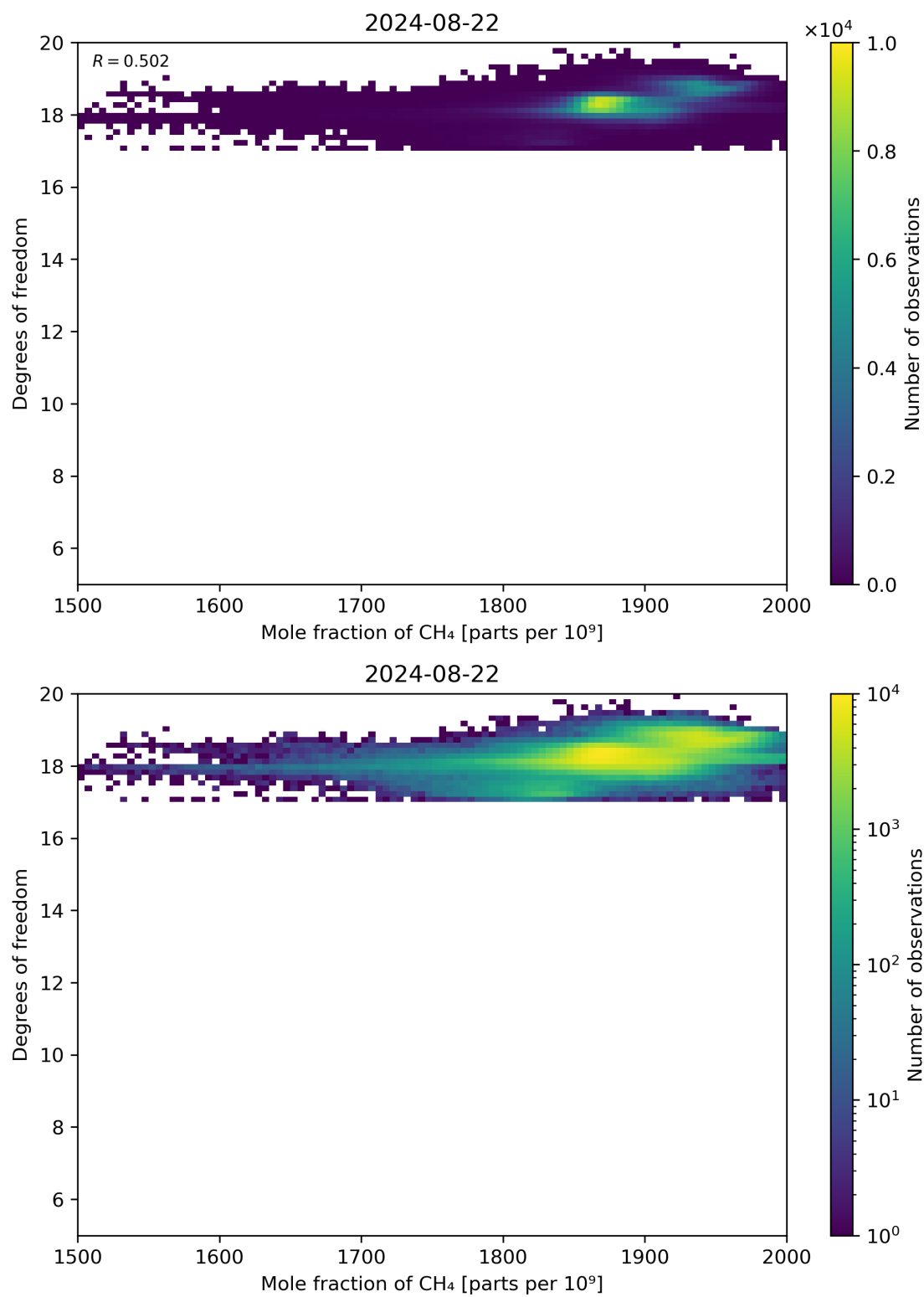
Figure 72: Scatter density plot of “Mole fraction of CH 4 ” against “Degrees of freedom” for 2024-08-22 to 2024-08-23.
