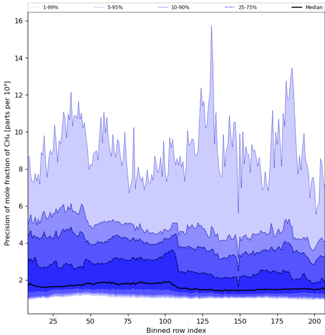
Figure 35: Along track statistics of “Precision of mole fraction of CH 4 ” for 2024-08-22 to 2024-08-23
