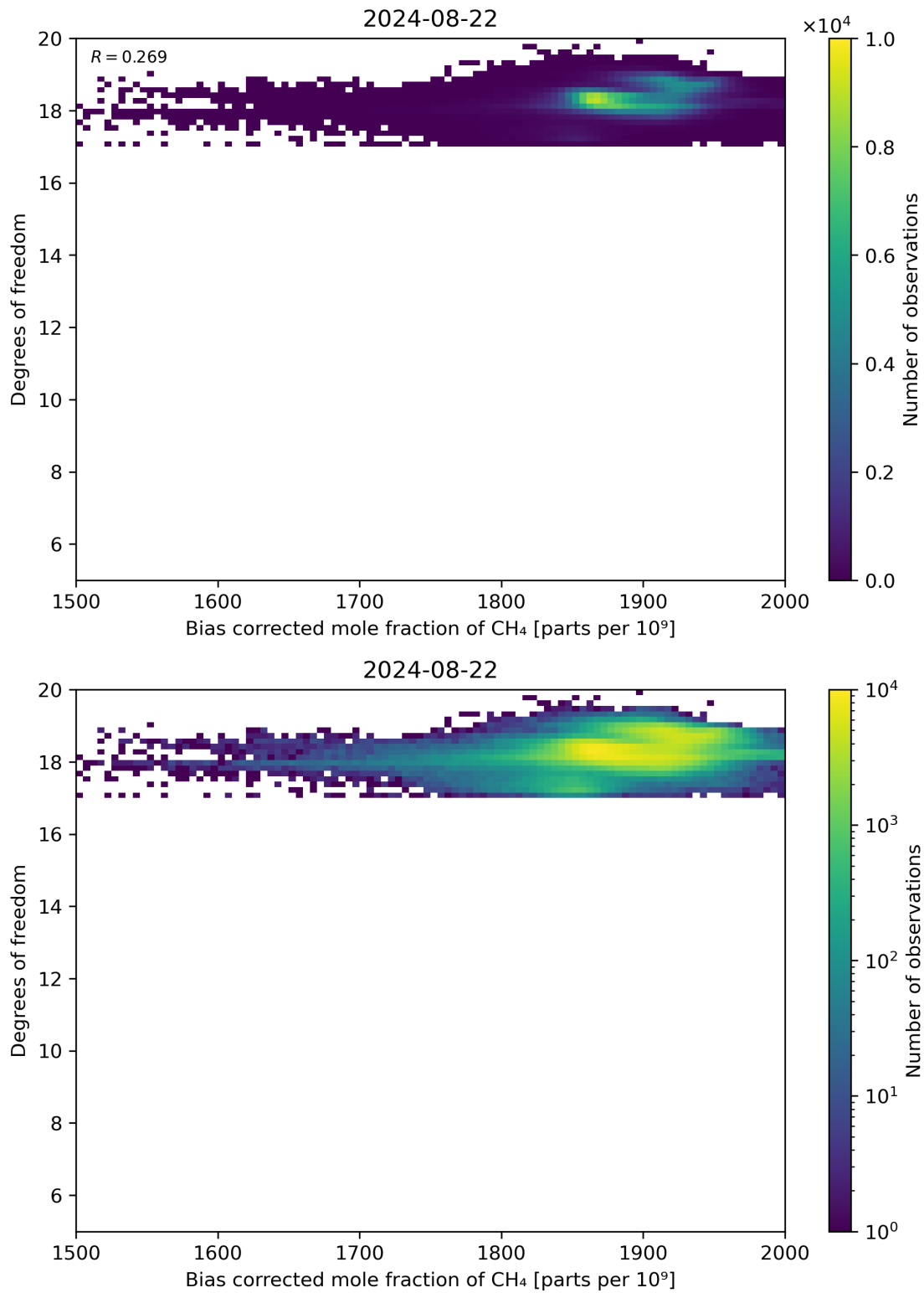
Figure 65: Scatter density plot of “Bias corrected mole fraction of CH 4 ” against “Degrees of freedom” for 2024-08-22 to 2024-08-23.
