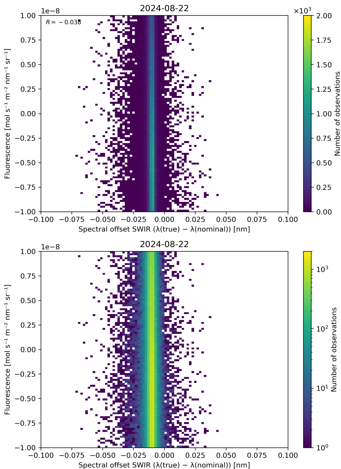
Figure 120: Scatter density plot of “Spectral offset SWIR ( \lambda(\text{true}) - \lambda(\text{nominal}) )” against “Fluorescence” for 2024-08-22 to 2024-08-23.
