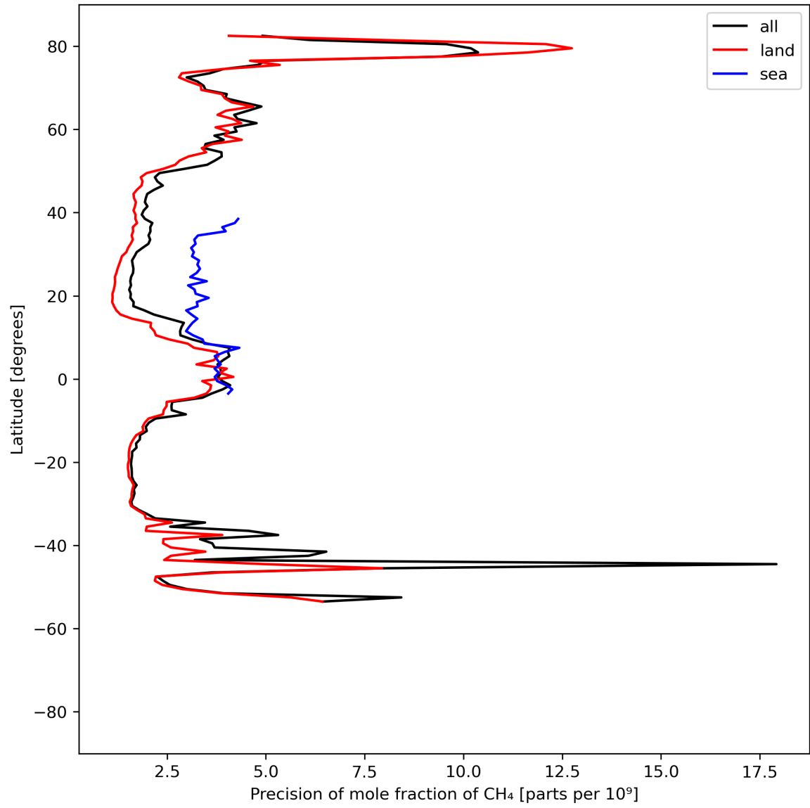
Figure 13: Zonal average of “Precision of mole fraction of CH 4 ” for 2024-08-22 to 2024-08-23.
