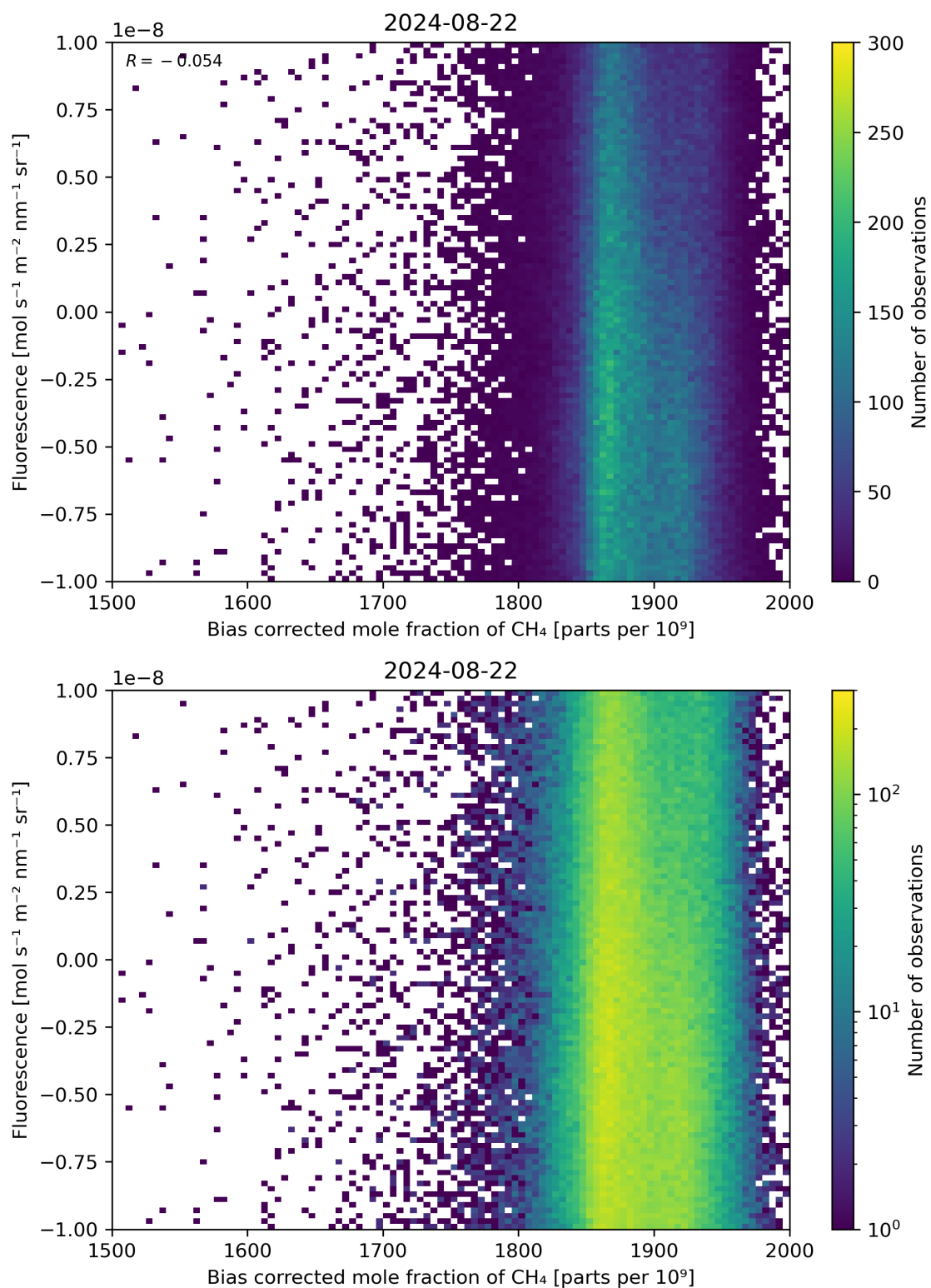
Figure 66: Scatter density plot of “Bias corrected mole fraction of \text{CH}_4 ” against “Fluorescence” for 2024-08-22 to 2024-08-23.
