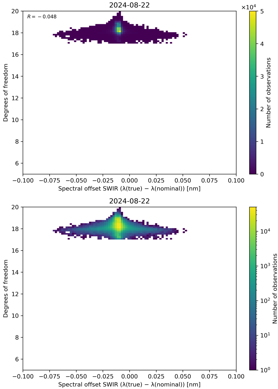
Figure 119: Scatter density plot of “Spectral offset SWIR ( \lambda(\text{true}) - \lambda(\text{nominal}) )” against “Degrees of freedom” for 2024-08-22 to 2024-08-23.
