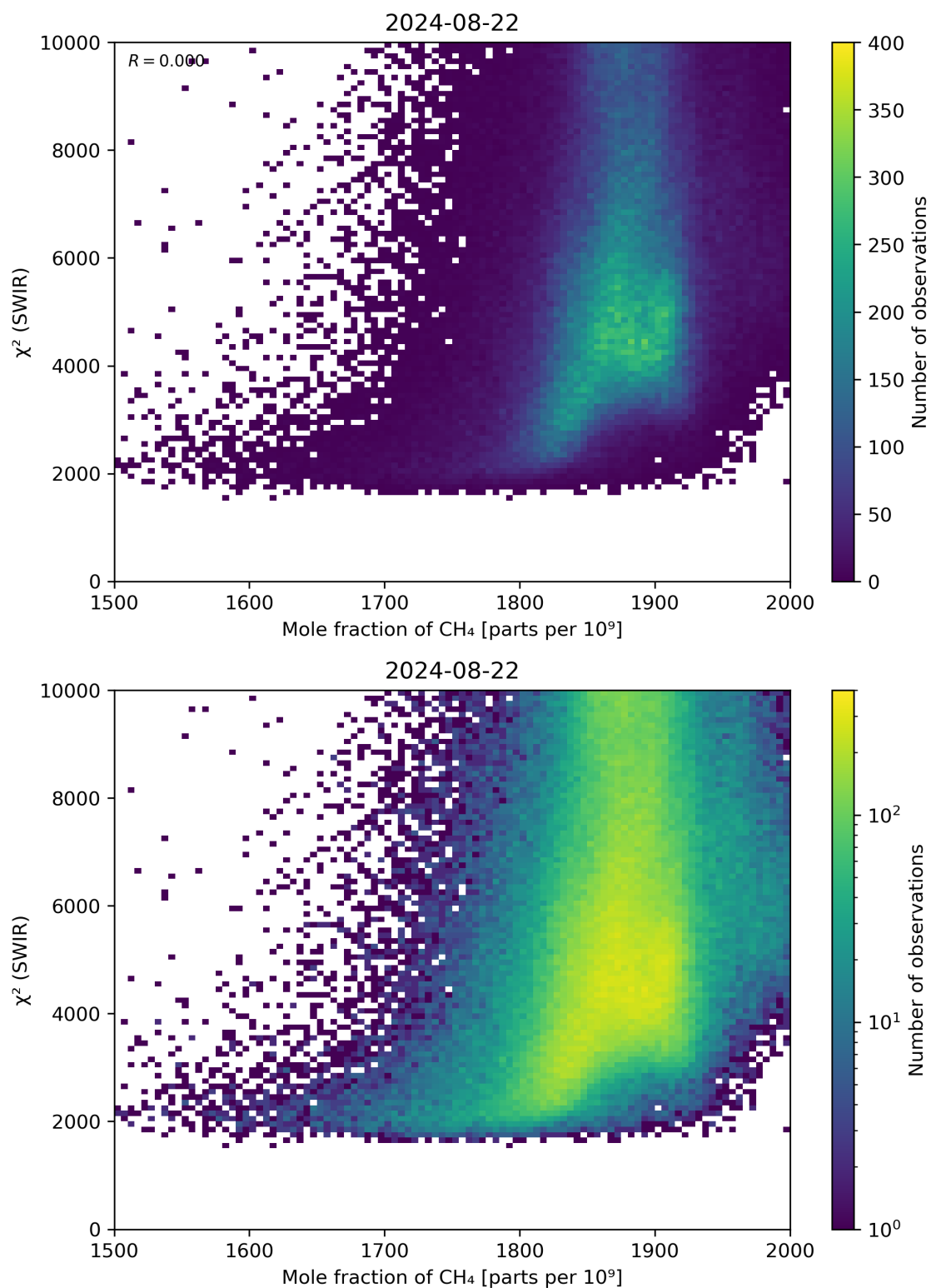
Figure 71: Scatter density plot of “Mole fraction of \text{CH}_4 ” against “ \chi^2 (SWIR)” for 2024-08-22 to 2024-08-23.
