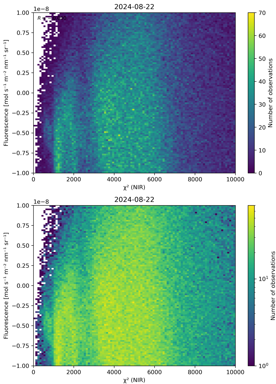
Figure 45: Scatter density plot of “ \chi^2 (NIR)” against “Fluorescence” for 2024-08-22 to 2024-08-23.
