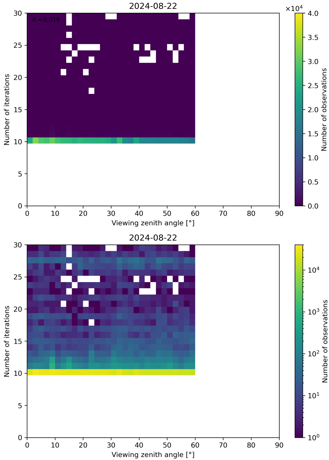
Figure 113: Scatter density plot of “Viewing zenith angle” against “Number of iterations” for 2024-08-22 to 2024-08-23.
