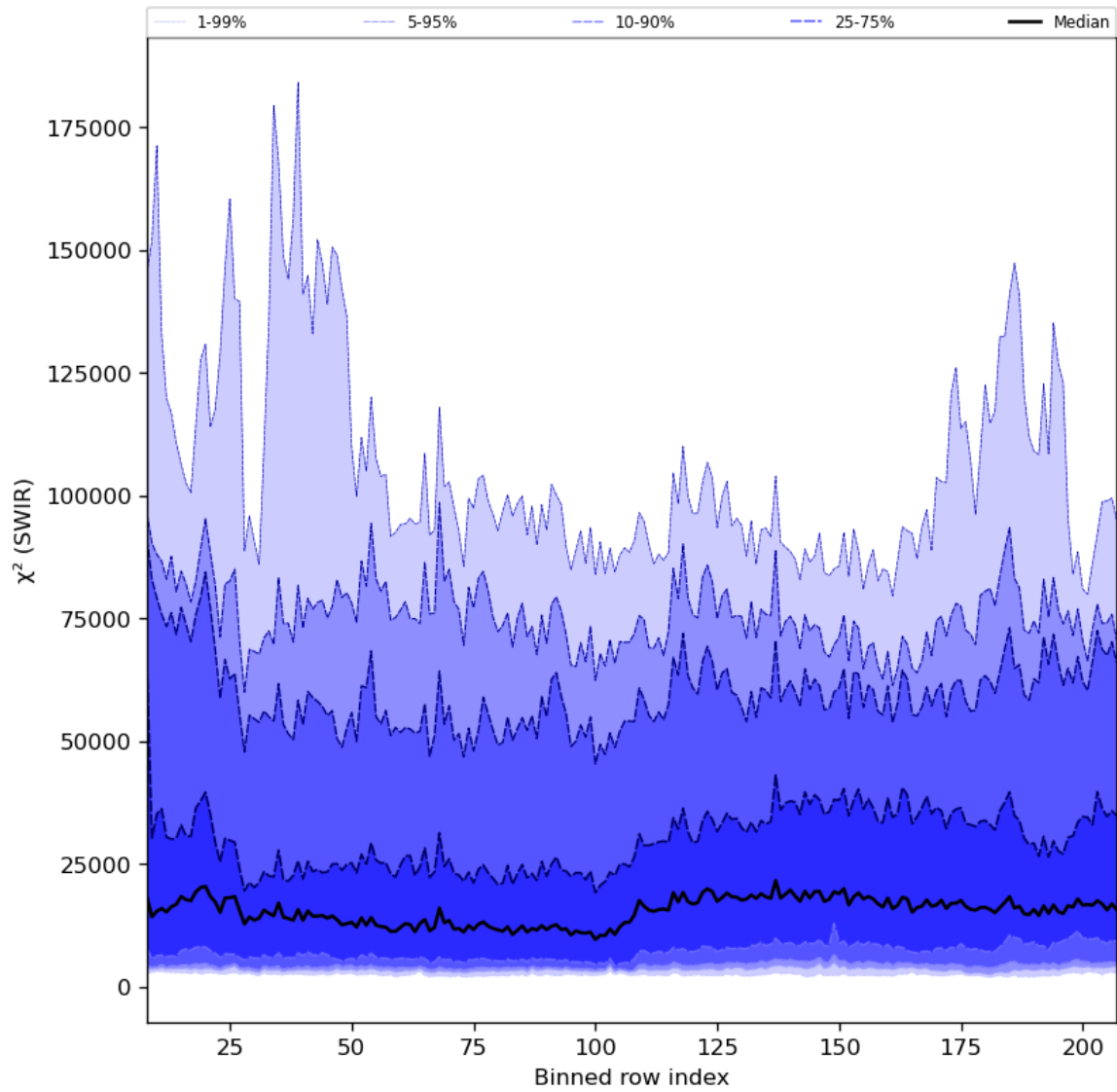
Figure 39: Along track statistics of " \chi^2 (SWIR)" for 2024-08-22 to 2024-08-23
