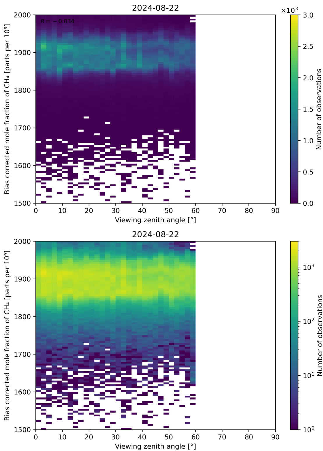
Figure 111: Scatter density plot of “Viewing zenith angle” against “Bias corrected mole fraction of CH 4 ” for 2024-08-22 to 2024-08-23.
