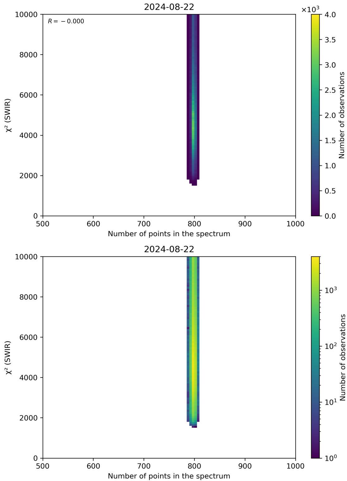
Figure 89: Scatter density plot of “Number of points in the spectrum” against “ \chi^2 (SWIR)” for 2024-08-22 to 2024-08-23.
