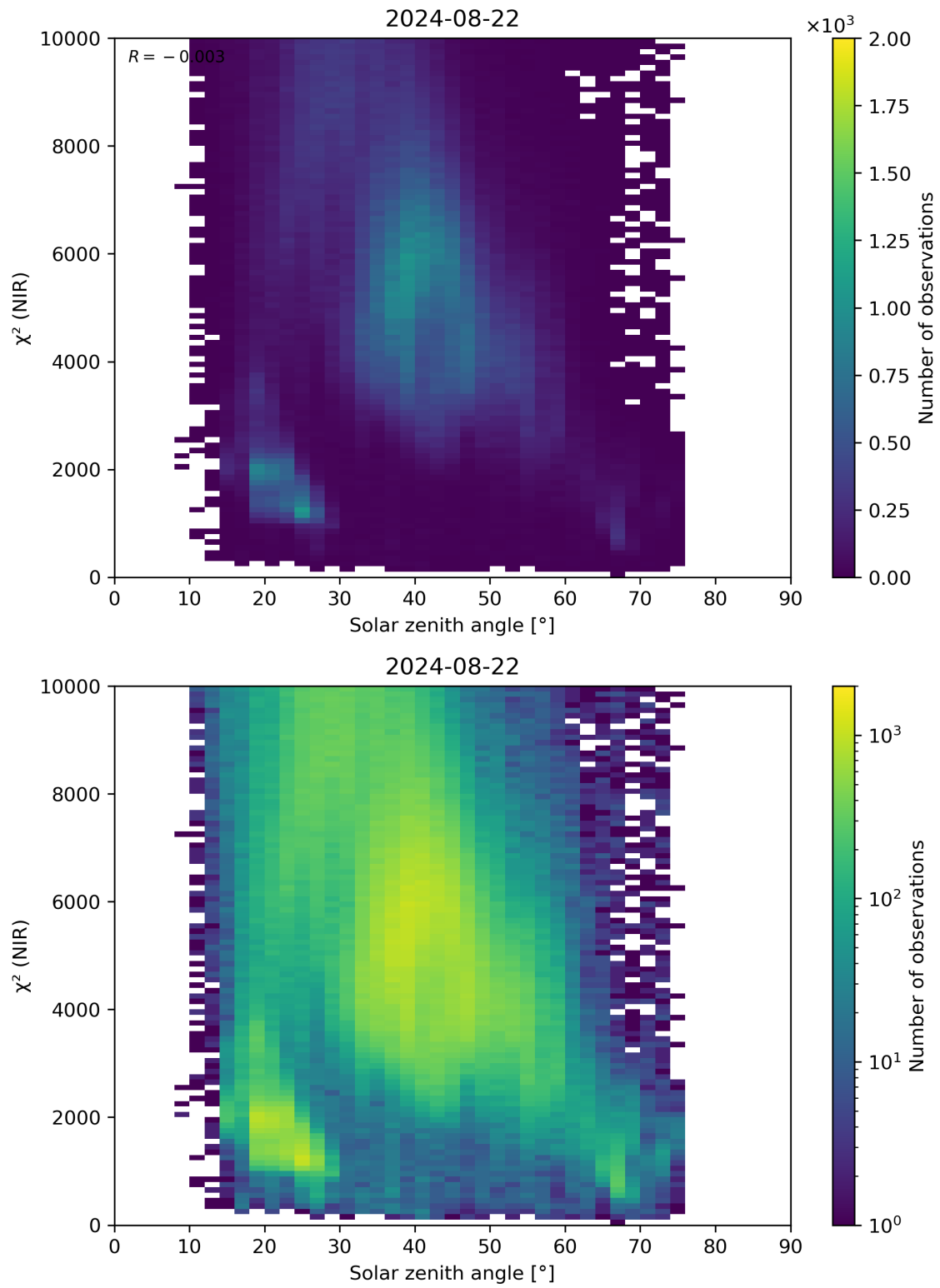
Figure 94: Scatter density plot of “Solar zenith angle” against “ \chi^2 (NIR)” for 2024-08-22 to 2024-08-23.
