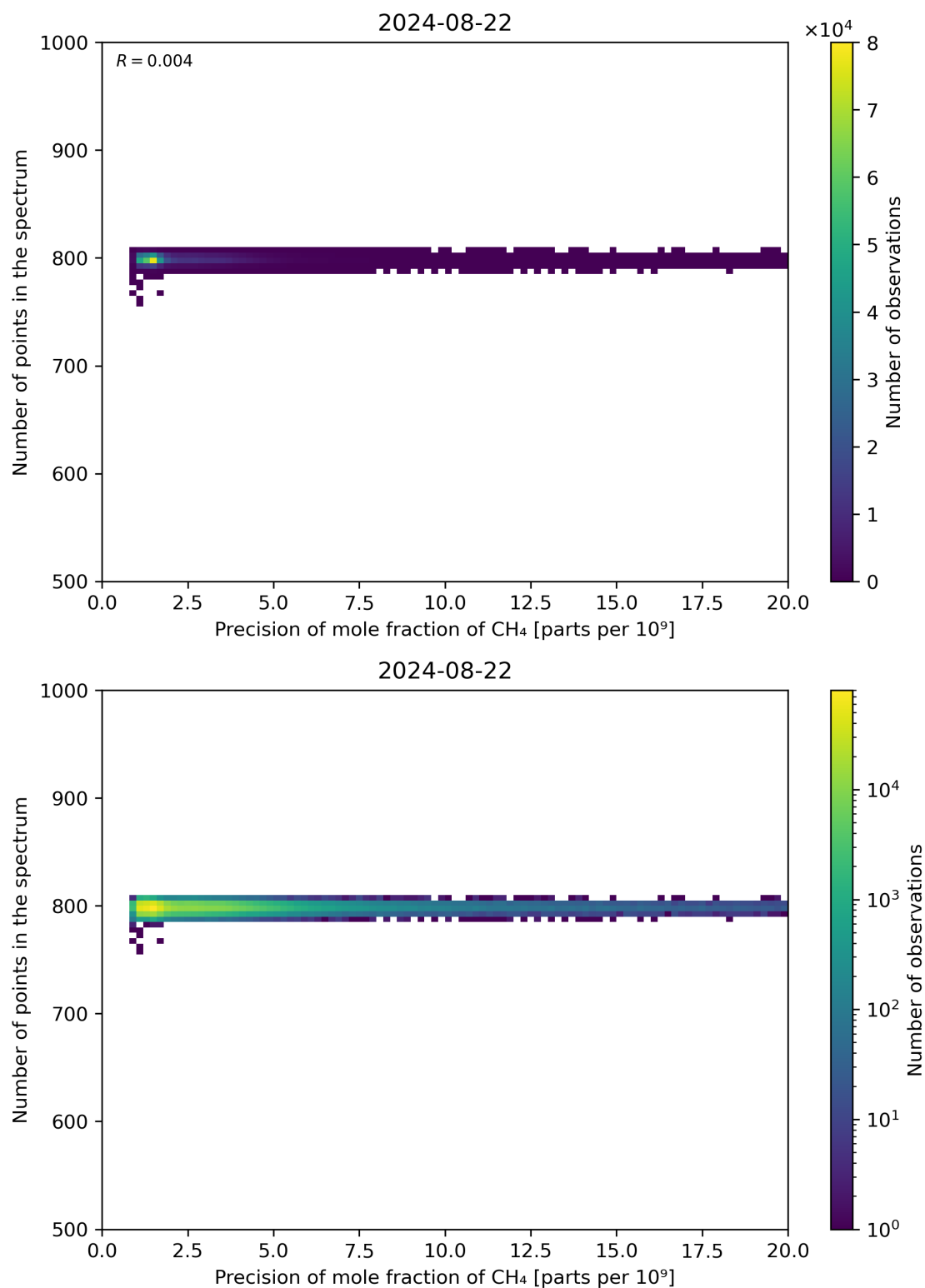
Figure 84: Scatter density plot of “Precision of mole fraction of CH 4 ” against “Number of points in the spectrum” for 2024-08-22 to 2024-08-23.
