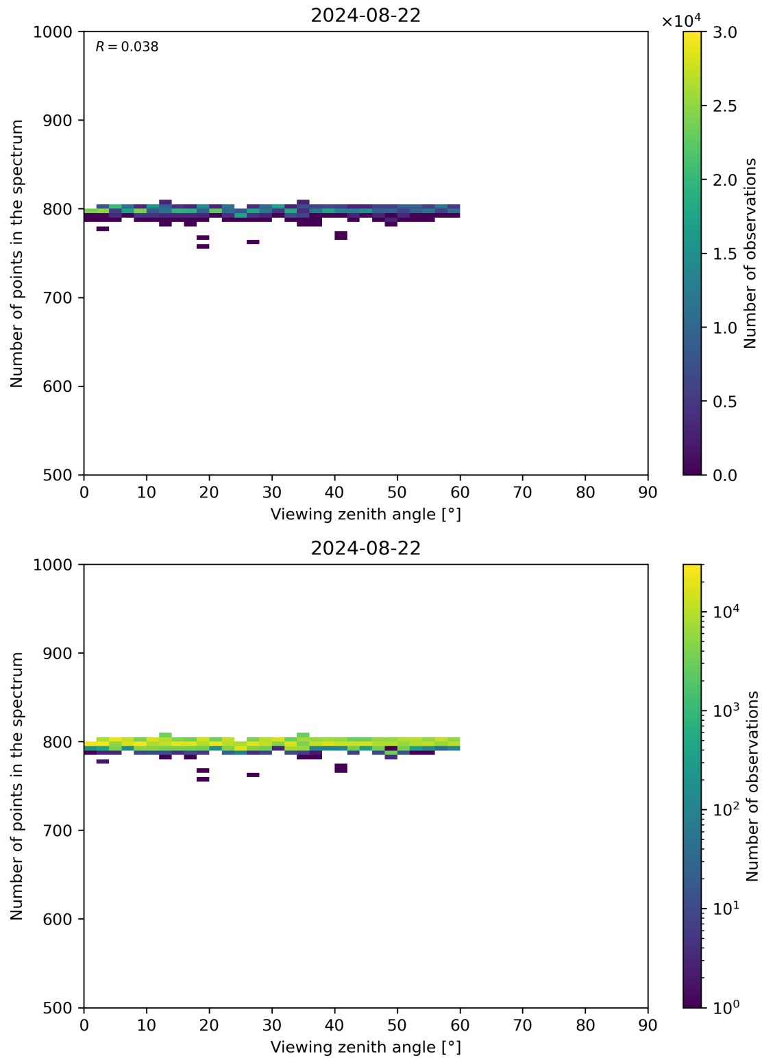
Figure 114: Scatter density plot of “Viewing zenith angle” against “Number of points in the spectrum” for 2024-08-22 to 2024-08-23.
