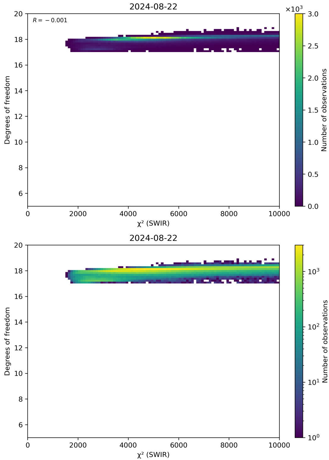
Figure 48: Scatter density plot of “ \chi^2 (SWIR)” against “Degrees of freedom” for 2024-08-22 to 2024-08-23.
