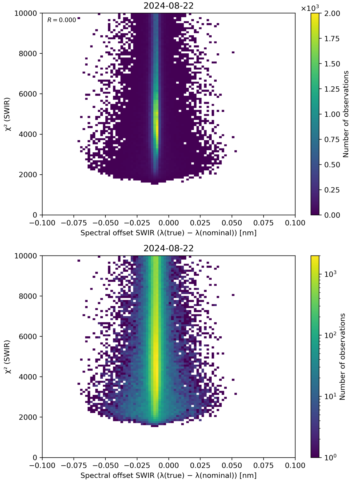
Figure 118: Scatter density plot of “Spectral offset SWIR ( \lambda(\text{true}) - \lambda(\text{nominal}) )” against “ \chi^2 (SWIR)” for 2024-08-22 to 2024-08-23.
