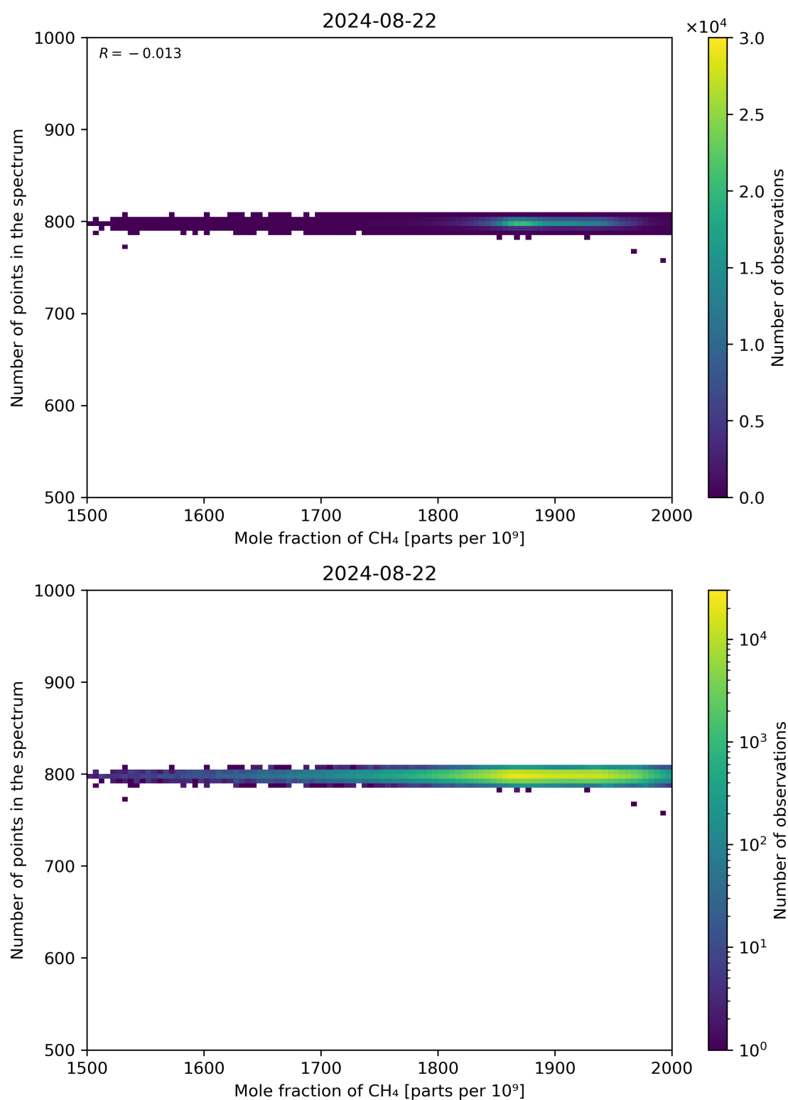
Figure 77: Scatter density plot of “Mole fraction of CH 4 ” against “Number of points in the spectrum” for 2024-08-22 to 2024-08-23.
