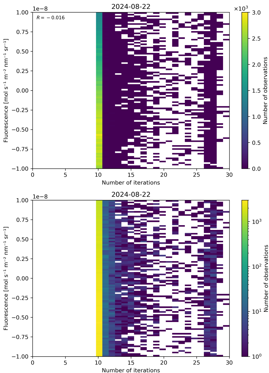
Figure 87: Scatter density plot of “Number of iterations” against “Fluorescence” for 2024-08-22 to 2024-08-23.
