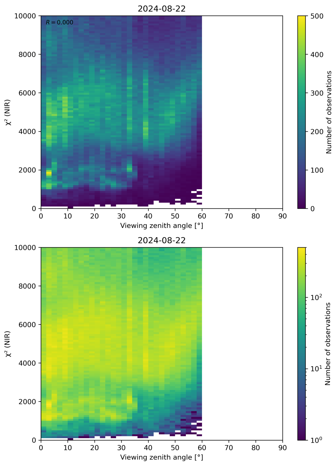
Figure 105: Scatter density plot of “Viewing zenith angle” against “ \chi^2 (NIR)” for 2024-08-22 to 2024-08-23.
