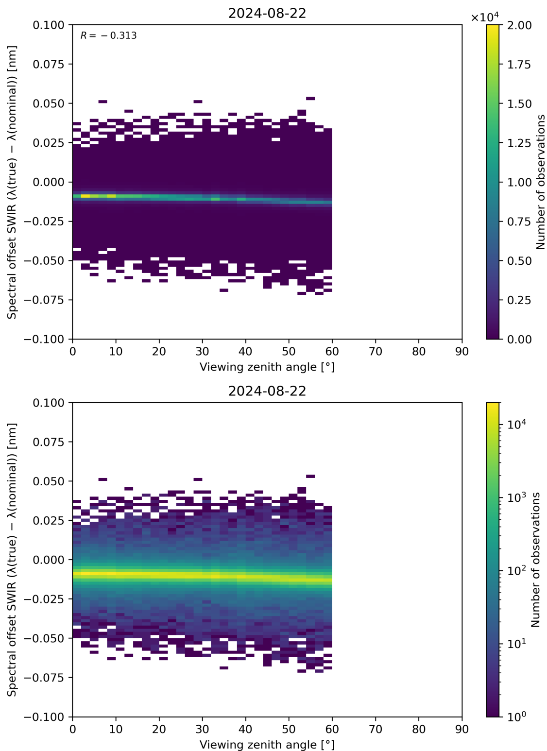
Figure 116: Scatter density plot of “Viewing zenith angle” against “Spectral offset SWIR ( \lambda(\text{true}) - \lambda(\text{nominal}) )” for 2024-08-22 to 2024-08-23.
