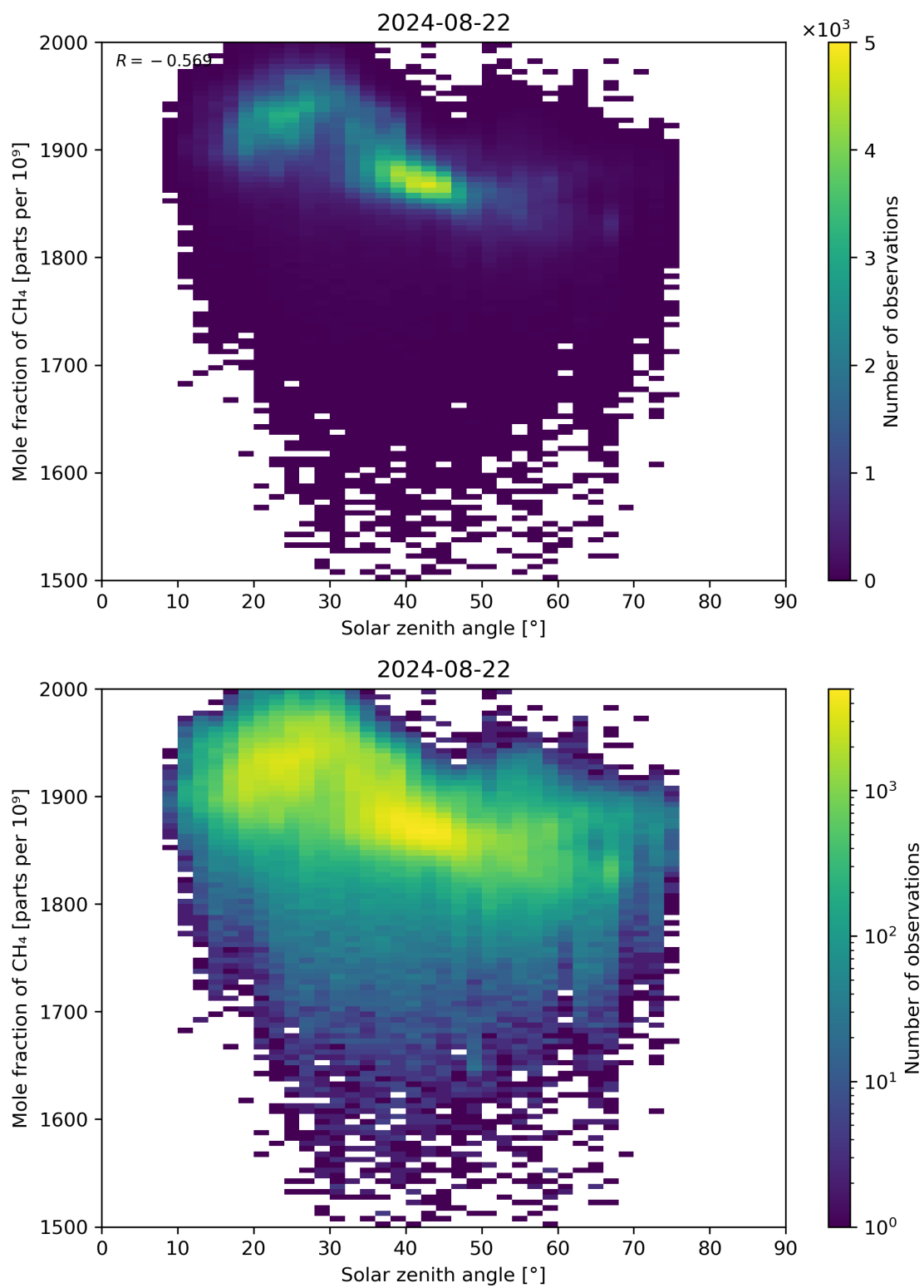
Figure 99: Scatter density plot of “Solar zenith angle” against “Mole fraction of CH 4 ” for 2024-08-22 to 2024-08-23.
