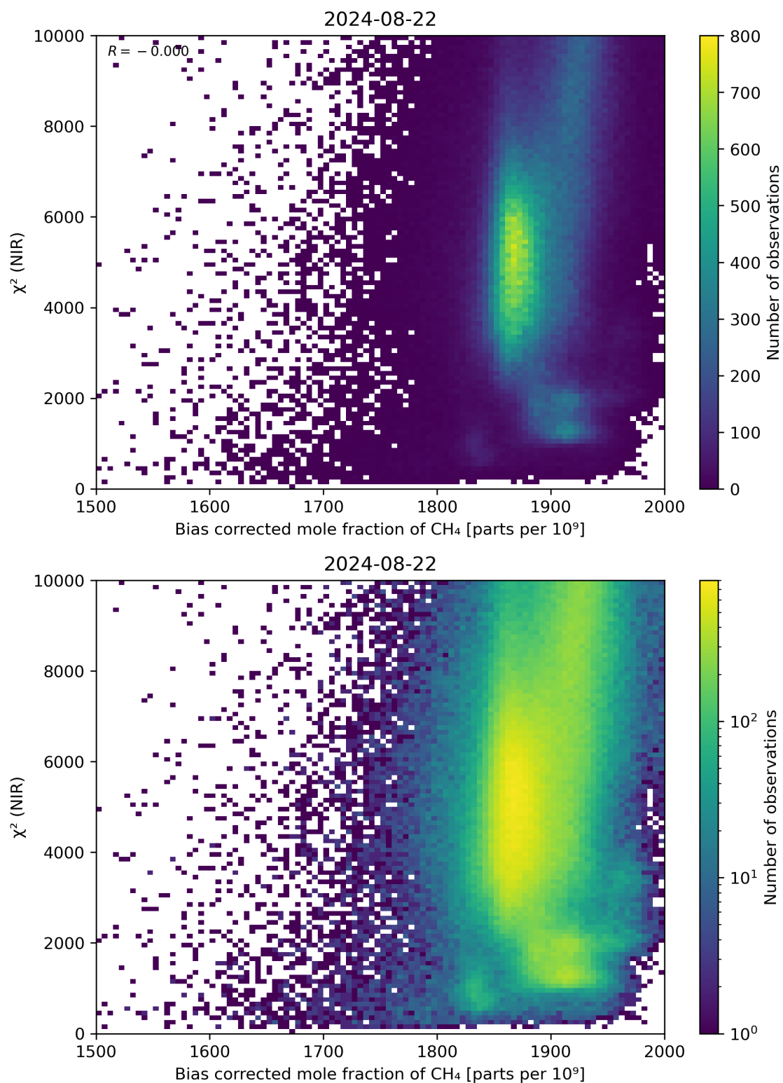
Figure 63: Scatter density plot of “Bias corrected mole fraction of CH 4 ” against “ \chi^2 (NIR)” for 2024-08-22 to 2024-08-23.
