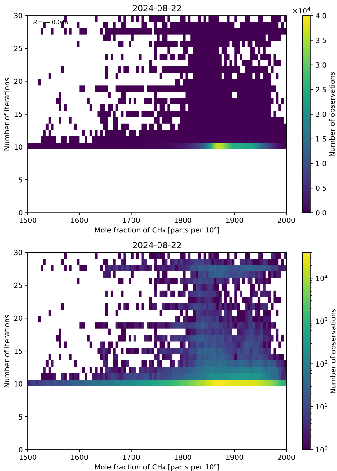
Figure 76: Scatter density plot of “Mole fraction of CH 4 ” against “Number of iterations” for 2024-08-22 to 2024-08-23.
