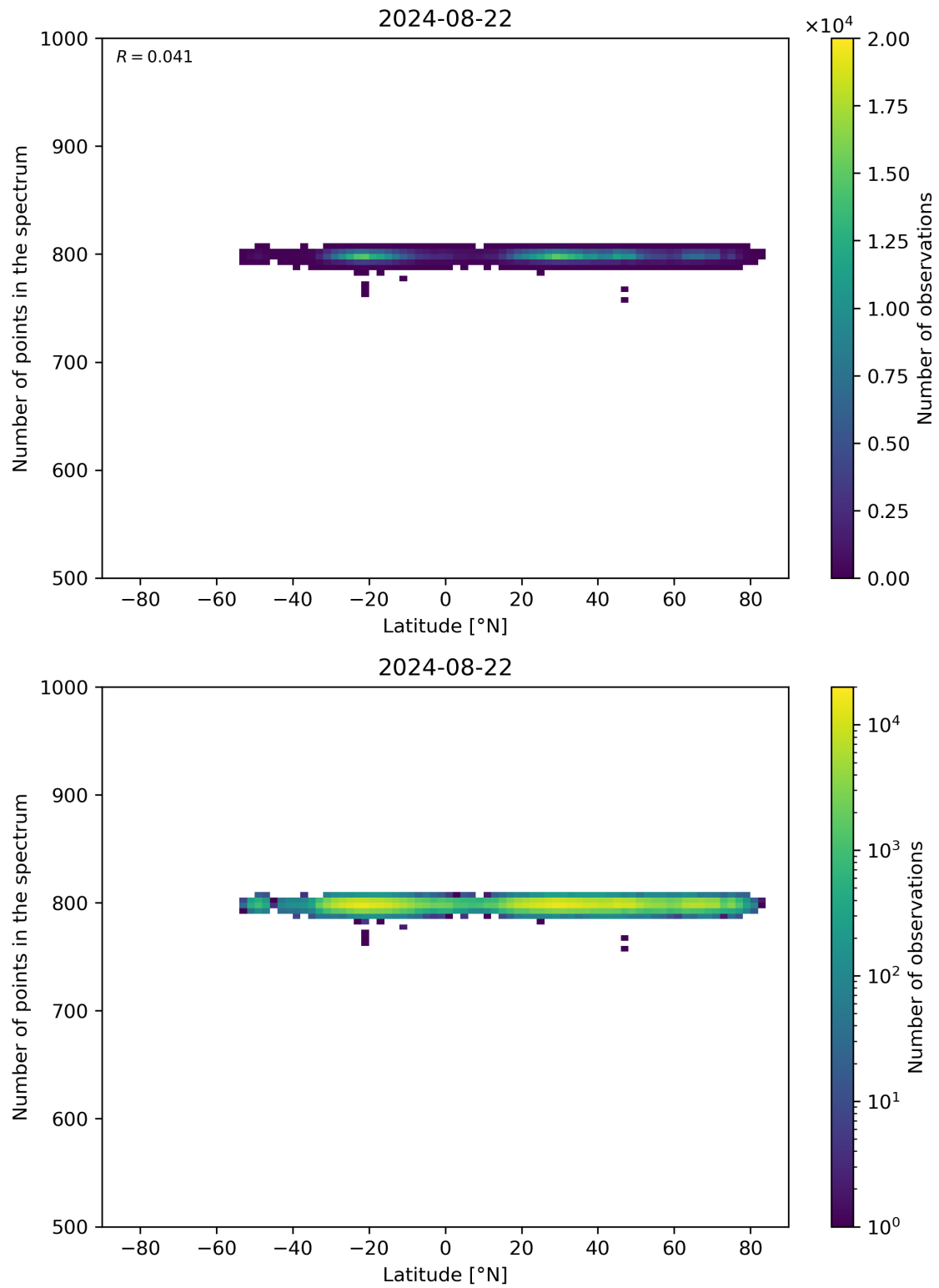
Figure 61: Scatter density plot of “Latitude” against “Number of points in the spectrum” for 2024-08-22 to 2024-08-23.
