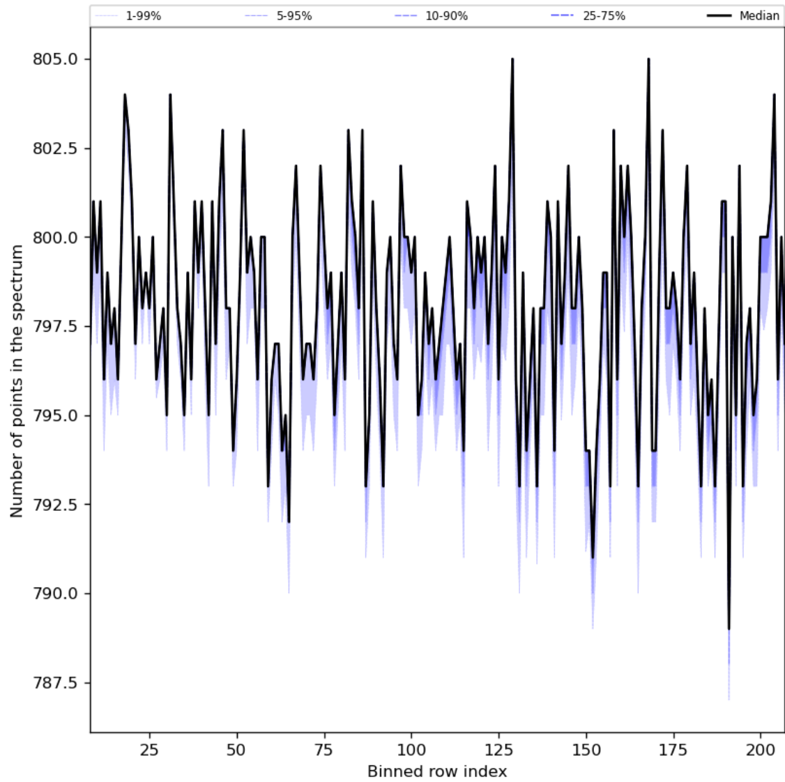
Figure 37: Along track statistics of “Number of points in the spectrum” for 2024-08-22 to 2024-08-23
