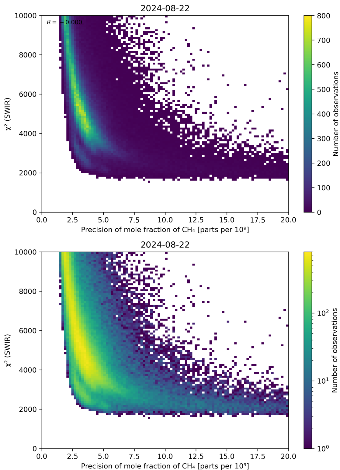
Figure 79: Scatter density plot of “Precision of mole fraction of \text{CH}_4 ” against “ \chi^2 (SWIR)” for 2024-08-22 to 2024-08-23.
