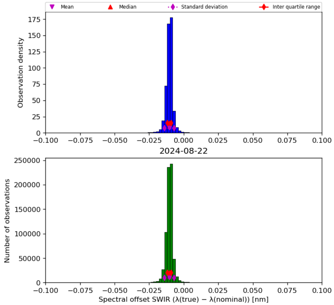
Figure 27: Histogram of “Spectral offset SWIR ( \lambda(\text{true}) - \lambda(\text{nominal}) )” for 2024-08-22 to 2024-08-23
