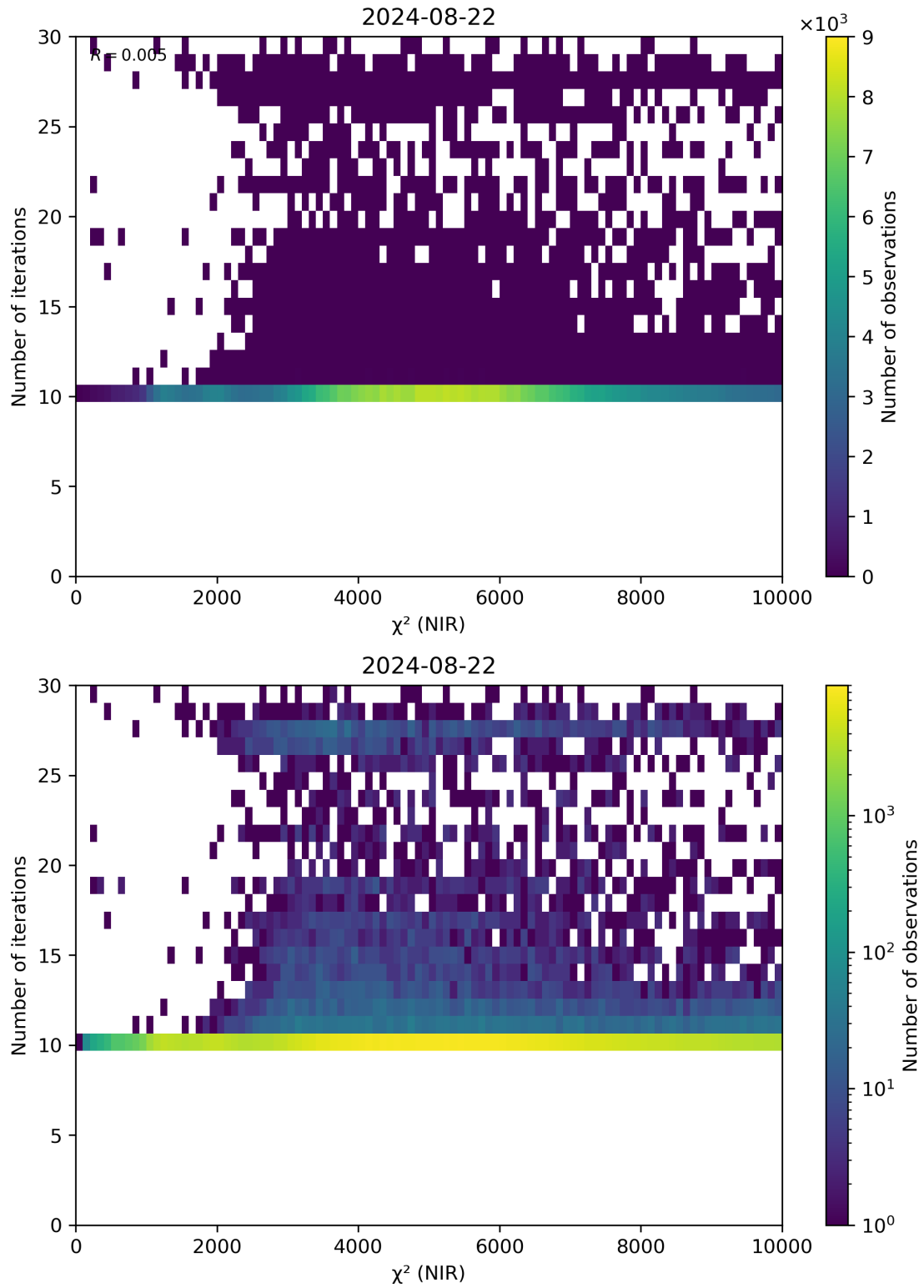
Figure 46: Scatter density plot of “ \chi^2 (NIR)” against “Number of iterations” for 2024-08-22 to 2024-08-23.
