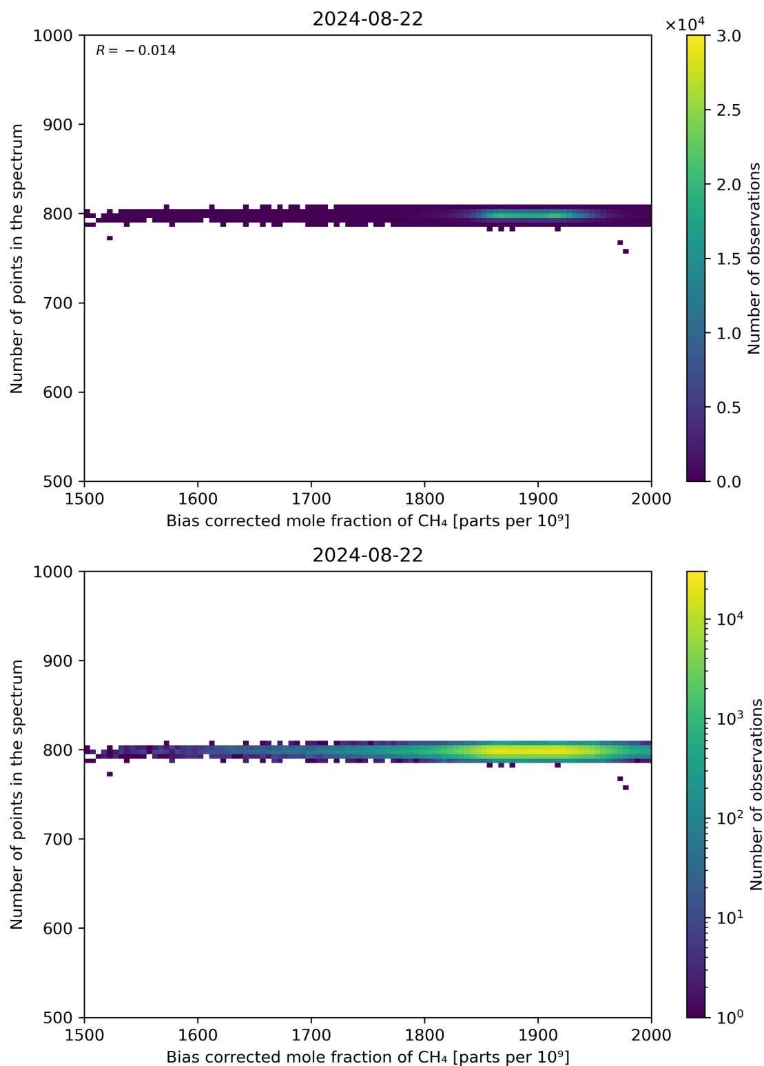
Figure 68: Scatter density plot of “Bias corrected mole fraction of CH 4 ” against “Number of points in the spectrum” for 2024-08-22 to 2024-08-23.
