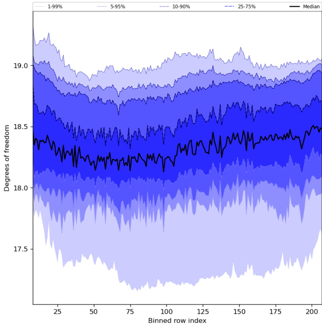
Figure 41: Along track statistics of “Degrees of freedom” for 2024-08-22 to 2024-08-23
