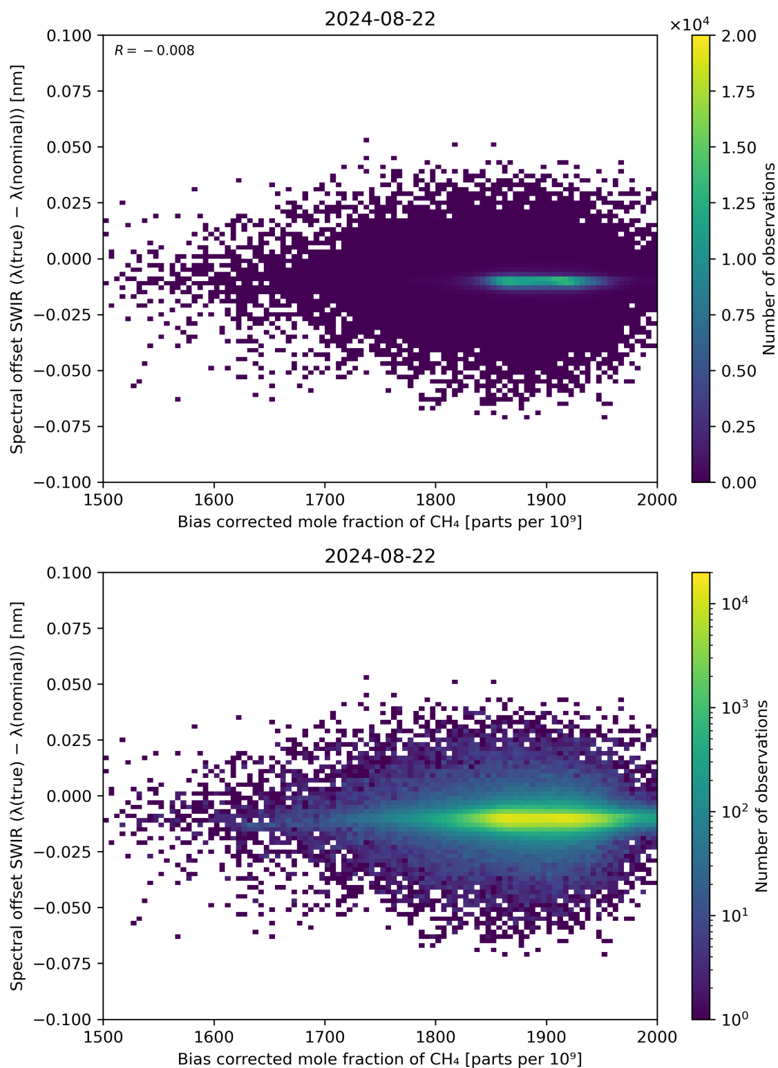
Figure 69: Scatter density plot of “Bias corrected mole fraction of \text{CH}_4 ” against “Spectral offset SWIR ( \lambda(\text{true}) - \lambda(\text{nominal}) )” for 2024-08-22 to 2024-08-23.
