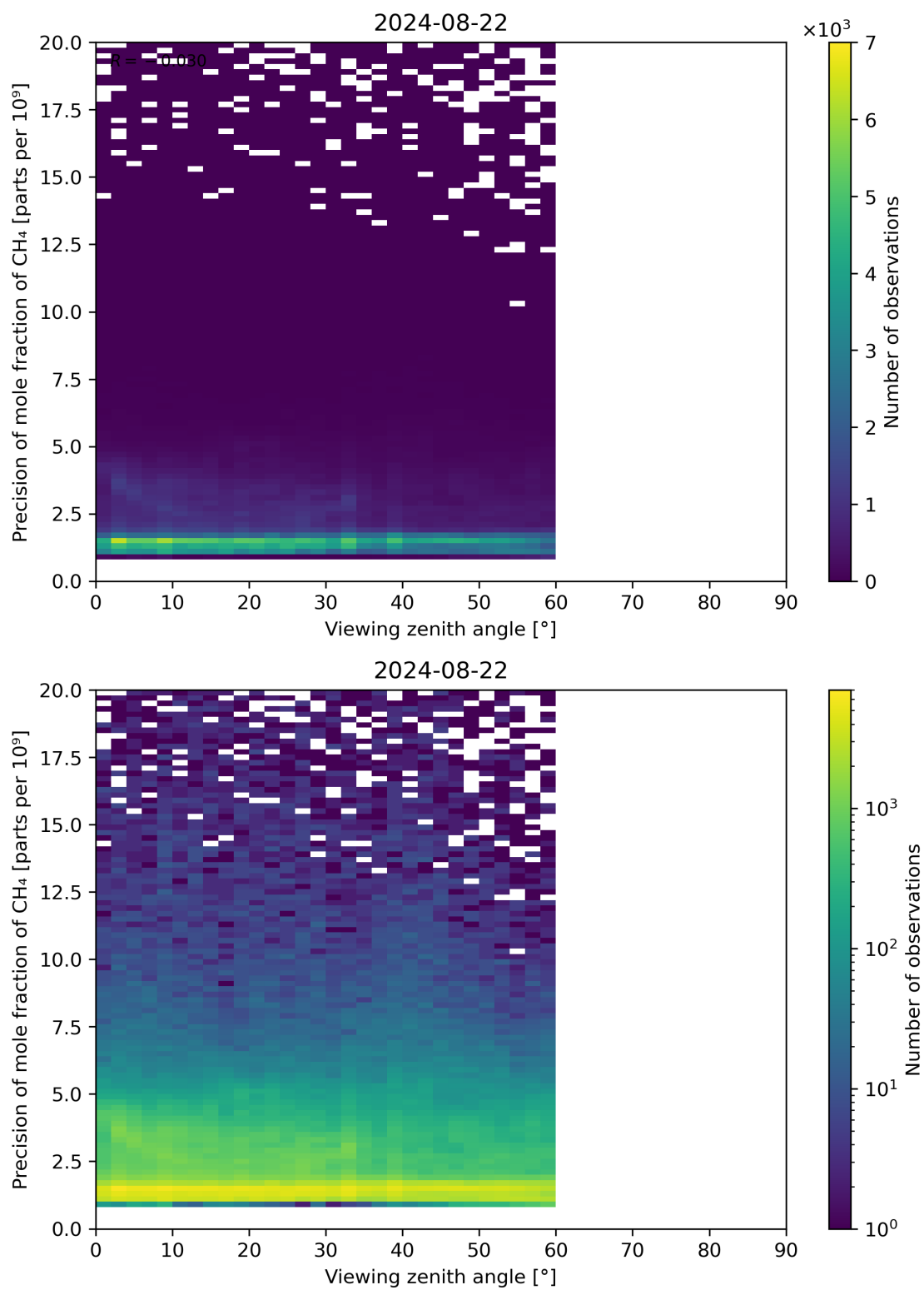
Figure 112: Scatter density plot of “Viewing zenith angle” against “Precision of mole fraction of CH 4 ” for 2024-08-22 to 2024-08-23.
