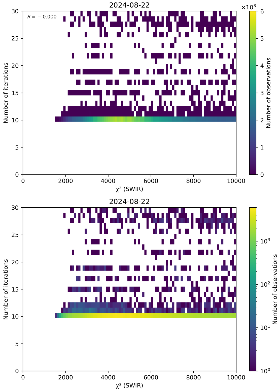
Figure 50: Scatter density plot of “ \chi^2 (SWIR)” against “Number of iterations” for 2024-08-22 to 2024-08-23.
