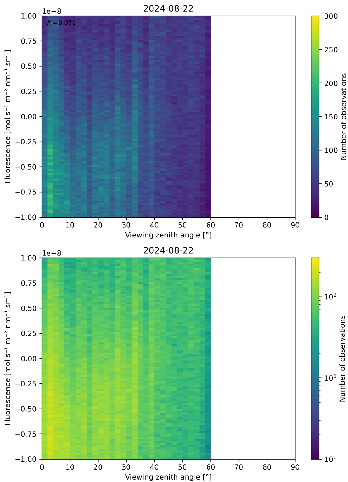
Figure 108: Scatter density plot of “Viewing zenith angle” against “Fluorescence” for 2024-08-22 to 2024-08-23.
