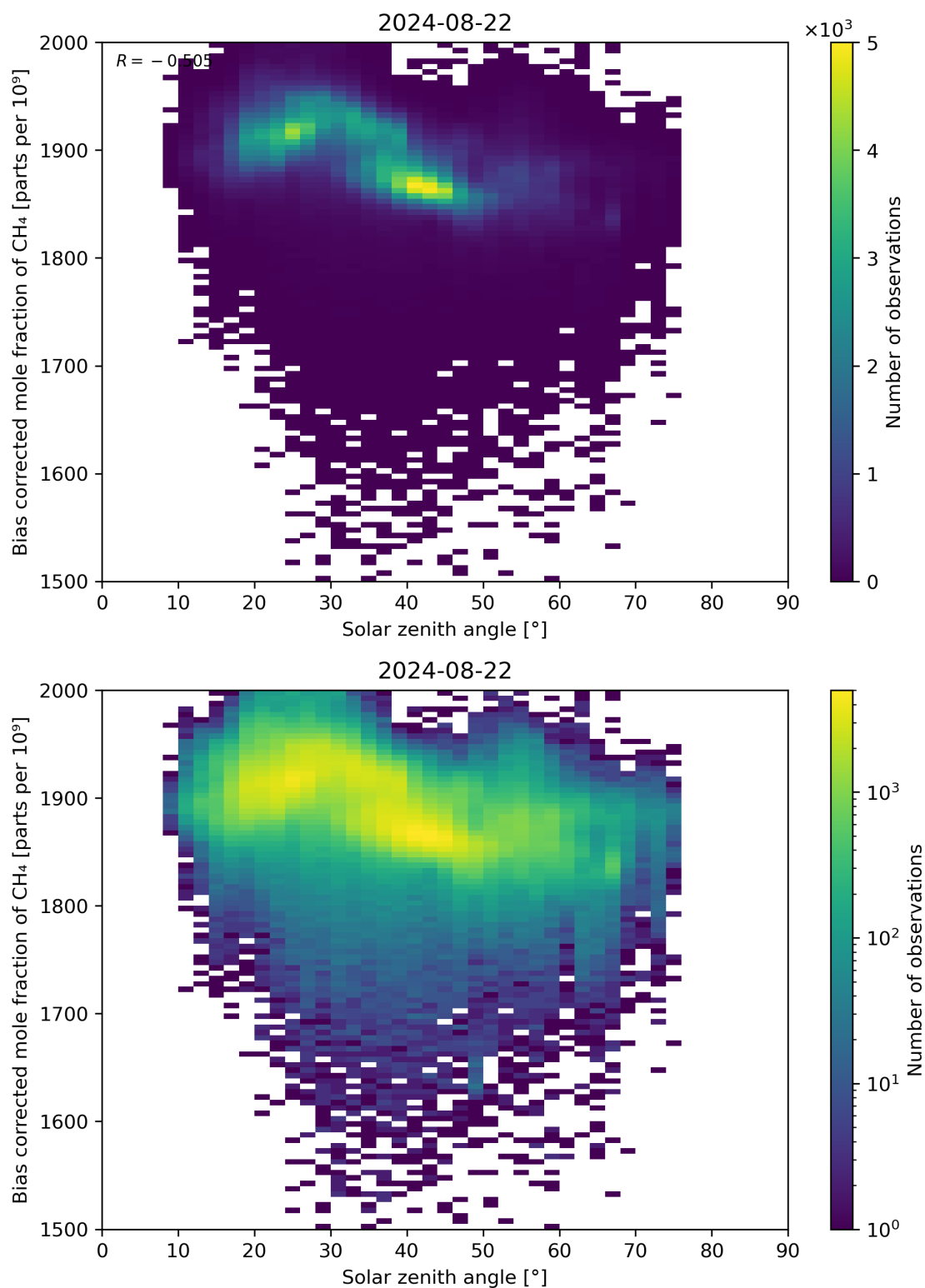
Figure 100: Scatter density plot of “Solar zenith angle” against “Bias corrected mole fraction of CH 4 ” for 2024-08-22 to 2024-08-23.
