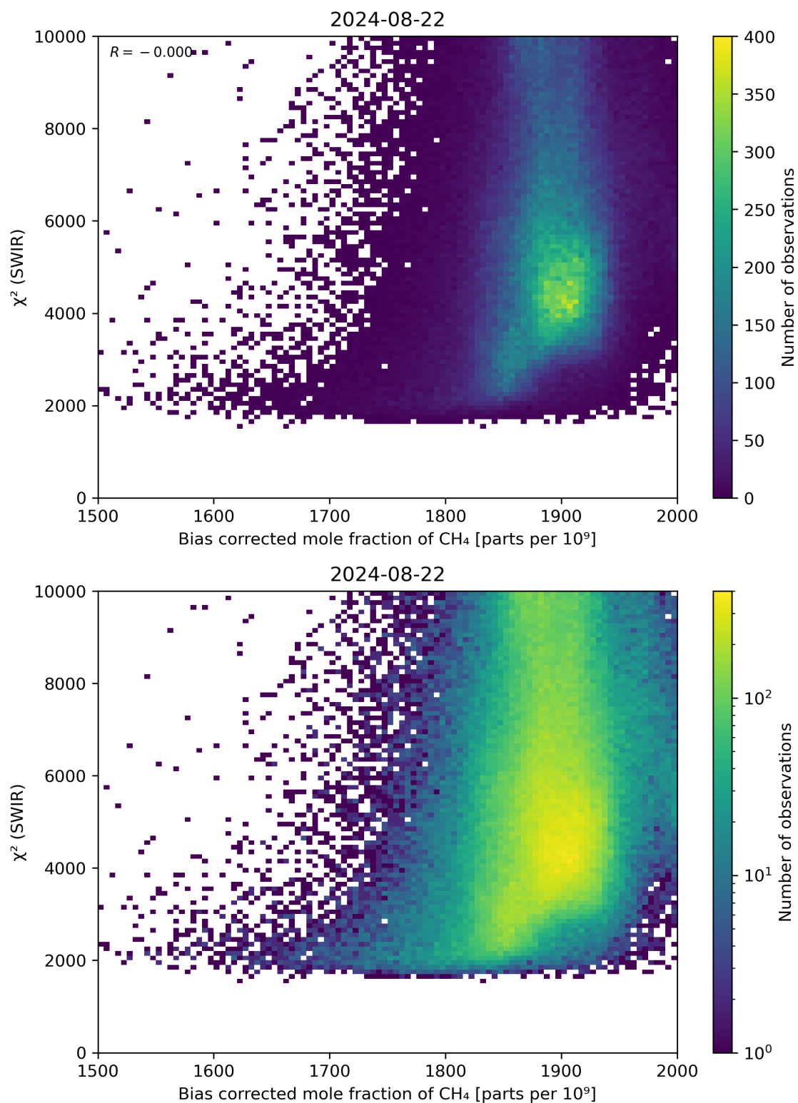
Figure 64: Scatter density plot of “Bias corrected mole fraction of CH 4 ” against “ \chi^2 (SWIR)” for 2024-08-22 to 2024-08-23.
