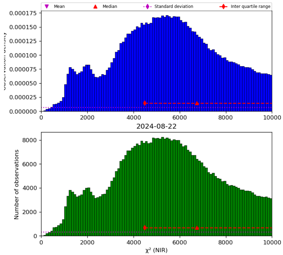
Figure 29: Histogram of “ \chi^2 (NIR)” for 2024-08-22 to 2024-08-23
