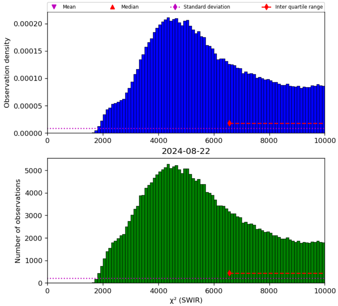
Figure 28: Histogram of “ \chi^2 (SWIR)” for 2024-08-22 to 2024-08-23
