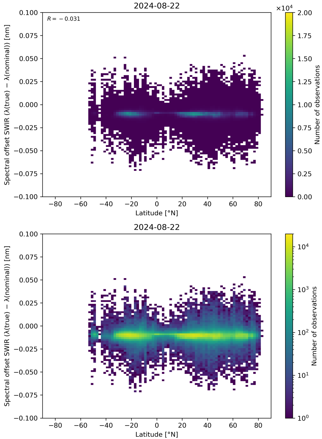
Figure 62: Scatter density plot of “Latitude” against “Spectral offset SWIR ( \lambda(\text{true}) - \lambda(\text{nominal}) )” for 2024-08-22 to 2024-08-23.
