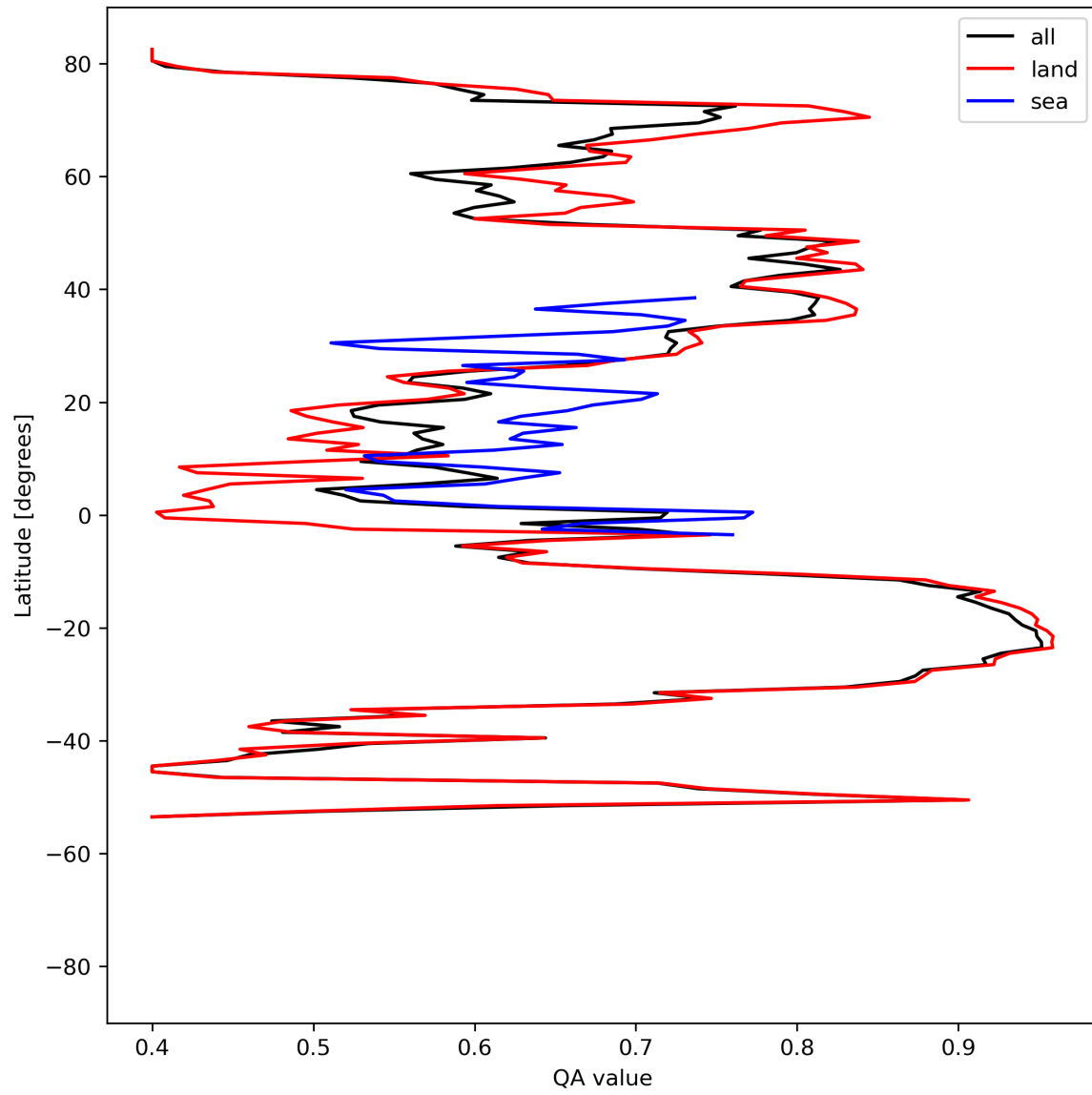
Figure 11: Zonal average of “QA value” for 2024-08-22 to 2024-08-23.
