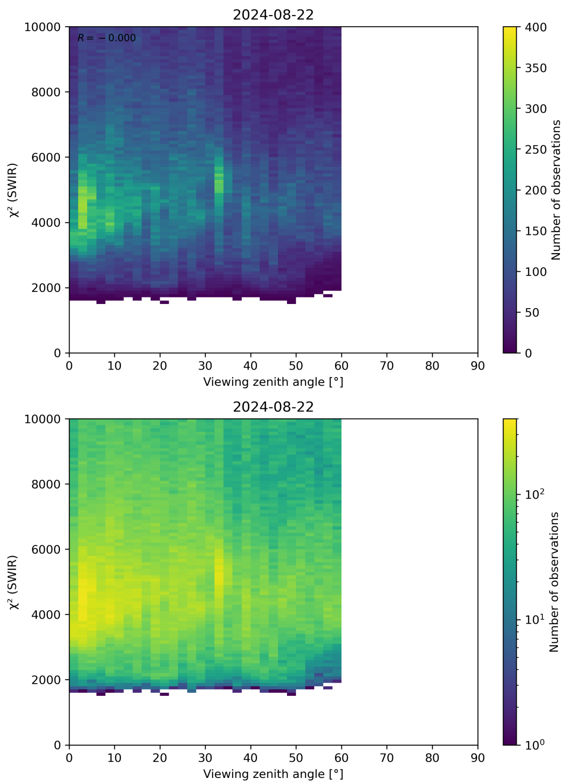
Figure 106: Scatter density plot of “Viewing zenith angle” against “ \chi^2 (SWIR)” for 2024-08-22 to 2024-08-23.
