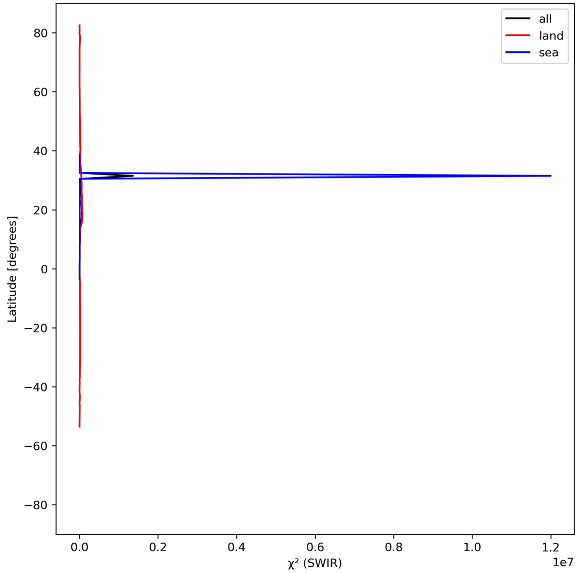
Figure 17: Zonal average of “ \chi^2 (SWIR)” for 2024-08-22 to 2024-08-23.
