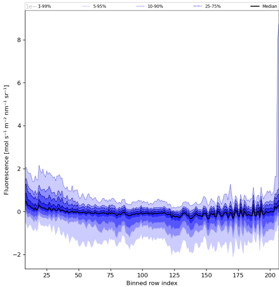
Figure 43: Along track statistics of “Fluorescence” for 2024-08-22 to 2024-08-23
