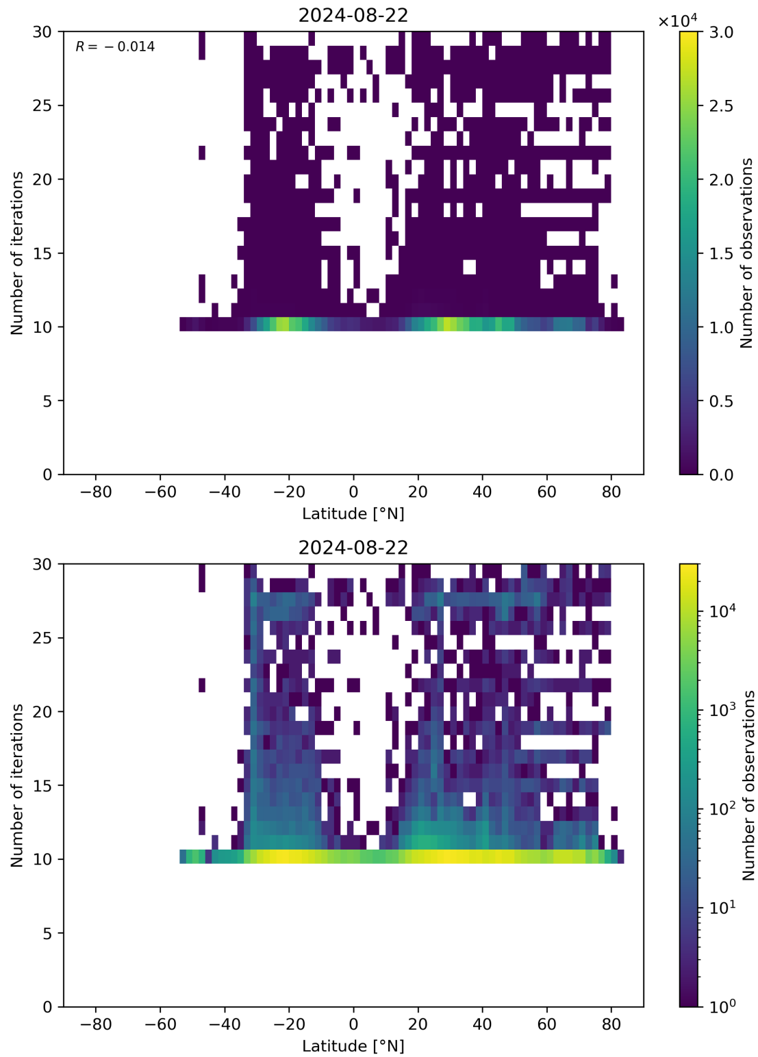
Figure 60: Scatter density plot of “Latitude” against “Number of iterations” for 2024-08-22 to 2024-08-23.
