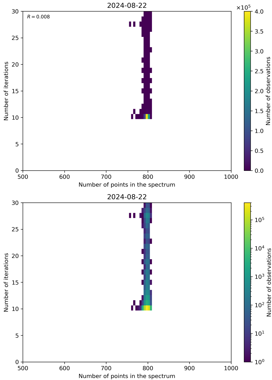
Figure 92: Scatter density plot of “Number of points in the spectrum” against “Number of iterations” for 2024-08-22 to 2024-08-23.
