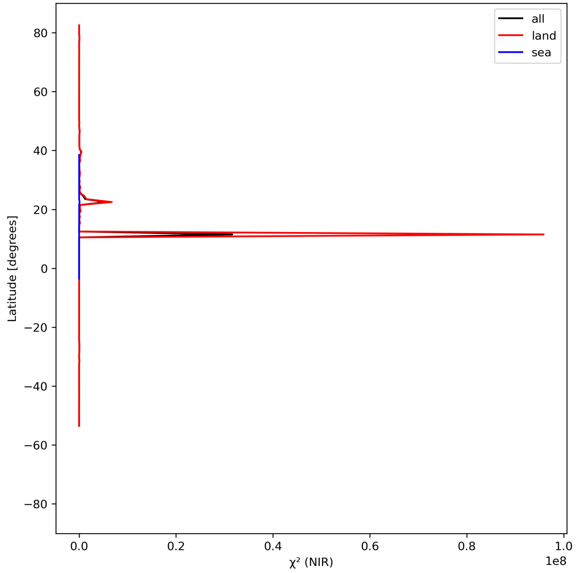
Figure 18: Zonal average of “ \chi^2 (NIR)” for 2024-08-22 to 2024-08-23.
