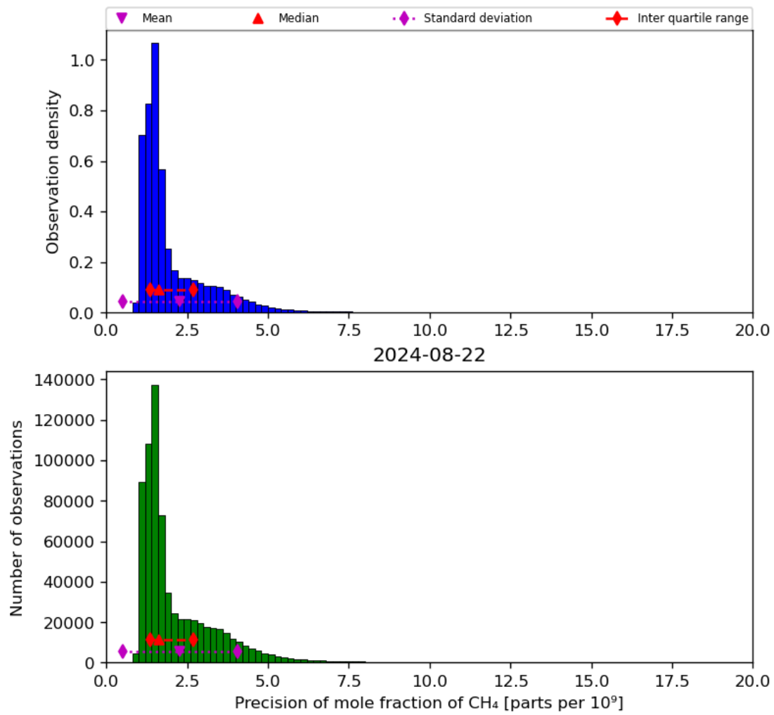
Figure 24: Histogram of “Precision of mole fraction of CH 4 ” for 2024-08-22 to 2024-08-23
