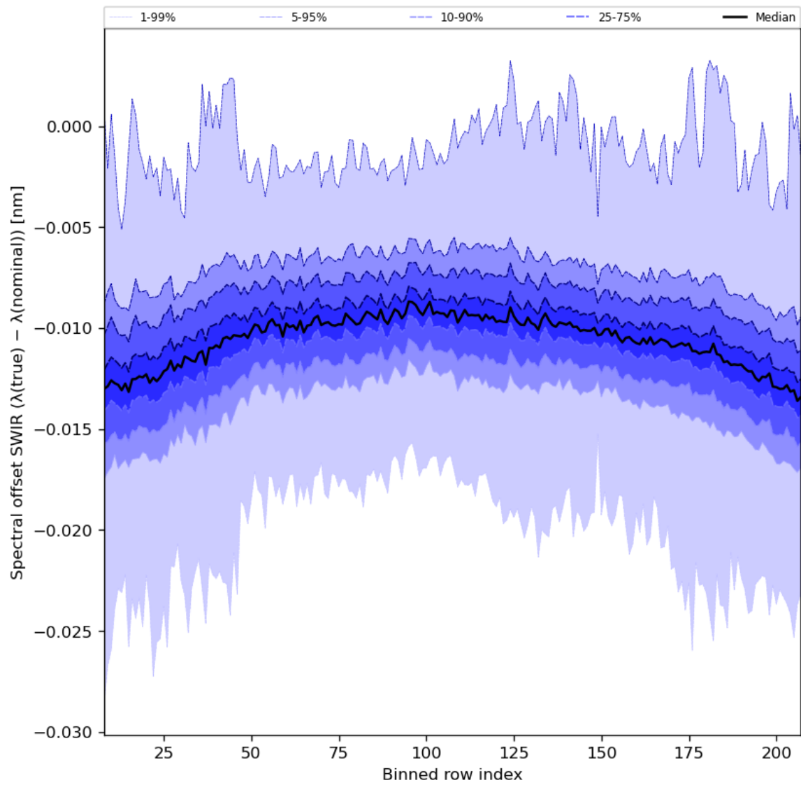
Figure 38: Along track statistics of “Spectral offset SWIR ( \lambda(\text{true}) - \lambda(\text{nominal}) )” for 2024-08-22 to 2024-08-23
