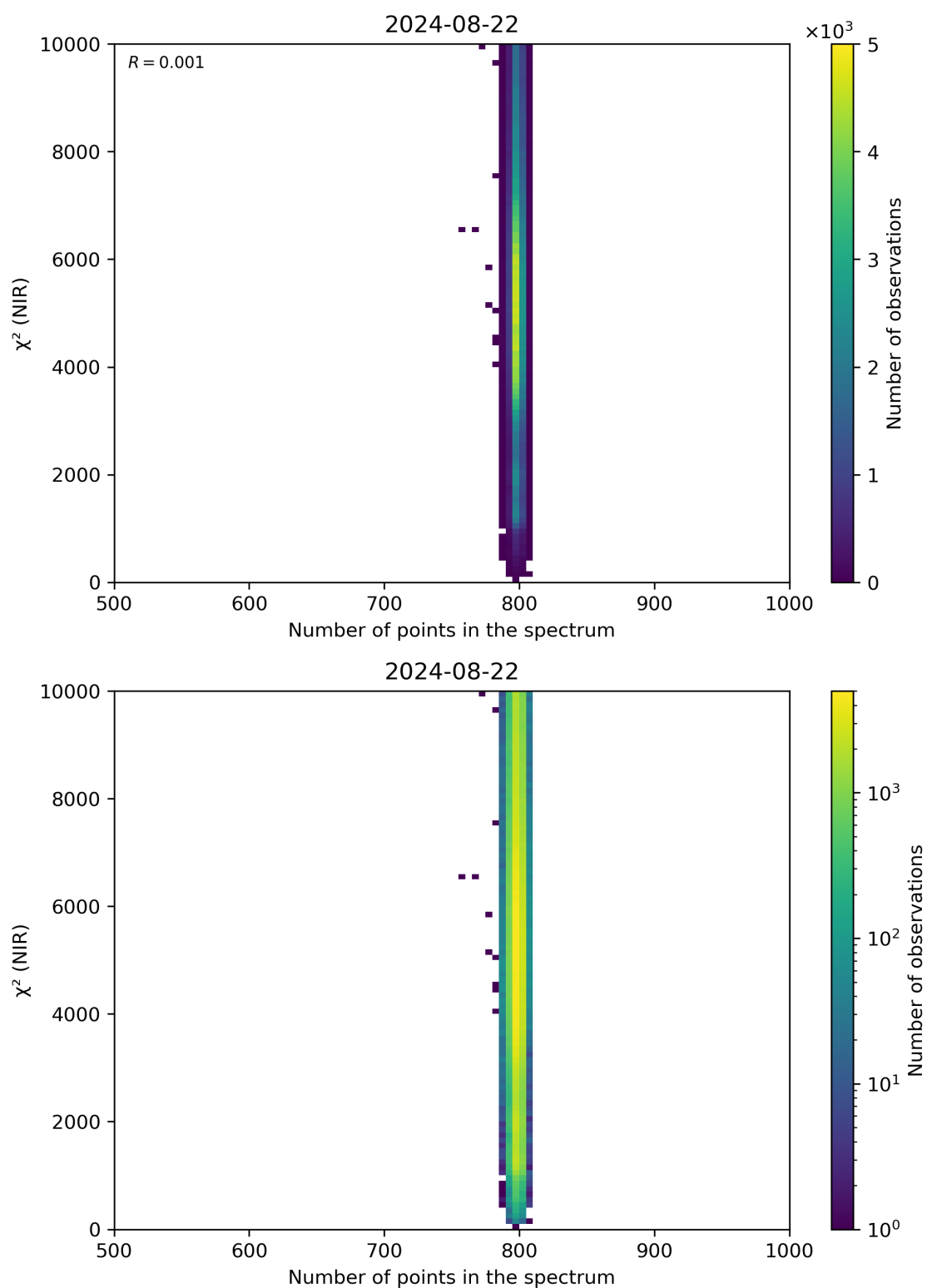
Figure 88: Scatter density plot of “Number of points in the spectrum” against “ \chi^2 (NIR)” for 2024-08-22 to 2024-08-23.
