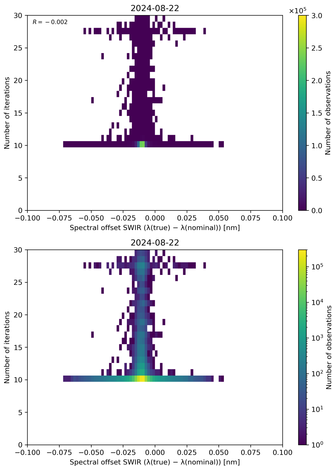
Figure 121: Scatter density plot of “Spectral offset SWIR ( \lambda(\text{true}) - \lambda(\text{nominal}) )” against “Number of iterations” for 2024-08-22 to 2024-08-23.
