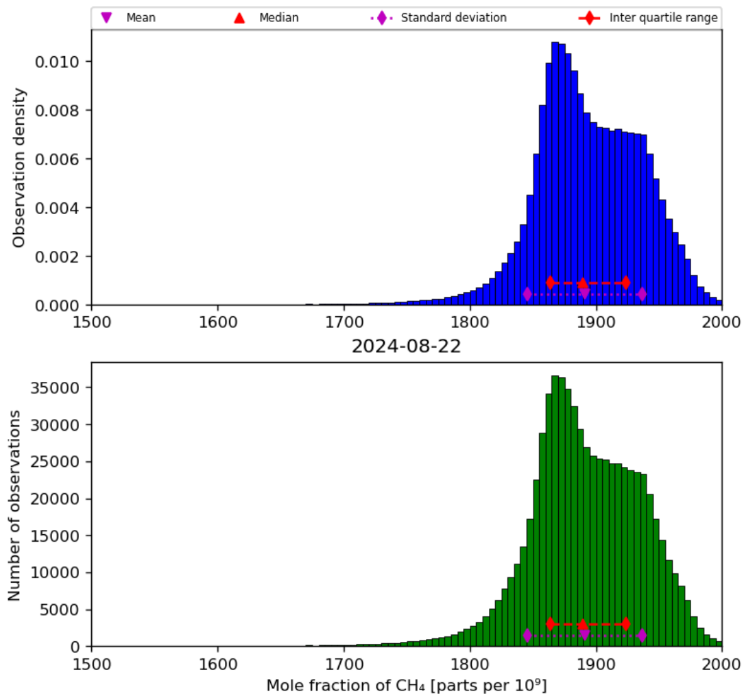
Figure 23: Histogram of “Mole fraction of CH 4 ” for 2024-08-22 to 2024-08-23
