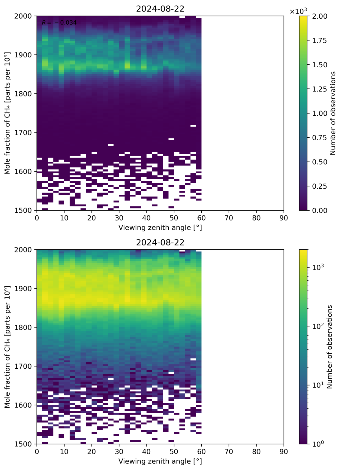
Figure 110: Scatter density plot of “Viewing zenith angle” against “Mole fraction of CH 4 ” for 2024-08-22 to 2024-08-23.
