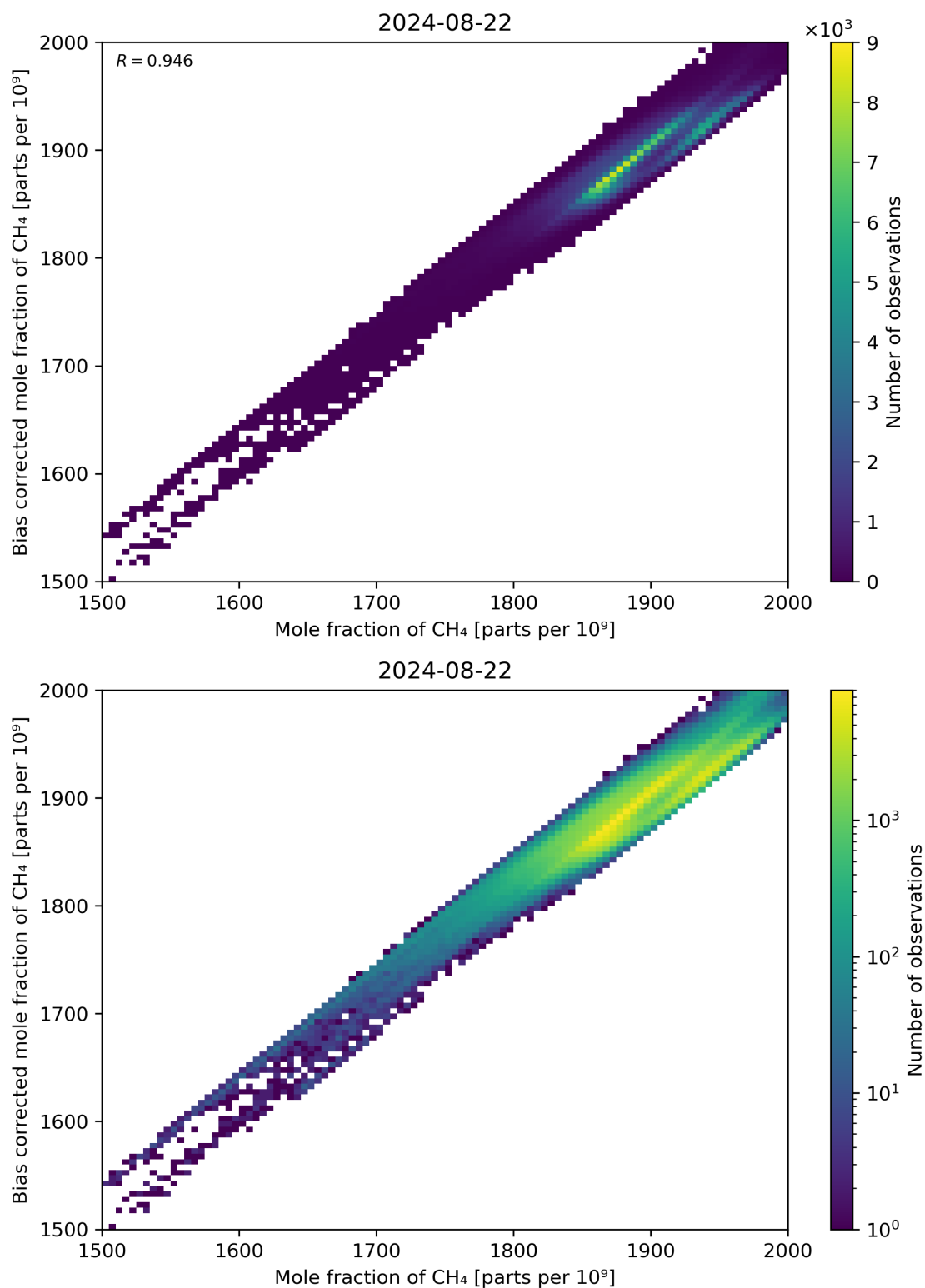
Figure 74: Scatter density plot of “Mole fraction of CH 4 ” against “Bias corrected mole fraction of CH 4 ” for 2024-08-22 to 2024-08-23.
