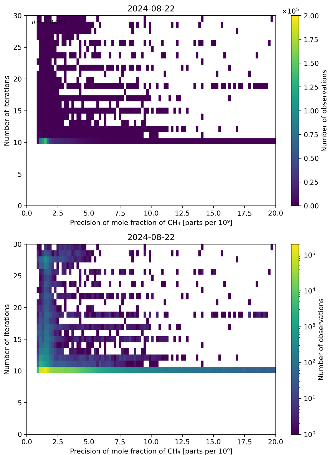
Figure 83: Scatter density plot of “Precision of mole fraction of CH 4 ” against “Number of iterations” for 2024-08-22 to 2024-08-23.
