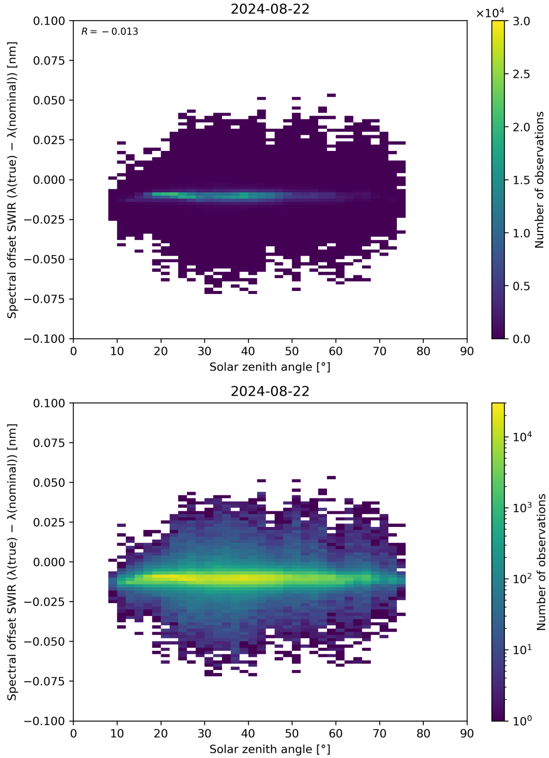
Figure 104: Scatter density plot of “Solar zenith angle” against “Spectral offset SWIR ( \lambda(\text{true}) - \lambda(\text{nominal}) )” for 2024-08-22 to 2024-08-23.
