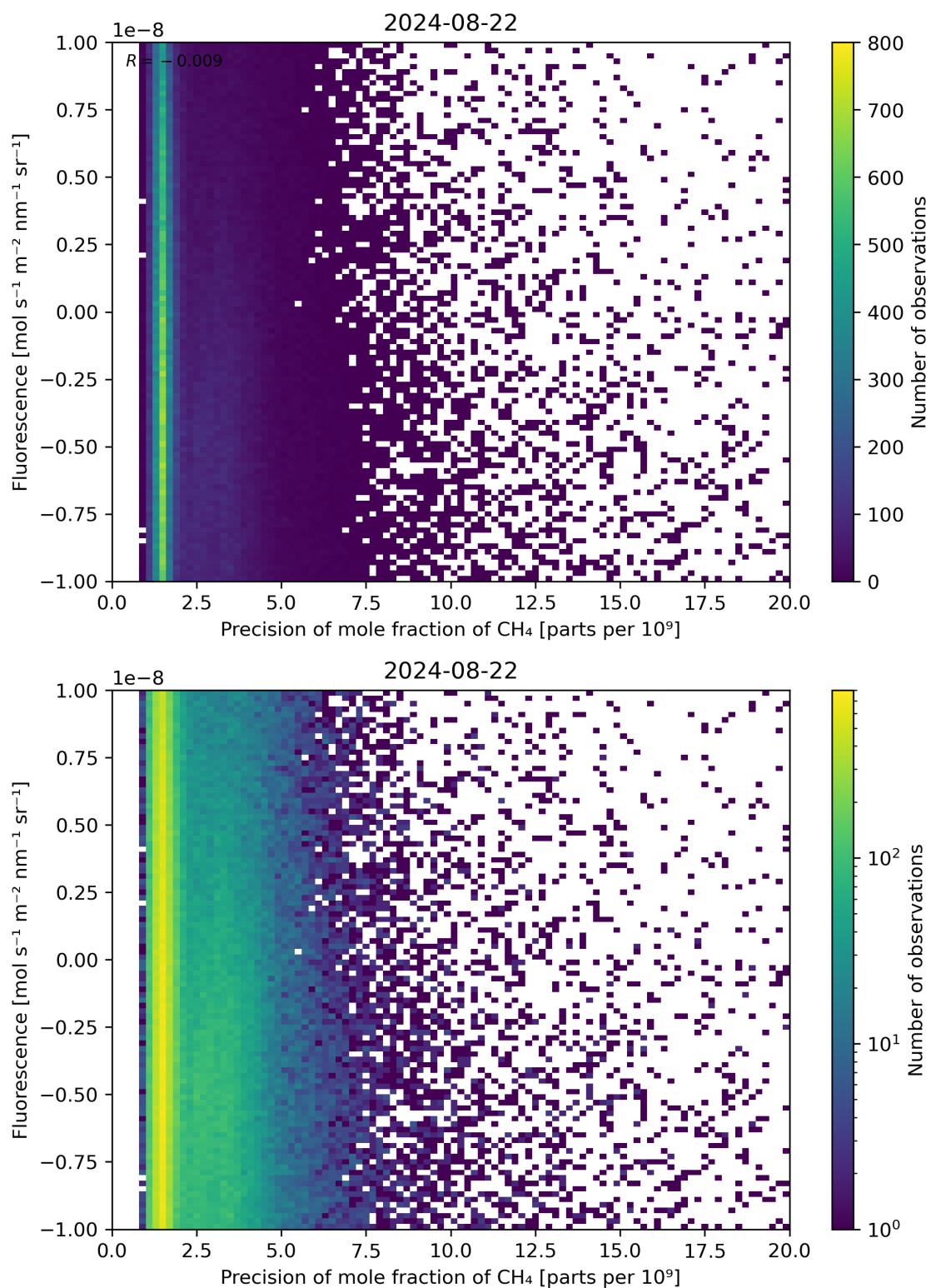
Figure 81: Scatter density plot of “Precision of mole fraction of \text{CH}_4 ” against “Fluorescence” for 2024-08-22 to 2024-08-23.
