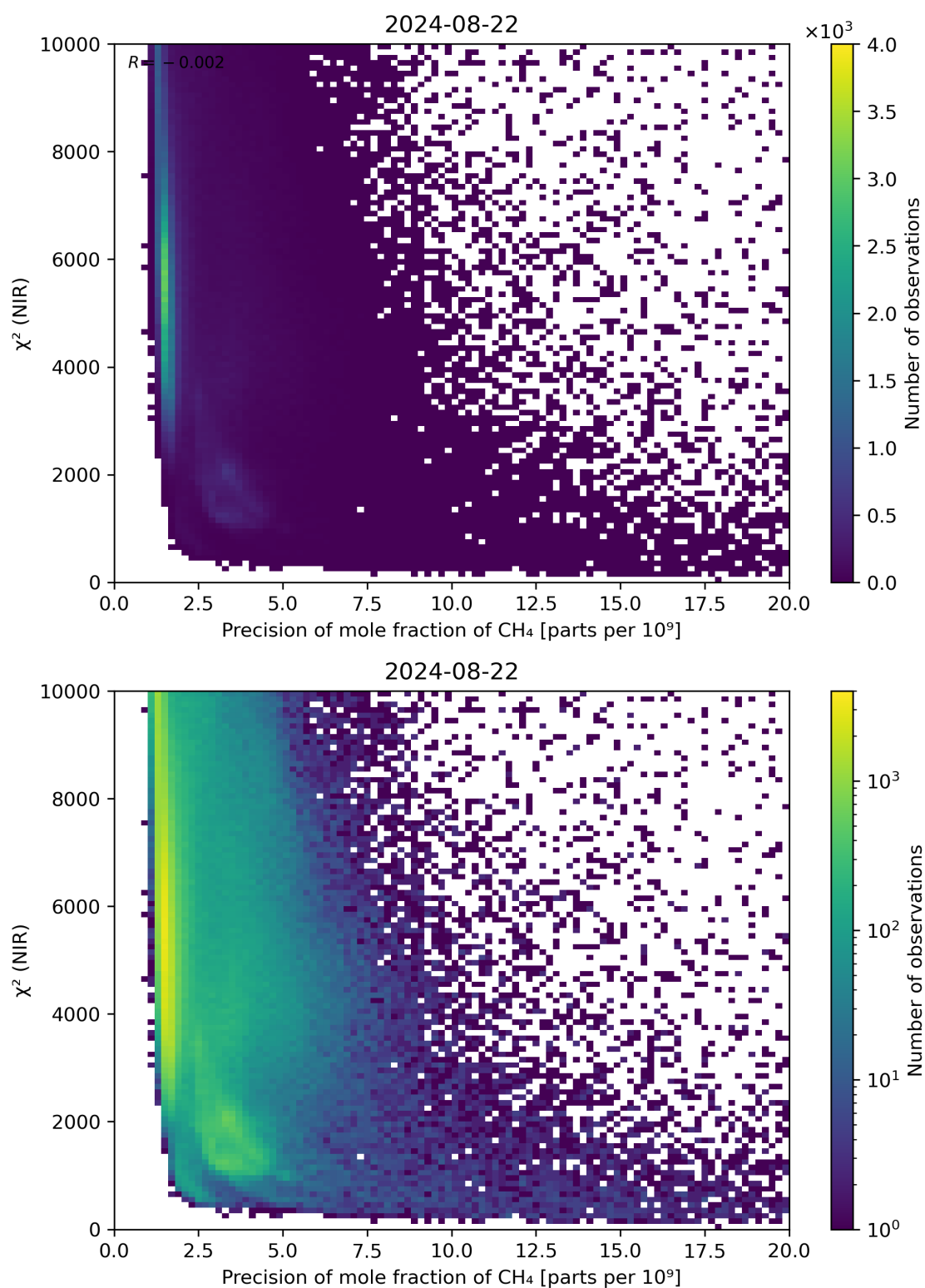
Figure 78: Scatter density plot of “Precision of mole fraction of CH 4 ” against “ \chi^2 (NIR)” for 2024-08-22 to 2024-08-23.
