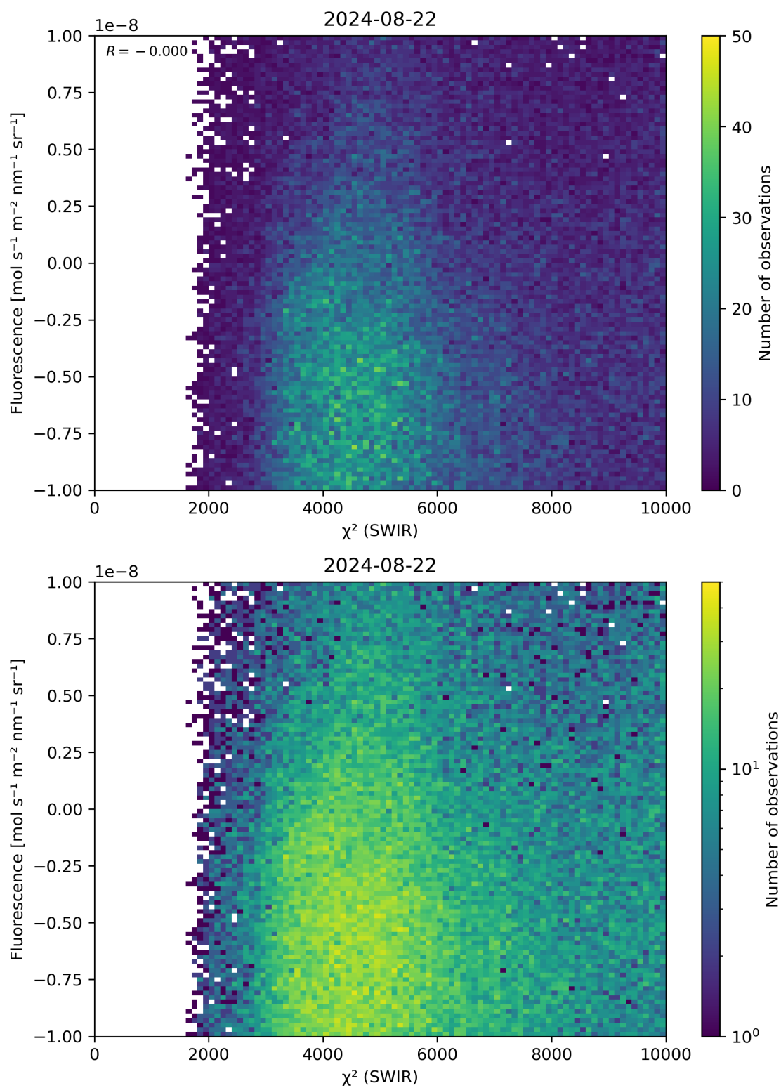
Figure 49: Scatter density plot of “ \chi^2 (SWIR)” against “Fluorescence” for 2024-08-22 to 2024-08-23.
