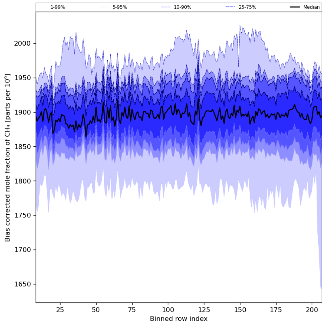
Figure 36: Along track statistics of “Bias corrected mole fraction of CH 4 ” for 2024-08-22 to 2024-08-23
