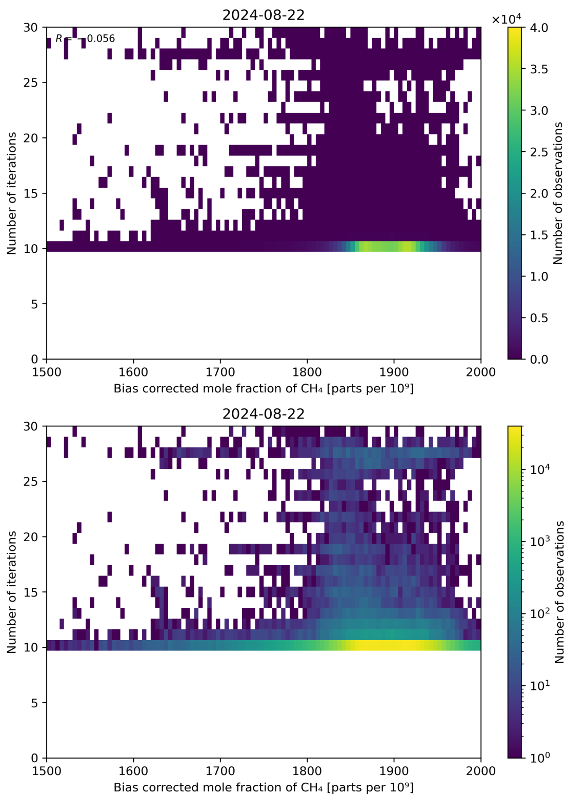
Figure 67: Scatter density plot of “Bias corrected mole fraction of \text{CH}_4 ” against “Number of iterations” for 2024-08-22 to 2024-08-23.
