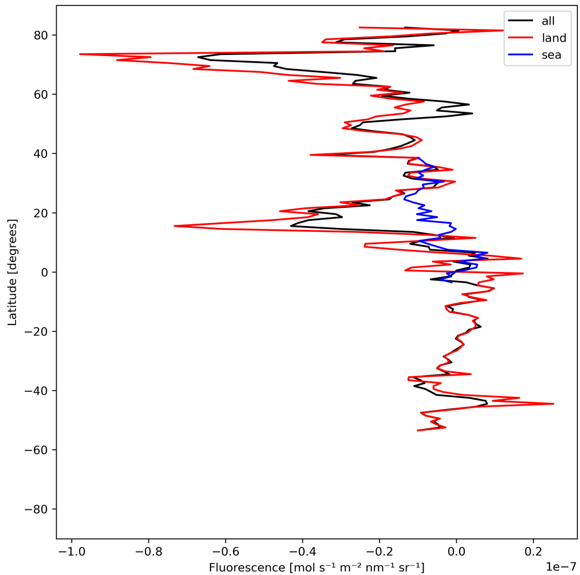
Figure 21: Zonal average of “Fluorescence” for 2024-08-22 to 2024-08-23.
