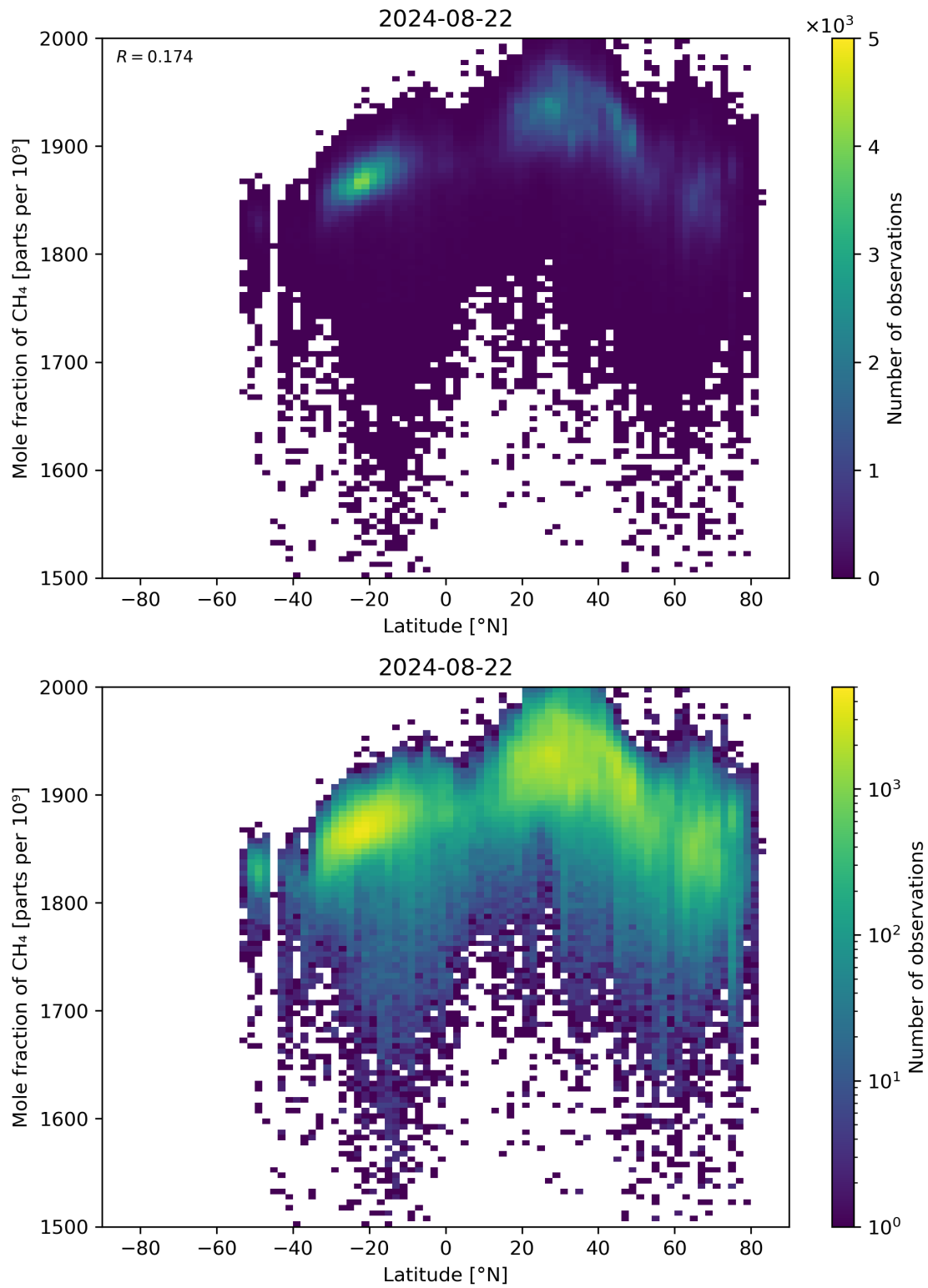
Figure 57: Scatter density plot of “Latitude” against “Mole fraction of \text{CH}_4 ” for 2024-08-22 to 2024-08-23.
