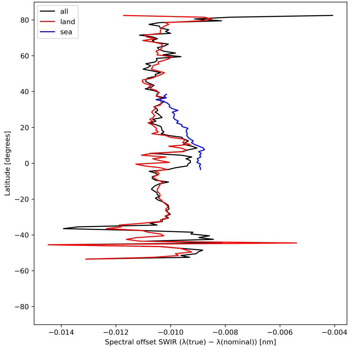
Figure 16: Zonal average of “Spectral offset SWIR ( \lambda(\text{true}) - \lambda(\text{nominal}) )” for 2024-08-22 to 2024-08-23.
