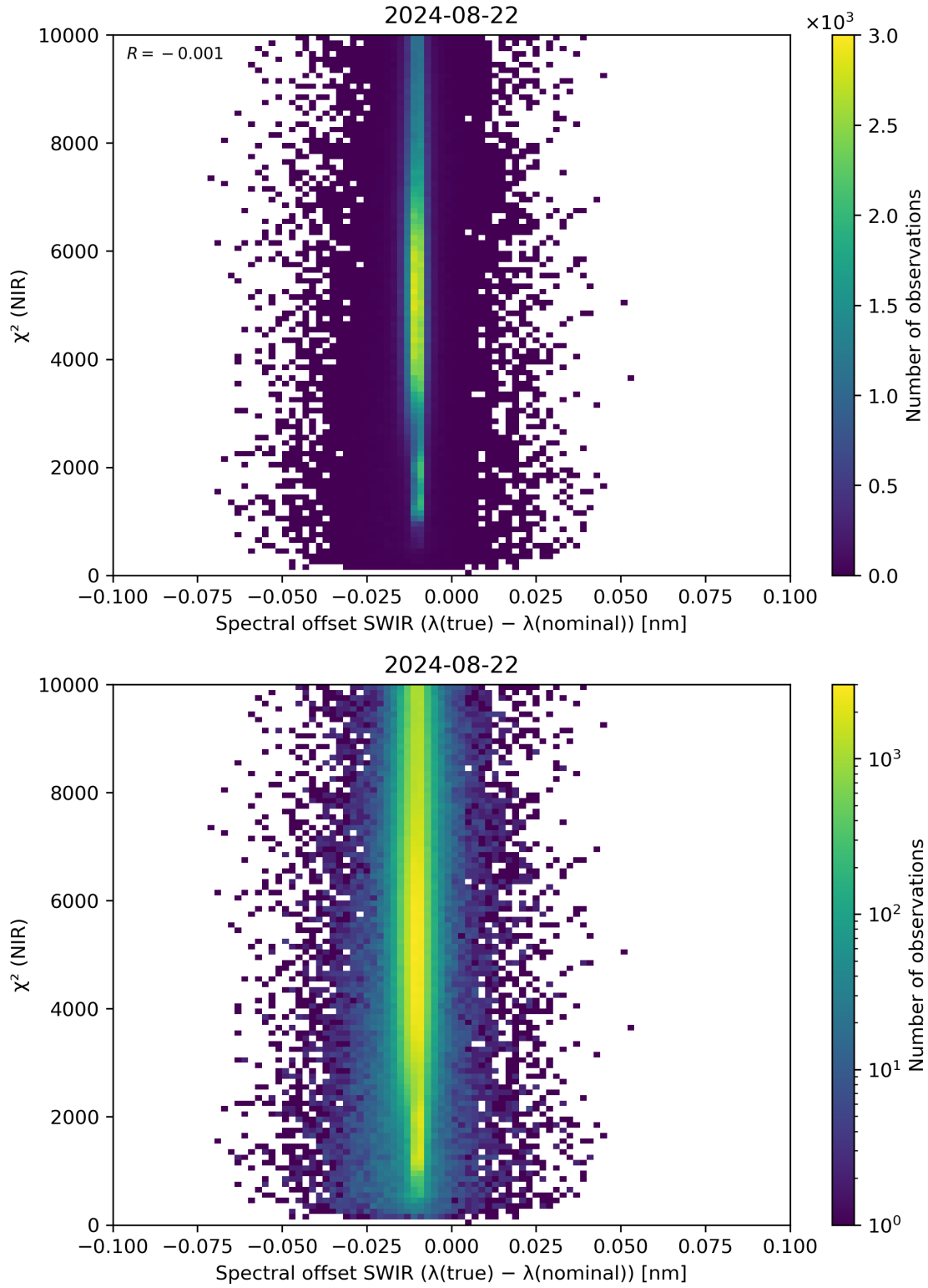
Figure 117: Scatter density plot of “Spectral offset SWIR ( \lambda(\text{true}) - \lambda(\text{nominal}) )” against “ \chi^2 (NIR)” for 2024-08-22 to 2024-08-23.
