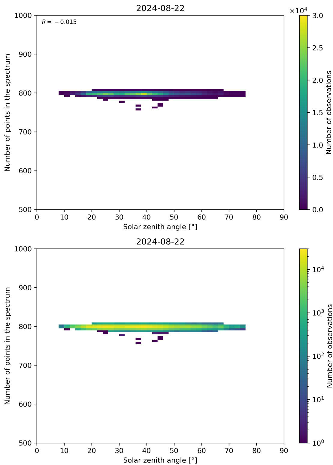
Figure 103: Scatter density plot of “Solar zenith angle” against “Number of points in the spectrum” for 2024-08-22 to 2024-08-23.
