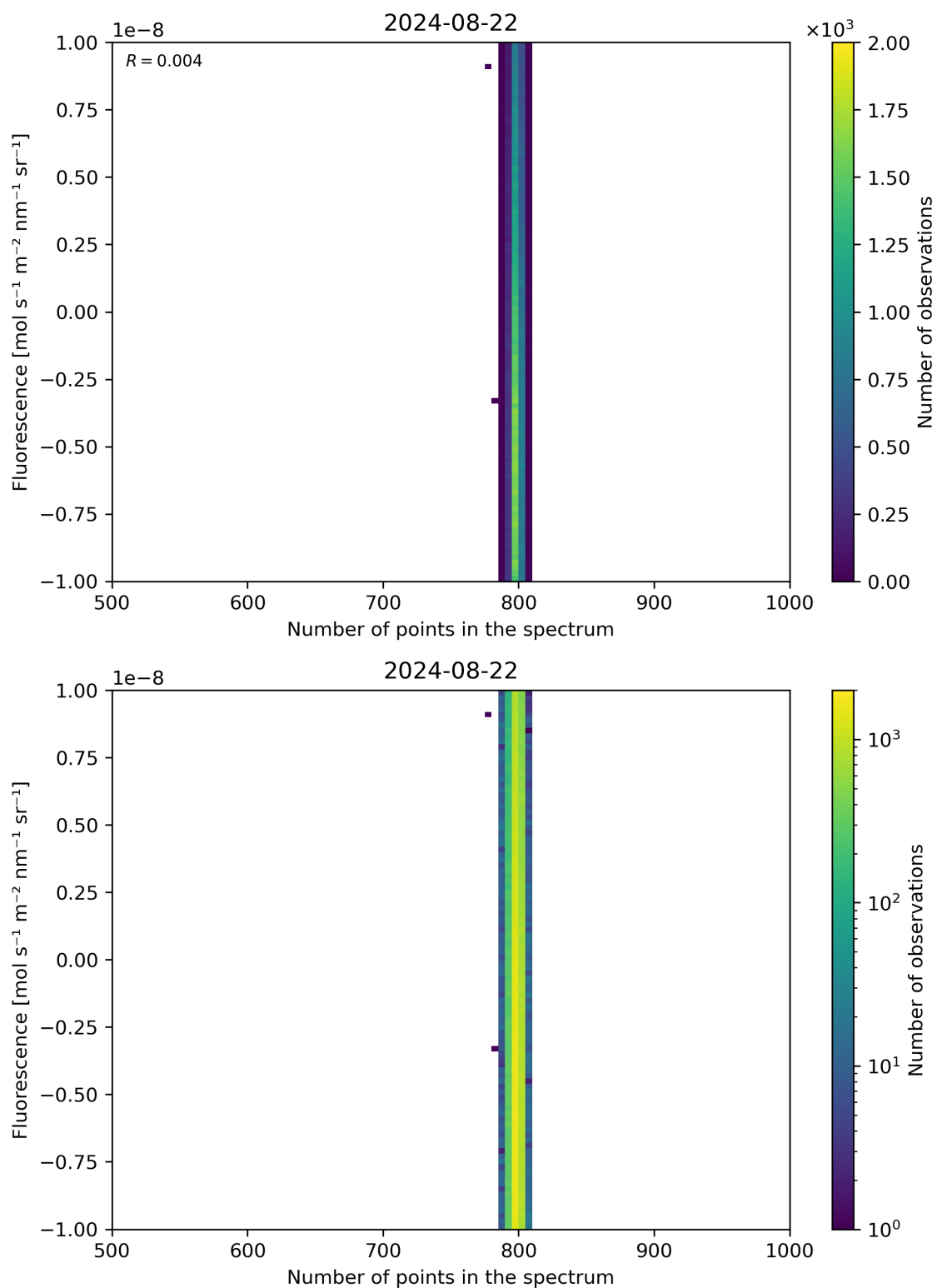
Figure 91: Scatter density plot of “Number of points in the spectrum” against “Fluorescence” for 2024-08-22 to 2024-08-23.
