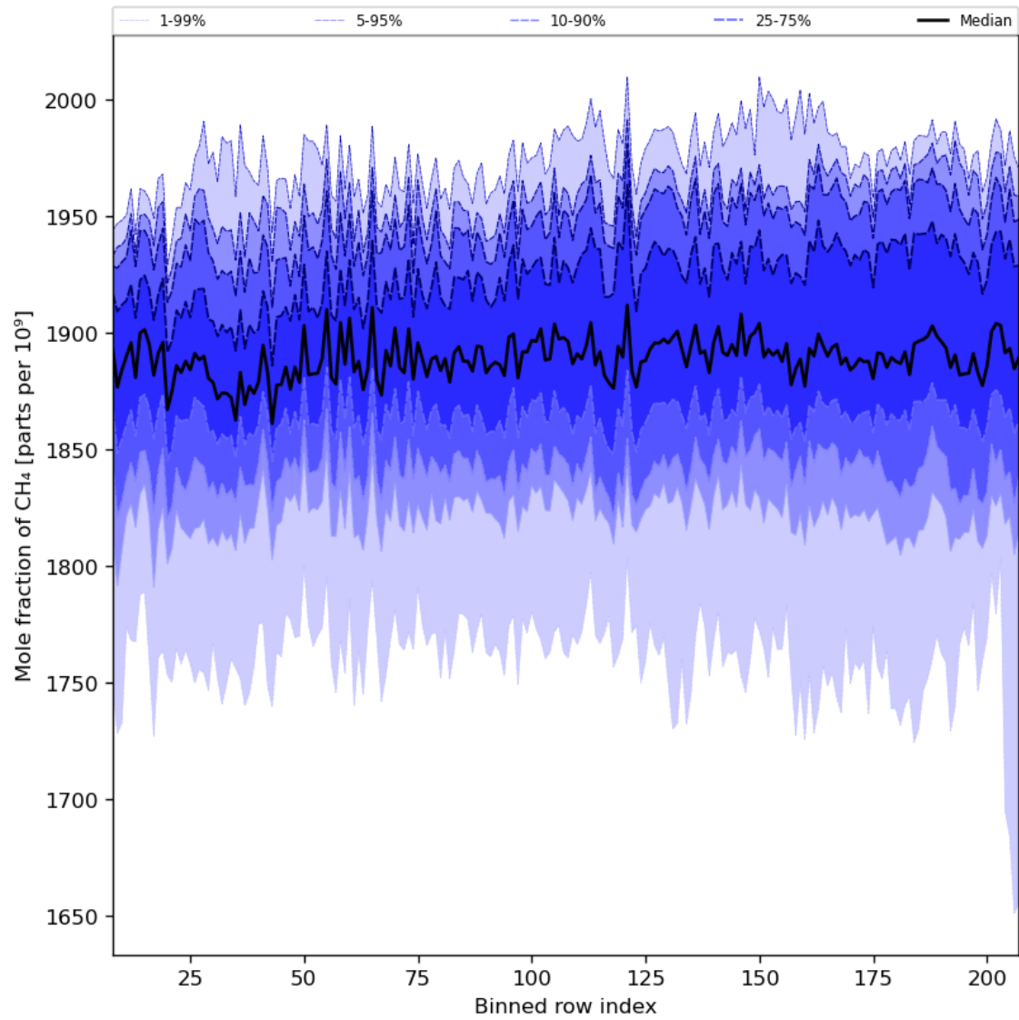
Figure 34: Along track statistics of “Mole fraction of CH 4 ” for 2024-08-22 to 2024-08-23
