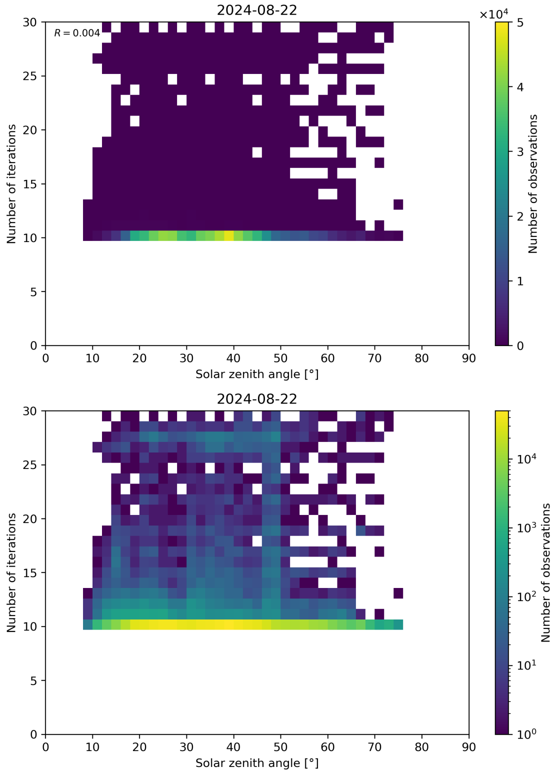
Figure 102: Scatter density plot of “Solar zenith angle” against “Number of iterations” for 2024-08-22 to 2024-08-23.
