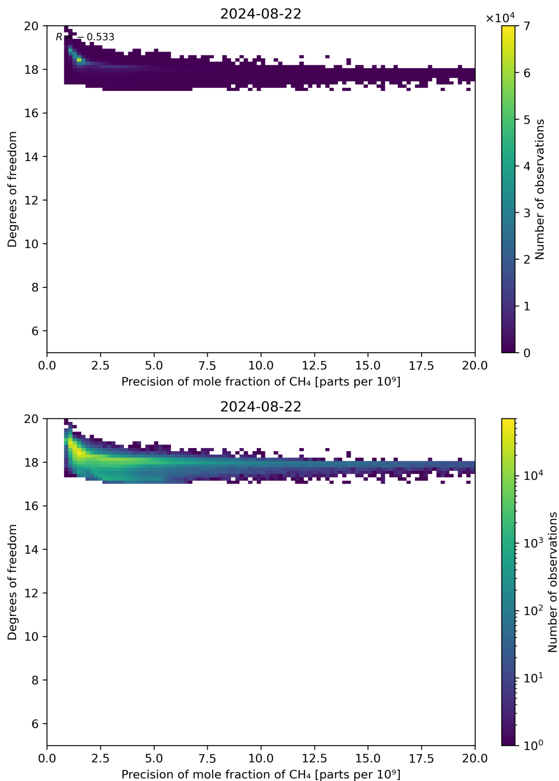
Figure 80: Scatter density plot of “Precision of mole fraction of CH 4 ” against “Degrees of freedom” for 2024-08-22 to 2024-08-23.
