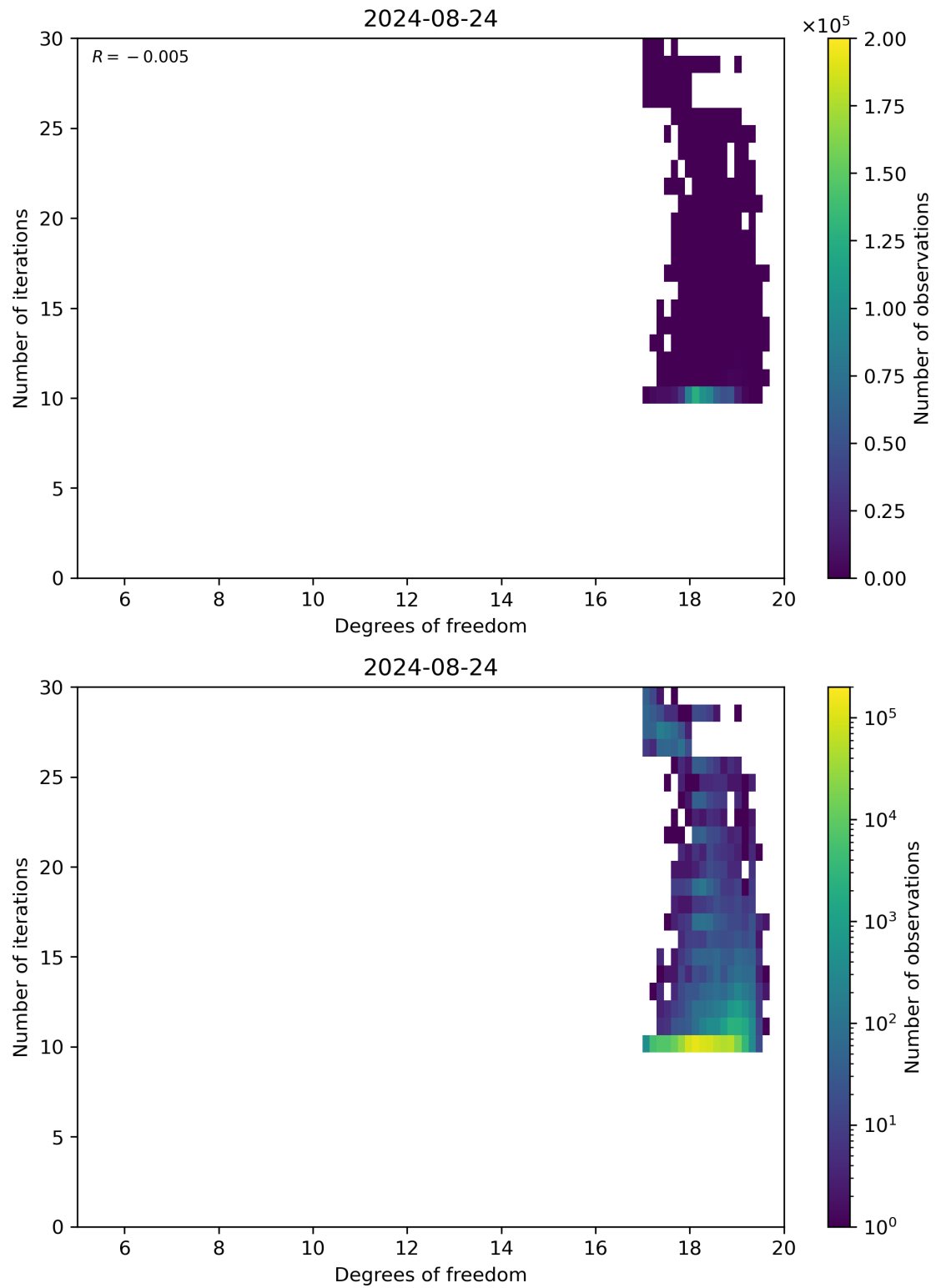
Figure 52: Scatter density plot of “Degrees of freedom” against “Number of iterations” for 2024-08-23 to 2024-08-25.
