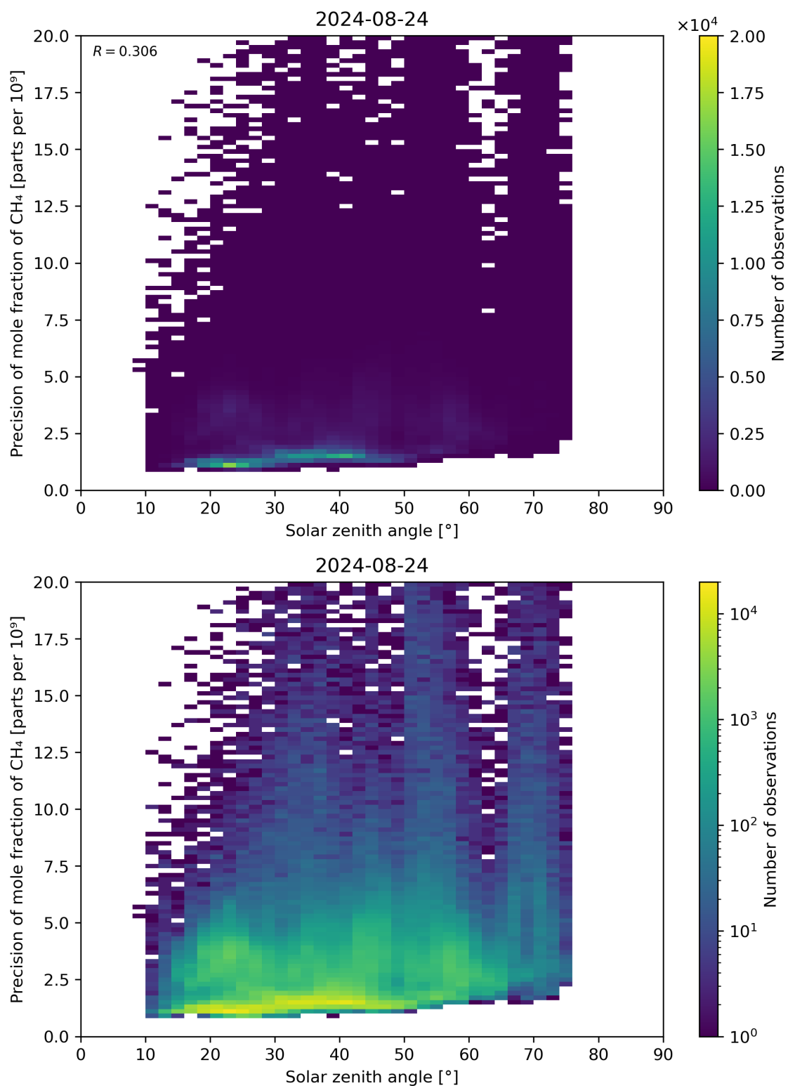
Figure 101: Scatter density plot of “Solar zenith angle” against “Precision of mole fraction of CH 4 ” for 2024-08-23 to 2024-08-25.
