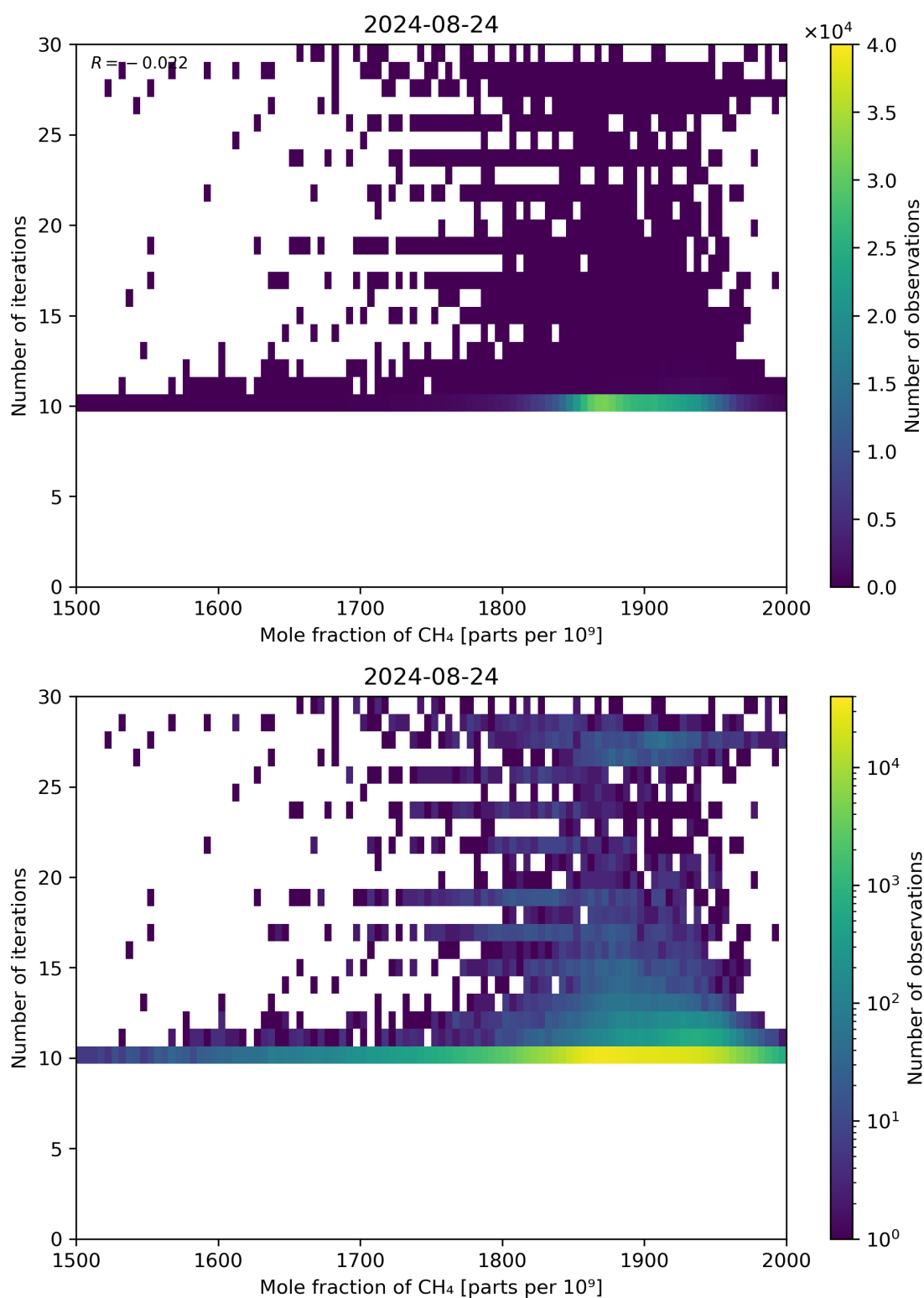
Figure 76: Scatter density plot of “Mole fraction of CH 4 ” against “Number of iterations” for 2024-08-23 to 2024-08-25.
