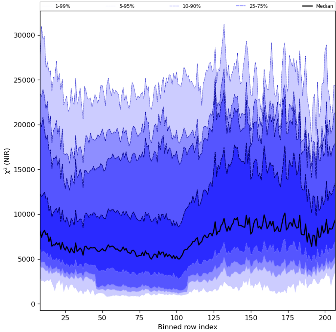
Figure 40: Along track statistics of “ \chi^2 (NIR)” for 2024-08-23 to 2024-08-25
