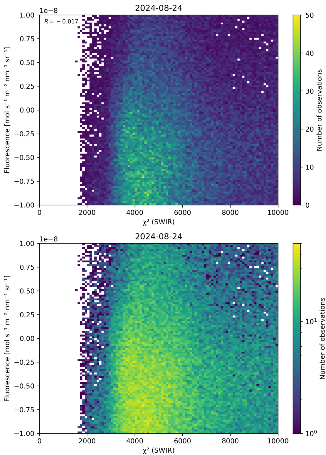
Figure 49: Scatter density plot of “ \chi^2 (SWIR)” against “Fluorescence” for 2024-08-23 to 2024-08-25.
