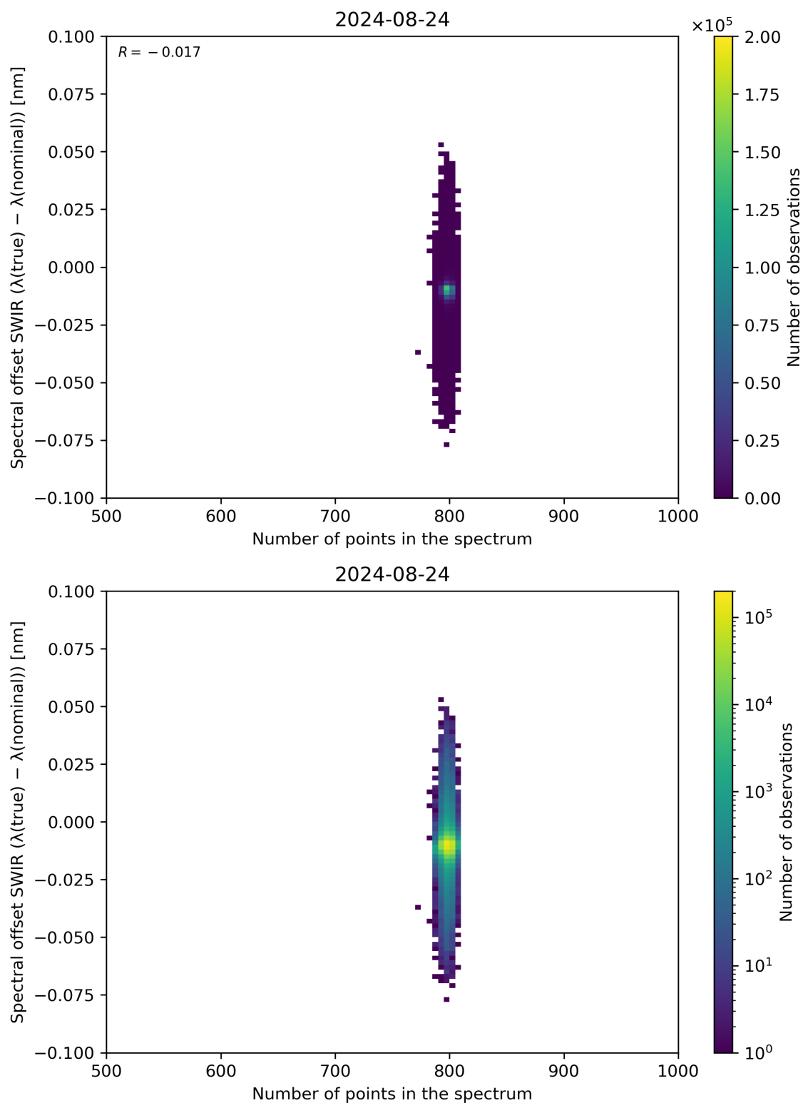
Figure 93: Scatter density plot of “Number of points in the spectrum” against “Spectral offset SWIR ( \lambda(\text{true}) - \lambda(\text{nominal}) )” for 2024-08-23 to 2024-08-25.
