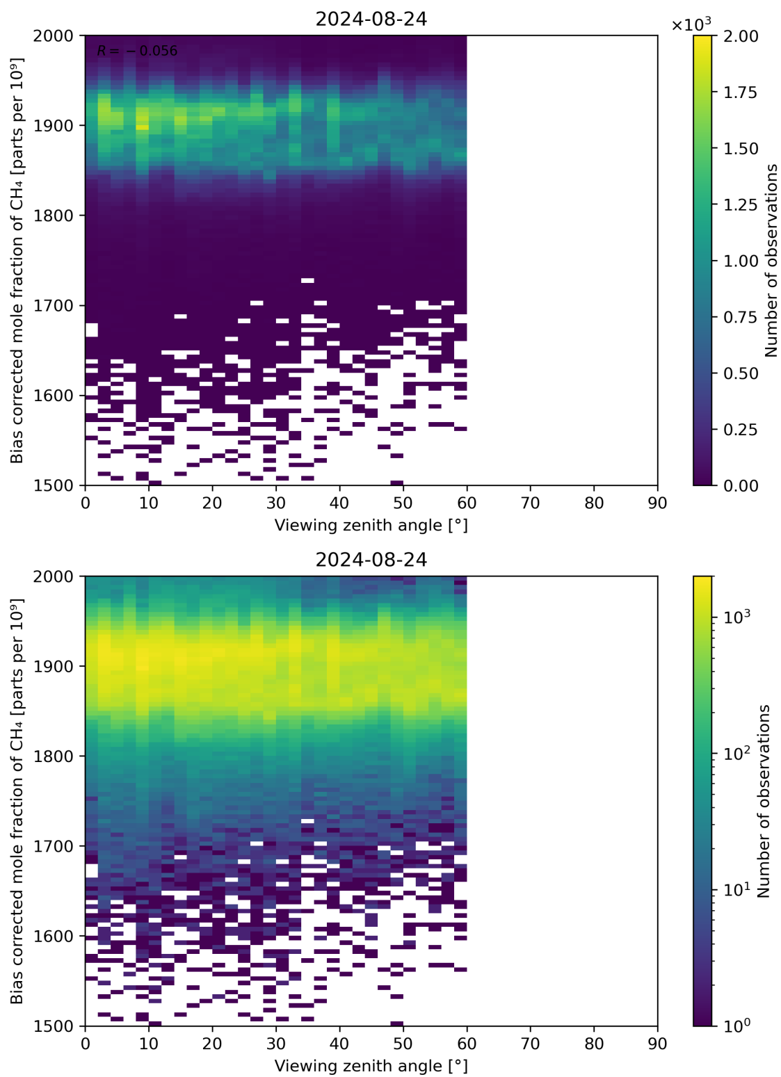
Figure 111: Scatter density plot of “Viewing zenith angle” against “Bias corrected mole fraction of CH 4 ” for 2024-08-23 to 2024-08-25.
