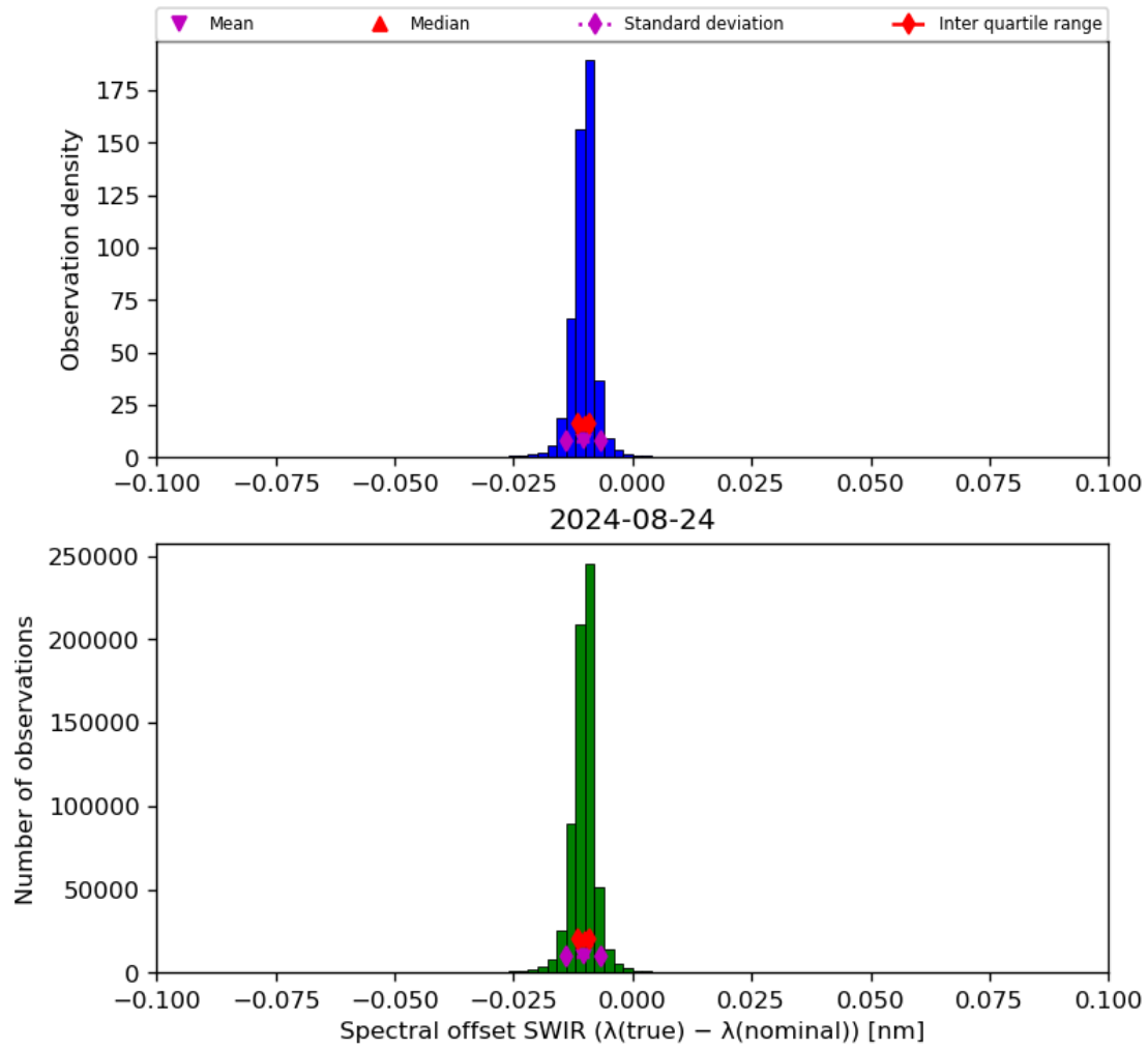
Figure 27: Histogram of “Spectral offset SWIR ( \lambda(\text{true}) - \lambda(\text{nominal}) )” for 2024-08-23 to 2024-08-25
