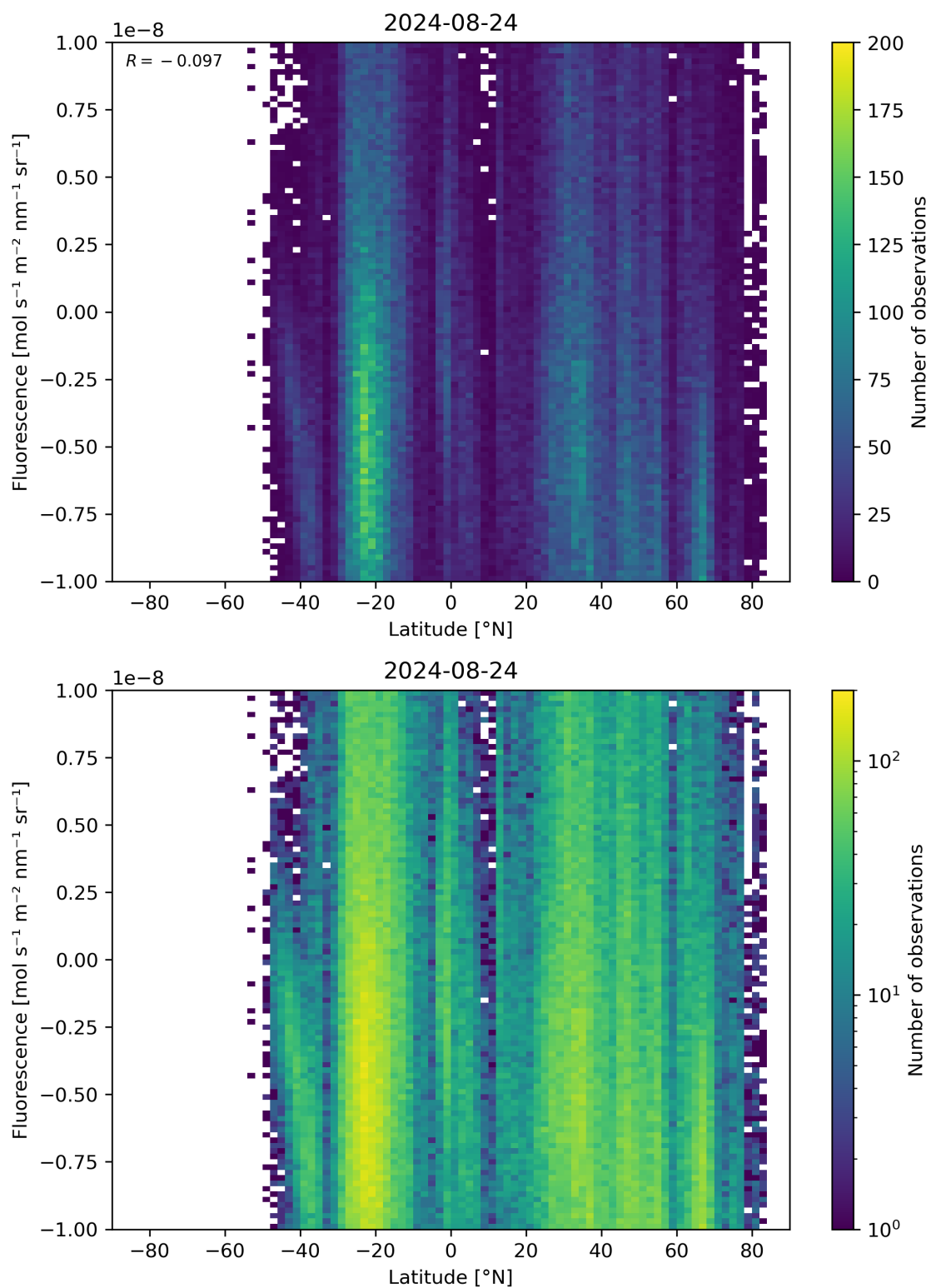
Figure 56: Scatter density plot of “Latitude” against “Fluorescence” for 2024-08-23 to 2024-08-25.
