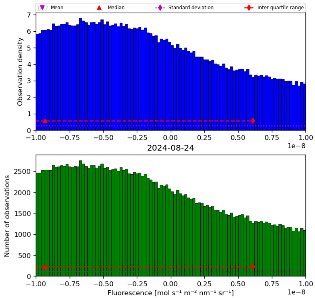
Figure 32: Histogram of “Fluorescence” for 2024-08-23 to 2024-08-25
