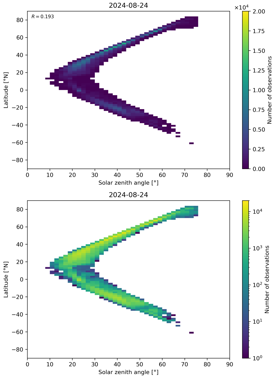
Figure 98: Scatter density plot of “Solar zenith angle” against “Latitude” for 2024-08-23 to 2024-08-25.
