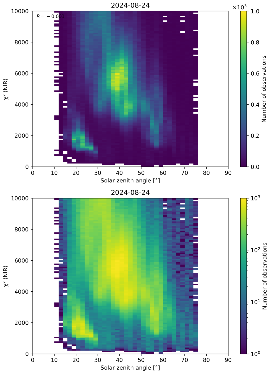
Figure 94: Scatter density plot of “Solar zenith angle” against “ \chi^2 (NIR)” for 2024-08-23 to 2024-08-25.
