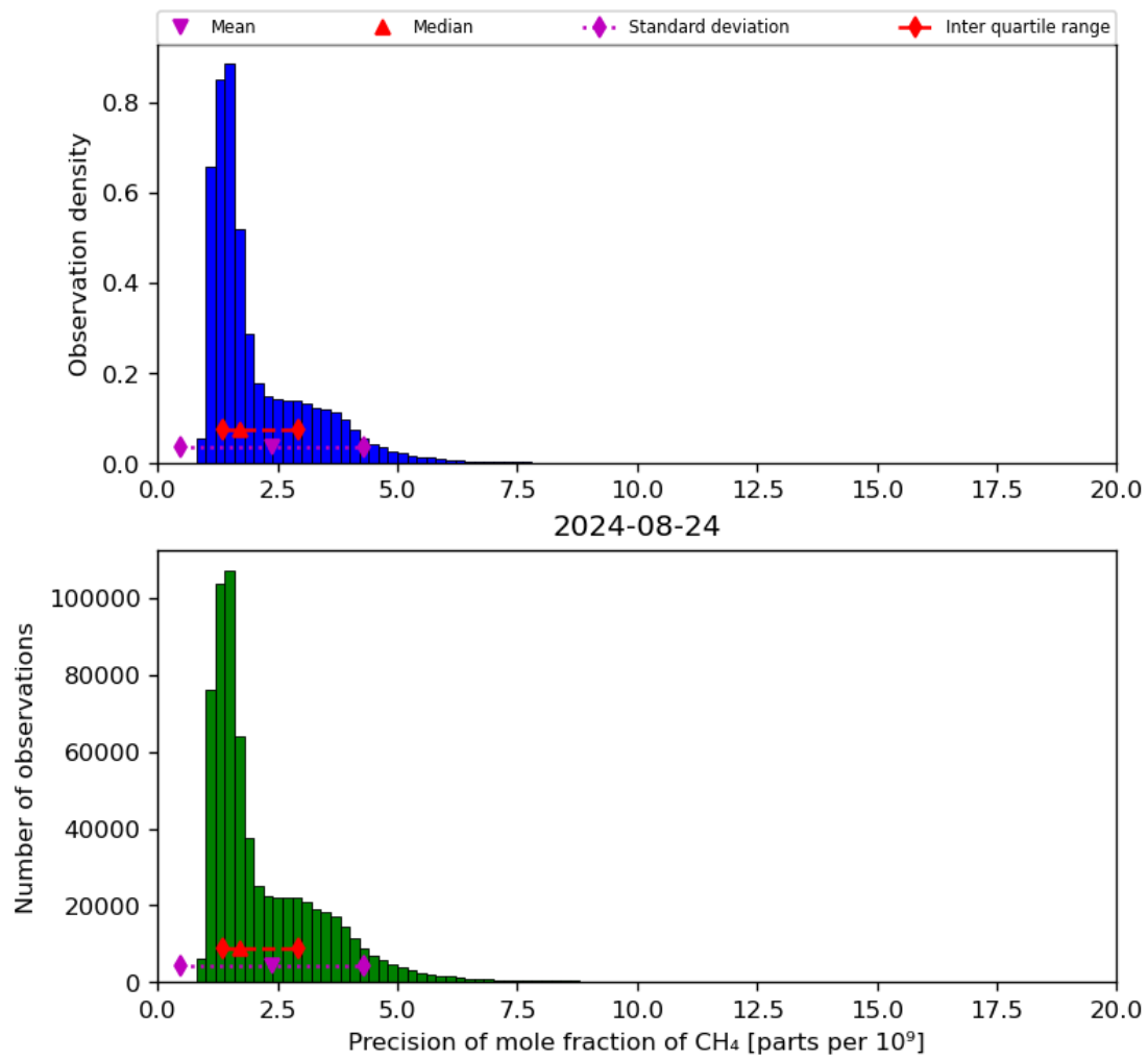
Figure 24: Histogram of “Precision of mole fraction of CH 4 ” for 2024-08-23 to 2024-08-25
