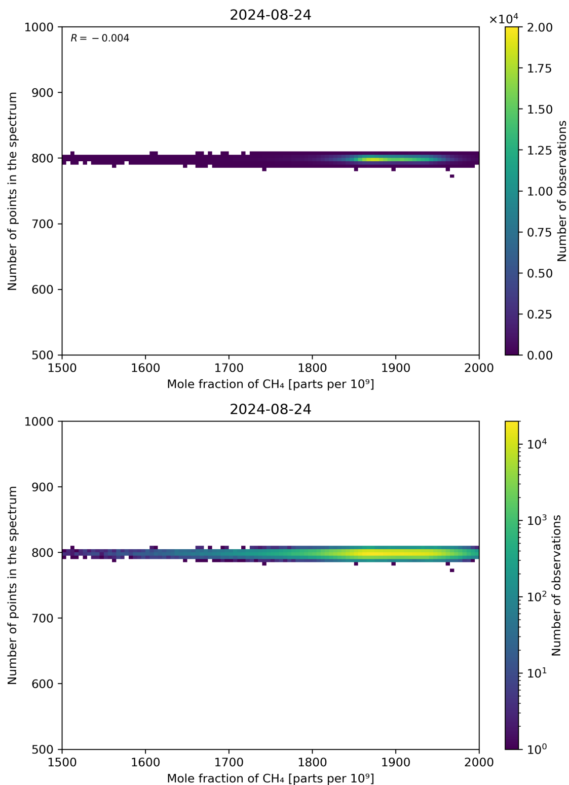
Figure 77: Scatter density plot of “Mole fraction of CH 4 ” against “Number of points in the spectrum” for 2024-08-23 to 2024-08-25.
