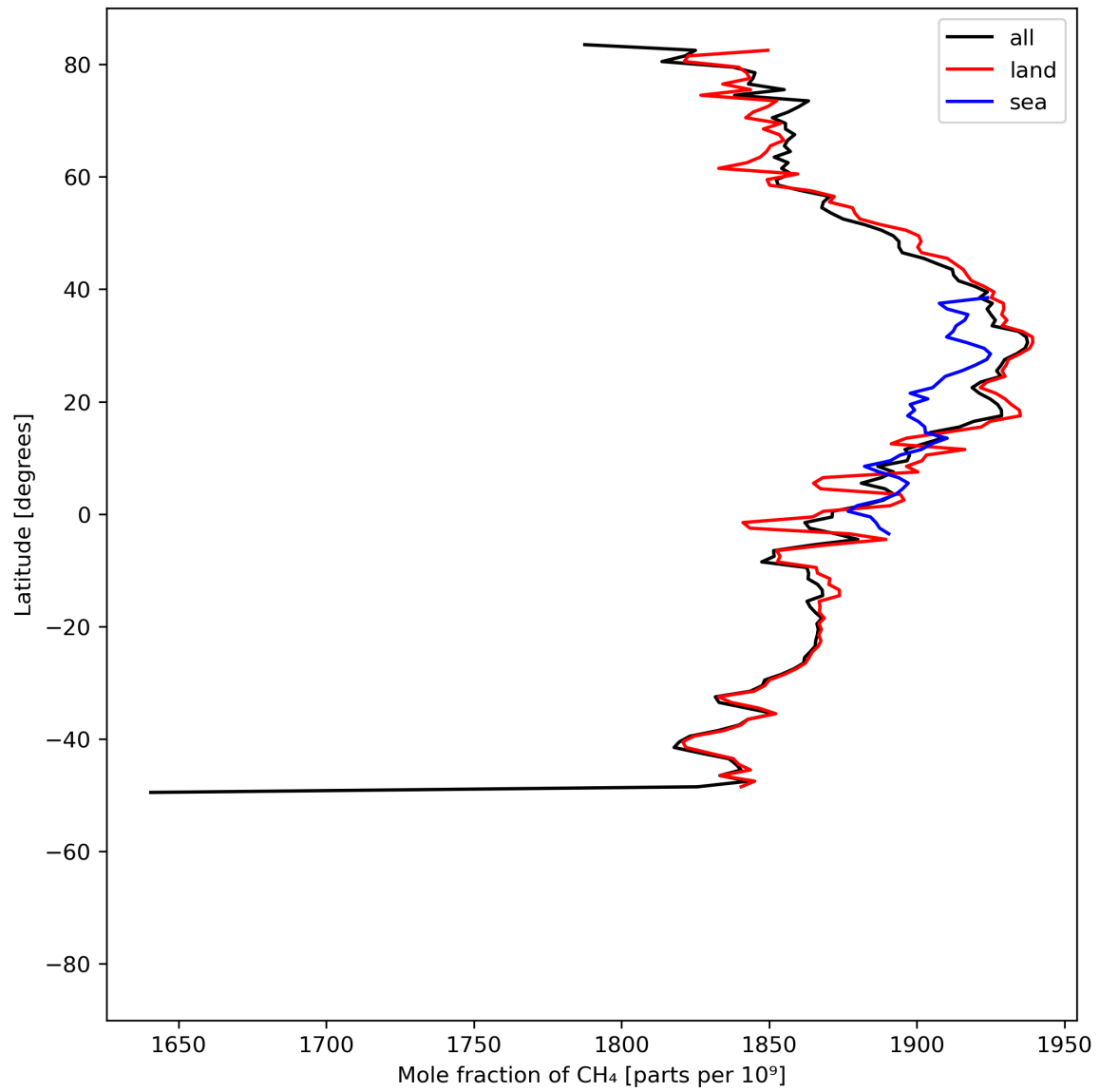
Figure 12: Zonal average of “Mole fraction of \text{CH}_4 ” for 2024-08-23 to 2024-08-25.
