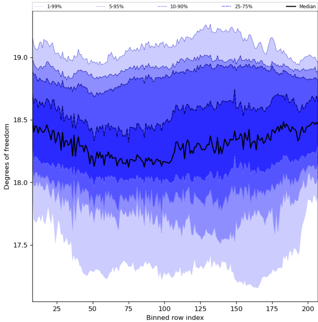
Figure 41: Along track statistics of “Degrees of freedom” for 2024-08-23 to 2024-08-25
