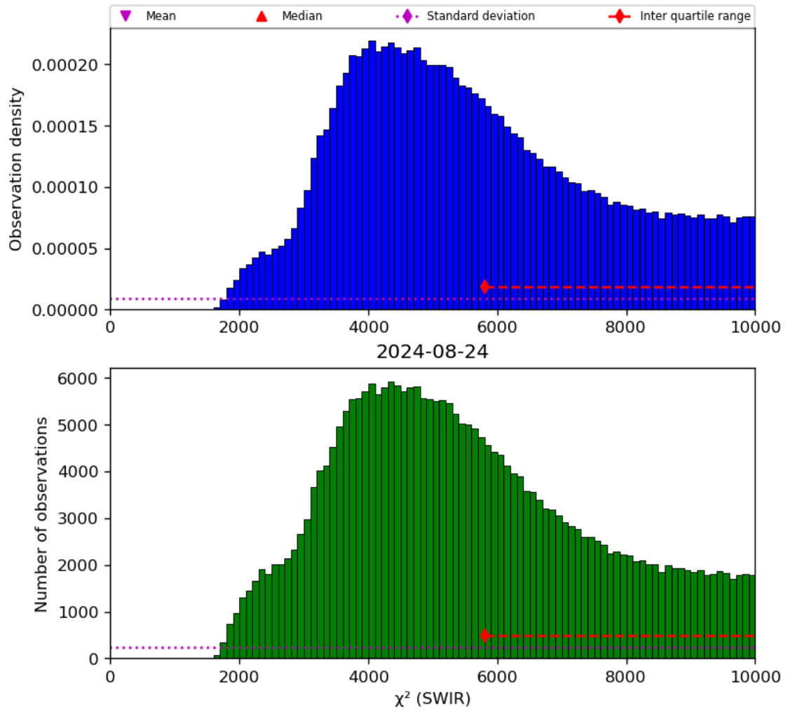
Figure 28: Histogram of " \chi^2 (SWIR)" for 2024-08-23 to 2024-08-25
