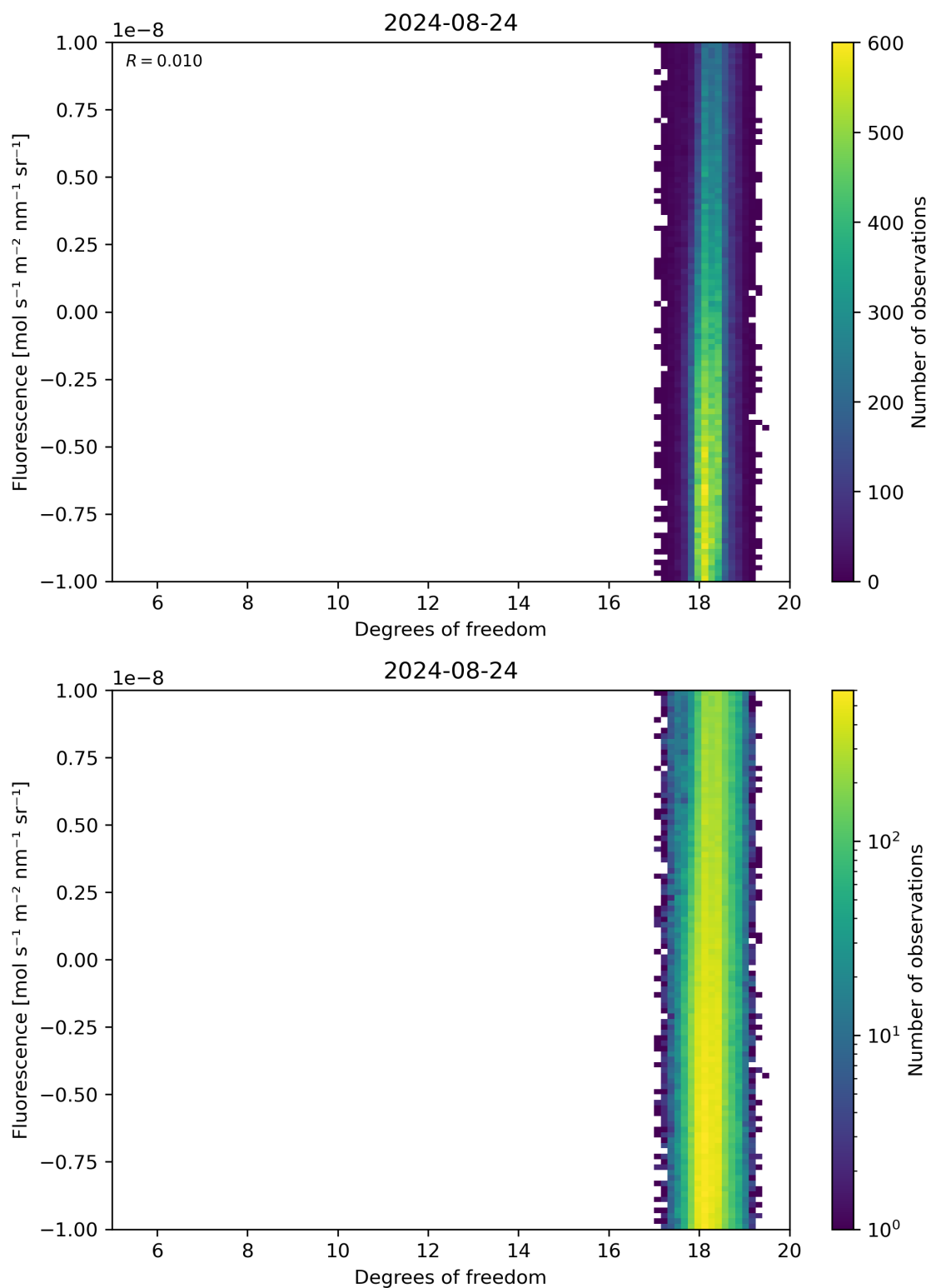
Figure 51: Scatter density plot of “Degrees of freedom” against “Fluorescence” for 2024-08-23 to 2024-08-25.
