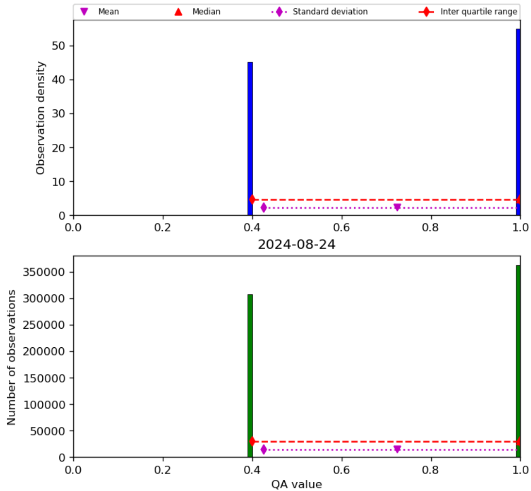
Figure 22: Histogram of "QA value" for 2024-08-23 to 2024-08-25
