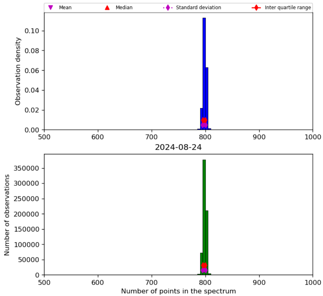
Figure 26: Histogram of “Number of points in the spectrum” for 2024-08-23 to 2024-08-25
