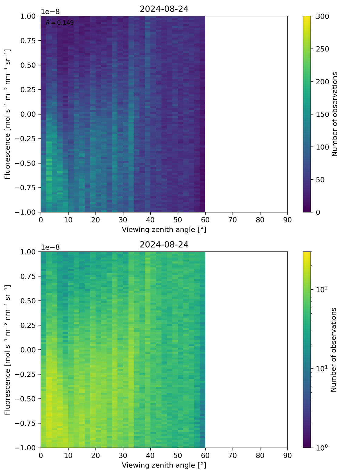
Figure 108: Scatter density plot of “Viewing zenith angle” against “Fluorescence” for 2024-08-23 to 2024-08-25.
