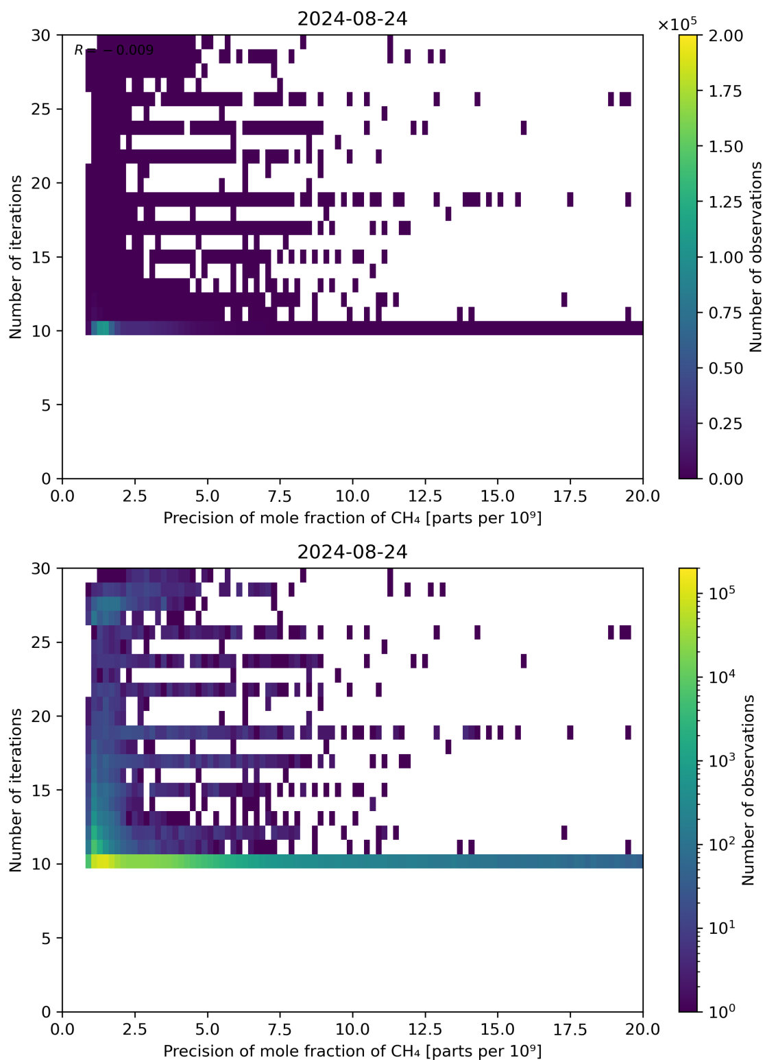
Figure 83: Scatter density plot of “Precision of mole fraction of CH 4 ” against “Number of iterations” for 2024-08-23 to 2024-08-25.
