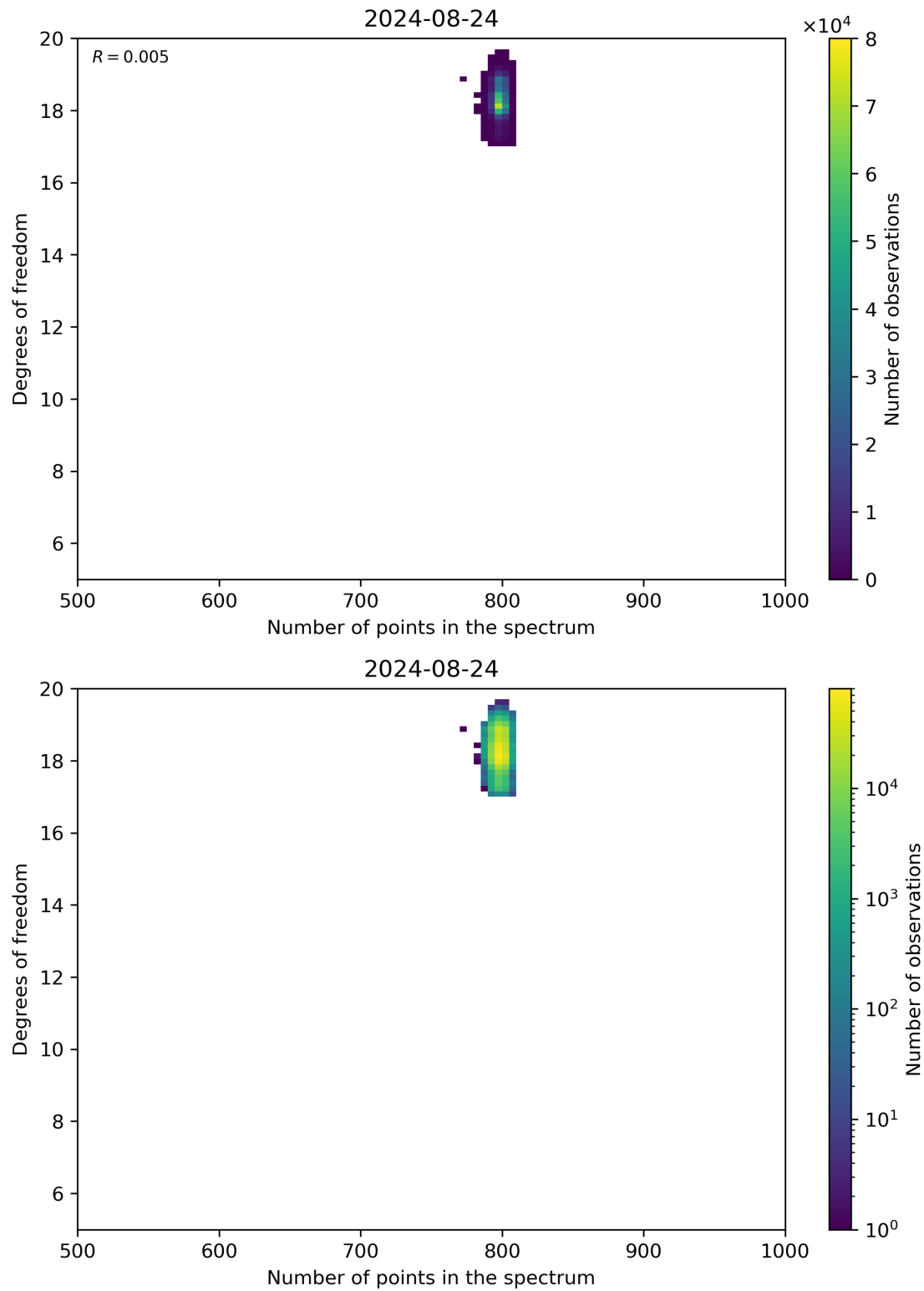
Figure 90: Scatter density plot of “Number of points in the spectrum” against “Degrees of freedom” for 2024-08-23 to 2024-08-25.
