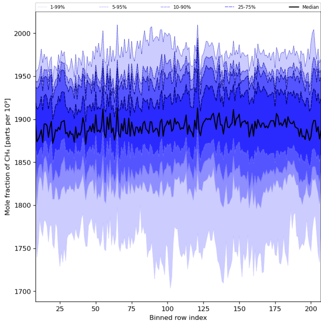
Figure 34: Along track statistics of “Mole fraction of CH 4 ” for 2024-08-23 to 2024-08-25
