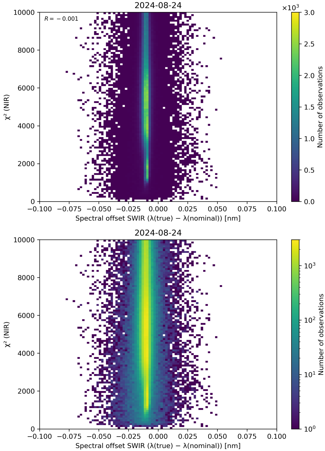
Figure 117: Scatter density plot of “Spectral offset SWIR ( \lambda(\text{true}) - \lambda(\text{nominal}) )” against “ \chi^2 (NIR)” for 2024-08-23 to 2024-08-25.
