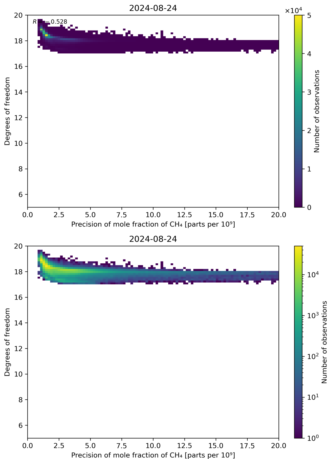
Figure 80: Scatter density plot of “Precision of mole fraction of CH 4 ” against “Degrees of freedom” for 2024-08-23 to 2024-08-25.
