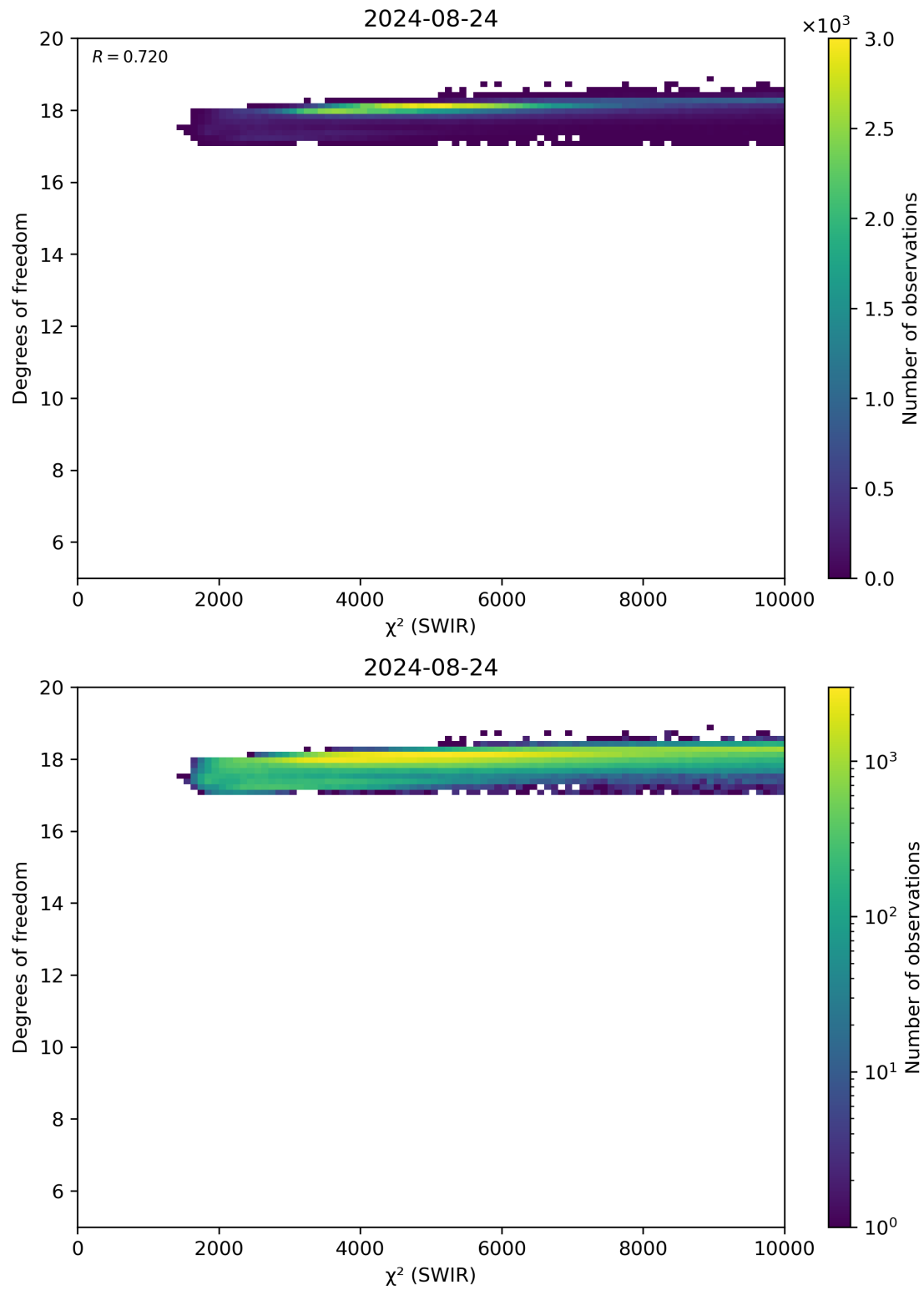
Figure 48: Scatter density plot of “ \chi^2 (SWIR)” against “Degrees of freedom” for 2024-08-23 to 2024-08-25.
