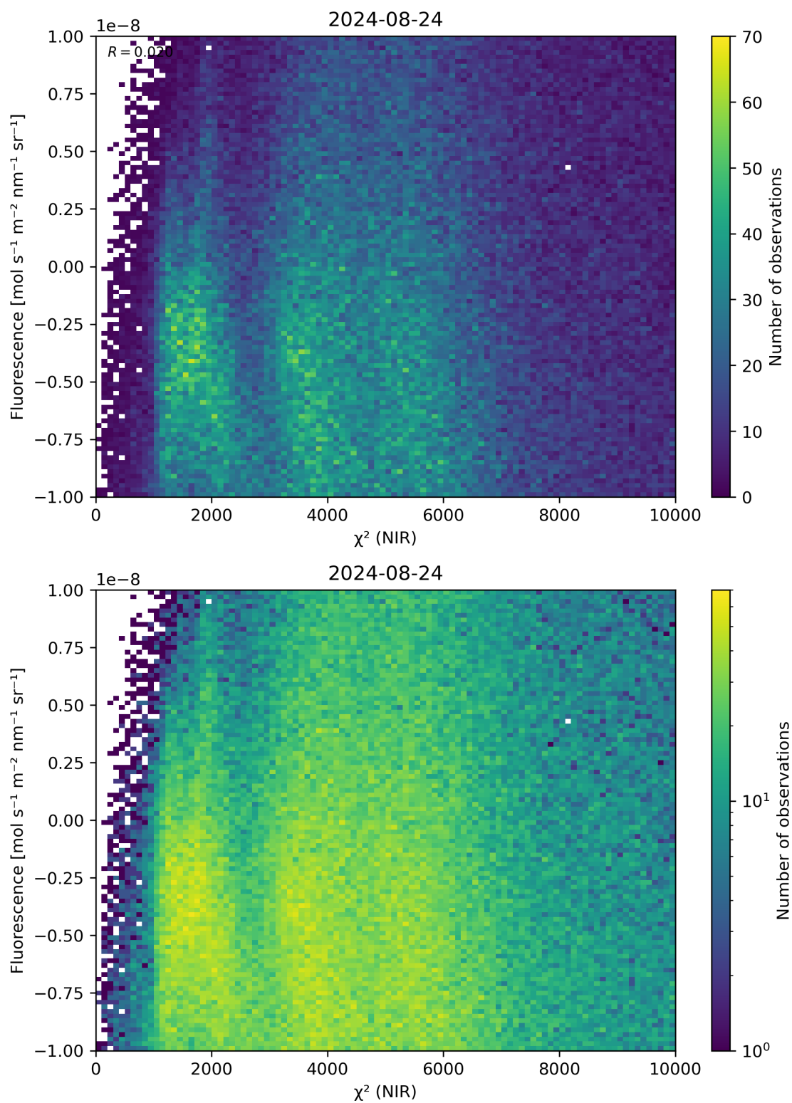
Figure 45: Scatter density plot of “ \chi^2 (NIR)” against “Fluorescence” for 2024-08-23 to 2024-08-25.
