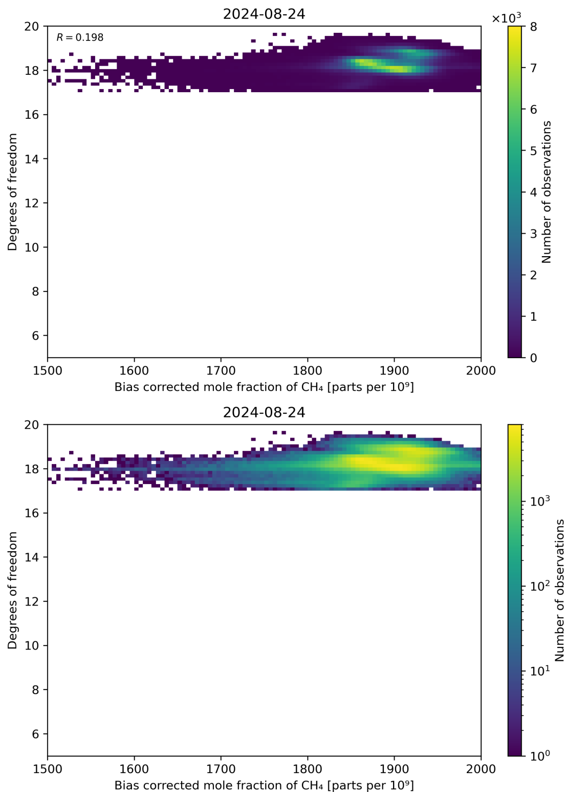
Figure 65: Scatter density plot of “Bias corrected mole fraction of CH 4 ” against “Degrees of freedom” for 2024-08-23 to 2024-08-25.
