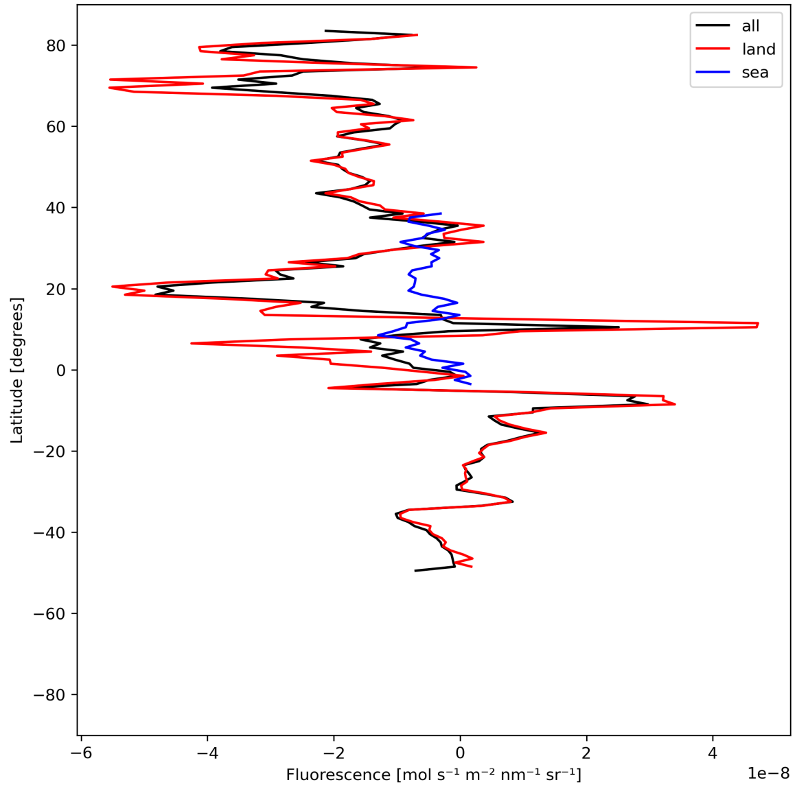
Figure 21: Zonal average of “Fluorescence” for 2024-08-23 to 2024-08-25.
