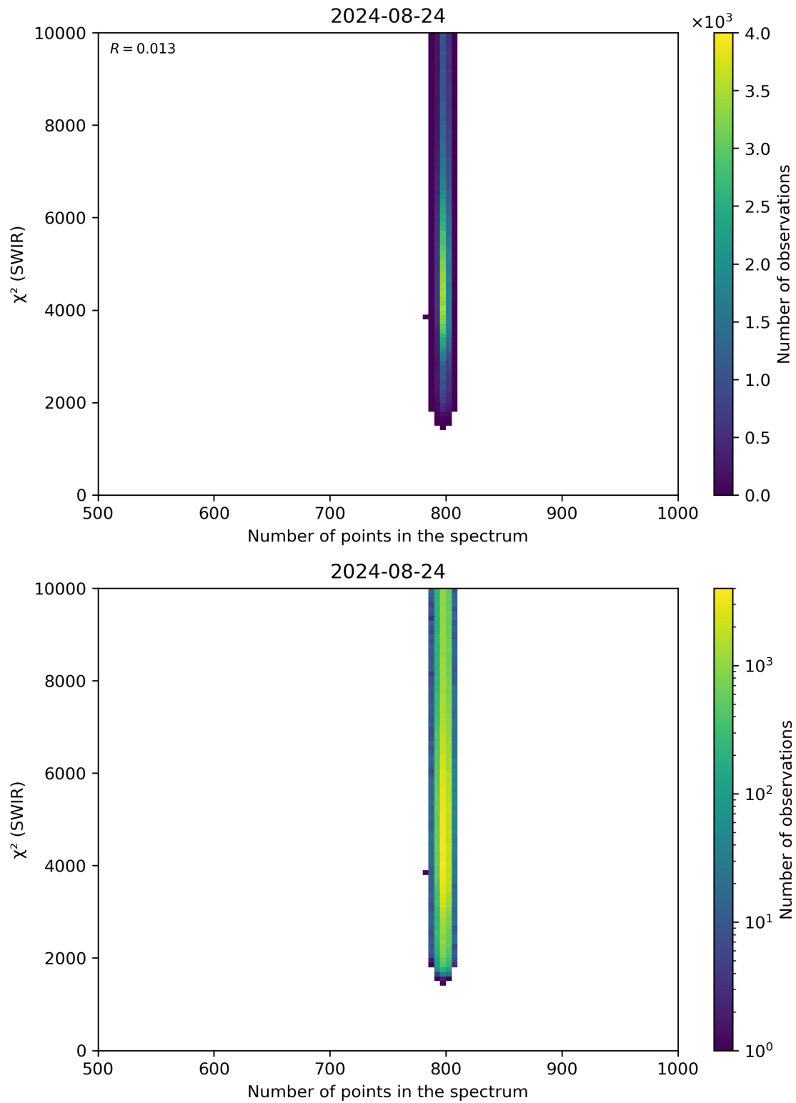
Figure 89: Scatter density plot of “Number of points in the spectrum” against “ \chi^2 (SWIR)” for 2024-08-23 to 2024-08-25.
