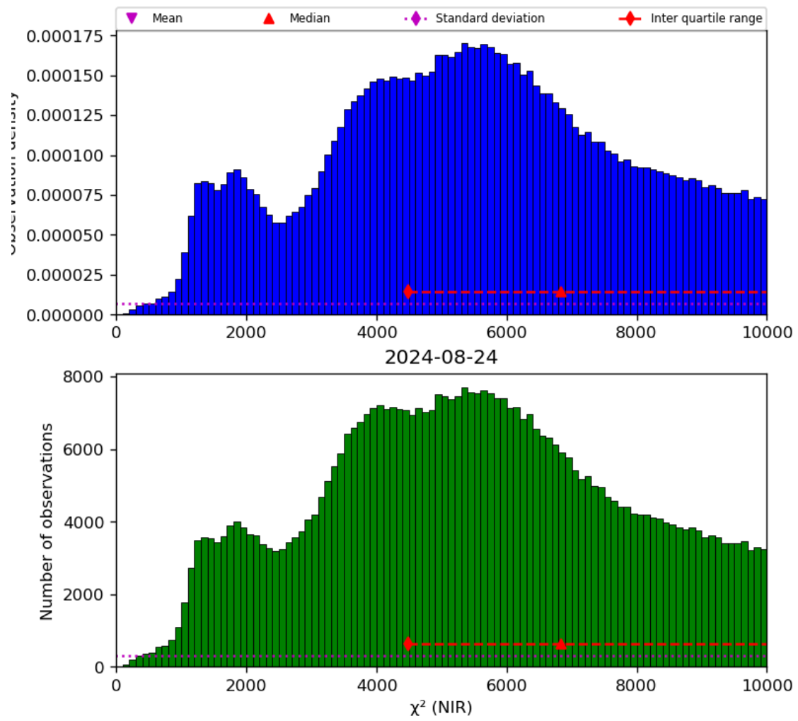
Figure 29: Histogram of “ \chi^2 (NIR)” for 2024-08-23 to 2024-08-25
