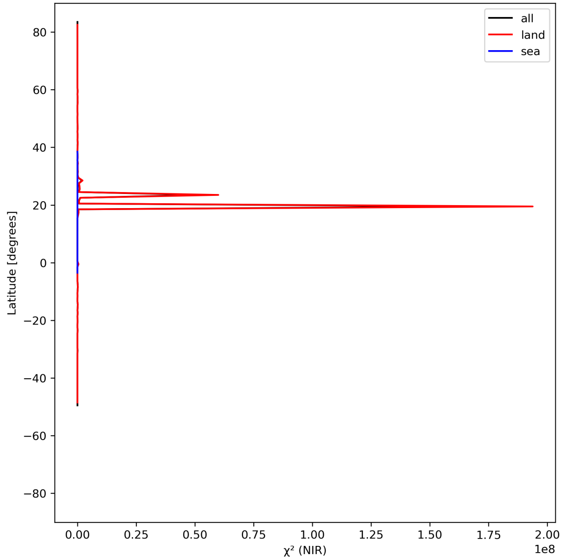
Figure 18: Zonal average of “ \chi^2 (NIR)” for 2024-08-23 to 2024-08-25.
