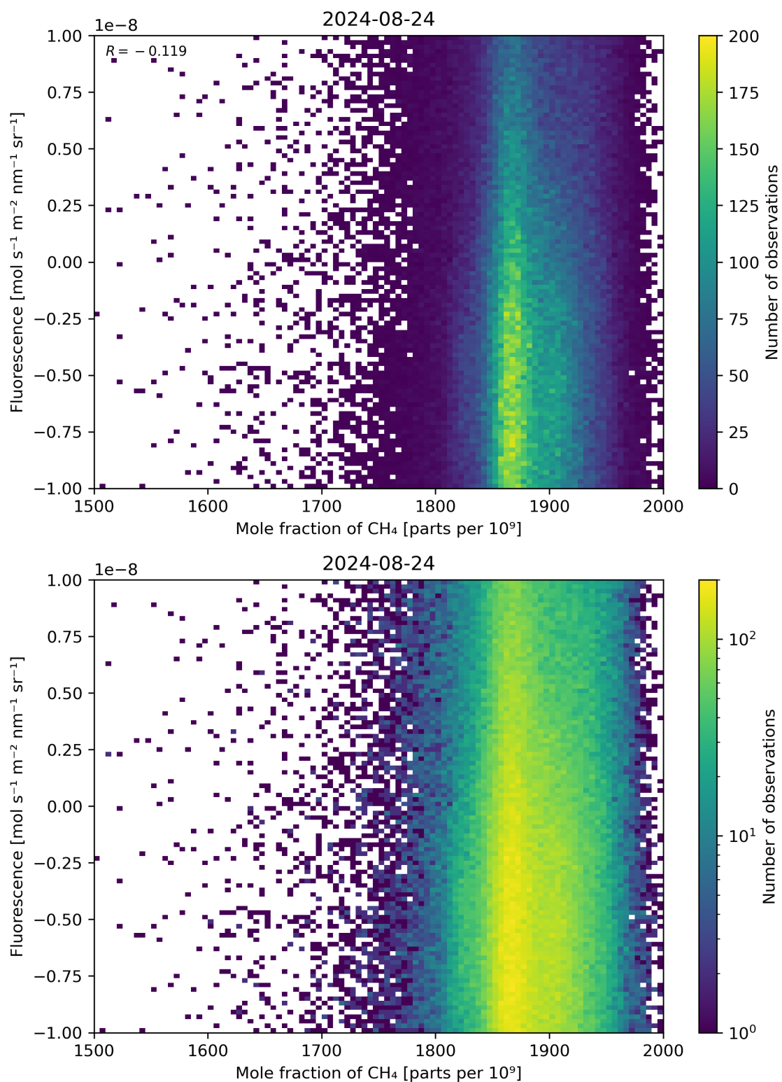
Figure 73: Scatter density plot of “Mole fraction of CH 4 ” against “Fluorescence” for 2024-08-23 to 2024-08-25.
