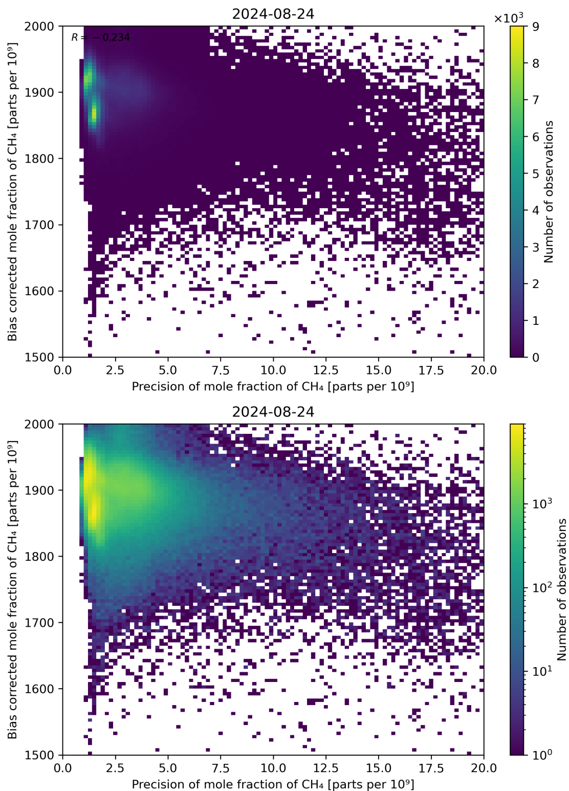
Figure 82: Scatter density plot of “Precision of mole fraction of \text{CH}_4 ” against “Bias corrected mole fraction of \text{CH}_4 ” for 2024-08-23 to 2024-08-25.
