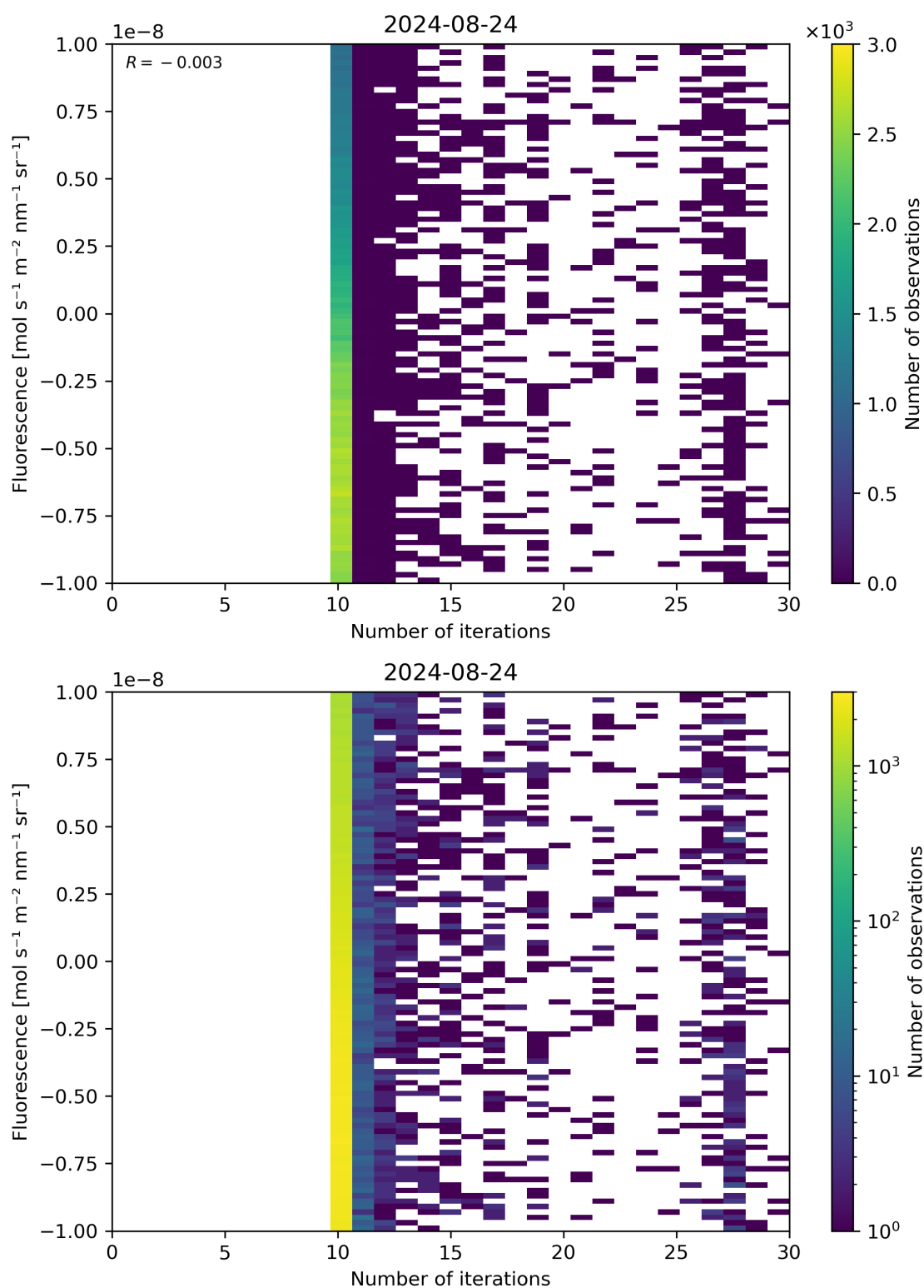
Figure 87: Scatter density plot of “Number of iterations” against “Fluorescence” for 2024-08-23 to 2024-08-25.
