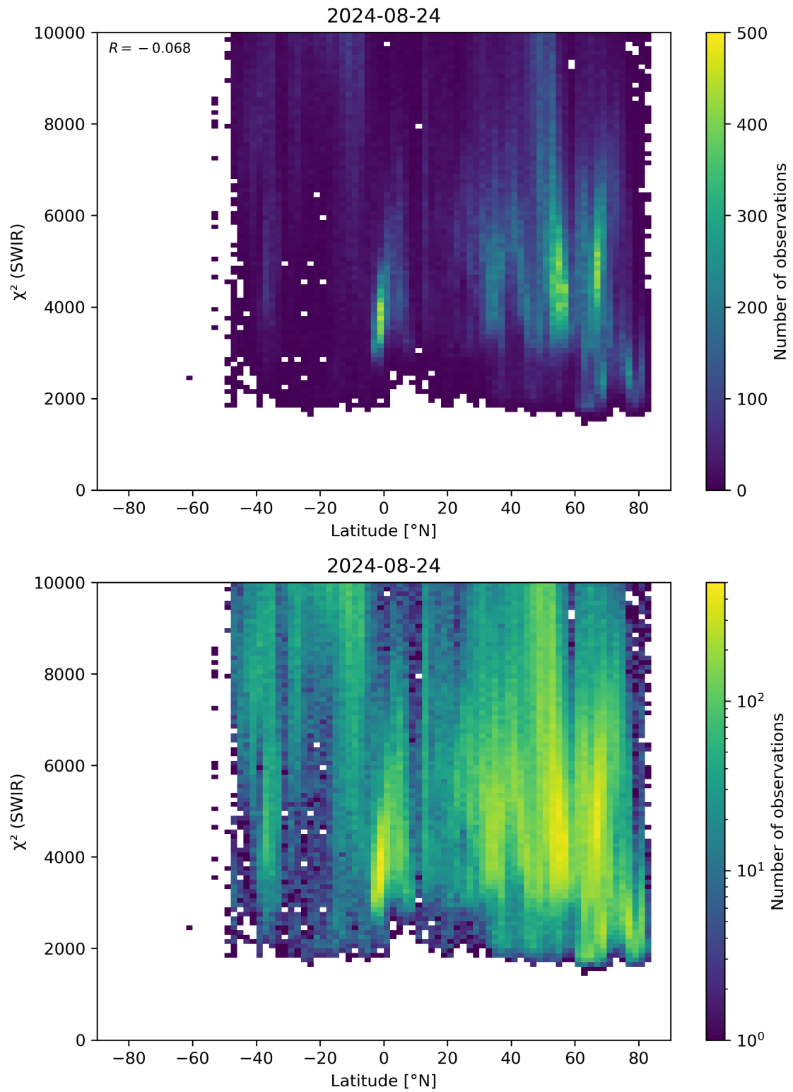
Figure 54: Scatter density plot of “Latitude” against “ \chi^2 (SWIR)” for 2024-08-23 to 2024-08-25.
