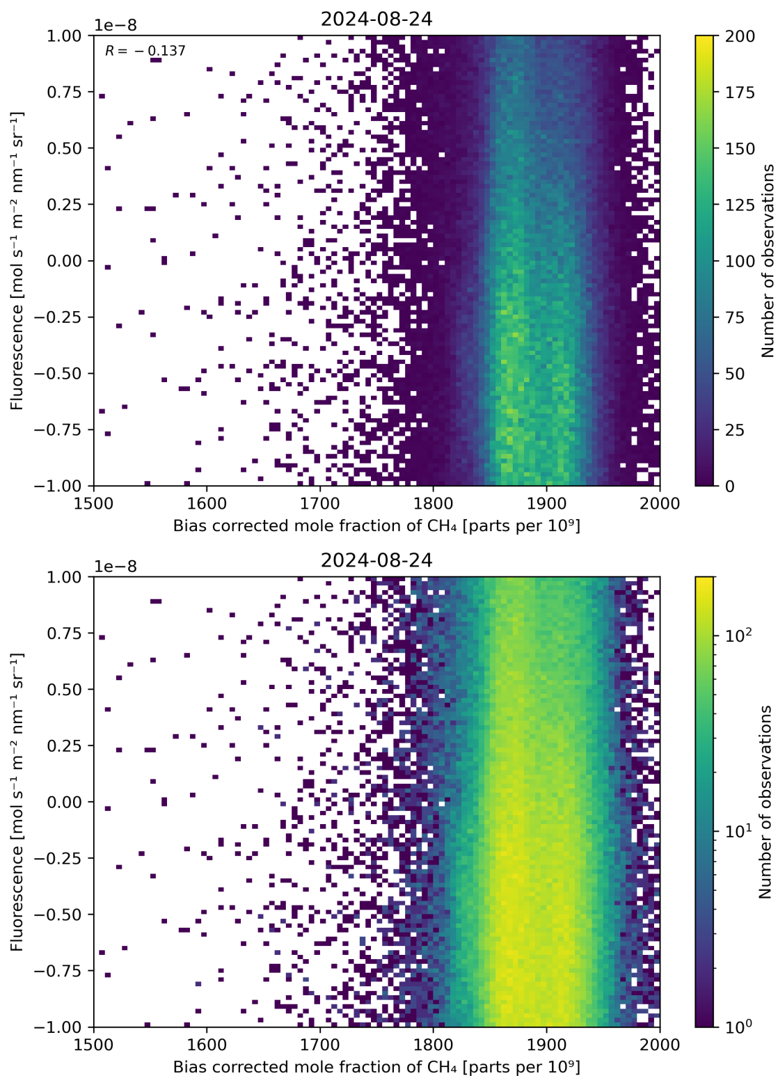
Figure 66: Scatter density plot of “Bias corrected mole fraction of \text{CH}_4 ” against “Fluorescence” for 2024-08-23 to 2024-08-25.
