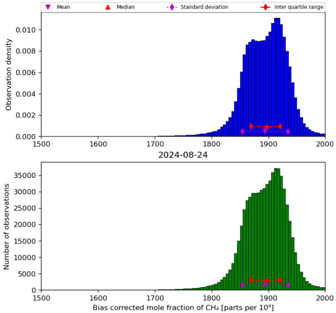
Figure 25: Histogram of “Bias corrected mole fraction of CH 4 ” for 2024-08-23 to 2024-08-25
