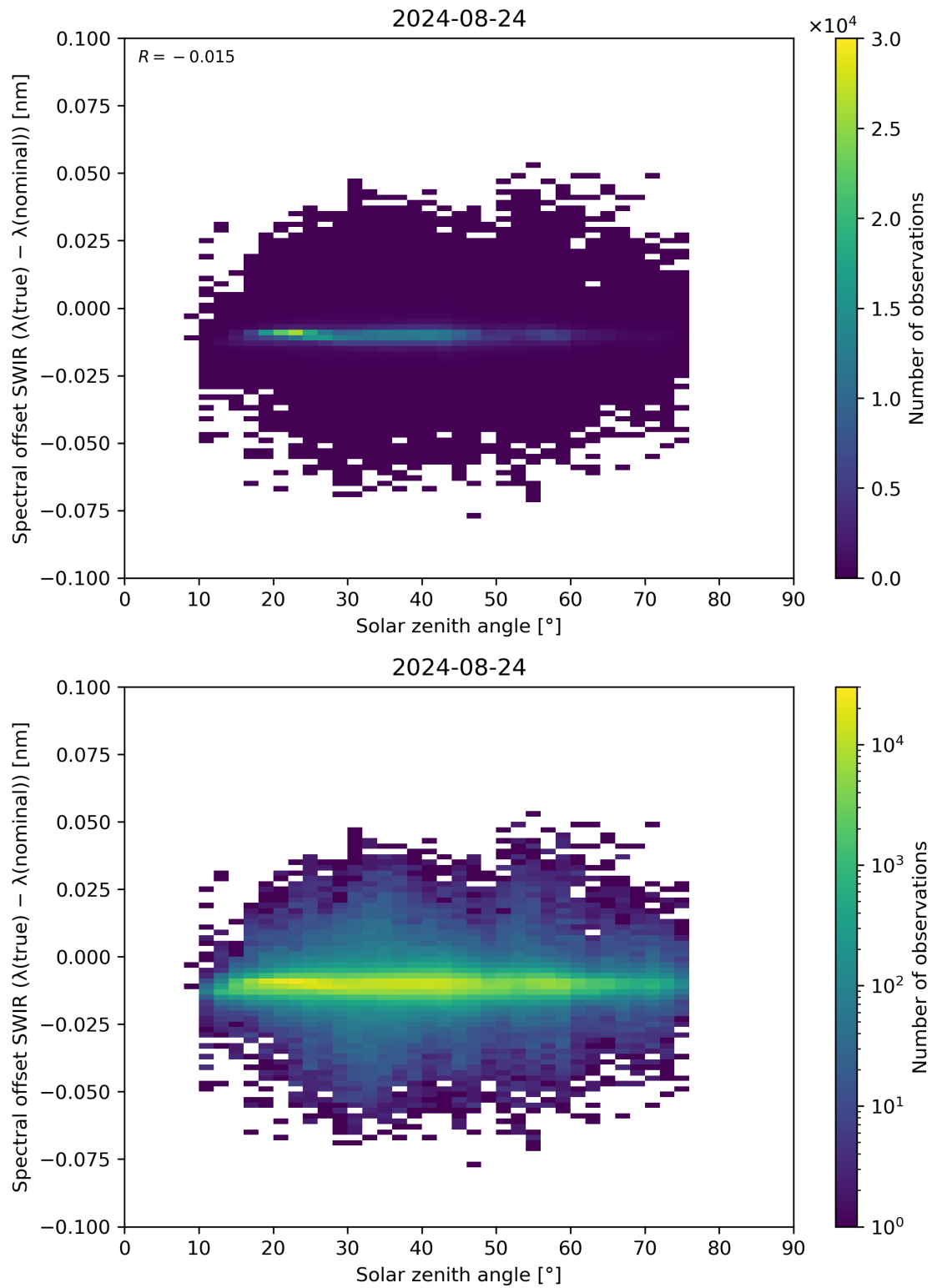
Figure 104: Scatter density plot of “Solar zenith angle” against “Spectral offset SWIR ( \lambda(\text{true}) - \lambda(\text{nominal}) )” for 2024-08-23 to 2024-08-25.
