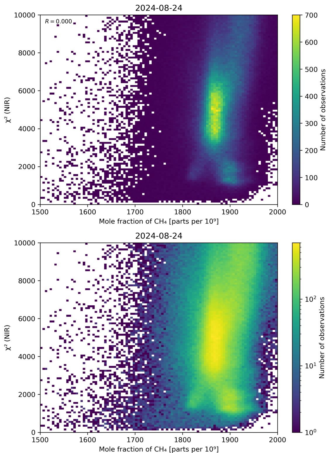
Figure 70: Scatter density plot of “Mole fraction of CH 4 ” against “ \chi^2 (NIR)” for 2024-08-23 to 2024-08-25.
