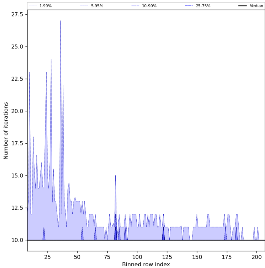
Figure 42: Along track statistics of “Number of iterations” for 2024-08-23 to 2024-08-25
