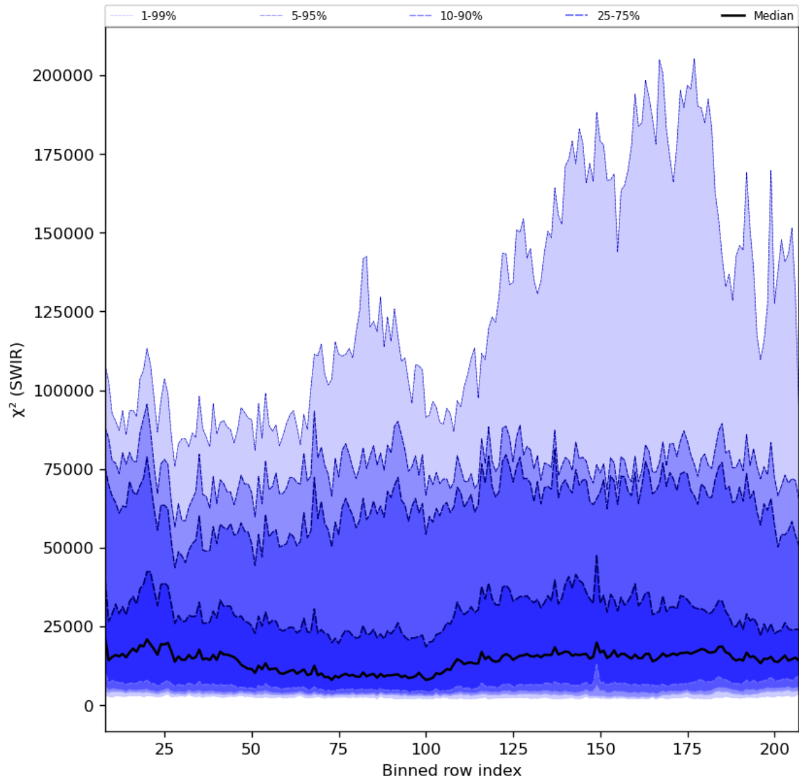
Figure 39: Along track statistics of “ \chi^2 (SWIR)” for 2024-08-23 to 2024-08-25
