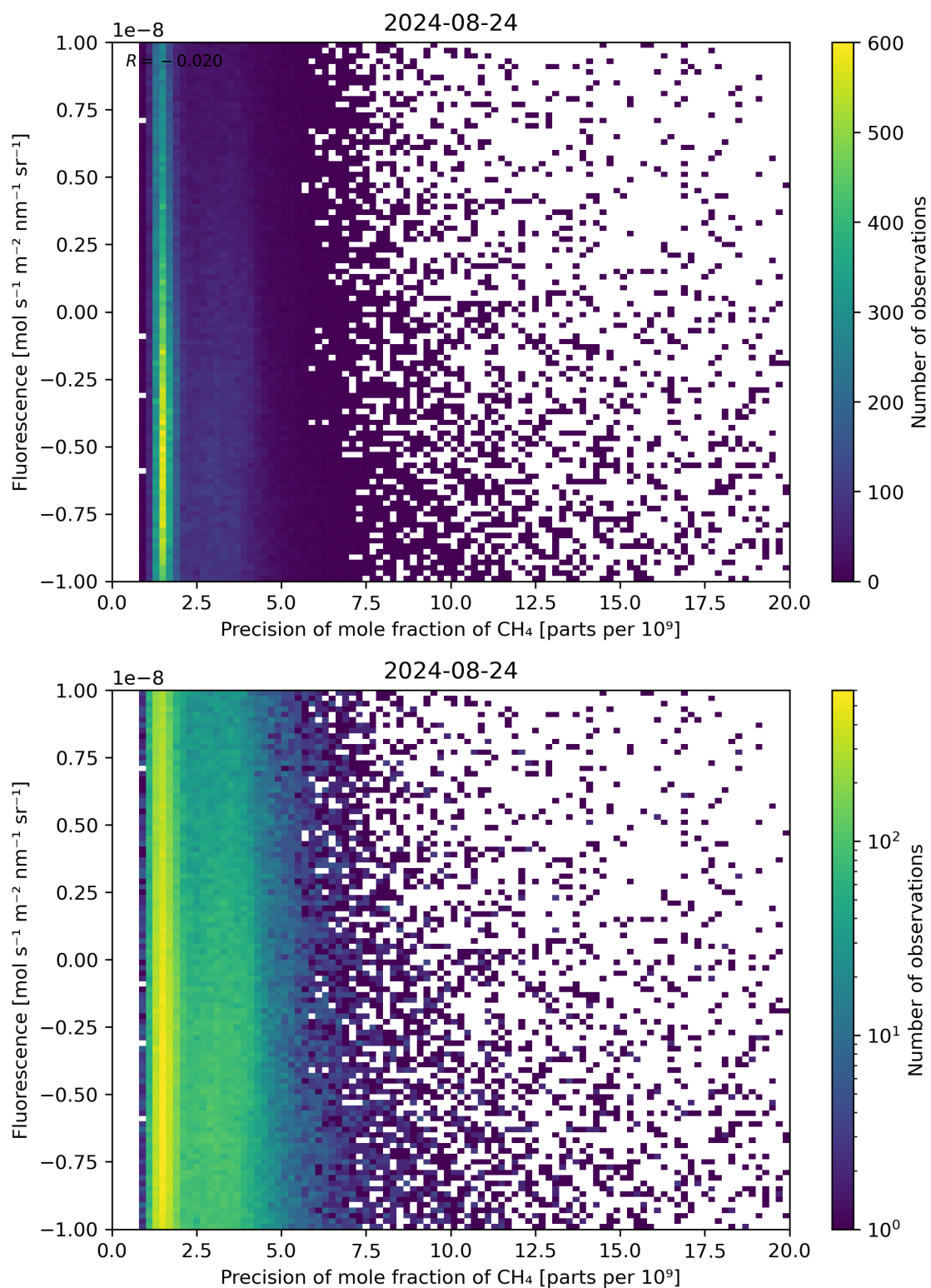
Figure 81: Scatter density plot of “Precision of mole fraction of \text{CH}_4 ” against “Fluorescence” for 2024-08-23 to 2024-08-25.
