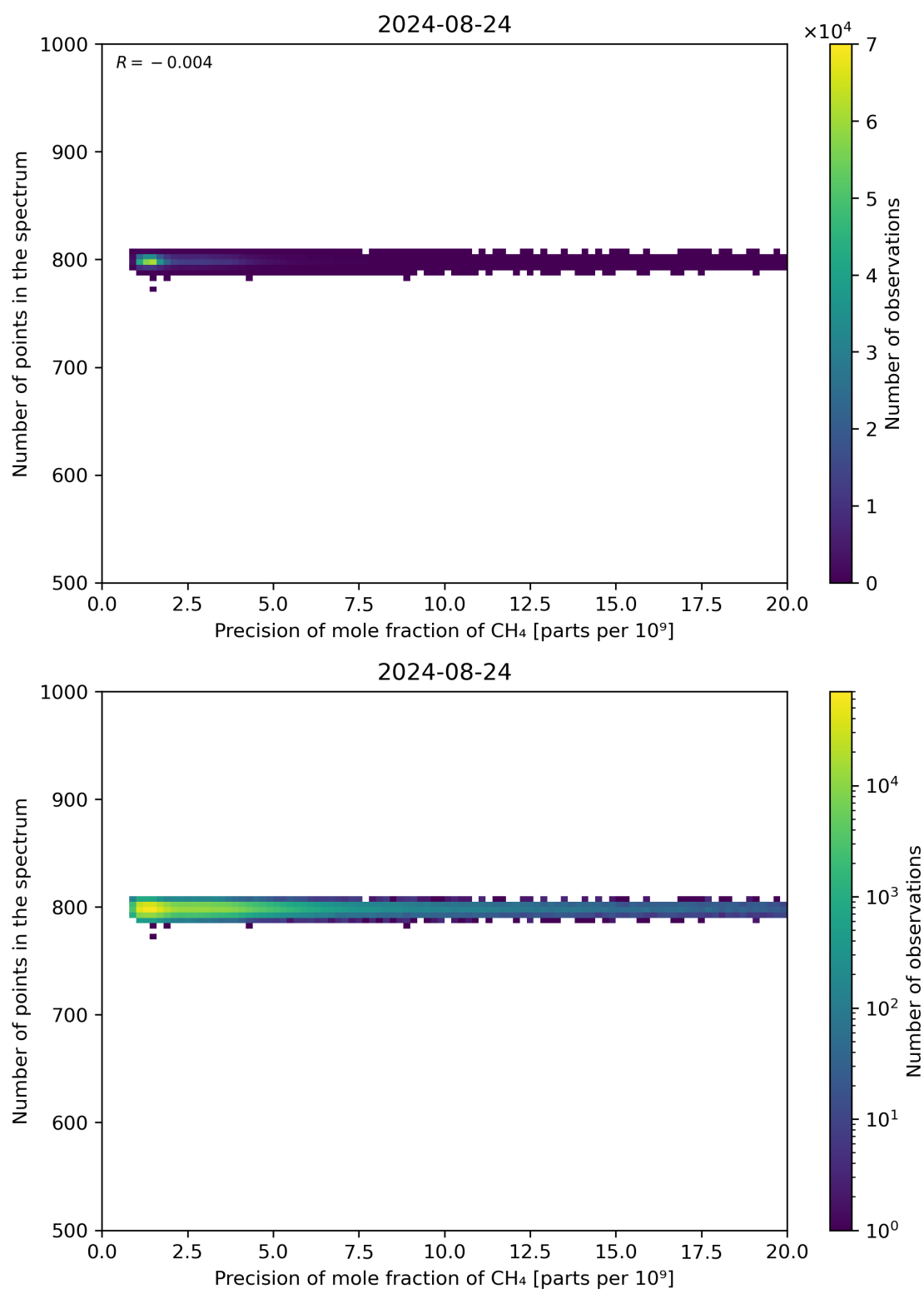
Figure 84: Scatter density plot of “Precision of mole fraction of CH 4 ” against “Number of points in the spectrum” for 2024-08-23 to 2024-08-25.
