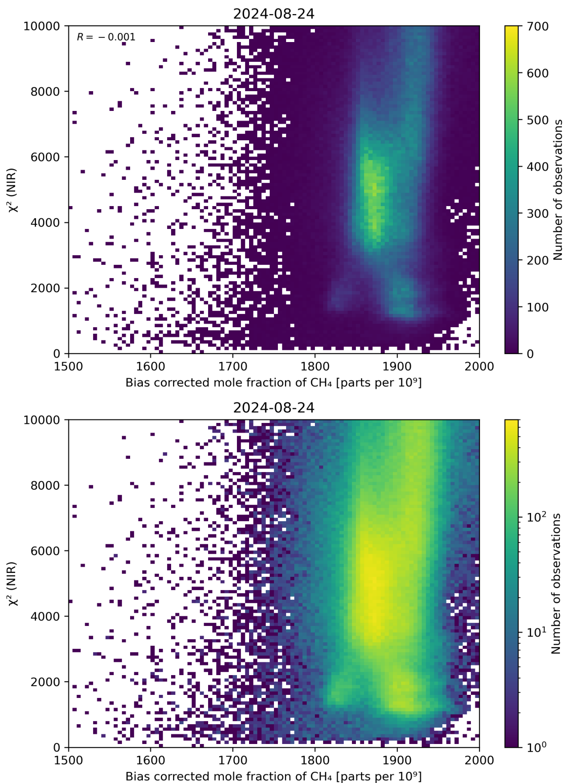
Figure 63: Scatter density plot of “Bias corrected mole fraction of CH 4 ” against “ \chi^2 (NIR)” for 2024-08-23 to 2024-08-25.
