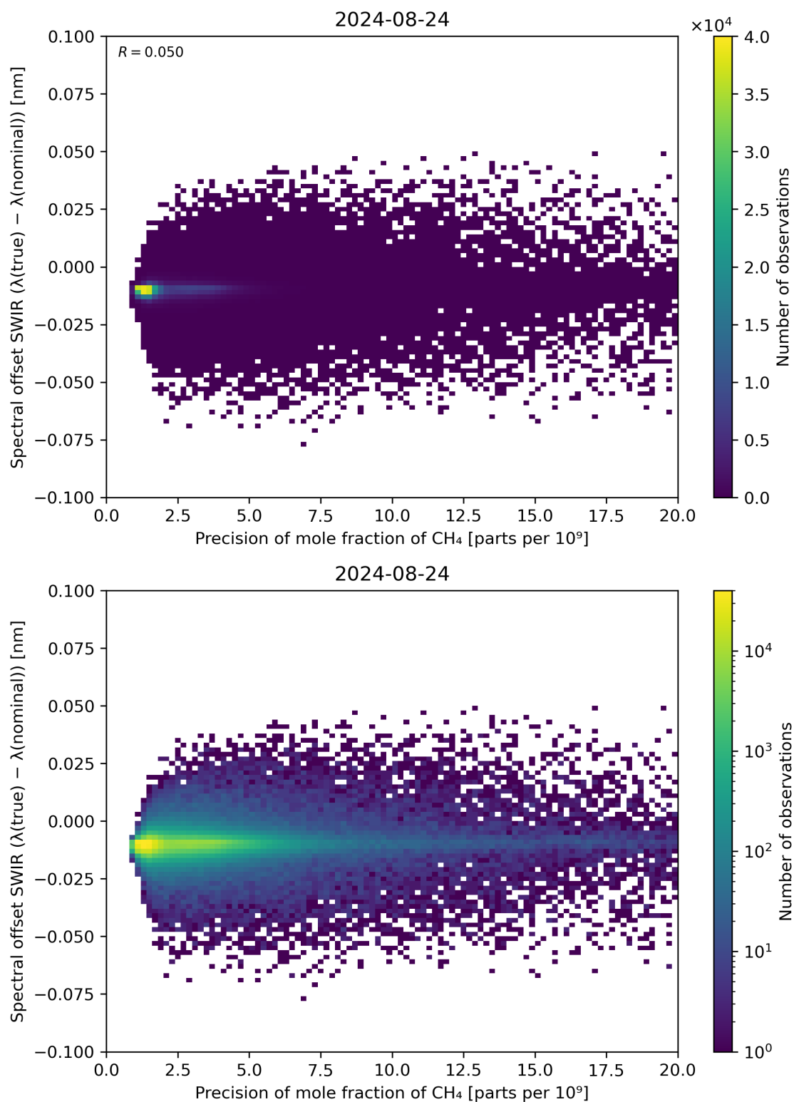
Figure 85: Scatter density plot of “Precision of mole fraction of CH 4 ” against “Spectral offset SWIR ( \lambda(\text{true}) - \lambda(\text{nominal}) )” for 2024-08-23 to 2024-08-25.
