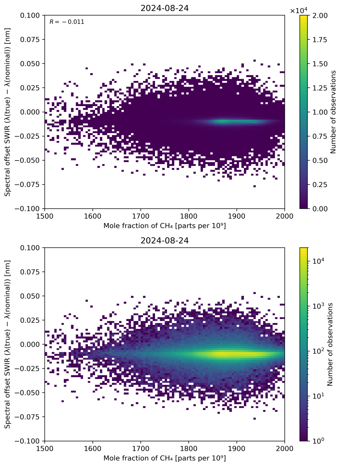
Figure 86: Scatter density plot of “Mole fraction of CH 4 ” against “Spectral offset SWIR ( \lambda(\text{true}) - \lambda(\text{nominal}) )” for 2024-08-23 to 2024-08-25.
