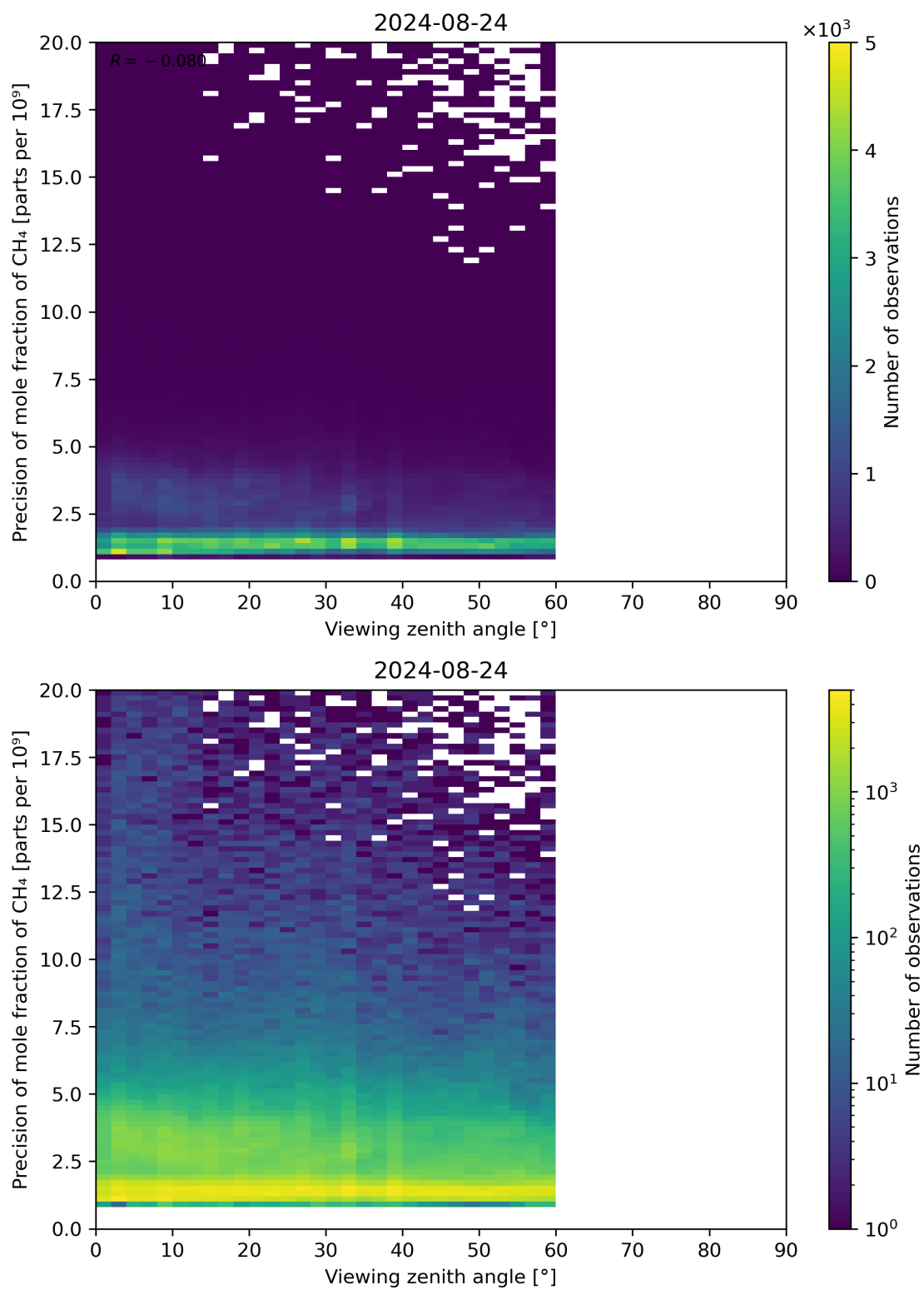
Figure 112: Scatter density plot of “Viewing zenith angle” against “Precision of mole fraction of CH 4 ” for 2024-08-23 to 2024-08-25.
