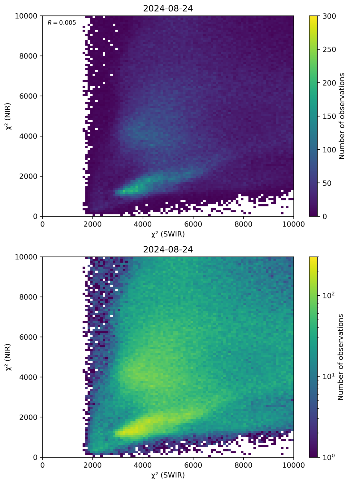
Figure 47: Scatter density plot of “ \chi^2 (SWIR)” against “ \chi^2 (NIR)” for 2024-08-23 to 2024-08-25.
