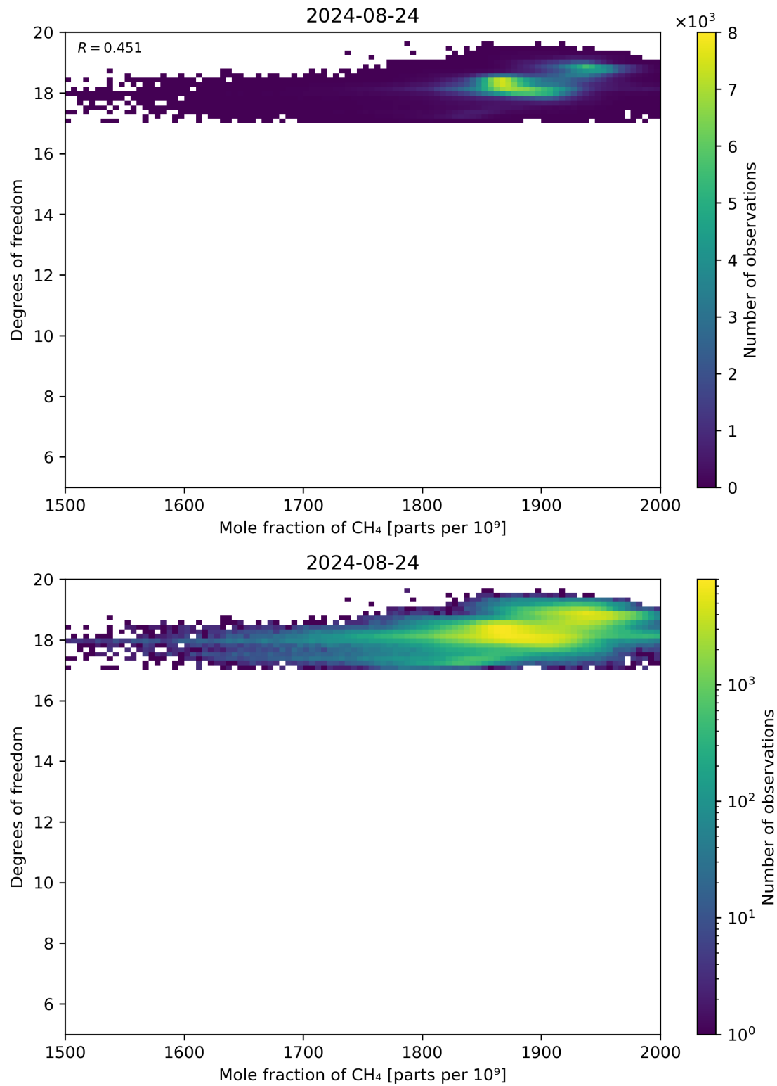
Figure 72: Scatter density plot of “Mole fraction of CH 4 ” against “Degrees of freedom” for 2024-08-23 to 2024-08-25.
