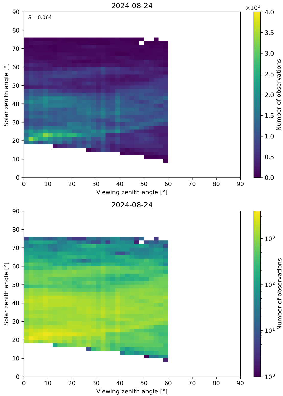
Figure 115: Scatter density plot of “Viewing zenith angle” against “Solar zenith angle” for 2024-08-23 to 2024-08-25.
