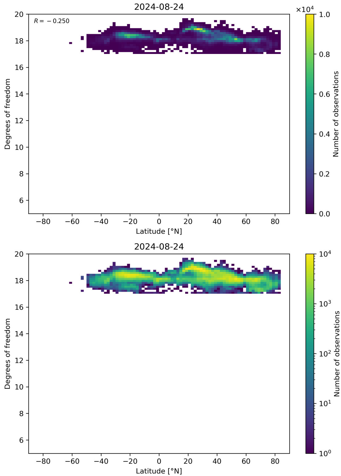
Figure 55: Scatter density plot of “Latitude” against “Degrees of freedom” for 2024-08-23 to 2024-08-25.
