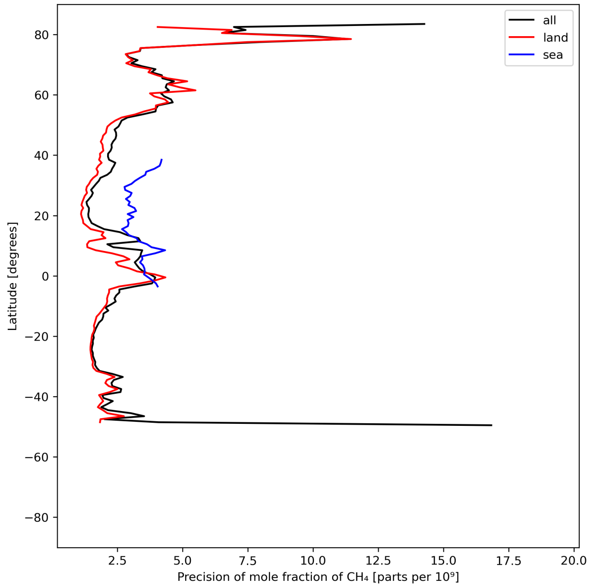
Figure 13: Zonal average of “Precision of mole fraction of CH 4 ” for 2024-08-23 to 2024-08-25.
