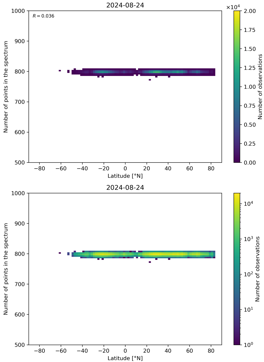
Figure 61: Scatter density plot of “Latitude” against “Number of points in the spectrum” for 2024-08-23 to 2024-08-25.
