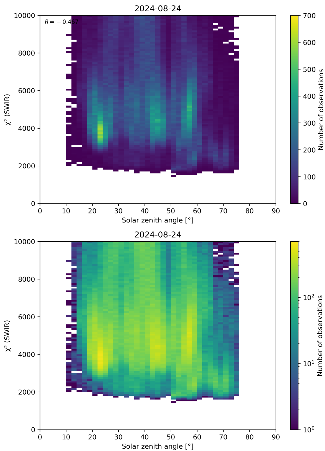
Figure 95: Scatter density plot of “Solar zenith angle” against “ \chi^2 (SWIR)” for 2024-08-23 to 2024-08-25.
