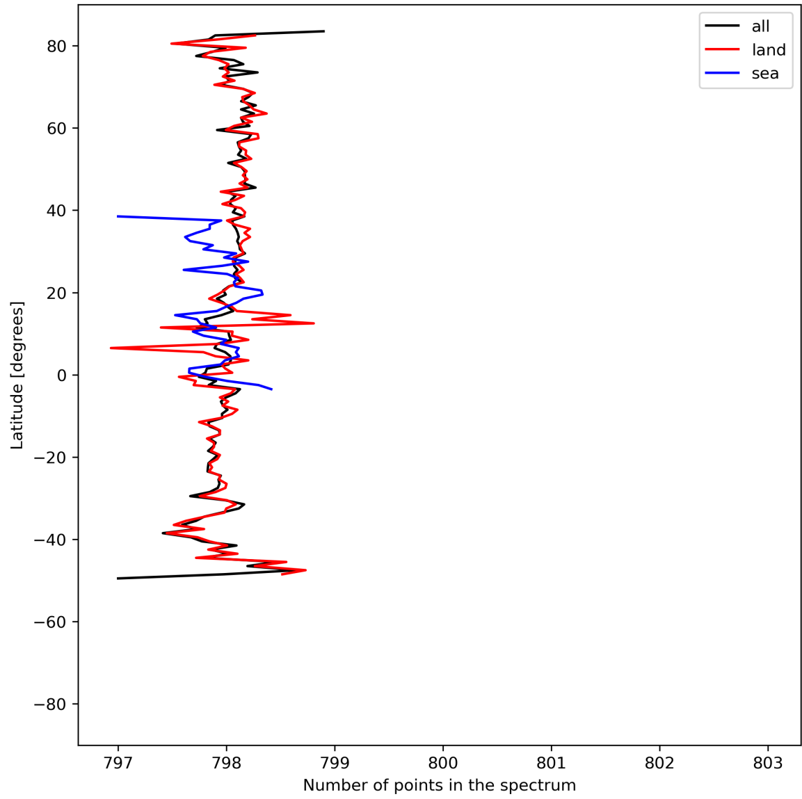
Figure 15: Zonal average of “Number of points in the spectrum” for 2024-08-23 to 2024-08-25.
