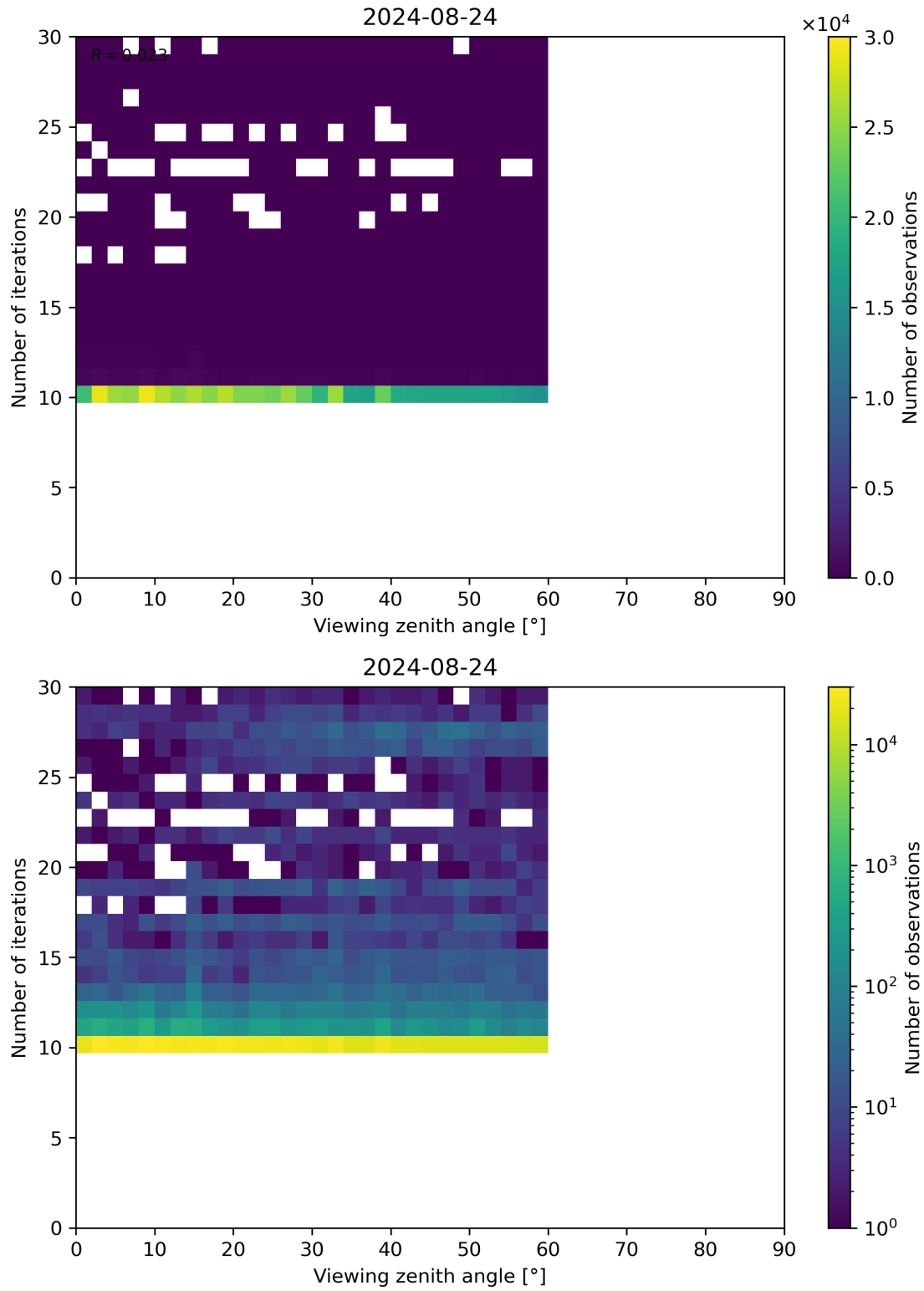
Figure 113: Scatter density plot of “Viewing zenith angle” against “Number of iterations” for 2024-08-23 to 2024-08-25.
