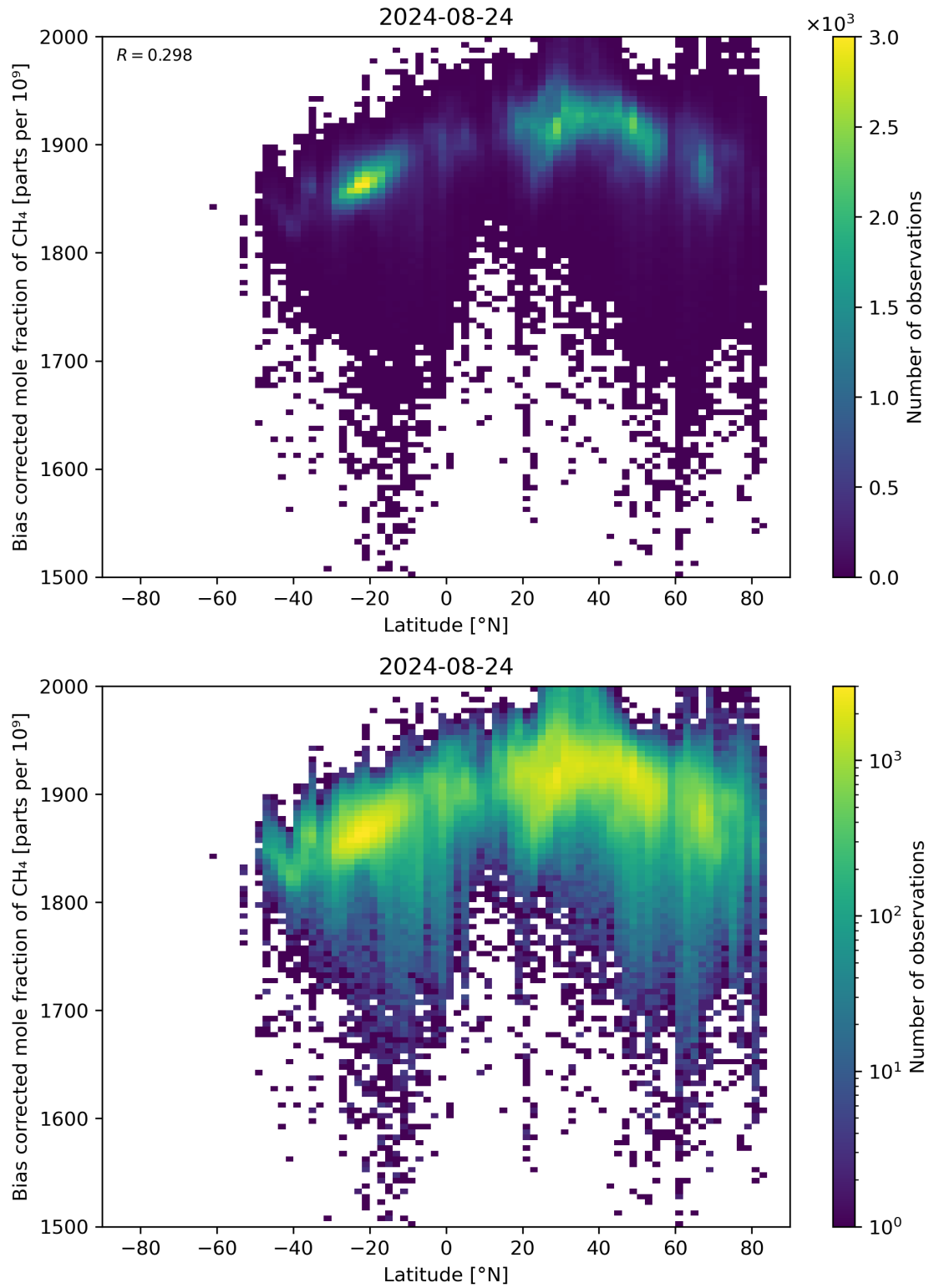
Figure 58: Scatter density plot of “Latitude” against “Bias corrected mole fraction of CH 4 ” for 2024-08-23 to 2024-08-25.
