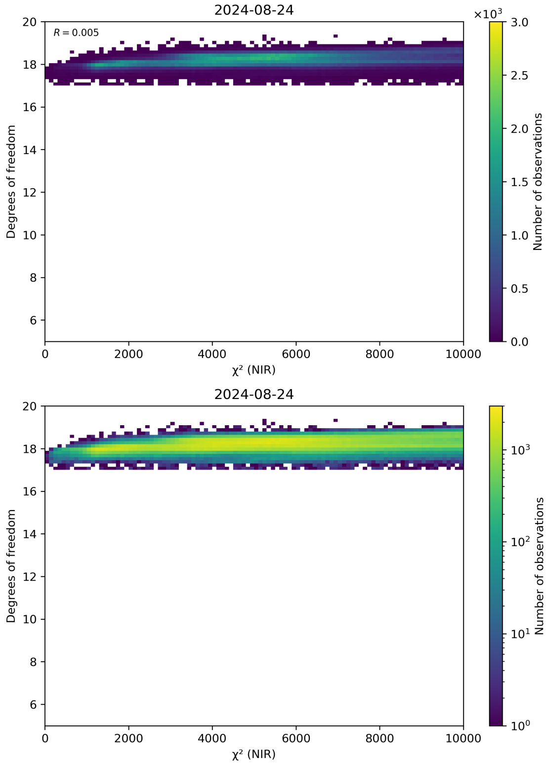
Figure 44: Scatter density plot of “ \chi^2 (NIR)” against “Degrees of freedom” for 2024-08-23 to 2024-08-25.
