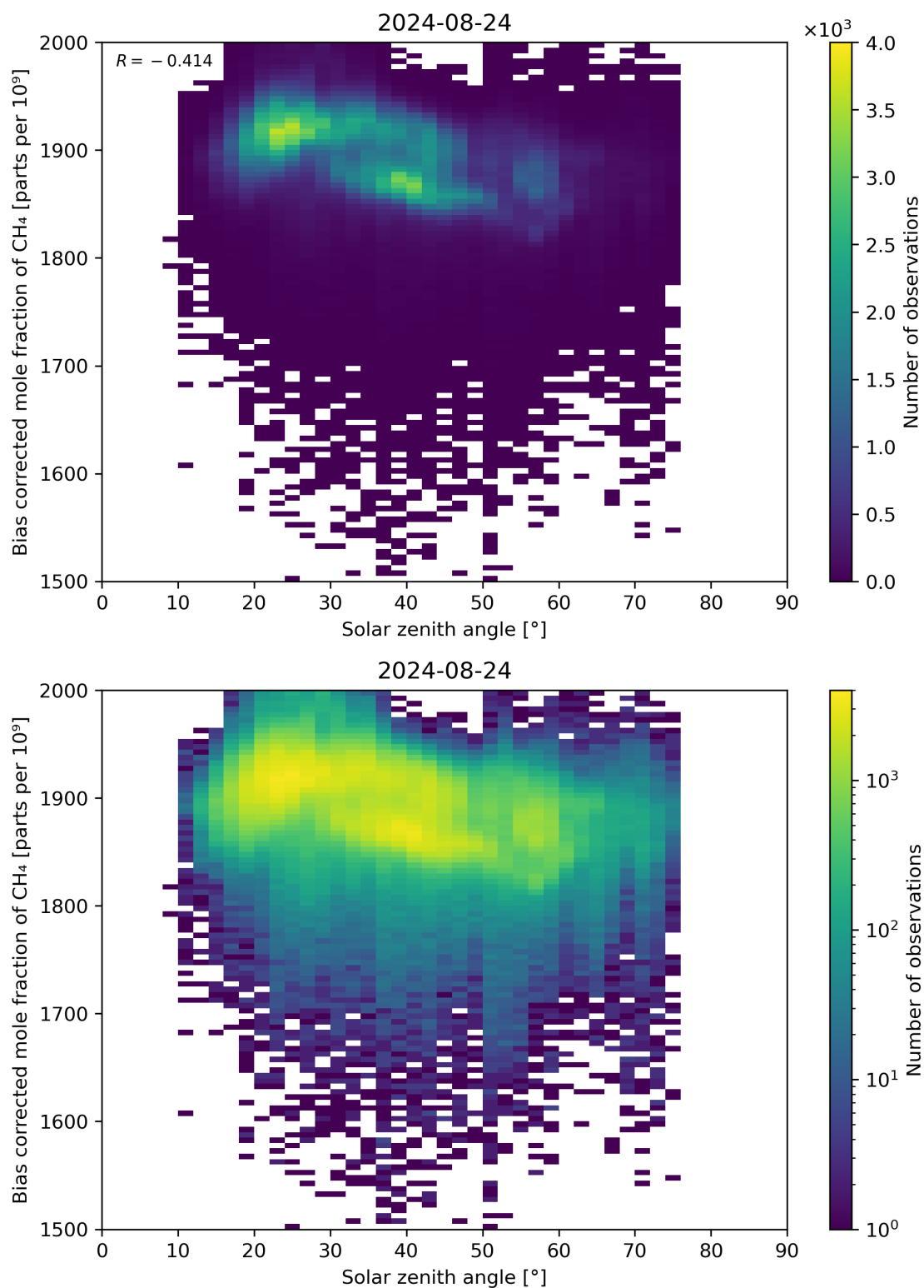
Figure 100: Scatter density plot of “Solar zenith angle” against “Bias corrected mole fraction of CH 4 ” for 2024-08-23 to 2024-08-25.
