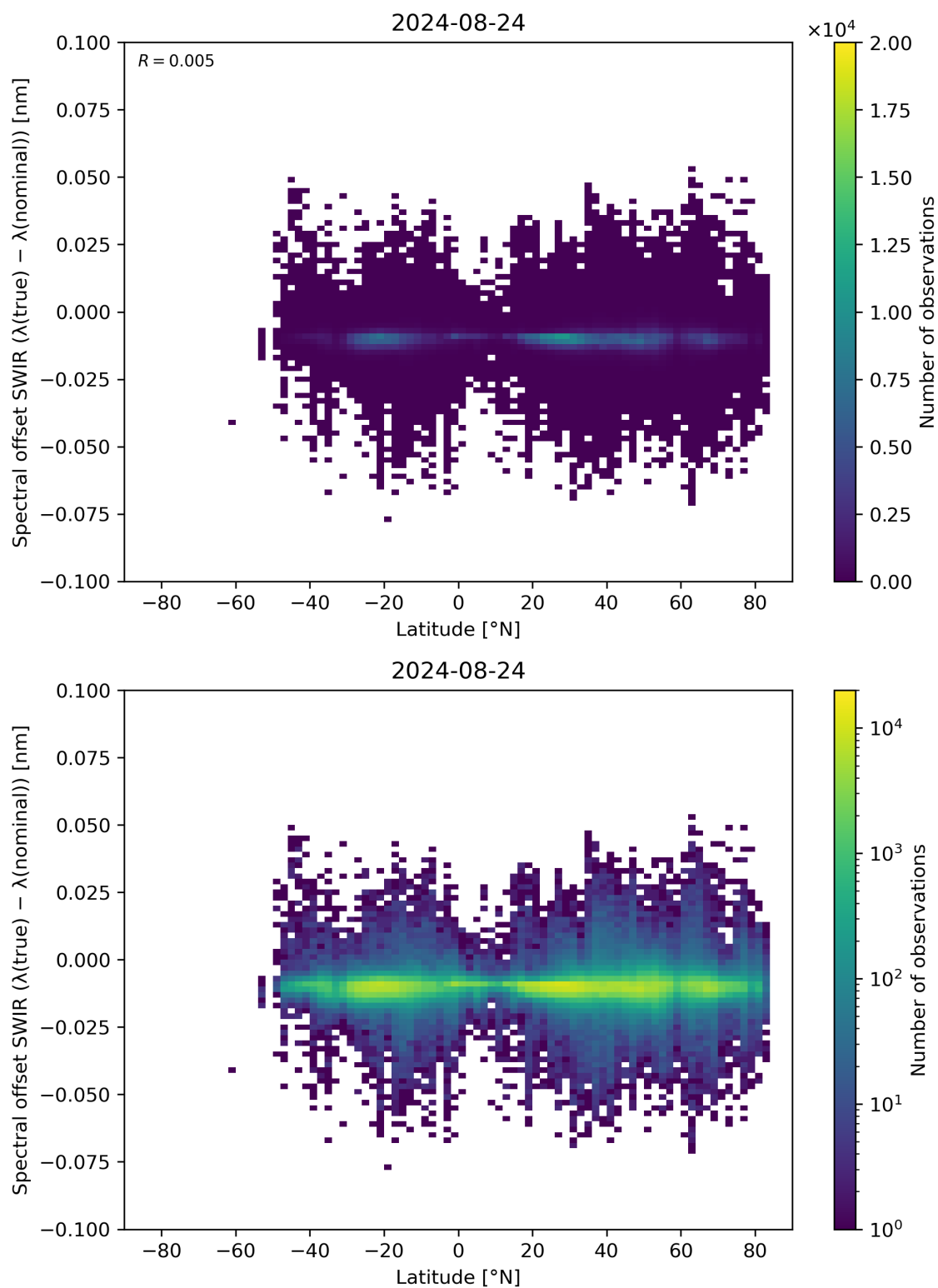
Figure 62: Scatter density plot of “Latitude” against “Spectral offset SWIR ( \lambda(\text{true}) - \lambda(\text{nominal}) )” for 2024-08-23 to 2024-08-25.
