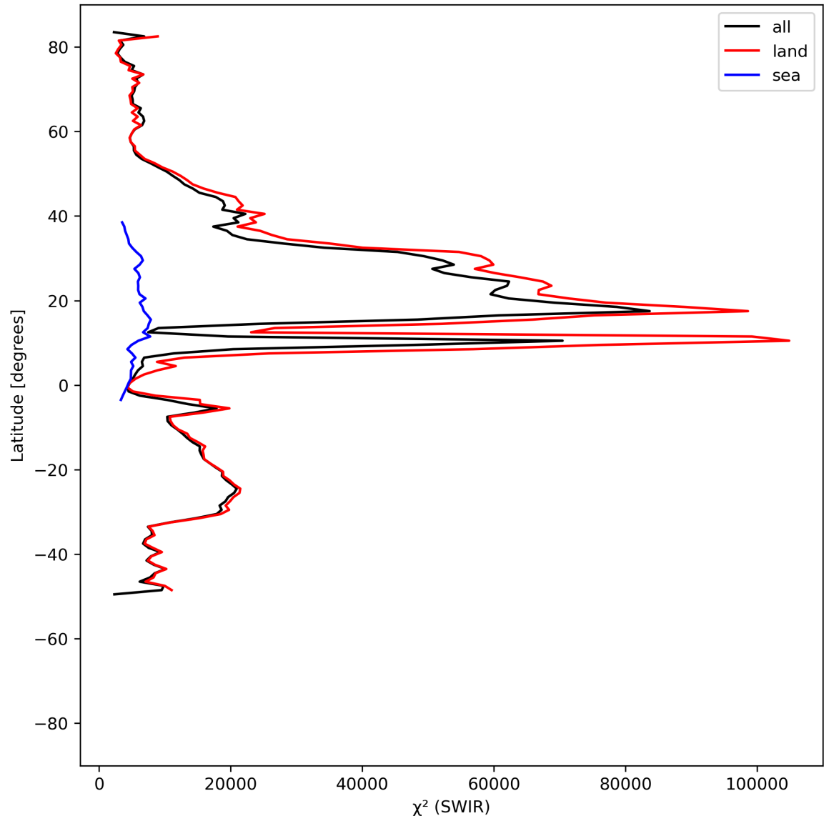
Figure 17: Zonal average of “ \chi^2 (SWIR)” for 2024-08-23 to 2024-08-25.
