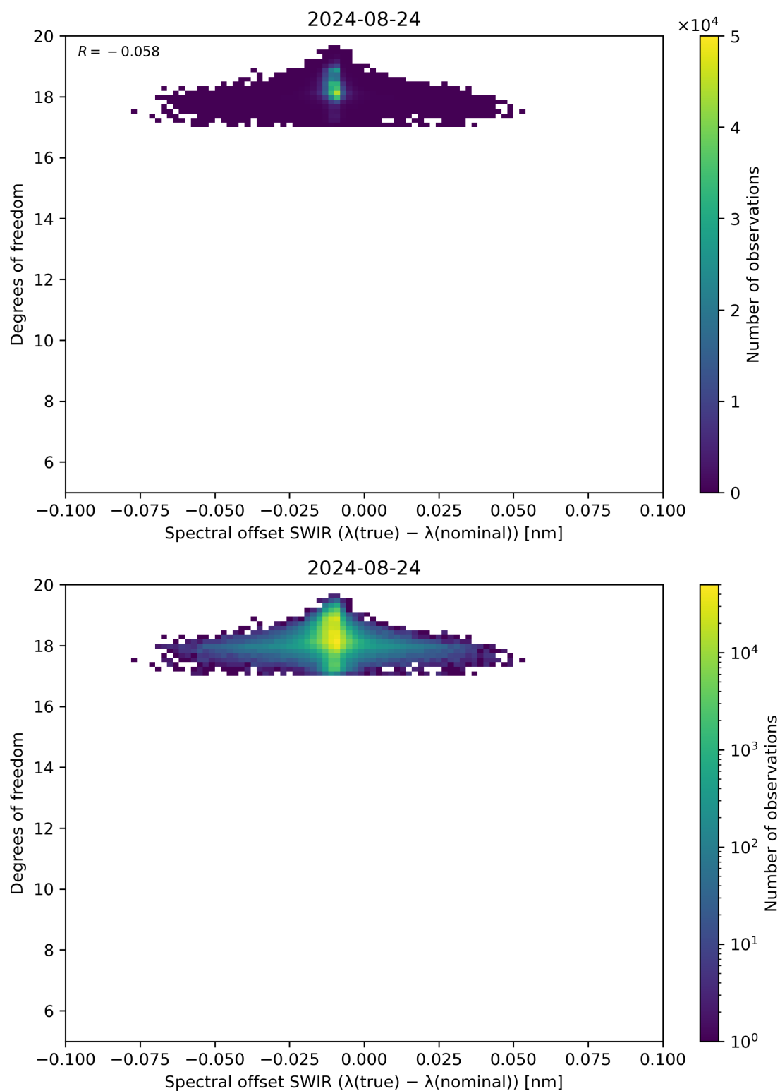
Figure 119: Scatter density plot of “Spectral offset SWIR ( \lambda(\text{true}) - \lambda(\text{nominal}) )” against “Degrees of freedom” for 2024-08-23 to 2024-08-25.
