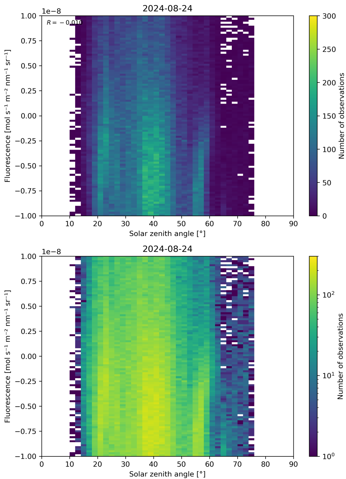
Figure 97: Scatter density plot of “Solar zenith angle” against “Fluorescence” for 2024-08-23 to 2024-08-25.
