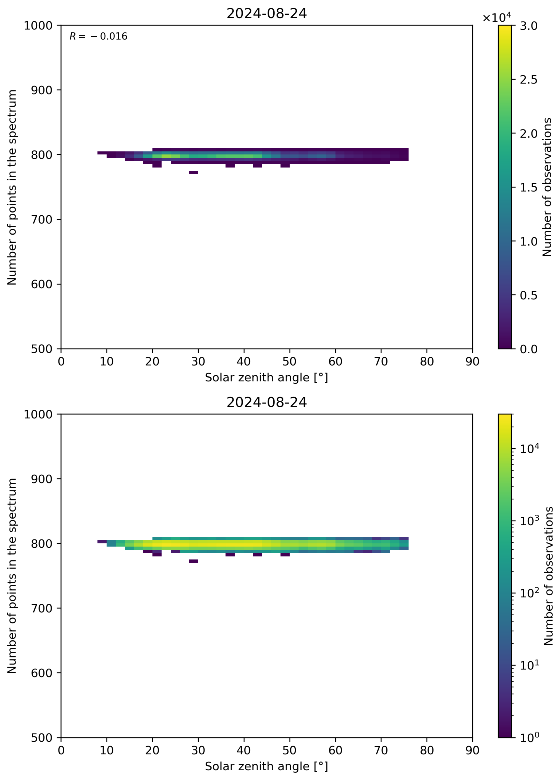
Figure 103: Scatter density plot of “Solar zenith angle” against “Number of points in the spectrum” for 2024-08-23 to 2024-08-25.
