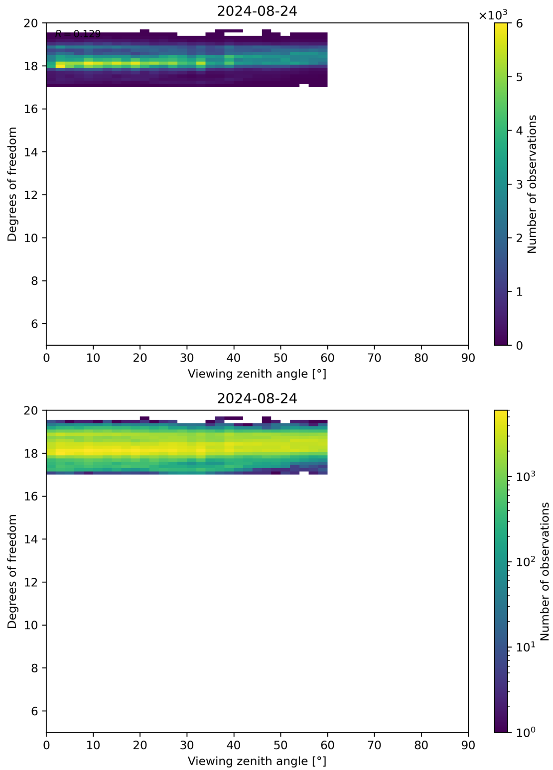
Figure 107: Scatter density plot of “Viewing zenith angle” against “Degrees of freedom” for 2024-08-23 to 2024-08-25.
