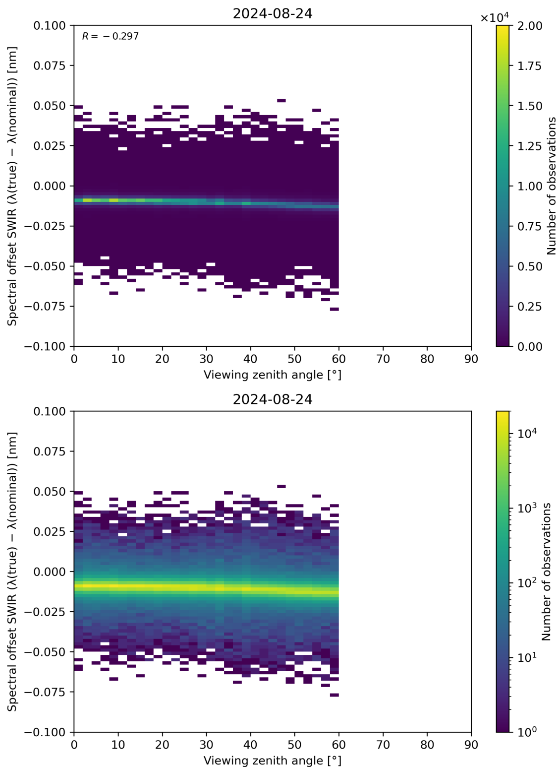
Figure 116: Scatter density plot of “Viewing zenith angle” against “Spectral offset SWIR ( \lambda(\text{true}) - \lambda(\text{nominal}) )” for 2024-08-23 to 2024-08-25.
