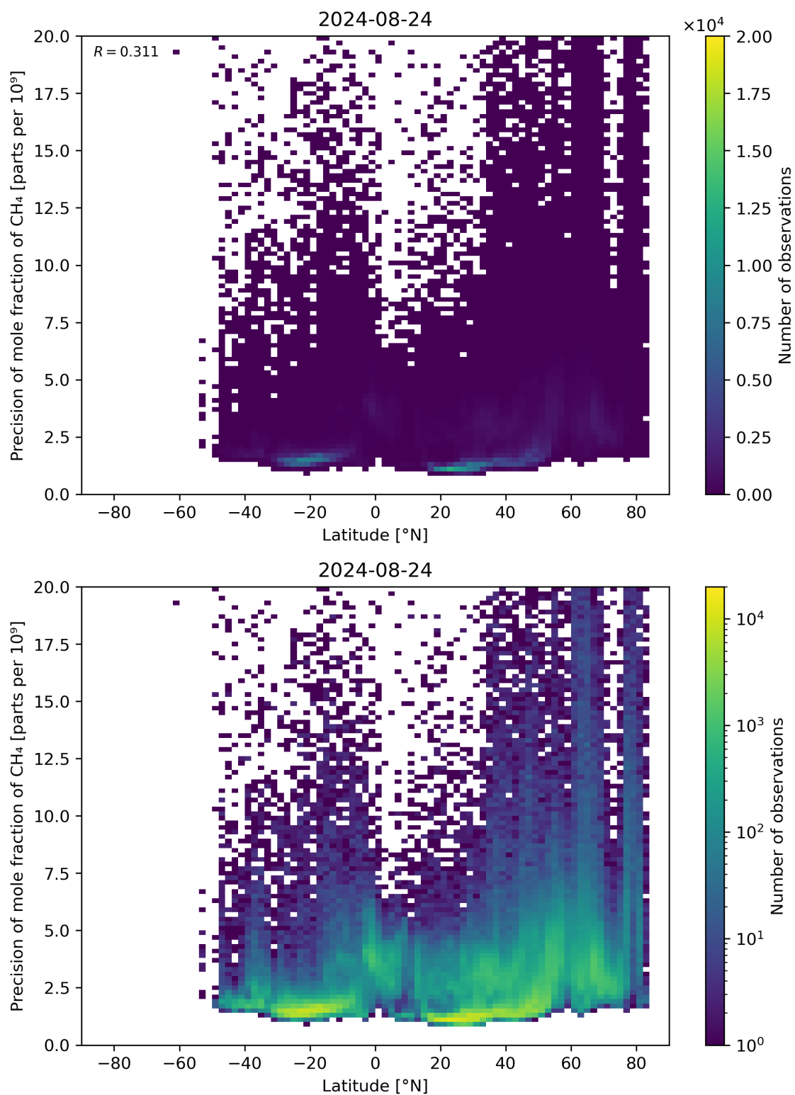
Figure 59: Scatter density plot of “Latitude” against “Precision of mole fraction of CH 4 ” for 2024-08-23 to 2024-08-25.
