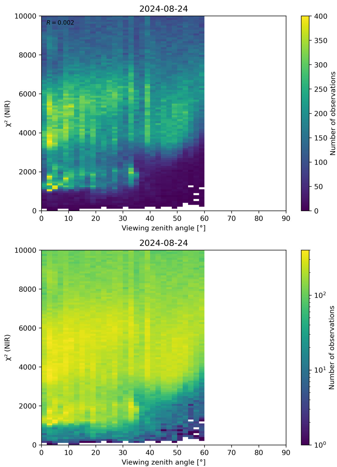
Figure 105: Scatter density plot of “Viewing zenith angle” against “ \chi^2 (NIR)” for 2024-08-23 to 2024-08-25.
