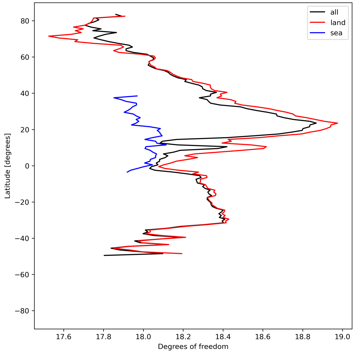
Figure 19: Zonal average of “Degrees of freedom” for 2024-08-23 to 2024-08-25.
