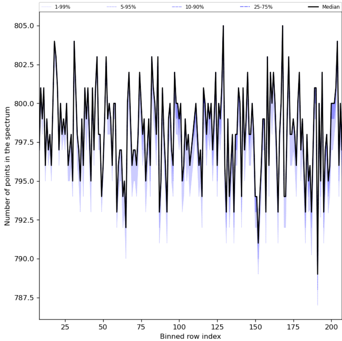
Figure 37: Along track statistics of “Number of points in the spectrum” for 2024-08-23 to 2024-08-25
