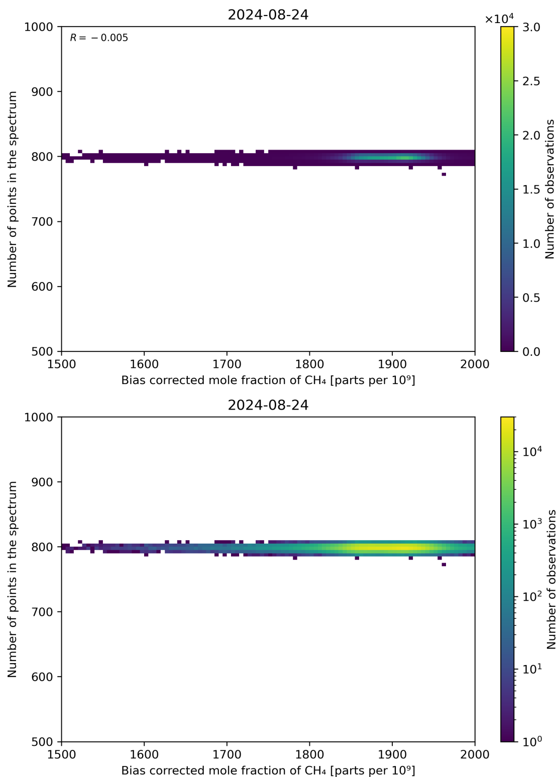
Figure 68: Scatter density plot of “Bias corrected mole fraction of CH 4 ” against “Number of points in the spectrum” for 2024-08-23 to 2024-08-25.
