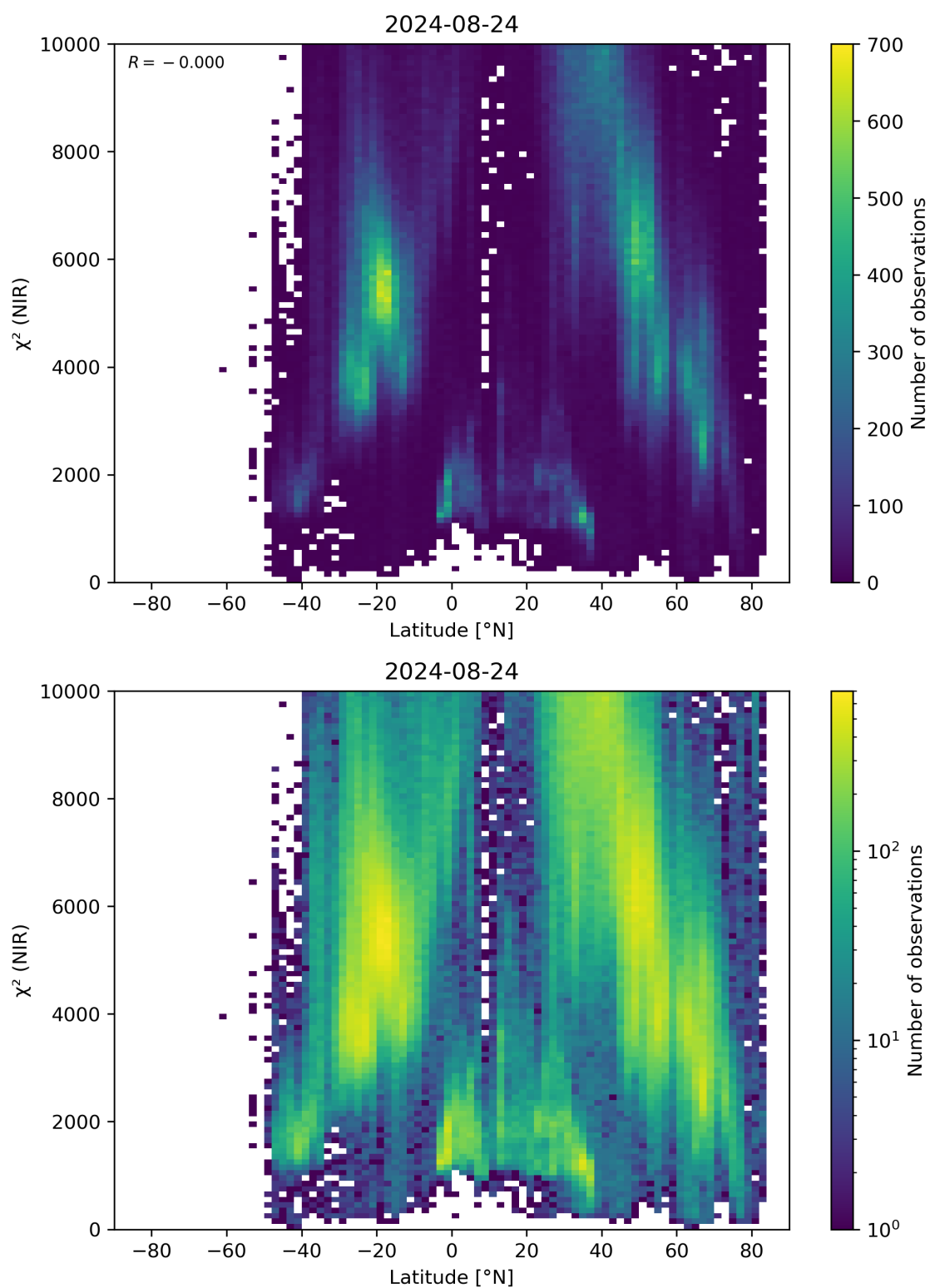
Figure 53: Scatter density plot of “Latitude” against “ \chi^2 (NIR)” for 2024-08-23 to 2024-08-25.
