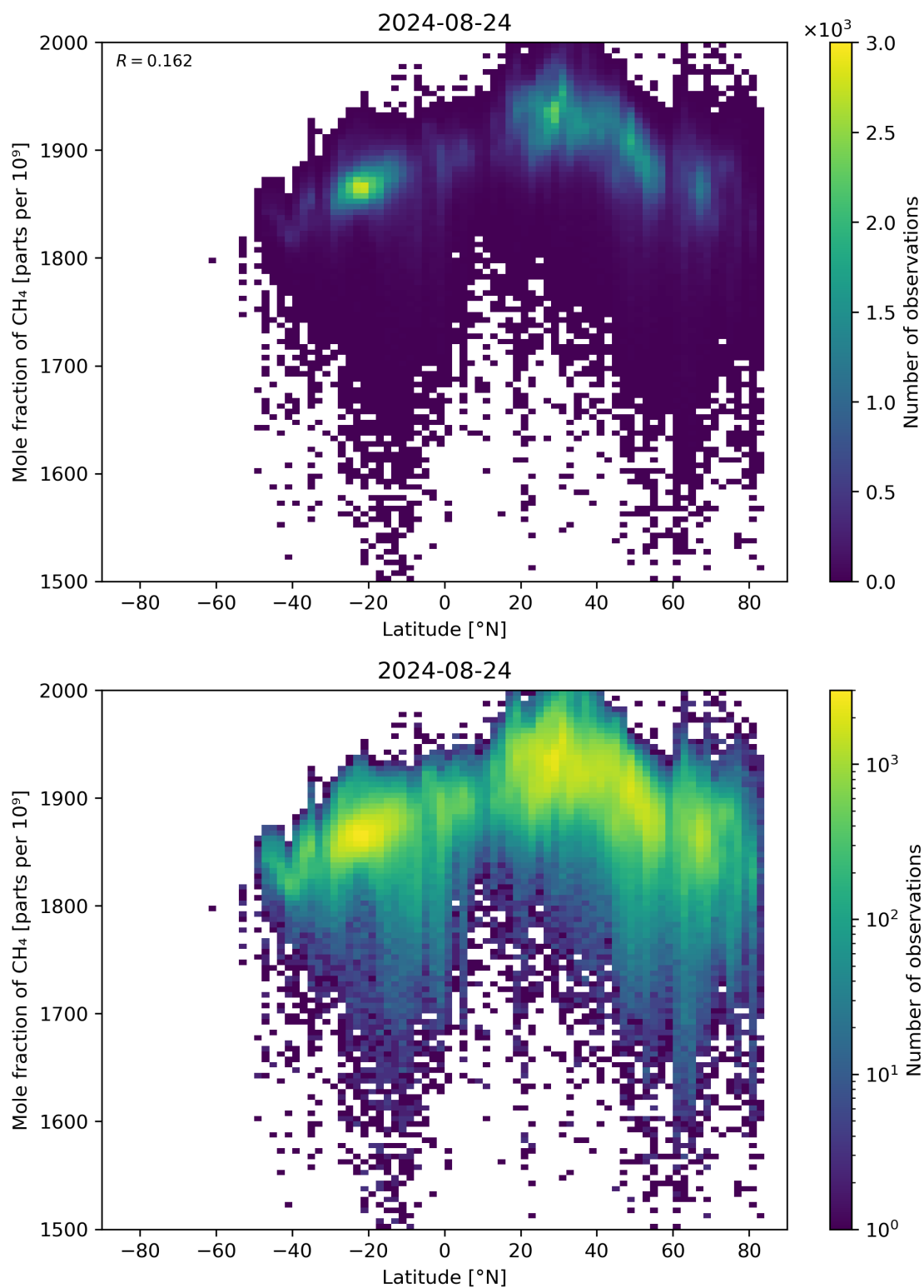
Figure 57: Scatter density plot of “Latitude” against “Mole fraction of CH 4 ” for 2024-08-23 to 2024-08-25.
