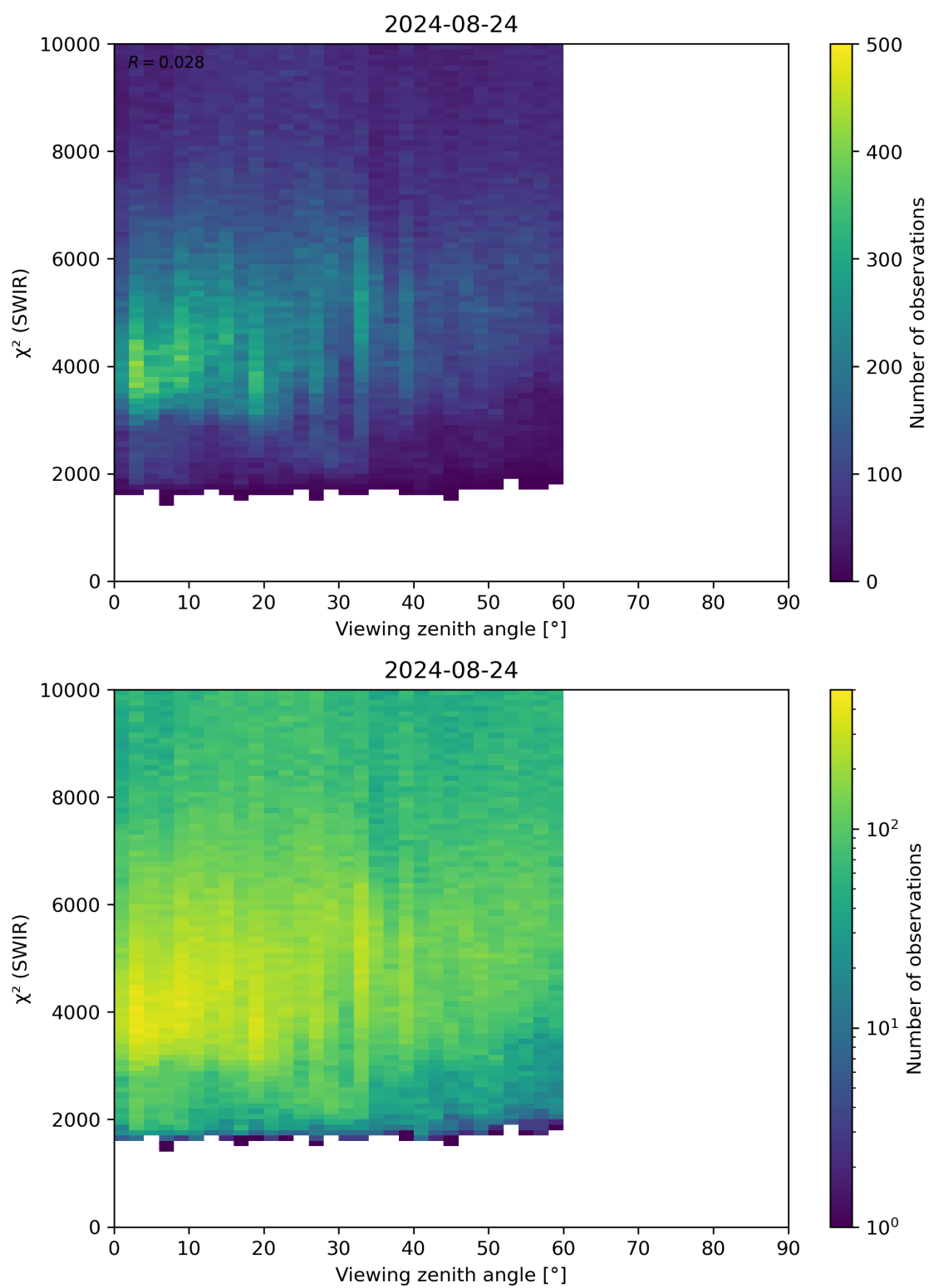
Figure 106: Scatter density plot of “Viewing zenith angle” against “ \chi^2 (SWIR)” for 2024-08-23 to 2024-08-25.
