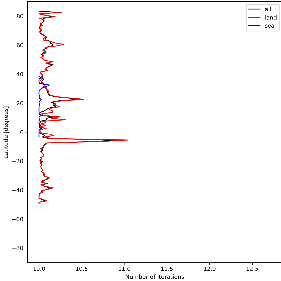
Figure 20: Zonal average of “Number of iterations” for 2024-08-23 to 2024-08-25.
