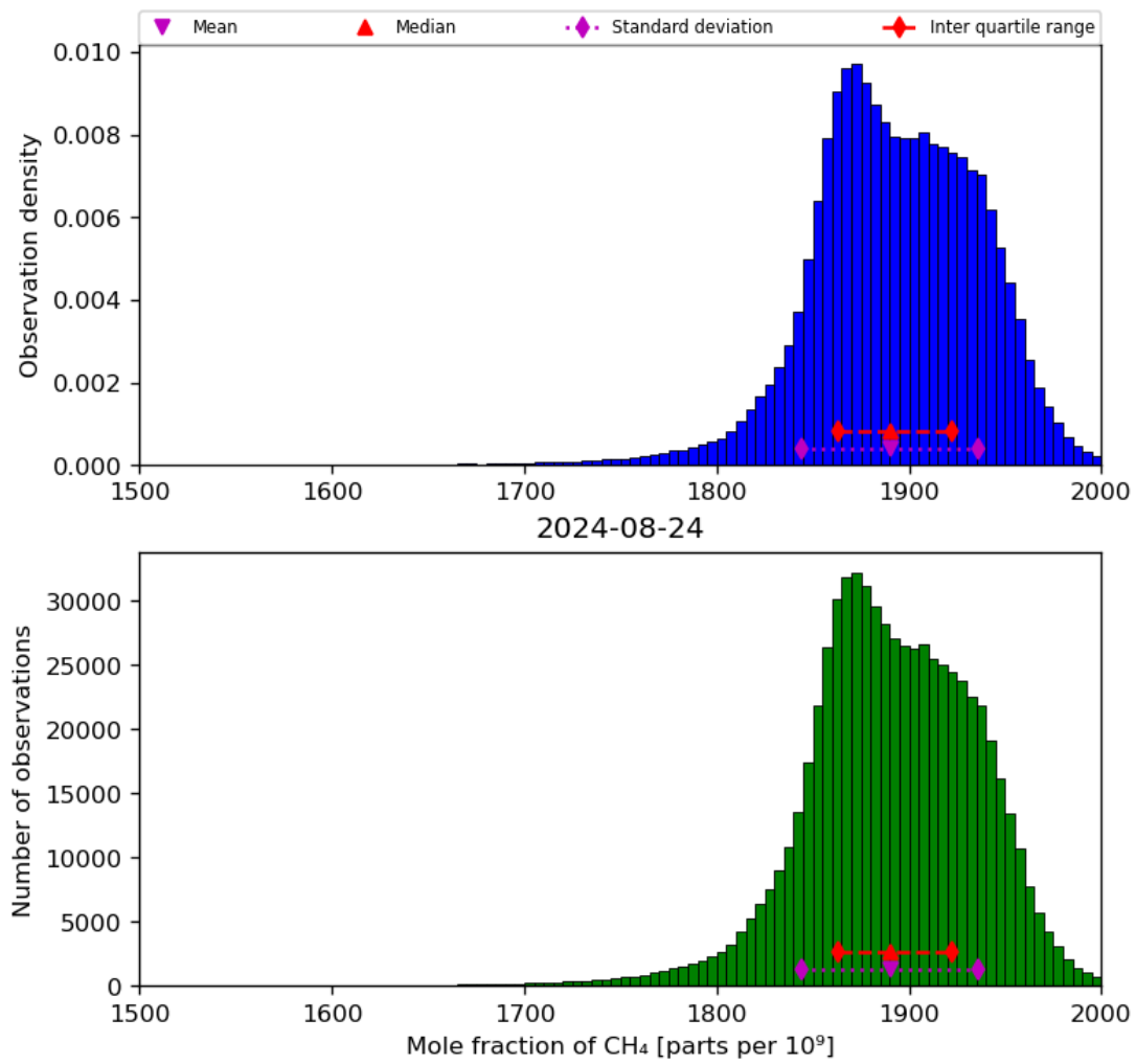
Figure 23: Histogram of “Mole fraction of CH 4 ” for 2024-08-23 to 2024-08-25
