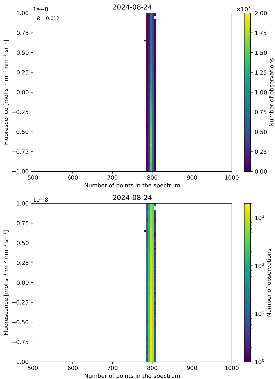
Figure 91: Scatter density plot of “Number of points in the spectrum” against “Fluorescence” for 2024-08-23 to 2024-08-25.
