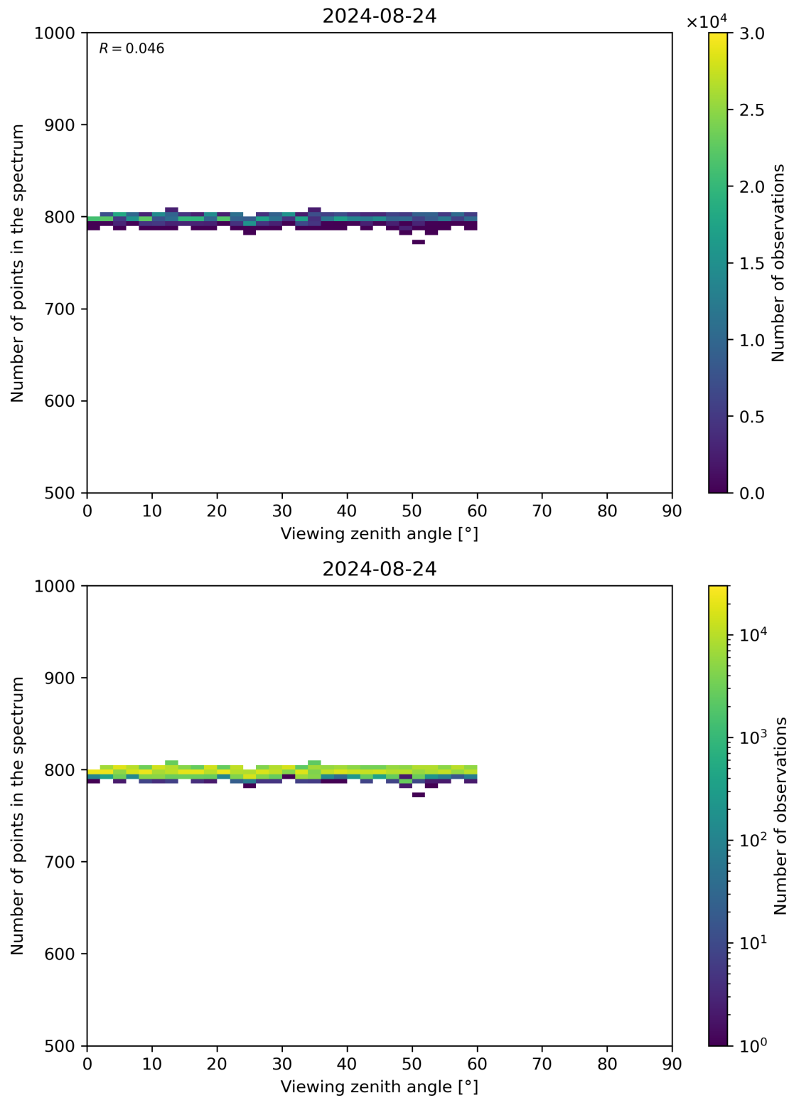
Figure 114: Scatter density plot of “Viewing zenith angle” against “Number of points in the spectrum” for 2024-08-23 to 2024-08-25.
