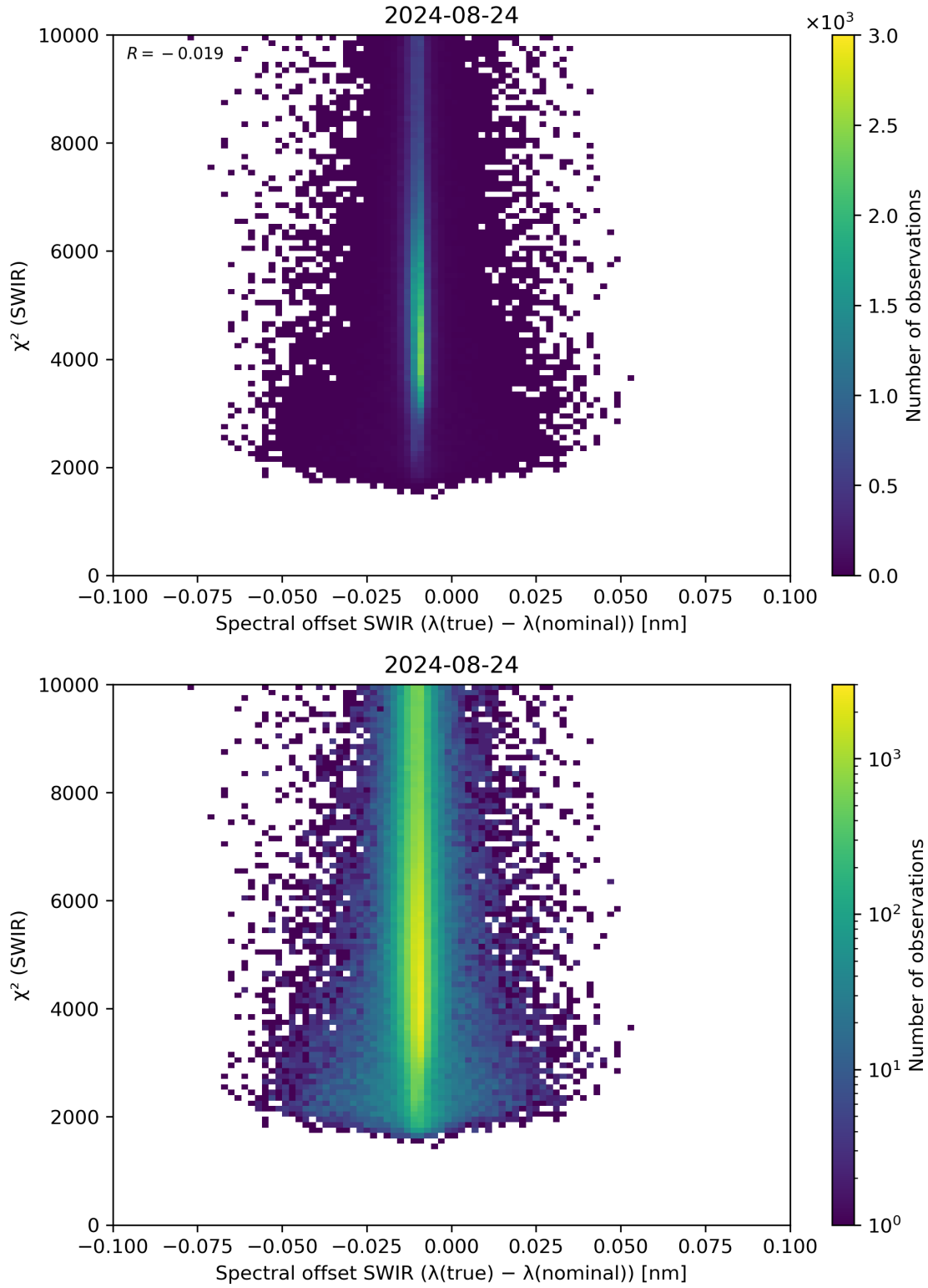
Figure 118: Scatter density plot of “Spectral offset SWIR ( \lambda(\text{true}) - \lambda(\text{nominal}) )” against “ \chi^2 (SWIR)” for 2024-08-23 to 2024-08-25.
