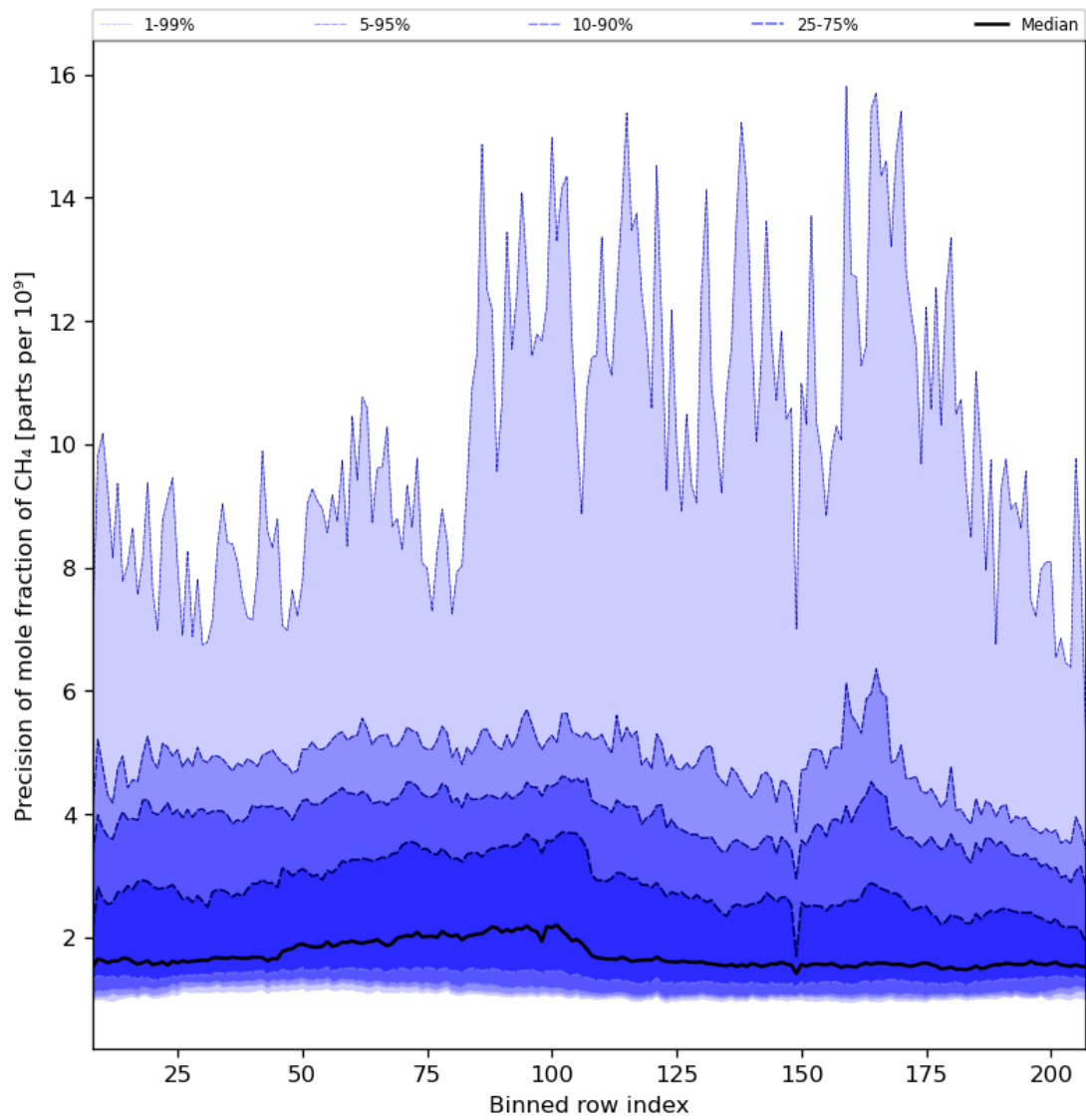
Figure 35: Along track statistics of “Precision of mole fraction of CH 4 ” for 2024-08-23 to 2024-08-25
