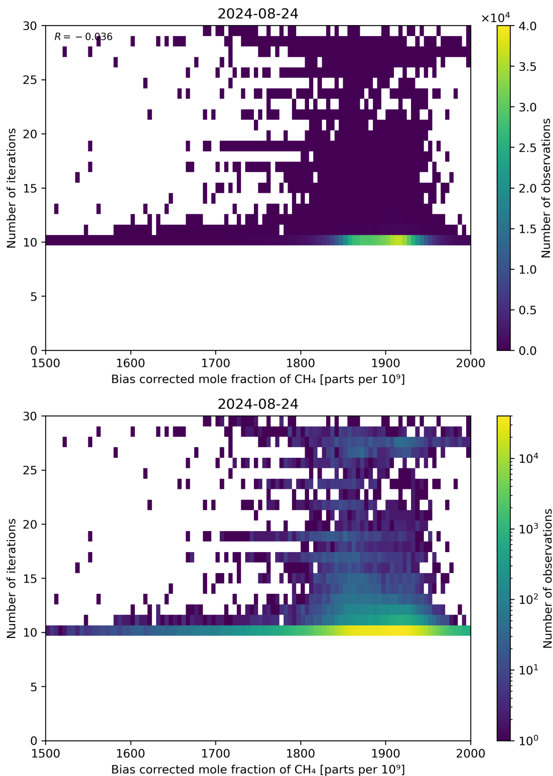
Figure 67: Scatter density plot of “Bias corrected mole fraction of \text{CH}_4 ” against “Number of iterations” for 2024-08-23 to 2024-08-25.
