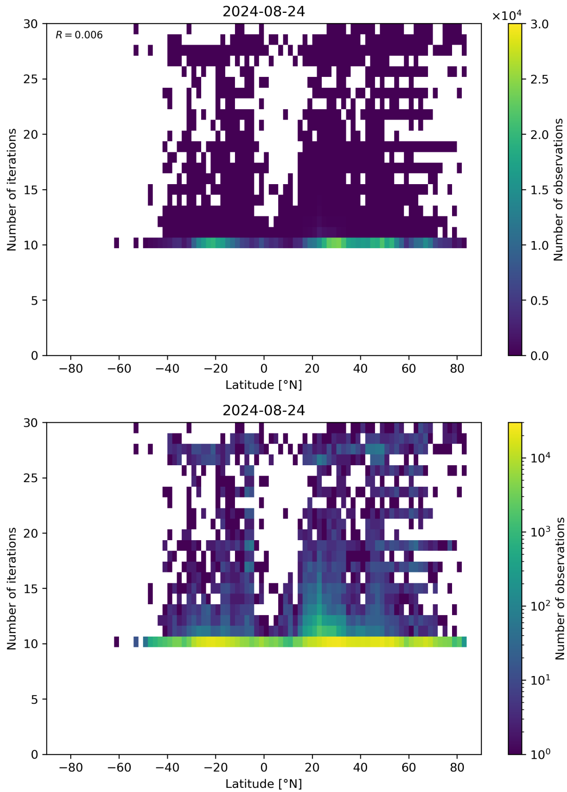
Figure 60: Scatter density plot of “Latitude” against “Number of iterations” for 2024-08-23 to 2024-08-25.
