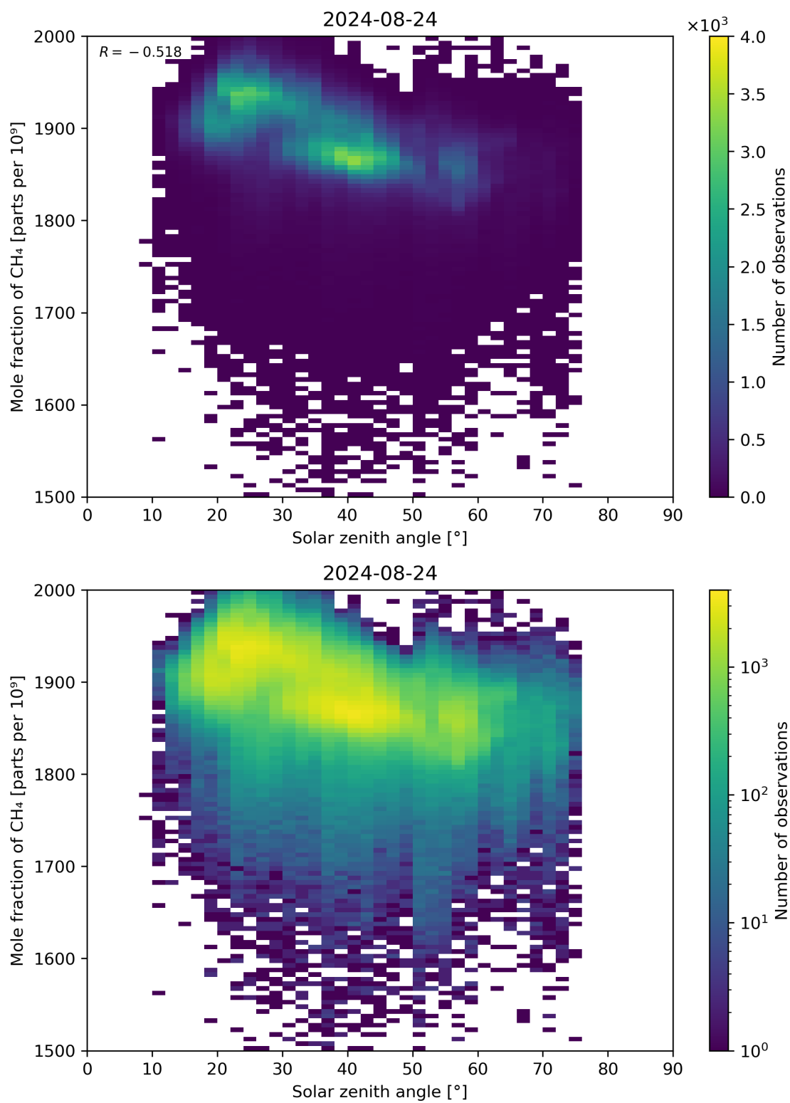
Figure 99: Scatter density plot of “Solar zenith angle” against “Mole fraction of CH 4 ” for 2024-08-23 to 2024-08-25.
