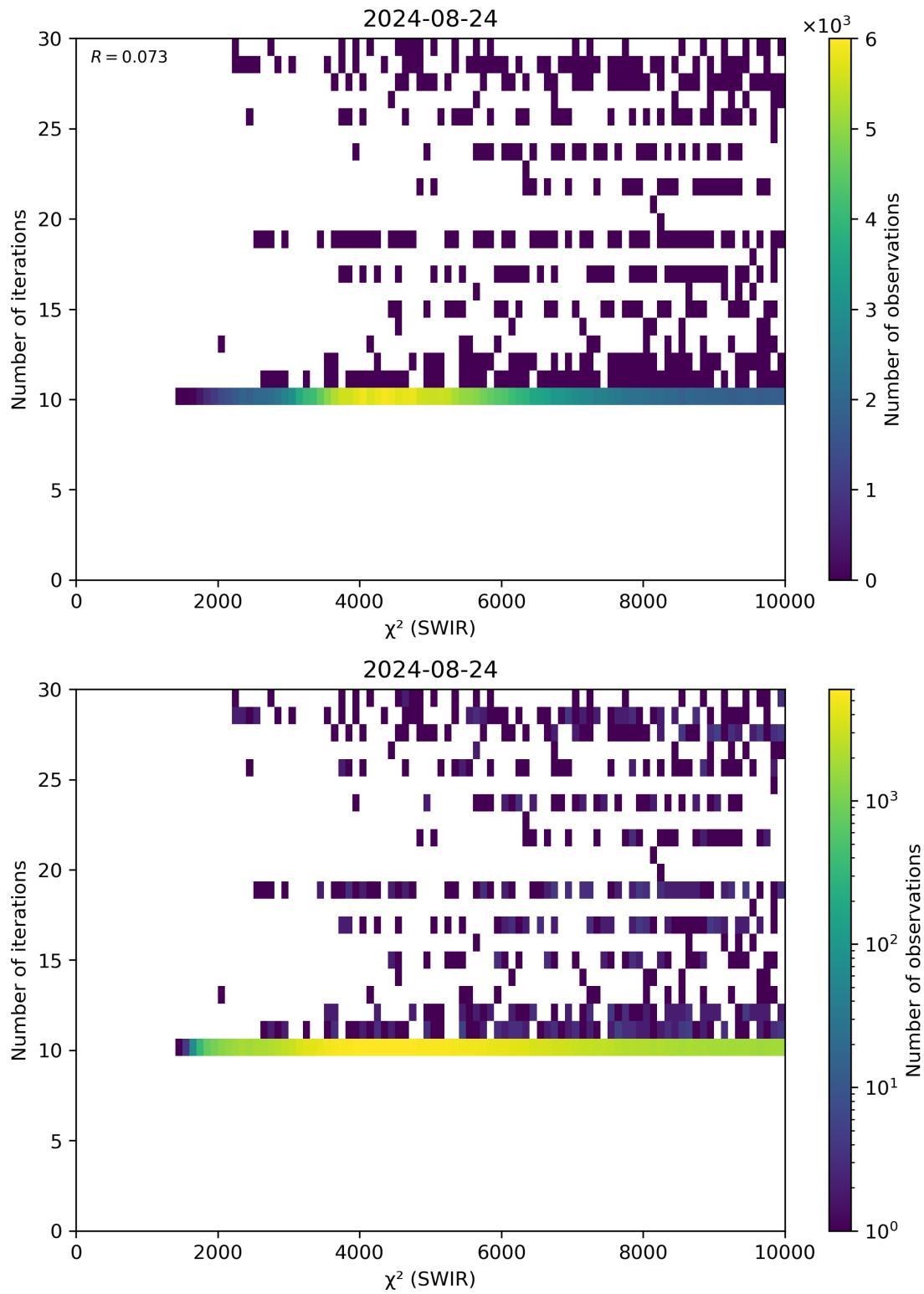
Figure 50: Scatter density plot of “ \chi^2 (SWIR)” against “Number of iterations” for 2024-08-23 to 2024-08-25.
