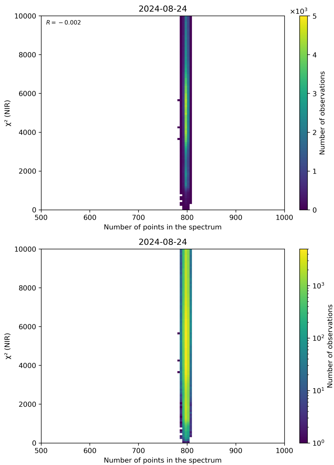
Figure 88: Scatter density plot of “Number of points in the spectrum” against “ \chi^2 (NIR)” for 2024-08-23 to 2024-08-25.
