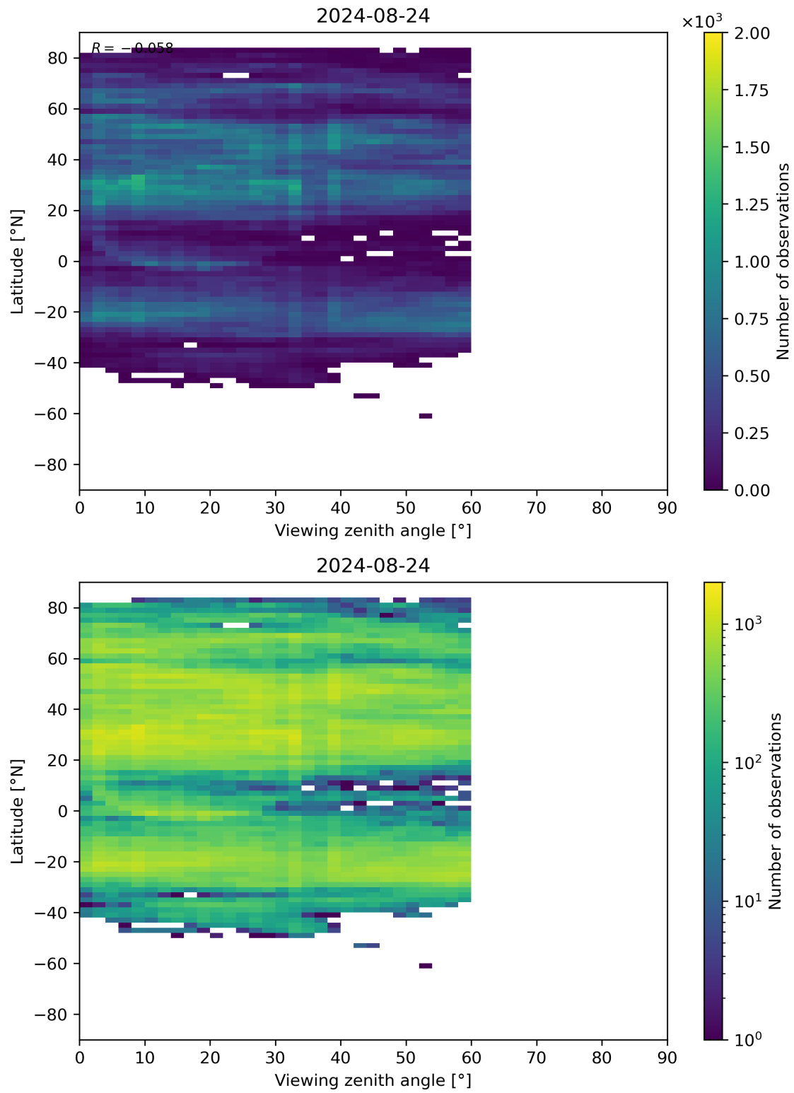
Figure 109: Scatter density plot of “Viewing zenith angle” against “Latitude” for 2024-08-23 to 2024-08-25.
