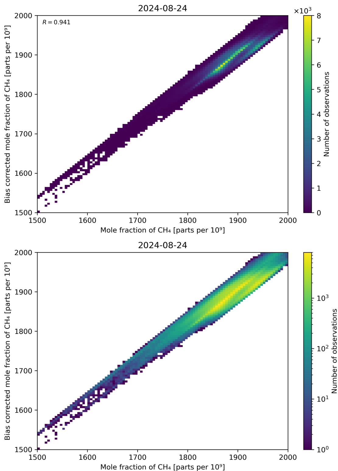
Figure 74: Scatter density plot of “Mole fraction of CH 4 ” against “Bias corrected mole fraction of CH 4 ” for 2024-08-23 to 2024-08-25.
