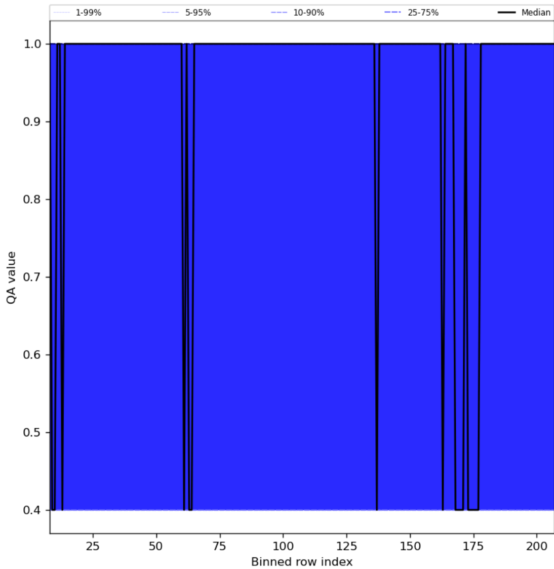
Figure 33: Along track statistics of “QA value” for 2024-08-23 to 2024-08-25
