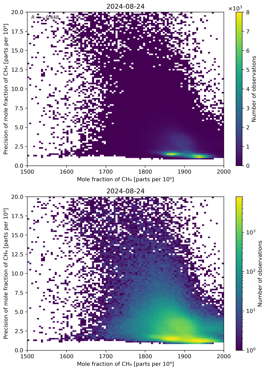
Figure 75: Scatter density plot of “Mole fraction of CH 4 ” against “Precision of mole fraction of CH 4 ” for 2024-08-23 to 2024-08-25.
