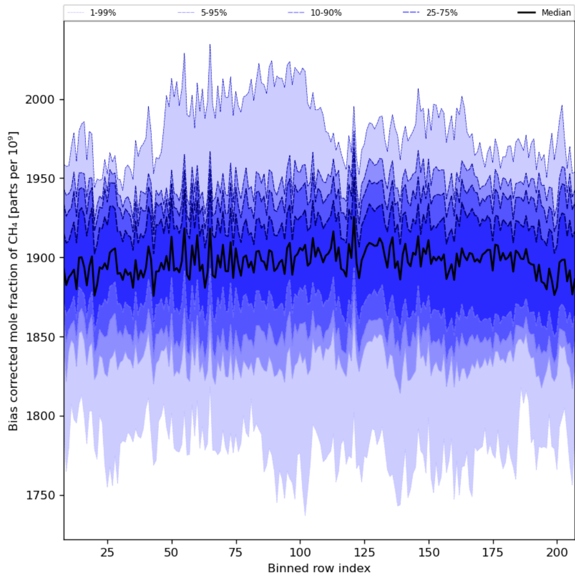
Figure 36: Along track statistics of “Bias corrected mole fraction of CH 4 ” for 2024-08-23 to 2024-08-25
