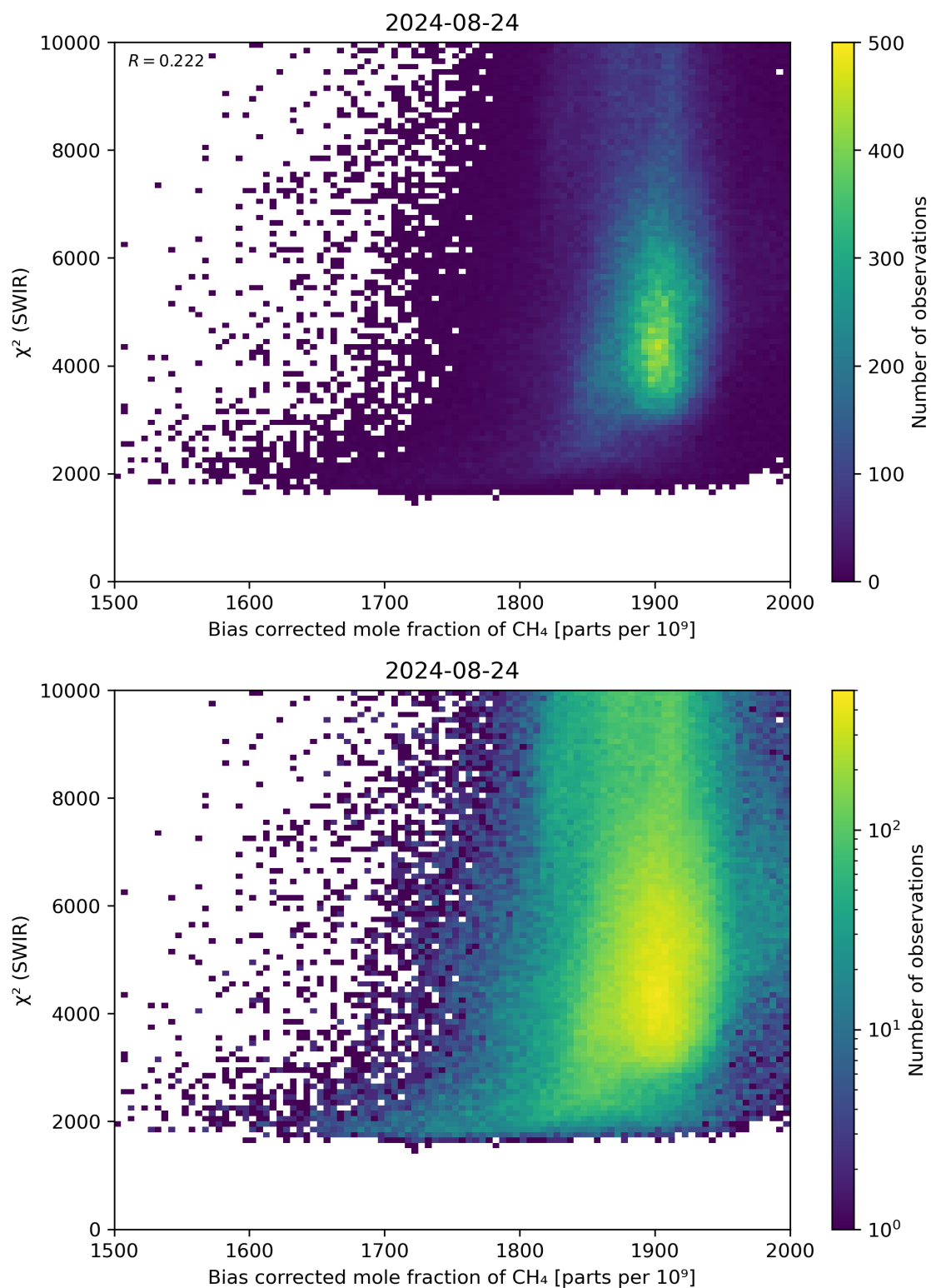
Figure 64: Scatter density plot of “Bias corrected mole fraction of CH 4 ” against “ \chi^2 (SWIR)” for 2024-08-23 to 2024-08-25.
