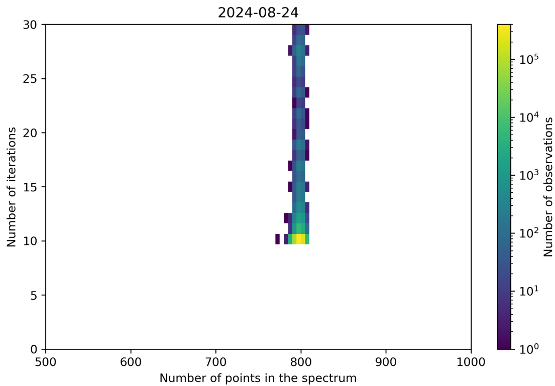
Figure 92: Scatter density plot of “Number of points in the spectrum” against “Number of iterations” for 2024-08-23 to 2024-08-25.
