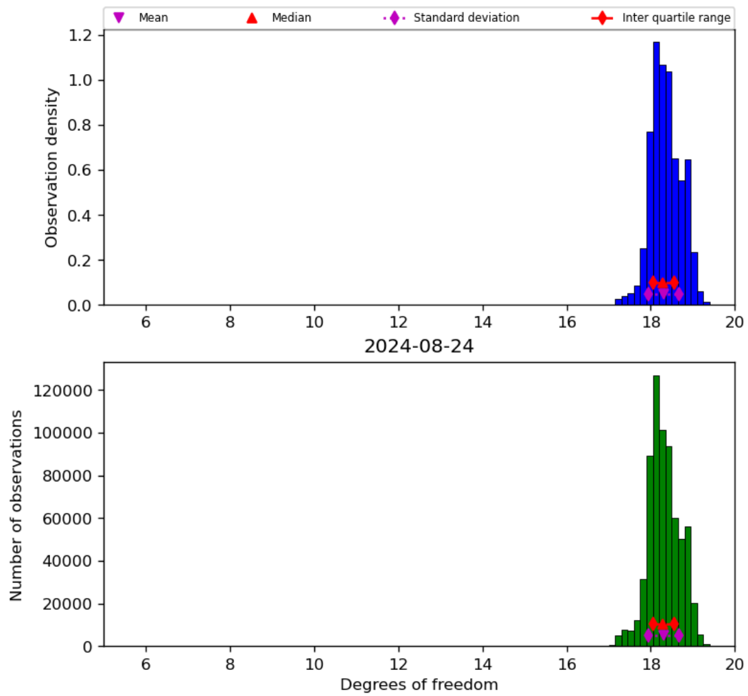
Figure 30: Histogram of “Degrees of freedom” for 2024-08-23 to 2024-08-25
