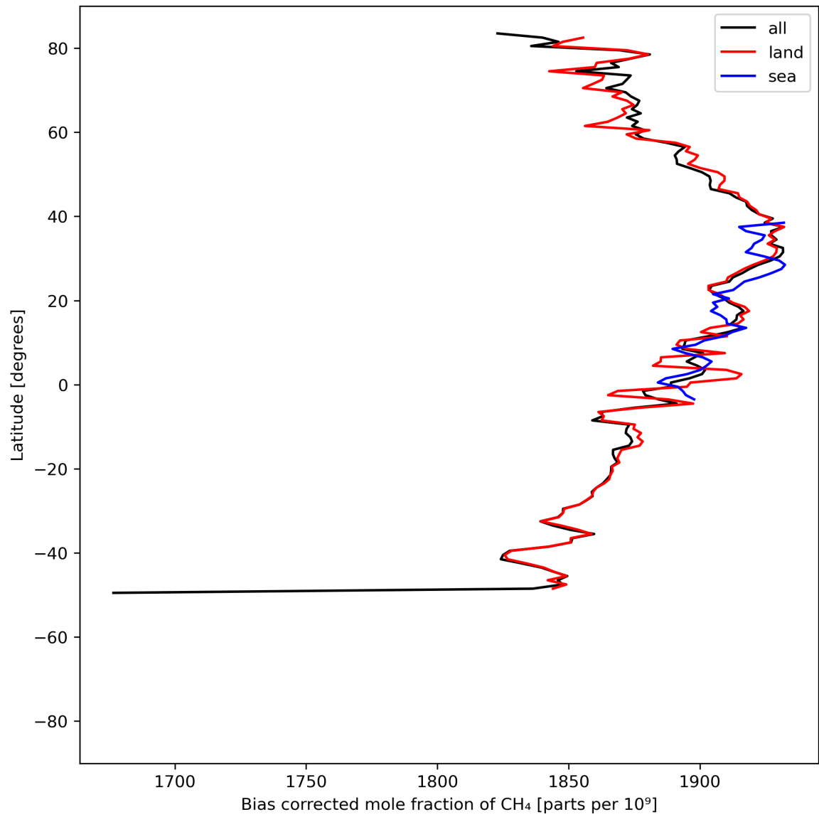
Figure 14: Zonal average of “Bias corrected mole fraction of CH 4 ” for 2024-08-23 to 2024-08-25.
