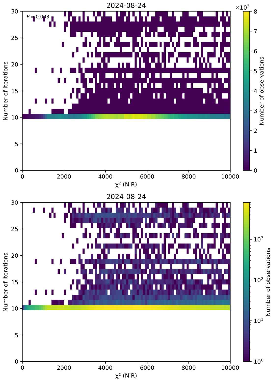
Figure 46: Scatter density plot of “ \chi^2 (NIR)” against “Number of iterations” for 2024-08-23 to 2024-08-25.
