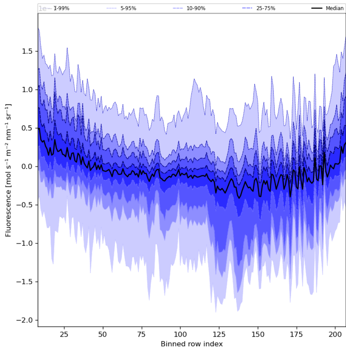
Figure 43: Along track statistics of “Fluorescence” for 2024-08-23 to 2024-08-25
