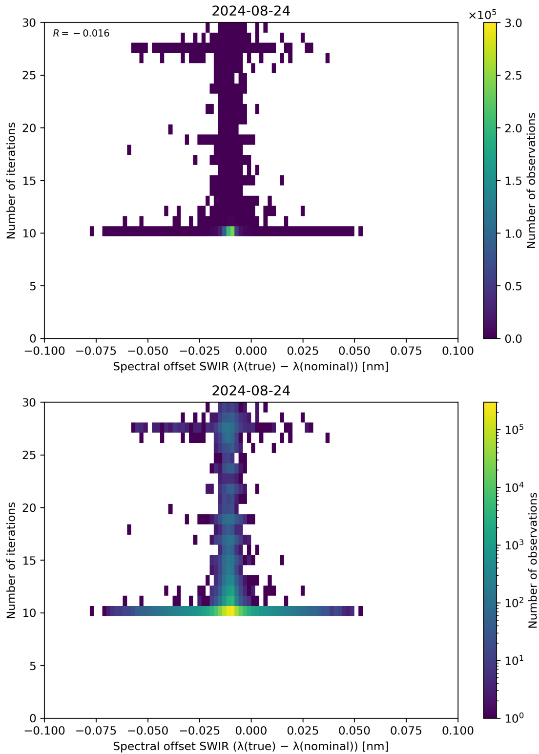
Figure 121: Scatter density plot of “Spectral offset SWIR ( \lambda(\text{true}) - \lambda(\text{nominal}) )” against “Number of iterations” for 2024-08-23 to 2024-08-25.
