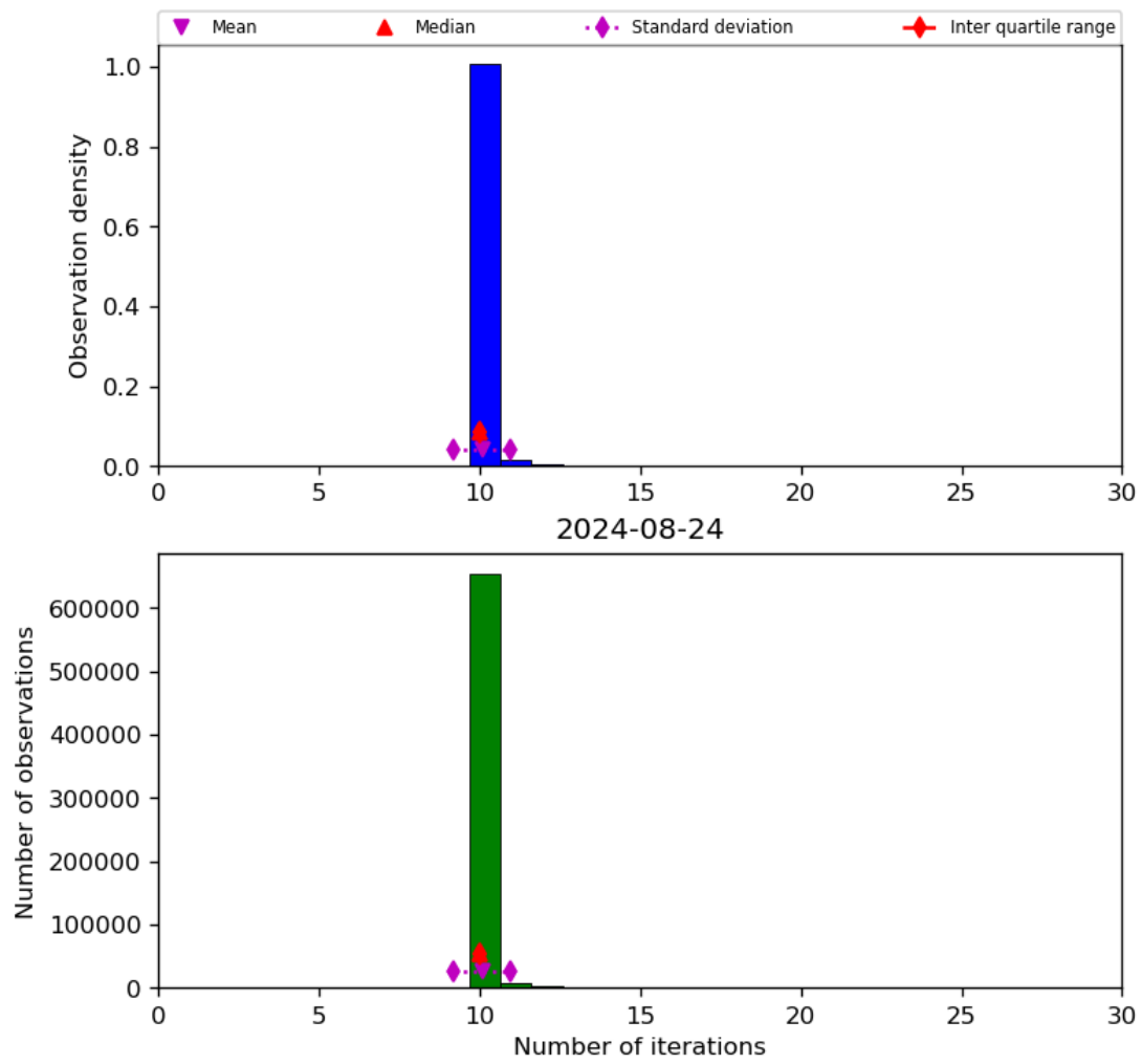
Figure 31: Histogram of “Number of iterations” for 2024-08-23 to 2024-08-25
