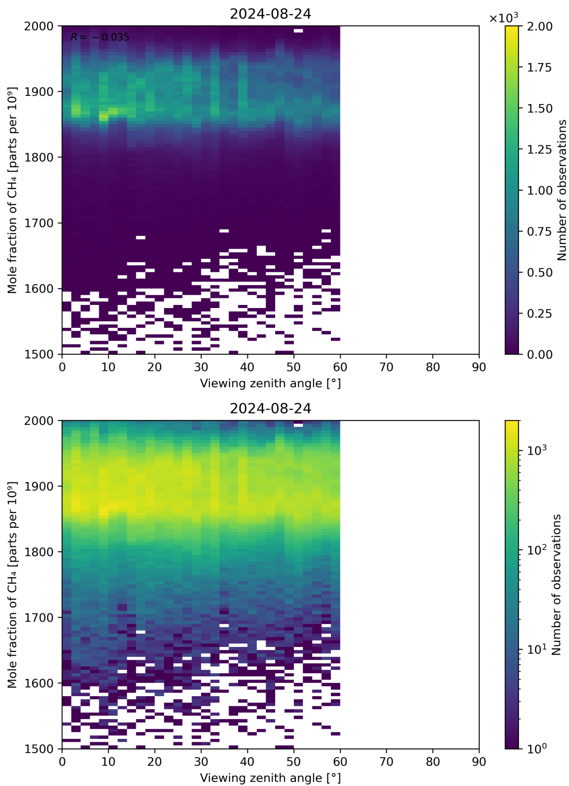
Figure 110: Scatter density plot of “Viewing zenith angle” against “Mole fraction of \text{CH}_4 ” for 2024-08-23 to 2024-08-25.
