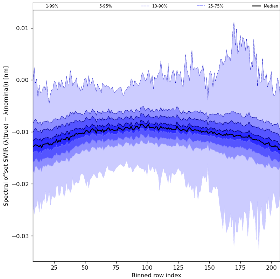
Figure 38: Along track statistics of “Spectral offset SWIR ( \lambda(\text{true}) - \lambda(\text{nominal}) )” for 2024-08-23 to 2024-08-25
