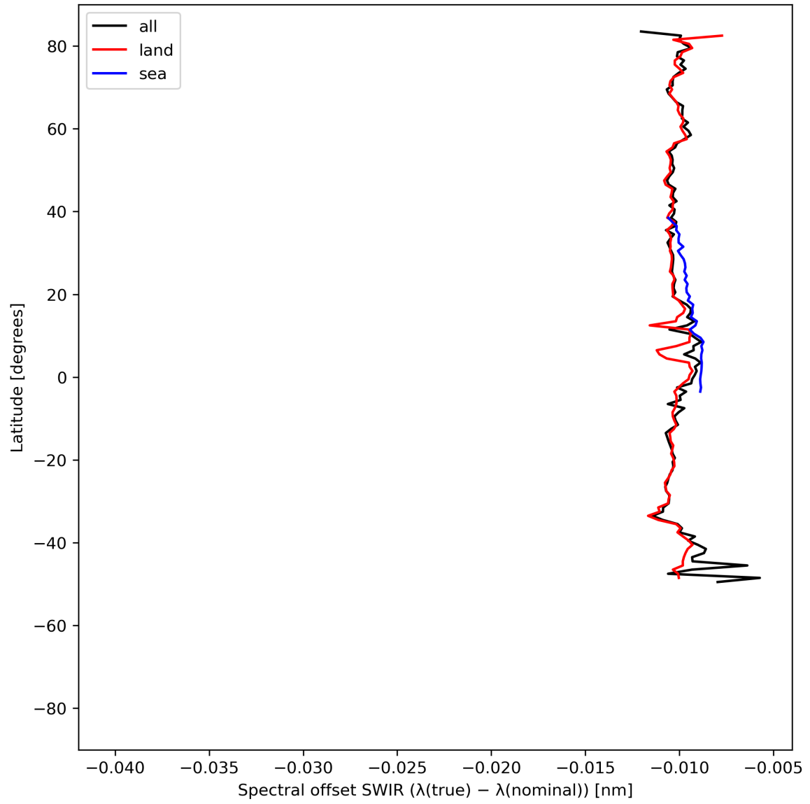
Figure 16: Zonal average of “Spectral offset SWIR ( \lambda(\text{true}) - \lambda(\text{nominal}) )” for 2024-08-23 to 2024-08-25.
