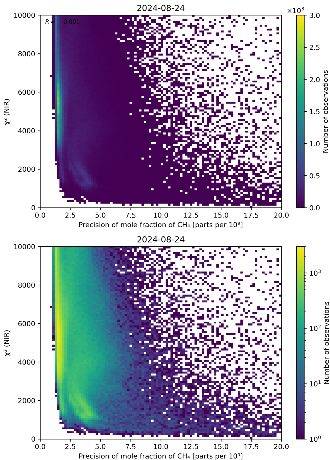
Figure 78: Scatter density plot of “Precision of mole fraction of \text{CH}_4 ” against “ \chi^2 (NIR)” for 2024-08-23 to 2024-08-25.
