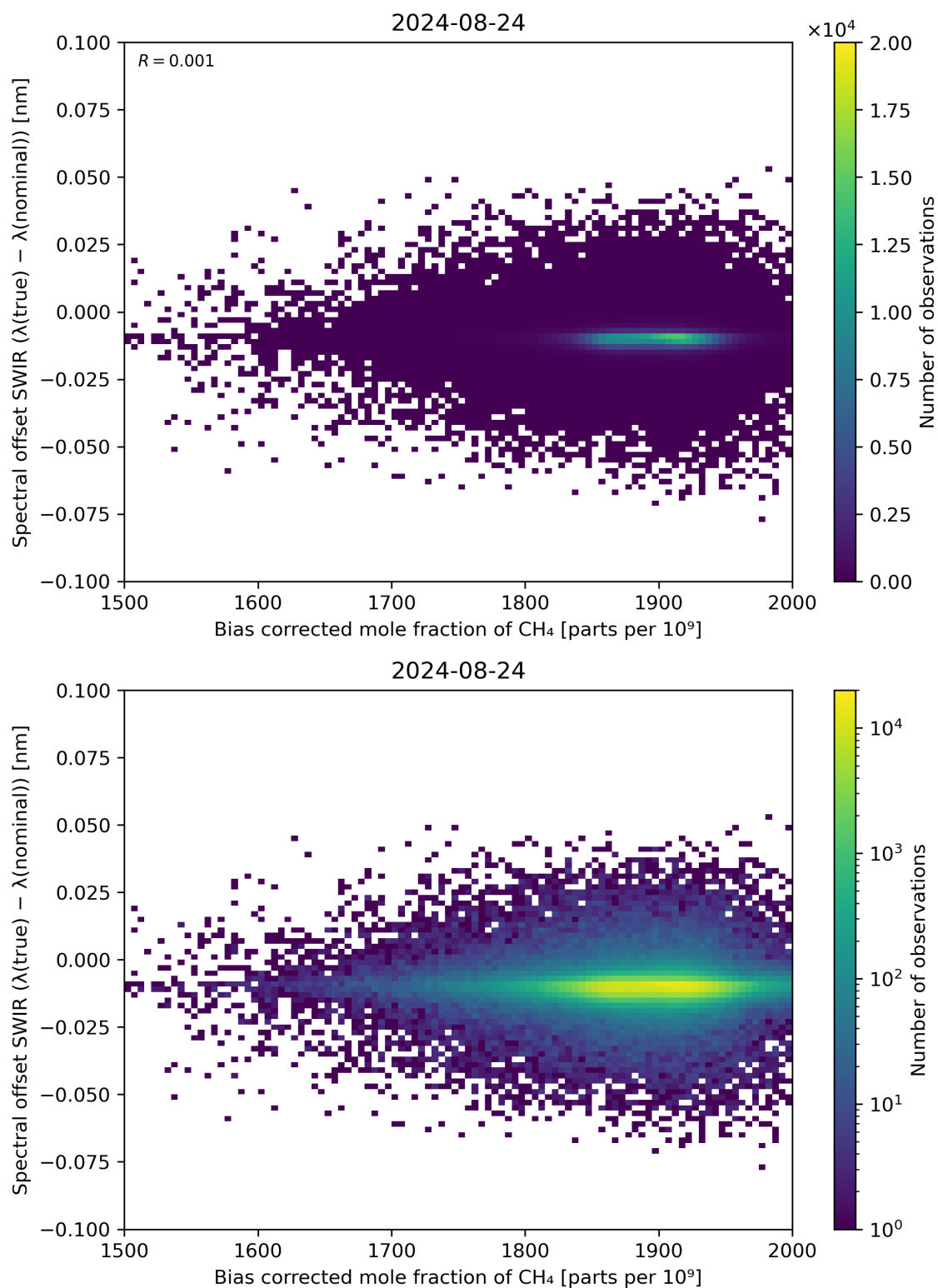
Figure 69: Scatter density plot of “Bias corrected mole fraction of \text{CH}_4 ” against “Spectral offset SWIR ( \lambda(\text{true}) - \lambda(\text{nominal}) )” for 2024-08-23 to 2024-08-25.
