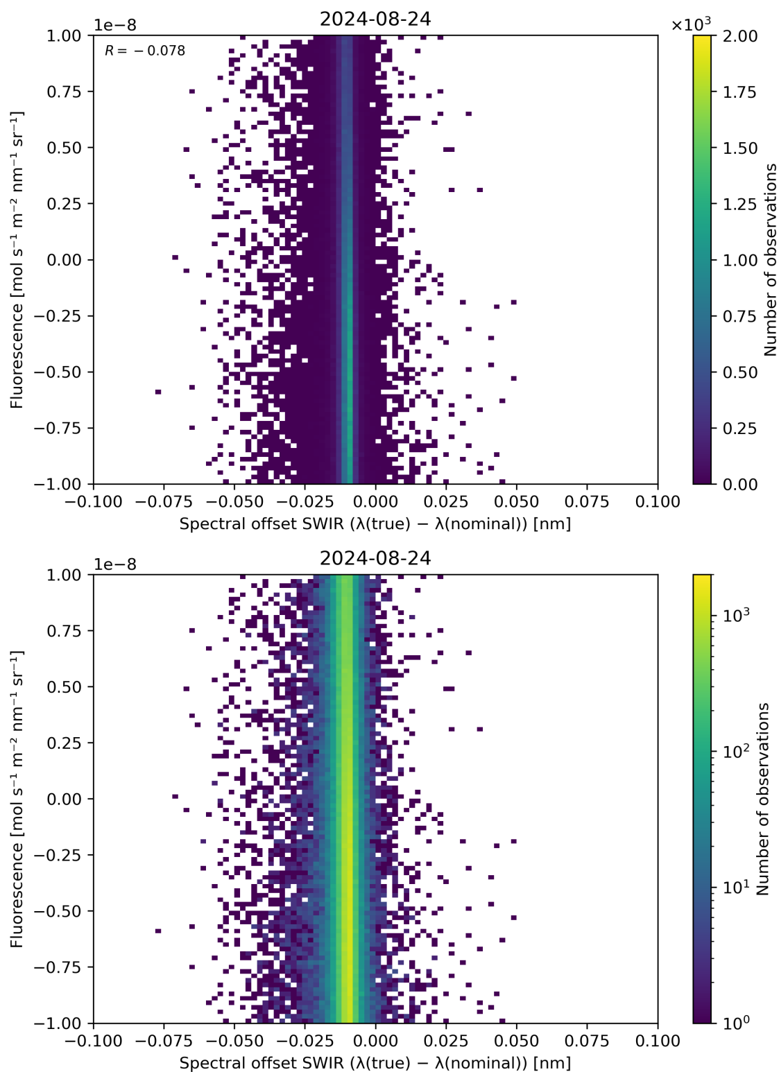
Figure 120: Scatter density plot of “Spectral offset SWIR ( \lambda(\text{true}) - \lambda(\text{nominal}) )” against “Fluorescence” for 2024-08-23 to 2024-08-25.
