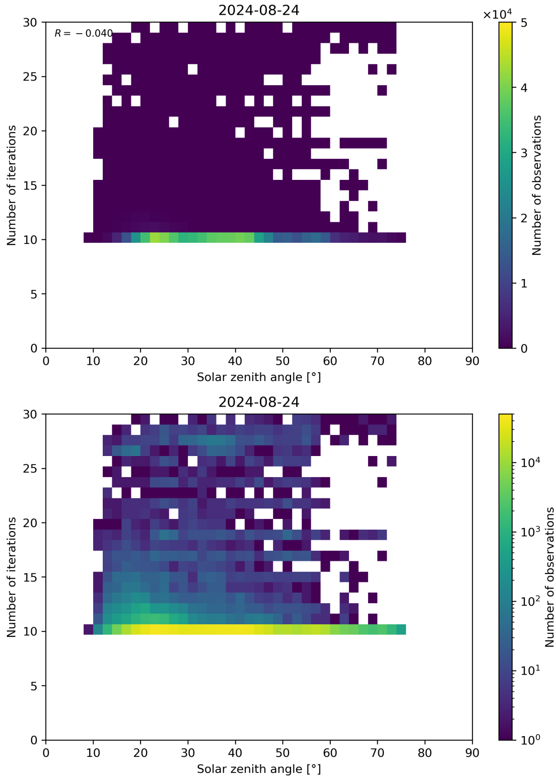
Figure 102: Scatter density plot of “Solar zenith angle” against “Number of iterations” for 2024-08-23 to 2024-08-25.
