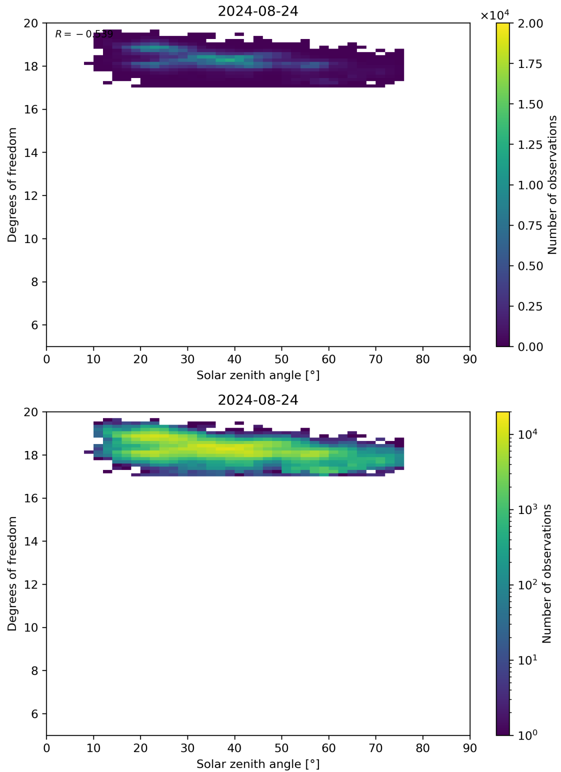
Figure 96: Scatter density plot of “Solar zenith angle” against “Degrees of freedom” for 2024-08-23 to 2024-08-25.
