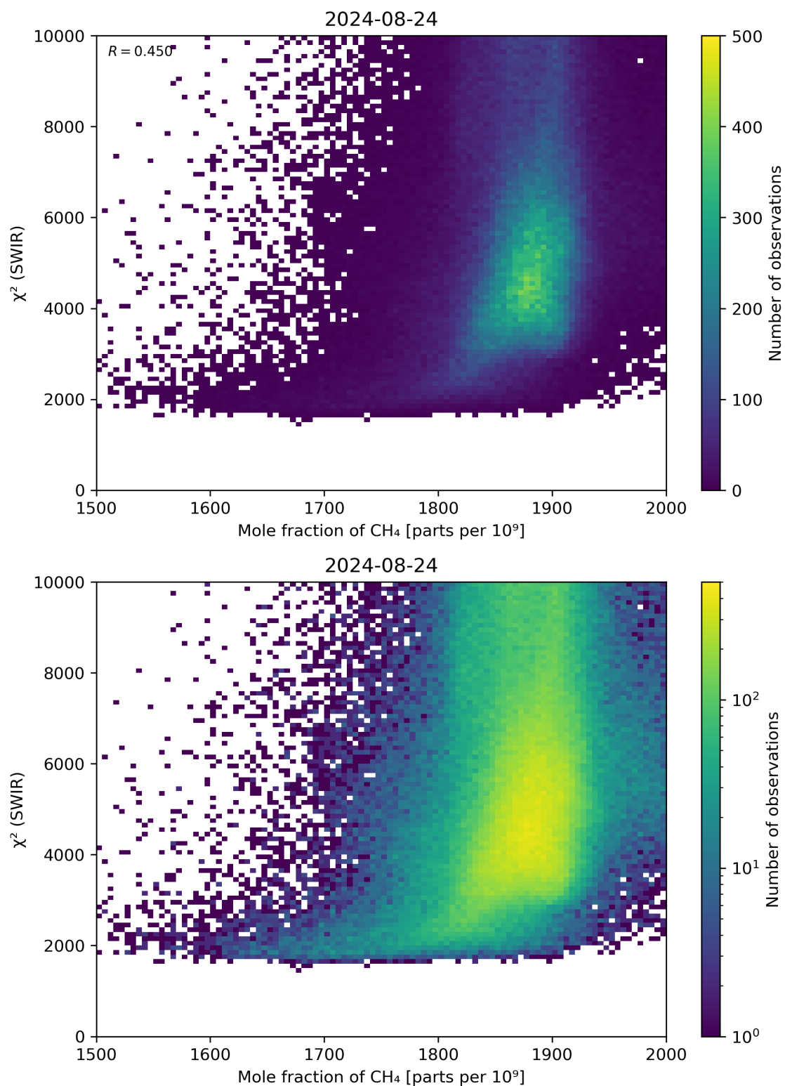
Figure 71: Scatter density plot of “Mole fraction of \text{CH}_4 ” against “ \chi^2 (SWIR)” for 2024-08-23 to 2024-08-25.
