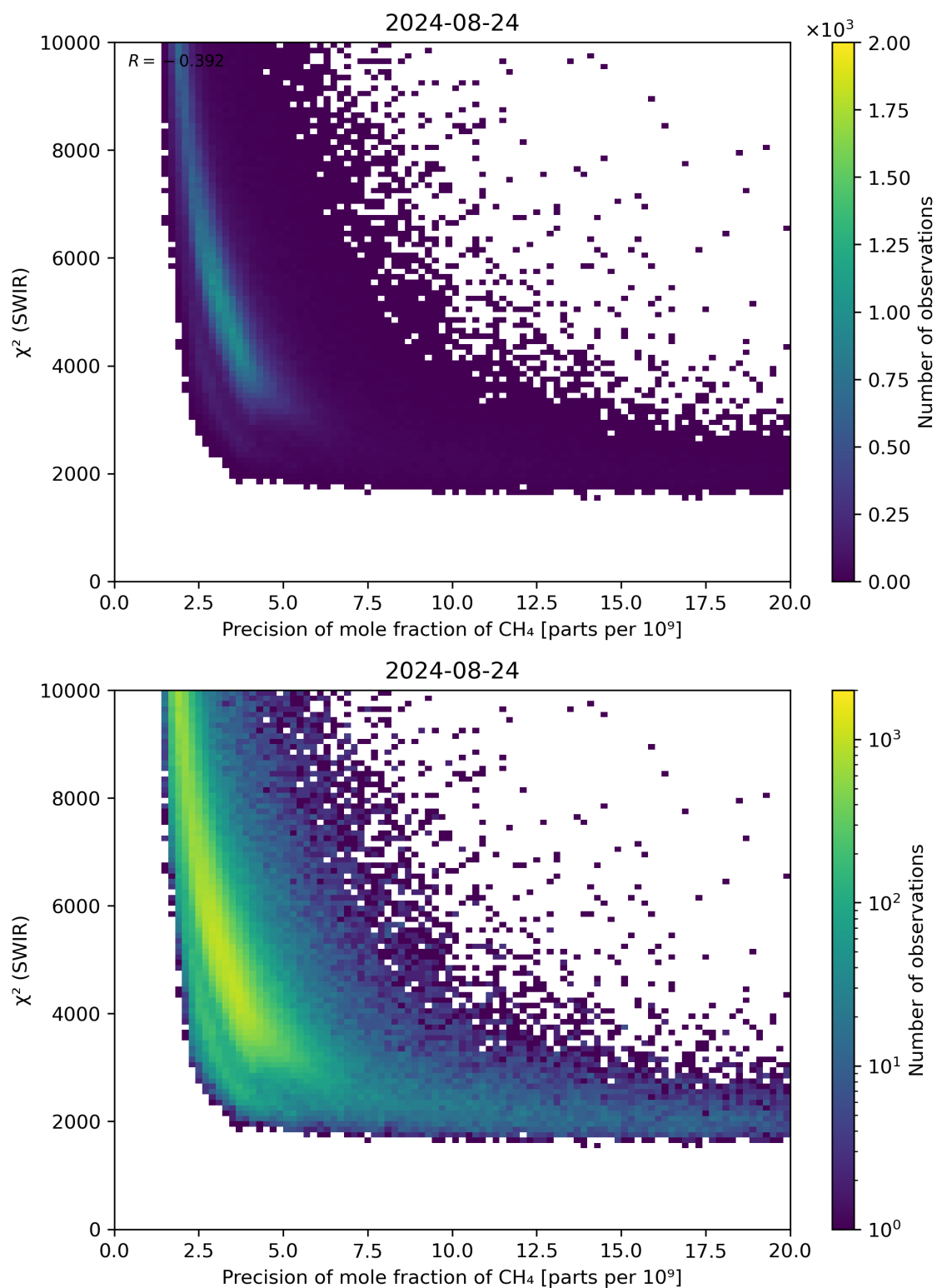
Figure 79: Scatter density plot of “Precision of mole fraction of CH 4 ” against “ \chi^2 (SWIR)” for 2024-08-23 to 2024-08-25.
