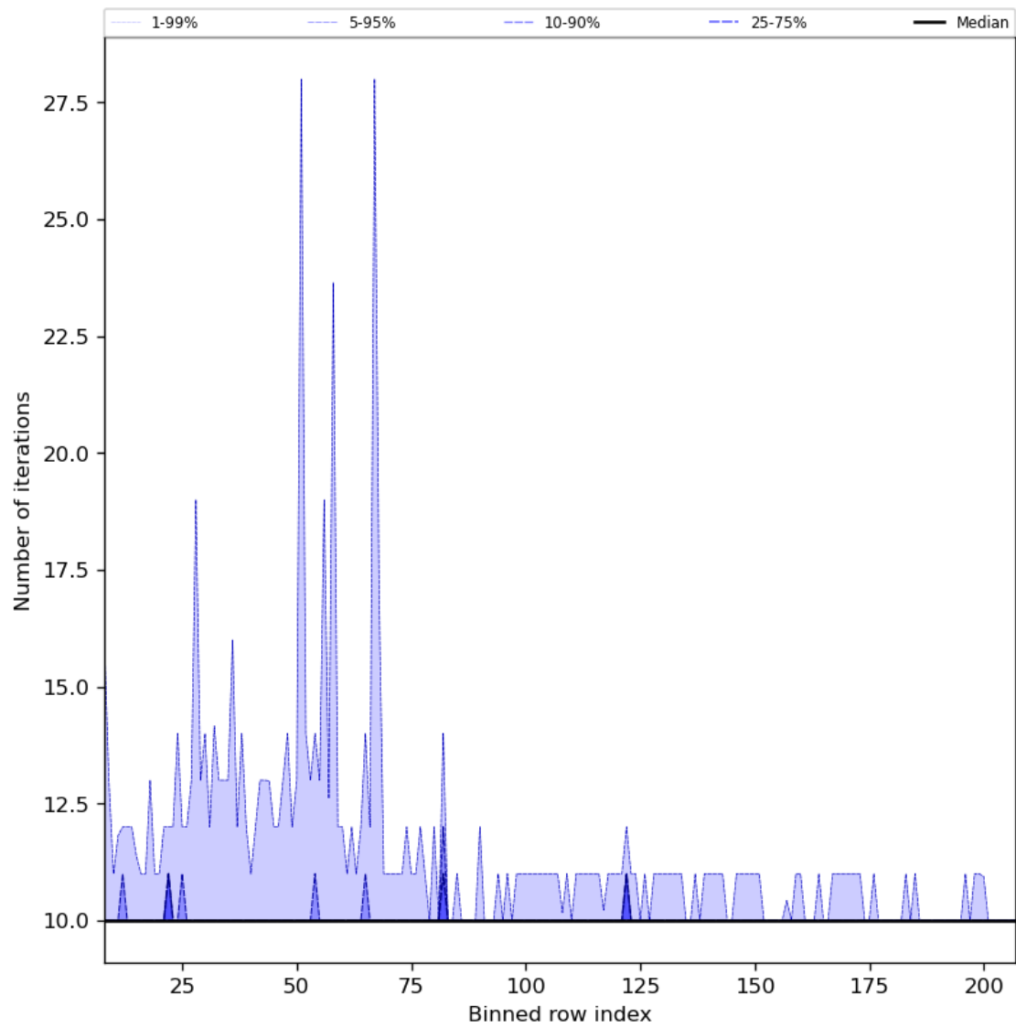
Figure 42: Along track statistics of “Number of iterations” for 2024-08-24 to 2024-08-26
