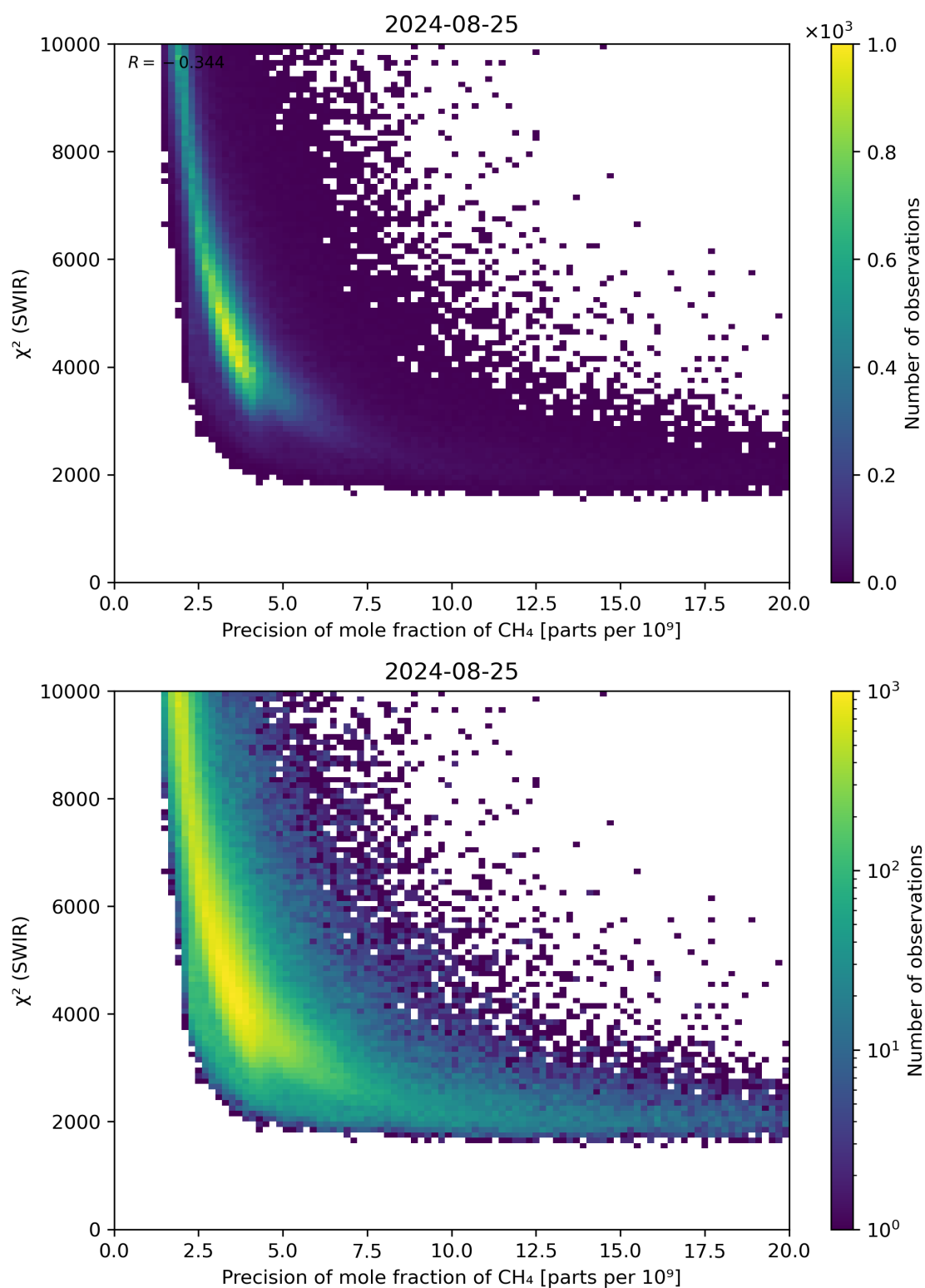
Figure 79: Scatter density plot of “Precision of mole fraction of \text{CH}_4 ” against “ \chi^2 (SWIR)” for 2024-08-24 to 2024-08-26.
