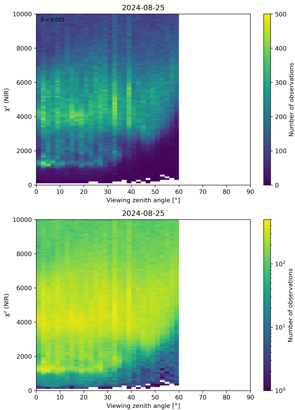
Figure 105: Scatter density plot of “Viewing zenith angle” against “ \chi^2 (NIR)” for 2024-08-24 to 2024-08-26.
