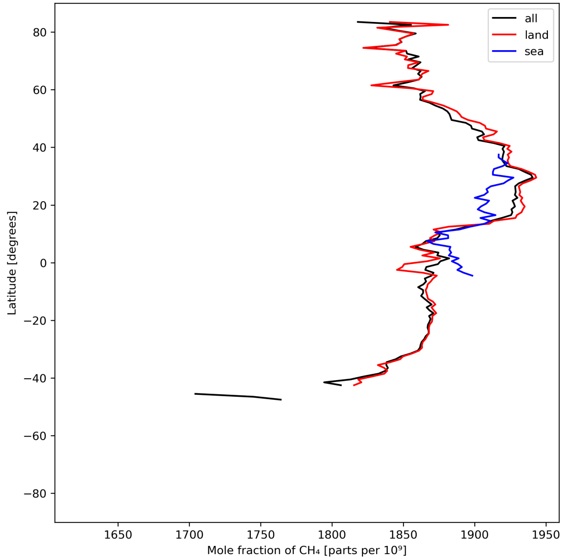
Figure 12: Zonal average of “Mole fraction of CH 4 ” for 2024-08-24 to 2024-08-26.
