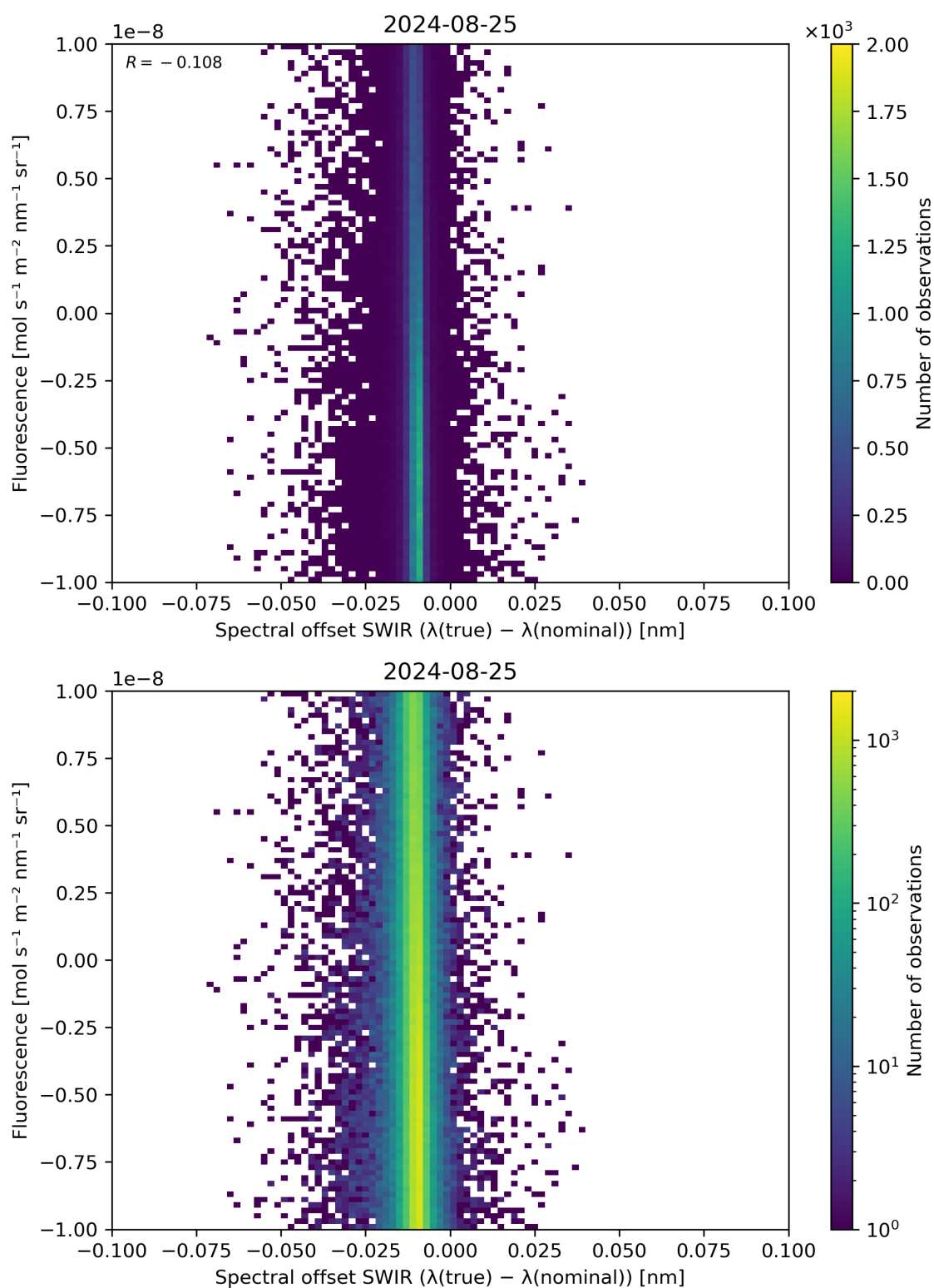
Figure 120: Scatter density plot of “Spectral offset SWIR ( \lambda(\text{true}) - \lambda(\text{nominal}) )” against “Fluorescence” for 2024-08-24 to 2024-08-26.
