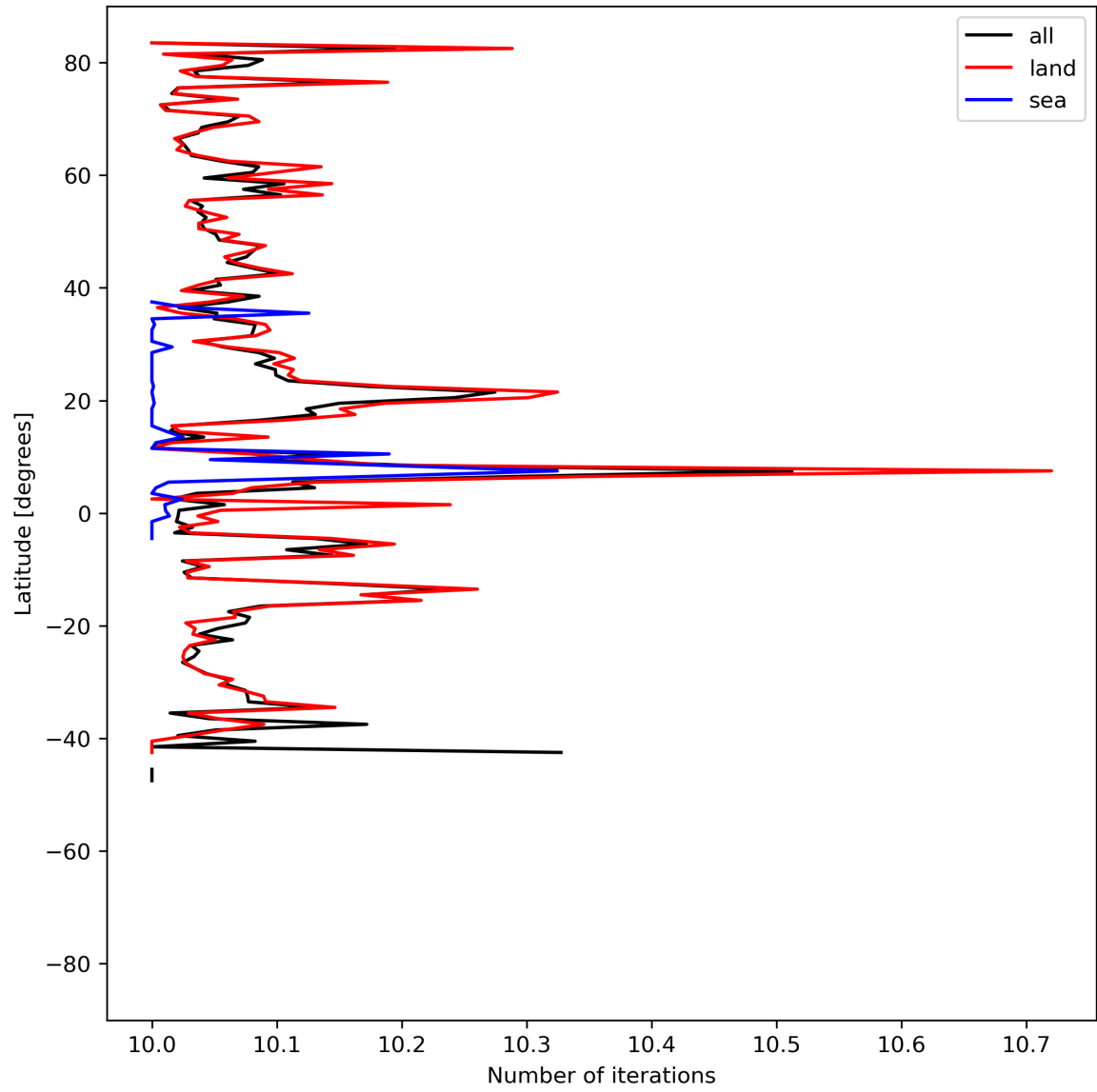
Figure 20: Zonal average of “Number of iterations” for 2024-08-24 to 2024-08-26.
