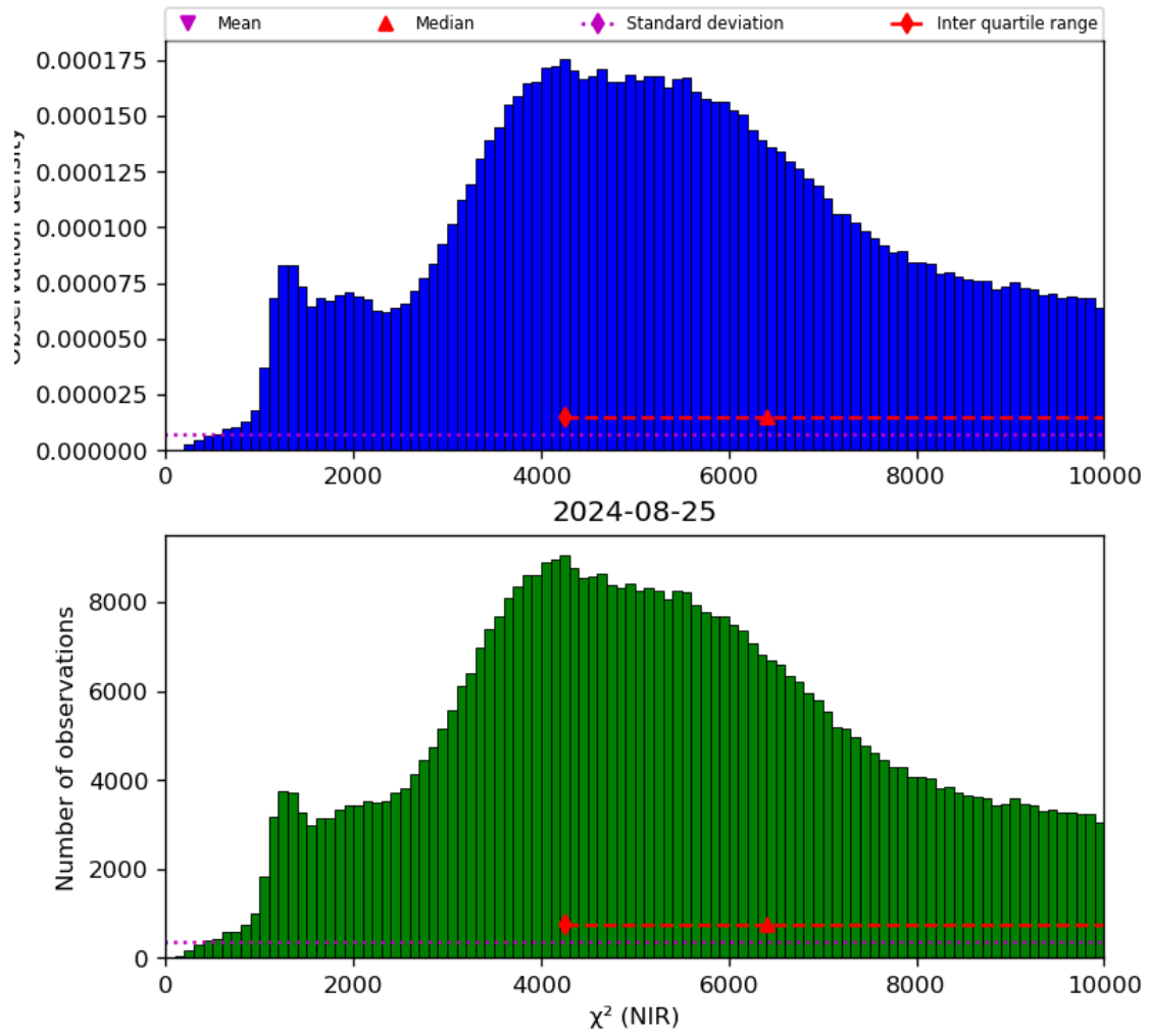
Figure 29: Histogram of “ \chi^2 (NIR)” for 2024-08-24 to 2024-08-26
