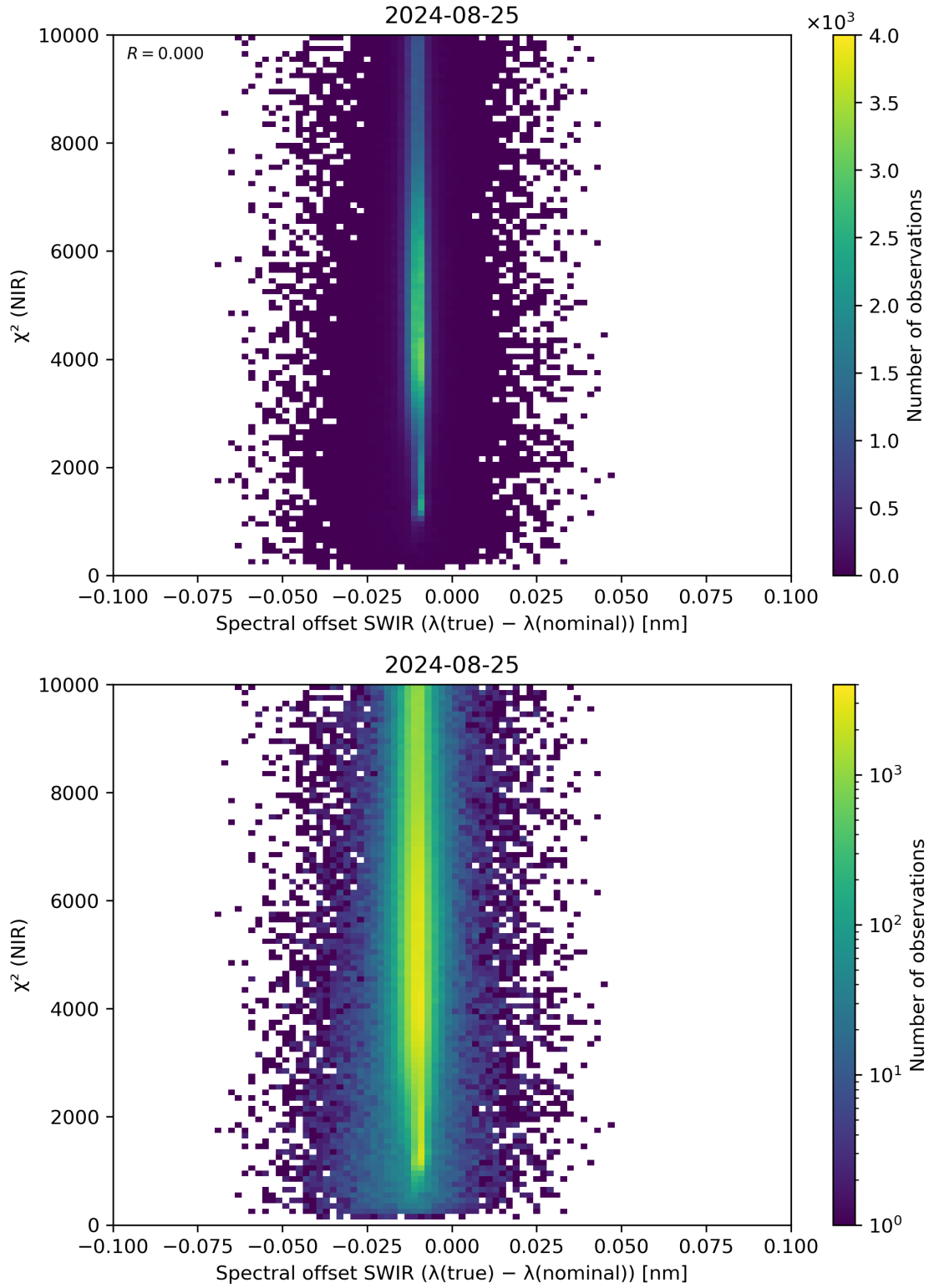
Figure 117: Scatter density plot of “Spectral offset SWIR ( \lambda(\text{true}) - \lambda(\text{nominal}) )” against “ \chi^2 (NIR)” for 2024-08-24 to 2024-08-26.
