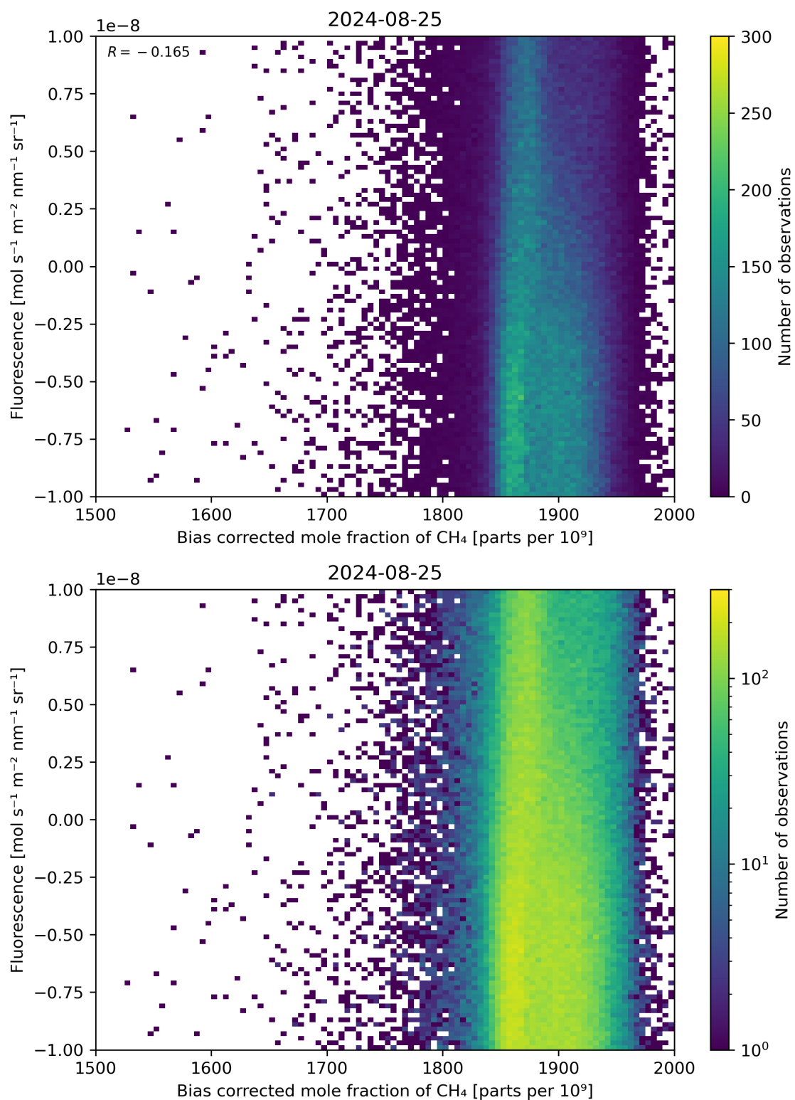
Figure 66: Scatter density plot of “Bias corrected mole fraction of \text{CH}_4 ” against “Fluorescence” for 2024-08-24 to 2024-08-26.
