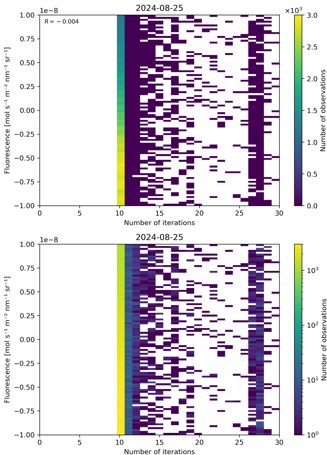
Figure 87: Scatter density plot of “Number of iterations” against “Fluorescence” for 2024-08-24 to 2024-08-26.
