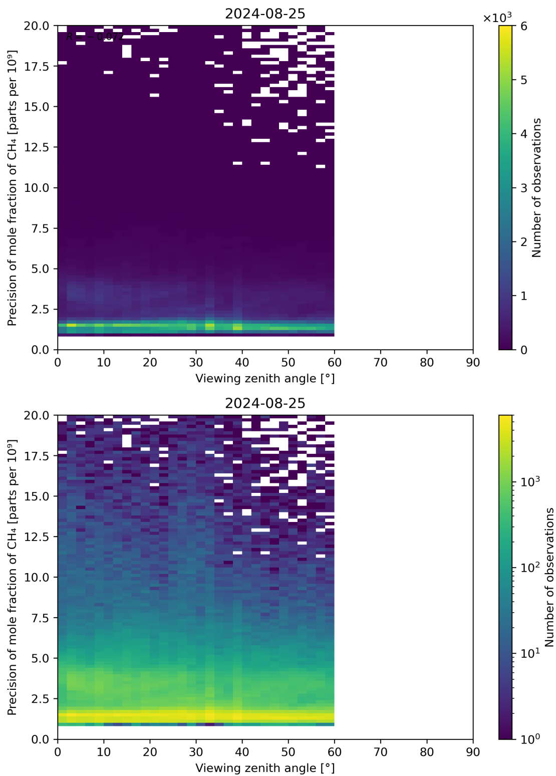
Figure 112: Scatter density plot of “Viewing zenith angle” against “Precision of mole fraction of CH 4 ” for 2024-08-24 to 2024-08-26.
