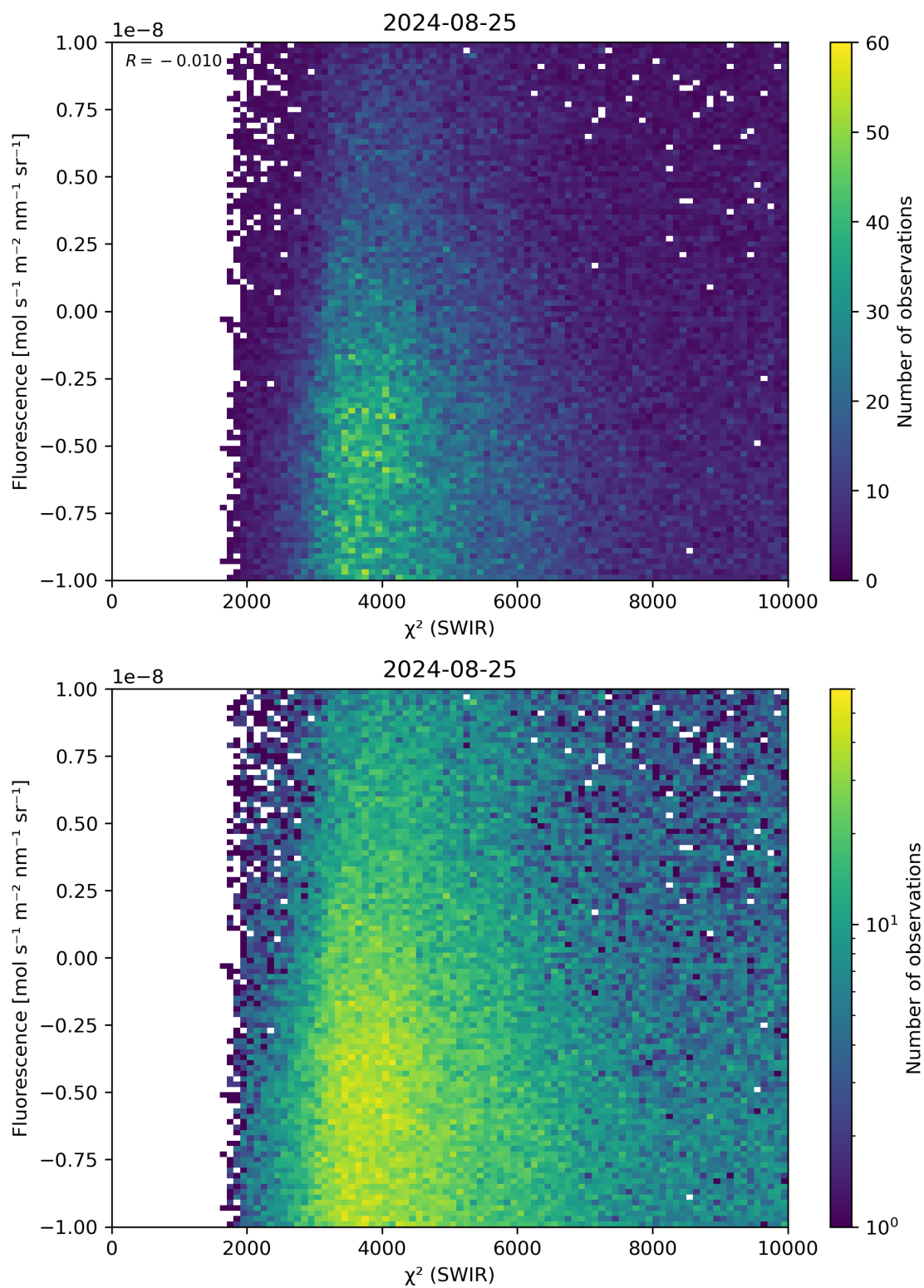
Figure 49: Scatter density plot of “ \chi^2 (SWIR)” against “Fluorescence” for 2024-08-24 to 2024-08-26.
