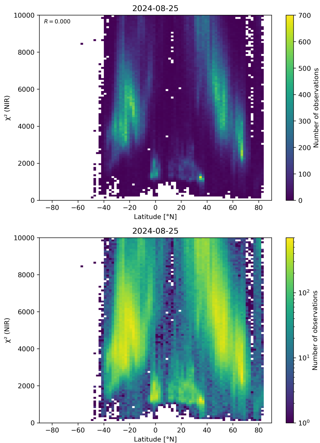
Figure 53: Scatter density plot of “Latitude” against “ \chi^2 (NIR)” for 2024-08-24 to 2024-08-26.
