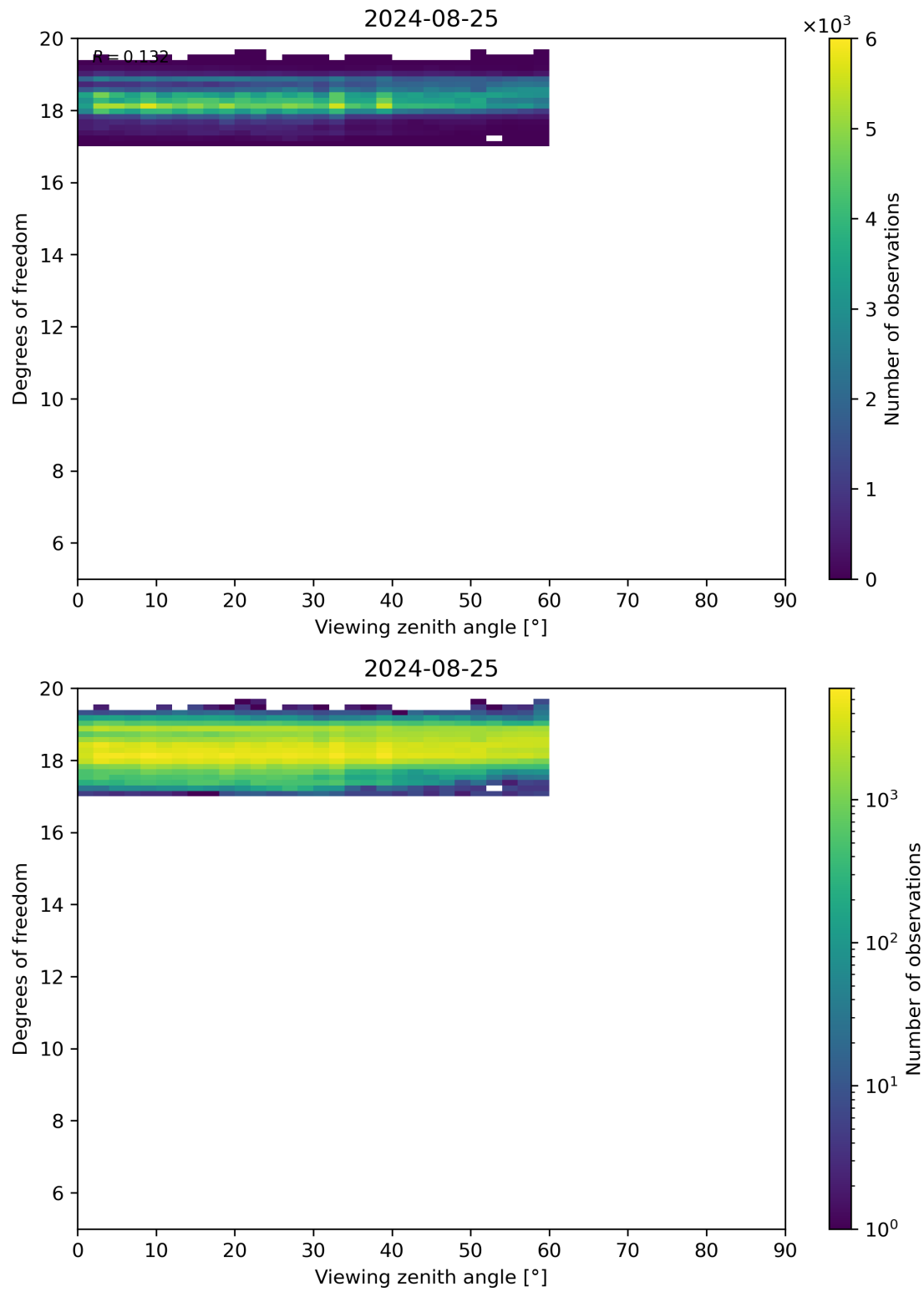
Figure 107: Scatter density plot of “Viewing zenith angle” against “Degrees of freedom” for 2024-08-24 to 2024-08-26.
