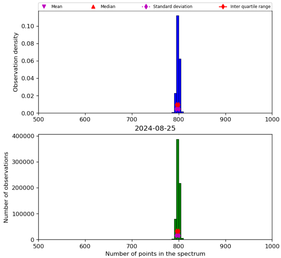
Figure 26: Histogram of “Number of points in the spectrum” for 2024-08-24 to 2024-08-26
