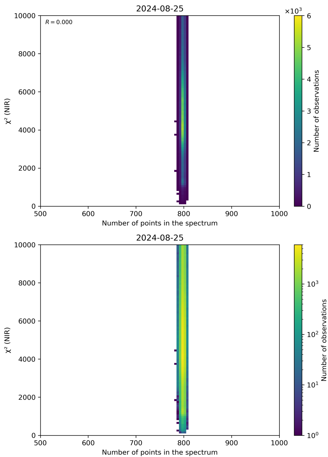
Figure 88: Scatter density plot of “Number of points in the spectrum” against “ \chi^2 (NIR)” for 2024-08-24 to 2024-08-26.
