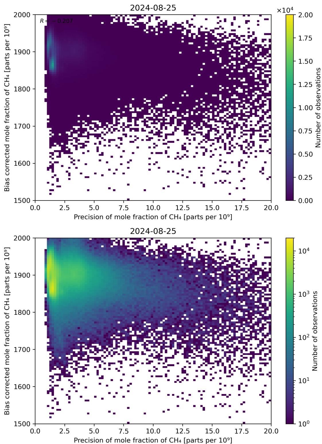
Figure 82: Scatter density plot of “Precision of mole fraction of CH 4 ” against “Bias corrected mole fraction of CH 4 ” for 2024-08-24 to 2024-08-26.
