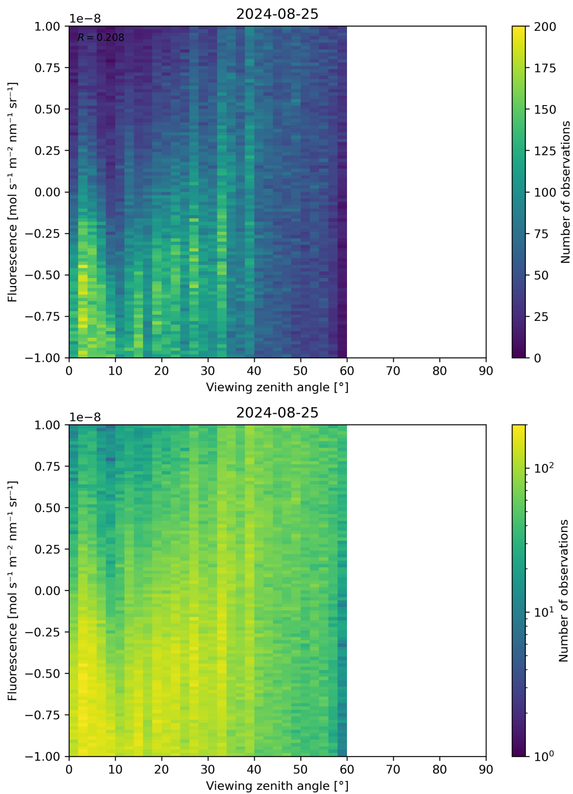
Figure 108: Scatter density plot of “Viewing zenith angle” against “Fluorescence” for 2024-08-24 to 2024-08-26.
