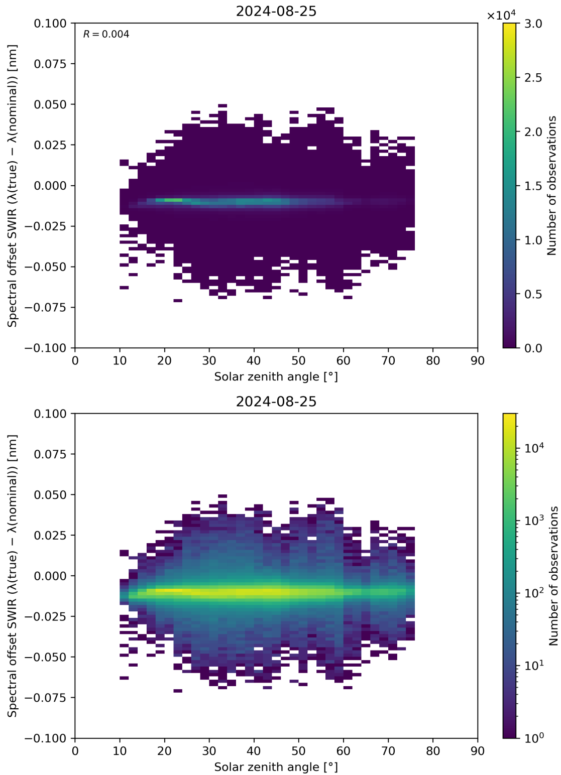
Figure 104: Scatter density plot of “Solar zenith angle” against “Spectral offset SWIR ( \lambda(\text{true}) - \lambda(\text{nominal}) )” for 2024-08-24 to 2024-08-26.
