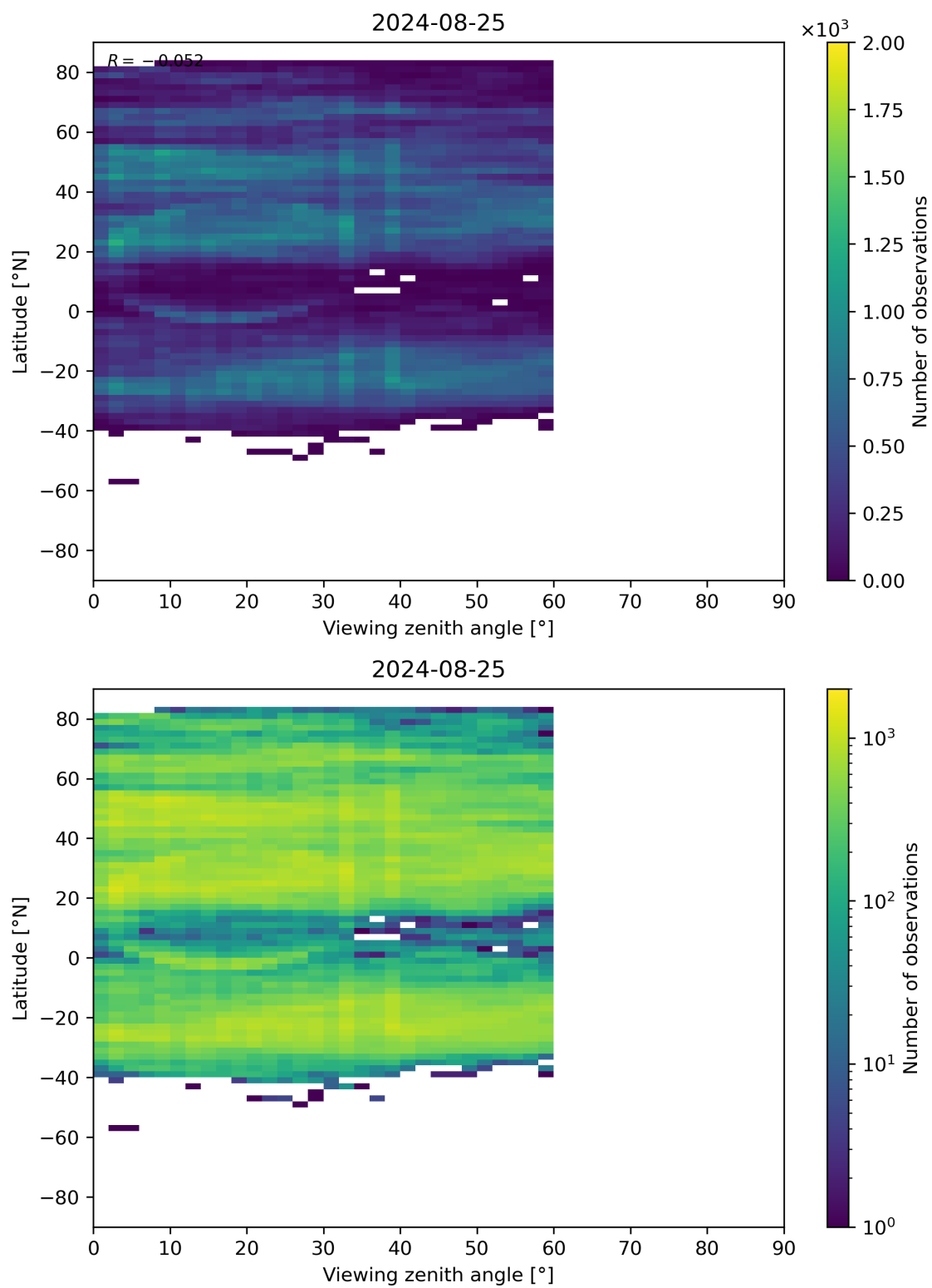
Figure 109: Scatter density plot of “Viewing zenith angle” against “Latitude” for 2024-08-24 to 2024-08-26.
