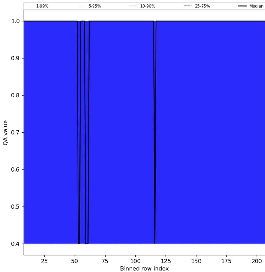
Figure 33: Along track statistics of “QA value” for 2024-08-24 to 2024-08-26
