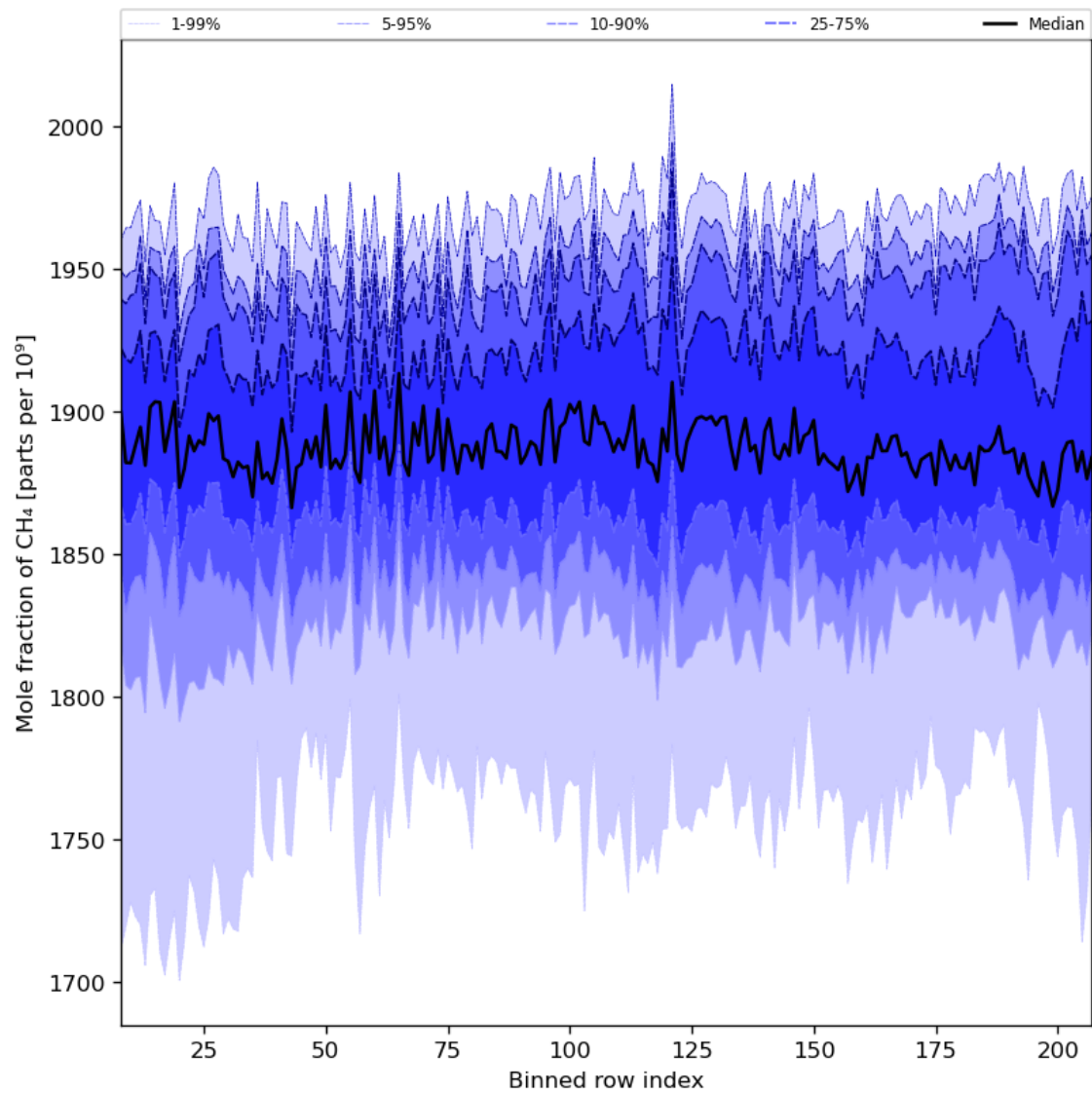
Figure 34: Along track statistics of “Mole fraction of CH 4 ” for 2024-08-24 to 2024-08-26
