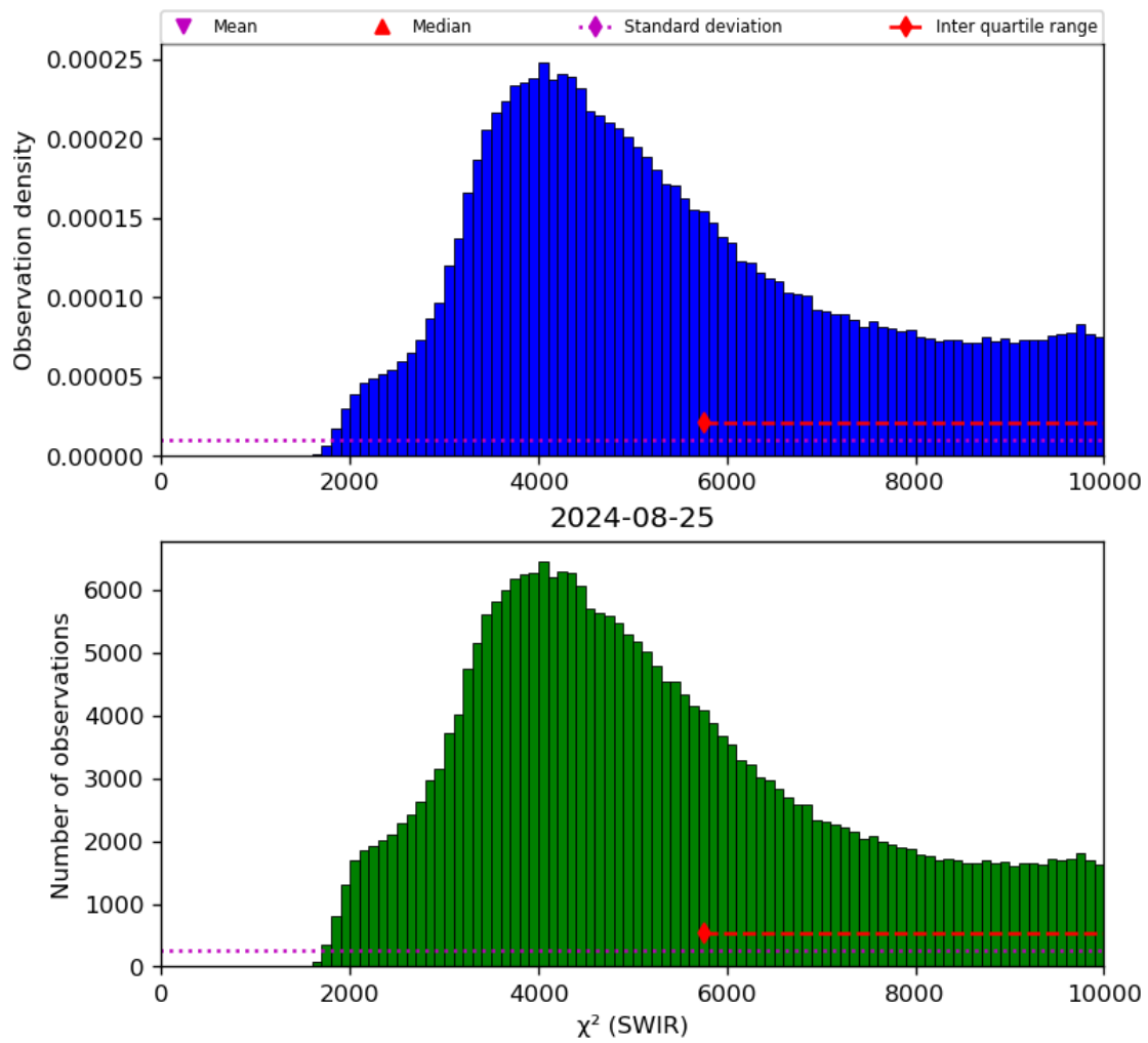
Figure 28: Histogram of “ \chi^2 (SWIR)” for 2024-08-24 to 2024-08-26
