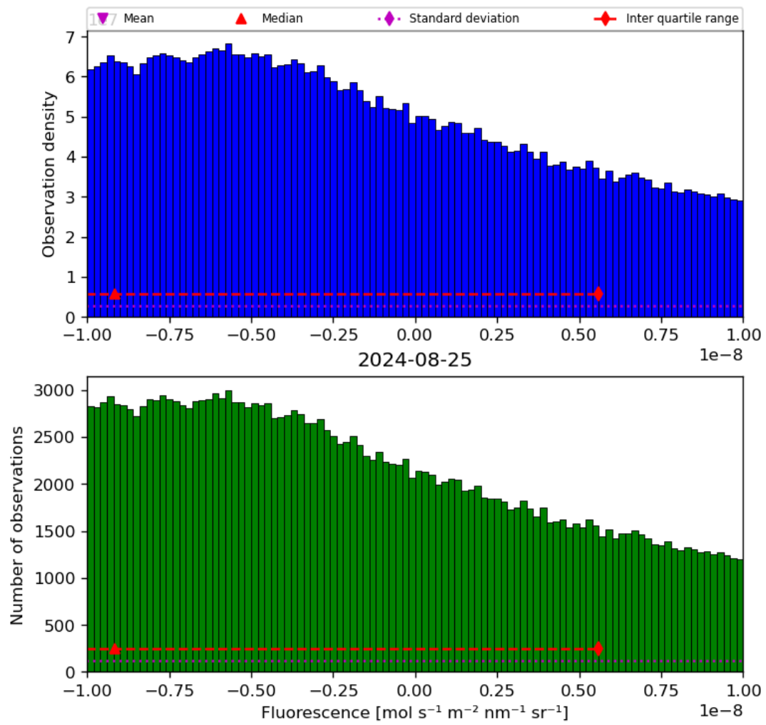
Figure 32: Histogram of “Fluorescence” for 2024-08-24 to 2024-08-26
