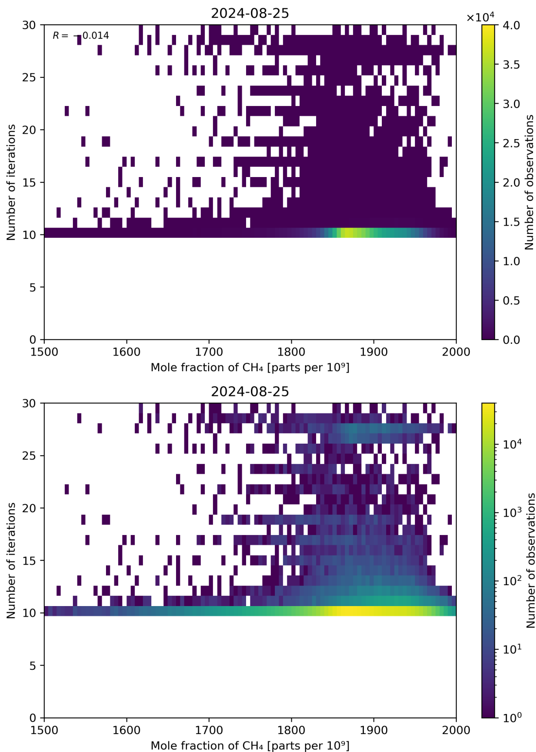
Figure 76: Scatter density plot of “Mole fraction of CH 4 ” against “Number of iterations” for 2024-08-24 to 2024-08-26.
