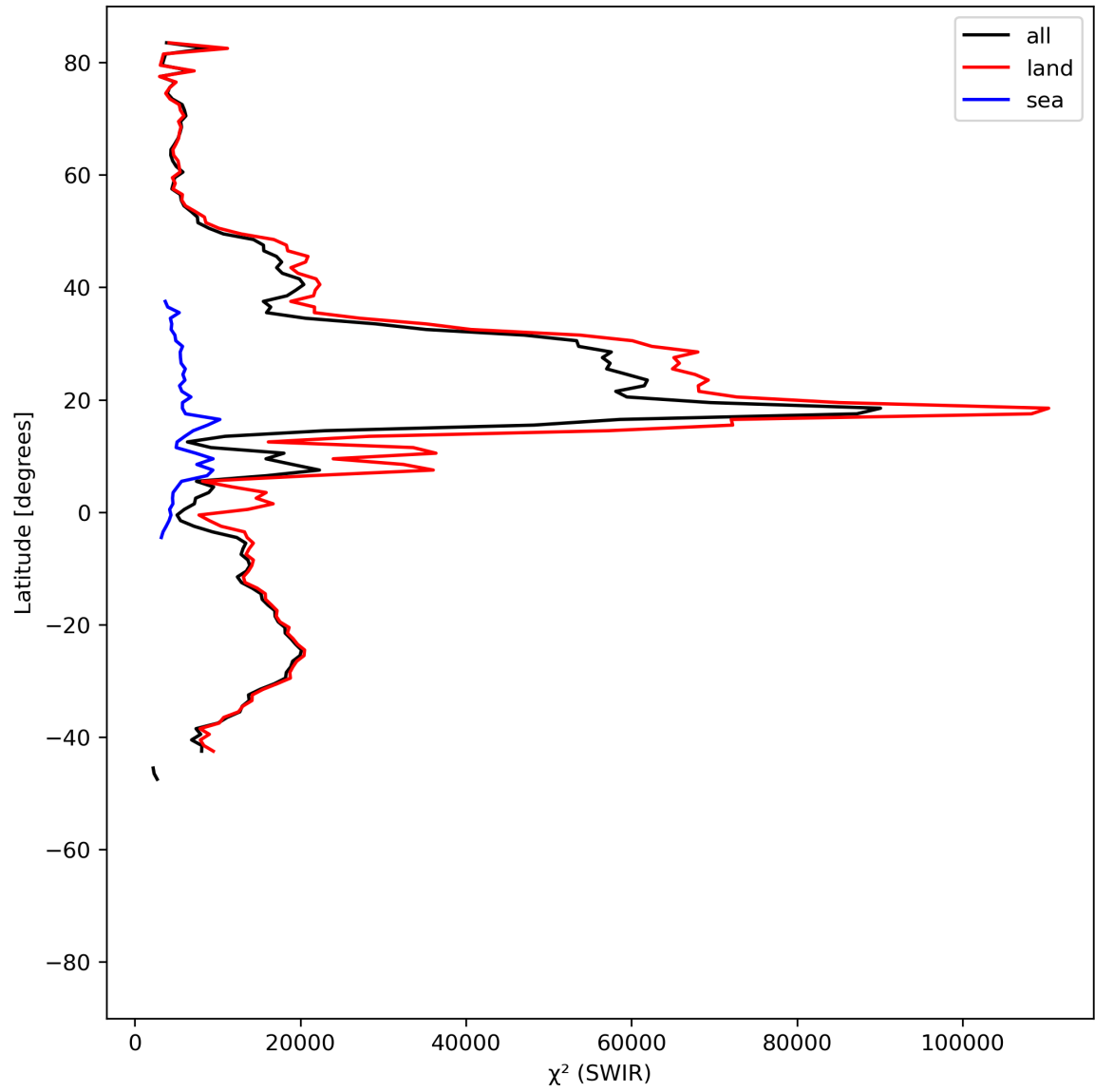
Figure 17: Zonal average of “ \chi^2 (SWIR)” for 2024-08-24 to 2024-08-26.
