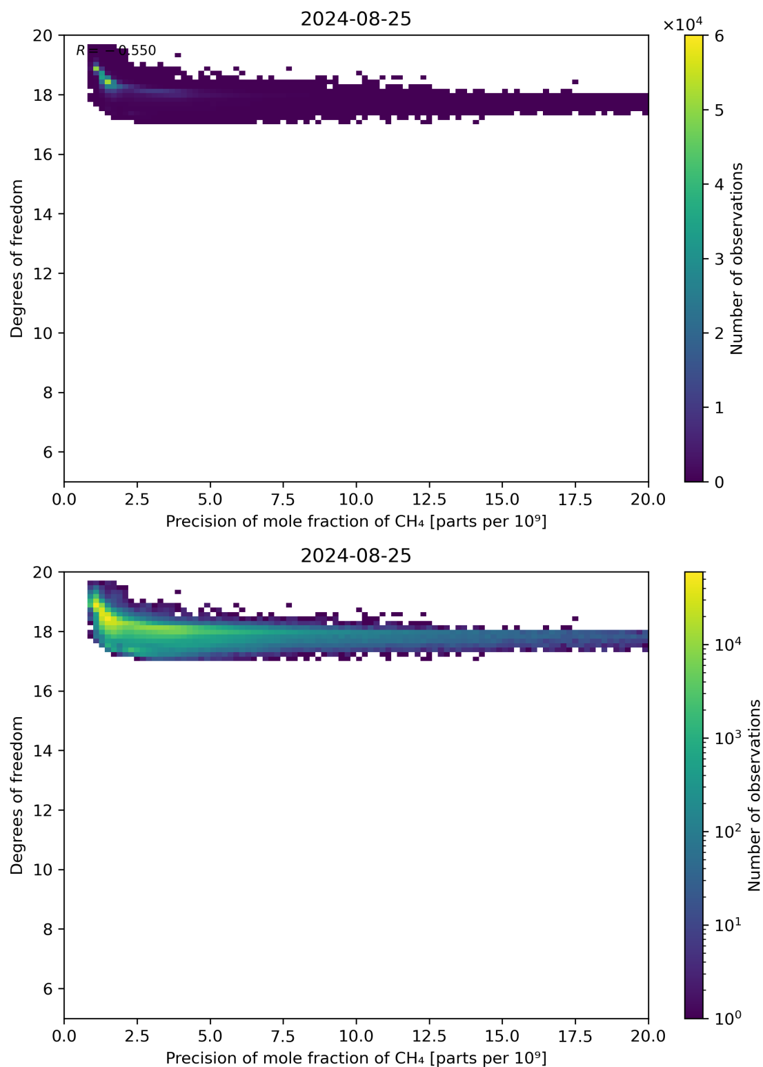
Figure 80: Scatter density plot of “Precision of mole fraction of CH 4 ” against “Degrees of freedom” for 2024-08-24 to 2024-08-26.
