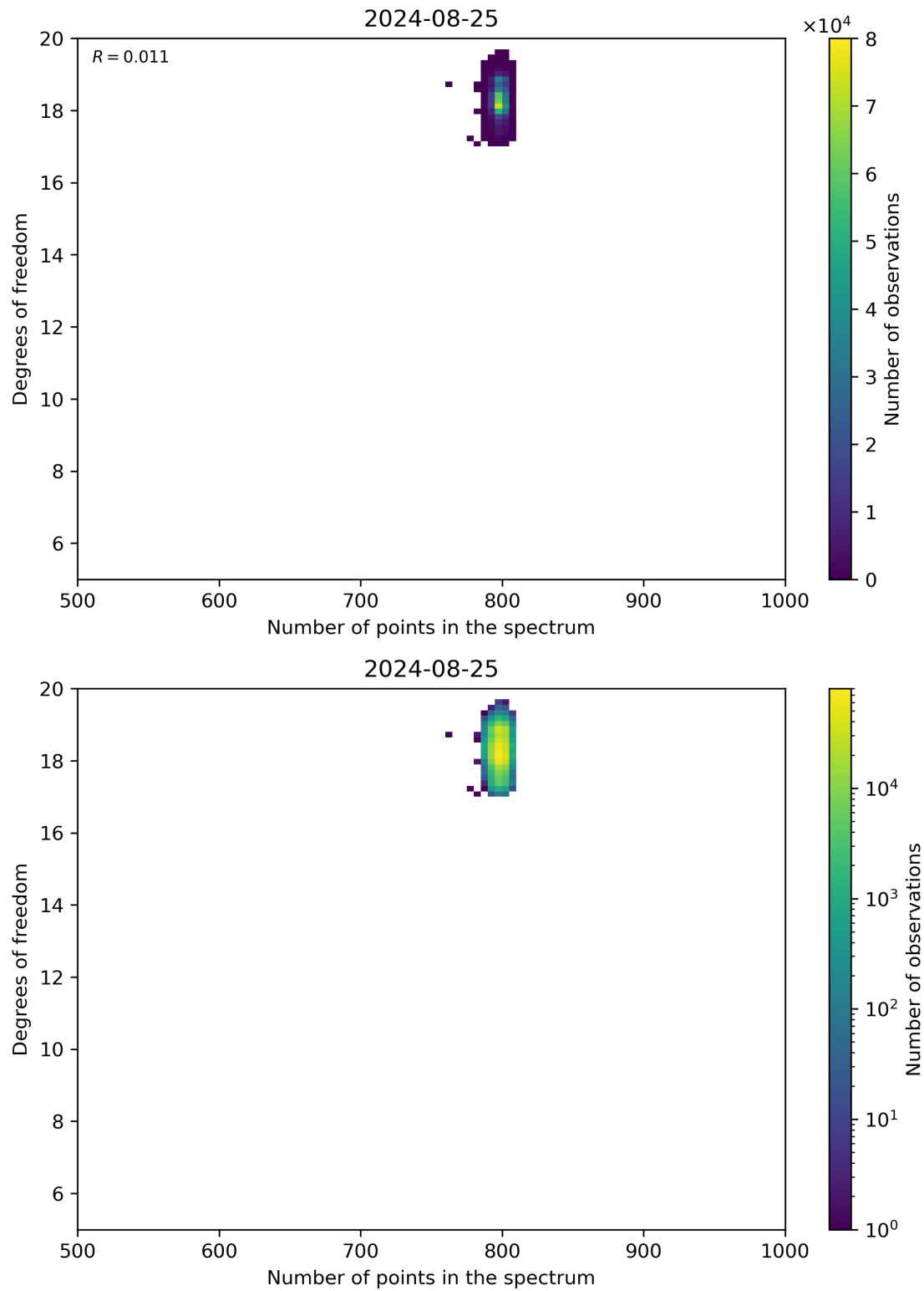
Figure 90: Scatter density plot of “Number of points in the spectrum” against “Degrees of freedom” for 2024-08-24 to 2024-08-26.
