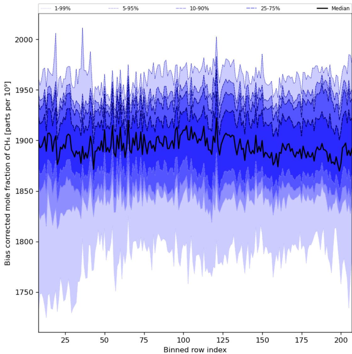
Figure 36: Along track statistics of “Bias corrected mole fraction of \text{CH}_4 ” for 2024-08-24 to 2024-08-26
