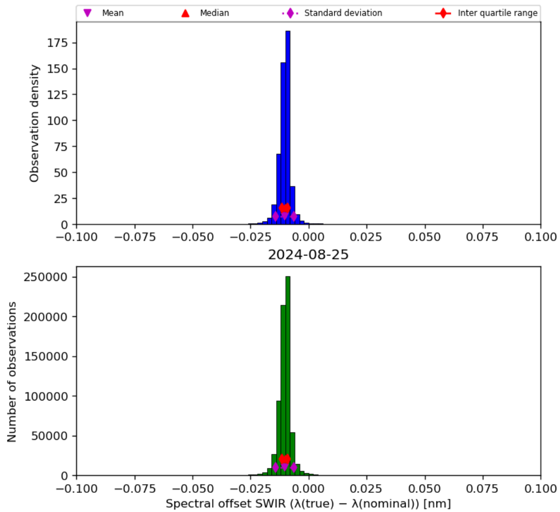
Figure 27: Histogram of “Spectral offset SWIR ( \lambda(\text{true}) - \lambda(\text{nominal}) )” for 2024-08-24 to 2024-08-26
