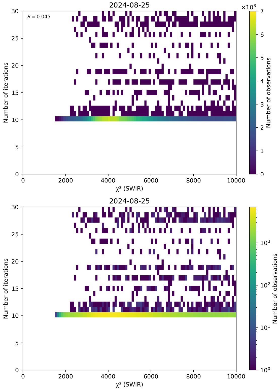
Figure 50: Scatter density plot of “ \chi^2 (SWIR)” against “Number of iterations” for 2024-08-24 to 2024-08-26.
