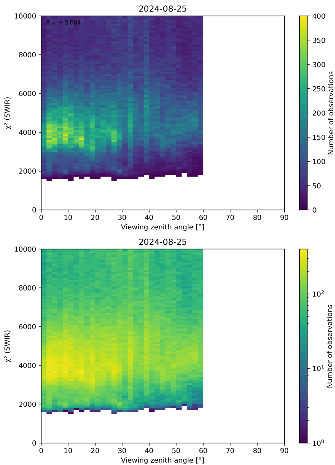
Figure 106: Scatter density plot of “Viewing zenith angle” against “ \chi^2 (SWIR)” for 2024-08-24 to 2024-08-26.
