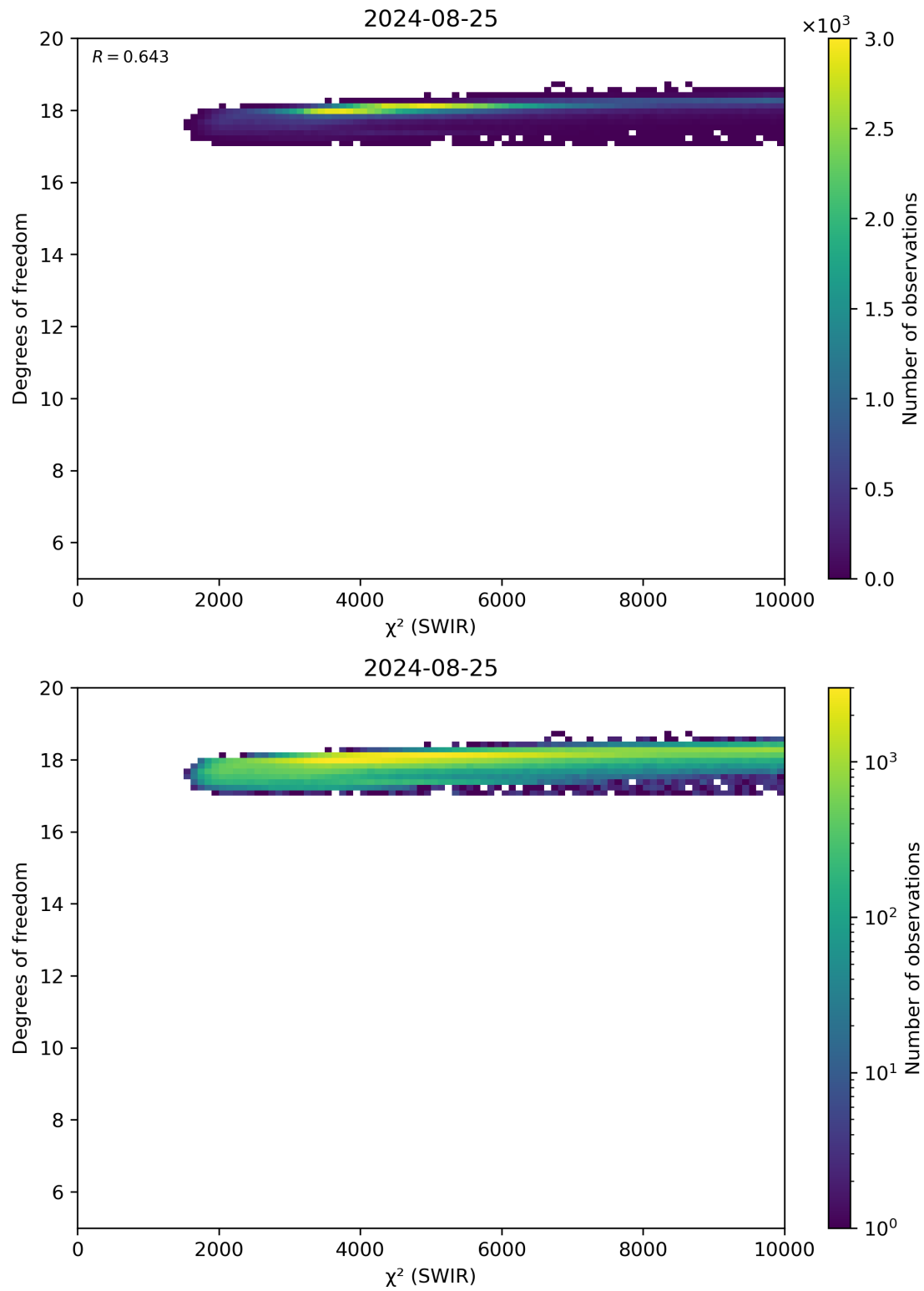
Figure 48: Scatter density plot of “ \chi^2 (SWIR)” against “Degrees of freedom” for 2024-08-24 to 2024-08-26.
