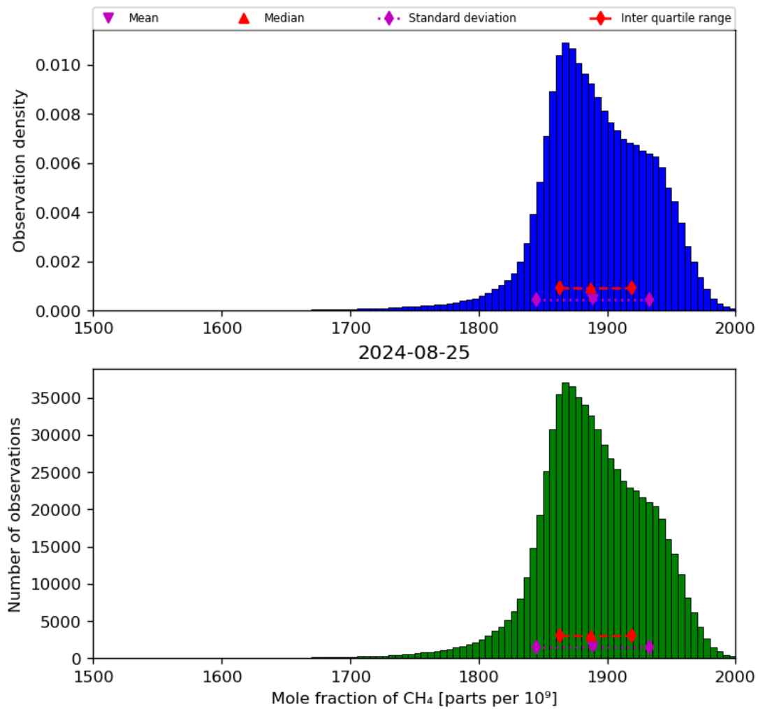
Figure 23: Histogram of “Mole fraction of CH 4 ” for 2024-08-24 to 2024-08-26
