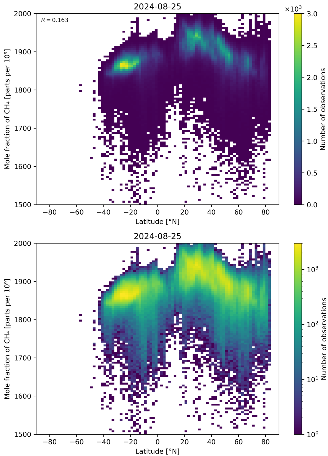
Figure 57: Scatter density plot of “Latitude” against “Mole fraction of \text{CH}_4 ” for 2024-08-24 to 2024-08-26.
