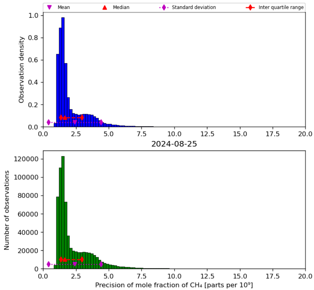
Figure 24: Histogram of “Precision of mole fraction of CH 4 ” for 2024-08-24 to 2024-08-26
