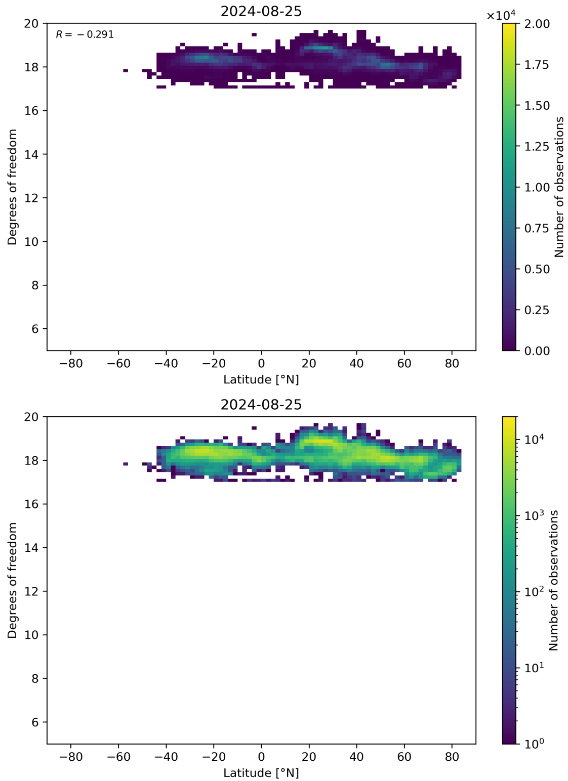
Figure 55: Scatter density plot of “Latitude” against “Degrees of freedom” for 2024-08-24 to 2024-08-26.
