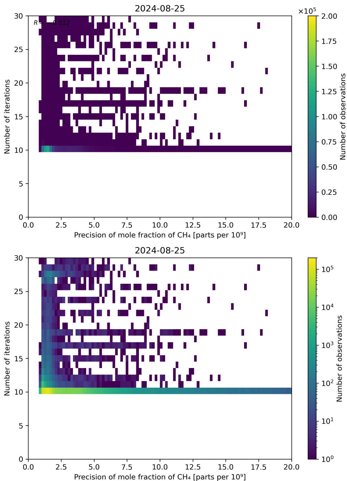
Figure 83: Scatter density plot of “Precision of mole fraction of CH 4 ” against “Number of iterations” for 2024-08-24 to 2024-08-26.
