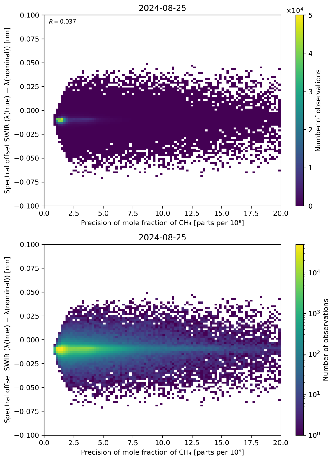
Figure 85: Scatter density plot of “Precision of mole fraction of CH 4 ” against “Spectral offset SWIR ( \lambda(\text{true}) - \lambda(\text{nominal}) )” for 2024-08-24 to 2024-08-26.
