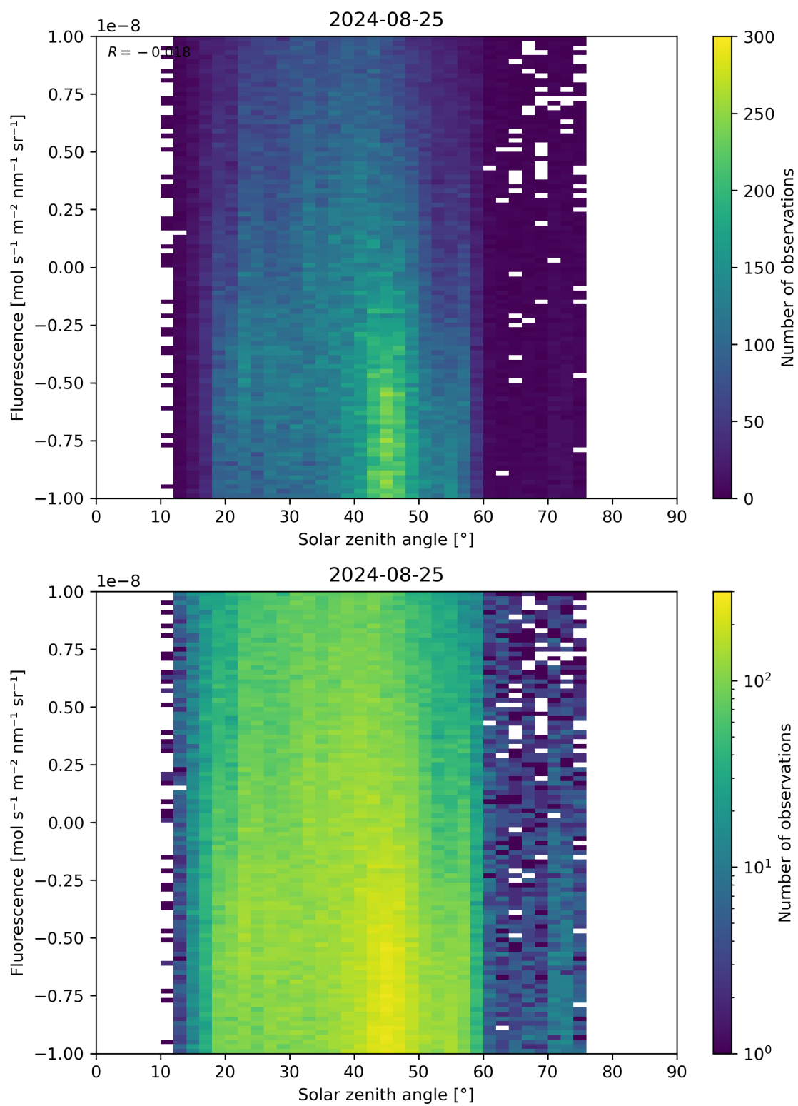
Figure 97: Scatter density plot of “Solar zenith angle” against “Fluorescence” for 2024-08-24 to 2024-08-26.
