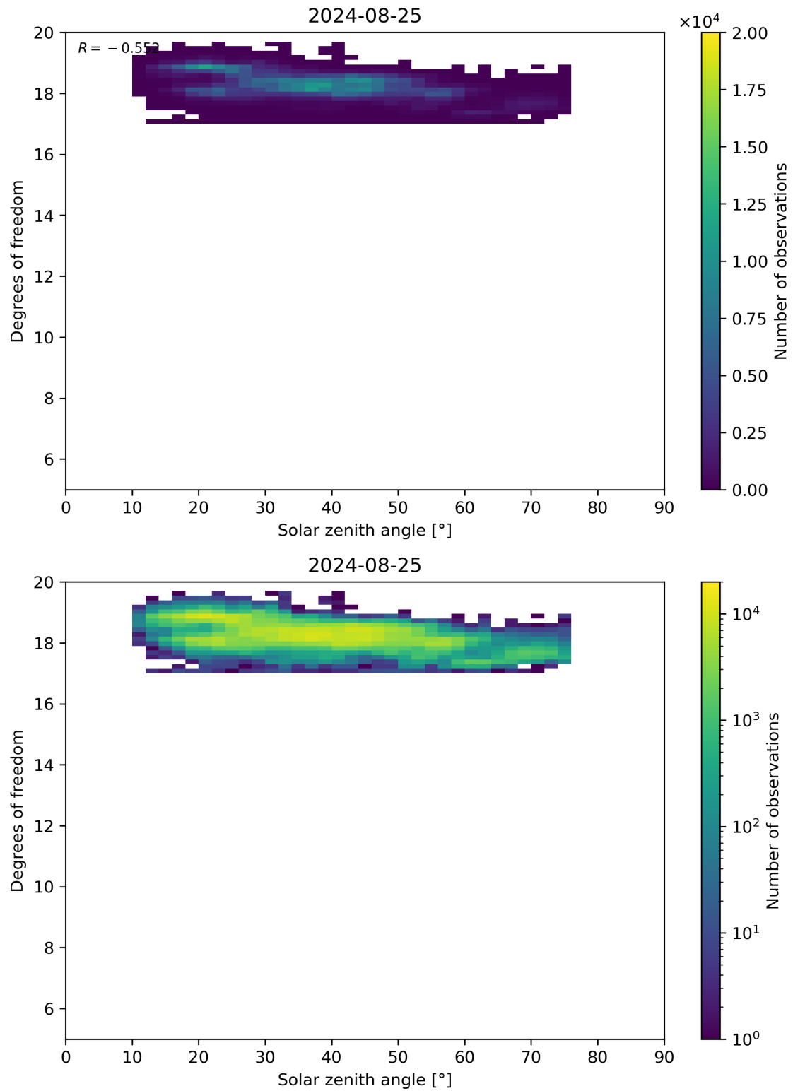
Figure 96: Scatter density plot of “Solar zenith angle” against “Degrees of freedom” for 2024-08-24 to 2024-08-26.
