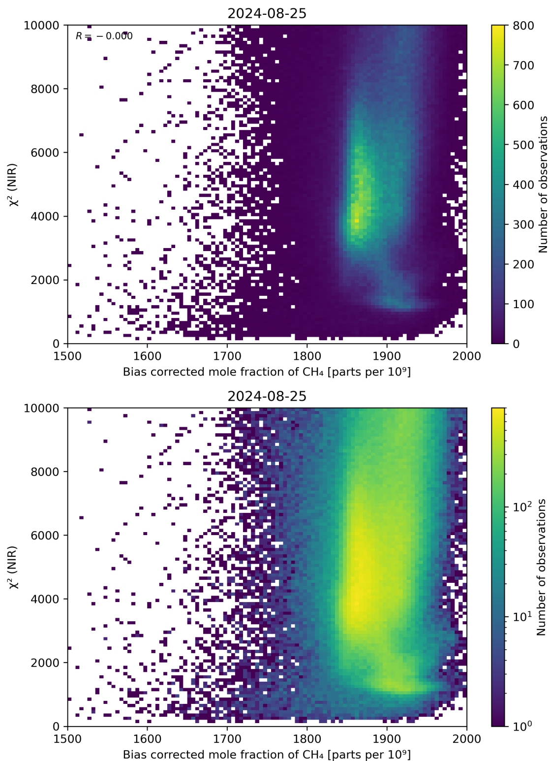
Figure 63: Scatter density plot of “Bias corrected mole fraction of CH 4 ” against “ \chi^2 (NIR)” for 2024-08-24 to 2024-08-26.
