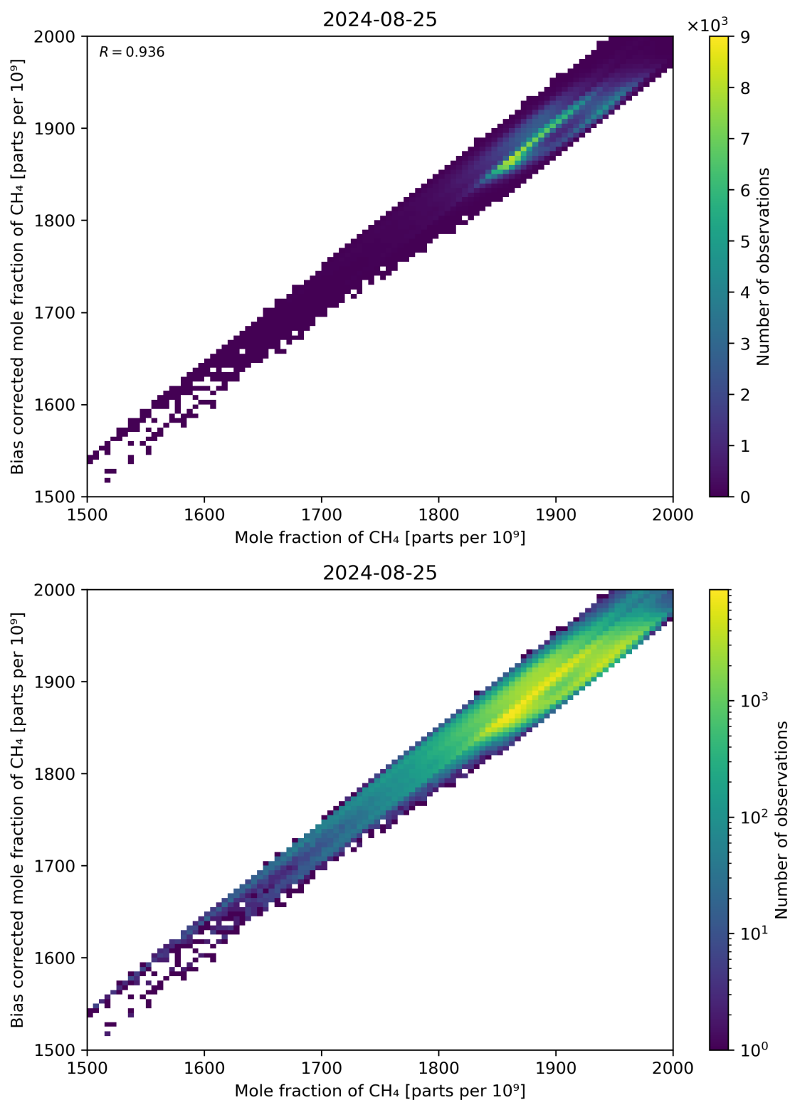
Figure 74: Scatter density plot of “Mole fraction of CH 4 ” against “Bias corrected mole fraction of CH 4 ” for 2024-08-24 to 2024-08-26.
