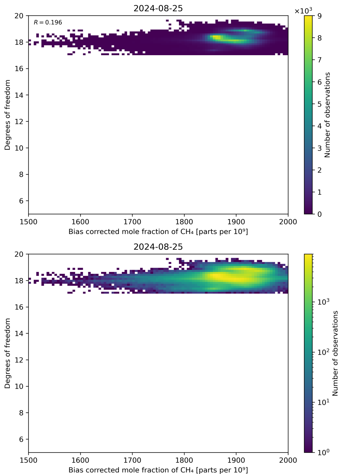
Figure 65: Scatter density plot of “Bias corrected mole fraction of CH 4 ” against “Degrees of freedom” for 2024-08-24 to 2024-08-26.
