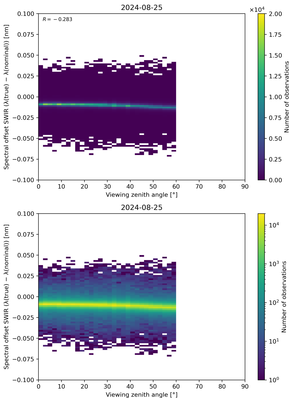
Figure 116: Scatter density plot of “Viewing zenith angle” against “Spectral offset SWIR ( \lambda(\text{true}) - \lambda(\text{nominal}) )” for 2024-08-24 to 2024-08-26.
