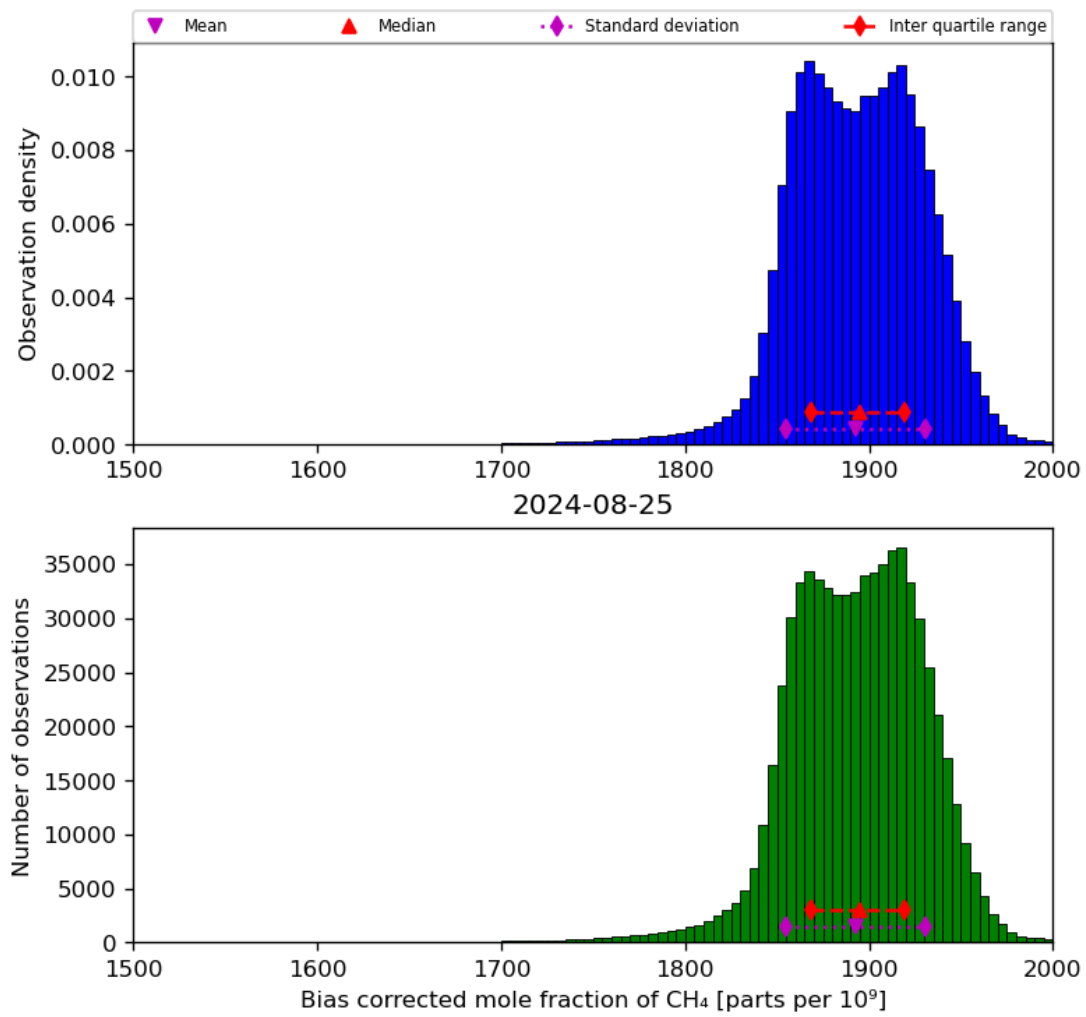
Figure 25: Histogram of “Bias corrected mole fraction of CH 4 ” for 2024-08-24 to 2024-08-26
