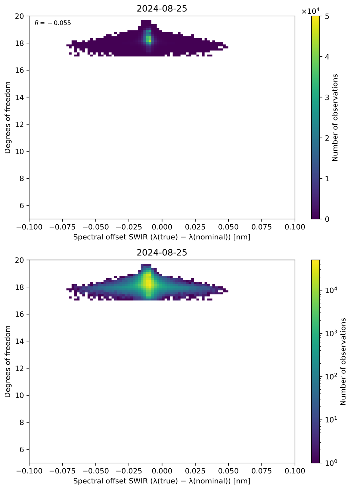
Figure 119: Scatter density plot of “Spectral offset SWIR ( \lambda(\text{true}) - \lambda(\text{nominal}) )” against “Degrees of freedom” for 2024-08-24 to 2024-08-26.
