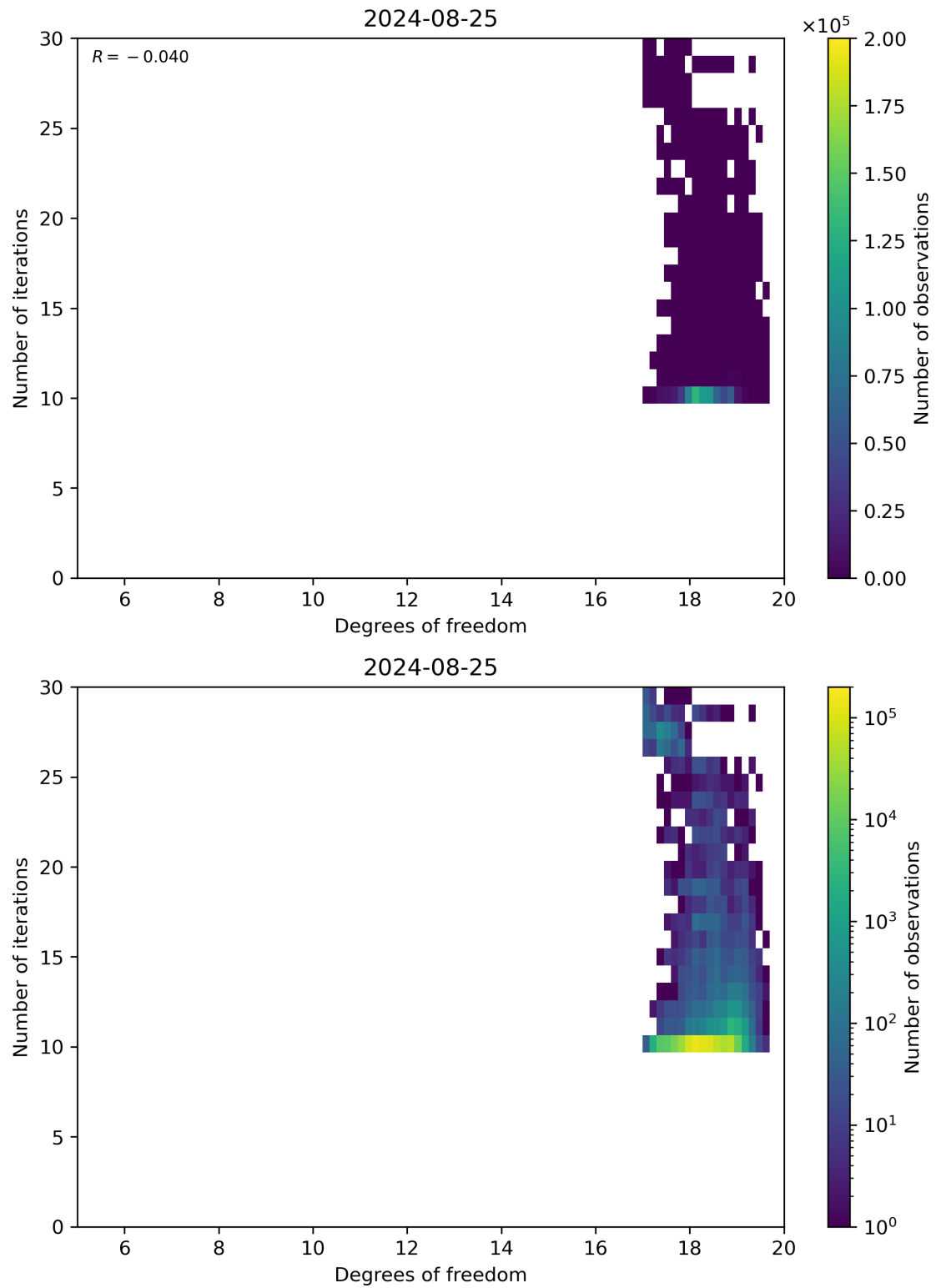
Figure 52: Scatter density plot of “Degrees of freedom” against “Number of iterations” for 2024-08-24 to 2024-08-26.
