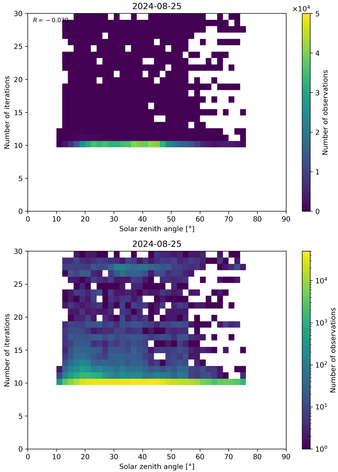
Figure 102: Scatter density plot of “Solar zenith angle” against “Number of iterations” for 2024-08-24 to 2024-08-26.
