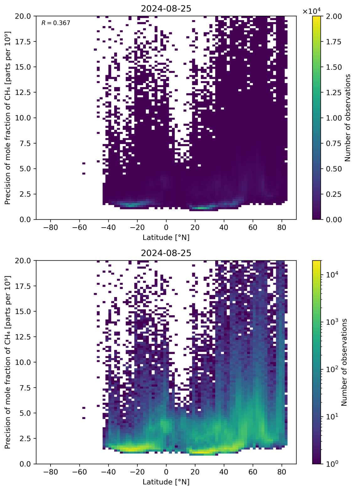
Figure 59: Scatter density plot of “Latitude” against “Precision of mole fraction of \text{CH}_4 ” for 2024-08-24 to 2024-08-26.
