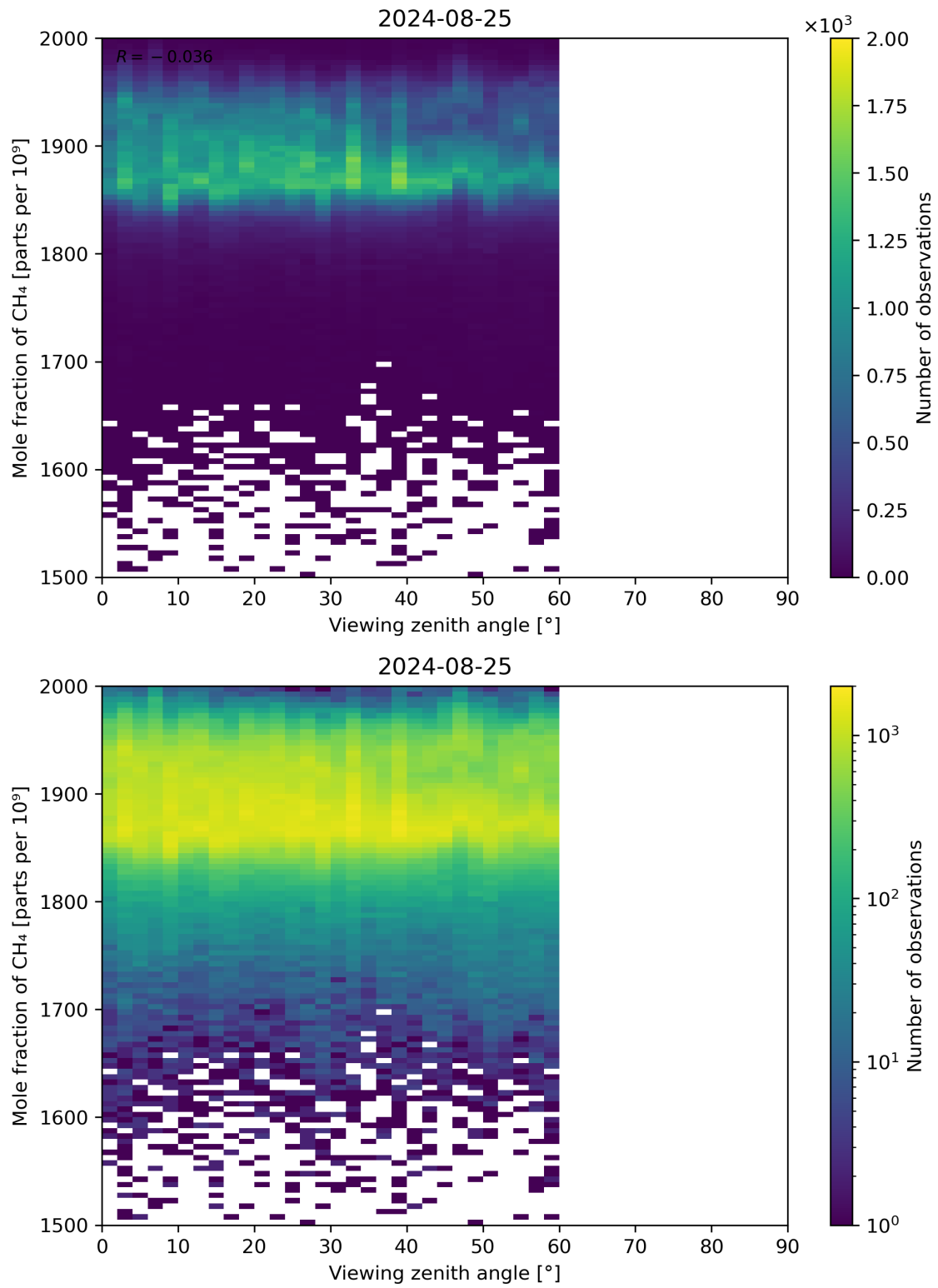
Figure 110: Scatter density plot of “Viewing zenith angle” against “Mole fraction of CH 4 ” for 2024-08-24 to 2024-08-26.
