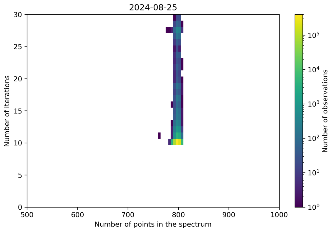
Figure 92: Scatter density plot of “Number of points in the spectrum” against “Number of iterations” for 2024-08-24 to 2024-08-26.
