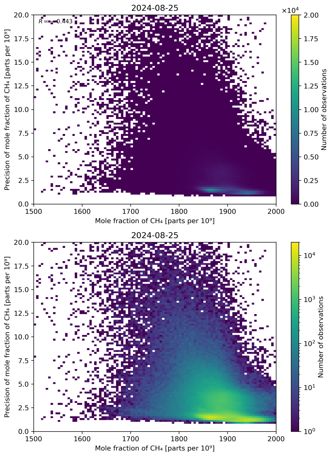
Figure 75: Scatter density plot of “Mole fraction of CH 4 ” against “Precision of mole fraction of CH 4 ” for 2024-08-24 to 2024-08-26.
