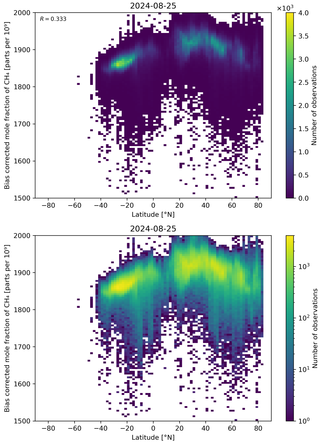
Figure 58: Scatter density plot of “Latitude” against “Bias corrected mole fraction of \text{CH}_4 ” for 2024-08-24 to 2024-08-26.
