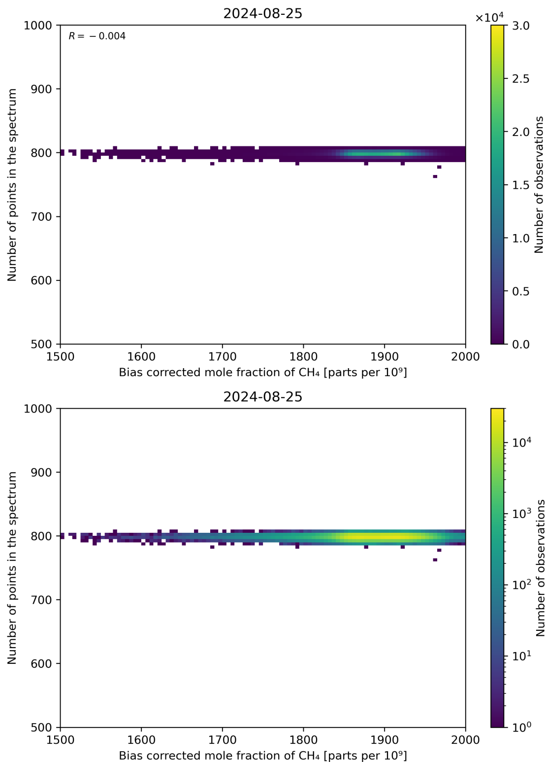
Figure 68: Scatter density plot of “Bias corrected mole fraction of CH 4 ” against “Number of points in the spectrum” for 2024-08-24 to 2024-08-26.
