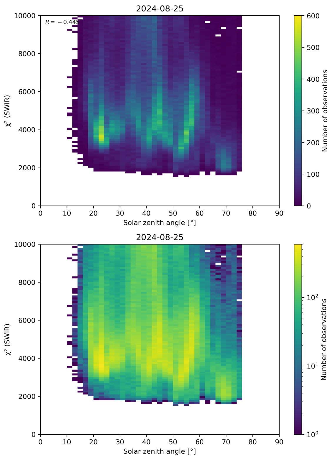
Figure 95: Scatter density plot of “Solar zenith angle” against “ \chi^2 (SWIR)” for 2024-08-24 to 2024-08-26.
