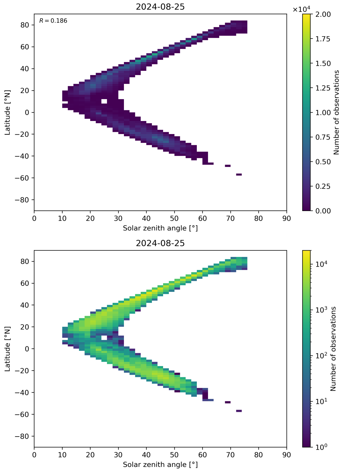
Figure 98: Scatter density plot of “Solar zenith angle” against “Latitude” for 2024-08-24 to 2024-08-26.
