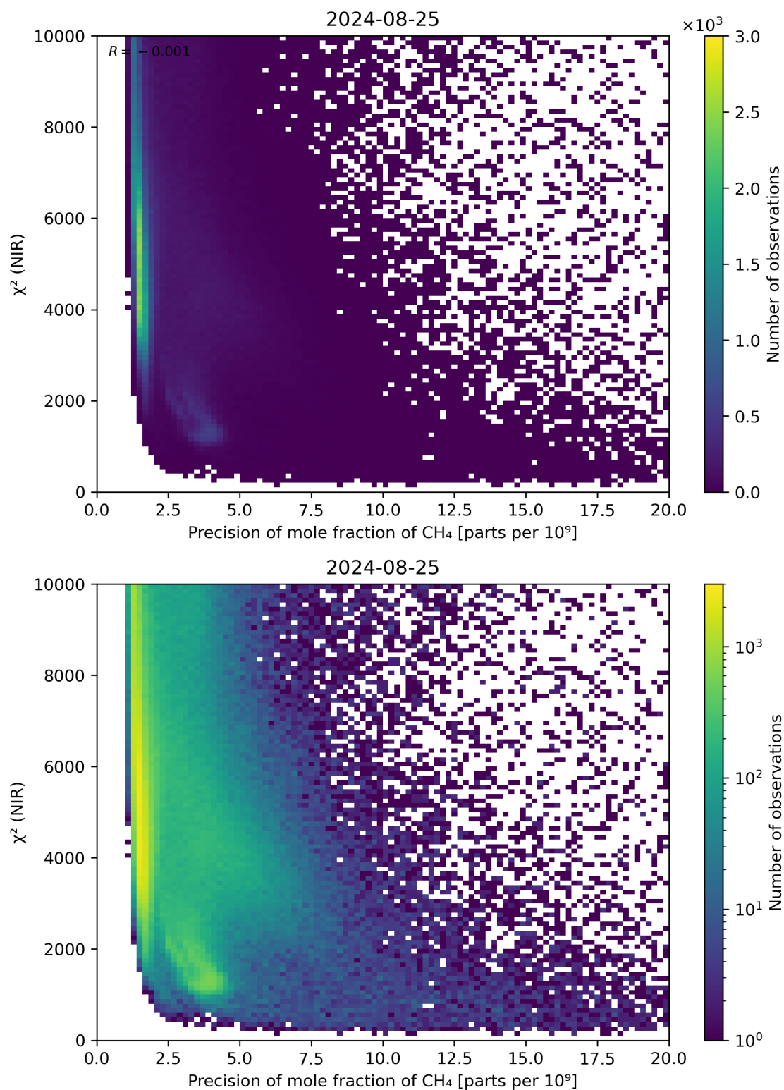
Figure 78: Scatter density plot of “Precision of mole fraction of CH 4 ” against “ \chi^2 (NIR)” for 2024-08-24 to 2024-08-26.
