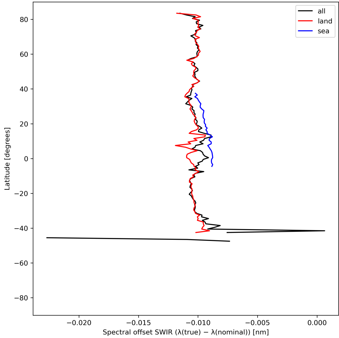
Figure 16: Zonal average of “Spectral offset SWIR ( \lambda(\text{true}) - \lambda(\text{nominal}) )” for 2024-08-24 to 2024-08-26.
