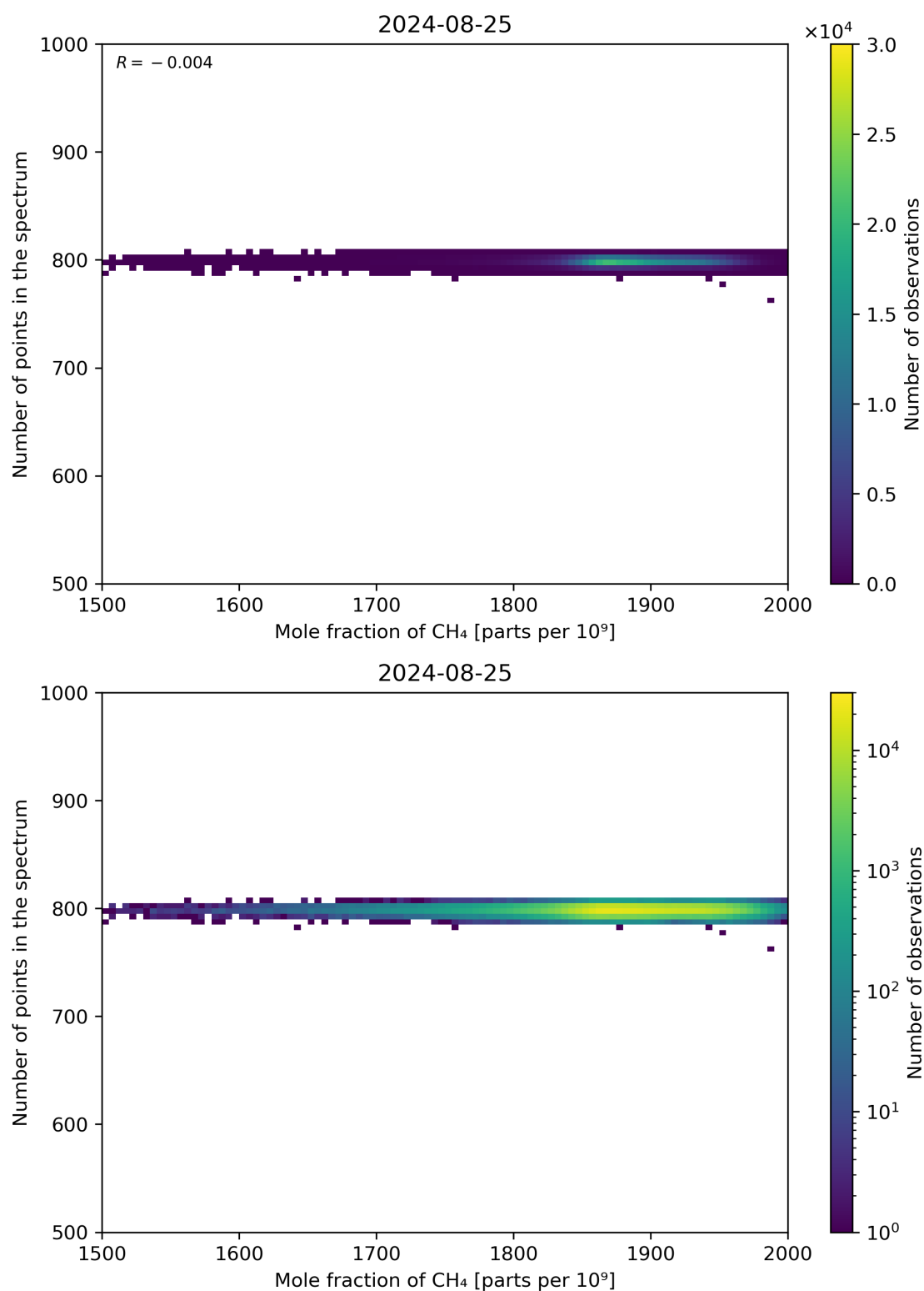
Figure 77: Scatter density plot of “Mole fraction of CH 4 ” against “Number of points in the spectrum” for 2024-08-24 to 2024-08-26.
