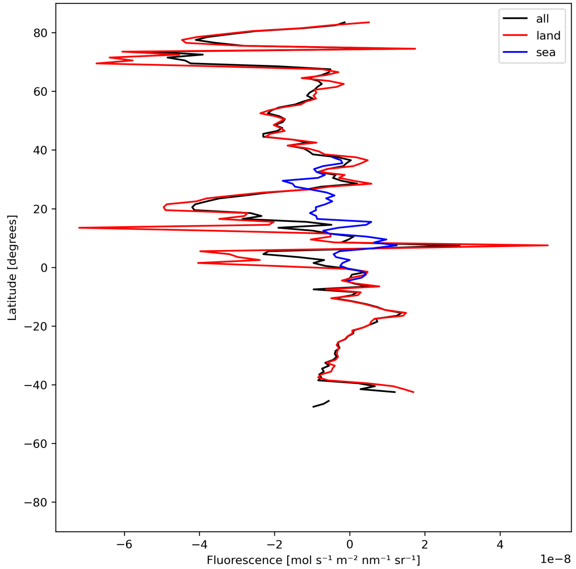
Figure 21: Zonal average of “Fluorescence” for 2024-08-24 to 2024-08-26.
