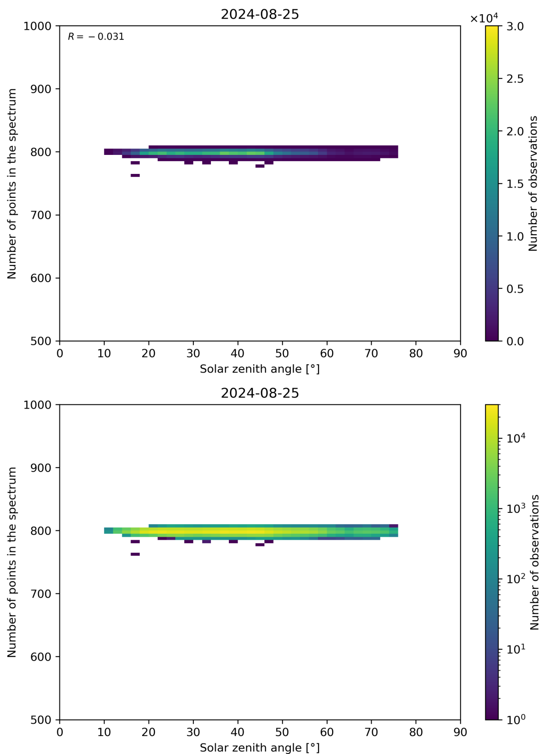
Figure 103: Scatter density plot of “Solar zenith angle” against “Number of points in the spectrum” for 2024-08-24 to 2024-08-26.
