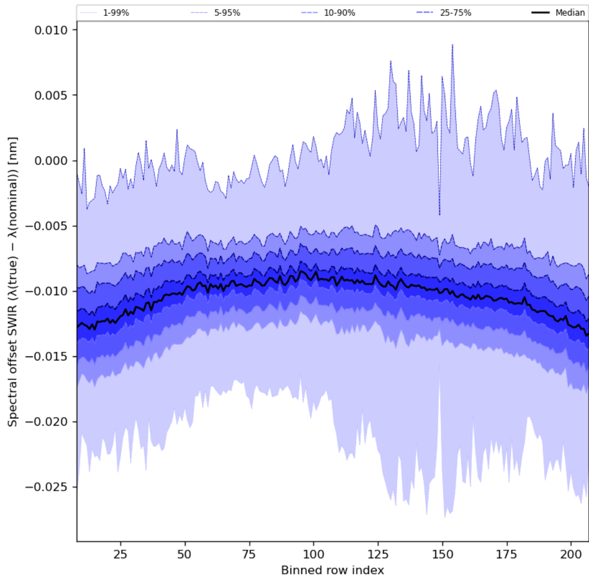
Figure 38: Along track statistics of “Spectral offset SWIR ( \lambda(\text{true}) - \lambda(\text{nominal}) )” for 2024-08-24 to 2024-08-26
