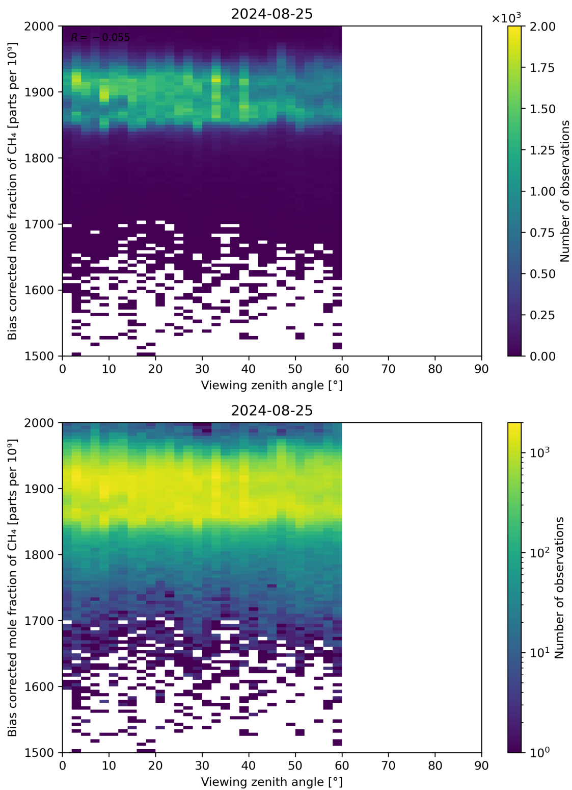
Figure 111: Scatter density plot of “Viewing zenith angle” against “Bias corrected mole fraction of CH 4 ” for 2024-08-24 to 2024-08-26.
