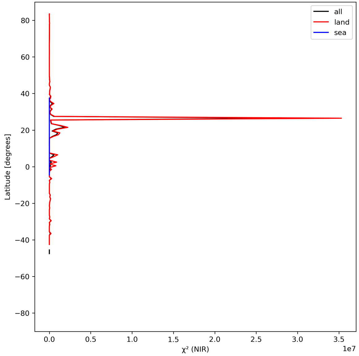
Figure 18: Zonal average of “ \chi^2 (NIR)” for 2024-08-24 to 2024-08-26.
