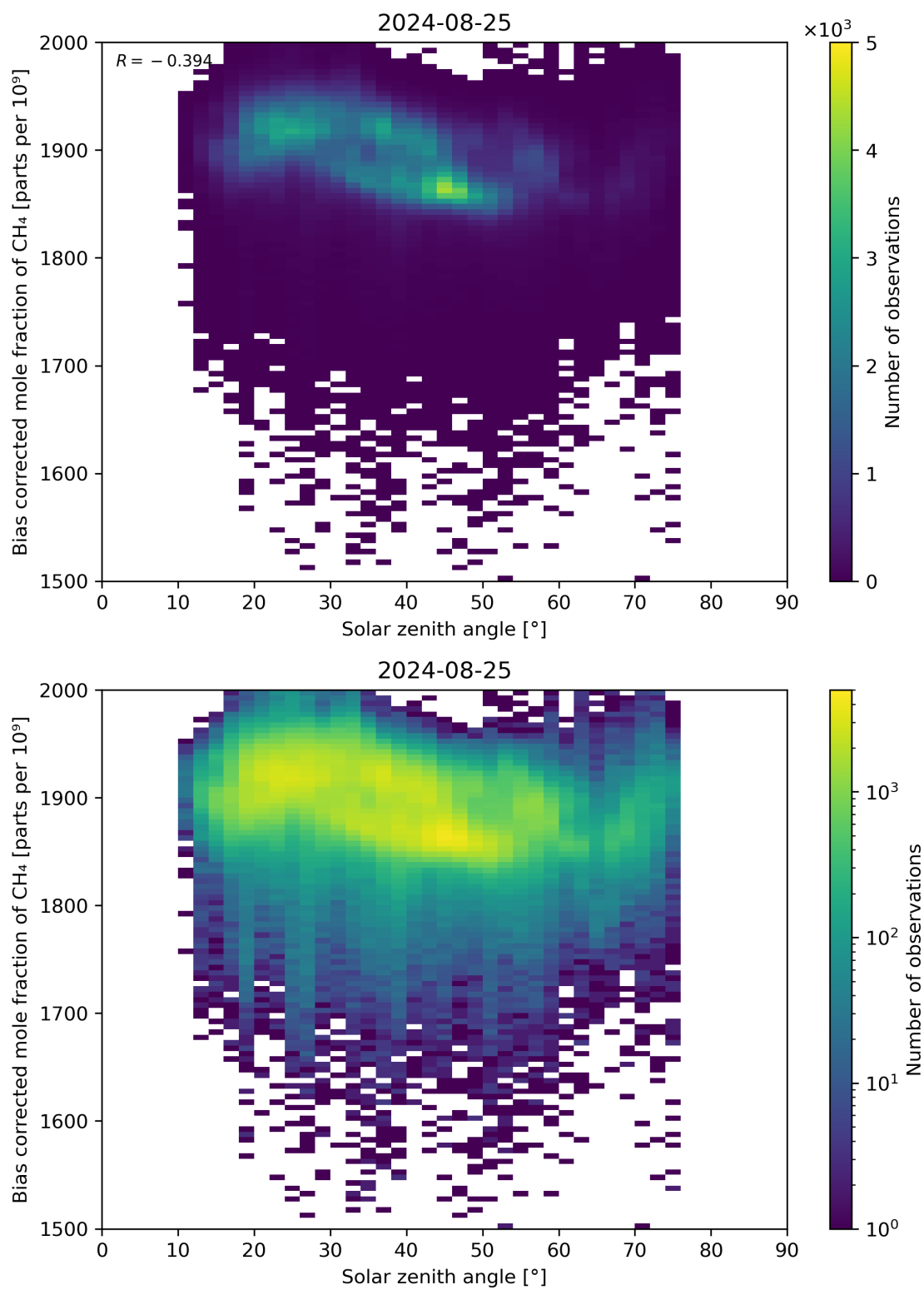
Figure 100: Scatter density plot of “Solar zenith angle” against “Bias corrected mole fraction of CH 4 ” for 2024-08-24 to 2024-08-26.
