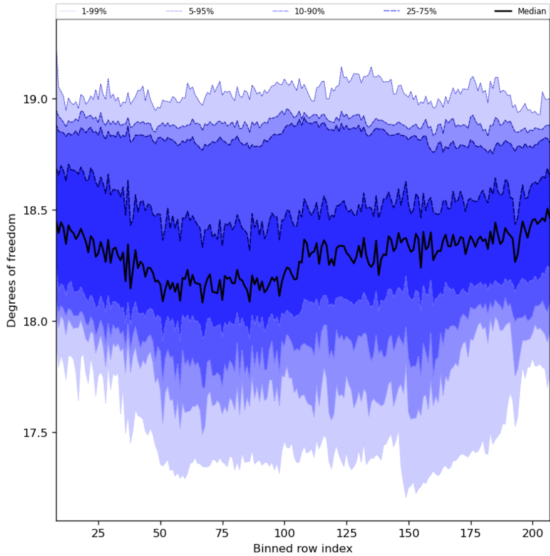
Figure 41: Along track statistics of “Degrees of freedom” for 2024-08-24 to 2024-08-26
