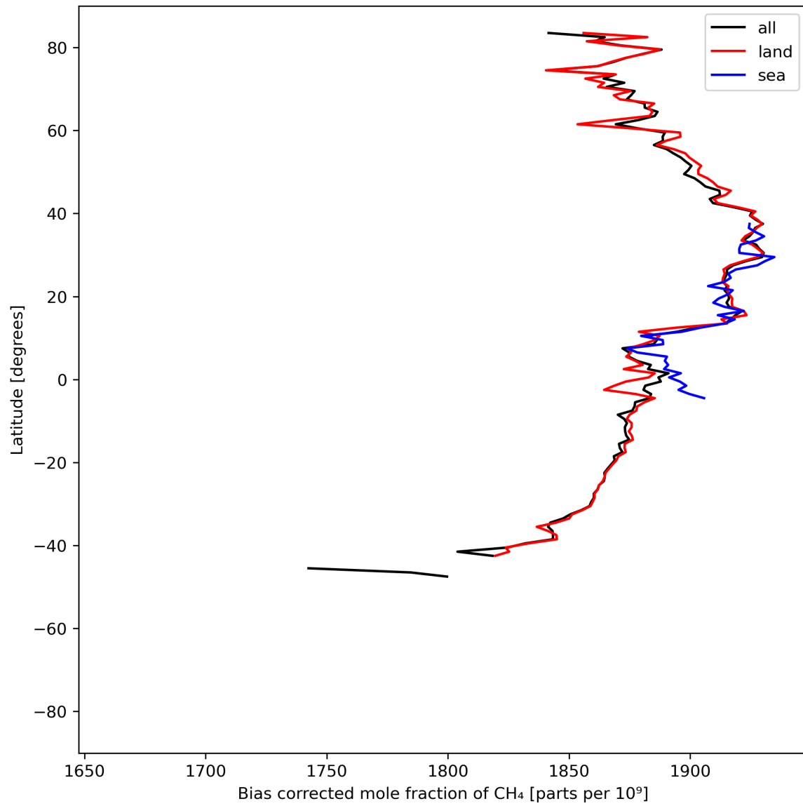
Figure 14: Zonal average of “Bias corrected mole fraction of CH 4 ” for 2024-08-24 to 2024-08-26.
