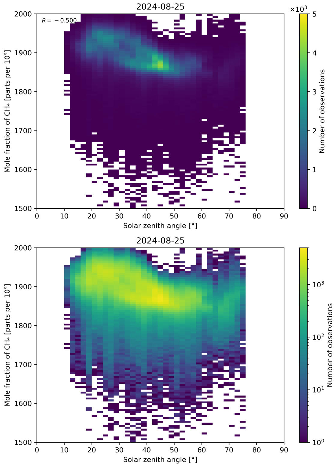
Figure 99: Scatter density plot of “Solar zenith angle” against “Mole fraction of CH 4 ” for 2024-08-24 to 2024-08-26.
