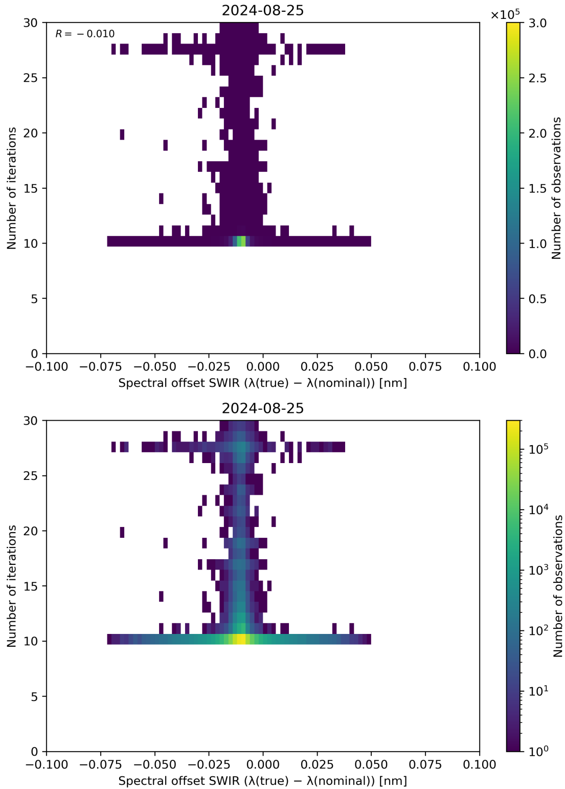
Figure 121: Scatter density plot of “Spectral offset SWIR ( \lambda(\text{true}) - \lambda(\text{nominal}) )” against “Number of iterations” for 2024-08-24 to 2024-08-26.
