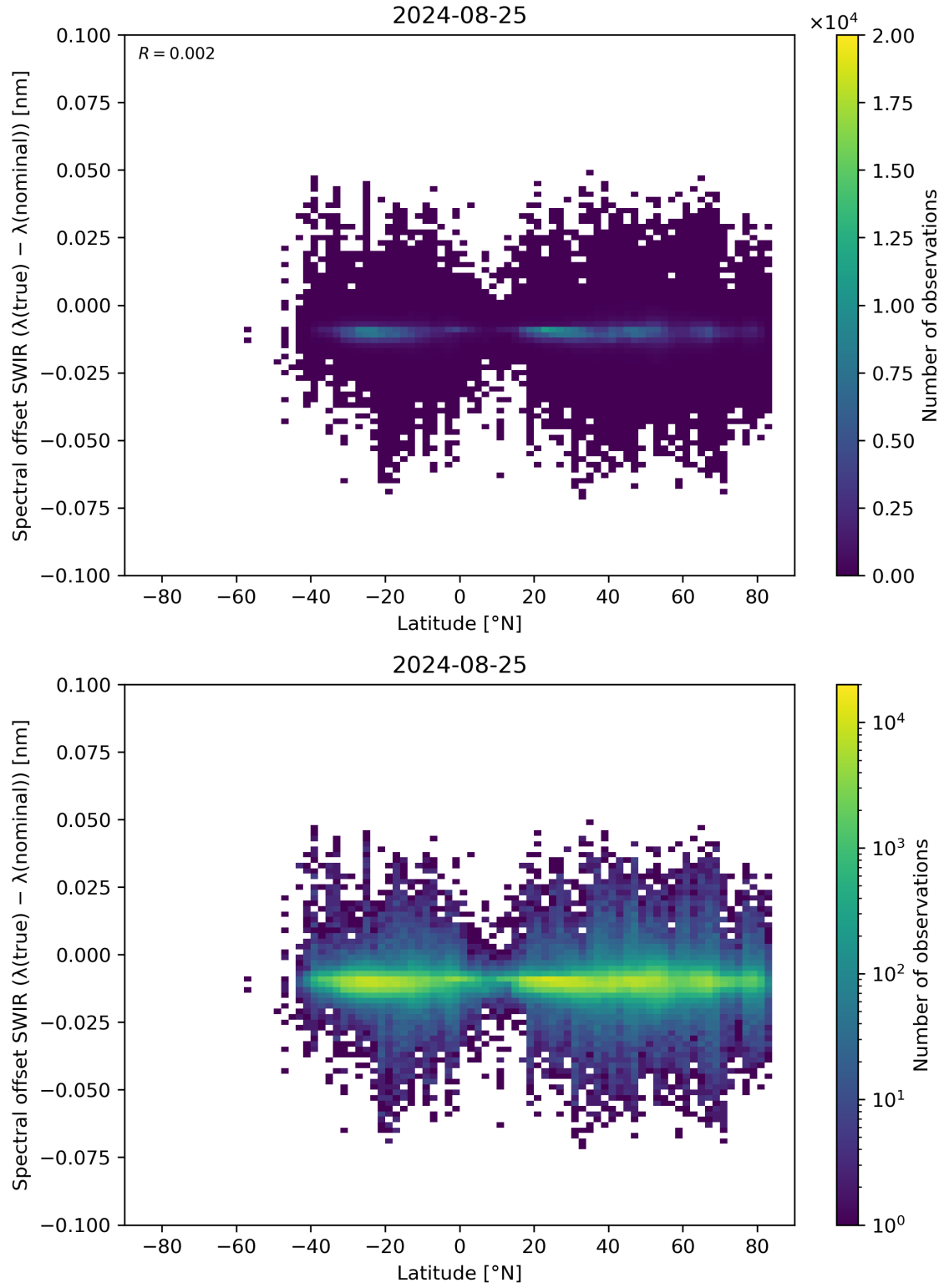
Figure 62: Scatter density plot of “Latitude” against “Spectral offset SWIR ( \lambda(\text{true}) - \lambda(\text{nominal}) )” for 2024-08-24 to 2024-08-26.
