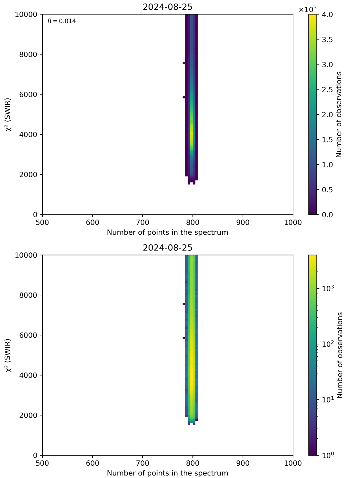
Figure 89: Scatter density plot of “Number of points in the spectrum” against “ \chi^2 (SWIR)” for 2024-08-24 to 2024-08-26.
