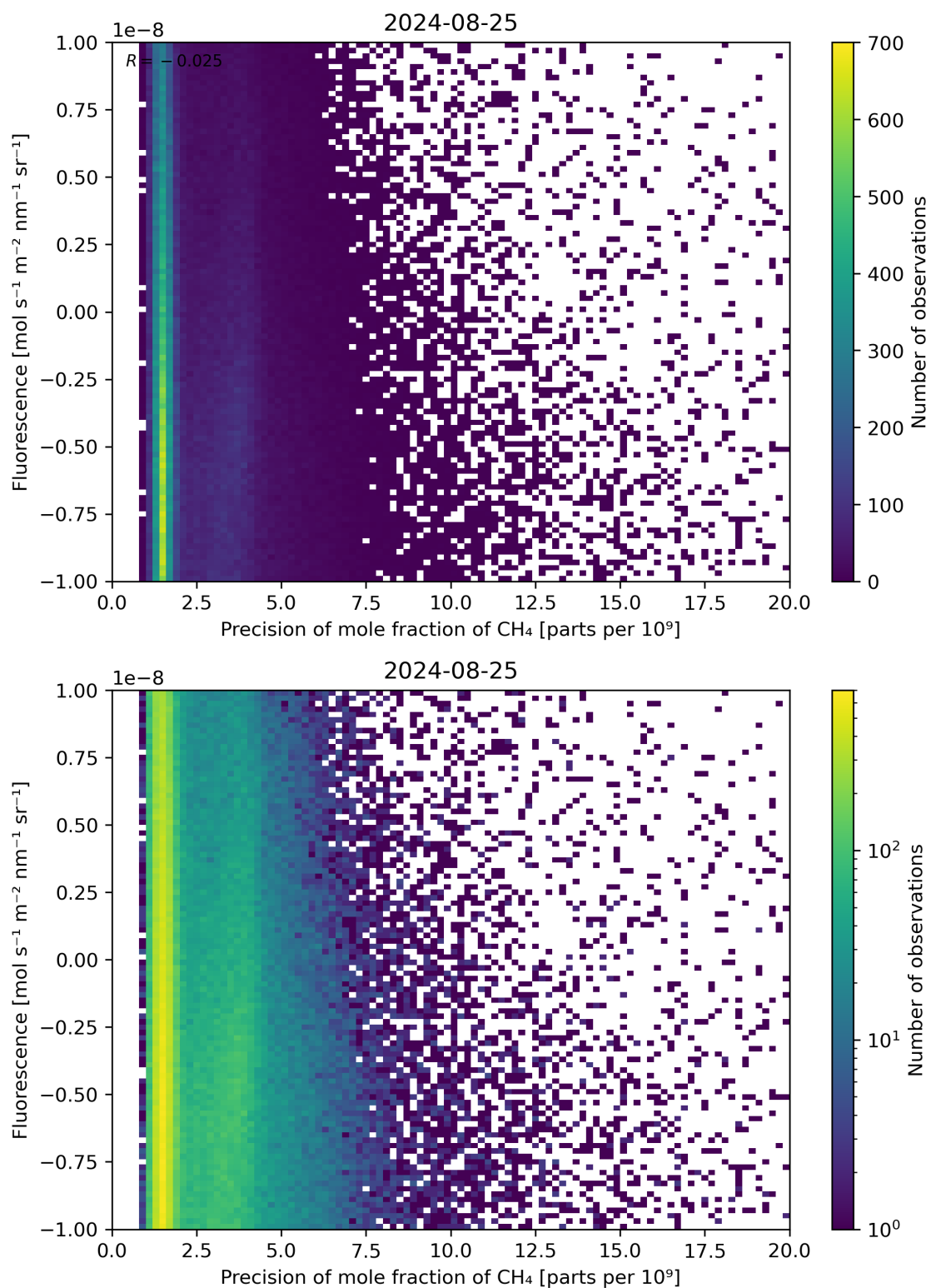
Figure 81: Scatter density plot of “Precision of mole fraction of CH 4 ” against “Fluorescence” for 2024-08-24 to 2024-08-26.
