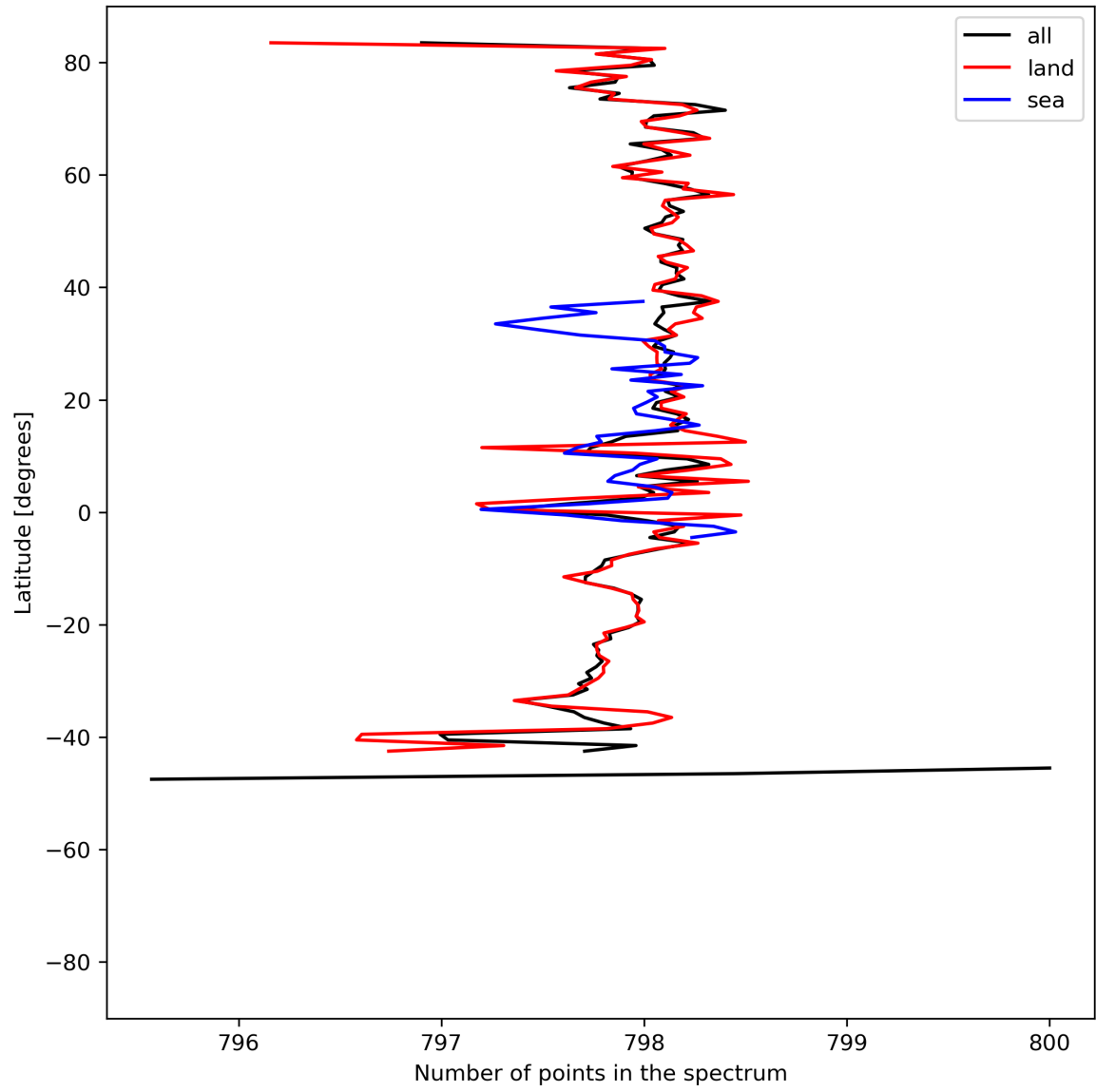
Figure 15: Zonal average of “Number of points in the spectrum” for 2024-08-24 to 2024-08-26.
