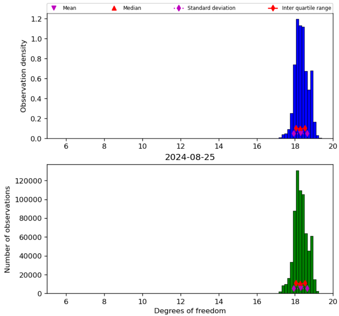
Figure 30: Histogram of “Degrees of freedom” for 2024-08-24 to 2024-08-26
