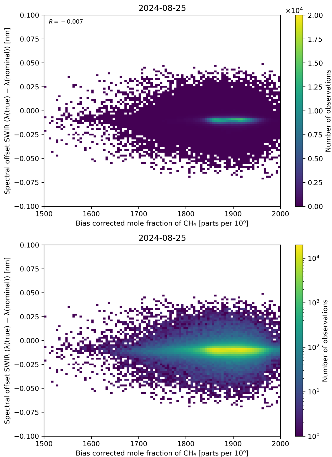
Figure 69: Scatter density plot of “Bias corrected mole fraction of \text{CH}_4 ” against “Spectral offset SWIR ( \lambda(\text{true}) - \lambda(\text{nominal}) )” for 2024-08-24 to 2024-08-26.
