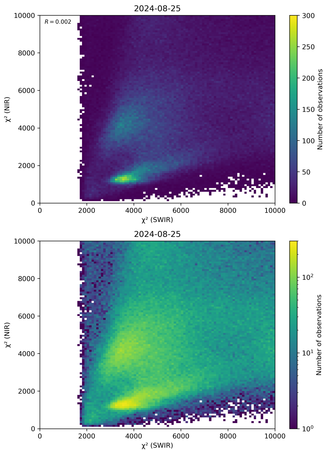
Figure 47: Scatter density plot of “ \chi^2 (SWIR)” against “ \chi^2 (NIR)” for 2024-08-24 to 2024-08-26.
