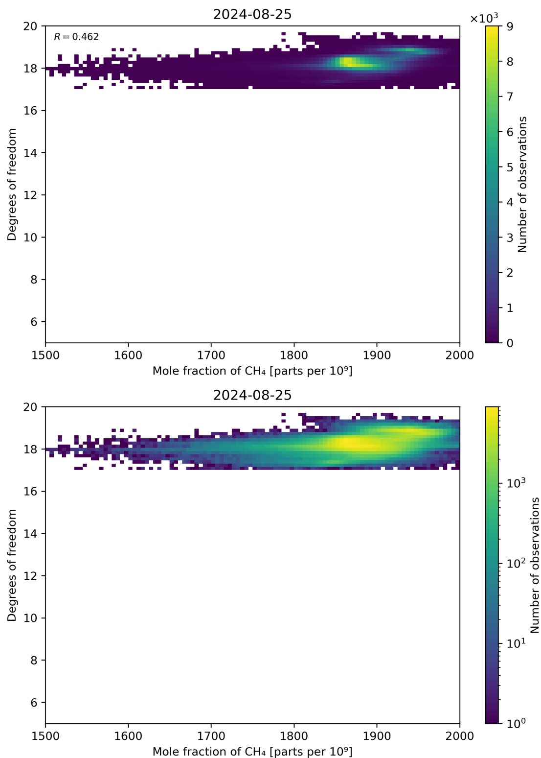
Figure 72: Scatter density plot of “Mole fraction of CH 4 ” against “Degrees of freedom” for 2024-08-24 to 2024-08-26.
