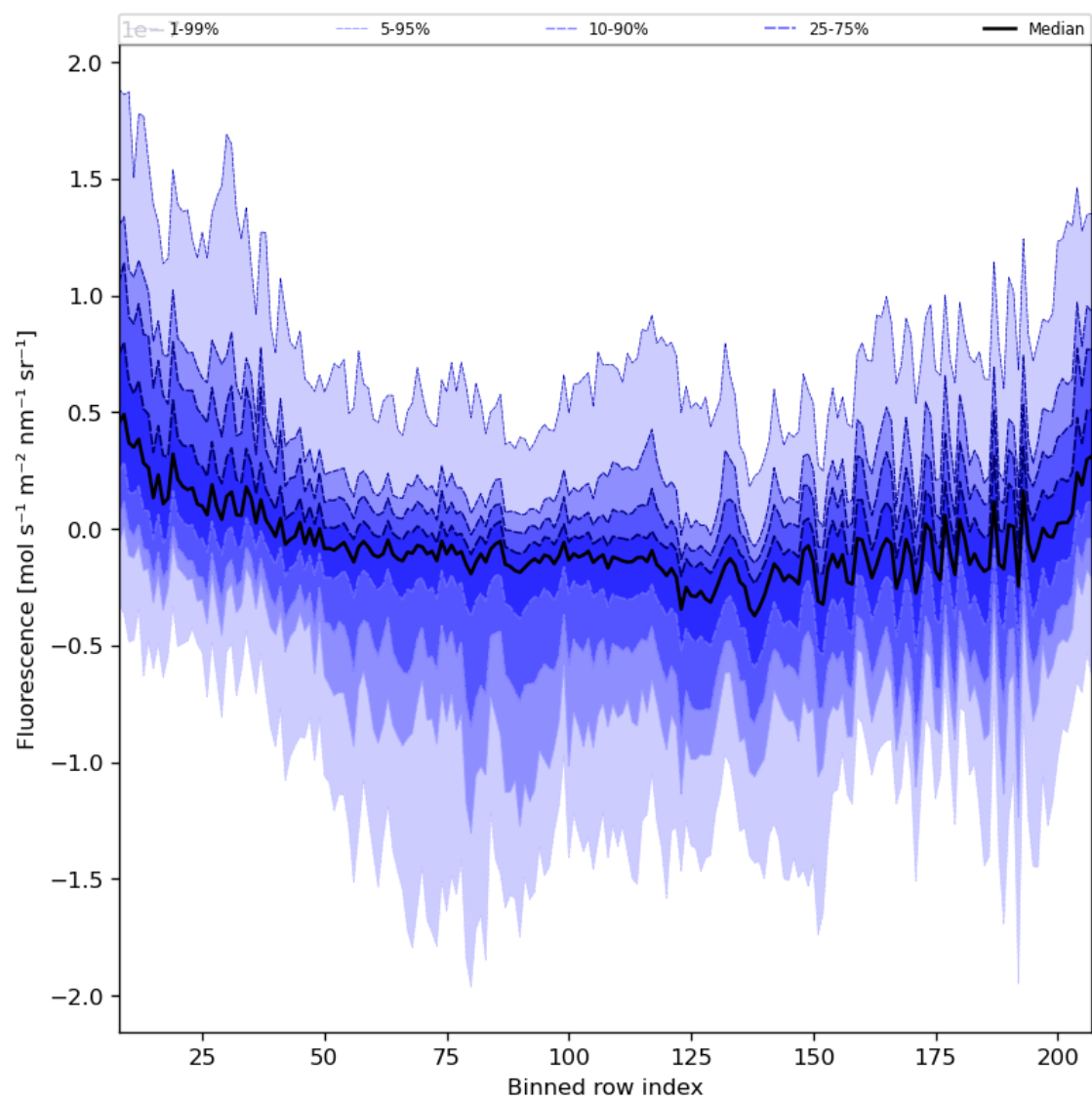
Figure 43: Along track statistics of “Fluorescence” for 2024-08-24 to 2024-08-26
