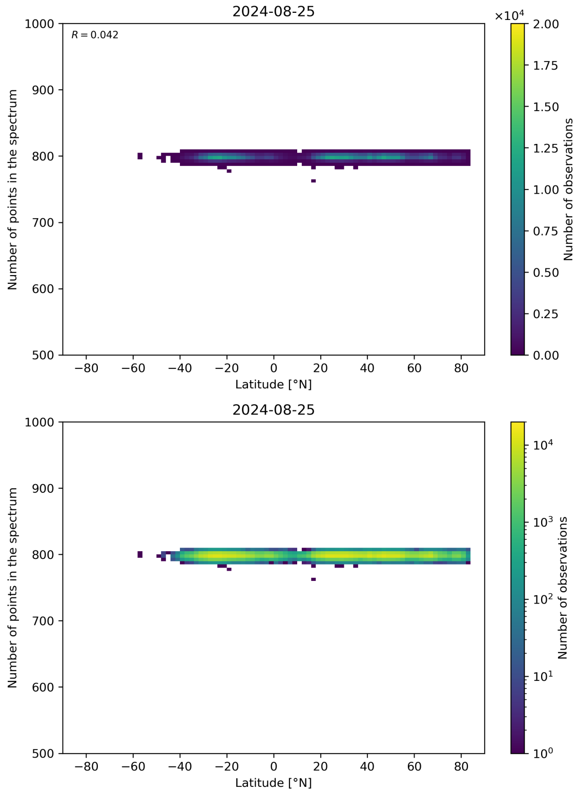
Figure 61: Scatter density plot of “Latitude” against “Number of points in the spectrum” for 2024-08-24 to 2024-08-26.
