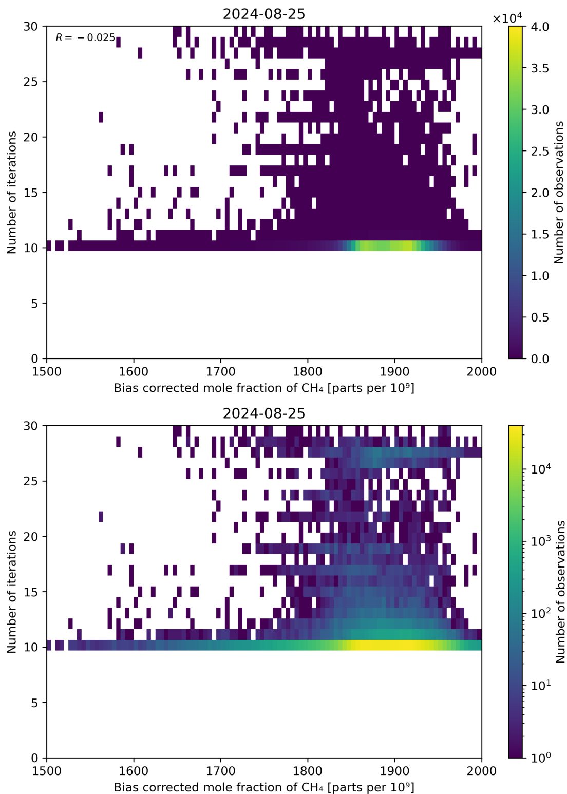
Figure 67: Scatter density plot of “Bias corrected mole fraction of CH 4 ” against “Number of iterations” for 2024-08-24 to 2024-08-26.
