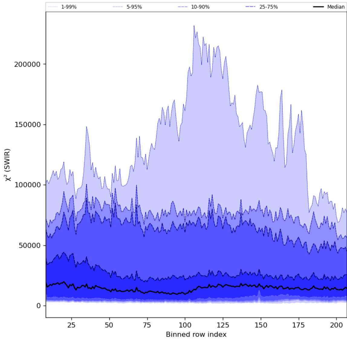
Figure 39: Along track statistics of “ \chi^2 (SWIR)” for 2024-08-24 to 2024-08-26
