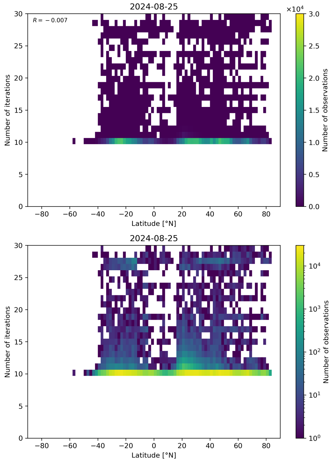
Figure 60: Scatter density plot of “Latitude” against “Number of iterations” for 2024-08-24 to 2024-08-26.
