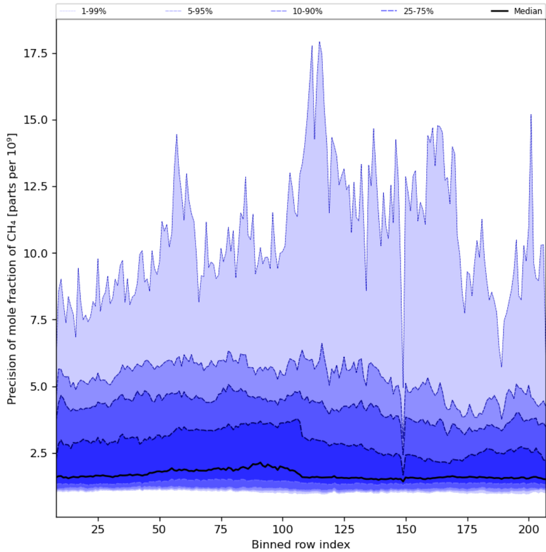
Figure 35: Along track statistics of “Precision of mole fraction of CH 4 ” for 2024-08-24 to 2024-08-26
