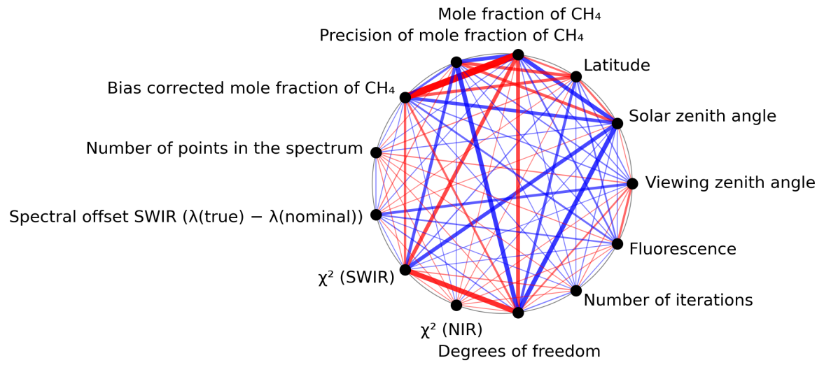
Figure 1: Map of correlation graph for 2024-08-24 to 2024-08-26.
