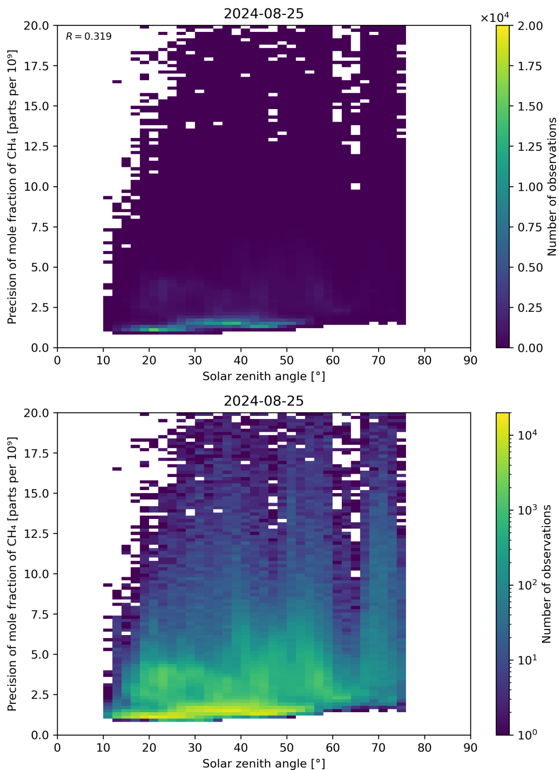
Figure 101: Scatter density plot of “Solar zenith angle” against “Precision of mole fraction of CH 4 ” for 2024-08-24 to 2024-08-26.
