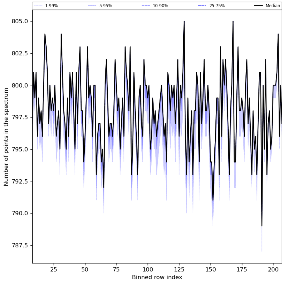
Figure 37: Along track statistics of “Number of points in the spectrum” for 2024-08-24 to 2024-08-26
