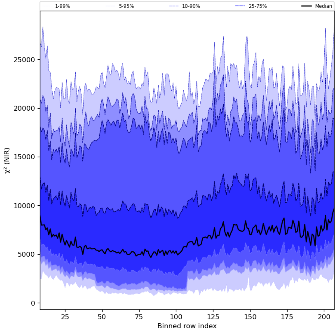
Figure 40: Along track statistics of “ \chi^2 (NIR)” for 2024-08-24 to 2024-08-26
