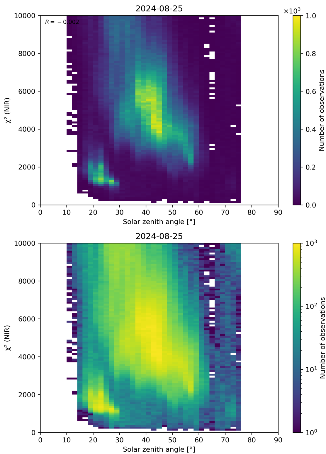
Figure 94: Scatter density plot of “Solar zenith angle” against “ \chi^2 (NIR)” for 2024-08-24 to 2024-08-26.
