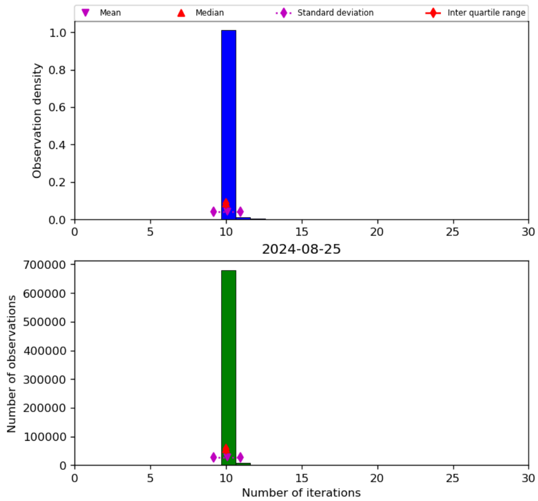
Figure 31: Histogram of “Number of iterations” for 2024-08-24 to 2024-08-26
