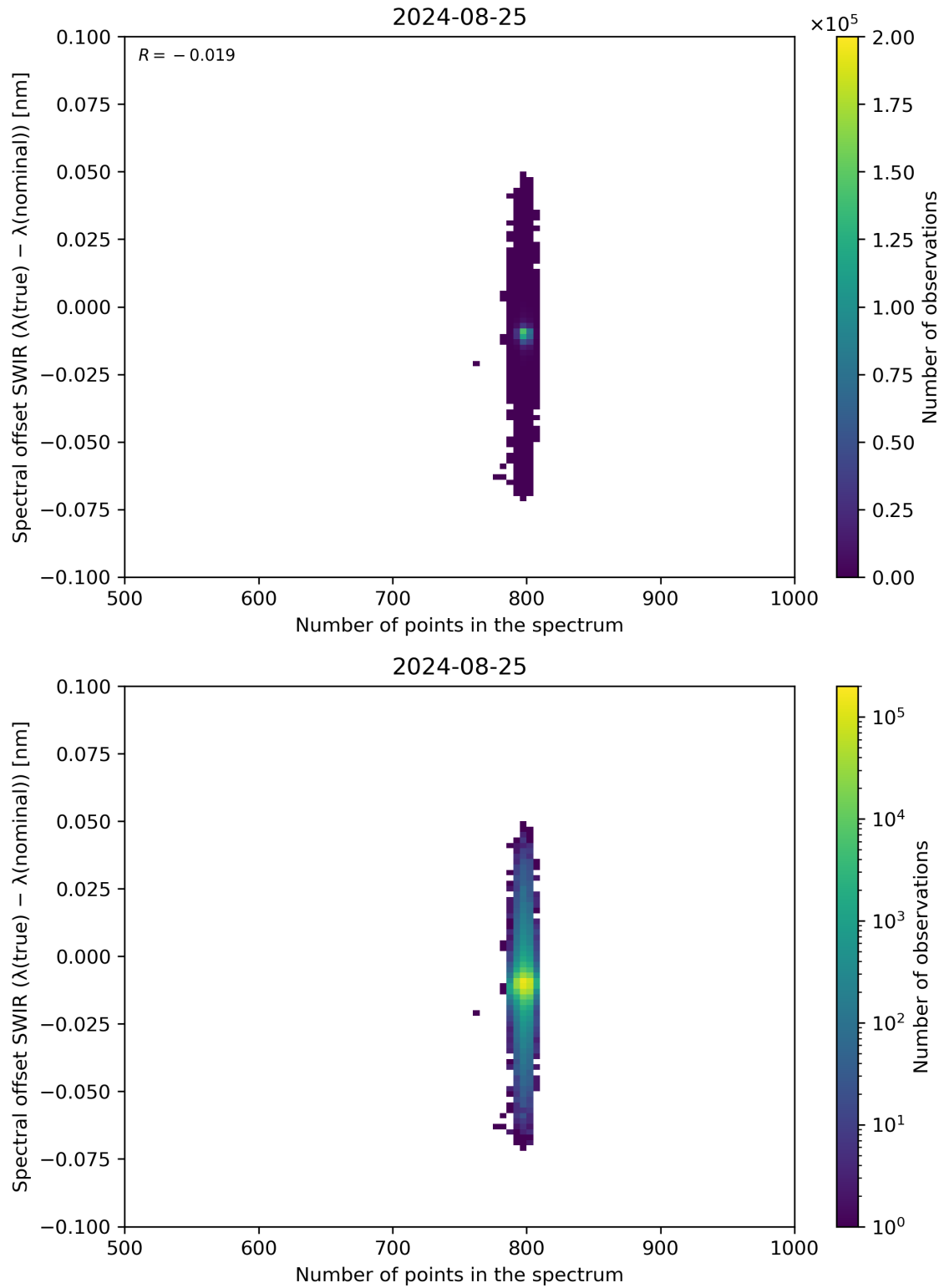
Figure 93: Scatter density plot of “Number of points in the spectrum” against “Spectral offset SWIR ( \lambda(\text{true}) - \lambda(\text{nominal}) )” for 2024-08-24 to 2024-08-26.
