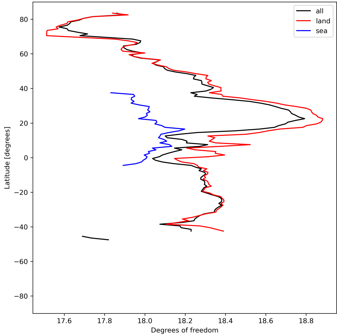
Figure 19: Zonal average of “Degrees of freedom” for 2024-08-24 to 2024-08-26.
