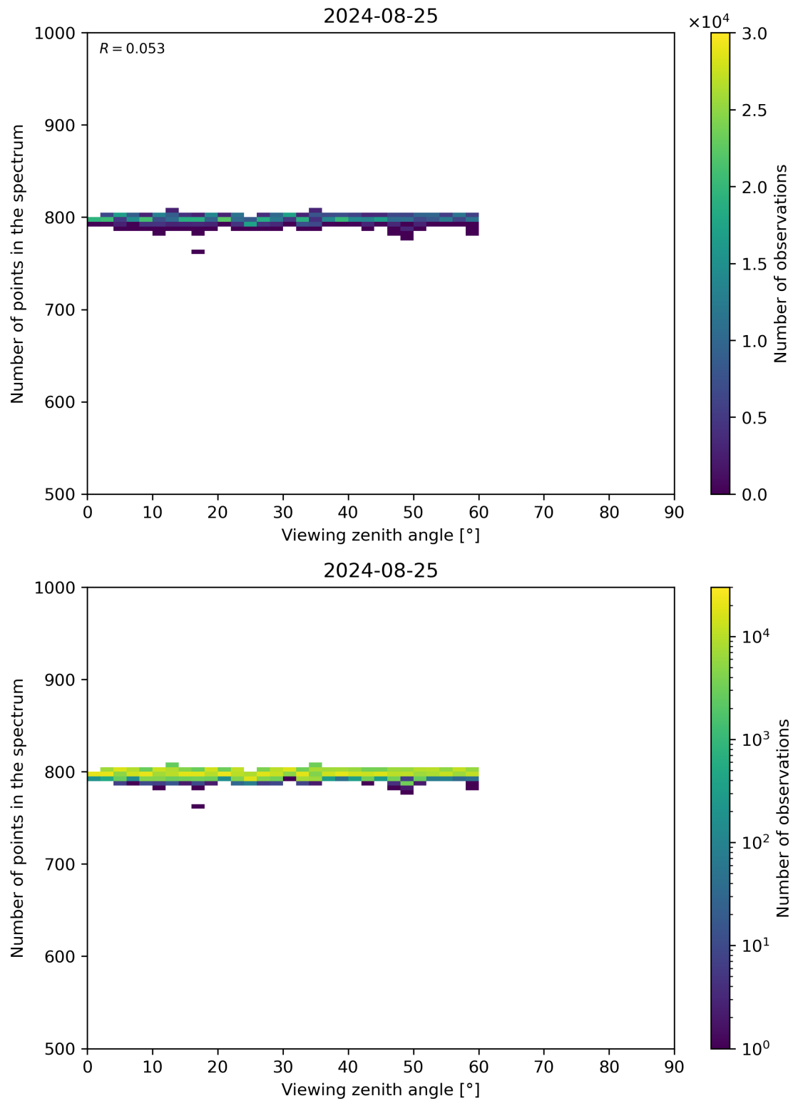
Figure 114: Scatter density plot of “Viewing zenith angle” against “Number of points in the spectrum” for 2024-08-24 to 2024-08-26.
