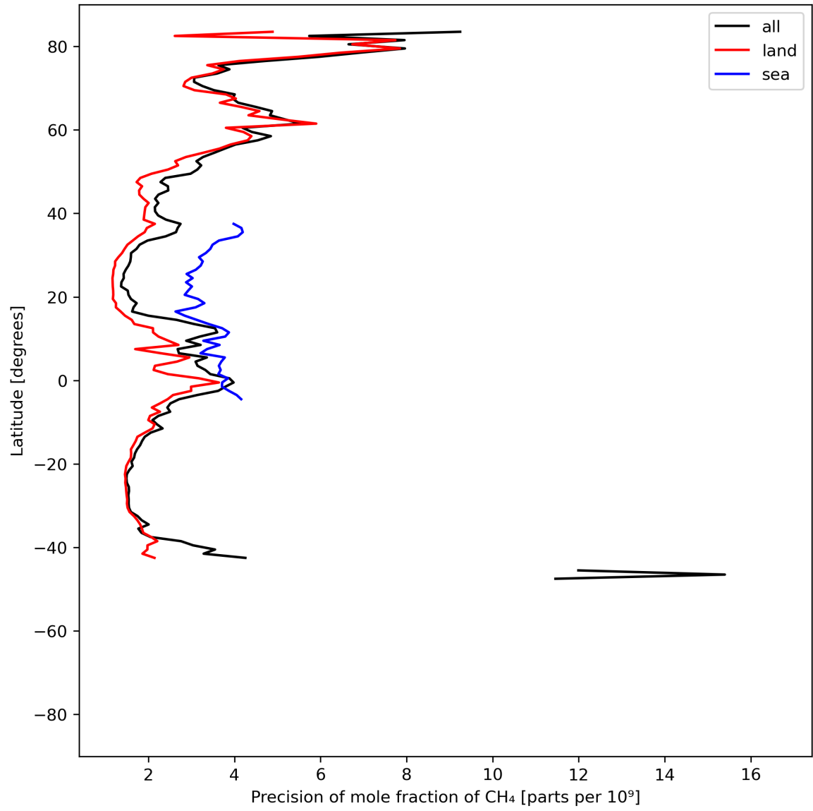
Figure 13: Zonal average of “Precision of mole fraction of CH 4 ” for 2024-08-24 to 2024-08-26.
