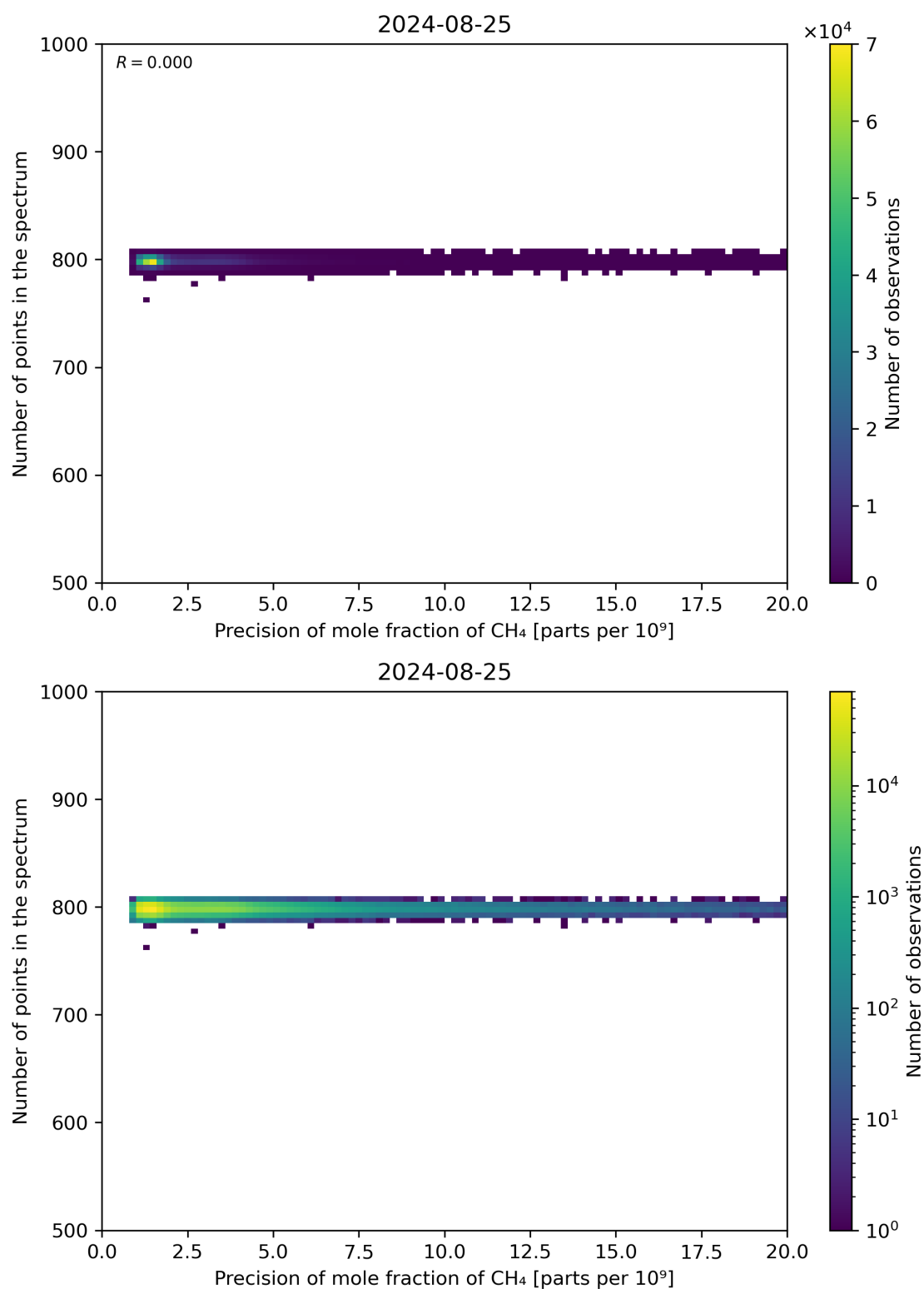
Figure 84: Scatter density plot of “Precision of mole fraction of CH 4 ” against “Number of points in the spectrum” for 2024-08-24 to 2024-08-26.
