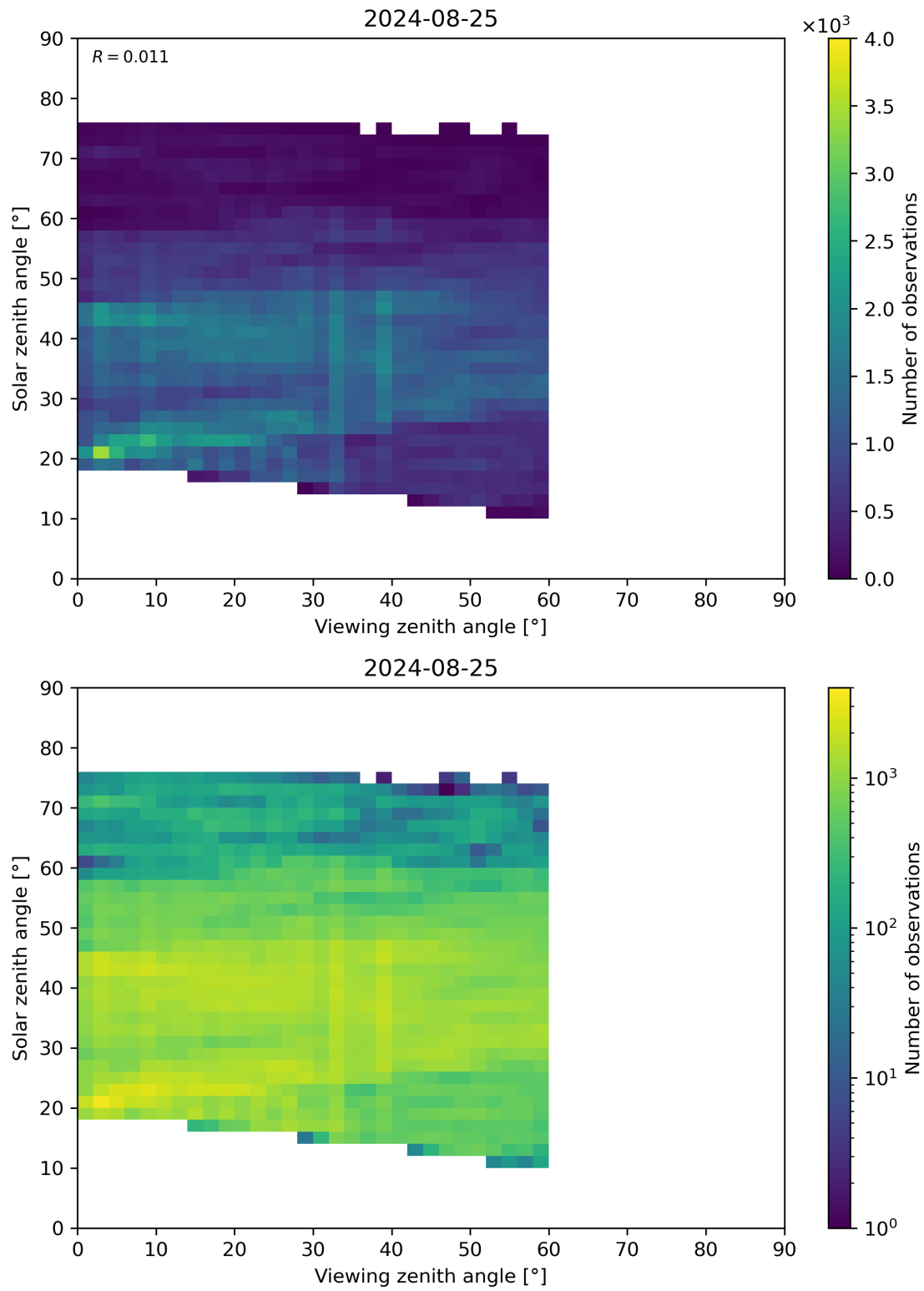
Figure 115: Scatter density plot of “Viewing zenith angle” against “Solar zenith angle” for 2024-08-24 to 2024-08-26.
