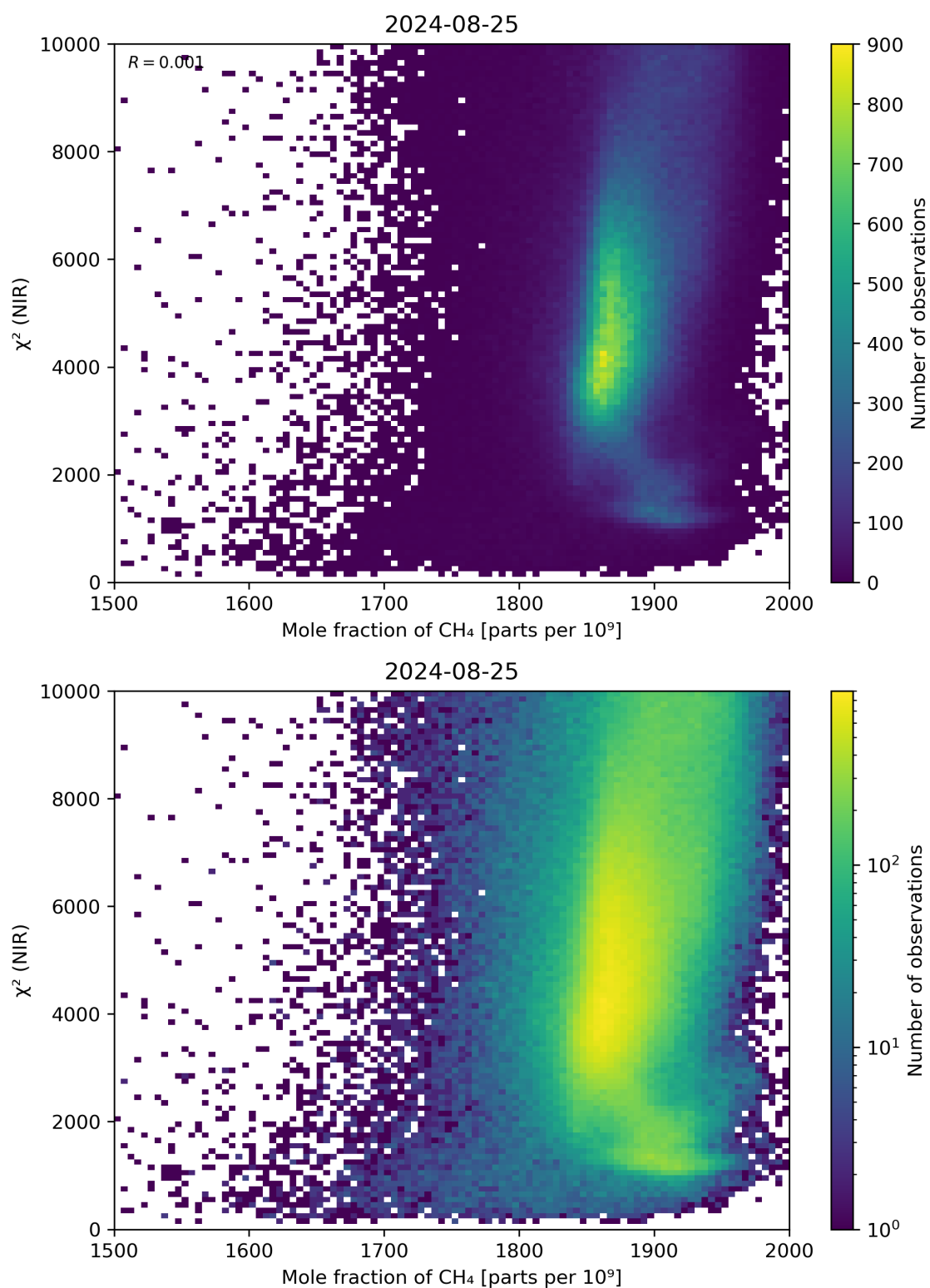
Figure 70: Scatter density plot of “Mole fraction of CH 4 ” against “ \chi^2 (NIR)” for 2024-08-24 to 2024-08-26.
