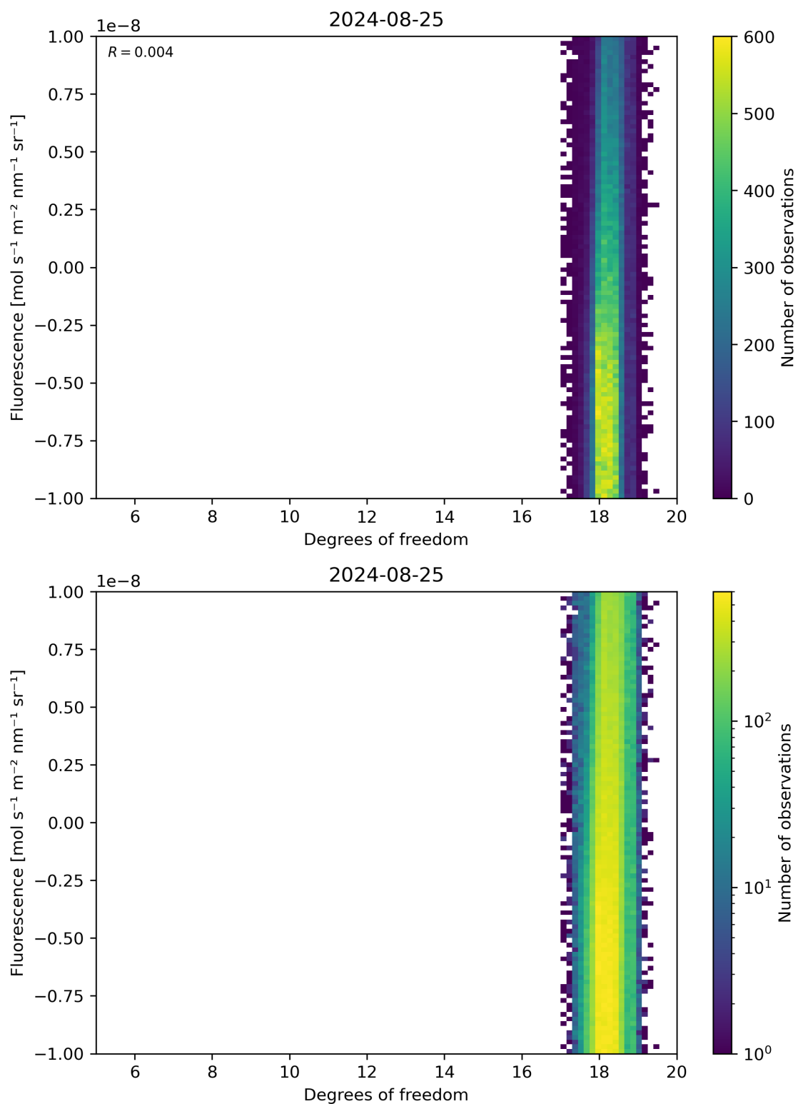
Figure 51: Scatter density plot of “Degrees of freedom” against “Fluorescence” for 2024-08-24 to 2024-08-26.
