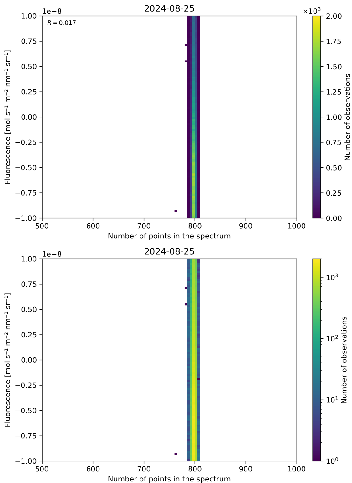
Figure 91: Scatter density plot of “Number of points in the spectrum” against “Fluorescence” for 2024-08-24 to 2024-08-26.
