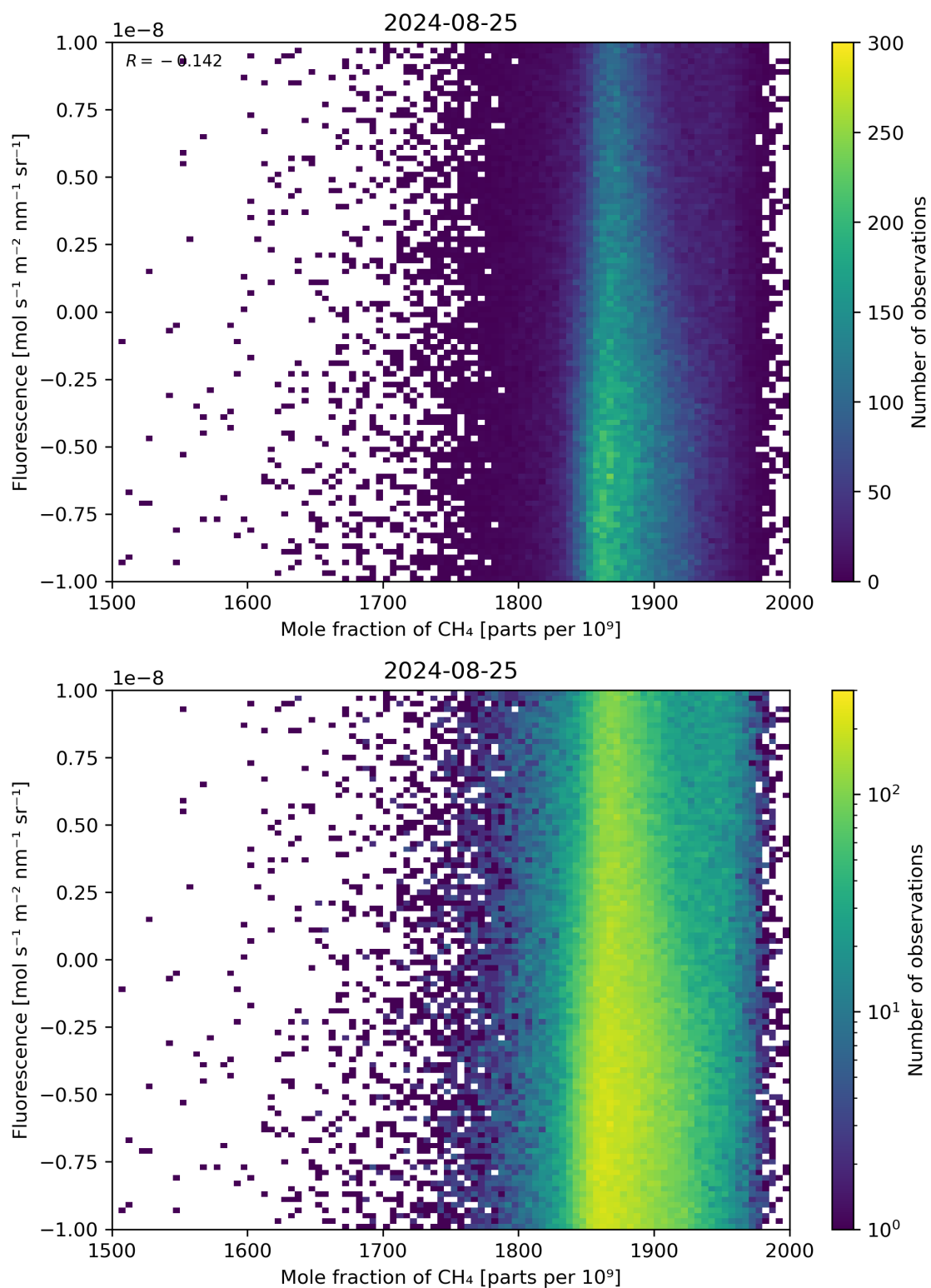
Figure 73: Scatter density plot of “Mole fraction of \text{CH}_4 ” against “Fluorescence” for 2024-08-24 to 2024-08-26.
