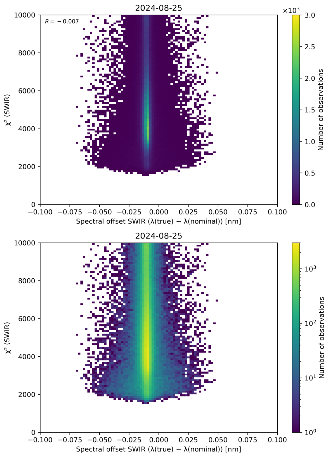
Figure 118: Scatter density plot of “Spectral offset SWIR ( \lambda(\text{true}) - \lambda(\text{nominal}) )” against “ \chi^2 (SWIR)” for 2024-08-24 to 2024-08-26.
