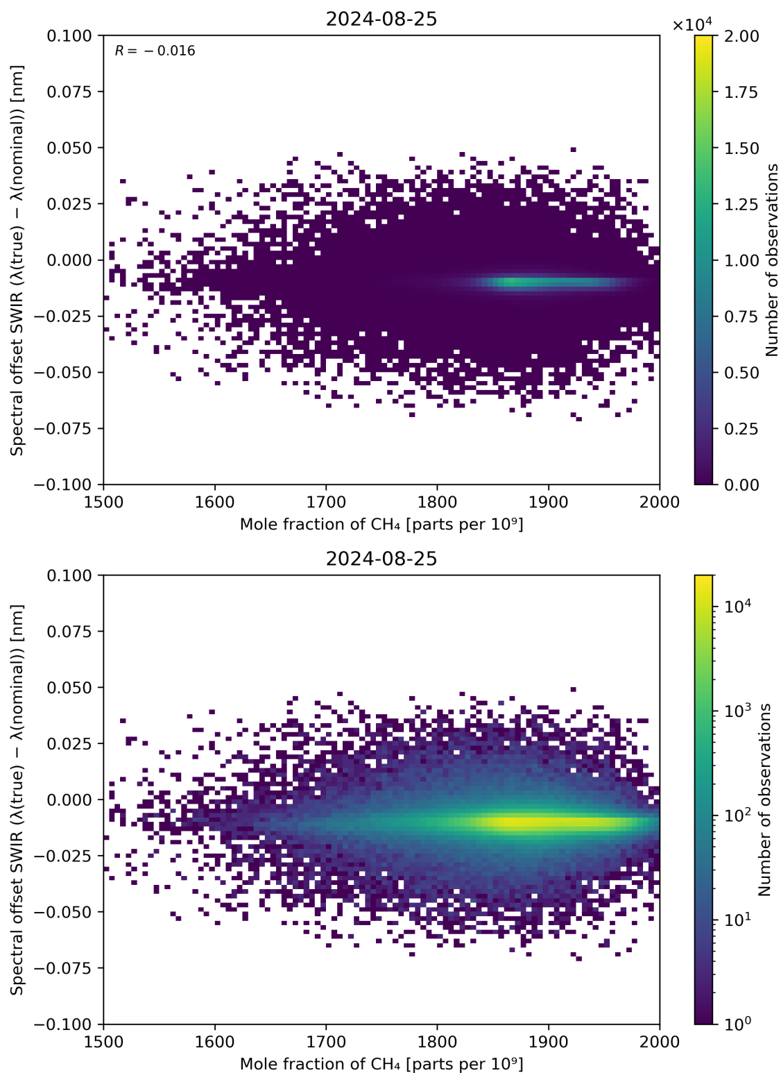
Figure 86: Scatter density plot of “Mole fraction of CH 4 ” against “Spectral offset SWIR ( \lambda(\text{true}) - \lambda(\text{nominal}) )” for 2024-08-24 to 2024-08-26.
