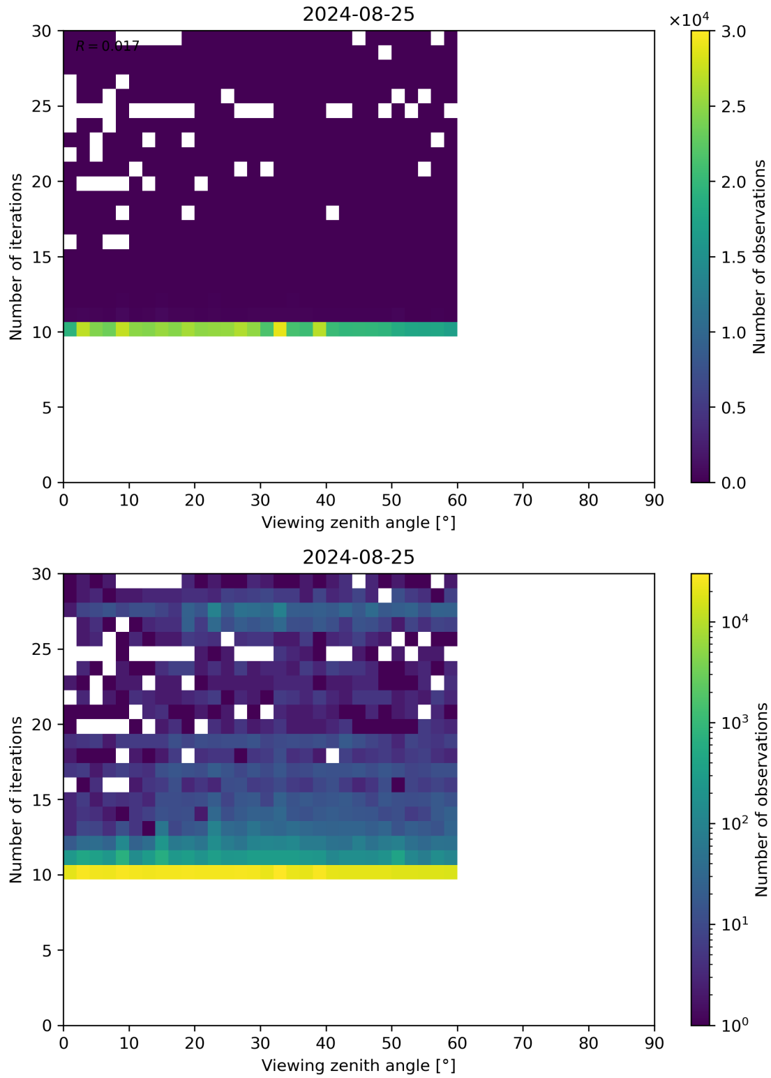
Figure 113: Scatter density plot of “Viewing zenith angle” against “Number of iterations” for 2024-08-24 to 2024-08-26.
