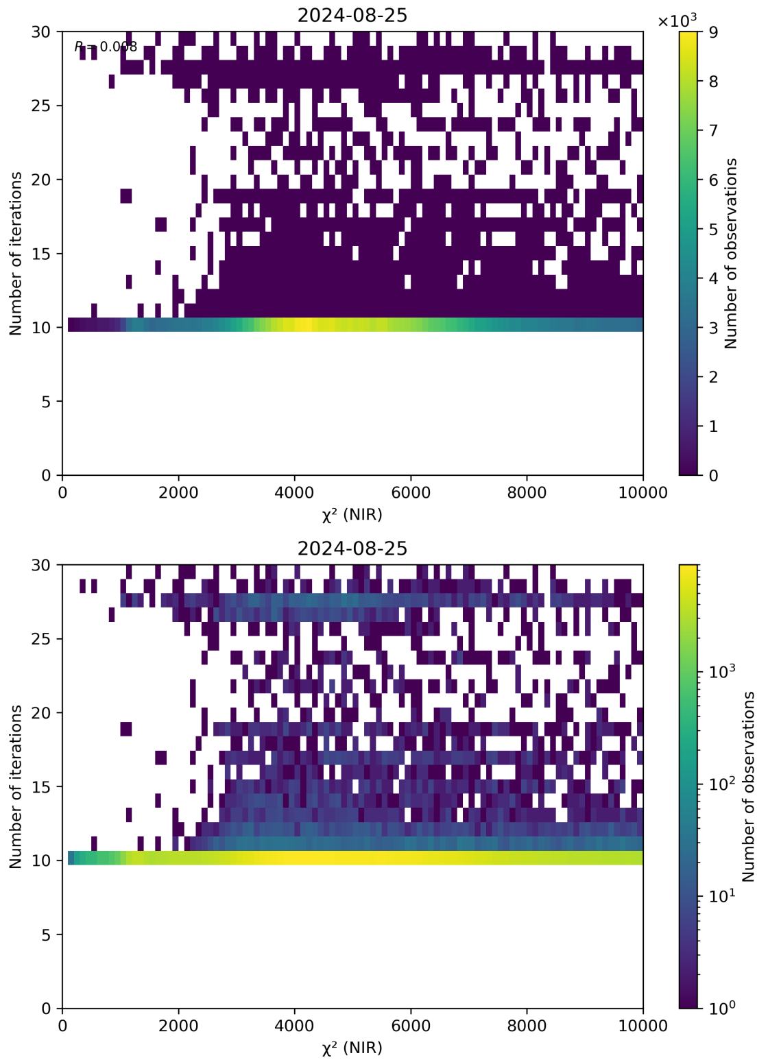
Figure 46: Scatter density plot of “ \chi^2 (NIR)” against “Number of iterations” for 2024-08-24 to 2024-08-26.
