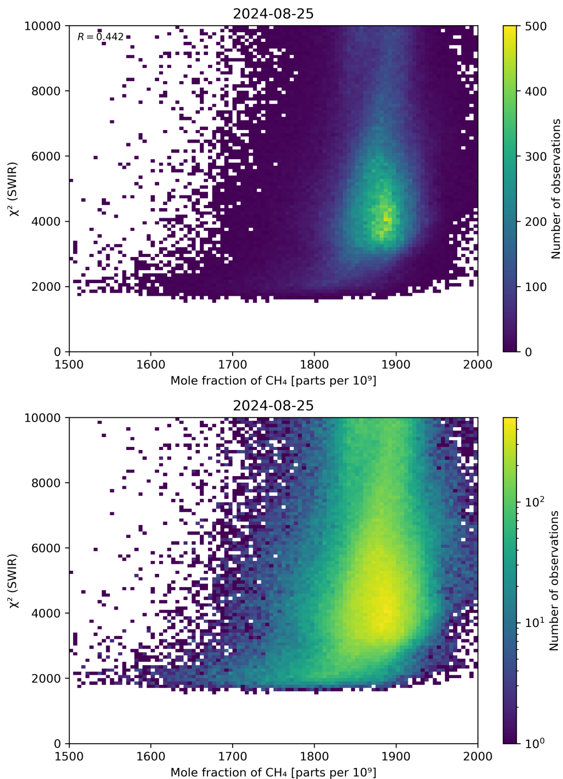
Figure 71: Scatter density plot of “Mole fraction of \text{CH}_4 ” against “ \chi^2 (SWIR)” for 2024-08-24 to 2024-08-26.
