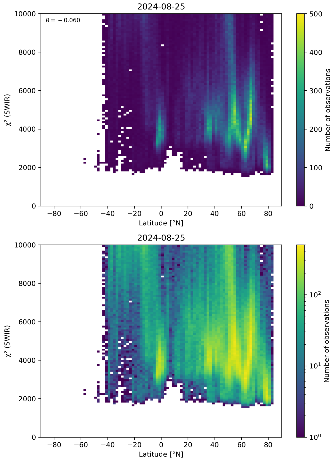
Figure 54: Scatter density plot of “Latitude” against “ \chi^2 (SWIR)” for 2024-08-24 to 2024-08-26.
