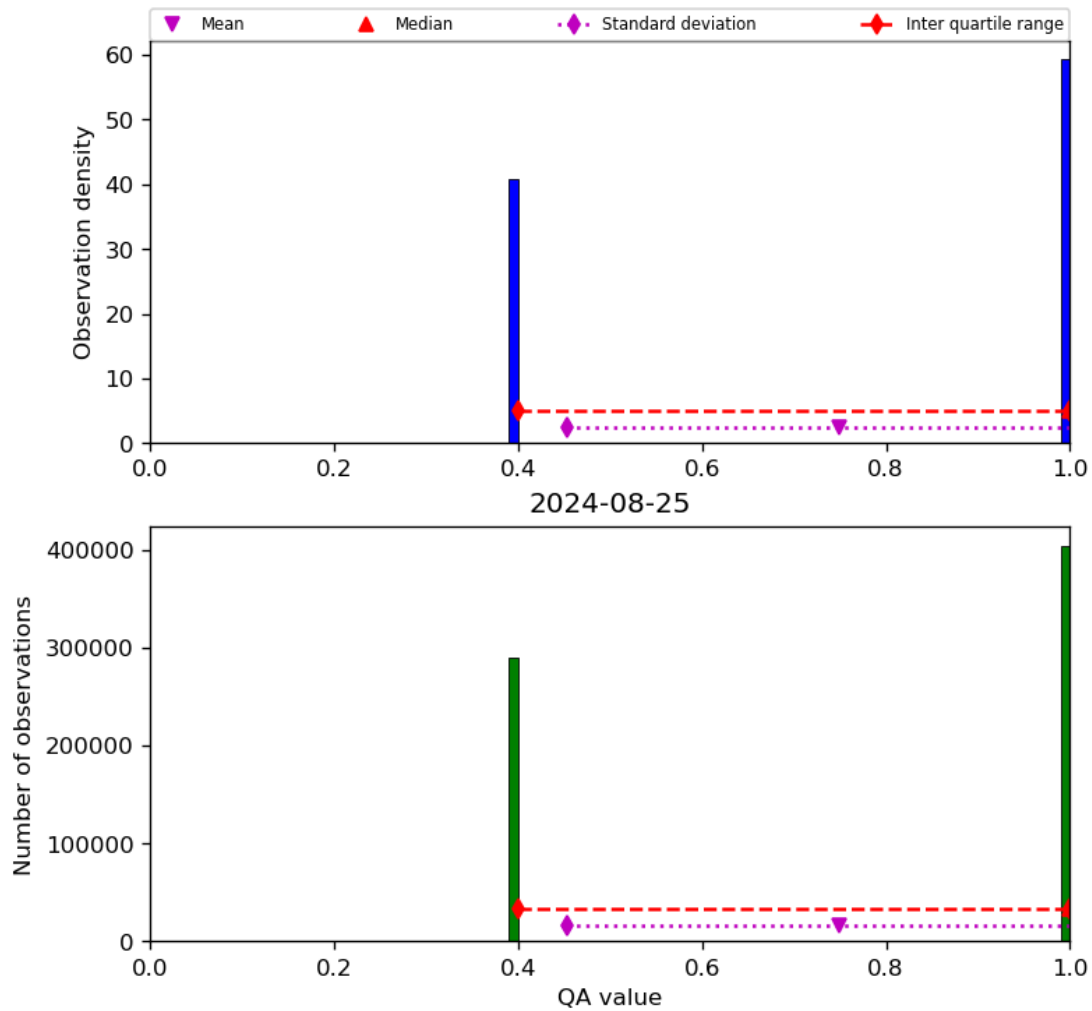
Figure 22: Histogram of “QA value” for 2024-08-24 to 2024-08-26
