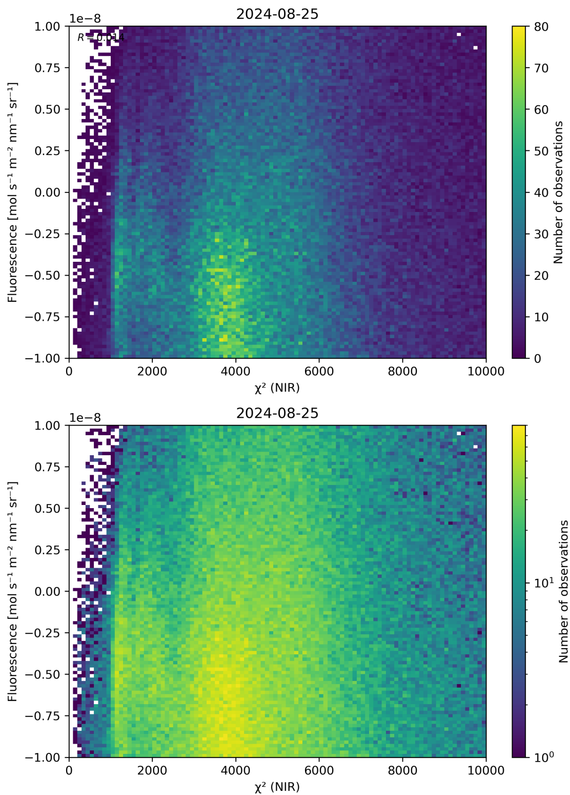
Figure 45: Scatter density plot of “ \chi^2 (NIR)” against “Fluorescence” for 2024-08-24 to 2024-08-26.
