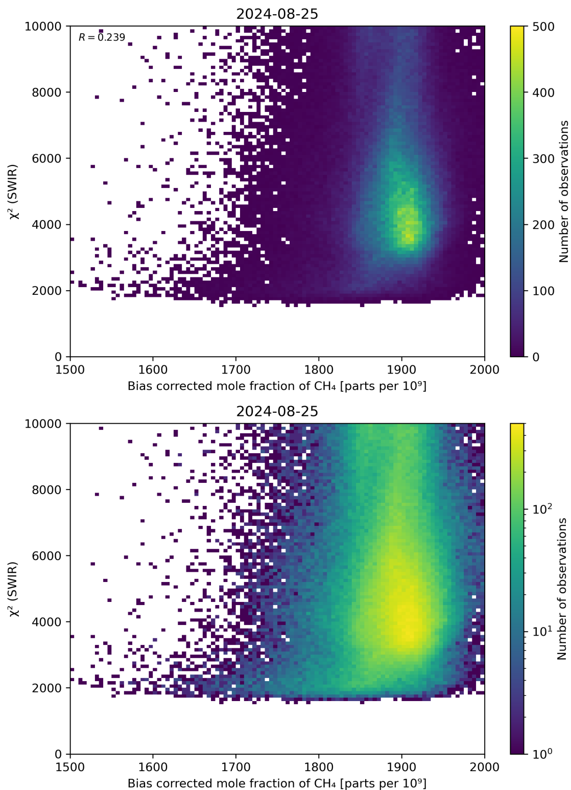
Figure 64: Scatter density plot of “Bias corrected mole fraction of CH 4 ” against “ \chi^2 (SWIR)” for 2024-08-24 to 2024-08-26.
