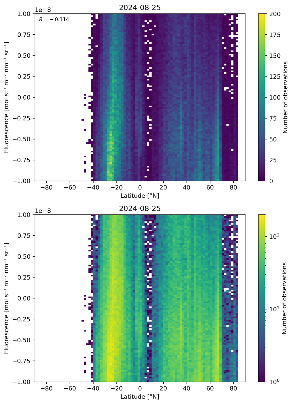
Figure 56: Scatter density plot of “Latitude” against “Fluorescence” for 2024-08-24 to 2024-08-26.
