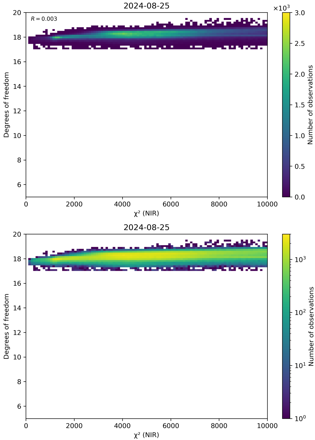
Figure 44: Scatter density plot of “ \chi^2 (NIR)” against “Degrees of freedom” for 2024-08-24 to 2024-08-26.
