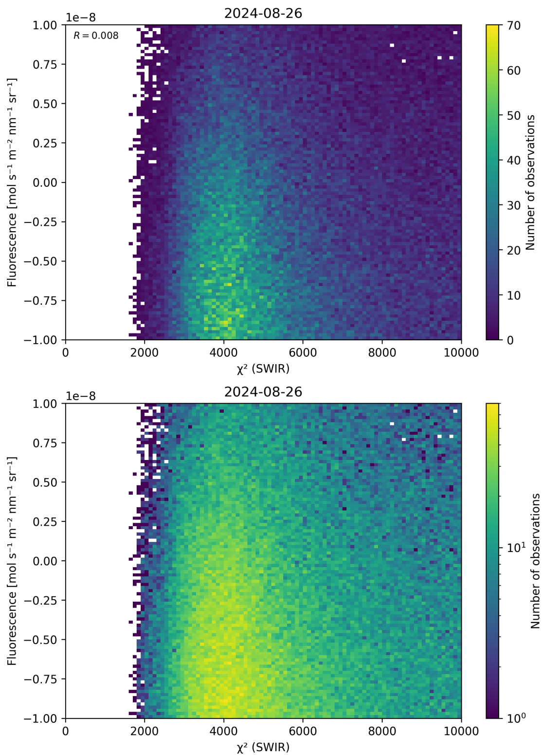
Figure 49: Scatter density plot of “ \chi^2 (SWIR)” against “Fluorescence” for 2024-08-25 to 2024-08-27.
