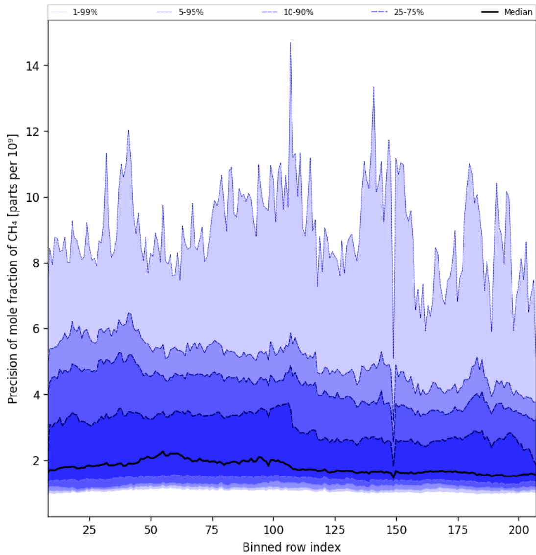
Figure 35: Along track statistics of “Precision of mole fraction of CH 4 ” for 2024-08-25 to 2024-08-27
