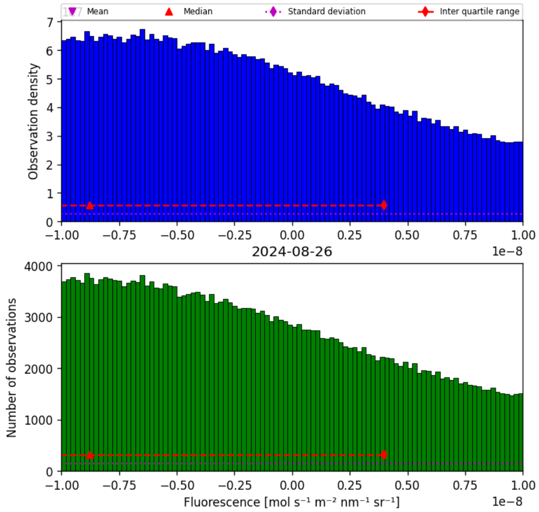
Figure 32: Histogram of “Fluorescence” for 2024-08-25 to 2024-08-27
