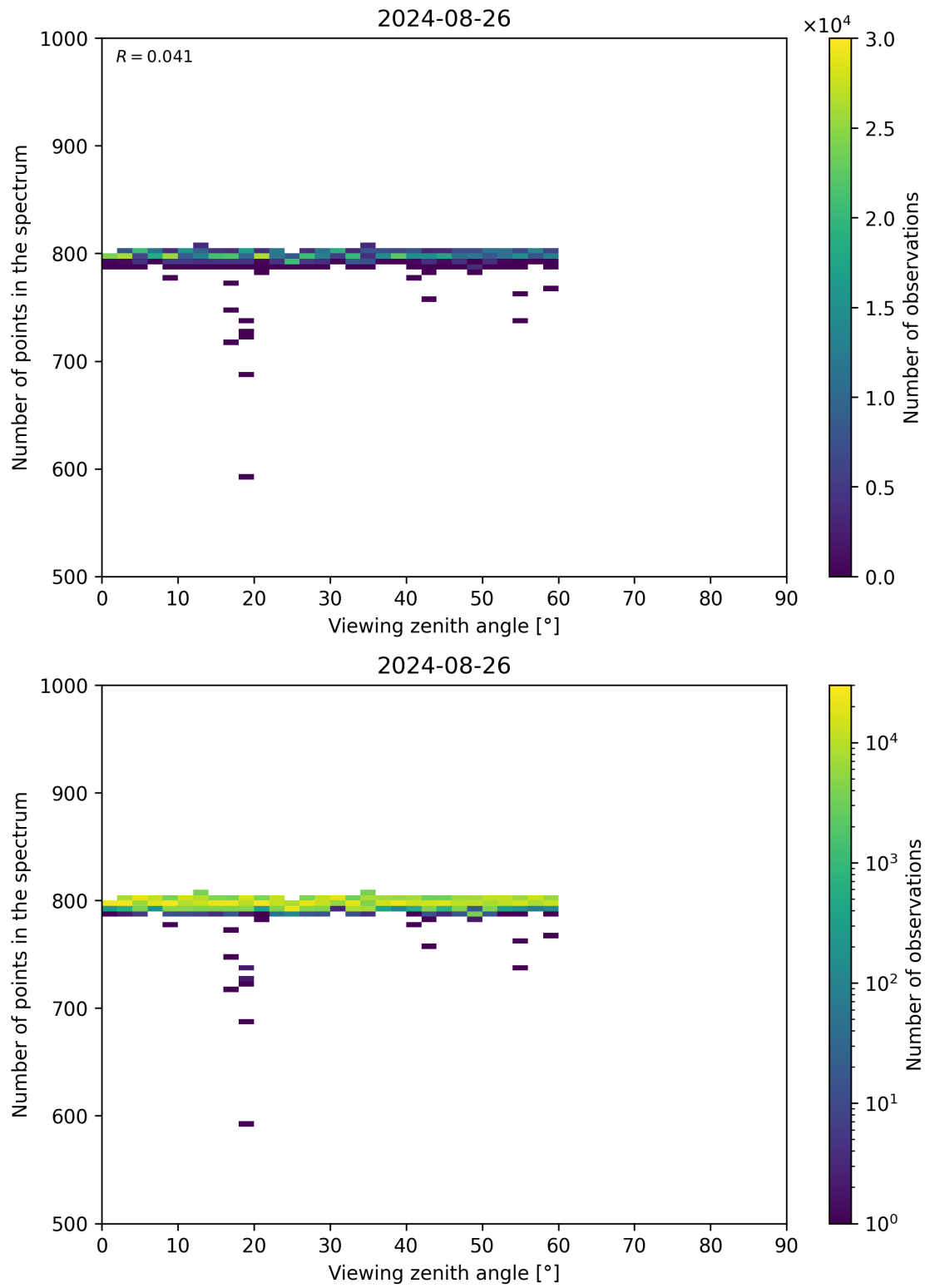
Figure 114: Scatter density plot of “Viewing zenith angle” against “Number of points in the spectrum” for 2024-08-25 to 2024-08-27.
