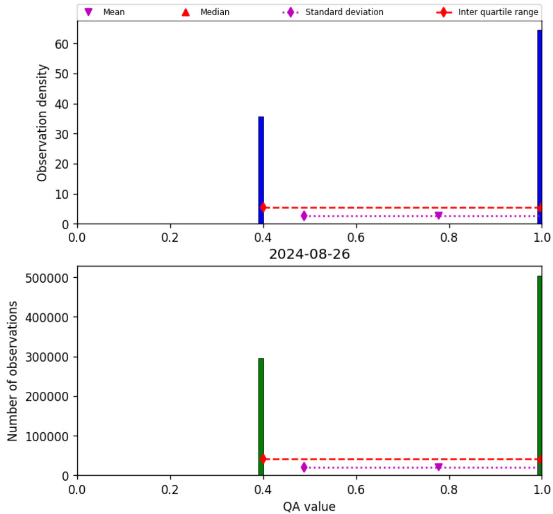
Figure 22: Histogram of “QA value” for 2024-08-25 to 2024-08-27
