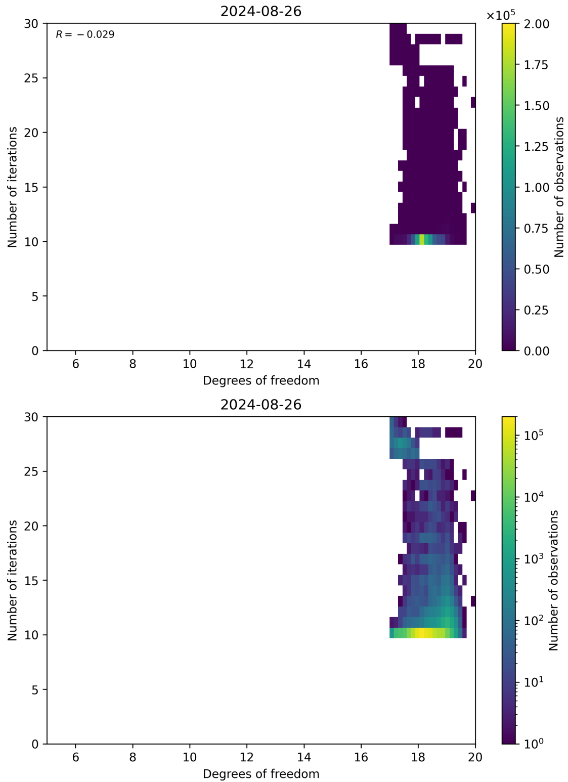
Figure 52: Scatter density plot of “Degrees of freedom” against “Number of iterations” for 2024-08-25 to 2024-08-27.
