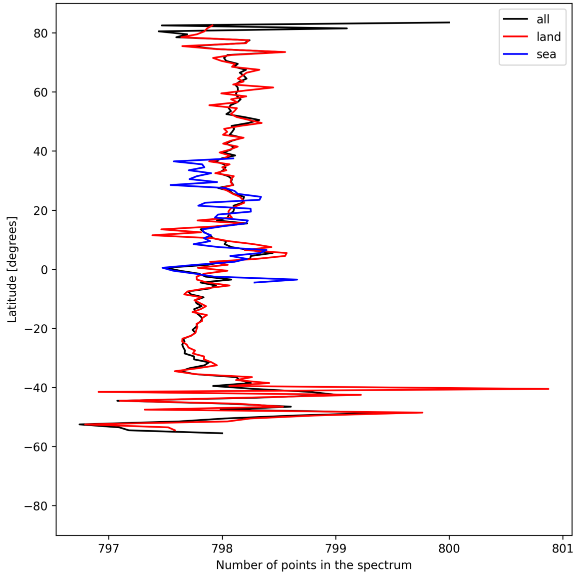
Figure 15: Zonal average of “Number of points in the spectrum” for 2024-08-25 to 2024-08-27.
