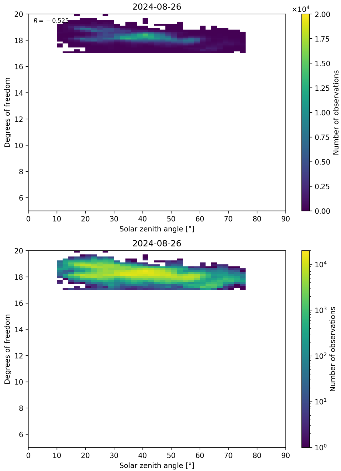
Figure 96: Scatter density plot of “Solar zenith angle” against “Degrees of freedom” for 2024-08-25 to 2024-08-27.
