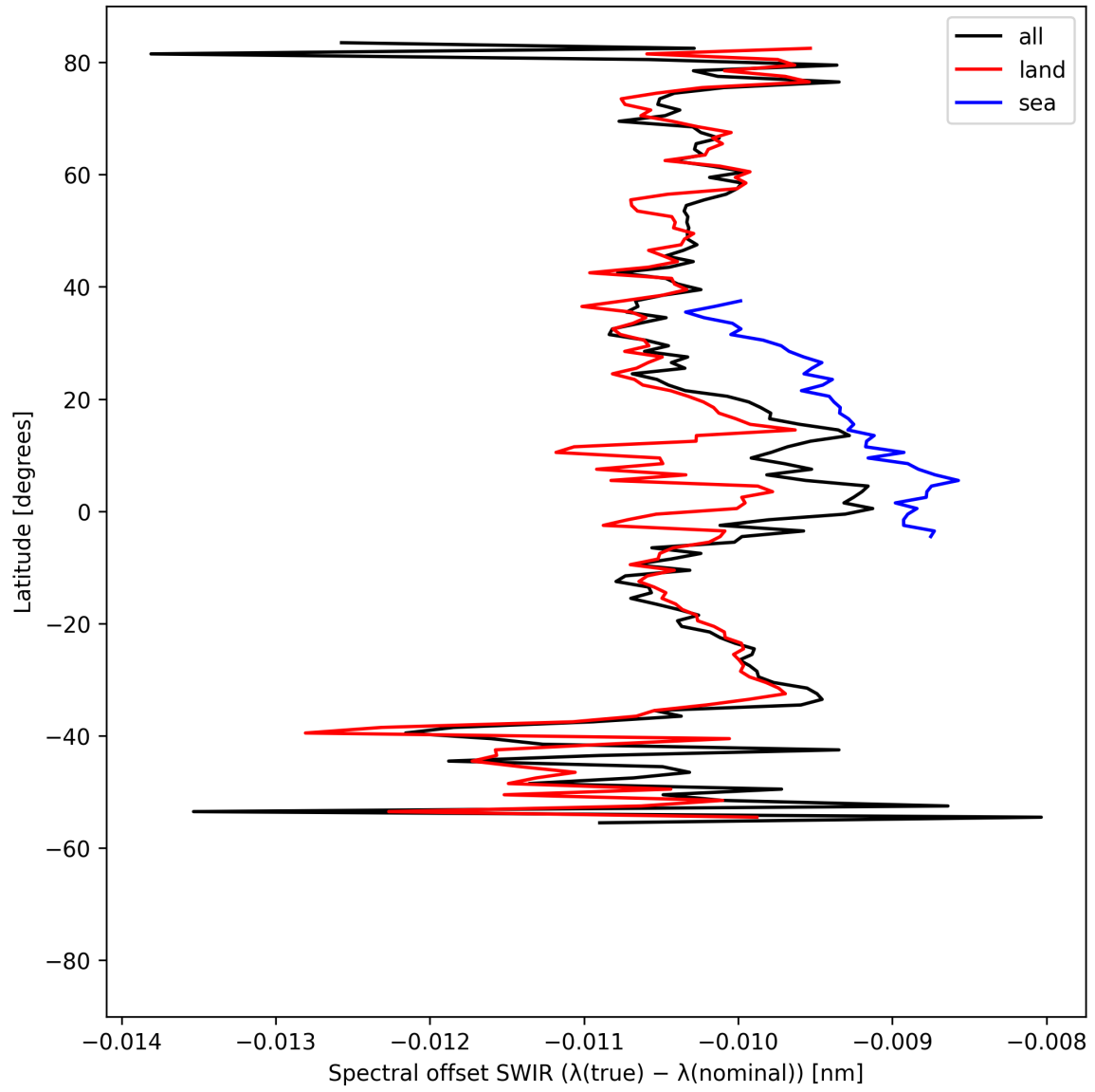
Figure 16: Zonal average of “Spectral offset SWIR ( \lambda_{\text{true}} - \lambda_{\text{nominal}} )” for 2024-08-25 to 2024-08-27.
