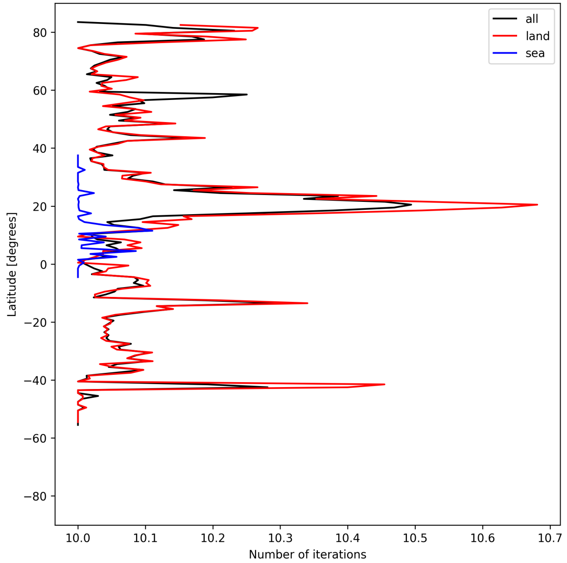
Figure 20: Zonal average of “Number of iterations” for 2024-08-25 to 2024-08-27.
