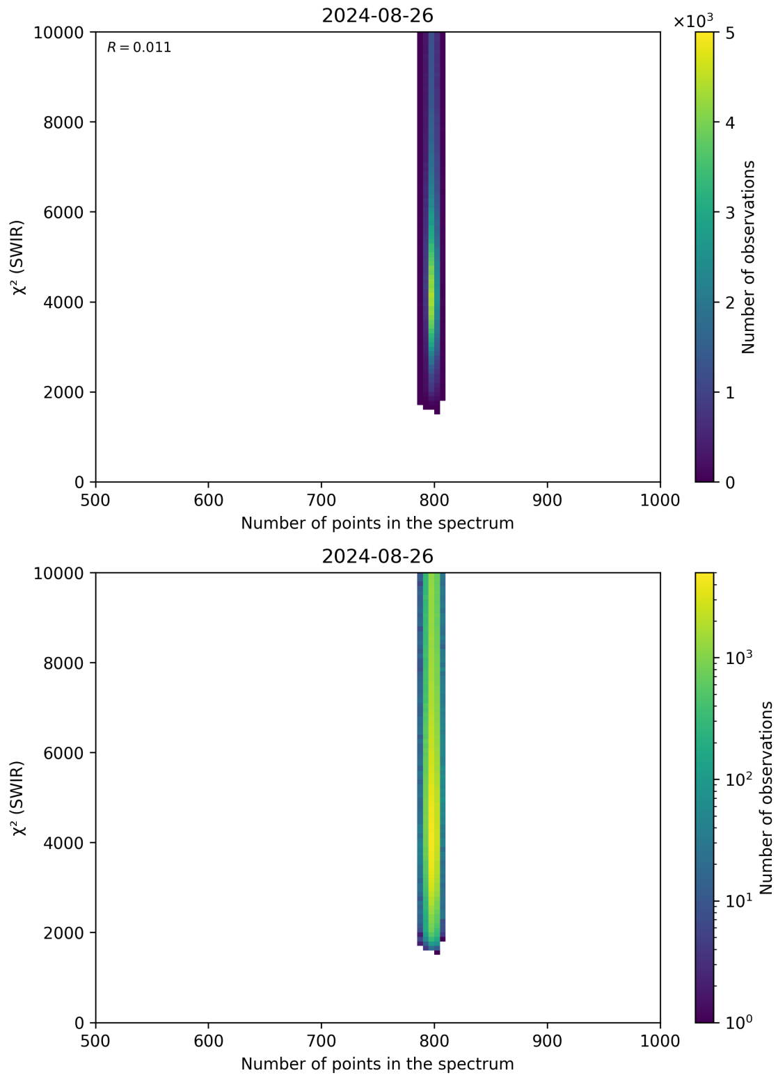
Figure 89: Scatter density plot of “Number of points in the spectrum” against “ \chi^2 (SWIR)” for 2024-08-25 to 2024-08-27.
