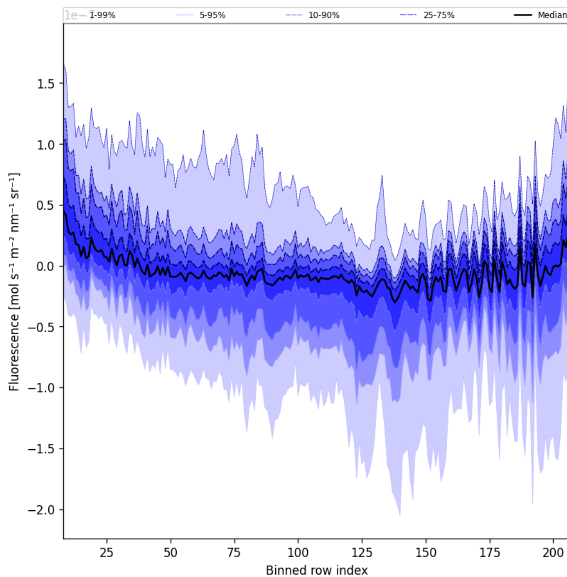
Figure 43: Along track statistics of “Fluorescence” for 2024-08-25 to 2024-08-27
