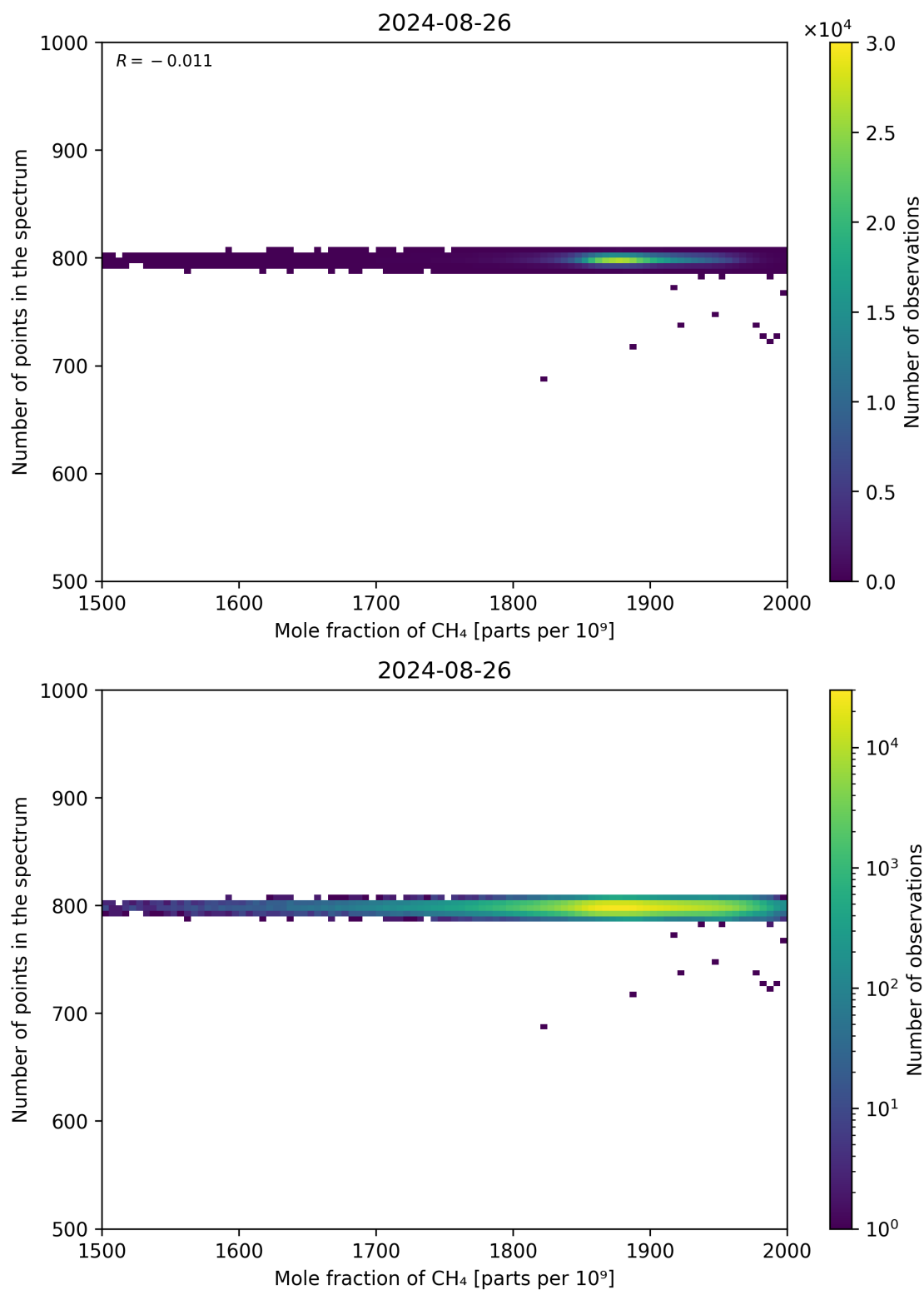
Figure 77: Scatter density plot of “Mole fraction of CH 4 ” against “Number of points in the spectrum” for 2024-08-25 to 2024-08-27.
