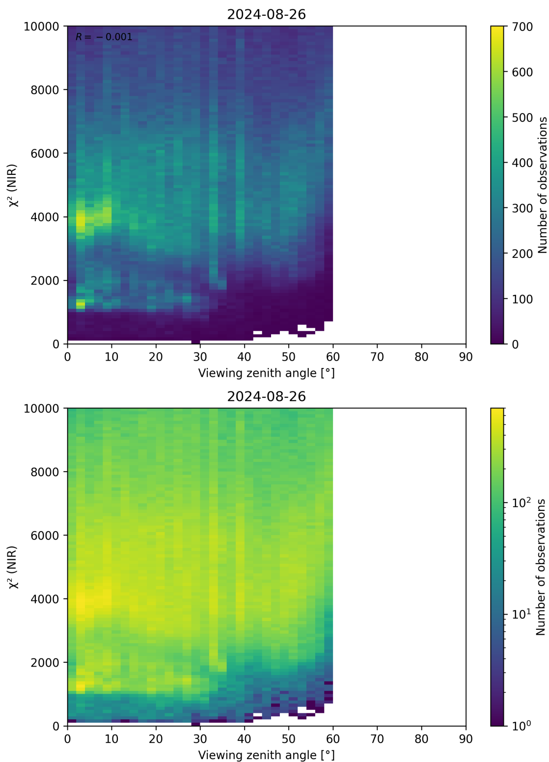
Figure 105: Scatter density plot of “Viewing zenith angle” against “ \chi^2 (NIR)” for 2024-08-25 to 2024-08-27.
