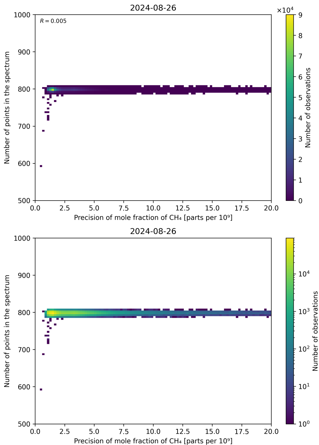
Figure 84: Scatter density plot of “Precision of mole fraction of CH 4 ” against “Number of points in the spectrum” for 2024-08-25 to 2024-08-27.
