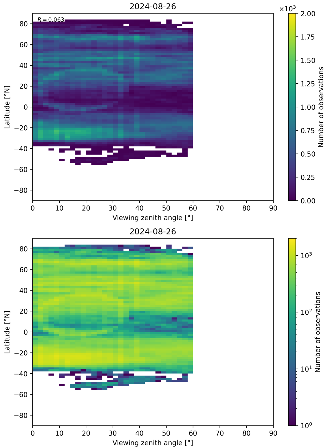
Figure 109: Scatter density plot of “Viewing zenith angle” against “Latitude” for 2024-08-25 to 2024-08-27.
