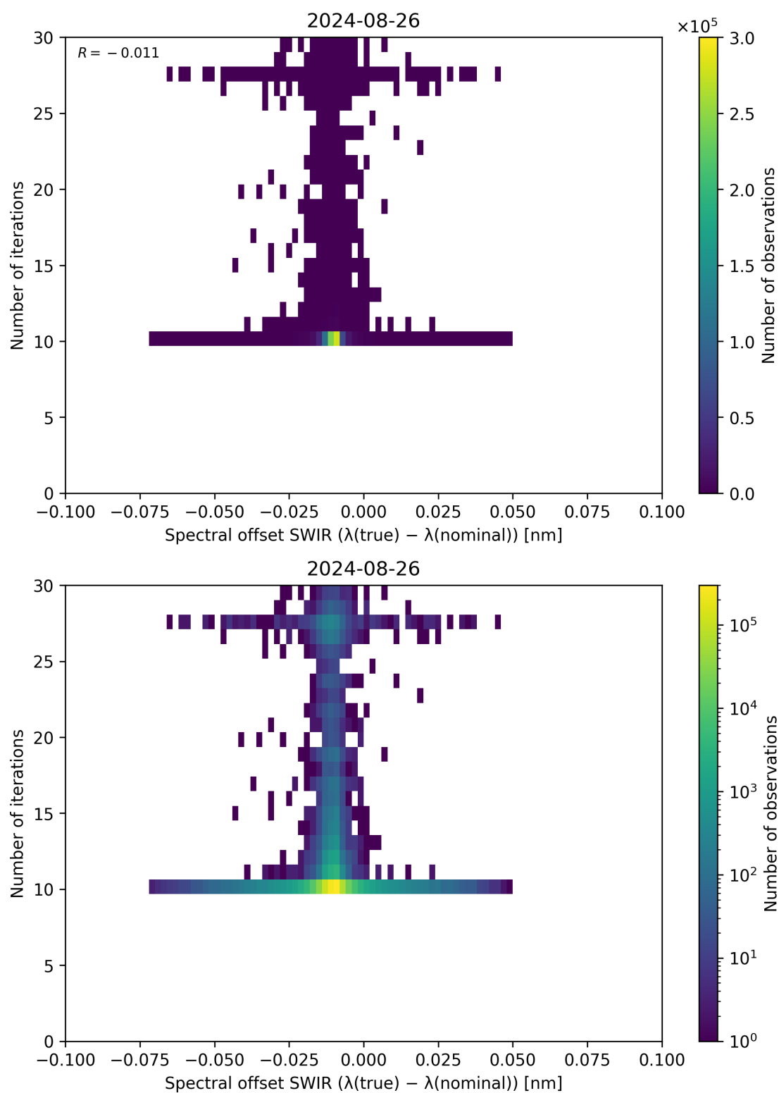
Figure 121: Scatter density plot of “Spectral offset SWIR ( \lambda_{\text{true}} - \lambda_{\text{nominal}} )” against “Number of iterations” for 2024-08-25 to 2024-08-27.
