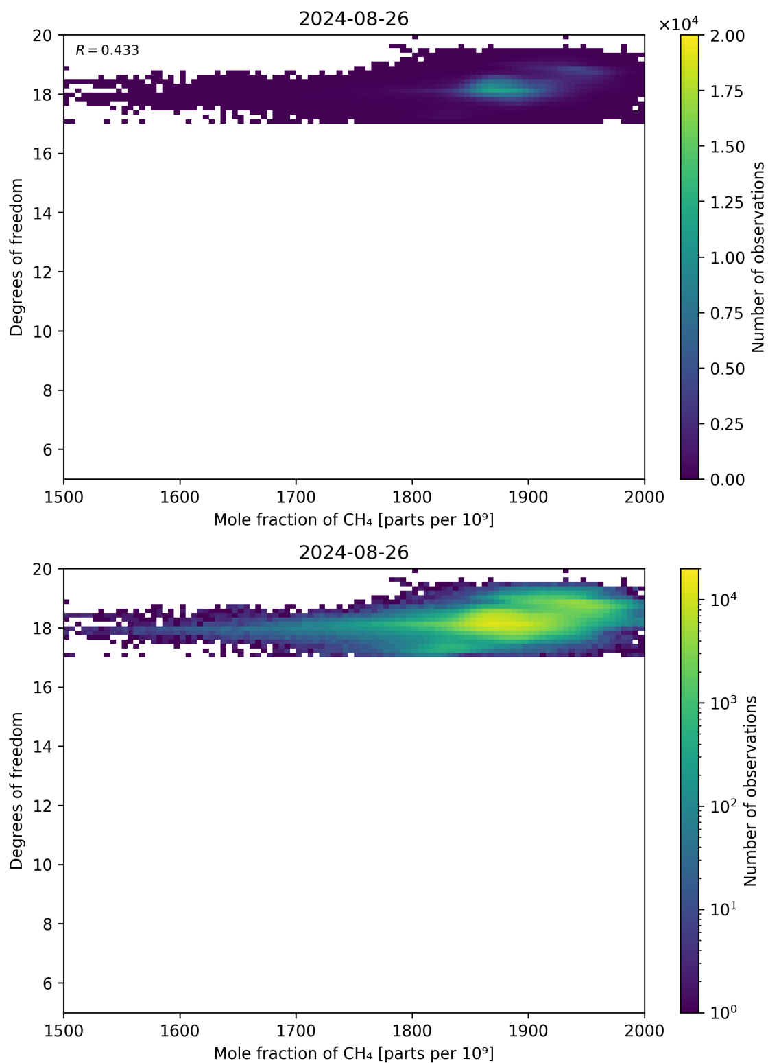
Figure 72: Scatter density plot of “Mole fraction of CH 4 ” against “Degrees of freedom” for 2024-08-25 to 2024-08-27.
