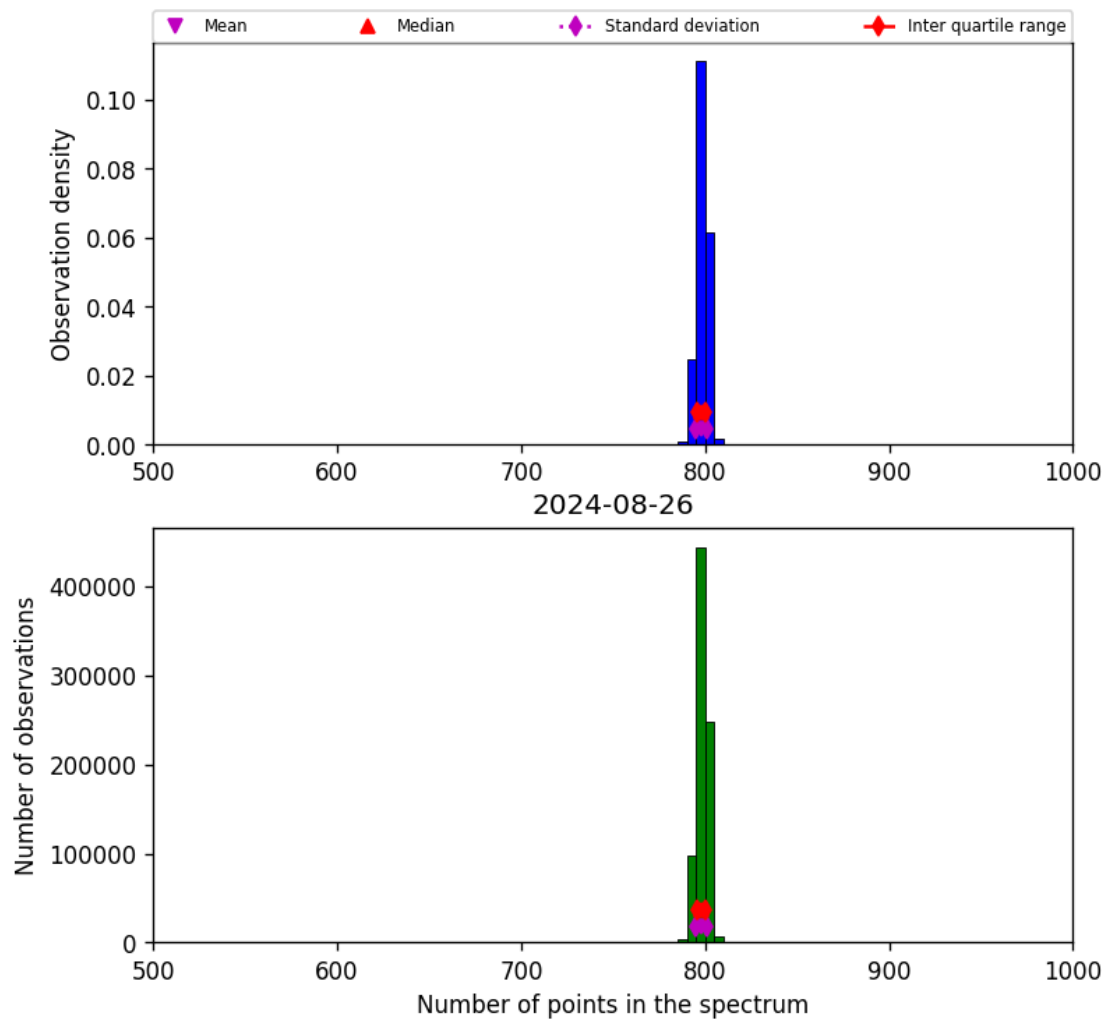
Figure 26: Histogram of “Number of points in the spectrum” for 2024-08-25 to 2024-08-27
