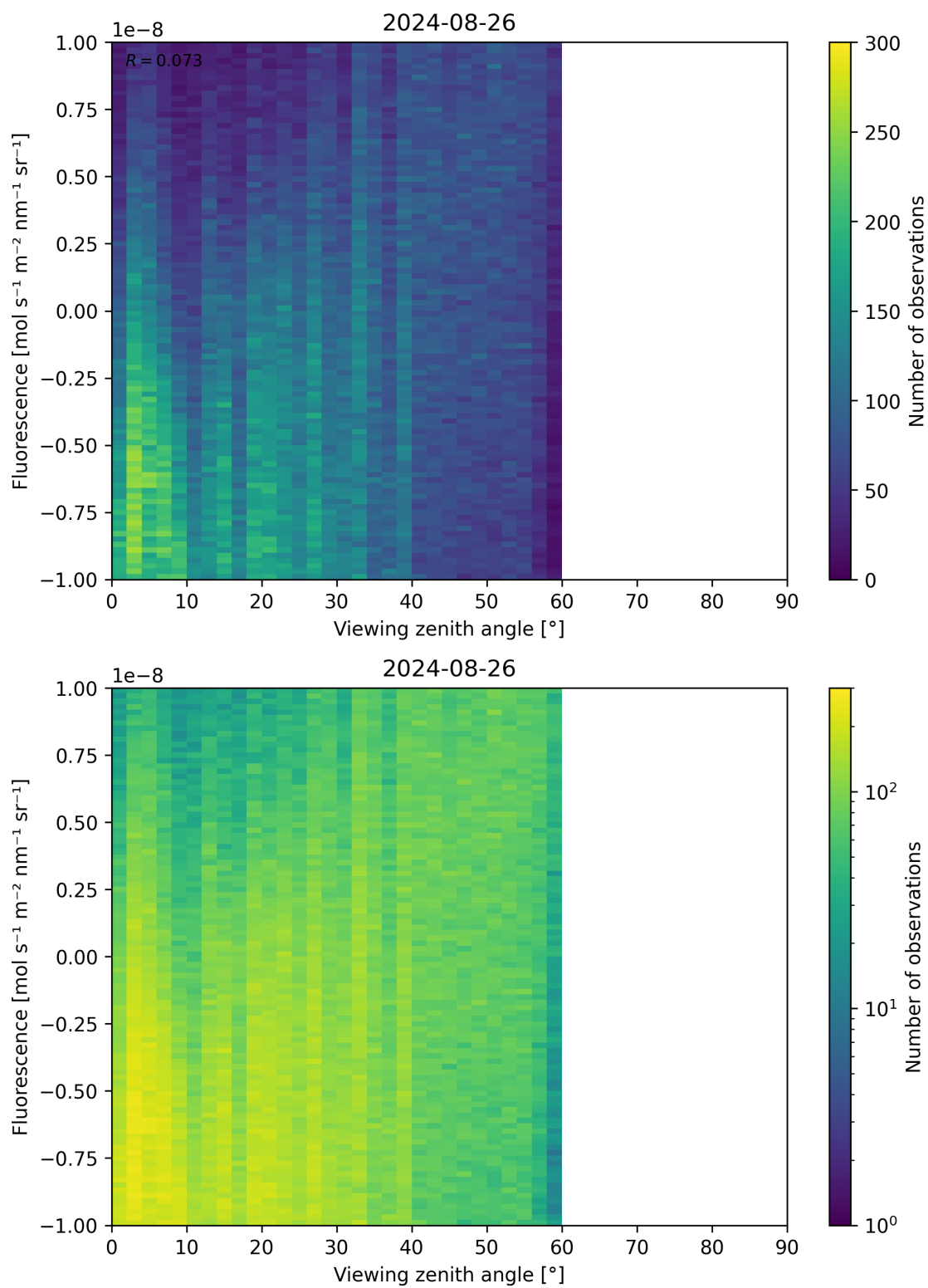
Figure 108: Scatter density plot of “Viewing zenith angle” against “Fluorescence” for 2024-08-25 to 2024-08-27.
