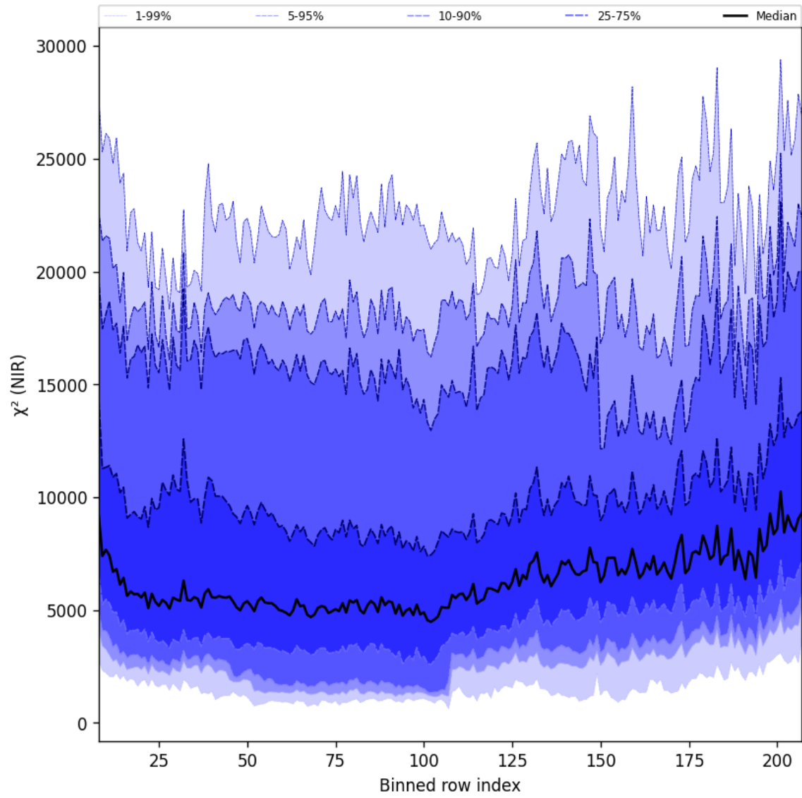
Figure 40: Along track statistics of " \chi^2 (NIR)" for 2024-08-25 to 2024-08-27
