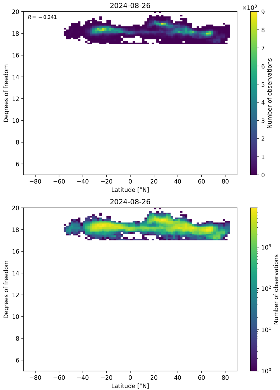
Figure 55: Scatter density plot of “Latitude” against “Degrees of freedom” for 2024-08-25 to 2024-08-27.
