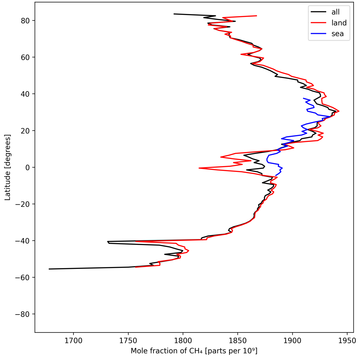
Figure 12: Zonal average of “Mole fraction of \text{CH}_4 ” for 2024-08-25 to 2024-08-27.
