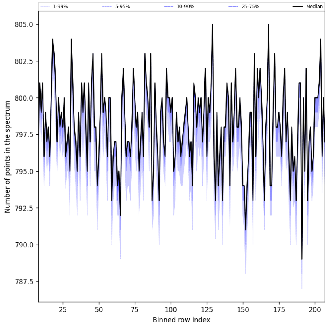
Figure 37: Along track statistics of “Number of points in the spectrum” for 2024-08-25 to 2024-08-27
