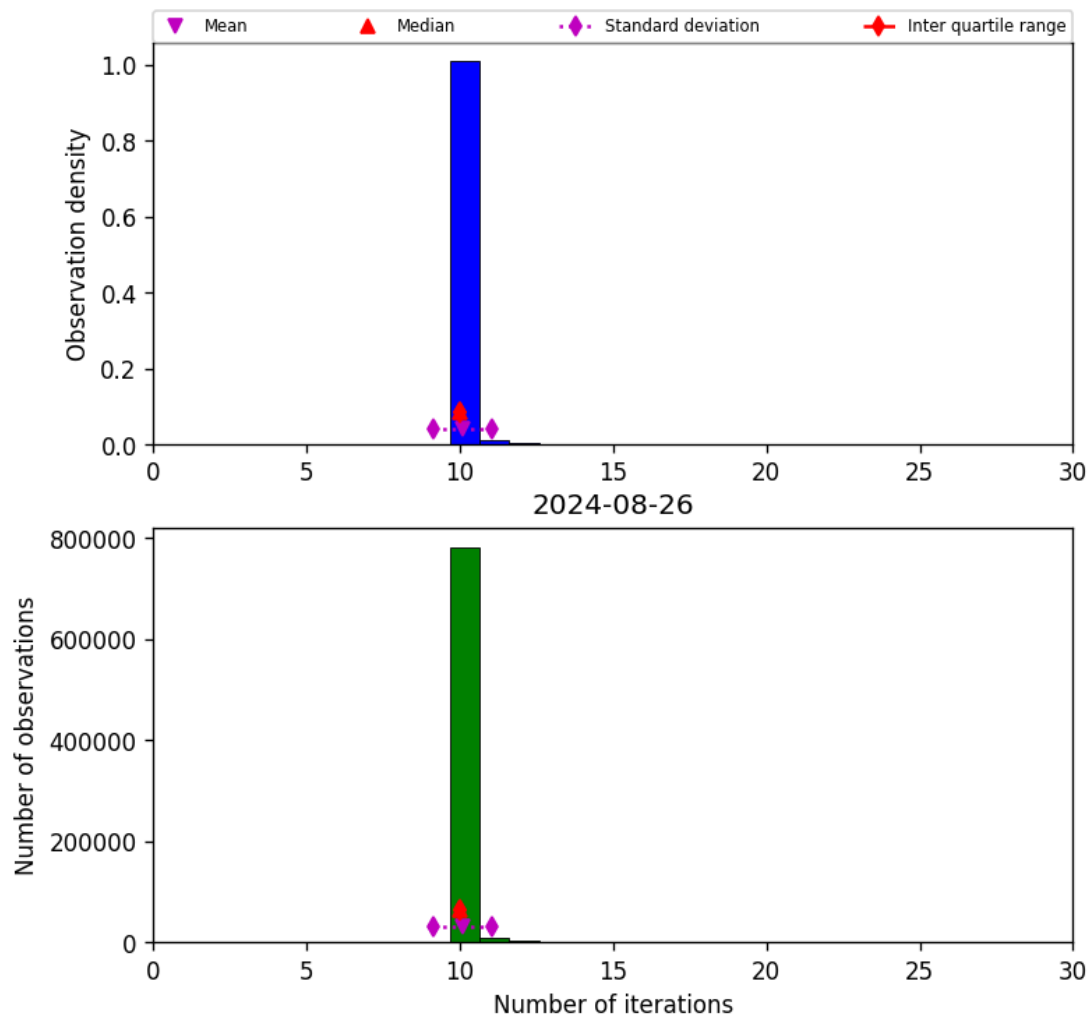
Figure 31: Histogram of “Number of iterations” for 2024-08-25 to 2024-08-27
