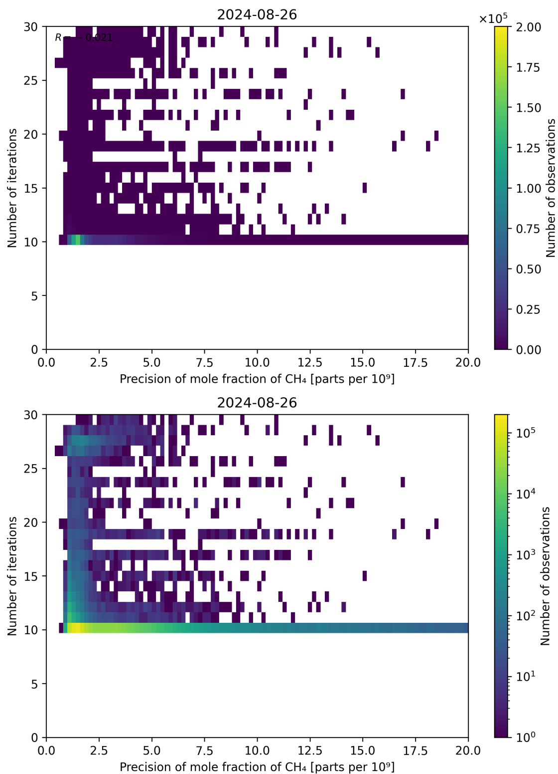
Figure 83: Scatter density plot of “Precision of mole fraction of CH 4 ” against “Number of iterations” for 2024-08-25 to 2024-08-27.
