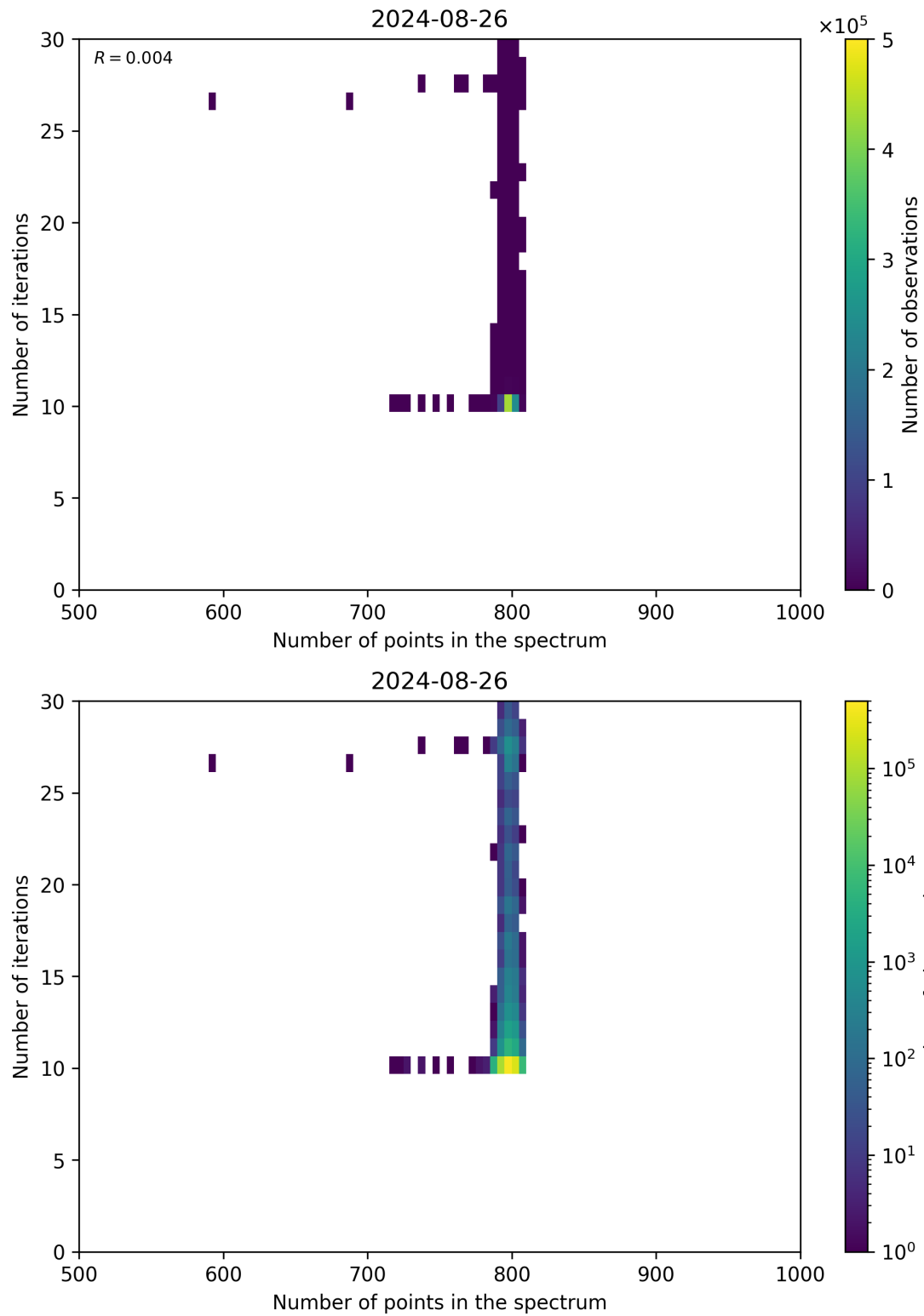
Figure 92: Scatter density plot of “Number of points in the spectrum” against “Number of iterations” for 2024-08-25 to 2024-08-27.
