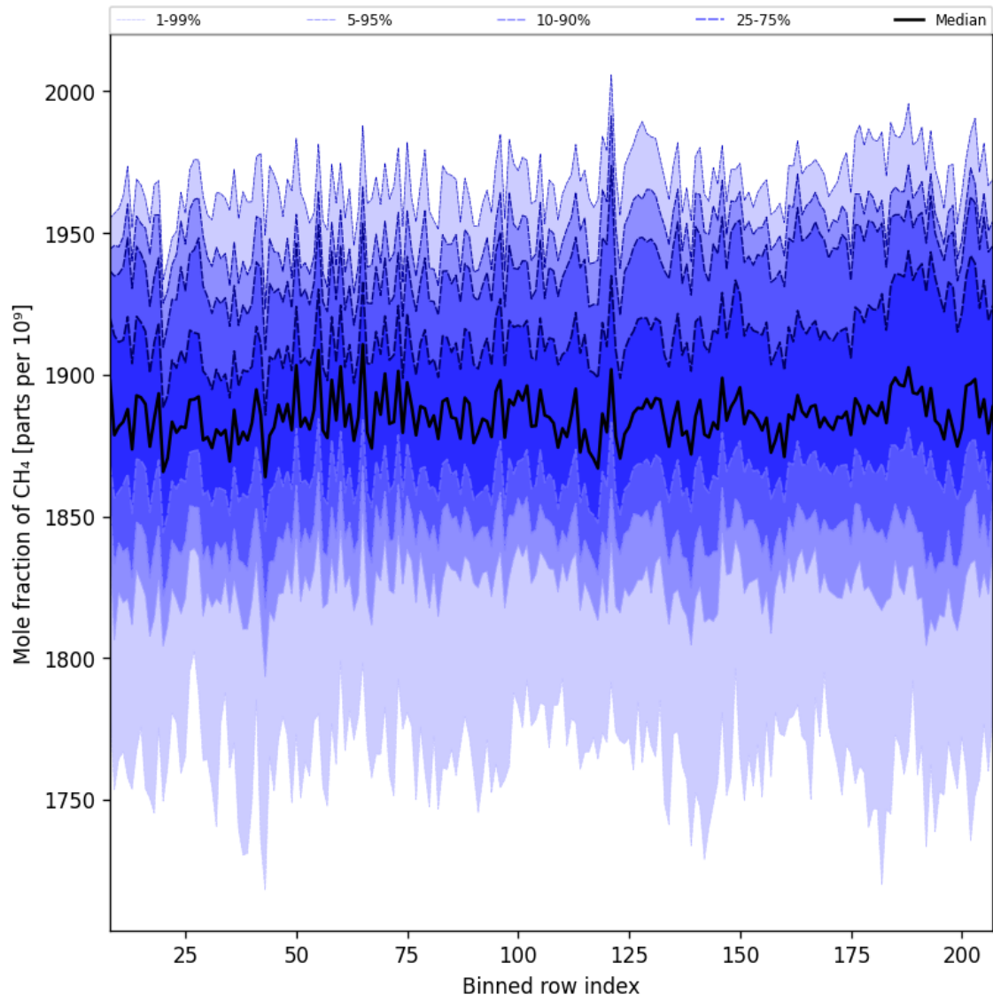
Figure 34: Along track statistics of “Mole fraction of CH 4 ” for 2024-08-25 to 2024-08-27
