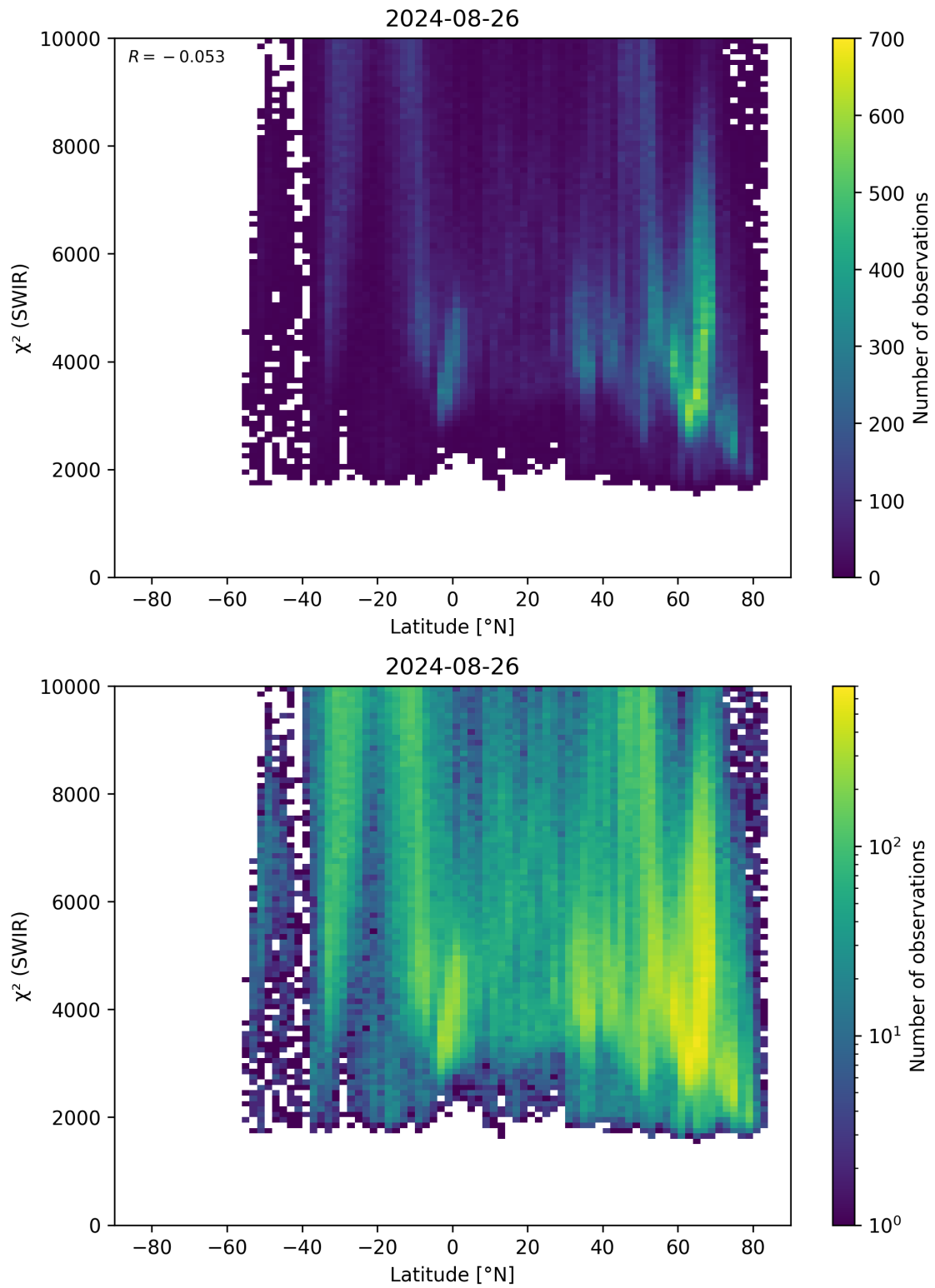
Figure 54: Scatter density plot of “Latitude” against “ \chi^2 (SWIR)” for 2024-08-25 to 2024-08-27.
