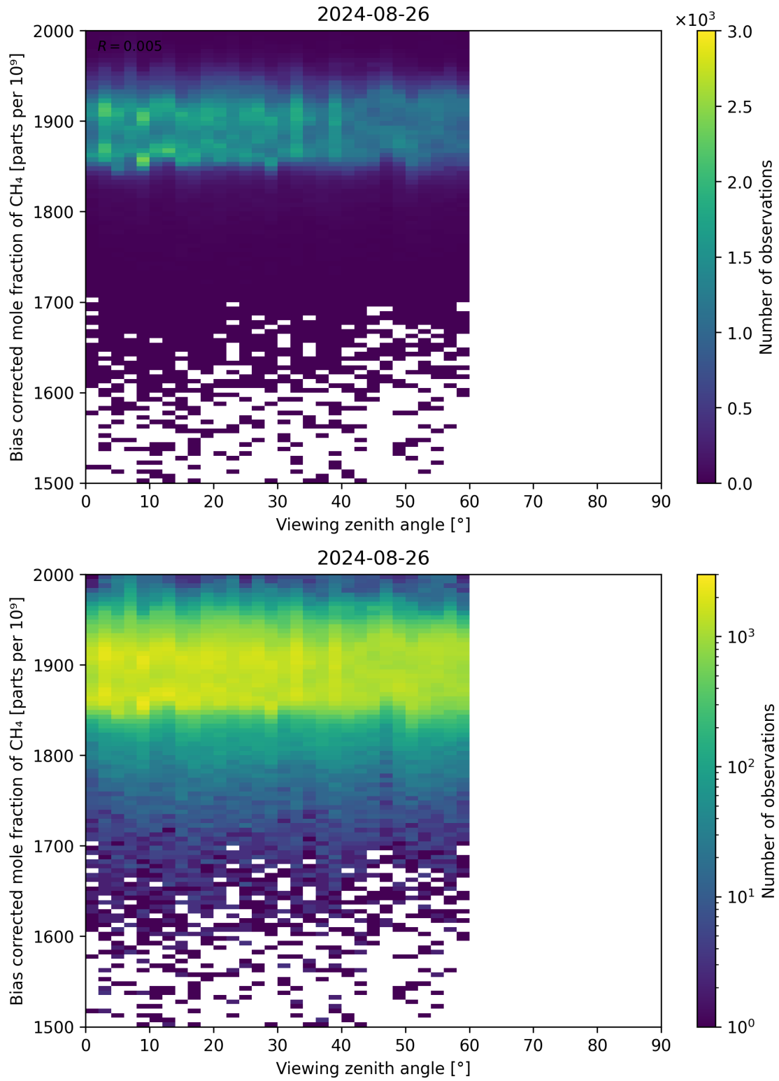
Figure 111: Scatter density plot of “Viewing zenith angle” against “Bias corrected mole fraction of CH 4 ” for 2024-08-25 to 2024-08-27.
