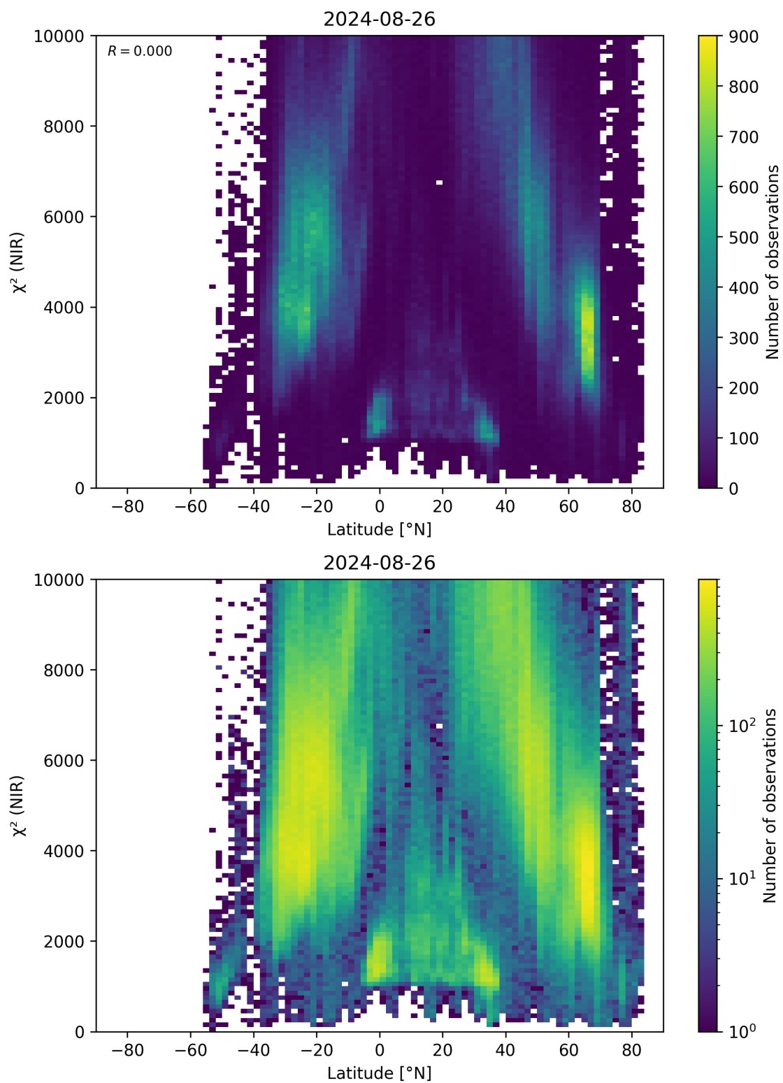
Figure 53: Scatter density plot of “Latitude” against “ \chi^2 (NIR)” for 2024-08-25 to 2024-08-27.
