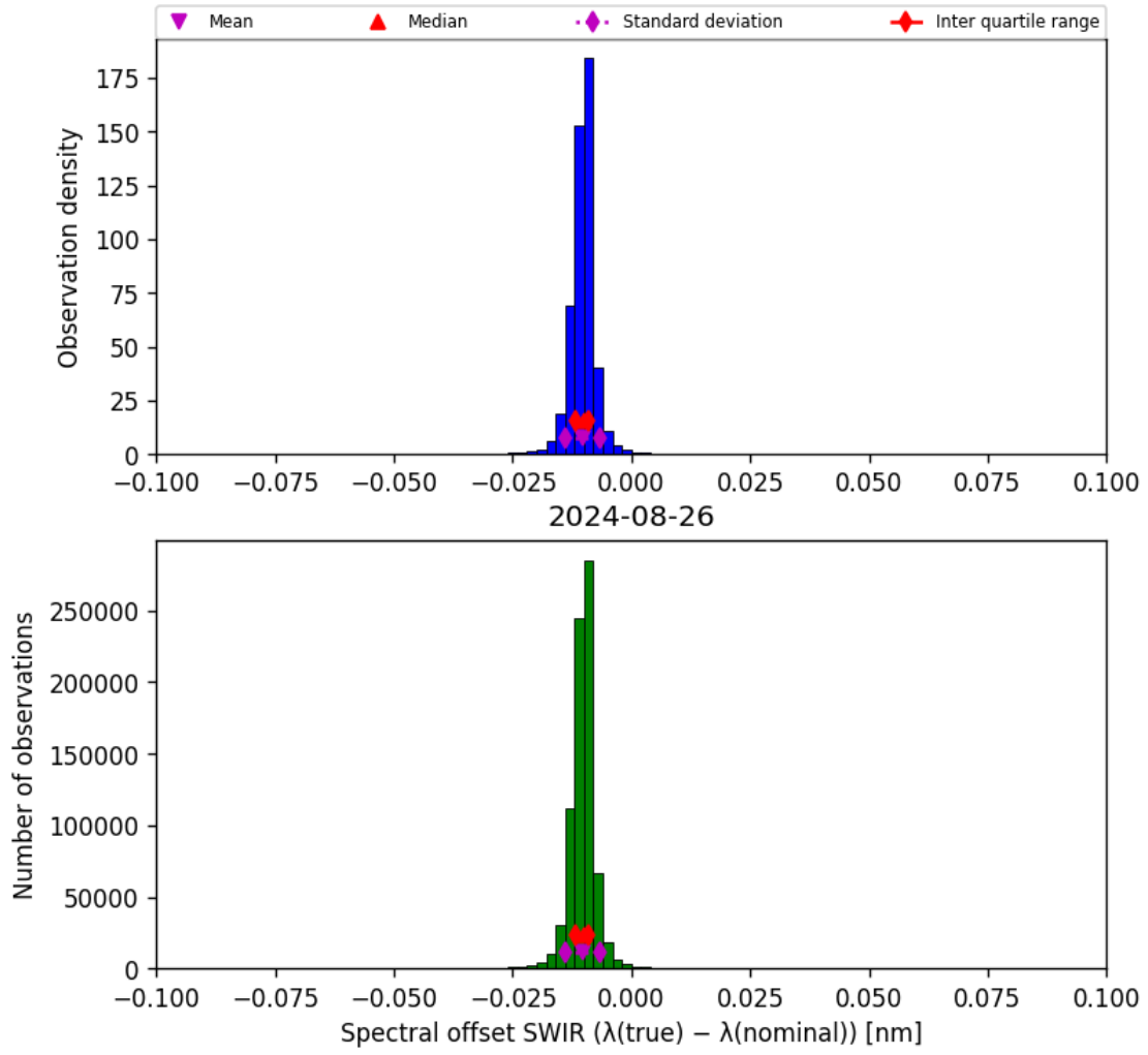
Figure 27: Histogram of “Spectral offset SWIR ( \lambda_{\text{true}} - \lambda_{\text{nominal}} )” for 2024-08-25 to 2024-08-27
