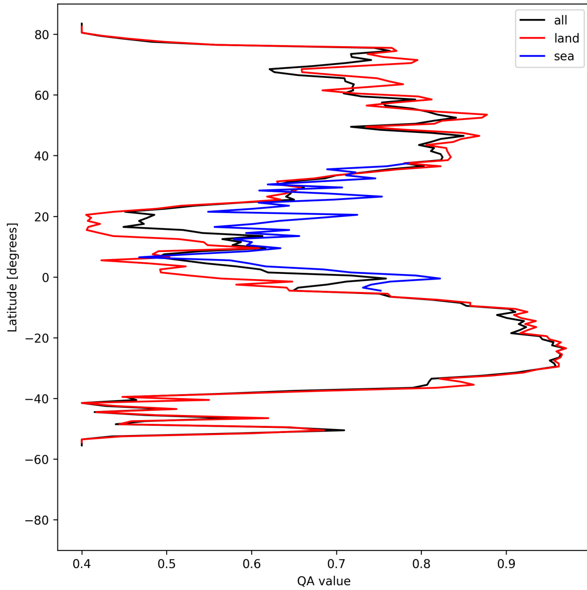
Figure 11: Zonal average of “QA value” for 2024-08-25 to 2024-08-27.
