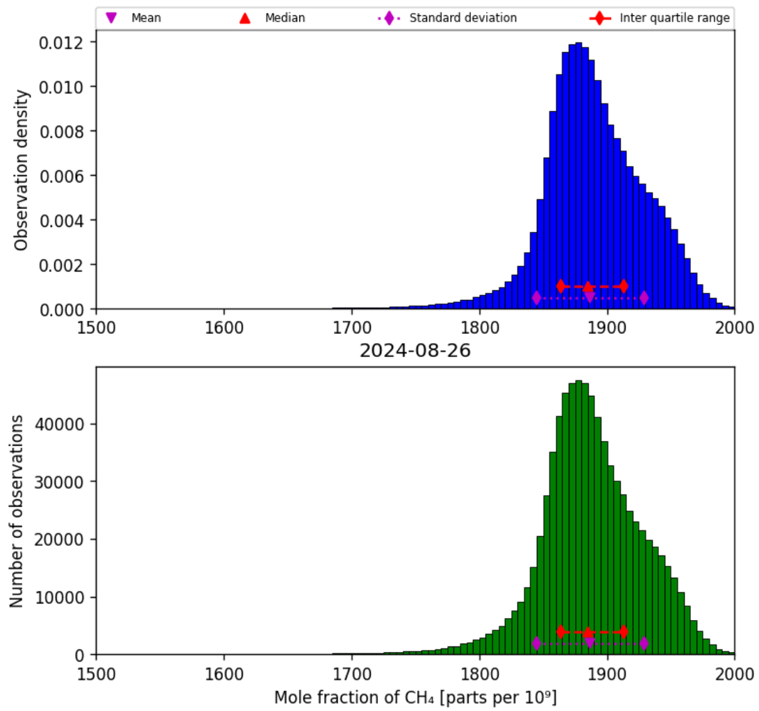
Figure 23: Histogram of “Mole fraction of CH 4 ” for 2024-08-25 to 2024-08-27
