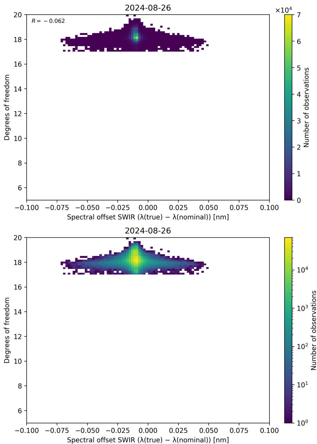
Figure 119: Scatter density plot of “Spectral offset SWIR ( \lambda_{\text{true}} - \lambda_{\text{nominal}} )” against “Degrees of freedom” for 2024-08-25 to 2024-08-27.
