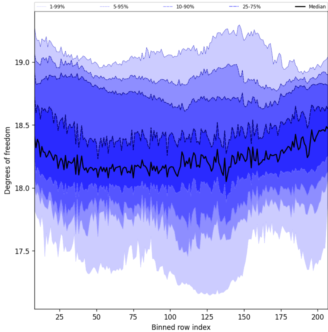
Figure 41: Along track statistics of “Degrees of freedom” for 2024-08-25 to 2024-08-27
