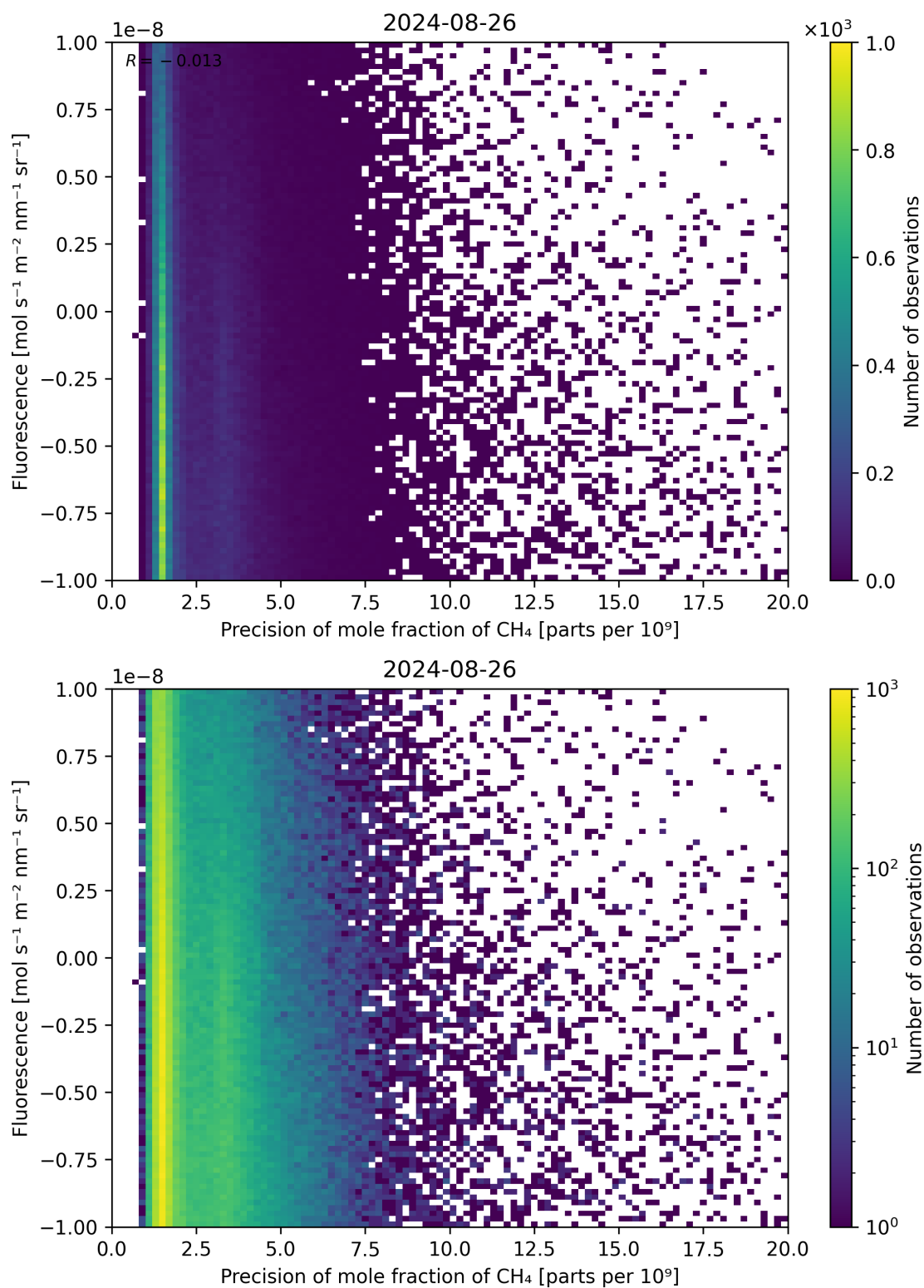
Figure 81: Scatter density plot of “Precision of mole fraction of CH 4 ” against “Fluorescence” for 2024-08-25 to 2024-08-27.
