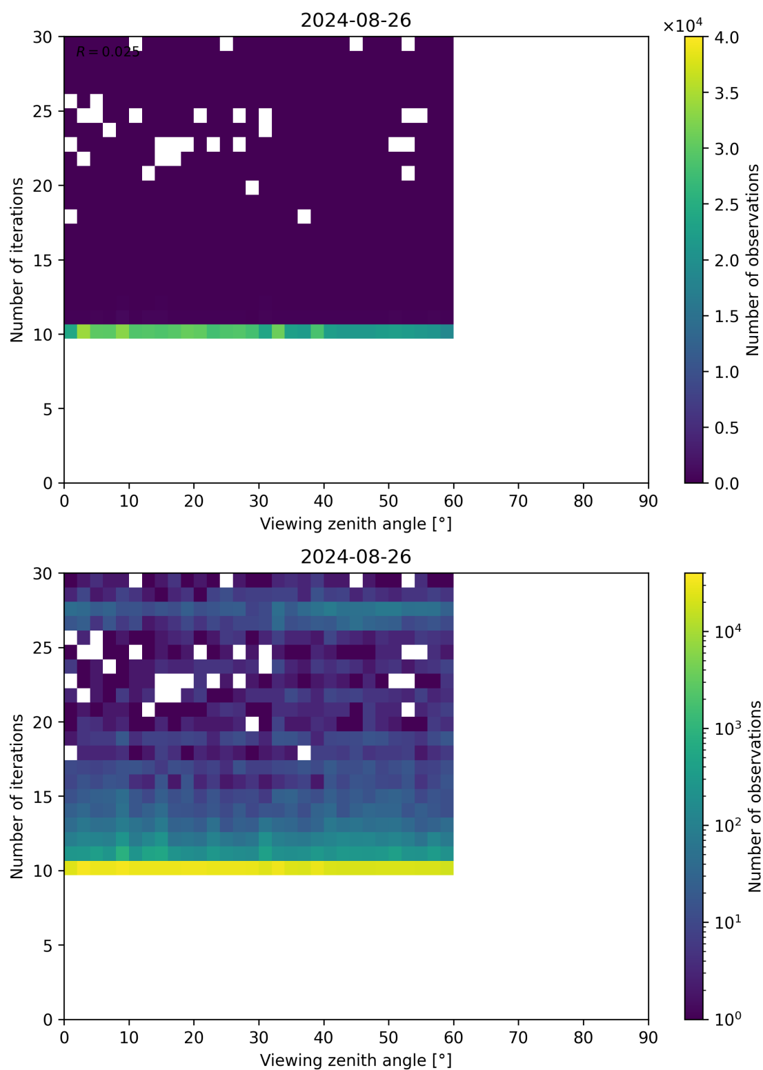
Figure 113: Scatter density plot of “Viewing zenith angle” against “Number of iterations” for 2024-08-25 to 2024-08-27.
