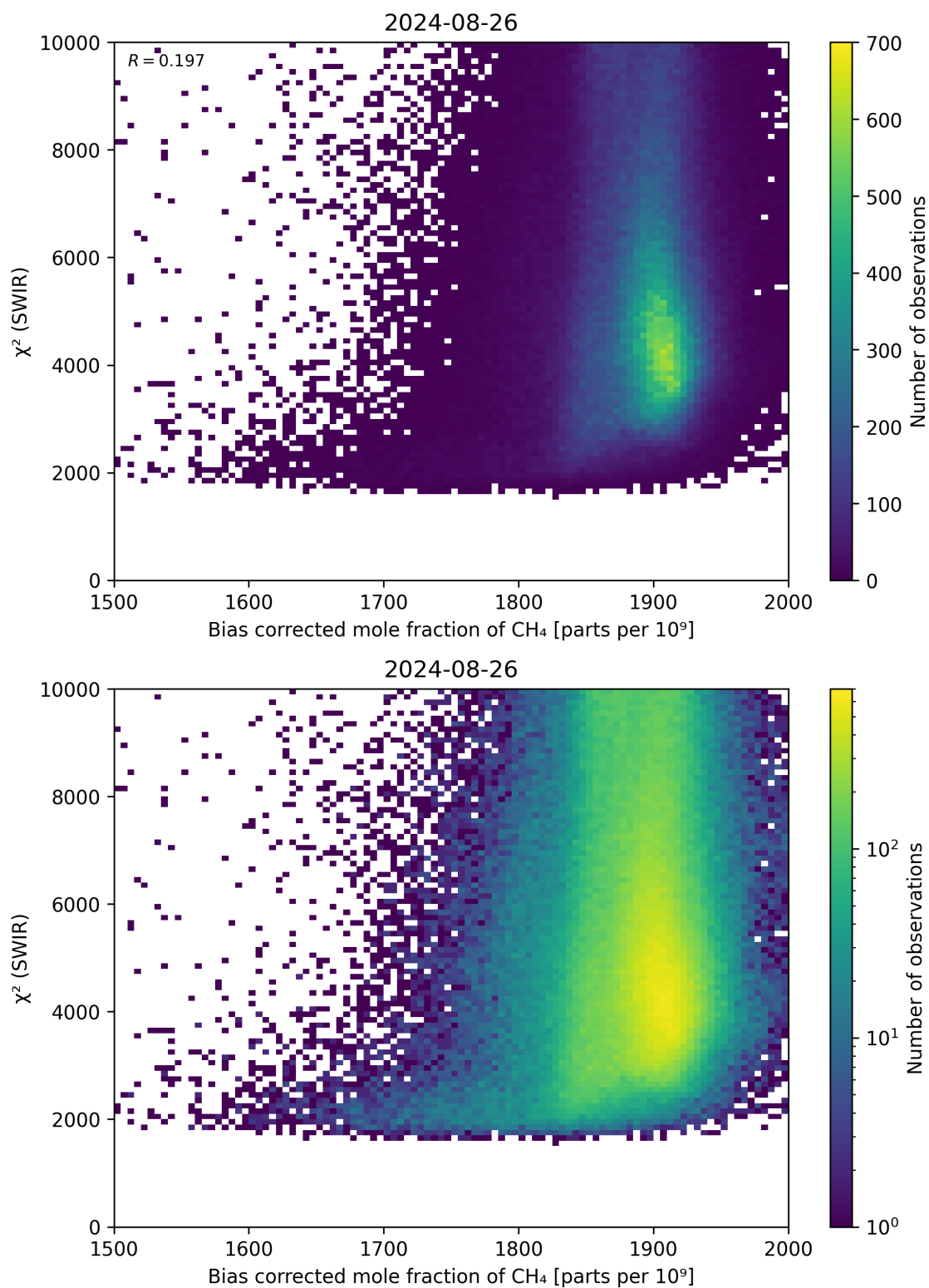
Figure 64: Scatter density plot of “Bias corrected mole fraction of \text{CH}_4 ” against “ \chi^2 (SWIR)” for 2024-08-25 to 2024-08-27.
