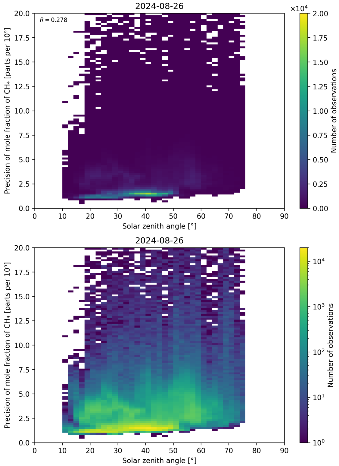
Figure 101: Scatter density plot of “Solar zenith angle” against “Precision of mole fraction of CH 4 ” for 2024-08-25 to 2024-08-27.
