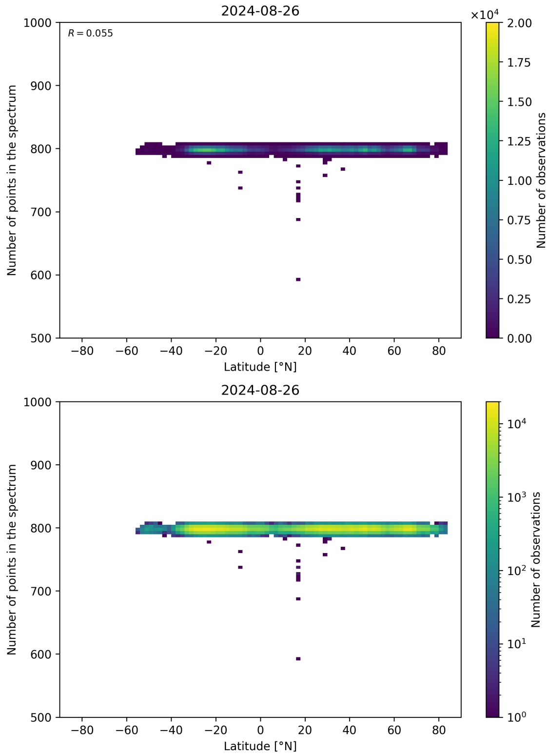
Figure 61: Scatter density plot of “Latitude” against “Number of points in the spectrum” for 2024-08-25 to 2024-08-27.
