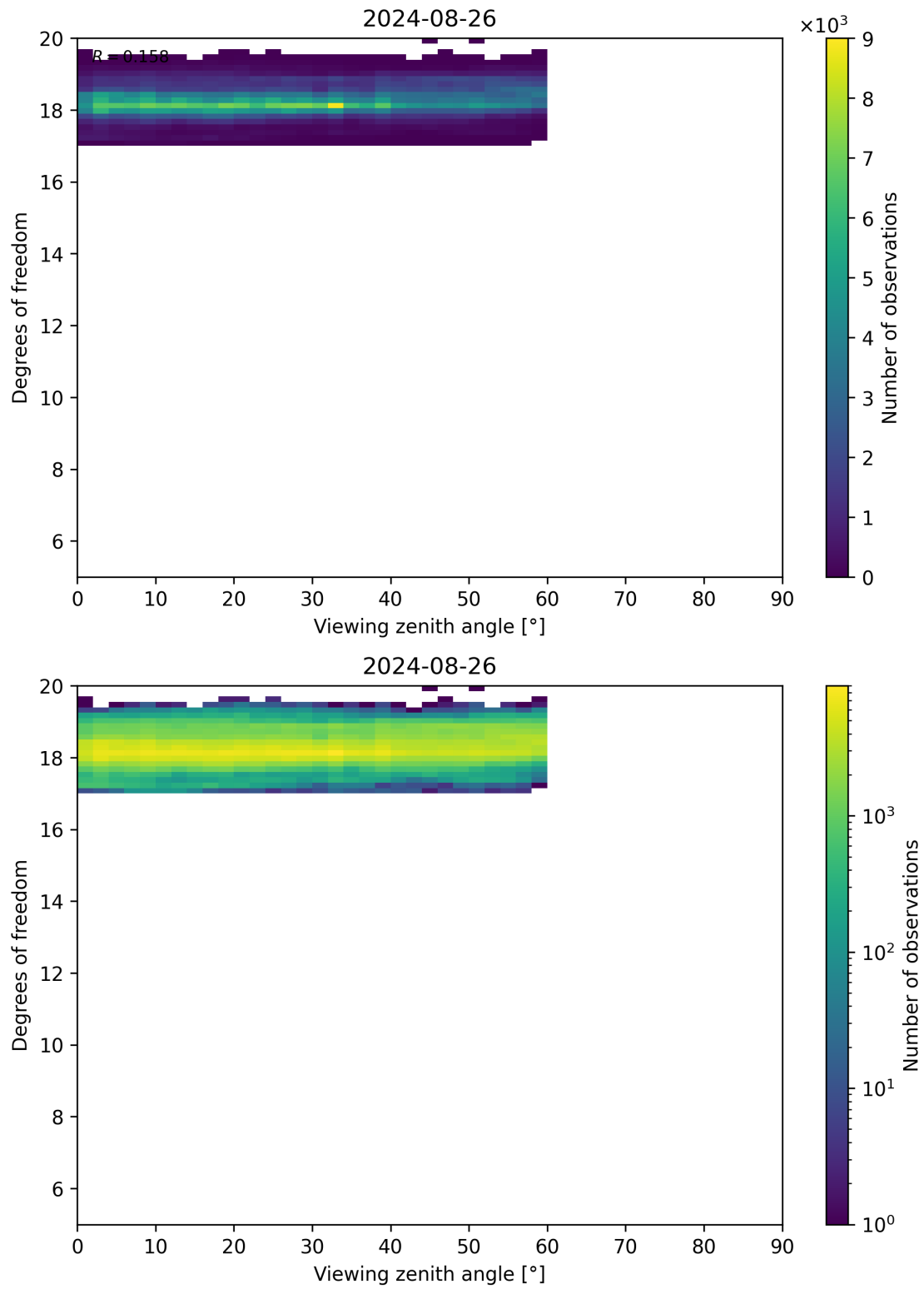
Figure 107: Scatter density plot of “Viewing zenith angle” against “Degrees of freedom” for 2024-08-25 to 2024-08-27.
