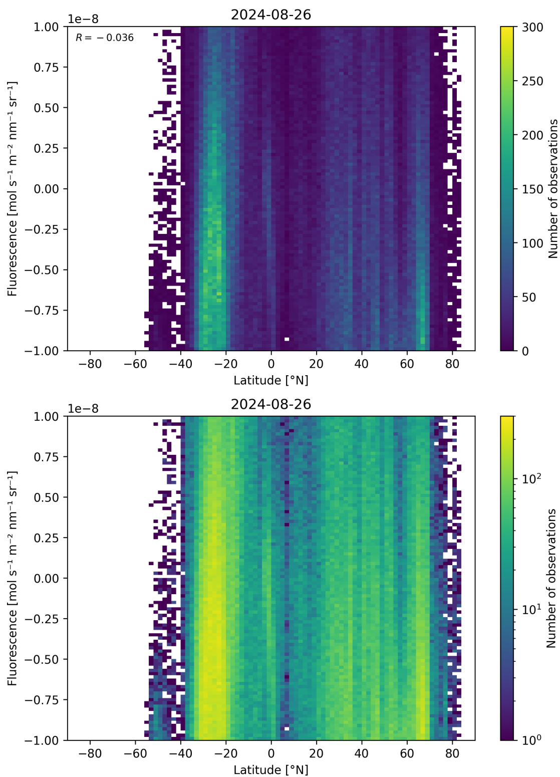
Figure 56: Scatter density plot of “Latitude” against “Fluorescence” for 2024-08-25 to 2024-08-27.
