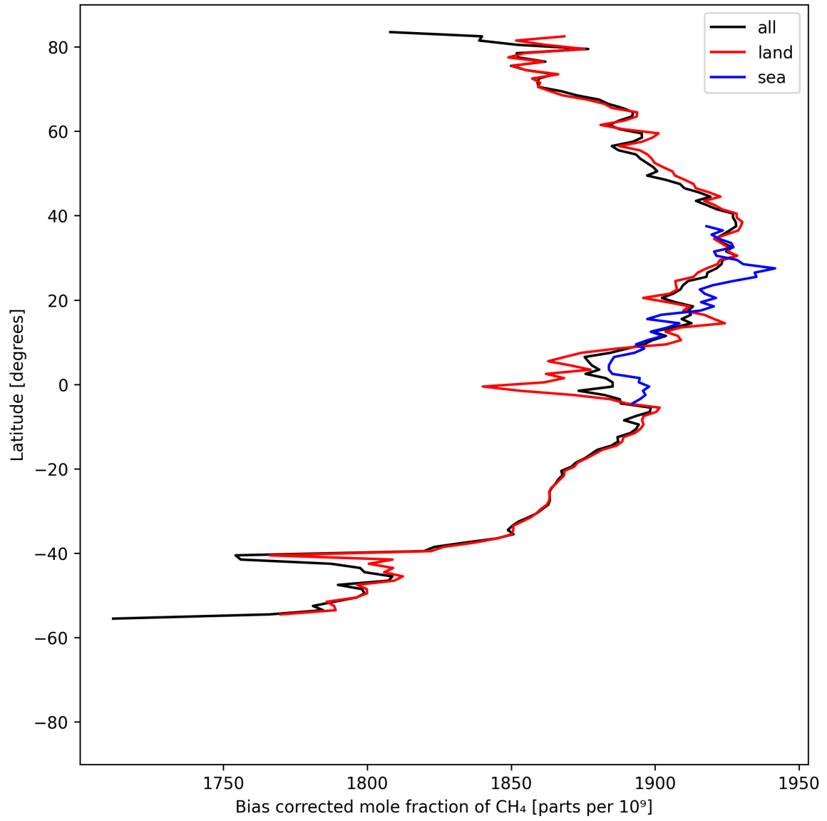
Figure 14: Zonal average of “Bias corrected mole fraction of \text{CH}_4 ” for 2024-08-25 to 2024-08-27.
