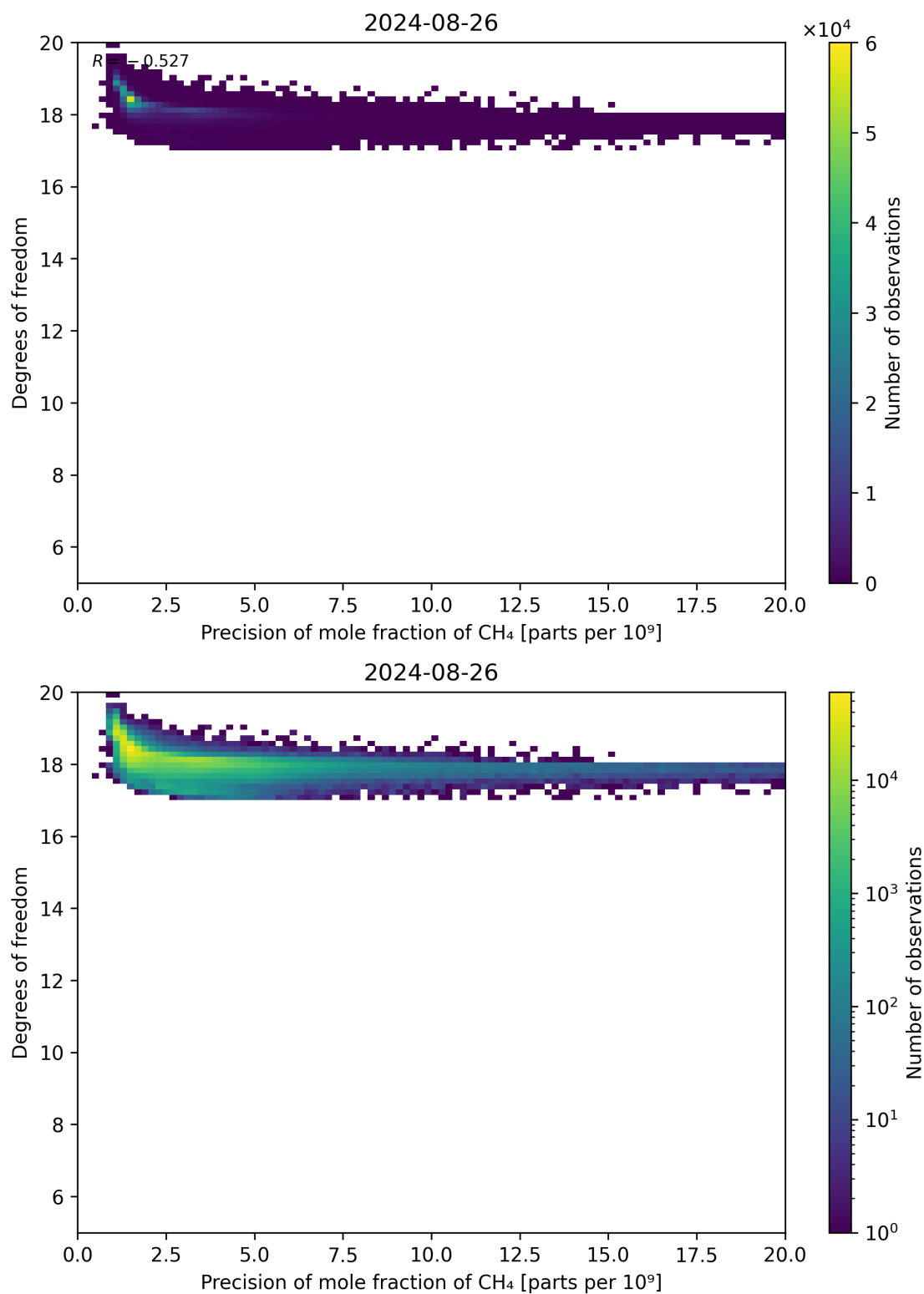
Figure 80: Scatter density plot of “Precision of mole fraction of CH 4 ” against “Degrees of freedom” for 2024-08-25 to 2024-08-27.
