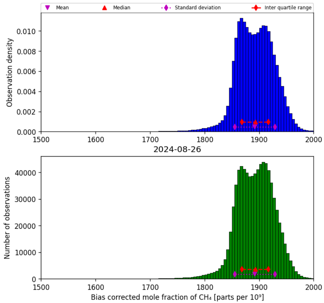
Figure 25: Histogram of “Bias corrected mole fraction of CH 4 ” for 2024-08-25 to 2024-08-27
