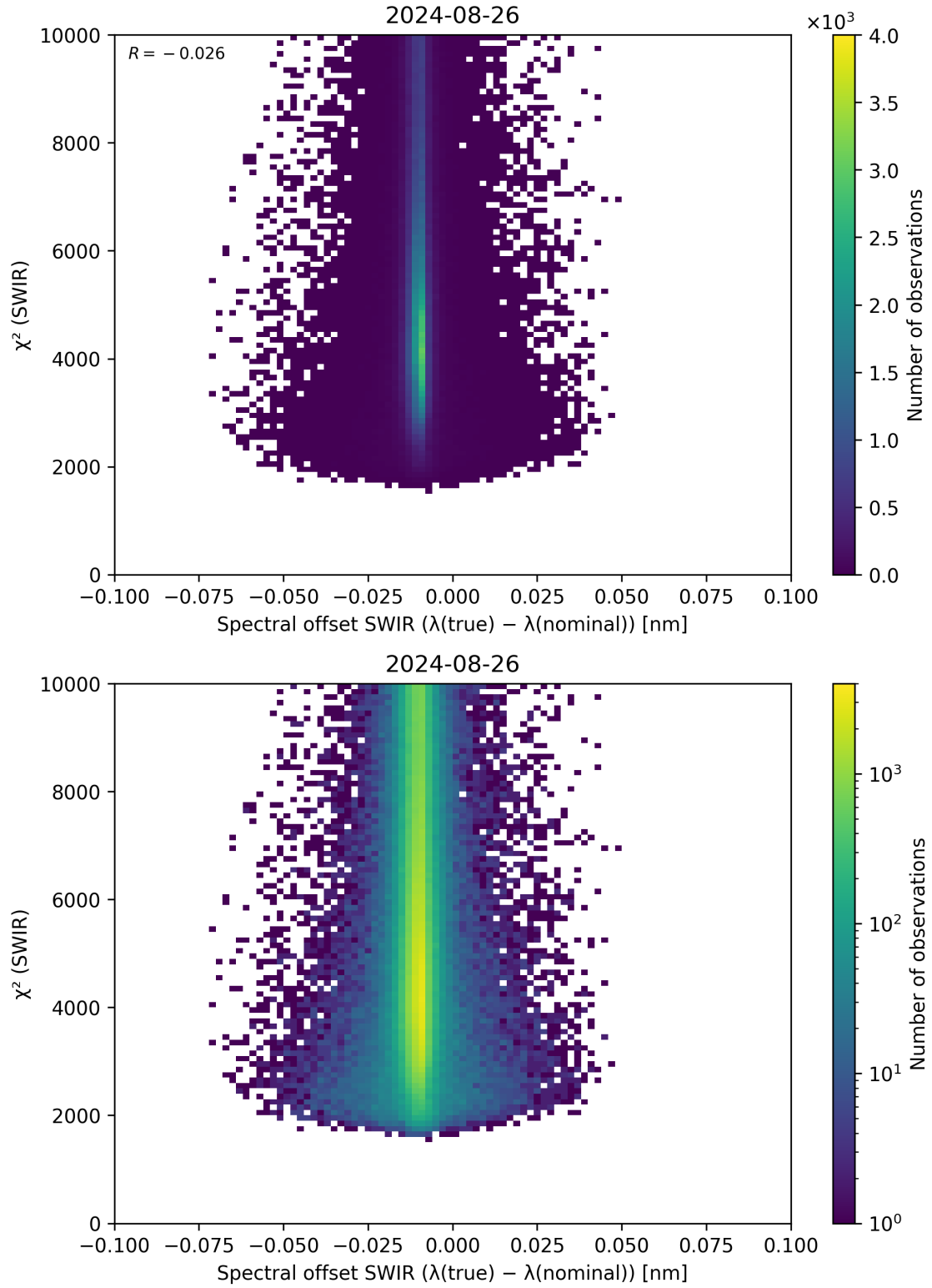
Figure 118: Scatter density plot of “Spectral offset SWIR ( \lambda_{\text{true}} - \lambda_{\text{nominal}} )” against “ \chi^2 (SWIR)” for 2024-08-25 to 2024-08-27.
