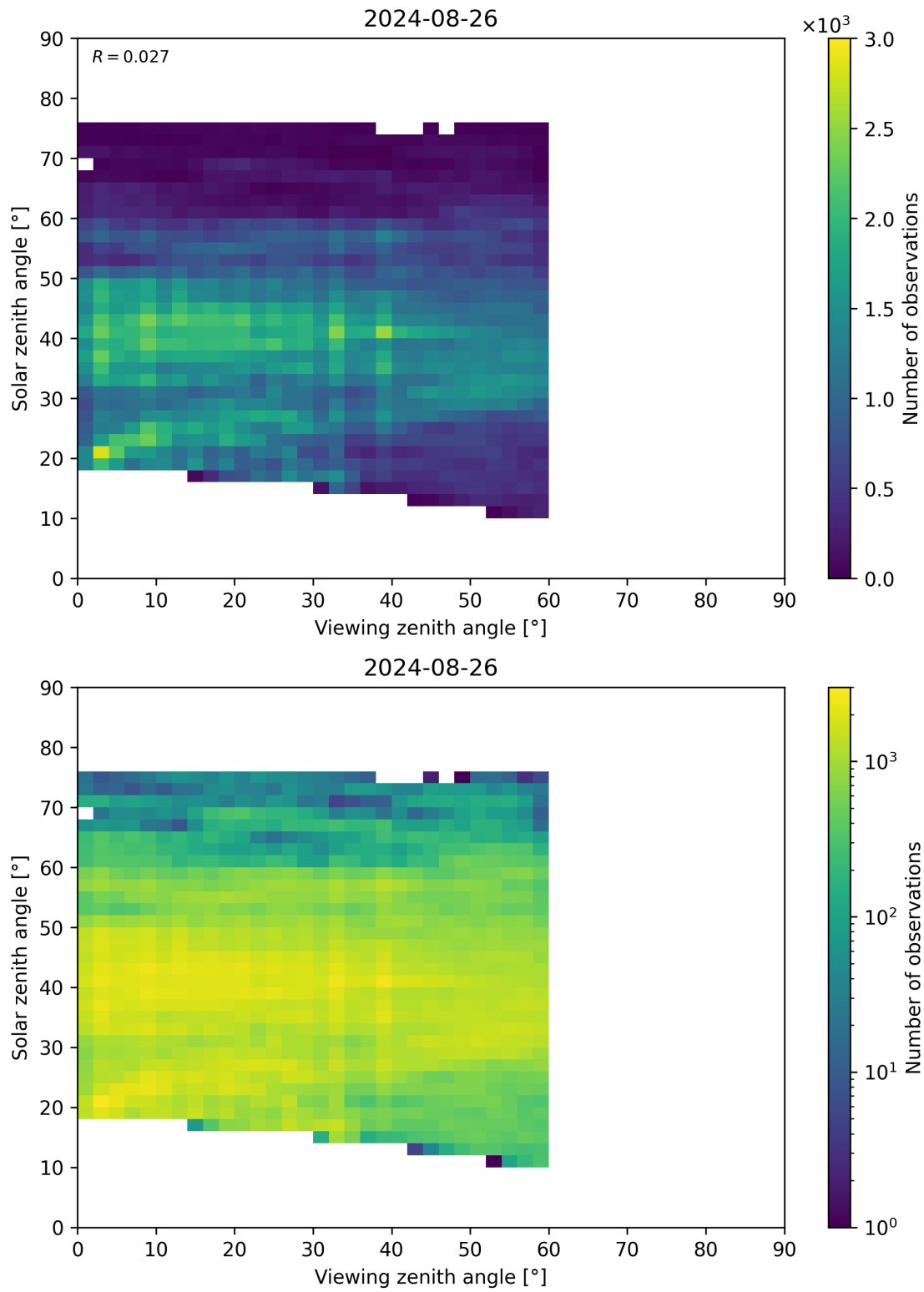
Figure 115: Scatter density plot of “Viewing zenith angle” against “Solar zenith angle” for 2024-08-25 to 2024-08-27.
