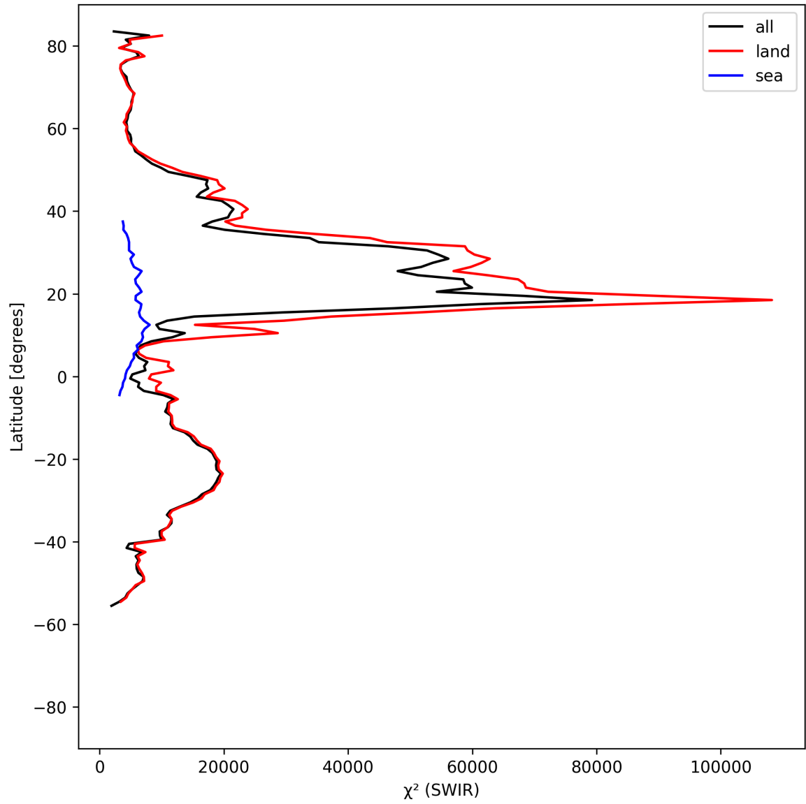
Figure 17: Zonal average of “ \chi^2 (SWIR)” for 2024-08-25 to 2024-08-27.
