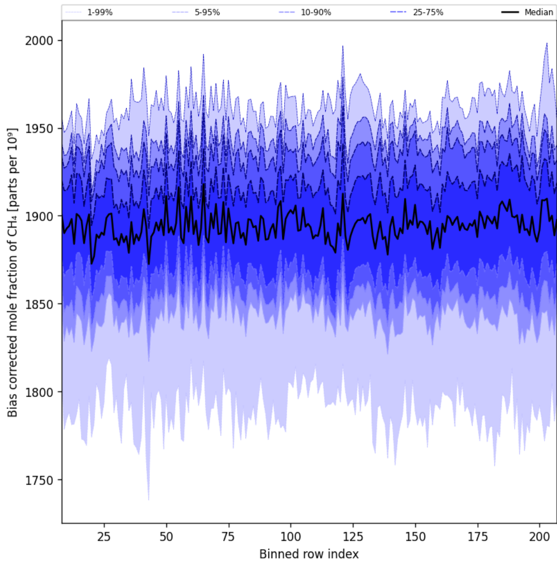
Figure 36: Along track statistics of “Bias corrected mole fraction of CH 4 ” for 2024-08-25 to 2024-08-27
