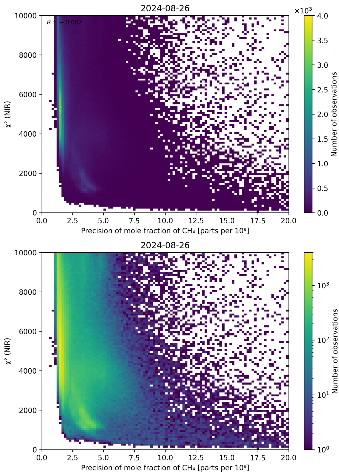
Figure 78: Scatter density plot of “Precision of mole fraction of CH 4 ” against “ \chi^2 (NIR)” for 2024-08-25 to 2024-08-27.
