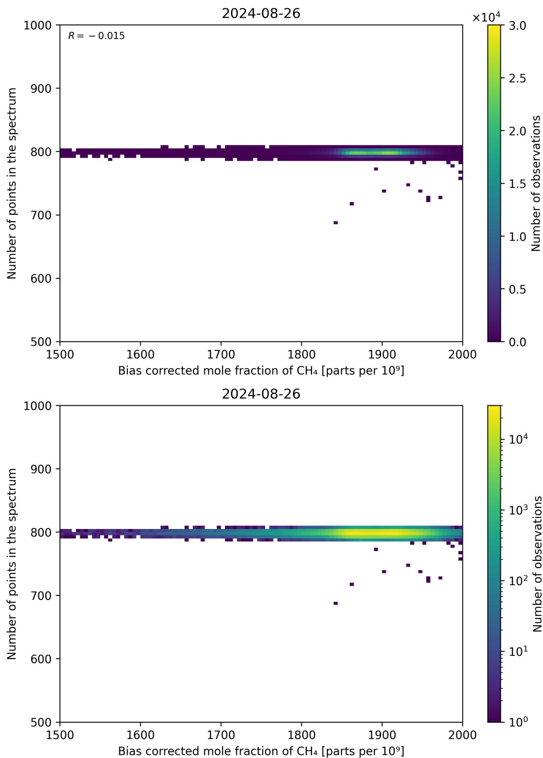
Figure 68: Scatter density plot of “Bias corrected mole fraction of CH 4 ” against “Number of points in the spectrum” for 2024-08-25 to 2024-08-27.
