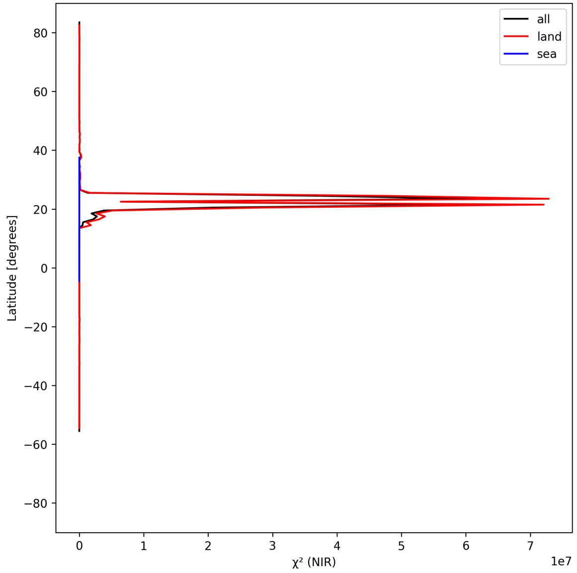
Figure 18: Zonal average of “ \chi^2 (NIR)” for 2024-08-25 to 2024-08-27.
