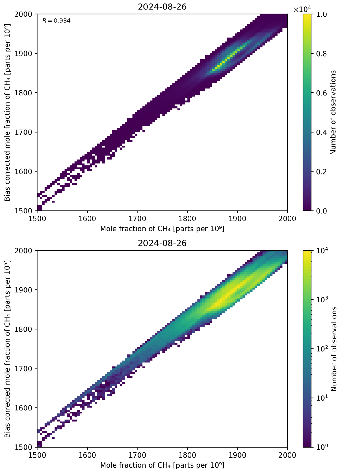
Figure 74: Scatter density plot of “Mole fraction of CH 4 ” against “Bias corrected mole fraction of CH 4 ” for 2024-08-25 to 2024-08-27.
