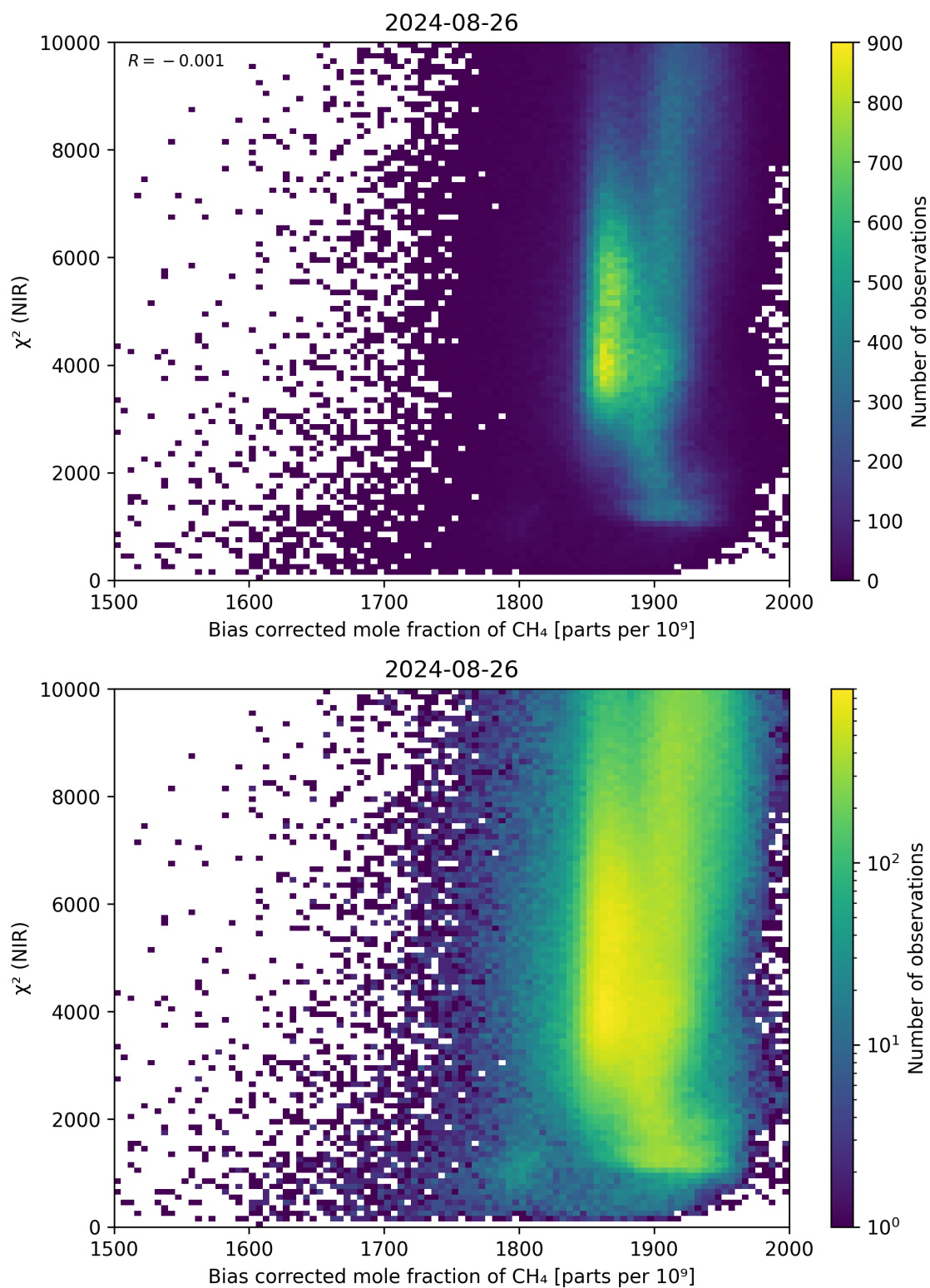
Figure 63: Scatter density plot of “Bias corrected mole fraction of CH 4 ” against “ \chi^2 (NIR)” for 2024-08-25 to 2024-08-27.
