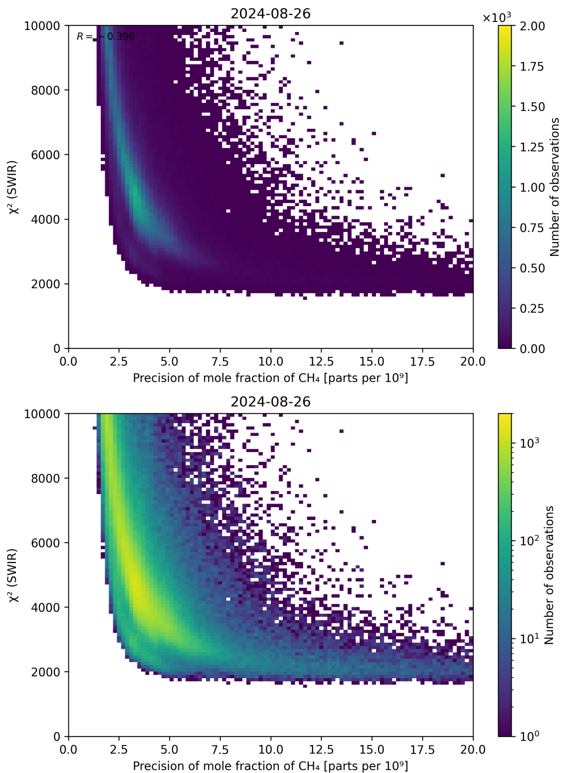
Figure 79: Scatter density plot of “Precision of mole fraction of \text{CH}_4 ” against “ \chi^2 (SWIR)” for 2024-08-25 to 2024-08-27.
