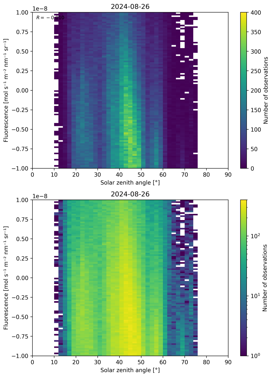
Figure 97: Scatter density plot of “Solar zenith angle” against “Fluorescence” for 2024-08-25 to 2024-08-27.
