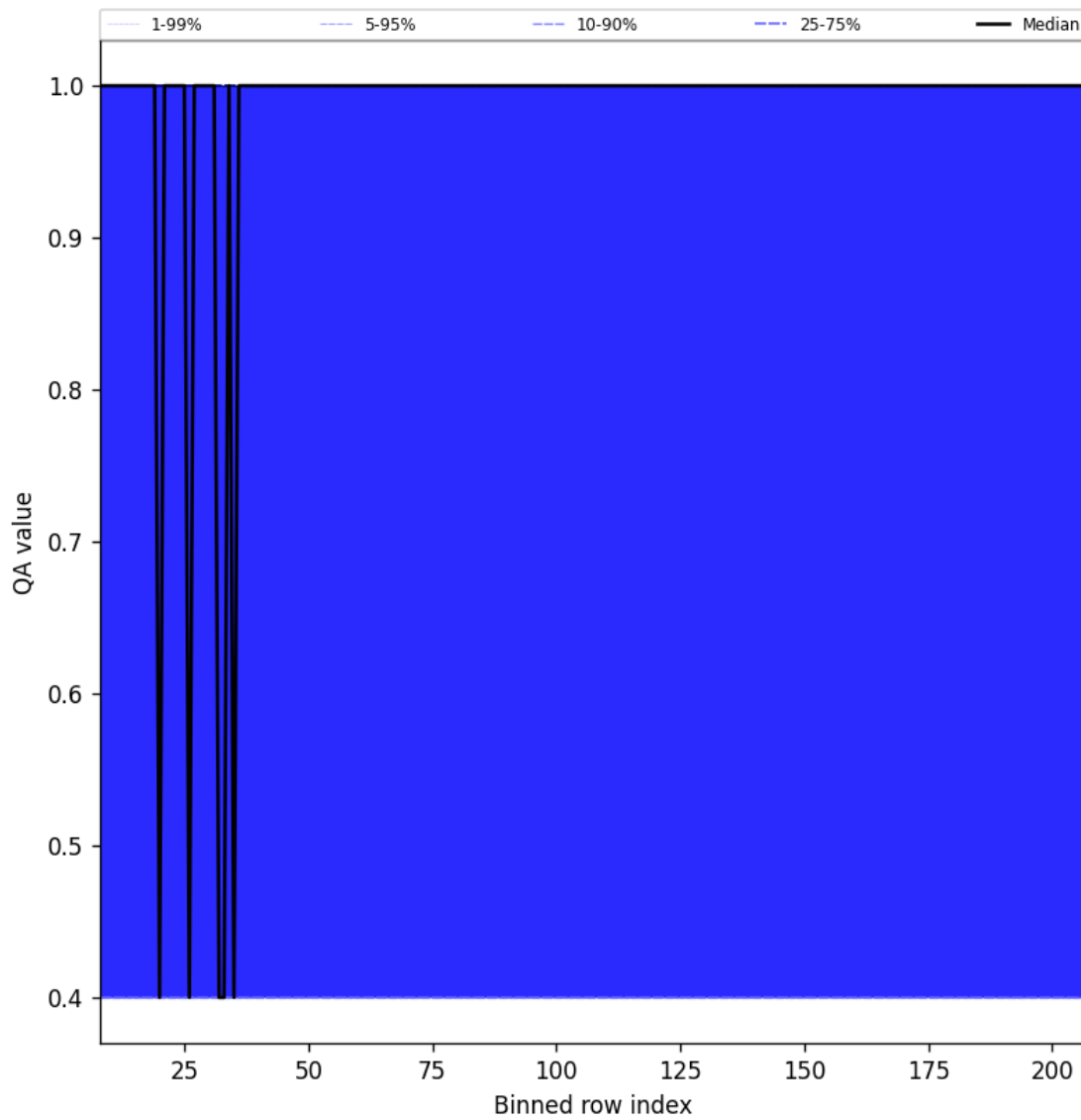
Figure 33: Along track statistics of “QA value” for 2024-08-25 to 2024-08-27
