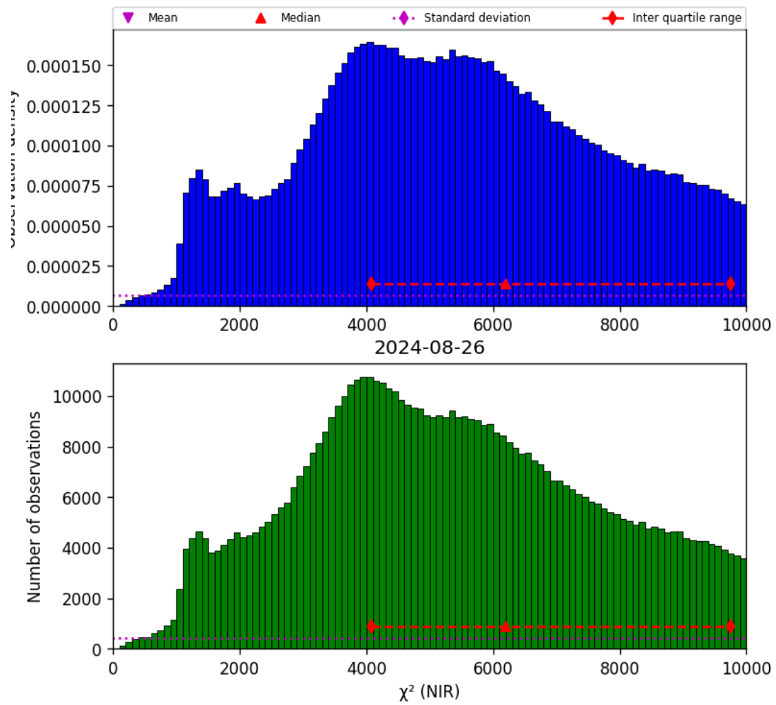
Figure 29: Histogram of “ \chi^2 (NIR)” for 2024-08-25 to 2024-08-27
