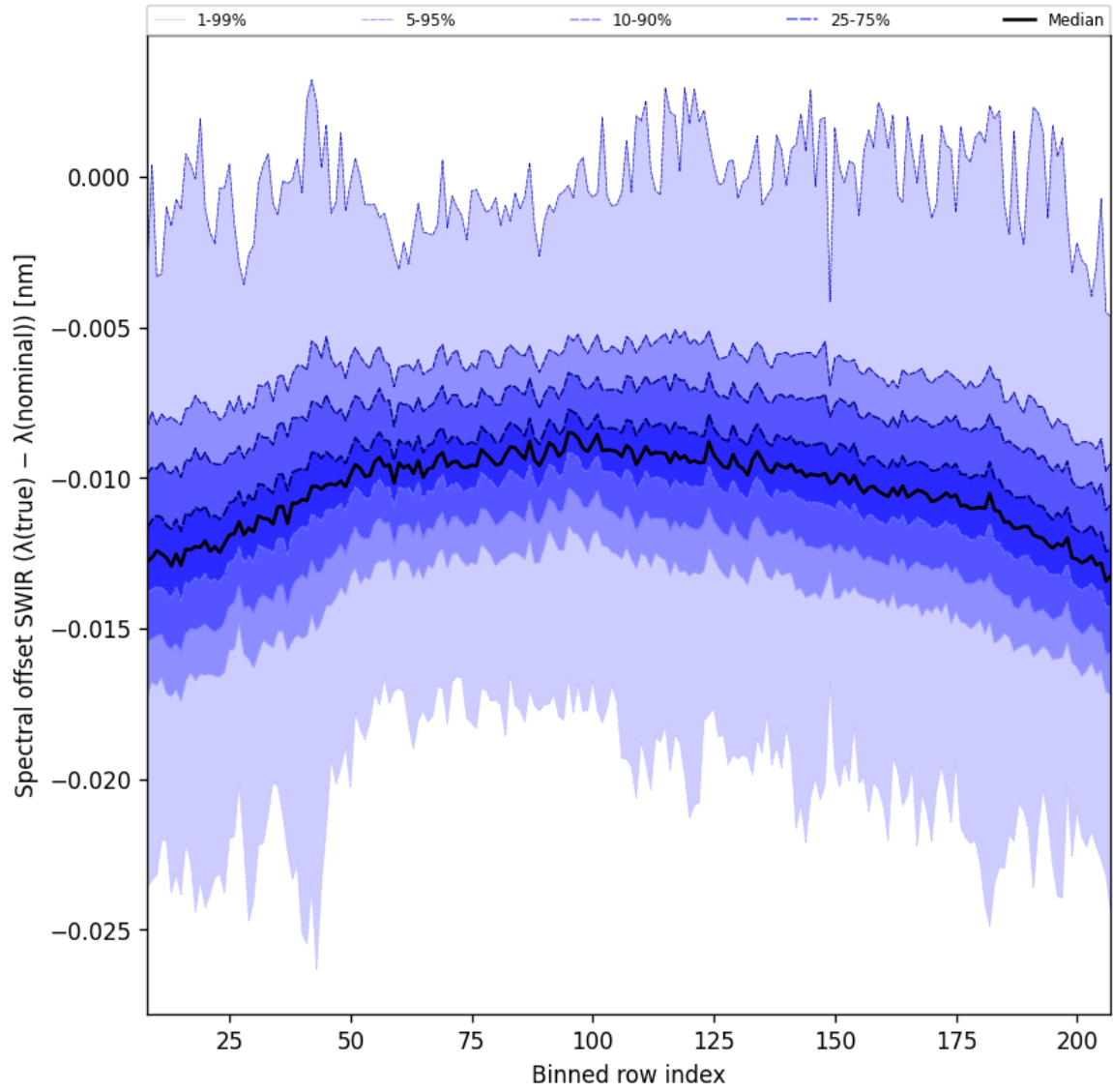
Figure 38: Along track statistics of “Spectral offset SWIR ( \lambda_{\text{true}} - \lambda_{\text{nominal}} )” for 2024-08-25 to 2024-08-27
