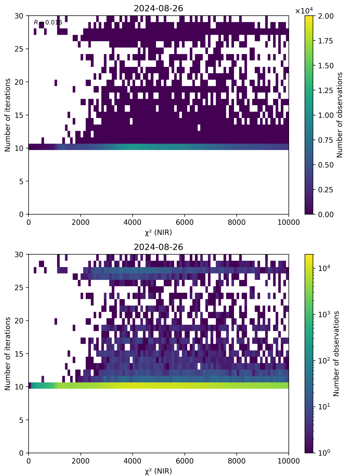
Figure 46: Scatter density plot of “ \chi^2 (NIR)” against “Number of iterations” for 2024-08-25 to 2024-08-27.
