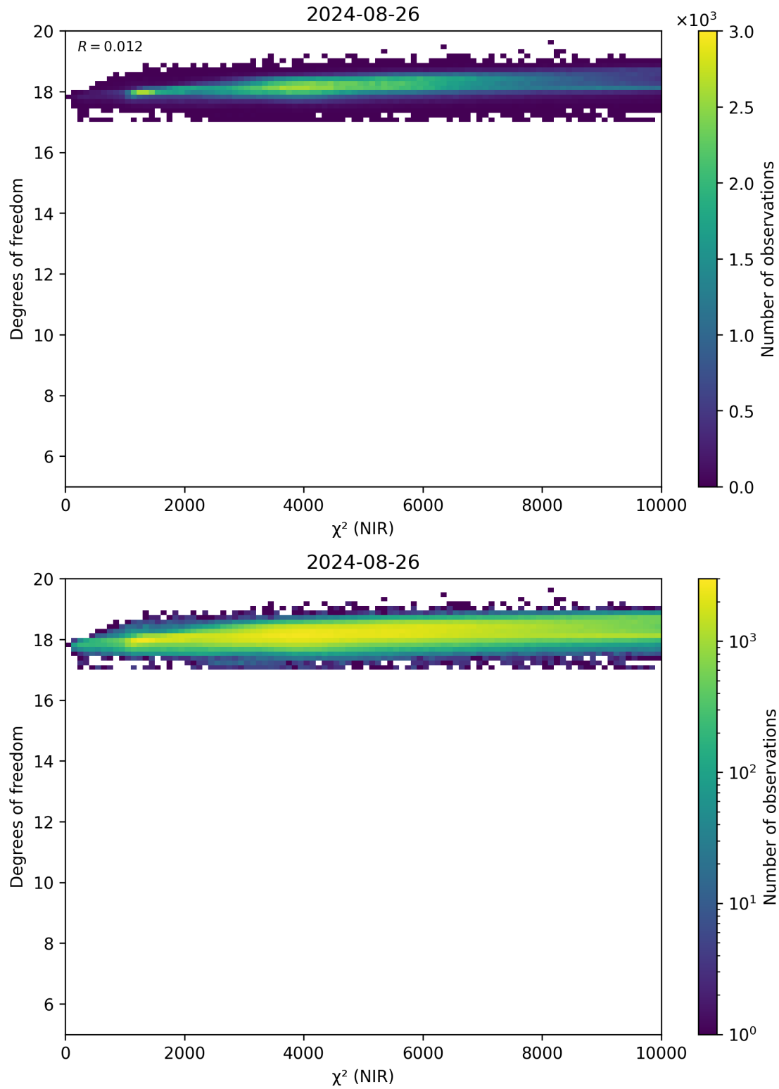
Figure 44: Scatter density plot of “ \chi^2 (NIR)” against “Degrees of freedom” for 2024-08-25 to 2024-08-27.
