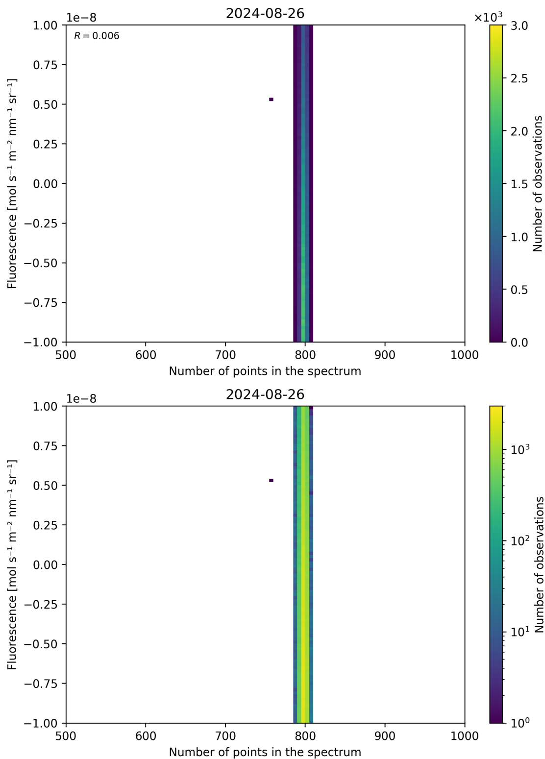
Figure 91: Scatter density plot of “Number of points in the spectrum” against “Fluorescence” for 2024-08-25 to 2024-08-27.
