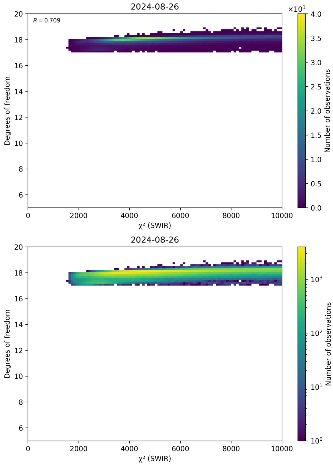
Figure 48: Scatter density plot of “ \chi^2 (SWIR)” against “Degrees of freedom” for 2024-08-25 to 2024-08-27.
