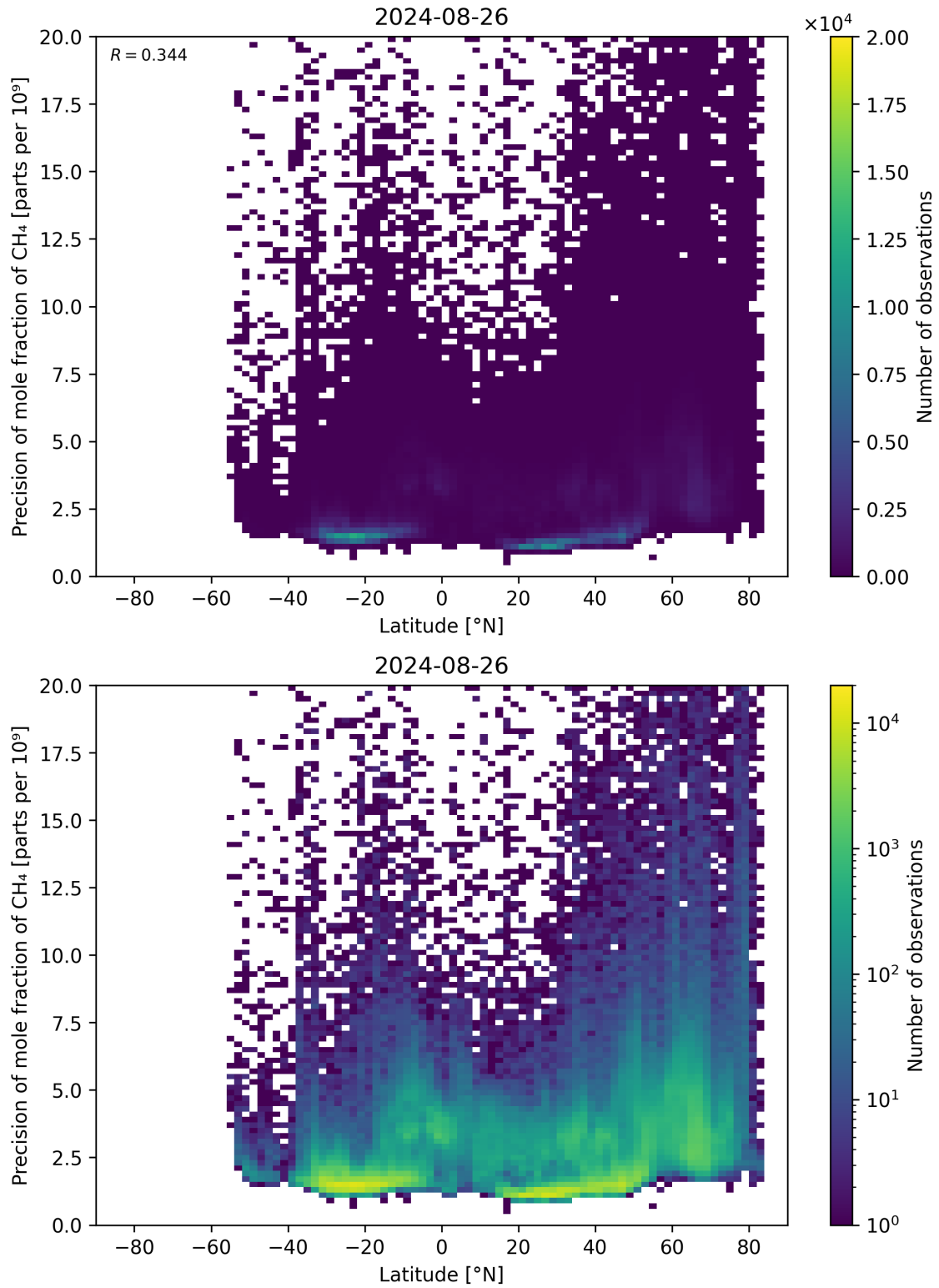
Figure 59: Scatter density plot of “Latitude” against “Precision of mole fraction of \text{CH}_4 ” for 2024-08-25 to 2024-08-27.
