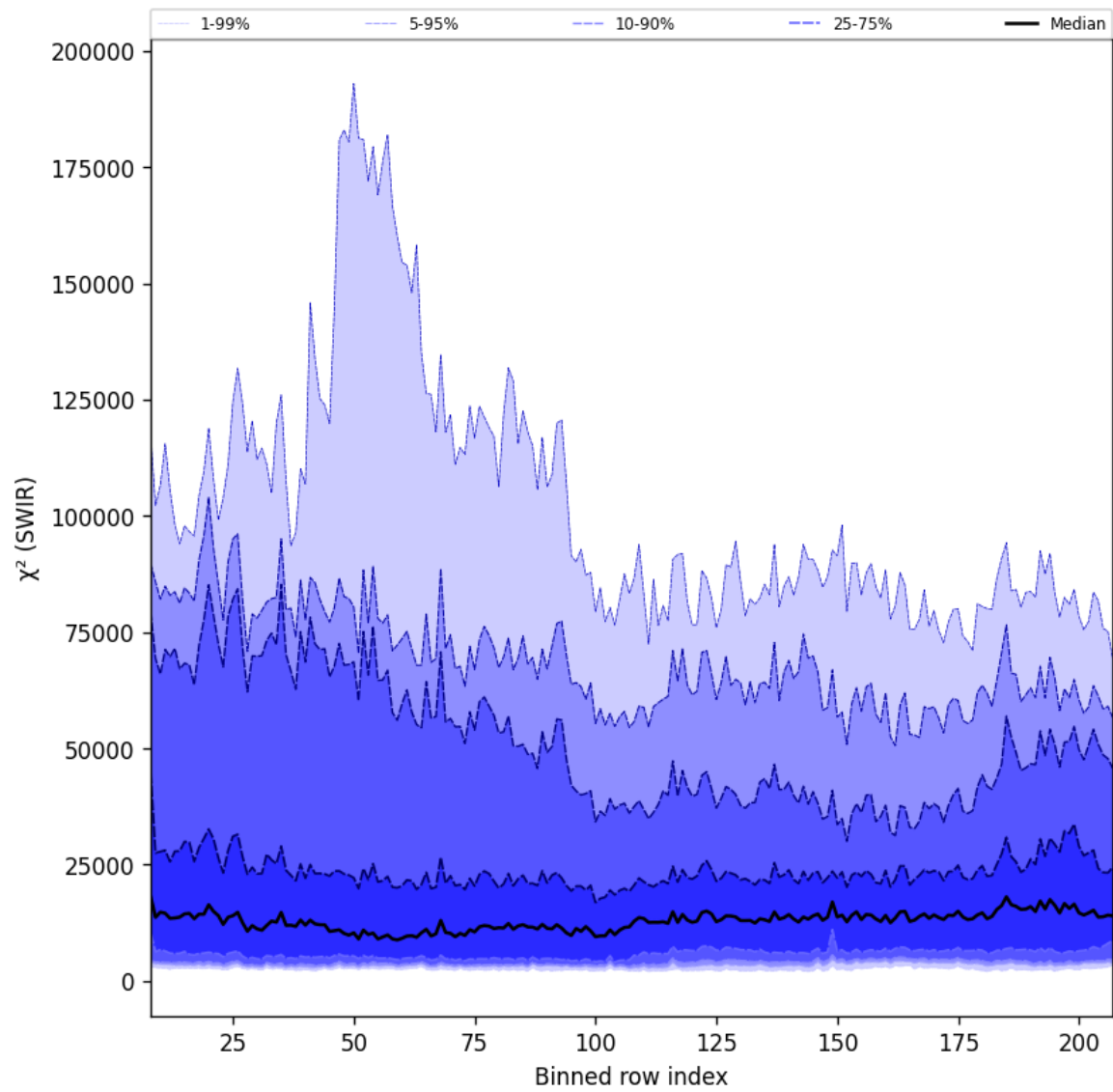
Figure 39: Along track statistics of “ \chi^2 (SWIR)” for 2024-08-25 to 2024-08-27
