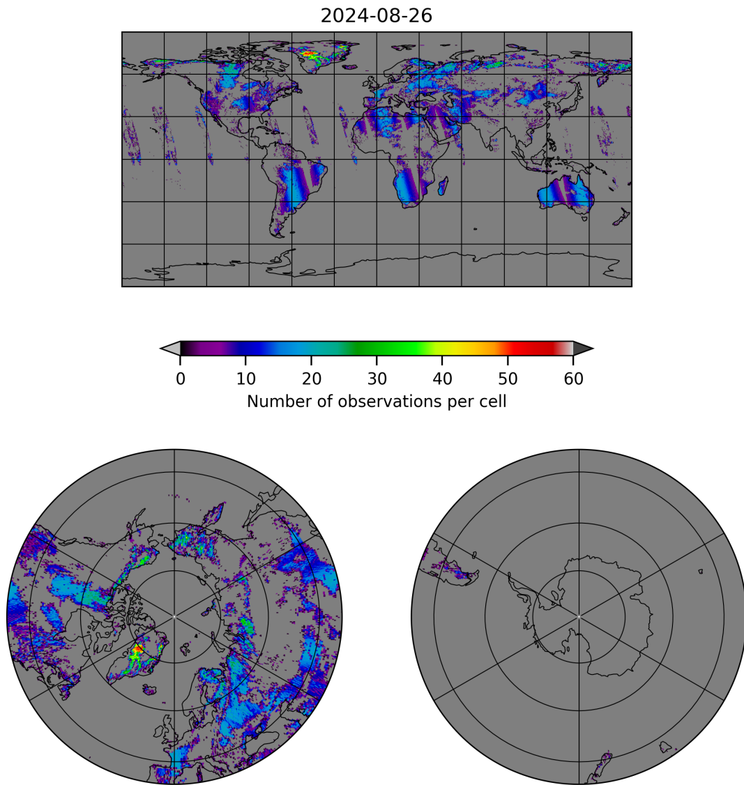
Figure 10: Map of the number of observations for 2024-08-25 to 2024-08-27
