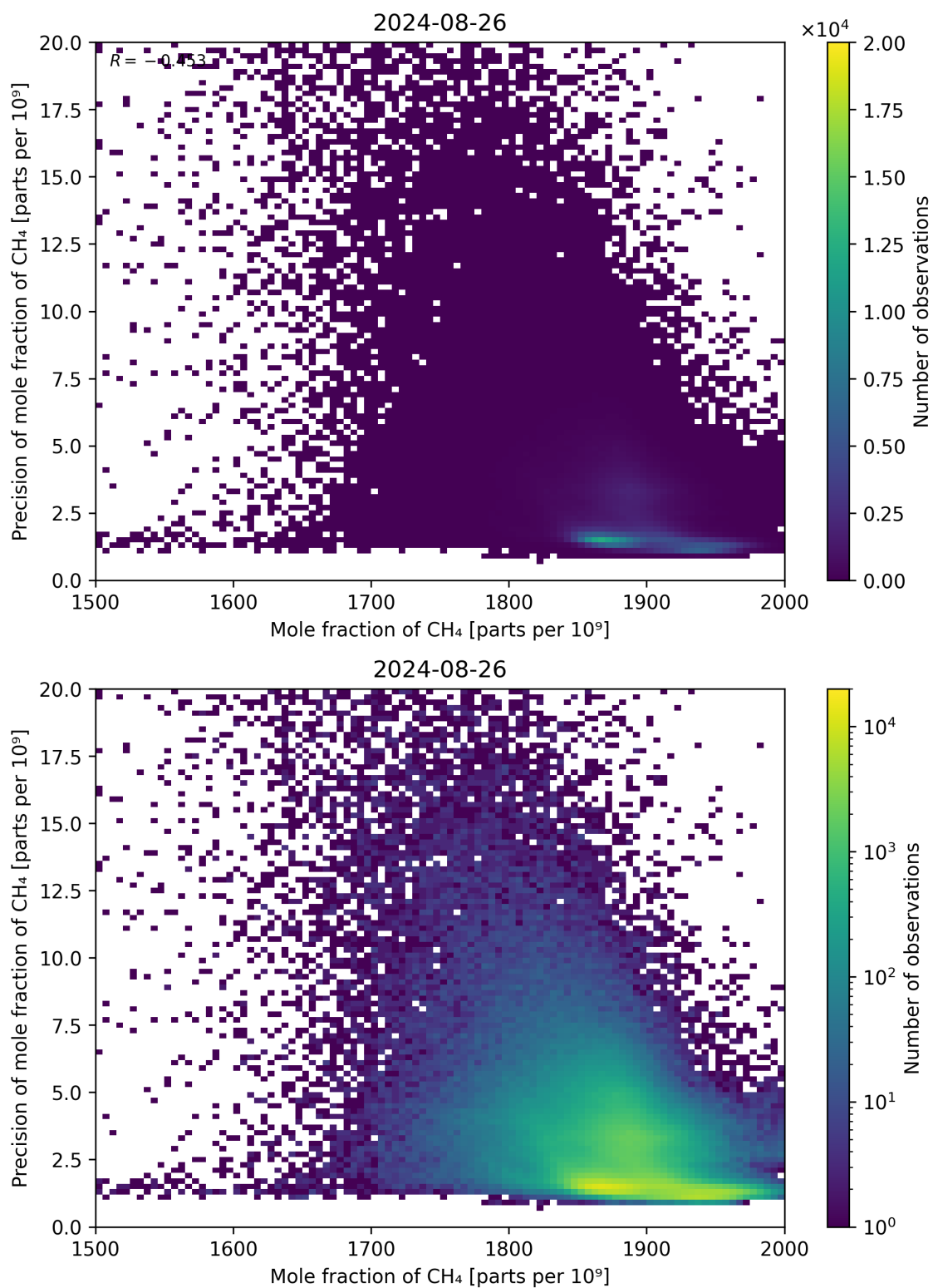
Figure 75: Scatter density plot of “Mole fraction of CH 4 ” against “Precision of mole fraction of CH 4 ” for 2024-08-25 to 2024-08-27.
