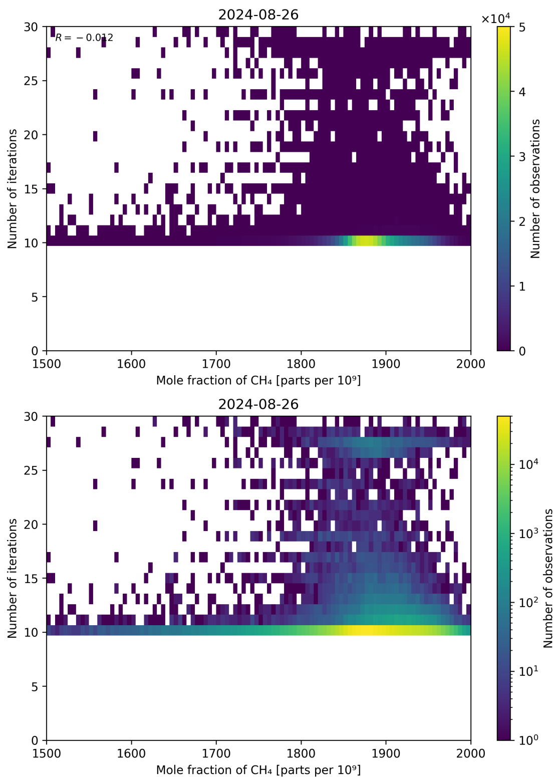
Figure 76: Scatter density plot of “Mole fraction of CH 4 ” against “Number of iterations” for 2024-08-25 to 2024-08-27.
