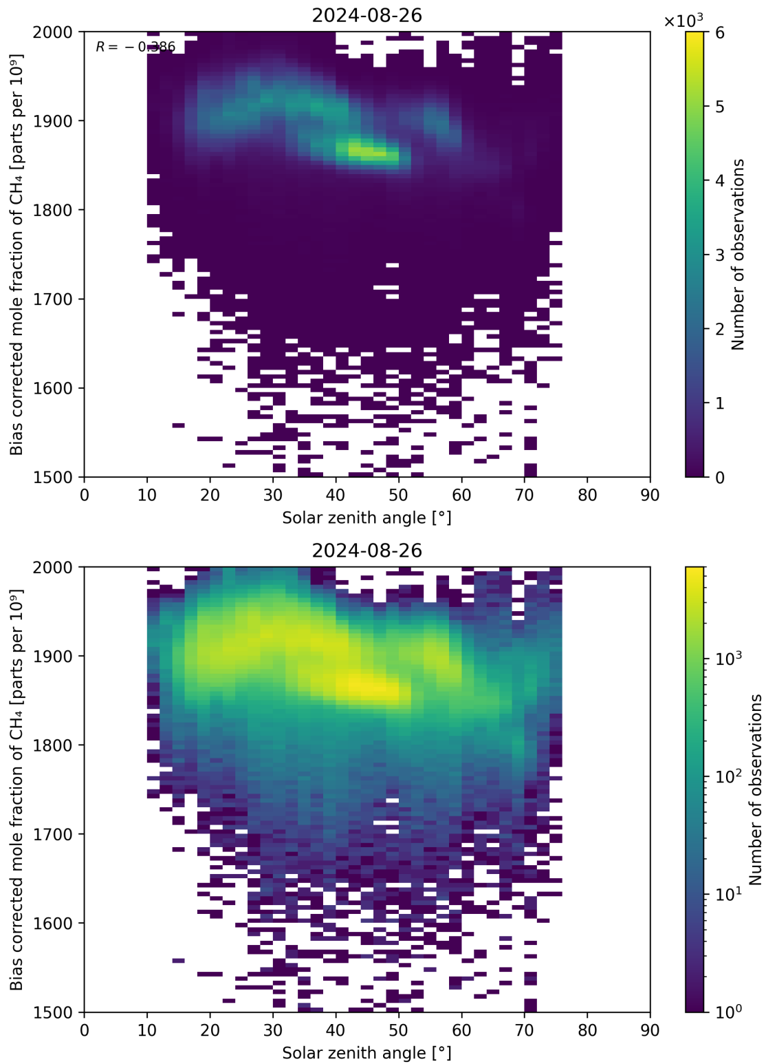
Figure 100: Scatter density plot of “Solar zenith angle” against “Bias corrected mole fraction of CH 4 ” for 2024-08-25 to 2024-08-27.
