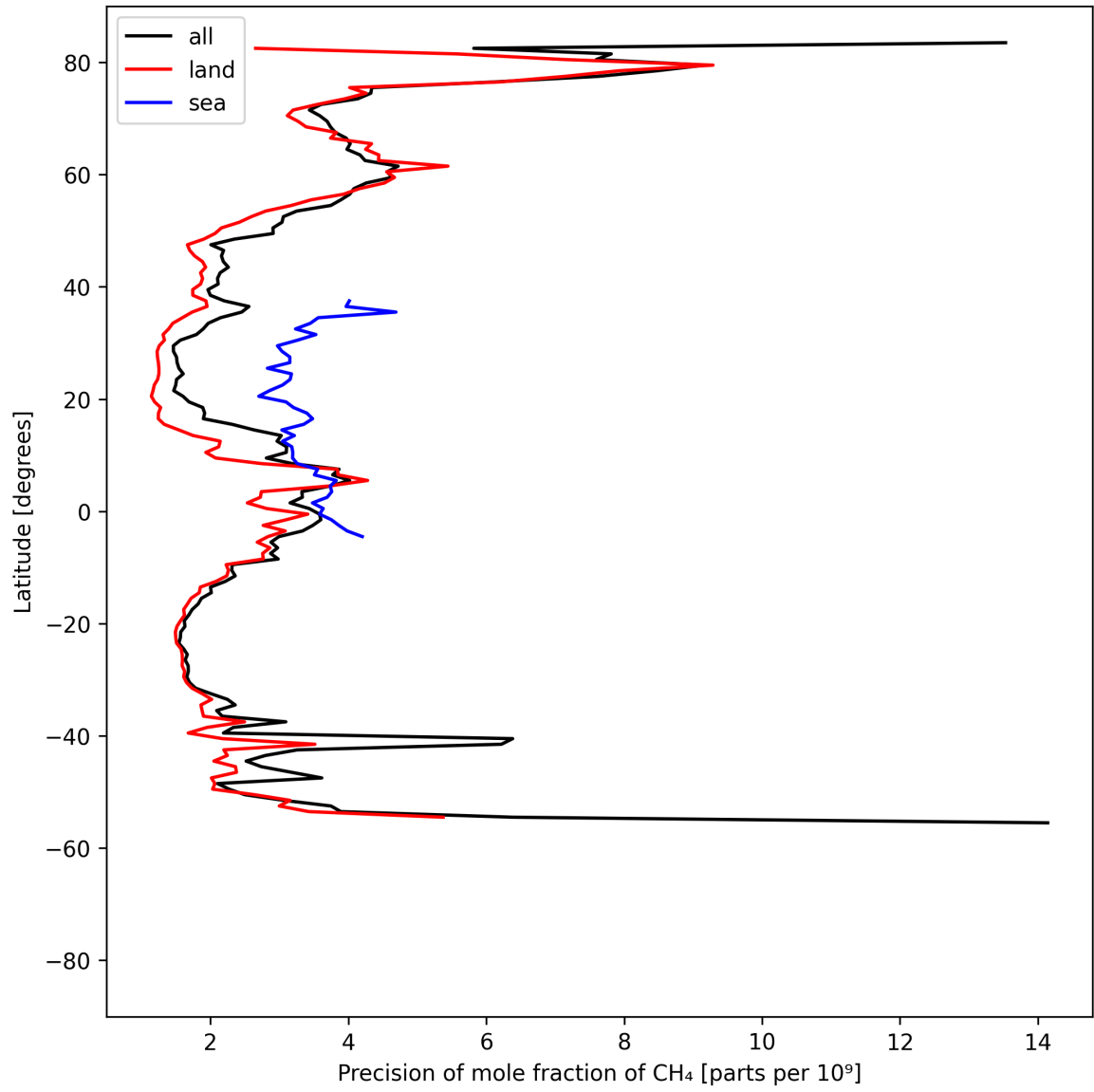
Figure 13: Zonal average of “Precision of mole fraction of CH 4 ” for 2024-08-25 to 2024-08-27.
