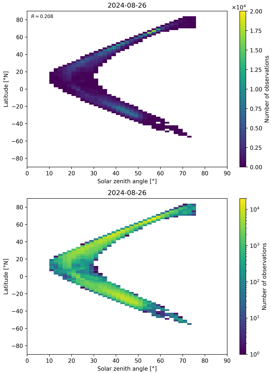
Figure 98: Scatter density plot of “Solar zenith angle” against “Latitude” for 2024-08-25 to 2024-08-27.
