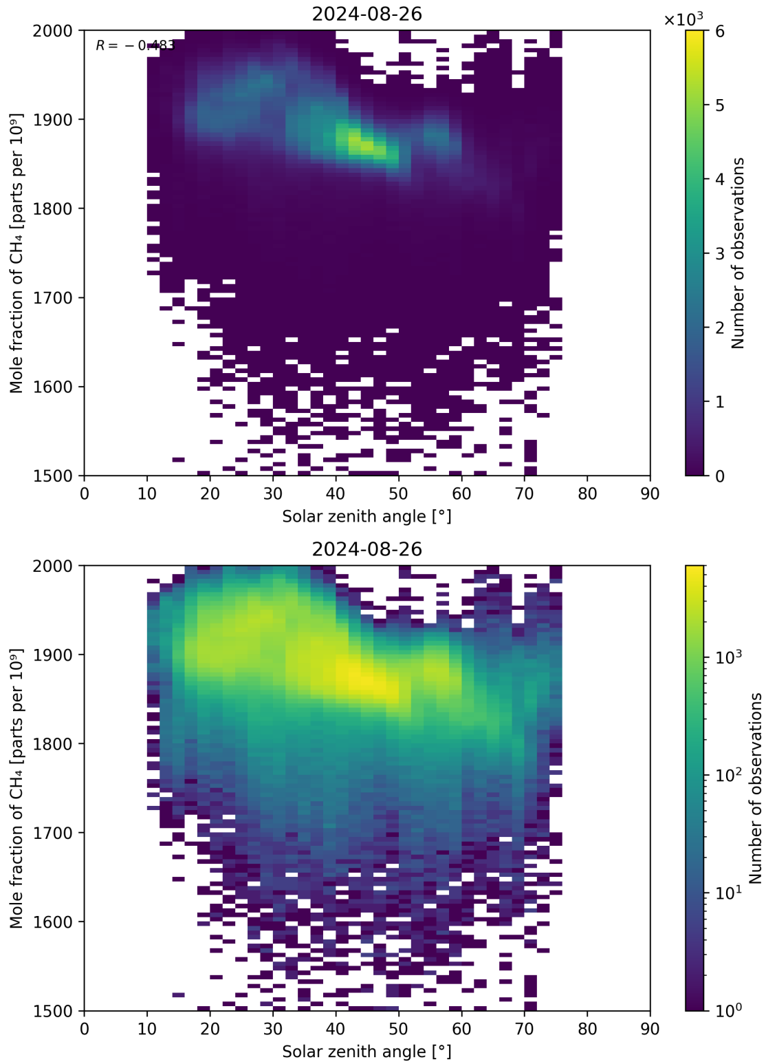
Figure 99: Scatter density plot of “Solar zenith angle” against “Mole fraction of CH 4 ” for 2024-08-25 to 2024-08-27.
