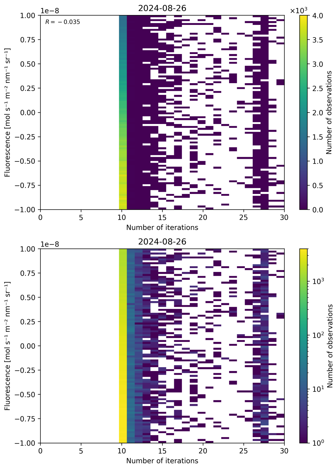
Figure 87: Scatter density plot of “Number of iterations” against “Fluorescence” for 2024-08-25 to 2024-08-27.
