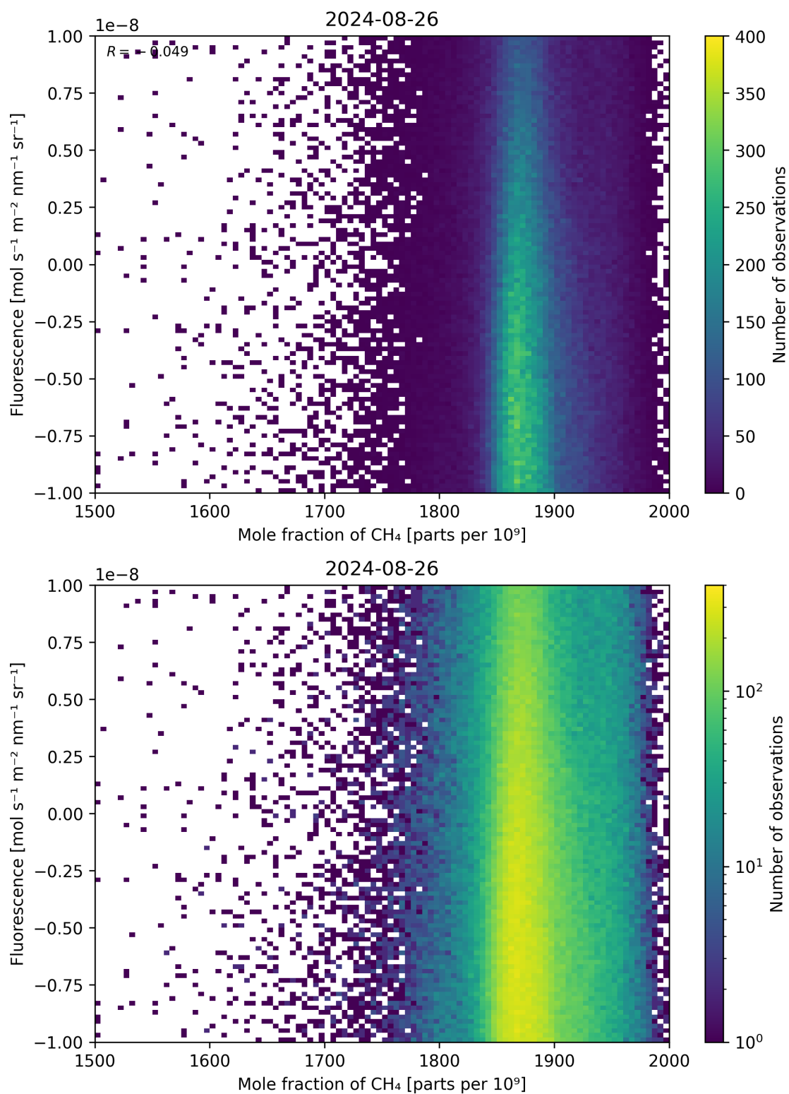
Figure 73: Scatter density plot of “Mole fraction of \text{CH}_4 ” against “Fluorescence” for 2024-08-25 to 2024-08-27.
