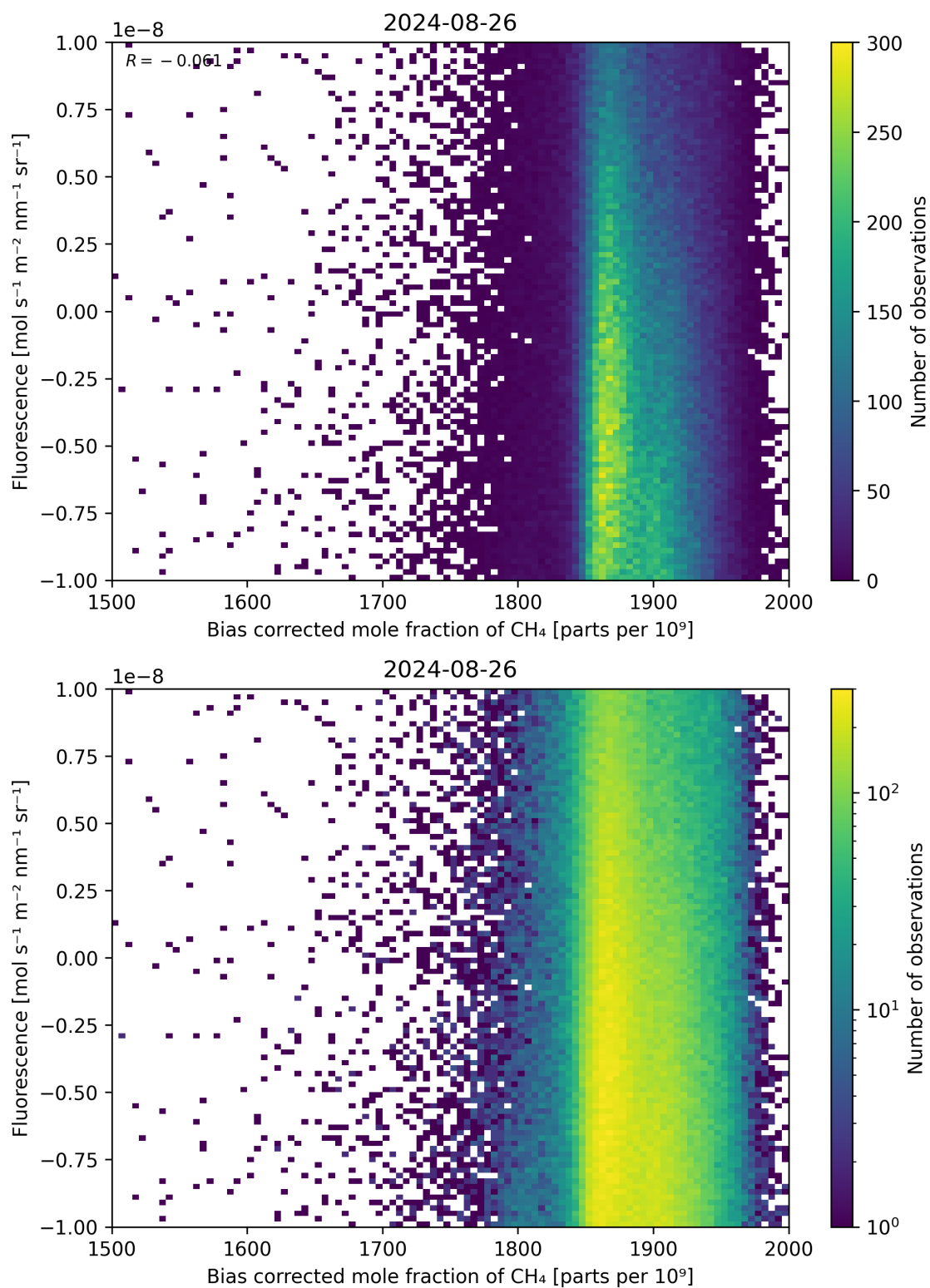
Figure 66: Scatter density plot of “Bias corrected mole fraction of CH 4 ” against “Fluorescence” for 2024-08-25 to 2024-08-27.
