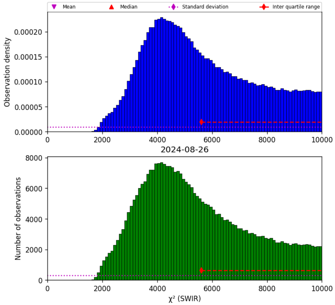
Figure 28: Histogram of “ \chi^2 (SWIR)” for 2024-08-25 to 2024-08-27
