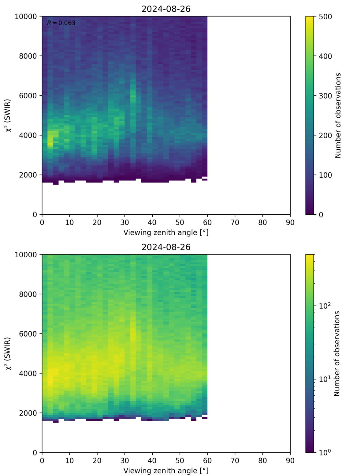
Figure 106: Scatter density plot of “Viewing zenith angle” against “ \chi^2 (SWIR)” for 2024-08-25 to 2024-08-27.
