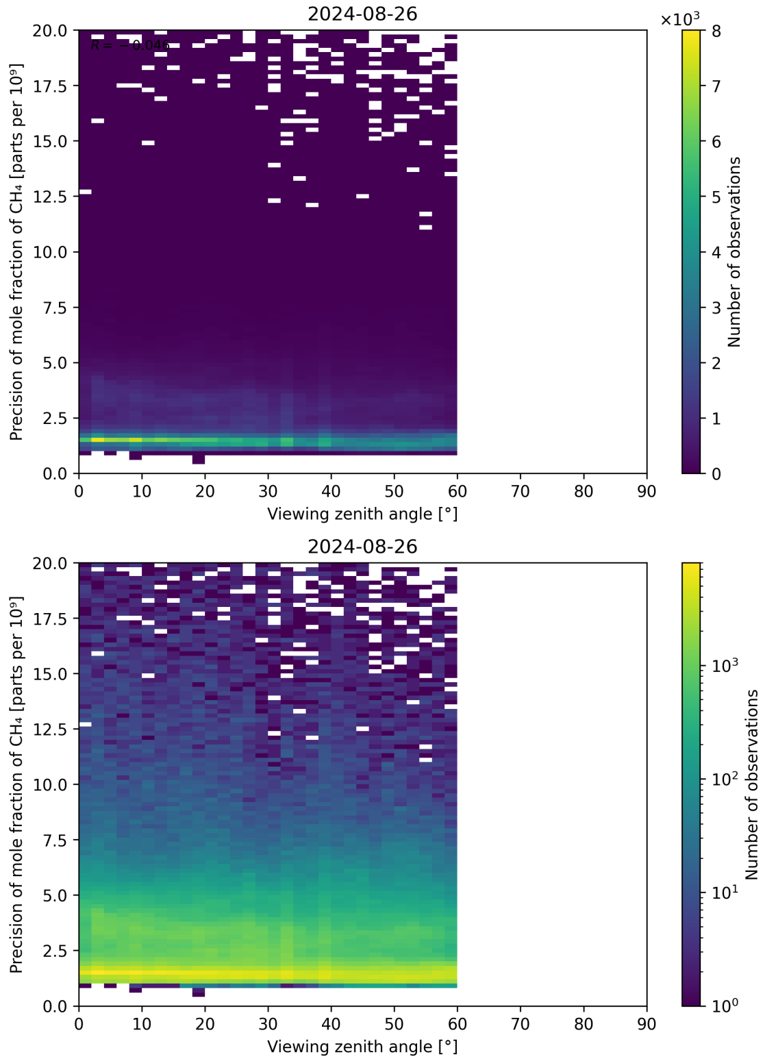
Figure 112: Scatter density plot of “Viewing zenith angle” against “Precision of mole fraction of CH 4 ” for 2024-08-25 to 2024-08-27.
