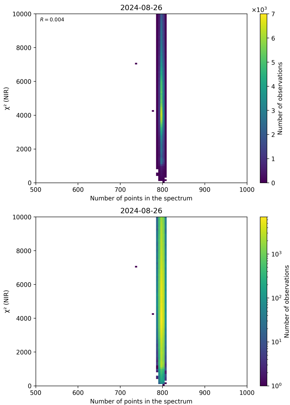
Figure 88: Scatter density plot of “Number of points in the spectrum” against “ \chi^2 (NIR)” for 2024-08-25 to 2024-08-27.
