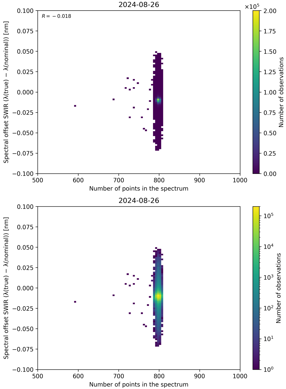
Figure 93: Scatter density plot of “Number of points in the spectrum” against “Spectral offset SWIR ( \lambda_{\text{true}} - \lambda_{\text{nominal}} )” for 2024-08-25 to 2024-08-27.
