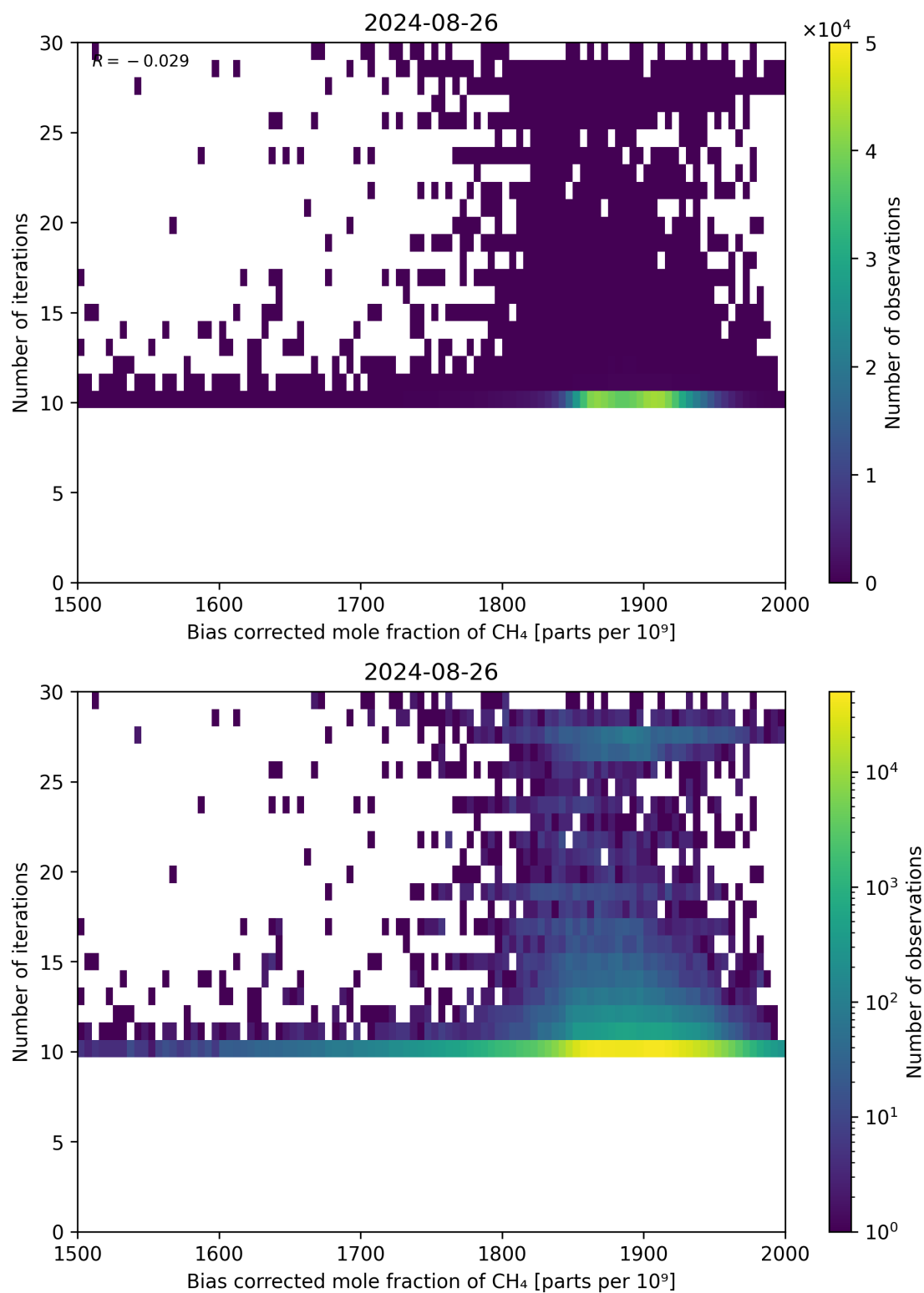
Figure 67: Scatter density plot of “Bias corrected mole fraction of CH 4 ” against “Number of iterations” for 2024-08-25 to 2024-08-27.
