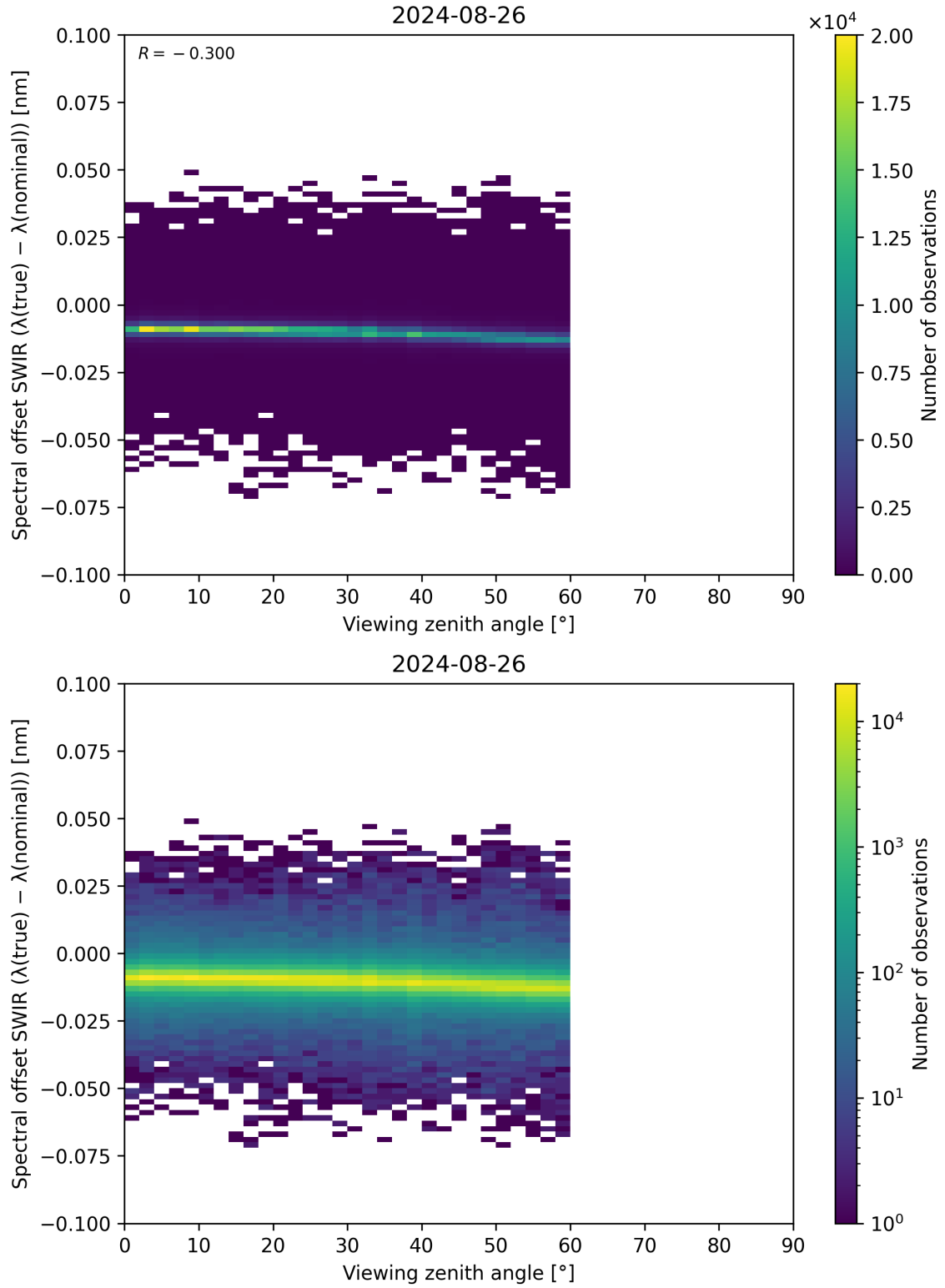
Figure 116: Scatter density plot of “Viewing zenith angle” against “Spectral offset SWIR ( \lambda_{\text{true}} - \lambda_{\text{nominal}} )” for 2024-08-25 to 2024-08-27.
