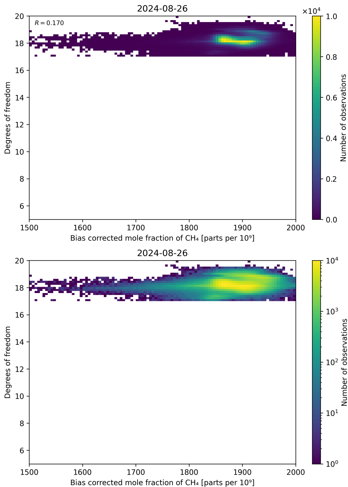
Figure 65: Scatter density plot of “Bias corrected mole fraction of CH 4 ” against “Degrees of freedom” for 2024-08-25 to 2024-08-27.
