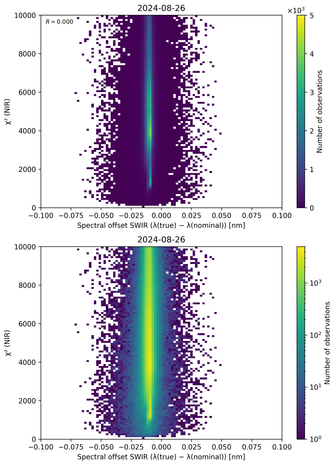
Figure 117: Scatter density plot of “Spectral offset SWIR ( \lambda_{\text{true}} - \lambda_{\text{nominal}} )” against “ \chi^2 (NIR)” for 2024-08-25 to 2024-08-27.
