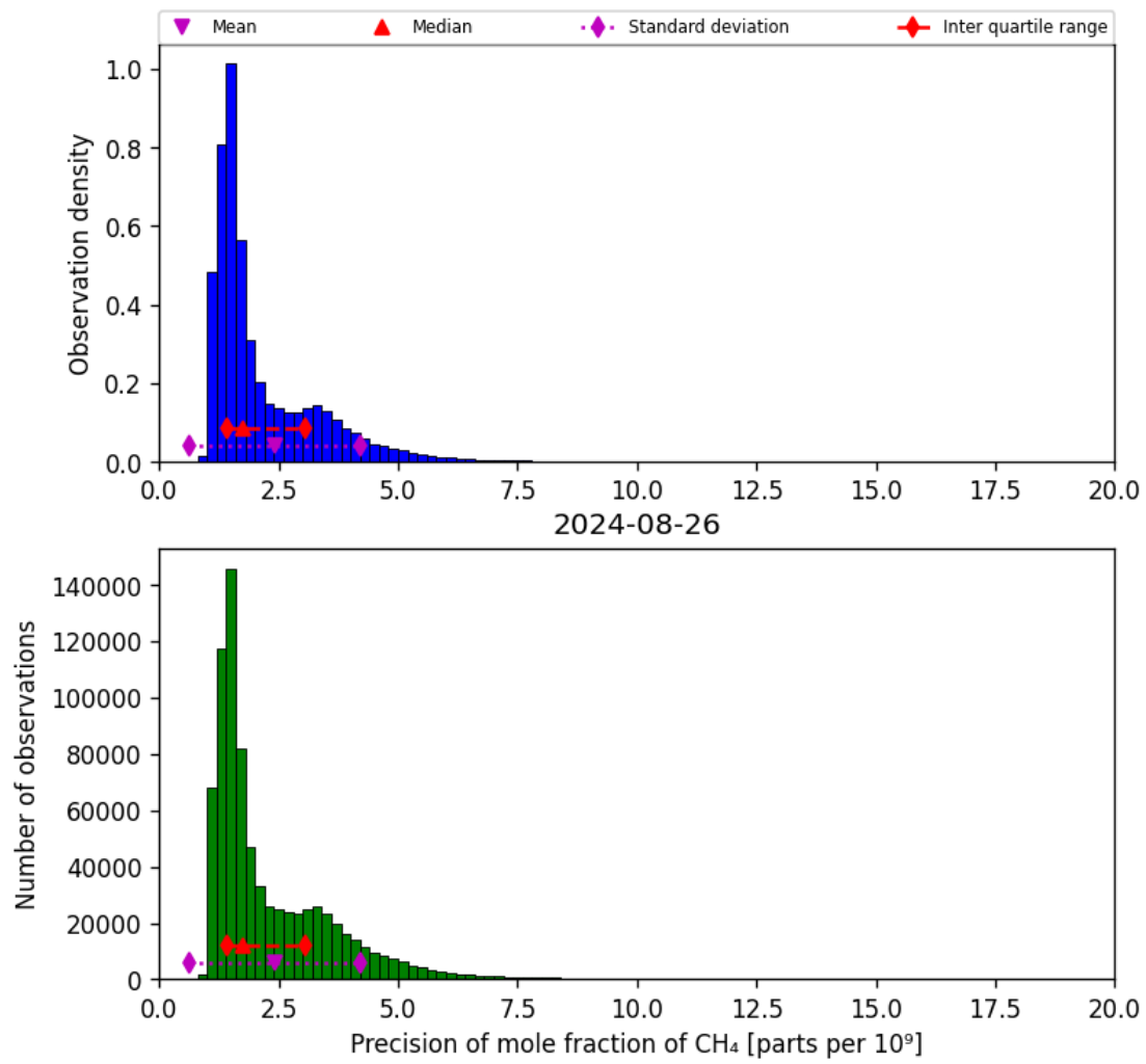
Figure 24: Histogram of “Precision of mole fraction of CH 4 ” for 2024-08-25 to 2024-08-27
