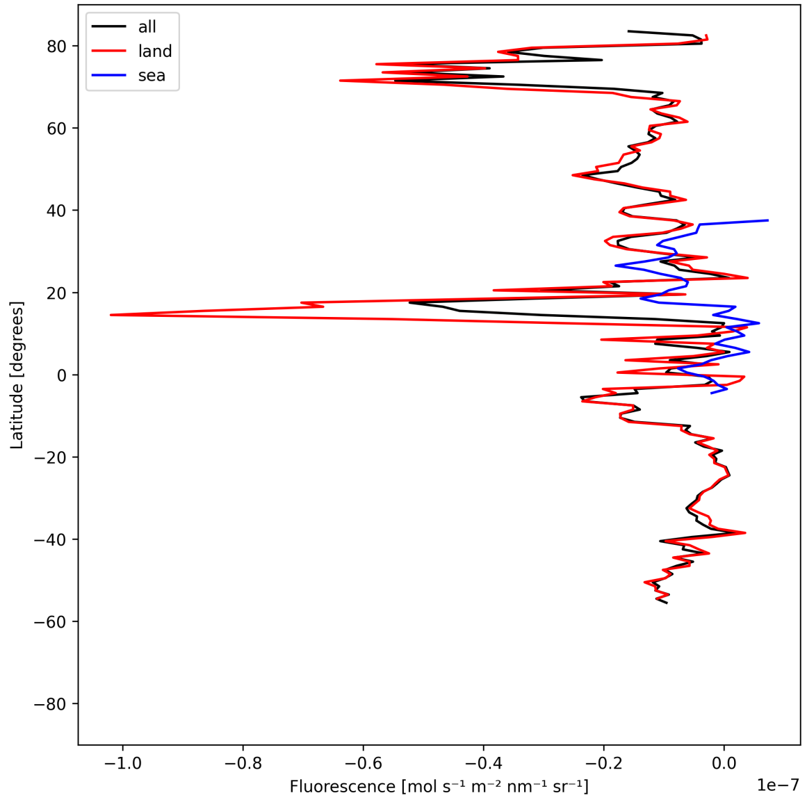
Figure 21: Zonal average of “Fluorescence” for 2024-08-25 to 2024-08-27.
