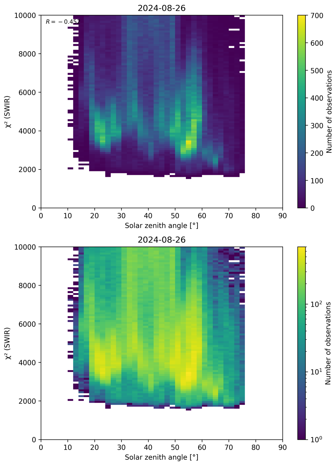
Figure 95: Scatter density plot of “Solar zenith angle” against “ \chi^2 (SWIR)” for 2024-08-25 to 2024-08-27.
