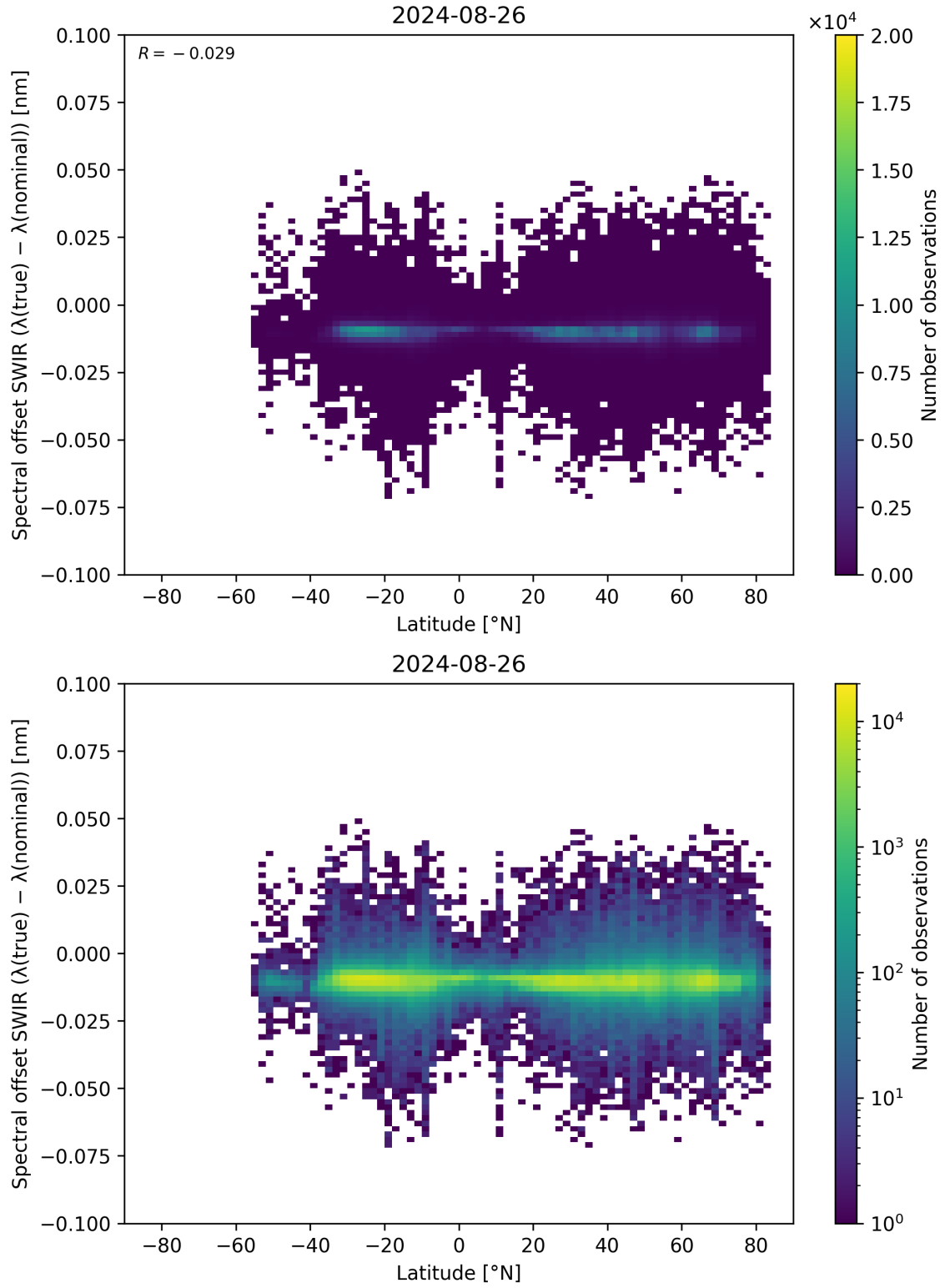
Figure 62: Scatter density plot of “Latitude” against “Spectral offset SWIR ( \lambda_{\text{true}} - \lambda_{\text{nominal}} )” for 2024-08-25 to 2024-08-27.
