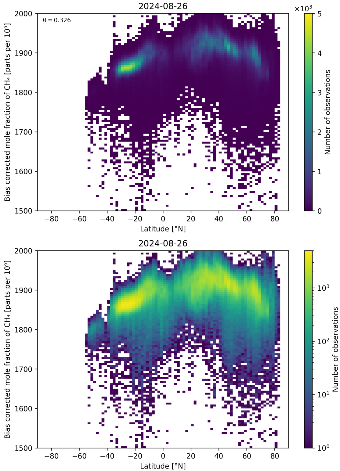
Figure 58: Scatter density plot of “Latitude” against “Bias corrected mole fraction of CH 4 ” for 2024-08-25 to 2024-08-27.
