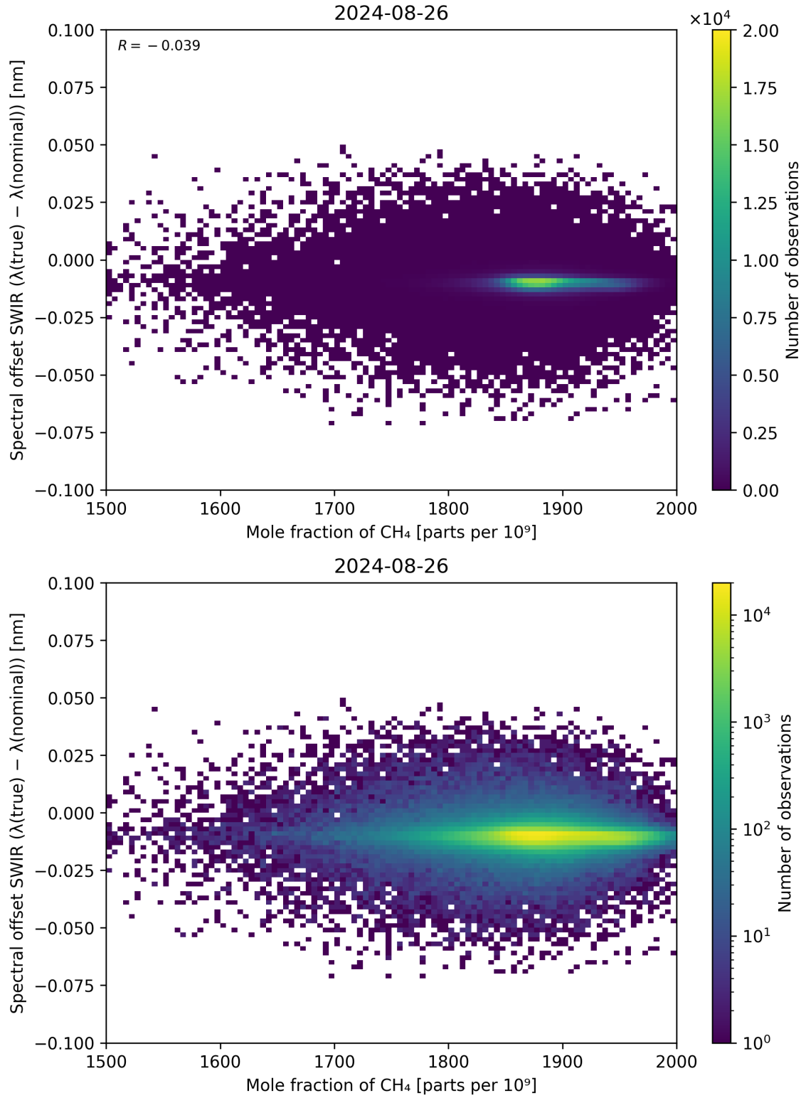
Figure 86: Scatter density plot of “Mole fraction of CH 4 ” against “Spectral offset SWIR ( \lambda_{\text{true}} - \lambda_{\text{nominal}} )” for 2024-08-25 to 2024-08-27.
