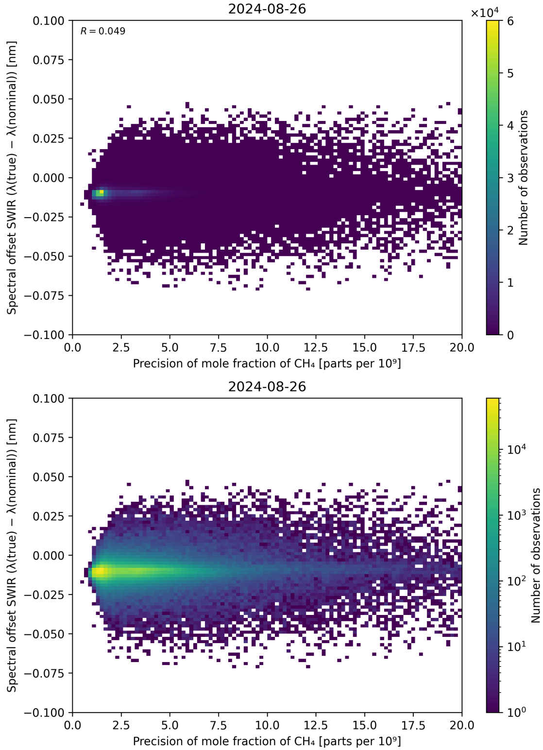
Figure 85: Scatter density plot of “Precision of mole fraction of CH 4 ” against “Spectral offset SWIR ( \lambda_{\text{true}} - \lambda_{\text{nominal}} )” for 2024-08-25 to 2024-08-27.
