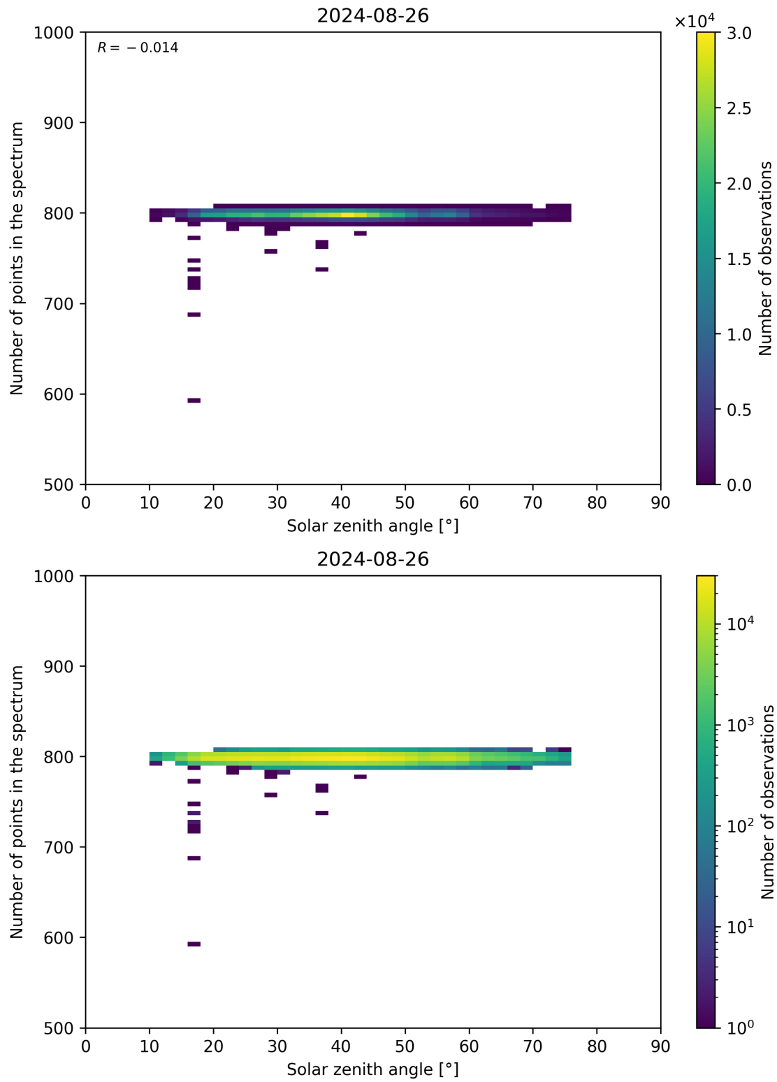
Figure 103: Scatter density plot of “Solar zenith angle” against “Number of points in the spectrum” for 2024-08-25 to 2024-08-27.
