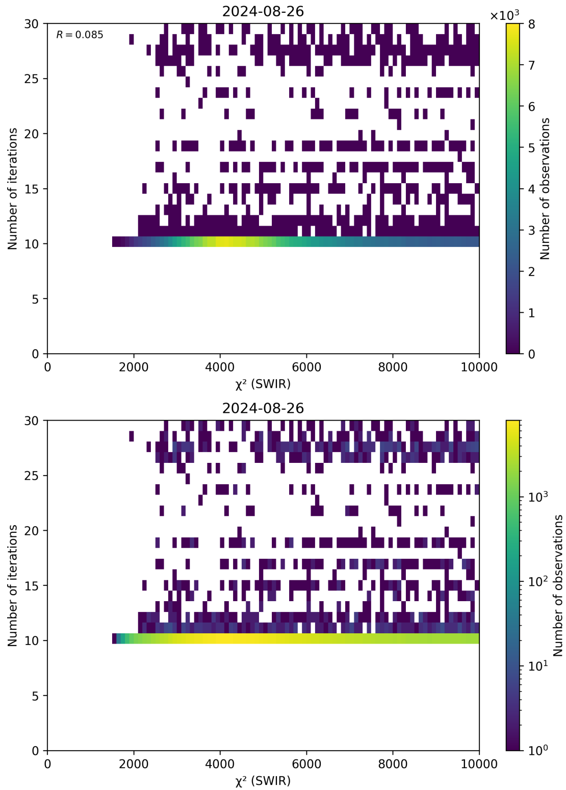
Figure 50: Scatter density plot of “ \chi^2 (SWIR)” against “Number of iterations” for 2024-08-25 to 2024-08-27.
