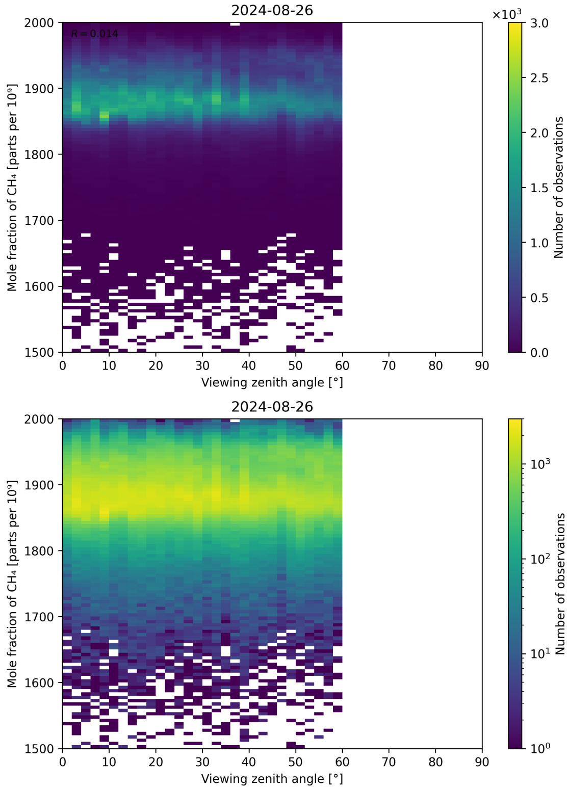
Figure 110: Scatter density plot of “Viewing zenith angle” against “Mole fraction of CH 4 ” for 2024-08-25 to 2024-08-27.
