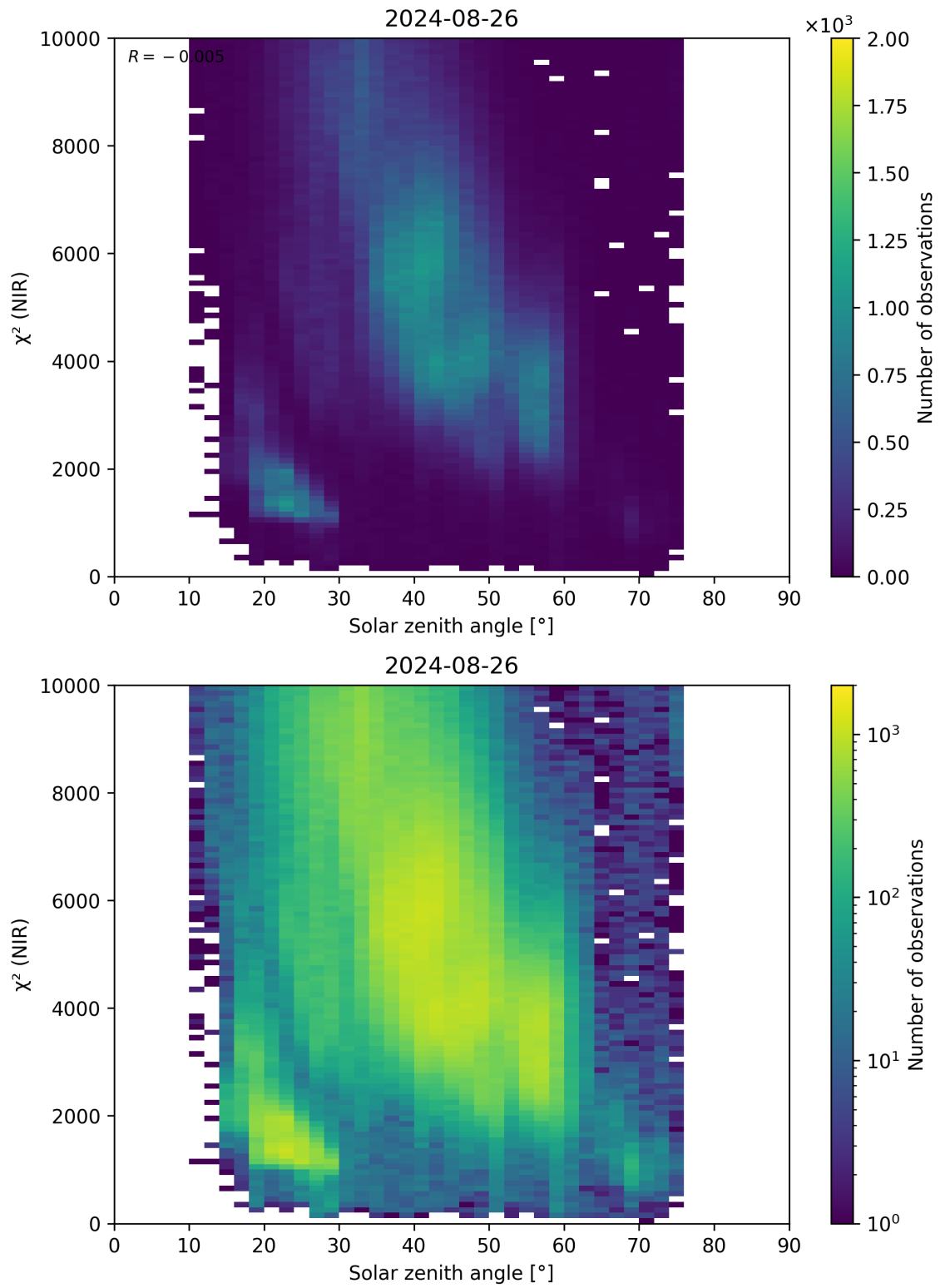
Figure 94: Scatter density plot of “Solar zenith angle” against “ \chi^2 (NIR)” for 2024-08-25 to 2024-08-27.
