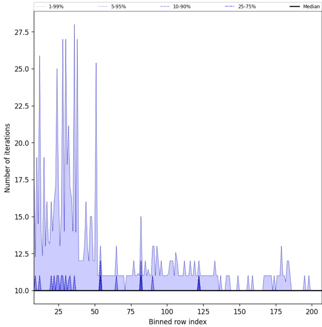
Figure 42: Along track statistics of “Number of iterations” for 2024-08-25 to 2024-08-27
