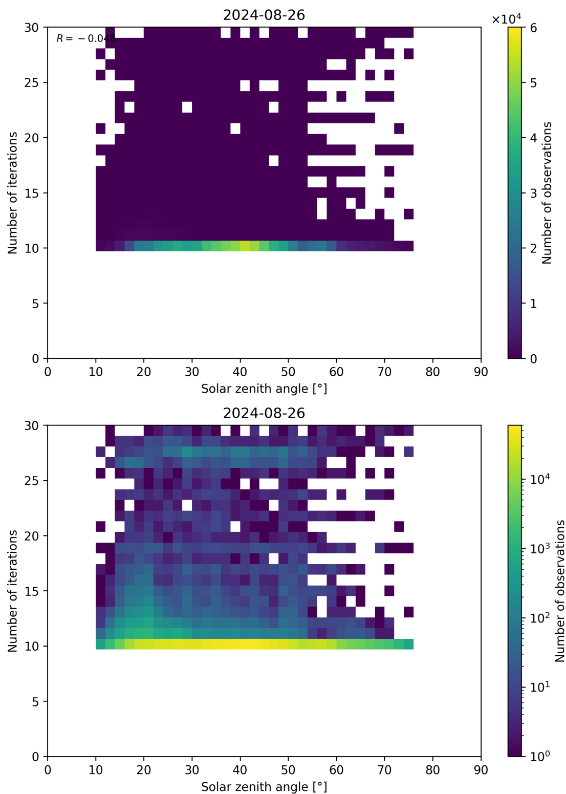
Figure 102: Scatter density plot of “Solar zenith angle” against “Number of iterations” for 2024-08-25 to 2024-08-27.
