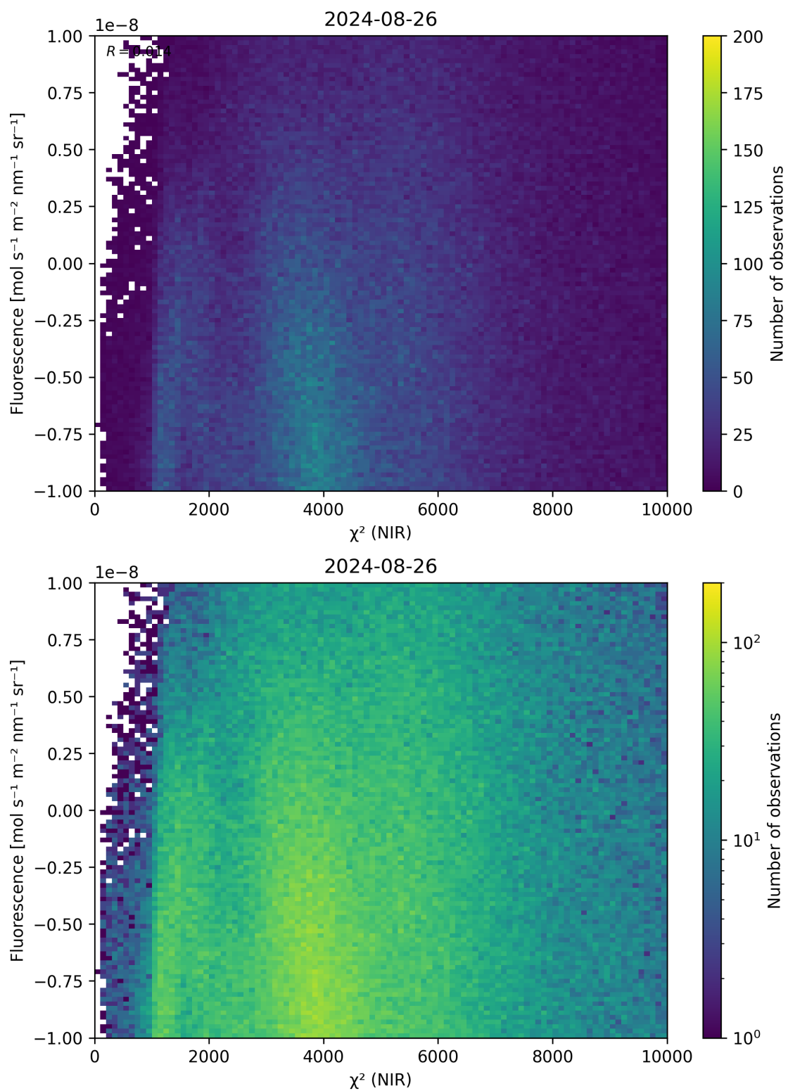
Figure 45: Scatter density plot of “ \chi^2 (NIR)” against “Fluorescence” for 2024-08-25 to 2024-08-27.
