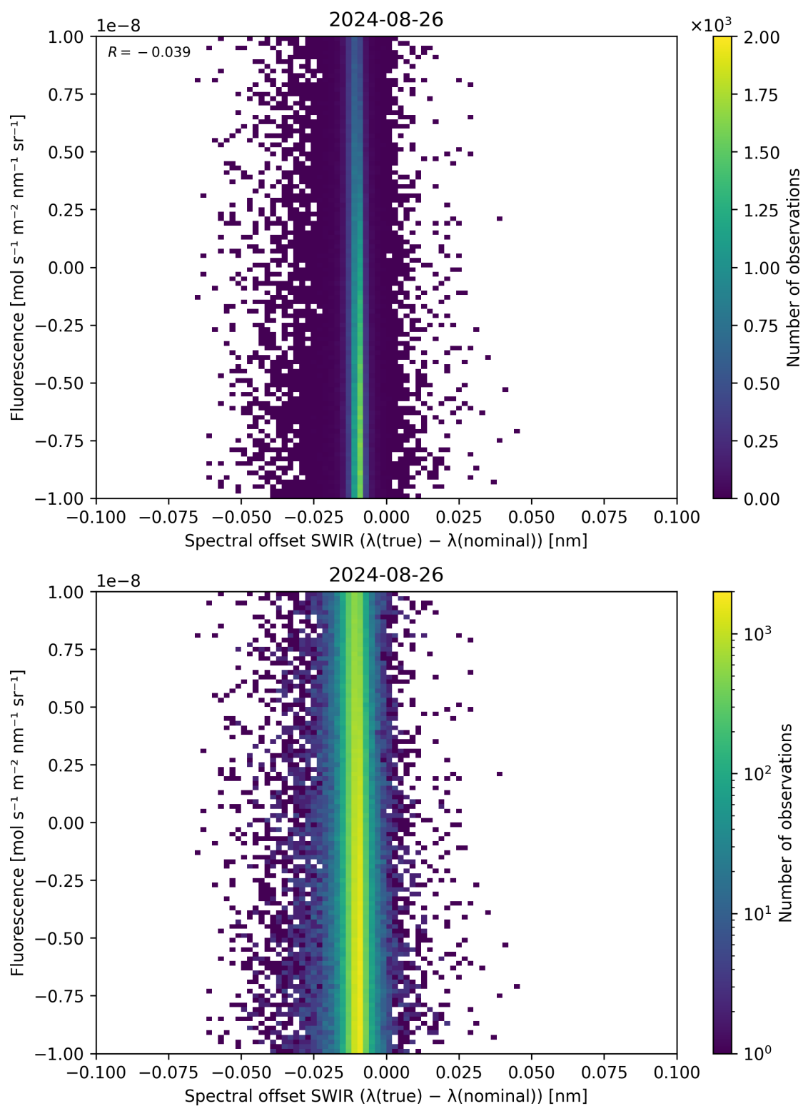
Figure 120: Scatter density plot of “Spectral offset SWIR ( \lambda_{\text{true}} - \lambda_{\text{nominal}} )” against “Fluorescence” for 2024-08-25 to 2024-08-27.
