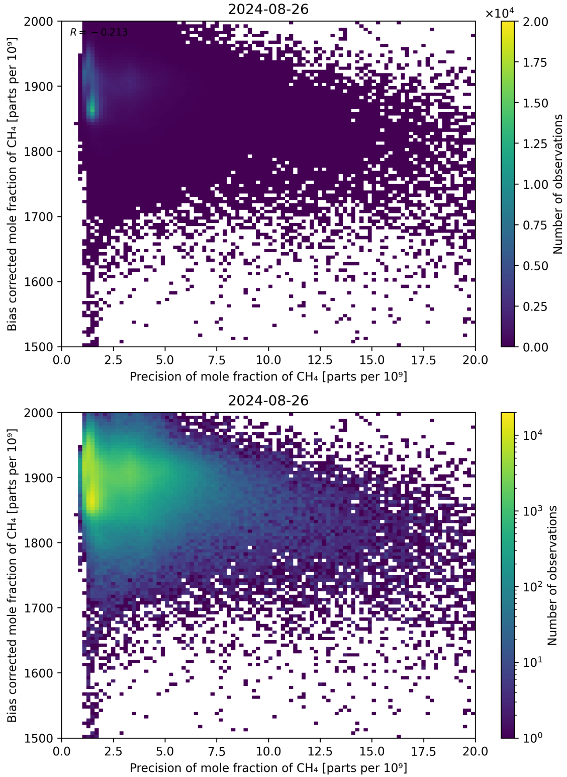
Figure 82: Scatter density plot of “Precision of mole fraction of CH 4 ” against “Bias corrected mole fraction of CH 4 ” for 2024-08-25 to 2024-08-27.
