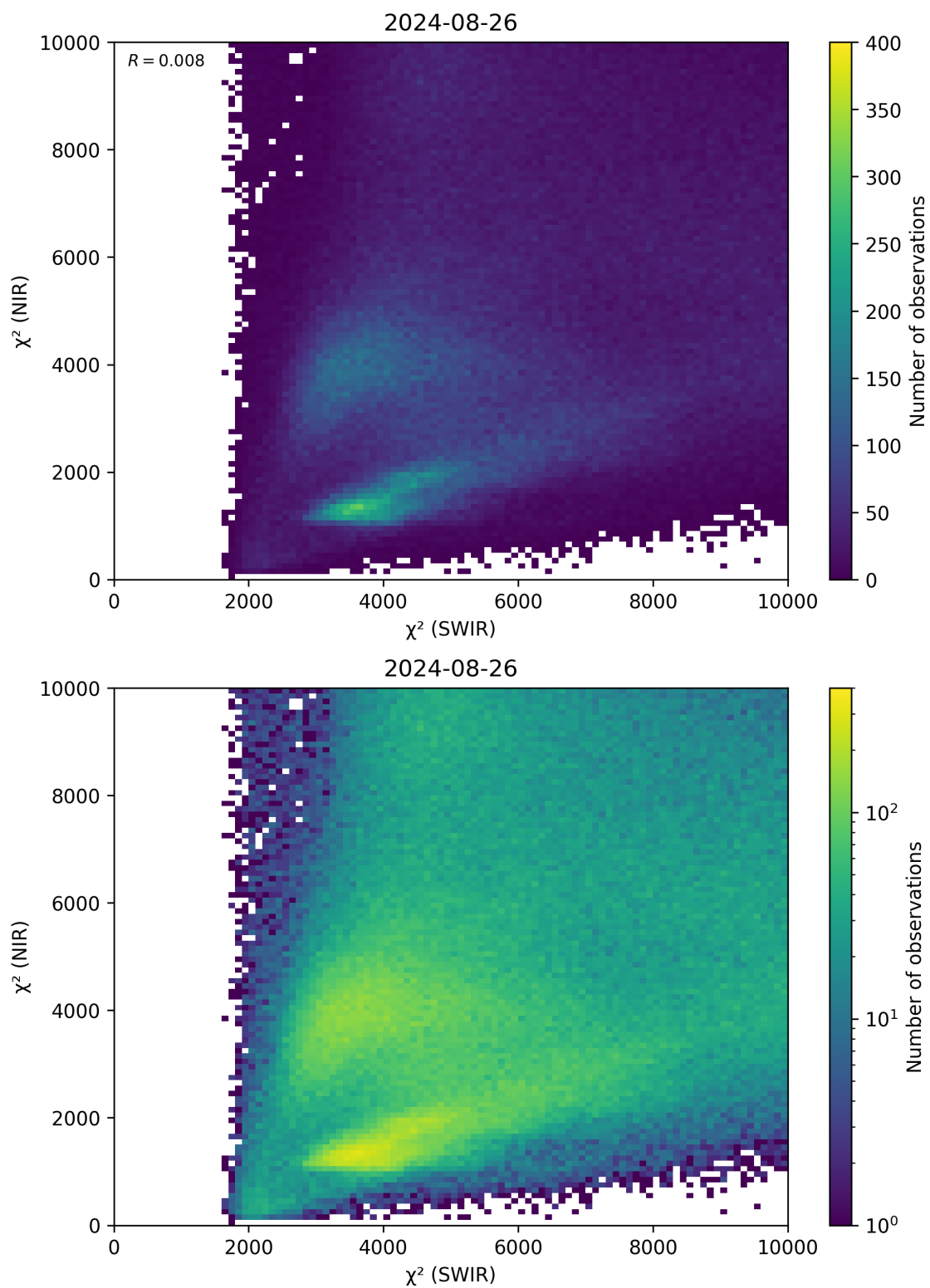
Figure 47: Scatter density plot of “ \chi^2 (SWIR)” against “ \chi^2 (NIR)” for 2024-08-25 to 2024-08-27.
