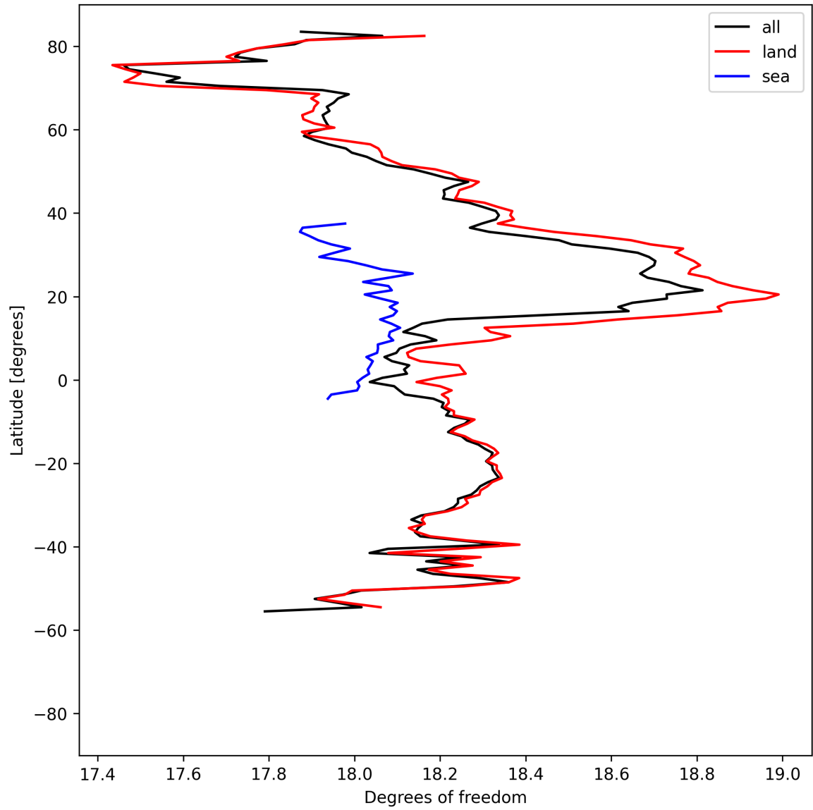
Figure 19: Zonal average of “Degrees of freedom” for 2024-08-25 to 2024-08-27.
