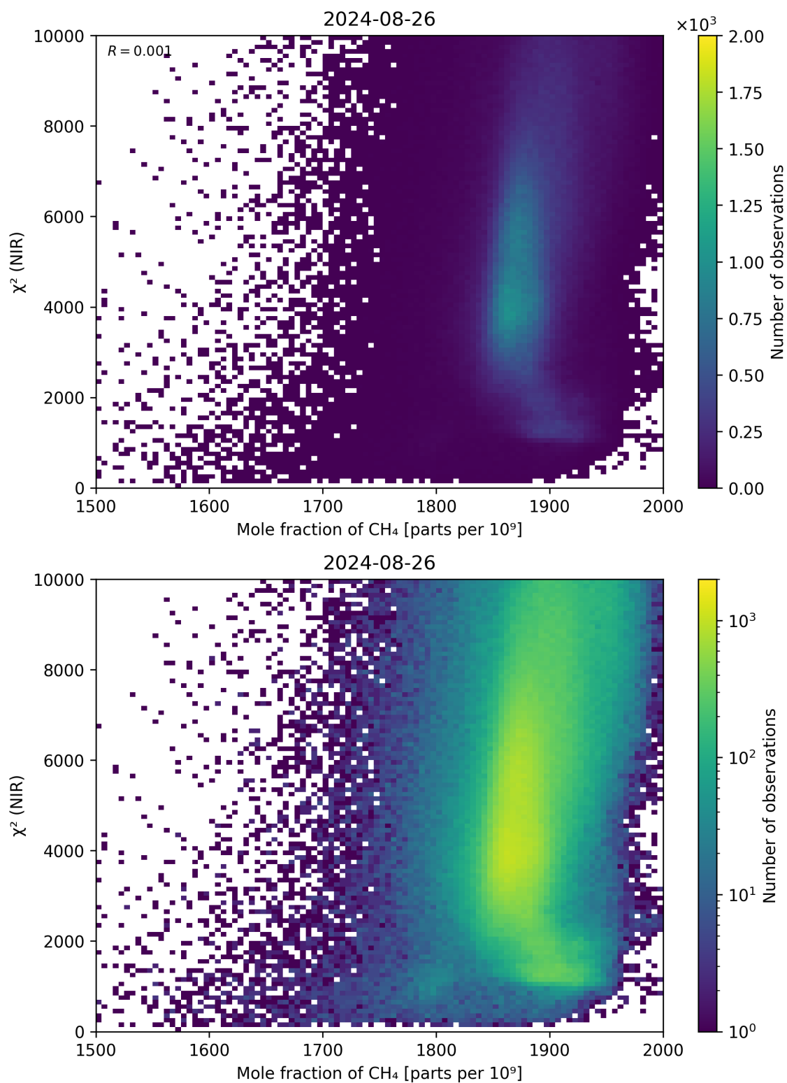
Figure 70: Scatter density plot of “Mole fraction of \text{CH}_4 ” against “ \chi^2 (NIR)” for 2024-08-25 to 2024-08-27.
