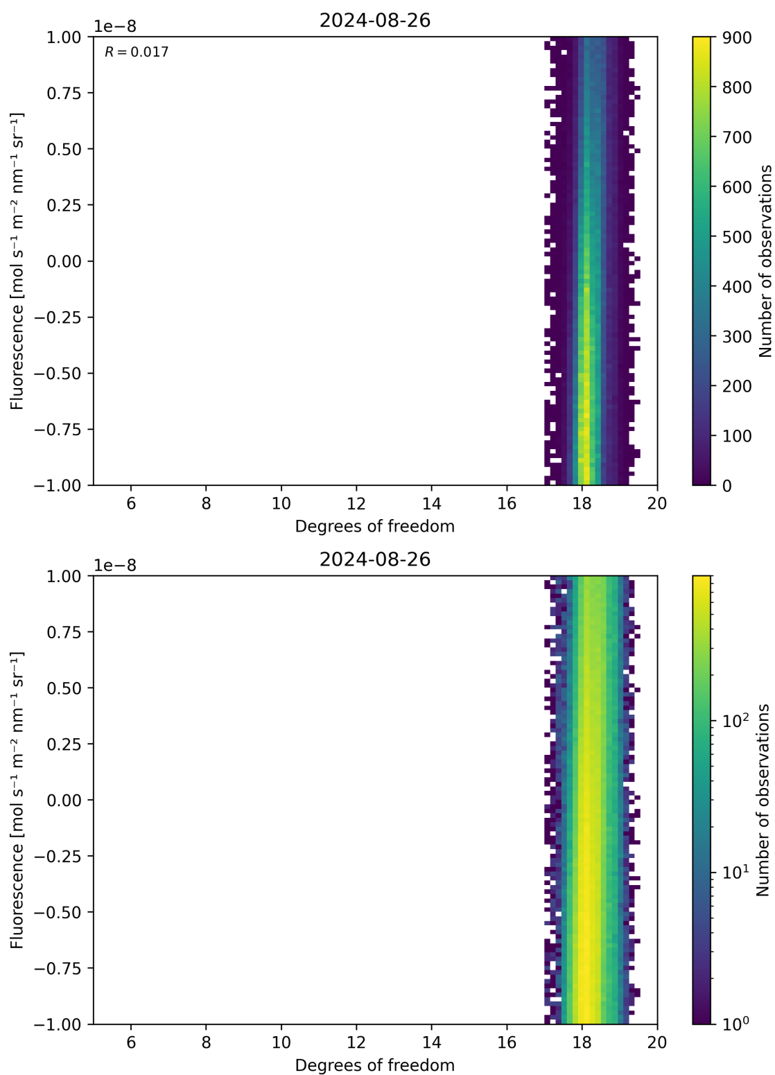
Figure 51: Scatter density plot of “Degrees of freedom” against “Fluorescence” for 2024-08-25 to 2024-08-27.
