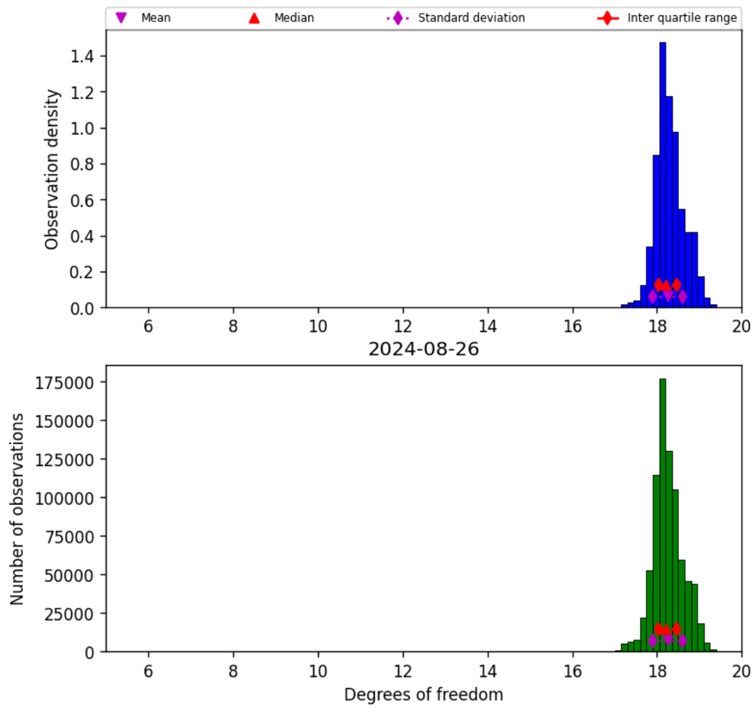
Figure 30: Histogram of “Degrees of freedom” for 2024-08-25 to 2024-08-27
