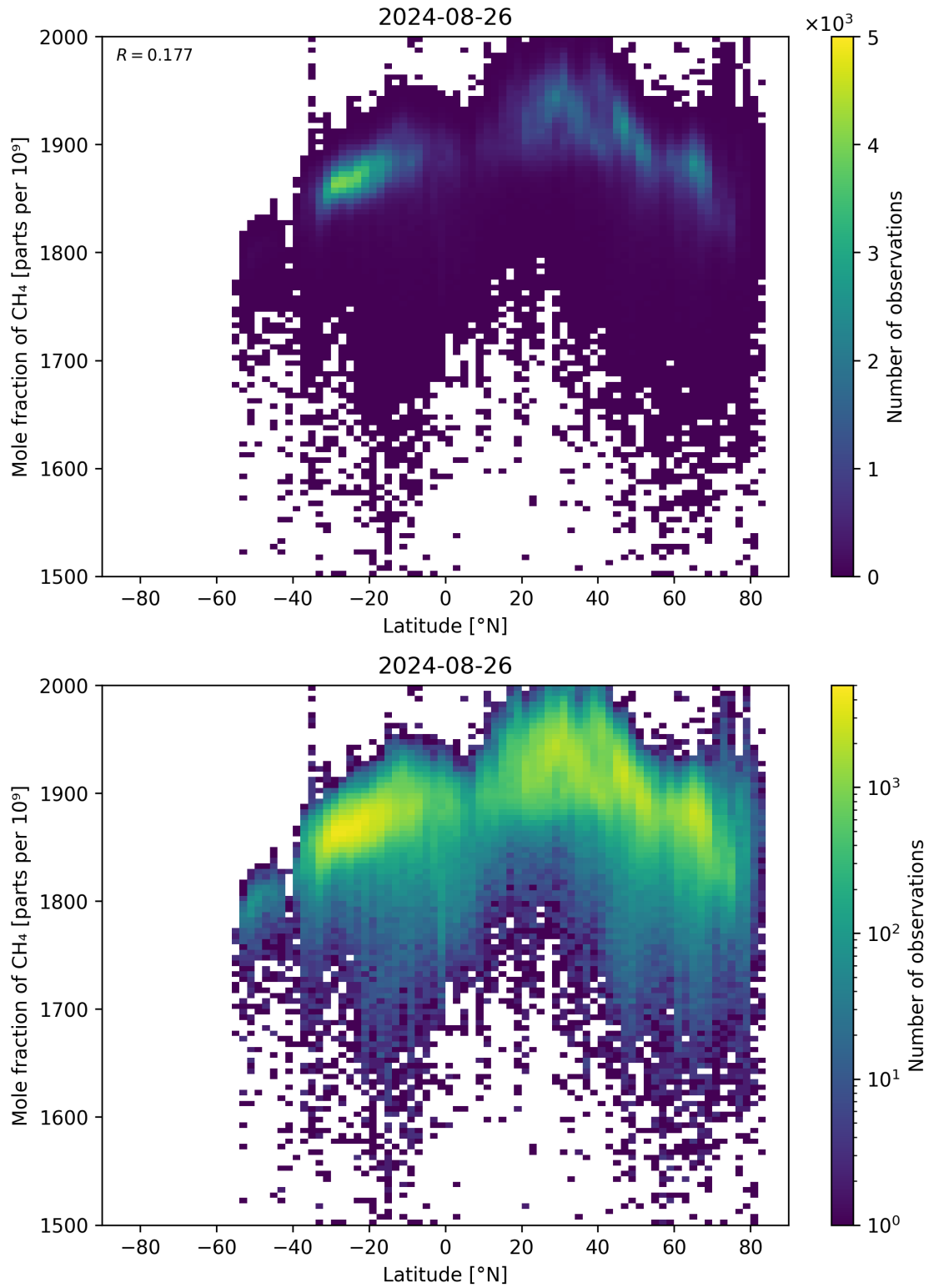
Figure 57: Scatter density plot of “Latitude” against “Mole fraction of CH 4 ” for 2024-08-25 to 2024-08-27.
