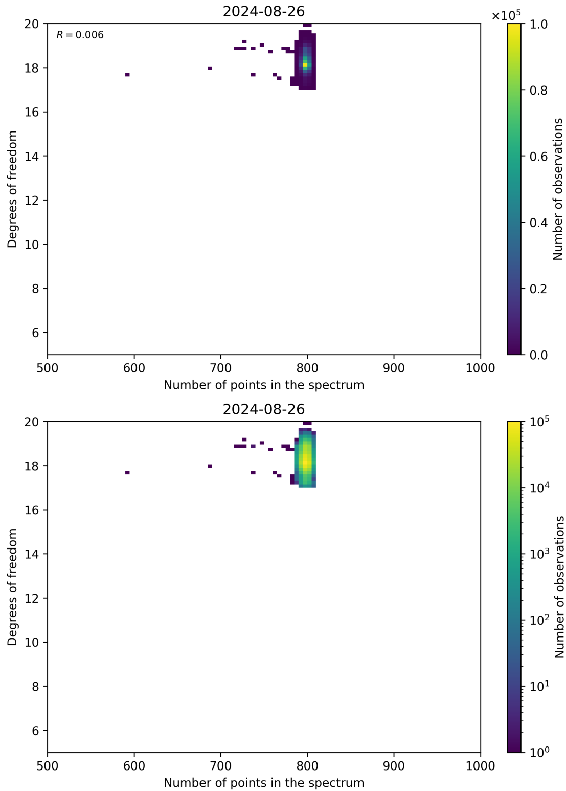
Figure 90: Scatter density plot of “Number of points in the spectrum” against “Degrees of freedom” for 2024-08-25 to 2024-08-27.
