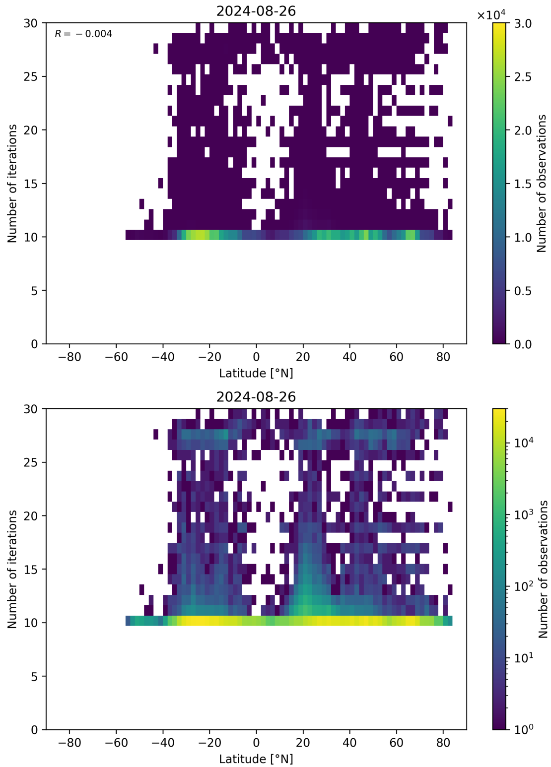
Figure 60: Scatter density plot of “Latitude” against “Number of iterations” for 2024-08-25 to 2024-08-27.
