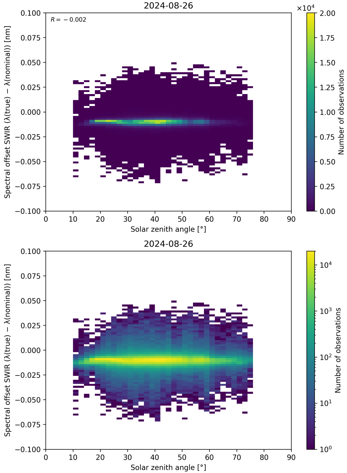
Figure 104: Scatter density plot of “Solar zenith angle” against “Spectral offset SWIR ( \lambda_{\text{true}} - \lambda_{\text{nominal}} )” for 2024-08-25 to 2024-08-27.
