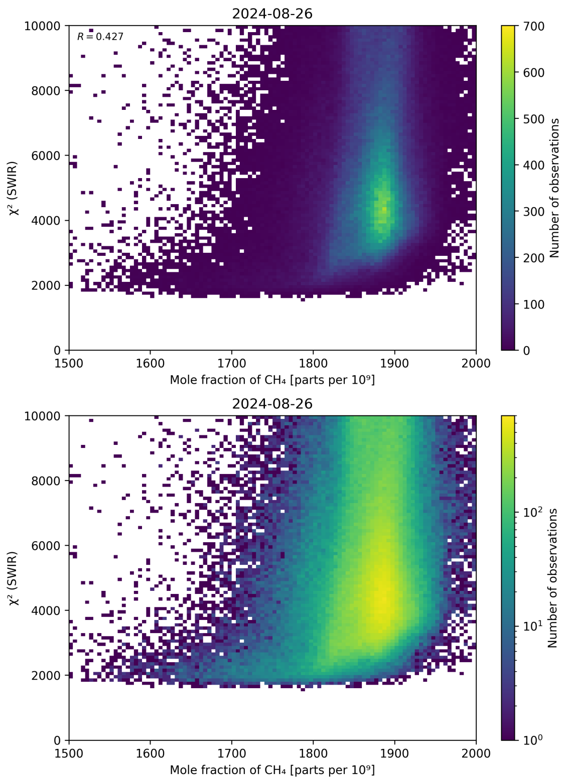
Figure 71: Scatter density plot of “Mole fraction of \text{CH}_4 ” against “ \chi^2 (SWIR)” for 2024-08-25 to 2024-08-27.
