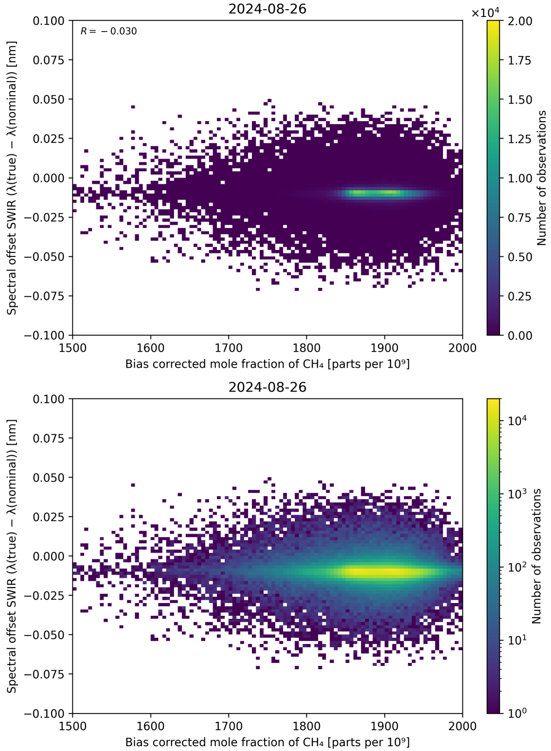
Figure 69: Scatter density plot of “Bias corrected mole fraction of \text{CH}_4 ” against “Spectral offset SWIR ( \lambda_{\text{true}} - \lambda_{\text{nominal}} )” for 2024-08-25 to 2024-08-27.
