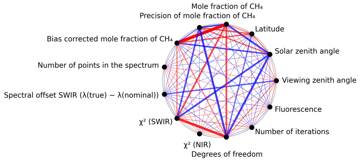
Figure 1: Map of correlation graph for 2024-08-25 to 2024-08-27.
