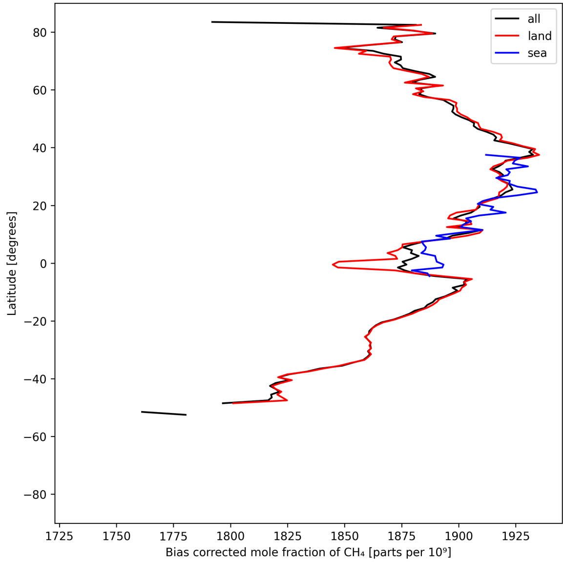
Figure 14: Zonal average of “Bias corrected mole fraction of CH 4 ” for 2024-08-27 to 2024-08-28.
