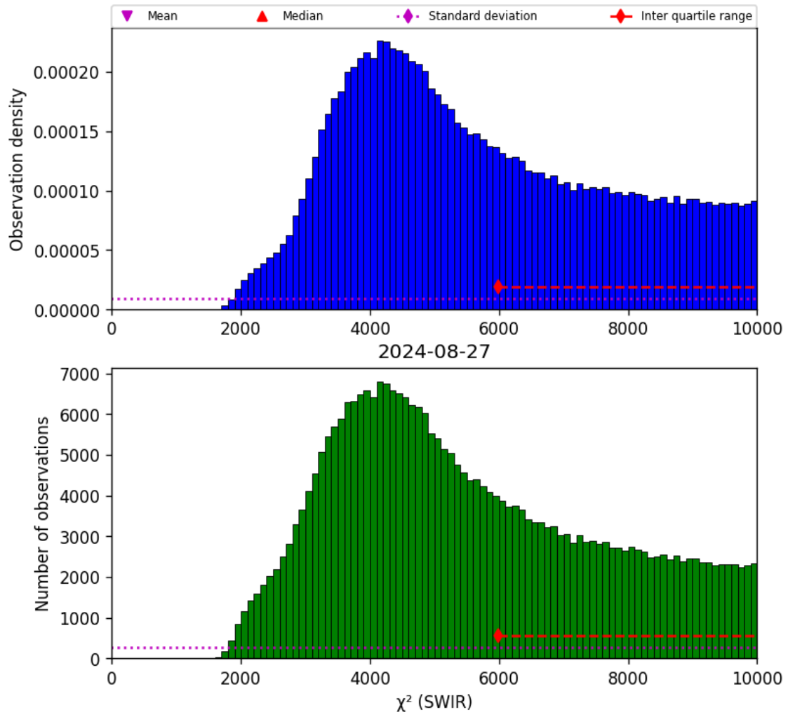
Figure 28: Histogram of " \chi^2 (SWIR)" for 2024-08-27 to 2024-08-28
