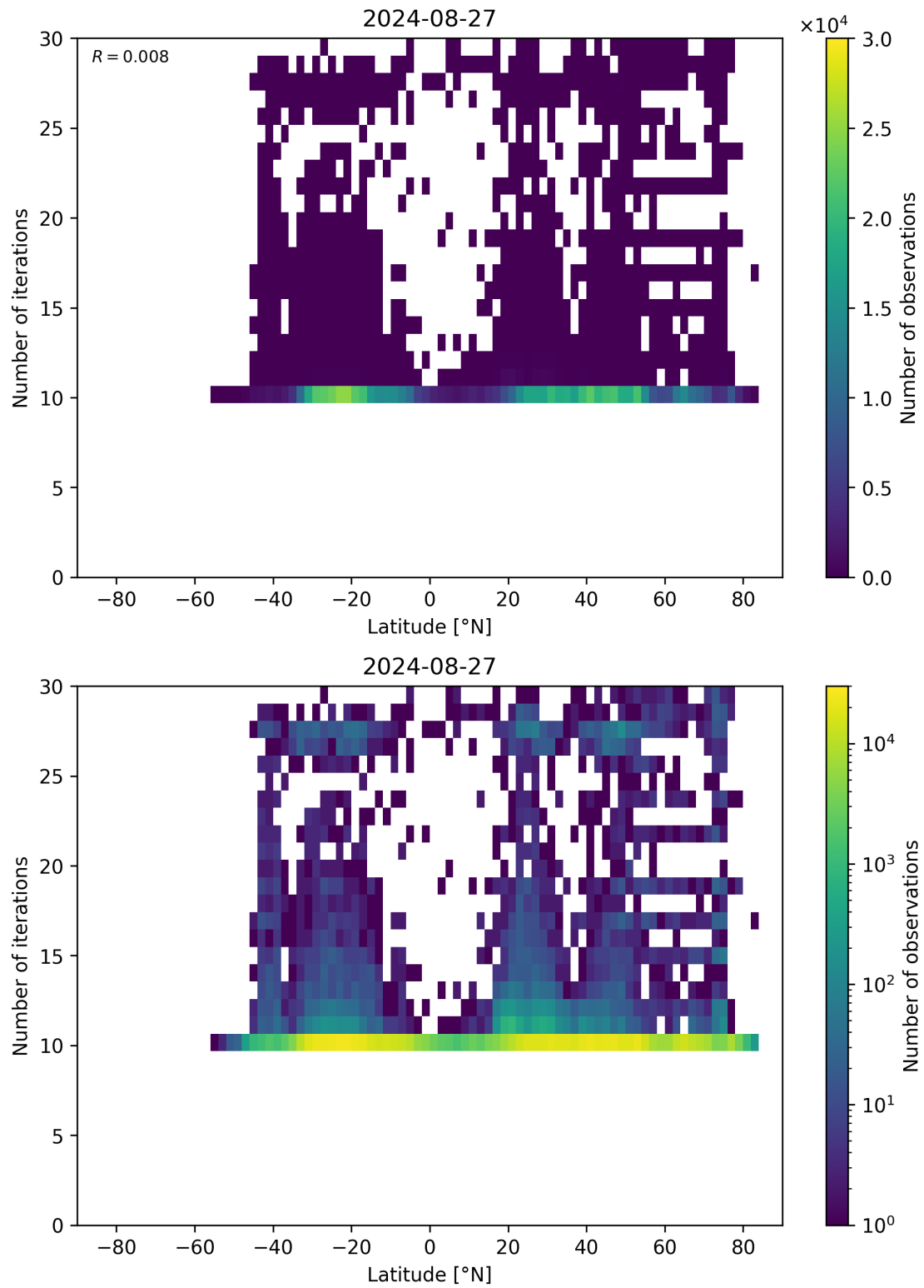
Figure 60: Scatter density plot of “Latitude” against “Number of iterations” for 2024-08-27 to 2024-08-28.
