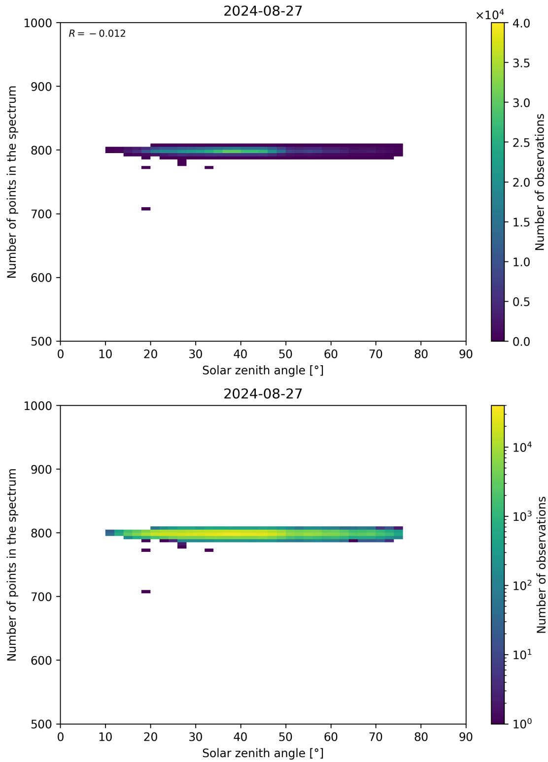
Figure 103: Scatter density plot of “Solar zenith angle” against “Number of points in the spectrum” for 2024-08-27 to 2024-08-28.
