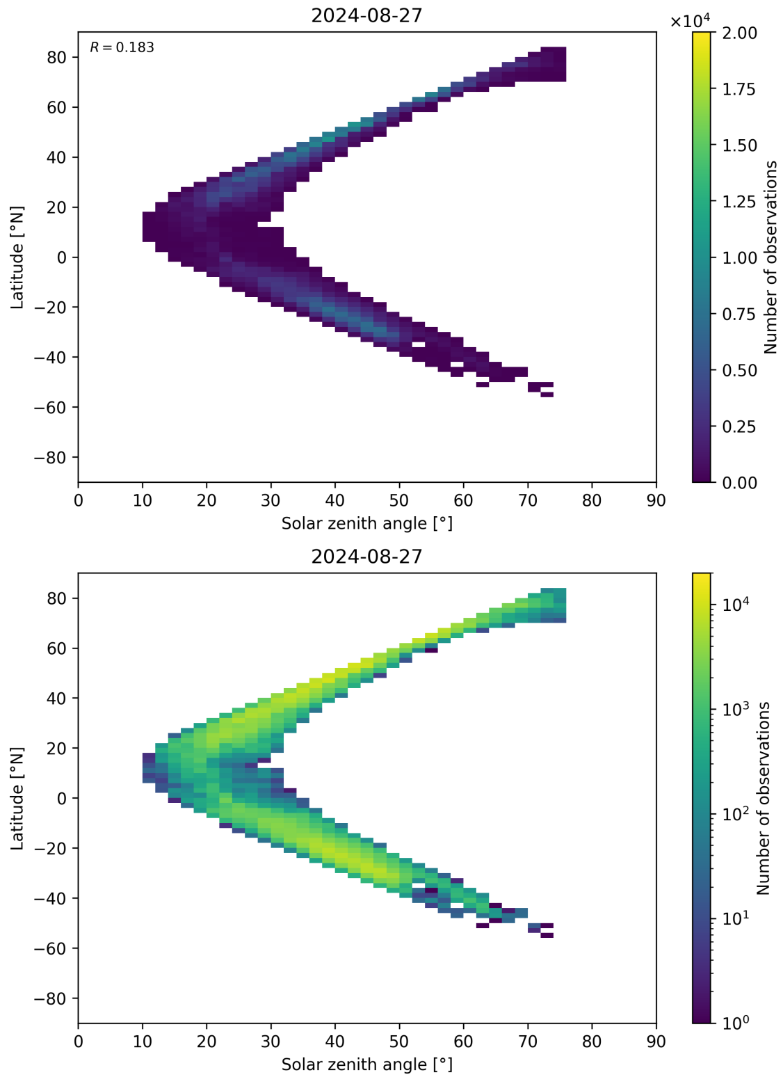
Figure 98: Scatter density plot of “Solar zenith angle” against “Latitude” for 2024-08-27 to 2024-08-28.
