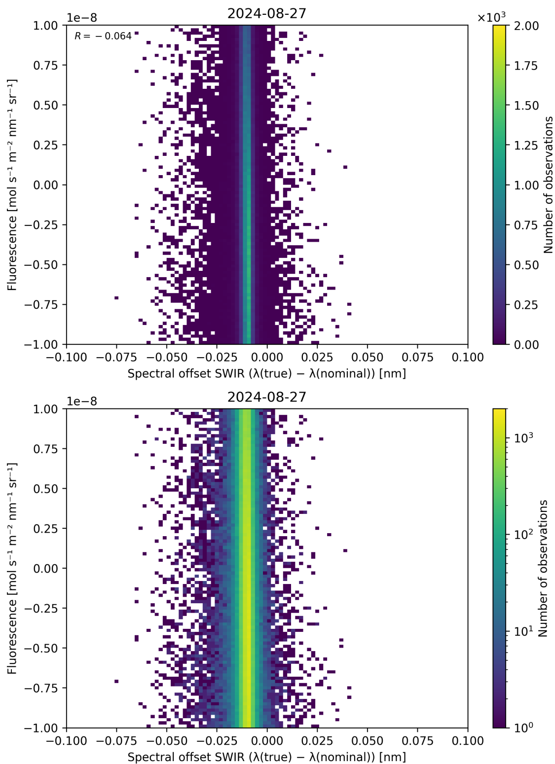
Figure 120: Scatter density plot of “Spectral offset SWIR ( \lambda_{\text{true}} - \lambda_{\text{nominal}} )” against “Fluorescence” for 2024-08-27 to 2024-08-28.
