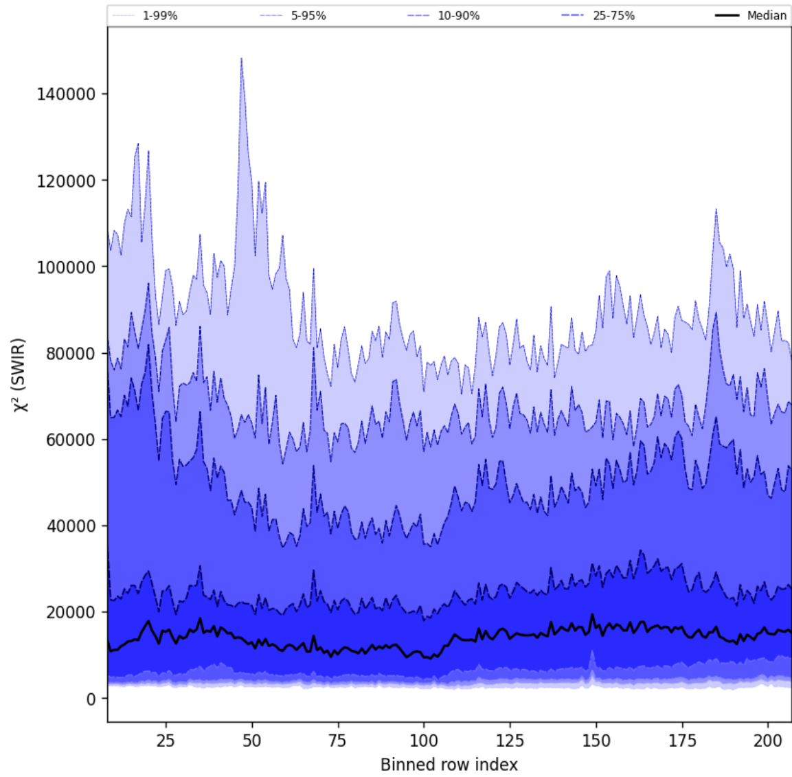
Figure 39: Along track statistics of “ \chi^2 (SWIR)” for 2024-08-27 to 2024-08-28
