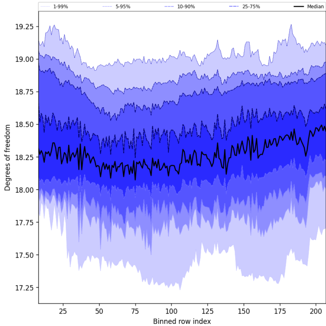
Figure 41: Along track statistics of “Degrees of freedom” for 2024-08-27 to 2024-08-28
