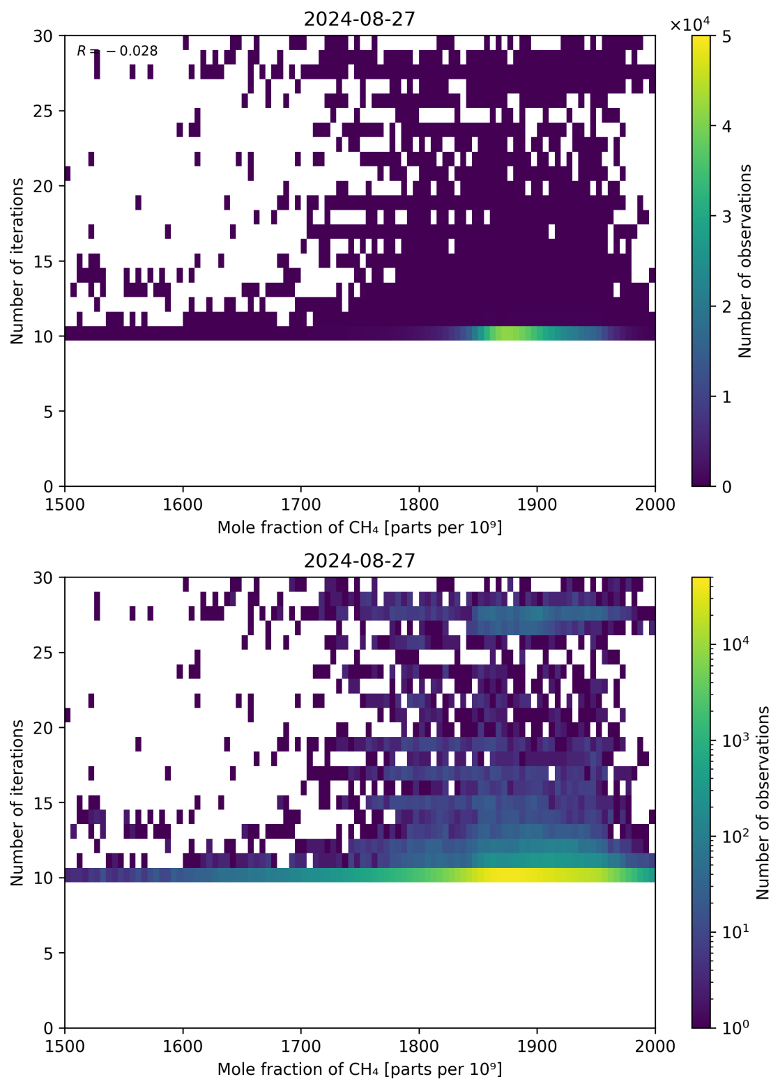
Figure 76: Scatter density plot of “Mole fraction of CH 4 ” against “Number of iterations” for 2024-08-27 to 2024-08-28.
