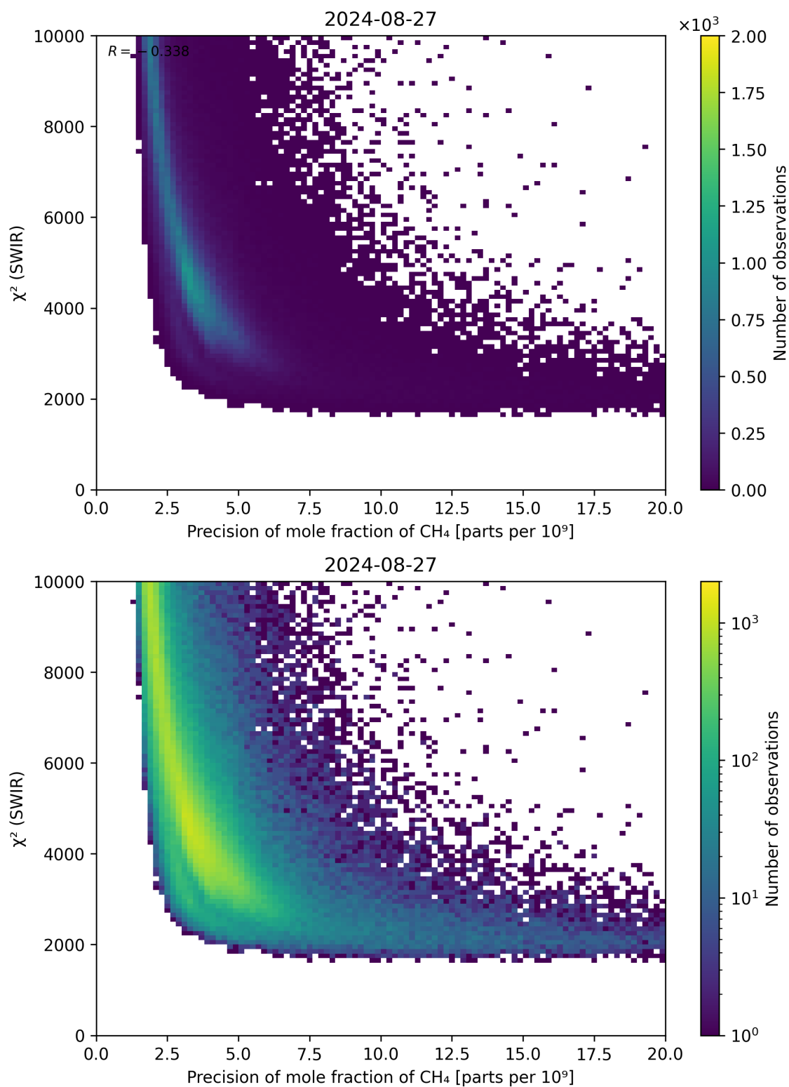
Figure 79: Scatter density plot of “Precision of mole fraction of \text{CH}_4 ” against “ \chi^2 (SWIR)” for 2024-08-27 to 2024-08-28.
