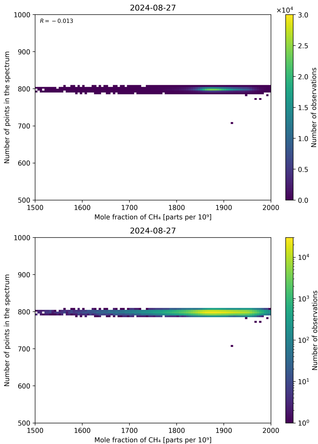
Figure 77: Scatter density plot of “Mole fraction of CH 4 ” against “Number of points in the spectrum” for 2024-08-27 to 2024-08-28.
