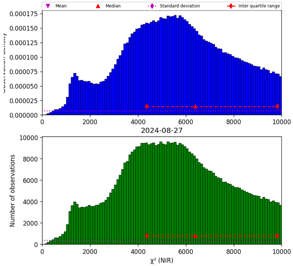
Figure 29: Histogram of “ \chi^2 (NIR)” for 2024-08-27 to 2024-08-28
