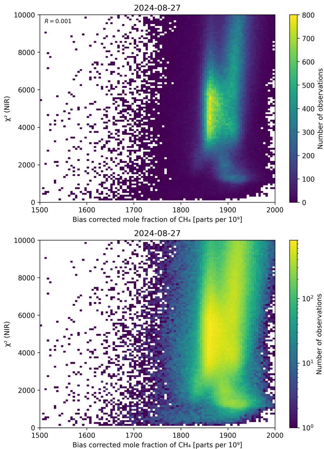
Figure 63: Scatter density plot of “Bias corrected mole fraction of CH 4 ” against “ \chi^2 (NIR)” for 2024-08-27 to 2024-08-28.
