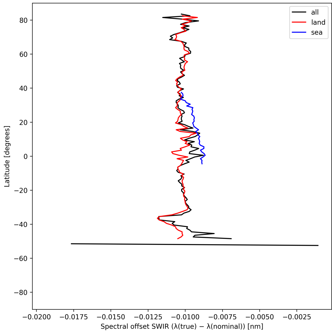
Figure 16: Zonal average of “Spectral offset SWIR ( \lambda_{\text{true}} - \lambda_{\text{nominal}} )” for 2024-08-27 to 2024-08-28.
