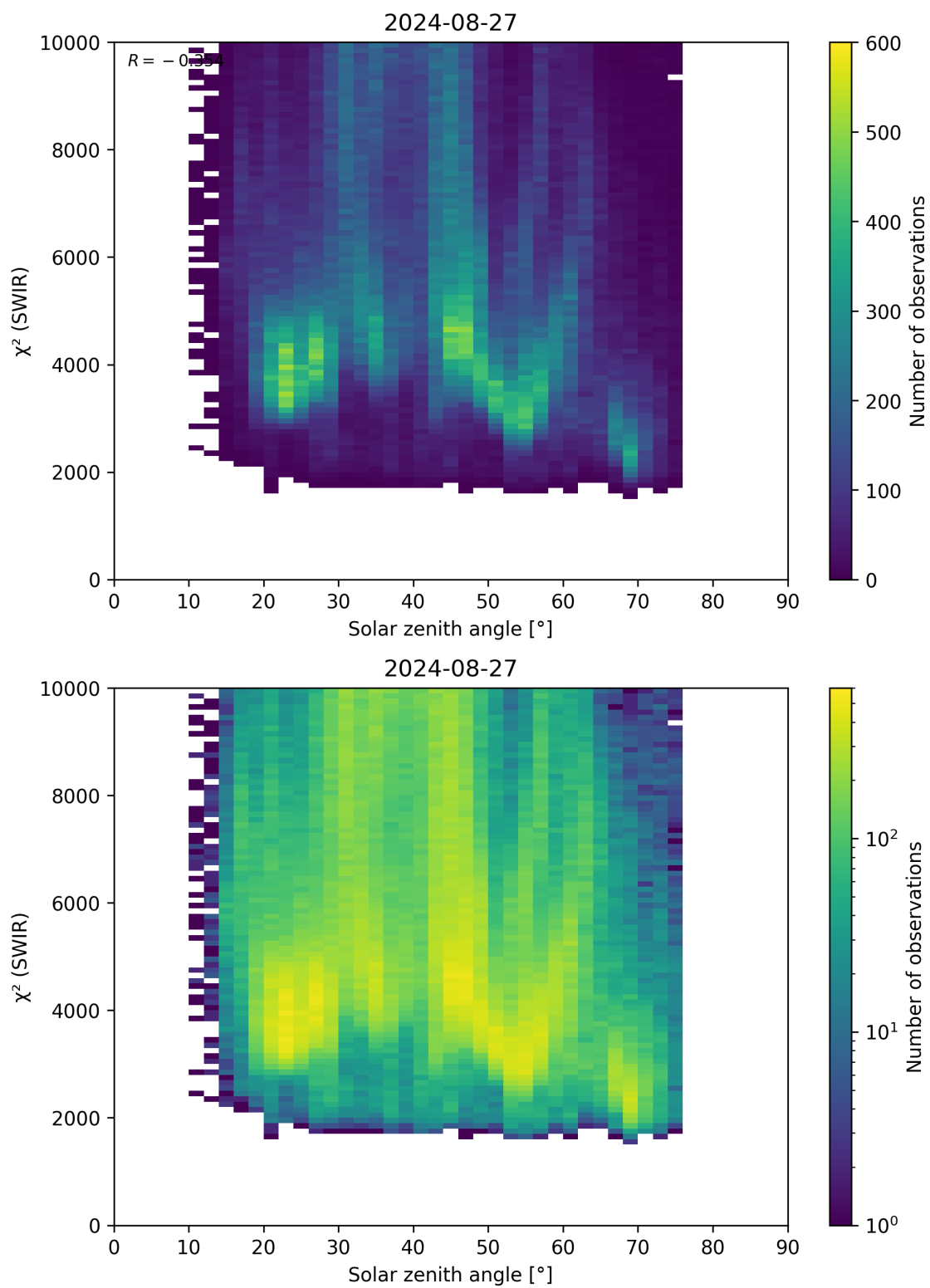
Figure 95: Scatter density plot of “Solar zenith angle” against “ \chi^2 (SWIR)” for 2024-08-27 to 2024-08-28.
