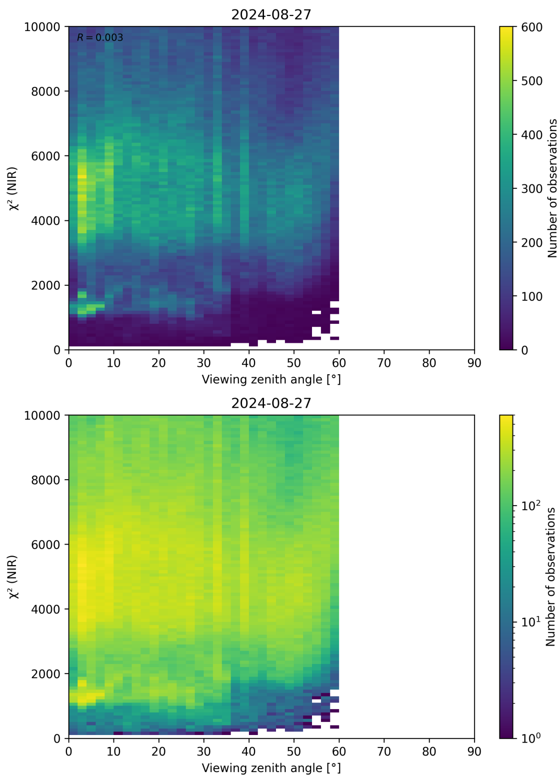
Figure 105: Scatter density plot of “Viewing zenith angle” against “ \chi^2 (NIR)” for 2024-08-27 to 2024-08-28.
