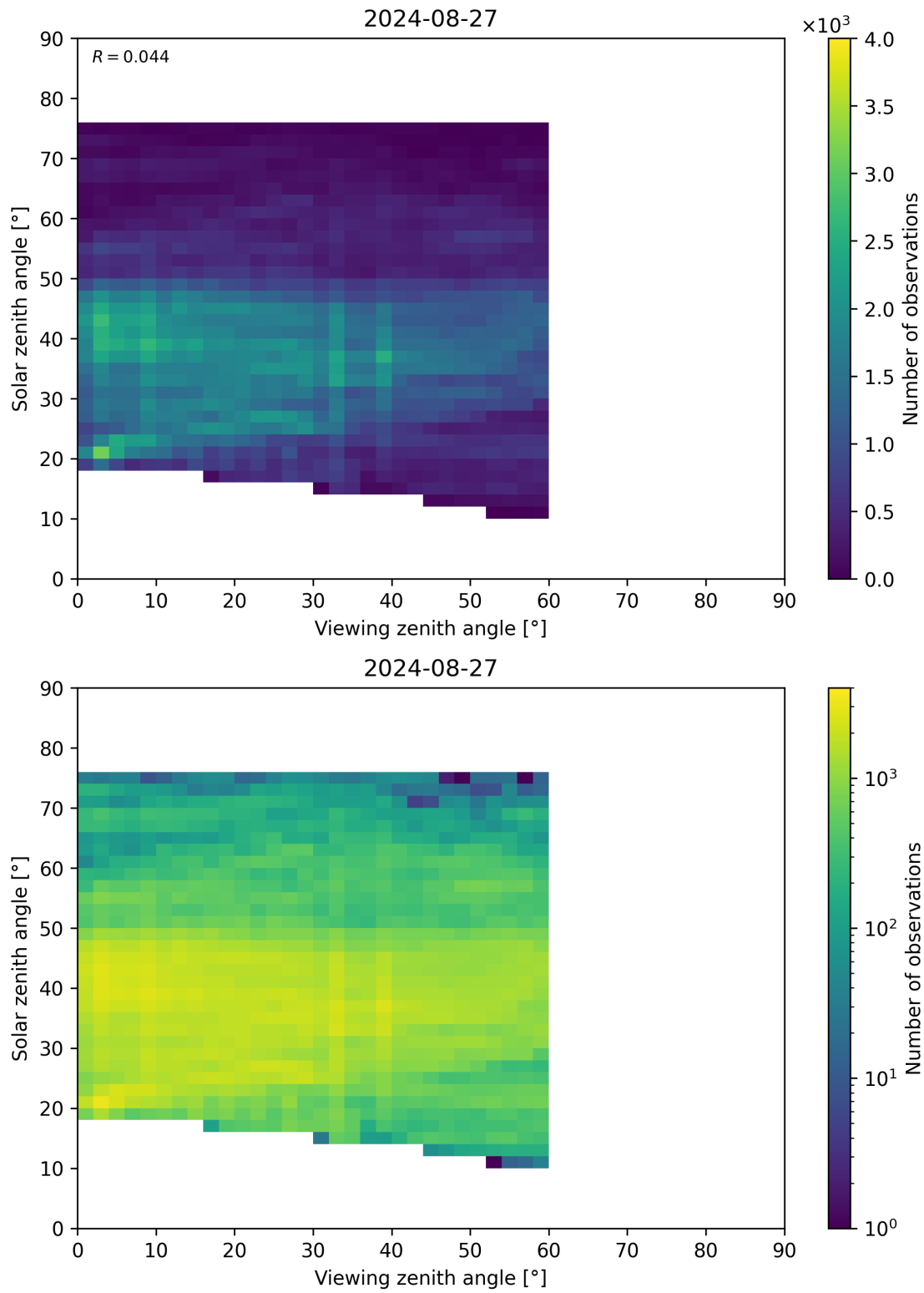
Figure 115: Scatter density plot of “Viewing zenith angle” against “Solar zenith angle” for 2024-08-27 to 2024-08-28.
