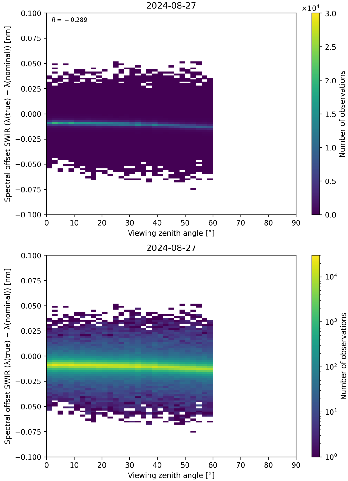
Figure 116: Scatter density plot of “Viewing zenith angle” against “Spectral offset SWIR ( \lambda_{\text{true}} - \lambda_{\text{nominal}} )” for 2024-08-27 to 2024-08-28.
