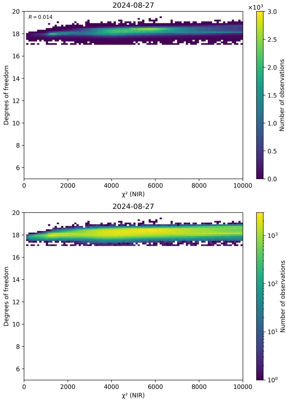
Figure 44: Scatter density plot of “ \chi^2 (NIR)” against “Degrees of freedom” for 2024-08-27 to 2024-08-28.
