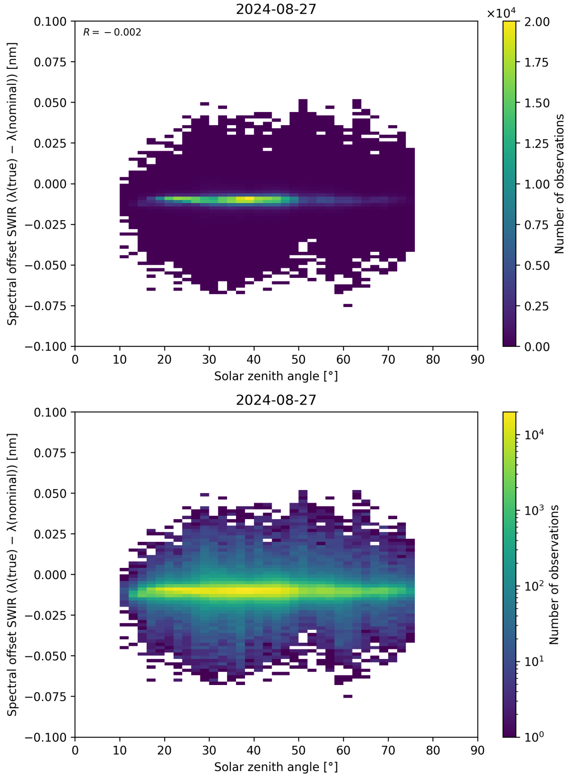
Figure 104: Scatter density plot of “Solar zenith angle” against “Spectral offset SWIR ( \lambda_{\text{true}} - \lambda_{\text{nominal}} )” for 2024-08-27 to 2024-08-28.
