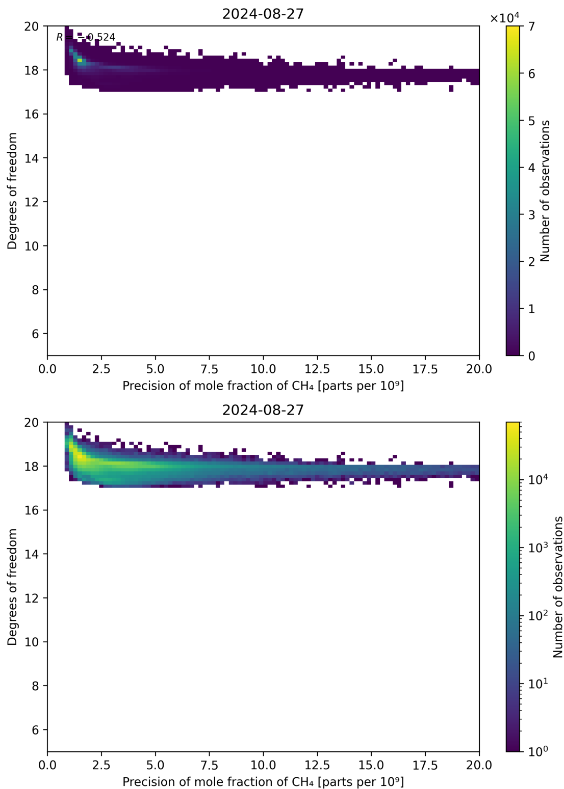
Figure 80: Scatter density plot of “Precision of mole fraction of CH 4 ” against “Degrees of freedom” for 2024-08-27 to 2024-08-28.
