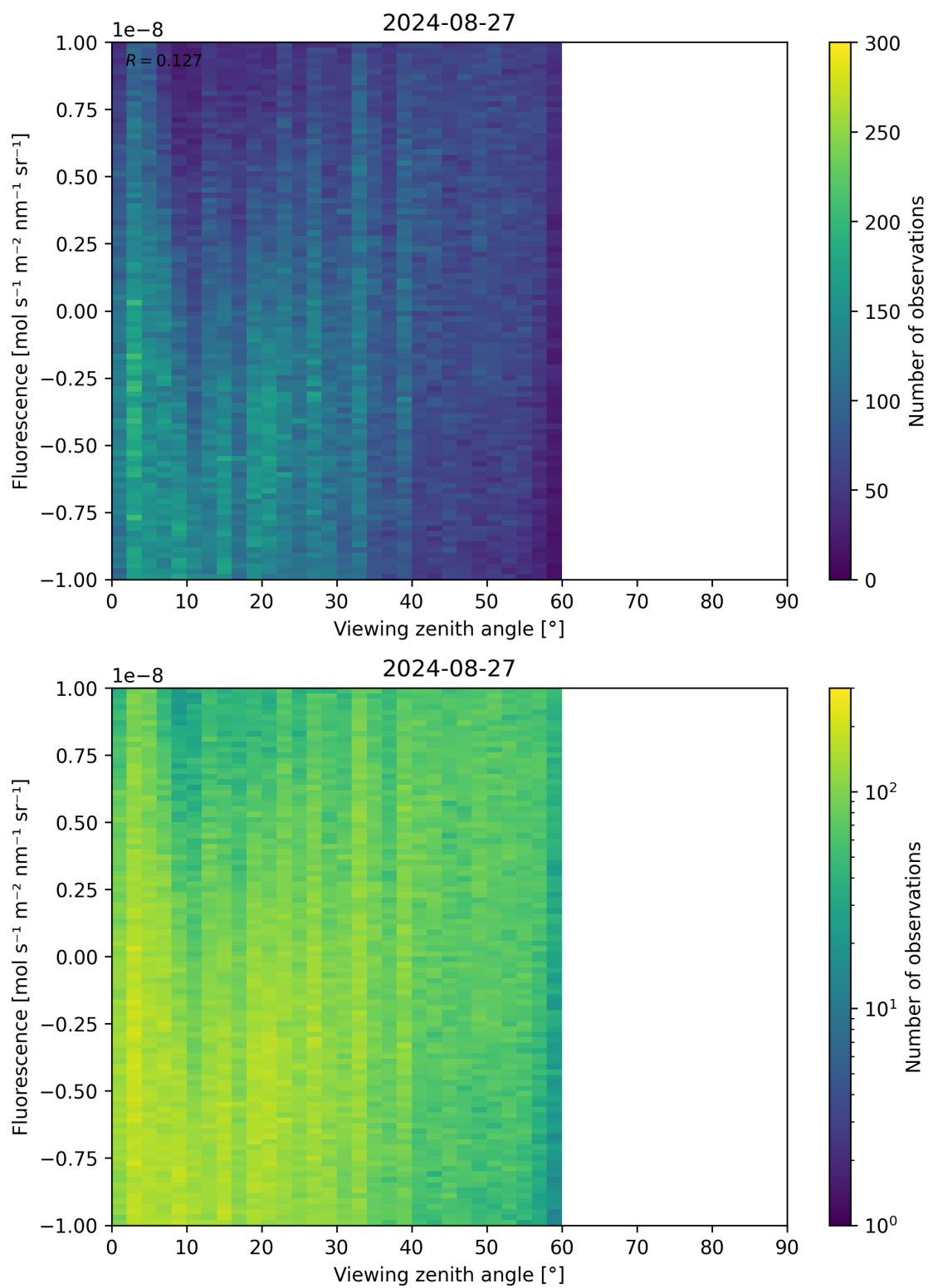
Figure 108: Scatter density plot of “Viewing zenith angle” against “Fluorescence” for 2024-08-27 to 2024-08-28.
