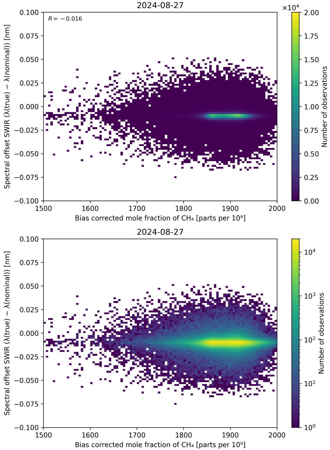
Figure 69: Scatter density plot of “Bias corrected mole fraction of CH 4 ” against “Spectral offset SWIR ( \lambda_{\text{true}} - \lambda_{\text{nominal}} )” for 2024-08-27 to 2024-08-28.
