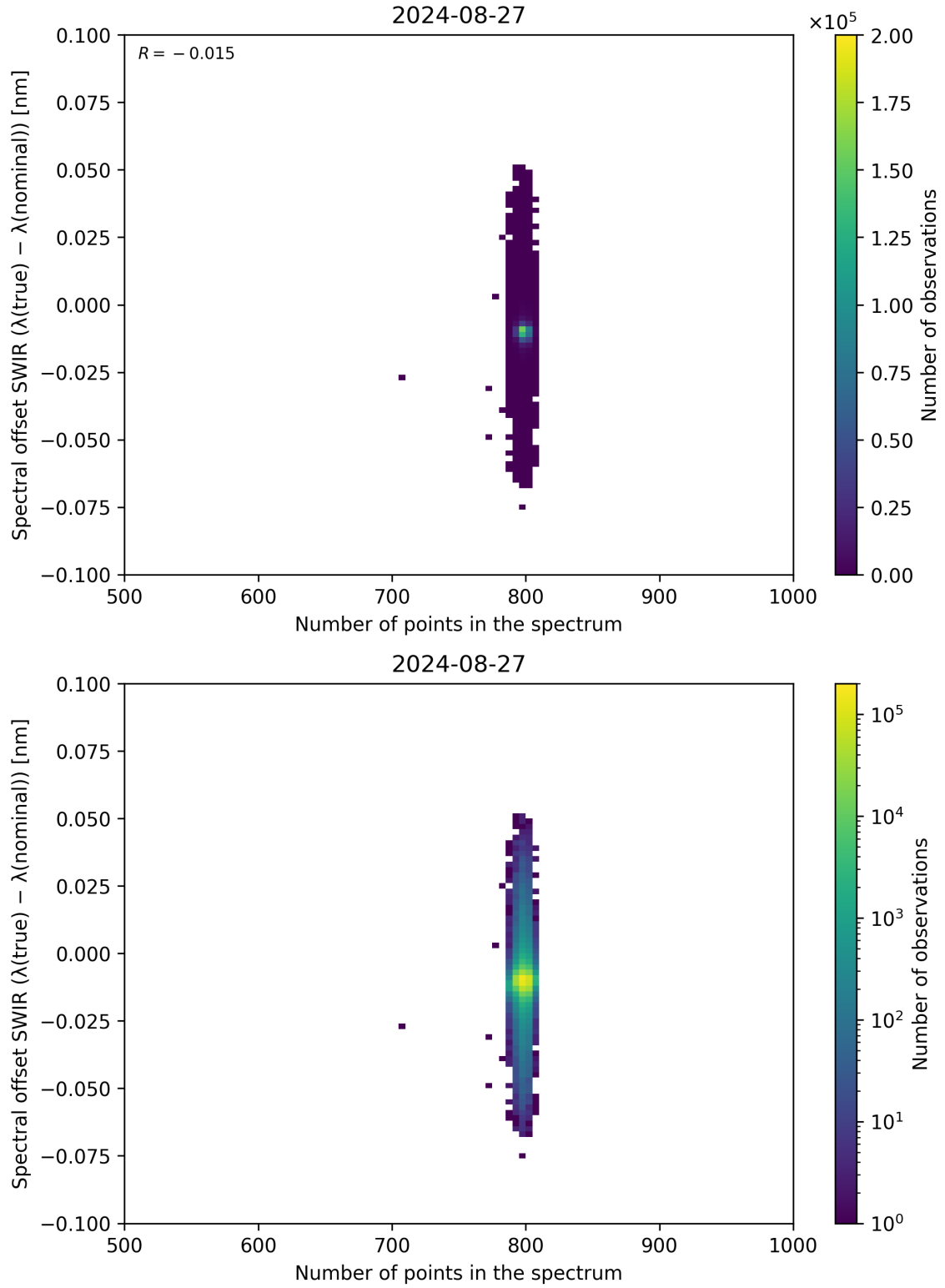
Figure 93: Scatter density plot of “Number of points in the spectrum” against “Spectral offset SWIR ( \lambda_{\text{true}} - \lambda_{\text{nominal}} )” for 2024-08-27 to 2024-08-28.
