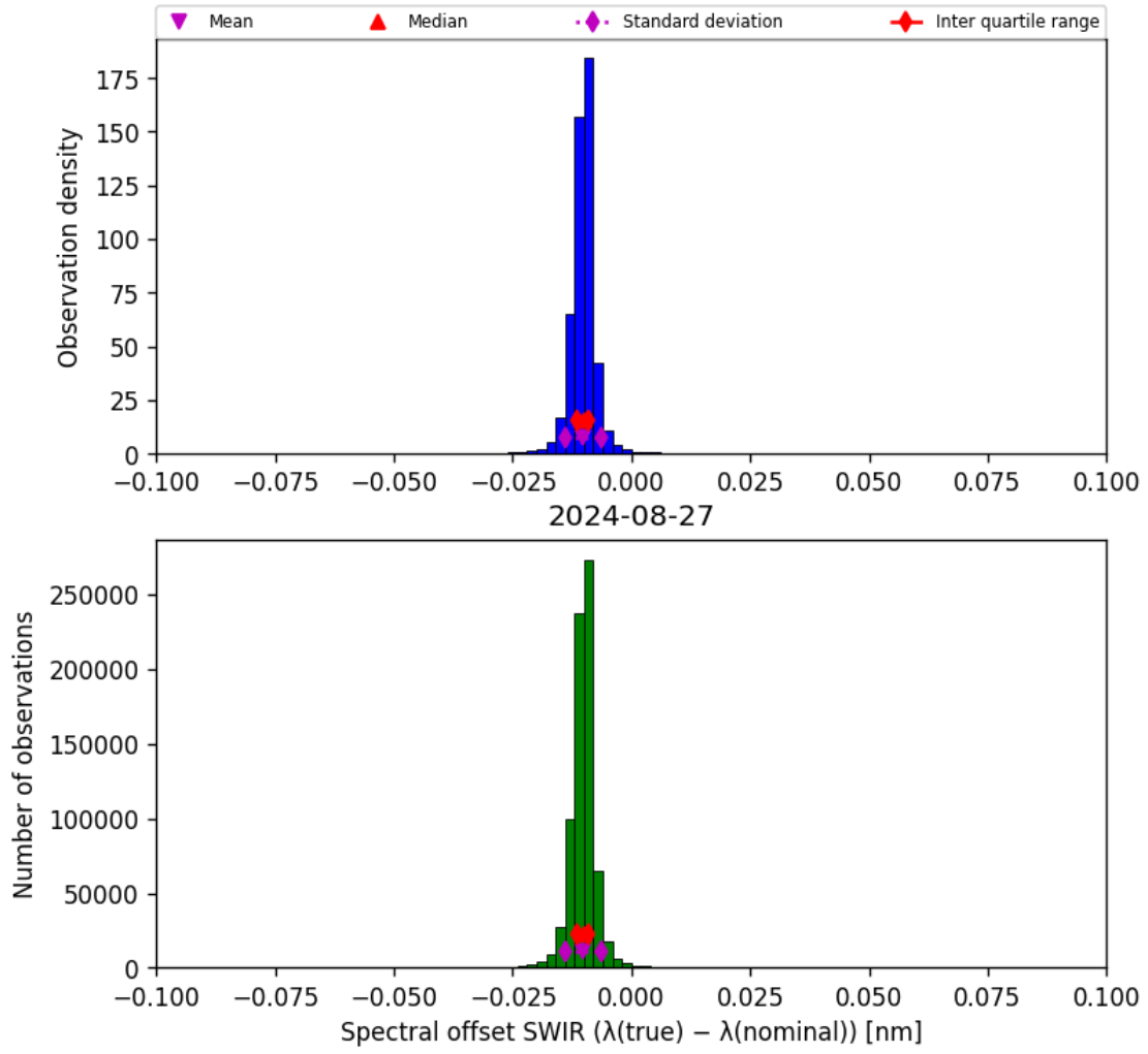
Figure 27: Histogram of “Spectral offset SWIR ( \lambda_{\text{true}} - \lambda_{\text{nominal}} )” for 2024-08-27 to 2024-08-28
