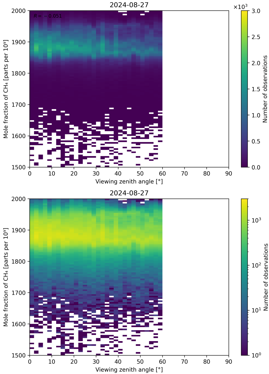
Figure 110: Scatter density plot of “Viewing zenith angle” against “Mole fraction of CH 4 ” for 2024-08-27 to 2024-08-28.
