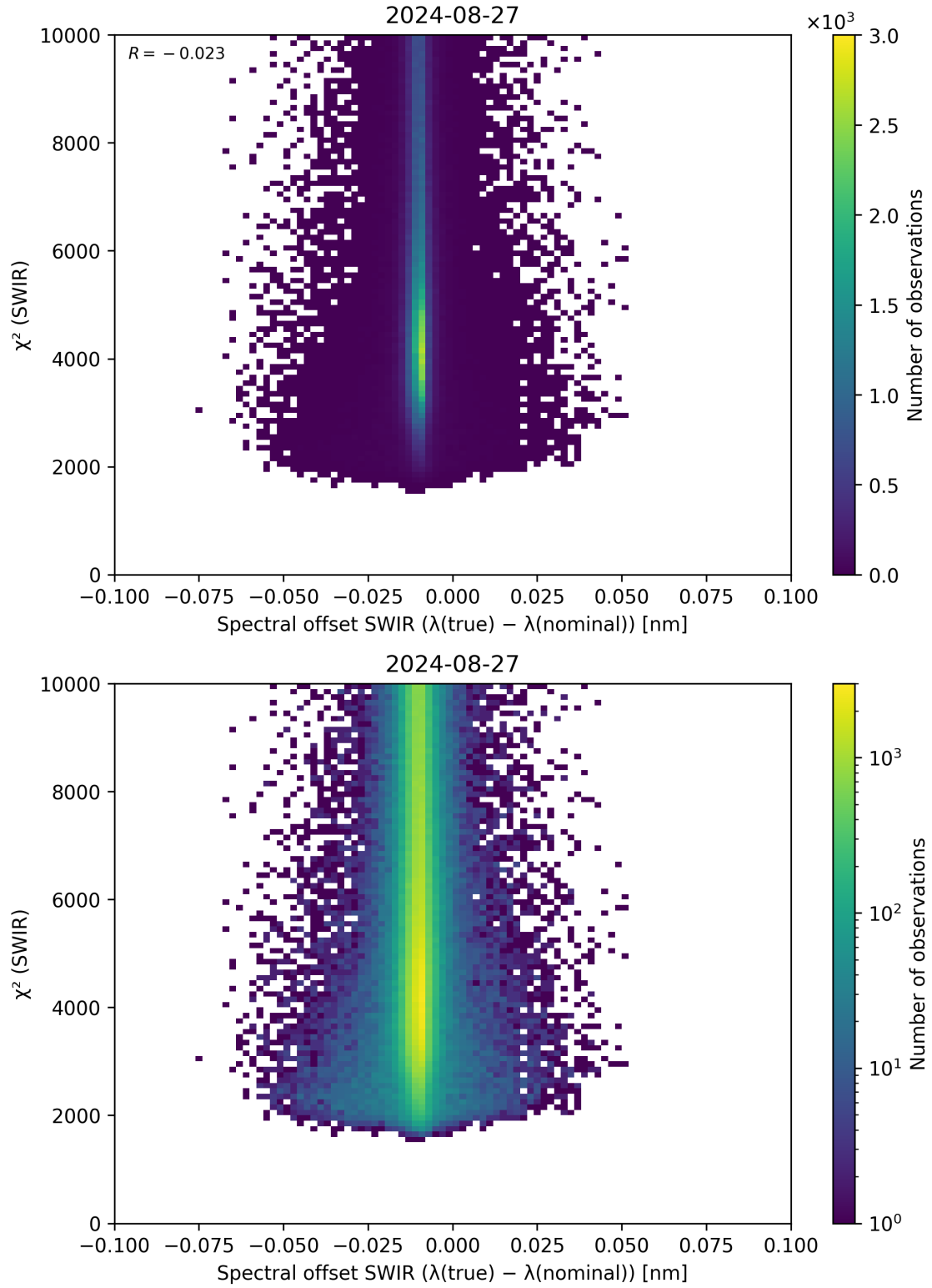
Figure 118: Scatter density plot of “Spectral offset SWIR ( \lambda_{\text{true}} - \lambda_{\text{nominal}} )” against “ \chi^2 (SWIR)” for 2024-08-27 to 2024-08-28.
