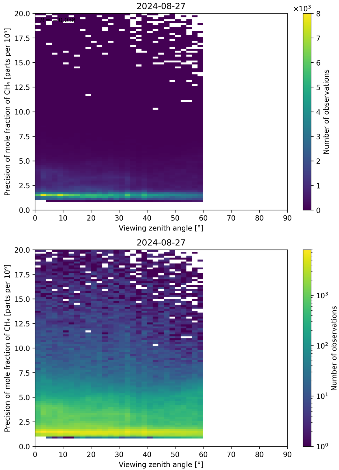
Figure 112: Scatter density plot of “Viewing zenith angle” against “Precision of mole fraction of CH 4 ” for 2024-08-27 to 2024-08-28.
