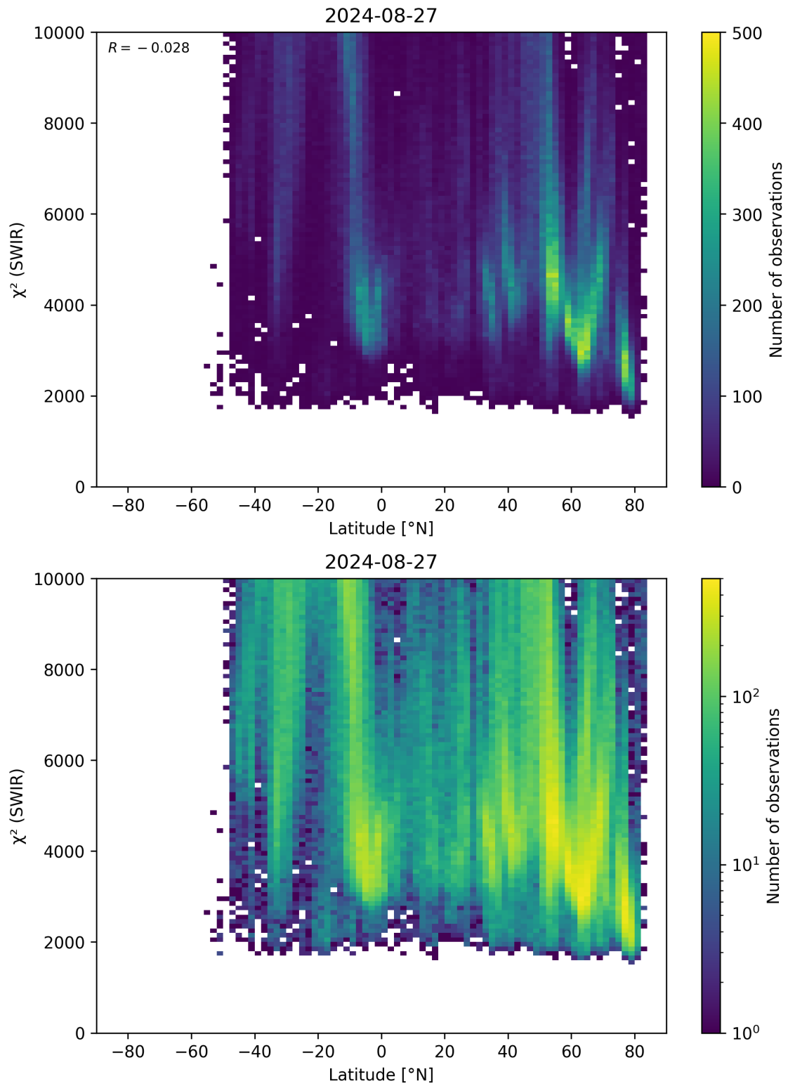
Figure 54: Scatter density plot of “Latitude” against “ \chi^2 (SWIR)” for 2024-08-27 to 2024-08-28.
