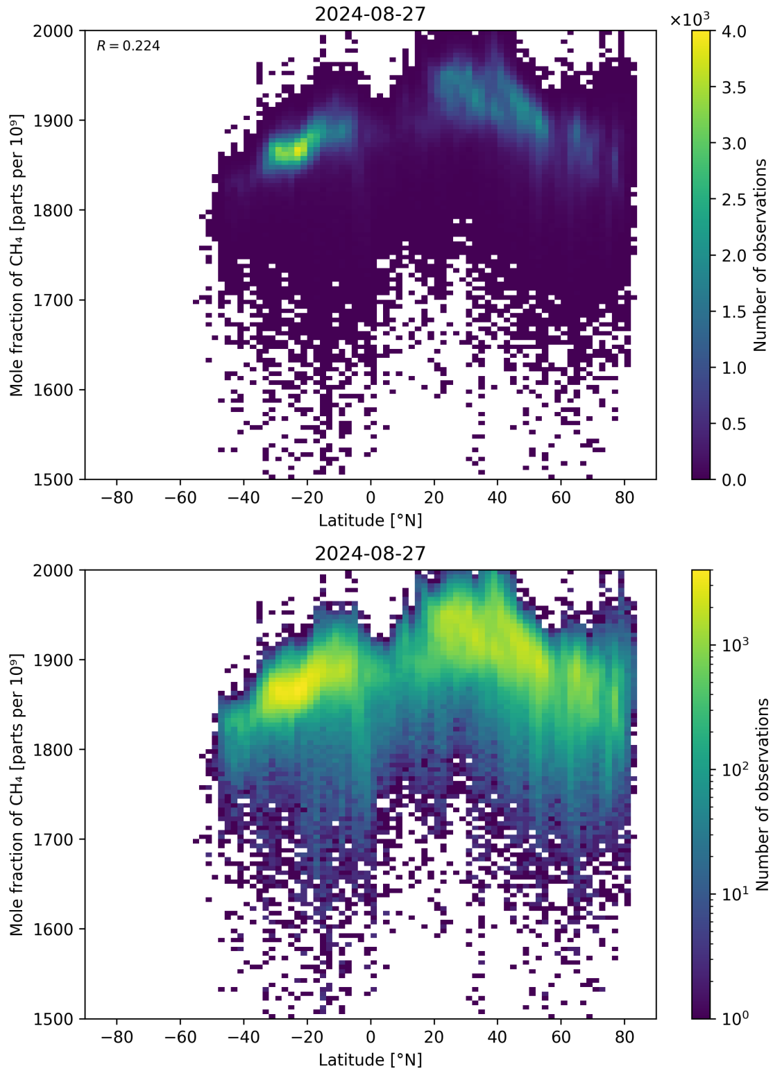
Figure 57: Scatter density plot of “Latitude” against “Mole fraction of \text{CH}_4 ” for 2024-08-27 to 2024-08-28.
