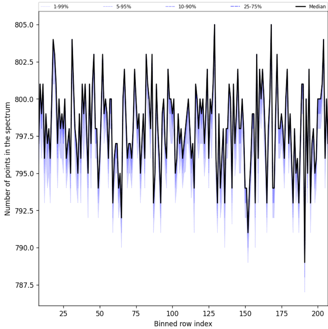
Figure 37: Along track statistics of “Number of points in the spectrum” for 2024-08-27 to 2024-08-28
