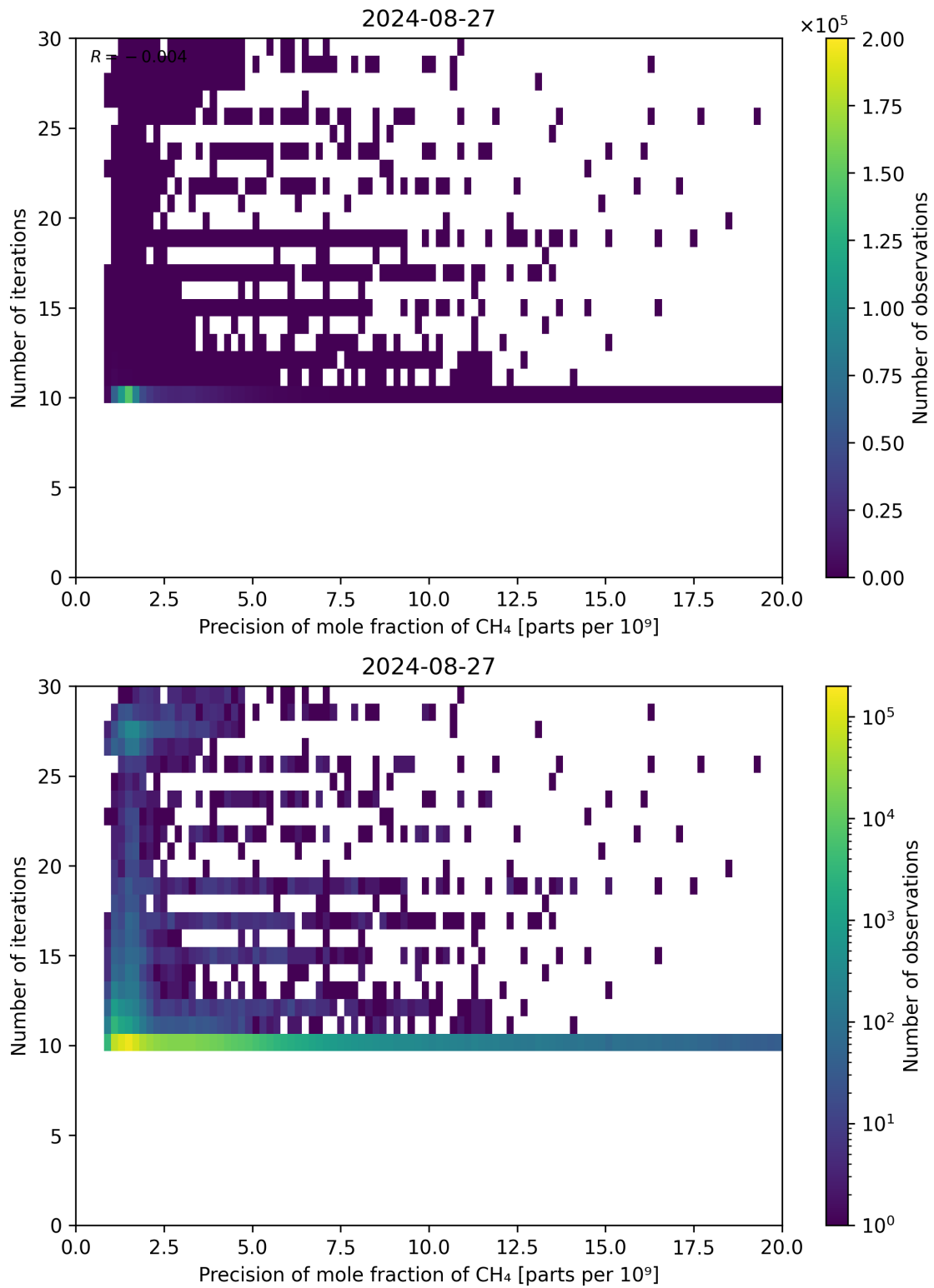
Figure 83: Scatter density plot of “Precision of mole fraction of CH 4 ” against “Number of iterations” for 2024-08-27 to 2024-08-28.
