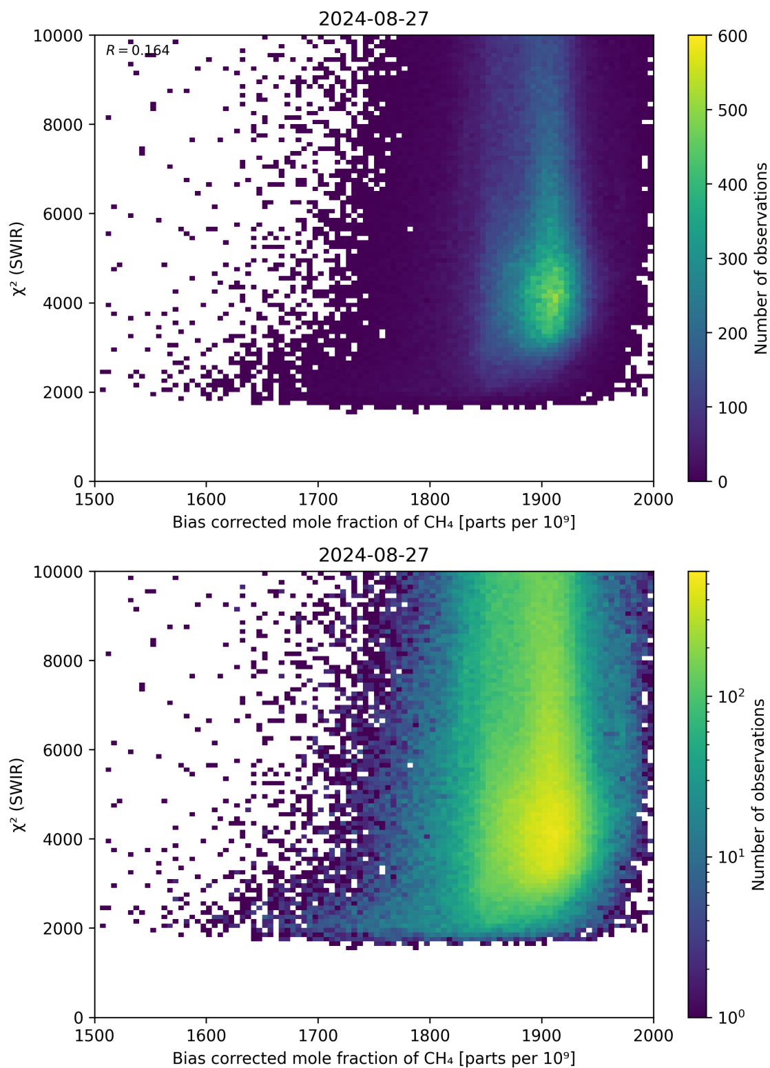
Figure 64: Scatter density plot of “Bias corrected mole fraction of \text{CH}_4 ” against “ \chi^2 (SWIR)” for 2024-08-27 to 2024-08-28.
