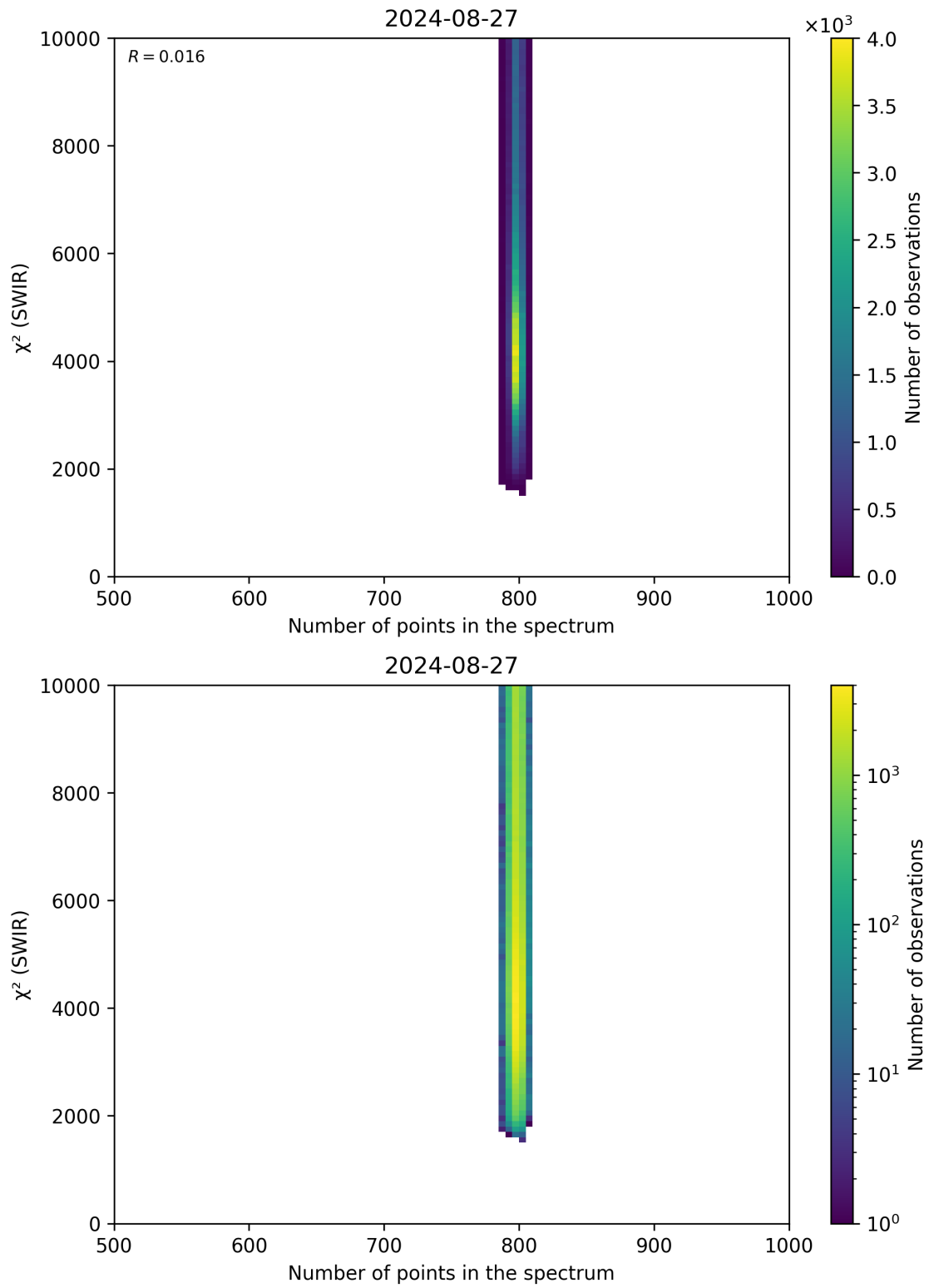
Figure 89: Scatter density plot of “Number of points in the spectrum” against “ \chi^2 (SWIR)” for 2024-08-27 to 2024-08-28.
