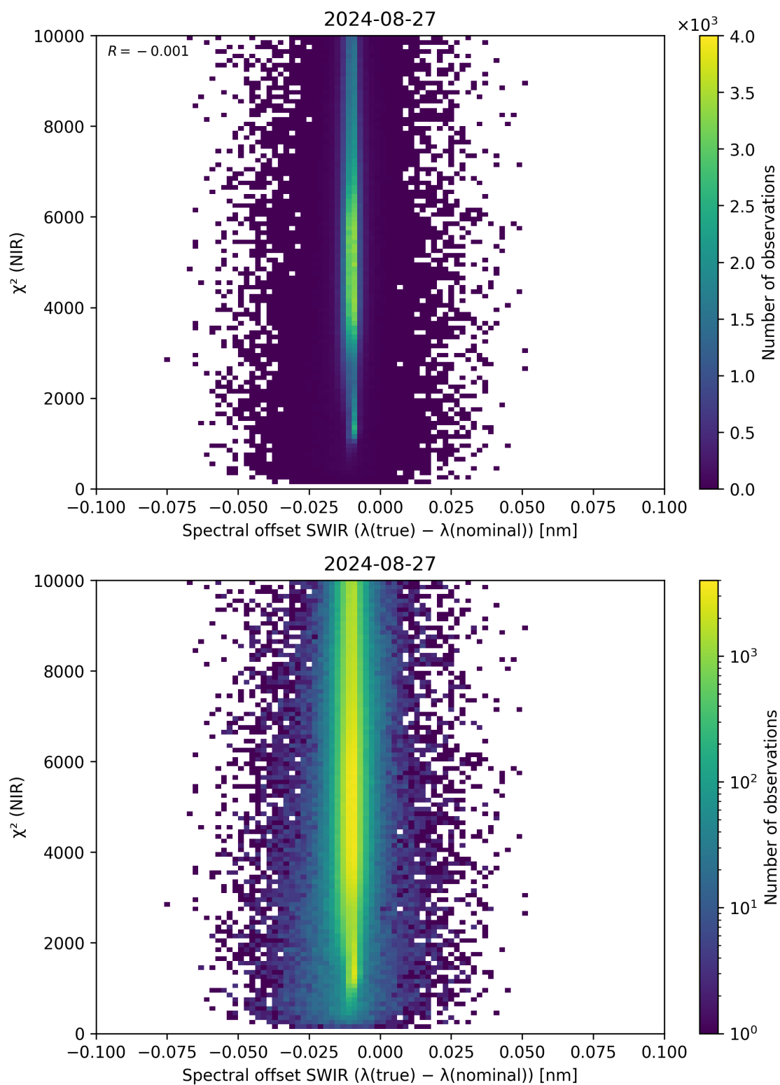
Figure 117: Scatter density plot of “Spectral offset SWIR ( \lambda_{\text{true}} - \lambda_{\text{nominal}} )” against “ \chi^2 (NIR)” for 2024-08-27 to 2024-08-28.
