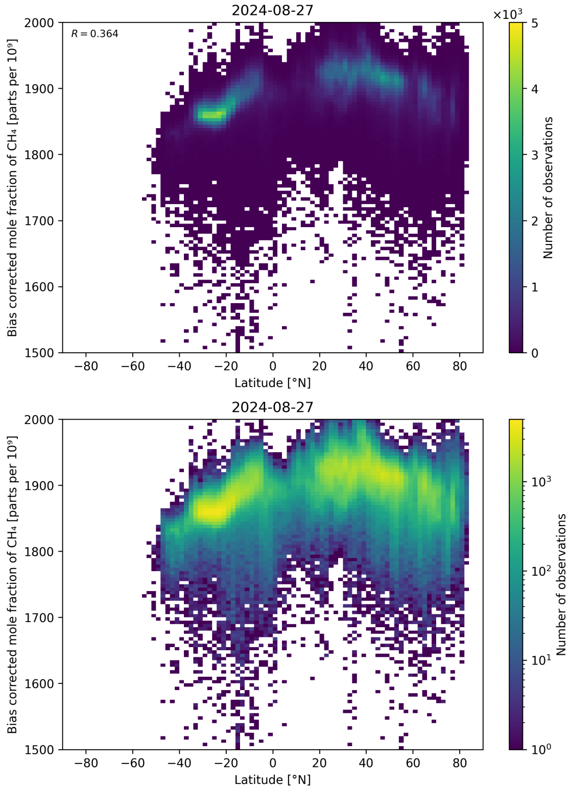
Figure 58: Scatter density plot of “Latitude” against “Bias corrected mole fraction of \text{CH}_4 ” for 2024-08-27 to 2024-08-28.
