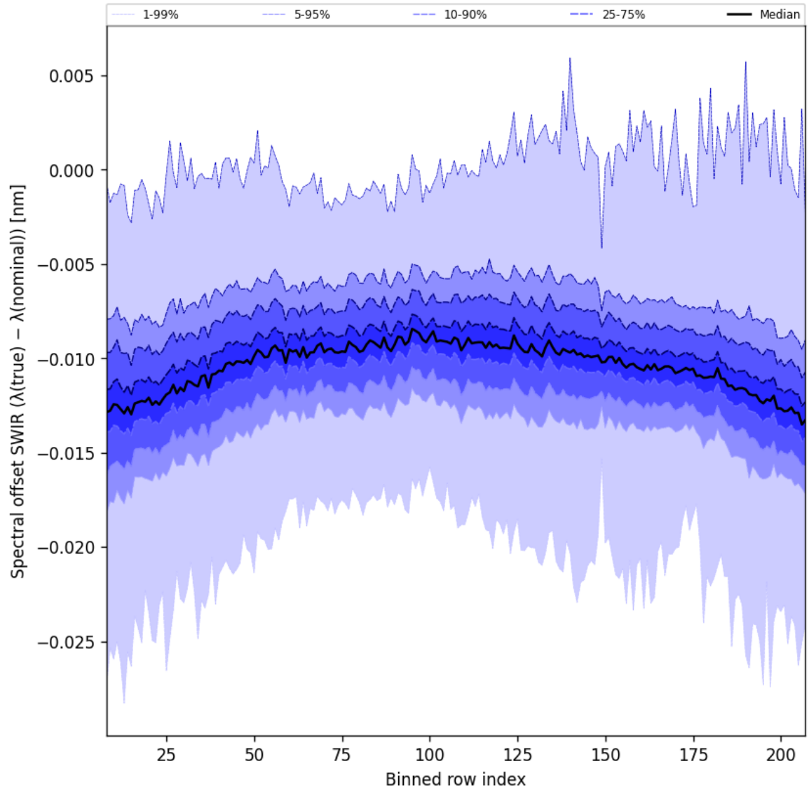
Figure 38: Along track statistics of “Spectral offset SWIR ( \lambda_{\text{true}} - \lambda_{\text{nominal}} )” for 2024-08-27 to 2024-08-28
