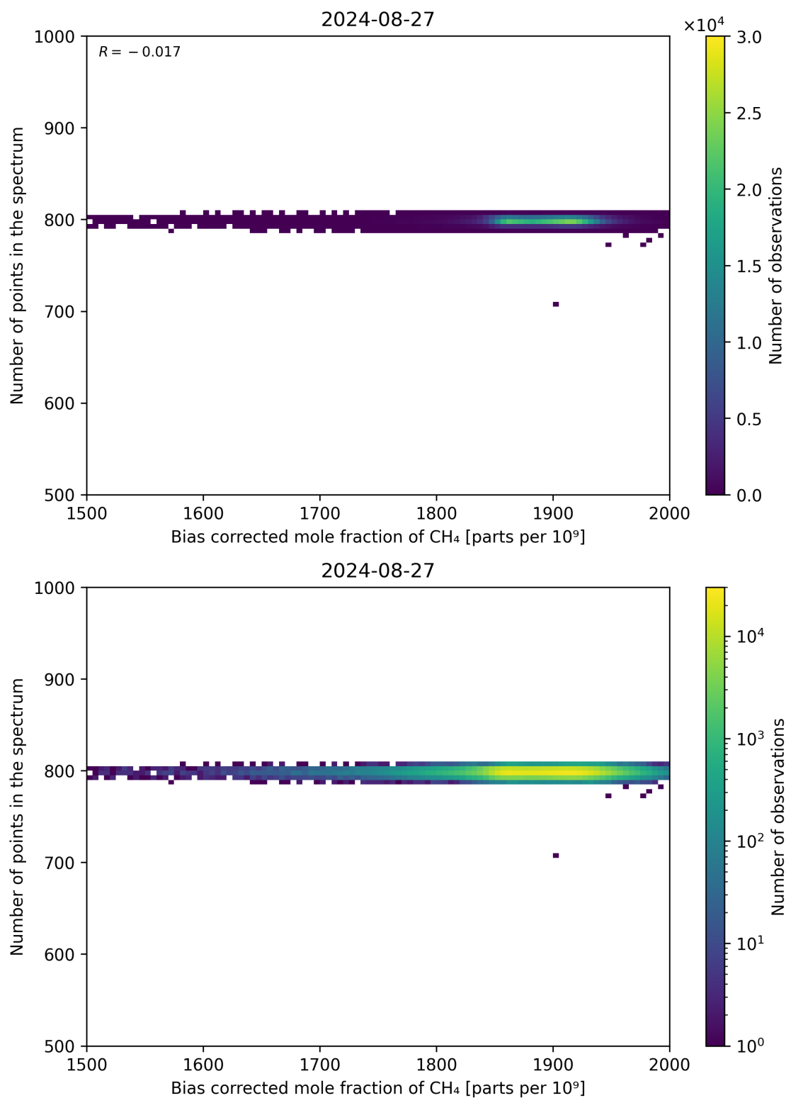
Figure 68: Scatter density plot of “Bias corrected mole fraction of CH 4 ” against “Number of points in the spectrum” for 2024-08-27 to 2024-08-28.
