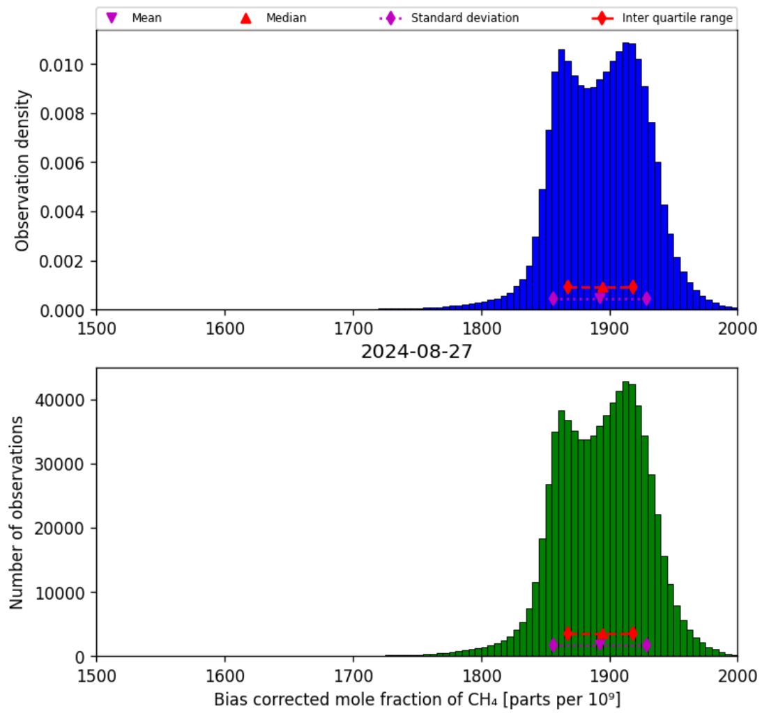
Figure 25: Histogram of “Bias corrected mole fraction of CH 4 ” for 2024-08-27 to 2024-08-28
