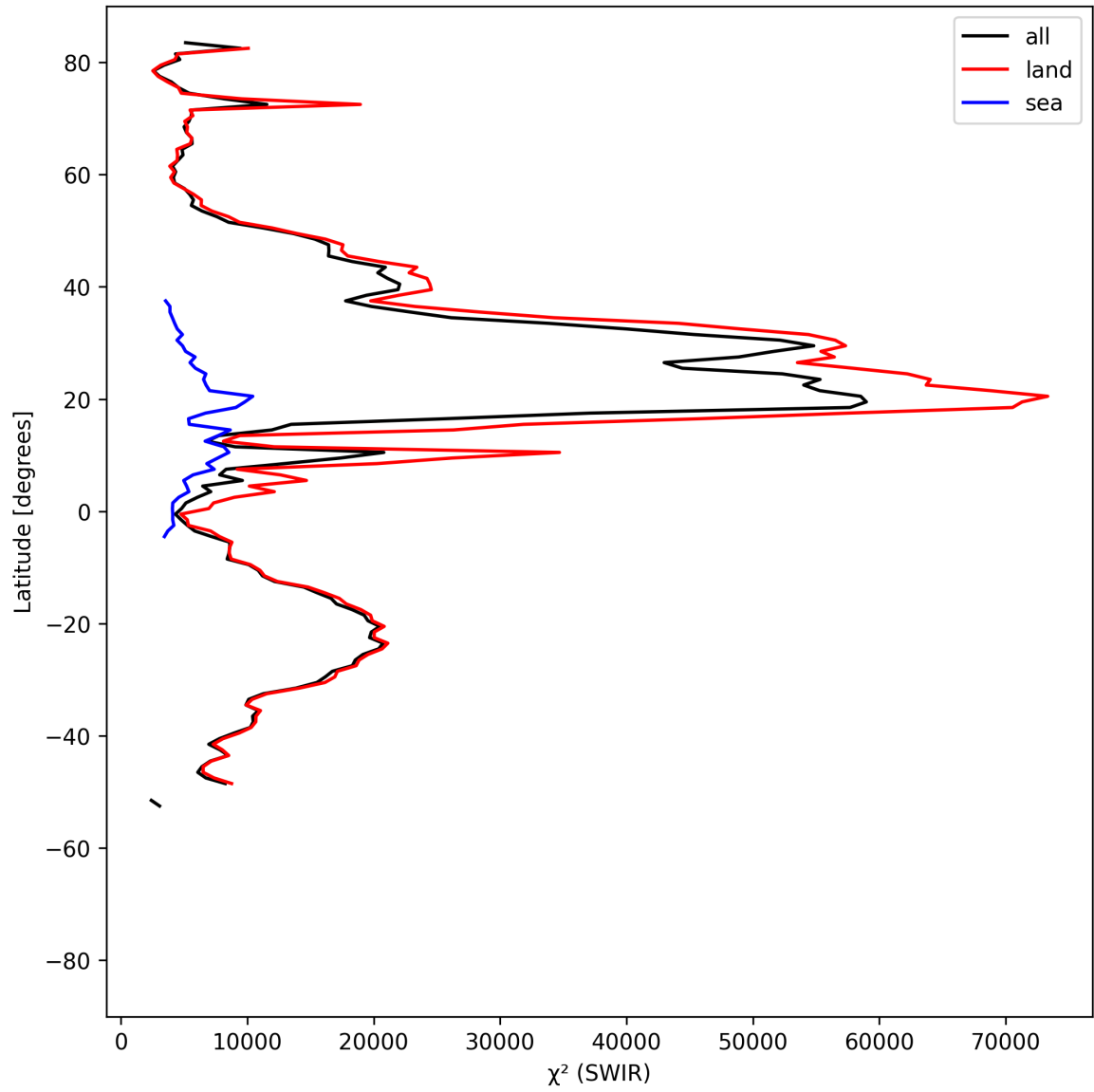
Figure 17: Zonal average of “ \chi^2 (SWIR)” for 2024-08-27 to 2024-08-28.
