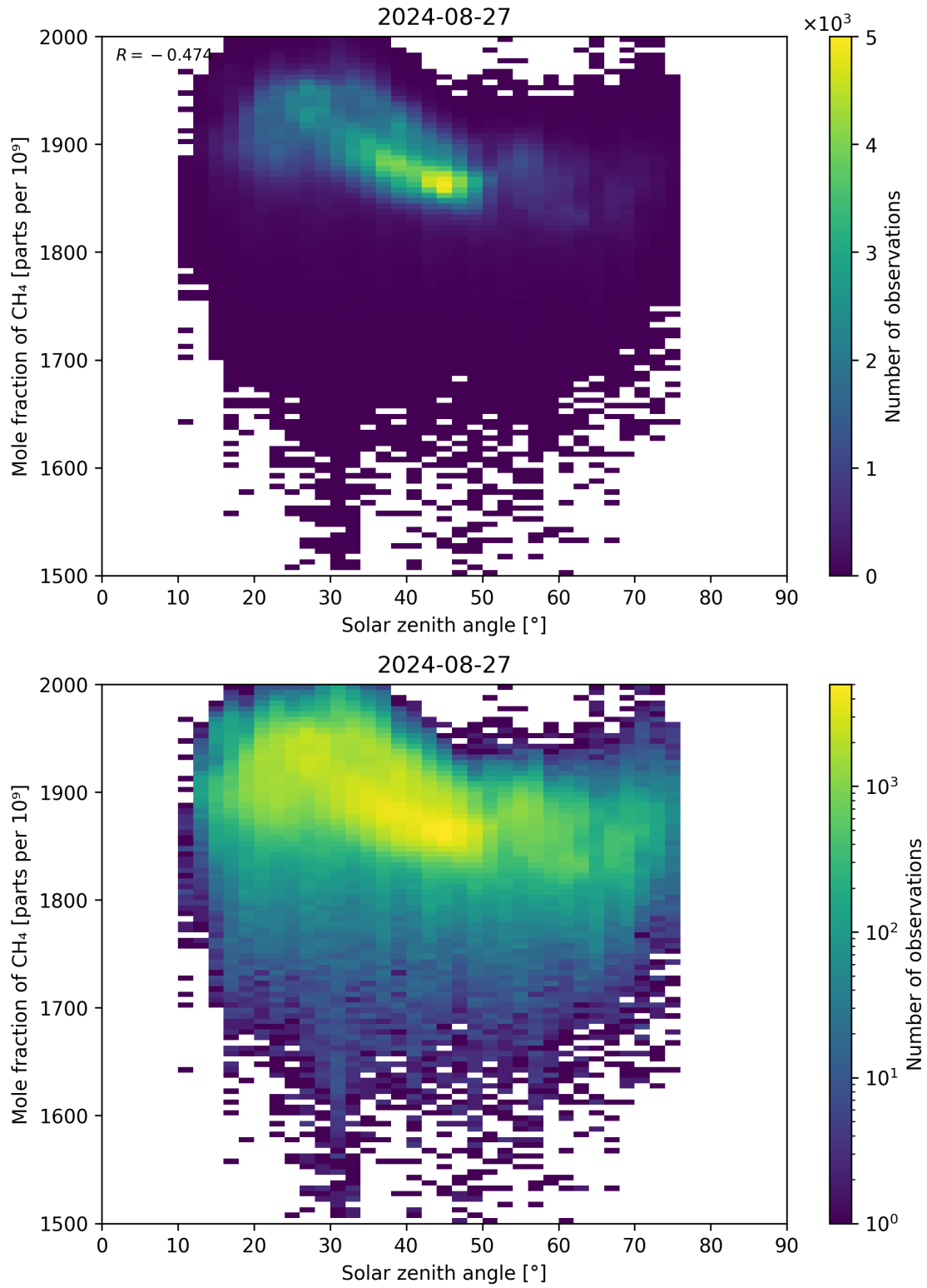
Figure 99: Scatter density plot of “Solar zenith angle” against “Mole fraction of \text{CH}_4 ” for 2024-08-27 to 2024-08-28.
