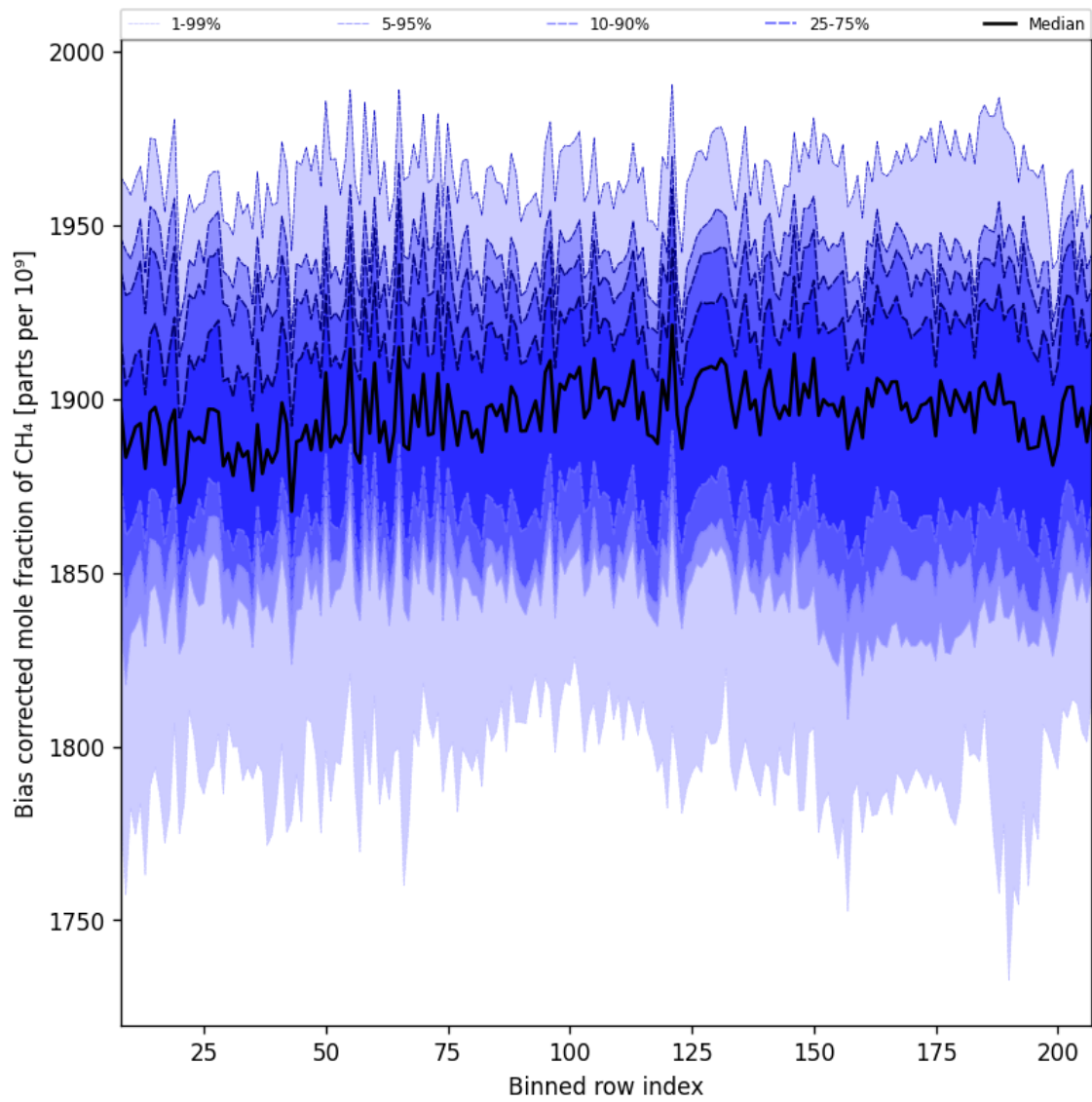
Figure 36: Along track statistics of “Bias corrected mole fraction of CH 4 ” for 2024-08-27 to 2024-08-28
