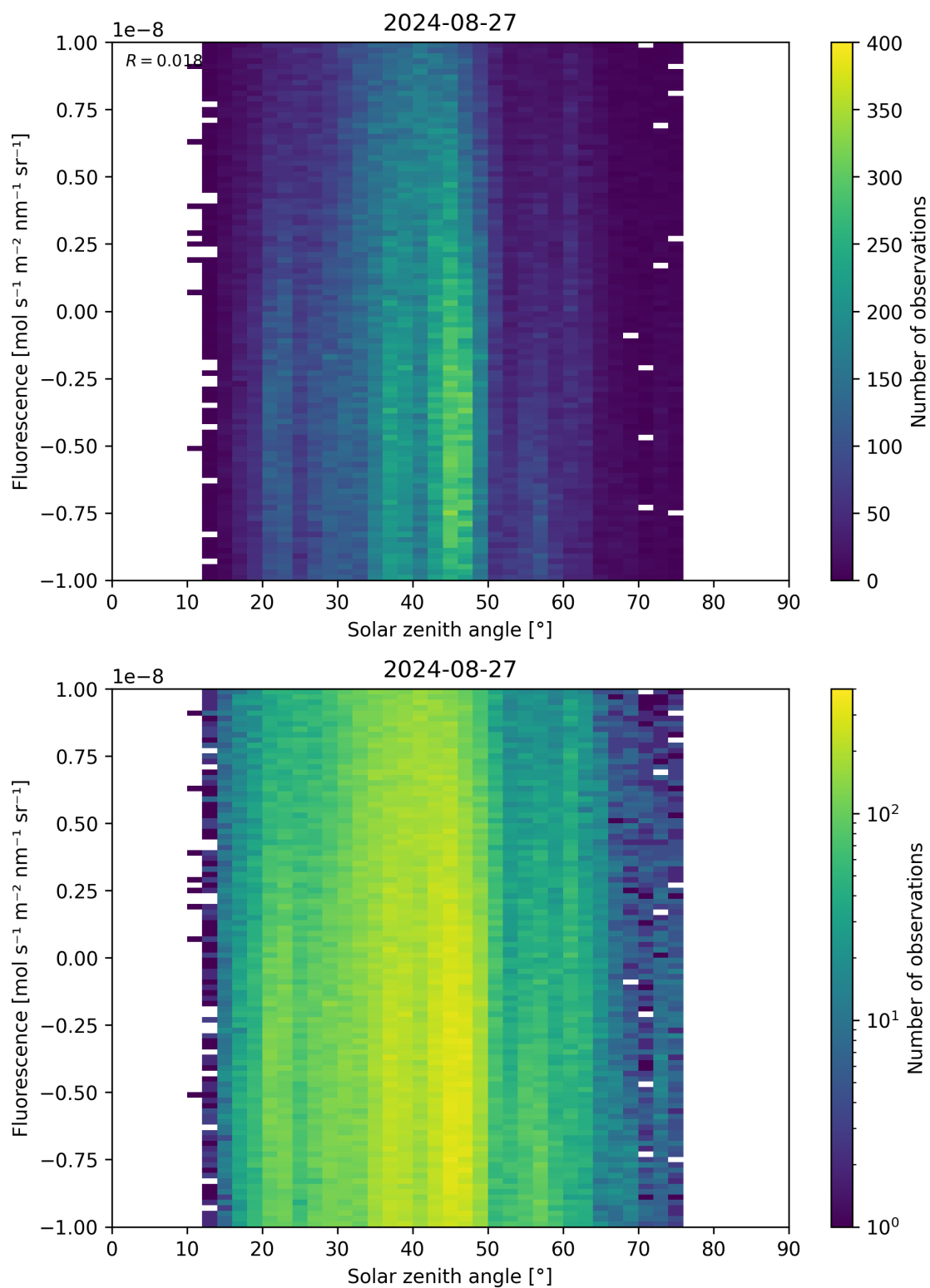
Figure 97: Scatter density plot of “Solar zenith angle” against “Fluorescence” for 2024-08-27 to 2024-08-28.
