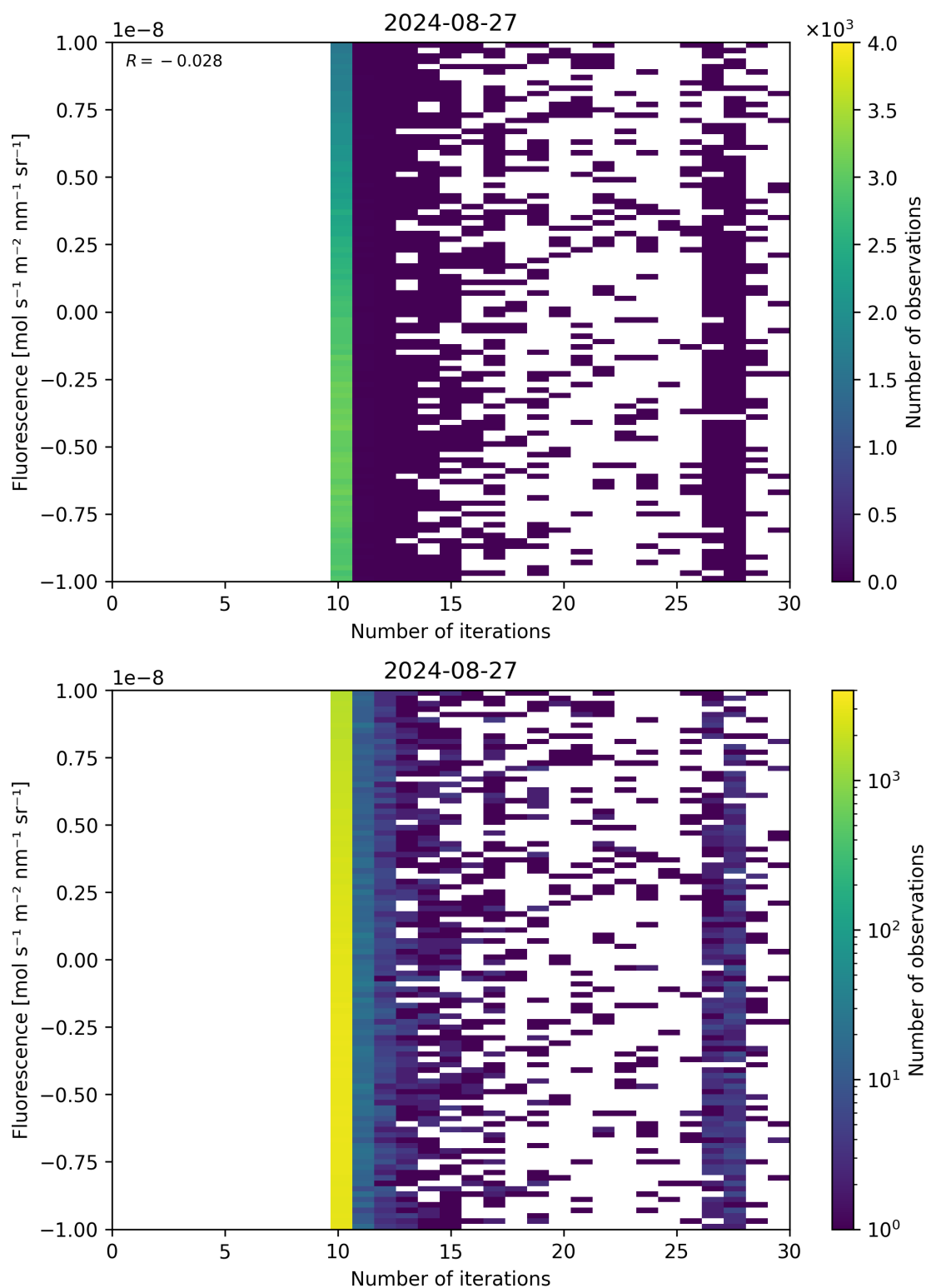
Figure 87: Scatter density plot of “Number of iterations” against “Fluorescence” for 2024-08-27 to 2024-08-28.
