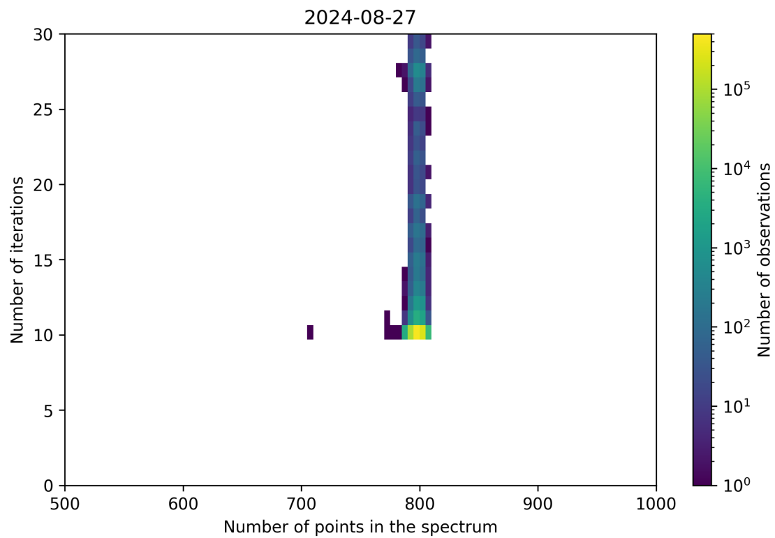
Figure 92: Scatter density plot of “Number of points in the spectrum” against “Number of iterations” for 2024-08-27 to 2024-08-28.
