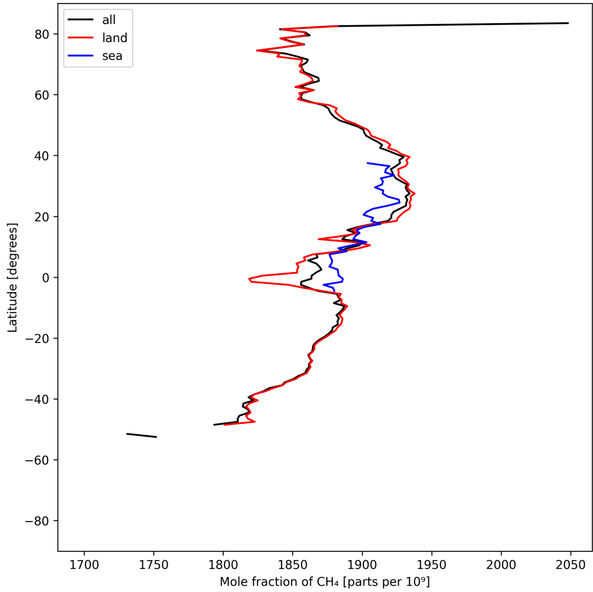
Figure 12: Zonal average of “Mole fraction of CH 4 ” for 2024-08-27 to 2024-08-28.
