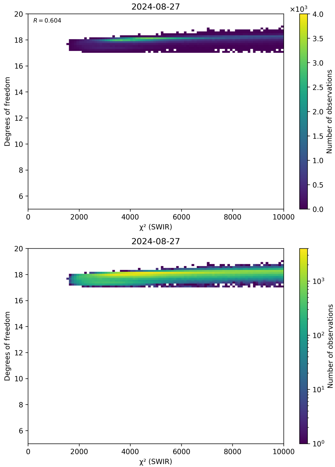
Figure 48: Scatter density plot of “ \chi^2 (SWIR)” against “Degrees of freedom” for 2024-08-27 to 2024-08-28.
