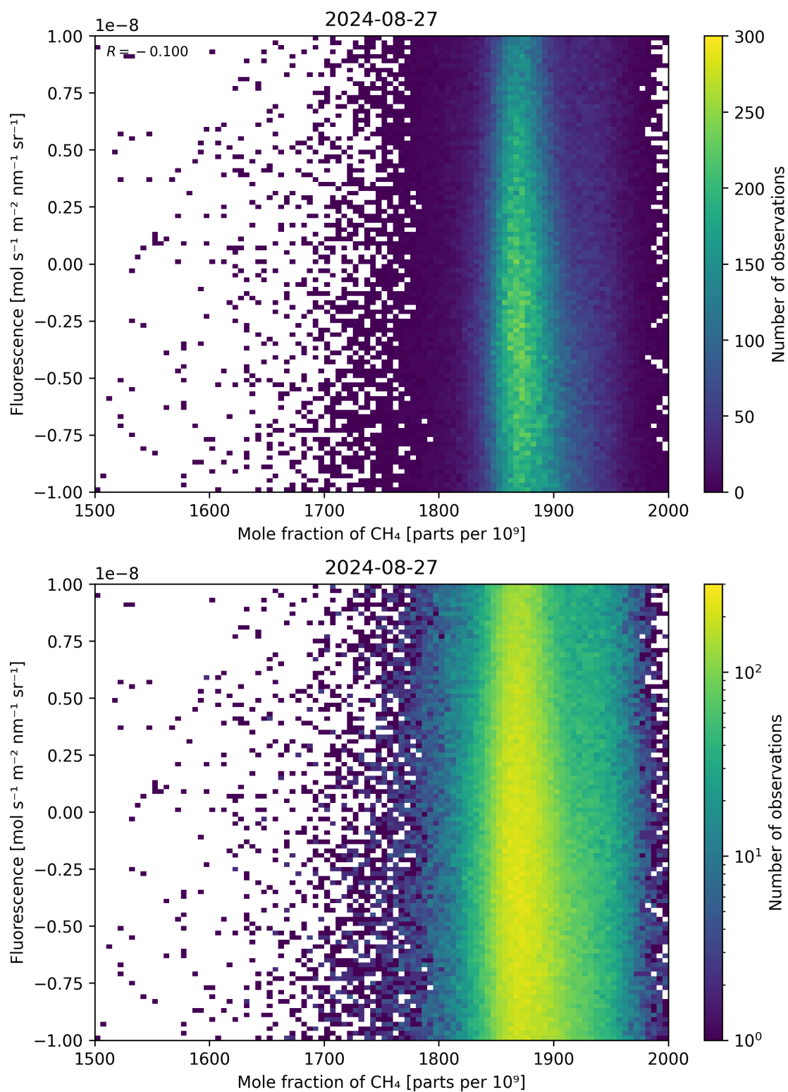
Figure 73: Scatter density plot of “Mole fraction of CH 4 ” against “Fluorescence” for 2024-08-27 to 2024-08-28.
