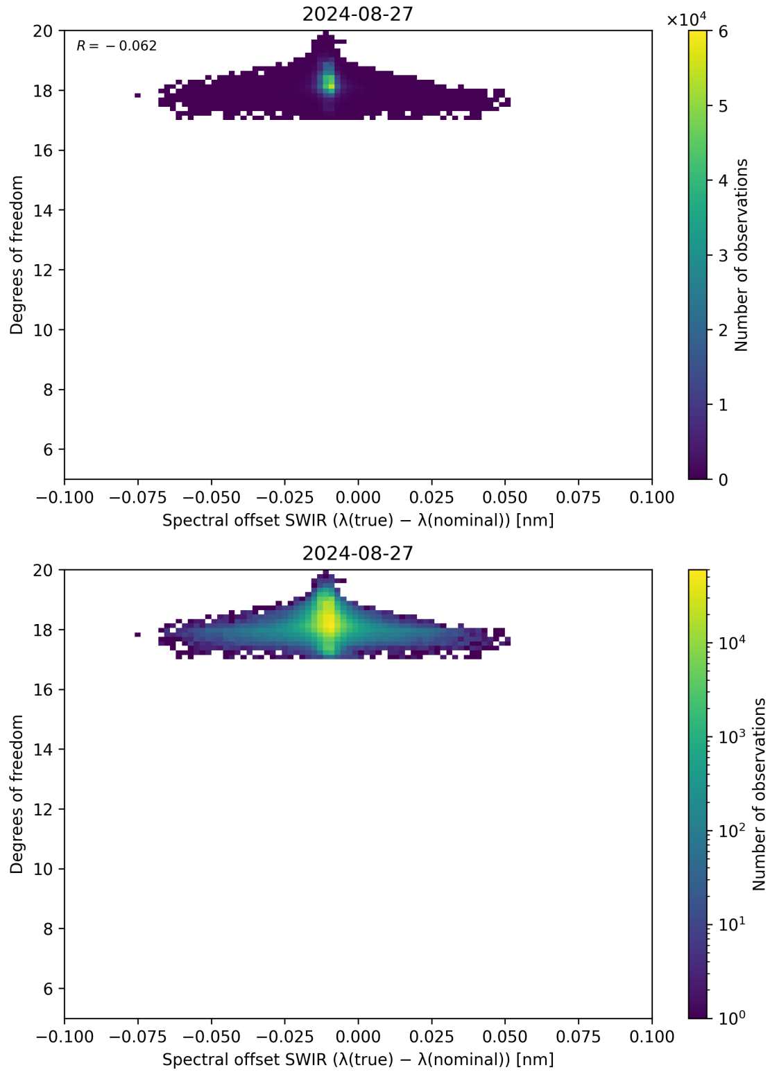
Figure 119: Scatter density plot of “Spectral offset SWIR ( \lambda_{\text{true}} - \lambda_{\text{nominal}} )” against “Degrees of freedom” for 2024-08-27 to 2024-08-28.
