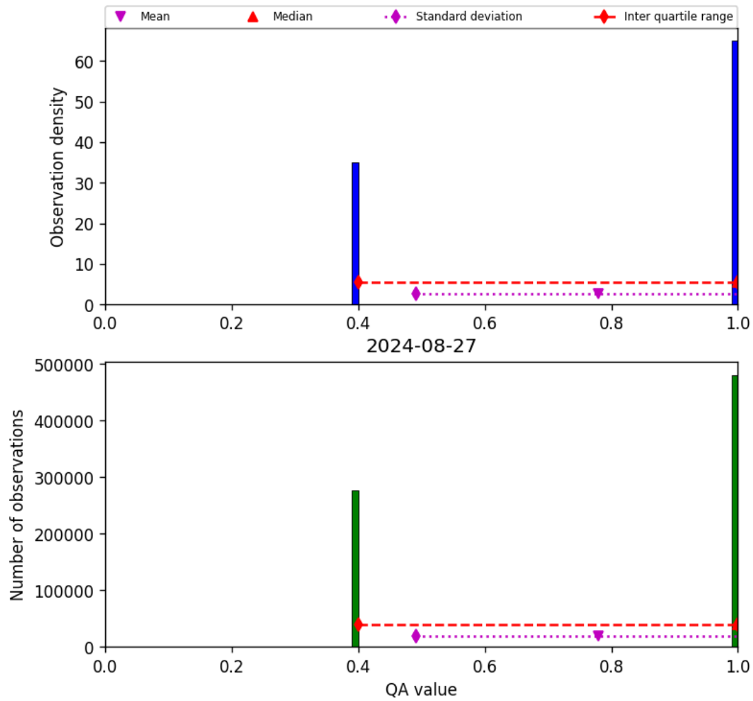
Figure 22: Histogram of “QA value” for 2024-08-27 to 2024-08-28
