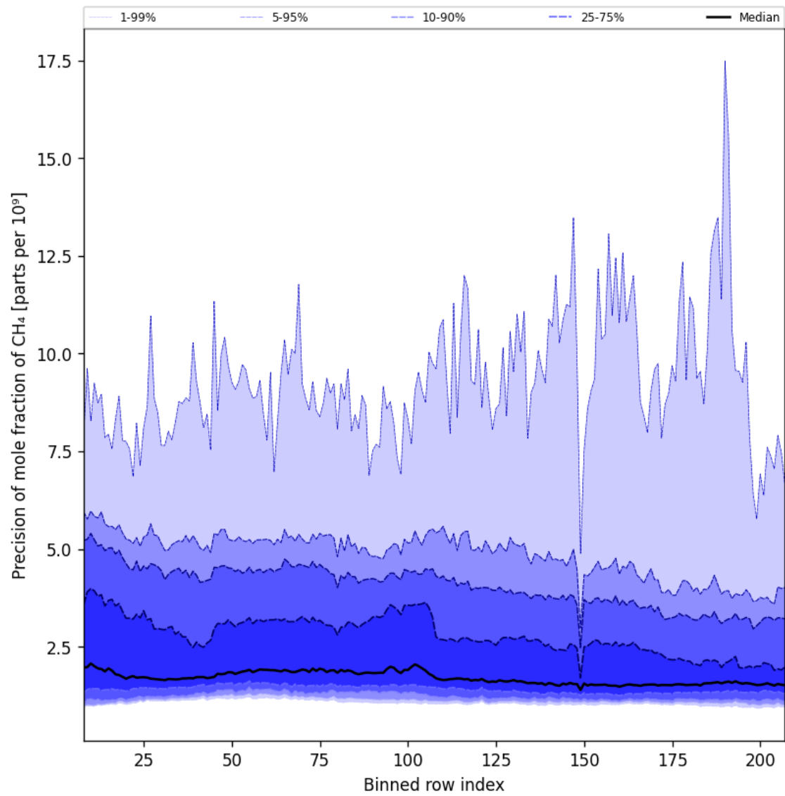
Figure 35: Along track statistics of “Precision of mole fraction of CH 4 ” for 2024-08-27 to 2024-08-28
