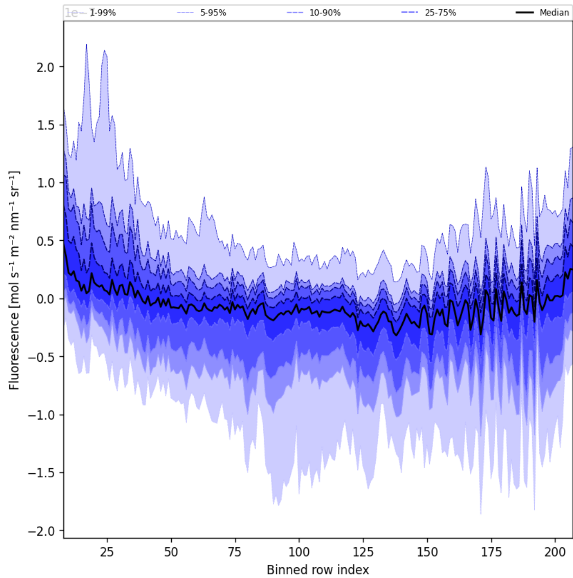
Figure 43: Along track statistics of “Fluorescence” for 2024-08-27 to 2024-08-28
