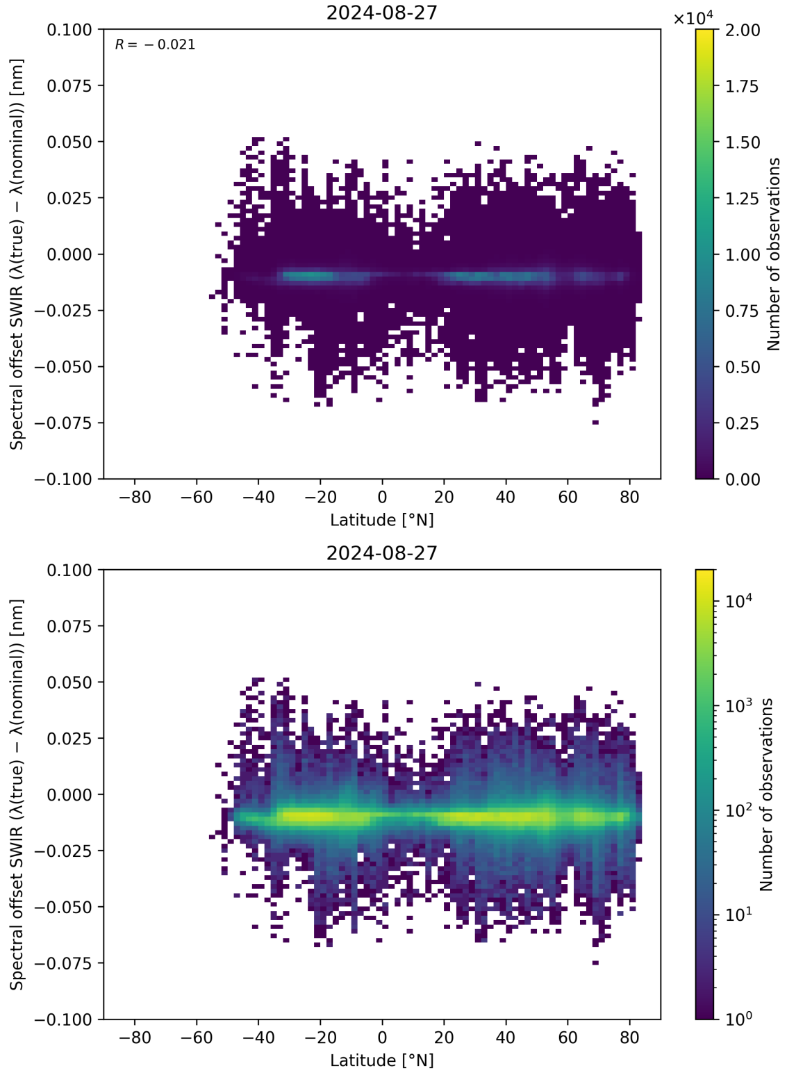
Figure 62: Scatter density plot of “Latitude” against “Spectral offset SWIR ( \lambda_{\text{true}} - \lambda_{\text{nominal}} )” for 2024-08-27 to 2024-08-28.
