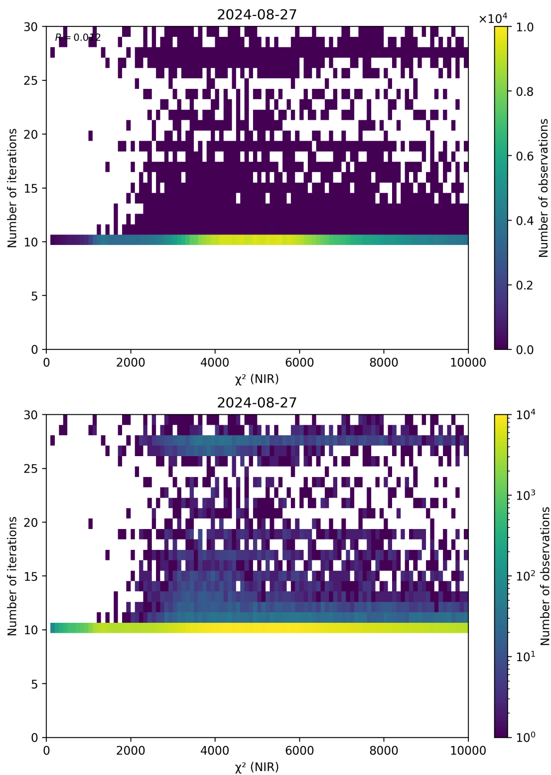
Figure 46: Scatter density plot of “ \chi^2 (NIR)” against “Number of iterations” for 2024-08-27 to 2024-08-28.
