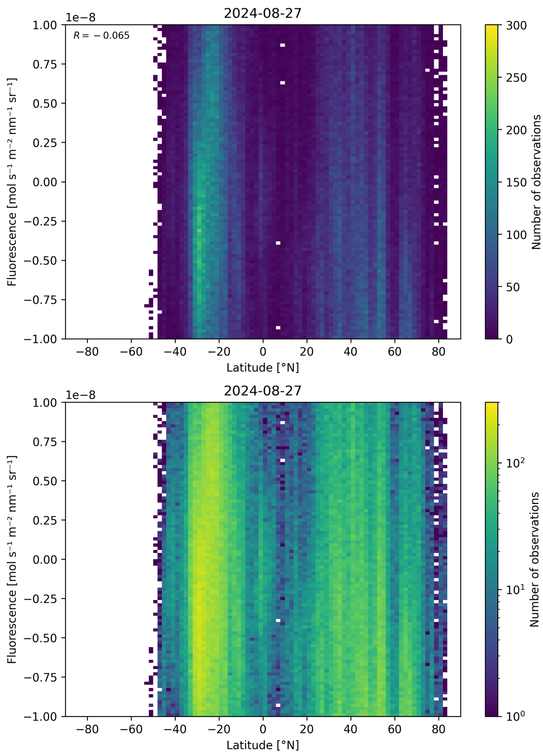
Figure 56: Scatter density plot of “Latitude” against “Fluorescence” for 2024-08-27 to 2024-08-28.
