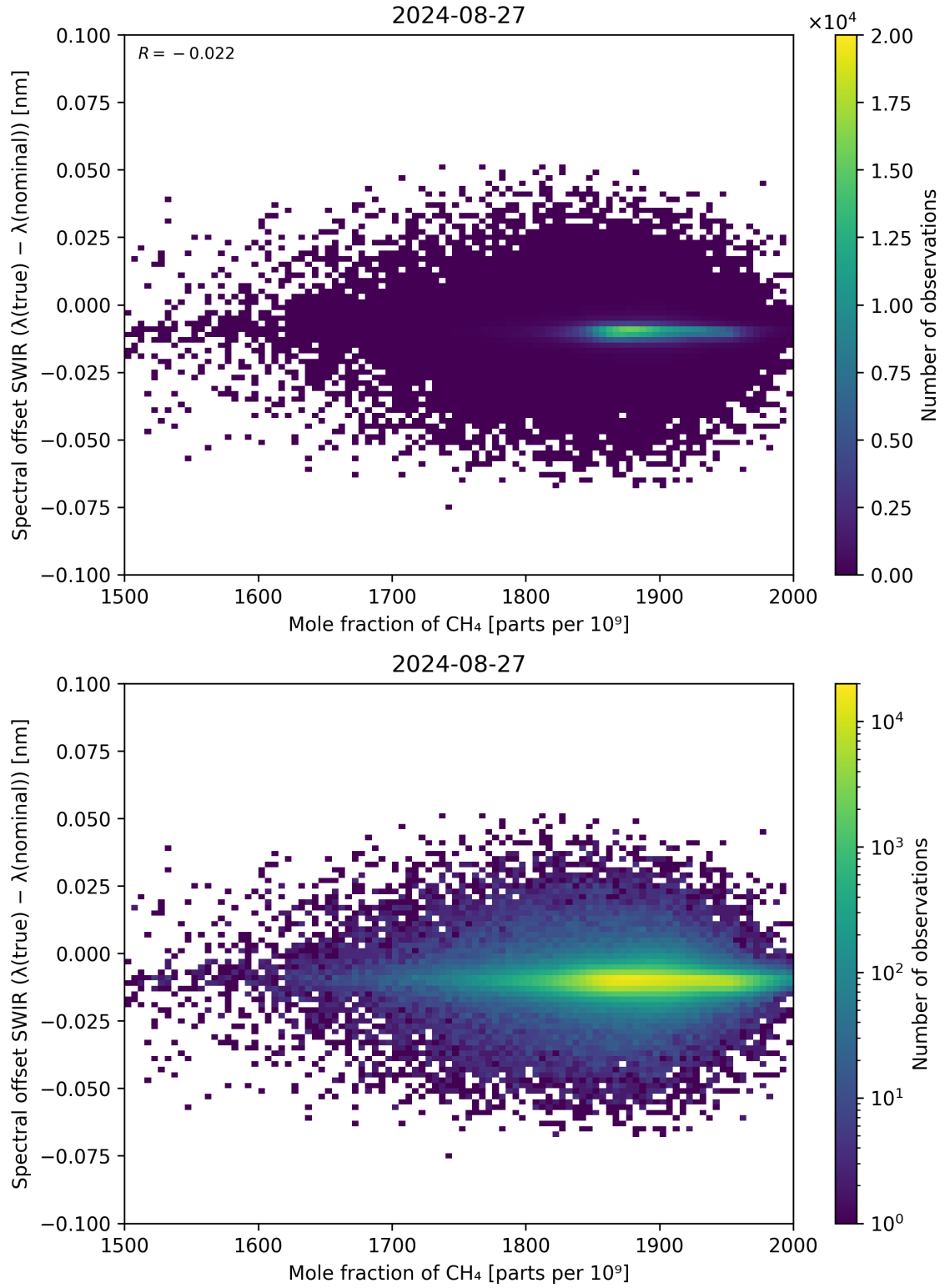
Figure 86: Scatter density plot of “Mole fraction of CH 4 ” against “Spectral offset SWIR ( \lambda_{\text{true}} - \lambda_{\text{nominal}} )” for 2024-08-27 to 2024-08-28.
