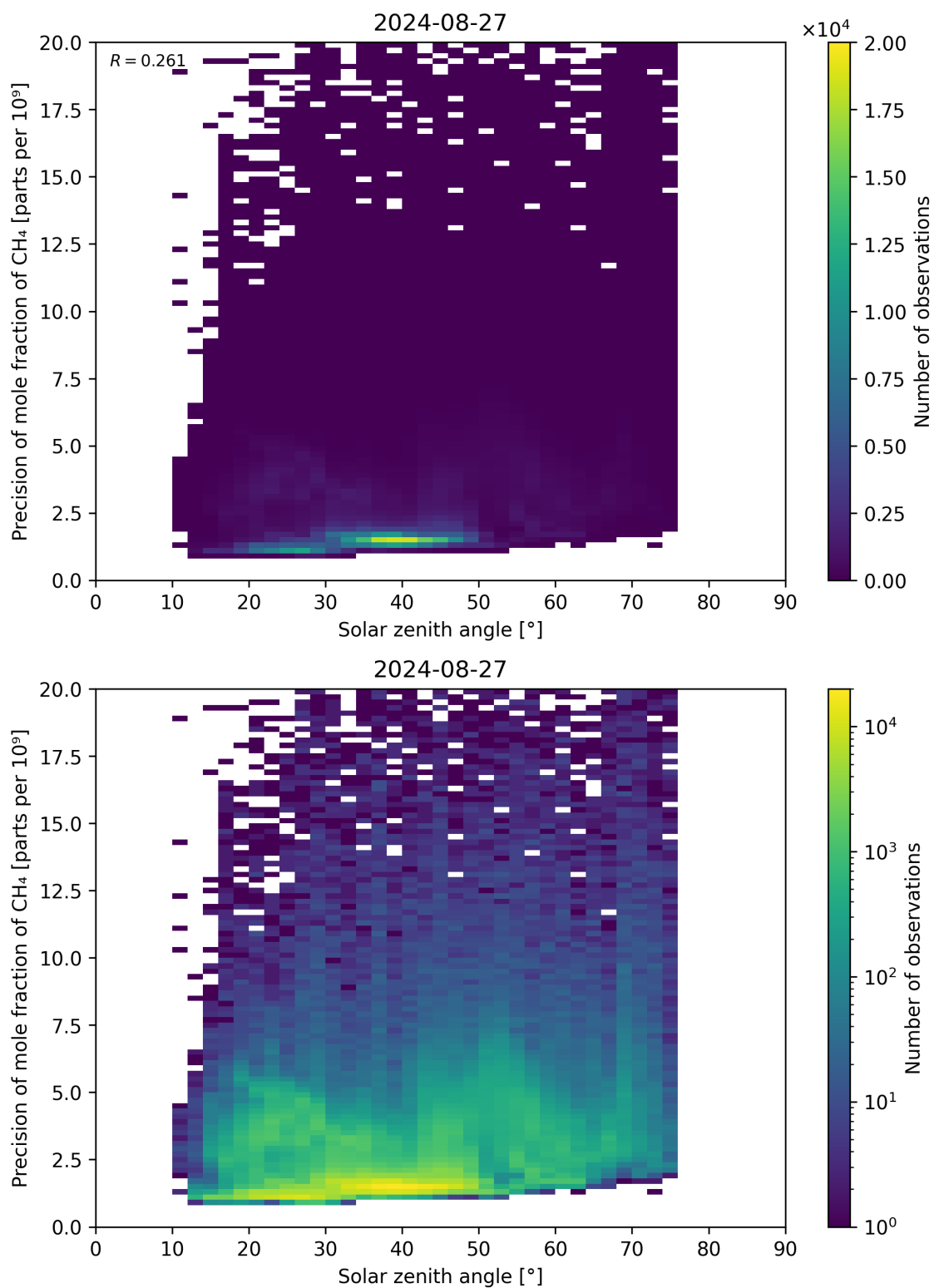
Figure 101: Scatter density plot of “Solar zenith angle” against “Precision of mole fraction of CH 4 ” for 2024-08-27 to 2024-08-28.
