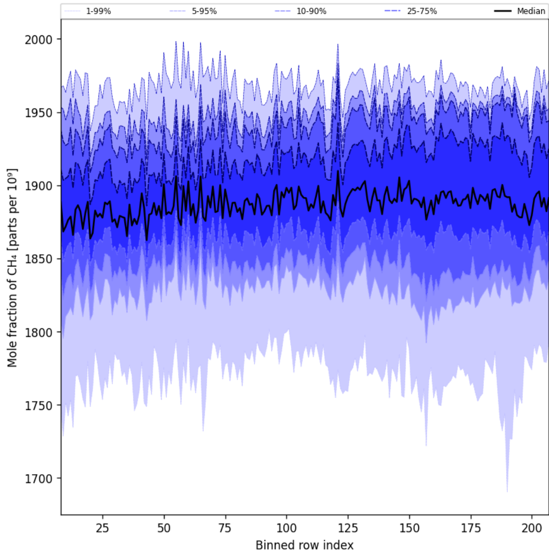
Figure 34: Along track statistics of “Mole fraction of CH 4 ” for 2024-08-27 to 2024-08-28
