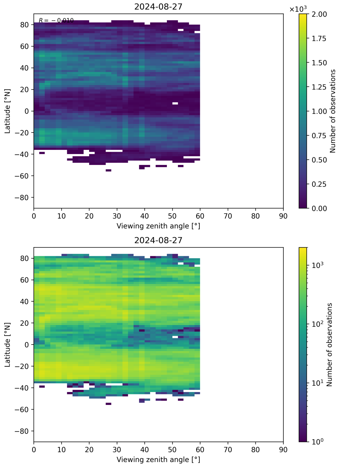
Figure 109: Scatter density plot of “Viewing zenith angle” against “Latitude” for 2024-08-27 to 2024-08-28.
