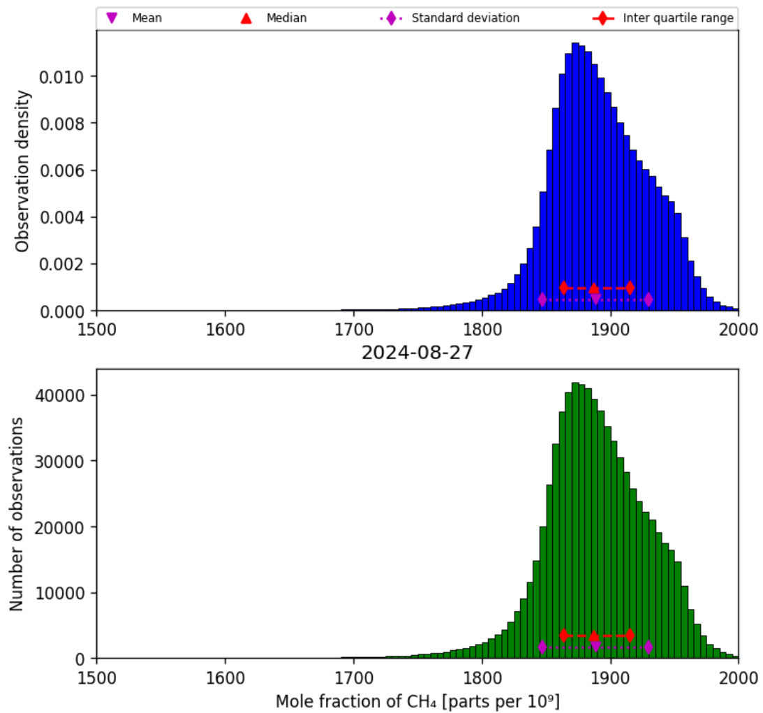
Figure 23: Histogram of “Mole fraction of CH 4 ” for 2024-08-27 to 2024-08-28
