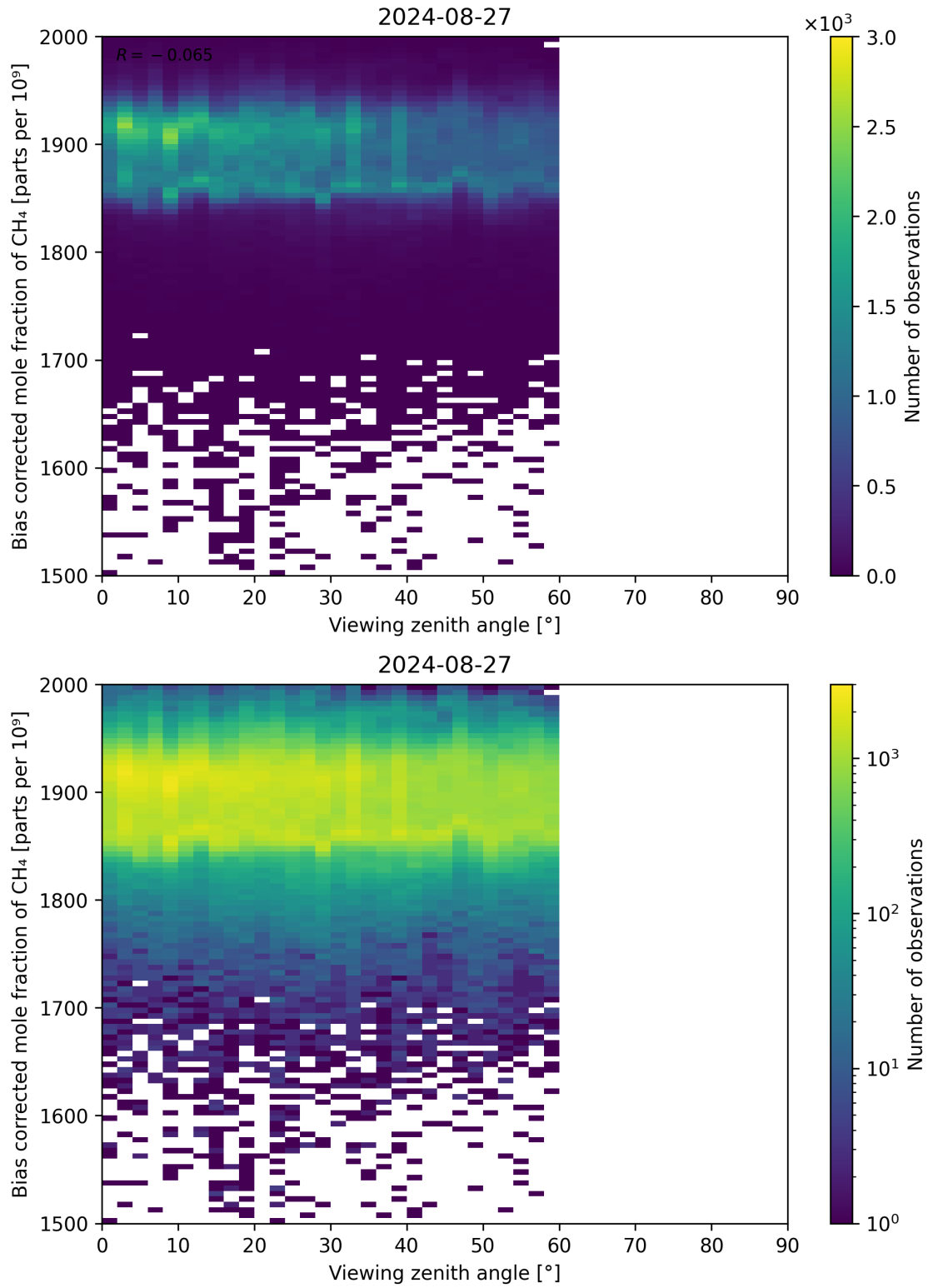
Figure 111: Scatter density plot of “Viewing zenith angle” against “Bias corrected mole fraction of CH 4 ” for 2024-08-27 to 2024-08-28.
