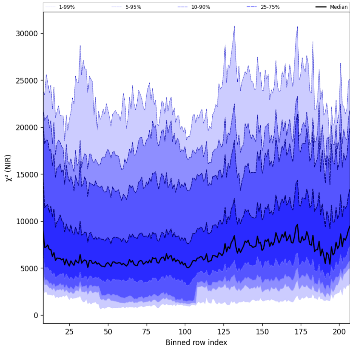
Figure 40: Along track statistics of “ \chi^2 (NIR)” for 2024-08-27 to 2024-08-28
