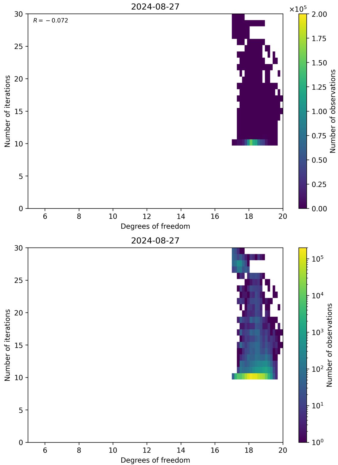
Figure 52: Scatter density plot of “Degrees of freedom” against “Number of iterations” for 2024-08-27 to 2024-08-28.
