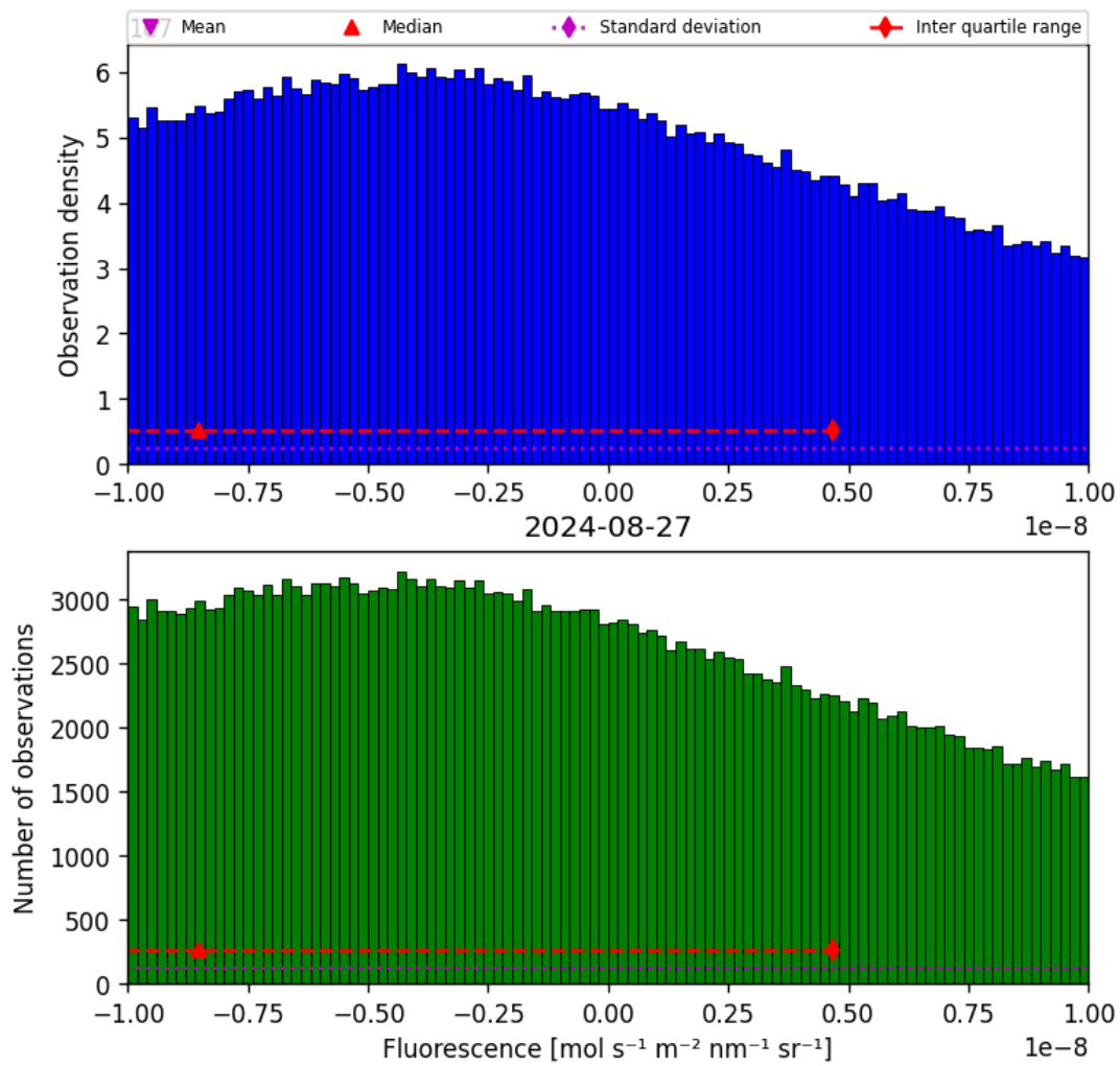
Figure 32: Histogram of “Fluorescence” for 2024-08-27 to 2024-08-28
