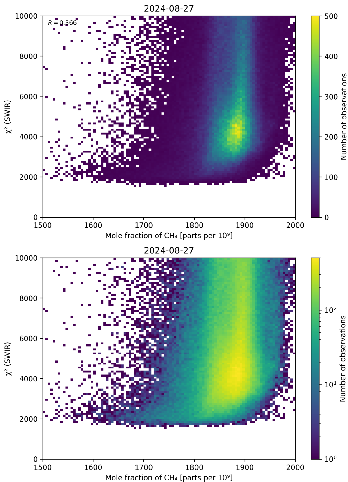
Figure 71: Scatter density plot of “Mole fraction of \text{CH}_4 ” against “ \chi^2 (SWIR)” for 2024-08-27 to 2024-08-28.
