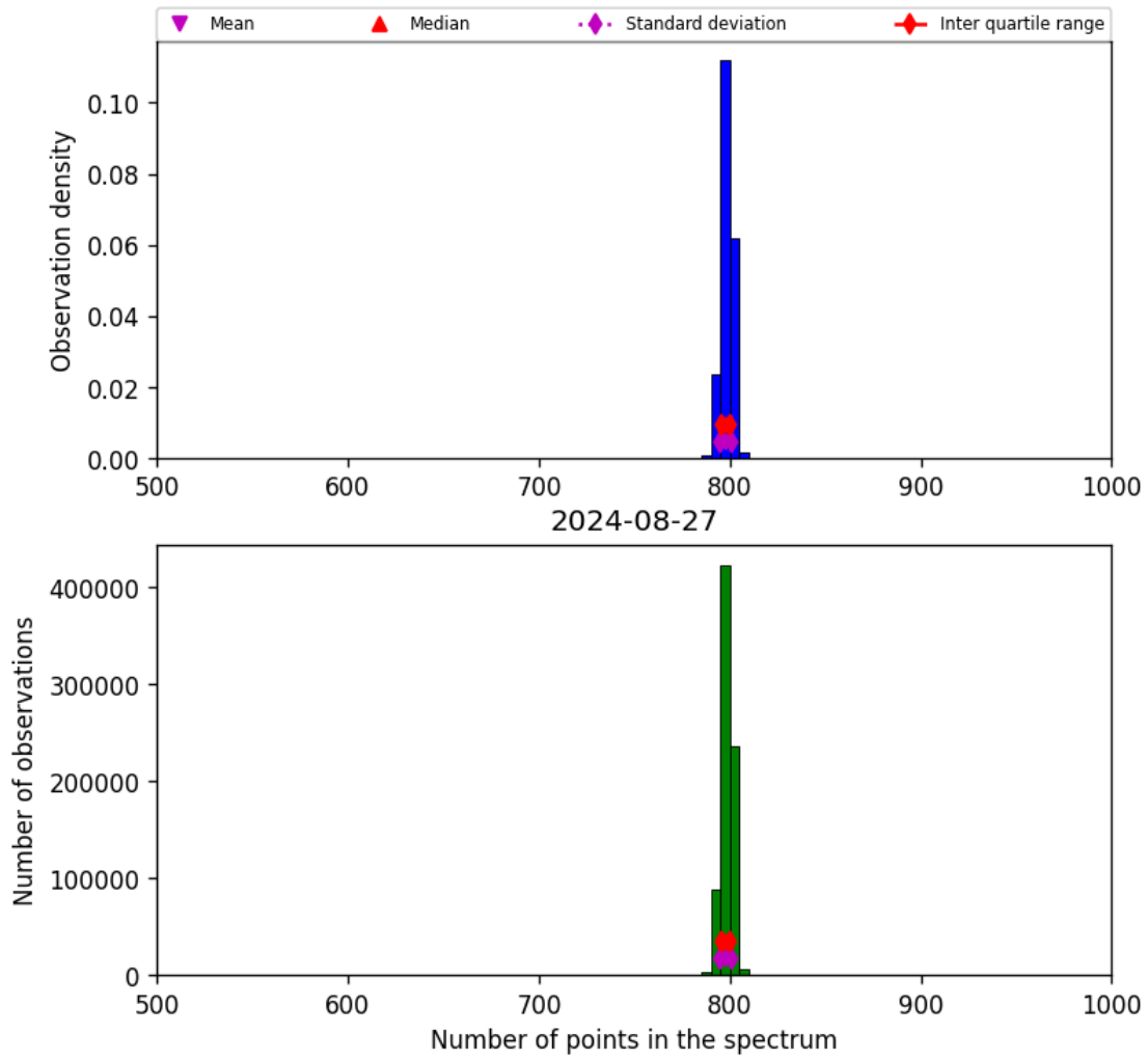
Figure 26: Histogram of “Number of points in the spectrum” for 2024-08-27 to 2024-08-28
