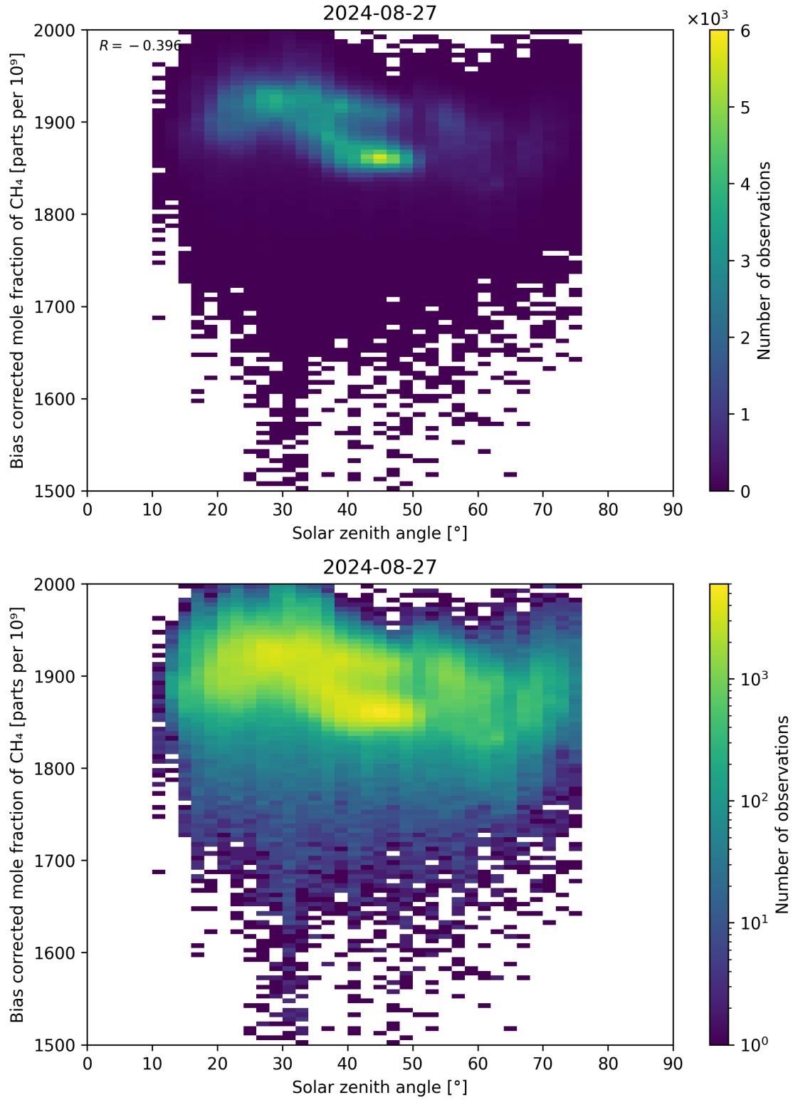
Figure 100: Scatter density plot of “Solar zenith angle” against “Bias corrected mole fraction of CH 4 ” for 2024-08-27 to 2024-08-28.
