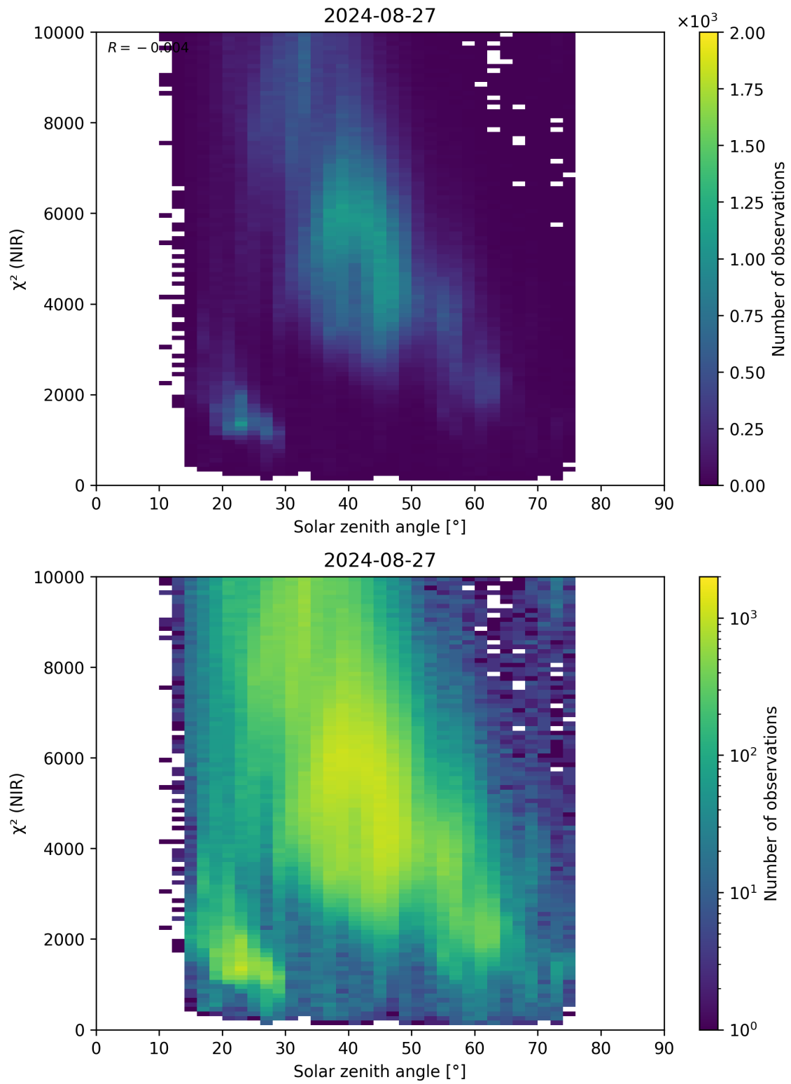
Figure 94: Scatter density plot of “Solar zenith angle” against “ \chi^2 (NIR)” for 2024-08-27 to 2024-08-28.
