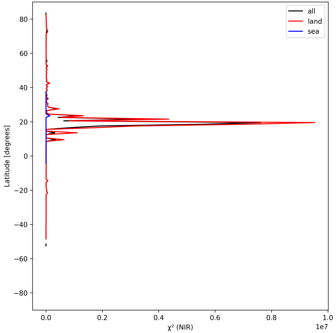
Figure 18: Zonal average of “ \chi^2 (NIR)” for 2024-08-27 to 2024-08-28.
