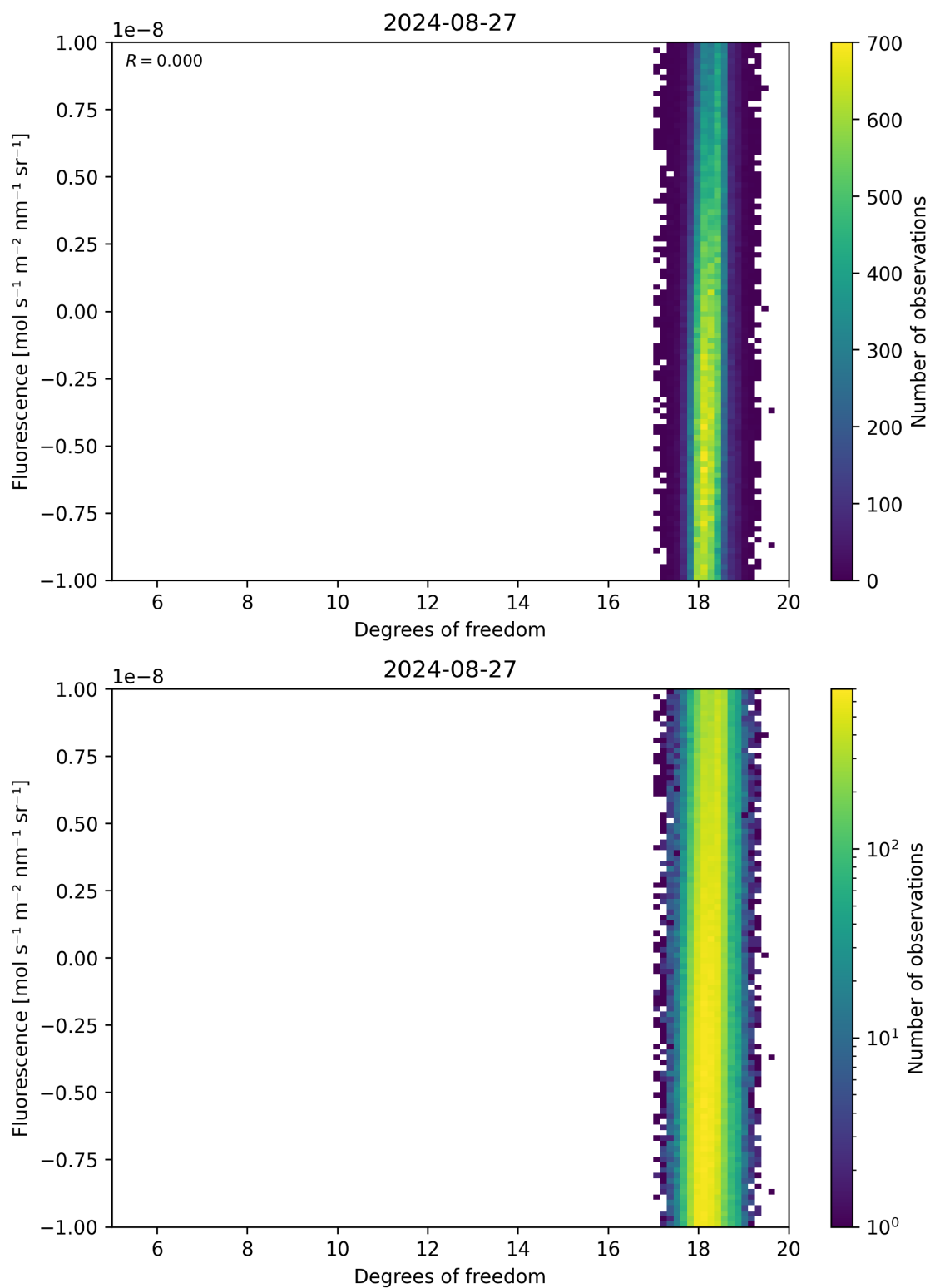
Figure 51: Scatter density plot of “Degrees of freedom” against “Fluorescence” for 2024-08-27 to 2024-08-28.
