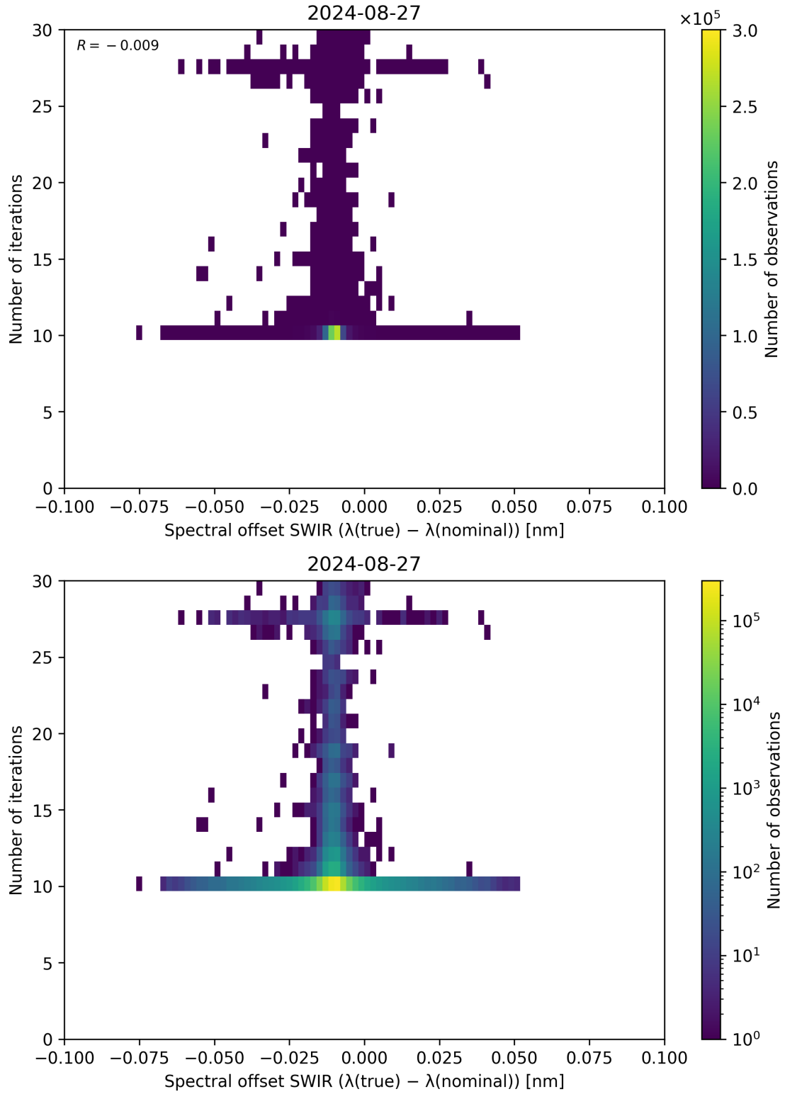
Figure 121: Scatter density plot of “Spectral offset SWIR ( \lambda_{\text{true}} - \lambda_{\text{nominal}} )” against “Number of iterations” for 2024-08-27 to 2024-08-28.
