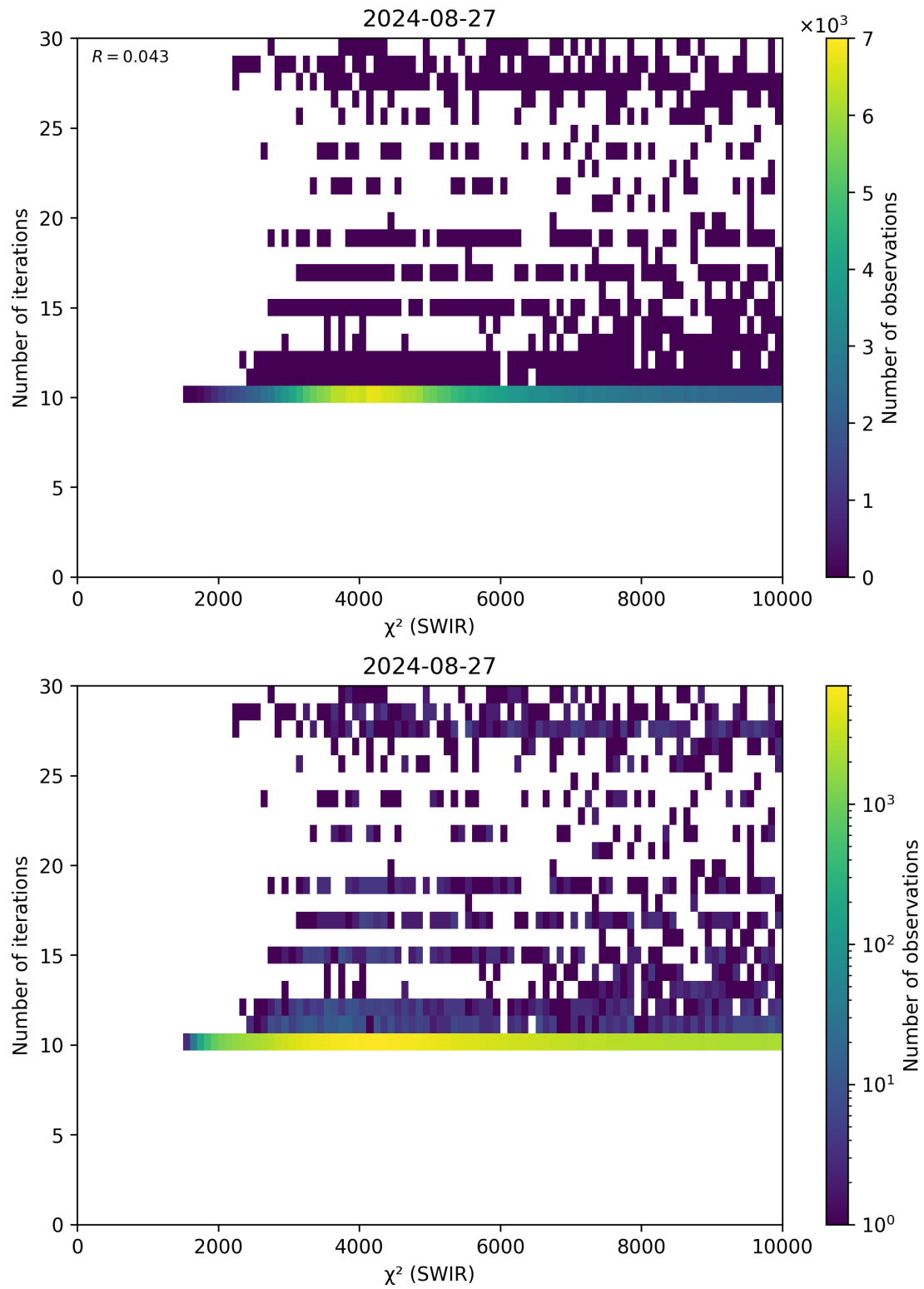
Figure 50: Scatter density plot of “ \chi^2 (SWIR)” against “Number of iterations” for 2024-08-27 to 2024-08-28.
