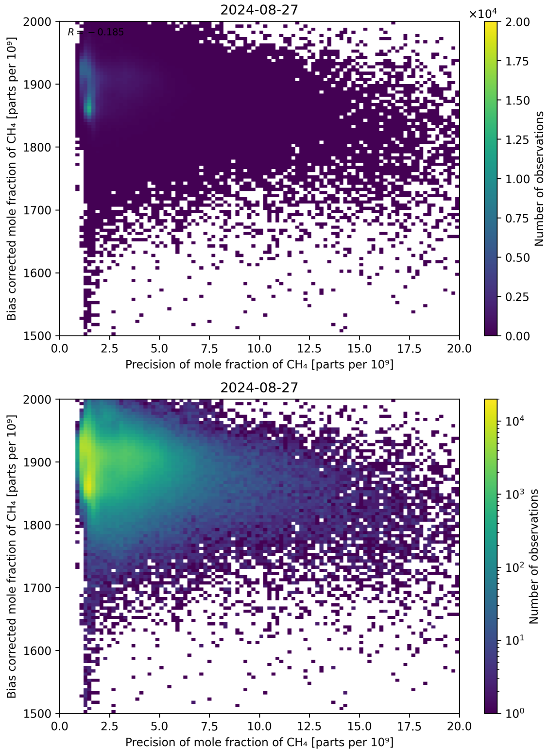
Figure 82: Scatter density plot of “Precision of mole fraction of CH 4 ” against “Bias corrected mole fraction of CH 4 ” for 2024-08-27 to 2024-08-28.
