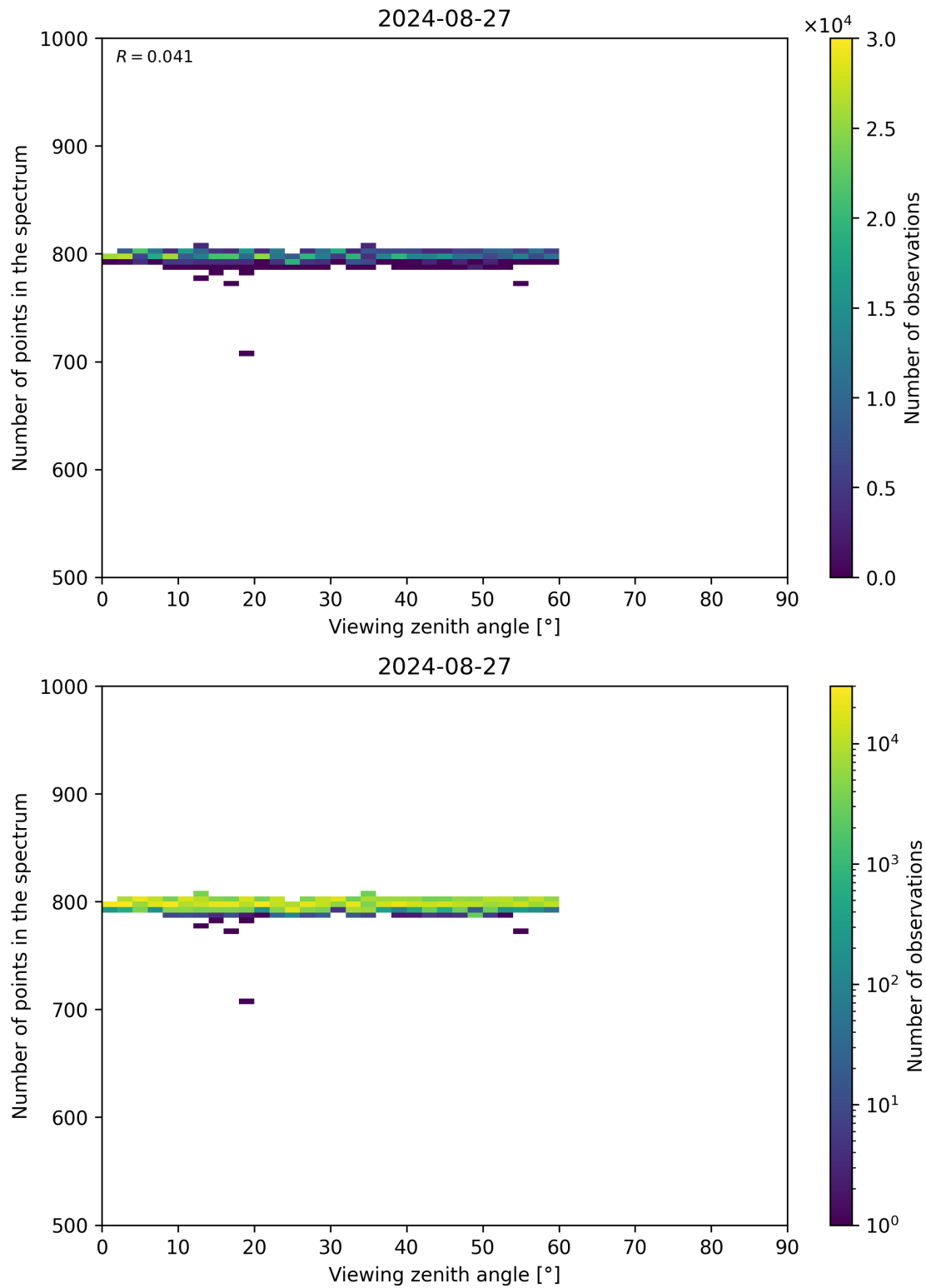
Figure 114: Scatter density plot of “Viewing zenith angle” against “Number of points in the spectrum” for 2024-08-27 to 2024-08-28.
