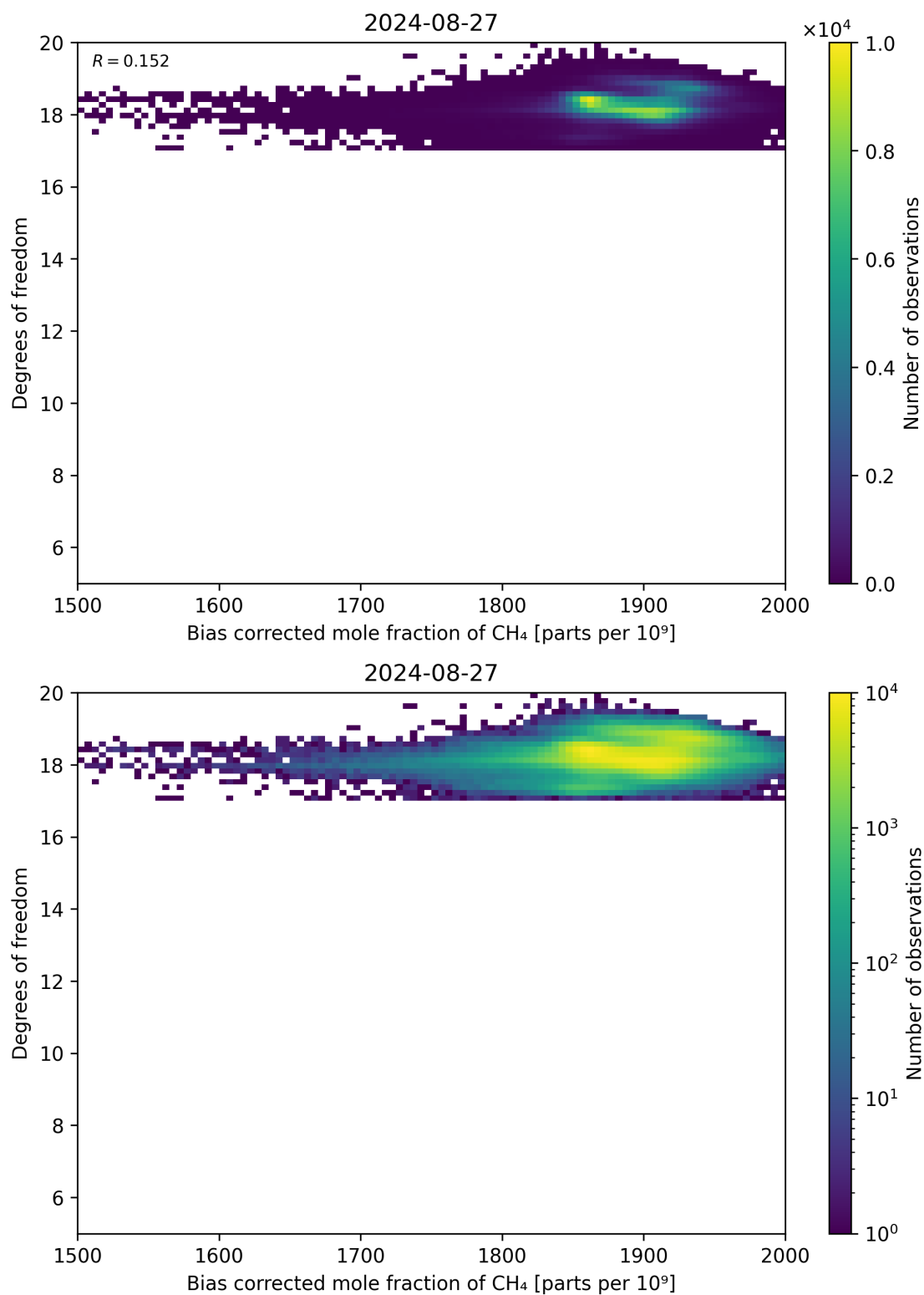
Figure 65: Scatter density plot of “Bias corrected mole fraction of CH 4 ” against “Degrees of freedom” for 2024-08-27 to 2024-08-28.
