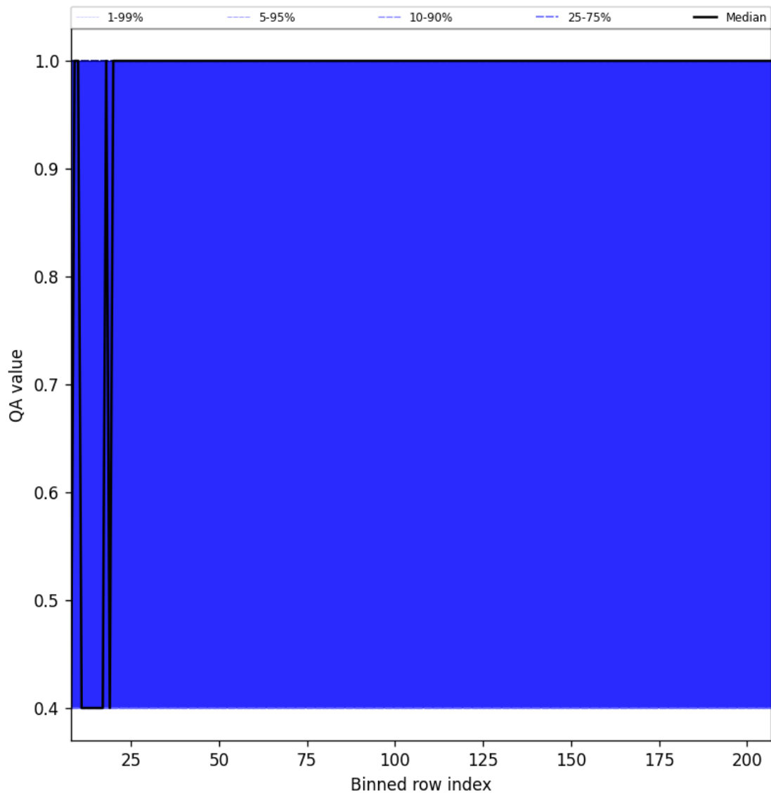
Figure 33: Along track statistics of “QA value” for 2024-08-27 to 2024-08-28
