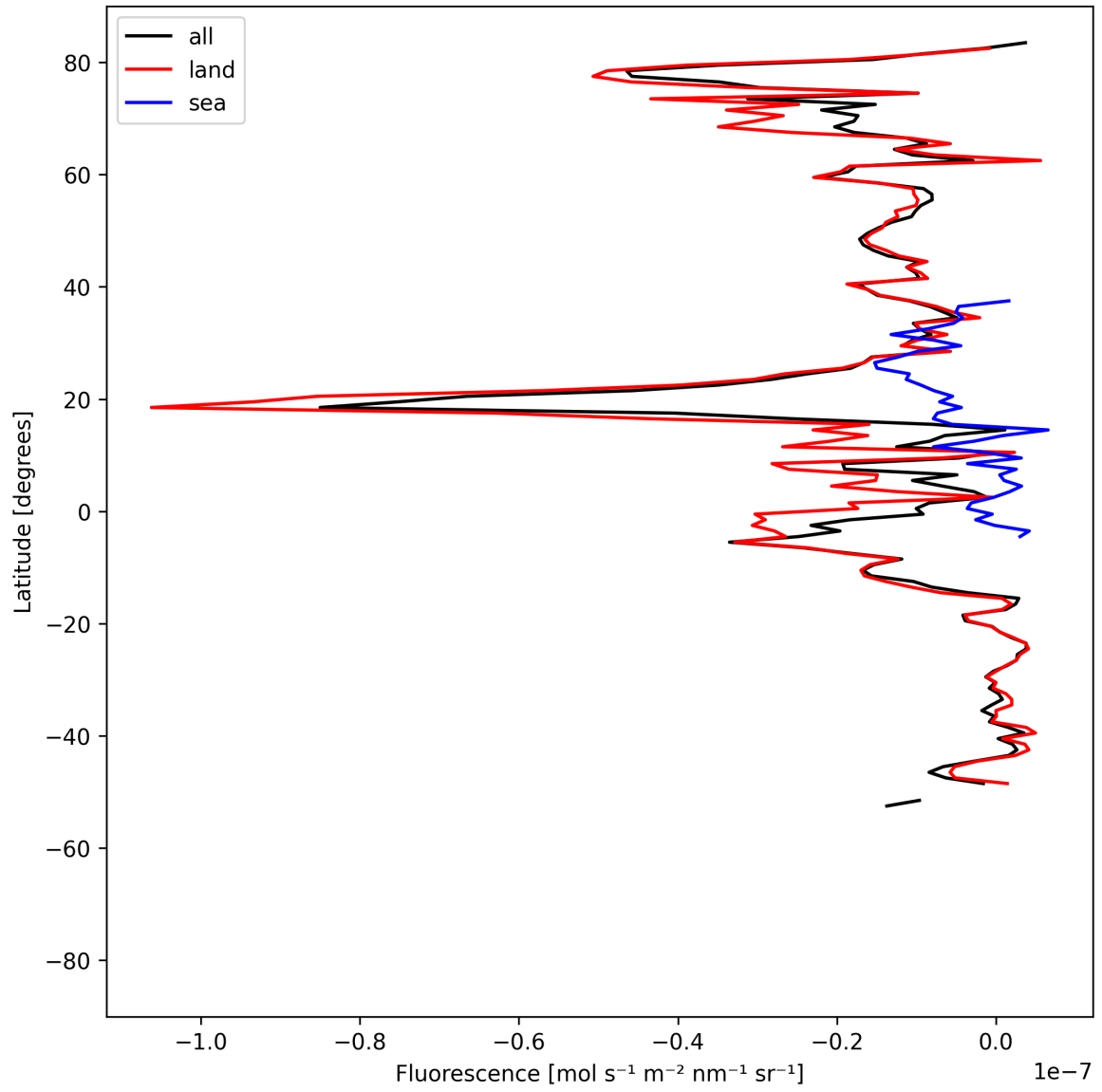
Figure 21: Zonal average of “Fluorescence” for 2024-08-27 to 2024-08-28.
