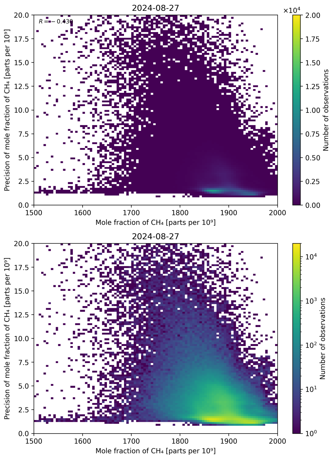
Figure 75: Scatter density plot of “Mole fraction of CH 4 ” against “Precision of mole fraction of CH 4 ” for 2024-08-27 to 2024-08-28.
