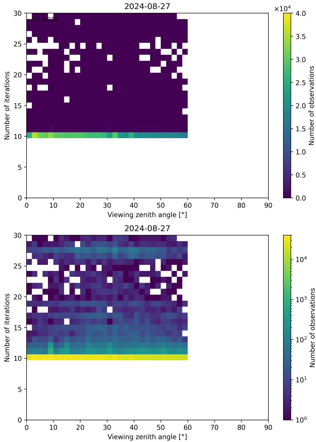
Figure 113: Scatter density plot of “Viewing zenith angle” against “Number of iterations” for 2024-08-27 to 2024-08-28.
