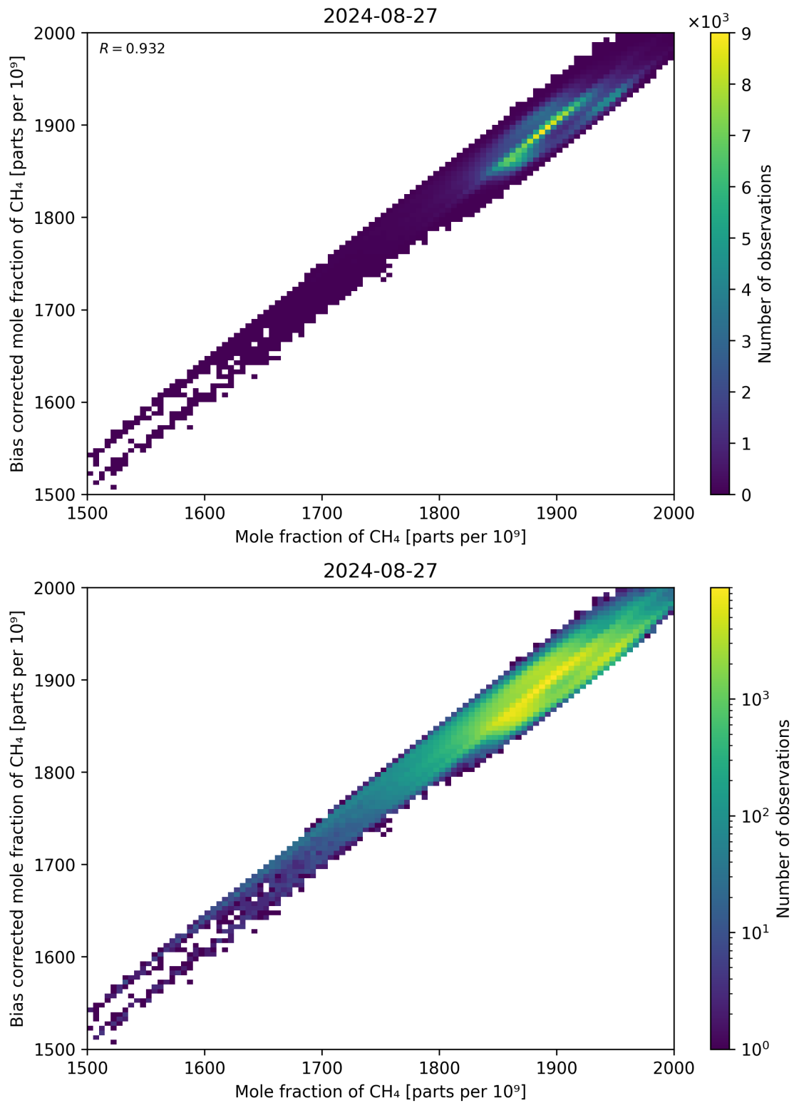
Figure 74: Scatter density plot of “Mole fraction of CH 4 ” against “Bias corrected mole fraction of CH 4 ” for 2024-08-27 to 2024-08-28.
