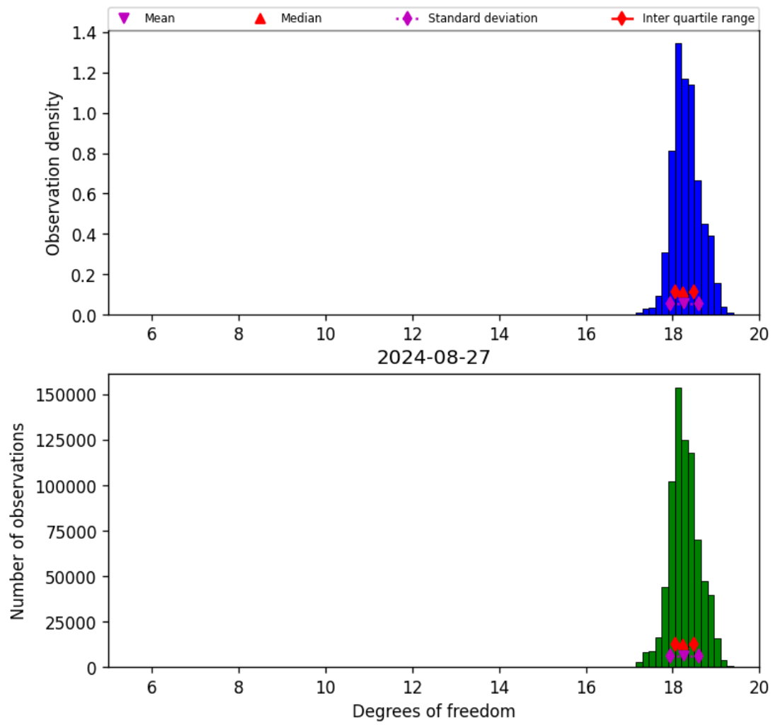
Figure 30: Histogram of “Degrees of freedom” for 2024-08-27 to 2024-08-28
