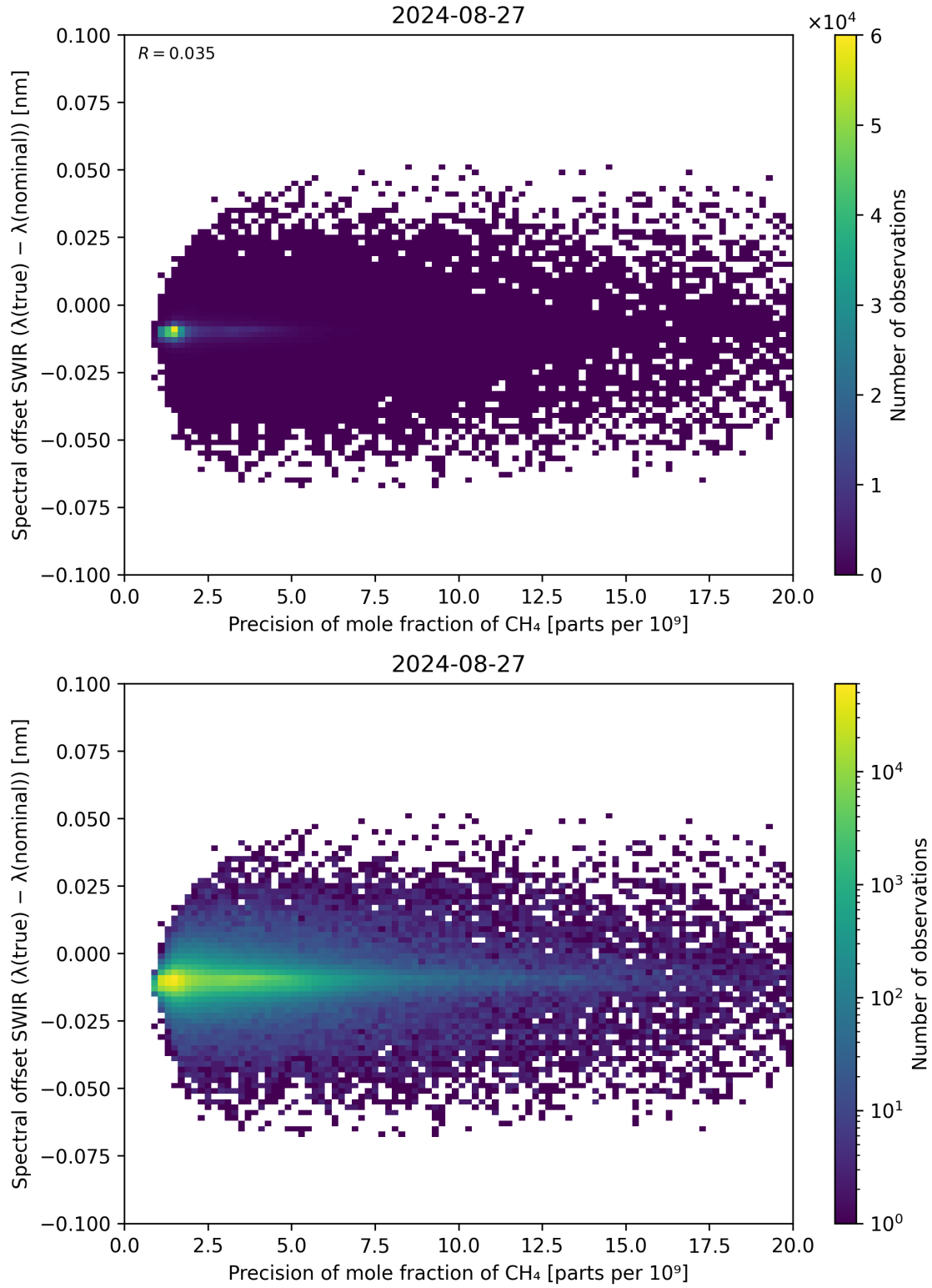
Figure 85: Scatter density plot of “Precision of mole fraction of CH 4 ” against “Spectral offset SWIR ( \lambda_{\text{true}} - \lambda_{\text{nominal}} )” for 2024-08-27 to 2024-08-28.
