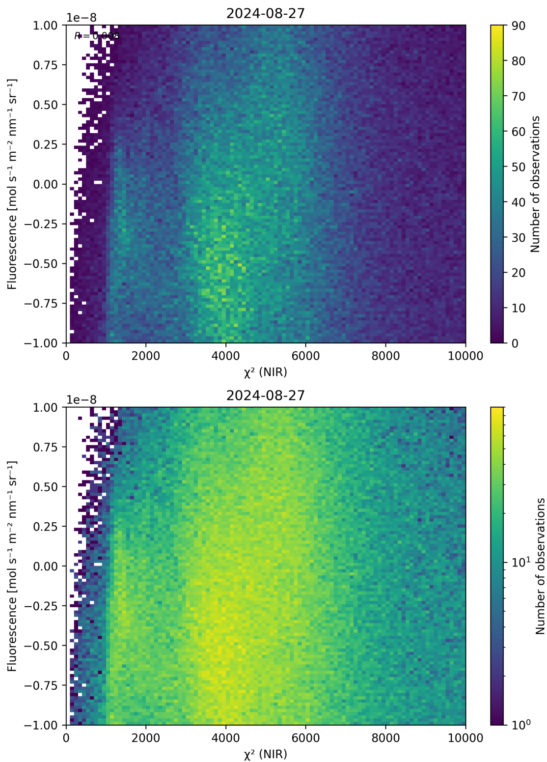
Figure 45: Scatter density plot of “ \chi^2 (NIR)” against “Fluorescence” for 2024-08-27 to 2024-08-28.
