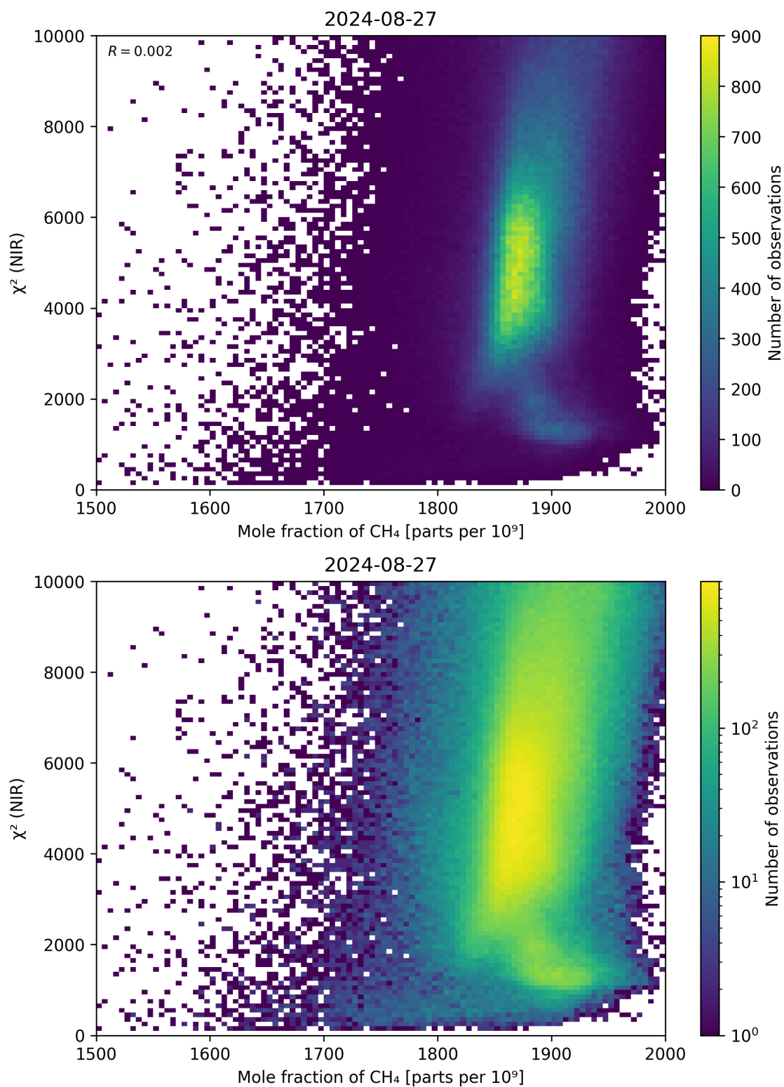
Figure 70: Scatter density plot of “Mole fraction of \text{CH}_4 ” against “ \chi^2 (NIR)” for 2024-08-27 to 2024-08-28.
