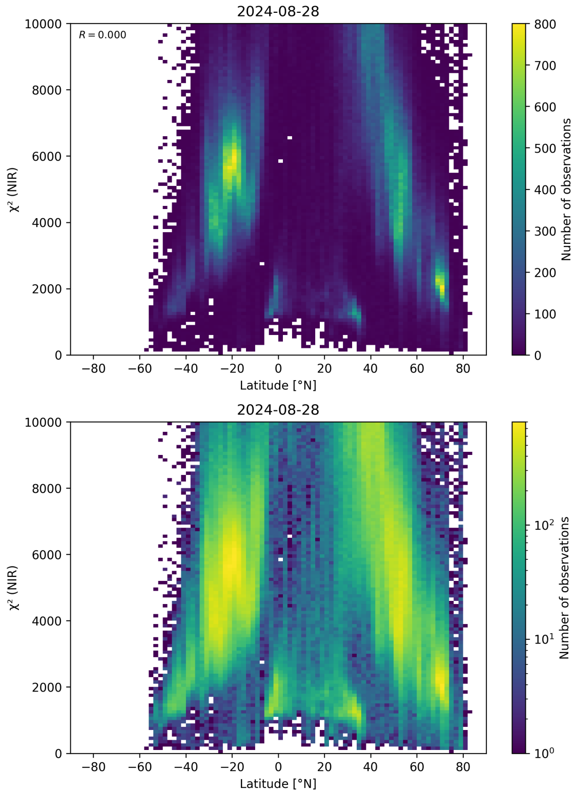
Figure 53: Scatter density plot of “Latitude” against “ \chi^2 (NIR)” for 2024-08-27 to 2024-08-29.
