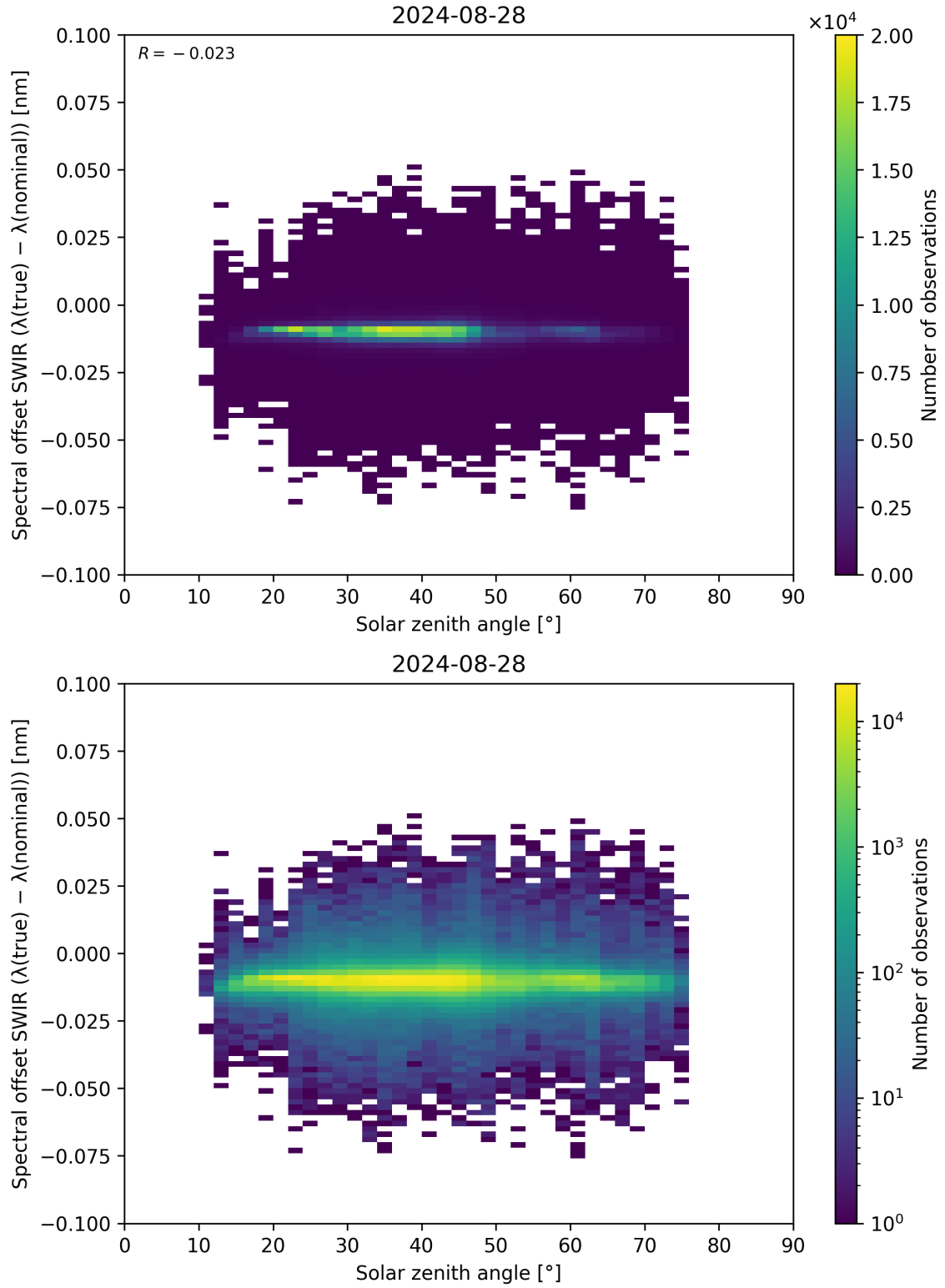
Figure 104: Scatter density plot of “Solar zenith angle” against “Spectral offset SWIR ( \lambda_{\text{true}} - \lambda_{\text{nominal}} )” for 2024-08-27 to 2024-08-29.
