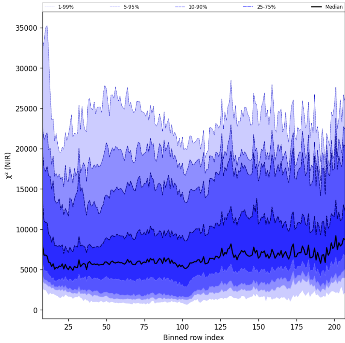
Figure 40: Along track statistics of “ \chi^2 (NIR)” for 2024-08-27 to 2024-08-29
