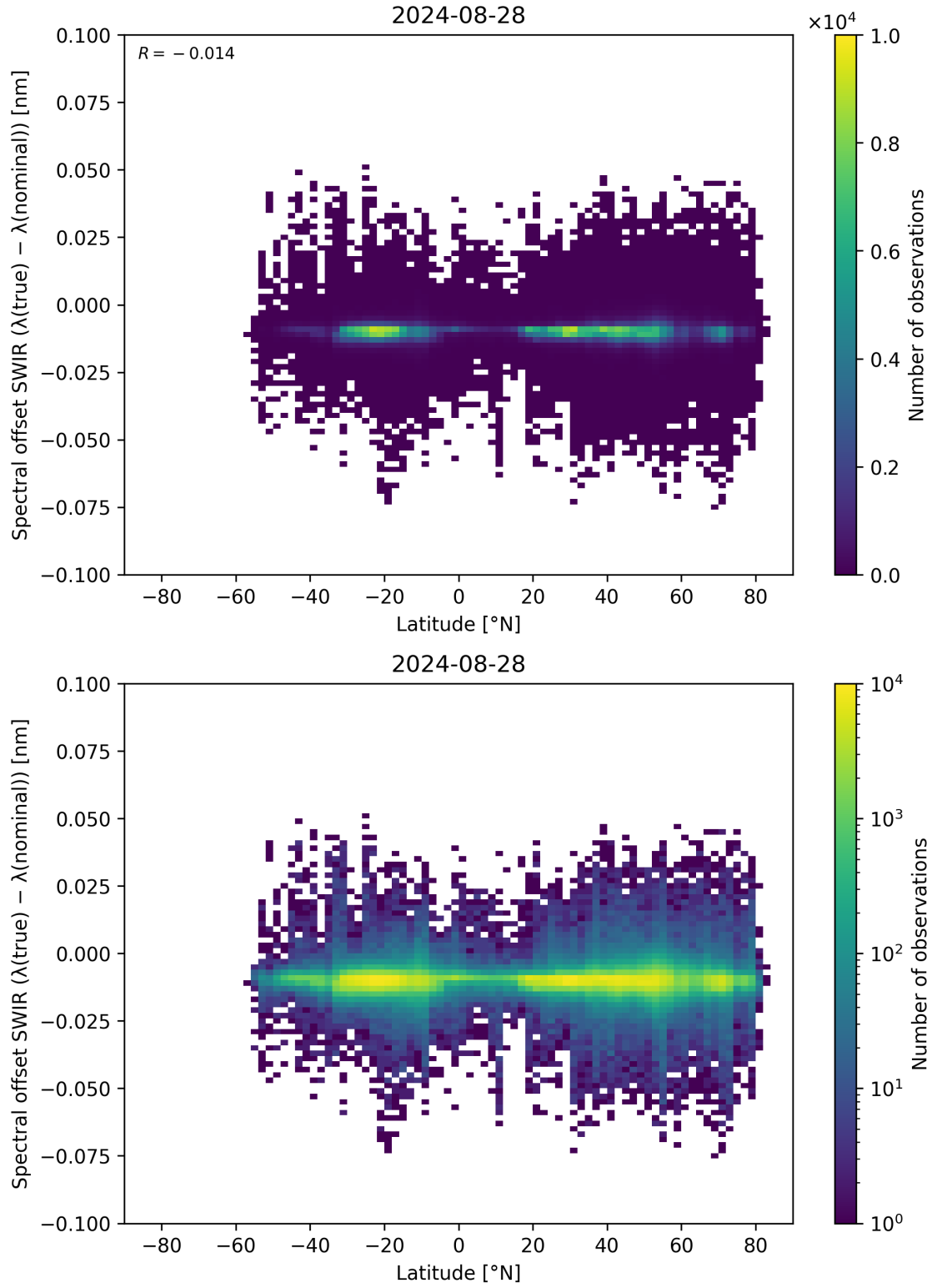
Figure 62: Scatter density plot of “Latitude” against “Spectral offset SWIR ( \lambda_{\text{true}} - \lambda_{\text{nominal}} )” for 2024-08-27 to 2024-08-29.
