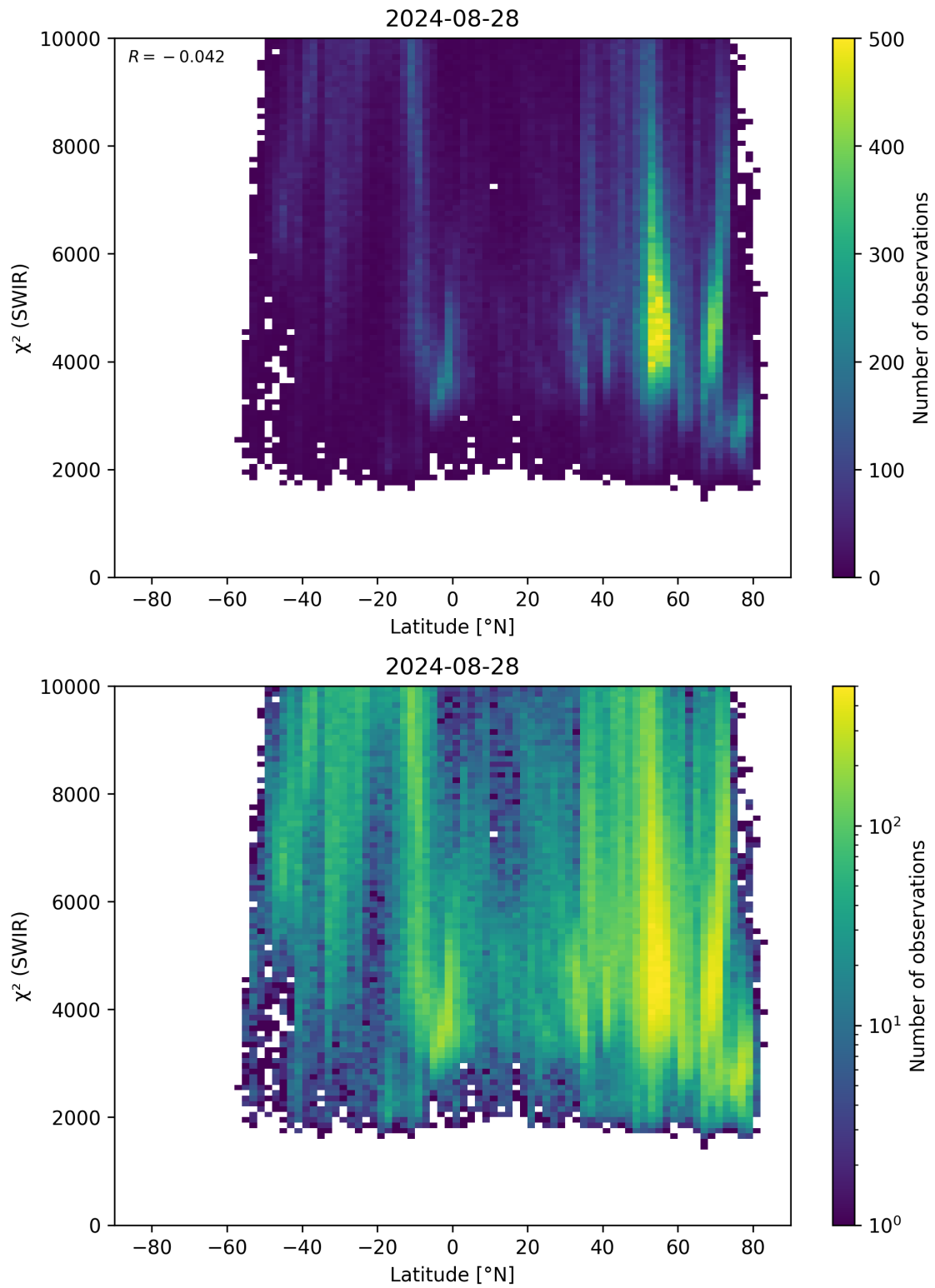
Figure 54: Scatter density plot of “Latitude” against “ \chi^2 (SWIR)” for 2024-08-27 to 2024-08-29.
