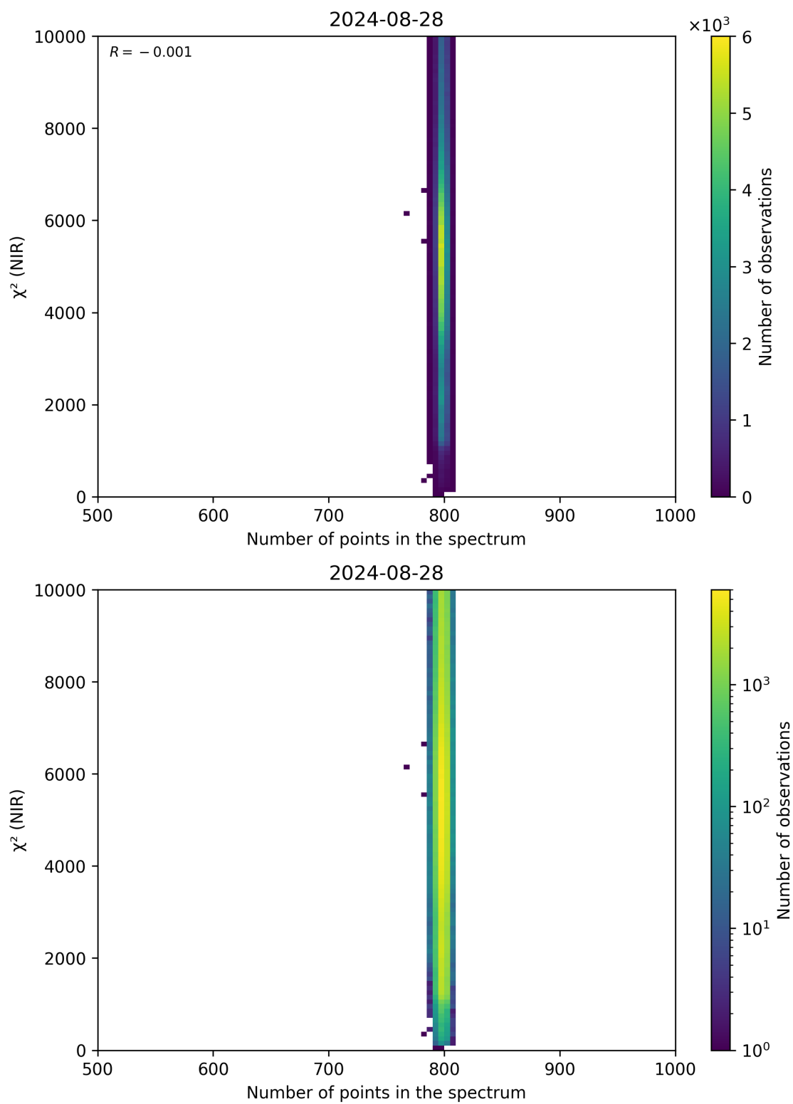
Figure 88: Scatter density plot of “Number of points in the spectrum” against “ \chi^2 (NIR)” for 2024-08-27 to 2024-08-29.
