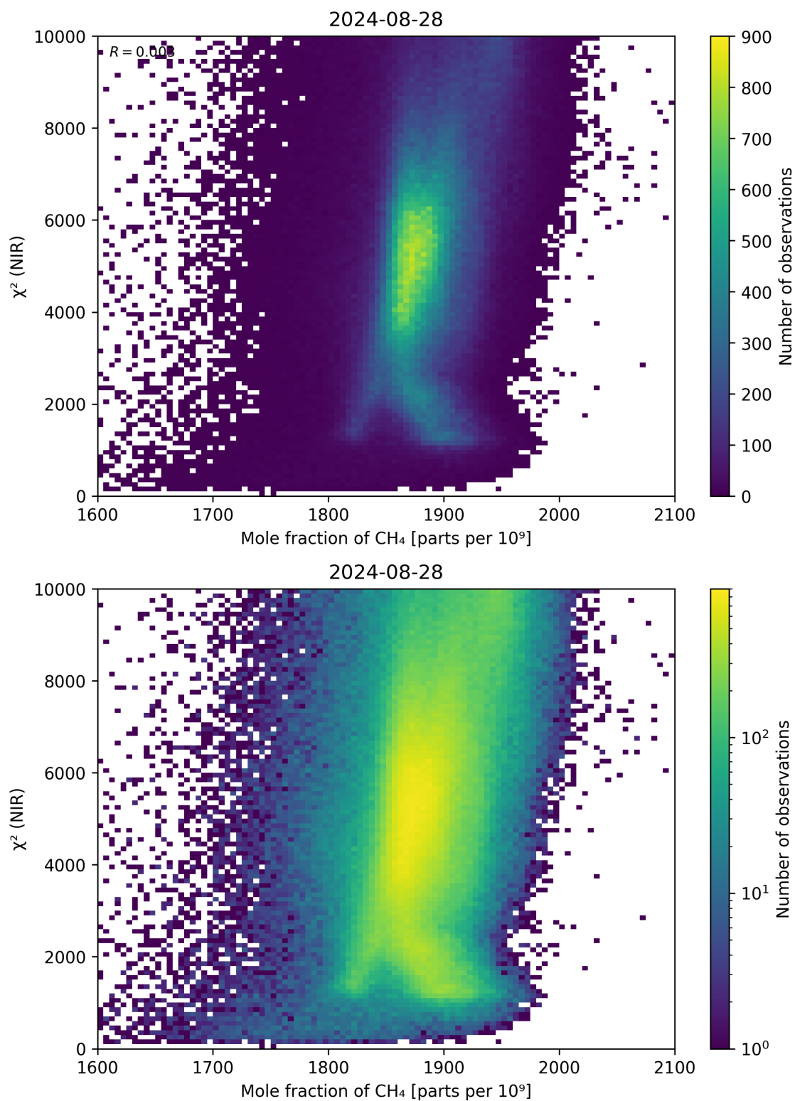
Figure 70: Scatter density plot of “Mole fraction of \text{CH}_4 ” against “ \chi^2 (NIR)” for 2024-08-27 to 2024-08-29.
