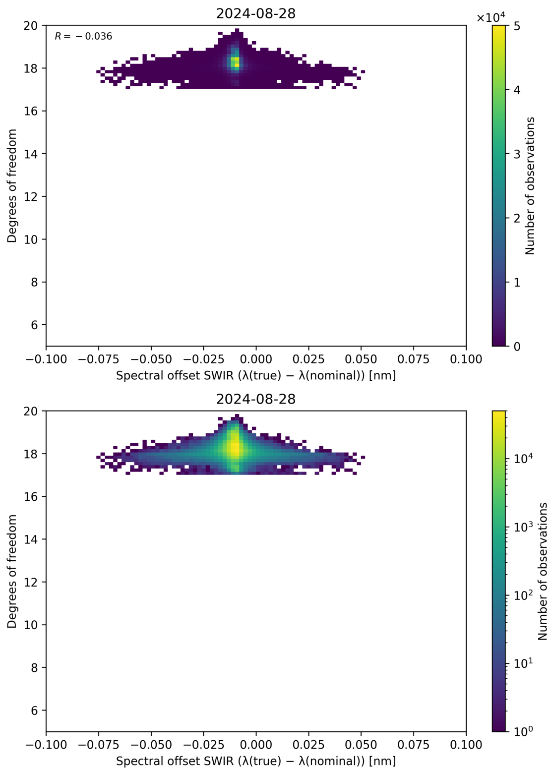
Figure 119: Scatter density plot of “Spectral offset SWIR ( \lambda_{\text{true}} - \lambda_{\text{nominal}} )” against “Degrees of freedom” for 2024-08-27 to 2024-08-29.
