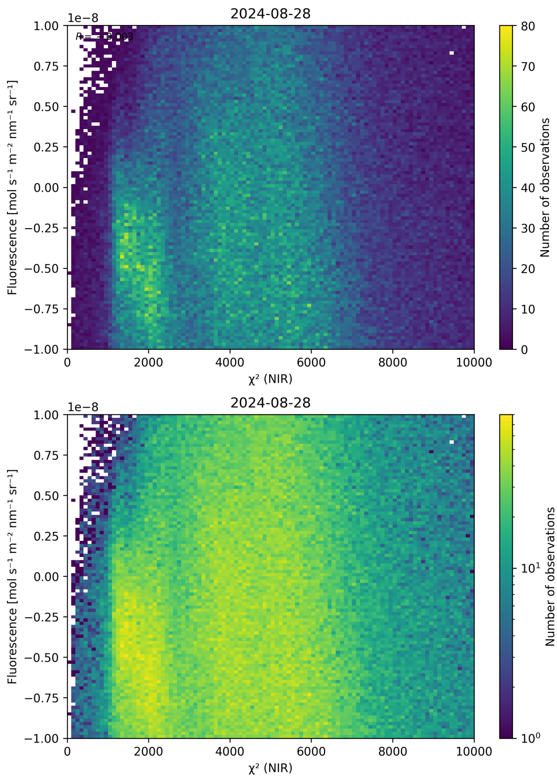
Figure 45: Scatter density plot of “ \chi^2 (NIR)” against “Fluorescence” for 2024-08-27 to 2024-08-29.
