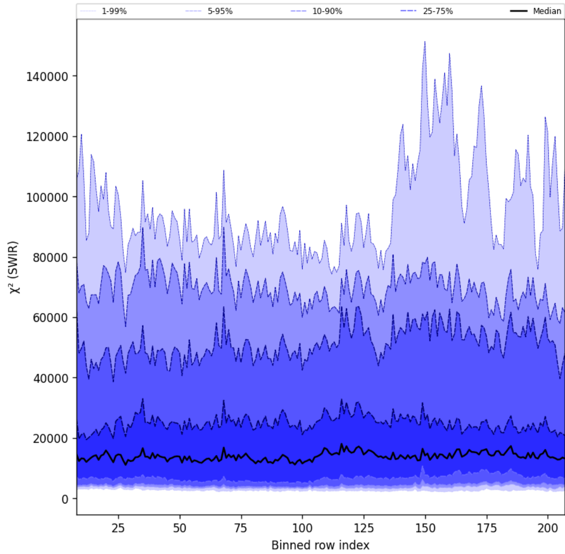
Figure 39: Along track statistics of “ \chi^2 (SWIR)” for 2024-08-27 to 2024-08-29
