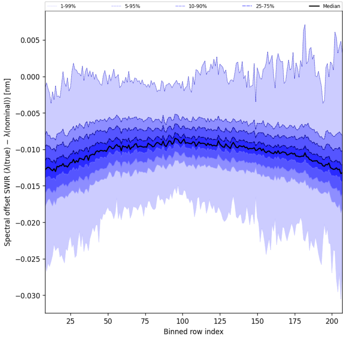
Figure 38: Along track statistics of “Spectral offset SWIR ( \lambda_{\text{true}} - \lambda_{\text{nominal}} )” for 2024-08-27 to 2024-08-29
