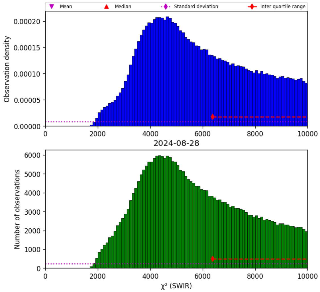
Figure 28: Histogram of " \chi^2 (SWIR)" for 2024-08-27 to 2024-08-29
