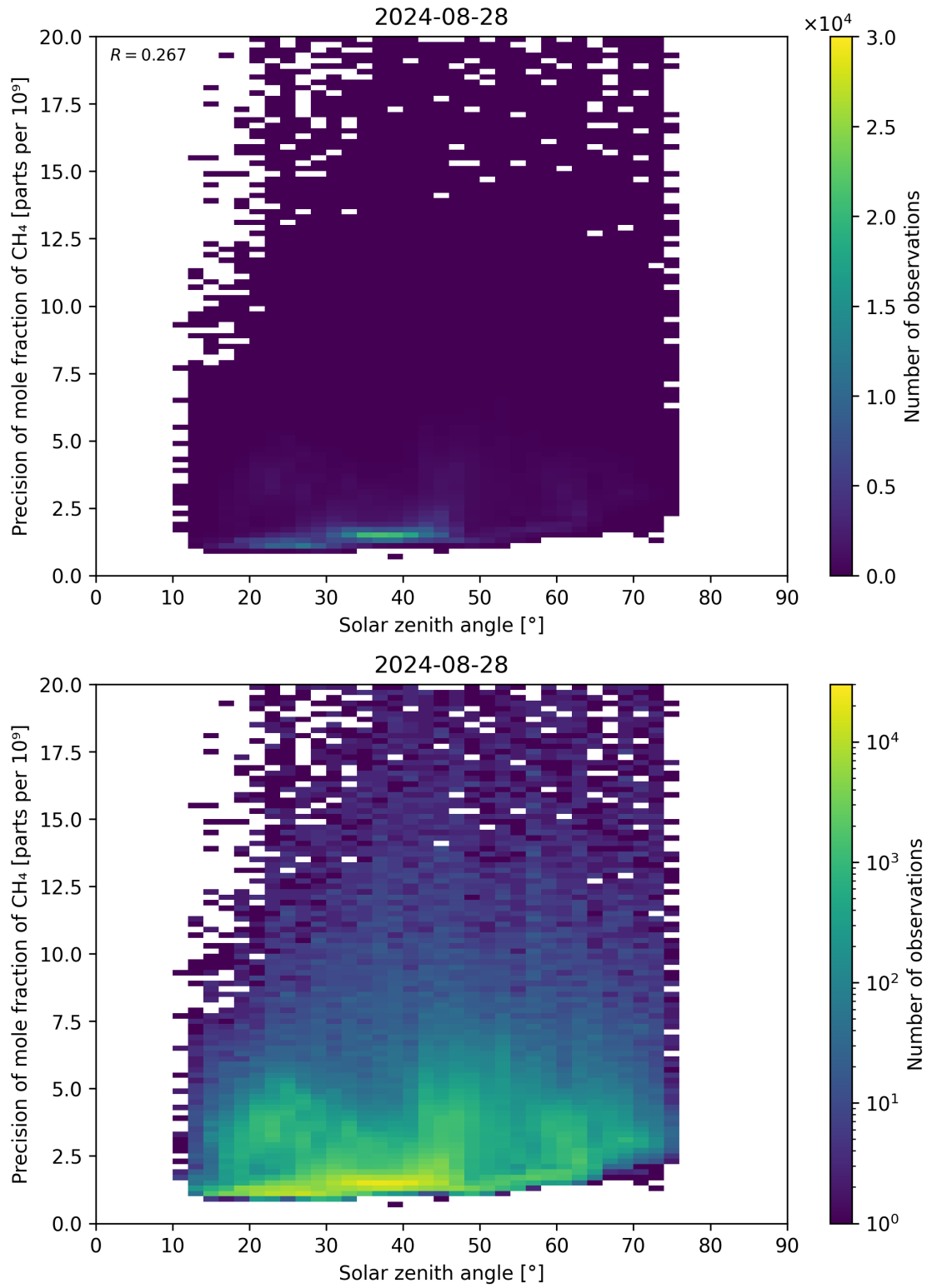
Figure 101: Scatter density plot of “Solar zenith angle” against “Precision of mole fraction of \text{CH}_4 ” for 2024-08-27 to 2024-08-29.
