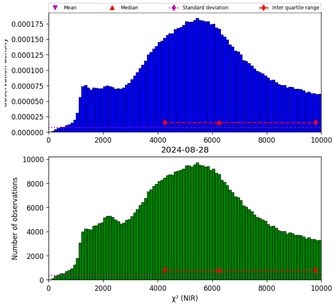
Figure 29: Histogram of “ \chi^2 (NIR)” for 2024-08-27 to 2024-08-29
