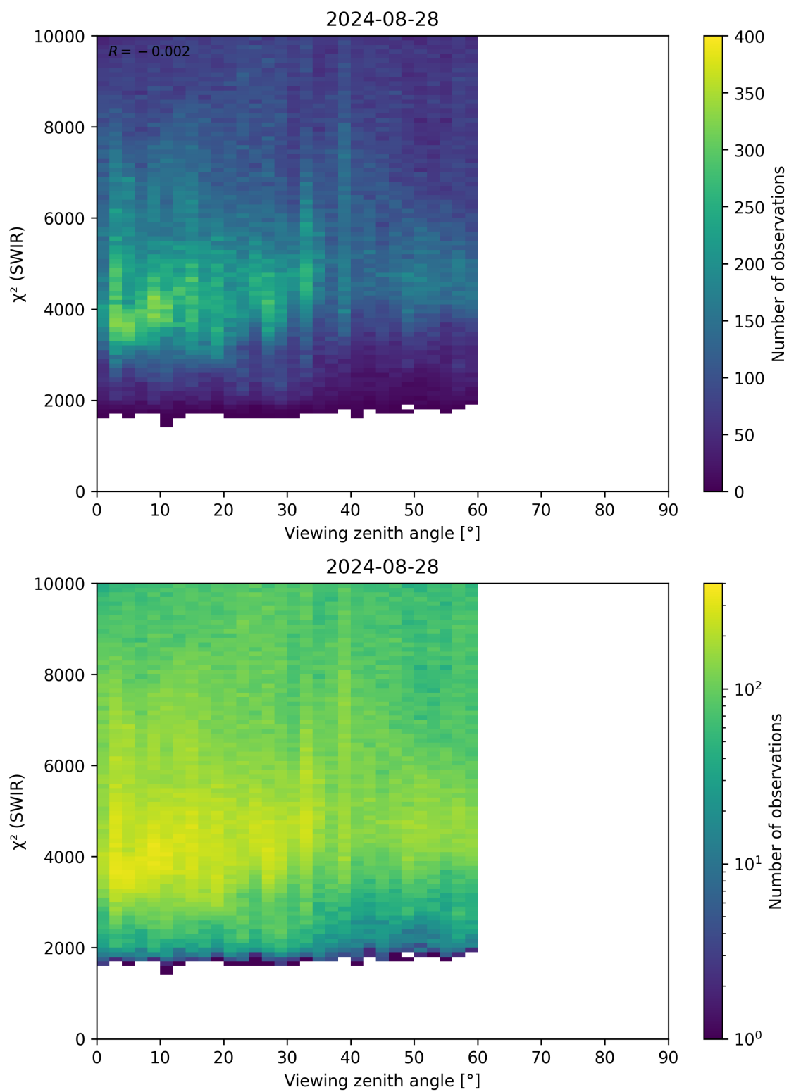
Figure 106: Scatter density plot of “Viewing zenith angle” against “ \chi^2 (SWIR)” for 2024-08-27 to 2024-08-29.
