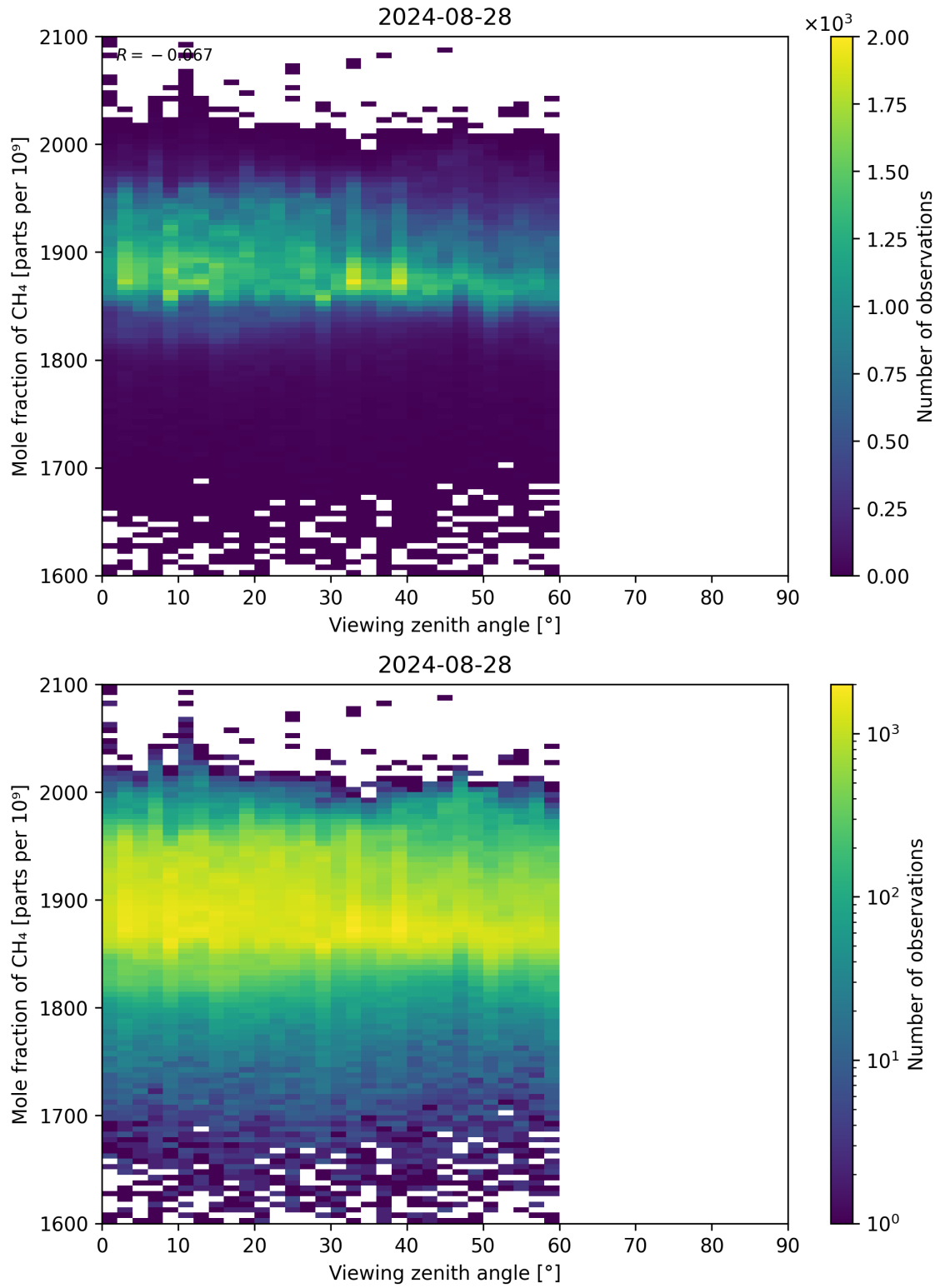
Figure 110: Scatter density plot of “Viewing zenith angle” against “Mole fraction of CH 4 ” for 2024-08-27 to 2024-08-29.
