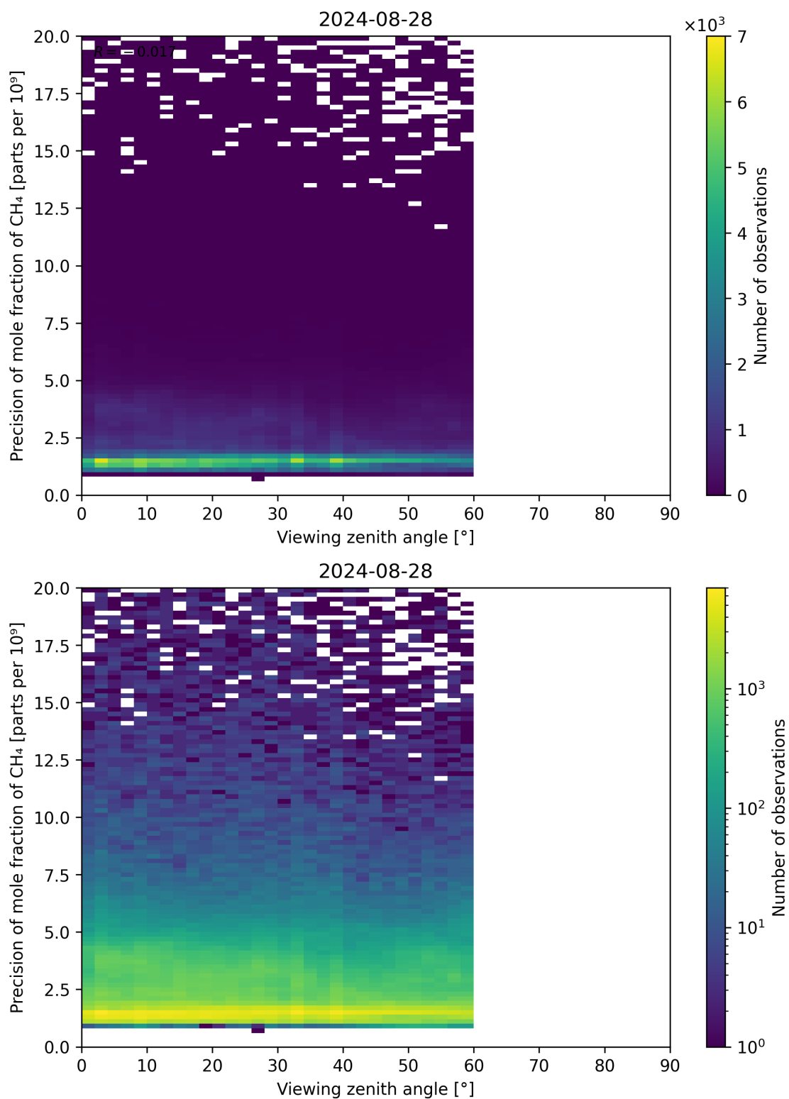
Figure 112: Scatter density plot of “Viewing zenith angle” against “Precision of mole fraction of CH 4 ” for 2024-08-27 to 2024-08-29.
