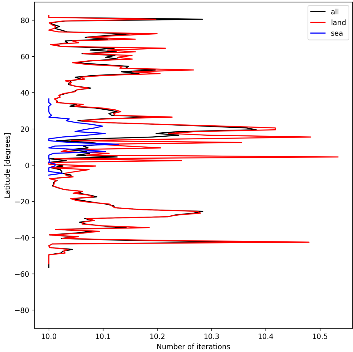
Figure 20: Zonal average of “Number of iterations” for 2024-08-27 to 2024-08-29.
