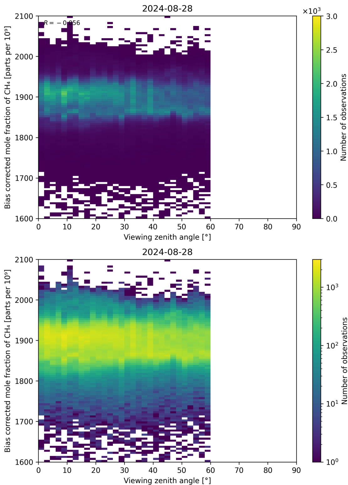
Figure 111: Scatter density plot of “Viewing zenith angle” against “Bias corrected mole fraction of CH 4 ” for 2024-08-27 to 2024-08-29.
