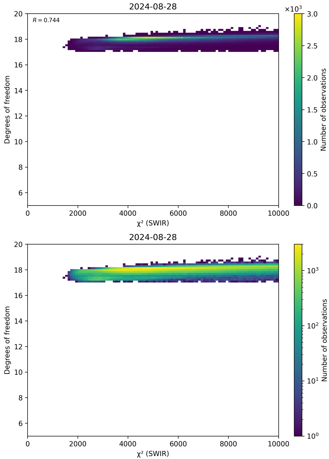
Figure 48: Scatter density plot of “ \chi^2 (SWIR)” against “Degrees of freedom” for 2024-08-27 to 2024-08-29.
