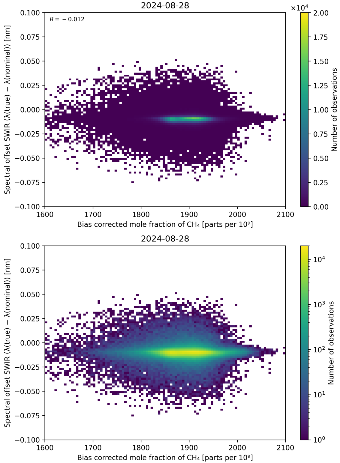
Figure 69: Scatter density plot of “Bias corrected mole fraction of \text{CH}_4 ” against “Spectral offset SWIR ( \lambda_{\text{true}} - \lambda_{\text{nominal}} )” for 2024-08-27 to 2024-08-29.
