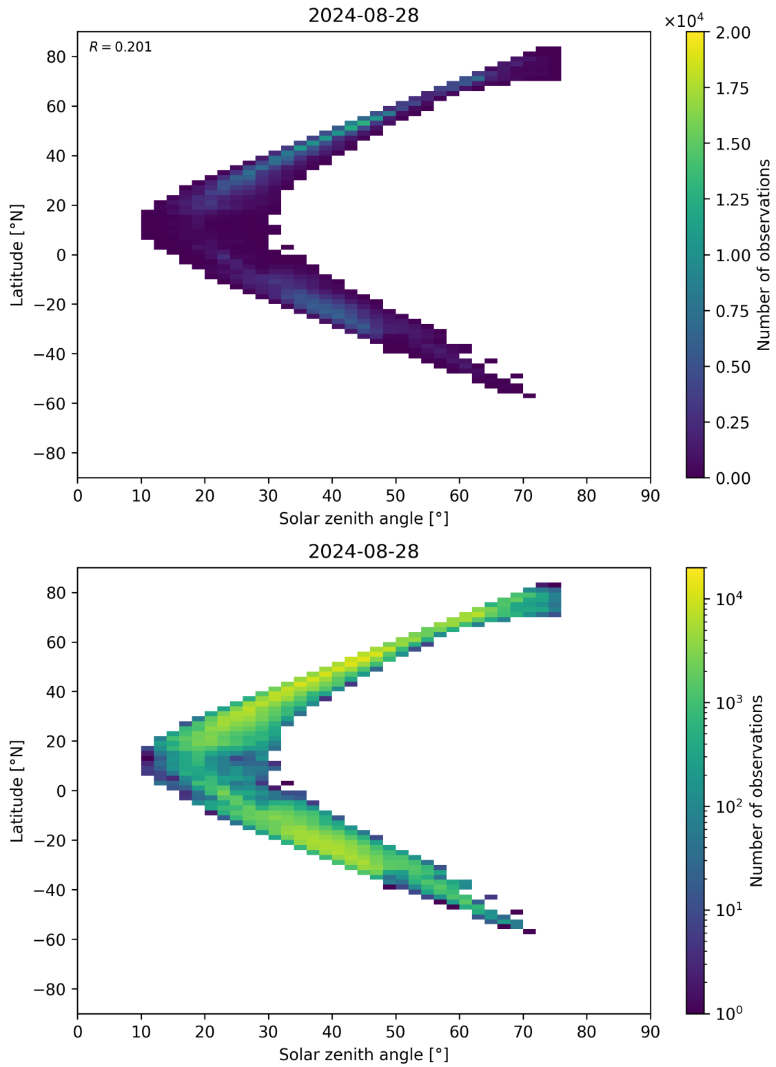
Figure 98: Scatter density plot of “Solar zenith angle” against “Latitude” for 2024-08-27 to 2024-08-29.
