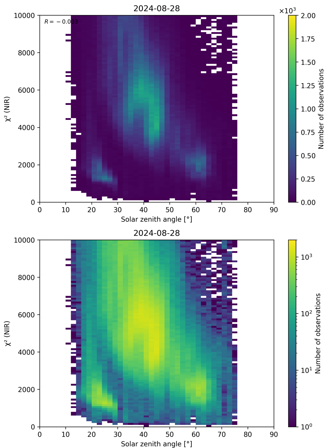
Figure 94: Scatter density plot of “Solar zenith angle” against “ \chi^2 (NIR)” for 2024-08-27 to 2024-08-29.
