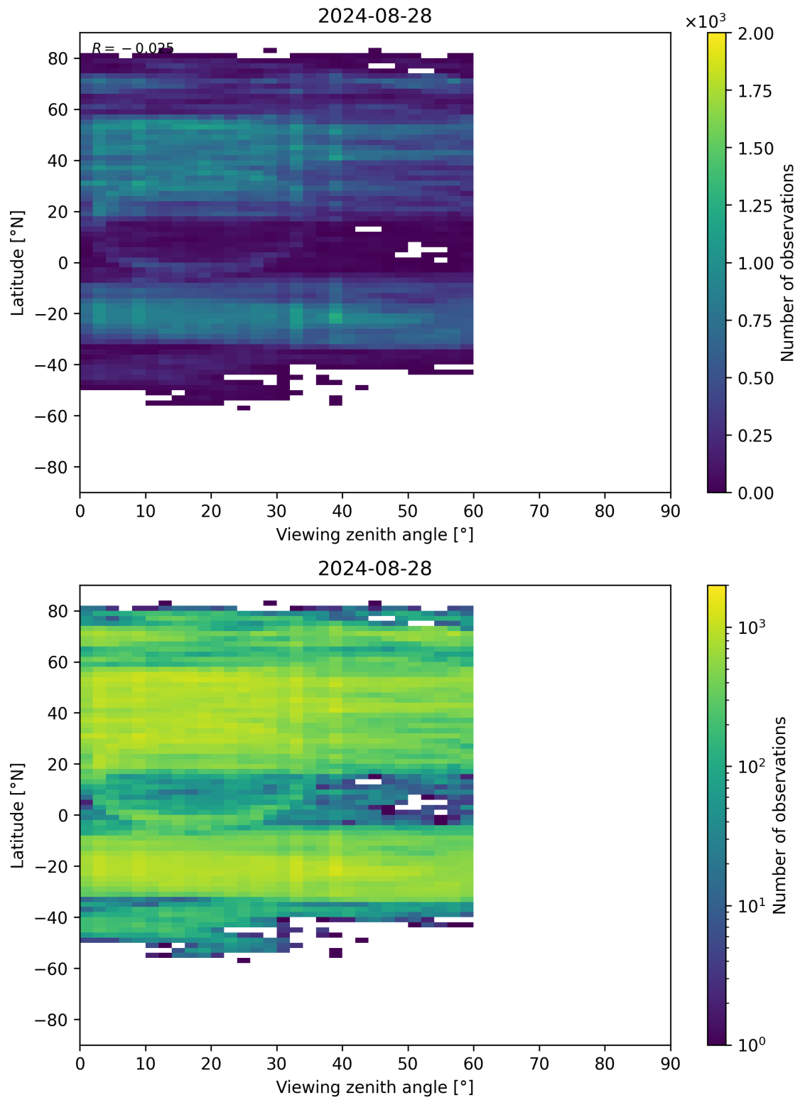
Figure 109: Scatter density plot of “Viewing zenith angle” against “Latitude” for 2024-08-27 to 2024-08-29.
