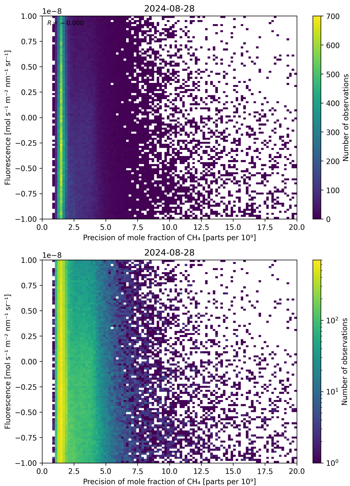
Figure 81: Scatter density plot of “Precision of mole fraction of \text{CH}_4 ” against “Fluorescence” for 2024-08-27 to 2024-08-29.
