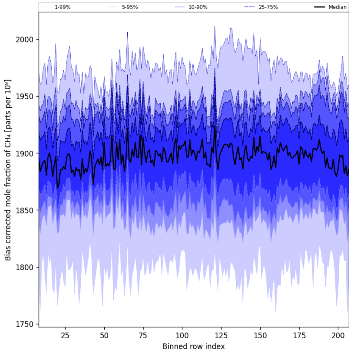
Figure 36: Along track statistics of “Bias corrected mole fraction of CH 4 ” for 2024-08-27 to 2024-08-29
