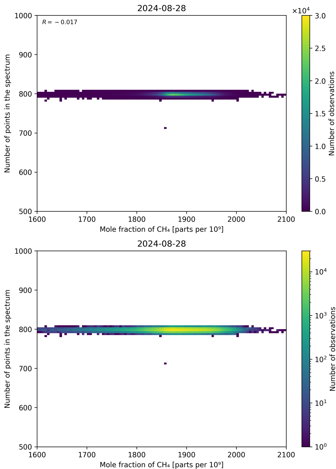
Figure 77: Scatter density plot of “Mole fraction of CH 4 ” against “Number of points in the spectrum” for 2024-08-27 to 2024-08-29.
