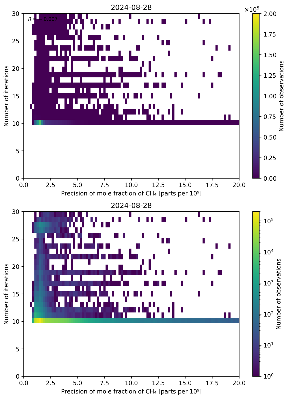
Figure 83: Scatter density plot of “Precision of mole fraction of CH 4 ” against “Number of iterations” for 2024-08-27 to 2024-08-29.
