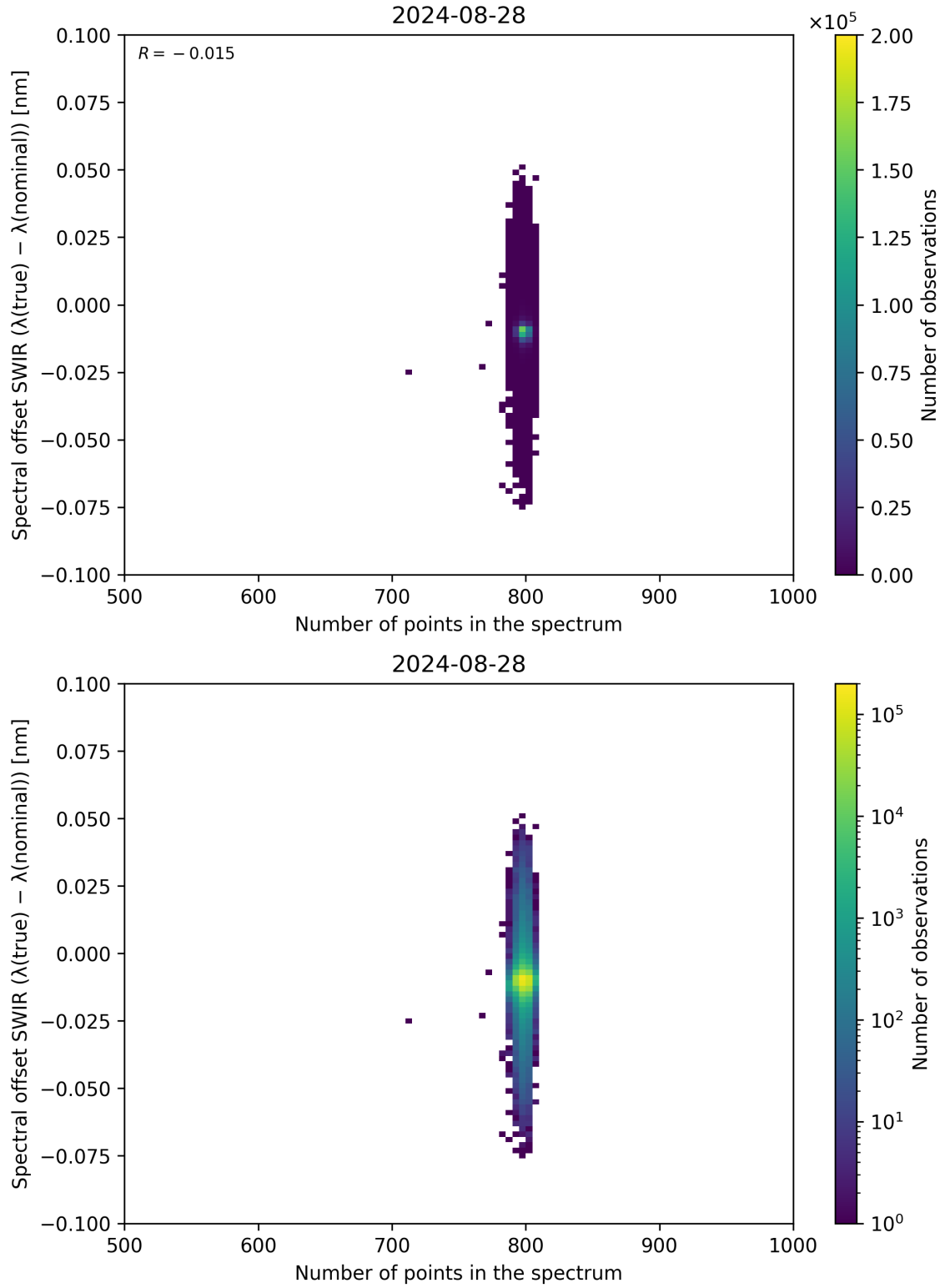
Figure 93: Scatter density plot of “Number of points in the spectrum” against “Spectral offset SWIR ( \lambda_{\text{true}} - \lambda_{\text{nominal}} )” for 2024-08-27 to 2024-08-29.
