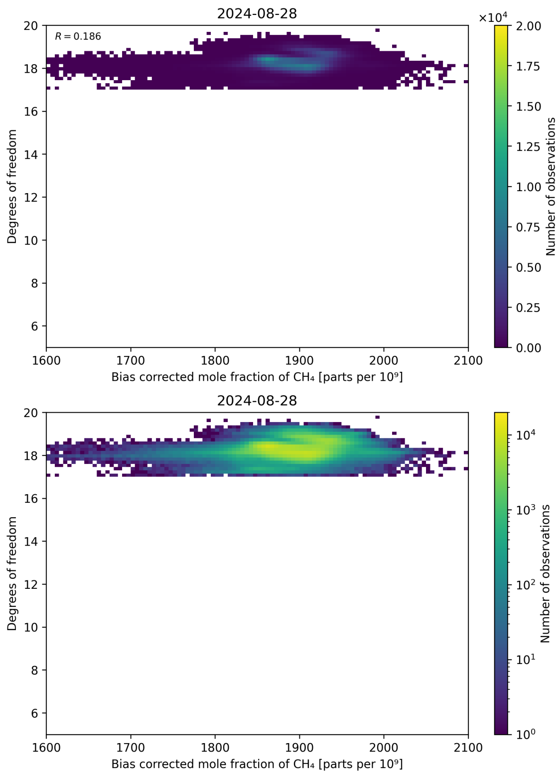
Figure 65: Scatter density plot of “Bias corrected mole fraction of CH 4 ” against “Degrees of freedom” for 2024-08-27 to 2024-08-29.
