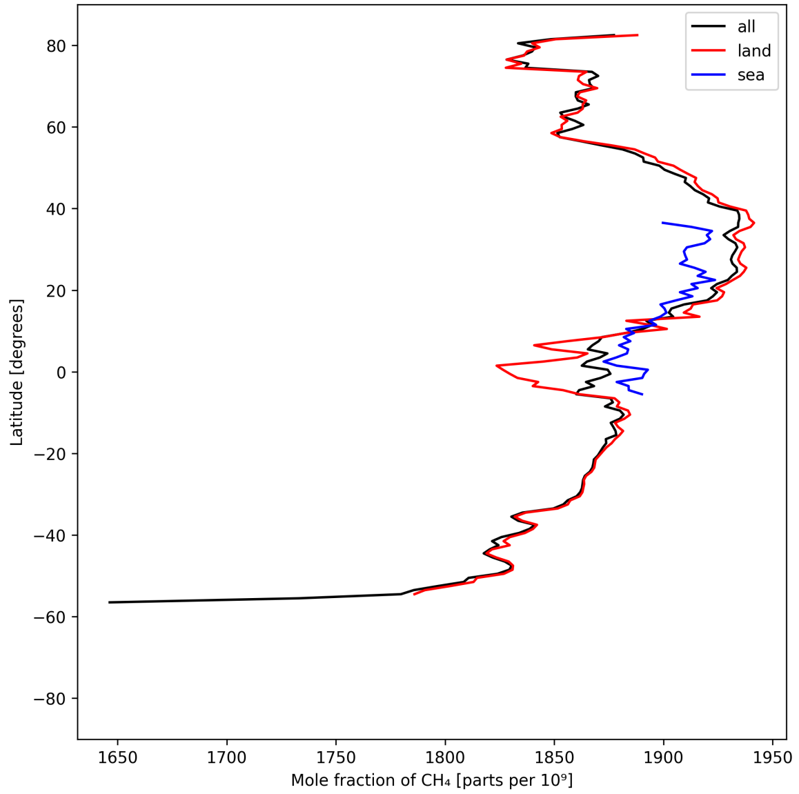
Figure 12: Zonal average of “Mole fraction of CH 4 ” for 2024-08-27 to 2024-08-29.
