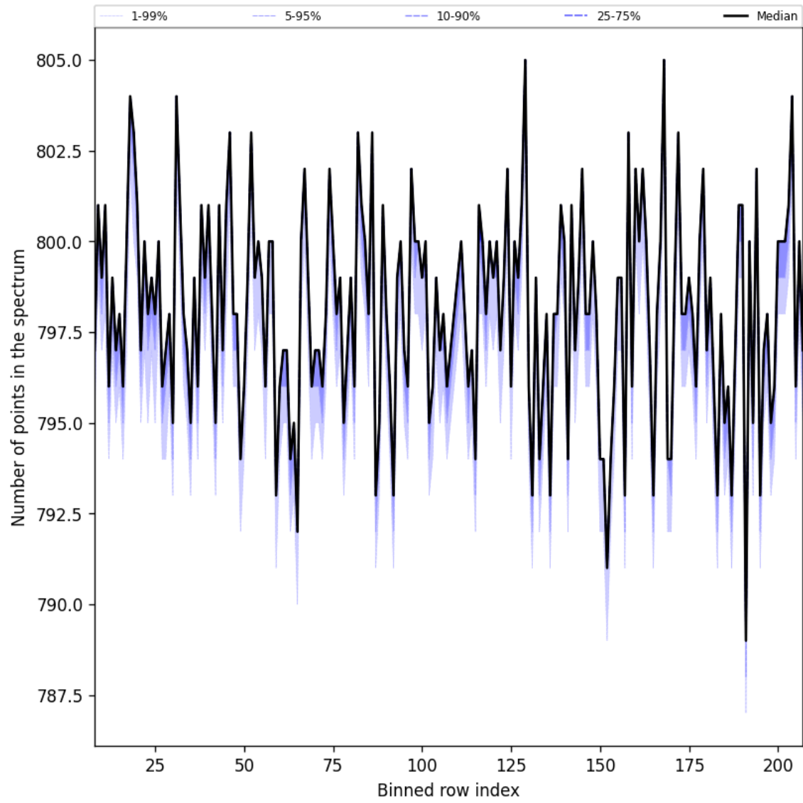
Figure 37: Along track statistics of “Number of points in the spectrum” for 2024-08-27 to 2024-08-29
