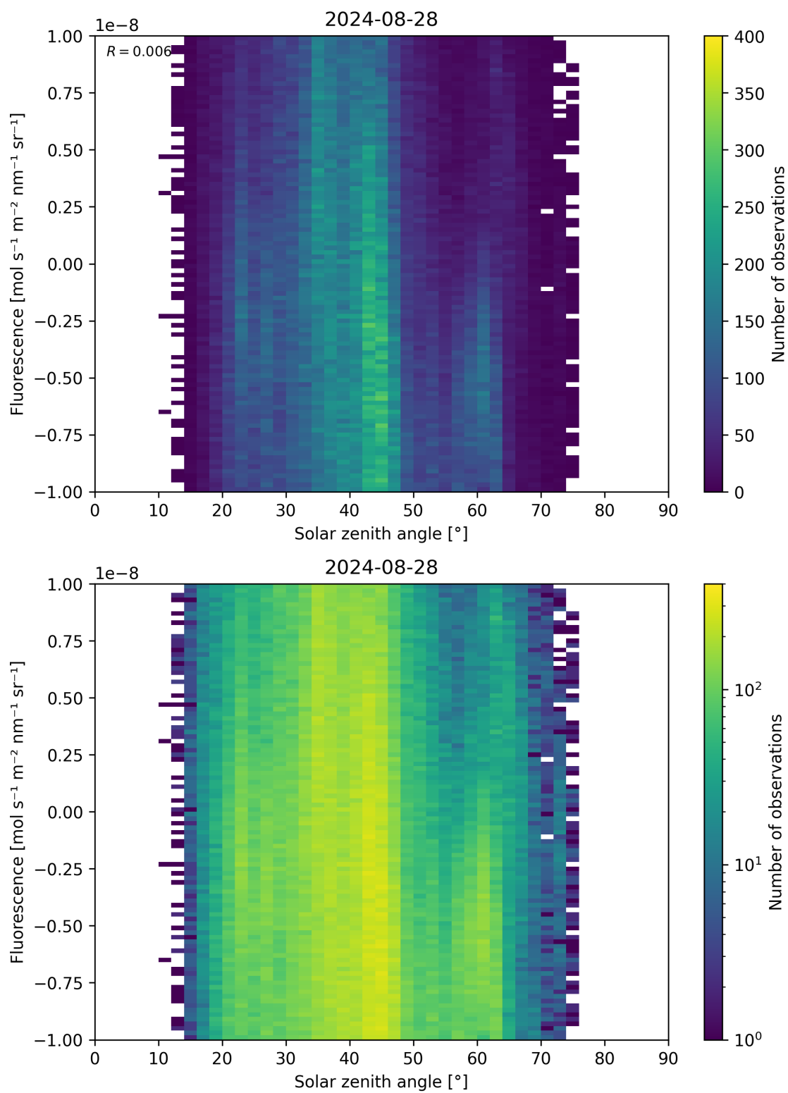
Figure 97: Scatter density plot of “Solar zenith angle” against “Fluorescence” for 2024-08-27 to 2024-08-29.
