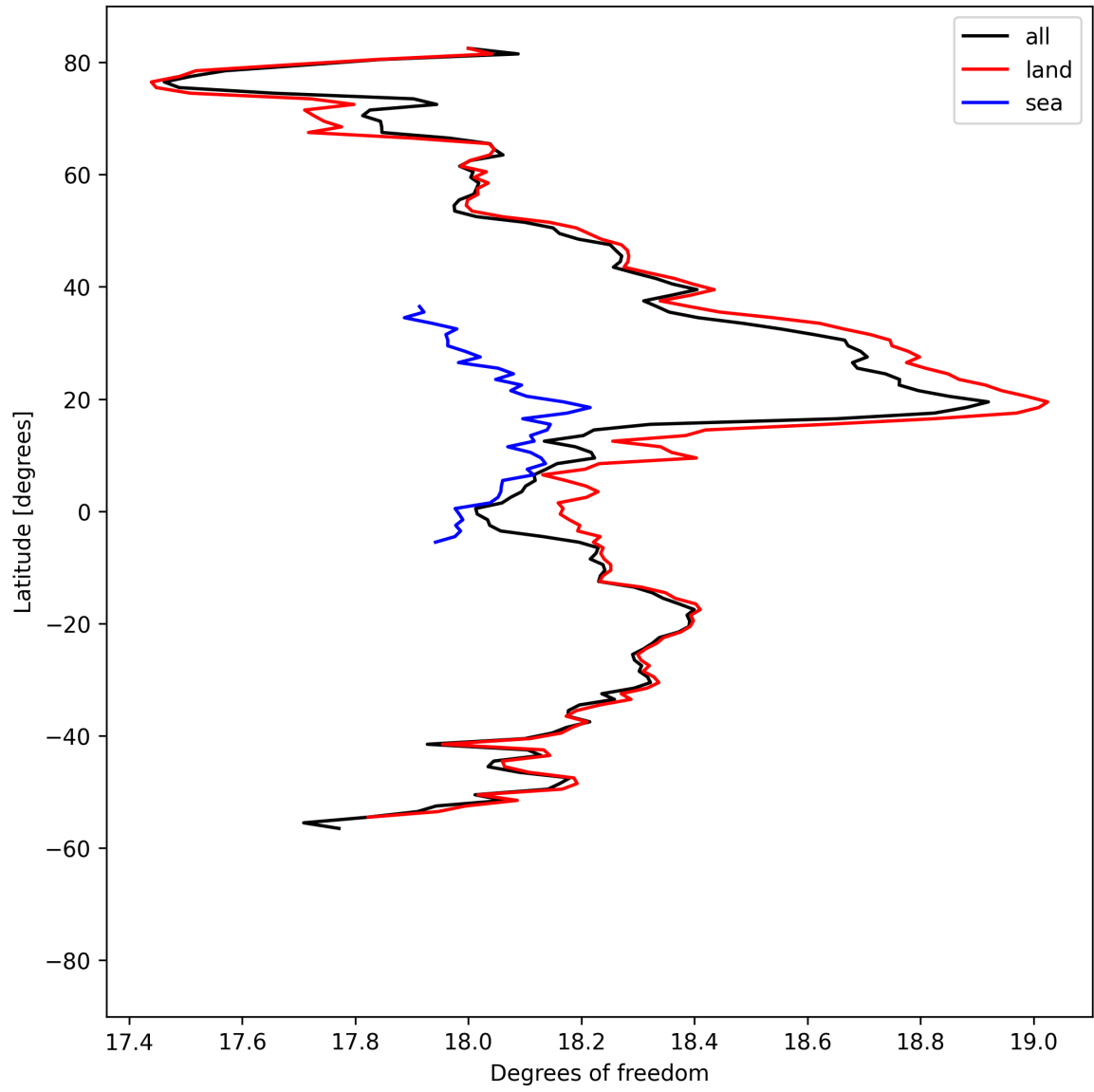
Figure 19: Zonal average of “Degrees of freedom” for 2024-08-27 to 2024-08-29.
