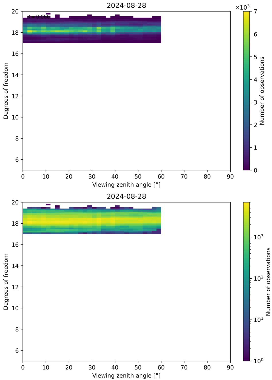
Figure 107: Scatter density plot of “Viewing zenith angle” against “Degrees of freedom” for 2024-08-27 to 2024-08-29.
