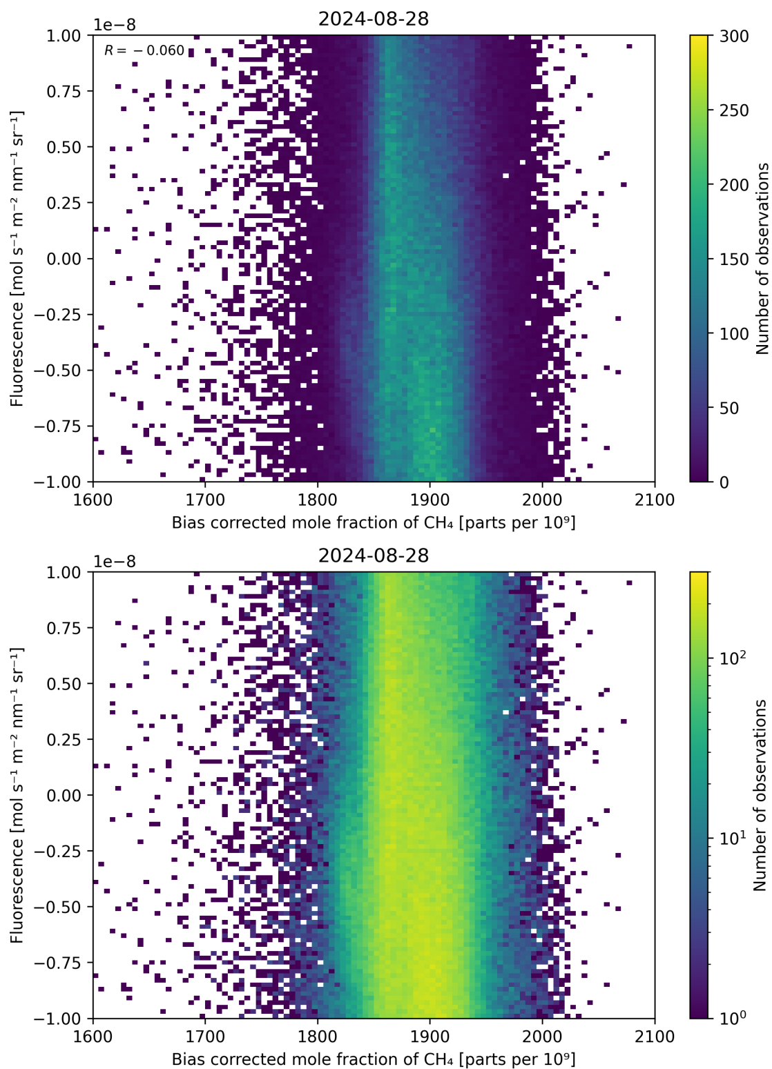
Figure 66: Scatter density plot of “Bias corrected mole fraction of \text{CH}_4 ” against “Fluorescence” for 2024-08-27 to 2024-08-29.
