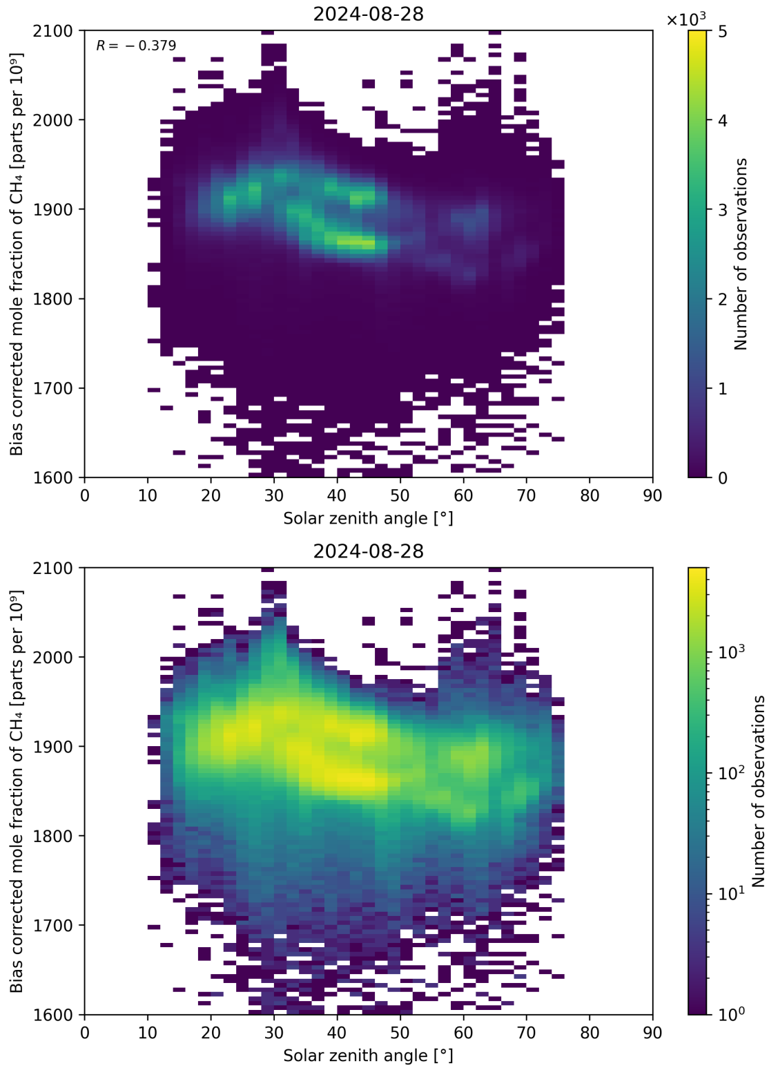
Figure 100: Scatter density plot of “Solar zenith angle” against “Bias corrected mole fraction of CH 4 ” for 2024-08-27 to 2024-08-29.
