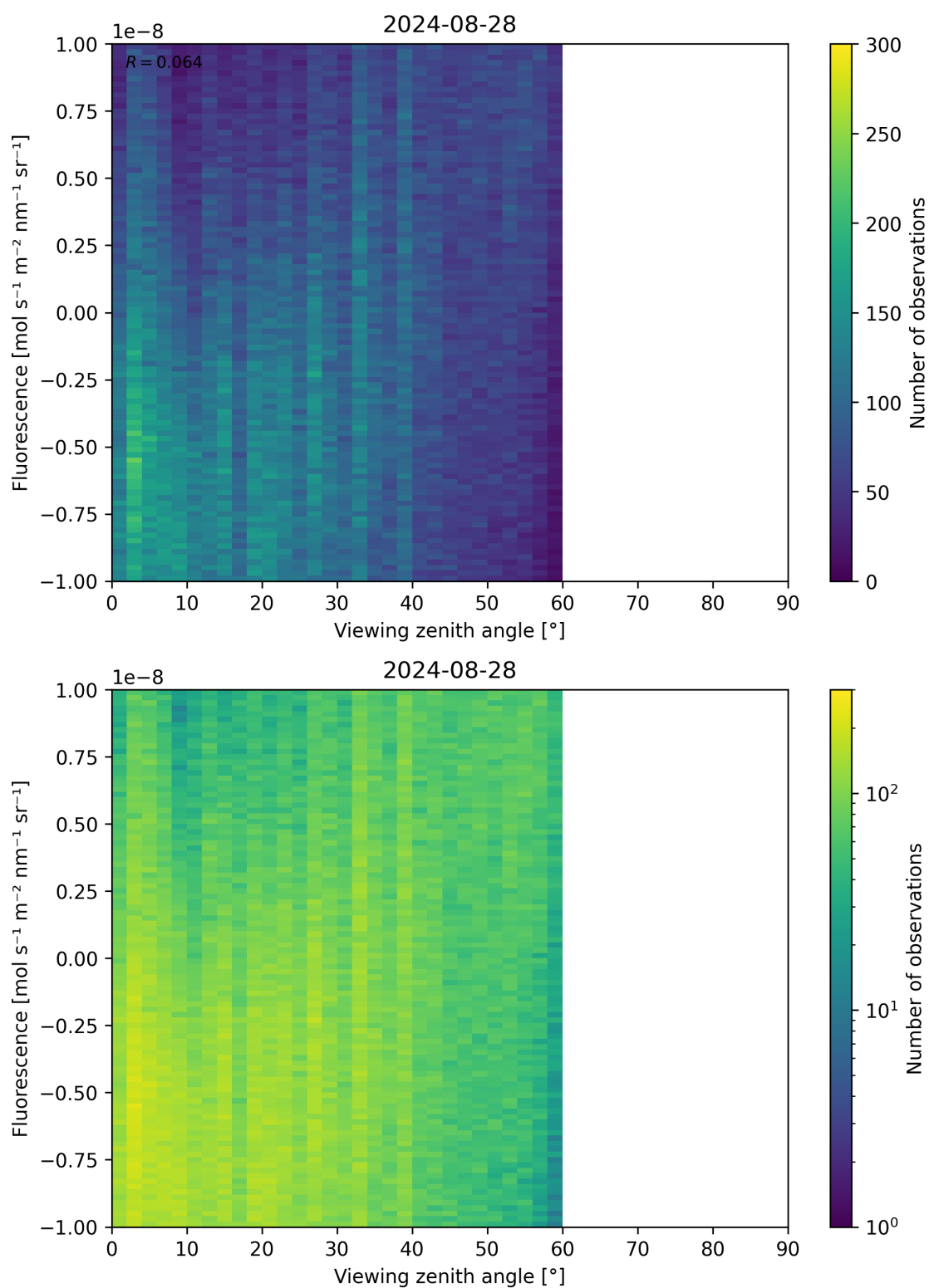
Figure 108: Scatter density plot of “Viewing zenith angle” against “Fluorescence” for 2024-08-27 to 2024-08-29.
