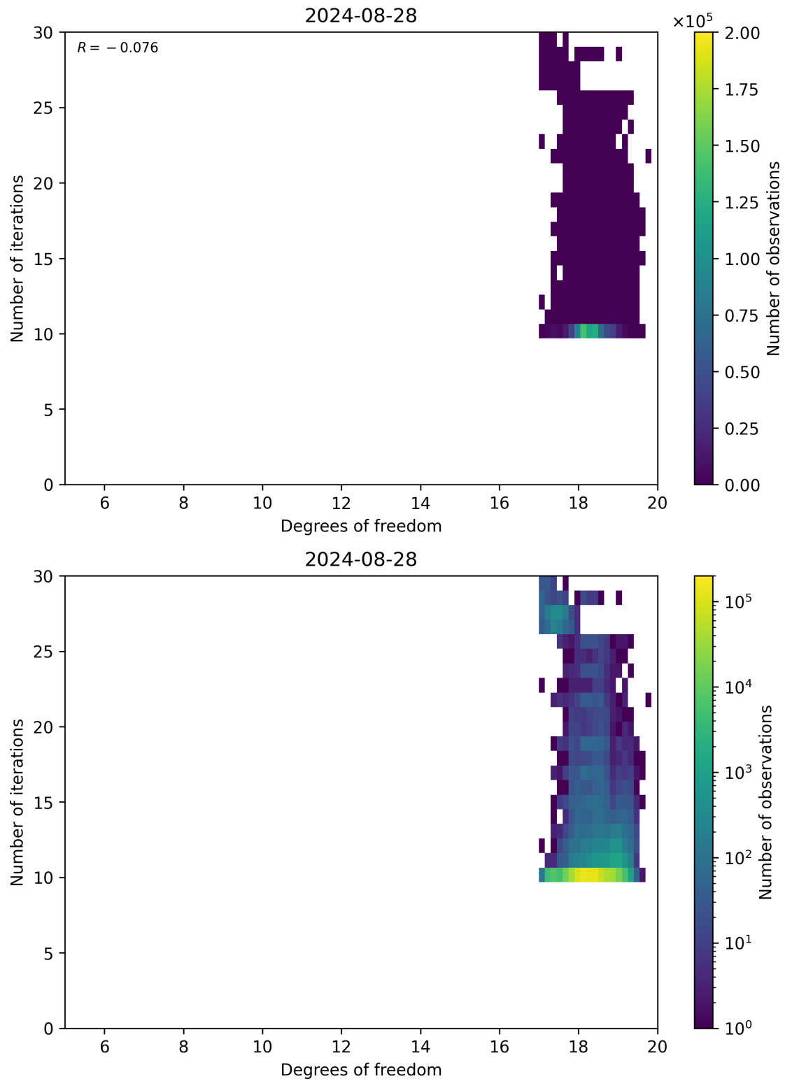
Figure 52: Scatter density plot of “Degrees of freedom” against “Number of iterations” for 2024-08-27 to 2024-08-29.
