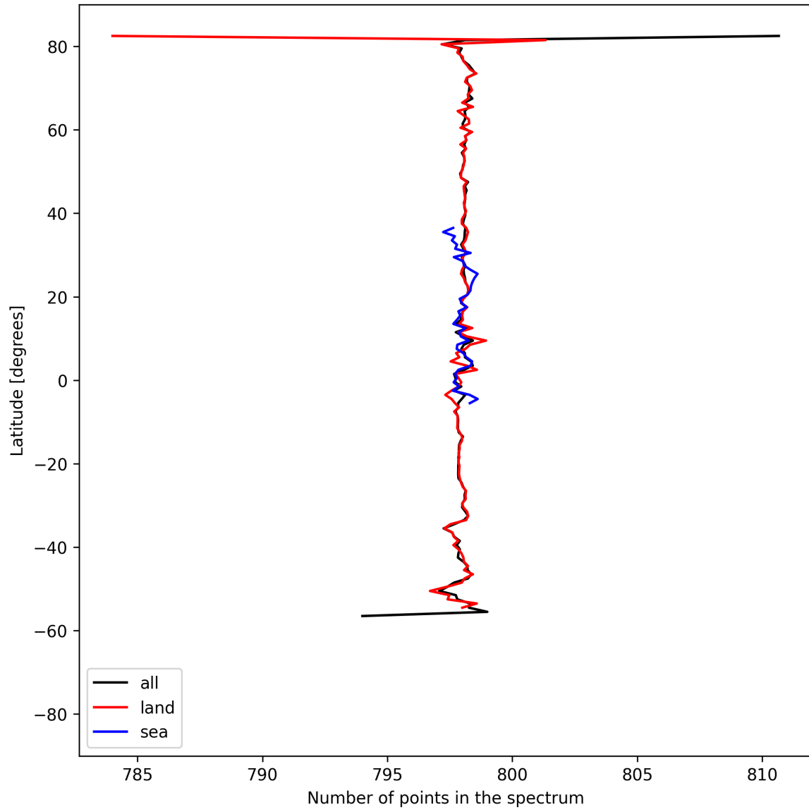
Figure 15: Zonal average of “Number of points in the spectrum” for 2024-08-27 to 2024-08-29.
