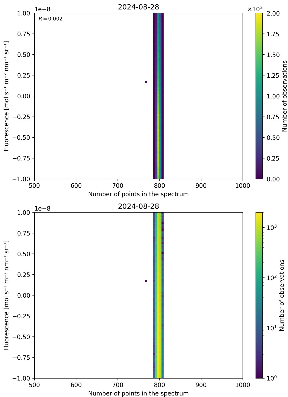
Figure 91: Scatter density plot of “Number of points in the spectrum” against “Fluorescence” for 2024-08-27 to 2024-08-29.
