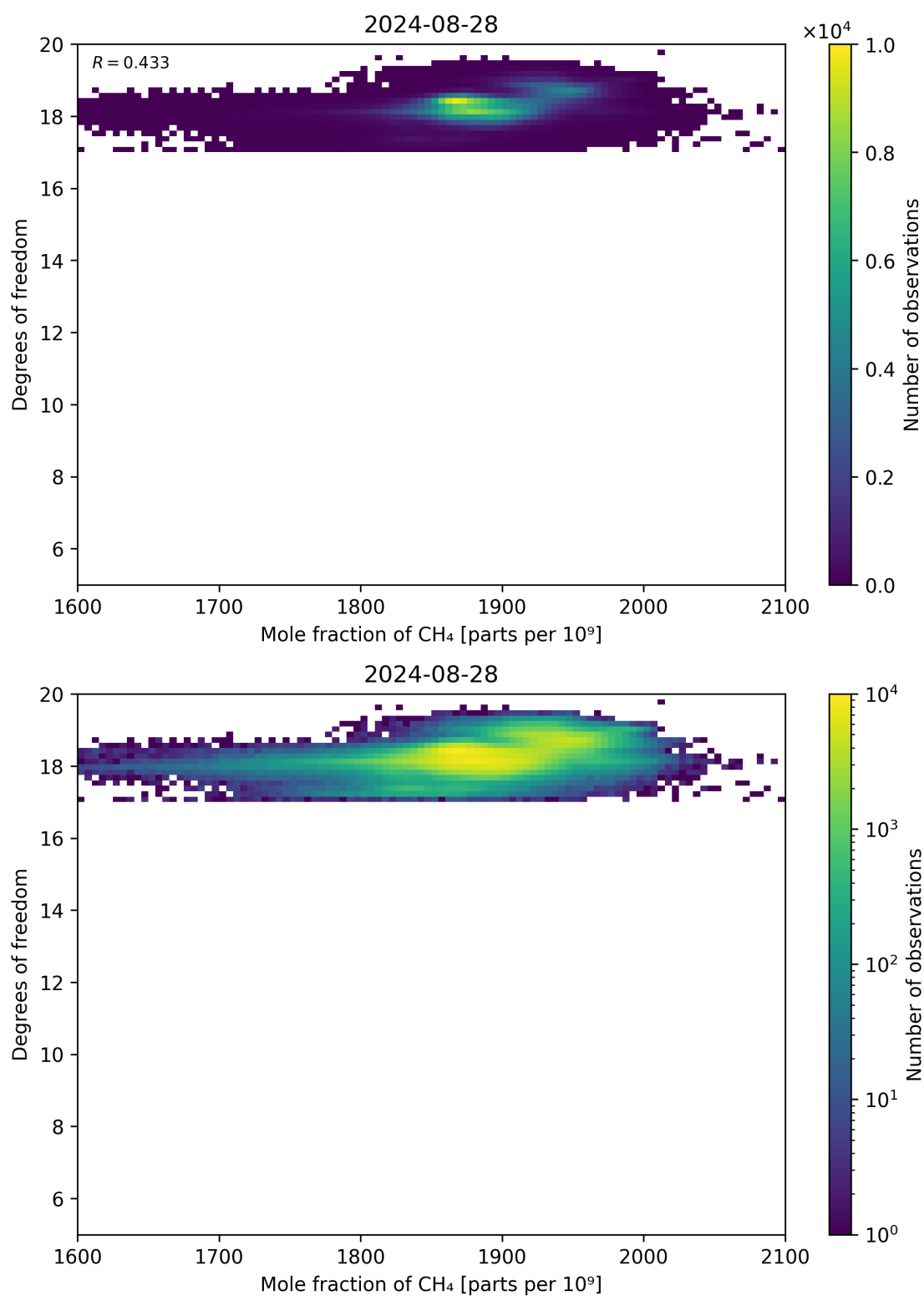
Figure 72: Scatter density plot of “Mole fraction of CH 4 ” against “Degrees of freedom” for 2024-08-27 to 2024-08-29.
