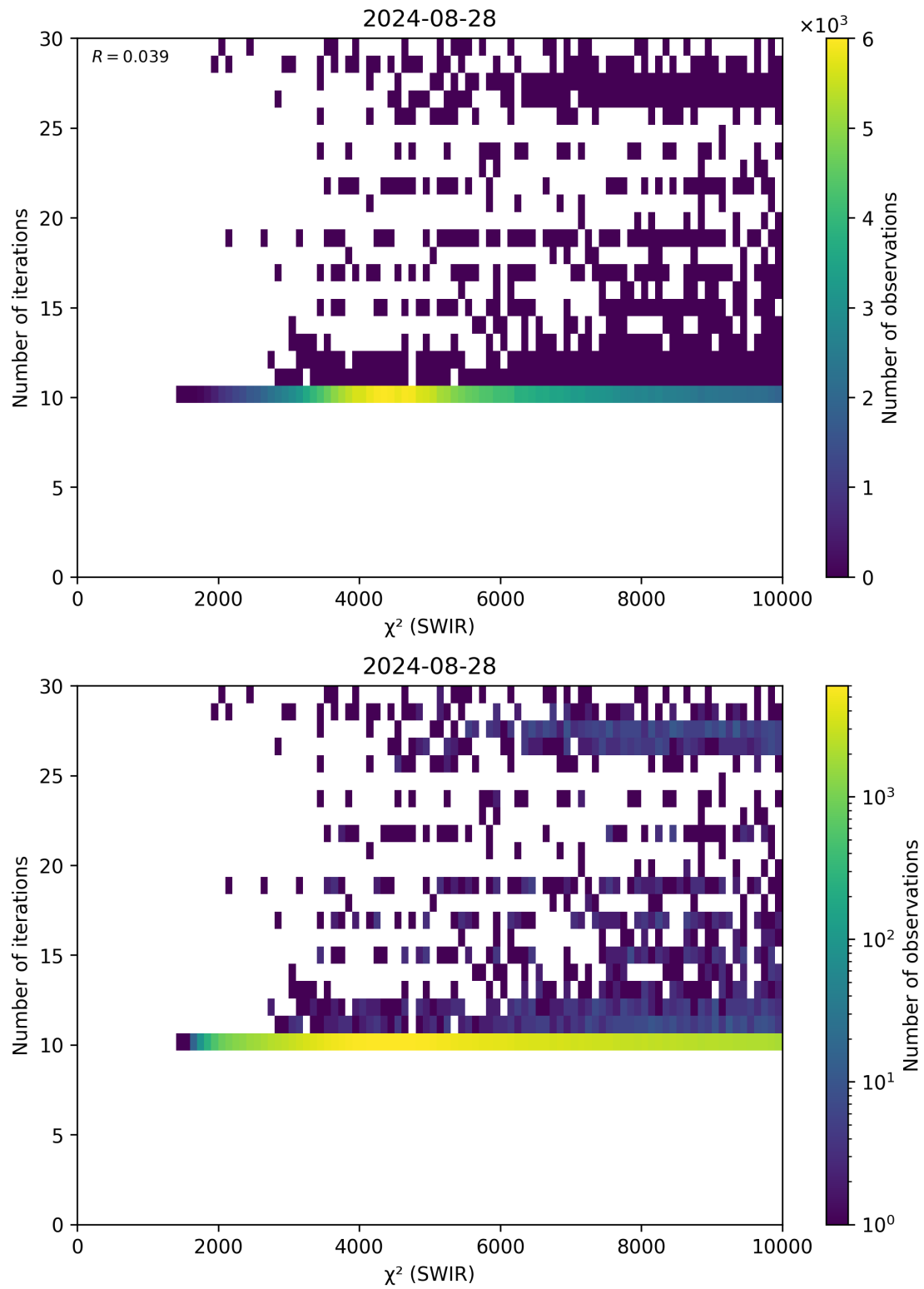
Figure 50: Scatter density plot of “ \chi^2 (SWIR)” against “Number of iterations” for 2024-08-27 to 2024-08-29.
