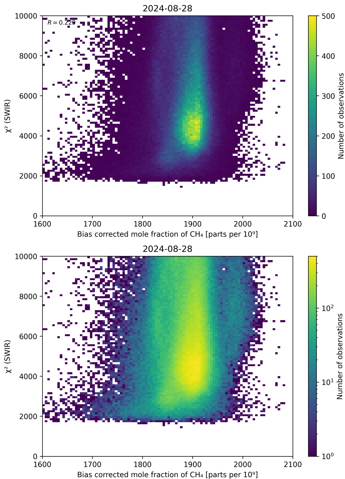
Figure 64: Scatter density plot of “Bias corrected mole fraction of \text{CH}_4 ” against “ \chi^2 (SWIR)” for 2024-08-27 to 2024-08-29.
