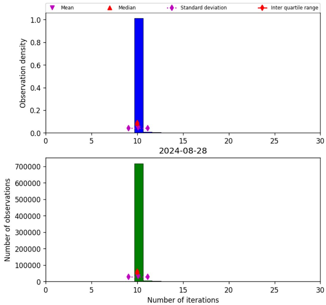
Figure 31: Histogram of “Number of iterations” for 2024-08-27 to 2024-08-29
