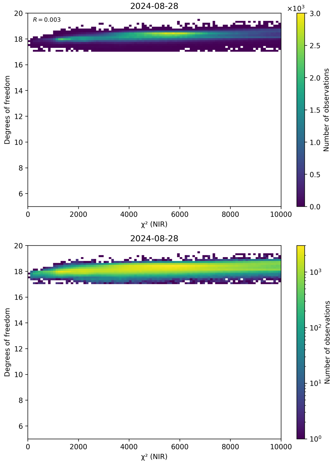
Figure 44: Scatter density plot of “ \chi^2 (NIR)” against “Degrees of freedom” for 2024-08-27 to 2024-08-29.
