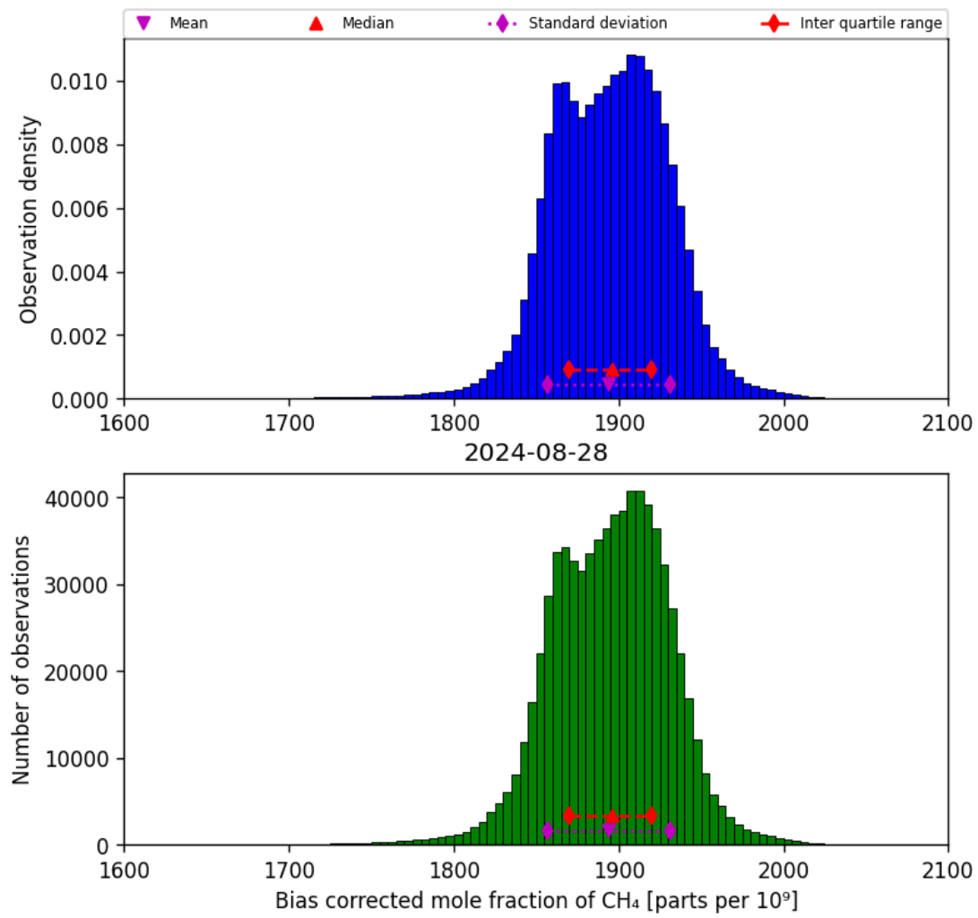
Figure 25: Histogram of “Bias corrected mole fraction of CH 4 ” for 2024-08-27 to 2024-08-29
