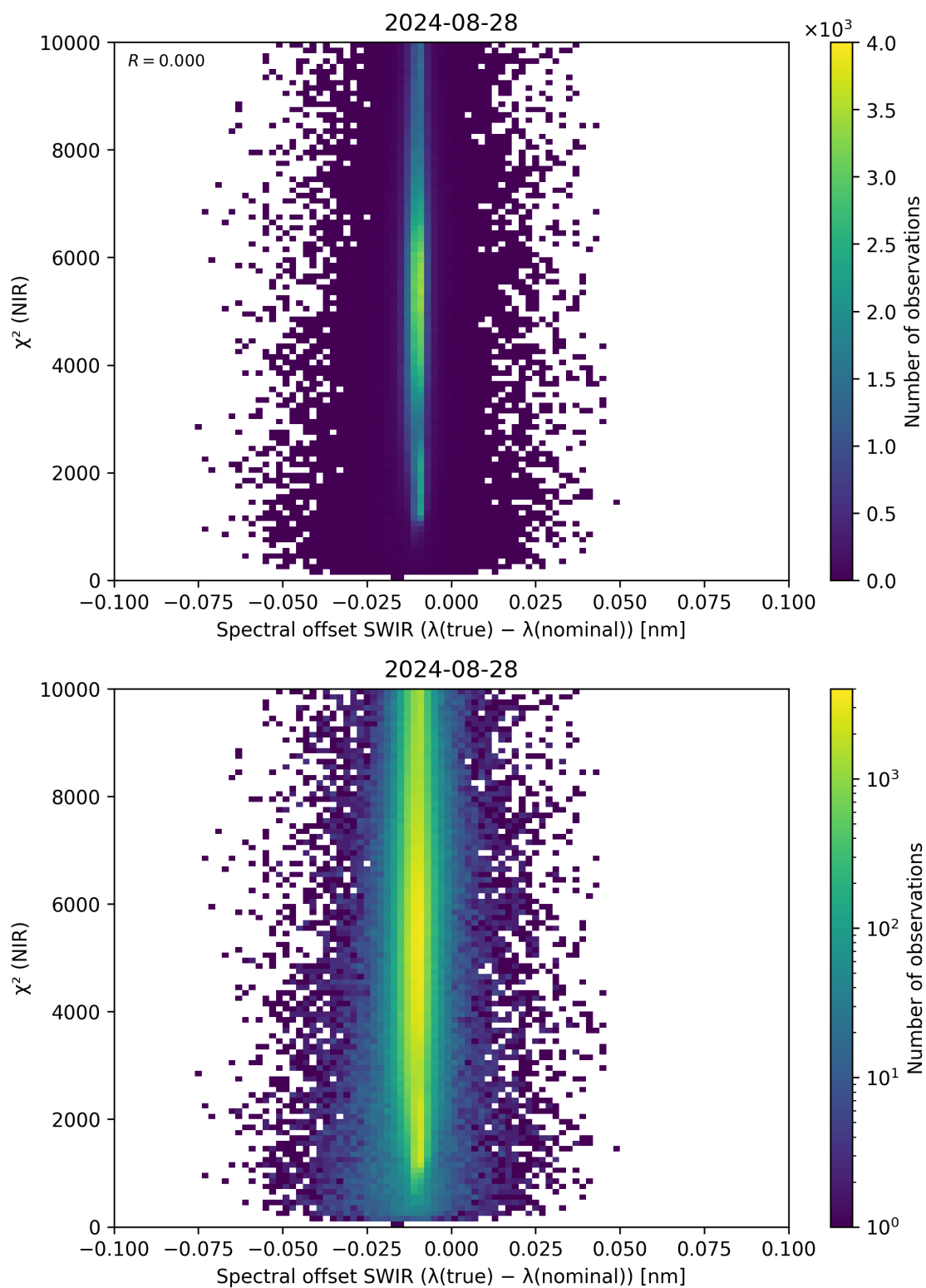
Figure 117: Scatter density plot of “Spectral offset SWIR ( \lambda_{\text{true}} - \lambda_{\text{nominal}} )” against “ \chi^2 (NIR)” for 2024-08-27 to 2024-08-29.
