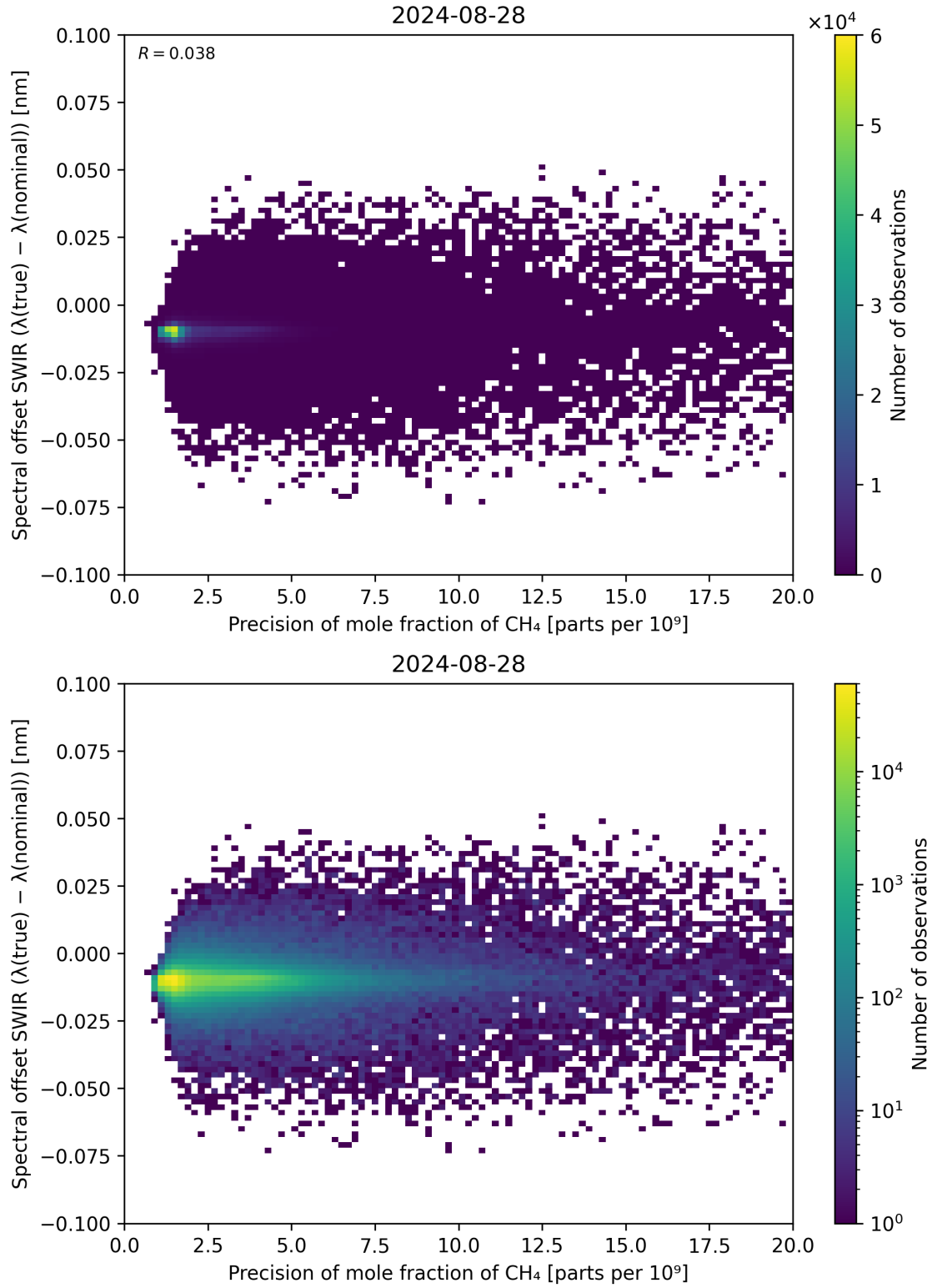
Figure 85: Scatter density plot of “Precision of mole fraction of \text{CH}_4 ” against “Spectral offset SWIR ( \lambda_{\text{true}} - \lambda_{\text{nominal}} )” for 2024-08-27 to 2024-08-29.
