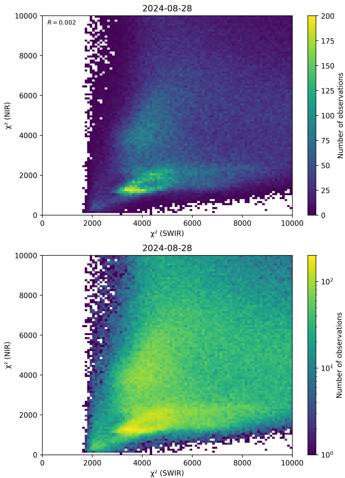
Figure 47: Scatter density plot of “ \chi^2 (SWIR)” against “ \chi^2 (NIR)” for 2024-08-27 to 2024-08-29.
