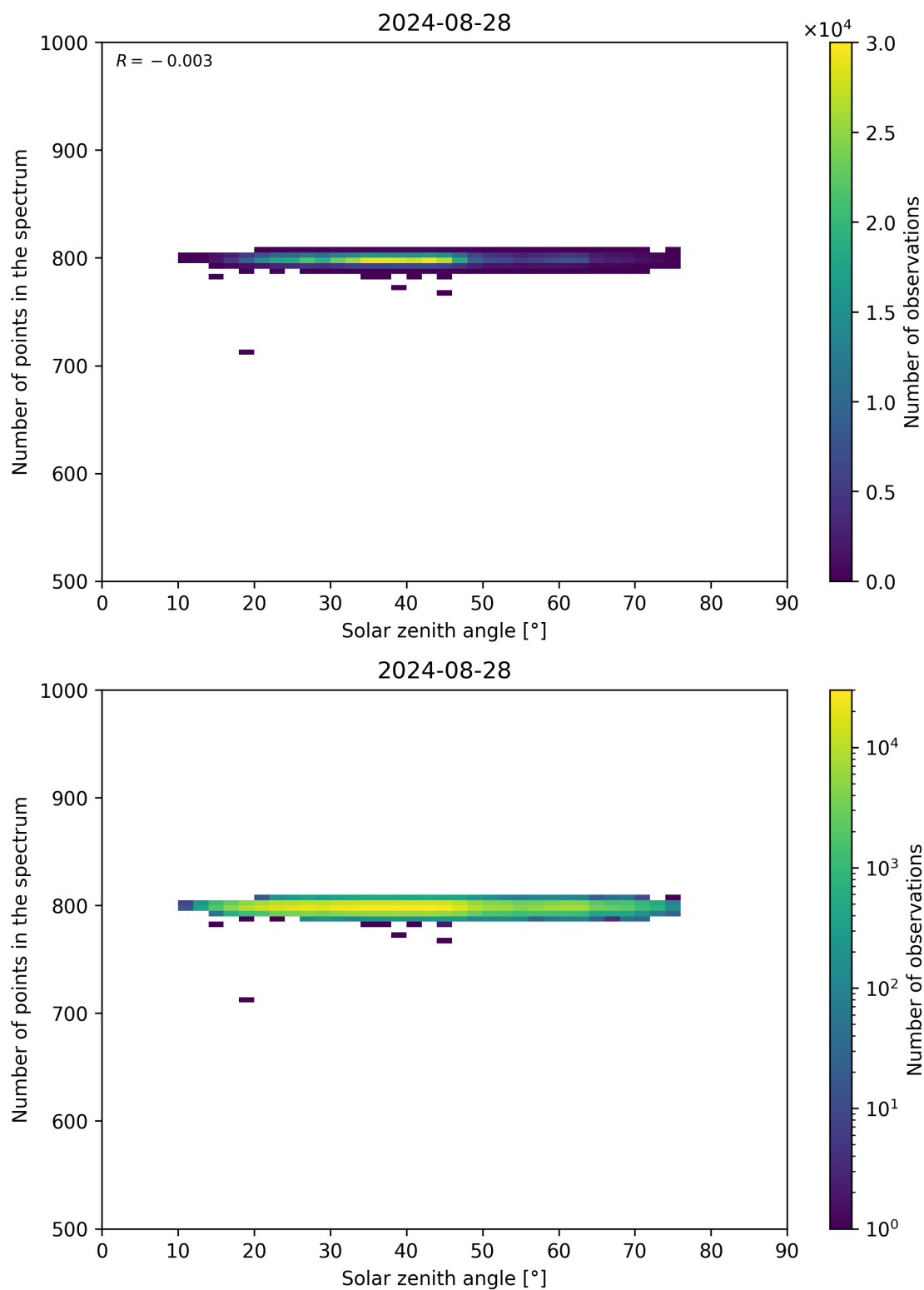
Figure 103: Scatter density plot of “Solar zenith angle” against “Number of points in the spectrum” for 2024-08-27 to 2024-08-29.
