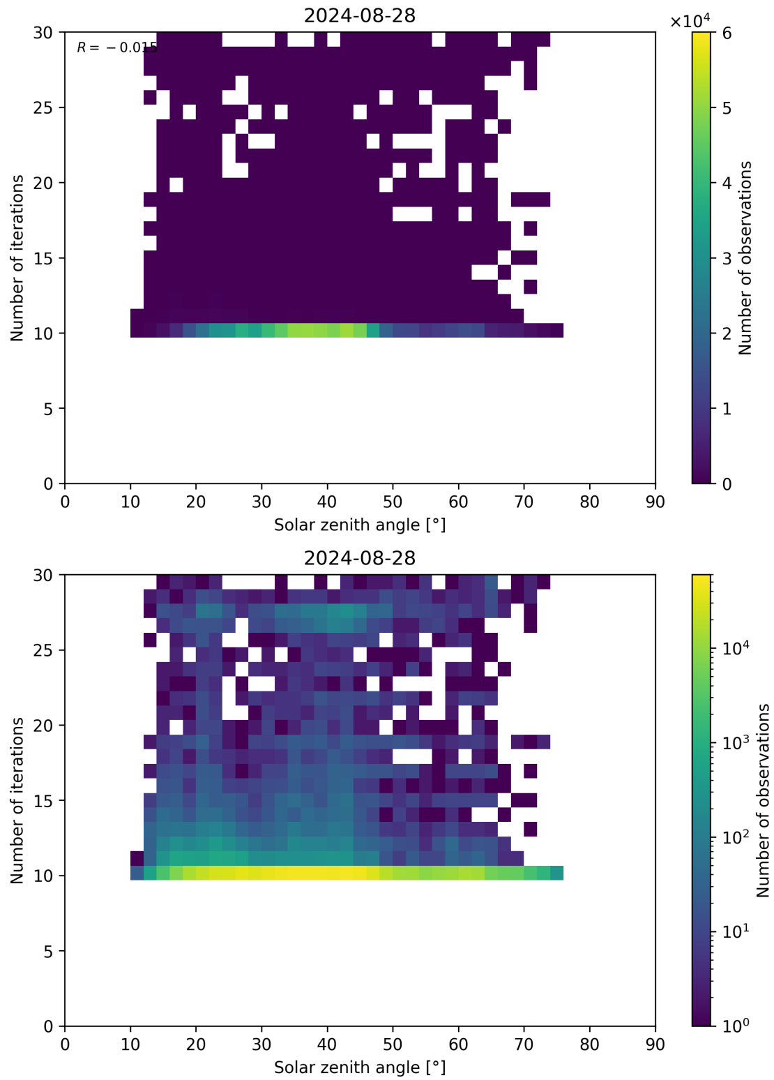
Figure 102: Scatter density plot of “Solar zenith angle” against “Number of iterations” for 2024-08-27 to 2024-08-29.
