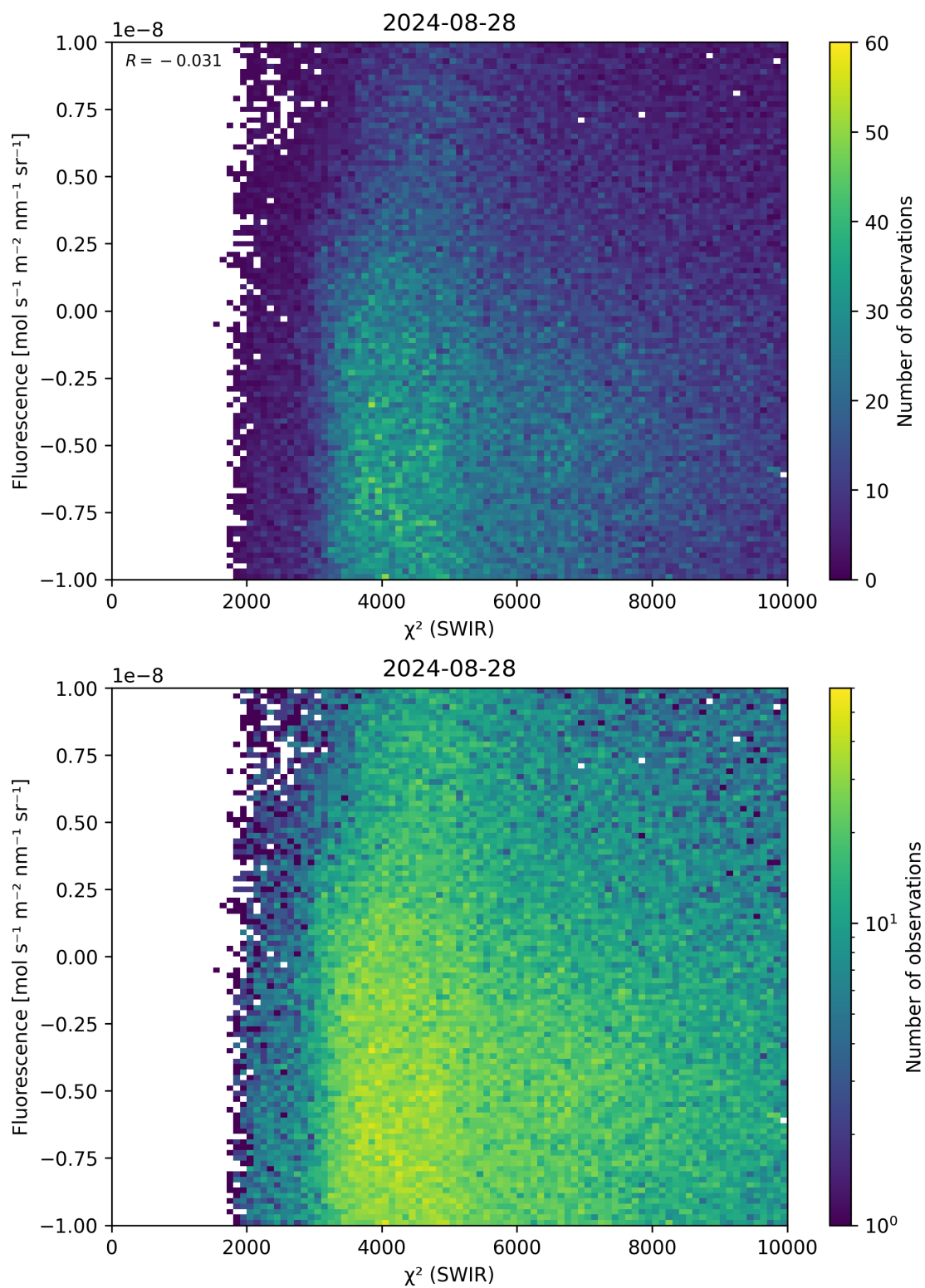
Figure 49: Scatter density plot of “ \chi^2 (SWIR)” against “Fluorescence” for 2024-08-27 to 2024-08-29.
