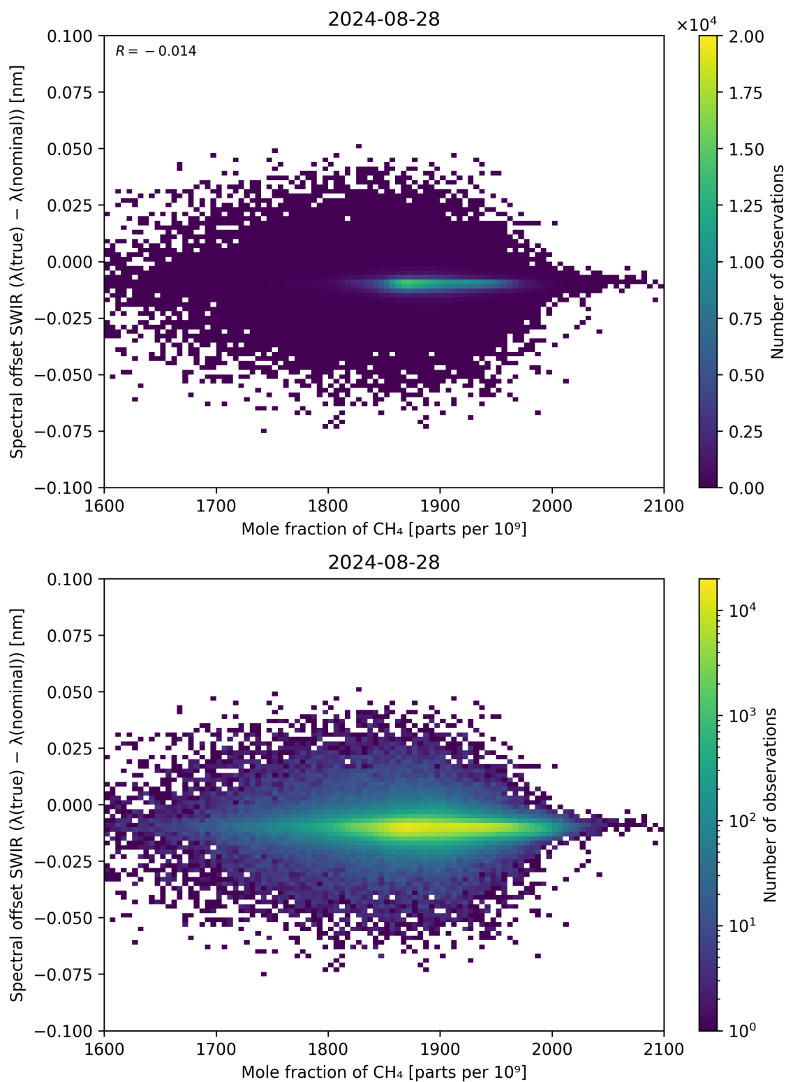
Figure 86: Scatter density plot of “Mole fraction of CH 4 ” against “Spectral offset SWIR ( \lambda_{\text{true}} - \lambda_{\text{nominal}} )” for 2024-08-27 to 2024-08-29.
