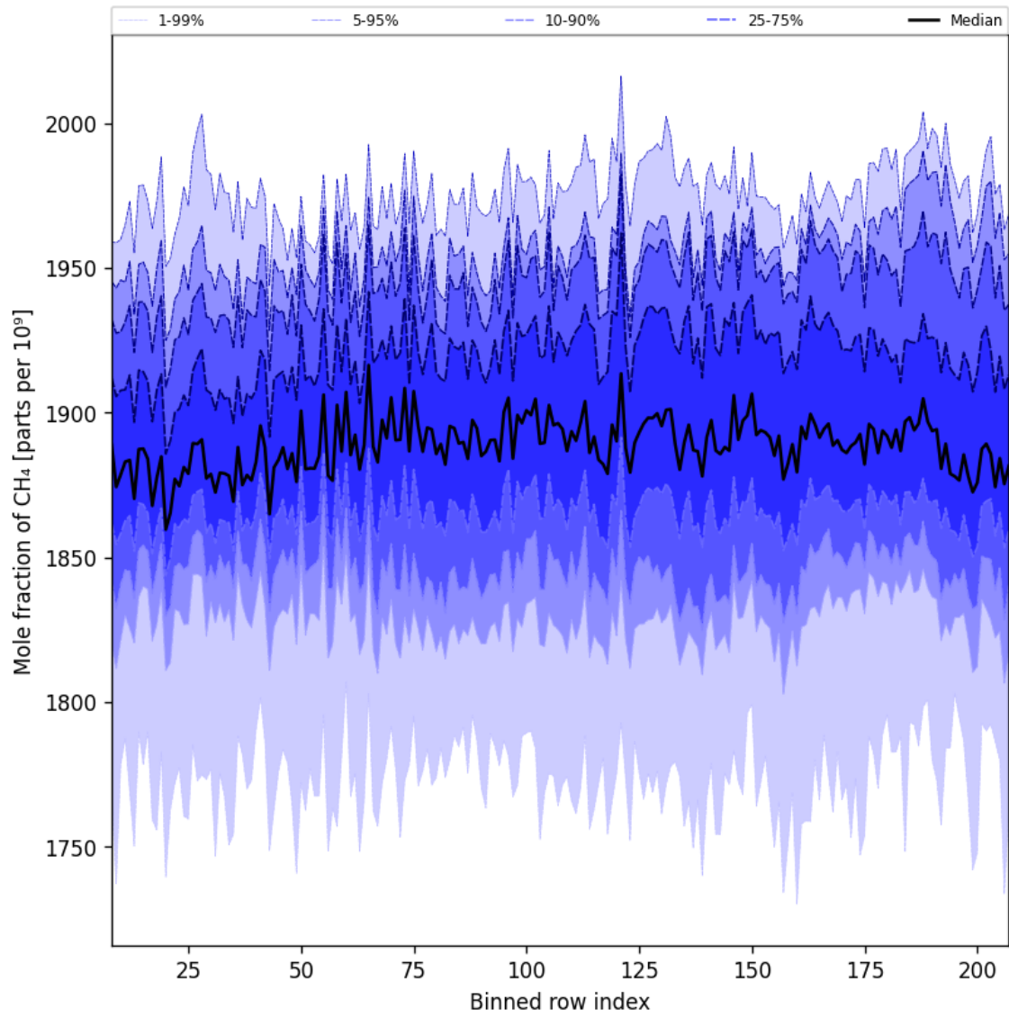
Figure 34: Along track statistics of “Mole fraction of CH 4 ” for 2024-08-27 to 2024-08-29
