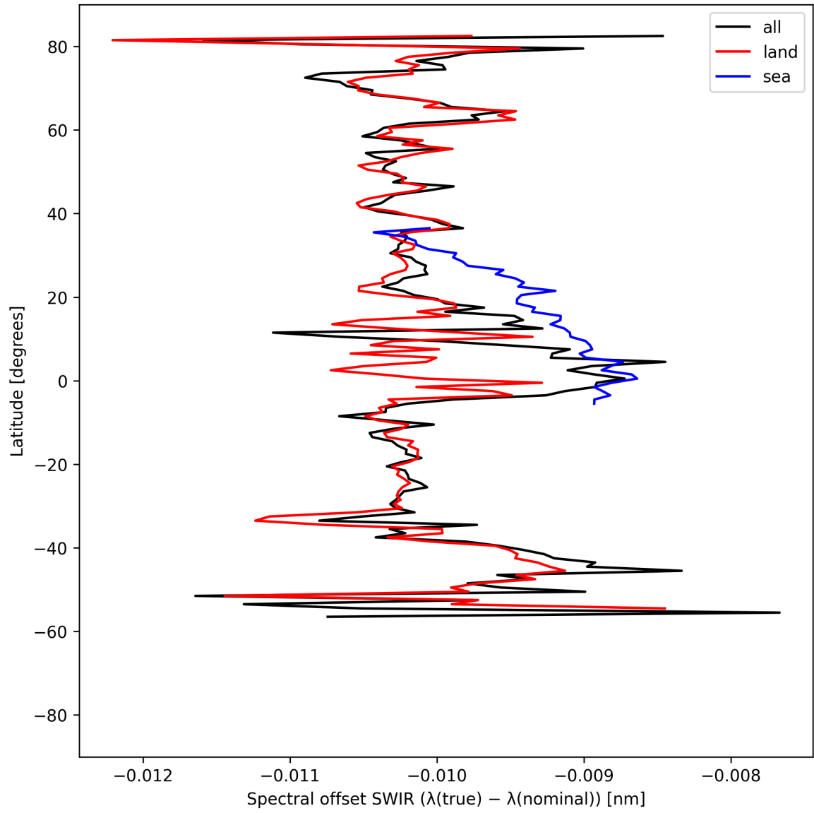
Figure 16: Zonal average of “Spectral offset SWIR ( \lambda_{\text{true}} - \lambda_{\text{nominal}} )” for 2024-08-27 to 2024-08-29.
