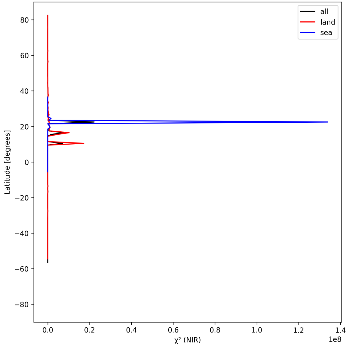
Figure 18: Zonal average of “ \chi^2 (NIR)” for 2024-08-27 to 2024-08-29.
