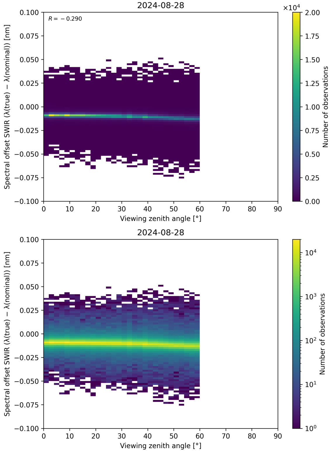
Figure 116: Scatter density plot of “Viewing zenith angle” against “Spectral offset SWIR ( \lambda_{\text{true}} - \lambda_{\text{nominal}} )” for 2024-08-27 to 2024-08-29.
