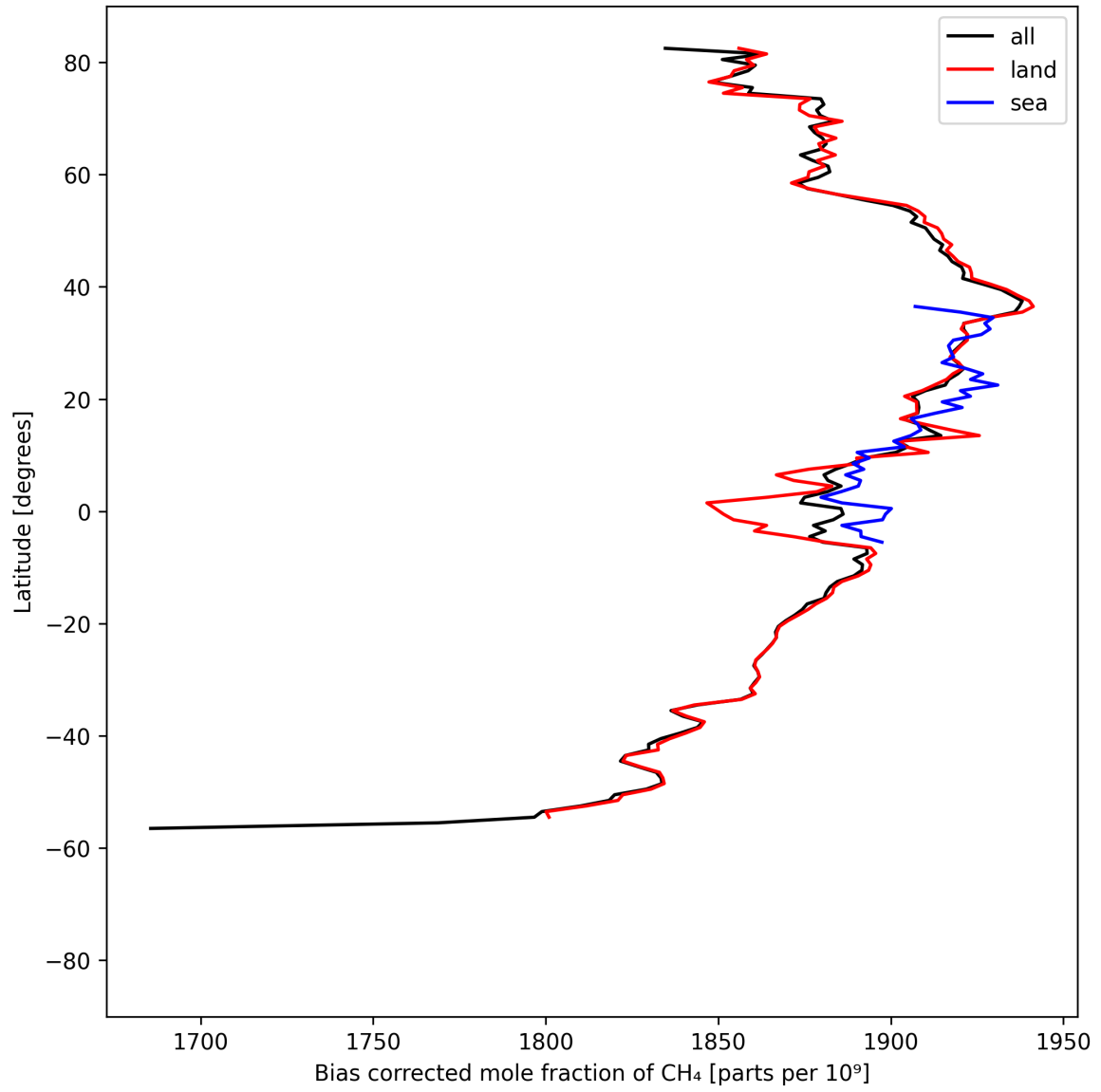
Figure 14: Zonal average of “Bias corrected mole fraction of CH 4 ” for 2024-08-27 to 2024-08-29.
