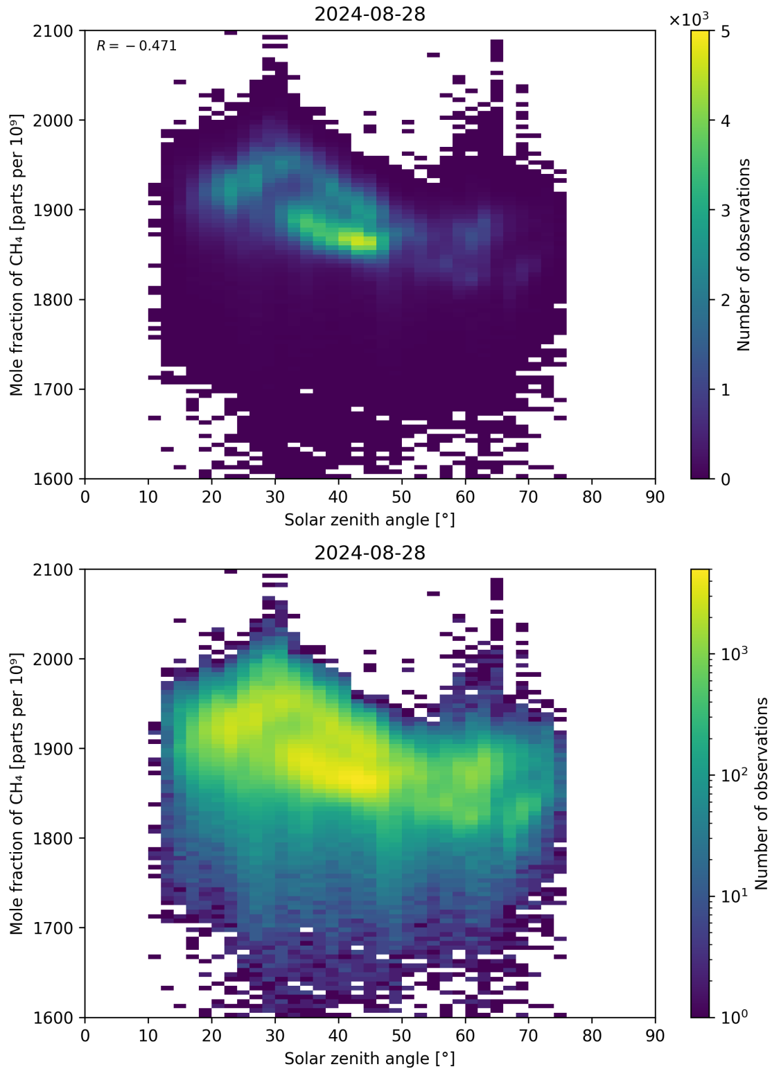
Figure 99: Scatter density plot of “Solar zenith angle” against “Mole fraction of CH 4 ” for 2024-08-27 to 2024-08-29.
