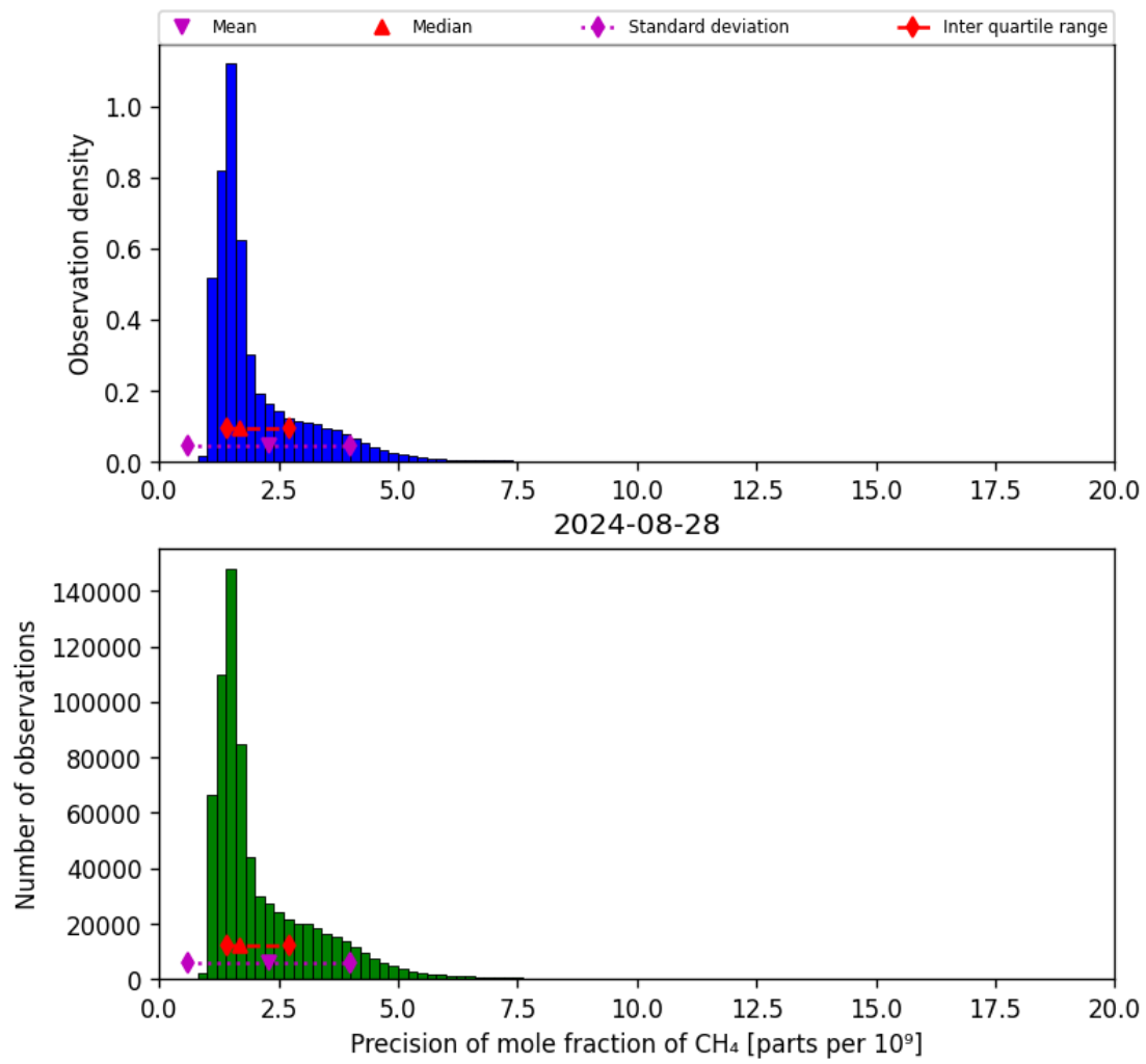
Figure 24: Histogram of “Precision of mole fraction of CH 4 ” for 2024-08-27 to 2024-08-29
