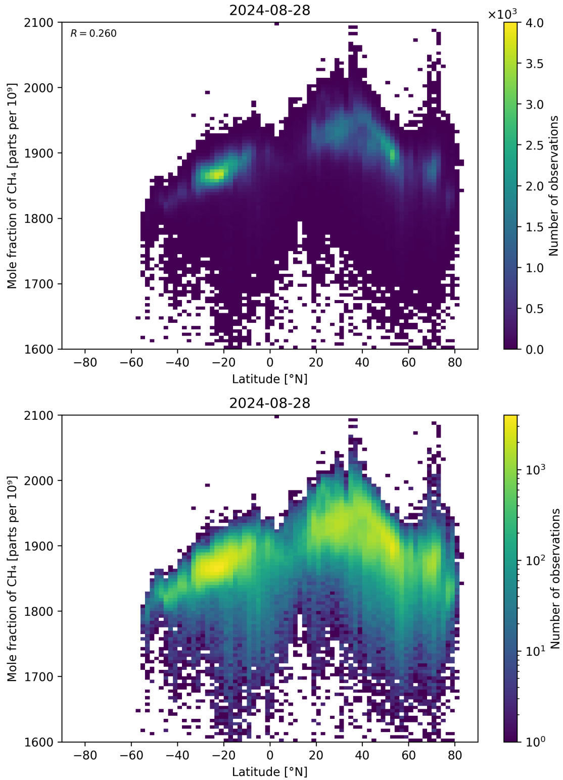
Figure 57: Scatter density plot of “Latitude” against “Mole fraction of \text{CH}_4 ” for 2024-08-27 to 2024-08-29.
