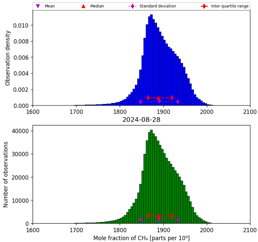
Figure 23: Histogram of “Mole fraction of CH 4 ” for 2024-08-27 to 2024-08-29
