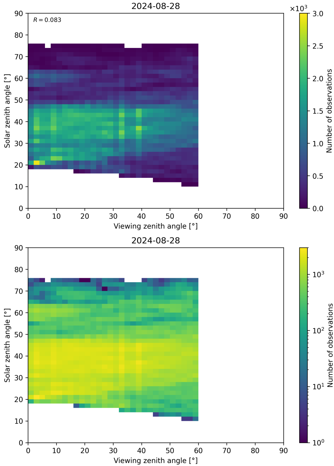
Figure 115: Scatter density plot of “Viewing zenith angle” against “Solar zenith angle” for 2024-08-27 to 2024-08-29.
