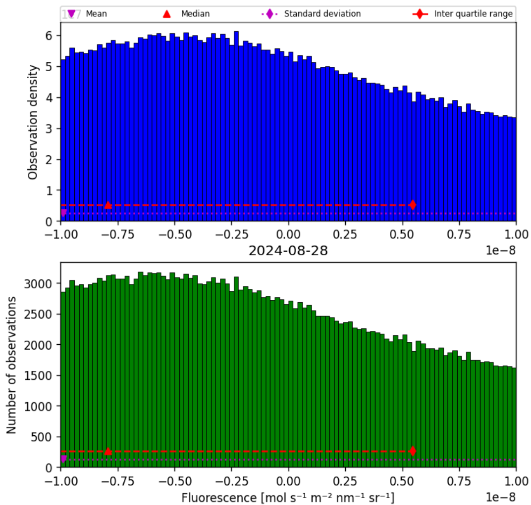
Figure 32: Histogram of “Fluorescence” for 2024-08-27 to 2024-08-29
