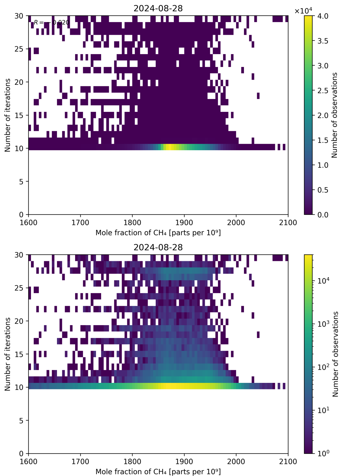
Figure 76: Scatter density plot of “Mole fraction of CH 4 ” against “Number of iterations” for 2024-08-27 to 2024-08-29.
