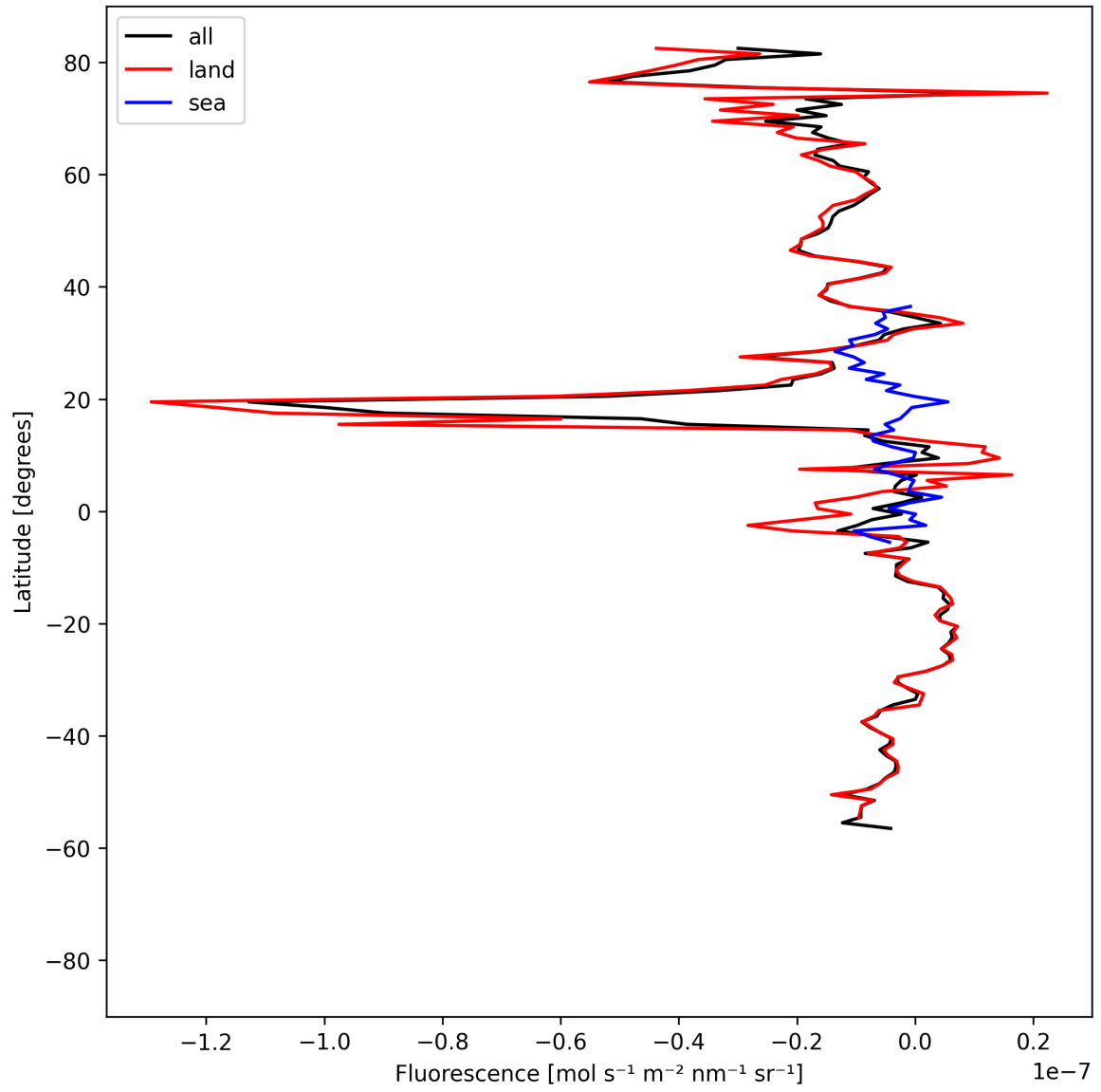
Figure 21: Zonal average of “Fluorescence” for 2024-08-27 to 2024-08-29.
