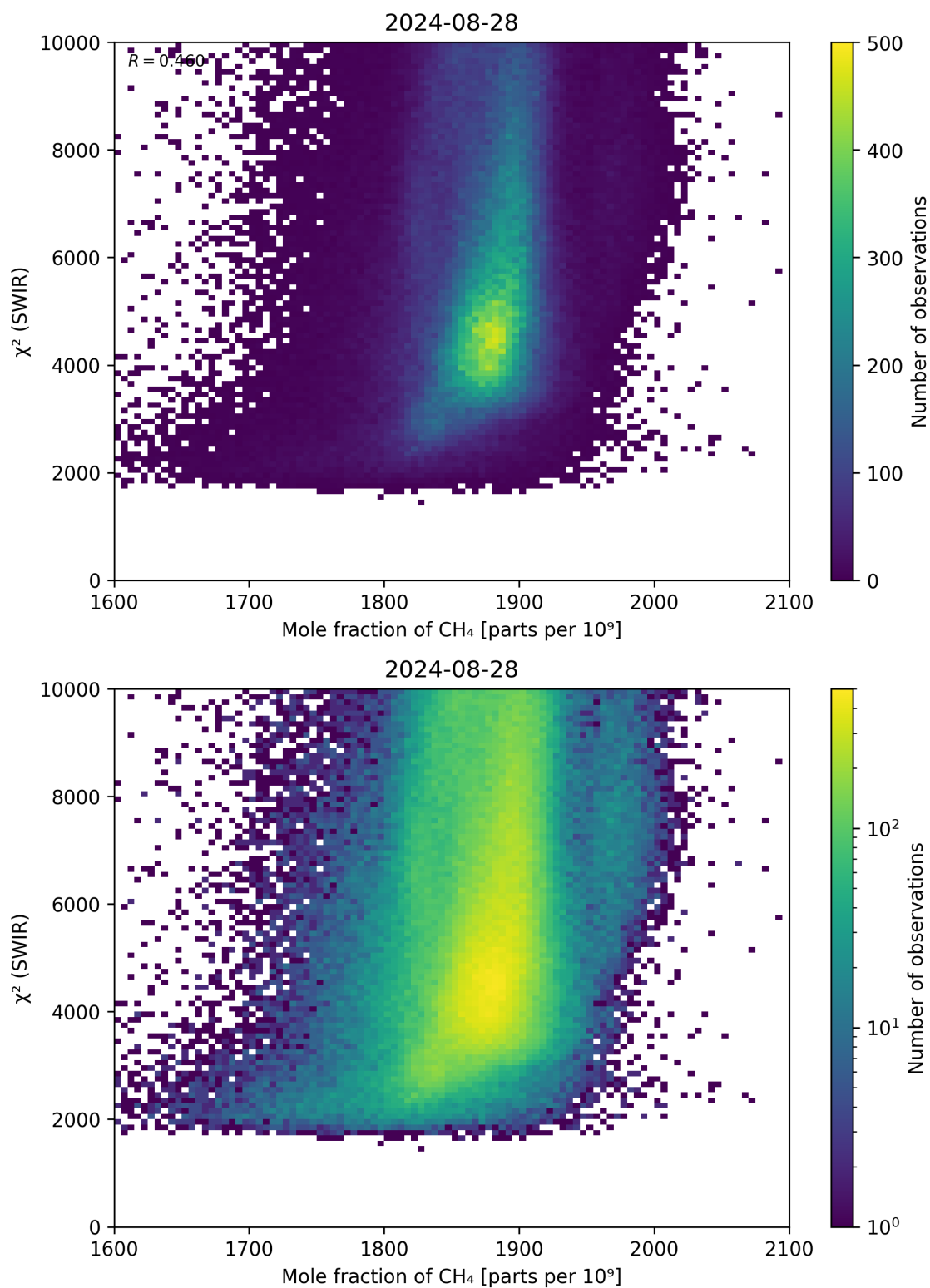
Figure 71: Scatter density plot of “Mole fraction of \text{CH}_4 ” against “ \chi^2 (SWIR)” for 2024-08-27 to 2024-08-29.
