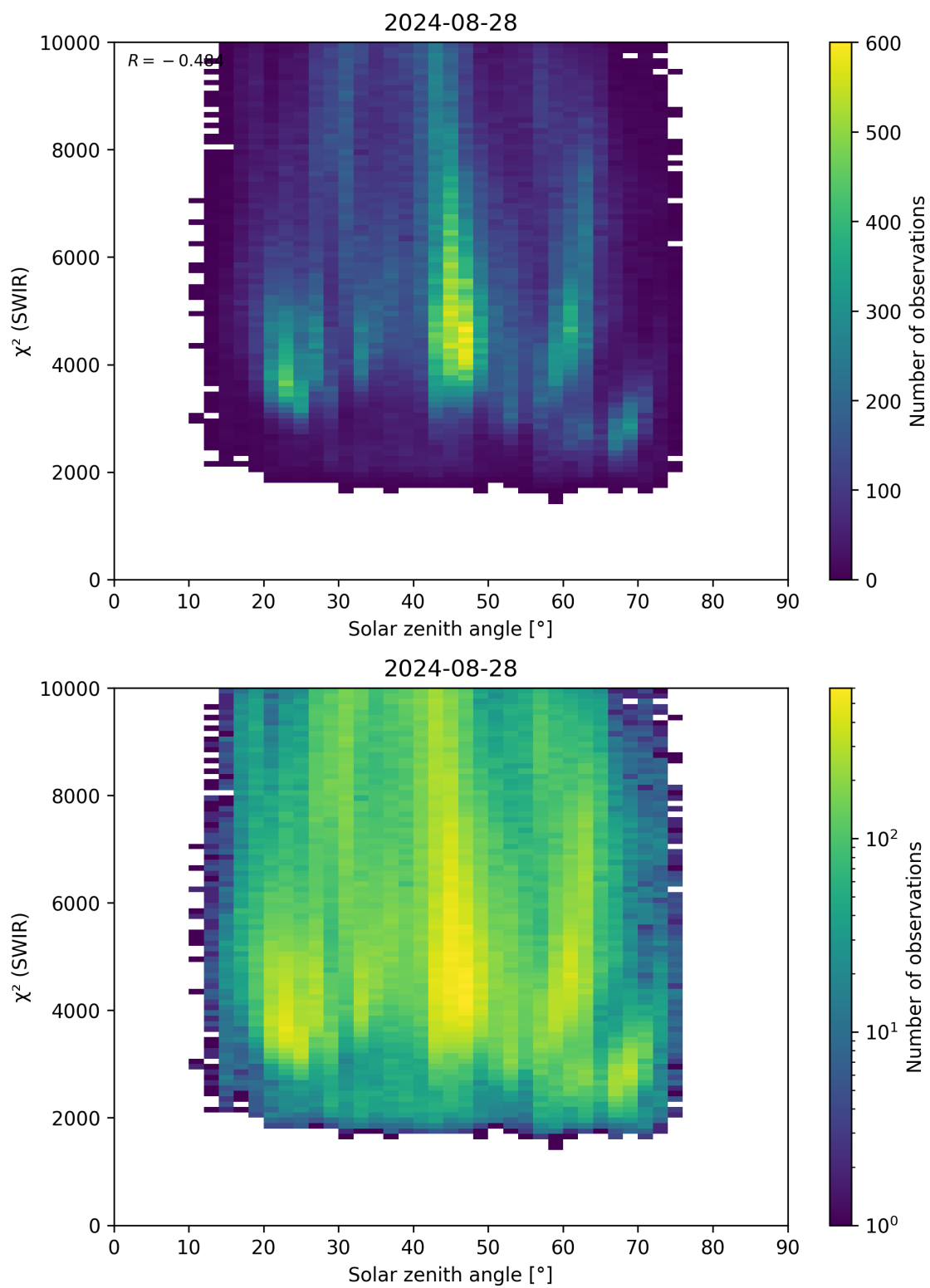
Figure 95: Scatter density plot of “Solar zenith angle” against “ \chi^2 (SWIR)” for 2024-08-27 to 2024-08-29.
