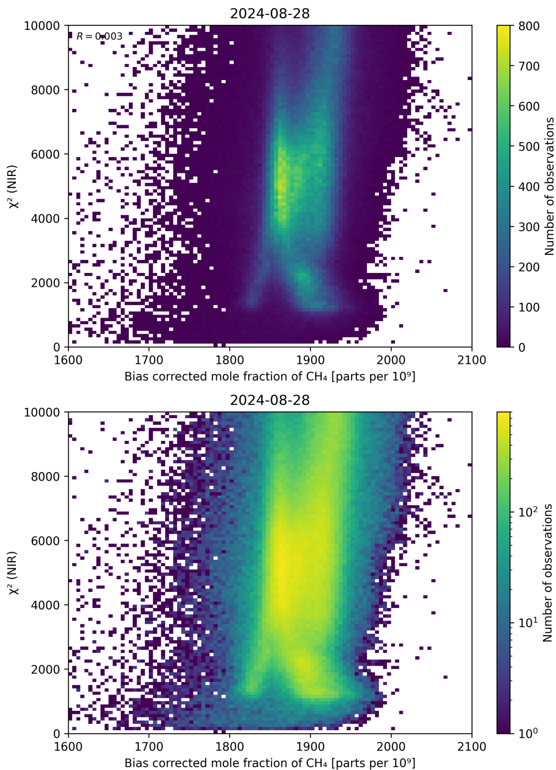
Figure 63: Scatter density plot of “Bias corrected mole fraction of CH 4 ” against “ \chi^2 (NIR)” for 2024-08-27 to 2024-08-29.
