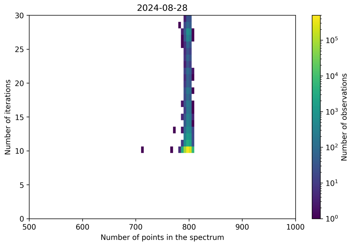
Figure 92: Scatter density plot of “Number of points in the spectrum” against “Number of iterations” for 2024-08-27 to 2024-08-29.
