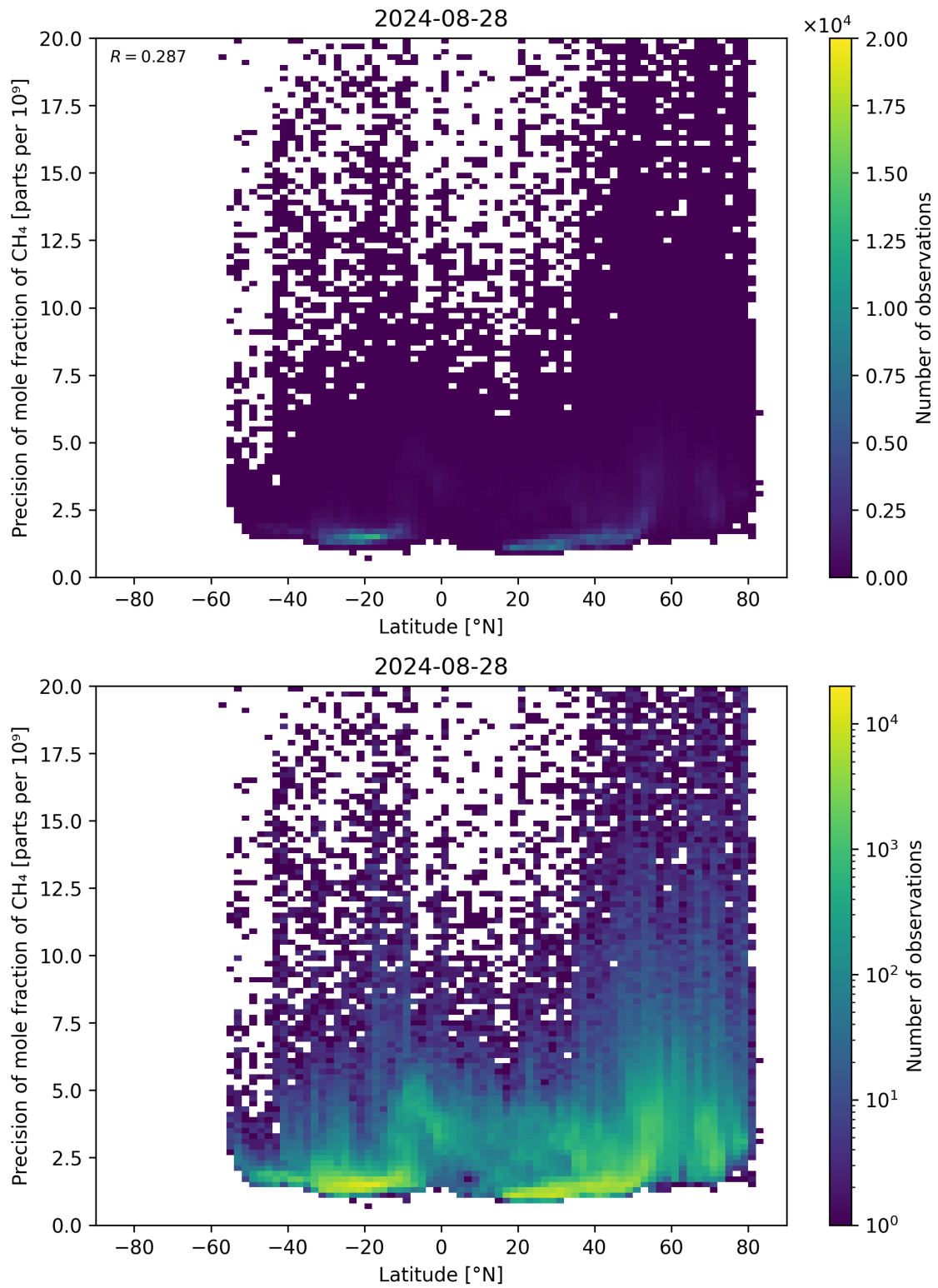
Figure 59: Scatter density plot of “Latitude” against “Precision of mole fraction of \text{CH}_4 ” for 2024-08-27 to 2024-08-29.
