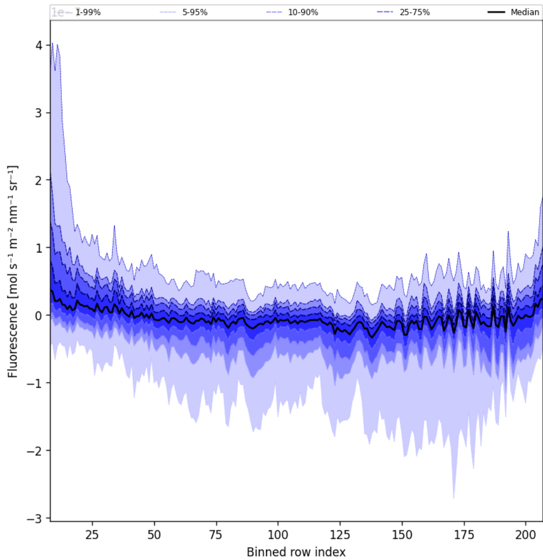
Figure 43: Along track statistics of “Fluorescence” for 2024-08-27 to 2024-08-29
