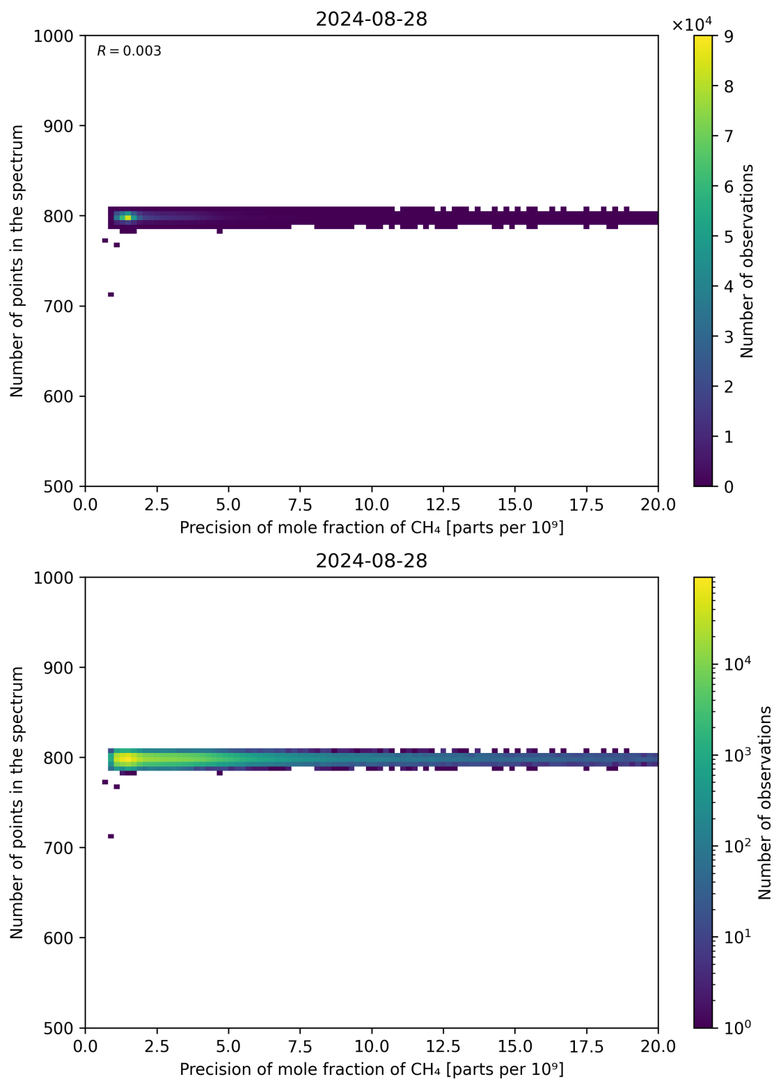
Figure 84: Scatter density plot of “Precision of mole fraction of CH 4 ” against “Number of points in the spectrum” for 2024-08-27 to 2024-08-29.
