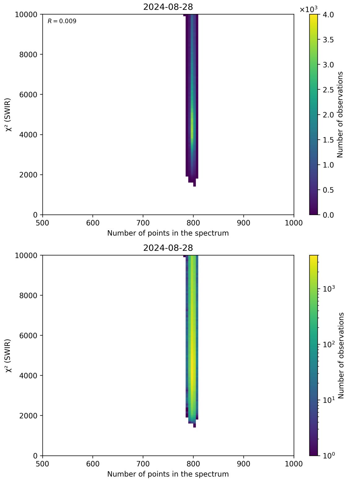
Figure 89: Scatter density plot of “Number of points in the spectrum” against “ \chi^2 (SWIR)” for 2024-08-27 to 2024-08-29.
