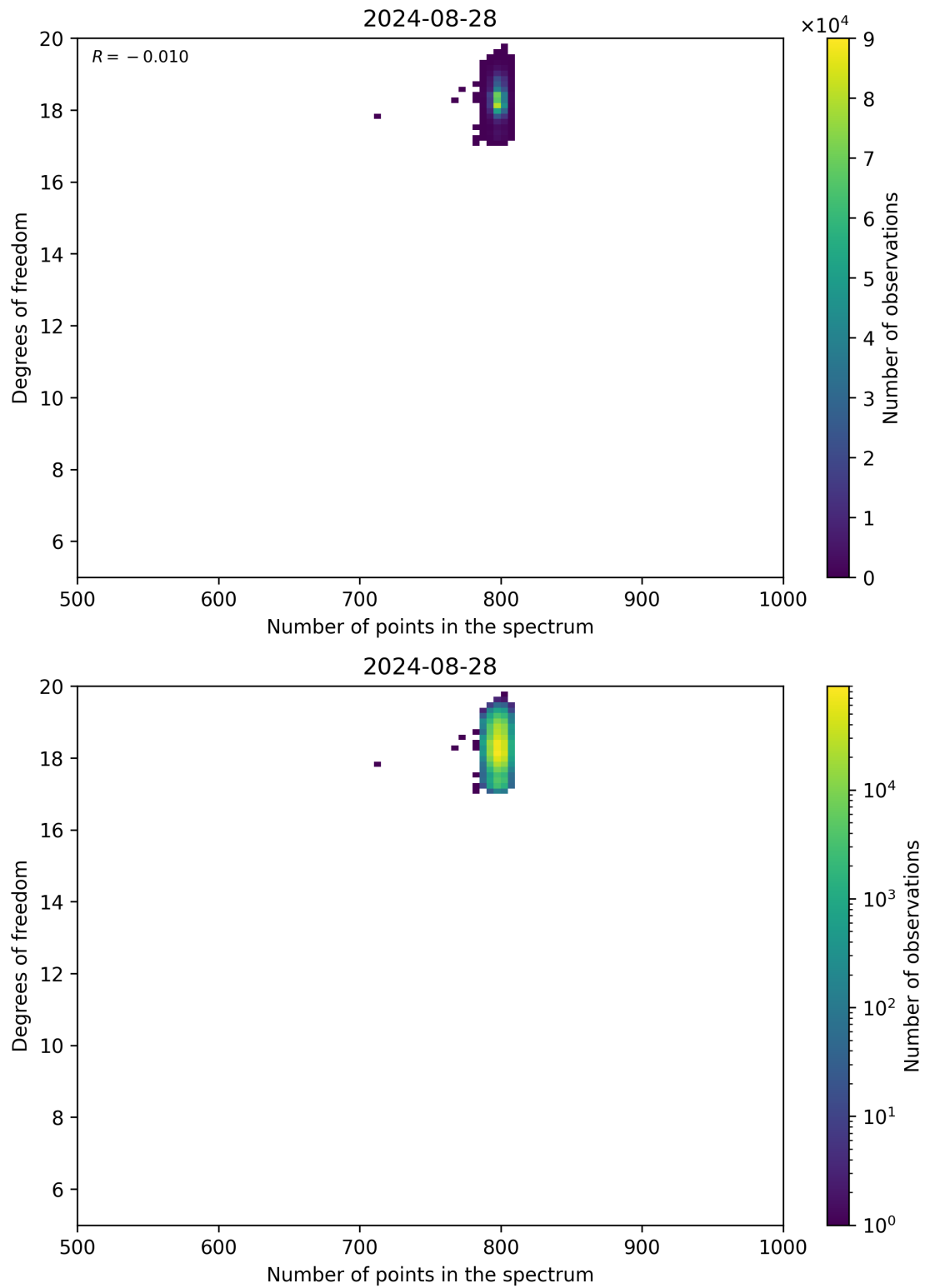
Figure 90: Scatter density plot of “Number of points in the spectrum” against “Degrees of freedom” for 2024-08-27 to 2024-08-29.
