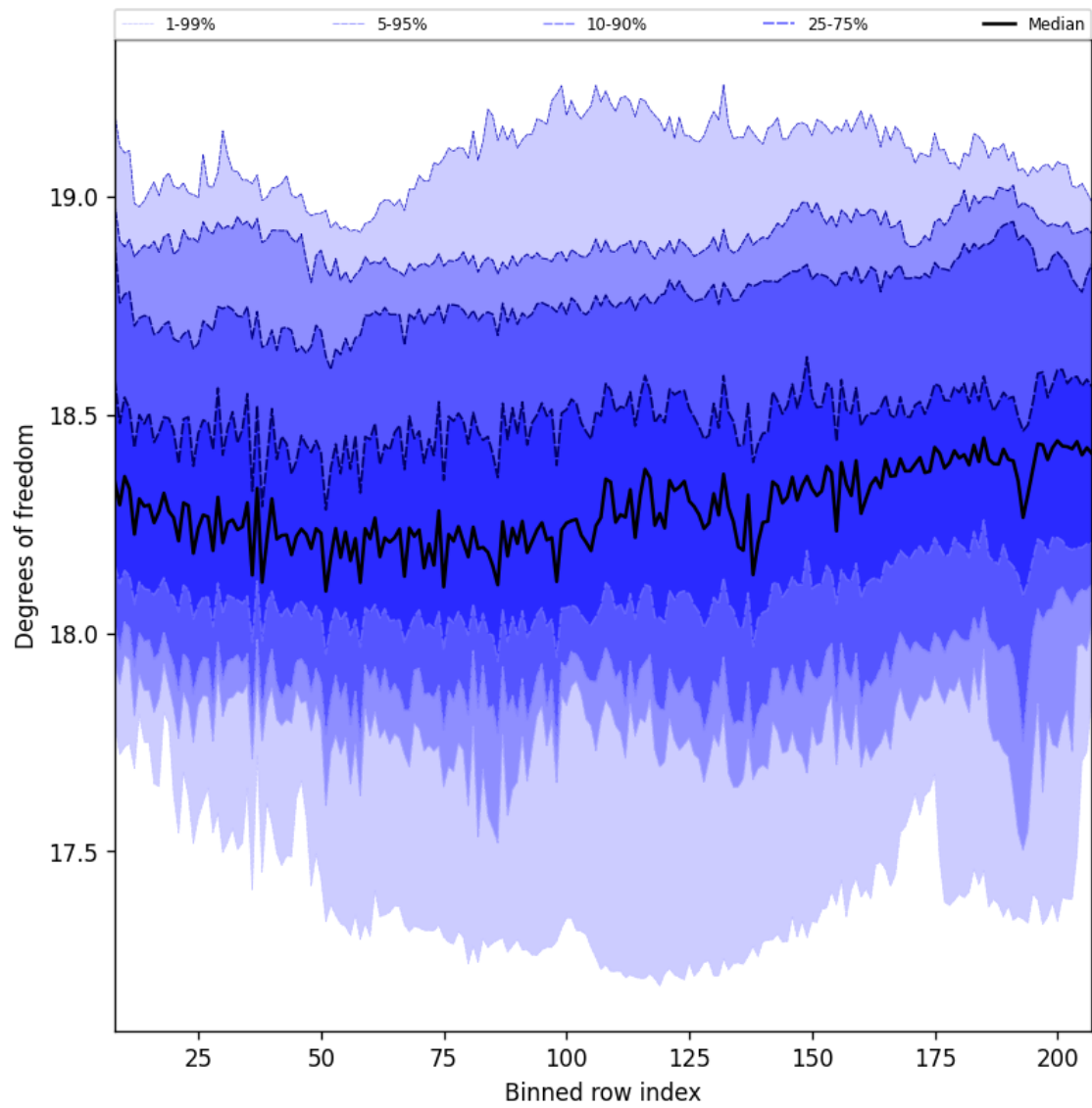
Figure 41: Along track statistics of “Degrees of freedom” for 2024-08-27 to 2024-08-29
