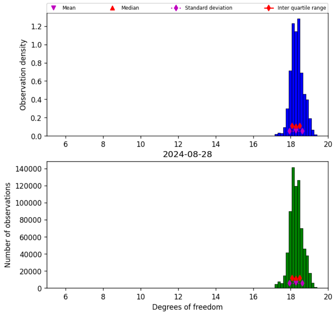
Figure 30: Histogram of “Degrees of freedom” for 2024-08-27 to 2024-08-29
