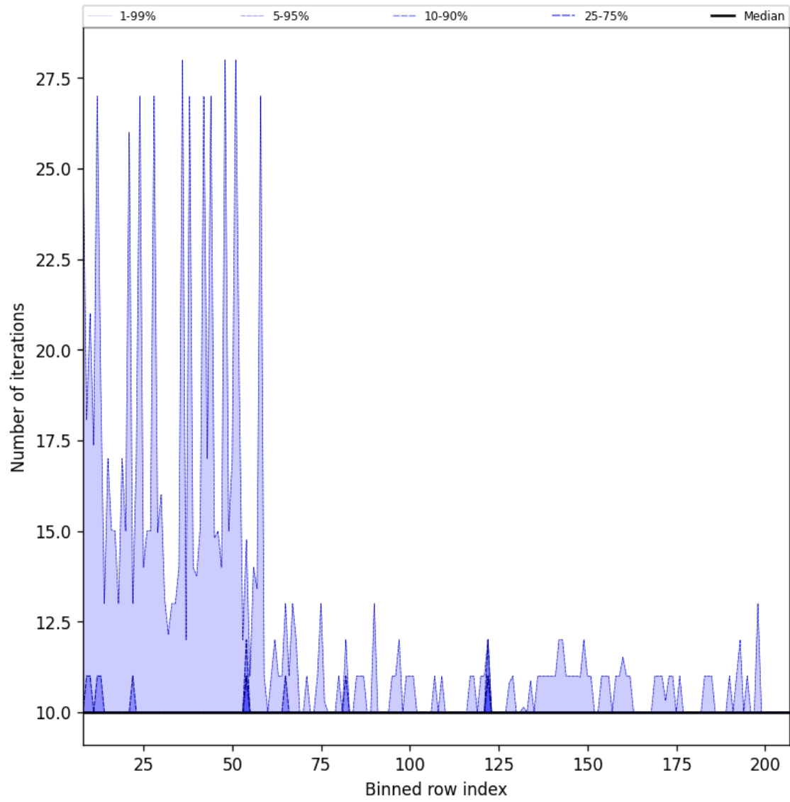
Figure 42: Along track statistics of “Number of iterations” for 2024-08-27 to 2024-08-29
