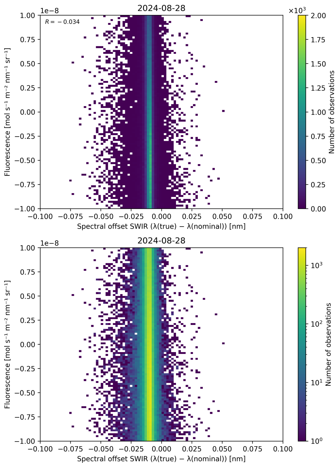
Figure 120: Scatter density plot of “Spectral offset SWIR ( \lambda_{\text{true}} - \lambda_{\text{nominal}} )” against “Fluorescence” for 2024-08-27 to 2024-08-29.
