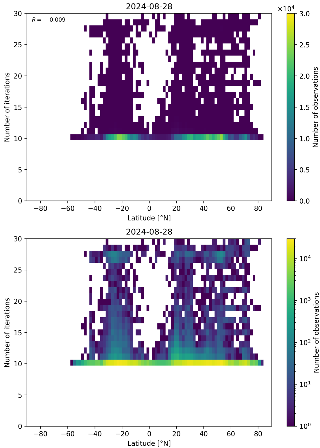
Figure 60: Scatter density plot of “Latitude” against “Number of iterations” for 2024-08-27 to 2024-08-29.
