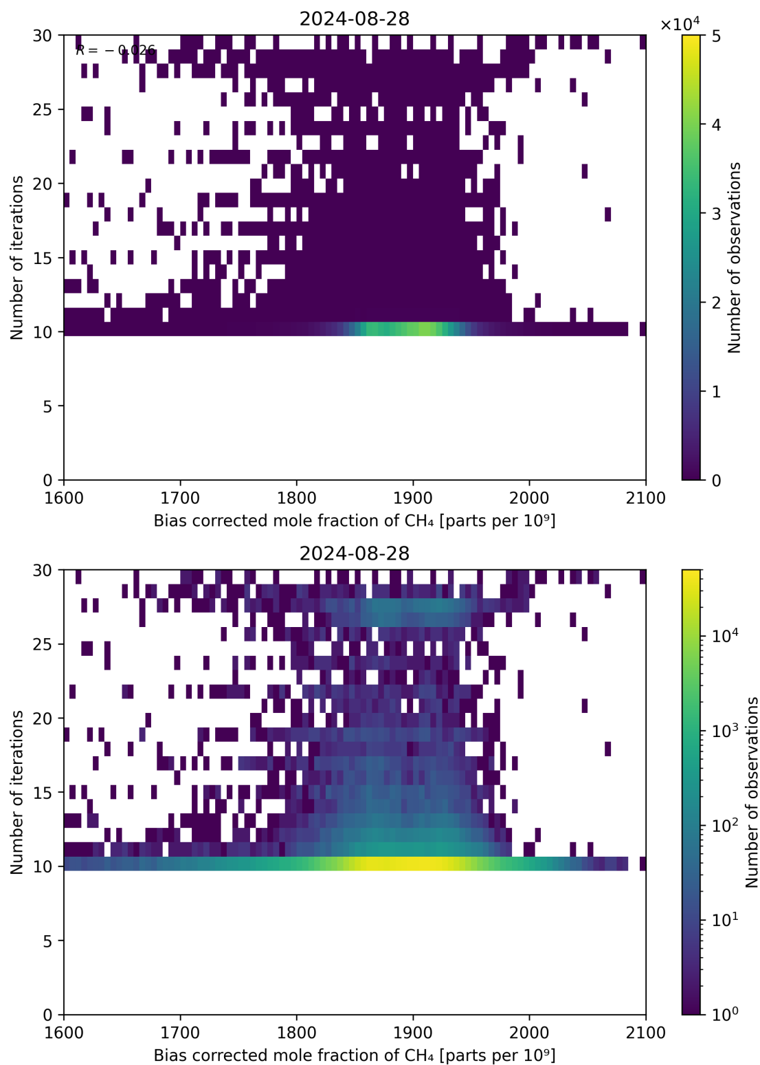
Figure 67: Scatter density plot of “Bias corrected mole fraction of CH 4 ” against “Number of iterations” for 2024-08-27 to 2024-08-29.
