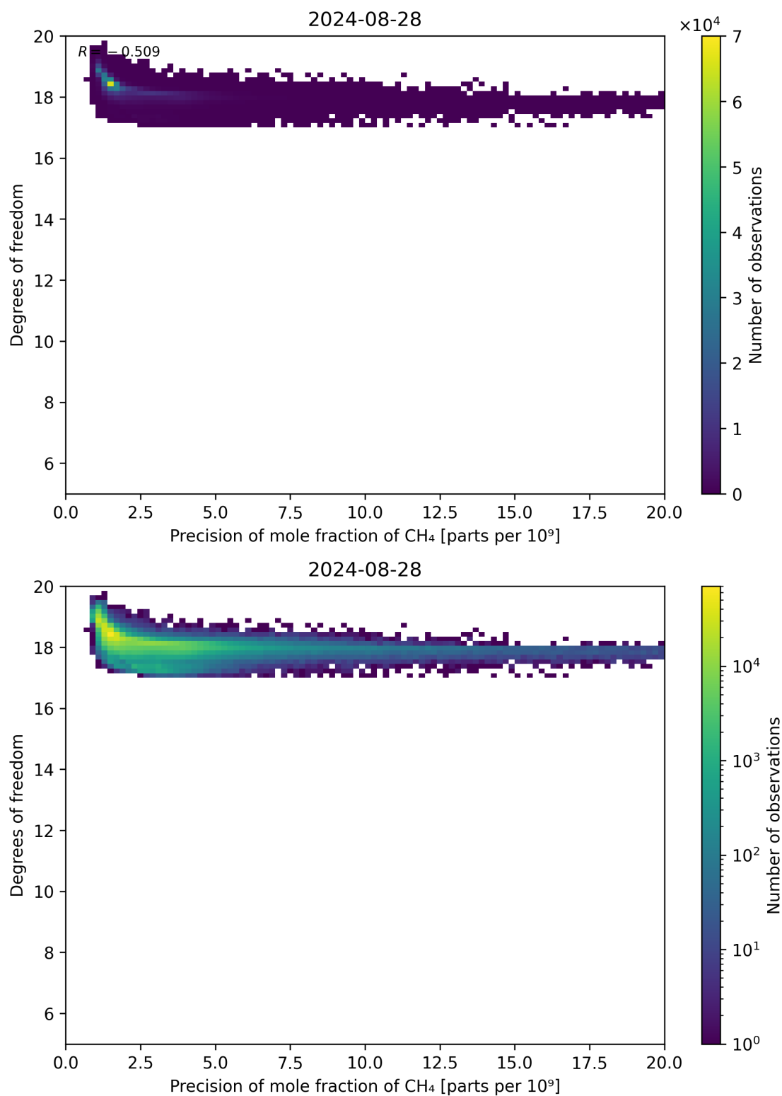
Figure 80: Scatter density plot of “Precision of mole fraction of CH 4 ” against “Degrees of freedom” for 2024-08-27 to 2024-08-29.
