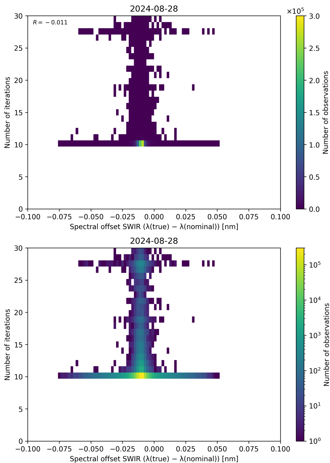
Figure 121: Scatter density plot of “Spectral offset SWIR ( \lambda_{\text{true}} - \lambda_{\text{nominal}} )” against “Number of iterations” for 2024-08-27 to 2024-08-29.
