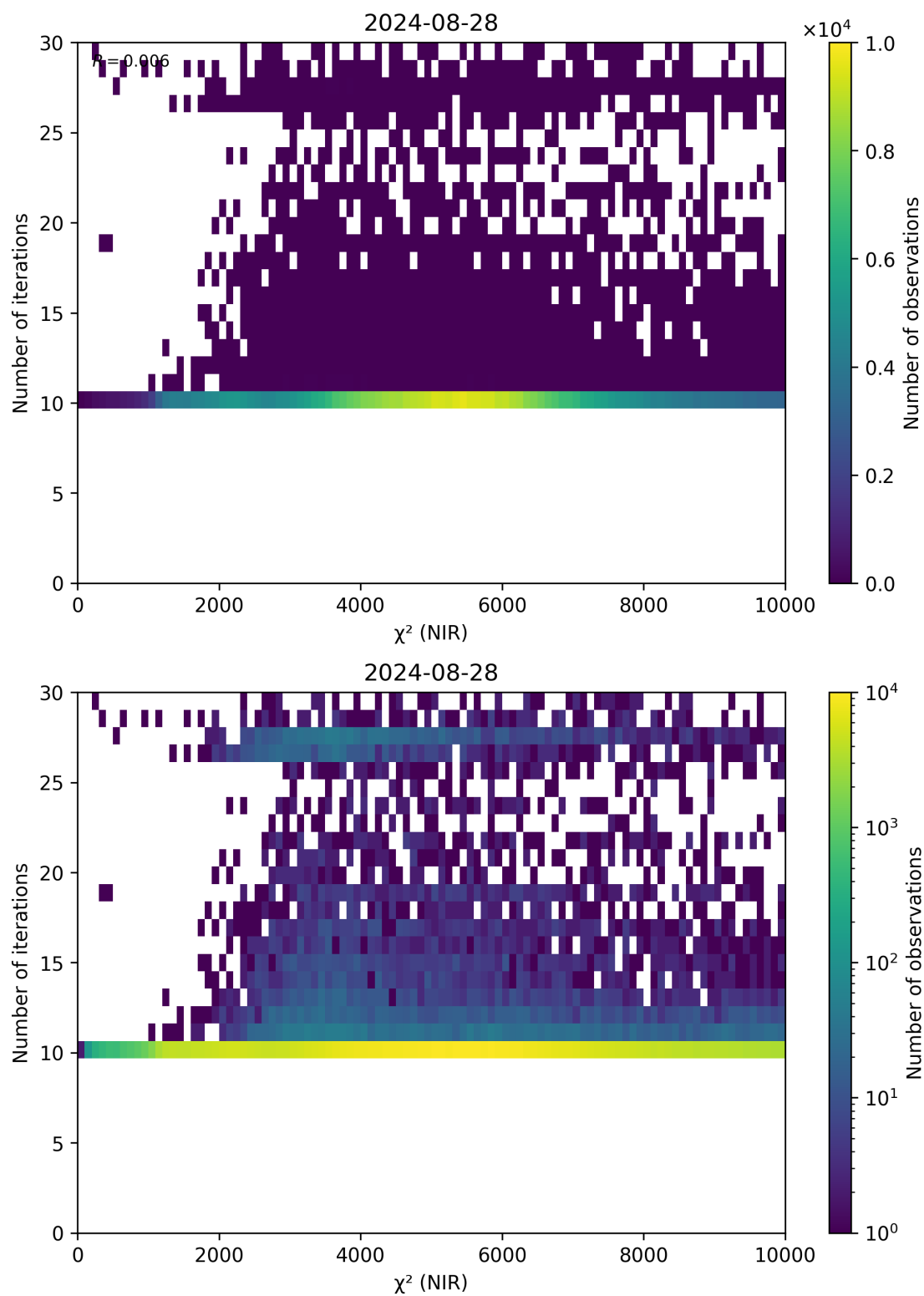
Figure 46: Scatter density plot of “ \chi^2 (NIR)” against “Number of iterations” for 2024-08-27 to 2024-08-29.
