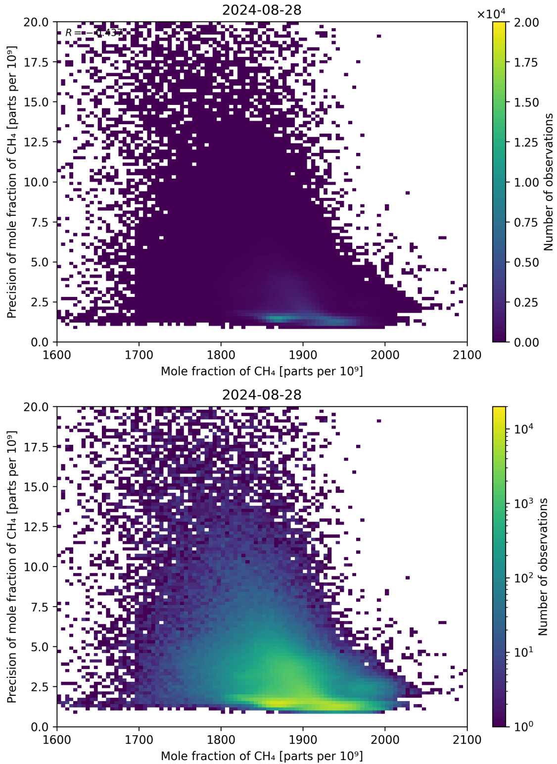
Figure 75: Scatter density plot of “Mole fraction of CH 4 ” against “Precision of mole fraction of CH 4 ” for 2024-08-27 to 2024-08-29.
