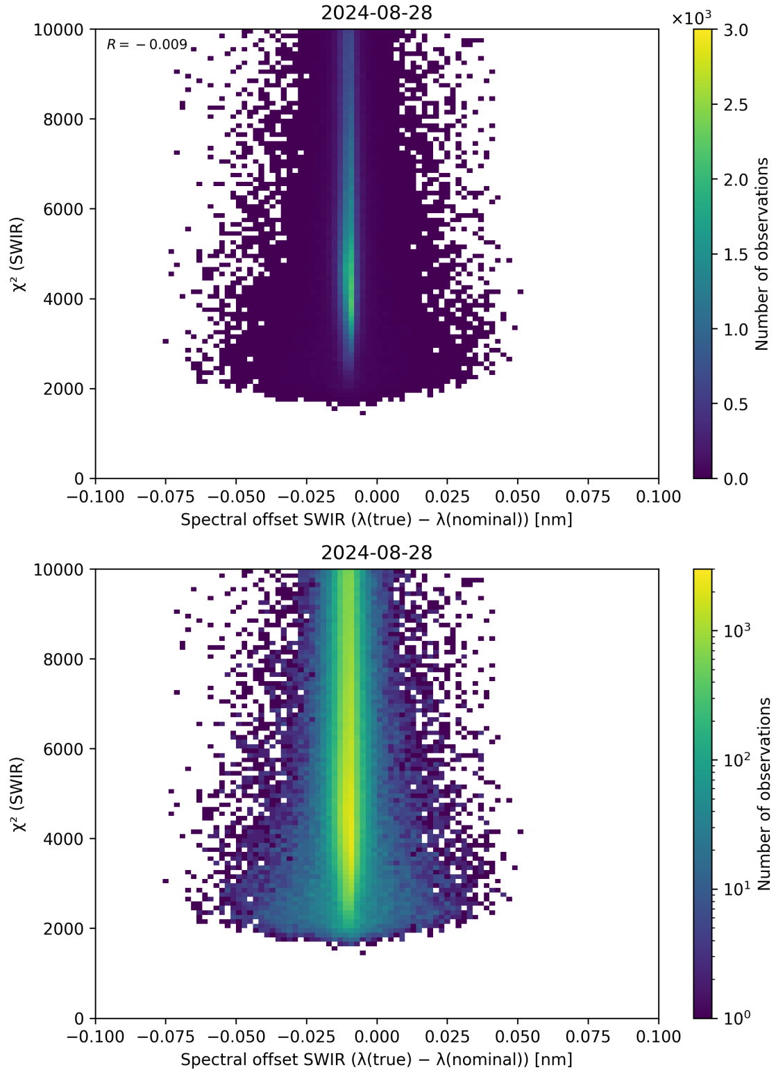
Figure 118: Scatter density plot of “Spectral offset SWIR ( \lambda_{\text{true}} - \lambda_{\text{nominal}} )” against “ \chi^2 (SWIR)” for 2024-08-27 to 2024-08-29.
