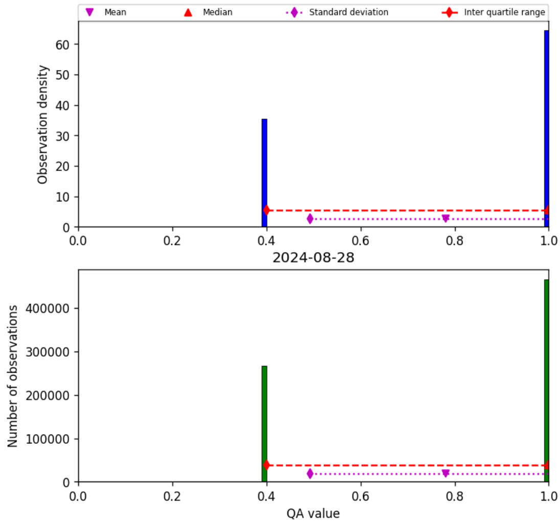
Figure 22: Histogram of “QA value” for 2024-08-27 to 2024-08-29
