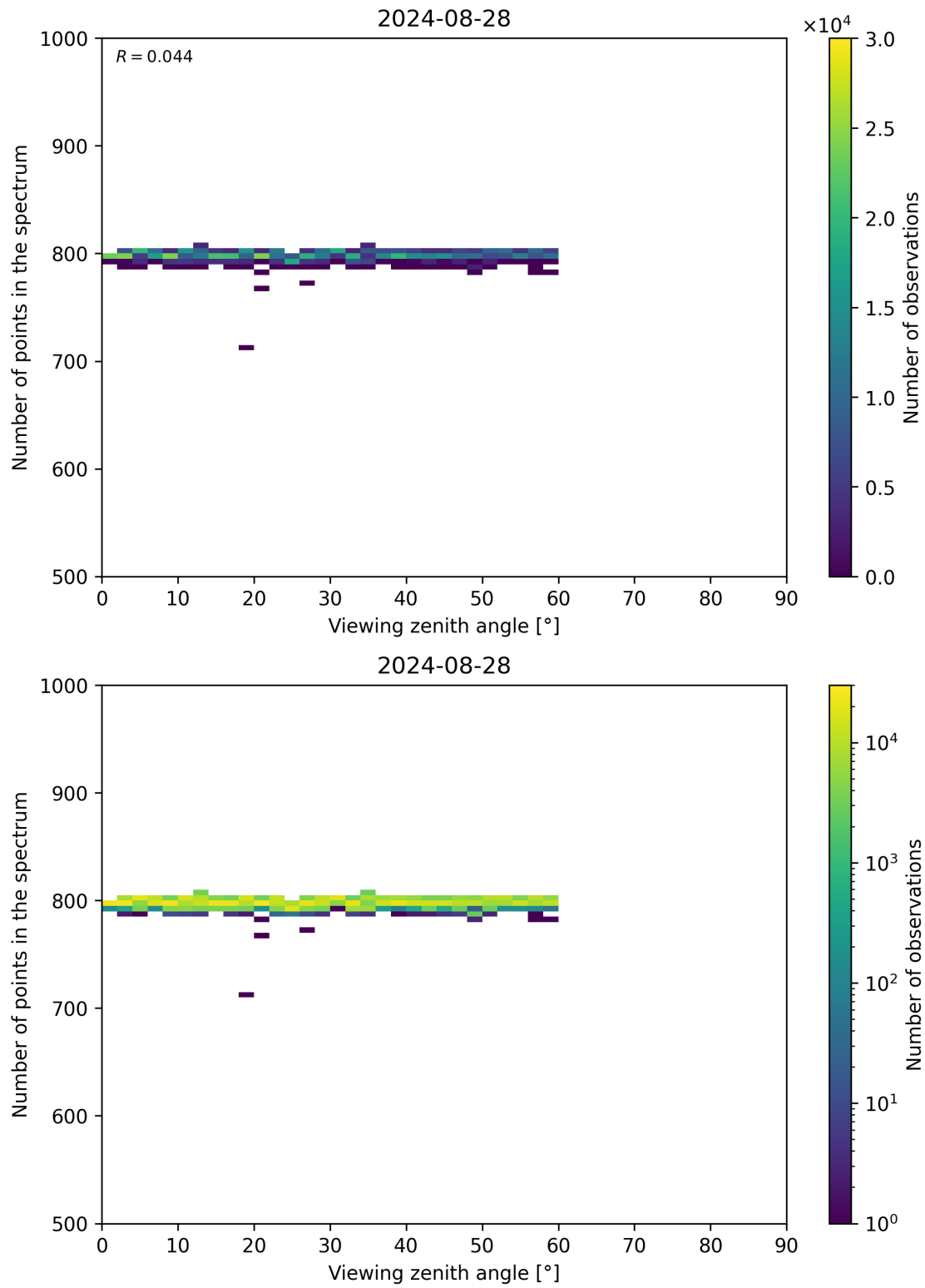
Figure 114: Scatter density plot of “Viewing zenith angle” against “Number of points in the spectrum” for 2024-08-27 to 2024-08-29.
