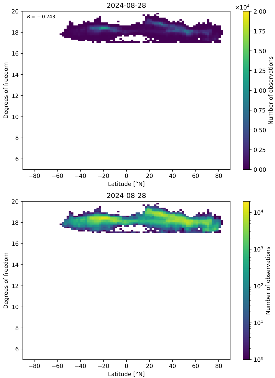
Figure 55: Scatter density plot of “Latitude” against “Degrees of freedom” for 2024-08-27 to 2024-08-29.
