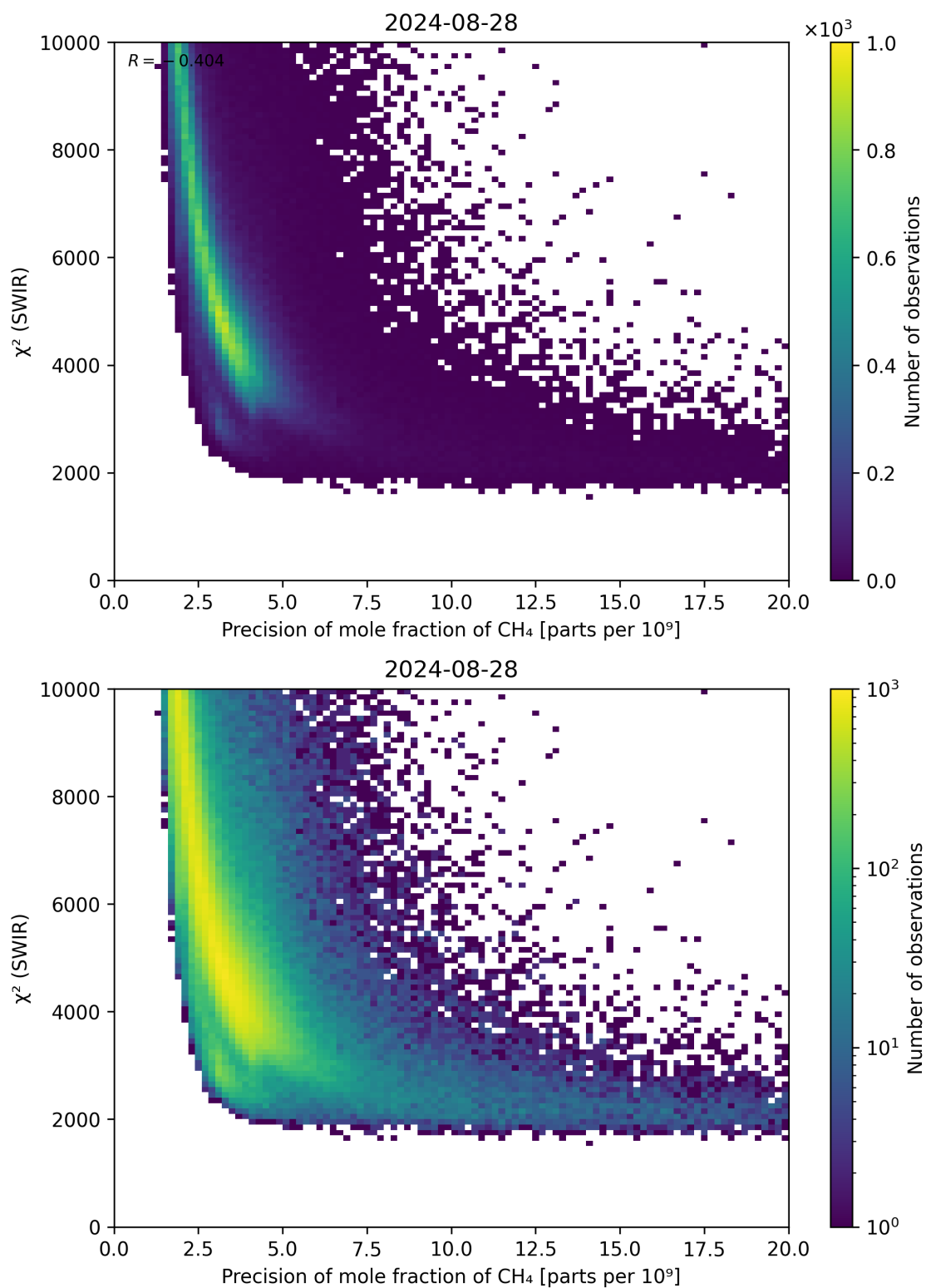
Figure 79: Scatter density plot of “Precision of mole fraction of \text{CH}_4 ” against “ \chi^2 (SWIR)” for 2024-08-27 to 2024-08-29.
