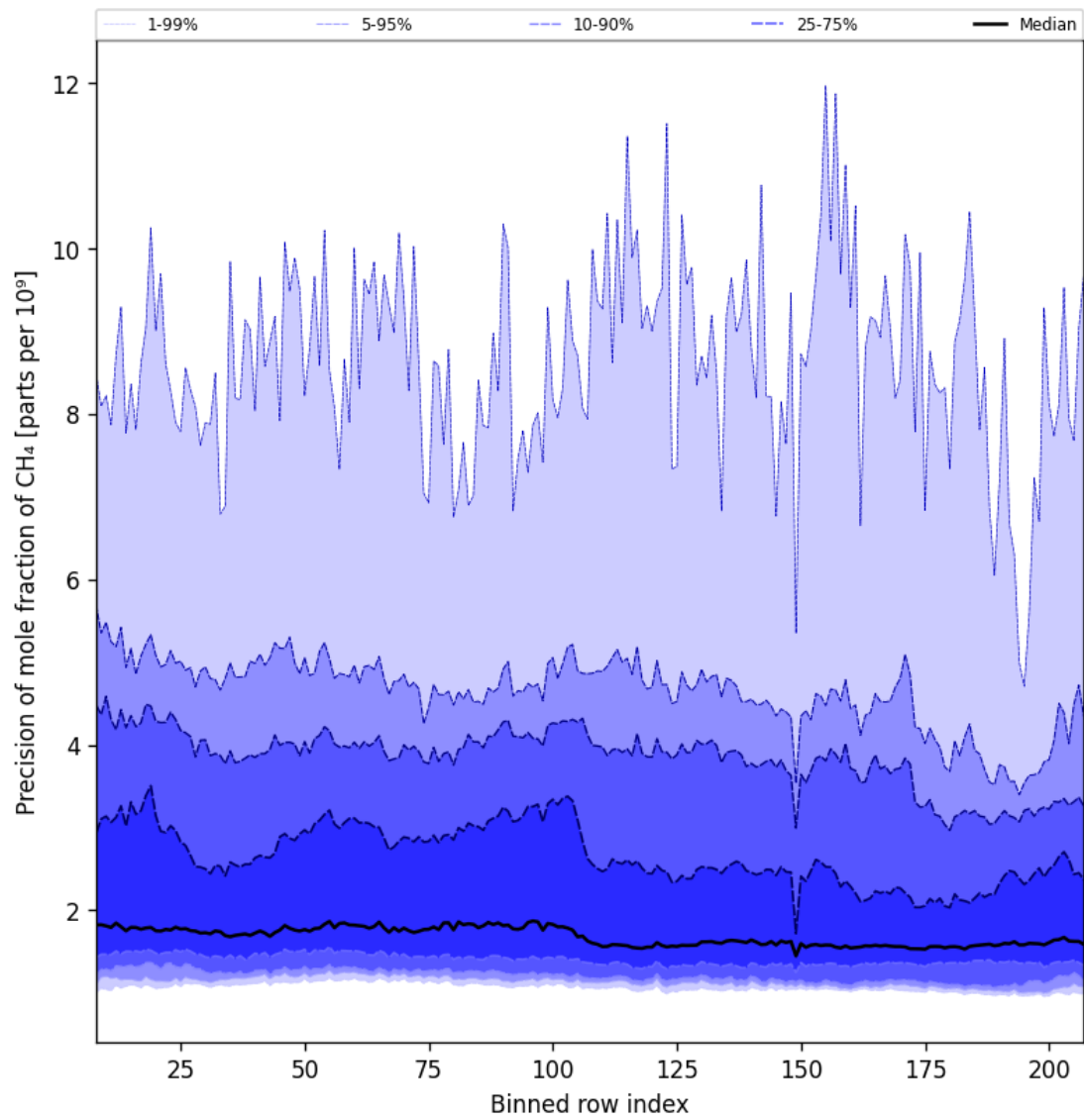
Figure 35: Along track statistics of “Precision of mole fraction of CH 4 ” for 2024-08-27 to 2024-08-29
