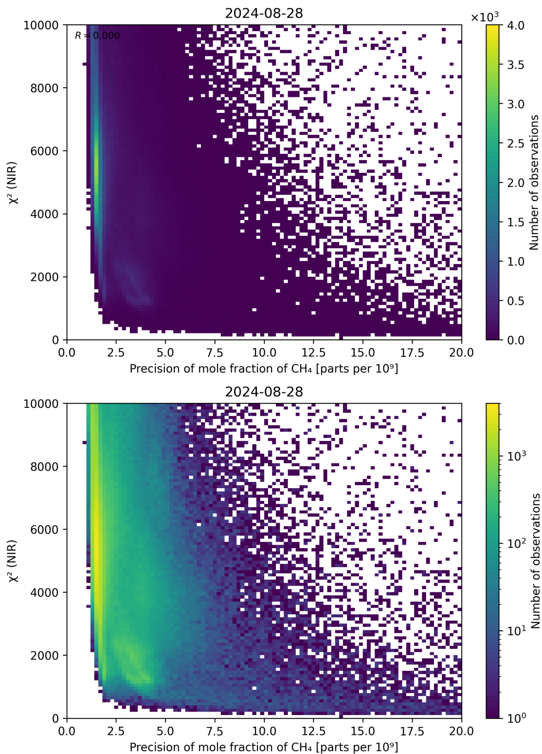
Figure 78: Scatter density plot of “Precision of mole fraction of \text{CH}_4 ” against “ \chi^2 (NIR)” for 2024-08-27 to 2024-08-29.
