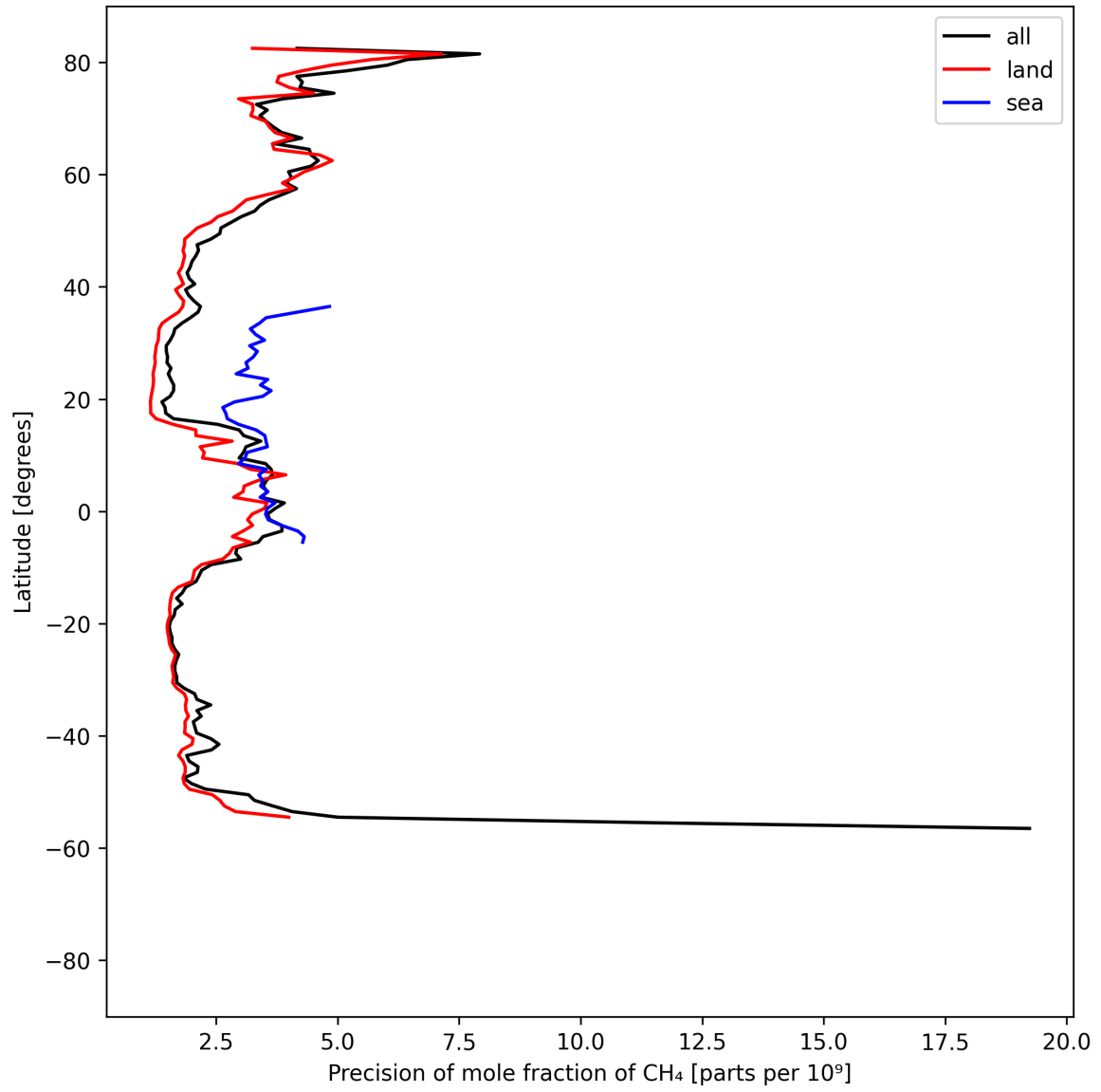
Figure 13: Zonal average of “Precision of mole fraction of CH 4 ” for 2024-08-27 to 2024-08-29.
