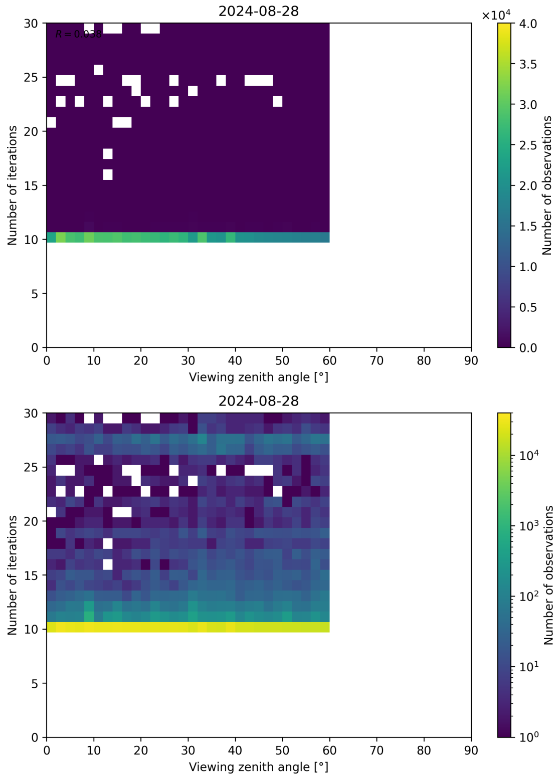
Figure 113: Scatter density plot of “Viewing zenith angle” against “Number of iterations” for 2024-08-27 to 2024-08-29.
