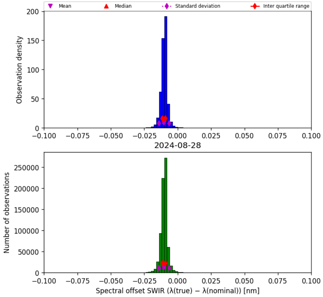
Figure 27: Histogram of “Spectral offset SWIR ( \lambda_{\text{true}} - \lambda_{\text{nominal}} )” for 2024-08-27 to 2024-08-29
