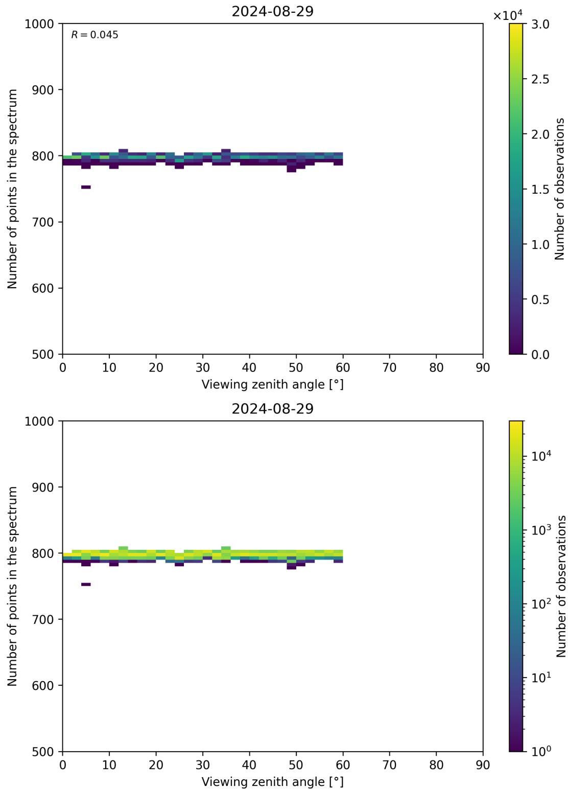
Figure 114: Scatter density plot of “Viewing zenith angle” against “Number of points in the spectrum” for 2024-08-28 to 2024-08-30.
