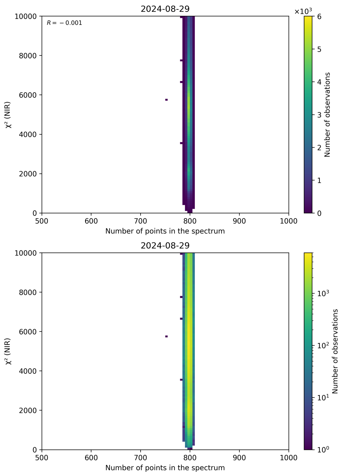
Figure 88: Scatter density plot of “Number of points in the spectrum” against “ \chi^2 (NIR)” for 2024-08-28 to 2024-08-30.
