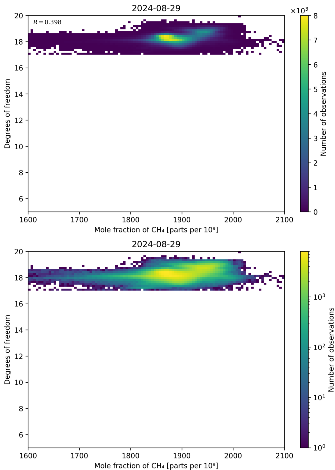
Figure 72: Scatter density plot of “Mole fraction of CH 4 ” against “Degrees of freedom” for 2024-08-28 to 2024-08-30.
