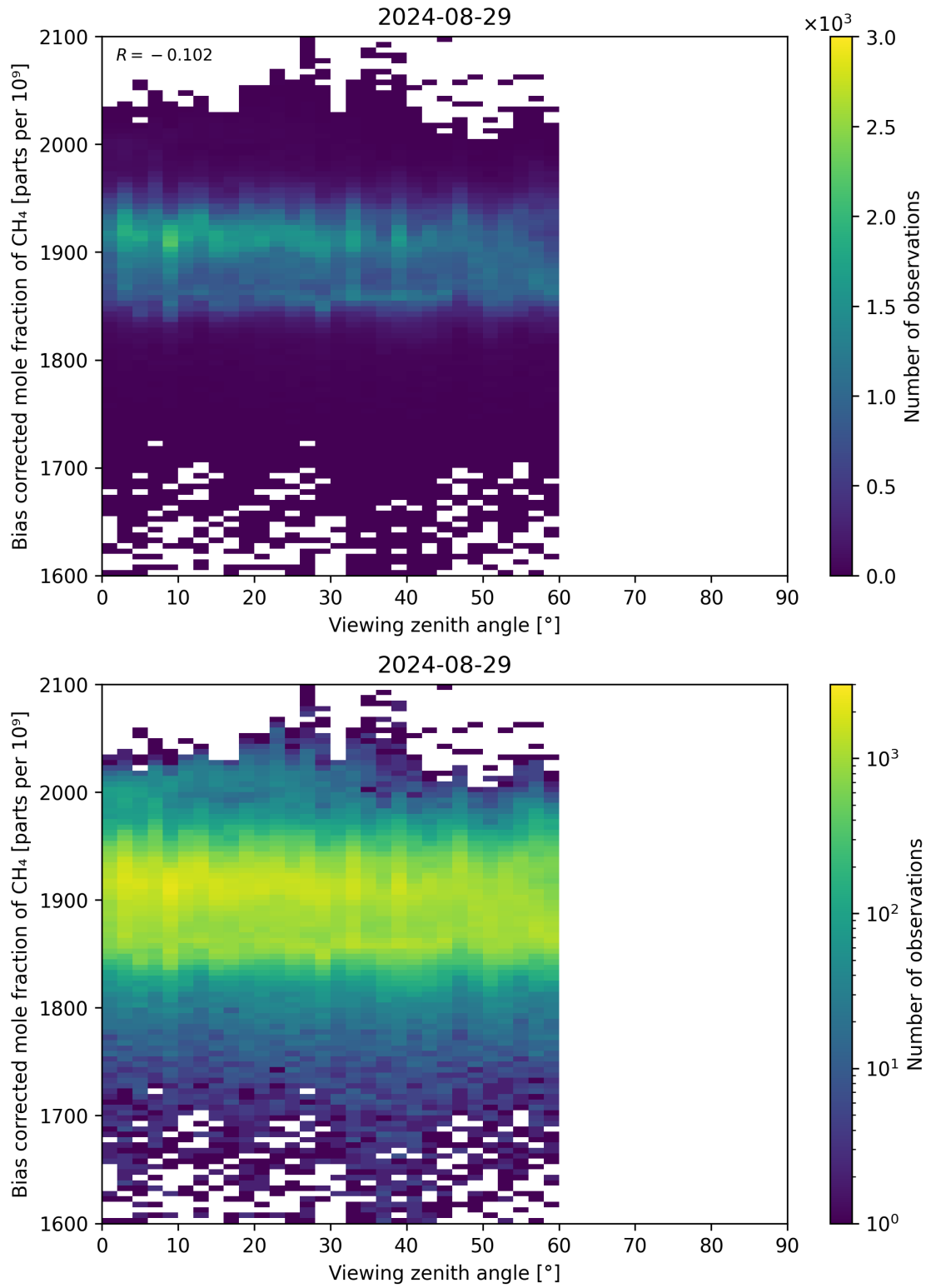
Figure 111: Scatter density plot of “Viewing zenith angle” against “Bias corrected mole fraction of CH 4 ” for 2024-08-28 to 2024-08-30.
