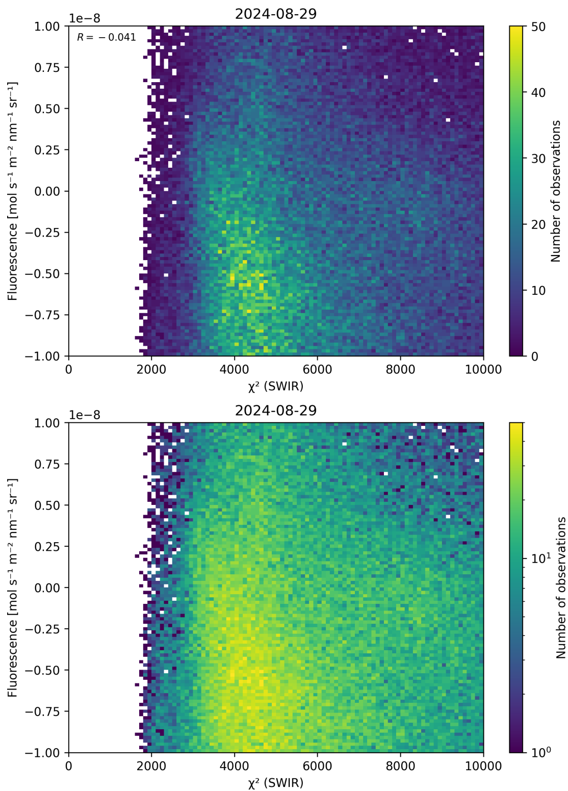
Figure 49: Scatter density plot of “ \chi^2 (SWIR)” against “Fluorescence” for 2024-08-28 to 2024-08-30.
