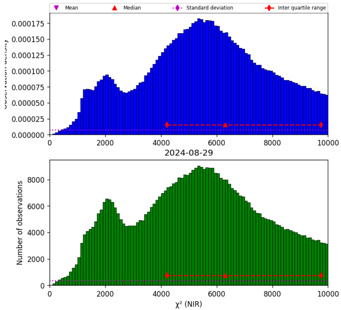
Figure 29: Histogram of “ \chi^2 (NIR)” for 2024-08-28 to 2024-08-30
