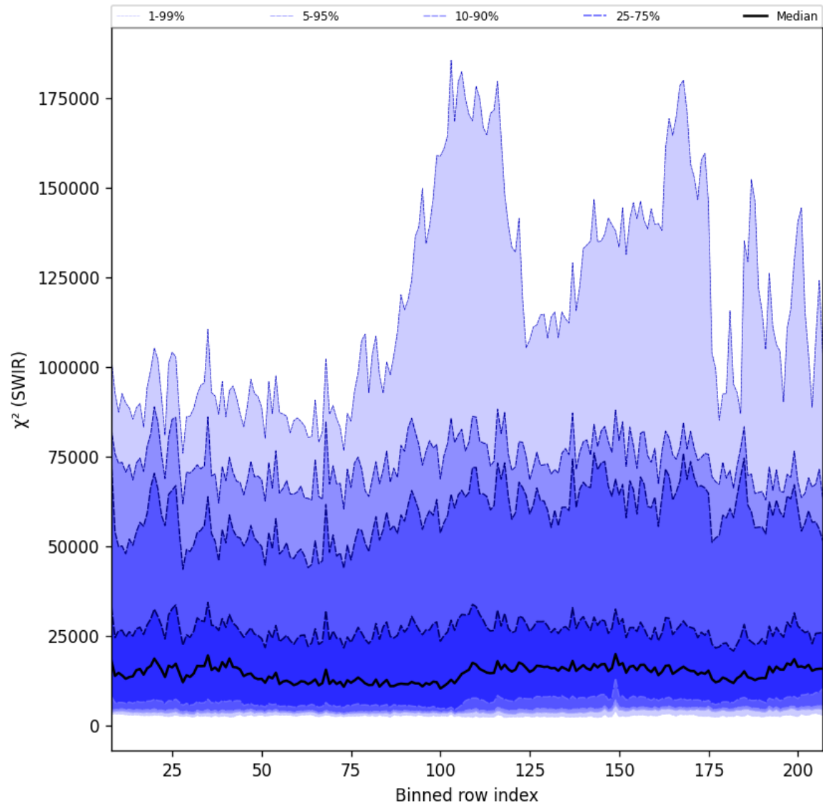
Figure 39: Along track statistics of “ \chi^2 (SWIR)” for 2024-08-28 to 2024-08-30
