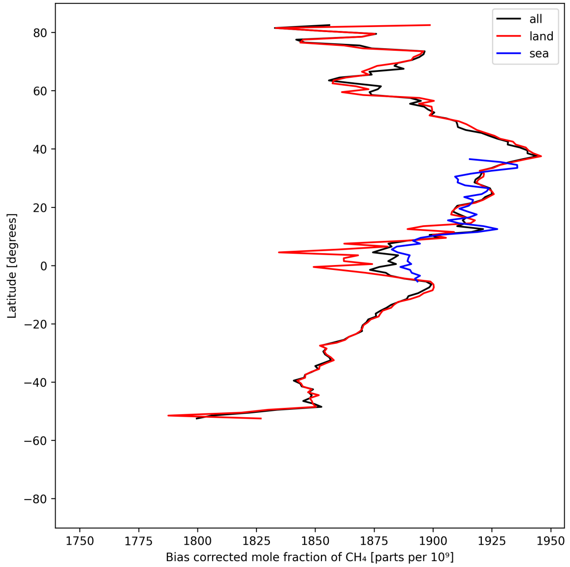
Figure 14: Zonal average of “Bias corrected mole fraction of CH 4 ” for 2024-08-28 to 2024-08-30.
