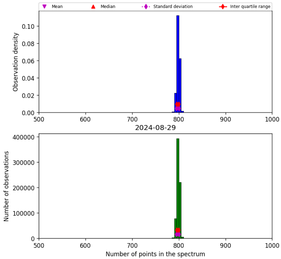
Figure 26: Histogram of “Number of points in the spectrum” for 2024-08-28 to 2024-08-30
