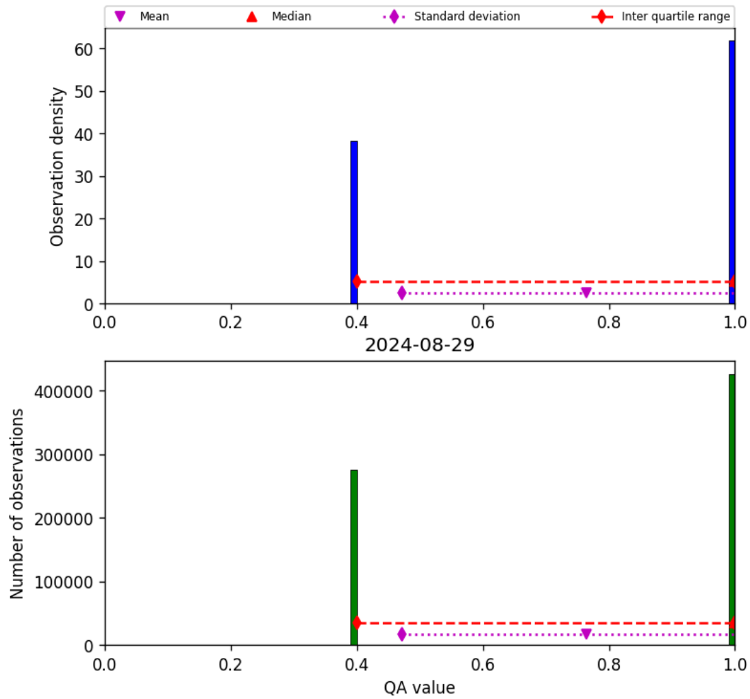
Figure 22: Histogram of “QA value” for 2024-08-28 to 2024-08-30
