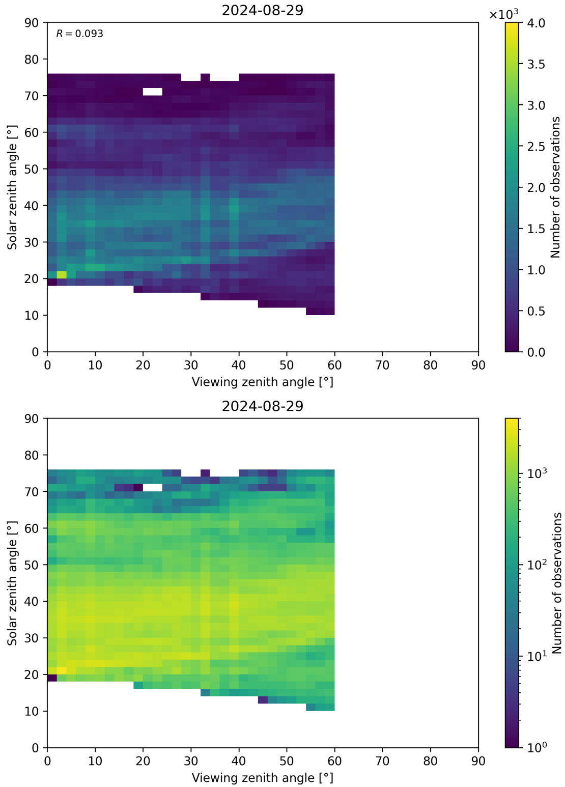
Figure 115: Scatter density plot of “Viewing zenith angle” against “Solar zenith angle” for 2024-08-28 to 2024-08-30.
