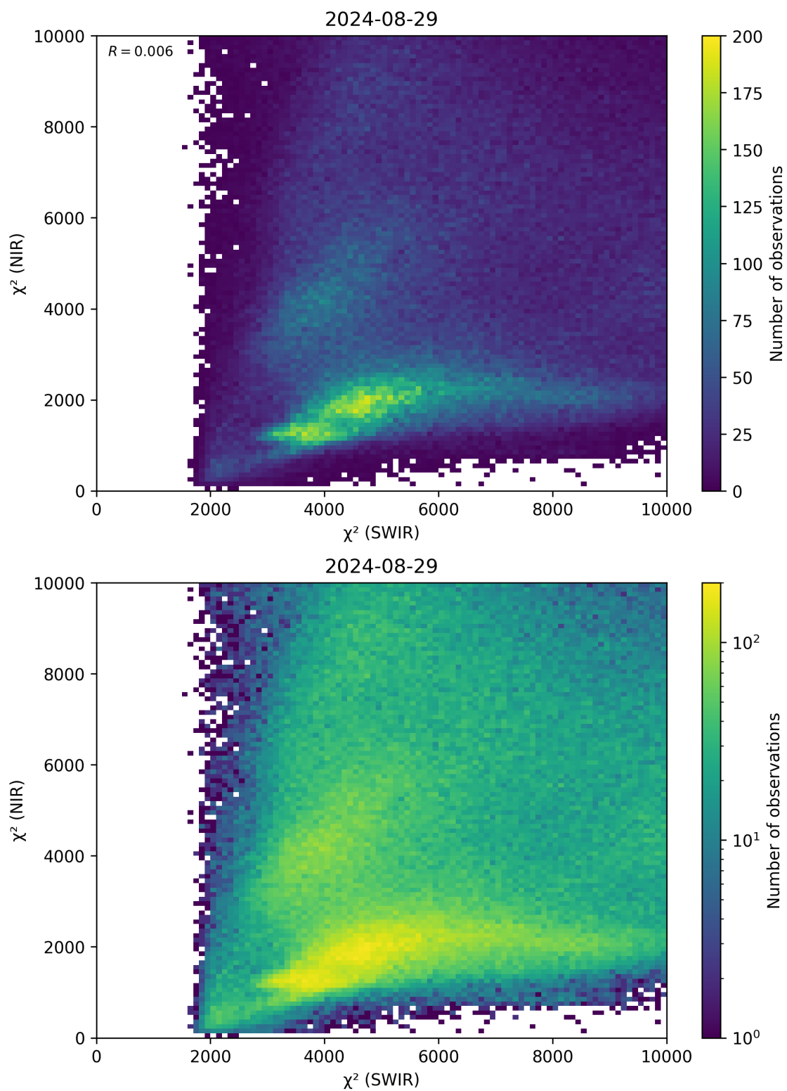
Figure 47: Scatter density plot of “ \chi^2 (SWIR)” against “ \chi^2 (NIR)” for 2024-08-28 to 2024-08-30.
