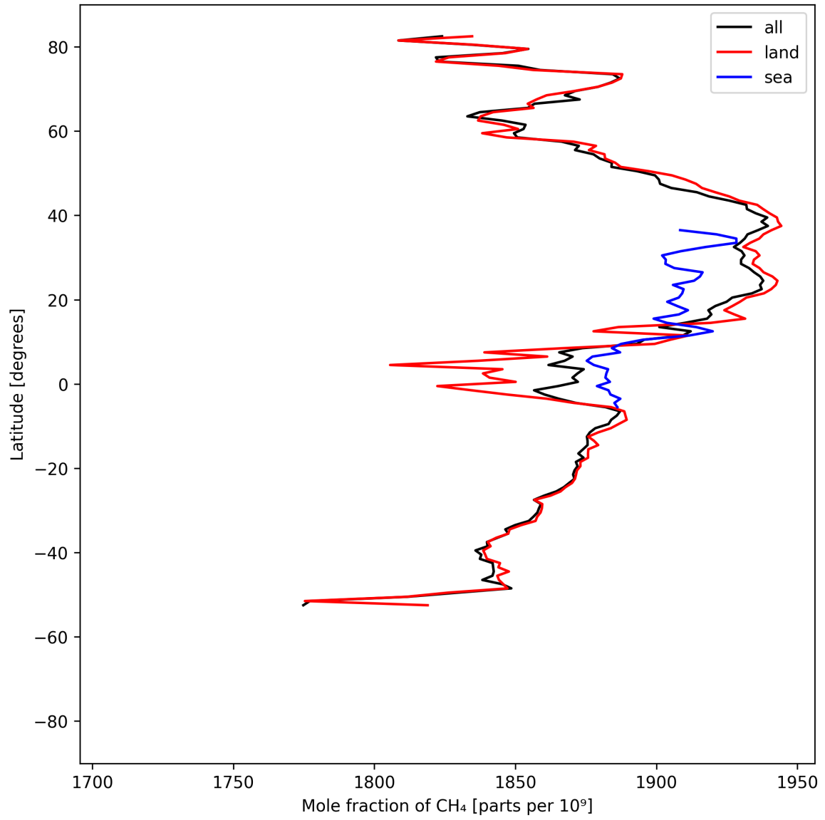
Figure 12: Zonal average of “Mole fraction of \text{CH}_4 ” for 2024-08-28 to 2024-08-30.
