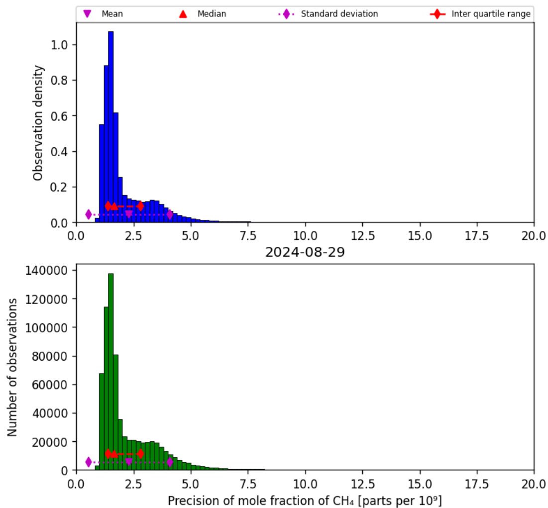
Figure 24: Histogram of “Precision of mole fraction of CH 4 ” for 2024-08-28 to 2024-08-30
