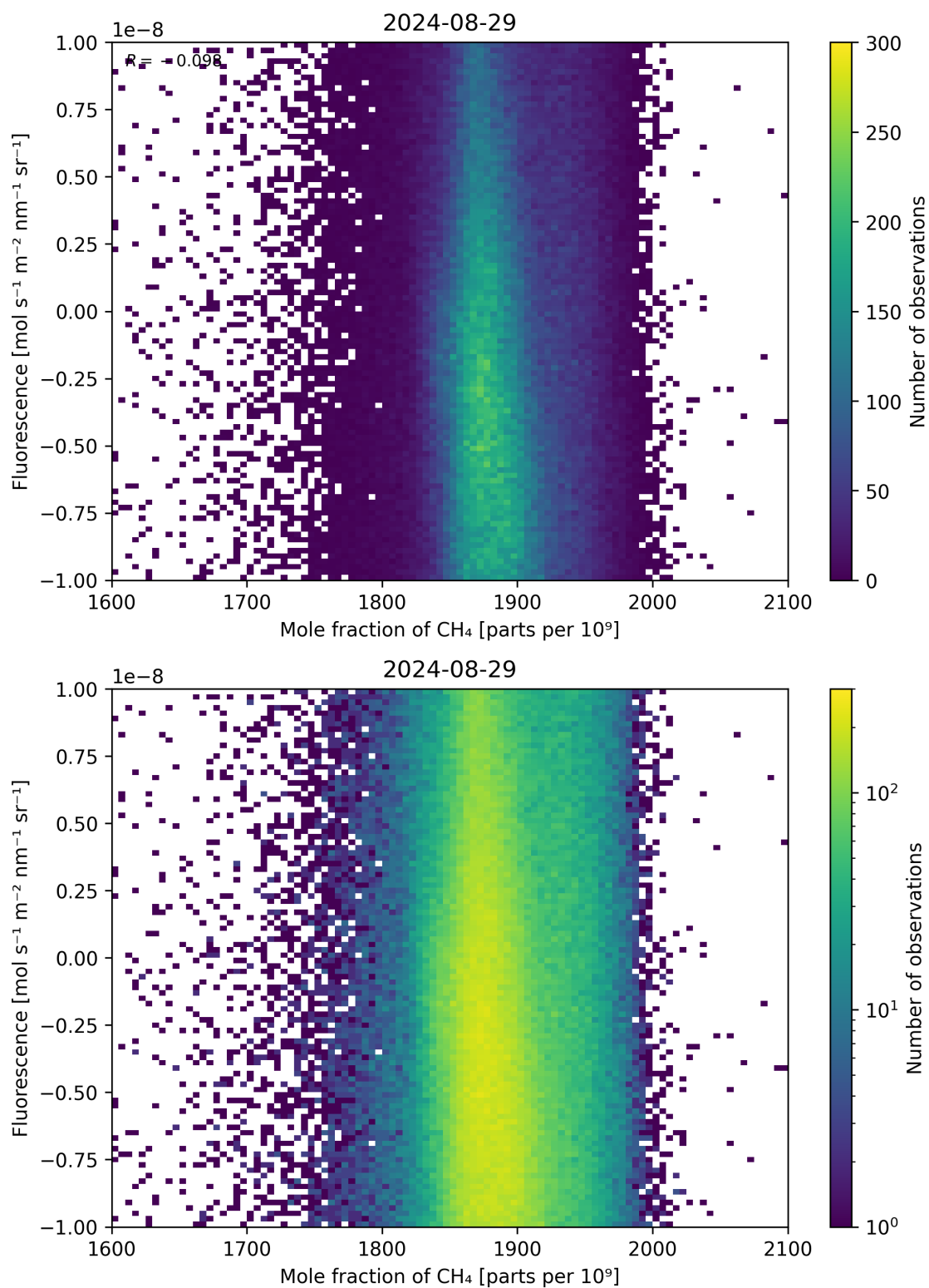
Figure 73: Scatter density plot of “Mole fraction of CH 4 ” against “Fluorescence” for 2024-08-28 to 2024-08-30.
