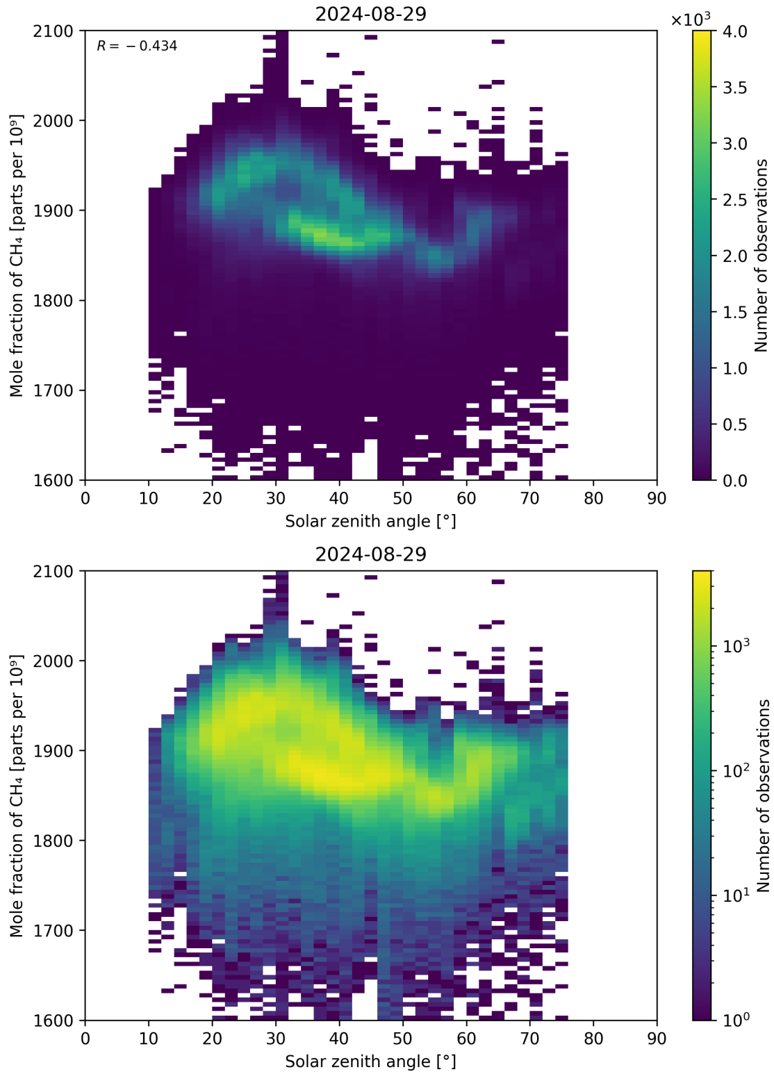
Figure 99: Scatter density plot of “Solar zenith angle” against “Mole fraction of CH 4 ” for 2024-08-28 to 2024-08-30.
