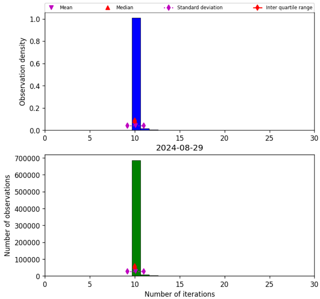
Figure 31: Histogram of “Number of iterations” for 2024-08-28 to 2024-08-30
