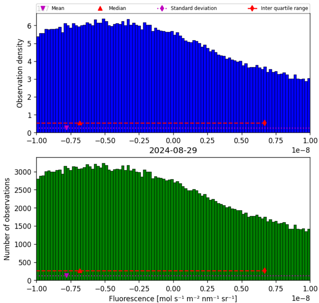
Figure 32: Histogram of “Fluorescence” for 2024-08-28 to 2024-08-30
