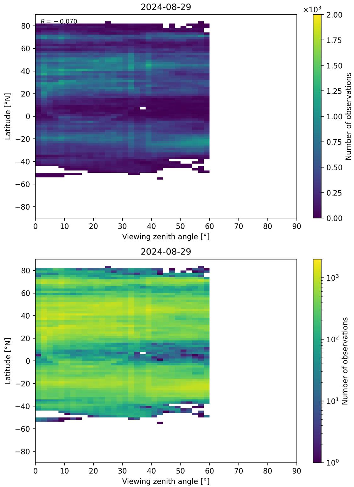
Figure 109: Scatter density plot of “Viewing zenith angle” against “Latitude” for 2024-08-28 to 2024-08-30.
