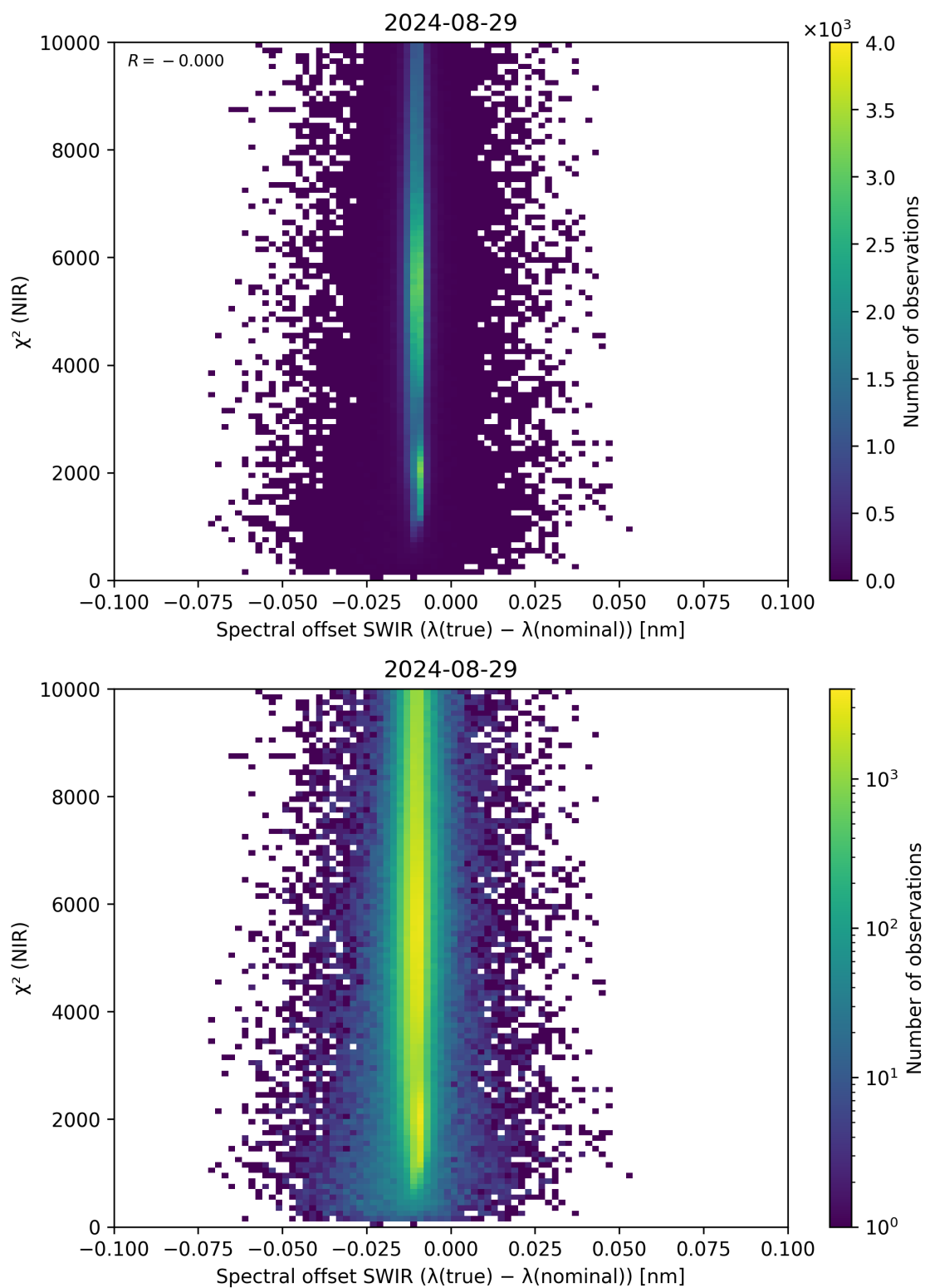
Figure 117: Scatter density plot of “Spectral offset SWIR ( \lambda_{\text{true}} - \lambda_{\text{nominal}} )” against “ \chi^2 (NIR)” for 2024-08-28 to 2024-08-30.
