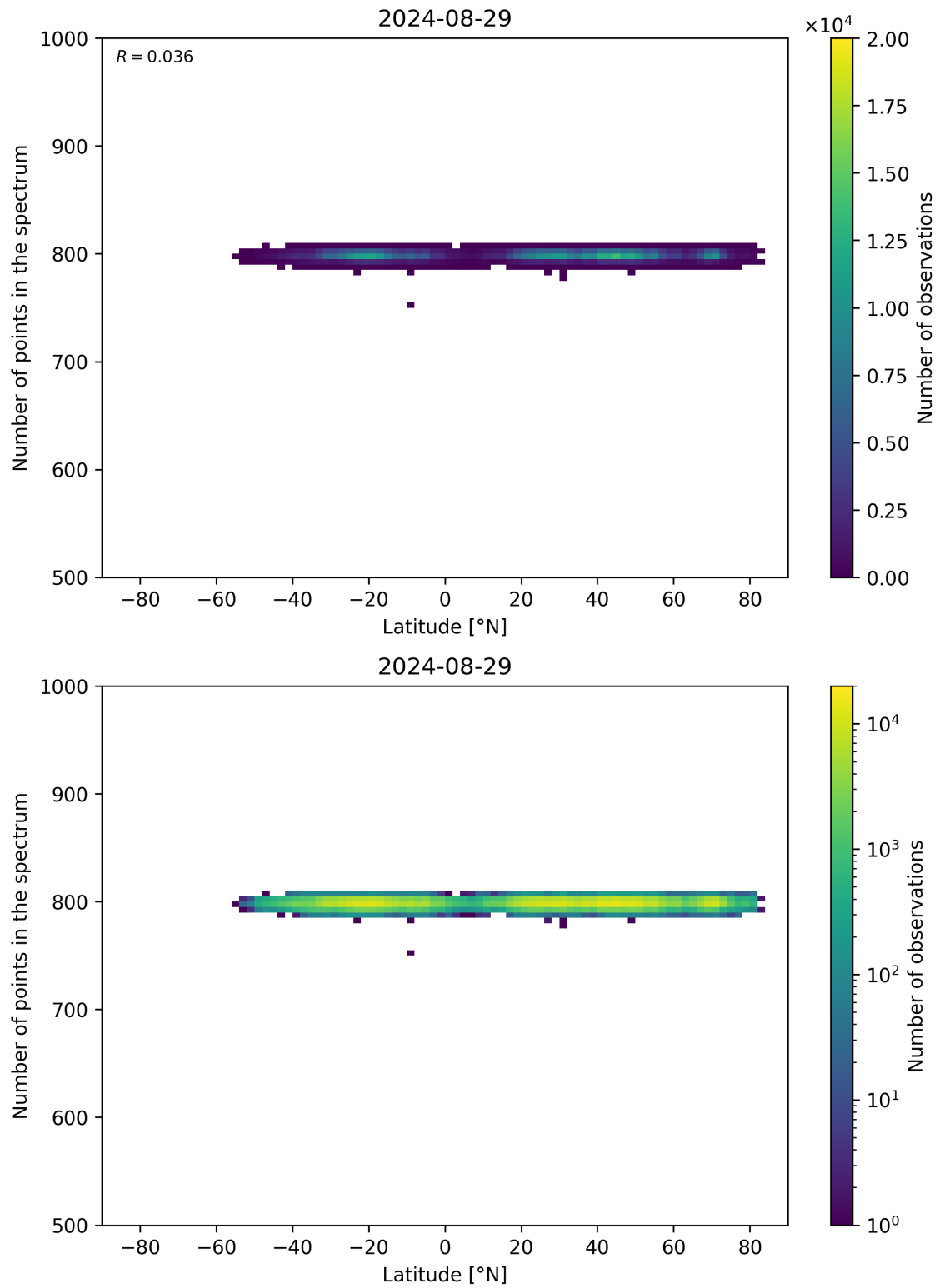
Figure 61: Scatter density plot of “Latitude” against “Number of points in the spectrum” for 2024-08-28 to 2024-08-30.
