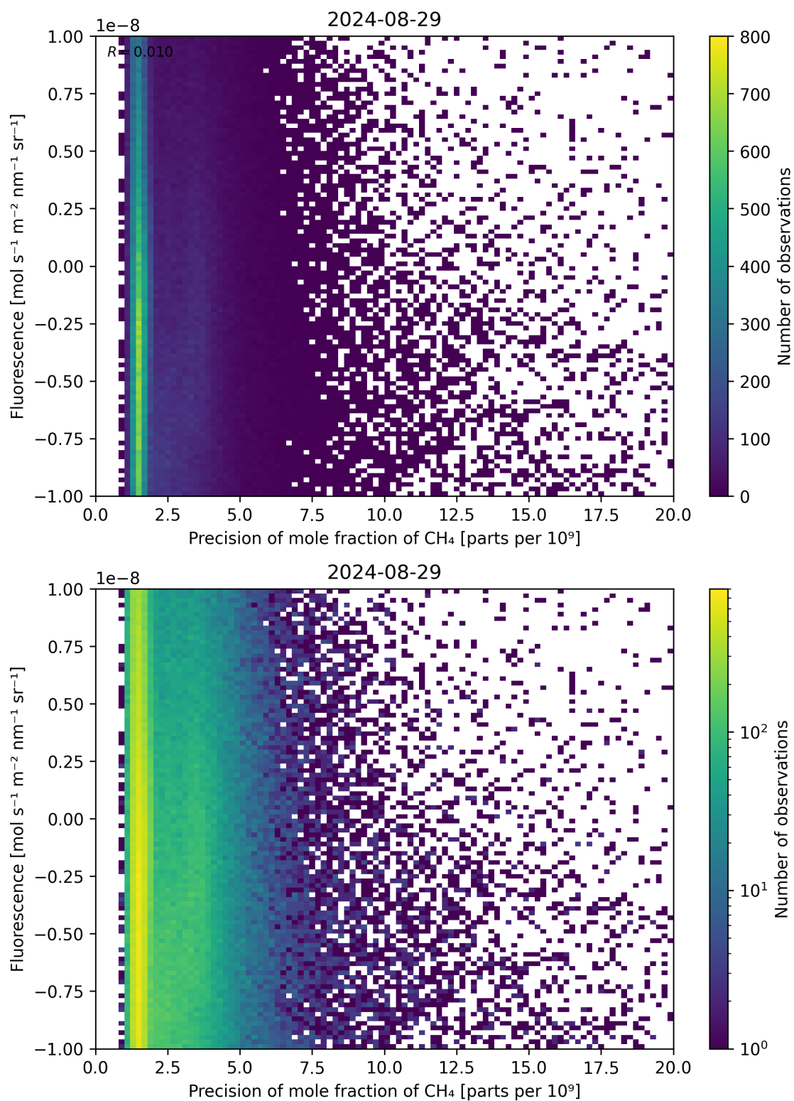
Figure 81: Scatter density plot of “Precision of mole fraction of \text{CH}_4 ” against “Fluorescence” for 2024-08-28 to 2024-08-30.
