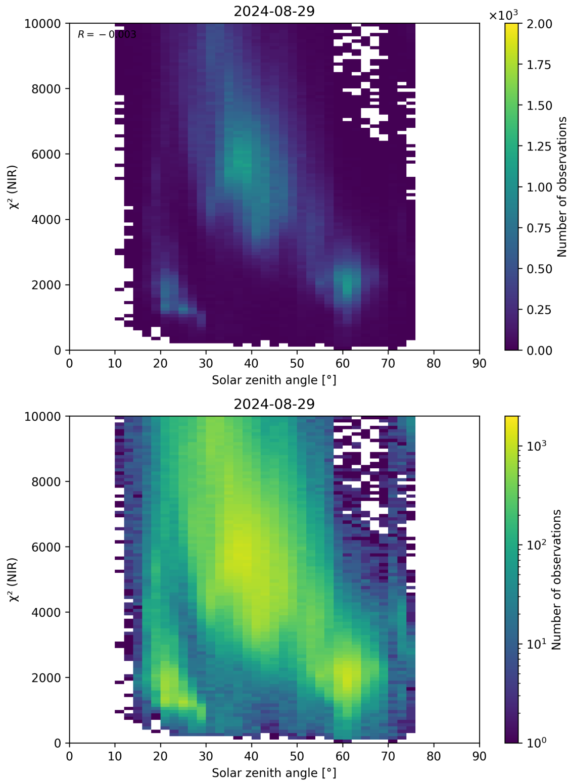
Figure 94: Scatter density plot of “Solar zenith angle” against “ \chi^2 (NIR)” for 2024-08-28 to 2024-08-30.
