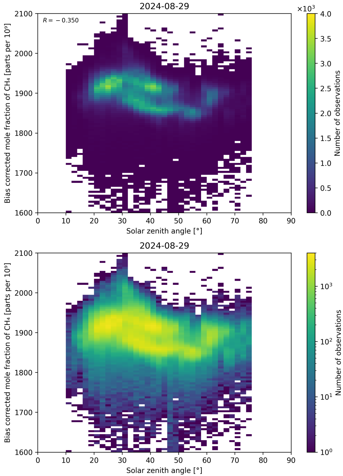
Figure 100: Scatter density plot of “Solar zenith angle” against “Bias corrected mole fraction of CH 4 ” for 2024-08-28 to 2024-08-30.
