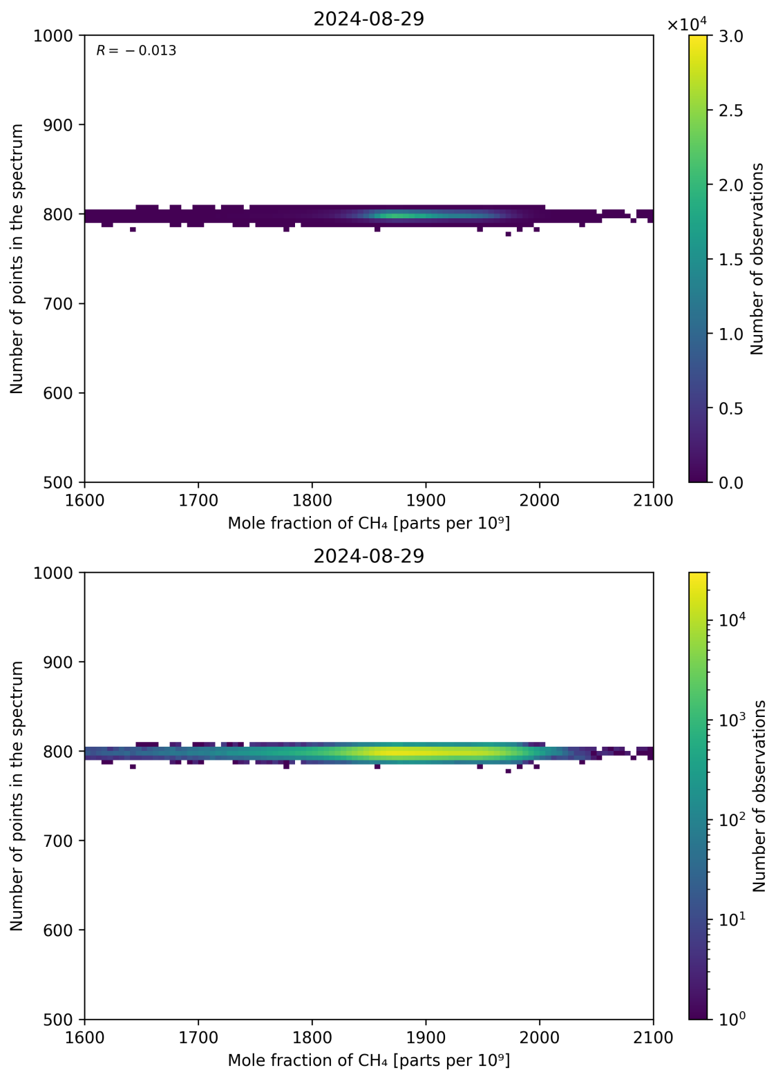
Figure 77: Scatter density plot of “Mole fraction of CH 4 ” against “Number of points in the spectrum” for 2024-08-28 to 2024-08-30.
