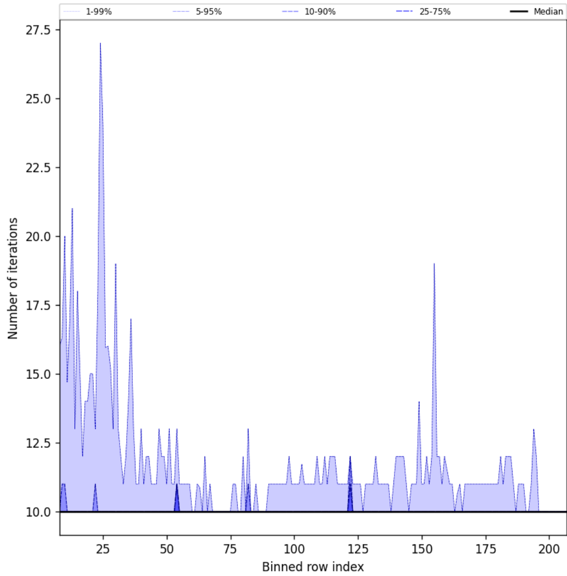
Figure 42: Along track statistics of “Number of iterations” for 2024-08-28 to 2024-08-30
