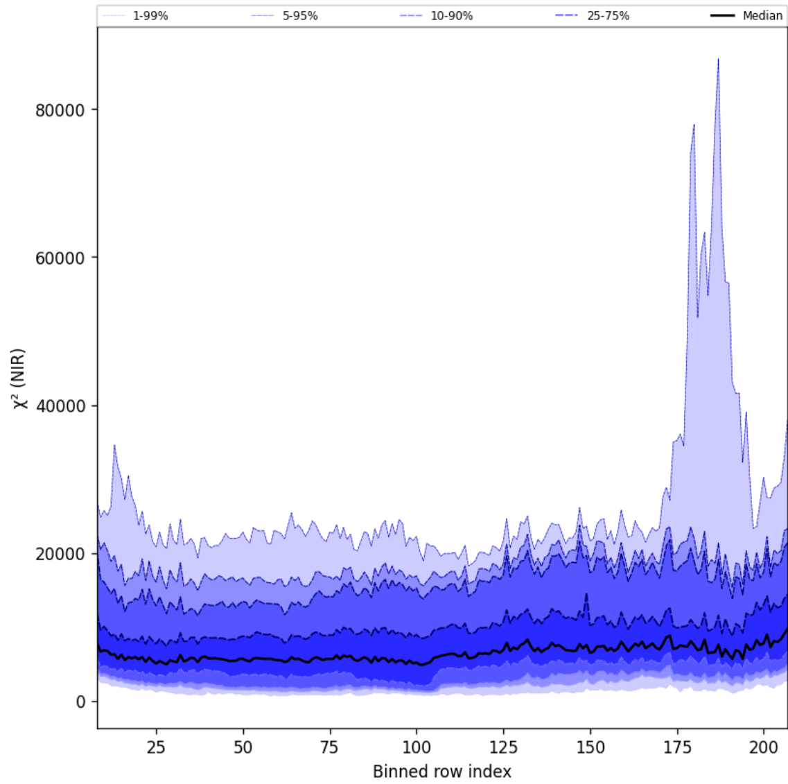
Figure 40: Along track statistics of “ \chi^2 (NIR)” for 2024-08-28 to 2024-08-30
