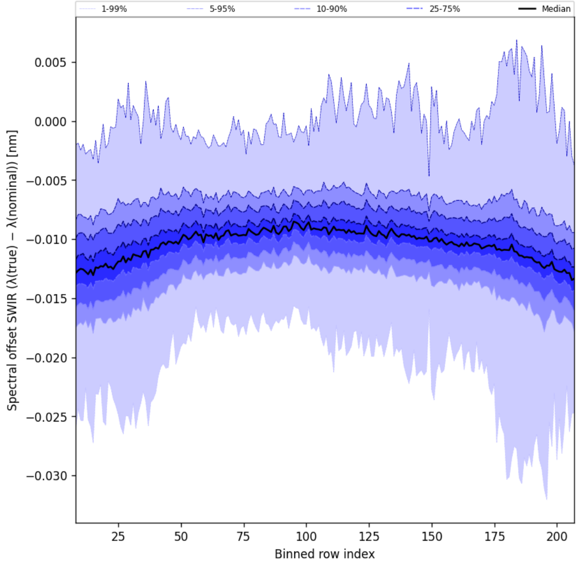
Figure 38: Along track statistics of “Spectral offset SWIR ( \lambda_{\text{true}} - \lambda_{\text{nominal}} )” for 2024-08-28 to 2024-08-30
