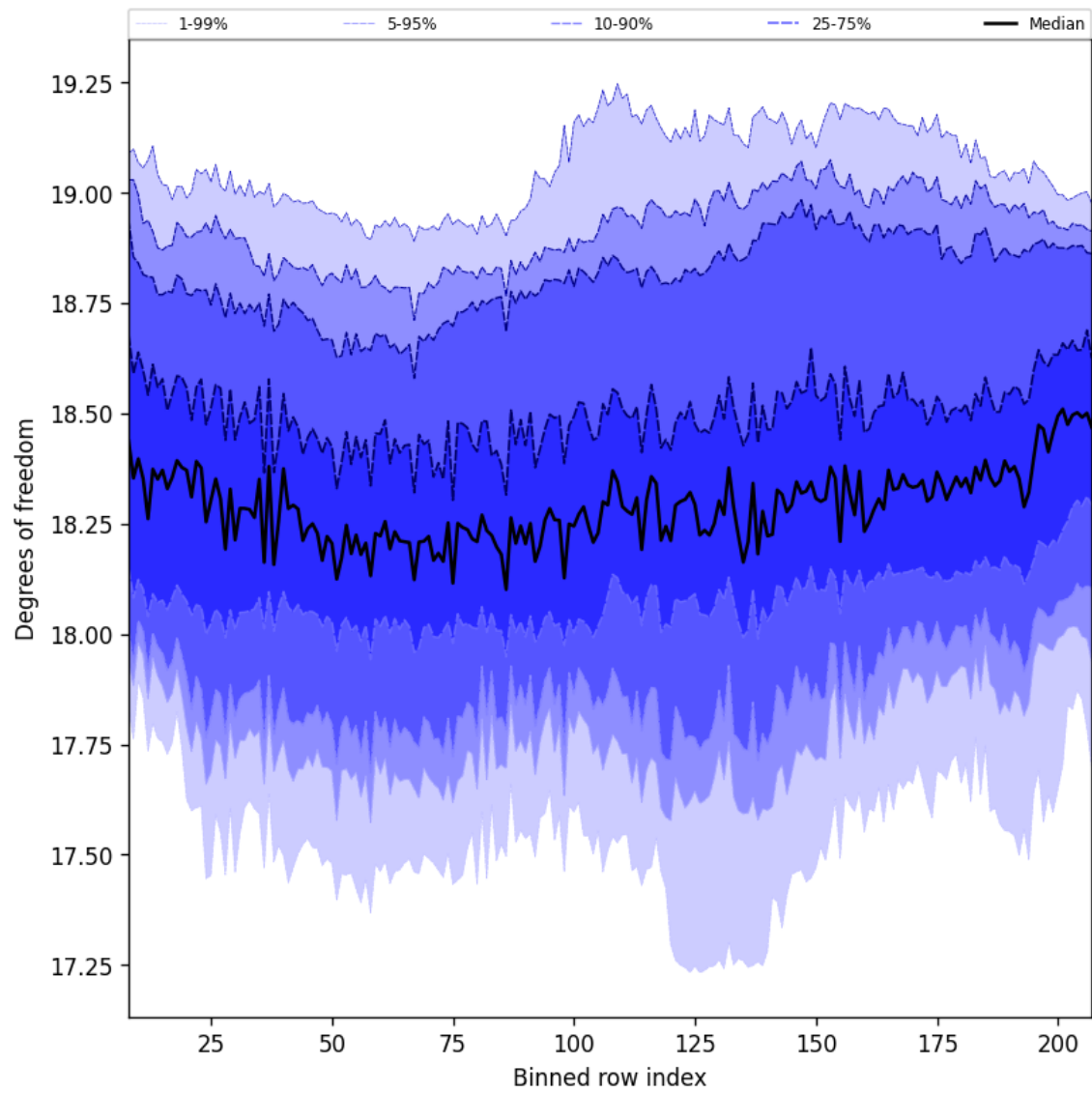
Figure 41: Along track statistics of “Degrees of freedom” for 2024-08-28 to 2024-08-30
