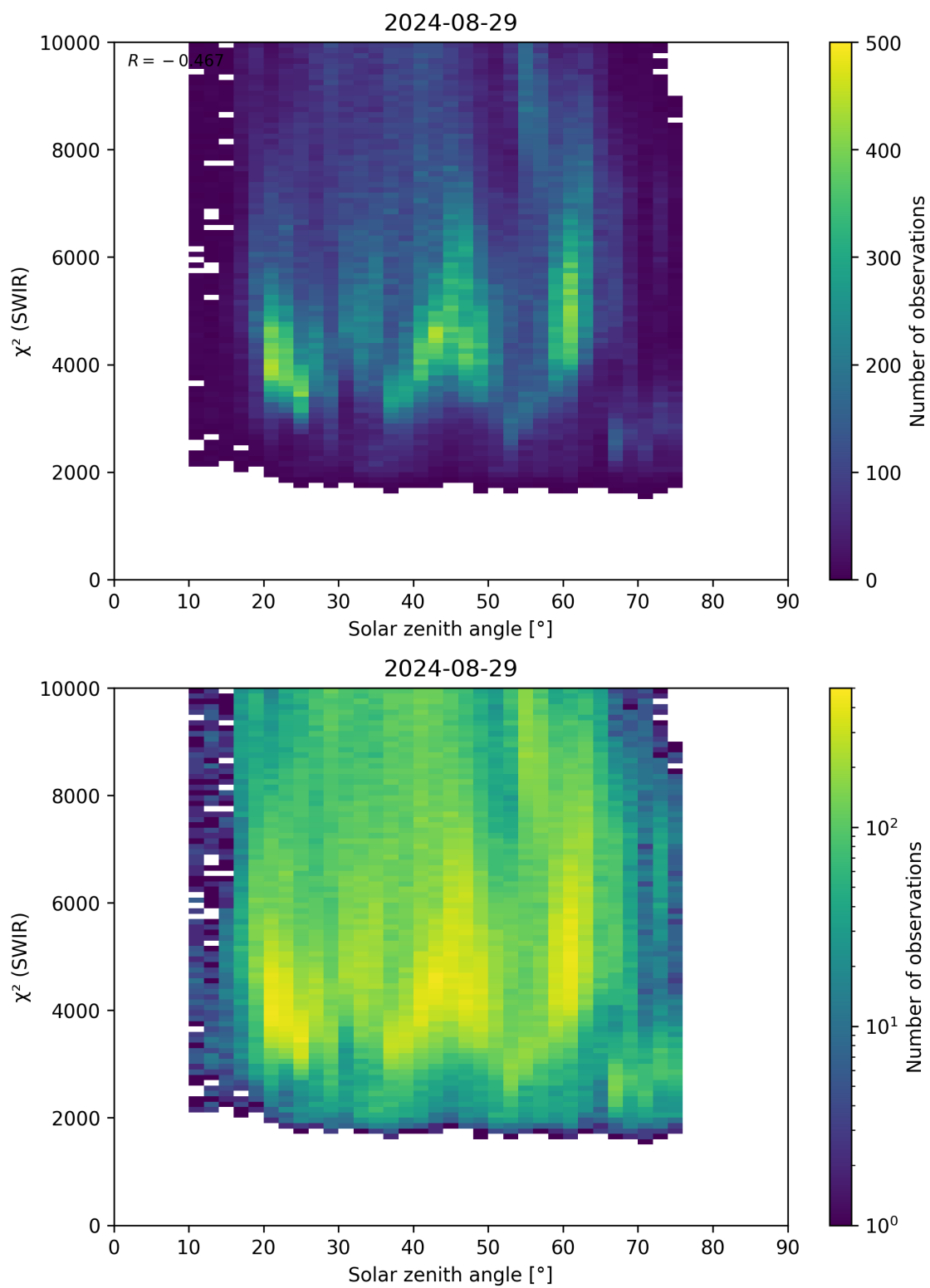
Figure 95: Scatter density plot of “Solar zenith angle” against “ \chi^2 (SWIR)” for 2024-08-28 to 2024-08-30.
