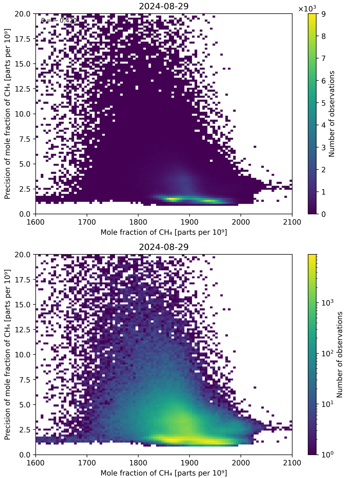
Figure 75: Scatter density plot of “Mole fraction of CH 4 ” against “Precision of mole fraction of CH 4 ” for 2024-08-28 to 2024-08-30.
