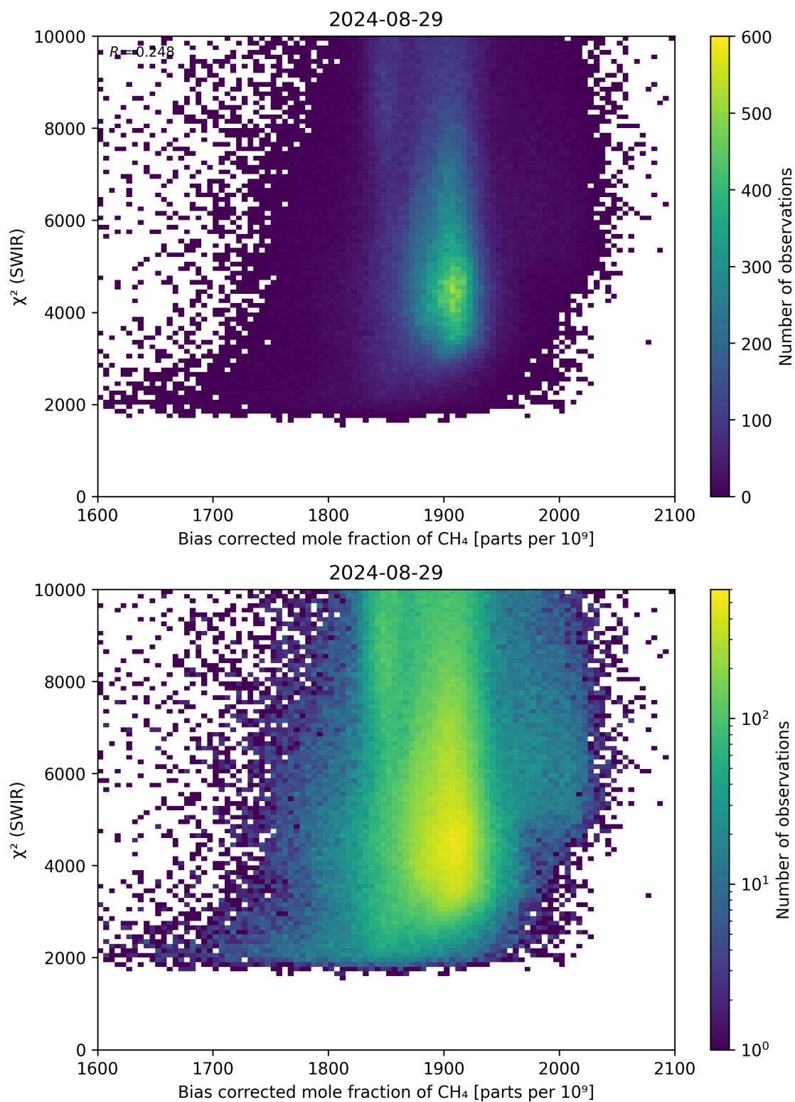
Figure 64: Scatter density plot of “Bias corrected mole fraction of \text{CH}_4 ” against “ \chi^2 (SWIR)” for 2024-08-28 to 2024-08-30.
