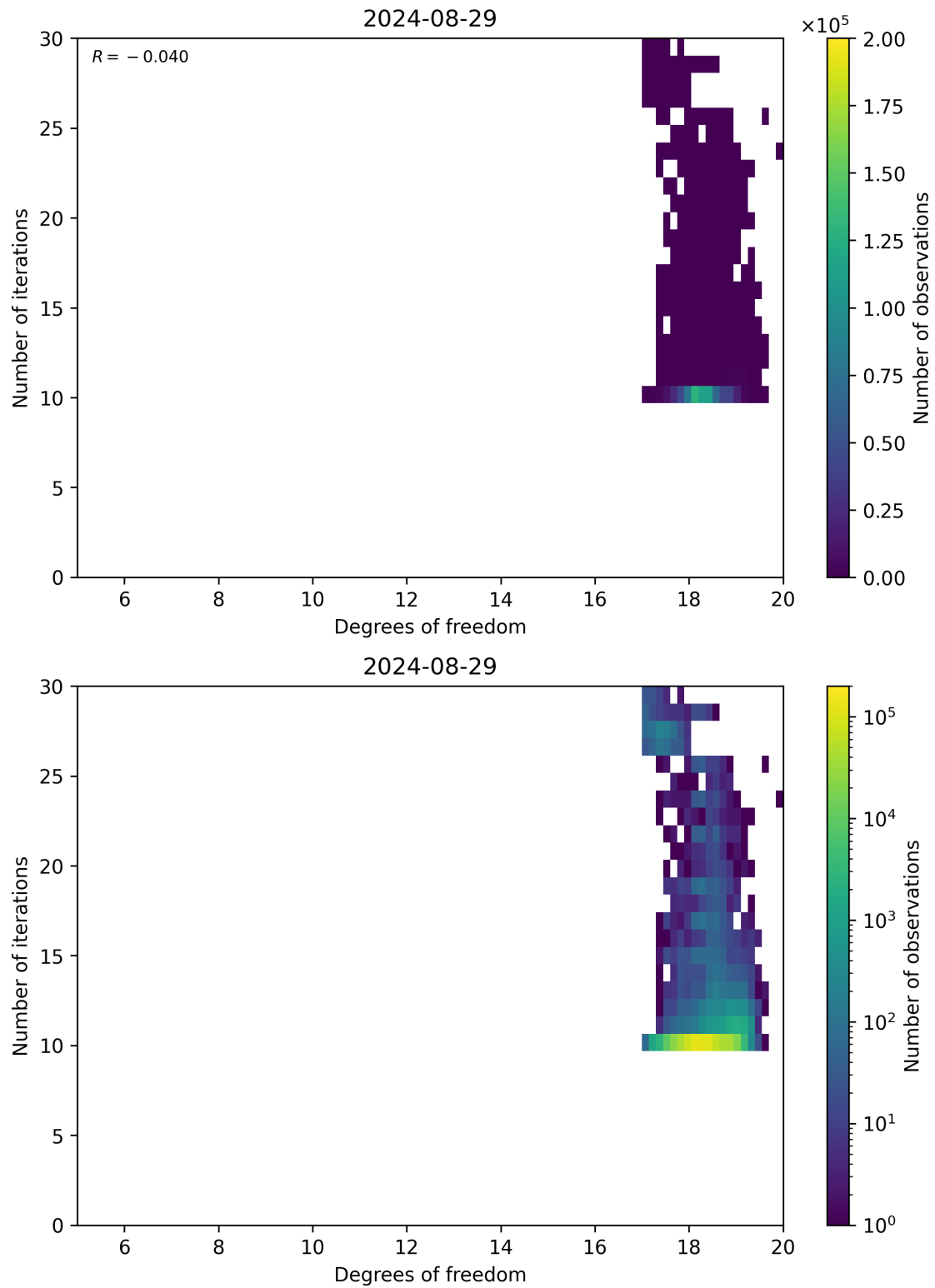
Figure 52: Scatter density plot of “Degrees of freedom” against “Number of iterations” for 2024-08-28 to 2024-08-30.
