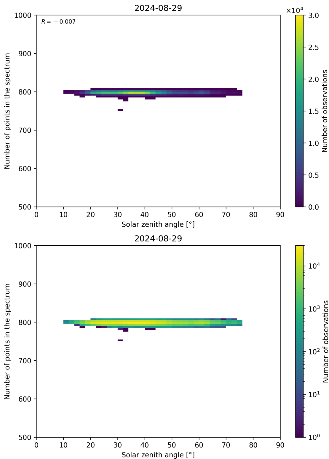
Figure 103: Scatter density plot of “Solar zenith angle” against “Number of points in the spectrum” for 2024-08-28 to 2024-08-30.
