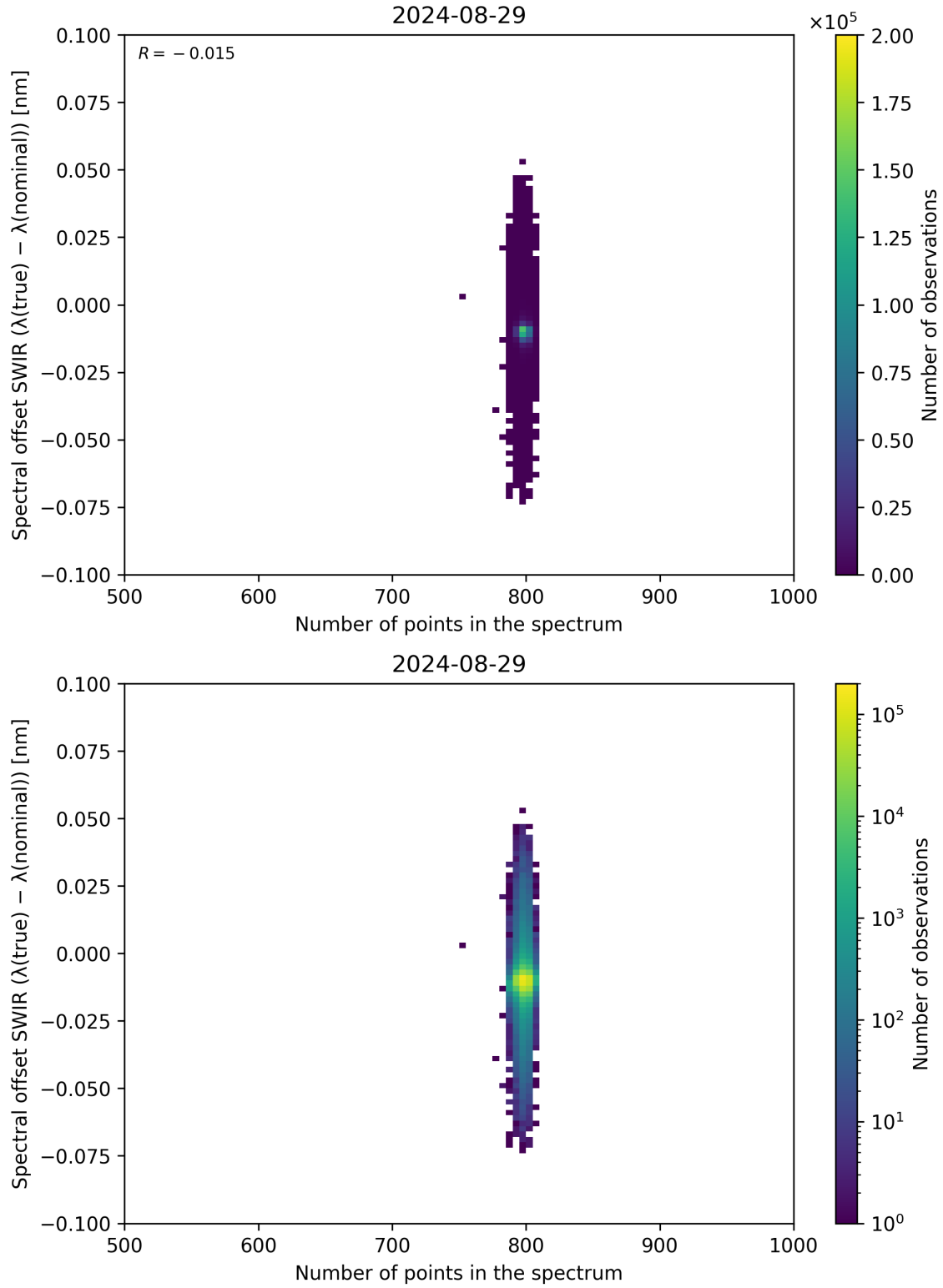
Figure 93: Scatter density plot of “Number of points in the spectrum” against “Spectral offset SWIR ( \lambda_{\text{true}} - \lambda_{\text{nominal}} )” for 2024-08-28 to 2024-08-30.
