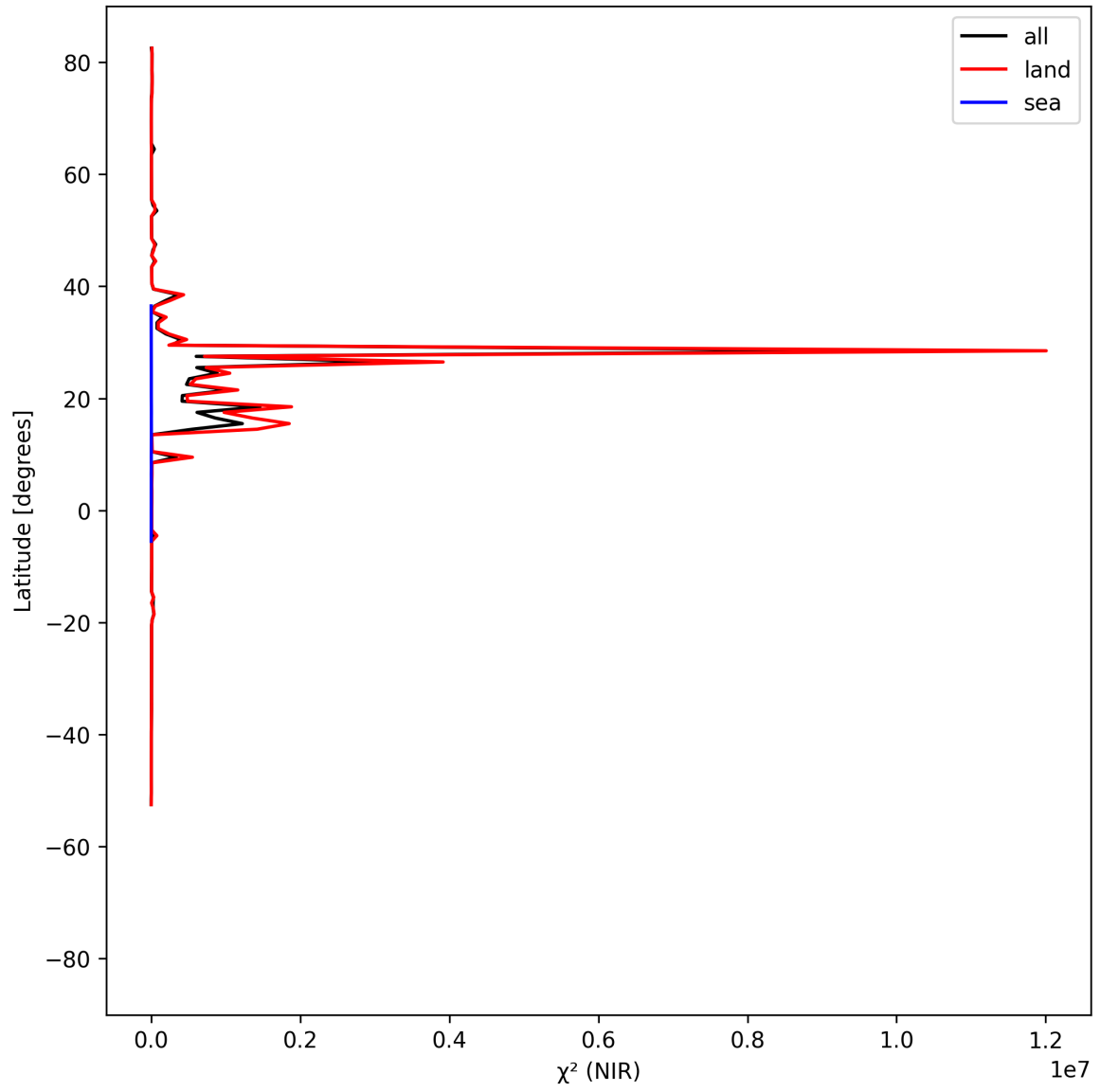
Figure 18: Zonal average of “ \chi^2 (NIR)” for 2024-08-28 to 2024-08-30.
