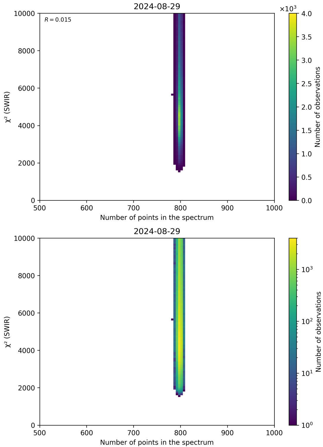
Figure 89: Scatter density plot of “Number of points in the spectrum” against “ \chi^2 (SWIR)” for 2024-08-28 to 2024-08-30.
