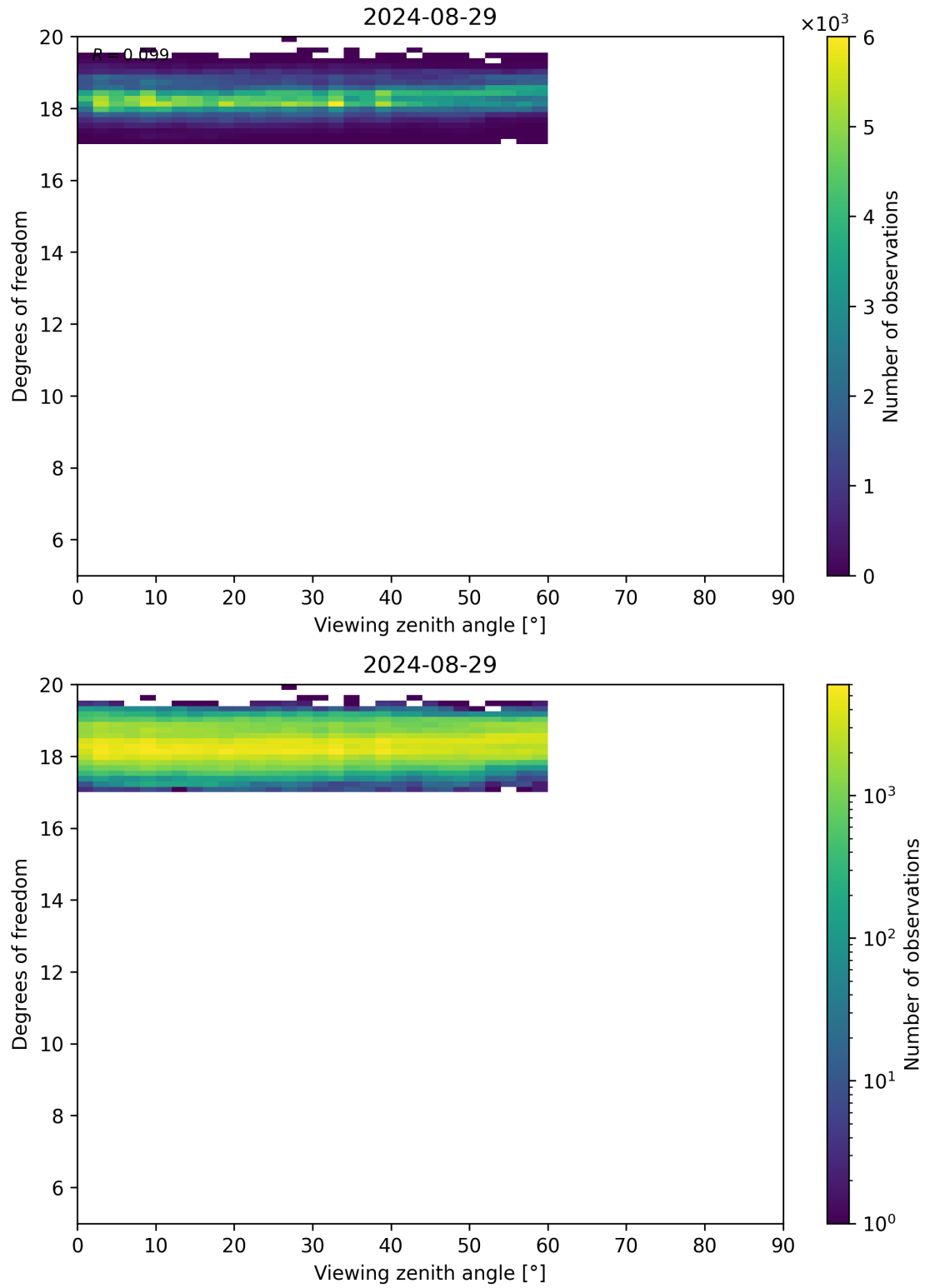
Figure 107: Scatter density plot of “Viewing zenith angle” against “Degrees of freedom” for 2024-08-28 to 2024-08-30.
