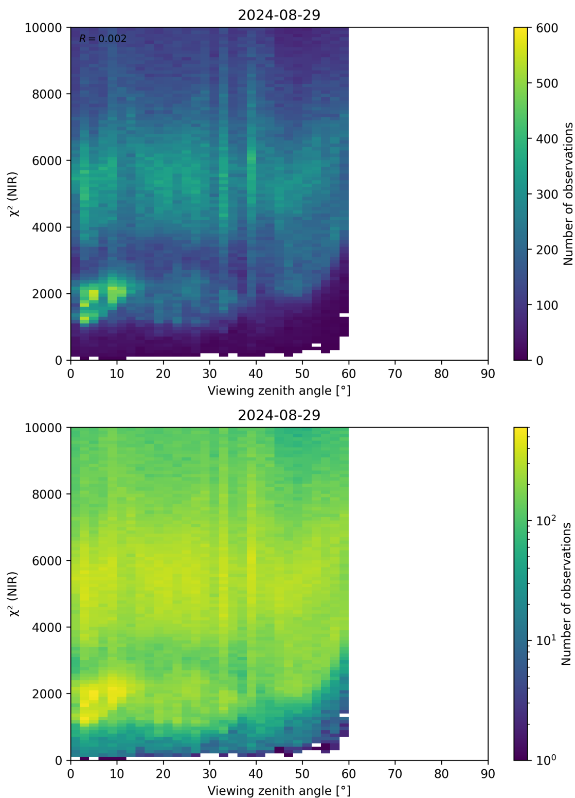
Figure 105: Scatter density plot of “Viewing zenith angle” against “ \chi^2 (NIR)” for 2024-08-28 to 2024-08-30.
