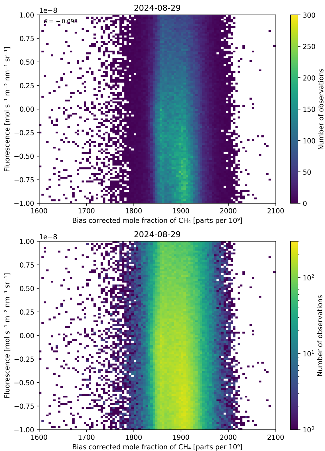
Figure 66: Scatter density plot of “Bias corrected mole fraction of \text{CH}_4 ” against “Fluorescence” for 2024-08-28 to 2024-08-30.
