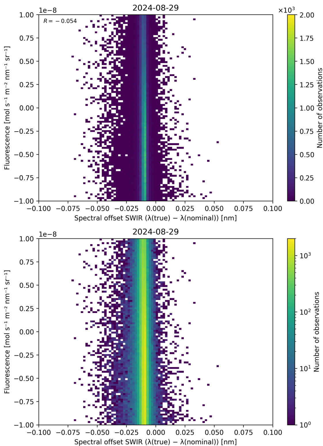
Figure 120: Scatter density plot of “Spectral offset SWIR ( \lambda_{\text{true}} - \lambda_{\text{nominal}} )” against “Fluorescence” for 2024-08-28 to 2024-08-30.
