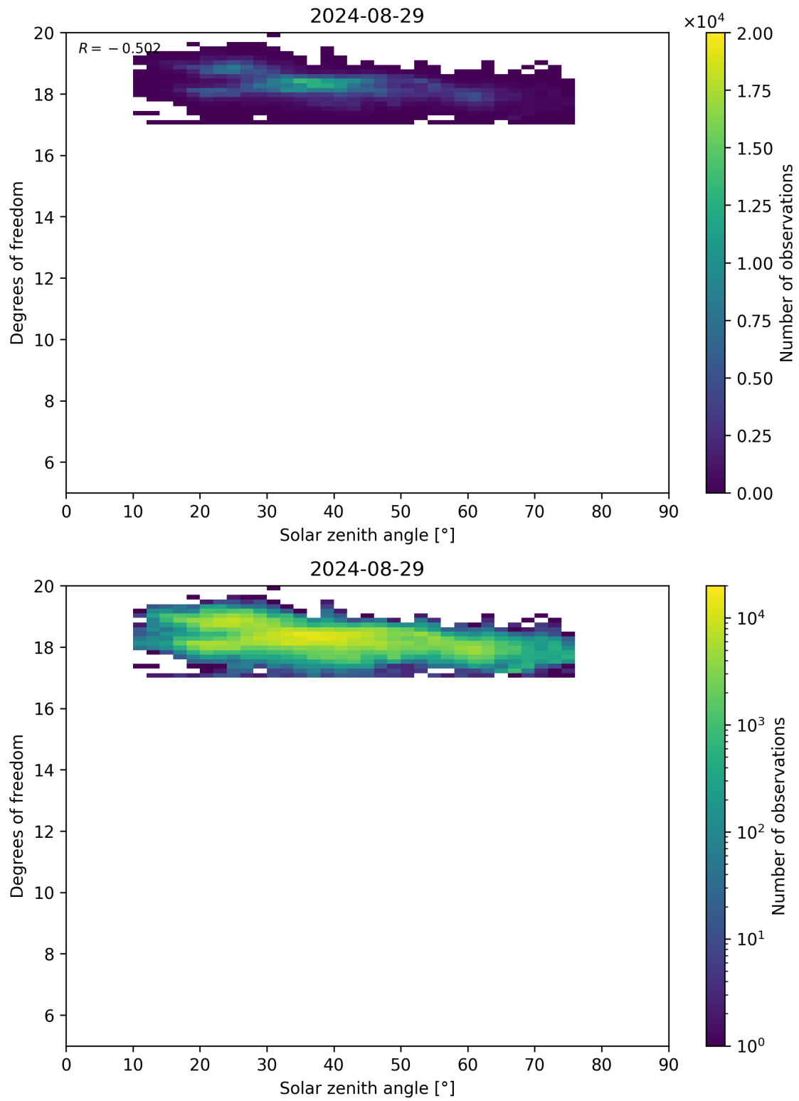
Figure 96: Scatter density plot of “Solar zenith angle” against “Degrees of freedom” for 2024-08-28 to 2024-08-30.
