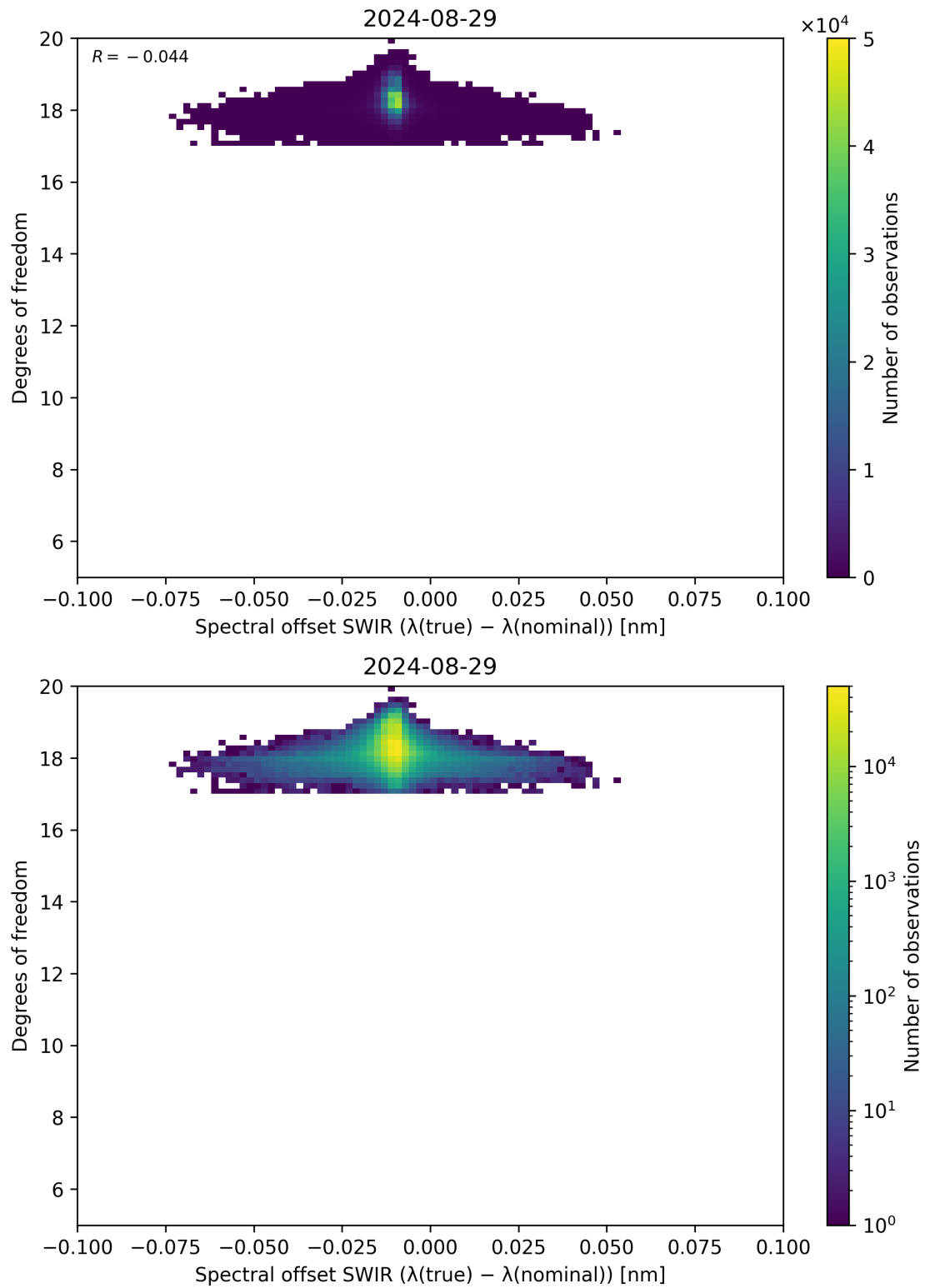
Figure 119: Scatter density plot of “Spectral offset SWIR ( \lambda_{\text{true}} - \lambda_{\text{nominal}} )” against “Degrees of freedom” for 2024-08-28 to 2024-08-30.
