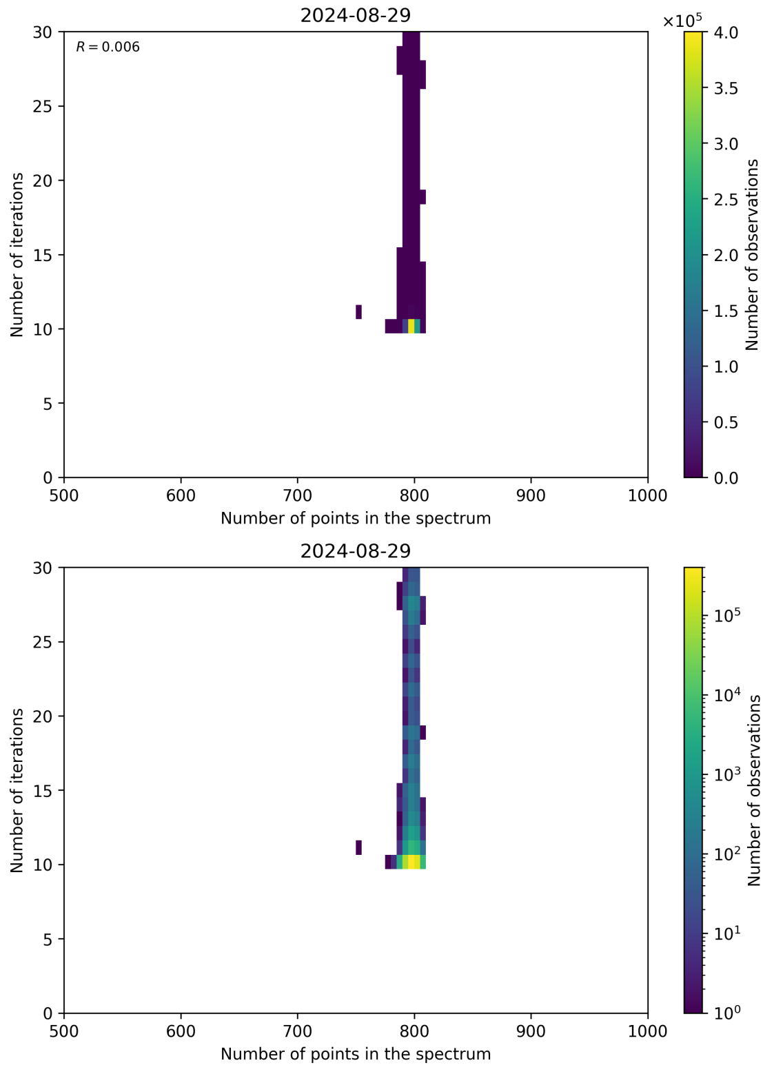
Figure 92: Scatter density plot of “Number of points in the spectrum” against “Number of iterations” for 2024-08-28 to 2024-08-30.
