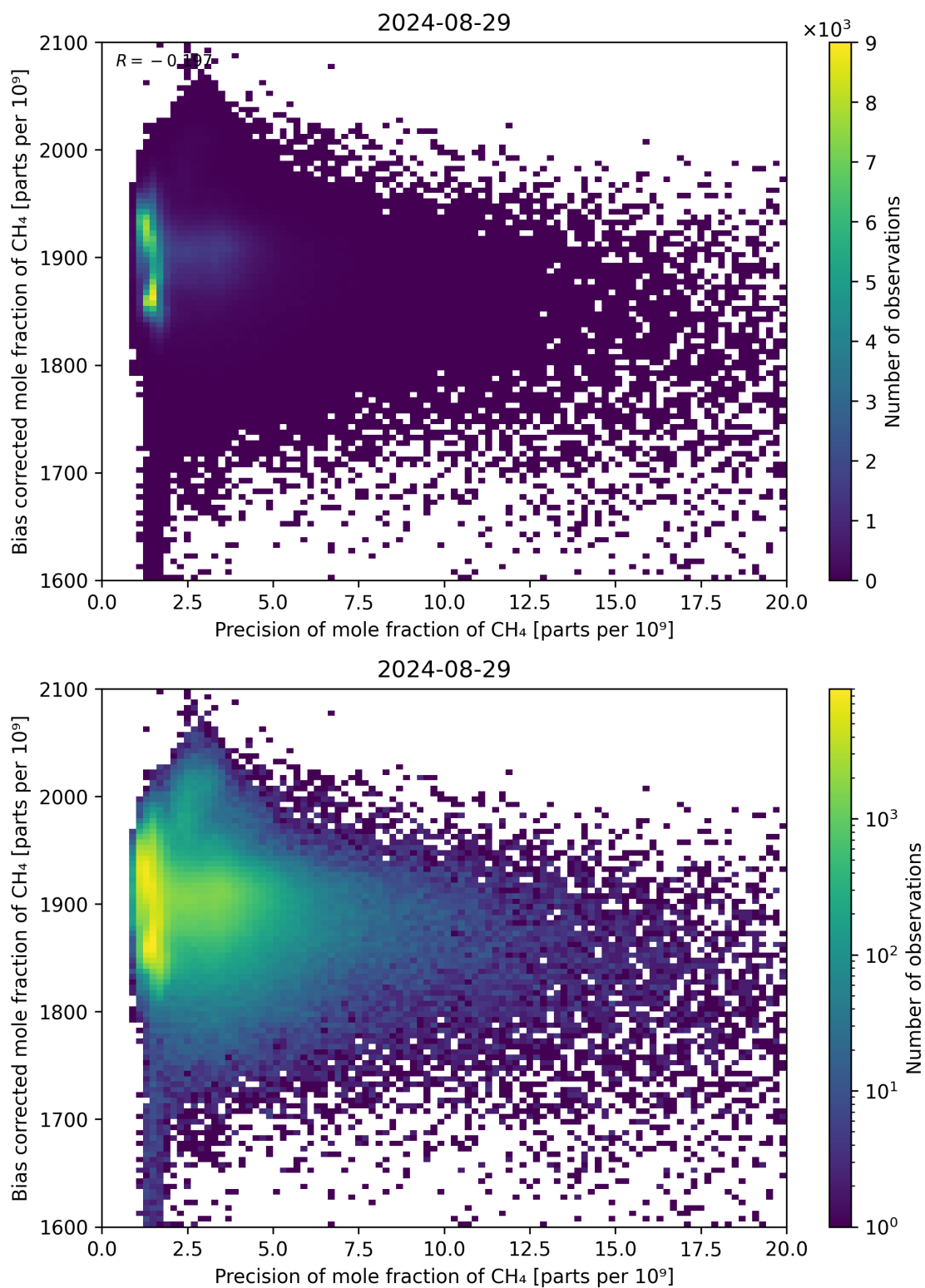
Figure 82: Scatter density plot of “Precision of mole fraction of CH 4 ” against “Bias corrected mole fraction of CH 4 ” for 2024-08-28 to 2024-08-30.
