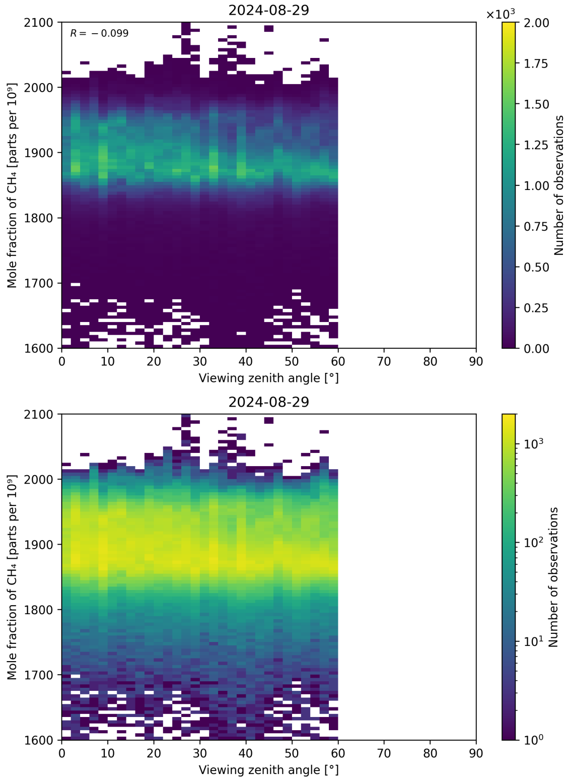
Figure 110: Scatter density plot of “Viewing zenith angle” against “Mole fraction of CH 4 ” for 2024-08-28 to 2024-08-30.
