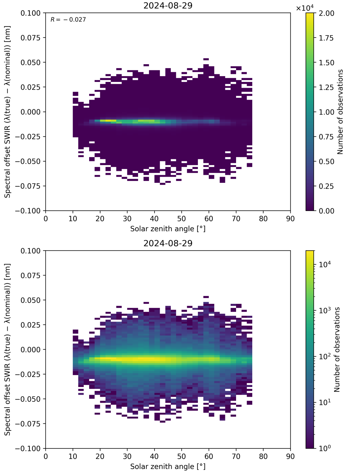
Figure 104: Scatter density plot of “Solar zenith angle” against “Spectral offset SWIR ( \lambda_{\text{true}} - \lambda_{\text{nominal}} )” for 2024-08-28 to 2024-08-30.
