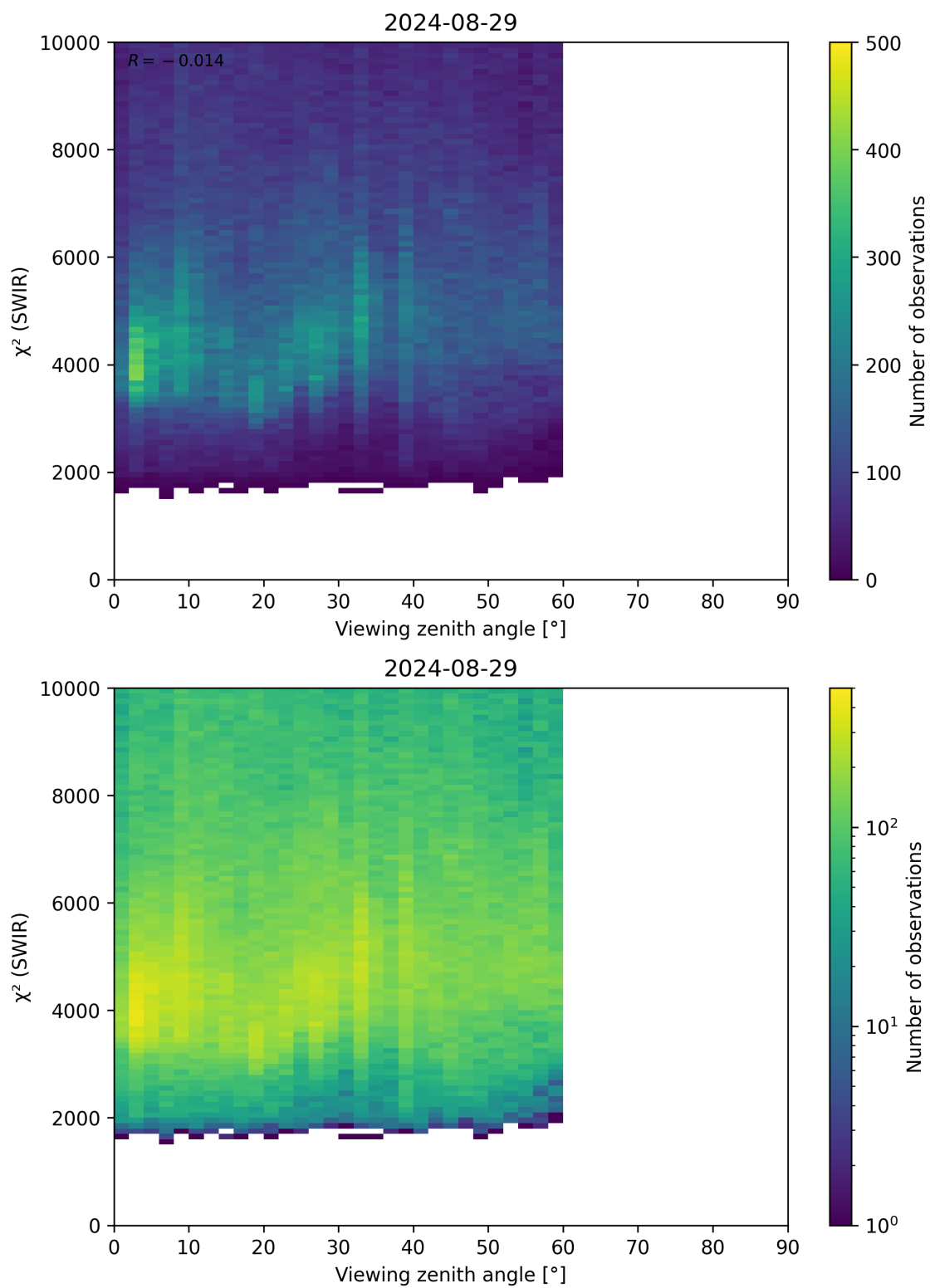
Figure 106: Scatter density plot of “Viewing zenith angle” against “ \chi^2 (SWIR)” for 2024-08-28 to 2024-08-30.
