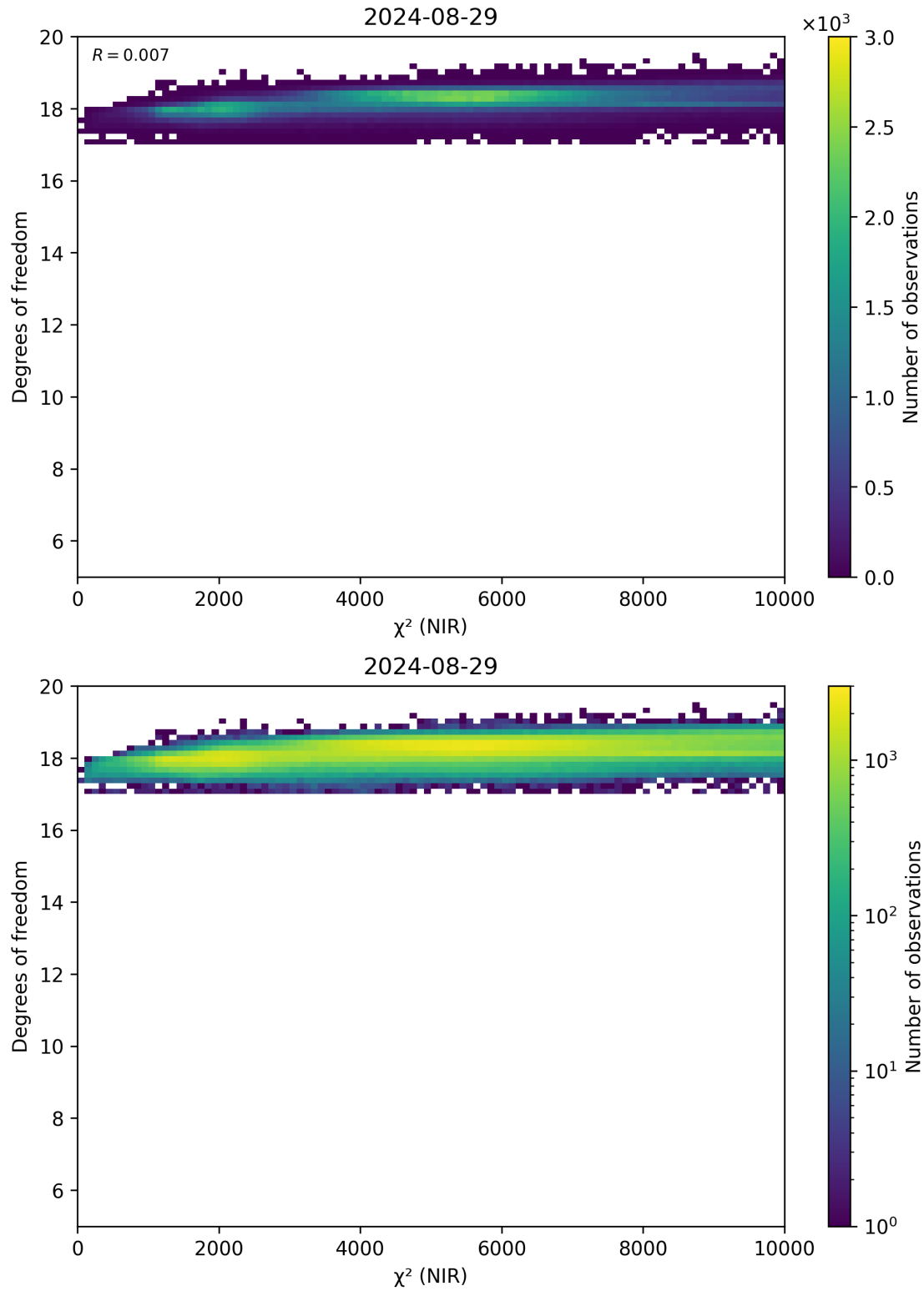
Figure 44: Scatter density plot of “ \chi^2 (NIR)” against “Degrees of freedom” for 2024-08-28 to 2024-08-30.
