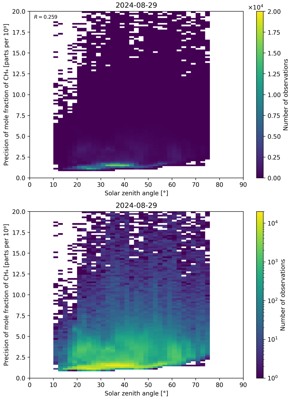
Figure 101: Scatter density plot of “Solar zenith angle” against “Precision of mole fraction of CH 4 ” for 2024-08-28 to 2024-08-30.
