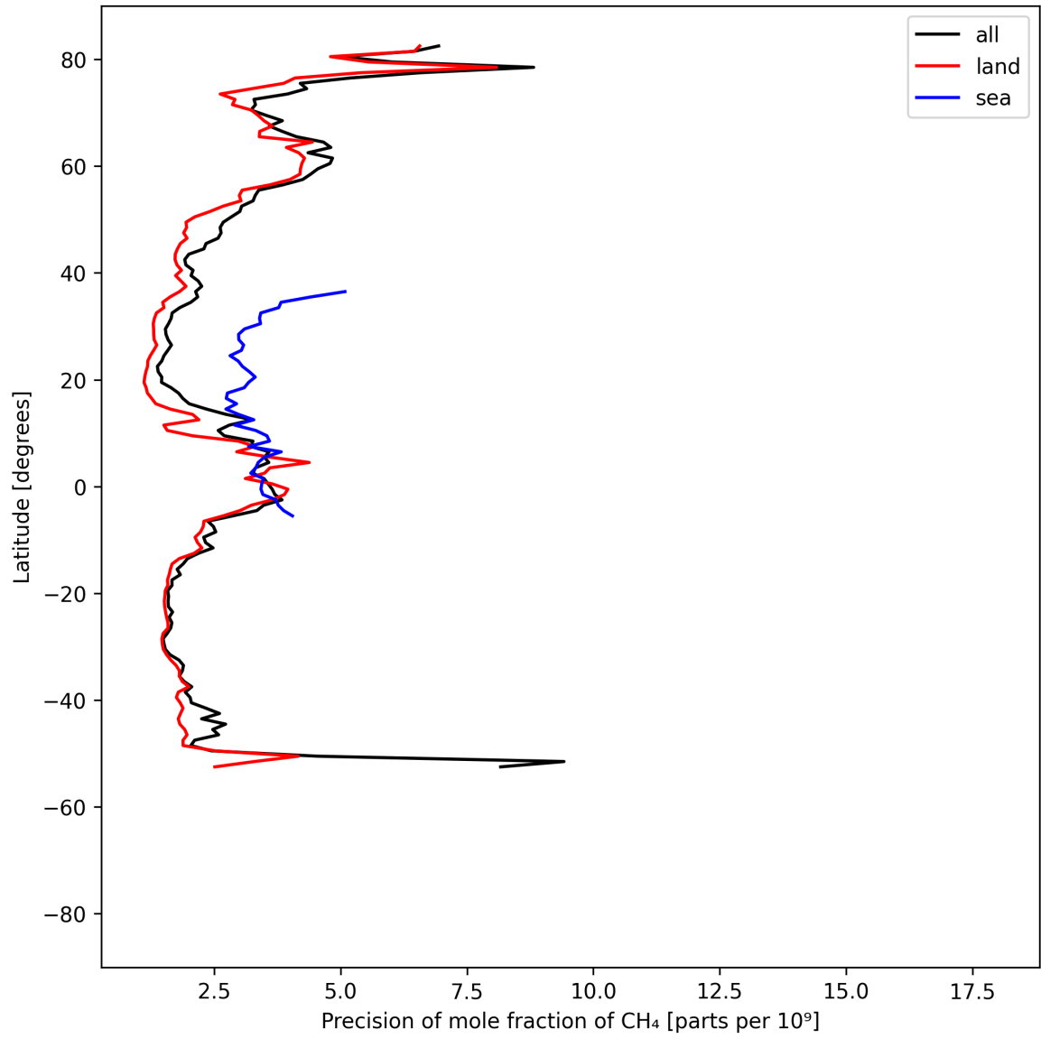
Figure 13: Zonal average of “Precision of mole fraction of CH 4 ” for 2024-08-28 to 2024-08-30.
