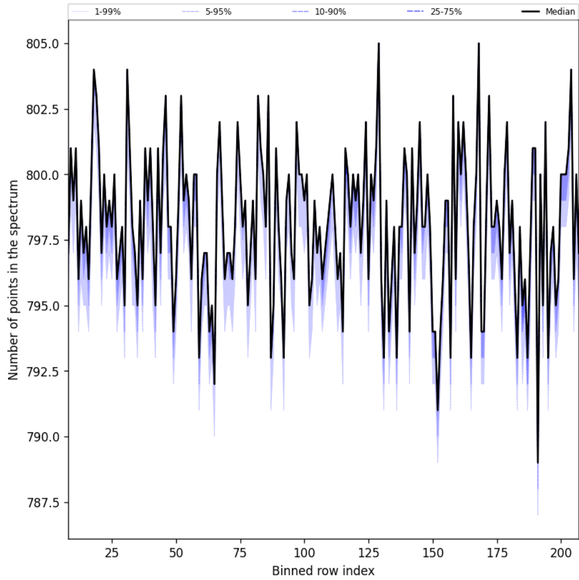
Figure 37: Along track statistics of “Number of points in the spectrum” for 2024-08-28 to 2024-08-30
