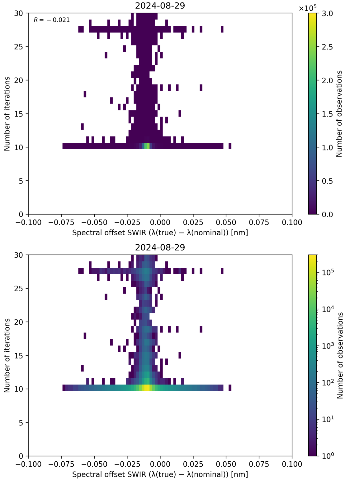
Figure 121: Scatter density plot of “Spectral offset SWIR ( \lambda_{\text{true}} - \lambda_{\text{nominal}} )” against “Number of iterations” for 2024-08-28 to 2024-08-30.
