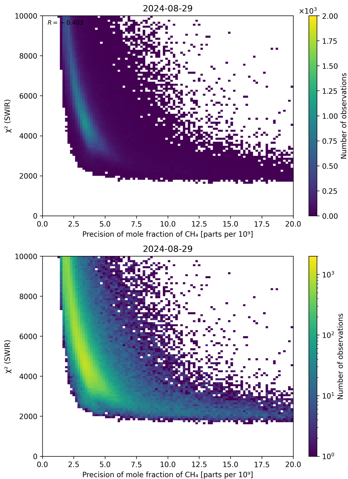
Figure 79: Scatter density plot of “Precision of mole fraction of \text{CH}_4 ” against “ \chi^2 (SWIR)” for 2024-08-28 to 2024-08-30.
