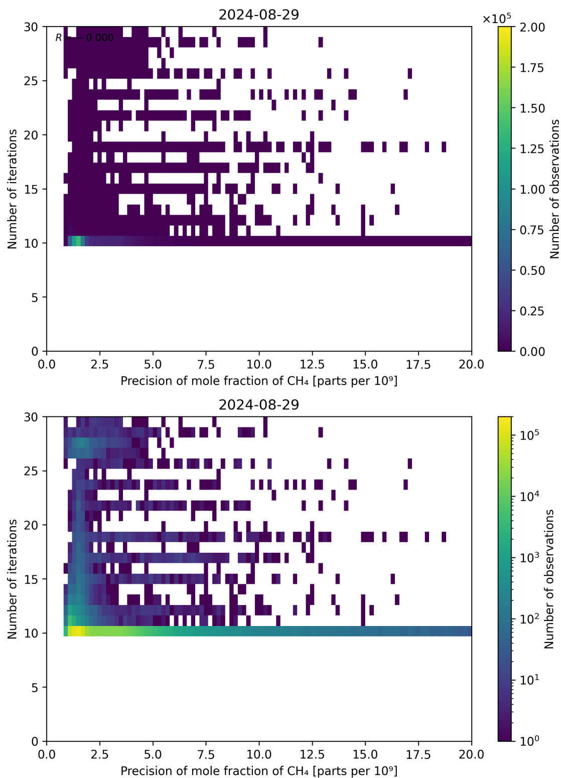
Figure 83: Scatter density plot of “Precision of mole fraction of CH 4 ” against “Number of iterations” for 2024-08-28 to 2024-08-30.
