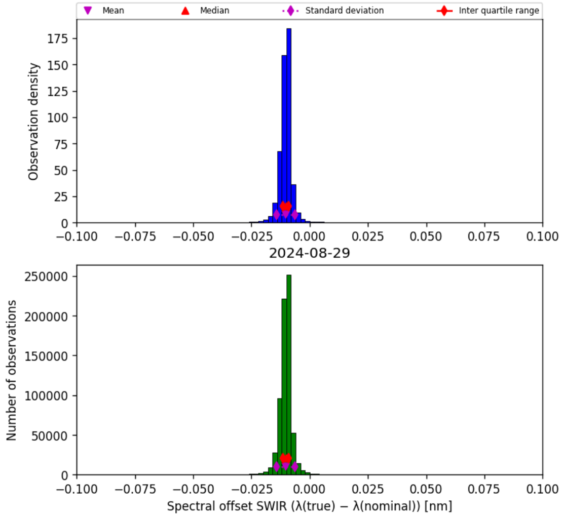
Figure 27: Histogram of “Spectral offset SWIR ( \lambda_{\text{true}} - \lambda_{\text{nominal}} )” for 2024-08-28 to 2024-08-30
