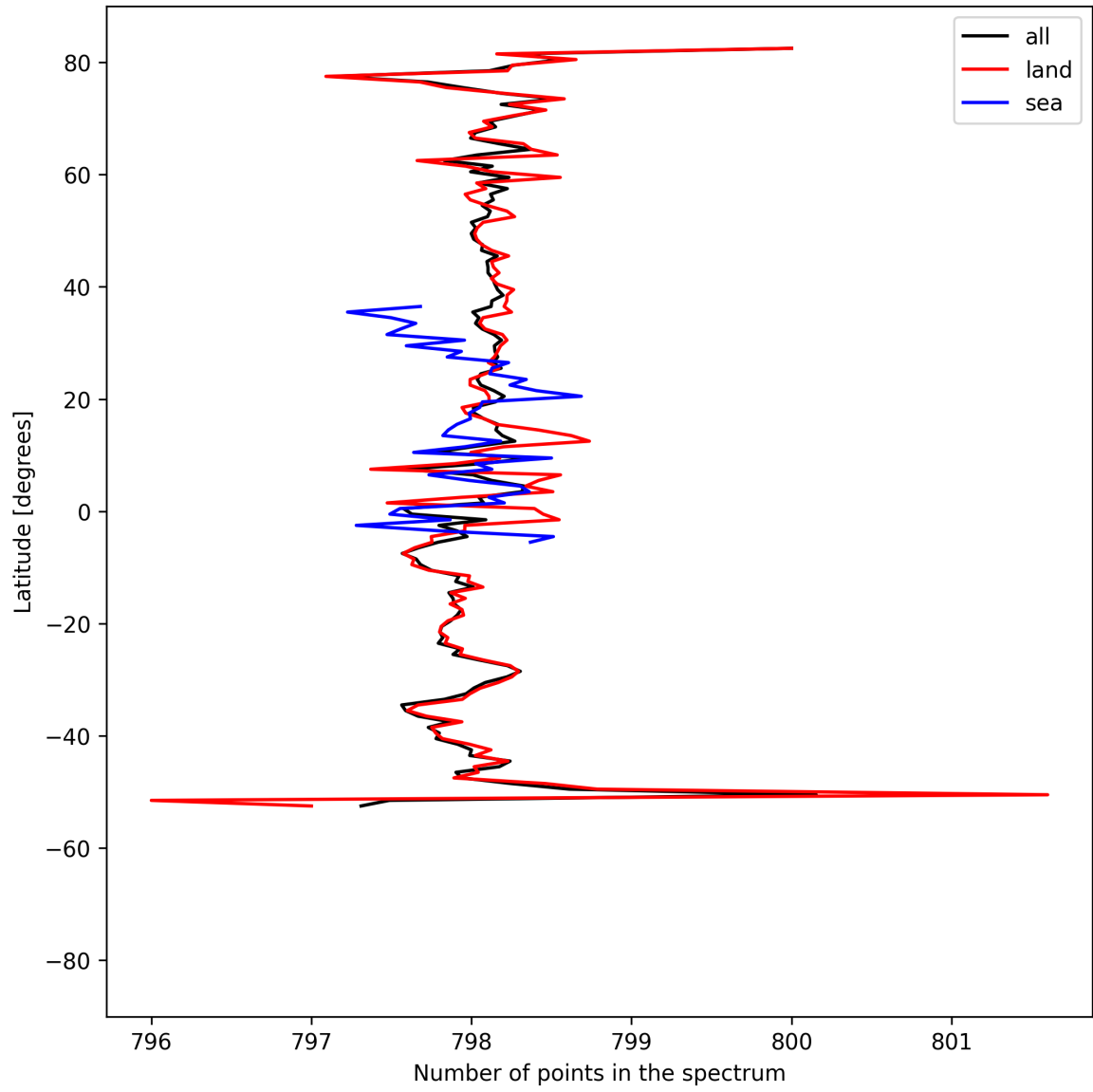
Figure 15: Zonal average of “Number of points in the spectrum” for 2024-08-28 to 2024-08-30.
