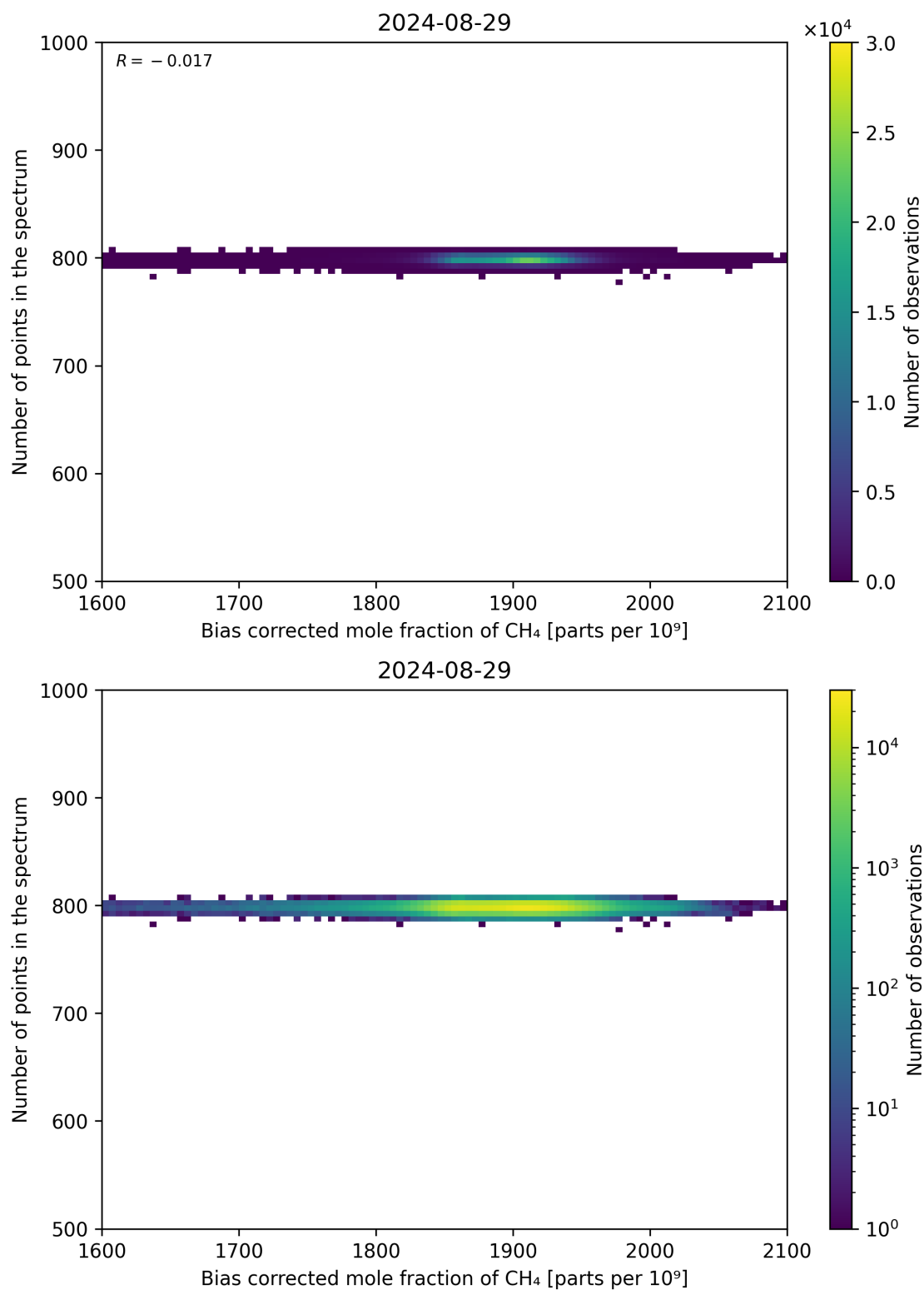
Figure 68: Scatter density plot of “Bias corrected mole fraction of CH 4 ” against “Number of points in the spectrum” for 2024-08-28 to 2024-08-30.
