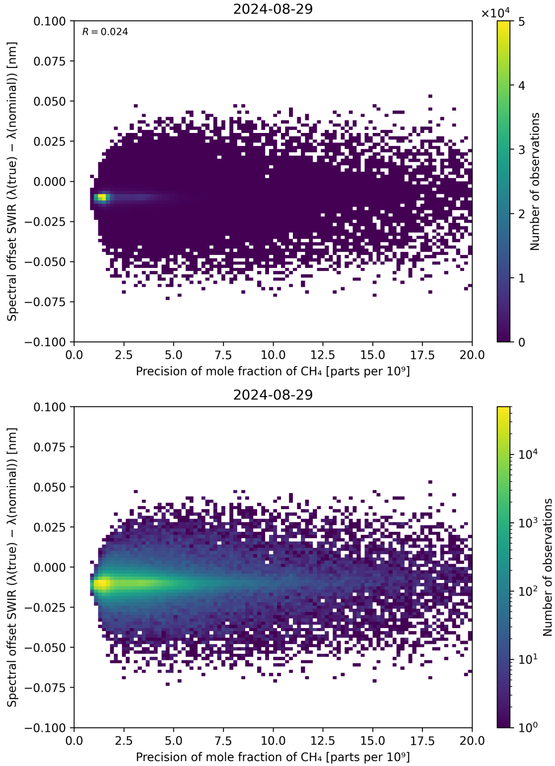
Figure 85: Scatter density plot of “Precision of mole fraction of CH 4 ” against “Spectral offset SWIR ( \lambda_{\text{true}} - \lambda_{\text{nominal}} )” for 2024-08-28 to 2024-08-30.
