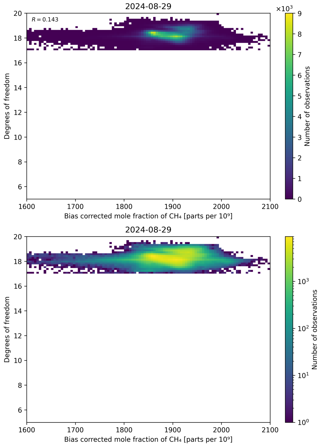
Figure 65: Scatter density plot of “Bias corrected mole fraction of CH 4 ” against “Degrees of freedom” for 2024-08-28 to 2024-08-30.
