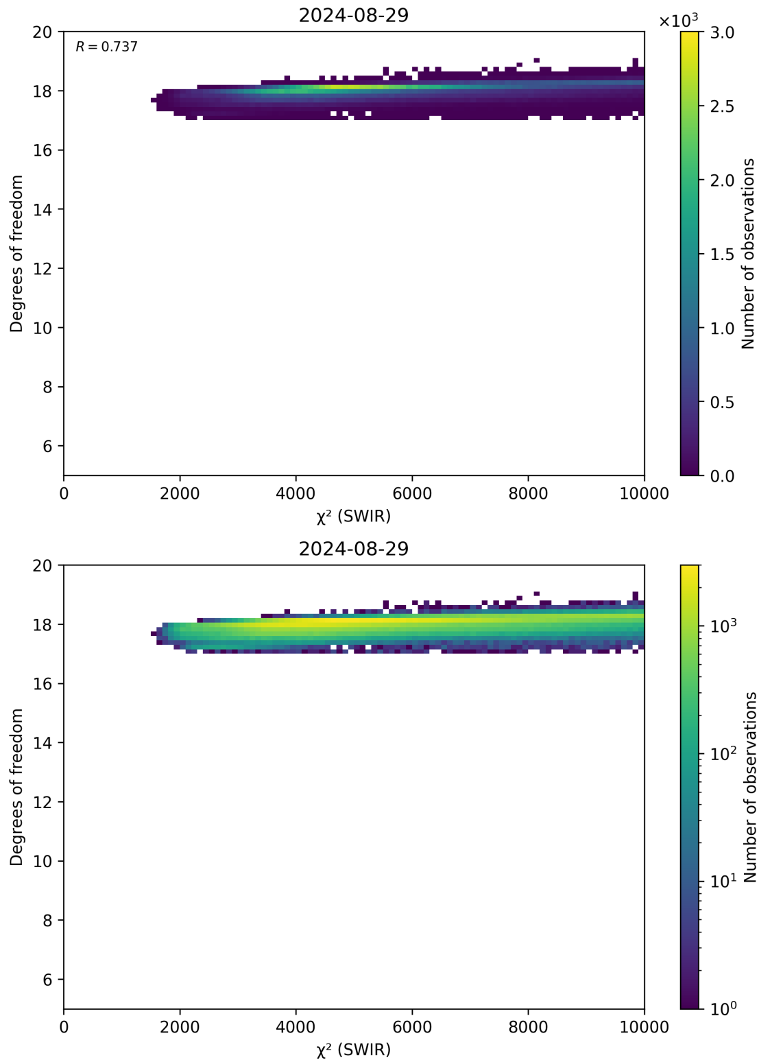
Figure 48: Scatter density plot of “ \chi^2 (SWIR)” against “Degrees of freedom” for 2024-08-28 to 2024-08-30.
