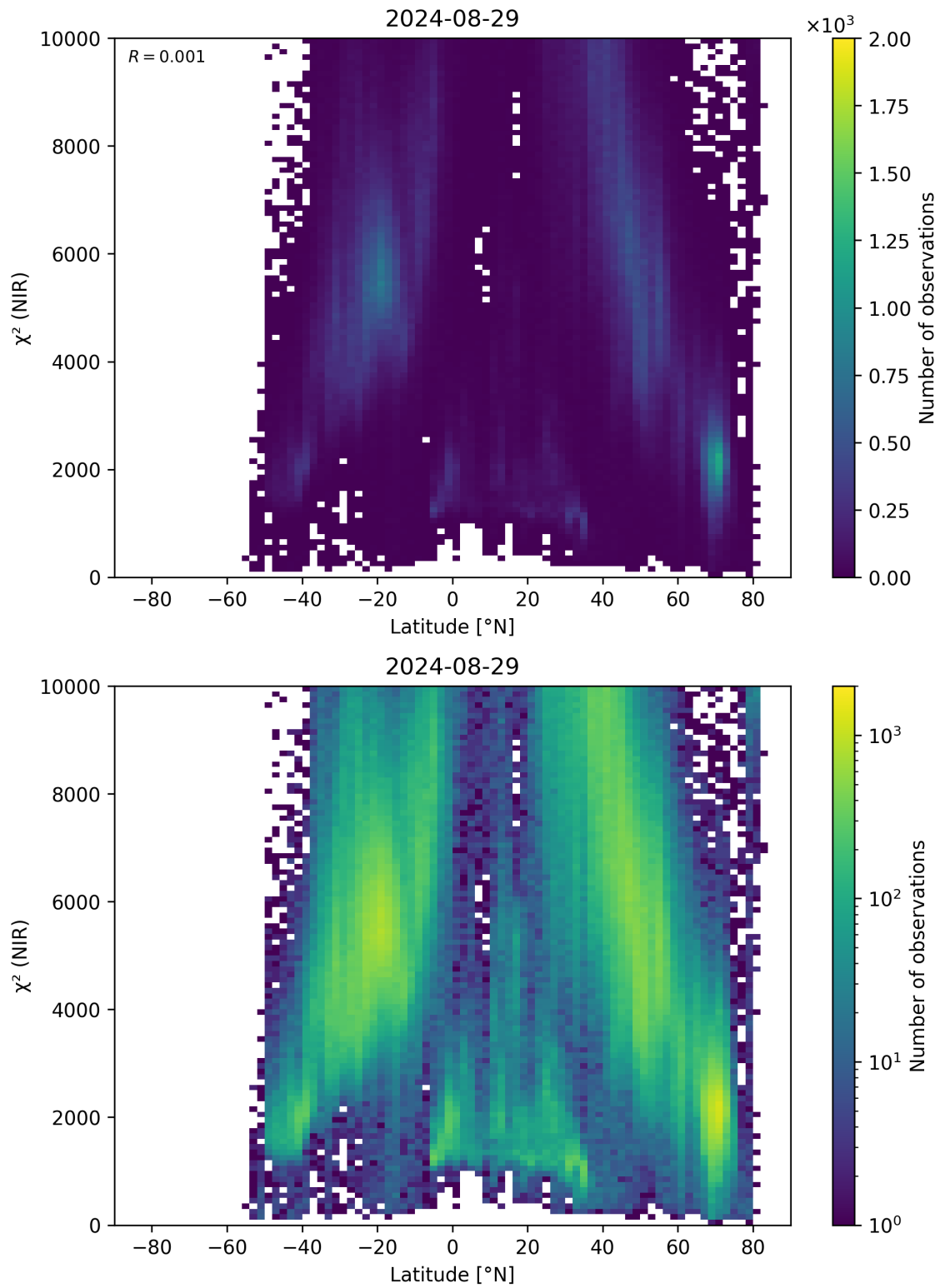
Figure 53: Scatter density plot of “Latitude” against “ \chi^2 (NIR)” for 2024-08-28 to 2024-08-30.
