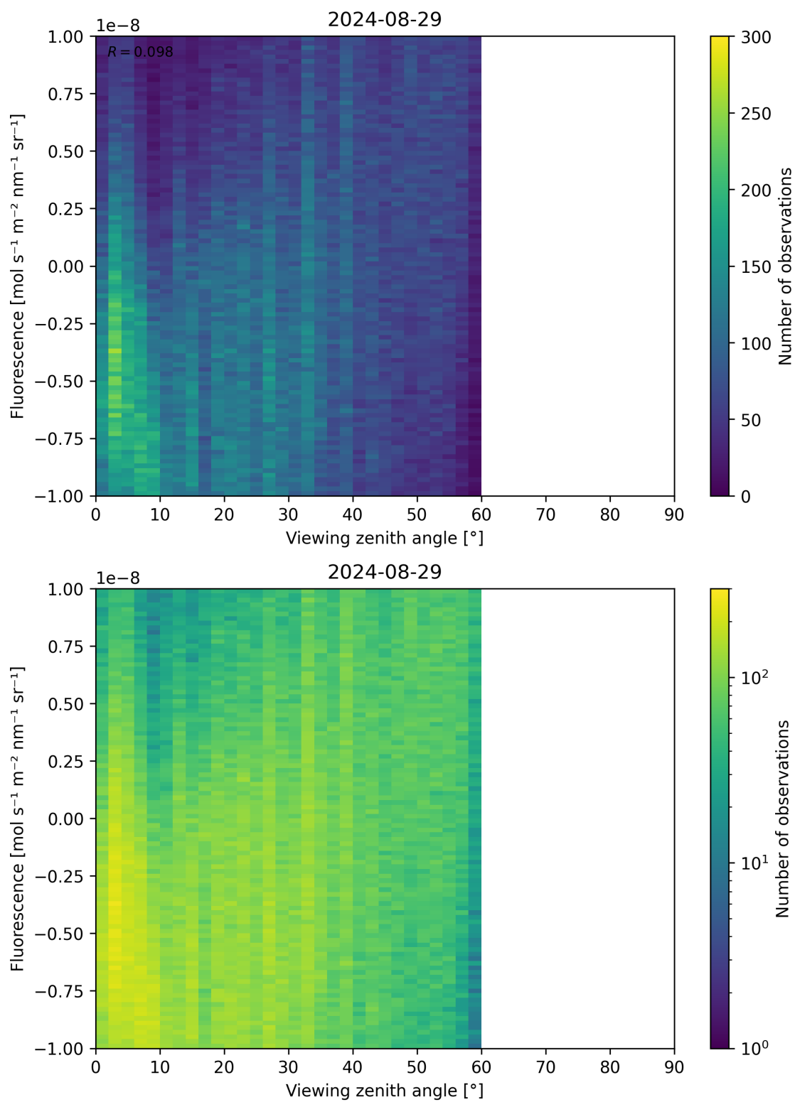
Figure 108: Scatter density plot of “Viewing zenith angle” against “Fluorescence” for 2024-08-28 to 2024-08-30.
