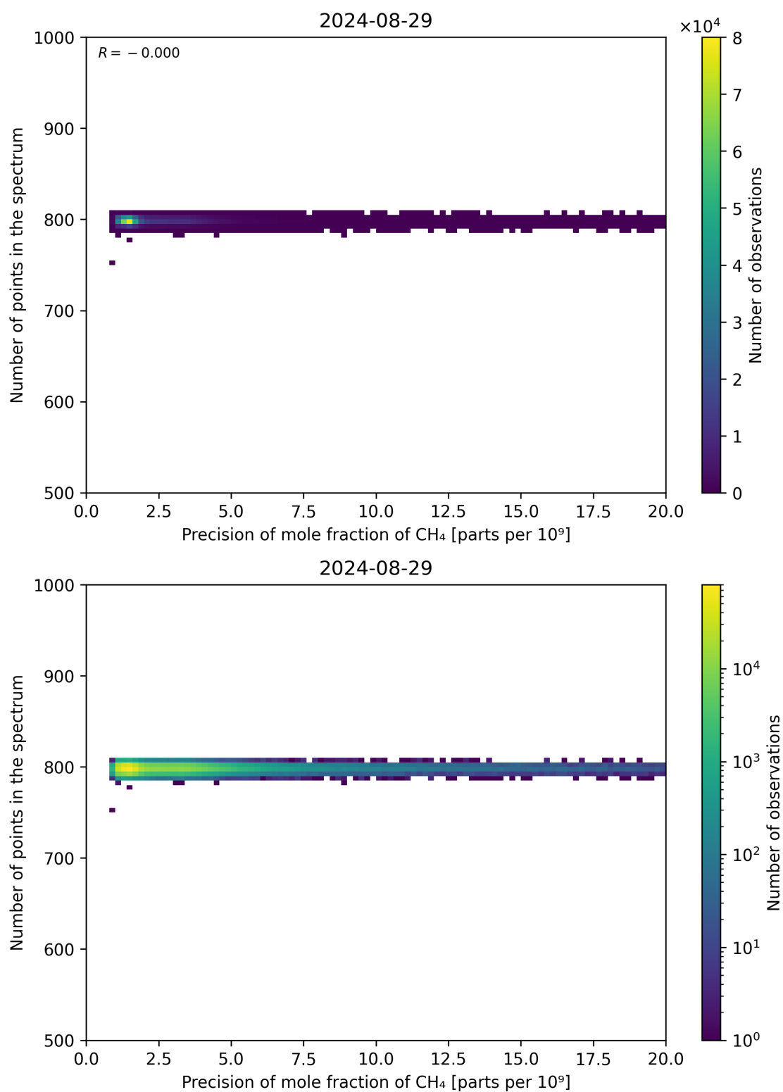
Figure 84: Scatter density plot of “Precision of mole fraction of CH 4 ” against “Number of points in the spectrum” for 2024-08-28 to 2024-08-30.
