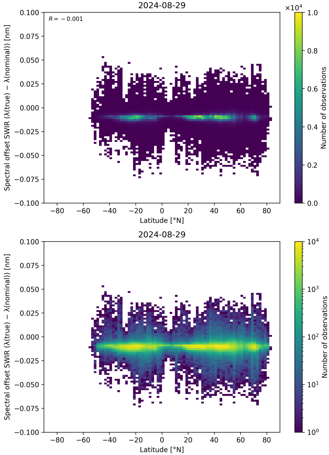
Figure 62: Scatter density plot of “Latitude” against “Spectral offset SWIR ( \lambda_{\text{true}} - \lambda_{\text{nominal}} )” for 2024-08-28 to 2024-08-30.
