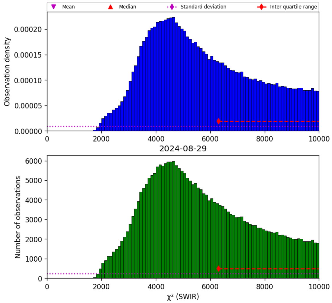
Figure 28: Histogram of “ \chi^2 (SWIR)” for 2024-08-28 to 2024-08-30
