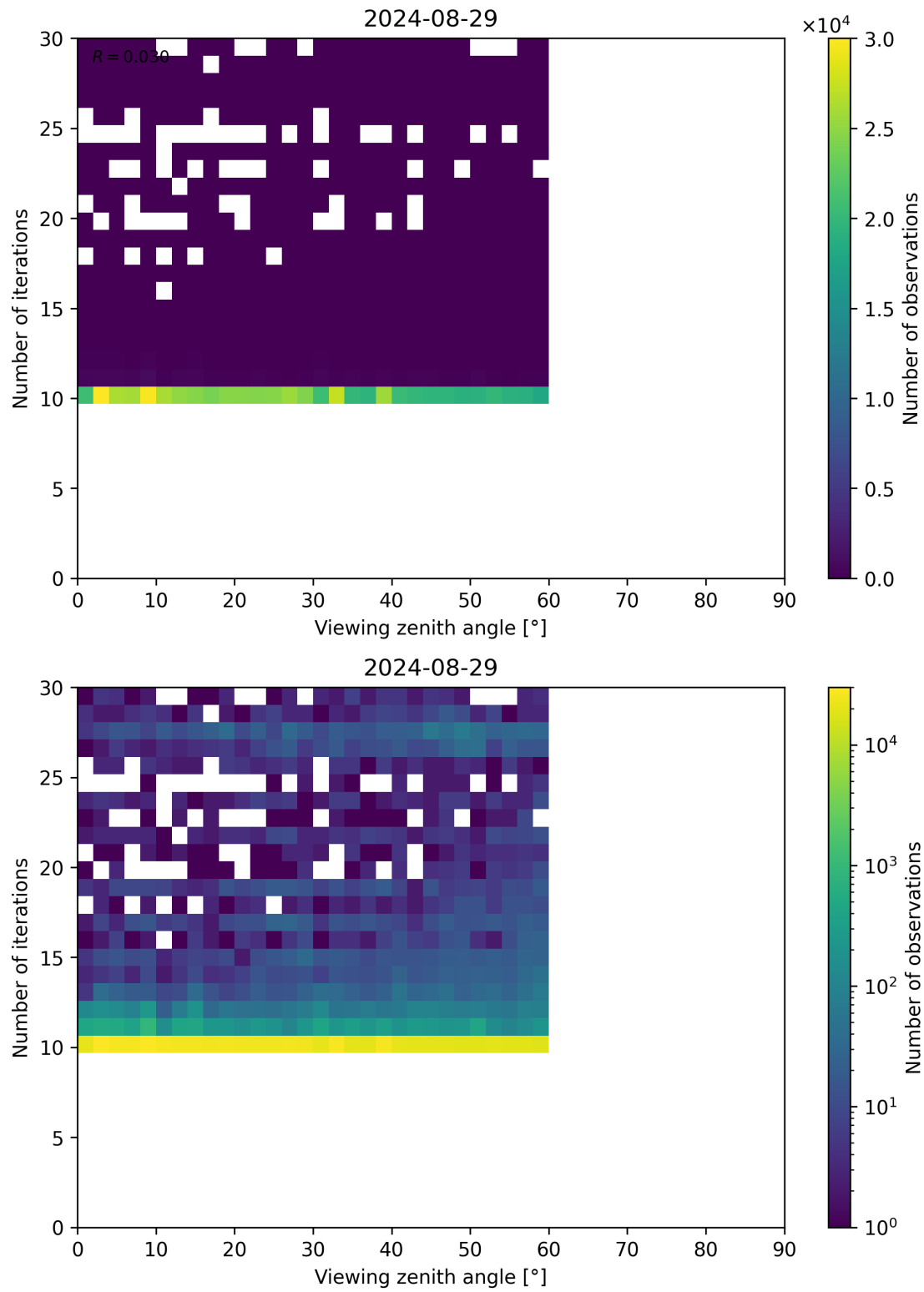
Figure 113: Scatter density plot of “Viewing zenith angle” against “Number of iterations” for 2024-08-28 to 2024-08-30.
