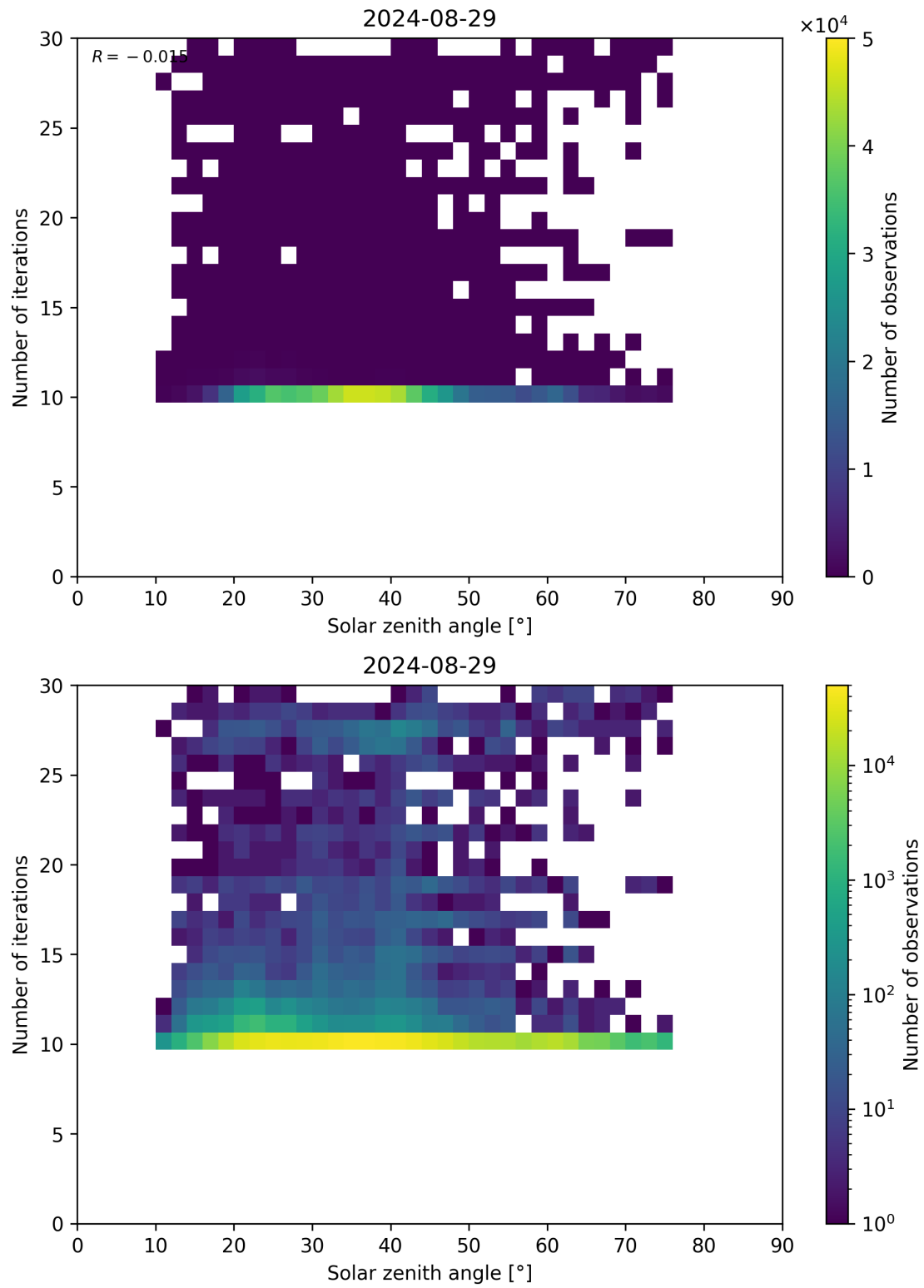
Figure 102: Scatter density plot of “Solar zenith angle” against “Number of iterations” for 2024-08-28 to 2024-08-30.
