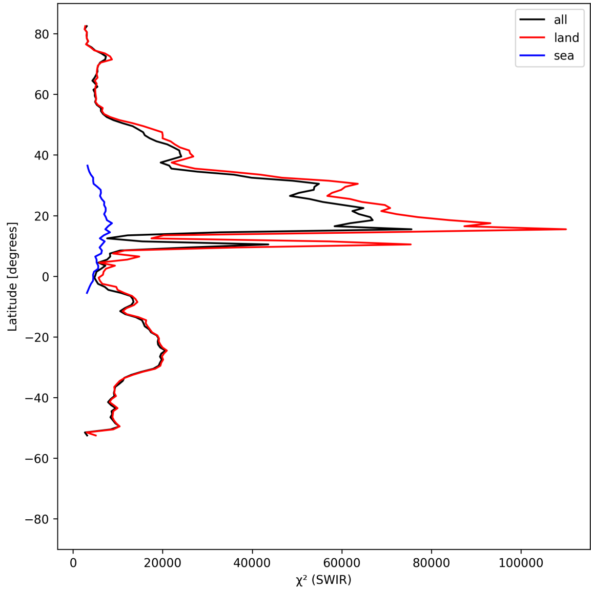
Figure 17: Zonal average of “ \chi^2 (SWIR)” for 2024-08-28 to 2024-08-30.
