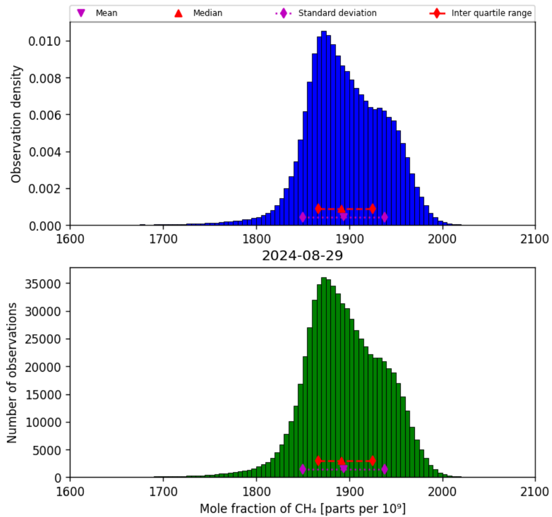
Figure 23: Histogram of “Mole fraction of CH 4 ” for 2024-08-28 to 2024-08-30
