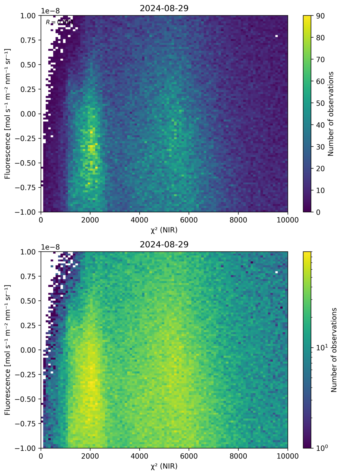
Figure 45: Scatter density plot of “ \chi^2 (NIR)” against “Fluorescence” for 2024-08-28 to 2024-08-30.
