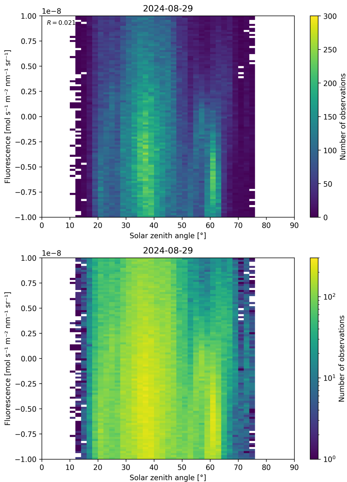
Figure 97: Scatter density plot of “Solar zenith angle” against “Fluorescence” for 2024-08-28 to 2024-08-30.
