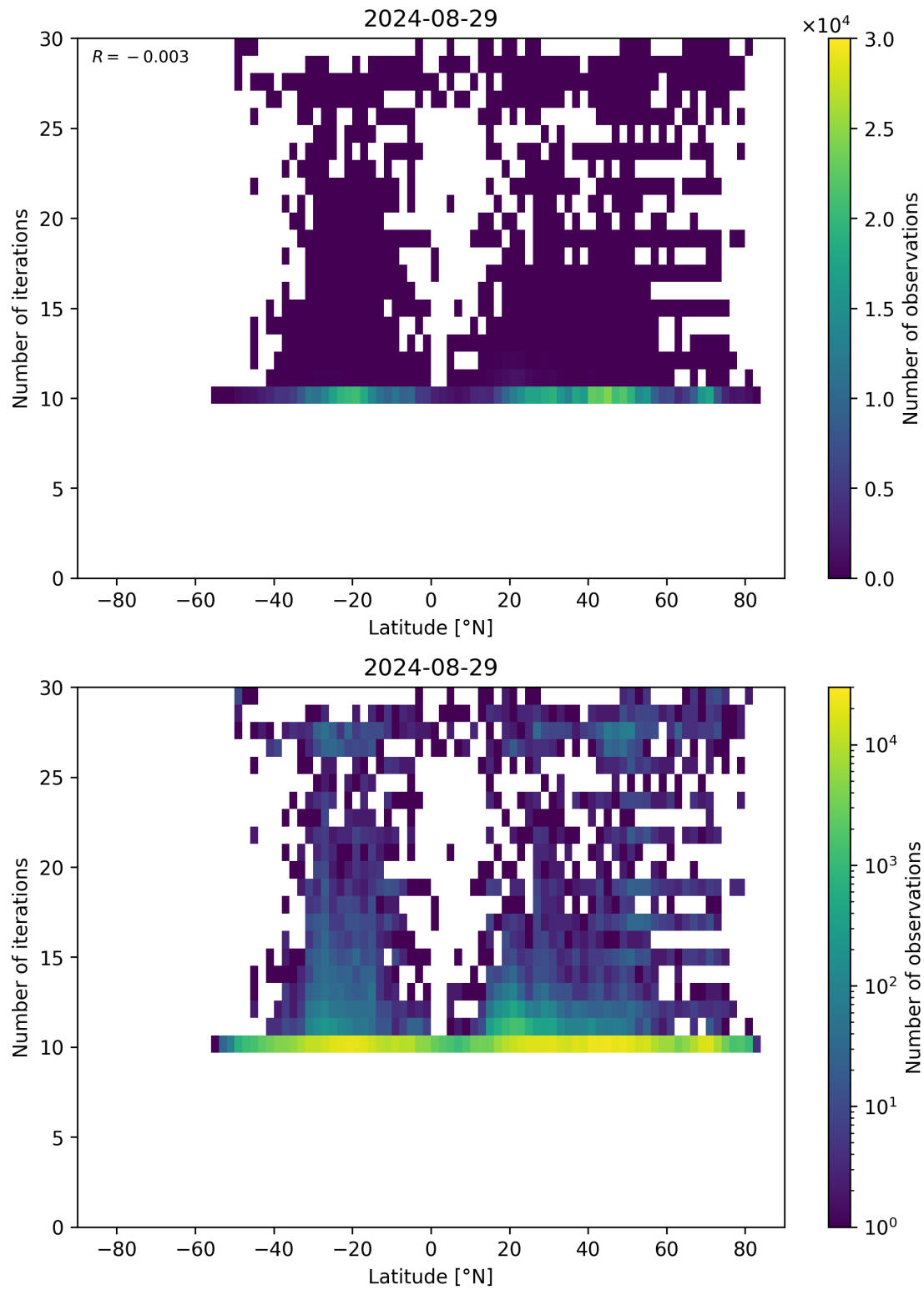
Figure 60: Scatter density plot of “Latitude” against “Number of iterations” for 2024-08-28 to 2024-08-30.
