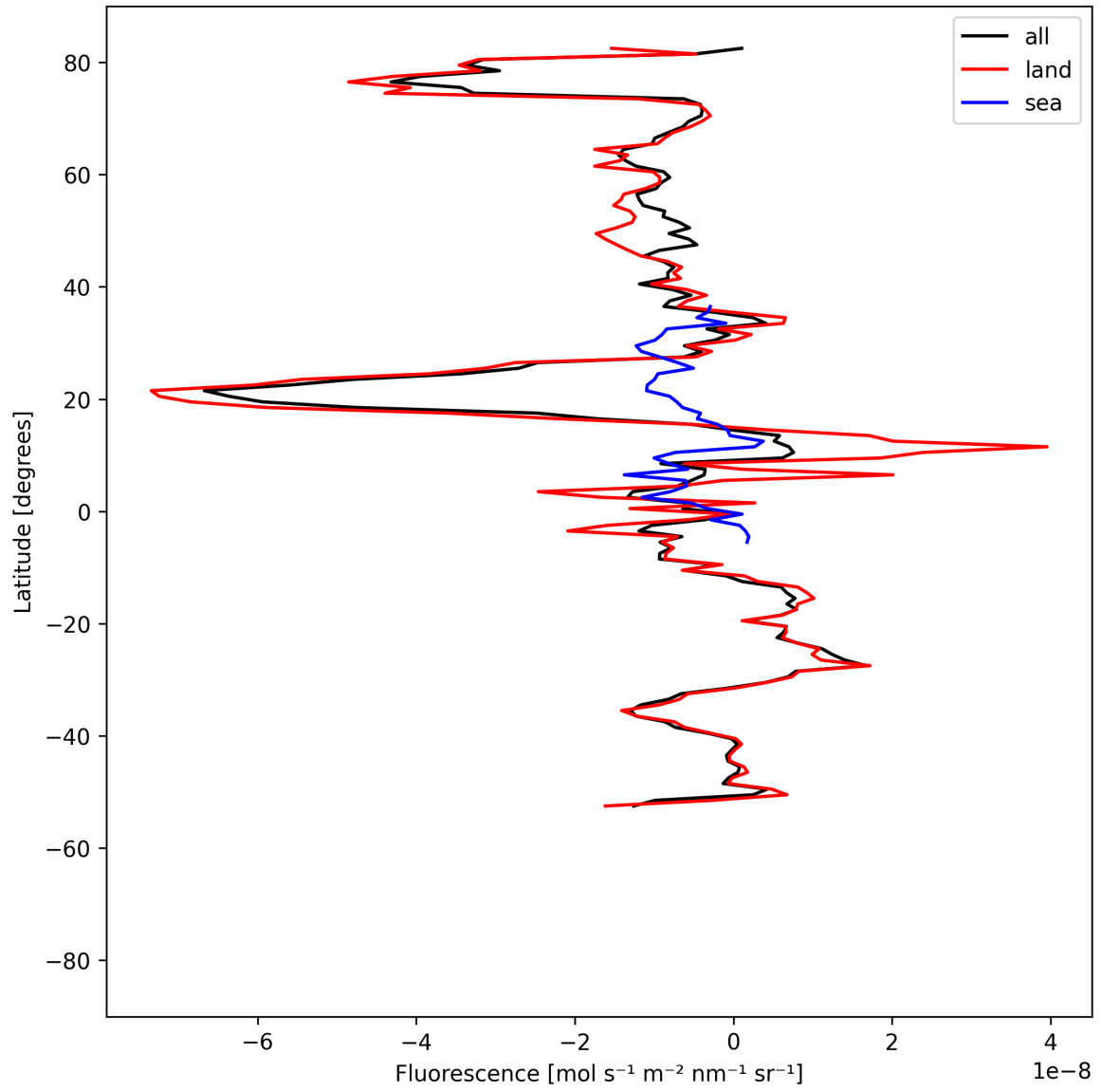
Figure 21: Zonal average of “Fluorescence” for 2024-08-28 to 2024-08-30.
