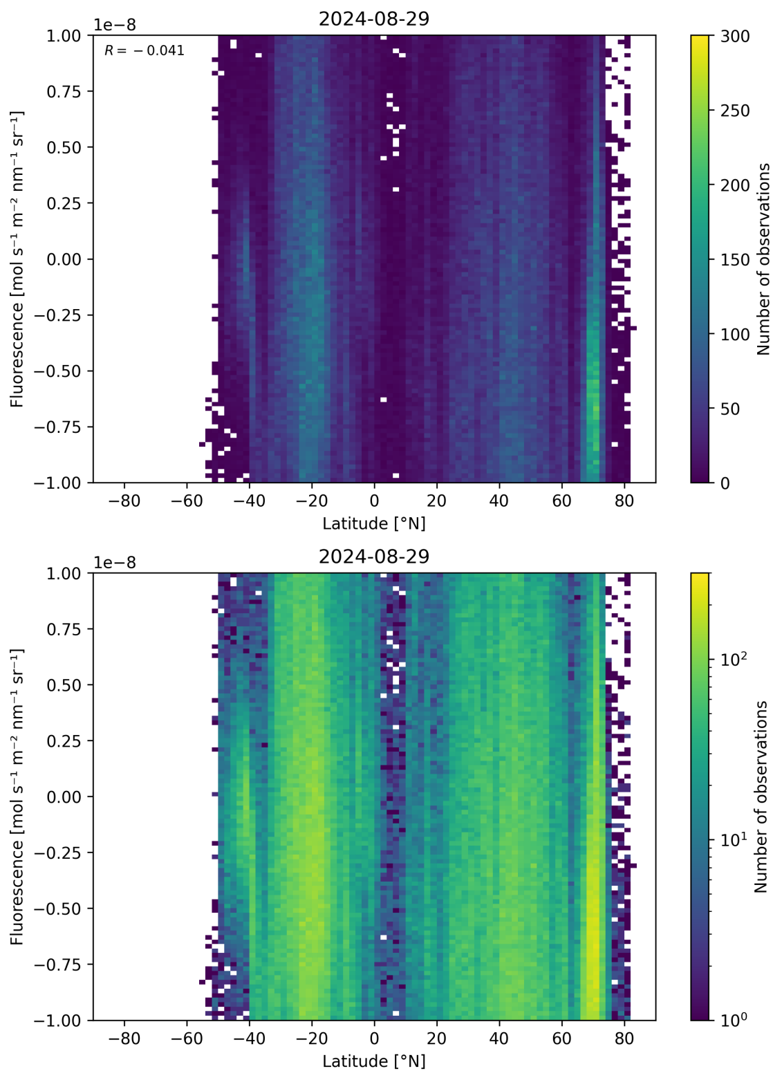
Figure 56: Scatter density plot of “Latitude” against “Fluorescence” for 2024-08-28 to 2024-08-30.
