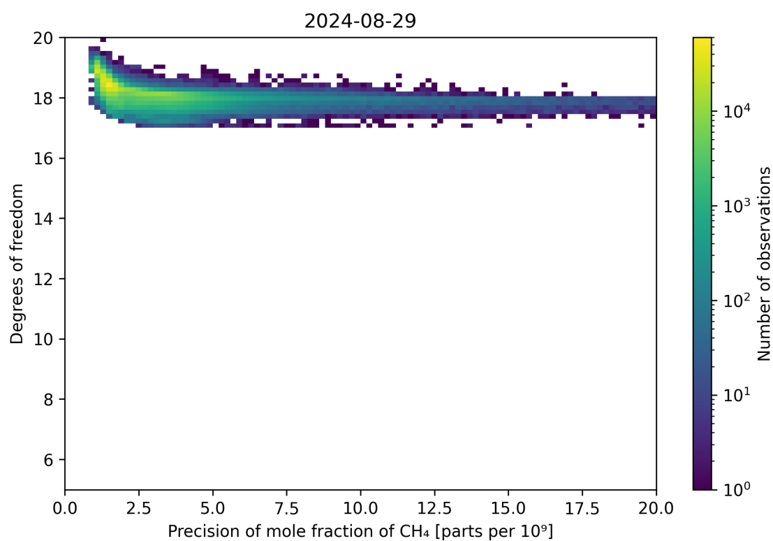
Figure 80: Scatter density plot of “Precision of mole fraction of CH 4 ” against “Degrees of freedom” for 2024-08-28 to 2024-08-30.
