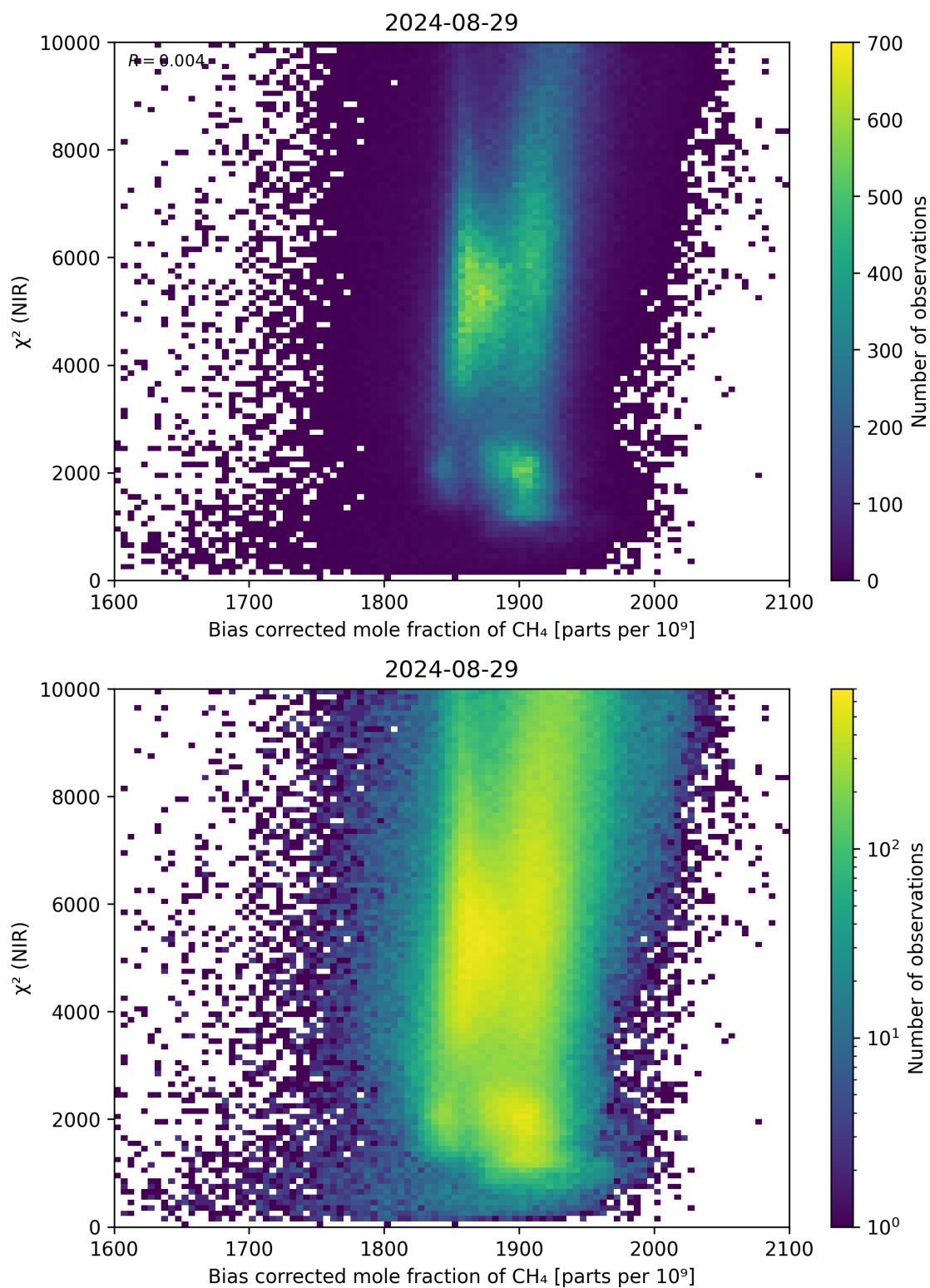
Figure 63: Scatter density plot of “Bias corrected mole fraction of \text{CH}_4 ” against “ \chi^2 (NIR)” for 2024-08-28 to 2024-08-30.
