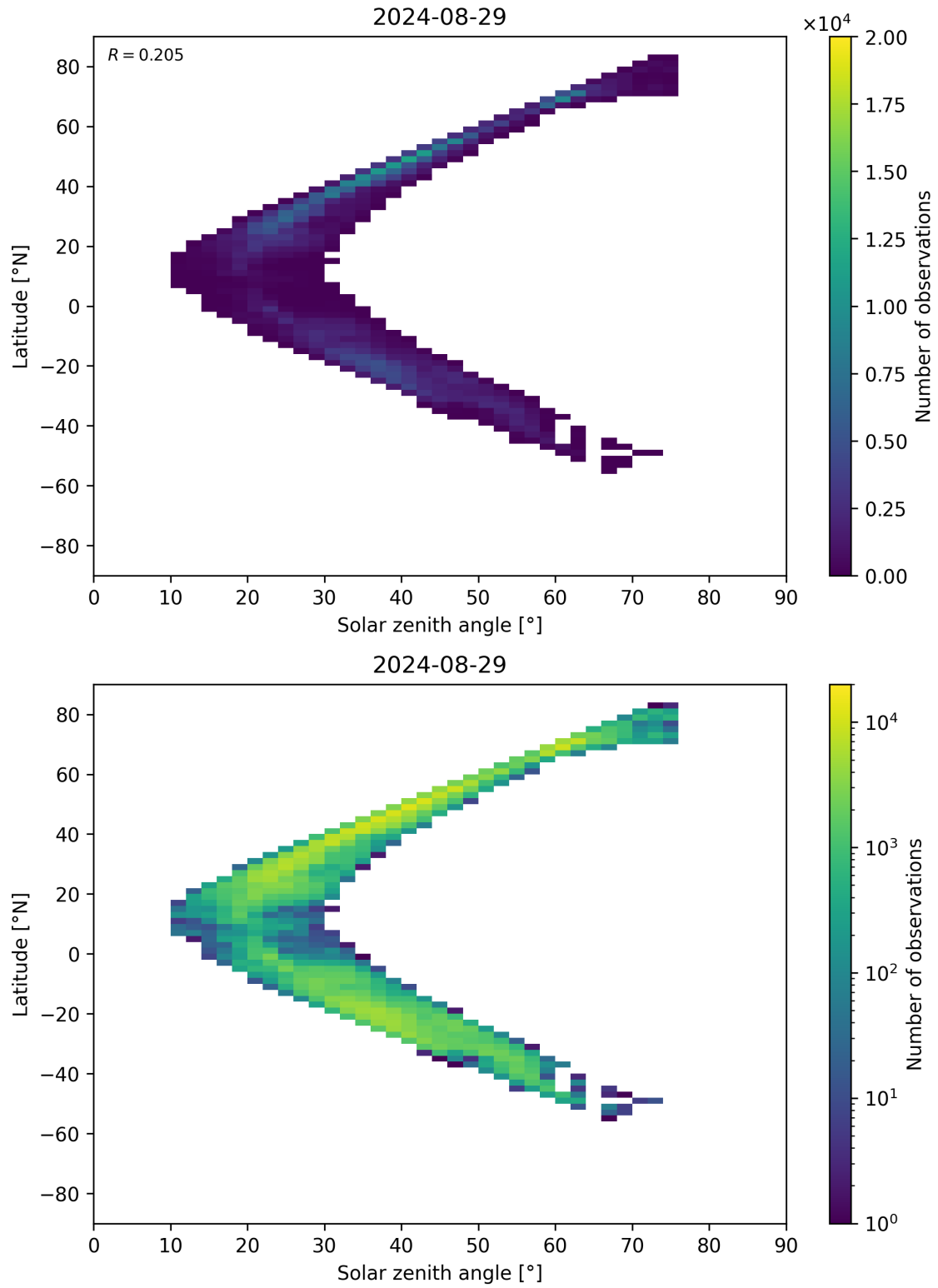
Figure 98: Scatter density plot of “Solar zenith angle” against “Latitude” for 2024-08-28 to 2024-08-30.
