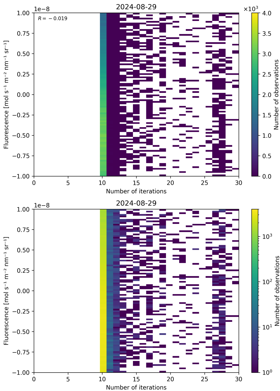
Figure 87: Scatter density plot of “Number of iterations” against “Fluorescence” for 2024-08-28 to 2024-08-30.
