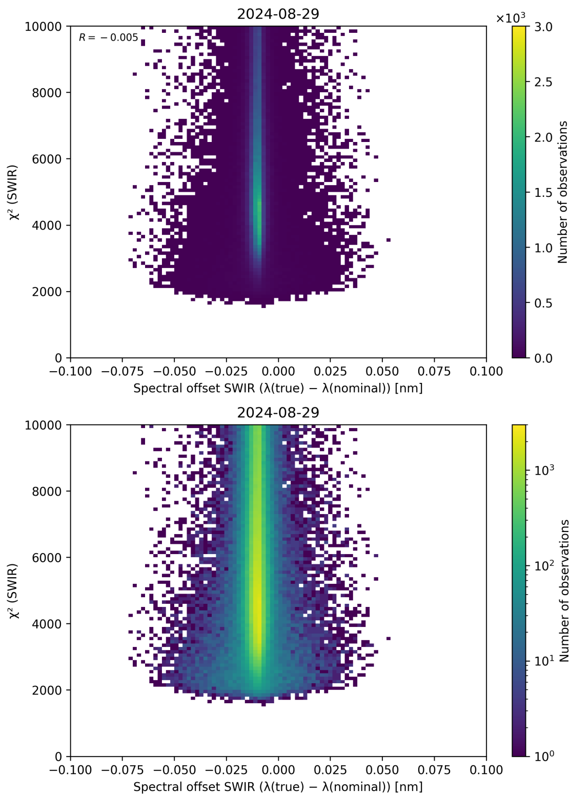
Figure 118: Scatter density plot of “Spectral offset SWIR ( \lambda_{\text{true}} - \lambda_{\text{nominal}} )” against “ \chi^2 (SWIR)” for 2024-08-28 to 2024-08-30.
