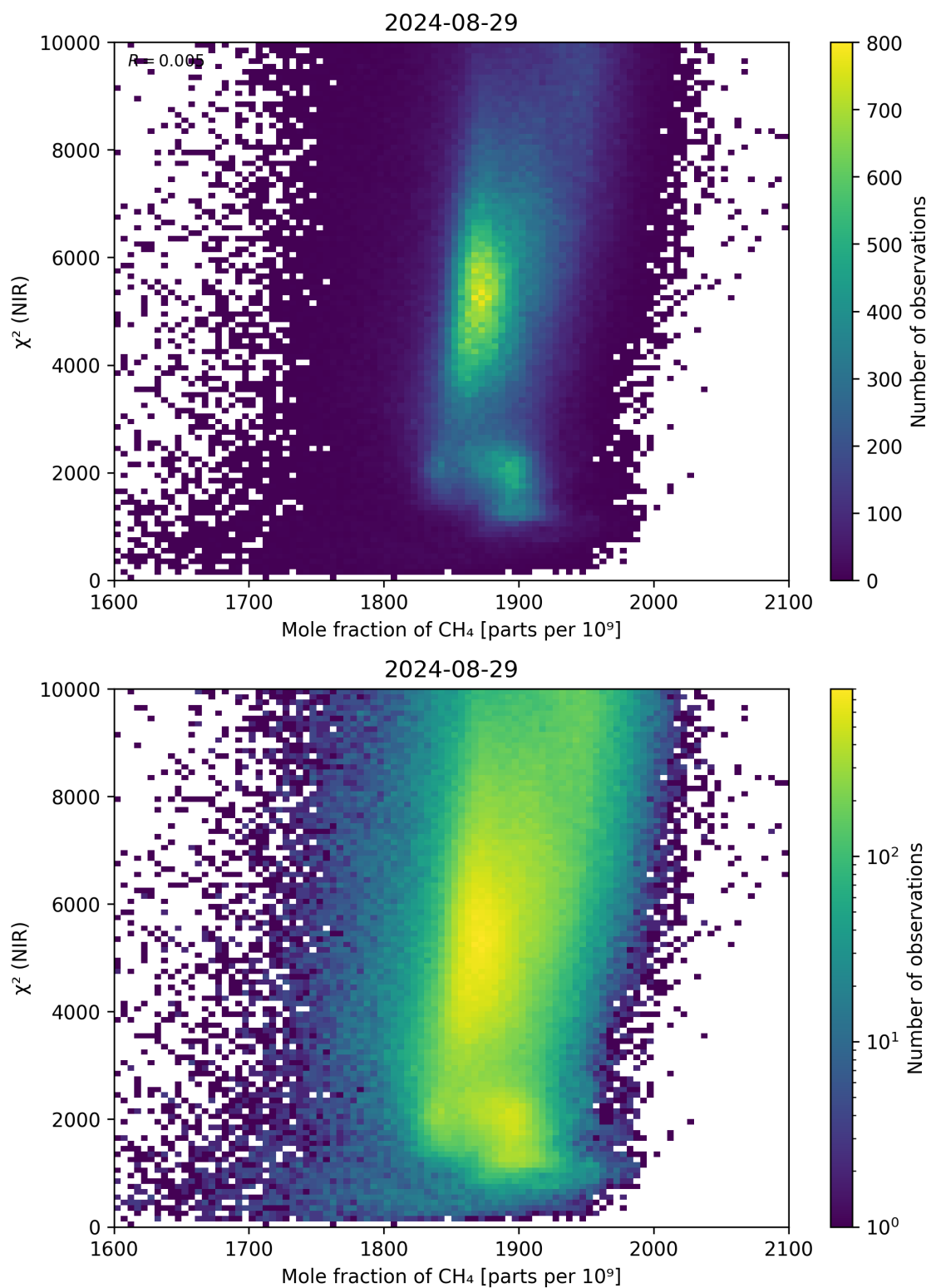
Figure 70: Scatter density plot of “Mole fraction of \text{CH}_4 ” against “ \chi^2 (NIR)” for 2024-08-28 to 2024-08-30.
