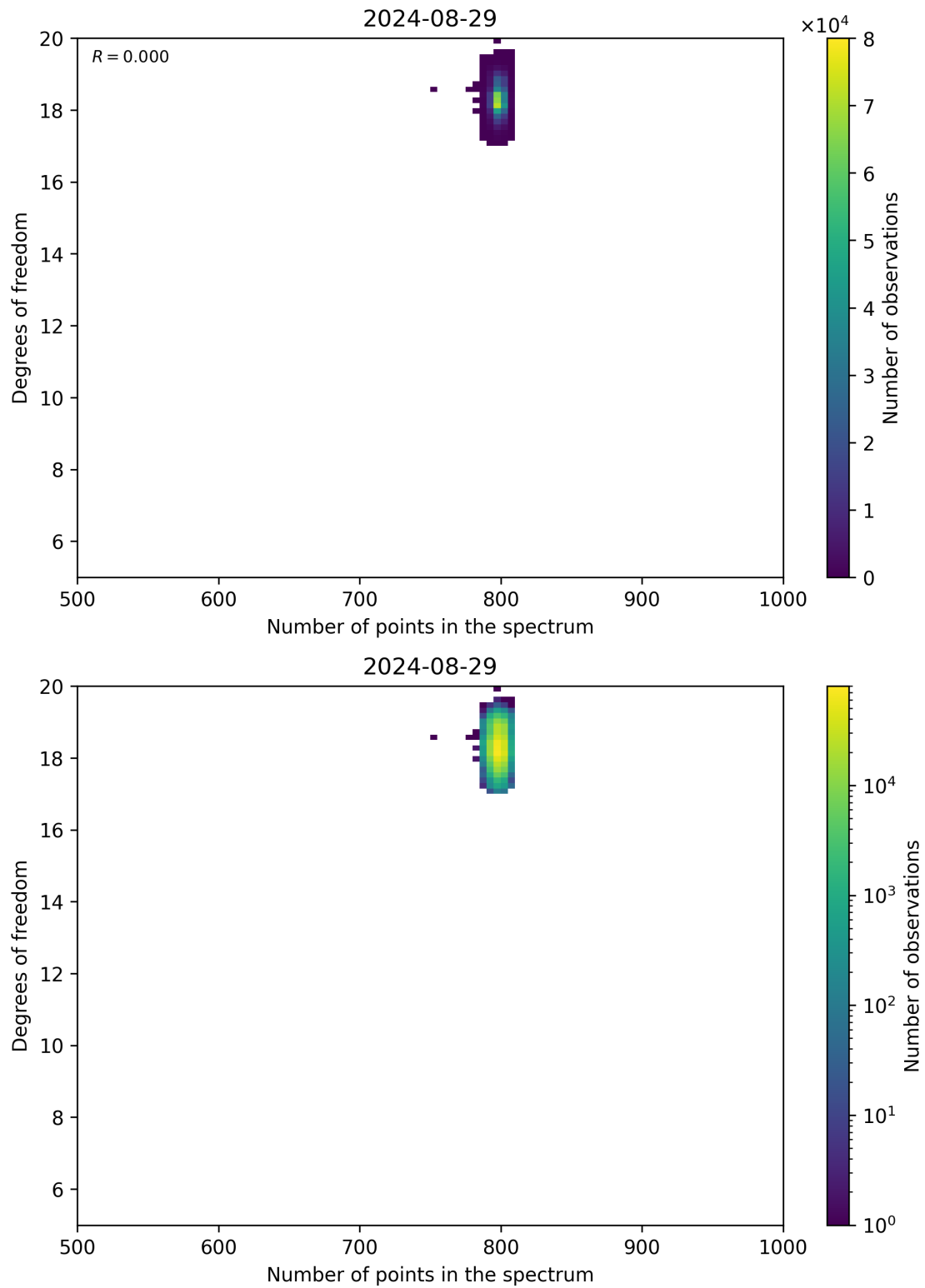
Figure 90: Scatter density plot of “Number of points in the spectrum” against “Degrees of freedom” for 2024-08-28 to 2024-08-30.
