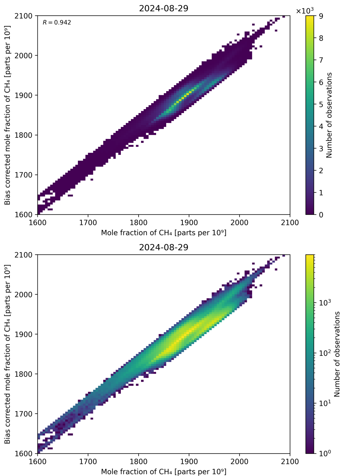
Figure 74: Scatter density plot of “Mole fraction of CH 4 ” against “Bias corrected mole fraction of CH 4 ” for 2024-08-28 to 2024-08-30.
