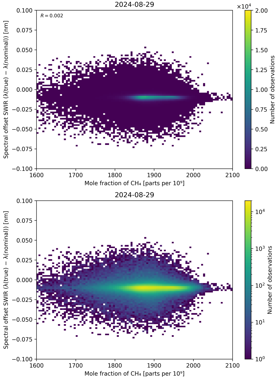
Figure 86: Scatter density plot of “Mole fraction of CH 4 ” against “Spectral offset SWIR ( \lambda_{\text{true}} - \lambda_{\text{nominal}} )” for 2024-08-28 to 2024-08-30.
