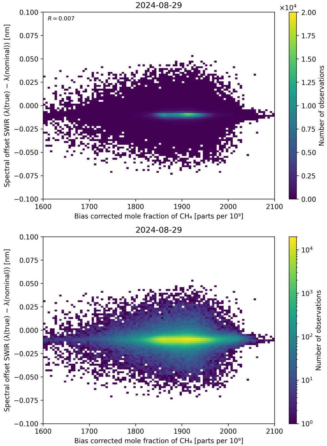
Figure 69: Scatter density plot of “Bias corrected mole fraction of CH 4 ” against “Spectral offset SWIR ( \lambda_{\text{true}} - \lambda_{\text{nominal}} )” for 2024-08-28 to 2024-08-30.
