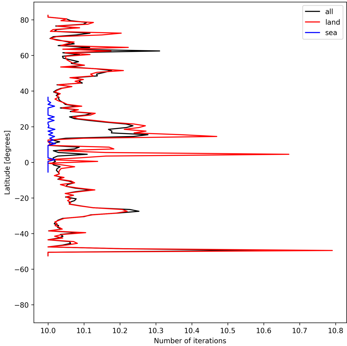
Figure 20: Zonal average of “Number of iterations” for 2024-08-28 to 2024-08-30.
