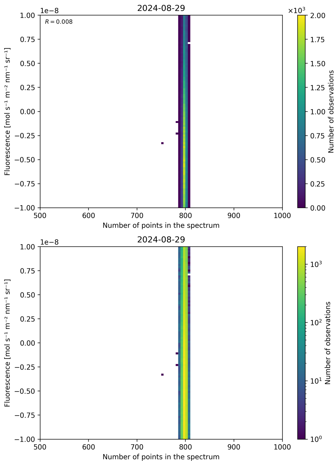
Figure 91: Scatter density plot of “Number of points in the spectrum” against “Fluorescence” for 2024-08-28 to 2024-08-30.
