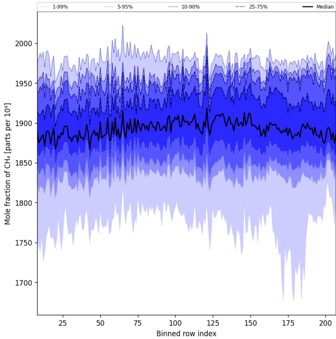
Figure 34: Along track statistics of “Mole fraction of CH 4 ” for 2024-08-28 to 2024-08-30
