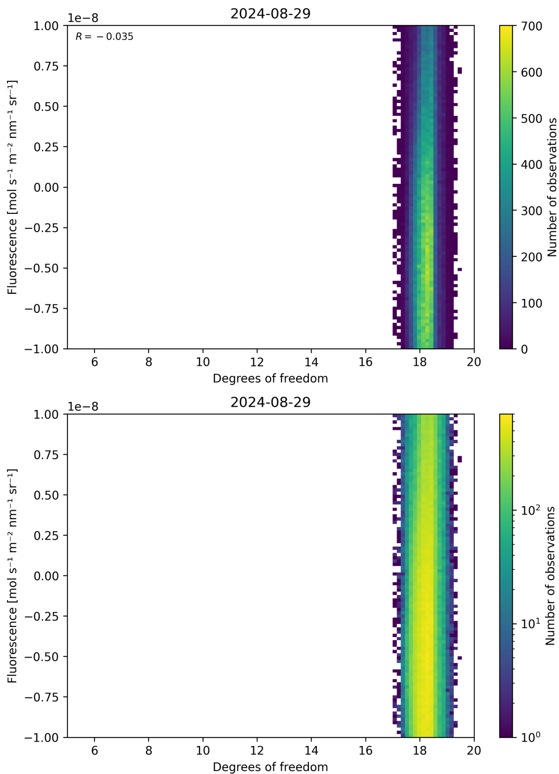
Figure 51: Scatter density plot of “Degrees of freedom” against “Fluorescence” for 2024-08-28 to 2024-08-30.
