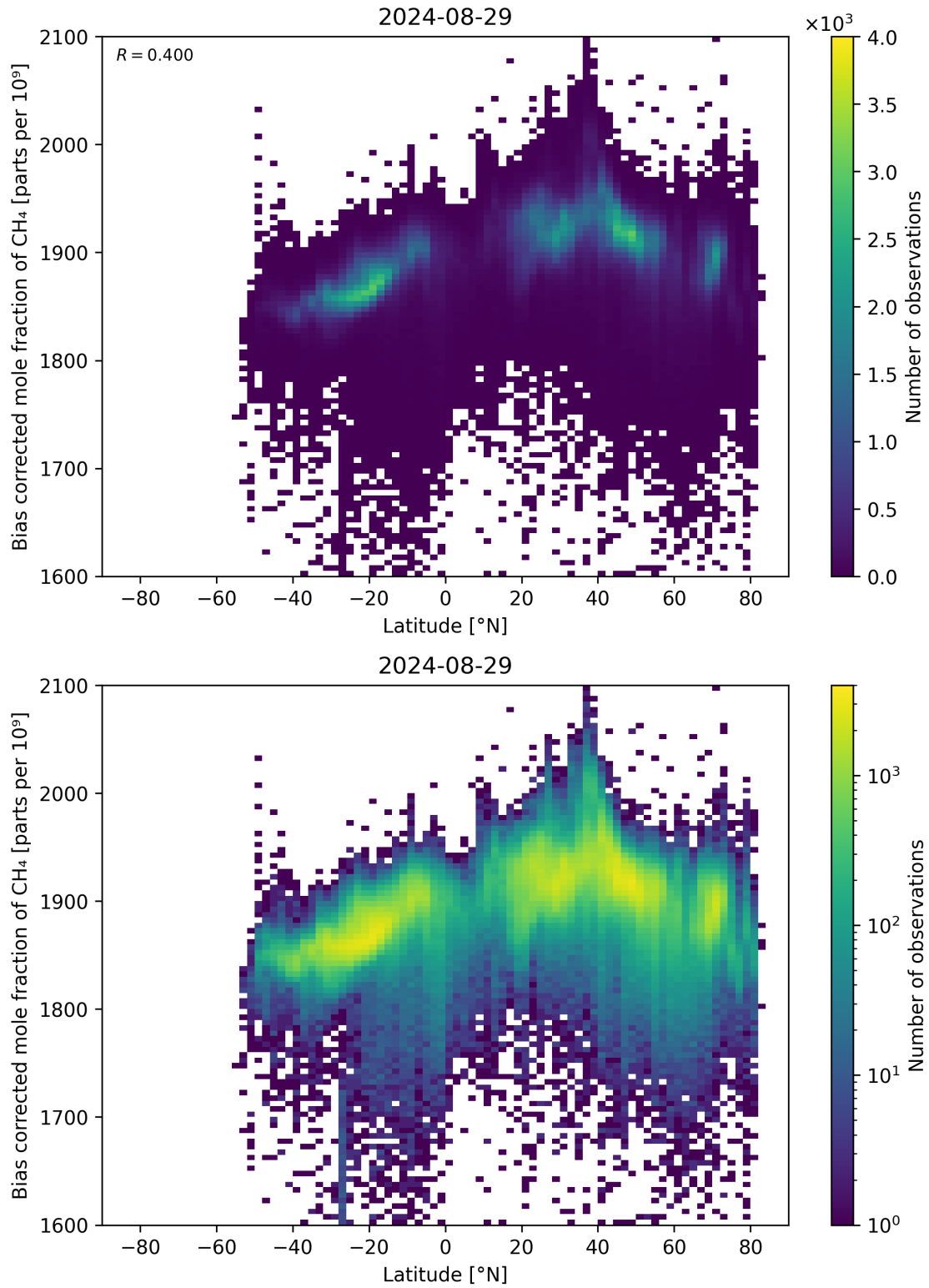
Figure 58: Scatter density plot of “Latitude” against “Bias corrected mole fraction of \text{CH}_4 ” for 2024-08-28 to 2024-08-30.
