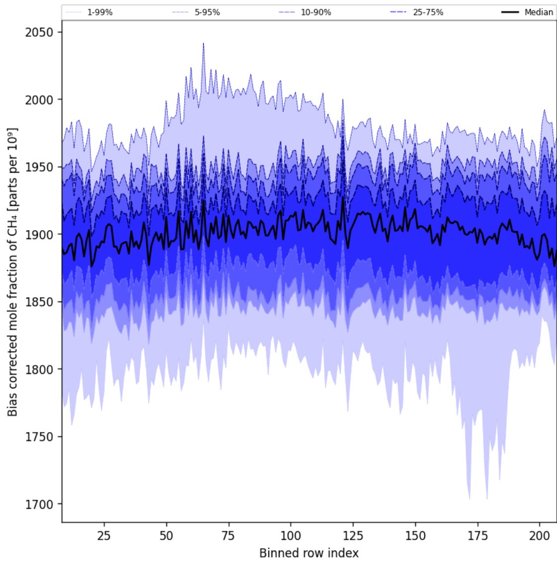
Figure 36: Along track statistics of “Bias corrected mole fraction of CH 4 ” for 2024-08-28 to 2024-08-30
