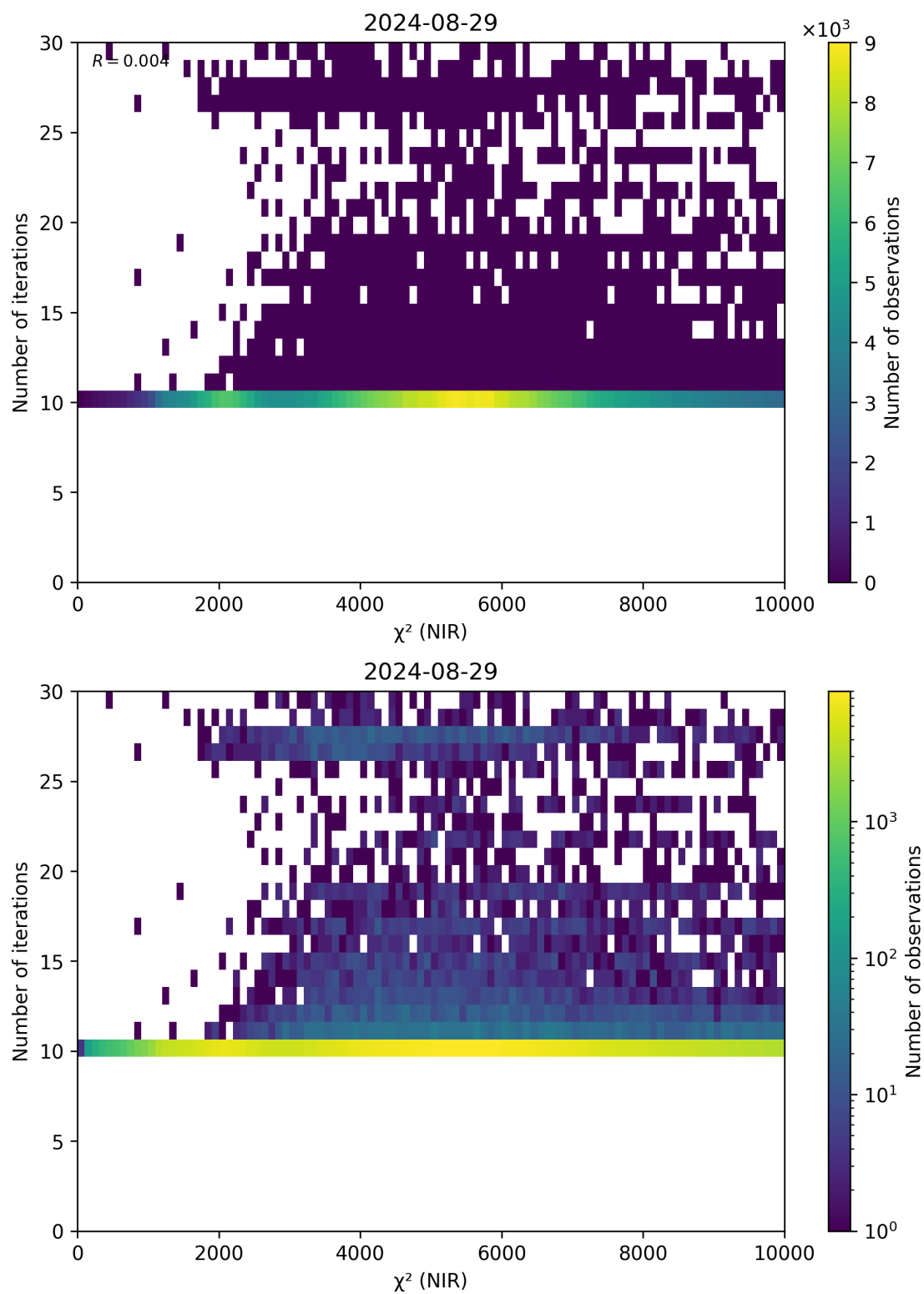
Figure 46: Scatter density plot of “ \chi^2 (NIR)” against “Number of iterations” for 2024-08-28 to 2024-08-30.
