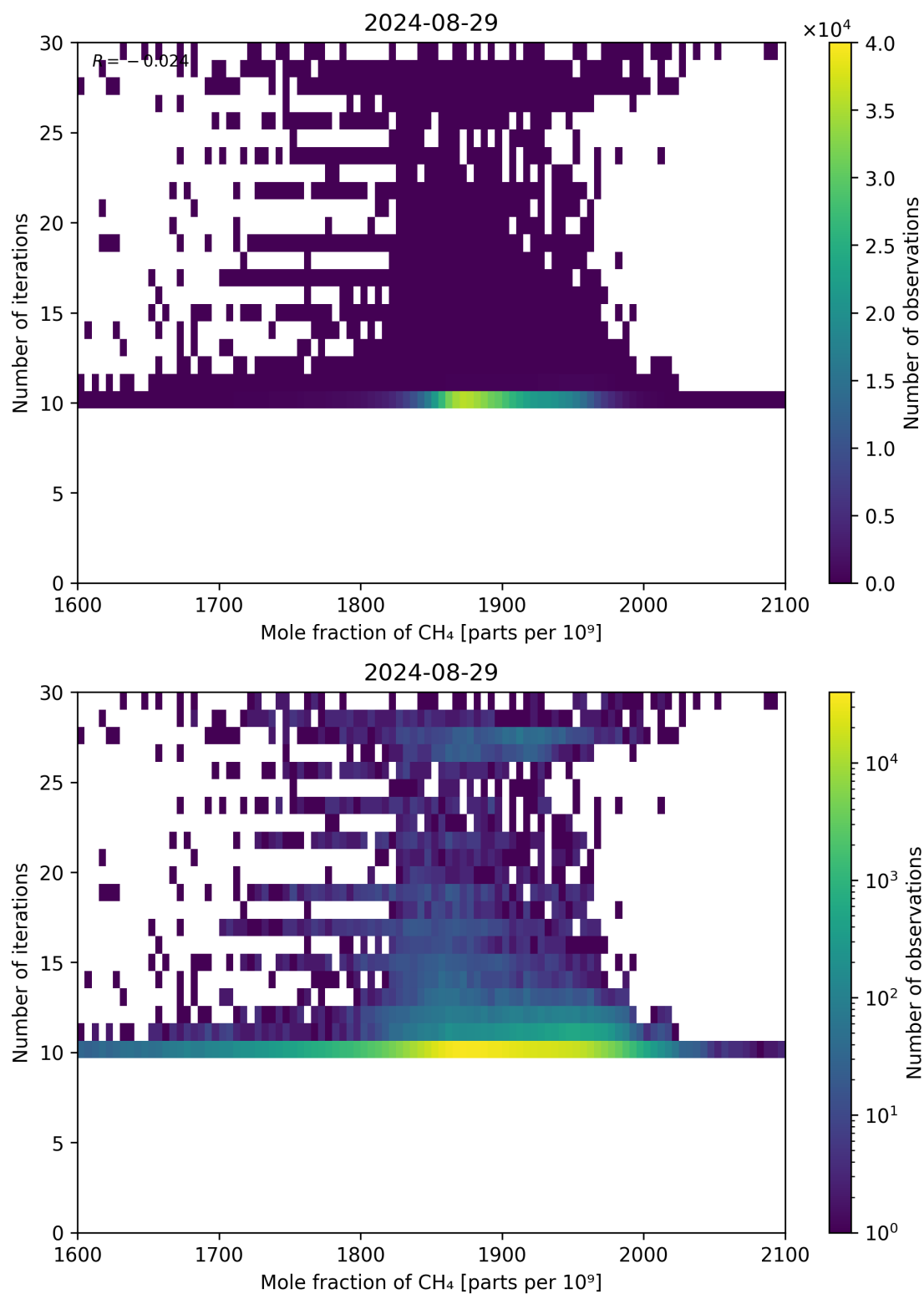
Figure 76: Scatter density plot of “Mole fraction of CH 4 ” against “Number of iterations” for 2024-08-28 to 2024-08-30.
