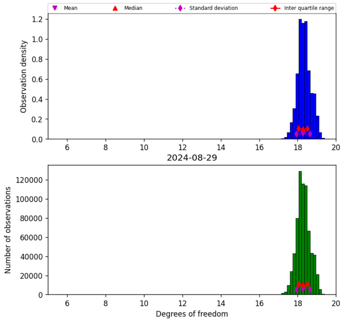
Figure 30: Histogram of “Degrees of freedom” for 2024-08-28 to 2024-08-30
