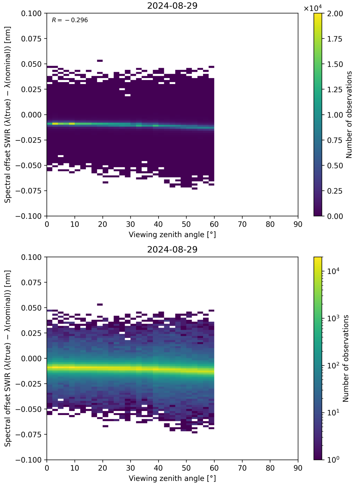
Figure 116: Scatter density plot of “Viewing zenith angle” against “Spectral offset SWIR ( \lambda_{\text{true}} - \lambda_{\text{nominal}} )” for 2024-08-28 to 2024-08-30.
