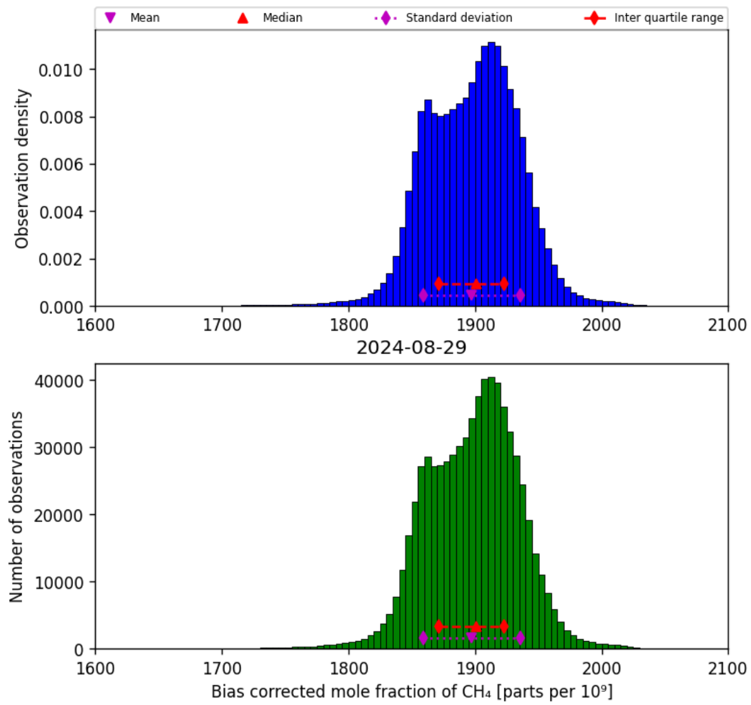
Figure 25: Histogram of “Bias corrected mole fraction of CH 4 ” for 2024-08-28 to 2024-08-30
