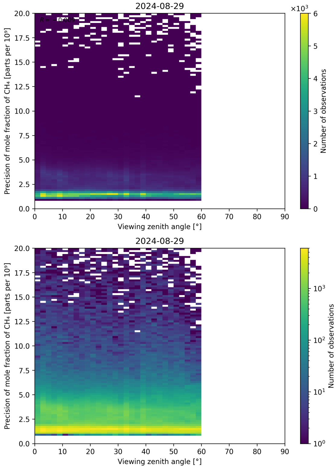
Figure 112: Scatter density plot of “Viewing zenith angle” against “Precision of mole fraction of \text{CH}_4 ” for 2024-08-28 to 2024-08-30.
