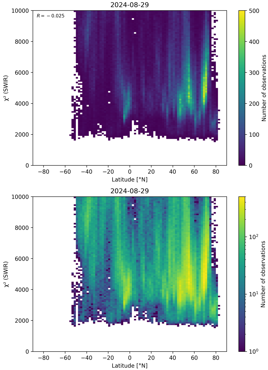
Figure 54: Scatter density plot of “Latitude” against “ \chi^2 (SWIR)” for 2024-08-28 to 2024-08-30.
