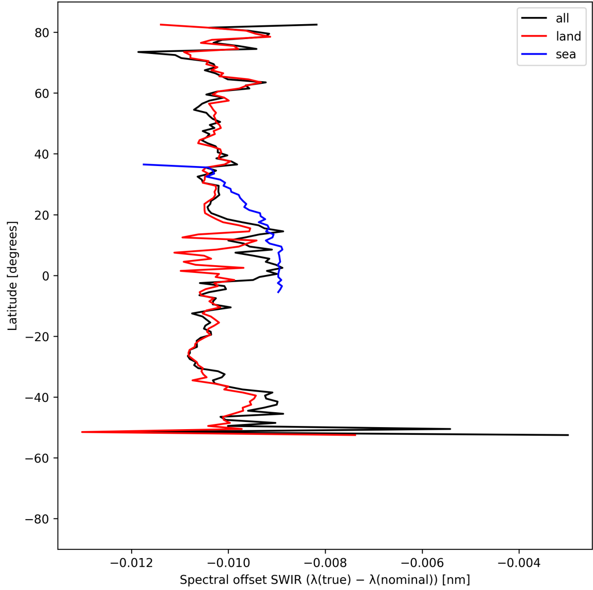
Figure 16: Zonal average of “Spectral offset SWIR ( \lambda_{\text{true}} - \lambda_{\text{nominal}} )” for 2024-08-28 to 2024-08-30.
