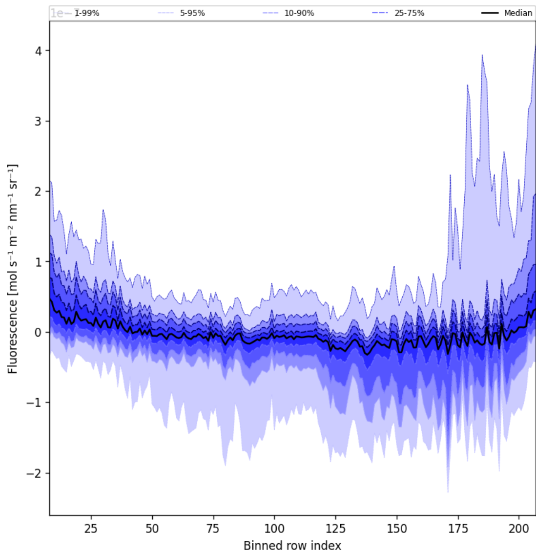
Figure 43: Along track statistics of “Fluorescence” for 2024-08-28 to 2024-08-30
