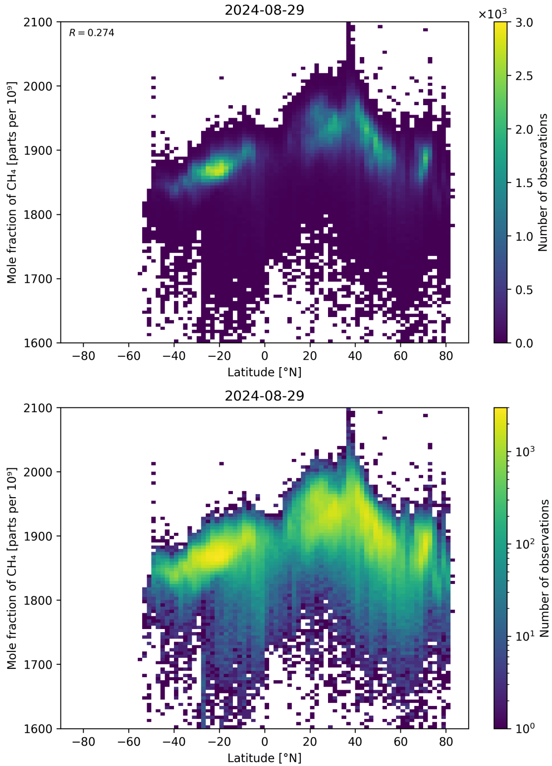
Figure 57: Scatter density plot of “Latitude” against “Mole fraction of \text{CH}_4 ” for 2024-08-28 to 2024-08-30.
