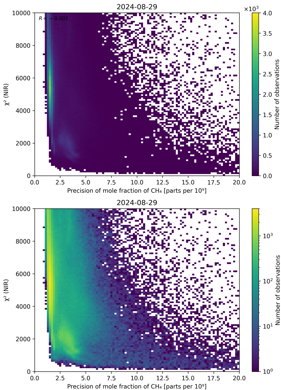
Figure 78: Scatter density plot of “Precision of mole fraction of CH 4 ” against “ \chi^2 (NIR)” for 2024-08-28 to 2024-08-30.
