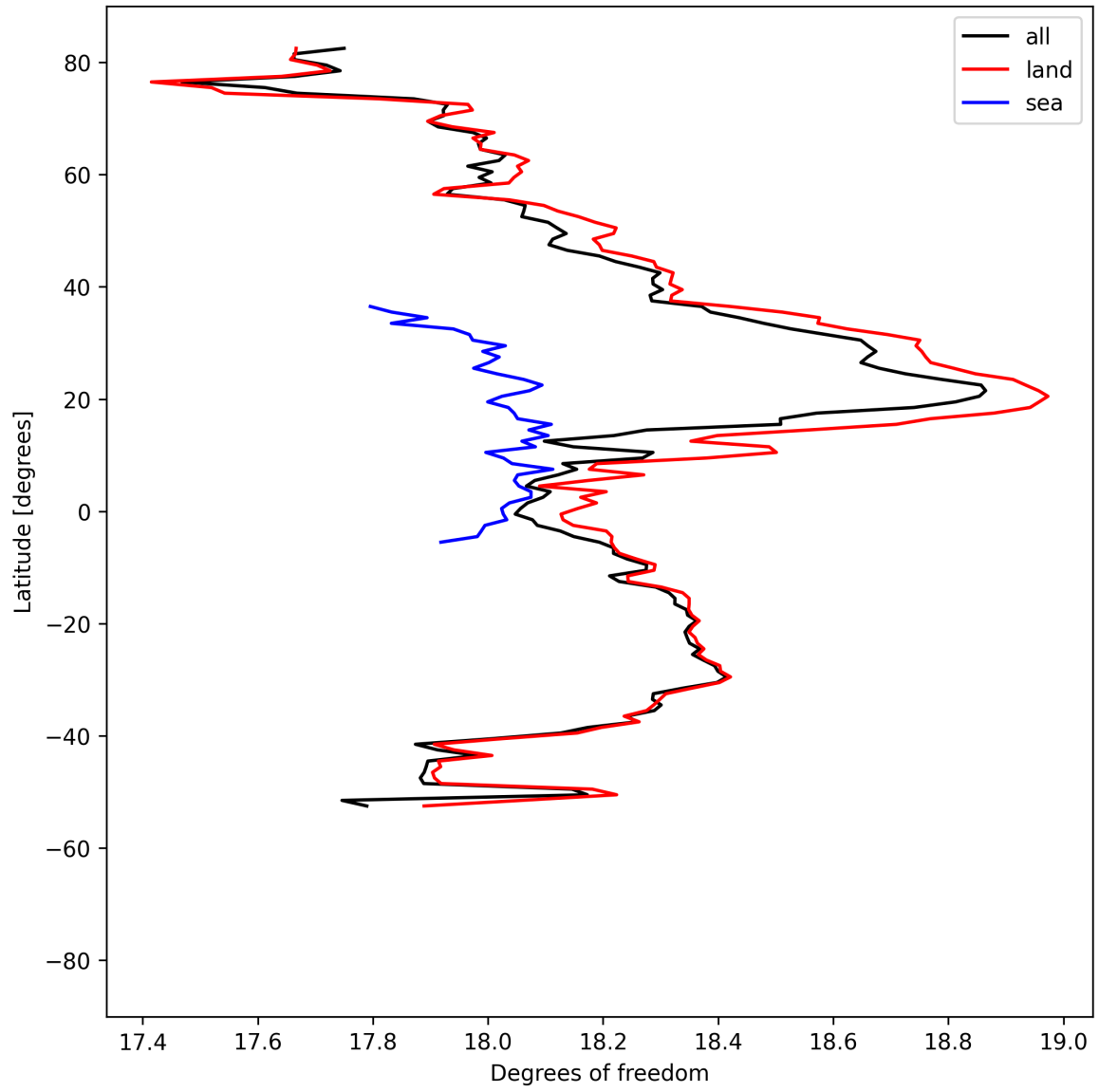
Figure 19: Zonal average of “Degrees of freedom” for 2024-08-28 to 2024-08-30.
