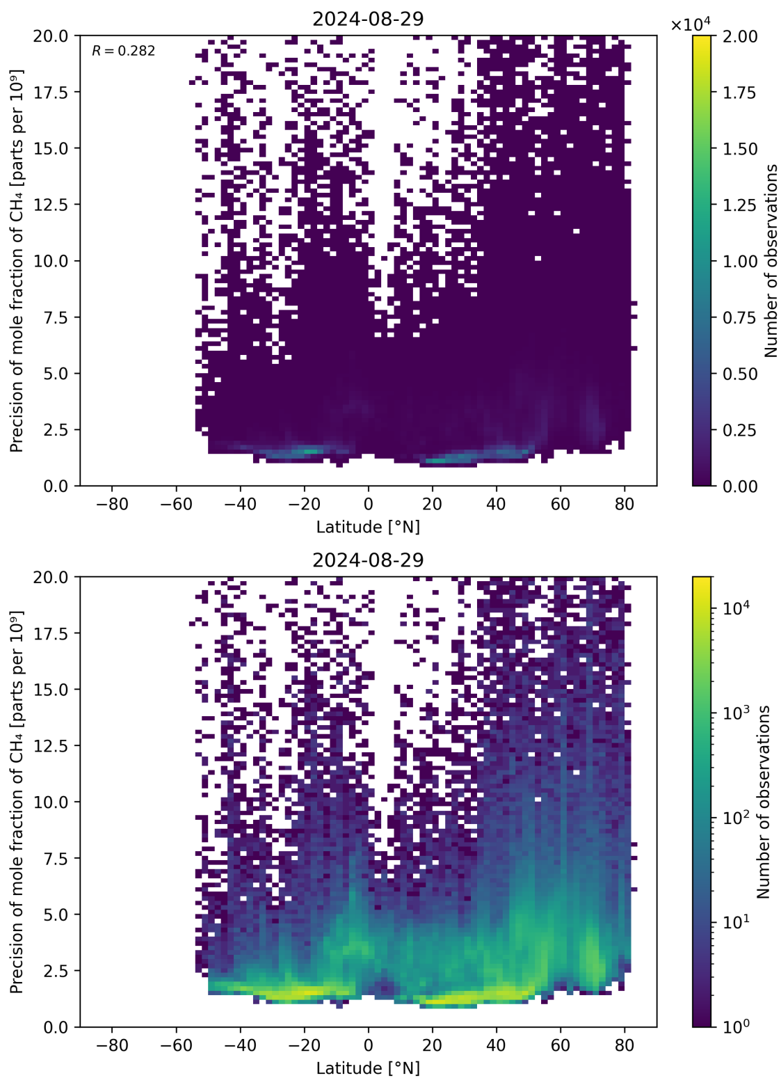
Figure 59: Scatter density plot of “Latitude” against “Precision of mole fraction of \text{CH}_4 ” for 2024-08-28 to 2024-08-30.
