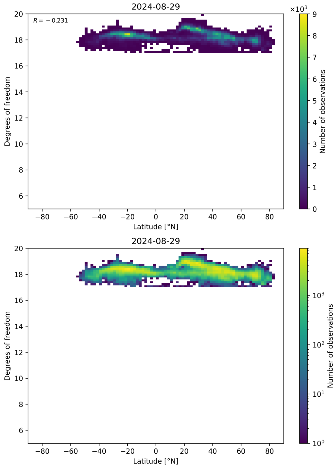
Figure 55: Scatter density plot of “Latitude” against “Degrees of freedom” for 2024-08-28 to 2024-08-30.
