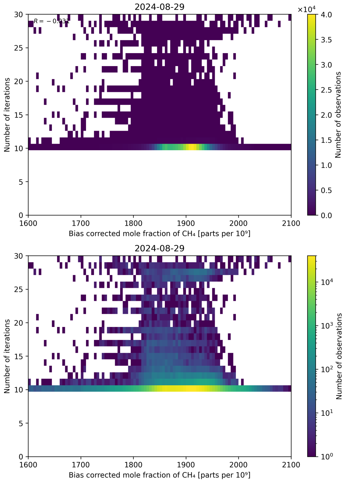
Figure 67: Scatter density plot of “Bias corrected mole fraction of CH 4 ” against “Number of iterations” for 2024-08-28 to 2024-08-30.
