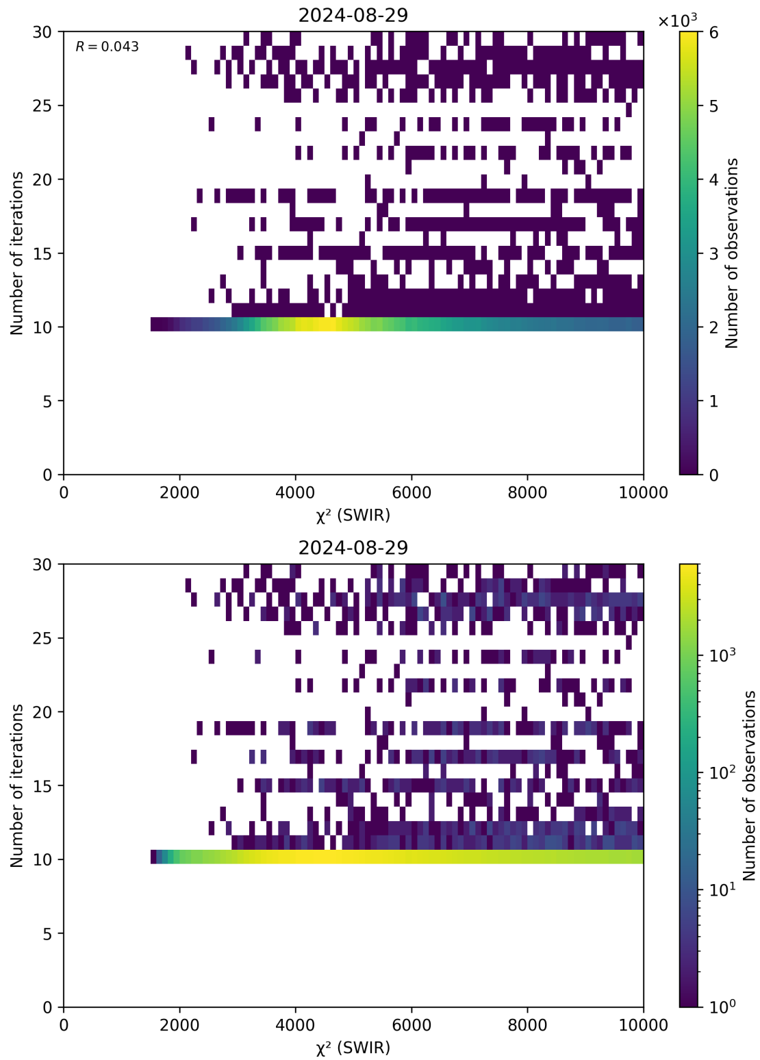
Figure 50: Scatter density plot of “ \chi^2 (SWIR)” against “Number of iterations” for 2024-08-28 to 2024-08-30.
