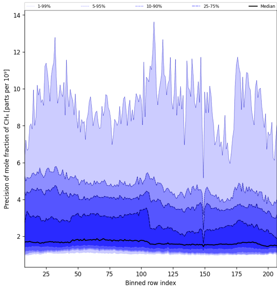
Figure 35: Along track statistics of “Precision of mole fraction of \text{CH}_4 ” for 2024-08-28 to 2024-08-30
