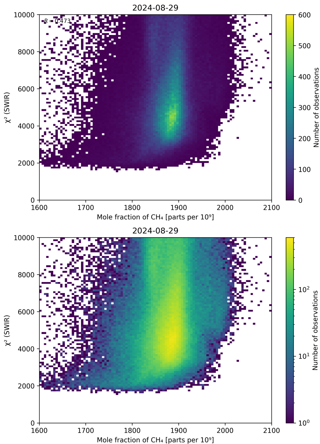
Figure 71: Scatter density plot of “Mole fraction of CH 4 ” against “ \chi^2 (SWIR)” for 2024-08-28 to 2024-08-30.
