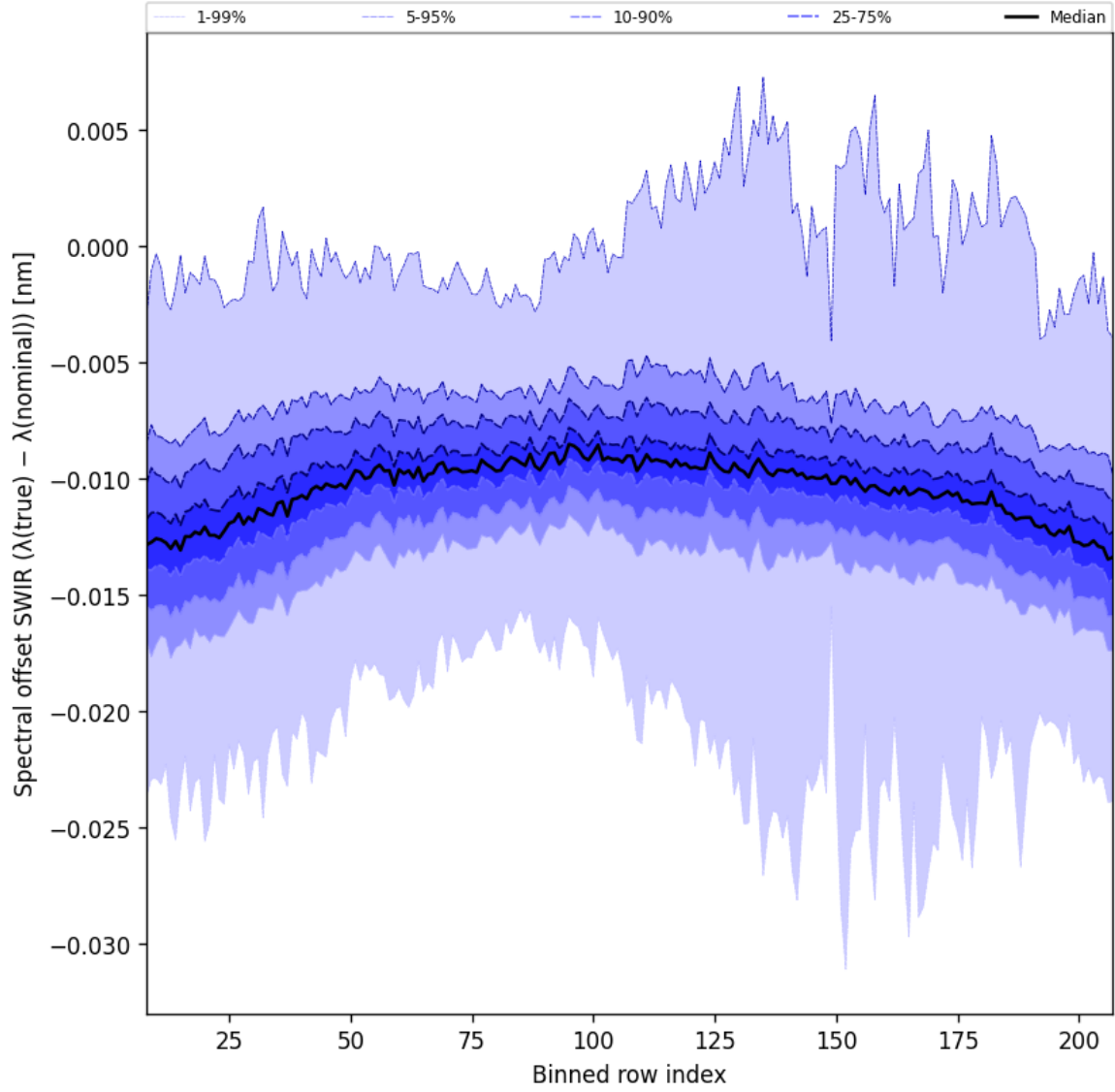
Figure 38: Along track statistics of “Spectral offset SWIR ( \lambda_{\text{true}} - \lambda_{\text{nominal}} )” for 2024-08-29 to 2024-08-31
