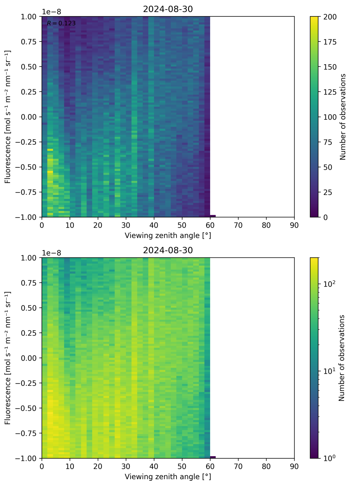
Figure 108: Scatter density plot of “Viewing zenith angle” against “Fluorescence” for 2024-08-29 to 2024-08-31.
