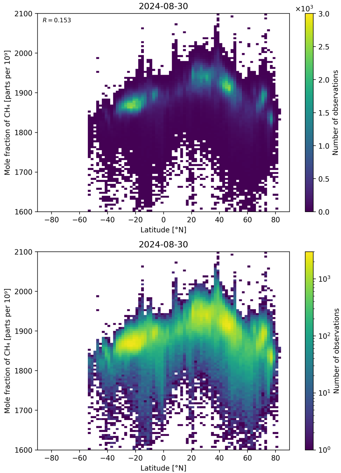
Figure 57: Scatter density plot of “Latitude” against “Mole fraction of CH 4 ” for 2024-08-29 to 2024-08-31.
