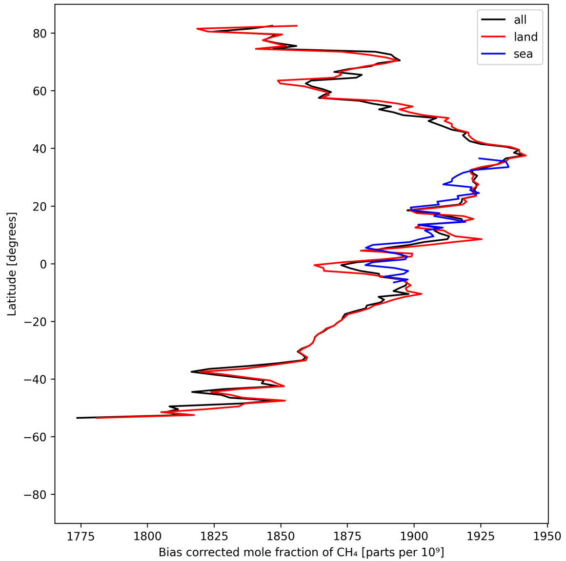
Figure 14: Zonal average of “Bias corrected mole fraction of CH 4 ” for 2024-08-29 to 2024-08-31.
