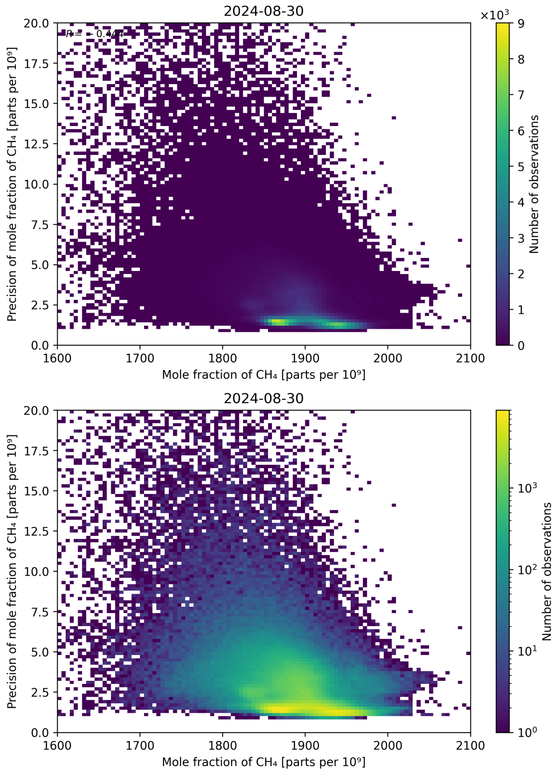
Figure 75: Scatter density plot of “Mole fraction of CH 4 ” against “Precision of mole fraction of CH 4 ” for 2024-08-29 to 2024-08-31.
