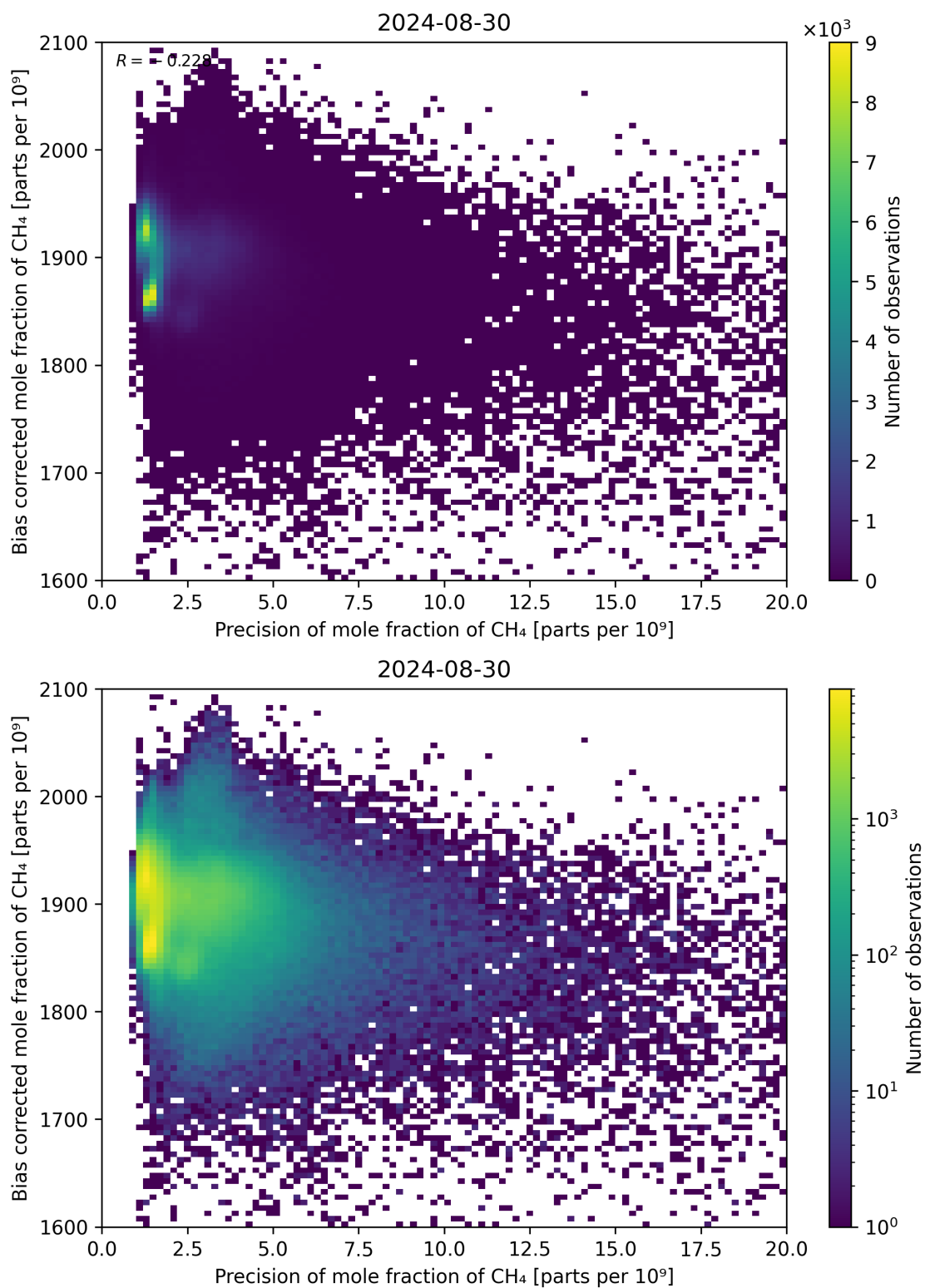
Figure 82: Scatter density plot of “Precision of mole fraction of CH 4 ” against “Bias corrected mole fraction of CH 4 ” for 2024-08-29 to 2024-08-31.
