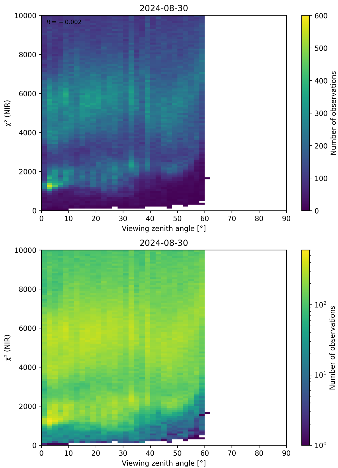
Figure 105: Scatter density plot of “Viewing zenith angle” against “ \chi^2 (NIR)” for 2024-08-29 to 2024-08-31.
