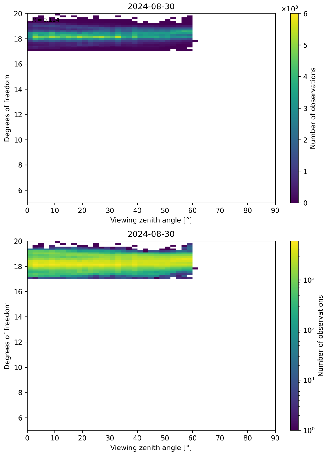
Figure 107: Scatter density plot of “Viewing zenith angle” against “Degrees of freedom” for 2024-08-29 to 2024-08-31.
