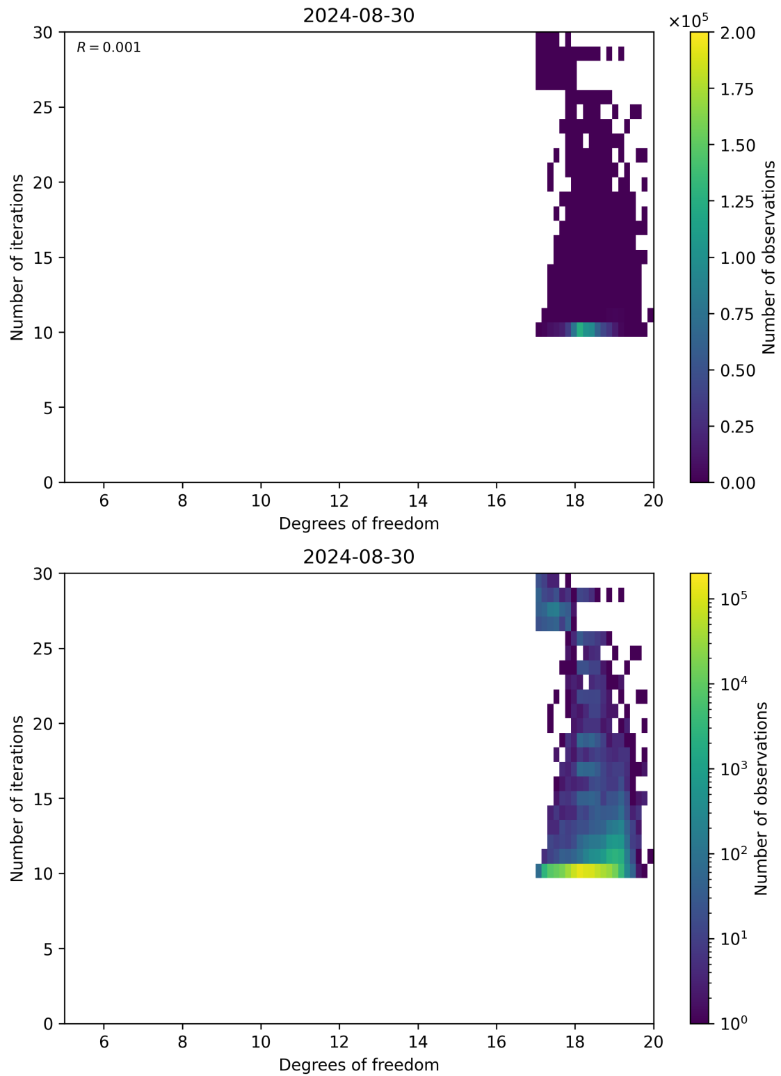
Figure 52: Scatter density plot of “Degrees of freedom” against “Number of iterations” for 2024-08-29 to 2024-08-31.
