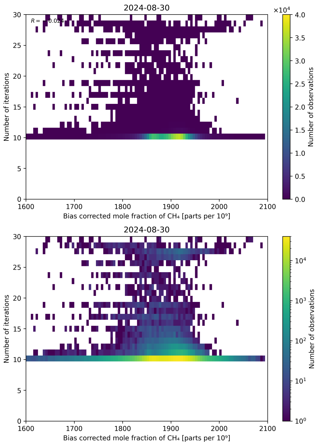
Figure 67: Scatter density plot of “Bias corrected mole fraction of \text{CH}_4 ” against “Number of iterations” for 2024-08-29 to 2024-08-31.
