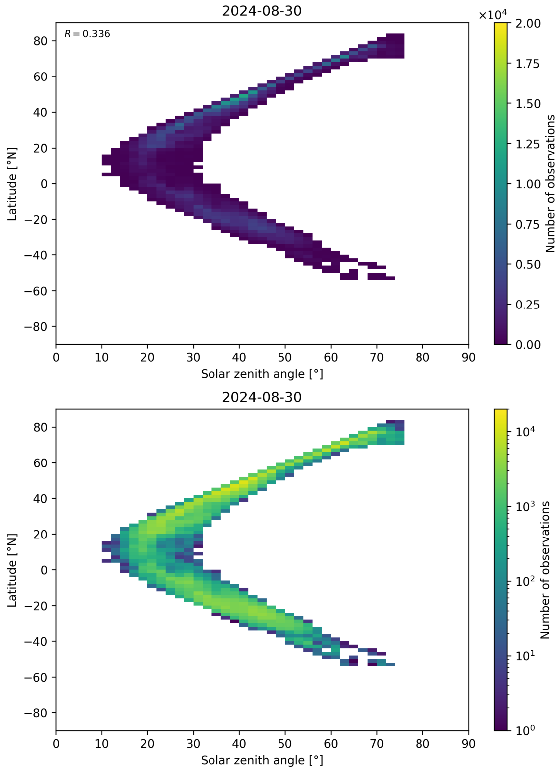
Figure 98: Scatter density plot of “Solar zenith angle” against “Latitude” for 2024-08-29 to 2024-08-31.
