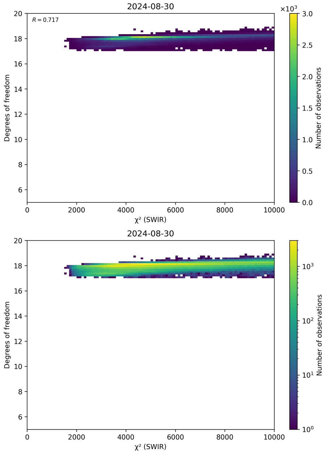
Figure 48: Scatter density plot of “ \chi^2 (SWIR)” against “Degrees of freedom” for 2024-08-29 to 2024-08-31.
