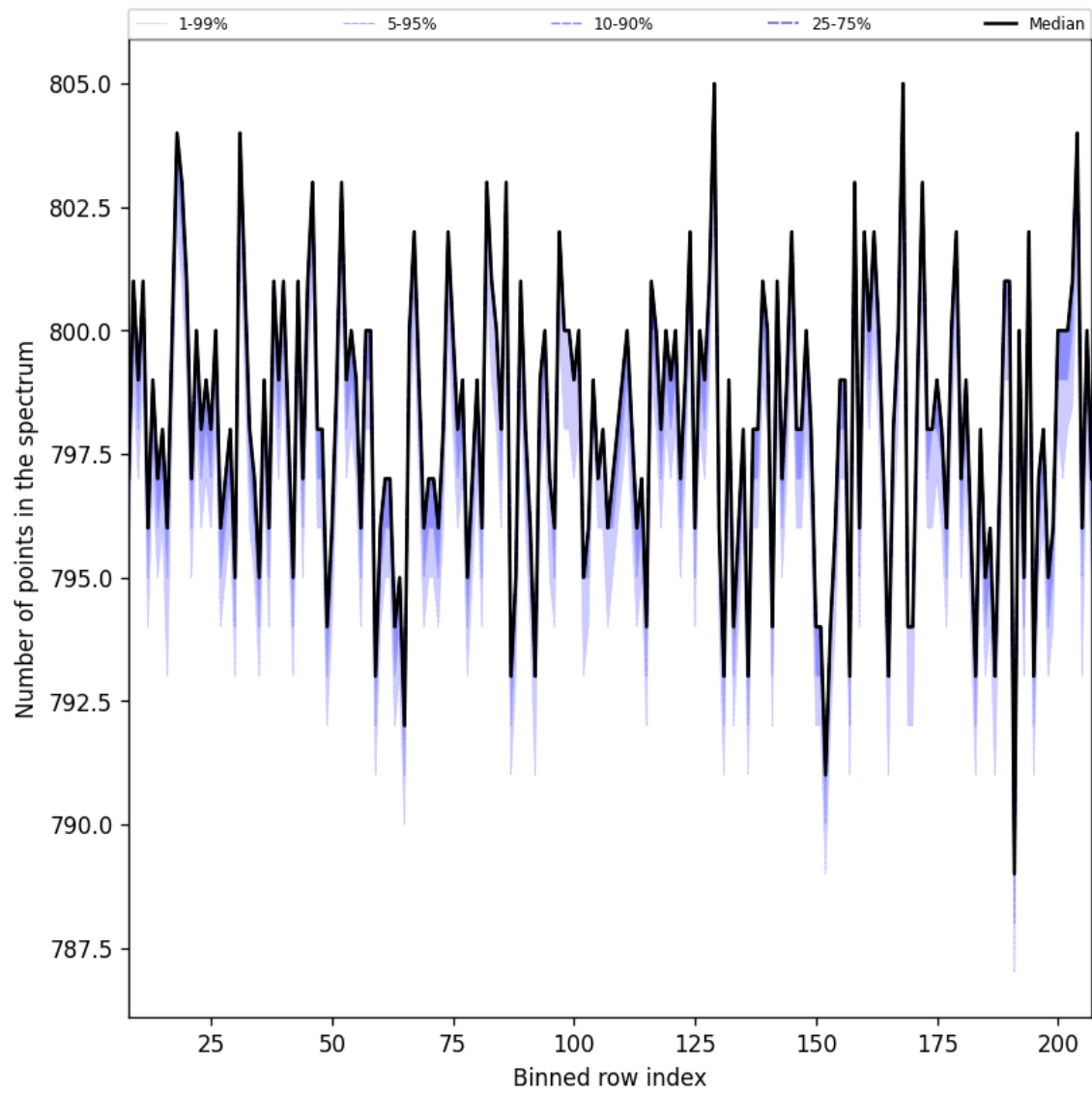
Figure 37: Along track statistics of “Number of points in the spectrum” for 2024-08-29 to 2024-08-31
