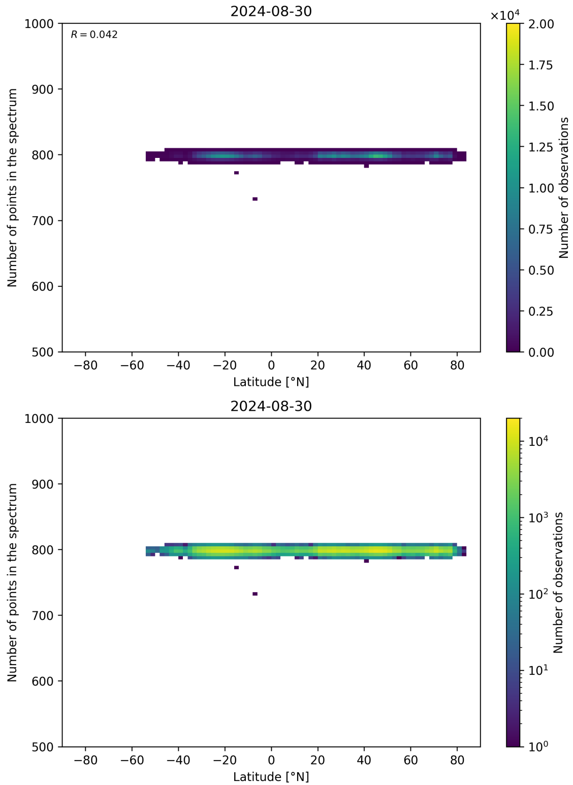
Figure 61: Scatter density plot of “Latitude” against “Number of points in the spectrum” for 2024-08-29 to 2024-08-31.
