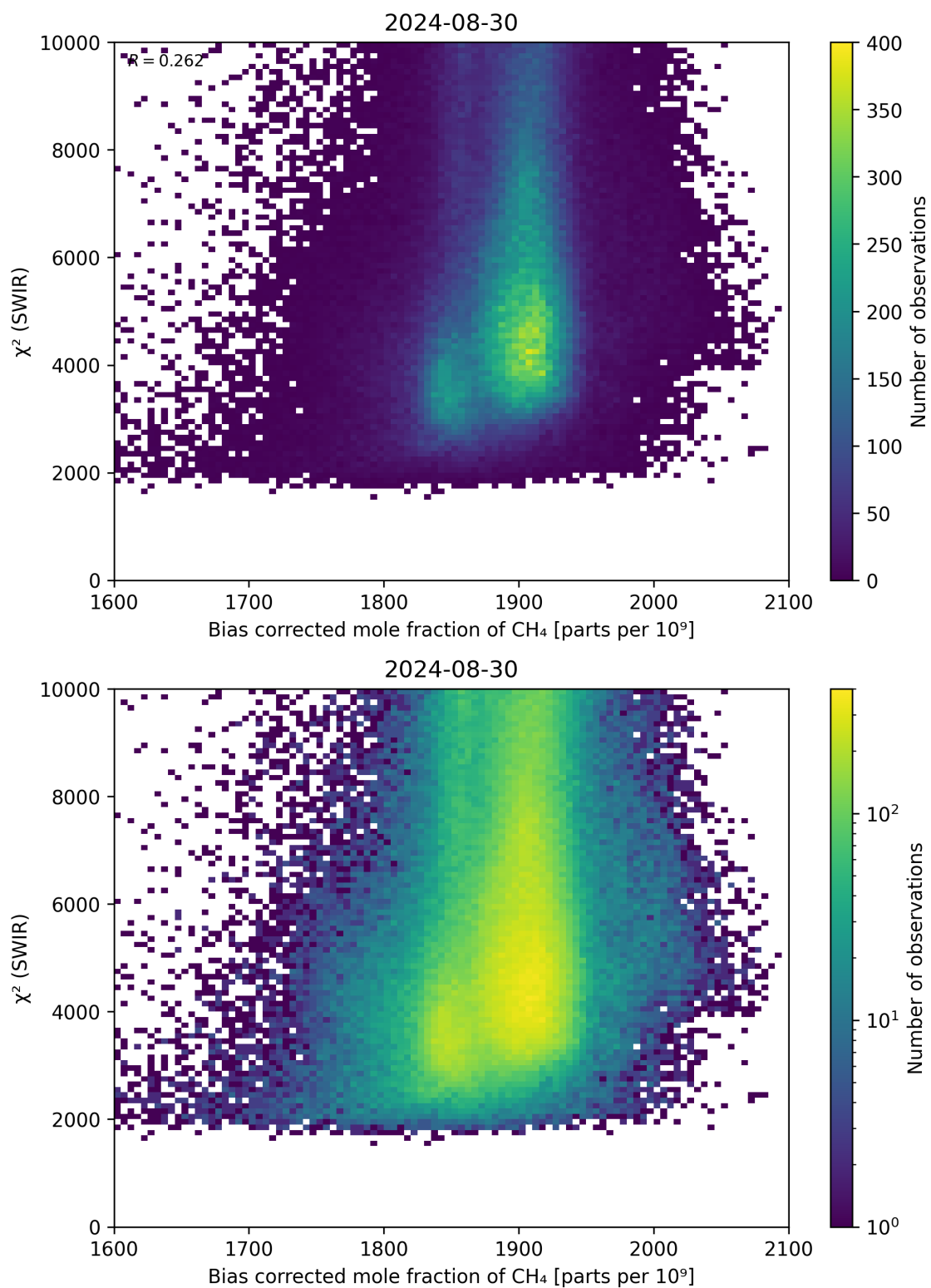
Figure 64: Scatter density plot of “Bias corrected mole fraction of \text{CH}_4 ” against “ \chi^2 (SWIR)” for 2024-08-29 to 2024-08-31.
