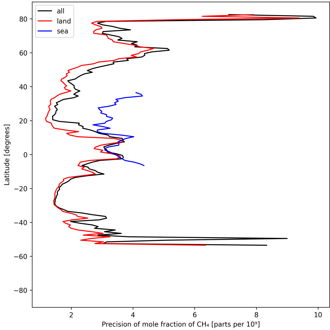
Figure 13: Zonal average of “Precision of mole fraction of \text{CH}_4 ” for 2024-08-29 to 2024-08-31.
