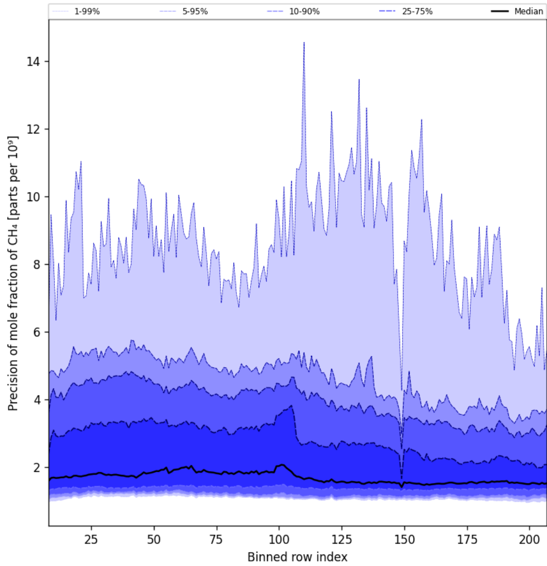
Figure 35: Along track statistics of “Precision of mole fraction of CH 4 ” for 2024-08-29 to 2024-08-31
