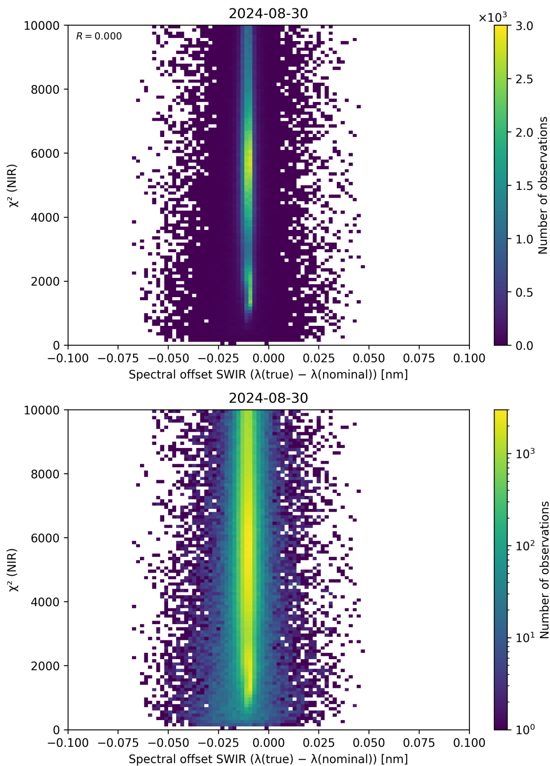
Figure 117: Scatter density plot of “Spectral offset SWIR ( \lambda_{\text{true}} - \lambda_{\text{nominal}} )” against “ \chi^2 (NIR)” for 2024-08-29 to 2024-08-31.
