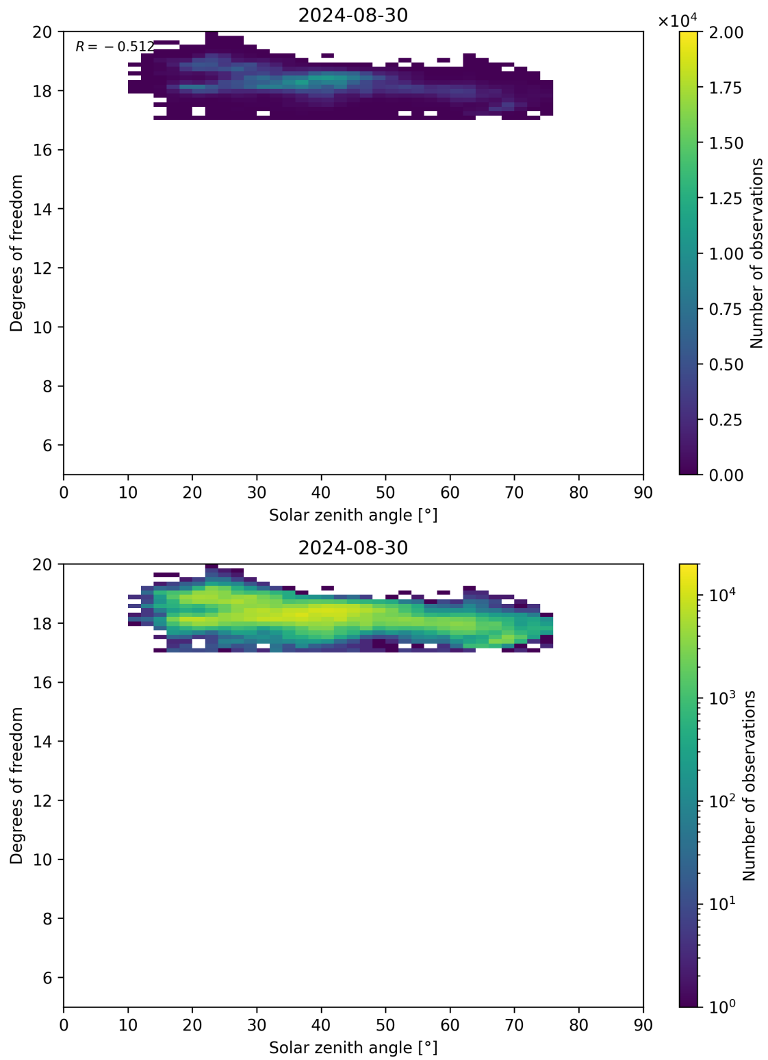
Figure 96: Scatter density plot of “Solar zenith angle” against “Degrees of freedom” for 2024-08-29 to 2024-08-31.
