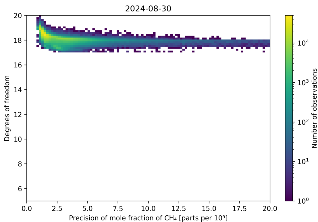
Figure 80: Scatter density plot of “Precision of mole fraction of CH 4 ” against “Degrees of freedom” for 2024-08-29 to 2024-08-31.
