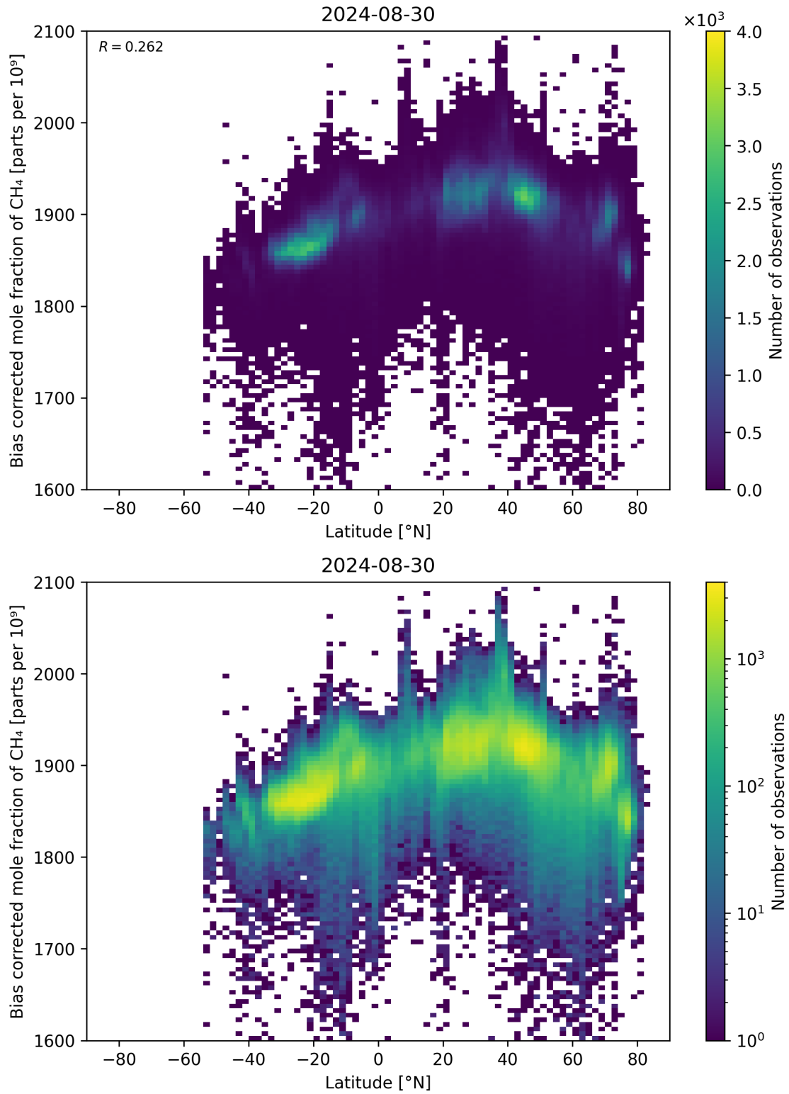
Figure 58: Scatter density plot of “Latitude” against “Bias corrected mole fraction of CH 4 ” for 2024-08-29 to 2024-08-31.
