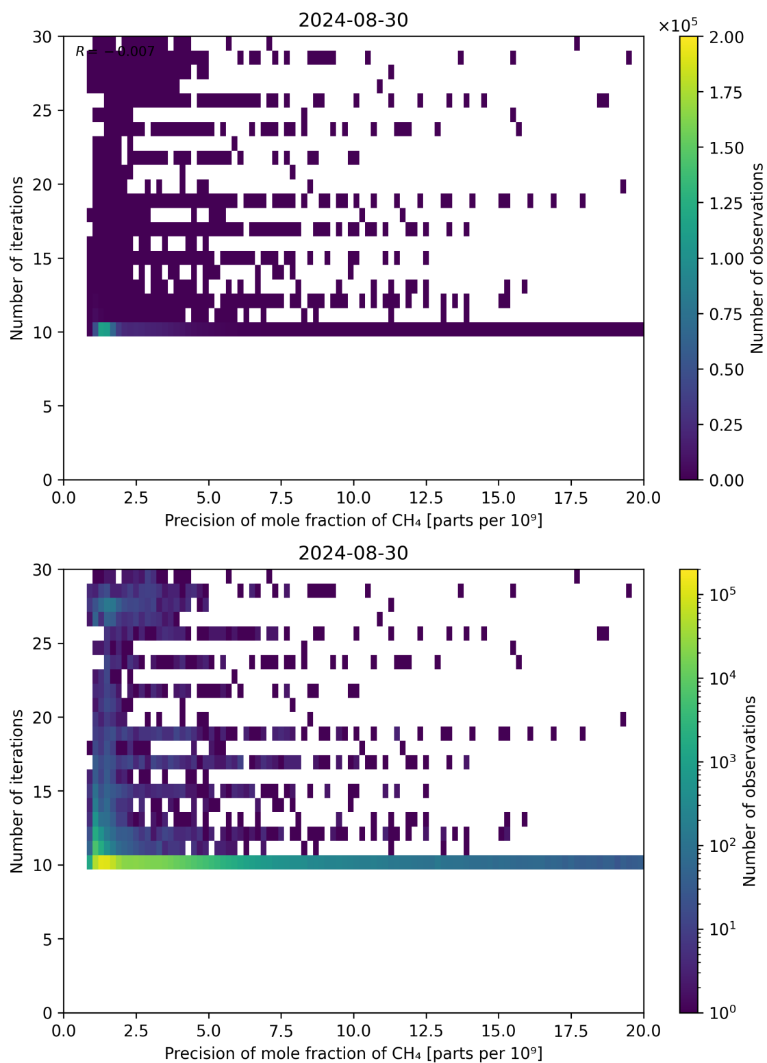
Figure 83: Scatter density plot of “Precision of mole fraction of CH 4 ” against “Number of iterations” for 2024-08-29 to 2024-08-31.
