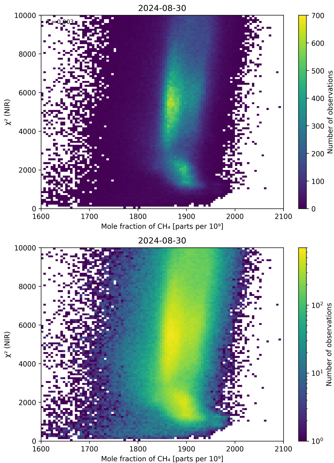
Figure 70: Scatter density plot of “Mole fraction of \text{CH}_4 ” against “ \chi^2 (NIR)” for 2024-08-29 to 2024-08-31.
