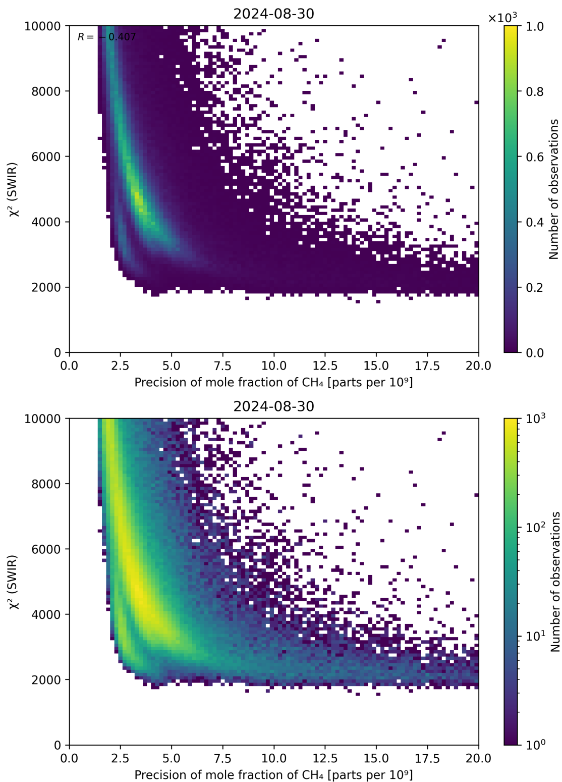
Figure 79: Scatter density plot of “Precision of mole fraction of \text{CH}_4 ” against “ \chi^2 (SWIR)” for 2024-08-29 to 2024-08-31.
