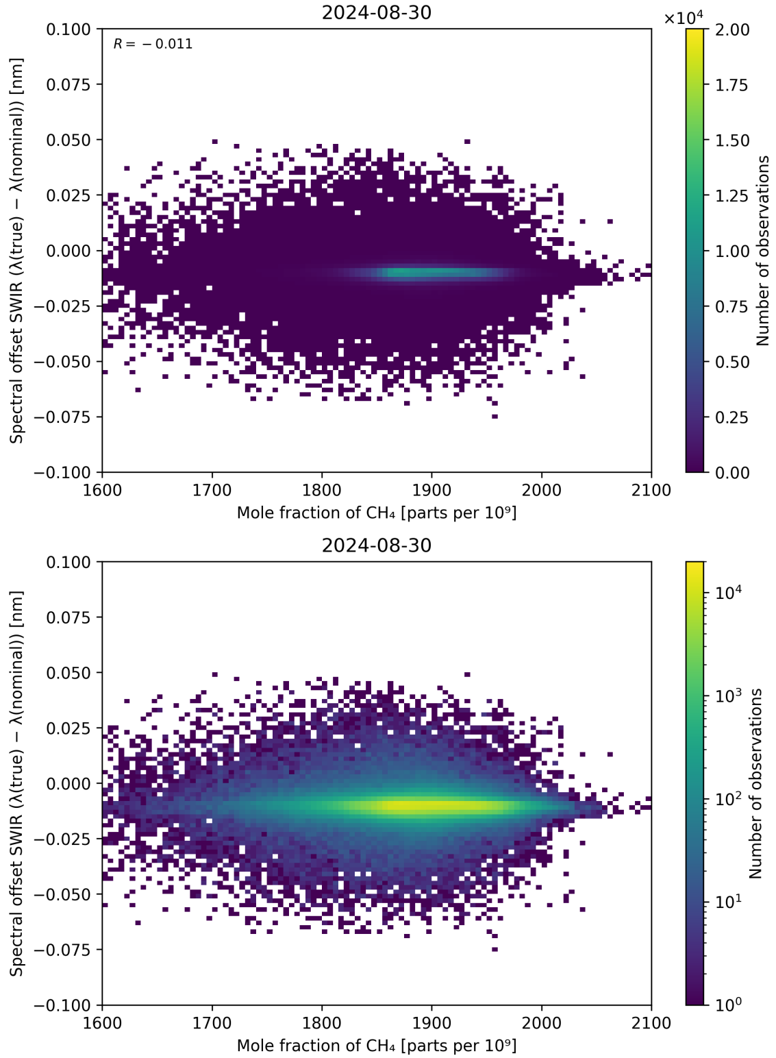
Figure 86: Scatter density plot of “Mole fraction of CH 4 ” against “Spectral offset SWIR ( \lambda_{\text{true}} - \lambda_{\text{nominal}} )” for 2024-08-29 to 2024-08-31.
