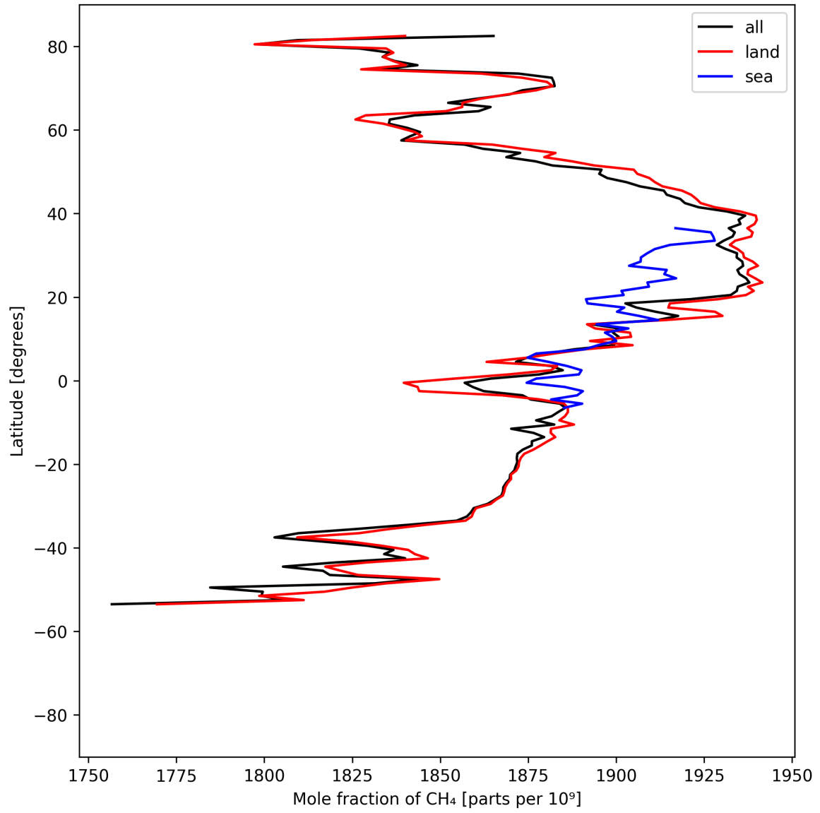
Figure 12: Zonal average of “Mole fraction of \text{CH}_4 ” for 2024-08-29 to 2024-08-31.
