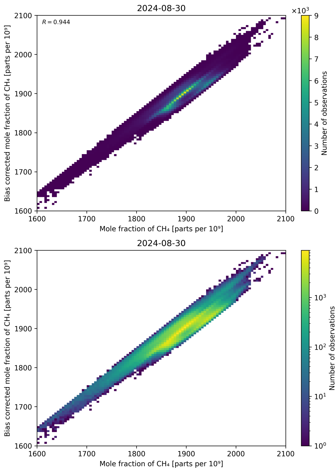
Figure 74: Scatter density plot of “Mole fraction of CH 4 ” against “Bias corrected mole fraction of CH 4 ” for 2024-08-29 to 2024-08-31.
