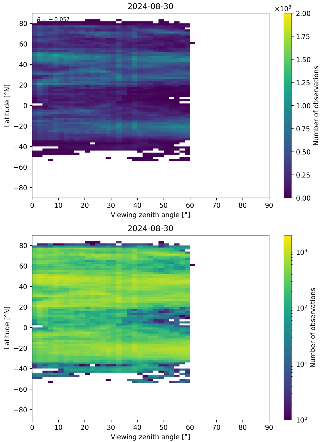
Figure 109: Scatter density plot of “Viewing zenith angle” against “Latitude” for 2024-08-29 to 2024-08-31.
