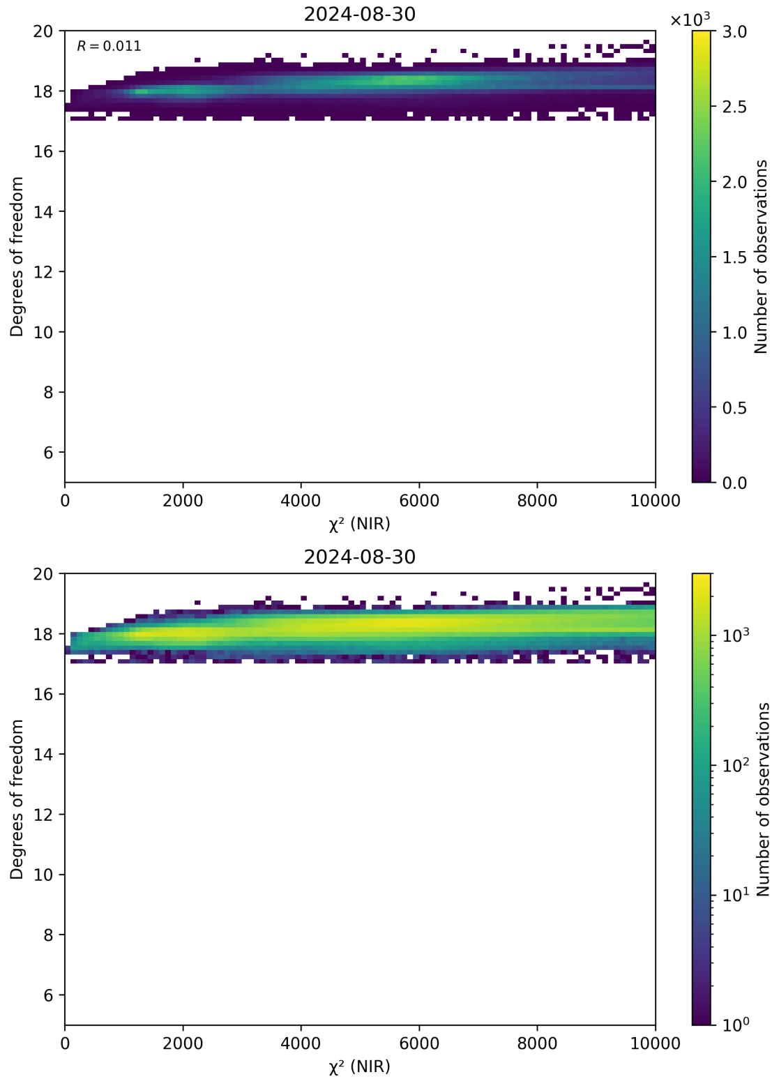
Figure 44: Scatter density plot of “ \chi^2 (NIR)” against “Degrees of freedom” for 2024-08-29 to 2024-08-31.
