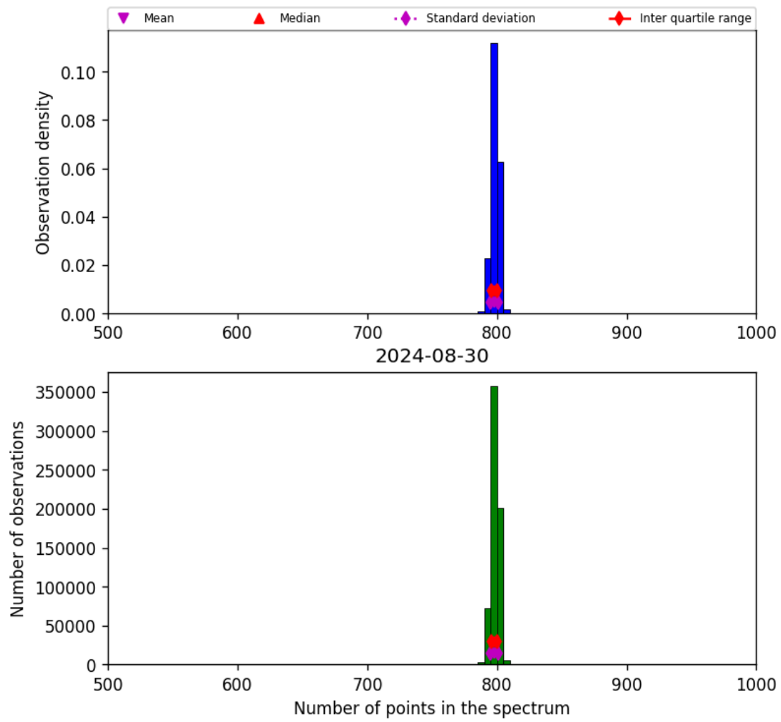
Figure 26: Histogram of “Number of points in the spectrum” for 2024-08-29 to 2024-08-31
