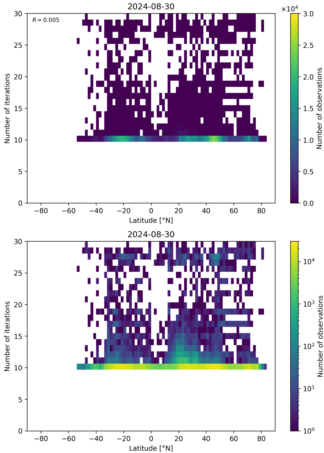
Figure 60: Scatter density plot of “Latitude” against “Number of iterations” for 2024-08-29 to 2024-08-31.
