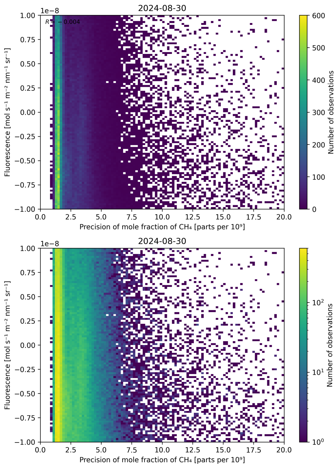
Figure 81: Scatter density plot of “Precision of mole fraction of \text{CH}_4 ” against “Fluorescence” for 2024-08-29 to 2024-08-31.
