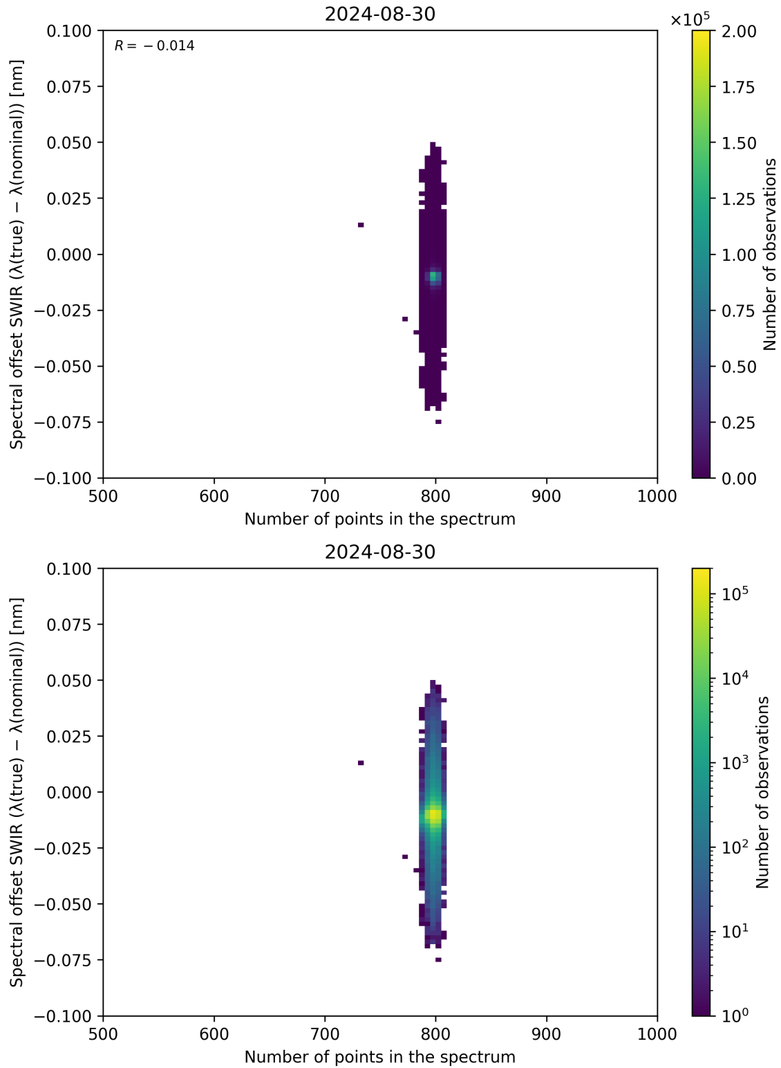
Figure 93: Scatter density plot of “Number of points in the spectrum” against “Spectral offset SWIR ( \lambda_{\text{true}} - \lambda_{\text{nominal}} )” for 2024-08-29 to 2024-08-31.
