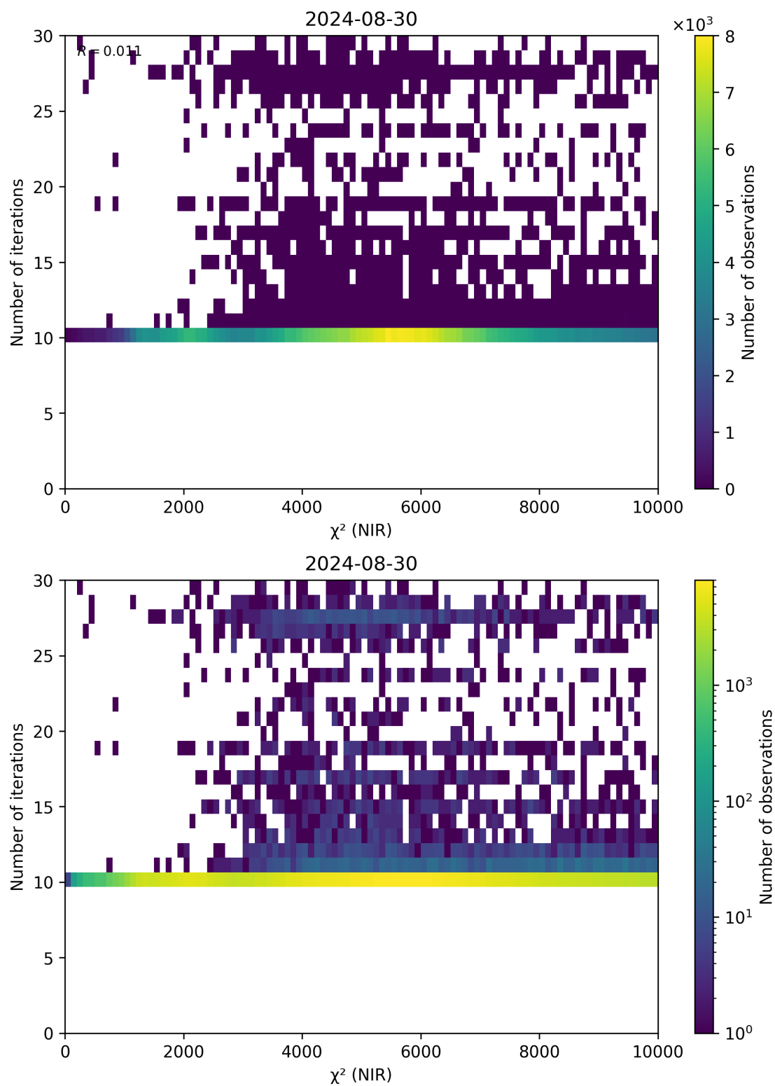
Figure 46: Scatter density plot of “ \chi^2 (NIR)” against “Number of iterations” for 2024-08-29 to 2024-08-31.
