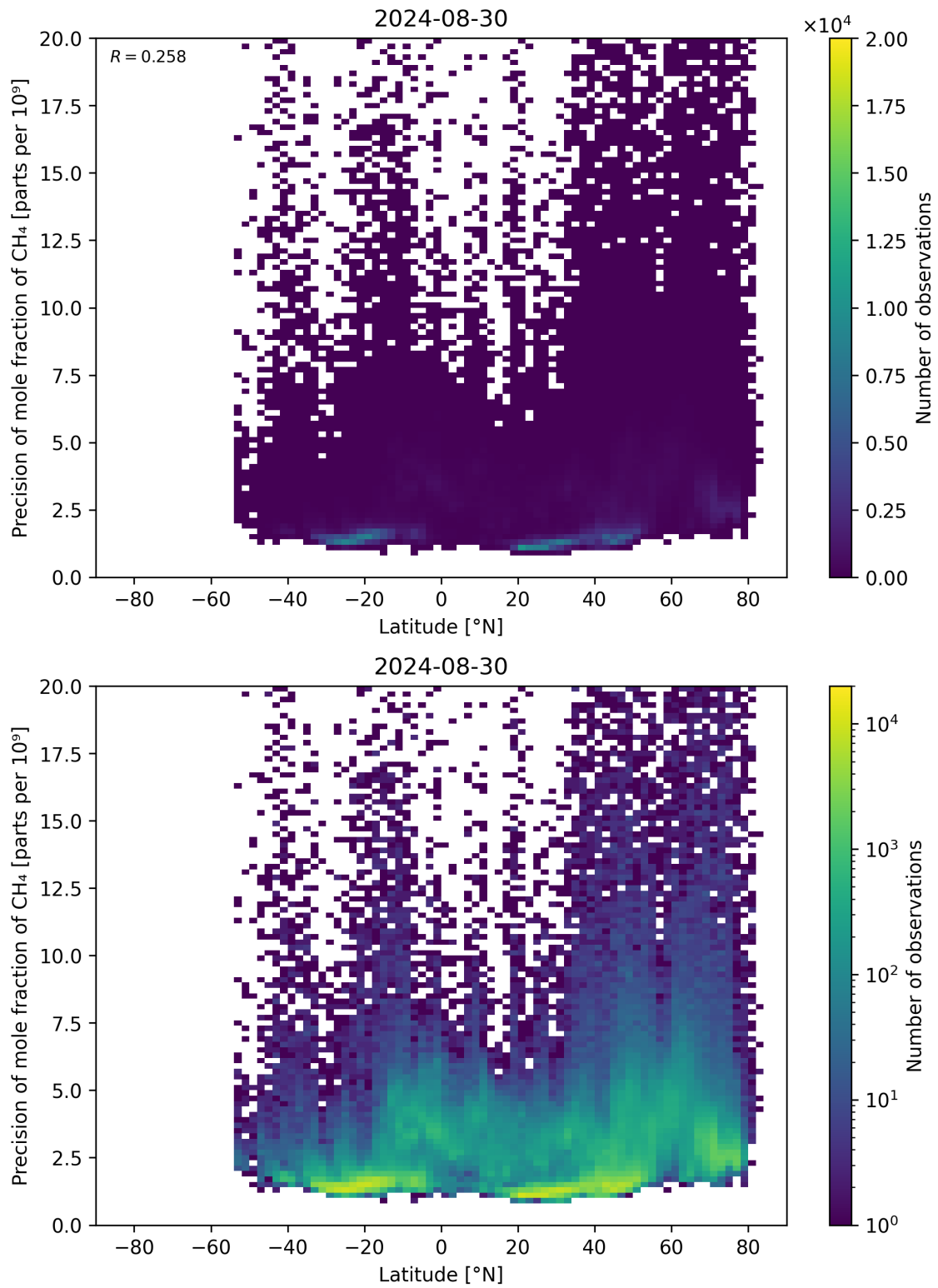
Figure 59: Scatter density plot of “Latitude” against “Precision of mole fraction of \text{CH}_4 ” for 2024-08-29 to 2024-08-31.
