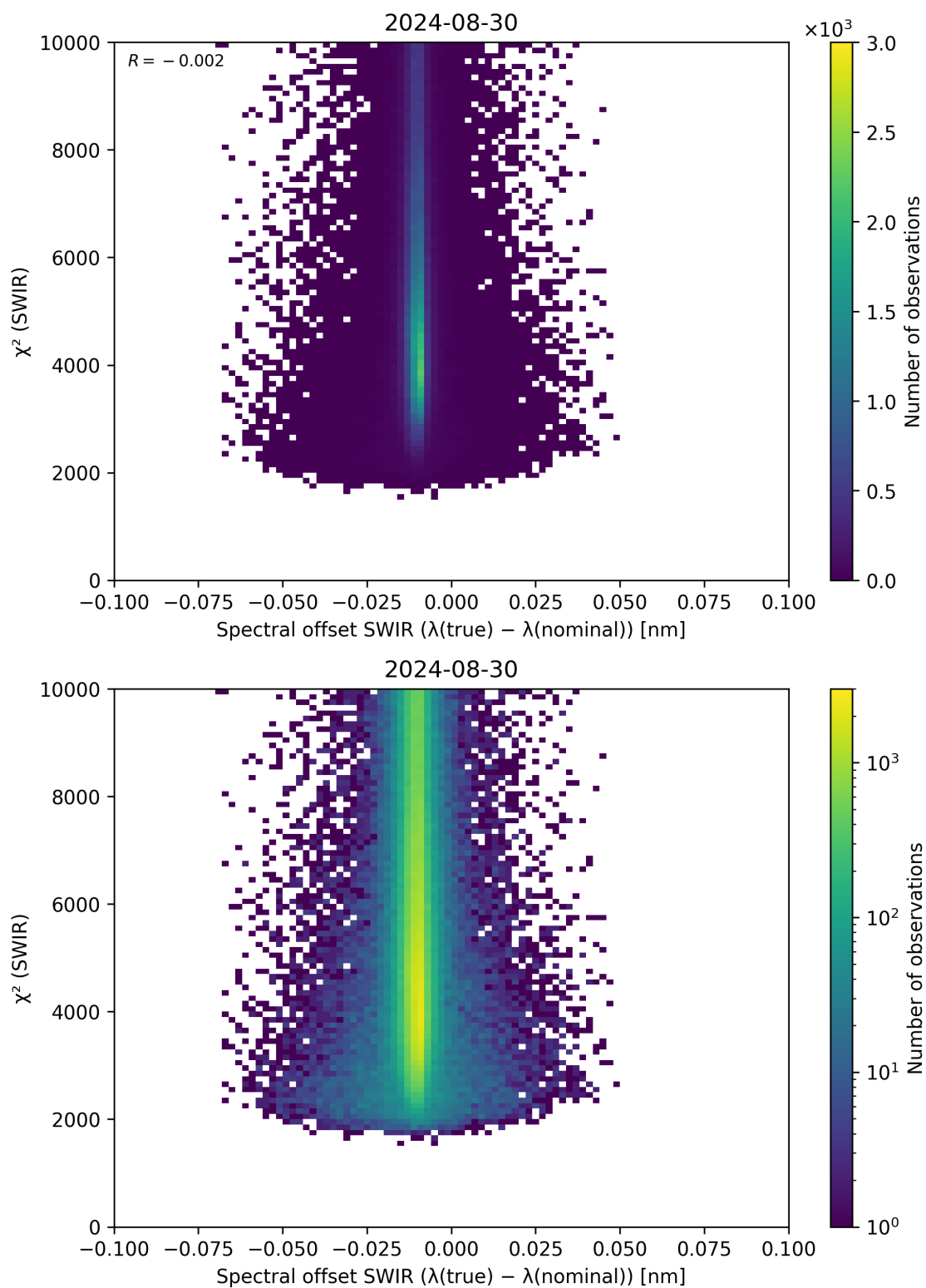
Figure 118: Scatter density plot of “Spectral offset SWIR ( \lambda_{\text{true}} - \lambda_{\text{nominal}} )” against “ \chi^2 (SWIR)” for 2024-08-29 to 2024-08-31.
