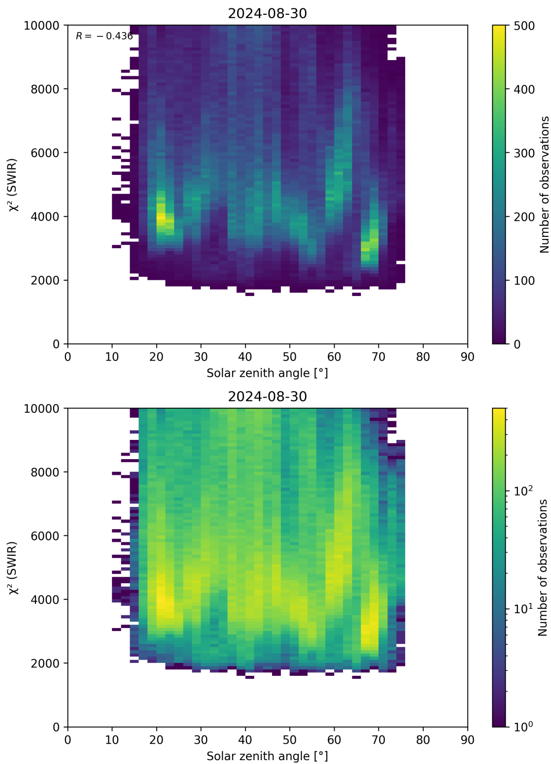
Figure 95: Scatter density plot of “Solar zenith angle” against “ \chi^2 (SWIR)” for 2024-08-29 to 2024-08-31.
