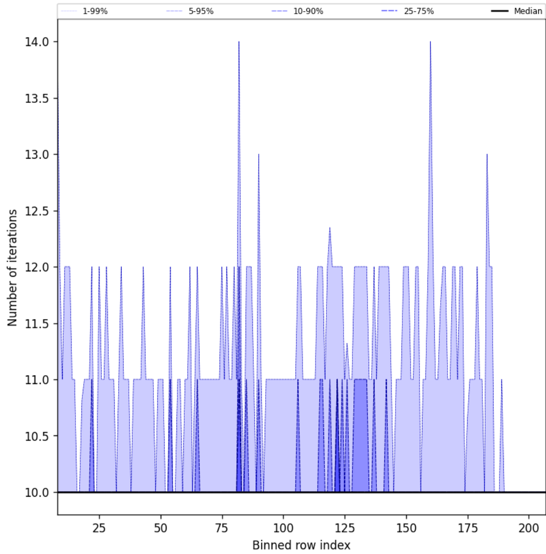
Figure 42: Along track statistics of “Number of iterations” for 2024-08-29 to 2024-08-31
