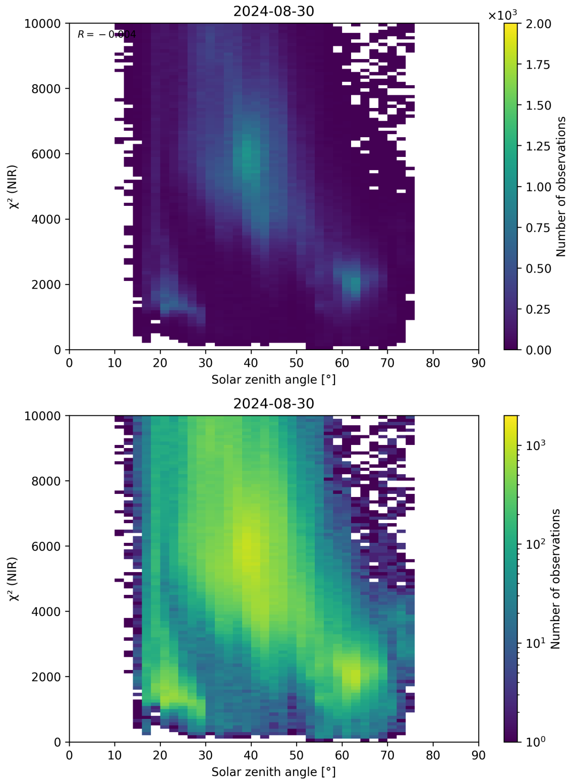
Figure 94: Scatter density plot of “Solar zenith angle” against “ \chi^2 (NIR)” for 2024-08-29 to 2024-08-31.
