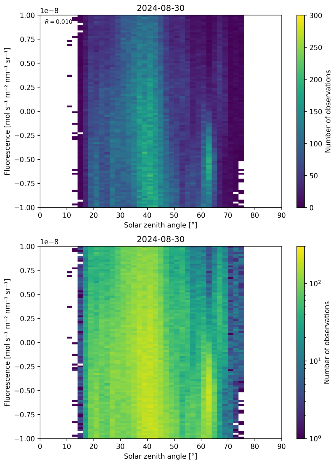
Figure 97: Scatter density plot of “Solar zenith angle” against “Fluorescence” for 2024-08-29 to 2024-08-31.
