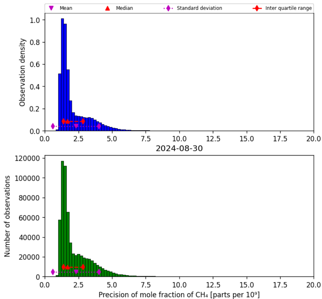
Figure 24: Histogram of “Precision of mole fraction of CH 4 ” for 2024-08-29 to 2024-08-31
