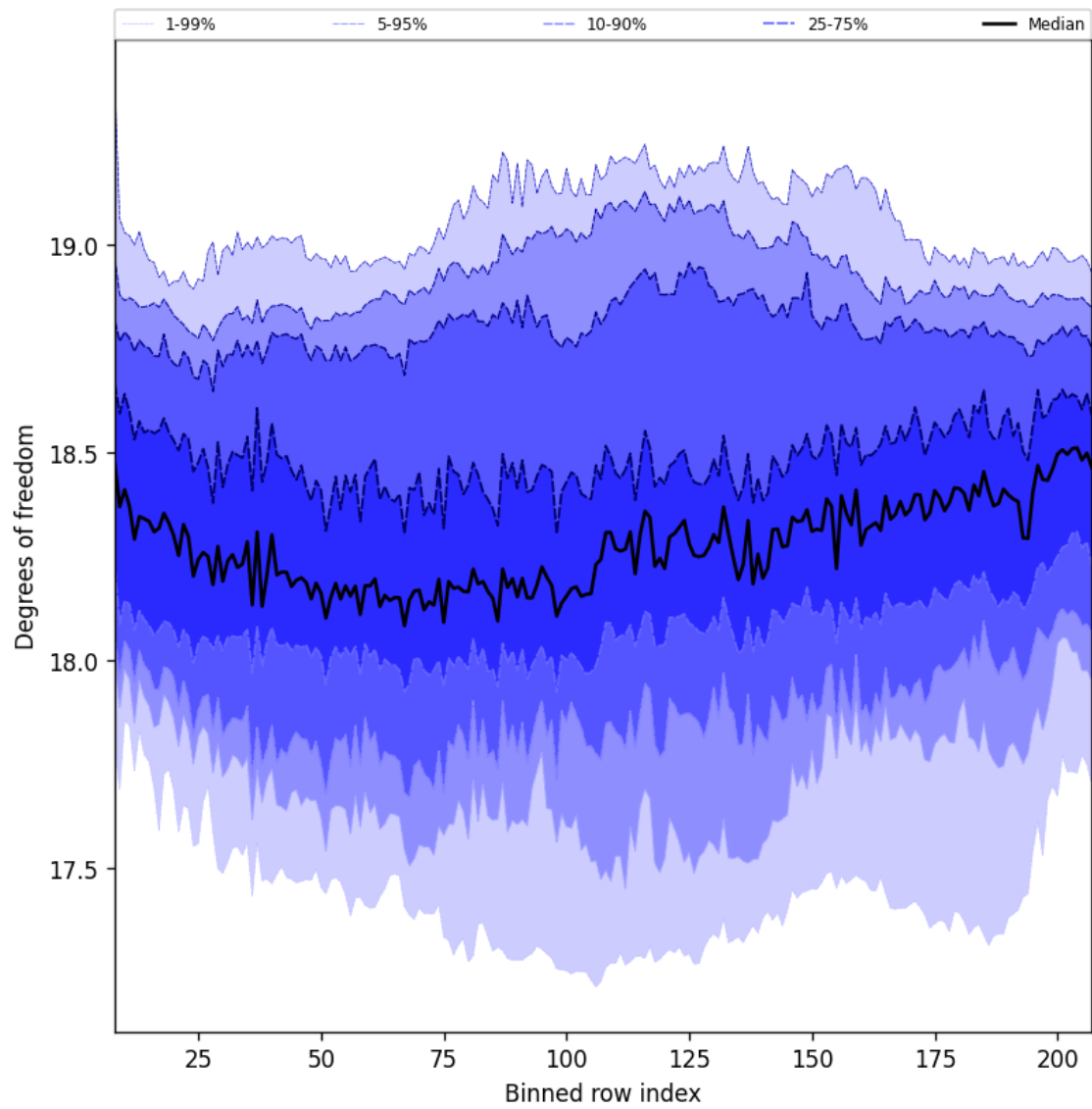
Figure 41: Along track statistics of “Degrees of freedom” for 2024-08-29 to 2024-08-31
