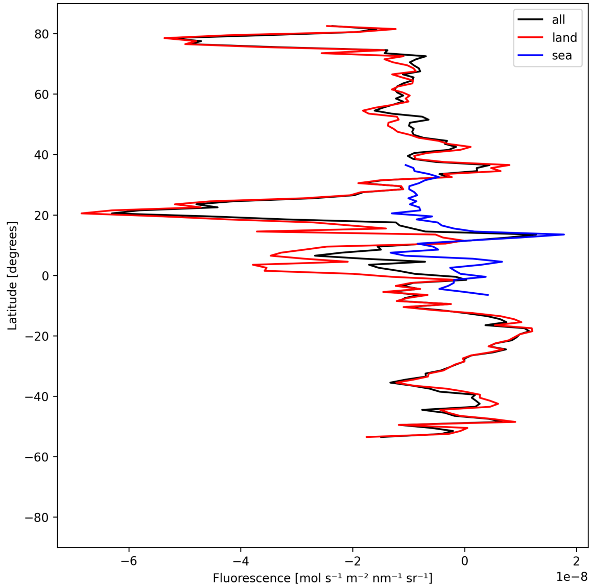
Figure 21: Zonal average of “Fluorescence” for 2024-08-29 to 2024-08-31.
