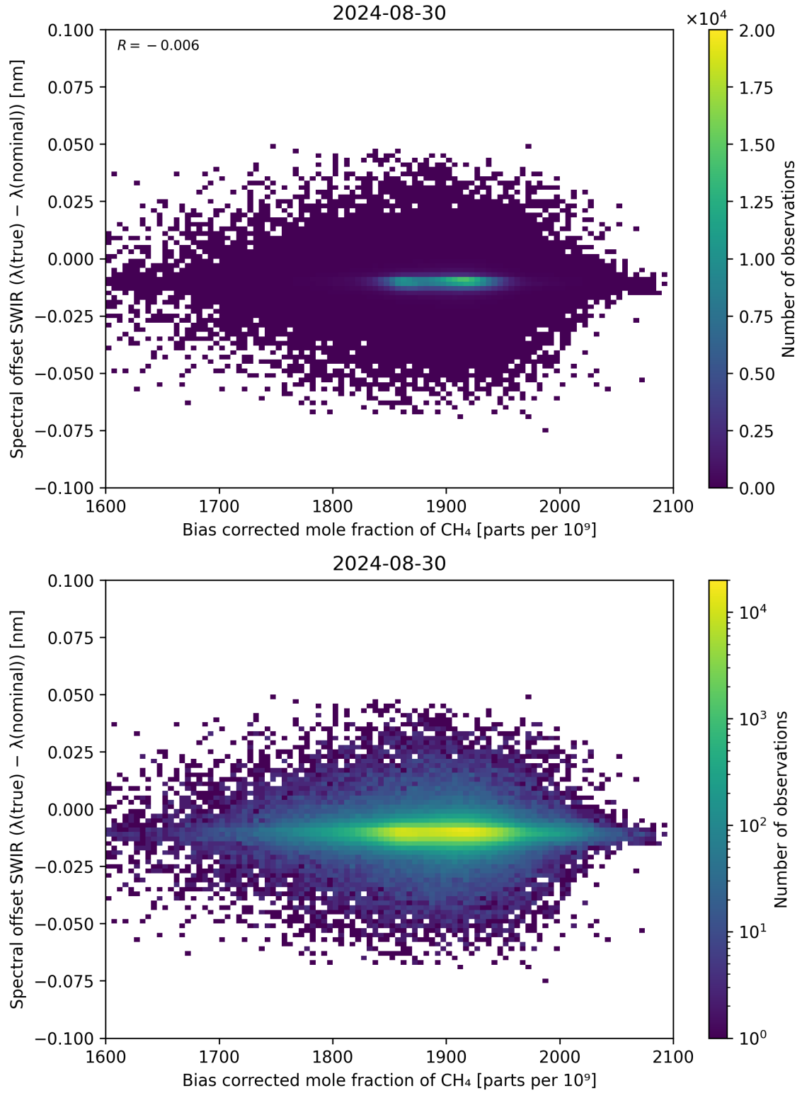
Figure 69: Scatter density plot of “Bias corrected mole fraction of CH 4 ” against “Spectral offset SWIR ( \lambda_{\text{true}} - \lambda_{\text{nominal}} )” for 2024-08-29 to 2024-08-31.
