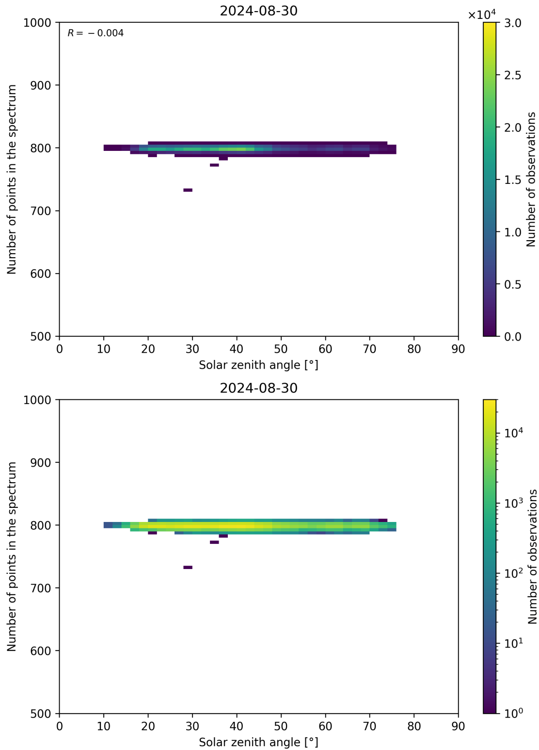
Figure 103: Scatter density plot of “Solar zenith angle” against “Number of points in the spectrum” for 2024-08-29 to 2024-08-31.
