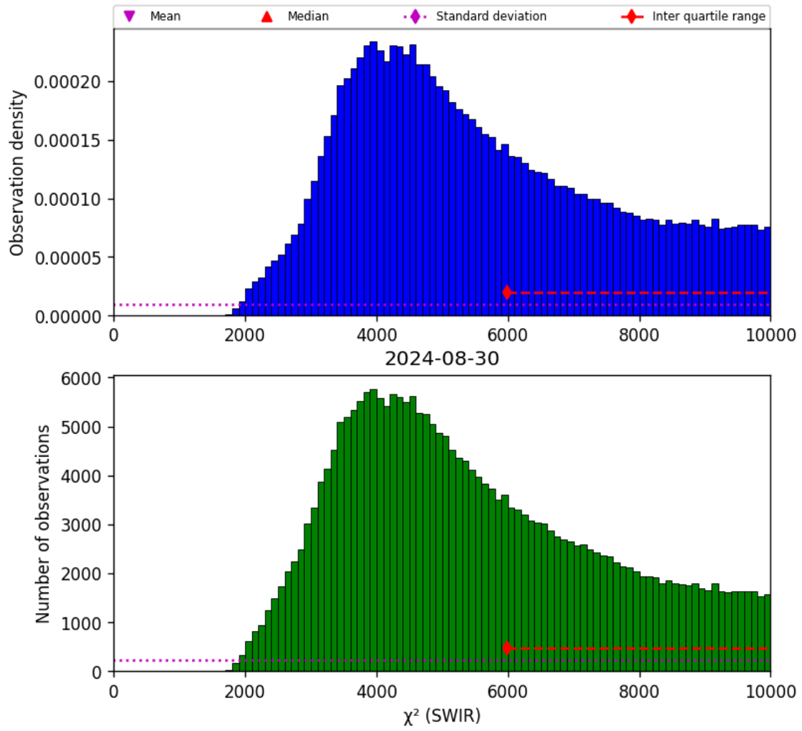
Figure 28: Histogram of “ \chi^2 (SWIR)” for 2024-08-29 to 2024-08-31
