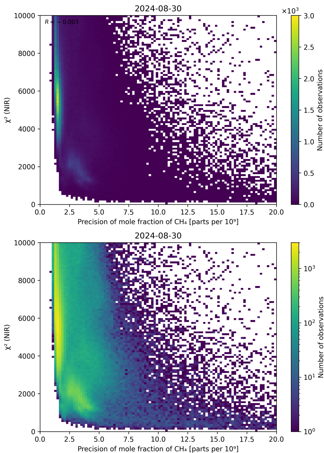
Figure 78: Scatter density plot of “Precision of mole fraction of \text{CH}_4 ” against “ \chi^2 (NIR)” for 2024-08-29 to 2024-08-31.
