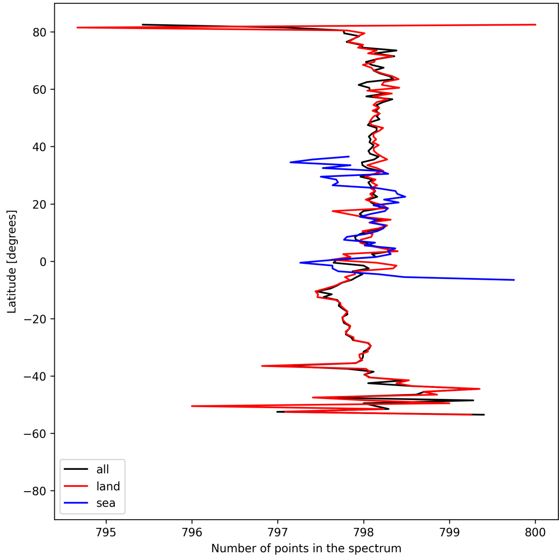
Figure 15: Zonal average of “Number of points in the spectrum” for 2024-08-29 to 2024-08-31.
