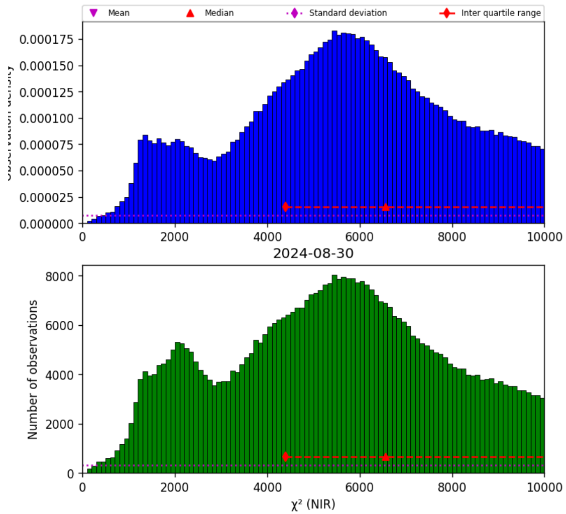
Figure 29: Histogram of “ \chi^2 (NIR)” for 2024-08-29 to 2024-08-31
