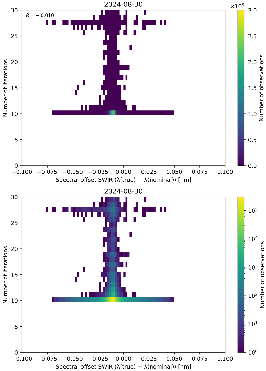
Figure 121: Scatter density plot of “Spectral offset SWIR ( \lambda_{\text{true}} - \lambda_{\text{nominal}} )” against “Number of iterations” for 2024-08-29 to 2024-08-31.
