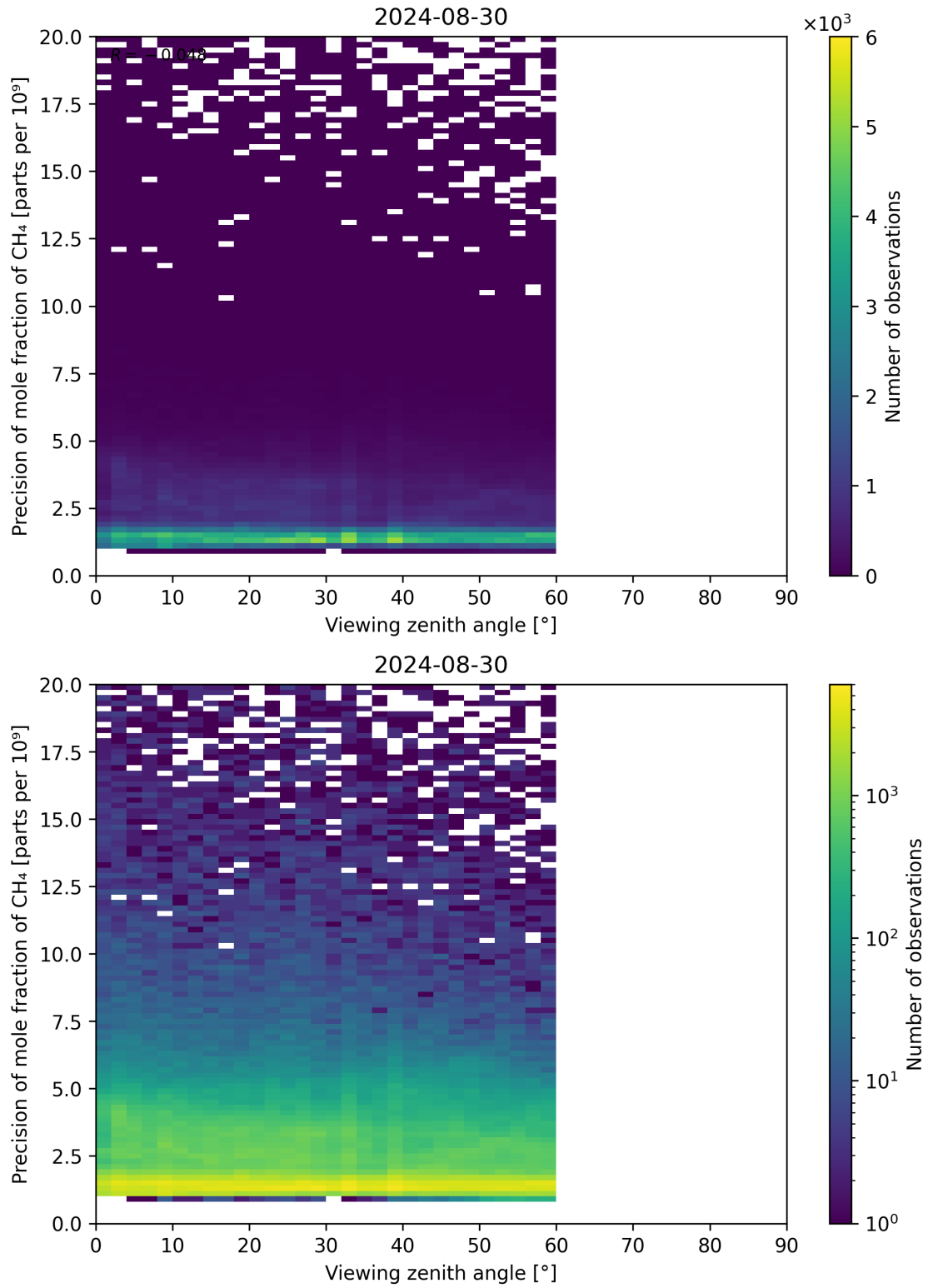
Figure 112: Scatter density plot of “Viewing zenith angle” against “Precision of mole fraction of CH 4 ” for 2024-08-29 to 2024-08-31.
