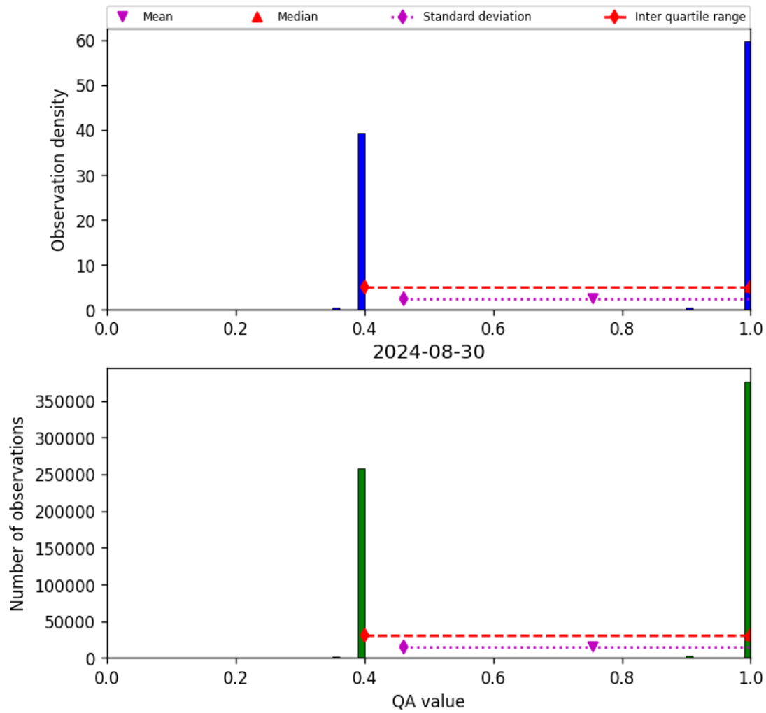
Figure 22: Histogram of “QA value” for 2024-08-29 to 2024-08-31
