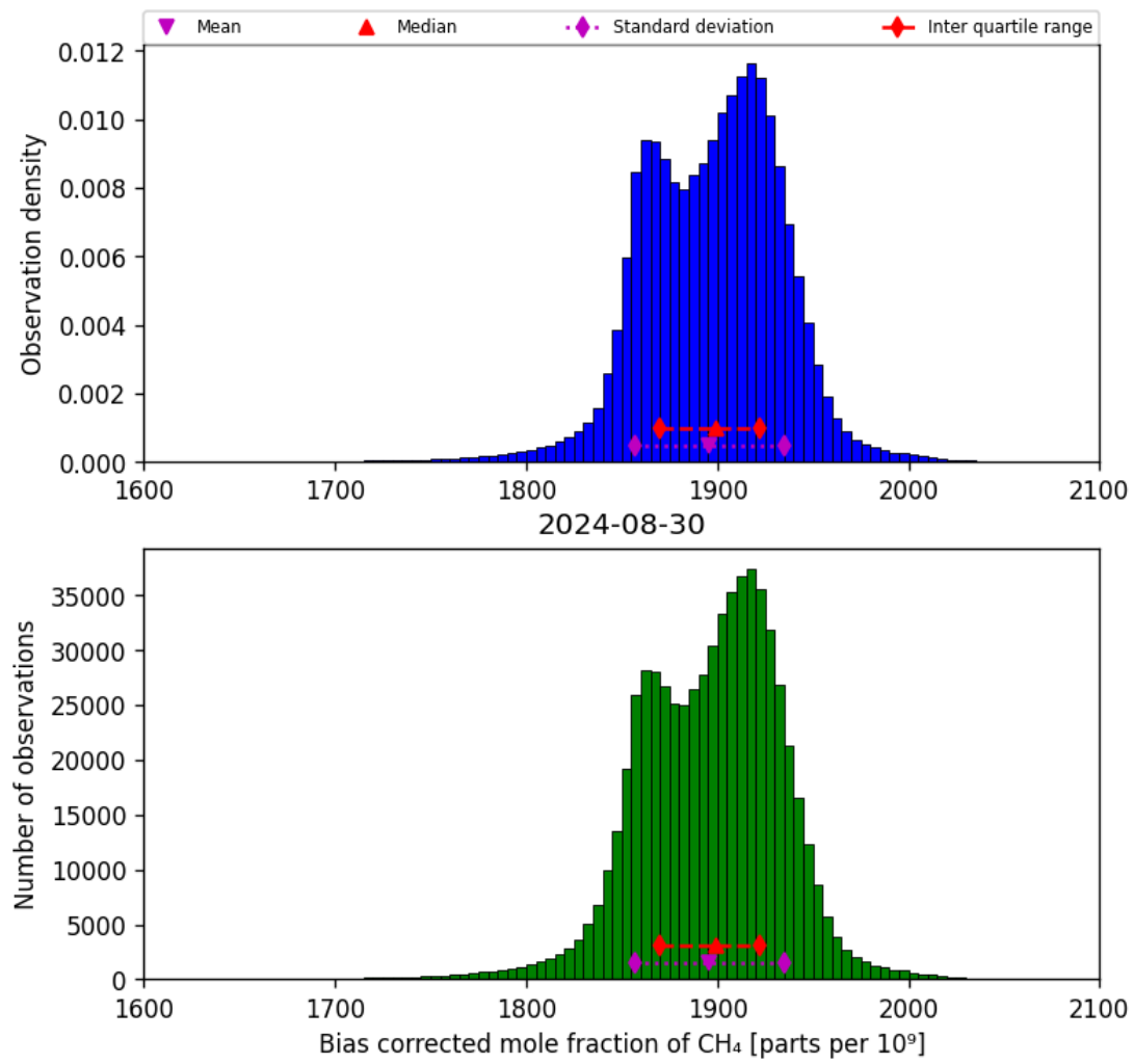
Figure 25: Histogram of “Bias corrected mole fraction of CH 4 ” for 2024-08-29 to 2024-08-31
