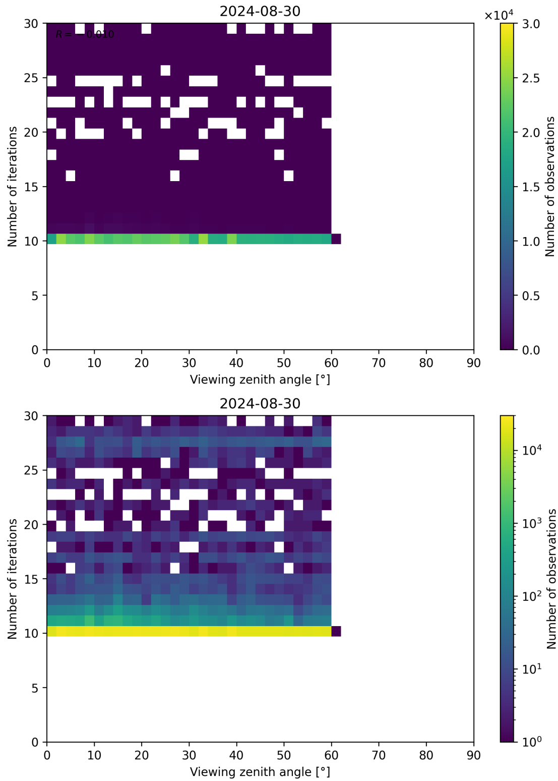
Figure 113: Scatter density plot of “Viewing zenith angle” against “Number of iterations” for 2024-08-29 to 2024-08-31.
