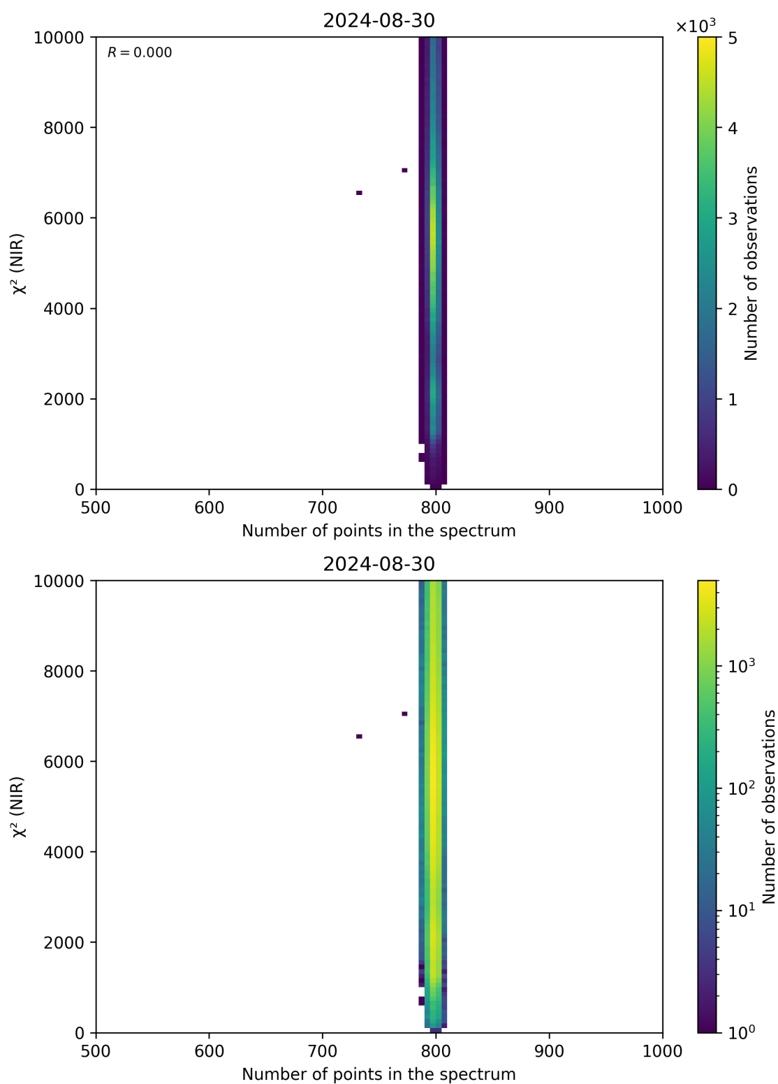
Figure 88: Scatter density plot of “Number of points in the spectrum” against “ \chi^2 (NIR)” for 2024-08-29 to 2024-08-31.
