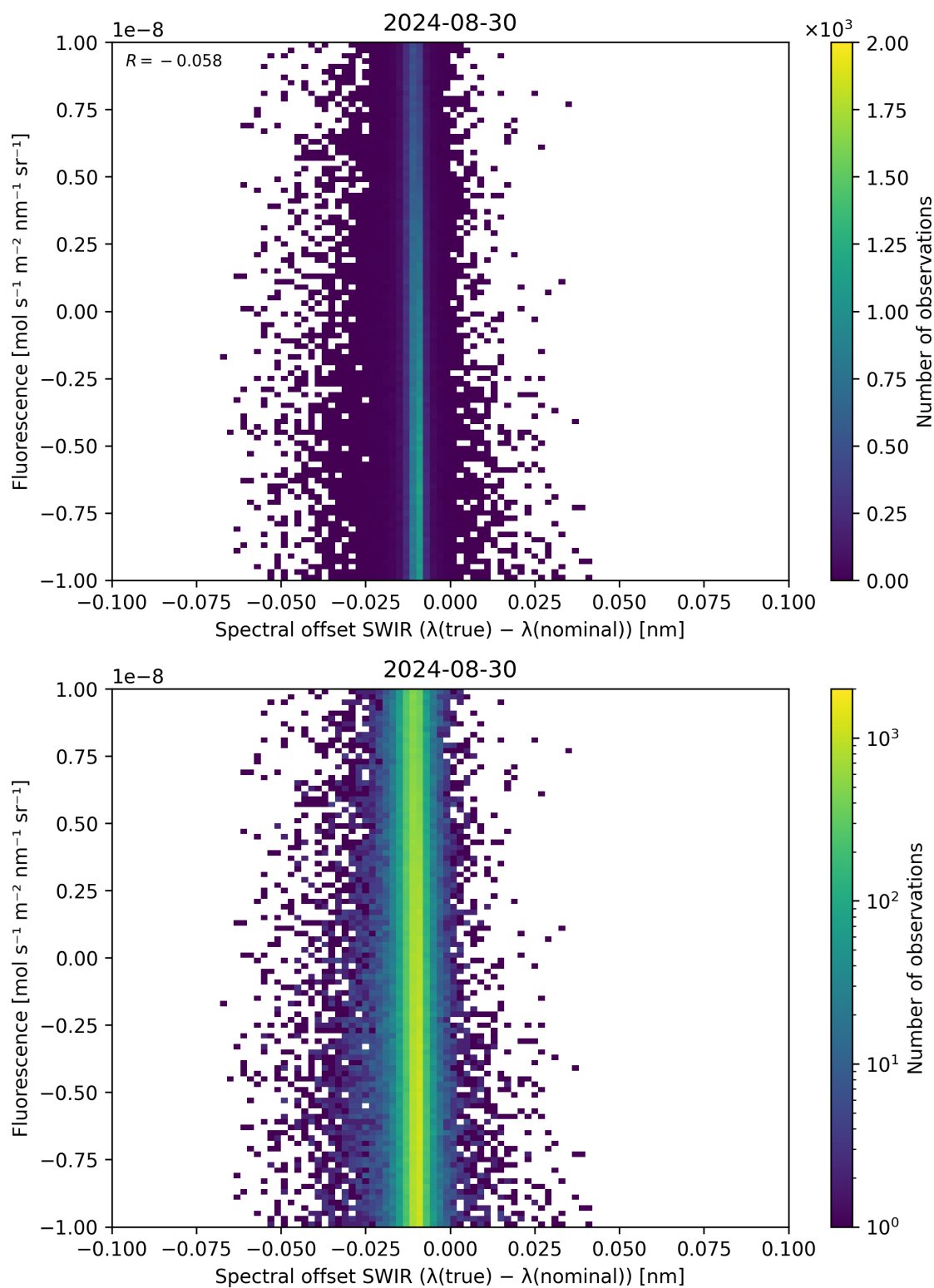
Figure 120: Scatter density plot of “Spectral offset SWIR ( \lambda_{\text{true}} - \lambda_{\text{nominal}} )” against “Fluorescence” for 2024-08-29 to 2024-08-31.
