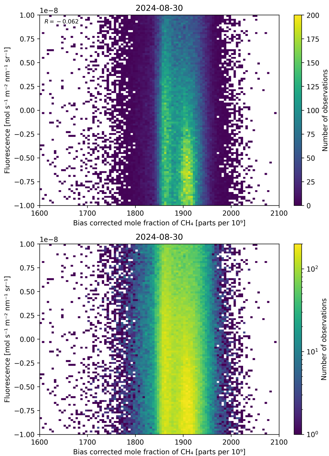
Figure 66: Scatter density plot of “Bias corrected mole fraction of \text{CH}_4 ” against “Fluorescence” for 2024-08-29 to 2024-08-31.
