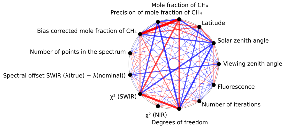
Figure 1: Map of correlation graph for 2024-08-29 to 2024-08-31.
