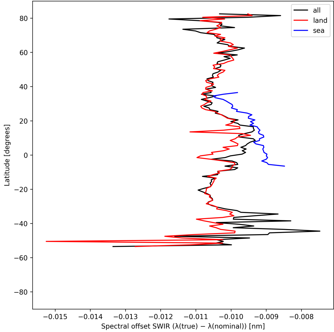
Figure 16: Zonal average of “Spectral offset SWIR ( \lambda_{\text{true}} - \lambda_{\text{nominal}} )” for 2024-08-29 to 2024-08-31.
