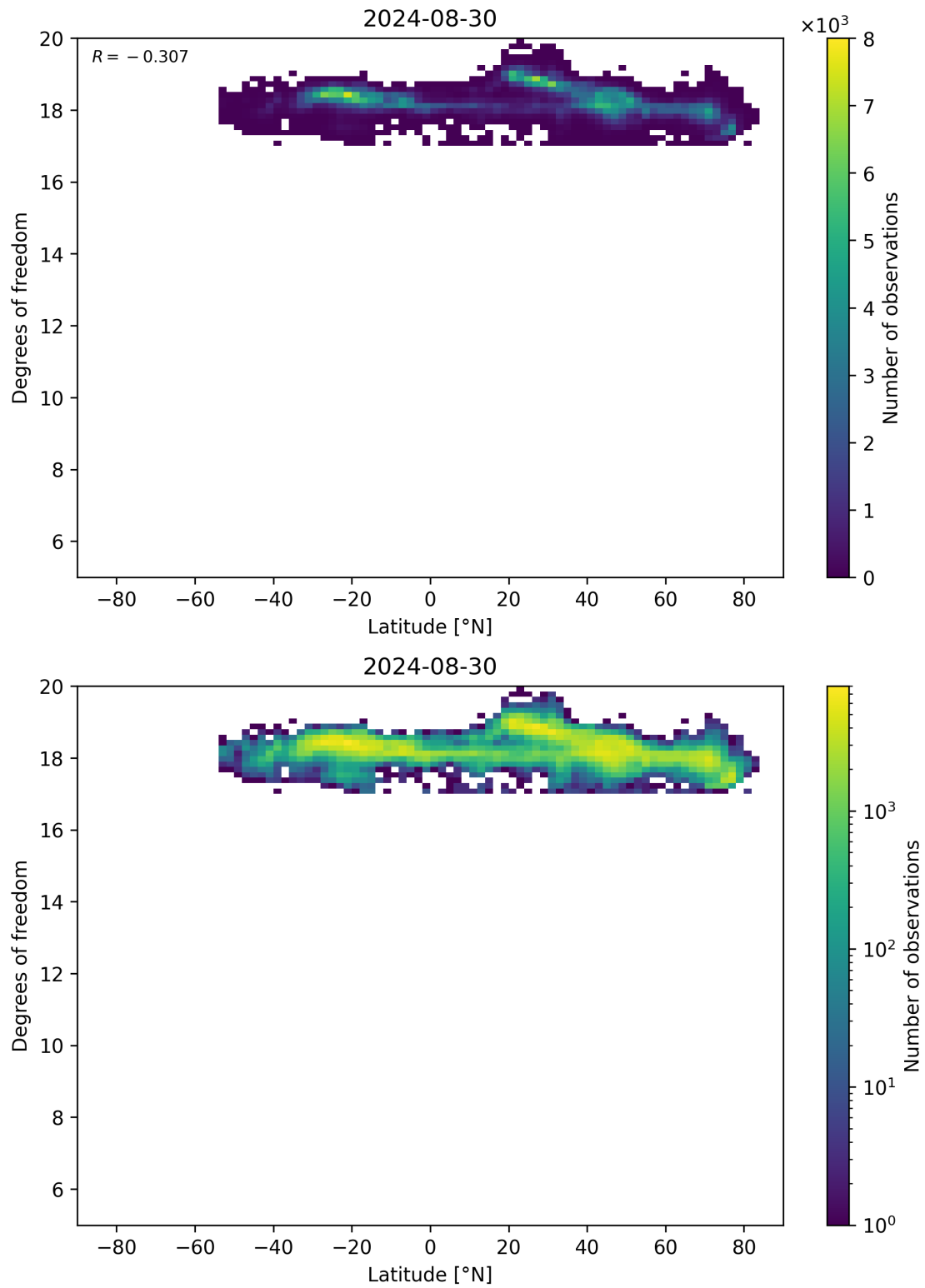
Figure 55: Scatter density plot of “Latitude” against “Degrees of freedom” for 2024-08-29 to 2024-08-31.
