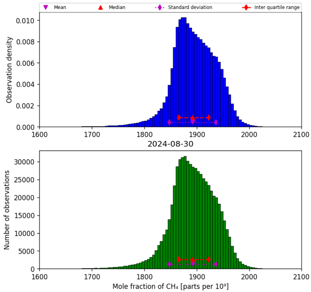
Figure 23: Histogram of "Mole fraction of CH 4 " for 2024-08-29 to 2024-08-31
