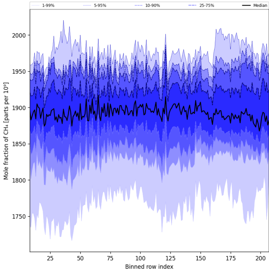
Figure 34: Along track statistics of “Mole fraction of CH 4 ” for 2024-08-29 to 2024-08-31
