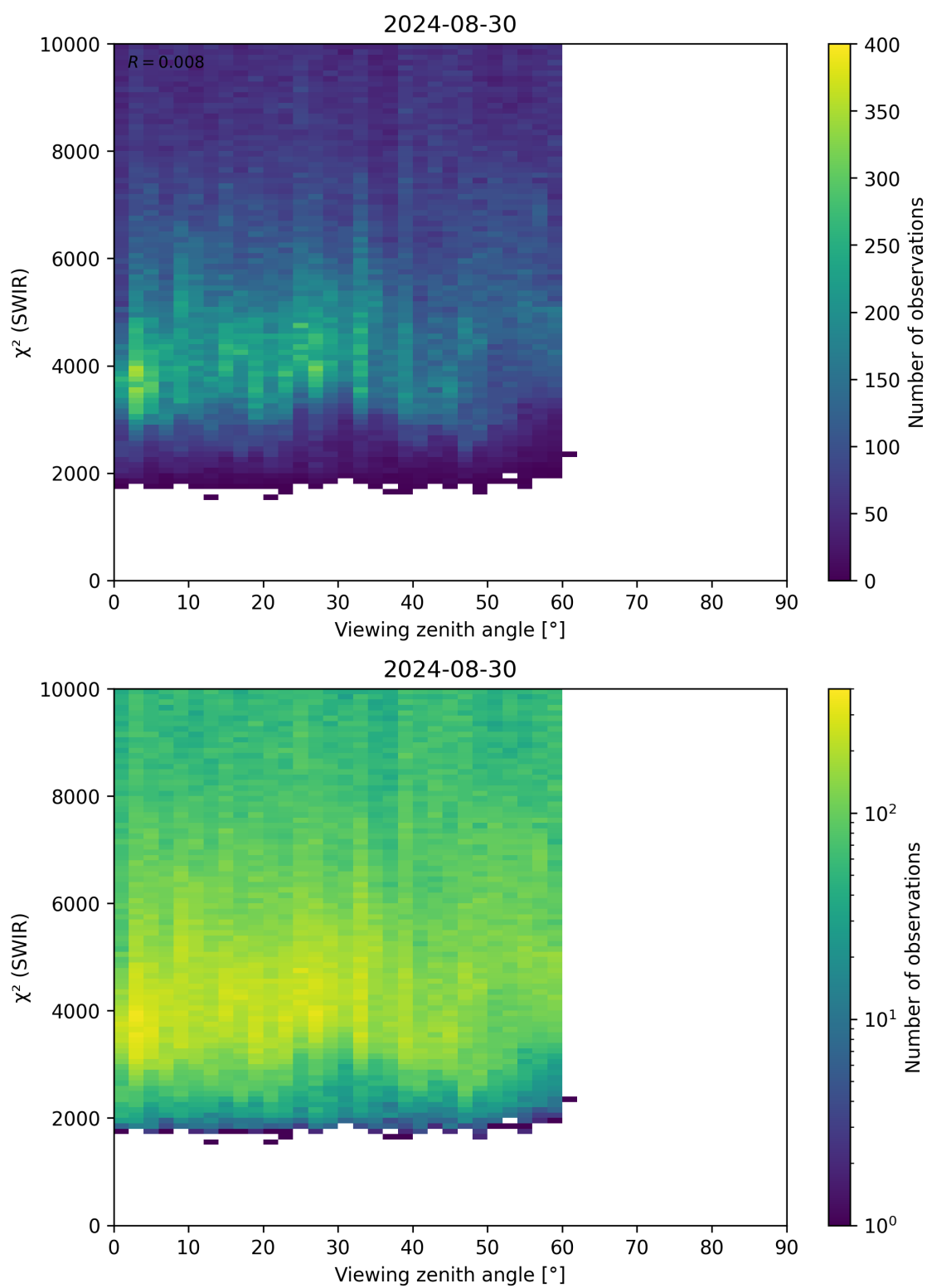
Figure 106: Scatter density plot of “Viewing zenith angle” against “ \chi^2 (SWIR)” for 2024-08-29 to 2024-08-31.
