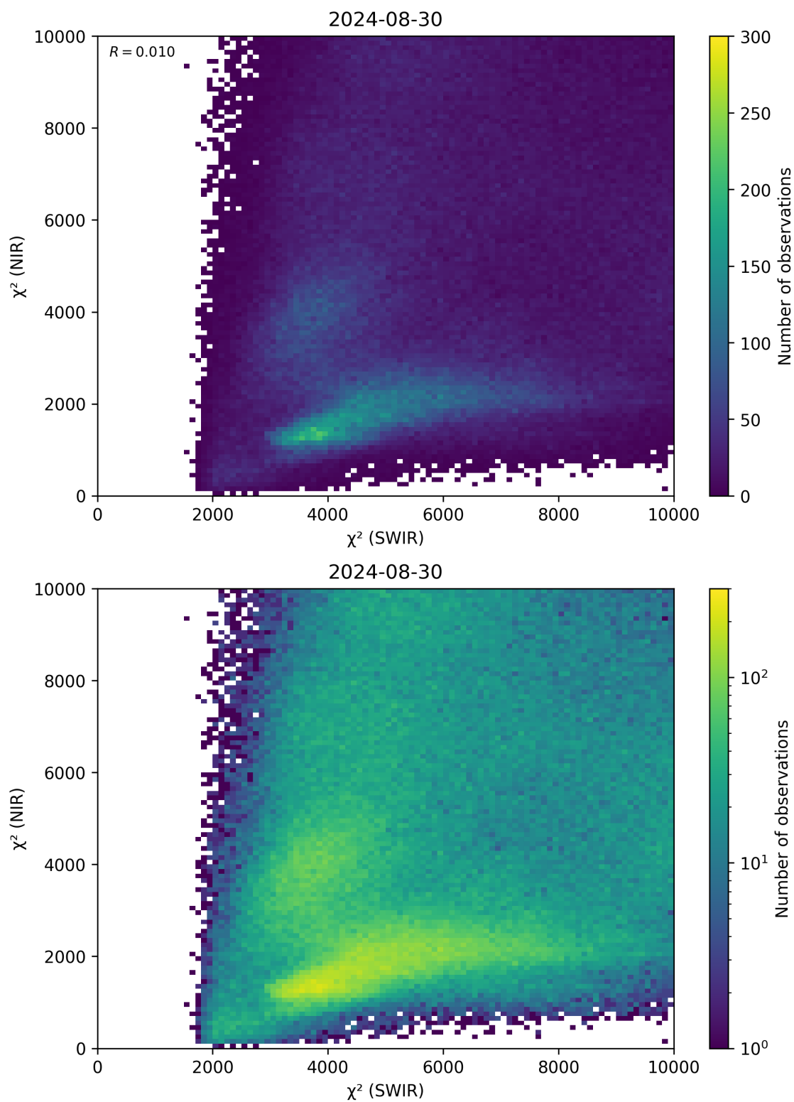
Figure 47: Scatter density plot of “ \chi^2 (SWIR)” against “ \chi^2 (NIR)” for 2024-08-29 to 2024-08-31.
