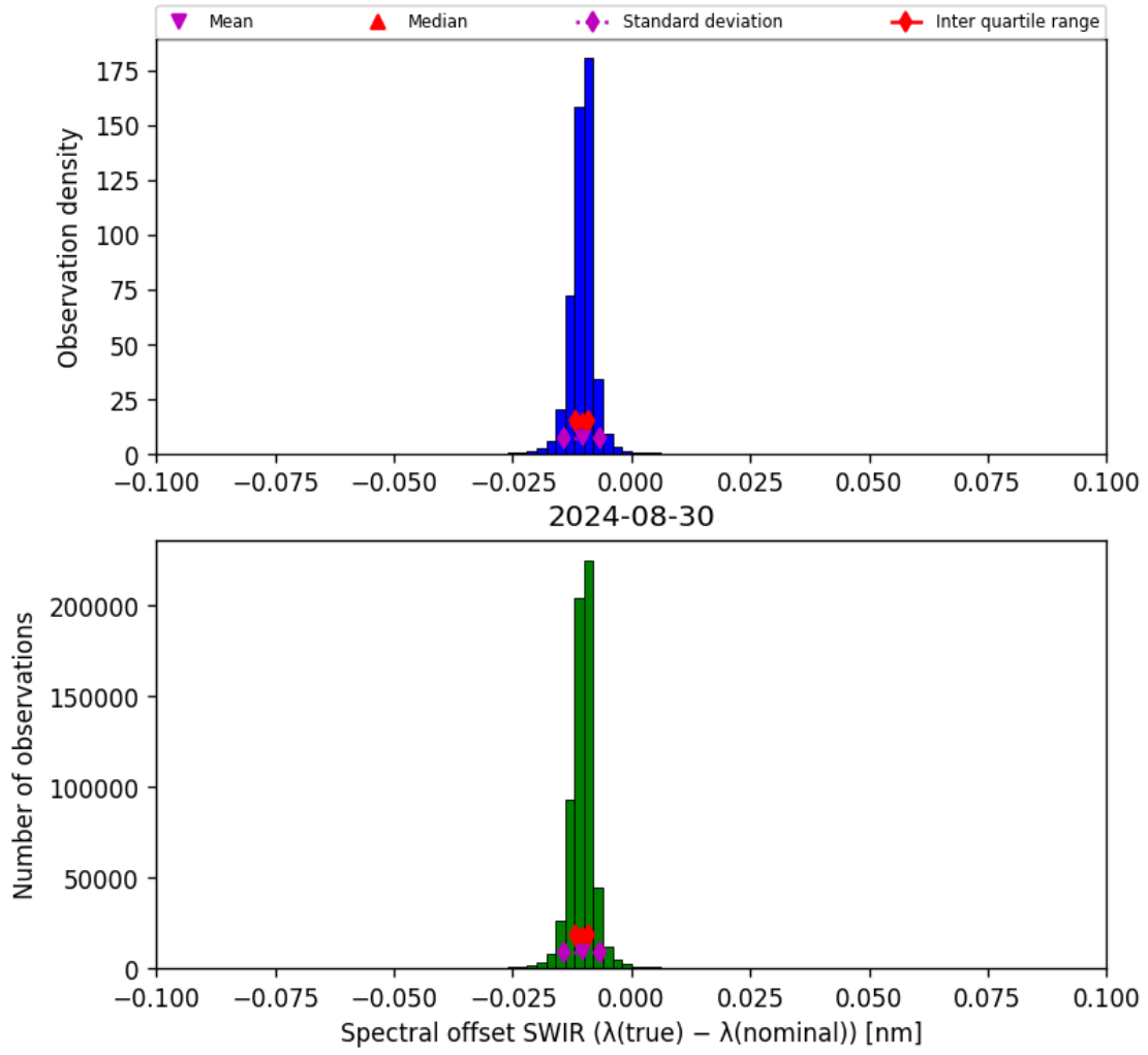
Figure 27: Histogram of “Spectral offset SWIR ( \lambda_{\text{true}} - \lambda_{\text{nominal}} )” for 2024-08-29 to 2024-08-31
