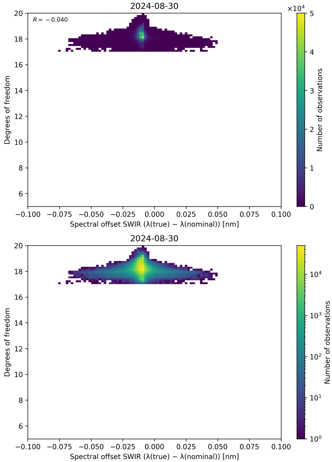
Figure 119: Scatter density plot of “Spectral offset SWIR ( \lambda_{\text{true}} - \lambda_{\text{nominal}} )” against “Degrees of freedom” for 2024-08-29 to 2024-08-31.
