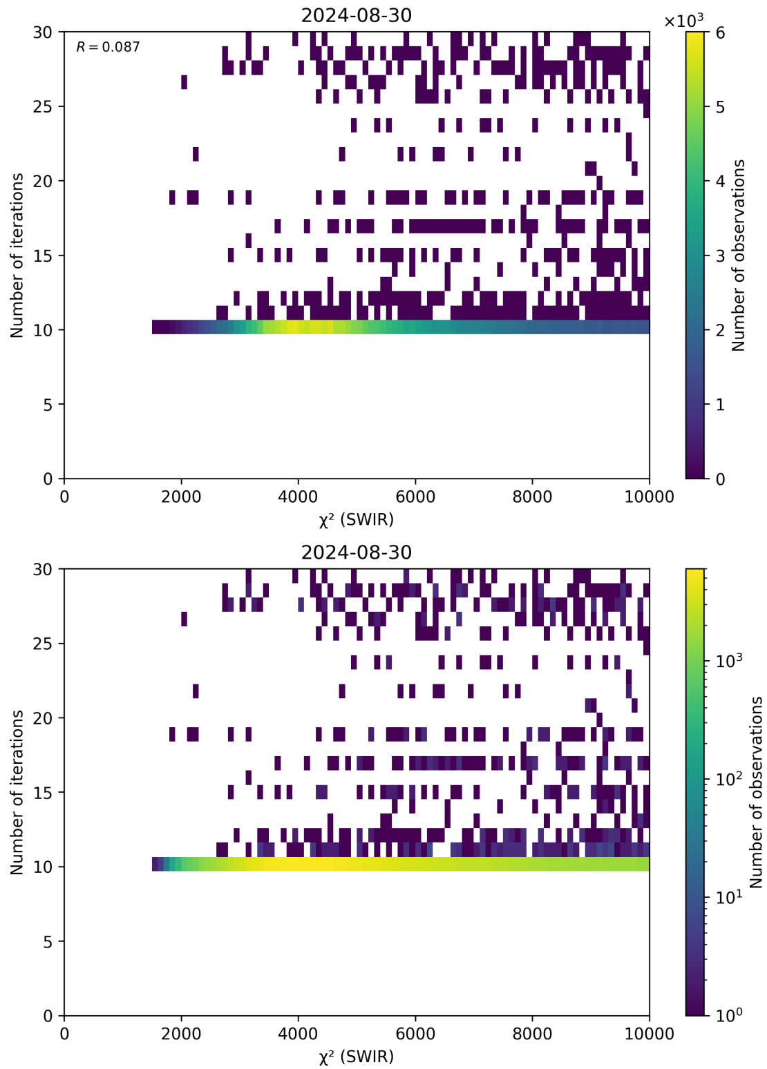
Figure 50: Scatter density plot of “ \chi^2 (SWIR)” against “Number of iterations” for 2024-08-29 to 2024-08-31.
