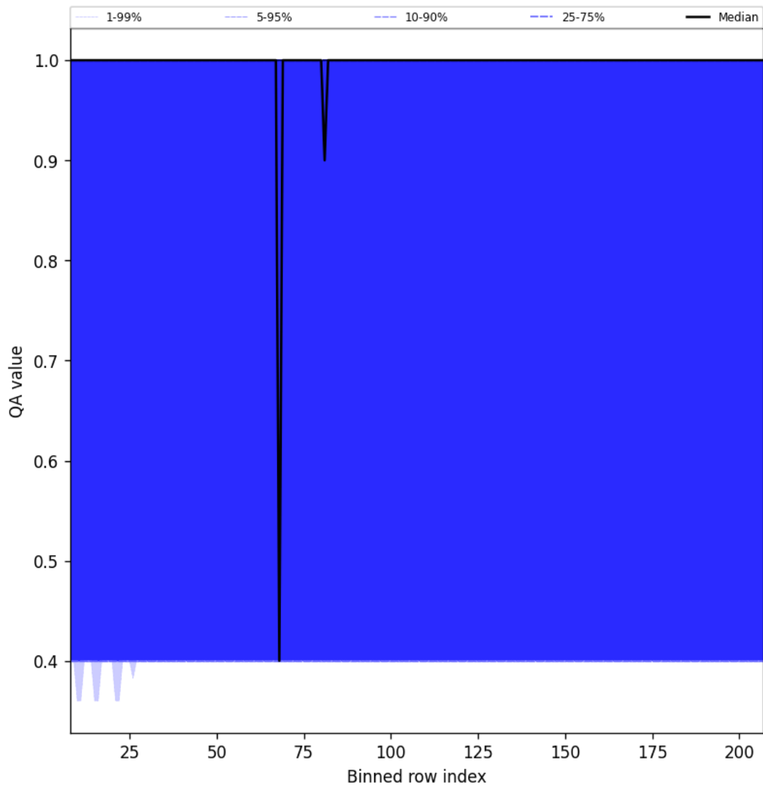
Figure 33: Along track statistics of “QA value” for 2024-08-29 to 2024-08-31
