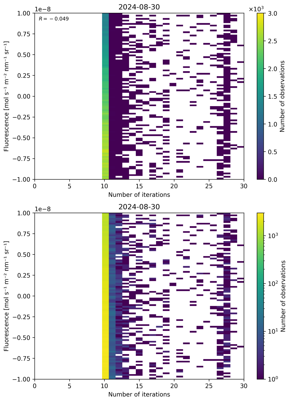
Figure 87: Scatter density plot of “Number of iterations” against “Fluorescence” for 2024-08-29 to 2024-08-31.
