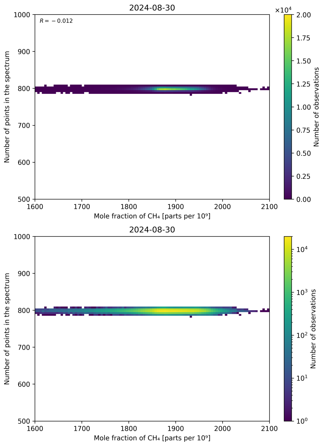
Figure 77: Scatter density plot of “Mole fraction of CH 4 ” against “Number of points in the spectrum” for 2024-08-29 to 2024-08-31.
