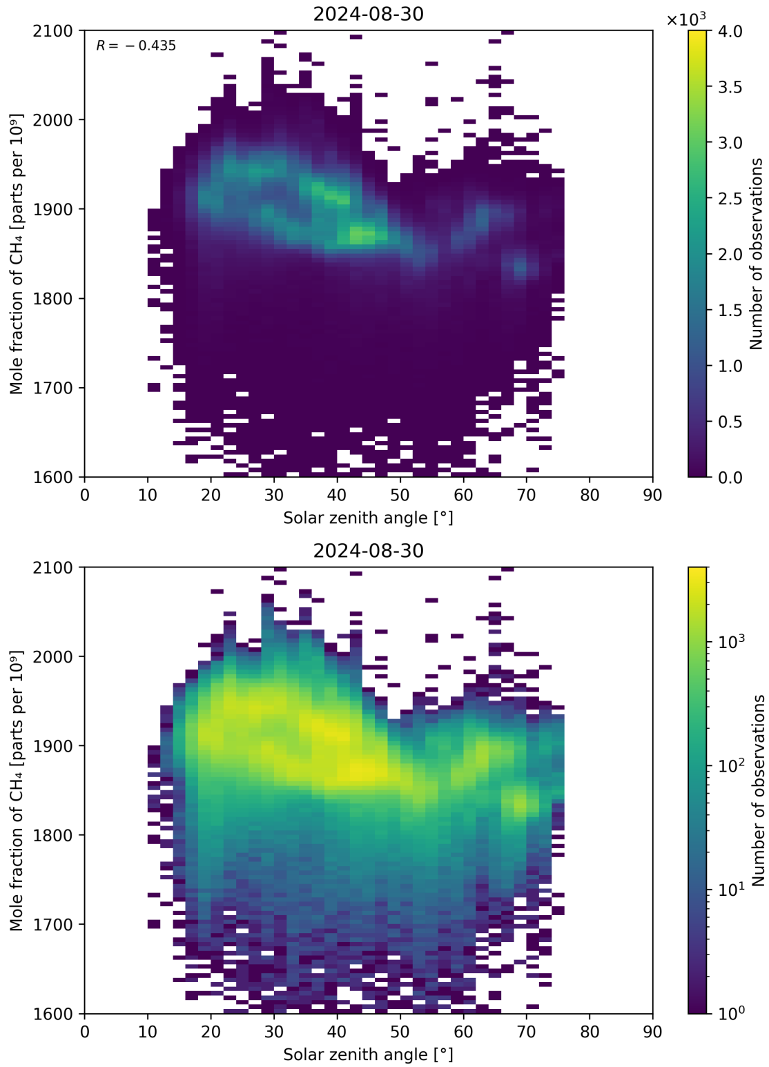
Figure 99: Scatter density plot of “Solar zenith angle” against “Mole fraction of CH 4 ” for 2024-08-29 to 2024-08-31.
