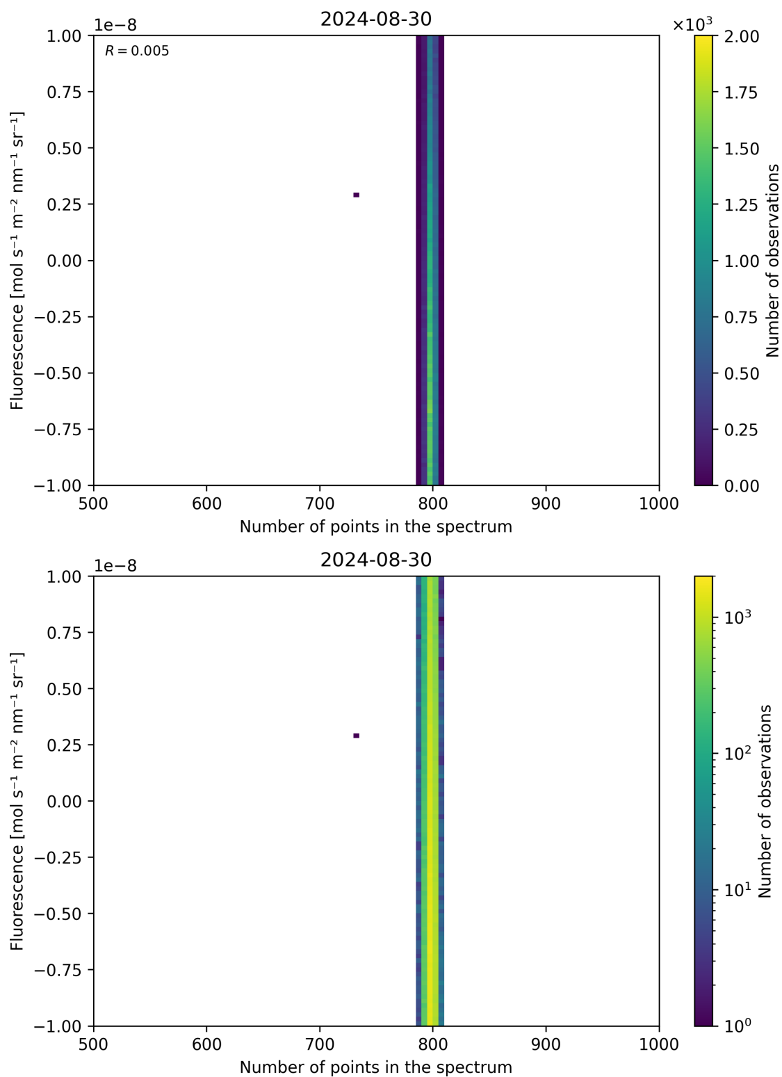
Figure 91: Scatter density plot of “Number of points in the spectrum” against “Fluorescence” for 2024-08-29 to 2024-08-31.
