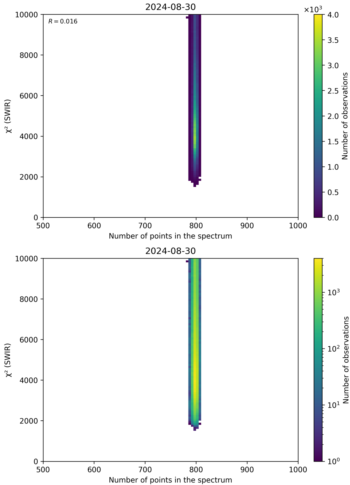
Figure 89: Scatter density plot of “Number of points in the spectrum” against “ \chi^2 (SWIR)” for 2024-08-29 to 2024-08-31.
