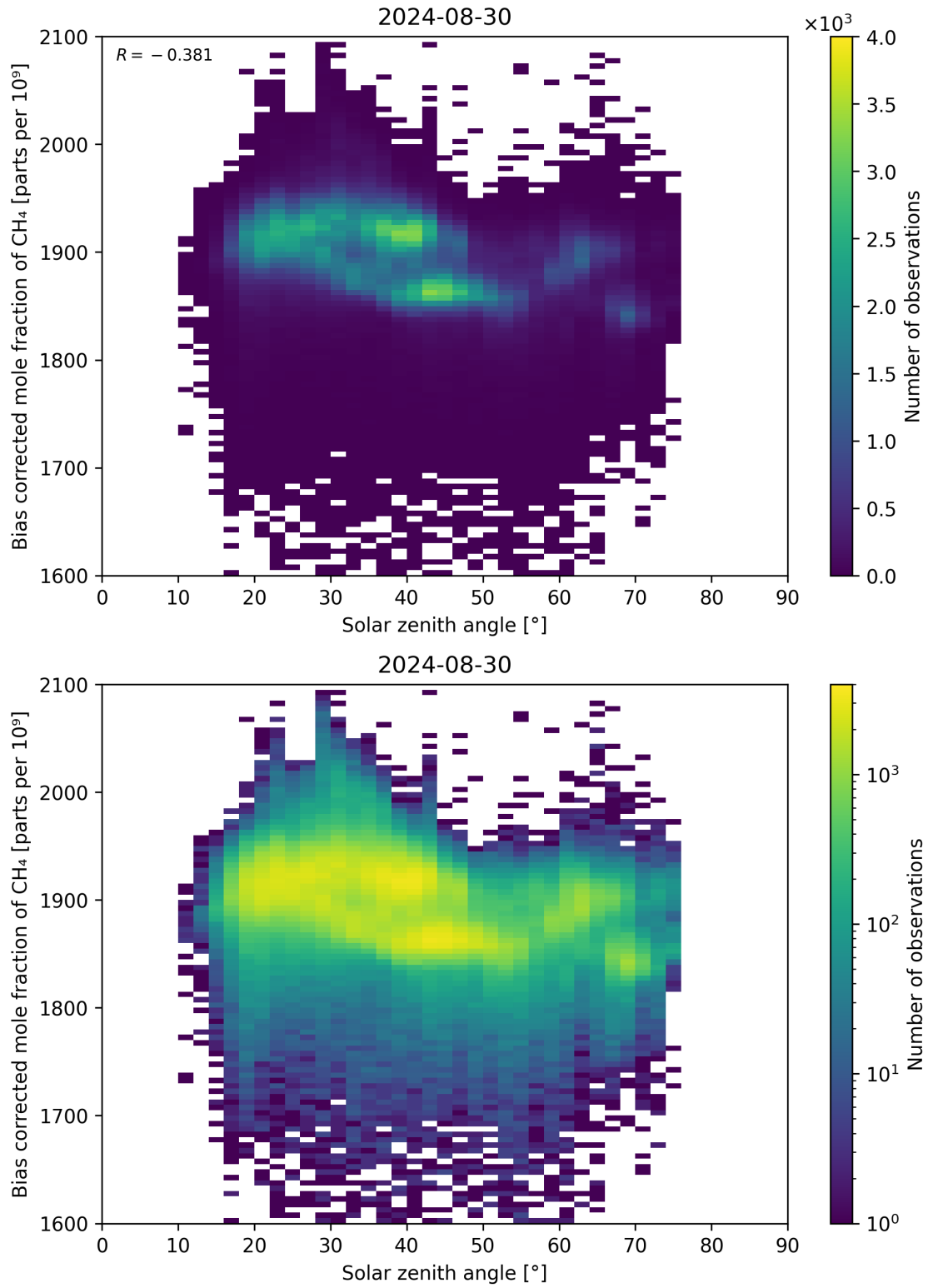
Figure 100: Scatter density plot of “Solar zenith angle” against “Bias corrected mole fraction of \text{CH}_4 ” for 2024-08-29 to 2024-08-31.
