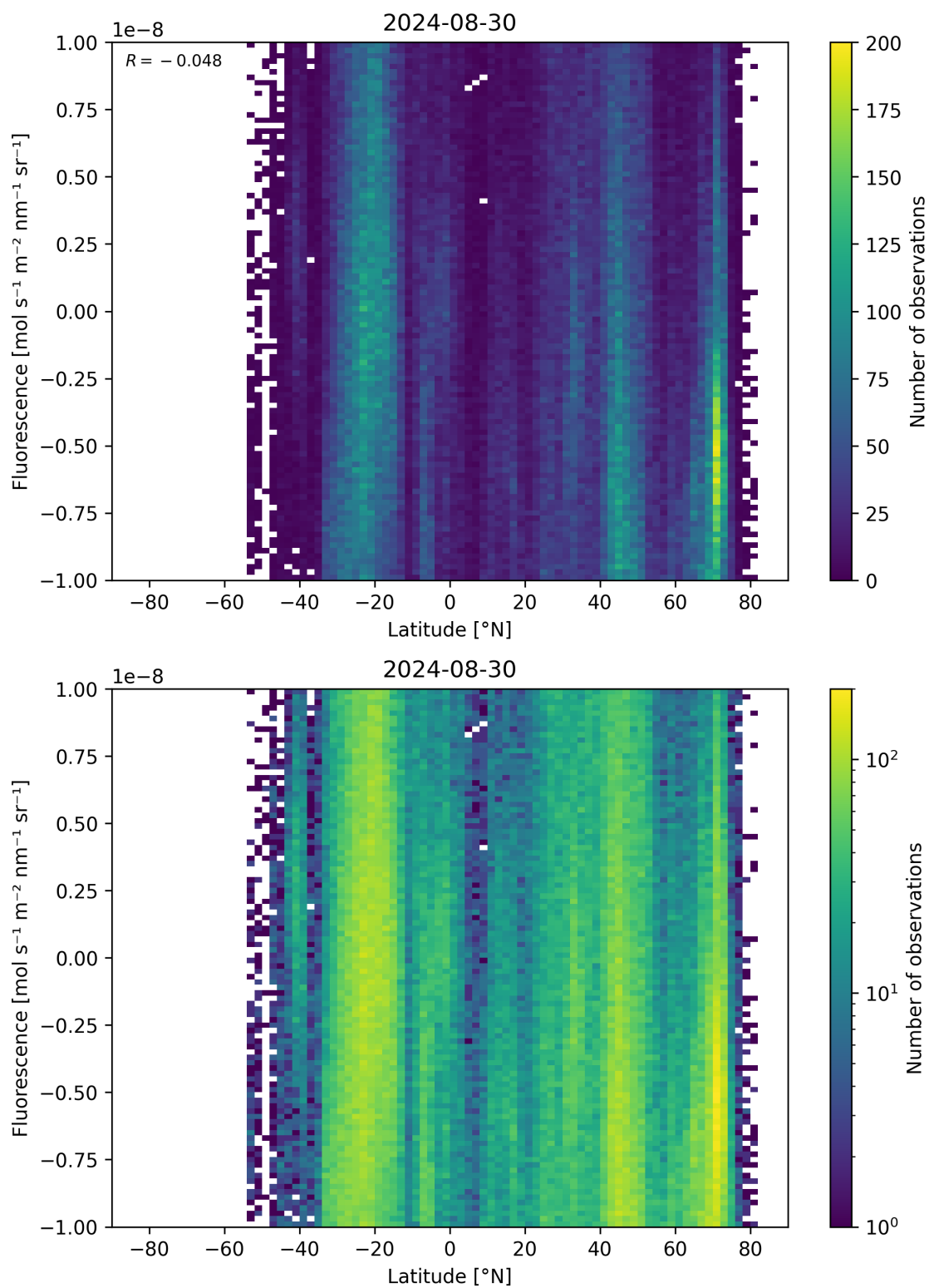
Figure 56: Scatter density plot of “Latitude” against “Fluorescence” for 2024-08-29 to 2024-08-31.
