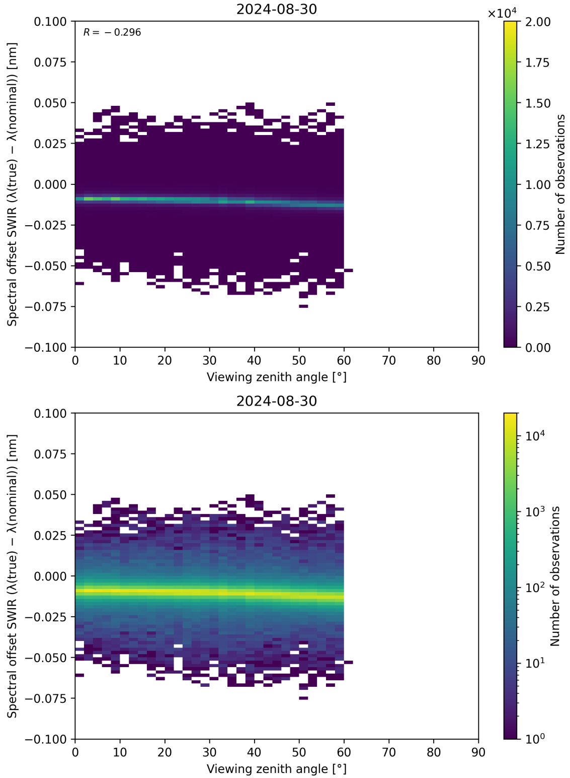
Figure 116: Scatter density plot of “Viewing zenith angle” against “Spectral offset SWIR ( \lambda_{\text{true}} - \lambda_{\text{nominal}} )” for 2024-08-29 to 2024-08-31.
