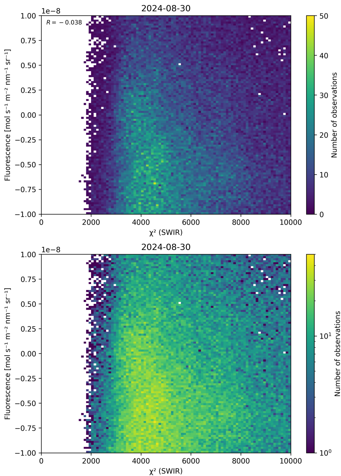
Figure 49: Scatter density plot of “ \chi^2 (SWIR)” against “Fluorescence” for 2024-08-29 to 2024-08-31.
