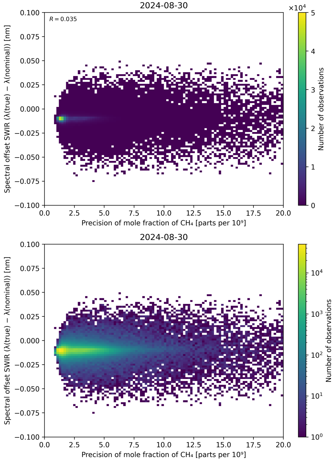
Figure 85: Scatter density plot of “Precision of mole fraction of \text{CH}_4 ” against “Spectral offset SWIR ( \lambda_{\text{true}} - \lambda_{\text{nominal}} )” for 2024-08-29 to 2024-08-31.
