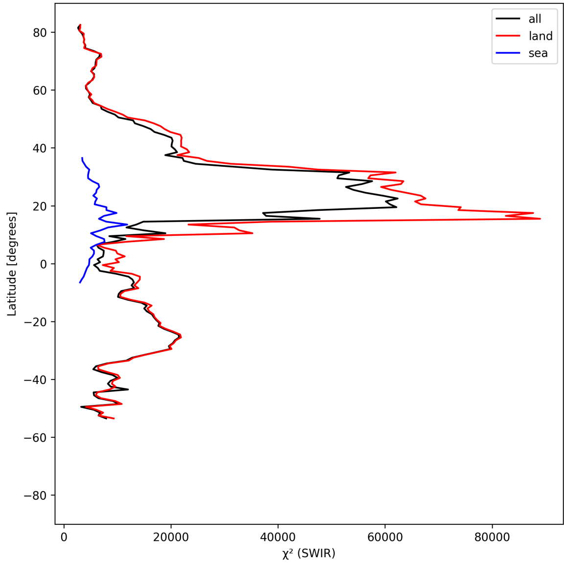
Figure 17: Zonal average of “ \chi^2 (SWIR)” for 2024-08-29 to 2024-08-31.
