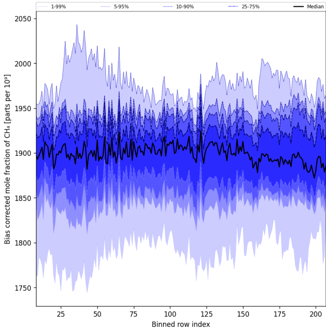
Figure 36: Along track statistics of “Bias corrected mole fraction of CH 4 ” for 2024-08-29 to 2024-08-31
