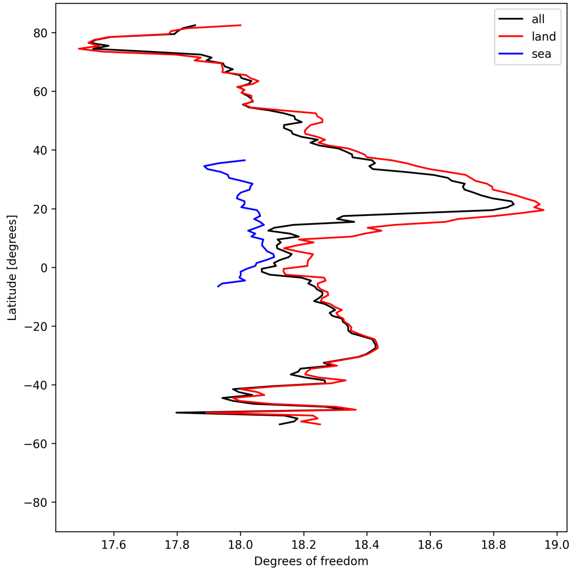
Figure 19: Zonal average of “Degrees of freedom” for 2024-08-29 to 2024-08-31.
