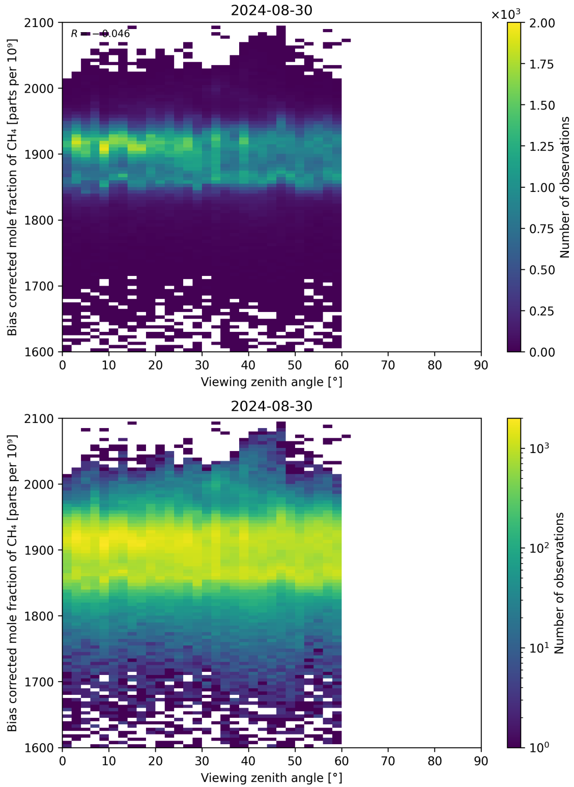
Figure 111: Scatter density plot of “Viewing zenith angle” against “Bias corrected mole fraction of CH 4 ” for 2024-08-29 to 2024-08-31.
