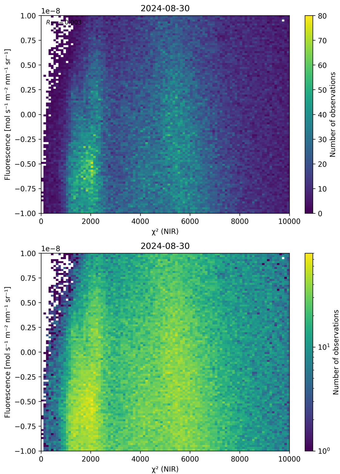
Figure 45: Scatter density plot of “ \chi^2 (NIR)” against “Fluorescence” for 2024-08-29 to 2024-08-31.
