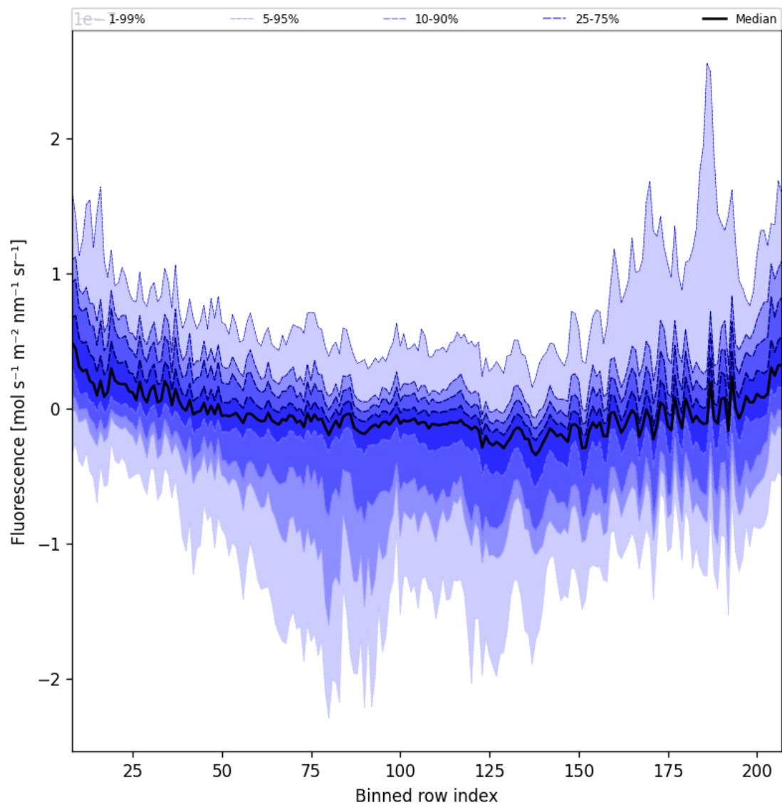
Figure 43: Along track statistics of “Fluorescence” for 2024-08-29 to 2024-08-31
