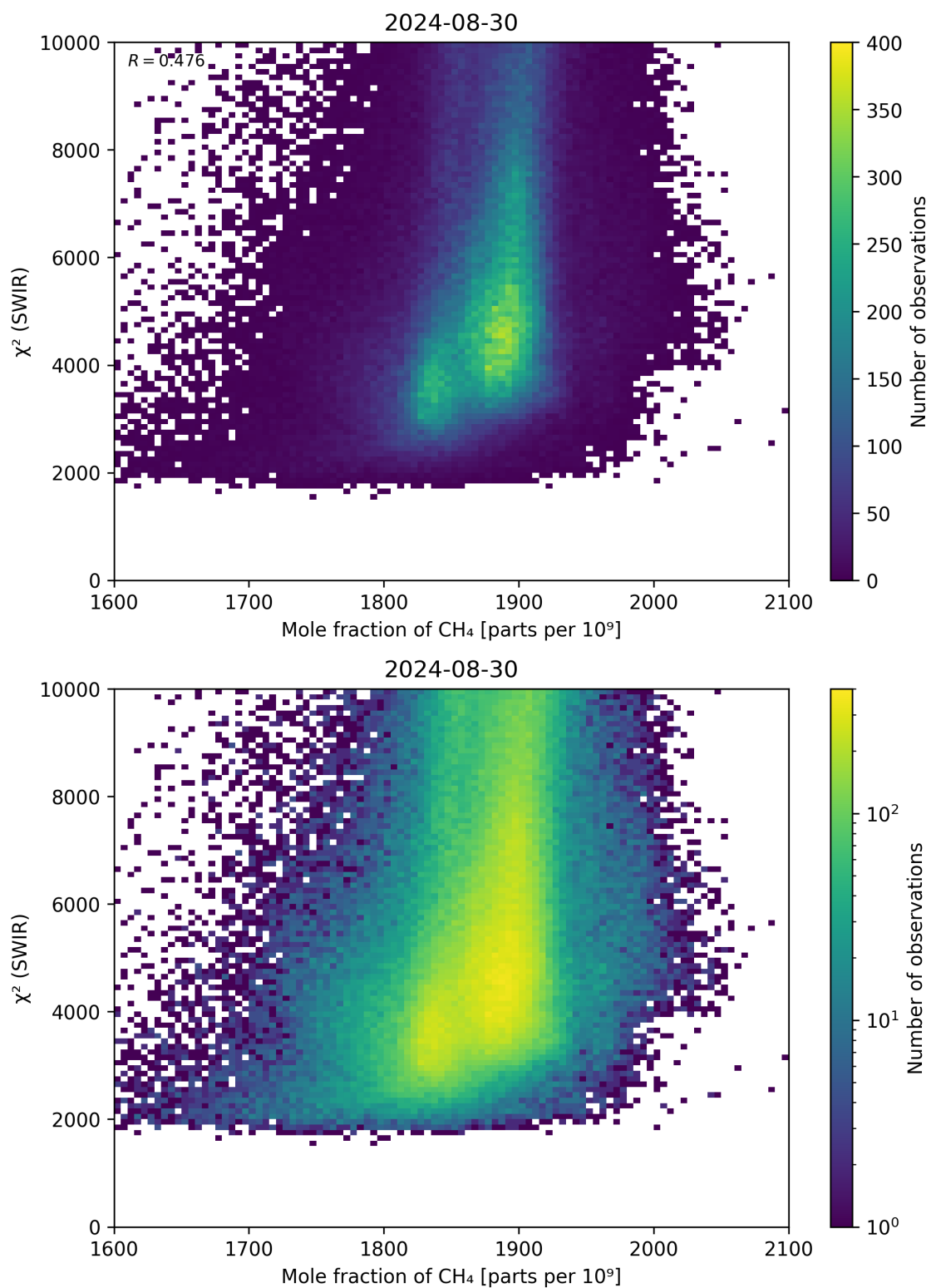
Figure 71: Scatter density plot of “Mole fraction of CH 4 ” against “ \chi^2 (SWIR)” for 2024-08-29 to 2024-08-31.
