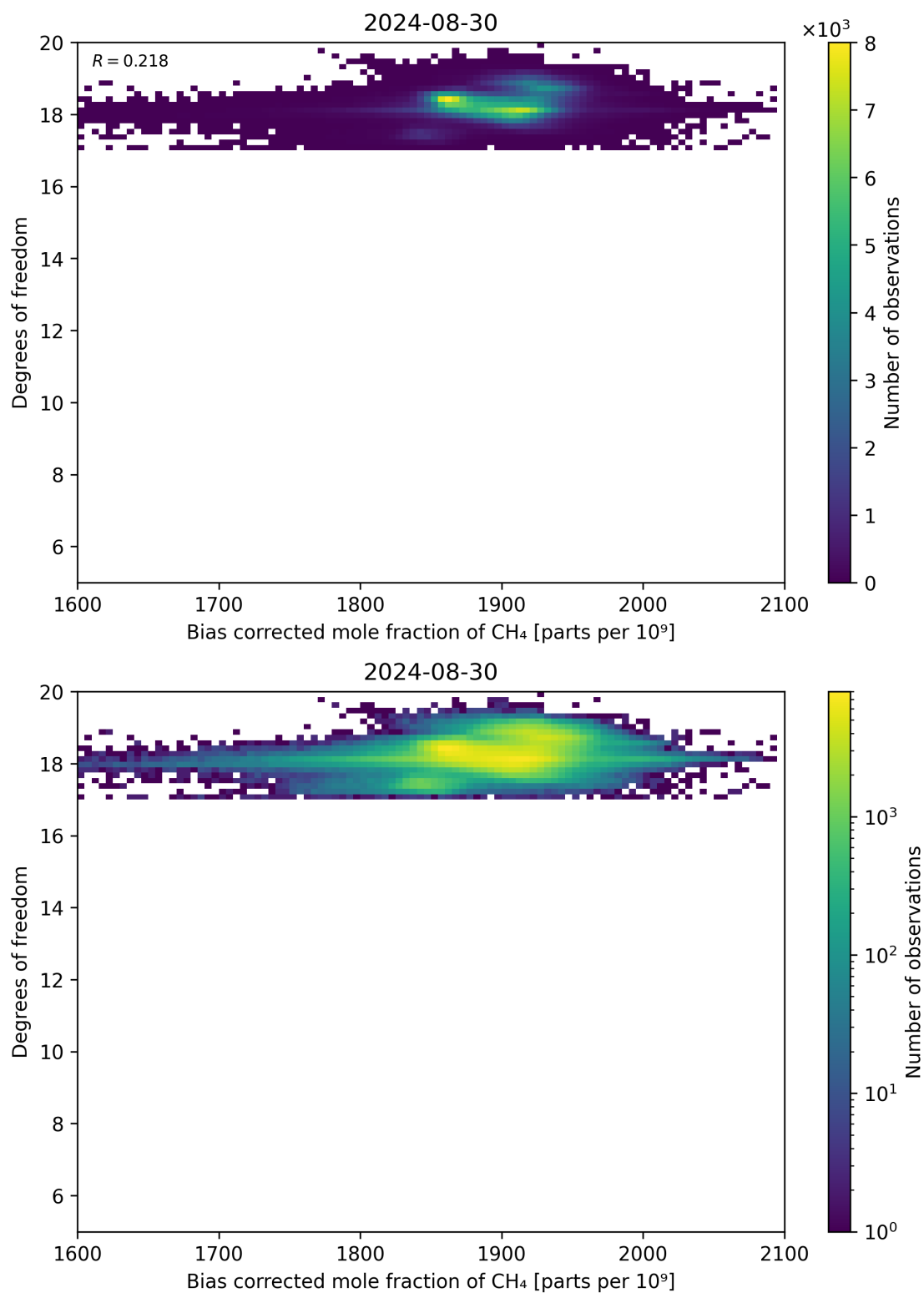
Figure 65: Scatter density plot of “Bias corrected mole fraction of CH 4 ” against “Degrees of freedom” for 2024-08-29 to 2024-08-31.
