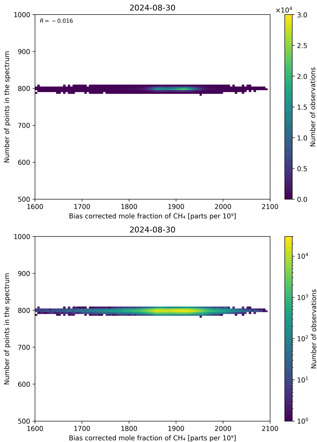
Figure 68: Scatter density plot of “Bias corrected mole fraction of CH 4 ” against “Number of points in the spectrum” for 2024-08-29 to 2024-08-31.
