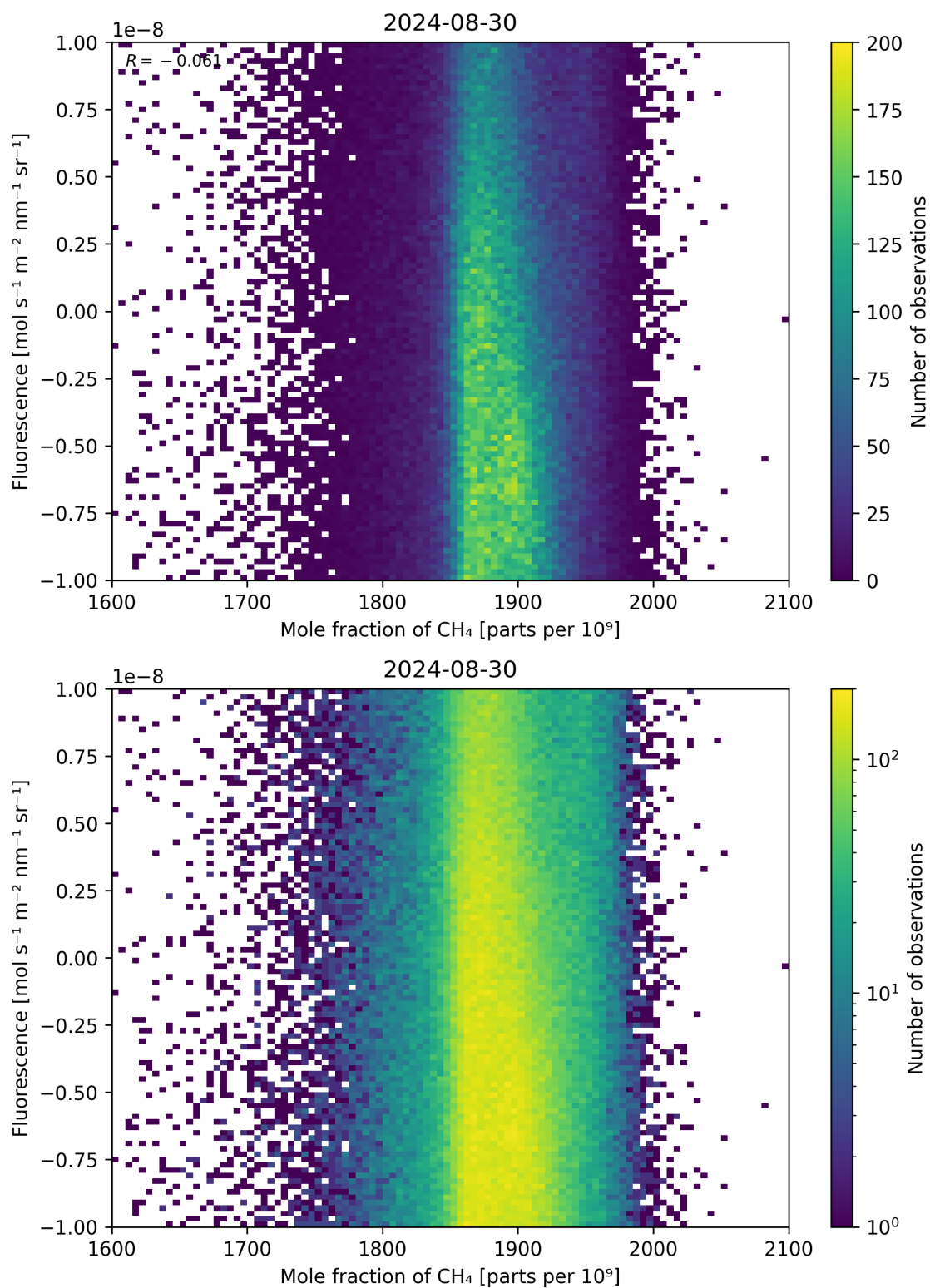
Figure 73: Scatter density plot of “Mole fraction of \text{CH}_4 ” against “Fluorescence” for 2024-08-29 to 2024-08-31.
