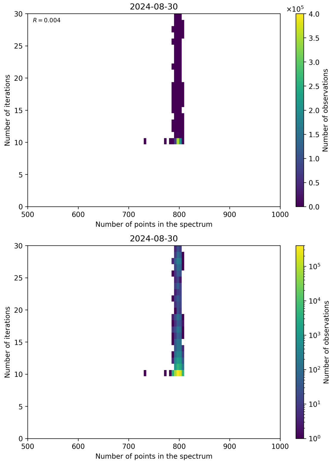
Figure 92: Scatter density plot of “Number of points in the spectrum” against “Number of iterations” for 2024-08-29 to 2024-08-31.
