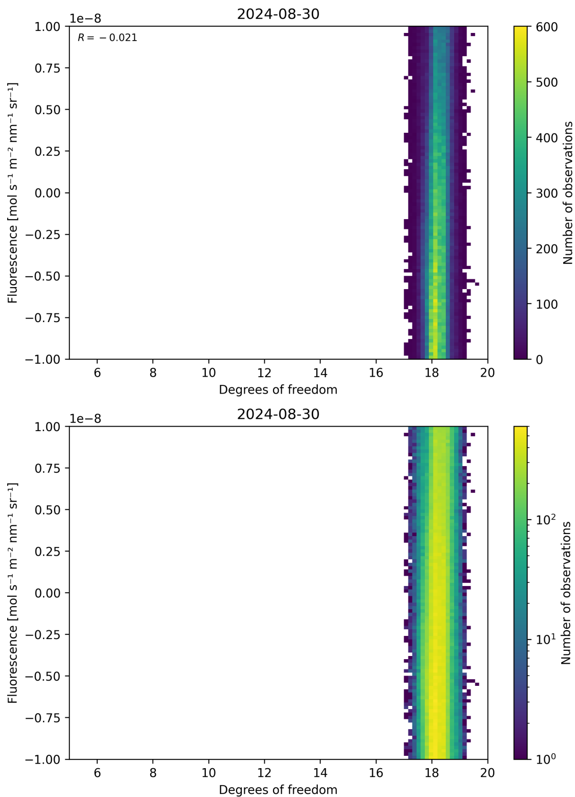
Figure 51: Scatter density plot of “Degrees of freedom” against “Fluorescence” for 2024-08-29 to 2024-08-31.
