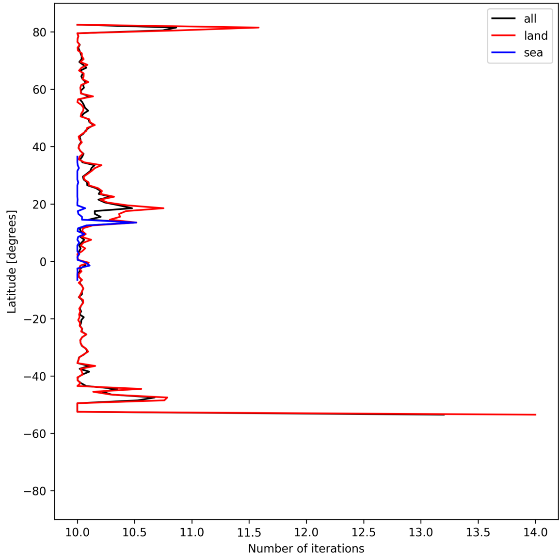
Figure 20: Zonal average of “Number of iterations” for 2024-08-29 to 2024-08-31.
