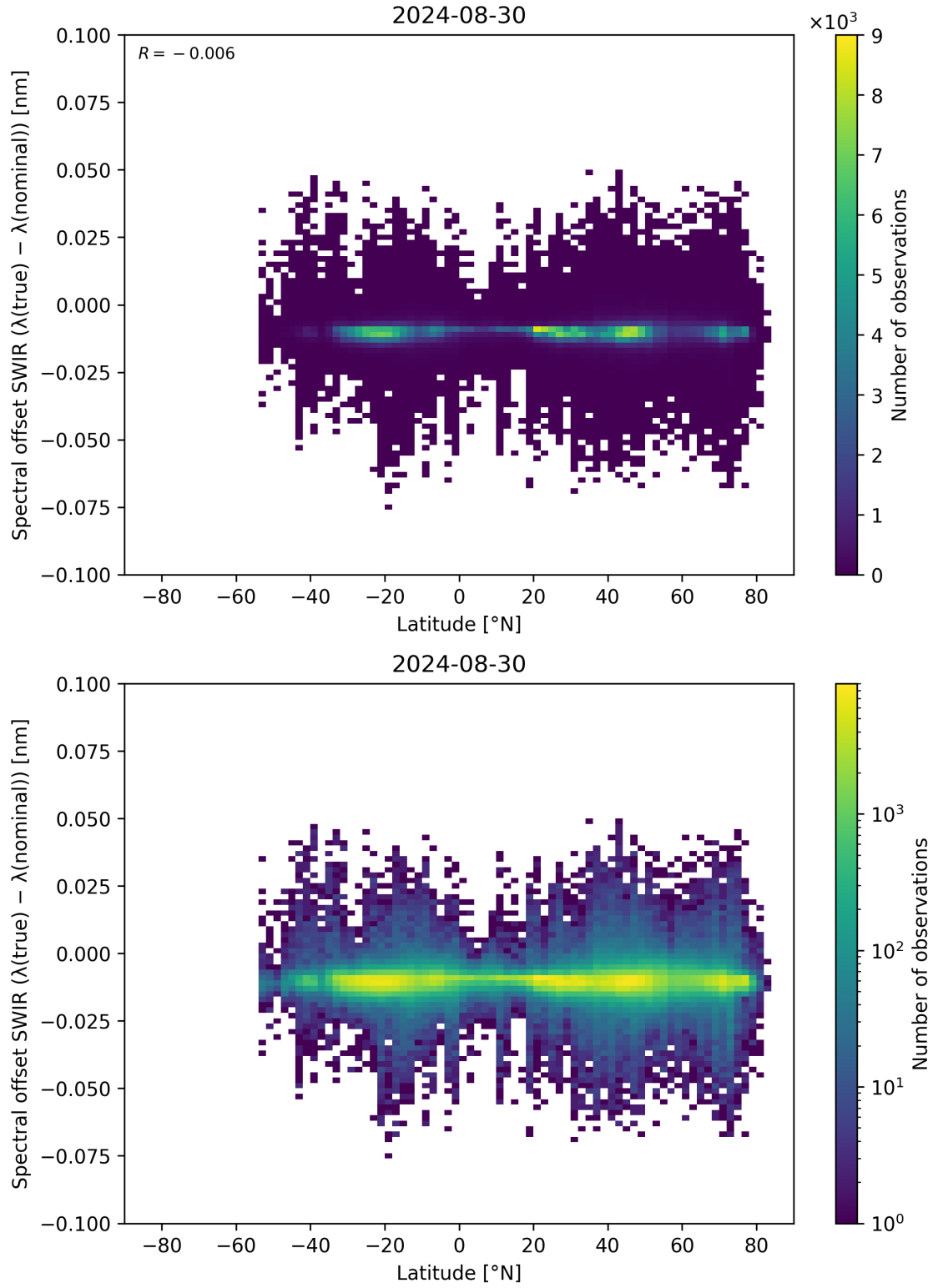
Figure 62: Scatter density plot of “Latitude” against “Spectral offset SWIR ( \lambda_{\text{true}} - \lambda_{\text{nominal}} )” for 2024-08-29 to 2024-08-31.
