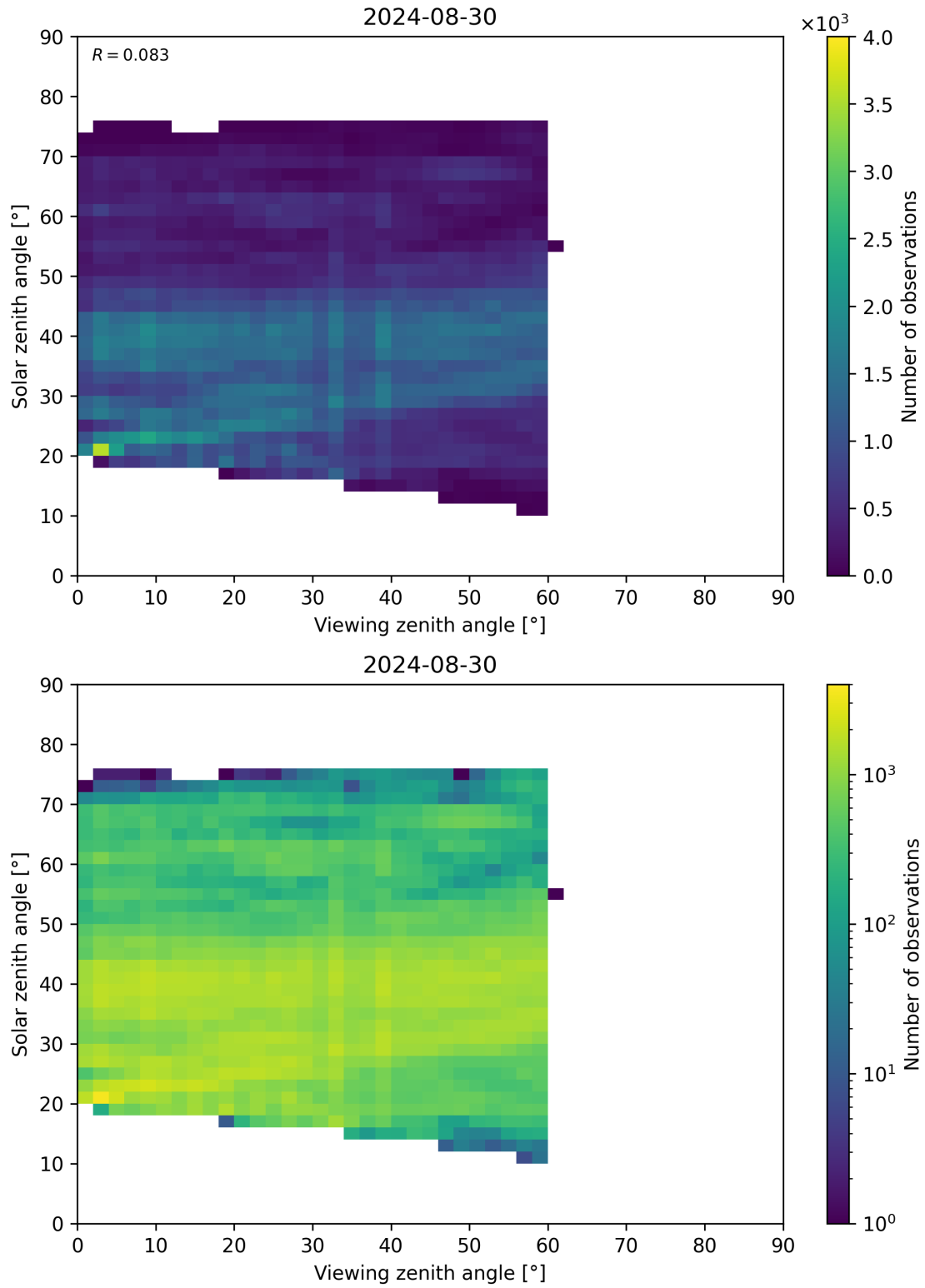
Figure 115: Scatter density plot of “Viewing zenith angle” against “Solar zenith angle” for 2024-08-29 to 2024-08-31.
