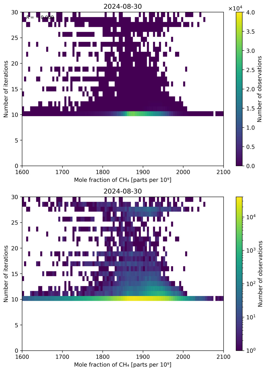
Figure 76: Scatter density plot of “Mole fraction of CH 4 ” against “Number of iterations” for 2024-08-29 to 2024-08-31.
