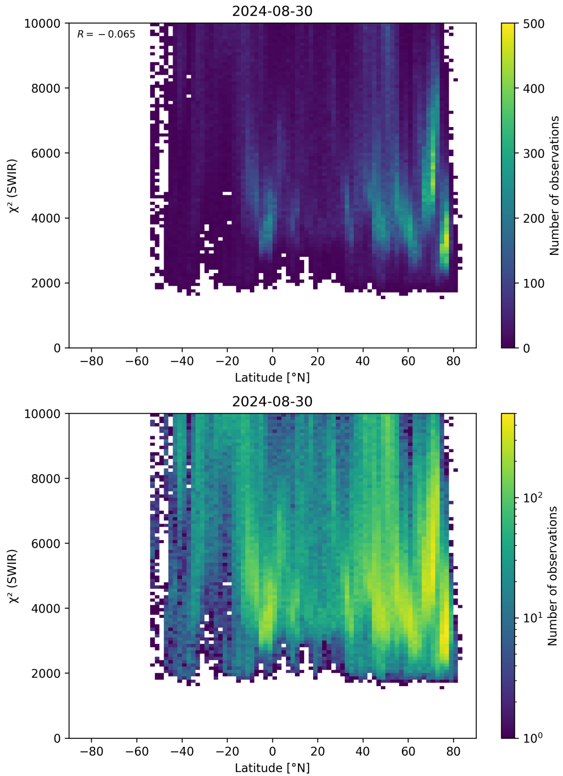
Figure 54: Scatter density plot of “Latitude” against “ \chi^2 (SWIR)” for 2024-08-29 to 2024-08-31.
