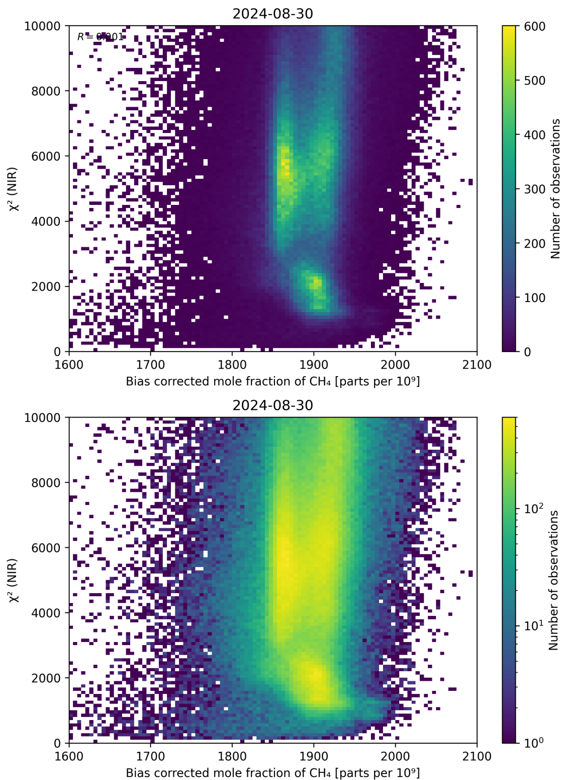
Figure 63: Scatter density plot of “Bias corrected mole fraction of CH 4 ” against “ \chi^2 (NIR)” for 2024-08-29 to 2024-08-31.
