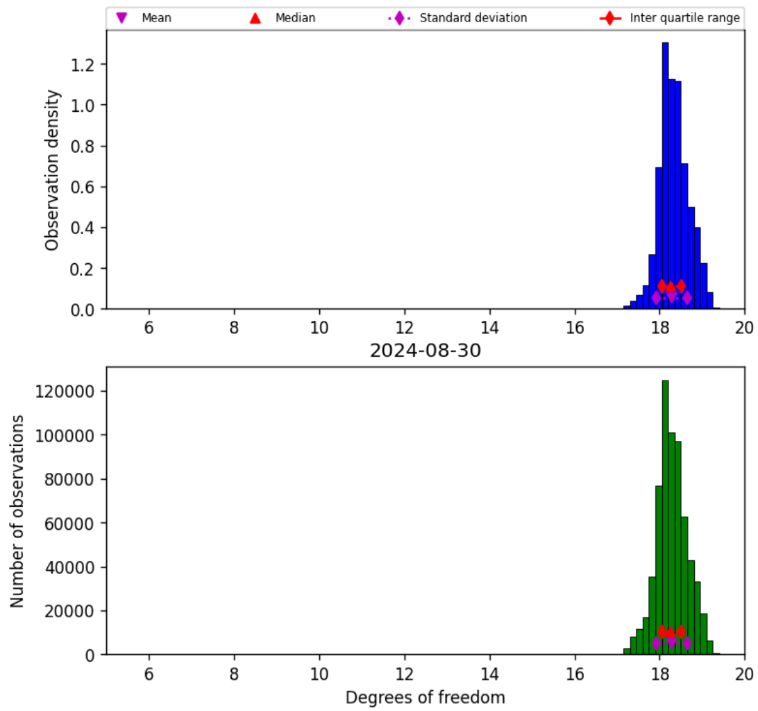
Figure 30: Histogram of “Degrees of freedom” for 2024-08-29 to 2024-08-31
