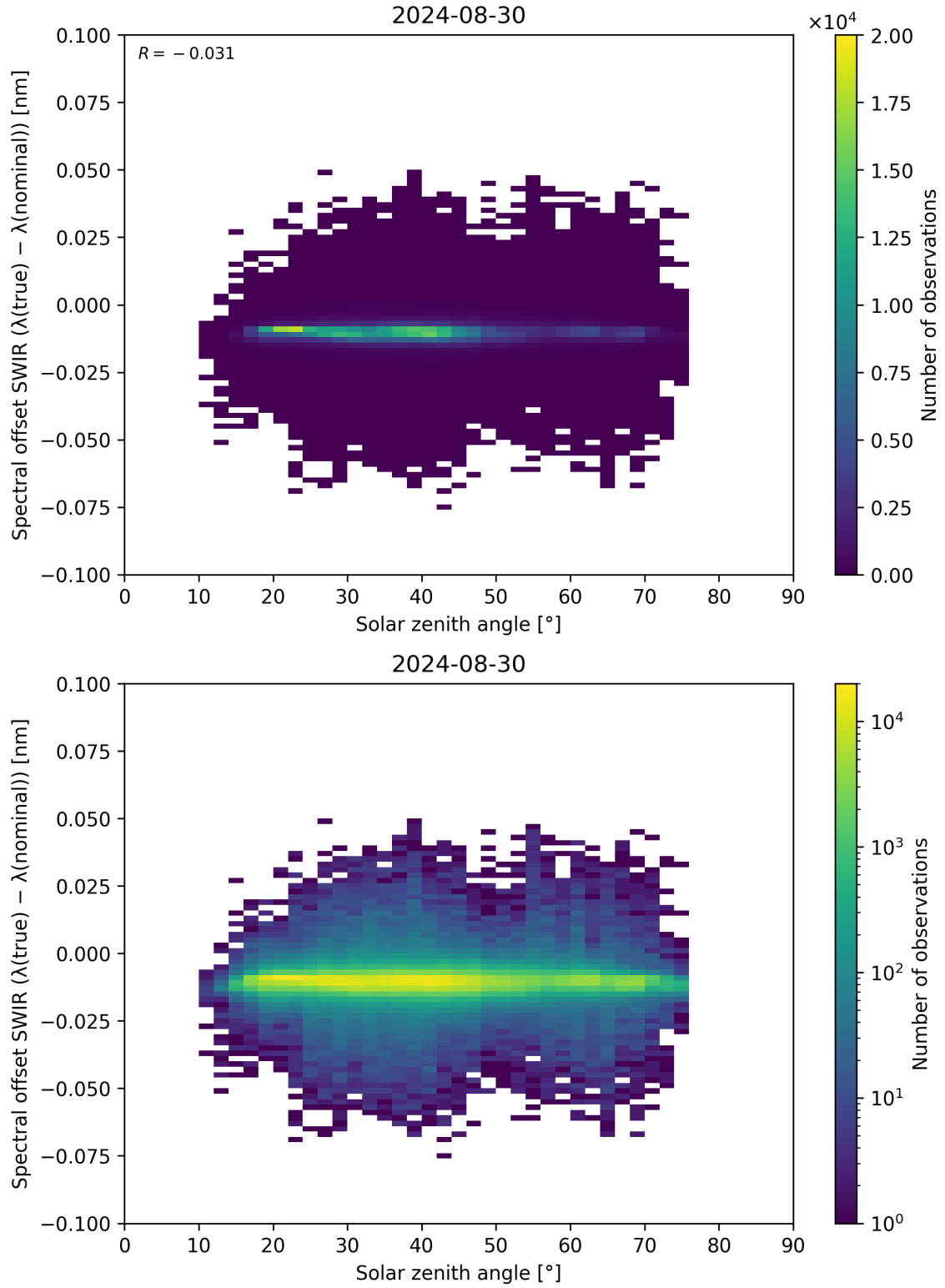
Figure 104: Scatter density plot of “Solar zenith angle” against “Spectral offset SWIR ( \lambda_{\text{true}} - \lambda_{\text{nominal}} )” for 2024-08-29 to 2024-08-31.
