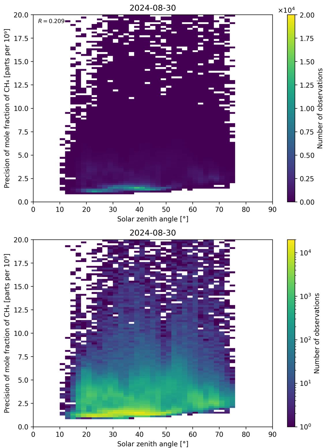
Figure 101: Scatter density plot of “Solar zenith angle” against “Precision of mole fraction of CH 4 ” for 2024-08-29 to 2024-08-31.
