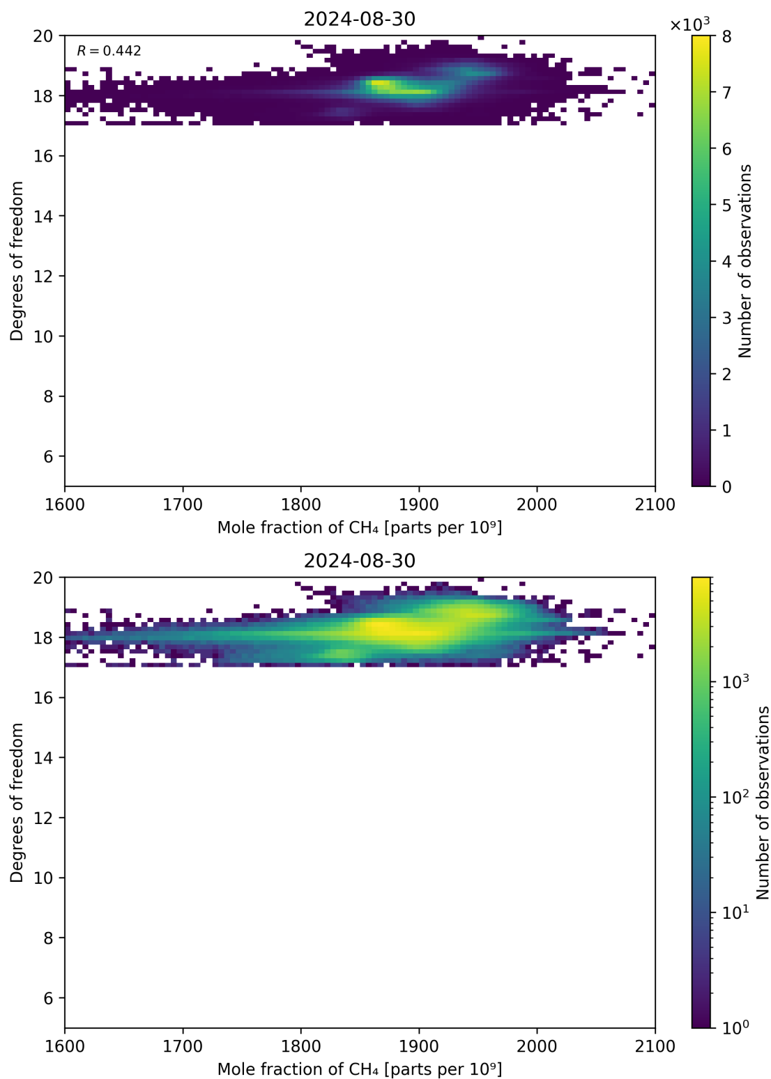
Figure 72: Scatter density plot of “Mole fraction of CH 4 ” against “Degrees of freedom” for 2024-08-29 to 2024-08-31.
