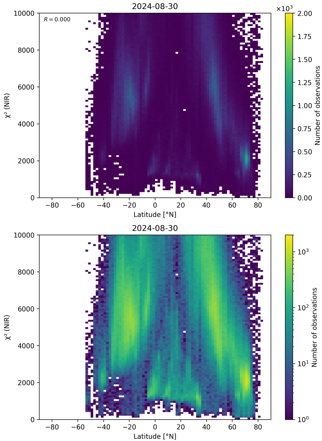
Figure 53: Scatter density plot of “Latitude” against “ \chi^2 (NIR)” for 2024-08-29 to 2024-08-31.
