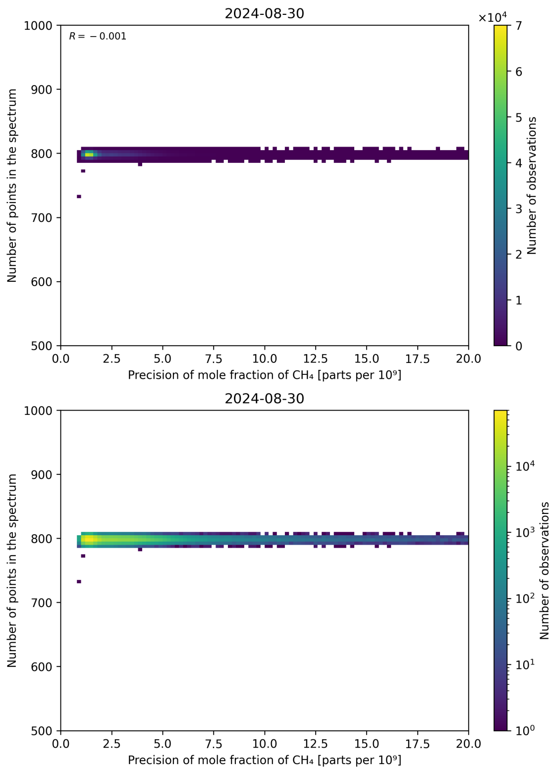
Figure 84: Scatter density plot of “Precision of mole fraction of CH 4 ” against “Number of points in the spectrum” for 2024-08-29 to 2024-08-31.
