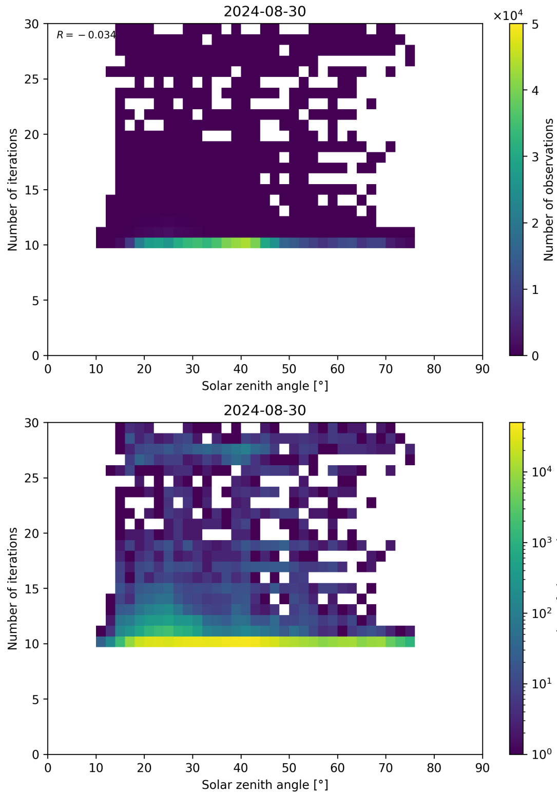
Figure 102: Scatter density plot of “Solar zenith angle” against “Number of iterations” for 2024-08-29 to 2024-08-31.
