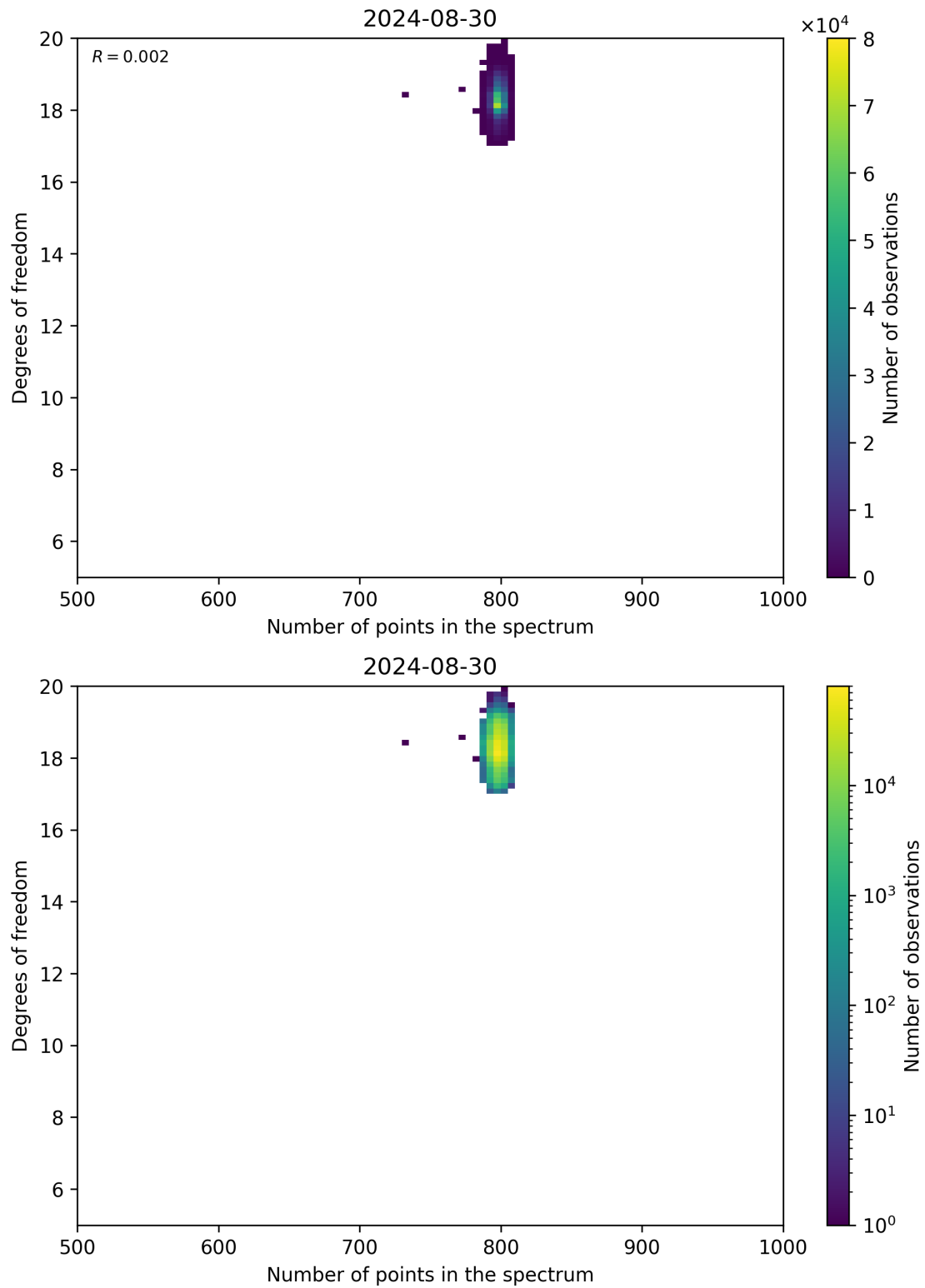
Figure 90: Scatter density plot of “Number of points in the spectrum” against “Degrees of freedom” for 2024-08-29 to 2024-08-31.
