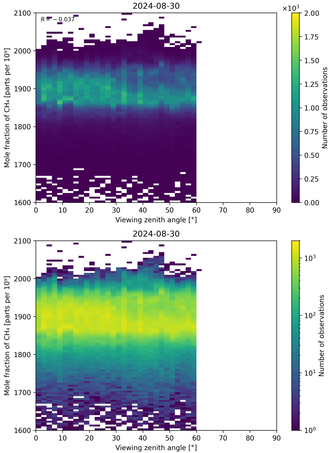
Figure 110: Scatter density plot of “Viewing zenith angle” against “Mole fraction of CH 4 ” for 2024-08-29 to 2024-08-31.
