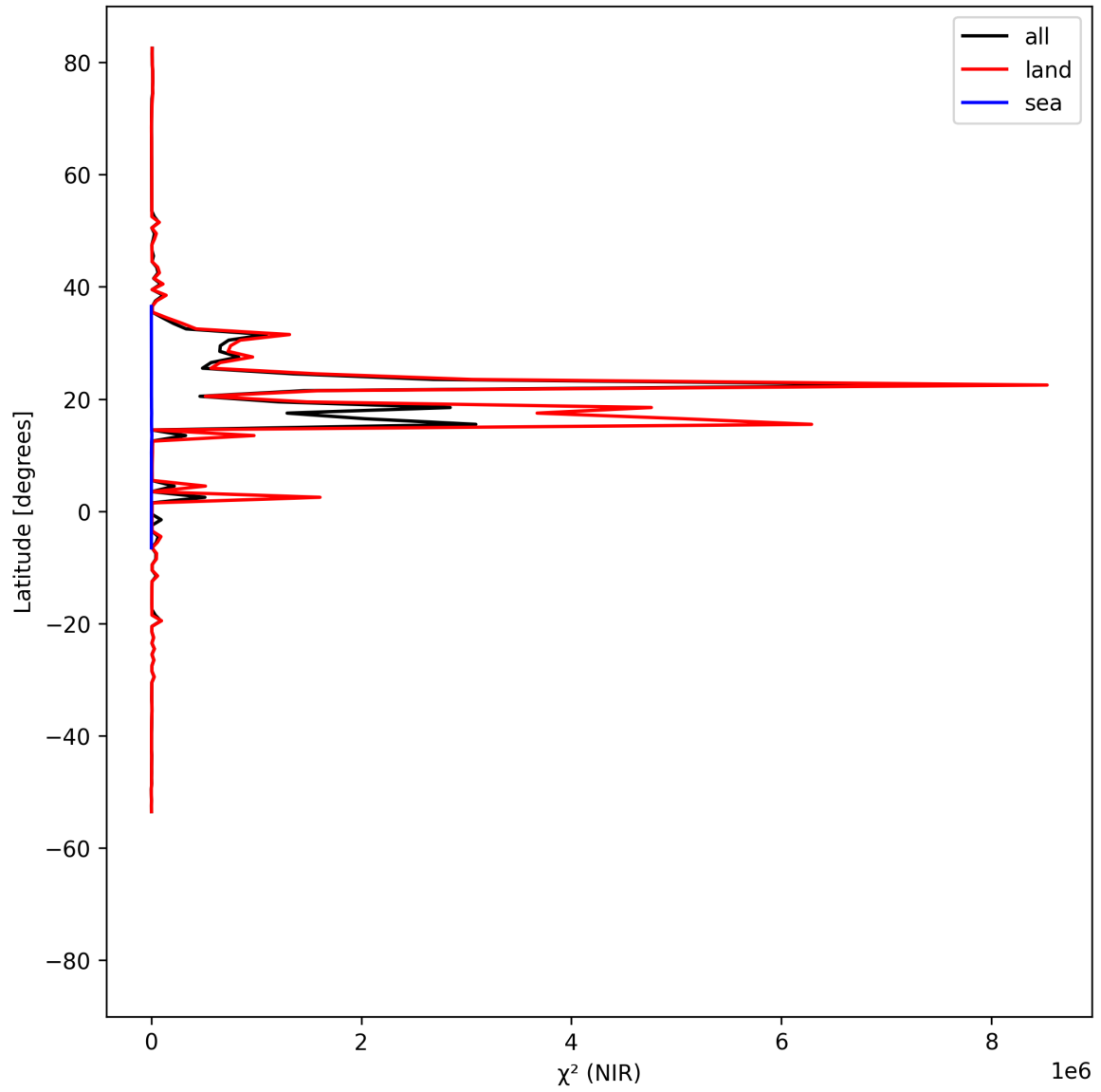
Figure 18: Zonal average of “ \chi^2 (NIR)” for 2024-08-29 to 2024-08-31.
