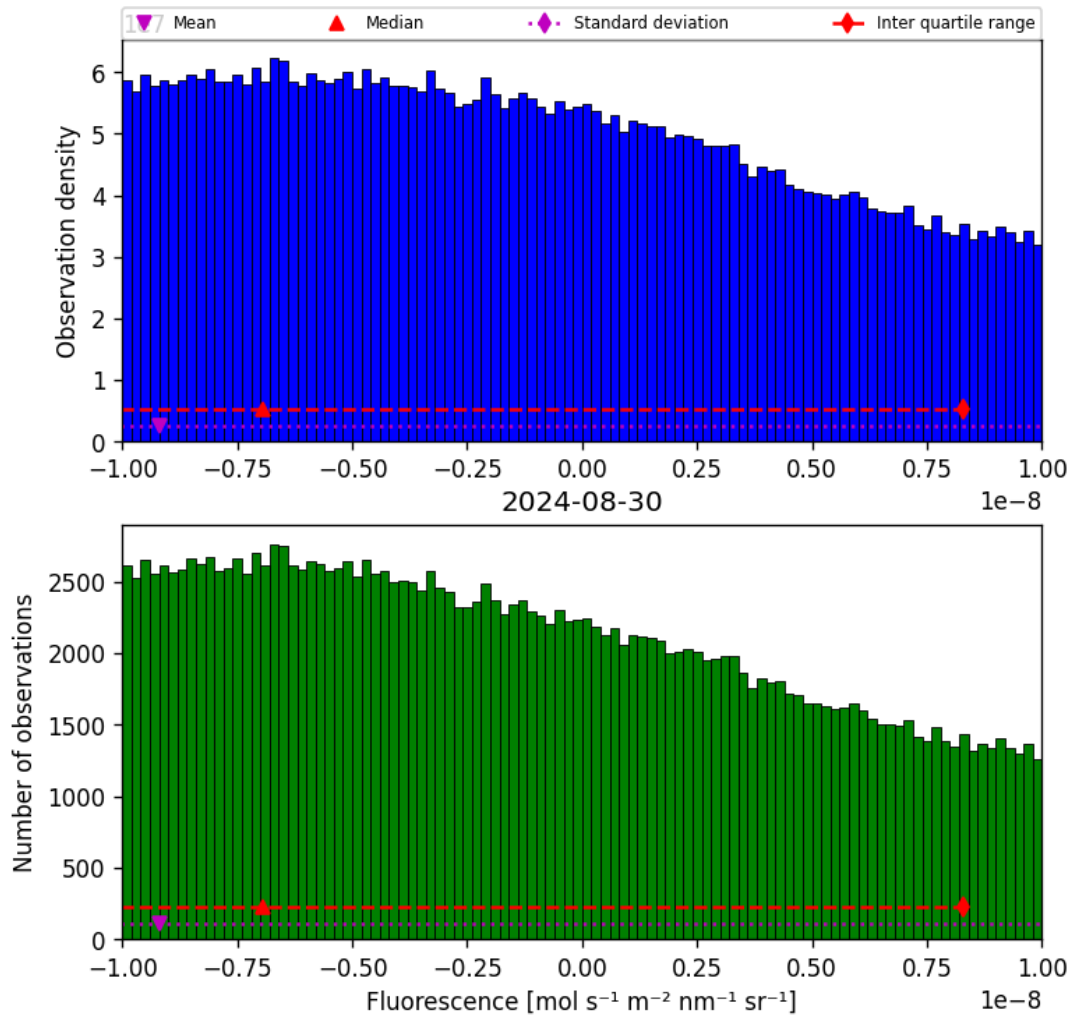
Figure 32: Histogram of “Fluorescence” for 2024-08-29 to 2024-08-31
