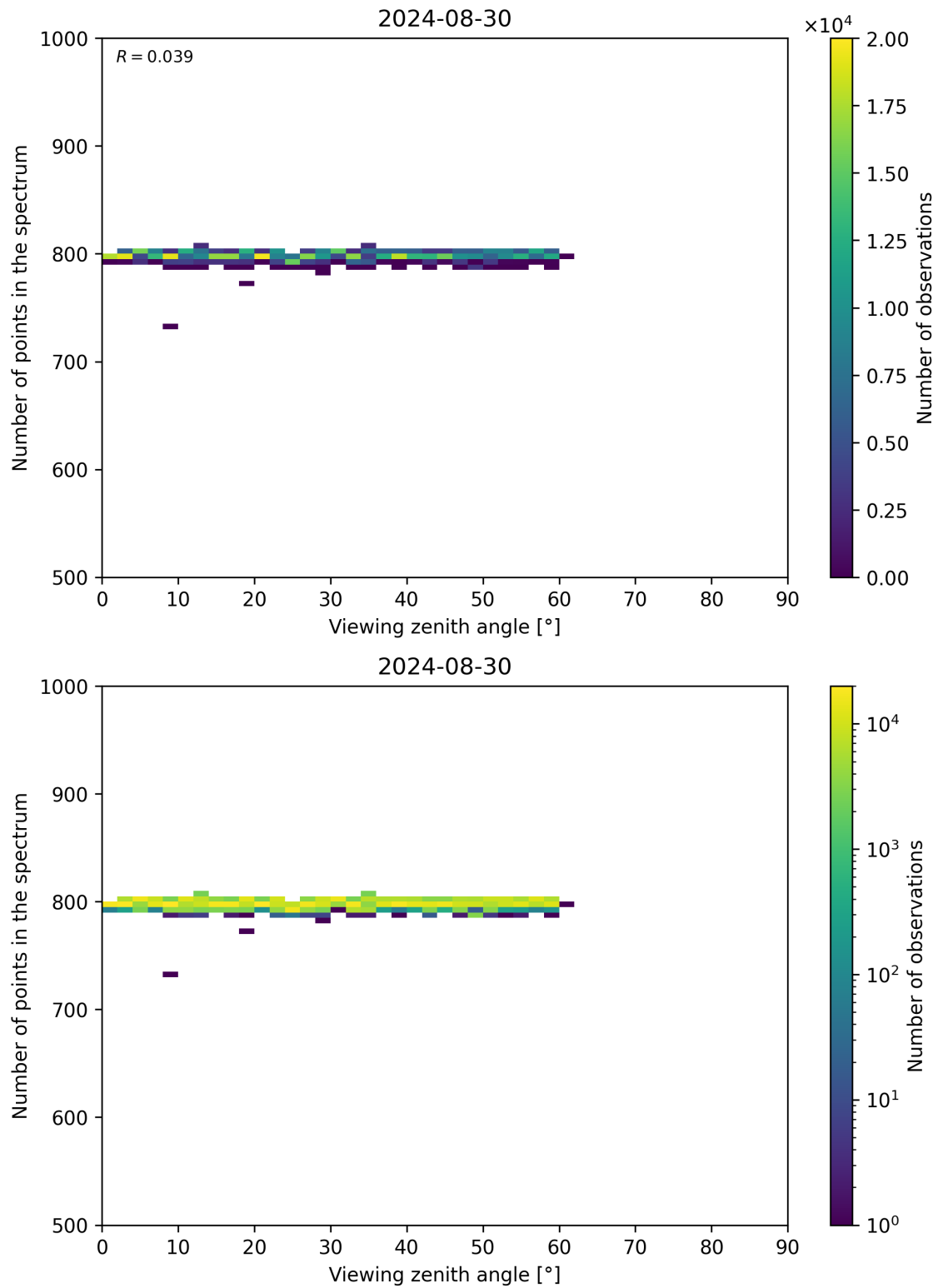
Figure 114: Scatter density plot of “Viewing zenith angle” against “Number of points in the spectrum” for 2024-08-29 to 2024-08-31.
