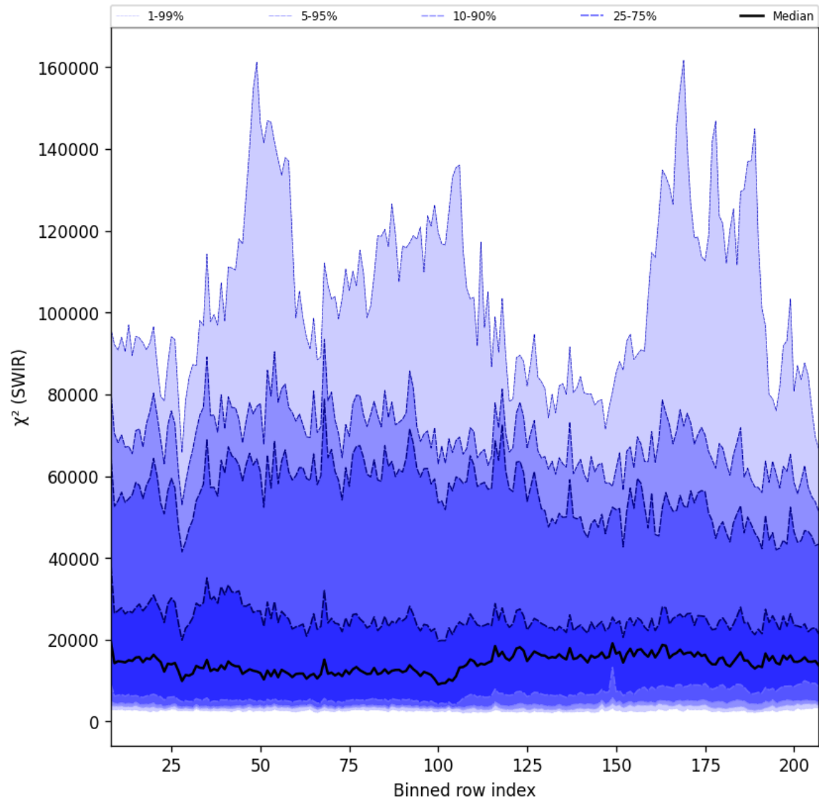
Figure 39: Along track statistics of " \chi^2 (SWIR)" for 2024-08-29 to 2024-08-31
