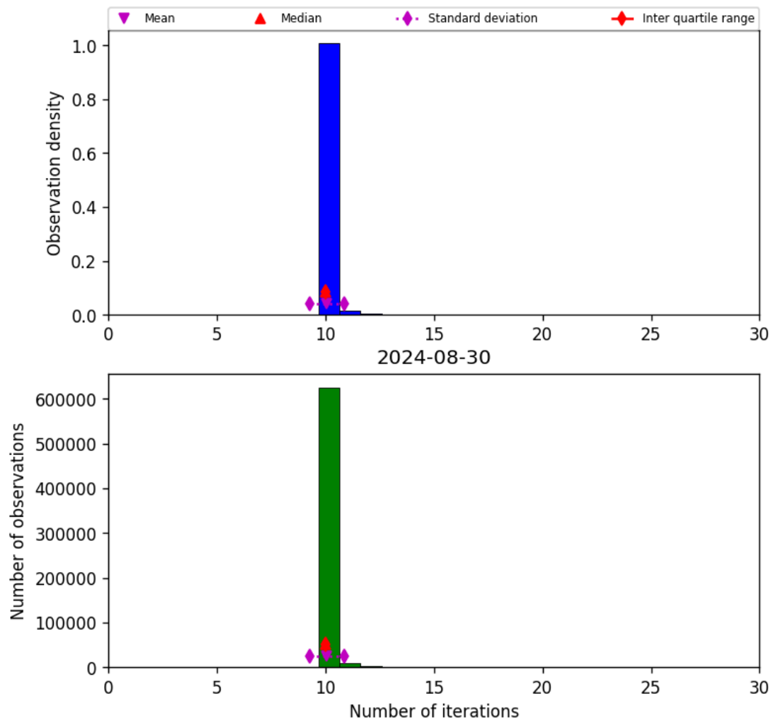
Figure 31: Histogram of “Number of iterations” for 2024-08-29 to 2024-08-31
