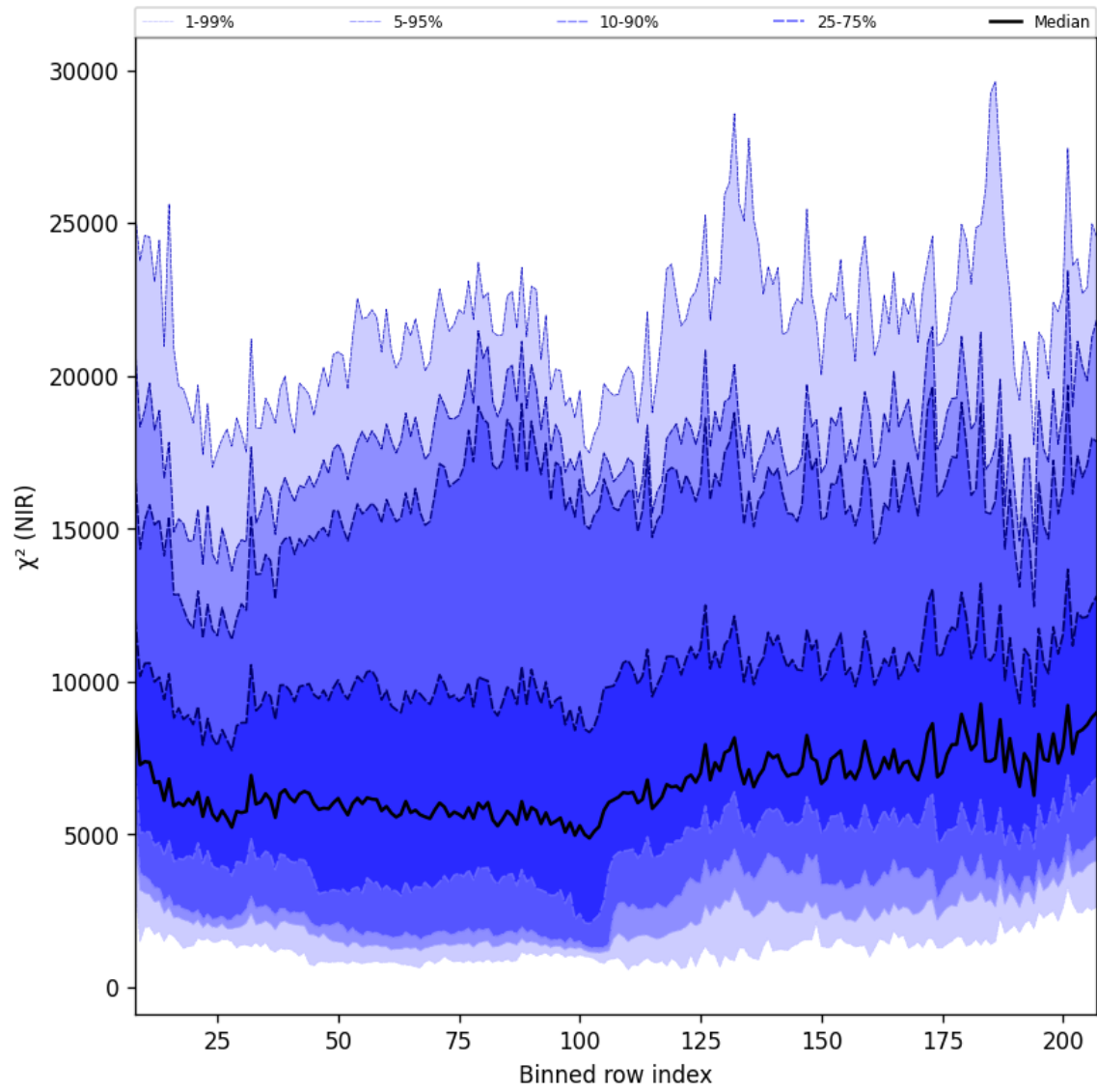
Figure 40: Along track statistics of " \chi^2 (NIR)" for 2024-08-29 to 2024-08-31
