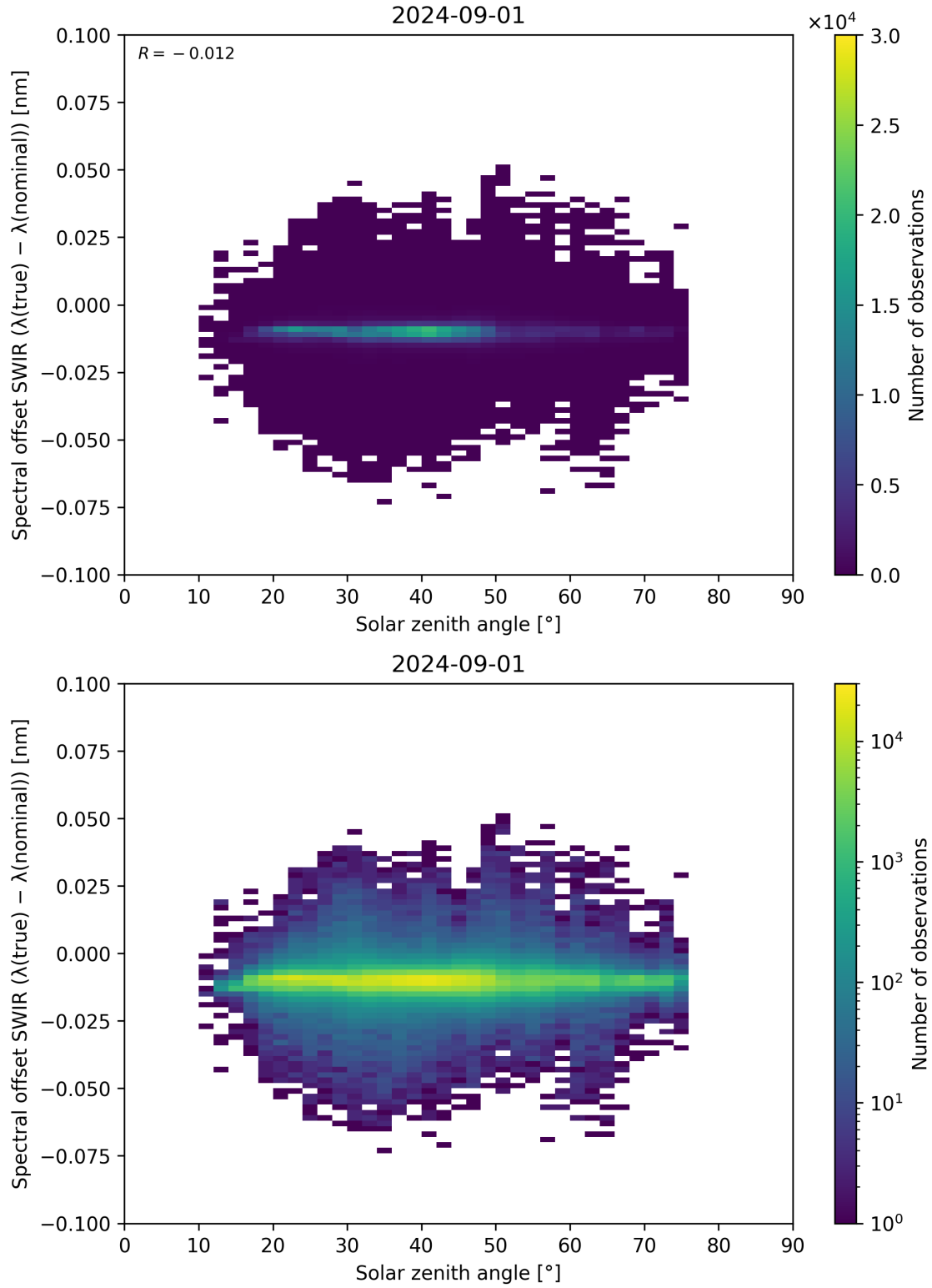
Figure 104: Scatter density plot of “Solar zenith angle” against “Spectral offset SWIR ( \lambda_{\text{true}} - \lambda_{\text{nominal}} )” for 2024-09-01 to 2024-09-02.
