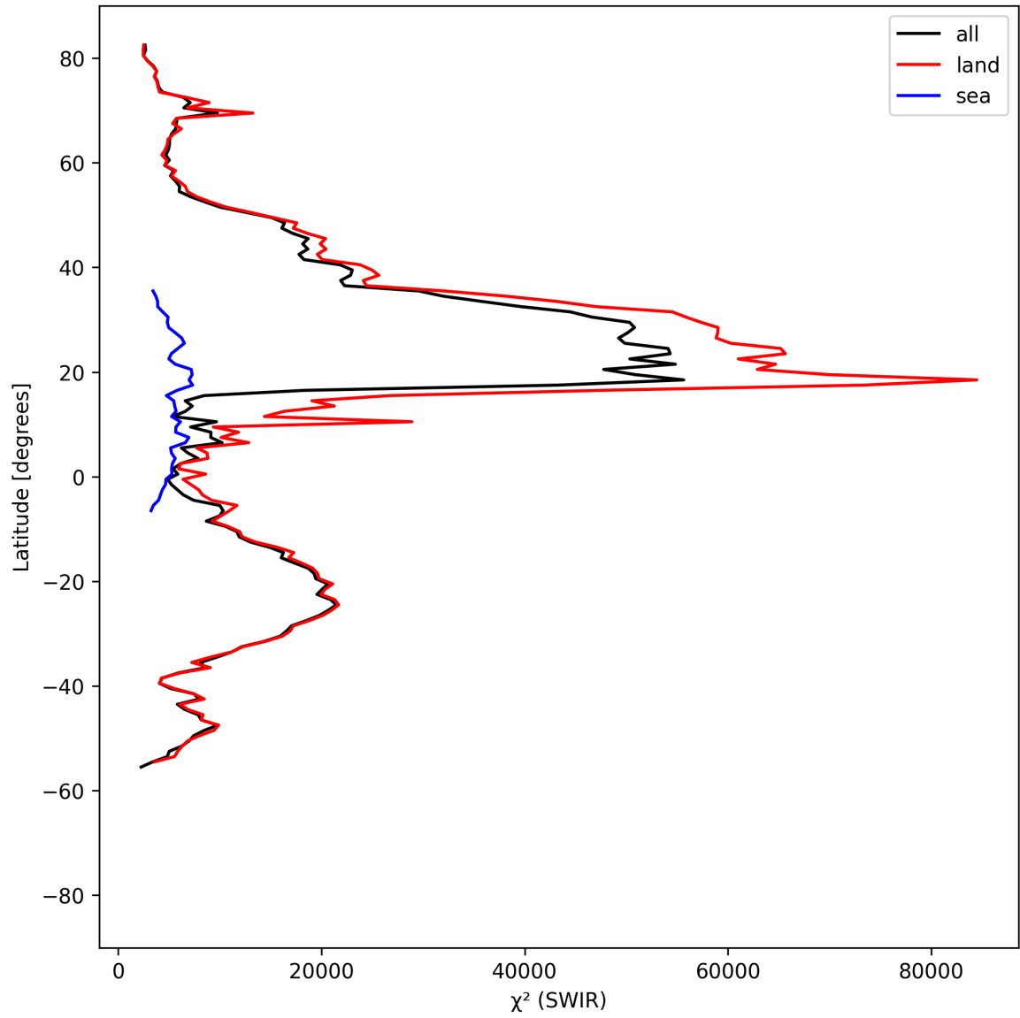
Figure 17: Zonal average of “ \chi^2 (SWIR)” for 2024-09-01 to 2024-09-02.
