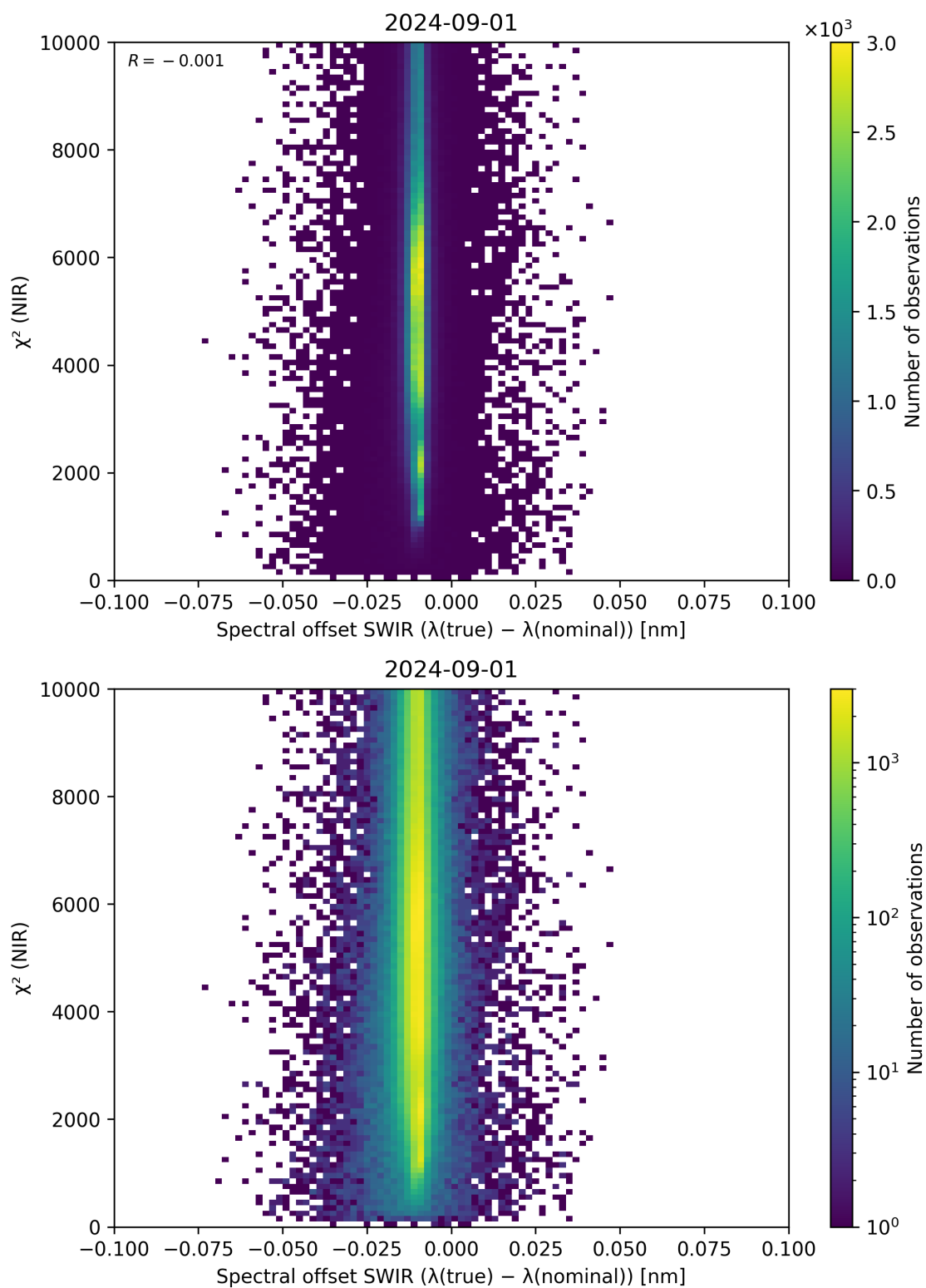
Figure 117: Scatter density plot of “Spectral offset SWIR ( \lambda_{\text{true}} - \lambda_{\text{nominal}} )” against “ \chi^2 (NIR)” for 2024-09-01 to 2024-09-02.
