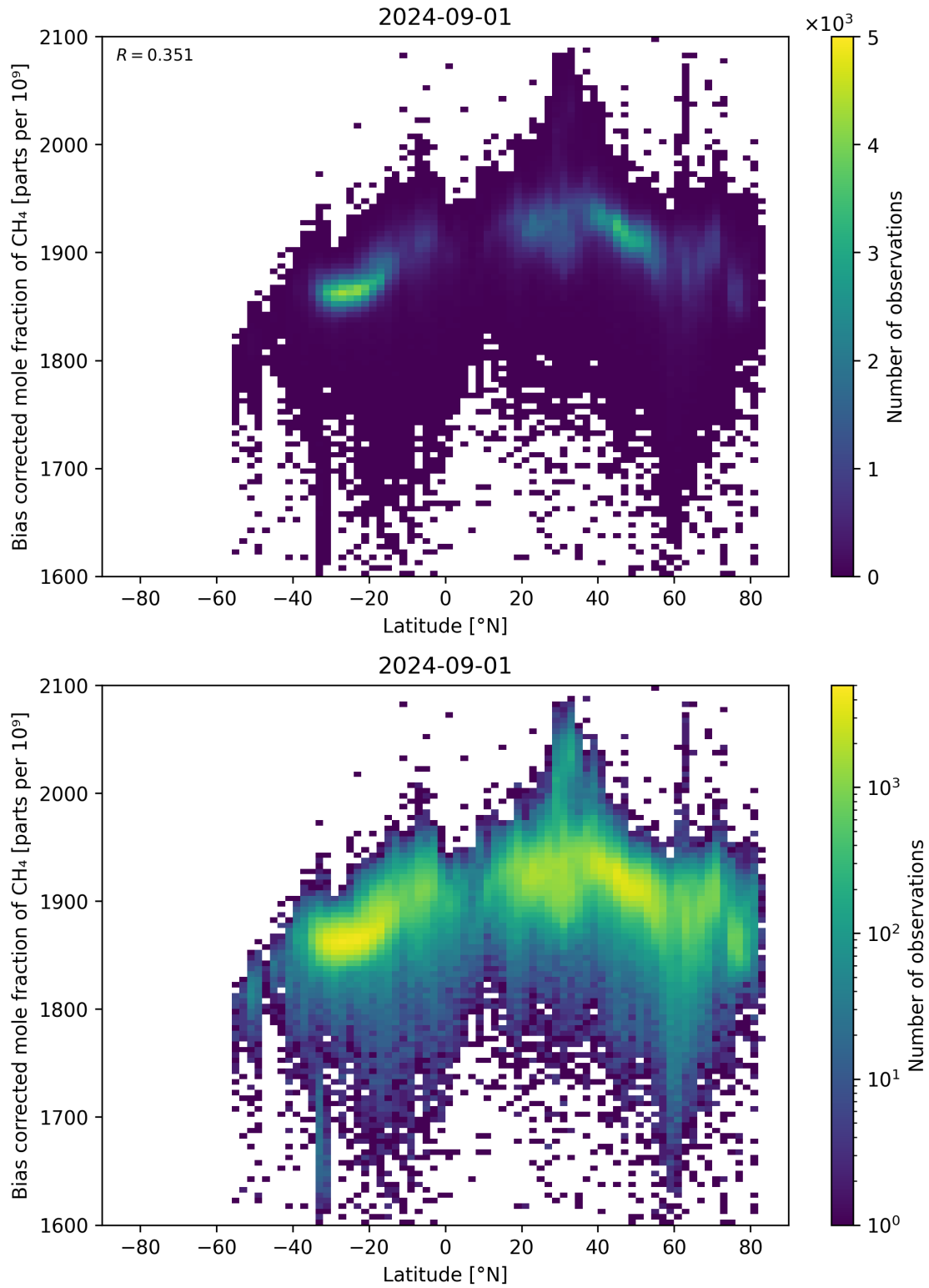
Figure 58: Scatter density plot of “Latitude” against “Bias corrected mole fraction of CH 4 ” for 2024-09-01 to 2024-09-02.
