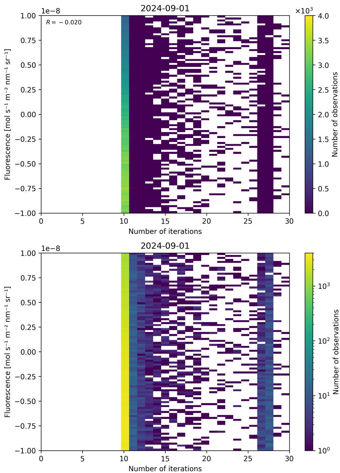
Figure 87: Scatter density plot of "Number of iterations" against "Fluorescence" for 2024-09-01 to 2024-09-02.
