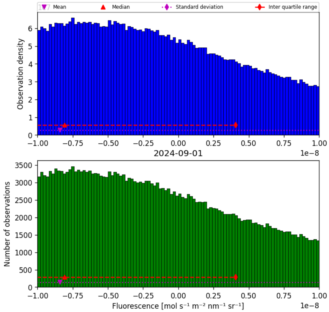
Figure 32: Histogram of “Fluorescence” for 2024-09-01 to 2024-09-02
