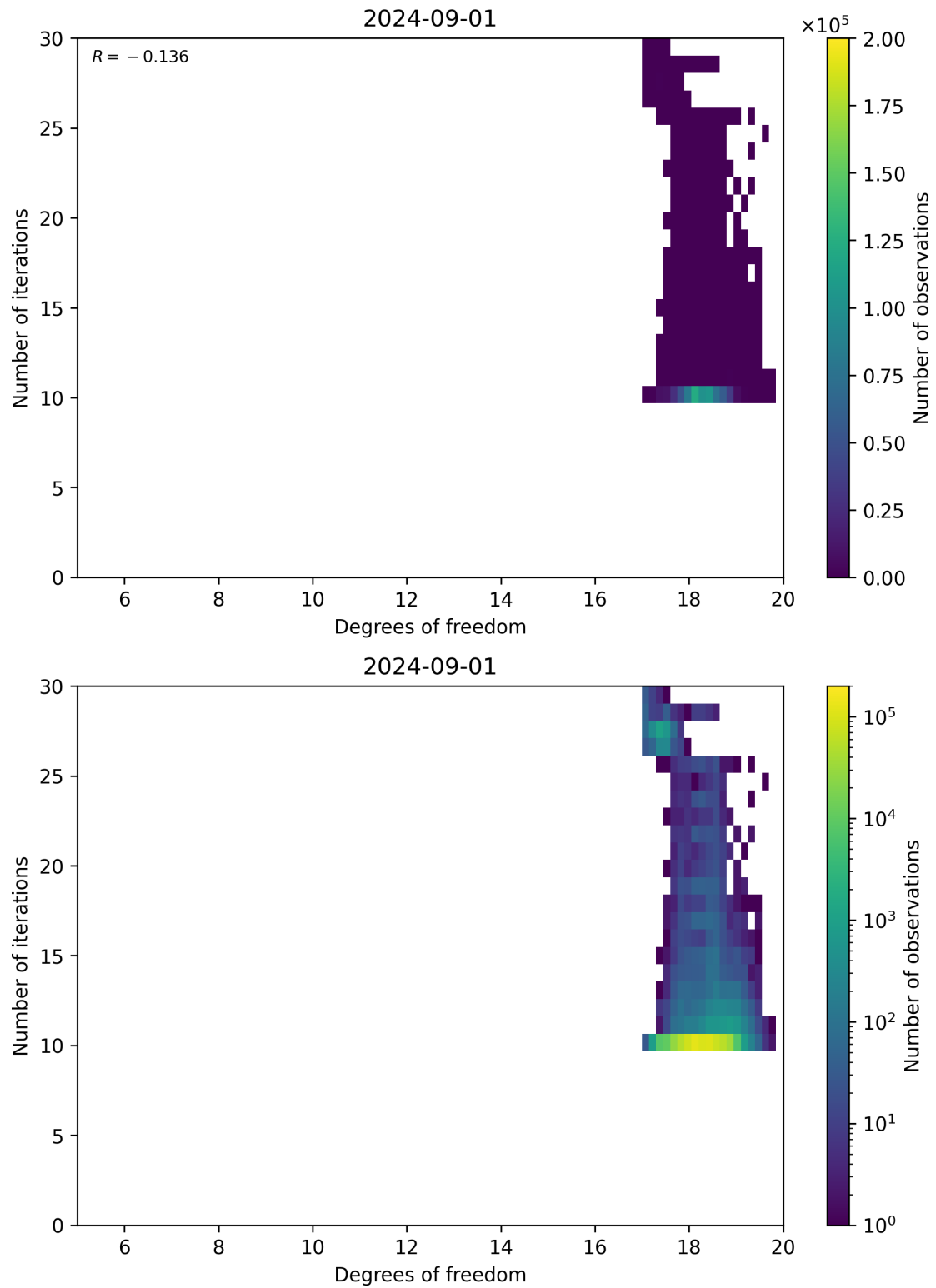
Figure 52: Scatter density plot of “Degrees of freedom” against “Number of iterations” for 2024-09-01 to 2024-09-02.
