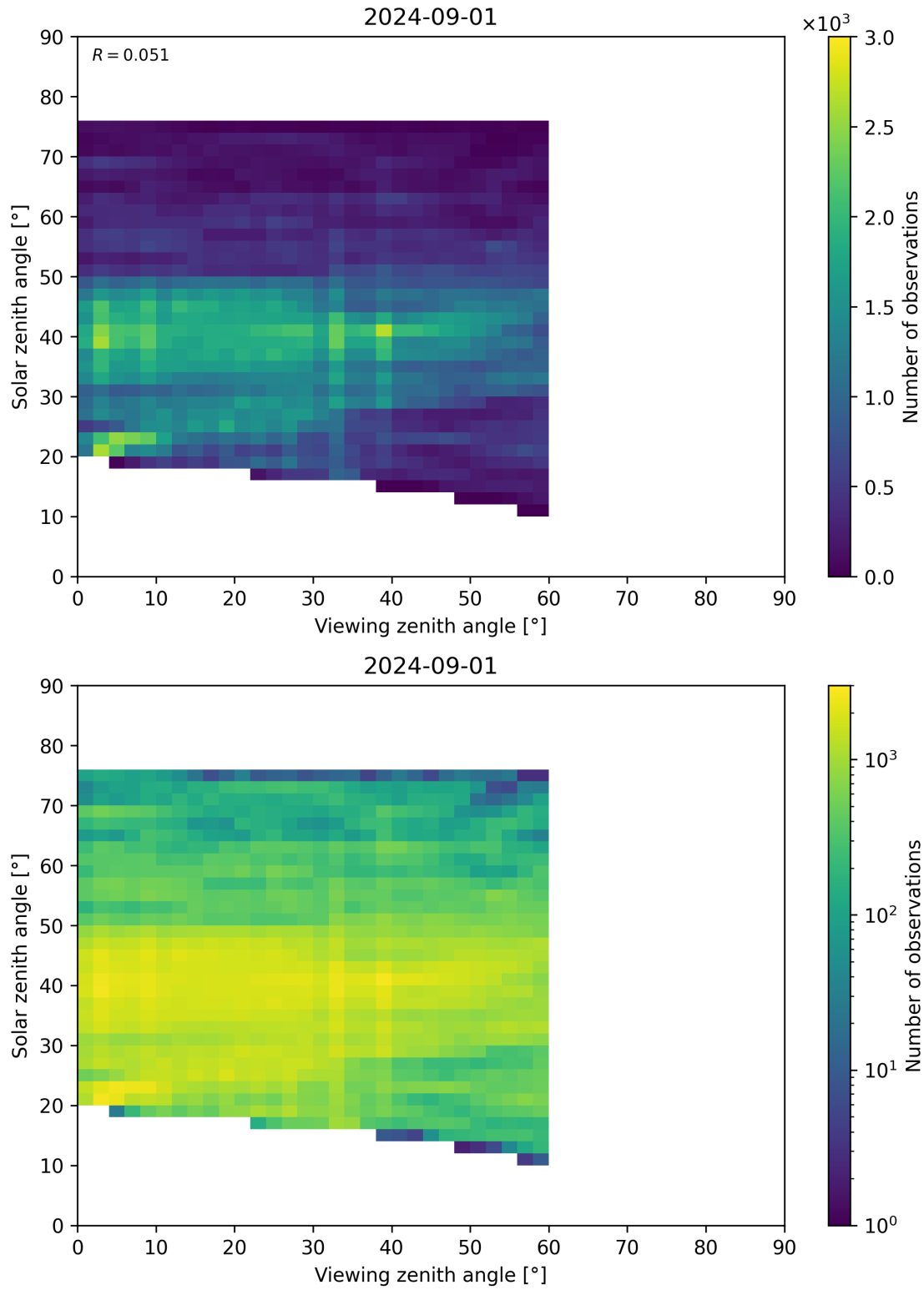
Figure 115: Scatter density plot of “Viewing zenith angle” against “Solar zenith angle” for 2024-09-01 to 2024-09-02.
