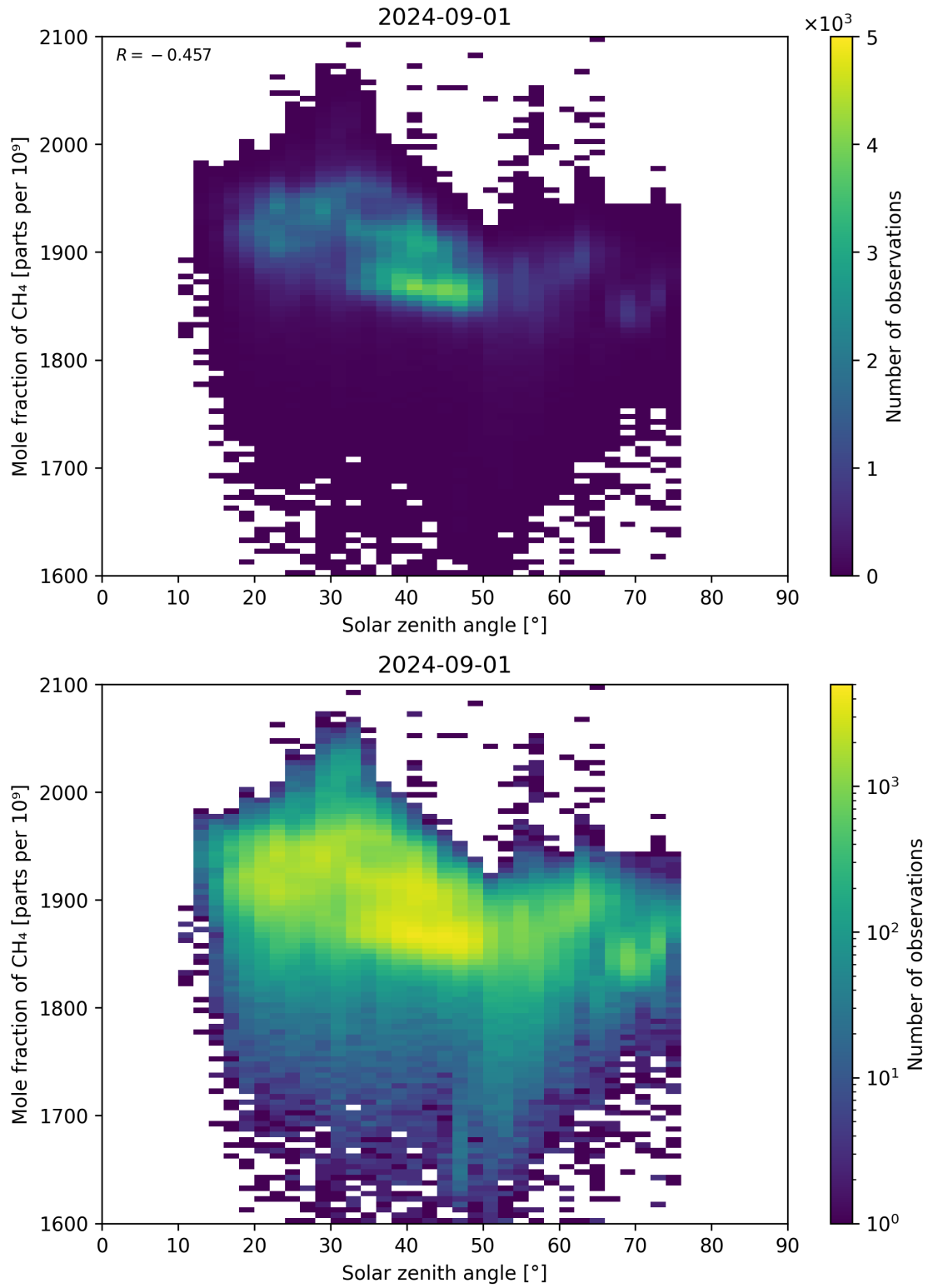
Figure 99: Scatter density plot of “Solar zenith angle” against “Mole fraction of CH 4 ” for 2024-09-01 to 2024-09-02.
