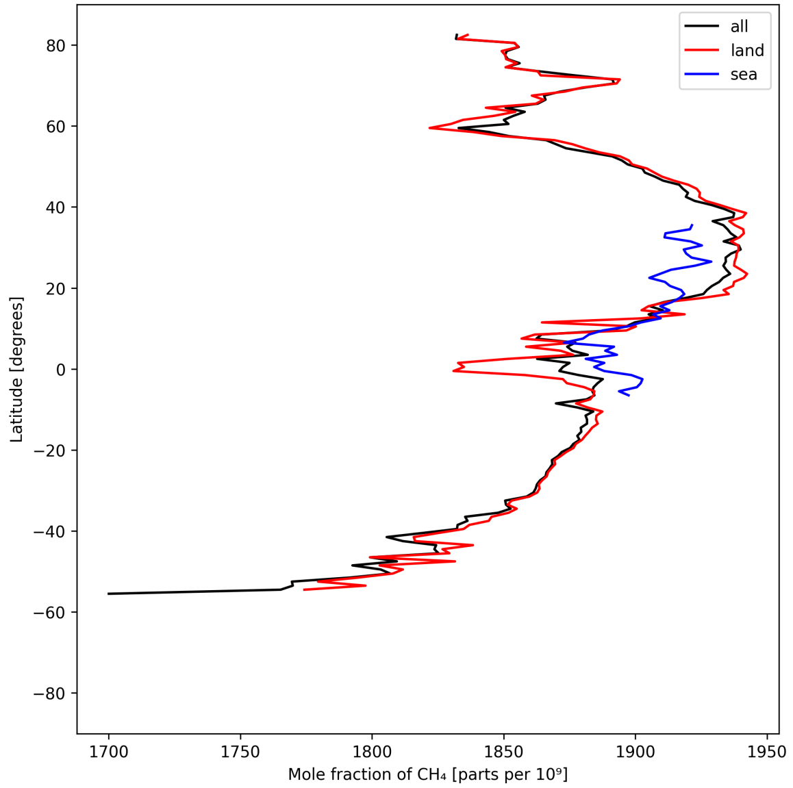
Figure 12: Zonal average of “Mole fraction of CH 4 ” for 2024-09-01 to 2024-09-02.
