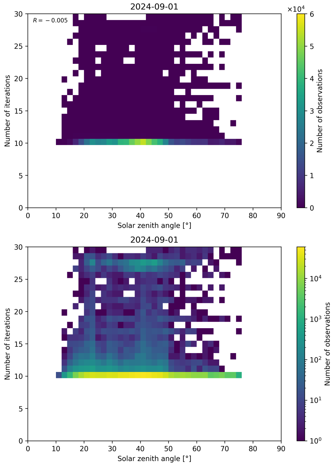
Figure 102: Scatter density plot of “Solar zenith angle” against “Number of iterations” for 2024-09-01 to 2024-09-02.
