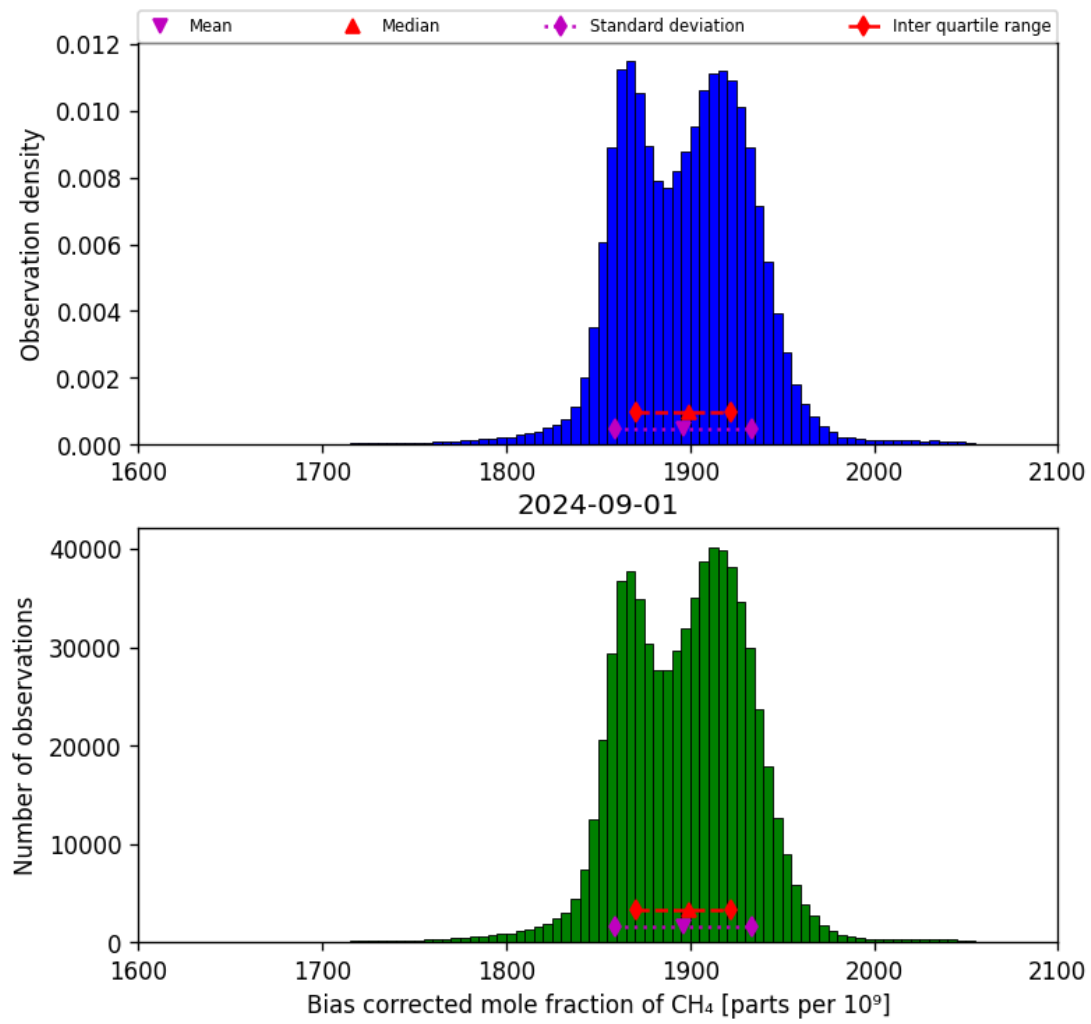
Figure 25: Histogram of “Bias corrected mole fraction of CH 4 ” for 2024-09-01 to 2024-09-02
