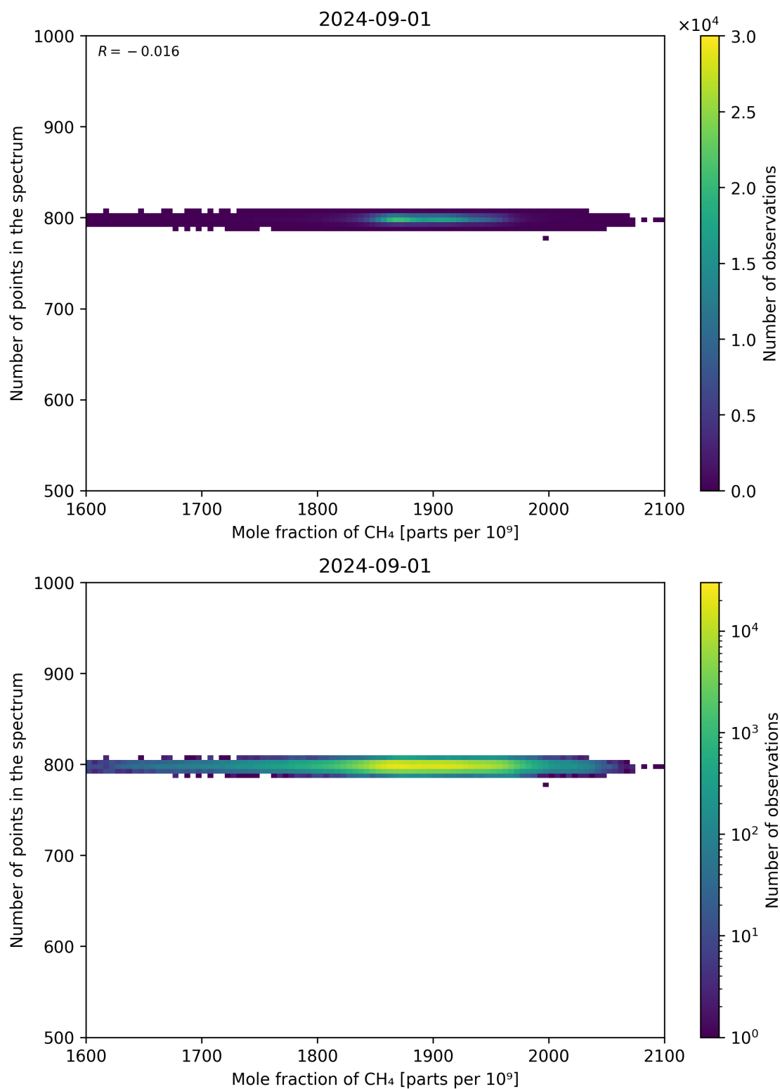
Figure 77: Scatter density plot of “Mole fraction of CH 4 ” against “Number of points in the spectrum” for 2024-09-01 to 2024-09-02.
