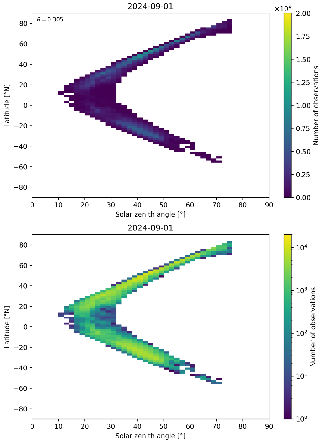
Figure 98: Scatter density plot of “Solar zenith angle” against “Latitude” for 2024-09-01 to 2024-09-02.
