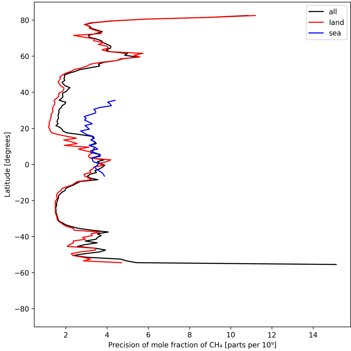
Figure 13: Zonal average of “Precision of mole fraction of CH 4 ” for 2024-09-01 to 2024-09-02.
