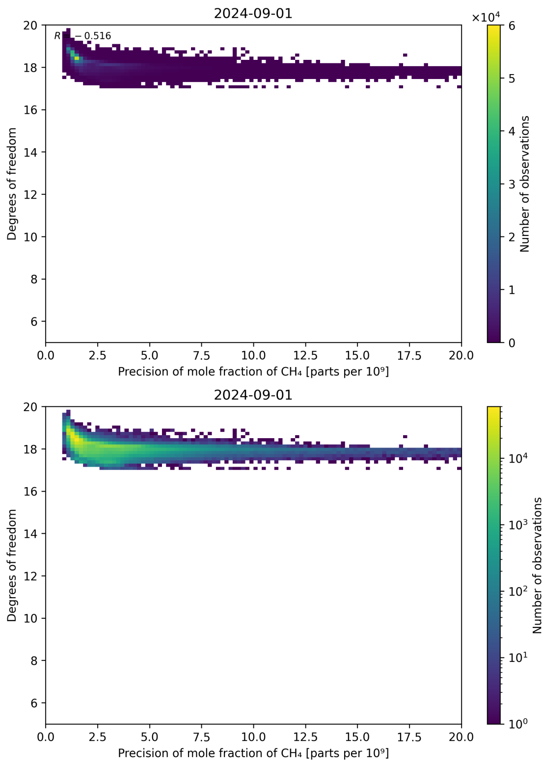
Figure 80: Scatter density plot of “Precision of mole fraction of CH 4 ” against “Degrees of freedom” for 2024-09-01 to 2024-09-02.
