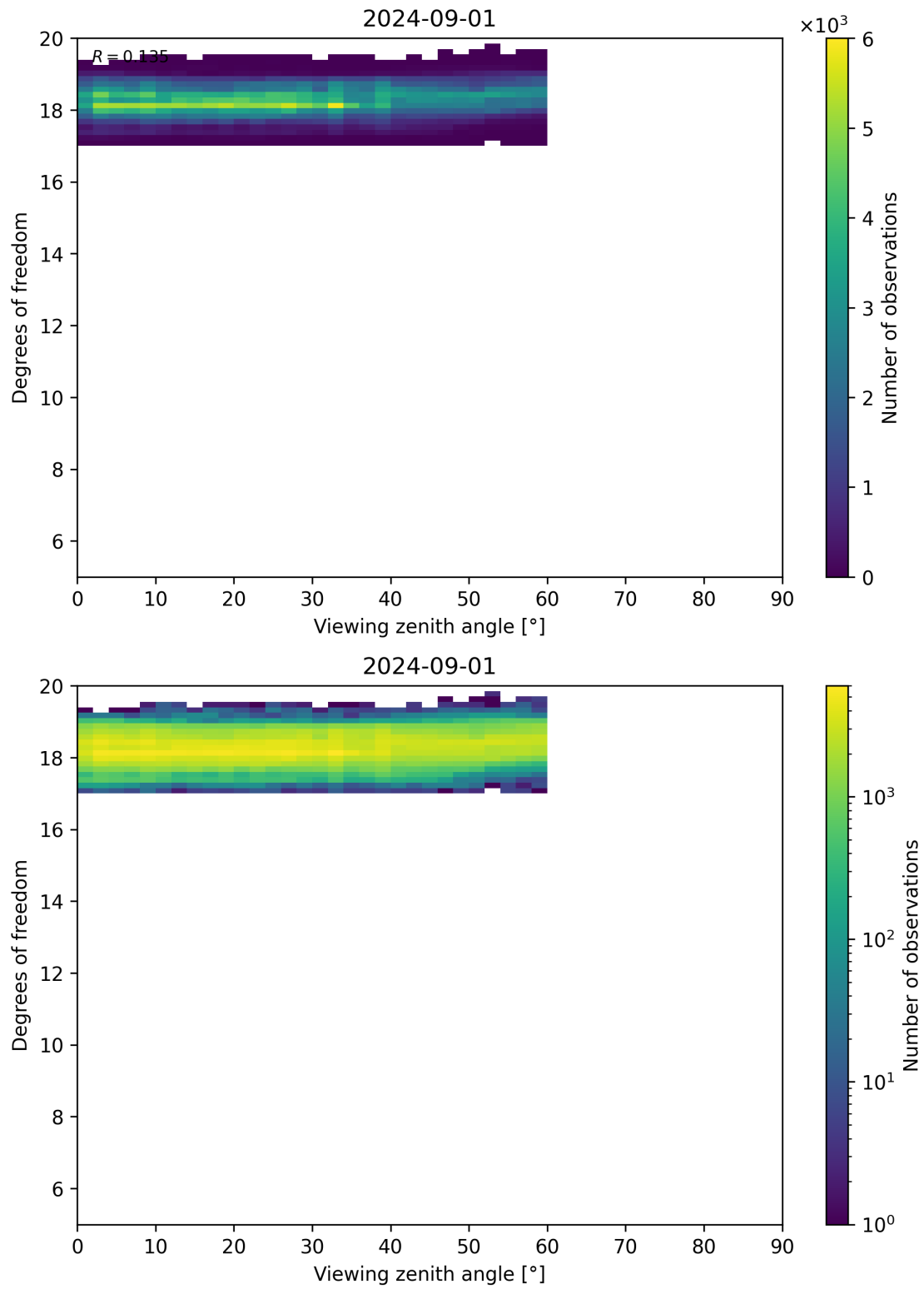
Figure 107: Scatter density plot of “Viewing zenith angle” against “Degrees of freedom” for 2024-09-01 to 2024-09-02.
