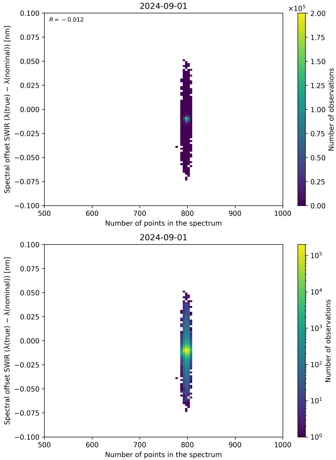
Figure 93: Scatter density plot of “Number of points in the spectrum” against “Spectral offset SWIR ( \lambda_{\text{true}} - \lambda_{\text{nominal}} )” for 2024-09-01 to 2024-09-02.
