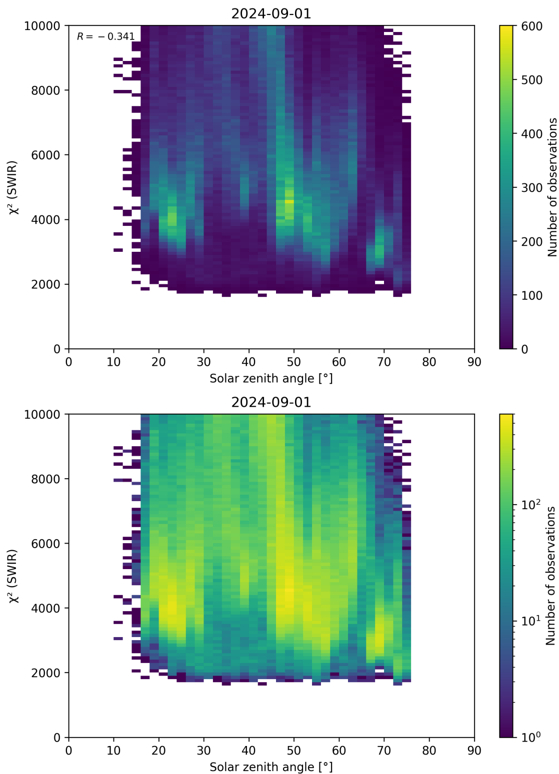
Figure 95: Scatter density plot of “Solar zenith angle” against “ \chi^2 (SWIR)” for 2024-09-01 to 2024-09-02.
