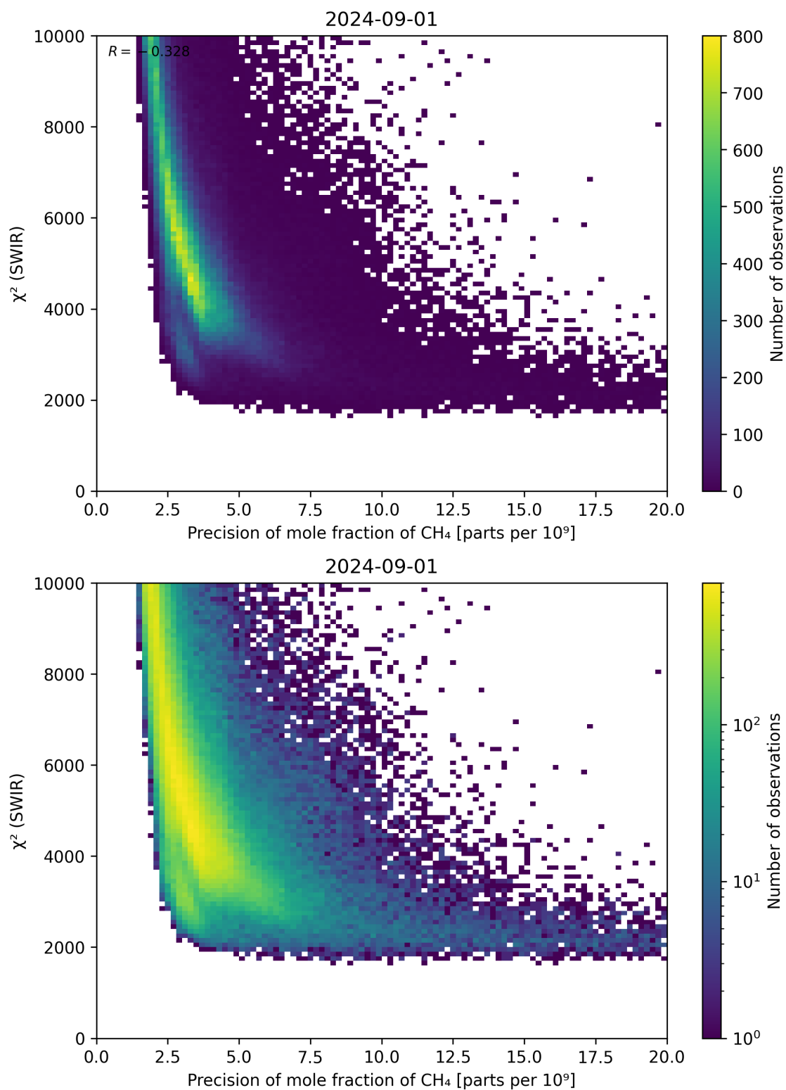
Figure 79: Scatter density plot of “Precision of mole fraction of \text{CH}_4 ” against “ \chi^2 (SWIR)” for 2024-09-01 to 2024-09-02.
