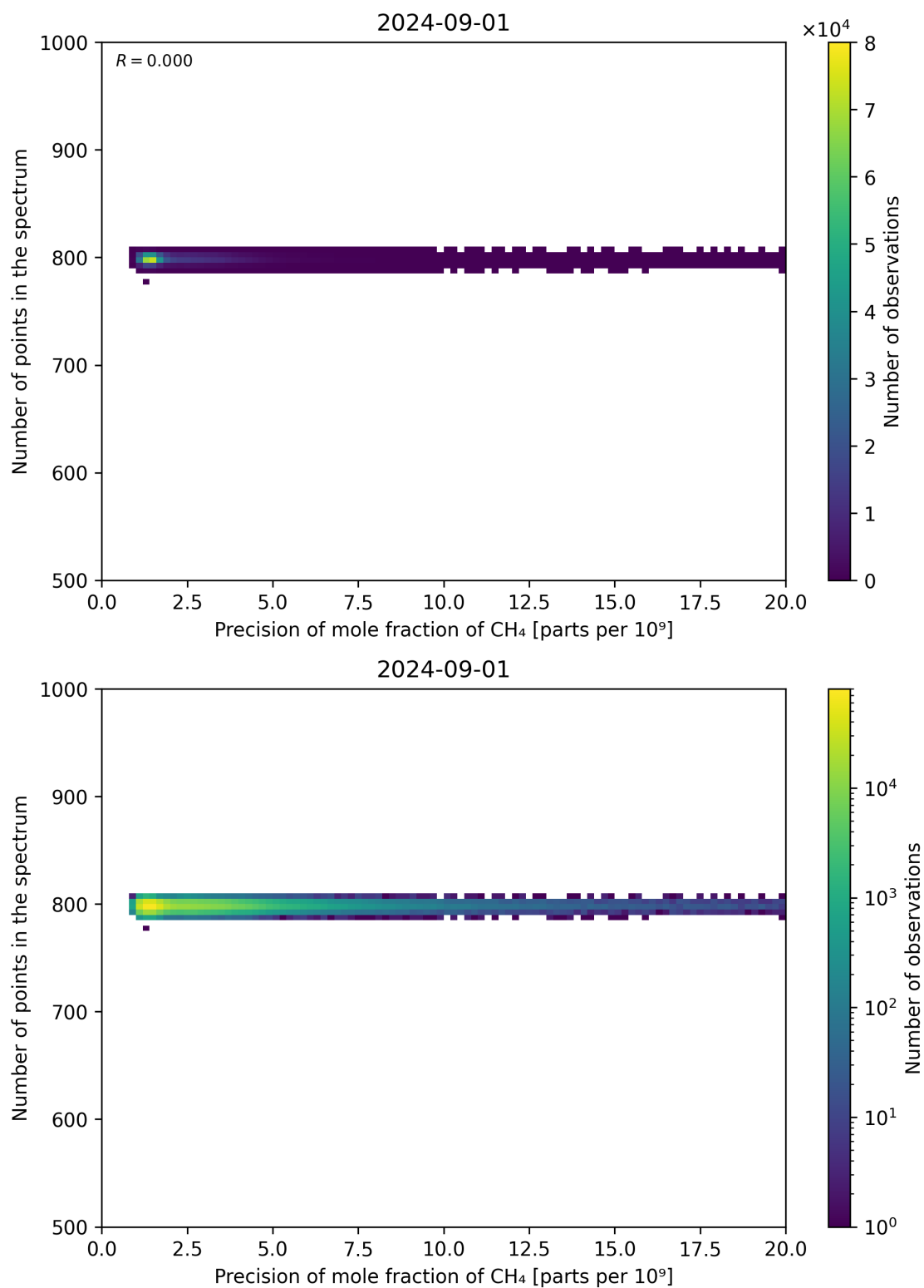
Figure 84: Scatter density plot of “Precision of mole fraction of CH 4 ” against “Number of points in the spectrum” for 2024-09-01 to 2024-09-02.
