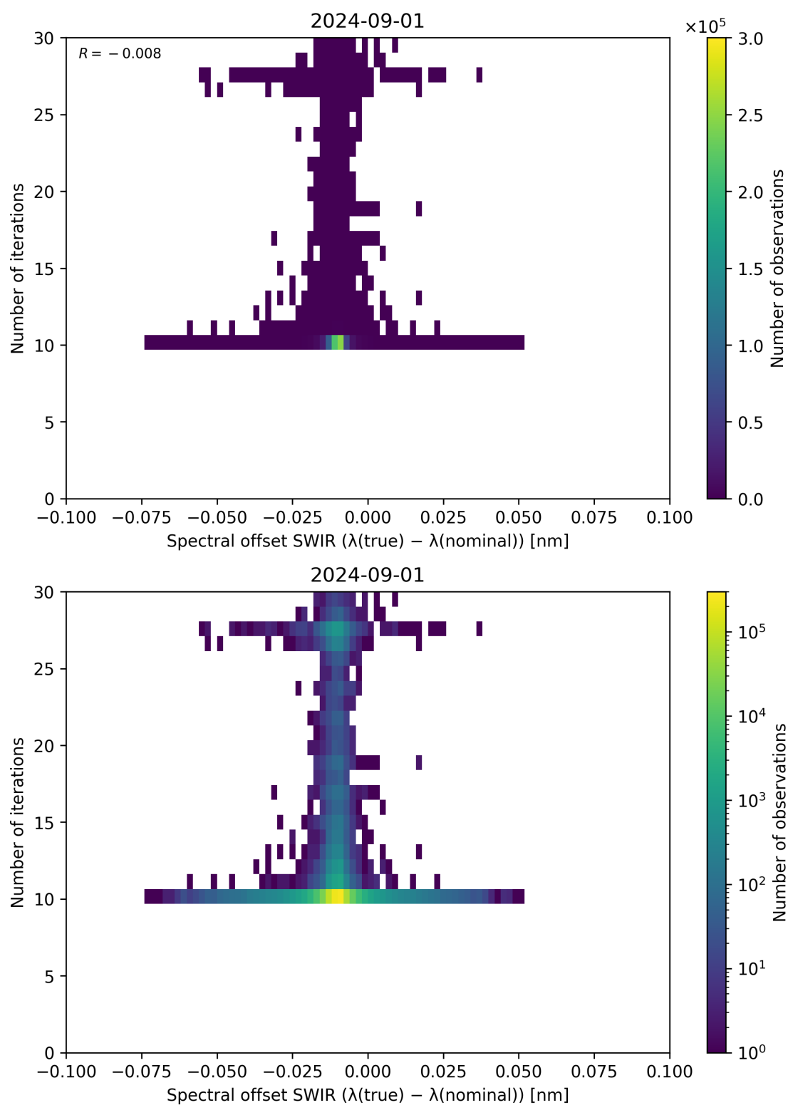
Figure 121: Scatter density plot of “Spectral offset SWIR ( \lambda_{\text{true}} - \lambda_{\text{nominal}} )” against “Number of iterations” for 2024-09-01 to 2024-09-02.
