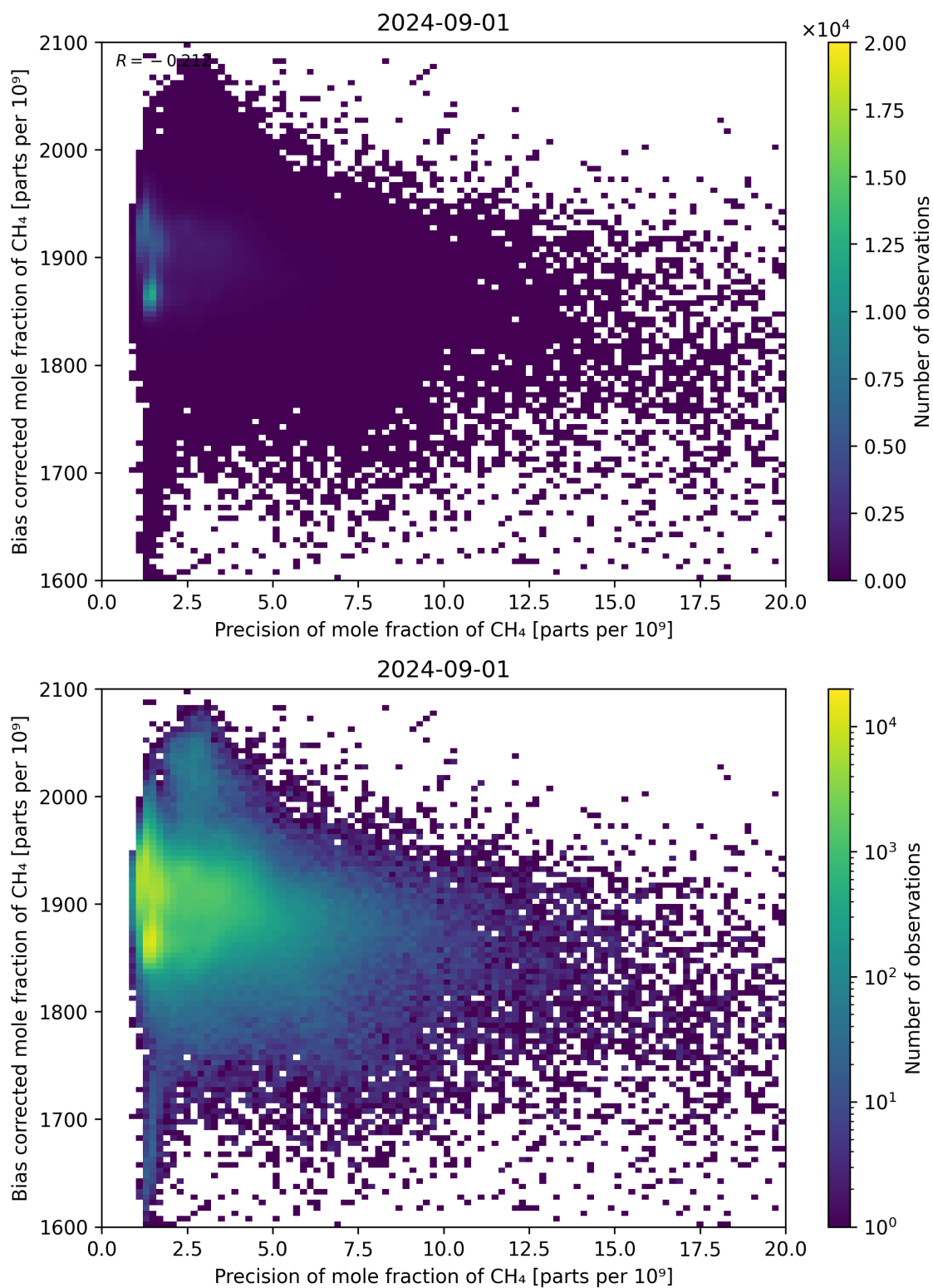
Figure 82: Scatter density plot of “Precision of mole fraction of CH 4 ” against “Bias corrected mole fraction of CH 4 ” for 2024-09-01 to 2024-09-02.
