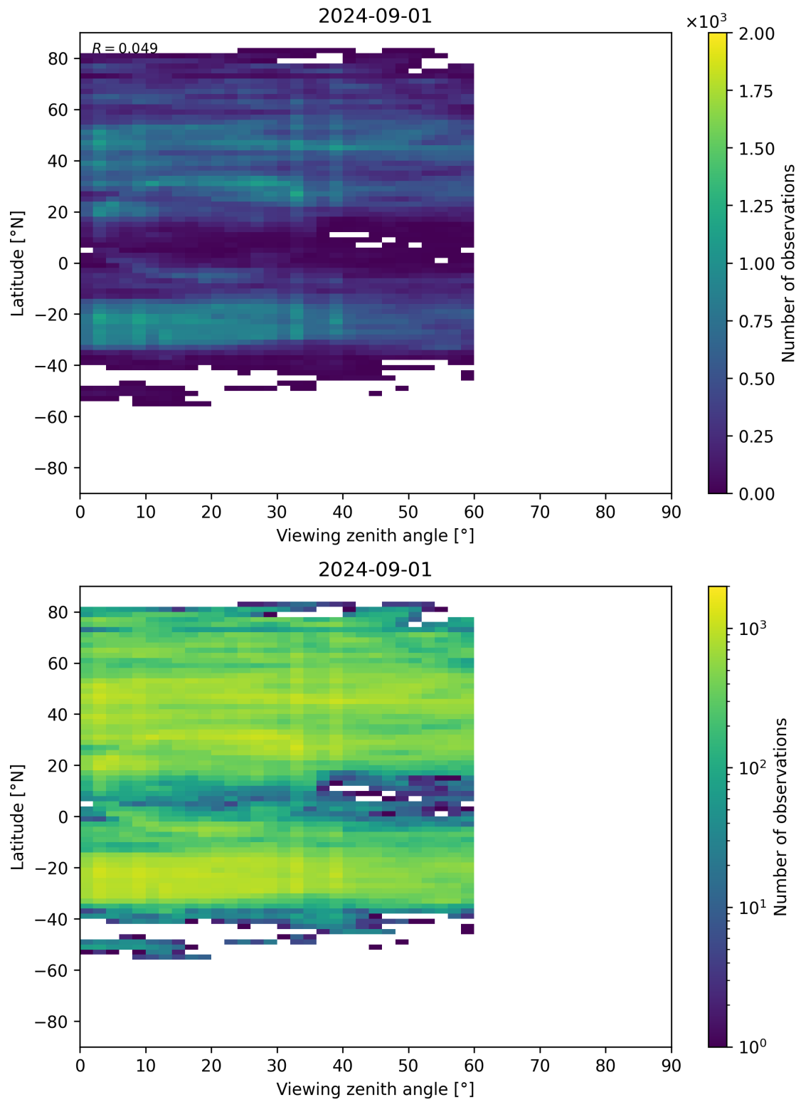
Figure 109: Scatter density plot of “Viewing zenith angle” against “Latitude” for 2024-09-01 to 2024-09-02.
