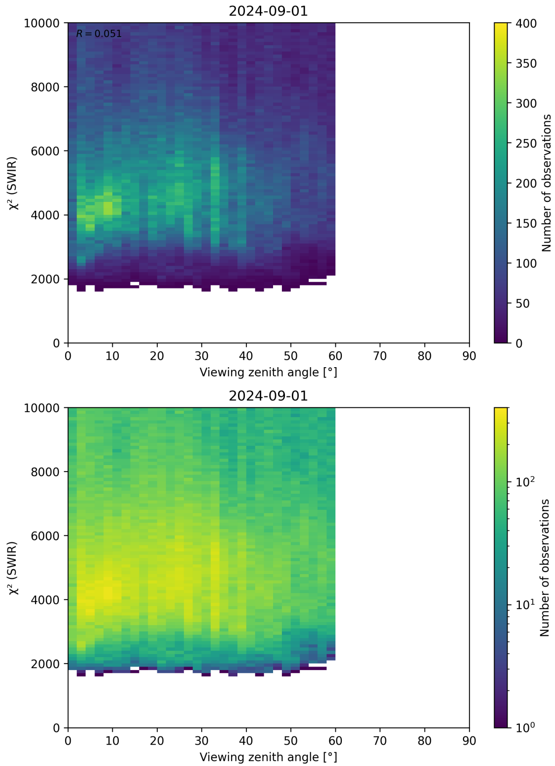
Figure 106: Scatter density plot of “Viewing zenith angle” against “ \chi^2 (SWIR)” for 2024-09-01 to 2024-09-02.
