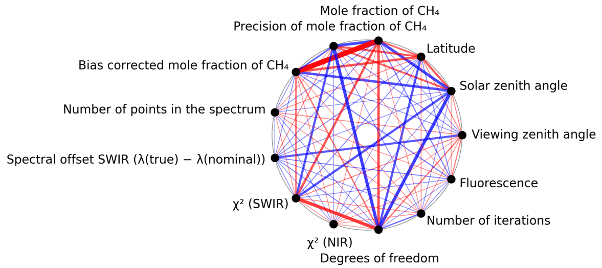
Figure 1: Map of correlation graph for 2024-09-01 to 2024-09-02.
