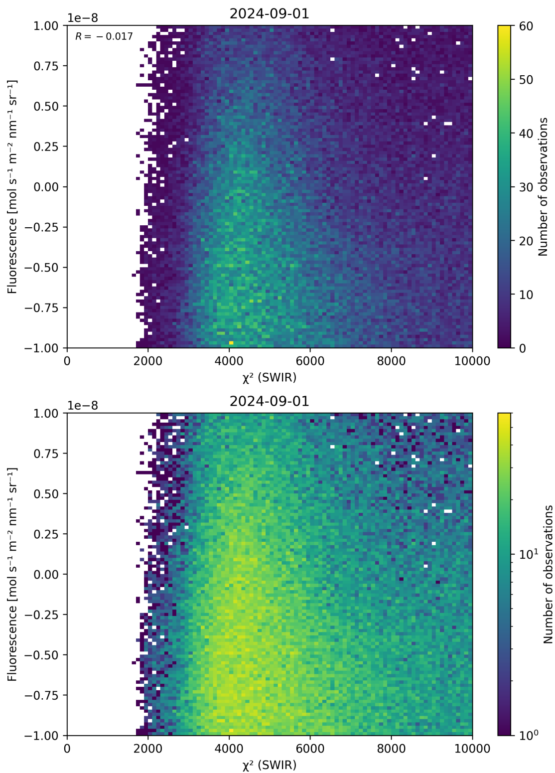
Figure 49: Scatter density plot of “ \chi^2 (SWIR)” against “Fluorescence” for 2024-09-01 to 2024-09-02.
