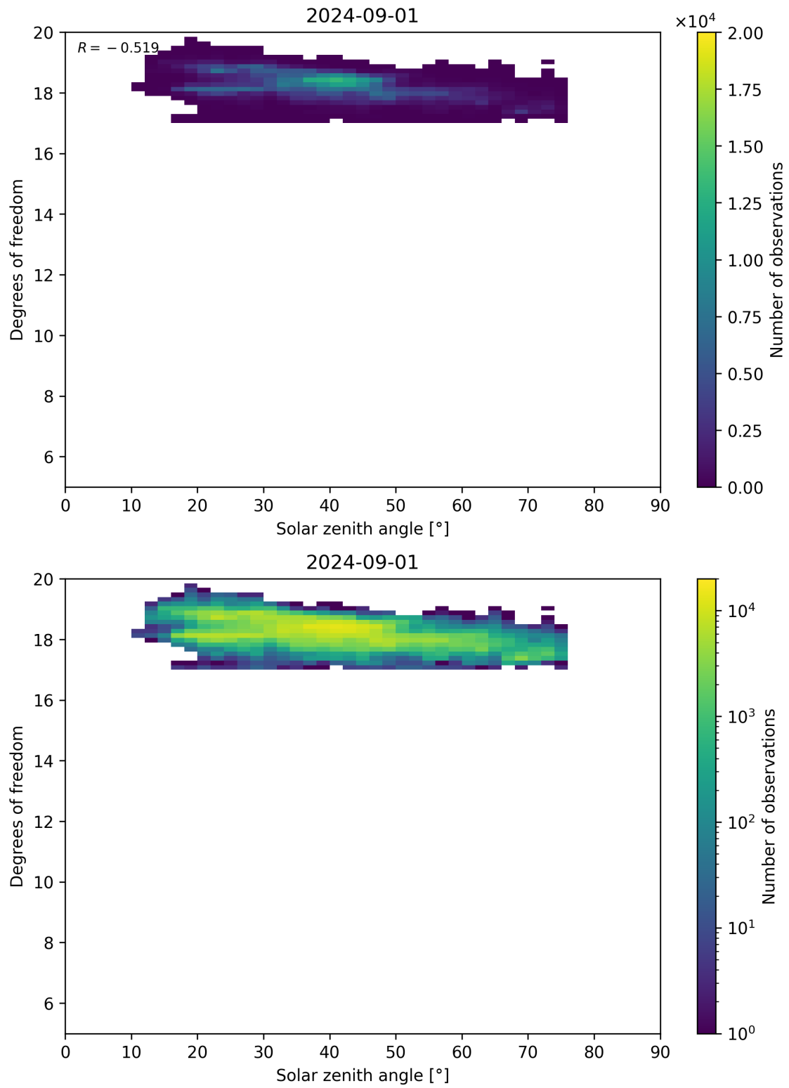
Figure 96: Scatter density plot of “Solar zenith angle” against “Degrees of freedom” for 2024-09-01 to 2024-09-02.
