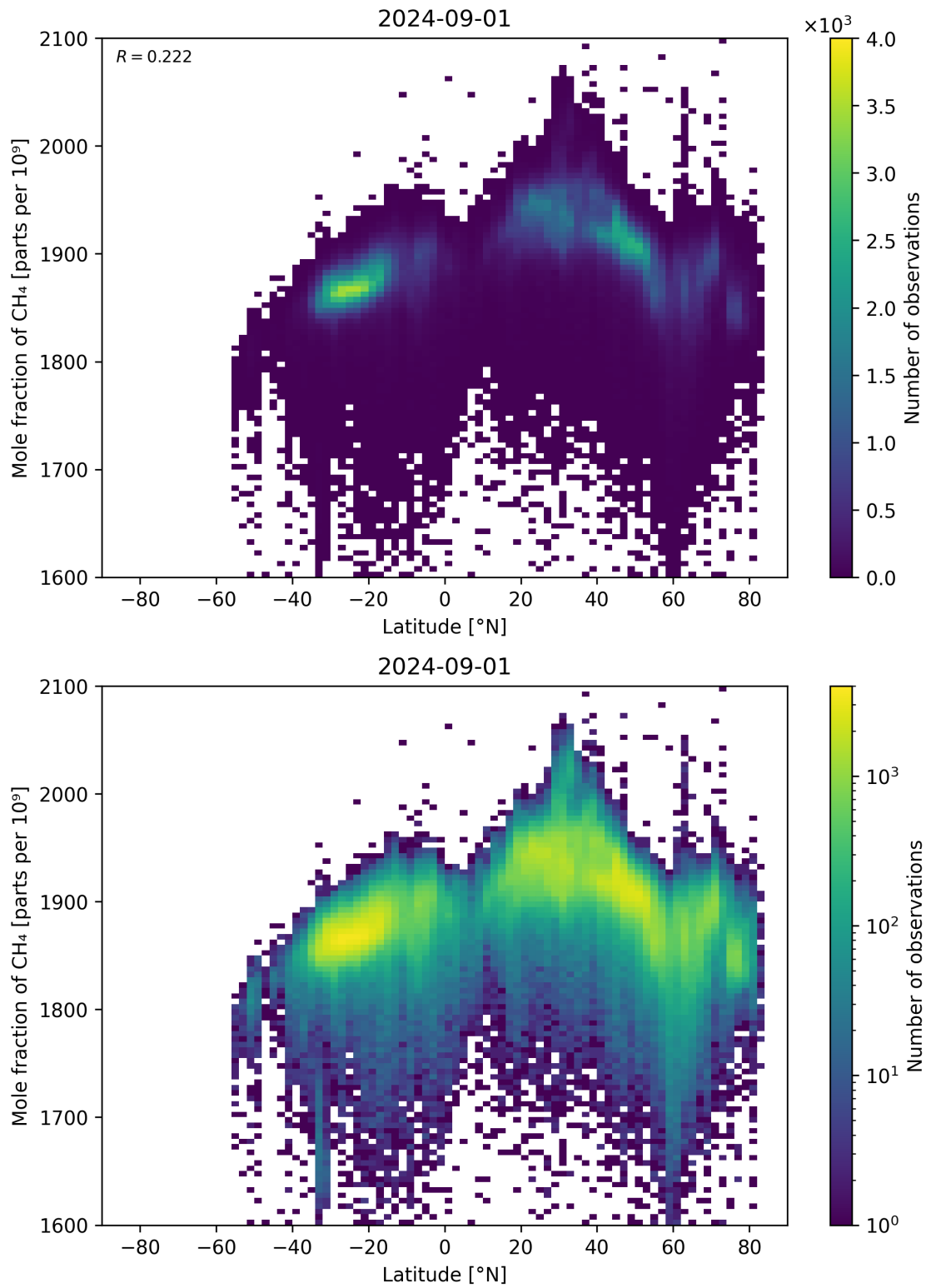
Figure 57: Scatter density plot of “Latitude” against “Mole fraction of \text{CH}_4 ” for 2024-09-01 to 2024-09-02.
