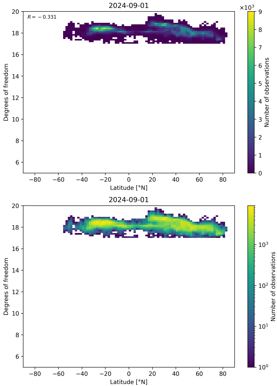
Figure 55: Scatter density plot of “Latitude” against “Degrees of freedom” for 2024-09-01 to 2024-09-02.
