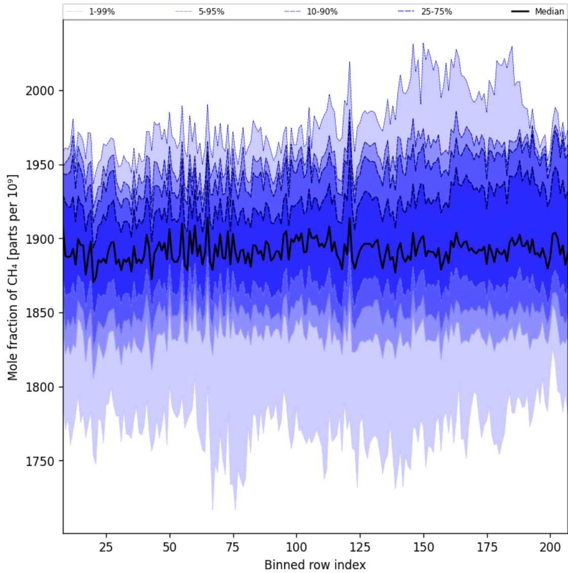
Figure 34: Along track statistics of “Mole fraction of CH 4 ” for 2024-09-01 to 2024-09-02
