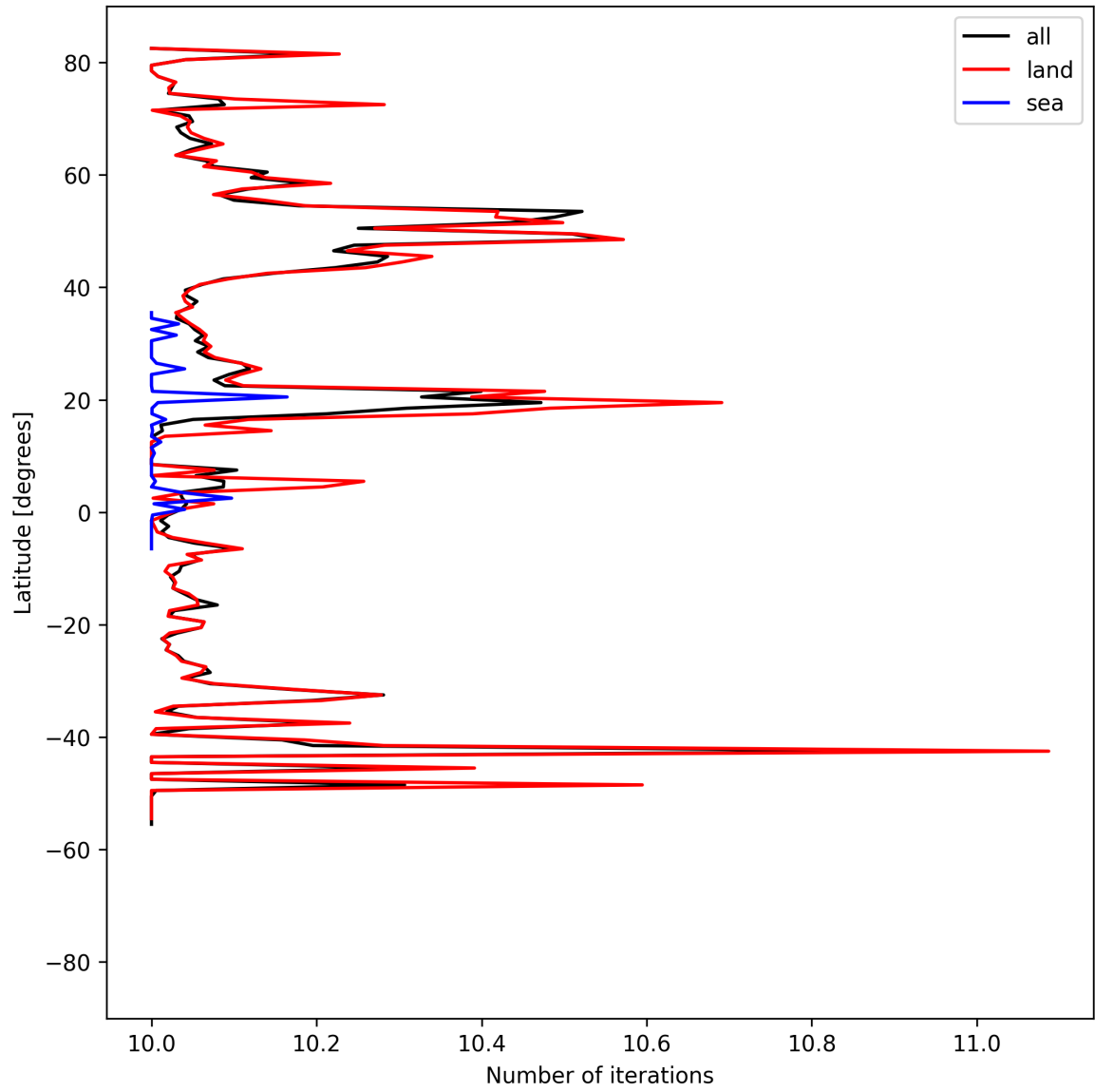
Figure 20: Zonal average of “Number of iterations” for 2024-09-01 to 2024-09-02.
