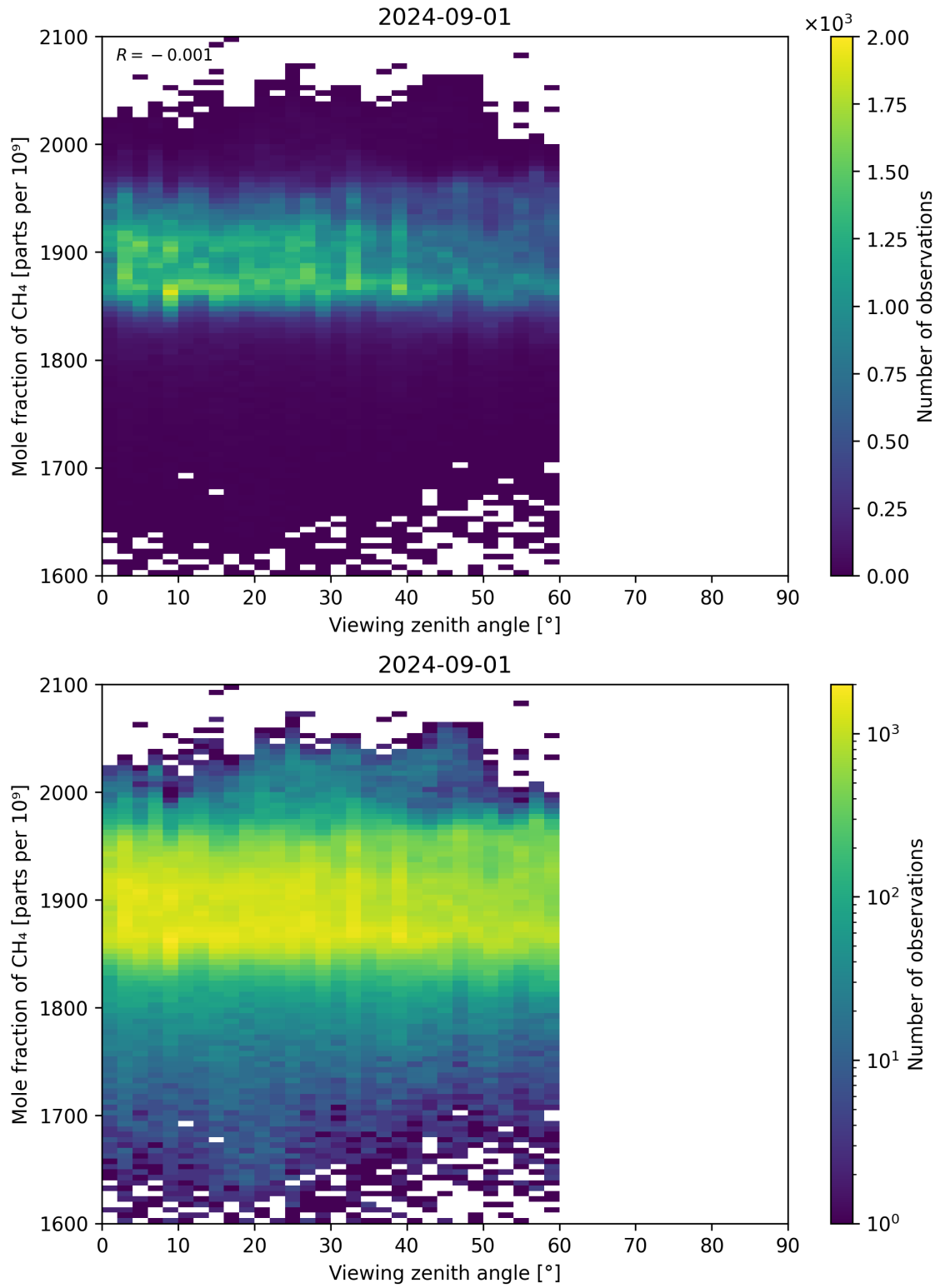
Figure 110: Scatter density plot of “Viewing zenith angle” against “Mole fraction of CH 4 ” for 2024-09-01 to 2024-09-02.
