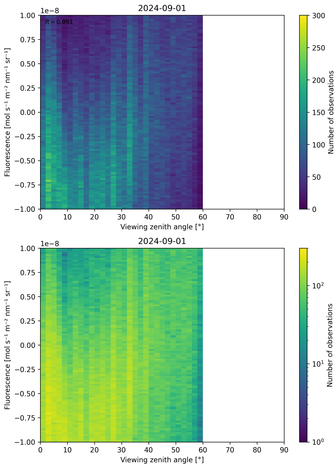
Figure 108: Scatter density plot of “Viewing zenith angle” against “Fluorescence” for 2024-09-01 to 2024-09-02.
