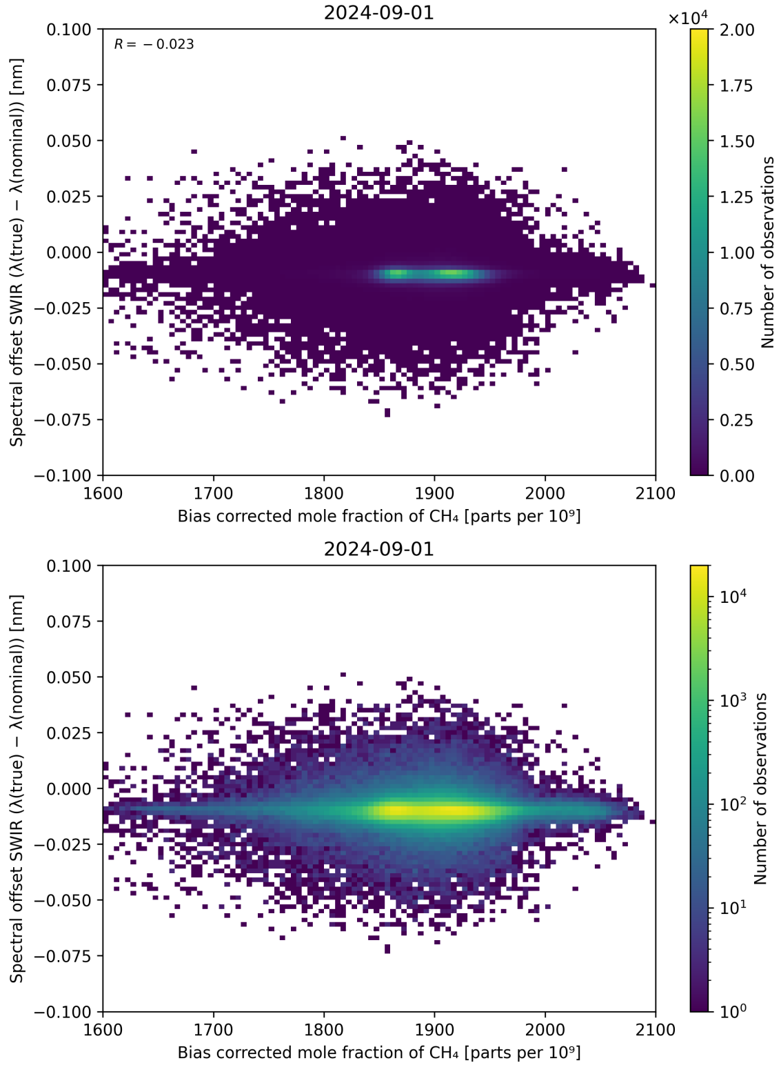
Figure 69: Scatter density plot of “Bias corrected mole fraction of \text{CH}_4 ” against “Spectral offset SWIR ( \lambda_{\text{true}} - \lambda_{\text{nominal}} )” for 2024-09-01 to 2024-09-02.
