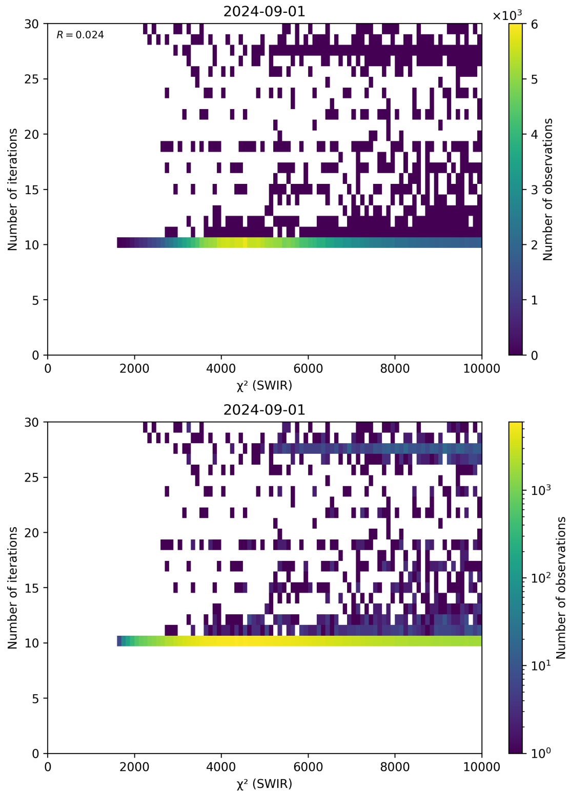
Figure 50: Scatter density plot of “ \chi^2 (SWIR)” against “Number of iterations” for 2024-09-01 to 2024-09-02.
