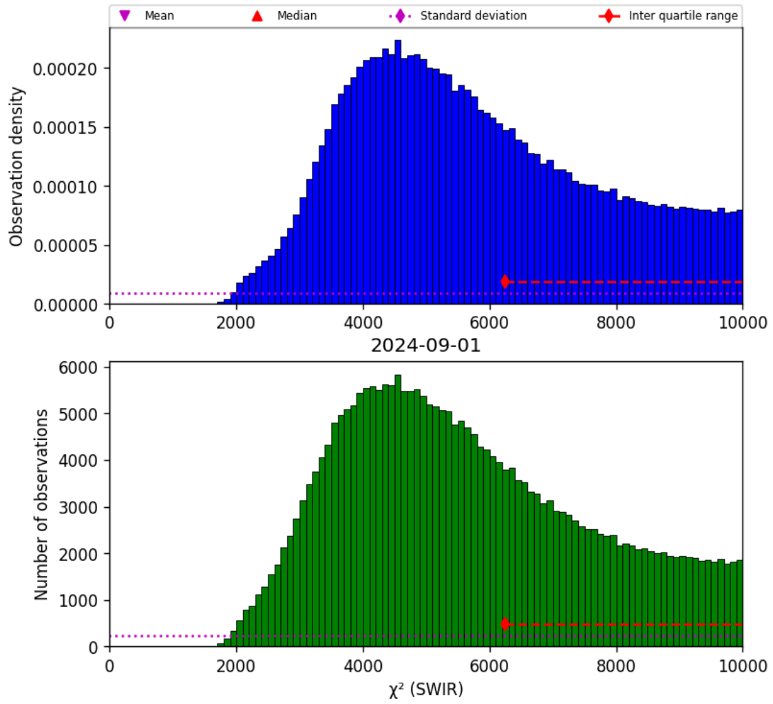
Figure 28: Histogram of " \chi^2 (SWIR)" for 2024-09-01 to 2024-09-02
