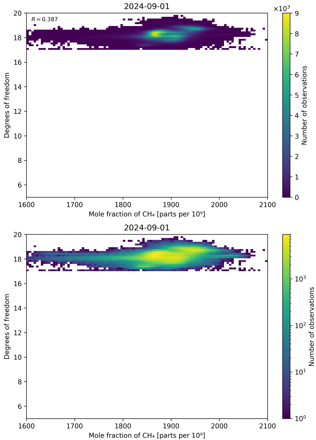
Figure 72: Scatter density plot of “Mole fraction of CH 4 ” against “Degrees of freedom” for 2024-09-01 to 2024-09-02.
