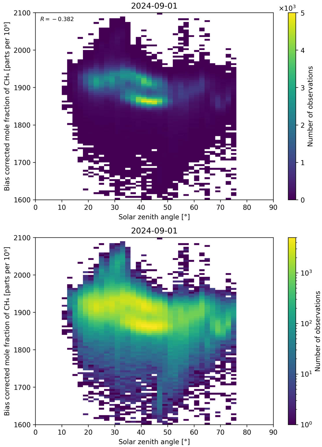
Figure 100: Scatter density plot of “Solar zenith angle” against “Bias corrected mole fraction of CH 4 ” for 2024-09-01 to 2024-09-02.
