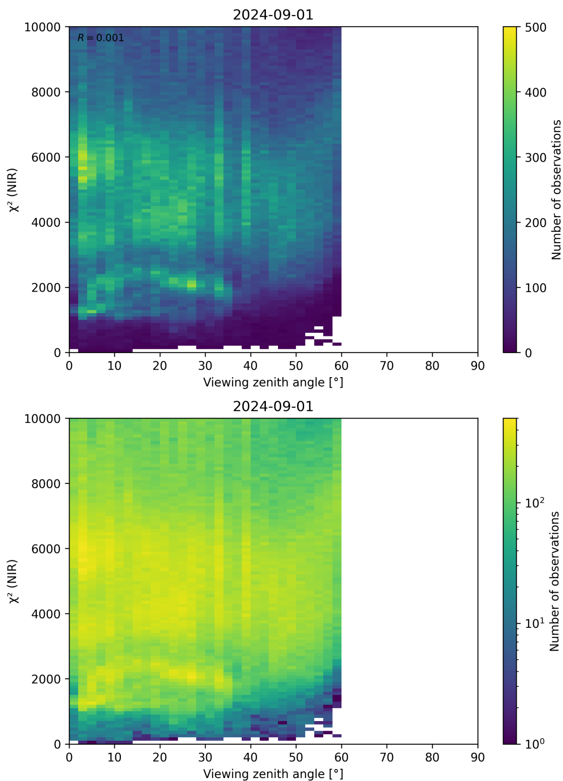
Figure 105: Scatter density plot of “Viewing zenith angle” against “ \chi^2 (NIR)” for 2024-09-01 to 2024-09-02.
