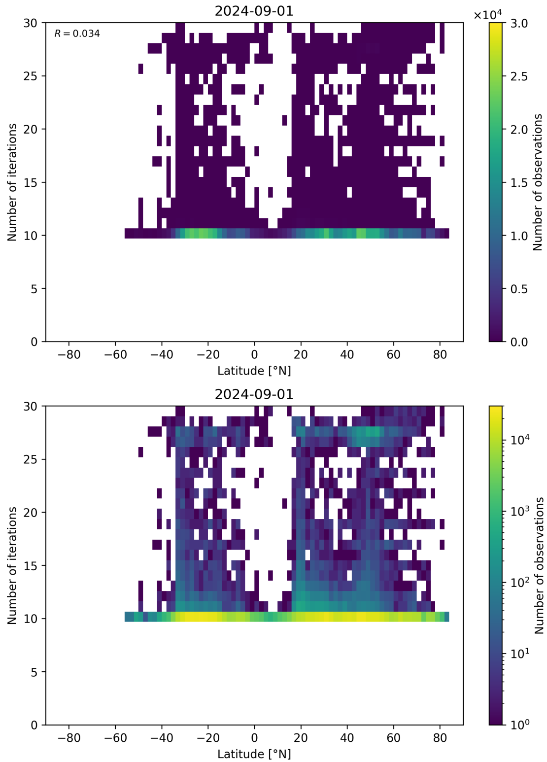
Figure 60: Scatter density plot of “Latitude” against “Number of iterations” for 2024-09-01 to 2024-09-02.
