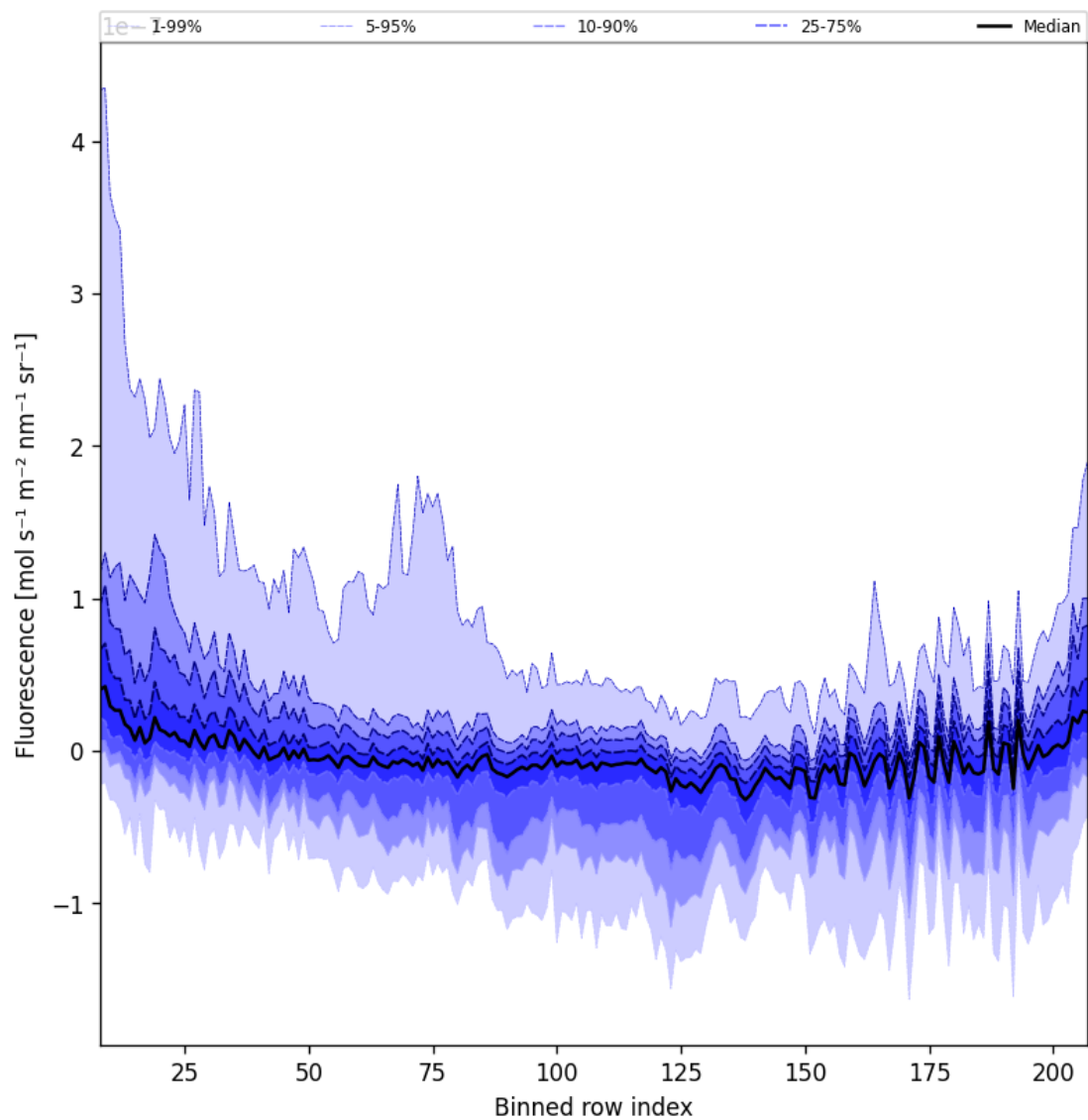
Figure 43: Along track statistics of “Fluorescence” for 2024-09-01 to 2024-09-02
