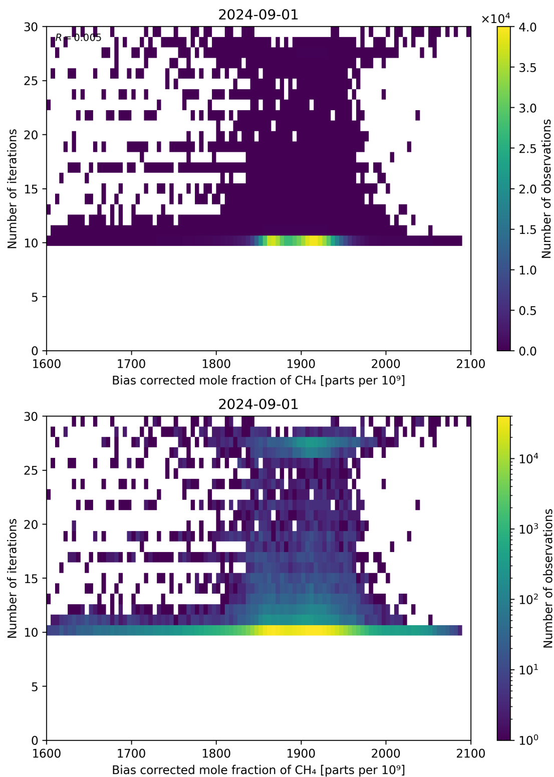
Figure 67: Scatter density plot of “Bias corrected mole fraction of CH 4 ” against “Number of iterations” for 2024-09-01 to 2024-09-02.
