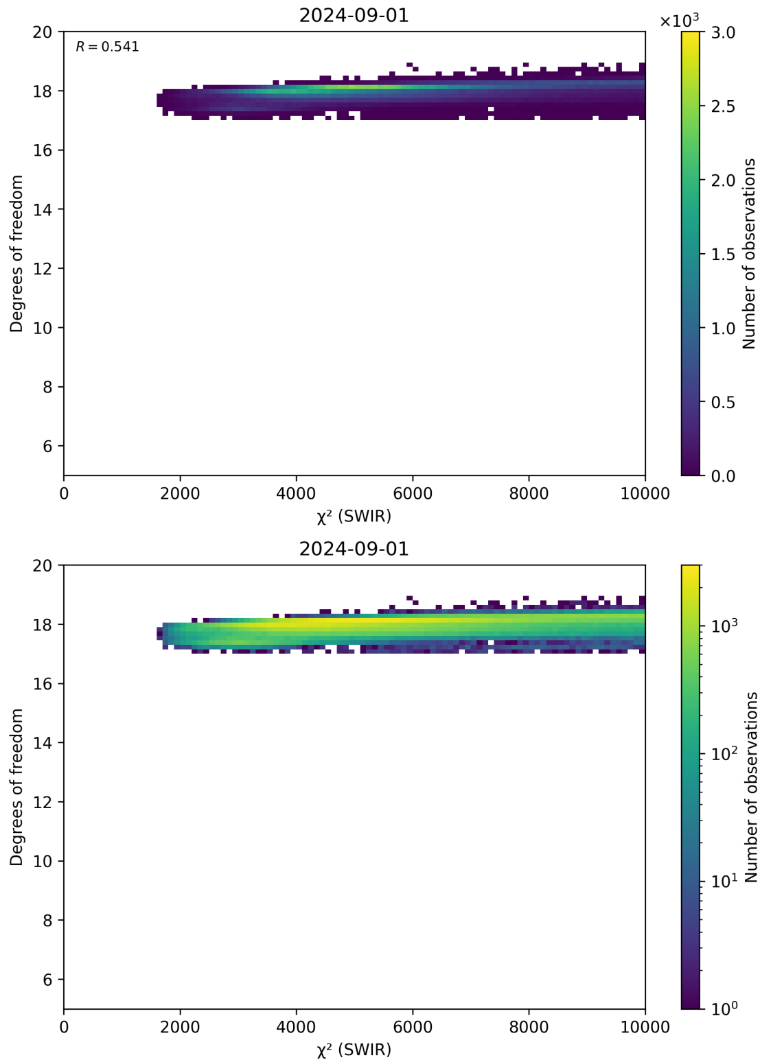
Figure 48: Scatter density plot of " \chi^2 (SWIR)" against "Degrees of freedom" for 2024-09-01 to 2024-09-02.
