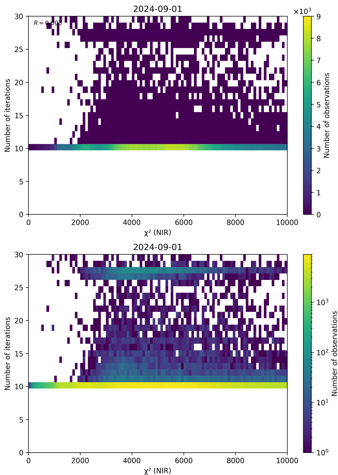
Figure 46: Scatter density plot of “ \chi^2 (NIR)” against “Number of iterations” for 2024-09-01 to 2024-09-02.
