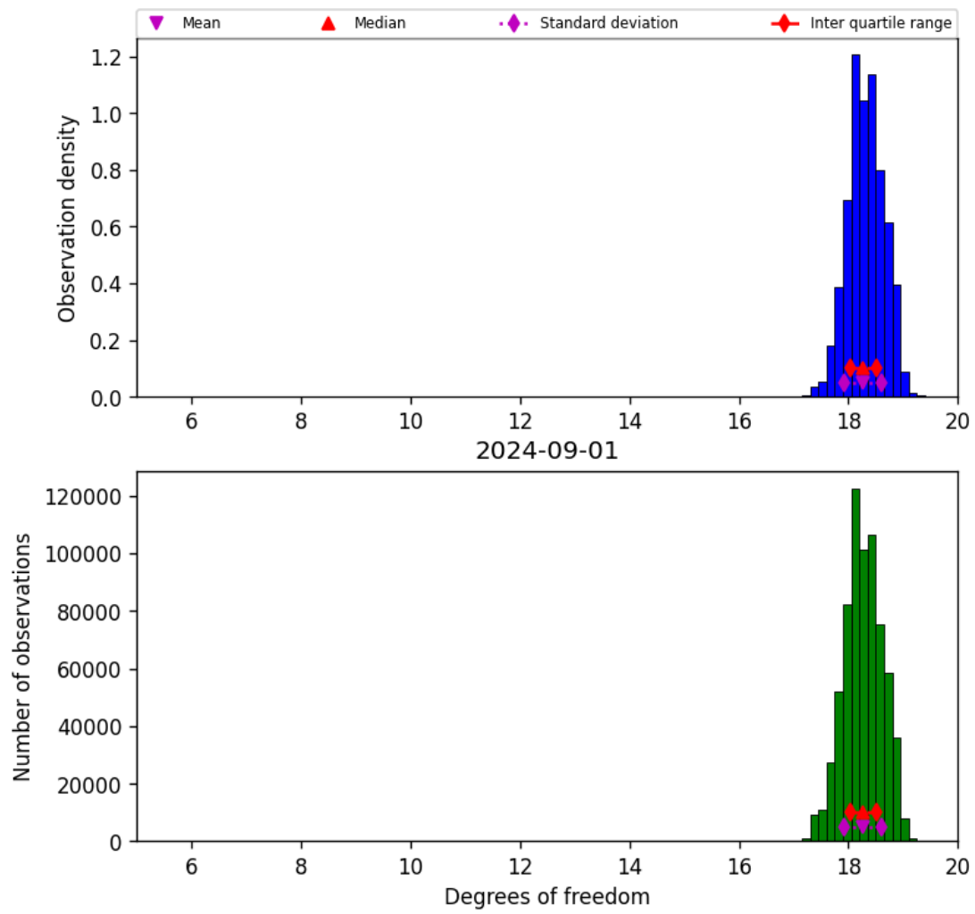
Figure 30: Histogram of “Degrees of freedom” for 2024-09-01 to 2024-09-02
