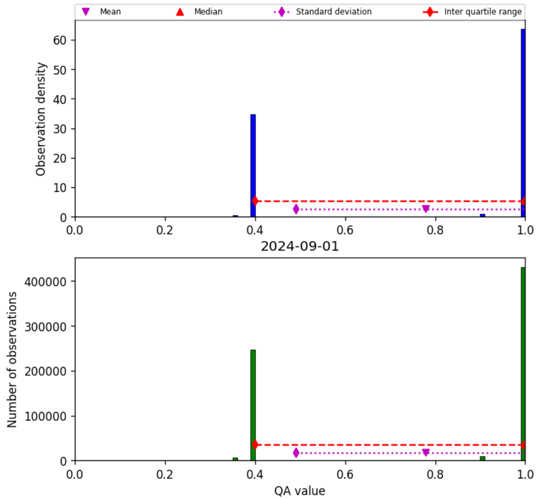
Figure 22: Histogram of “QA value” for 2024-09-01 to 2024-09-02
