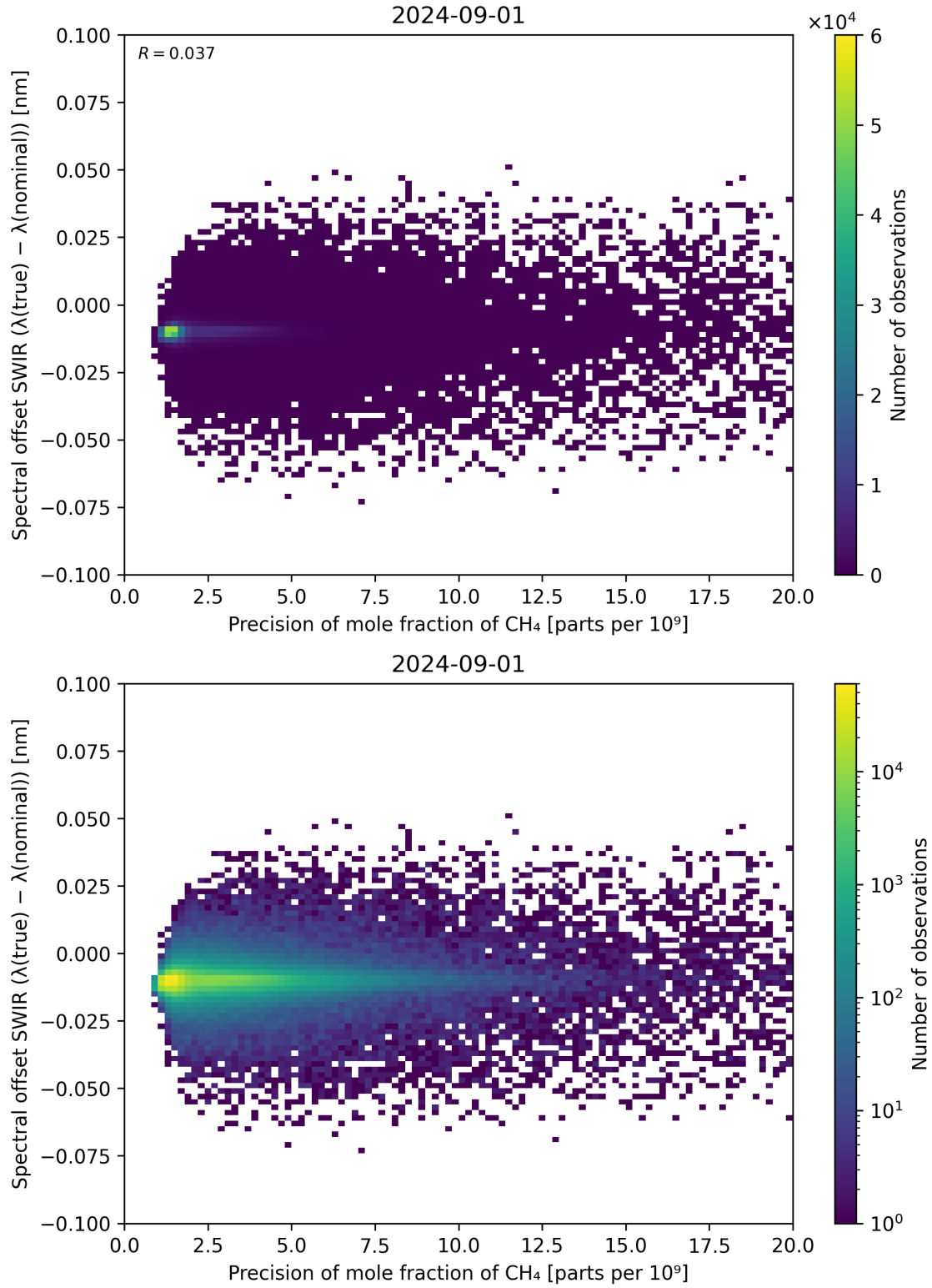
Figure 85: Scatter density plot of “Precision of mole fraction of \text{CH}_4 ” against “Spectral offset SWIR ( \lambda_{\text{true}} - \lambda_{\text{nominal}} )” for 2024-09-01 to 2024-09-02.
