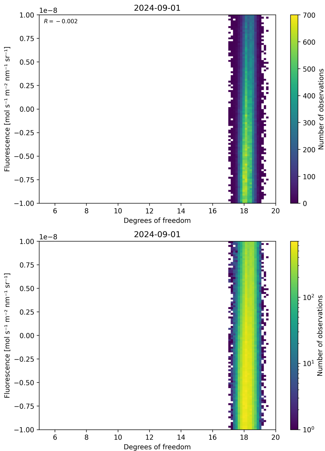
Figure 51: Scatter density plot of “Degrees of freedom” against “Fluorescence” for 2024-09-01 to 2024-09-02.
