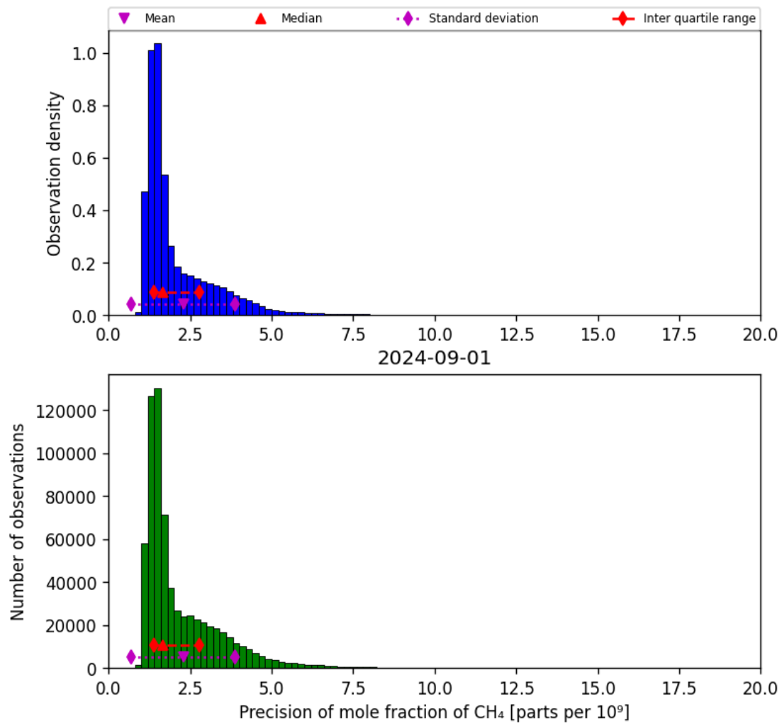
Figure 24: Histogram of “Precision of mole fraction of CH 4 ” for 2024-09-01 to 2024-09-02
