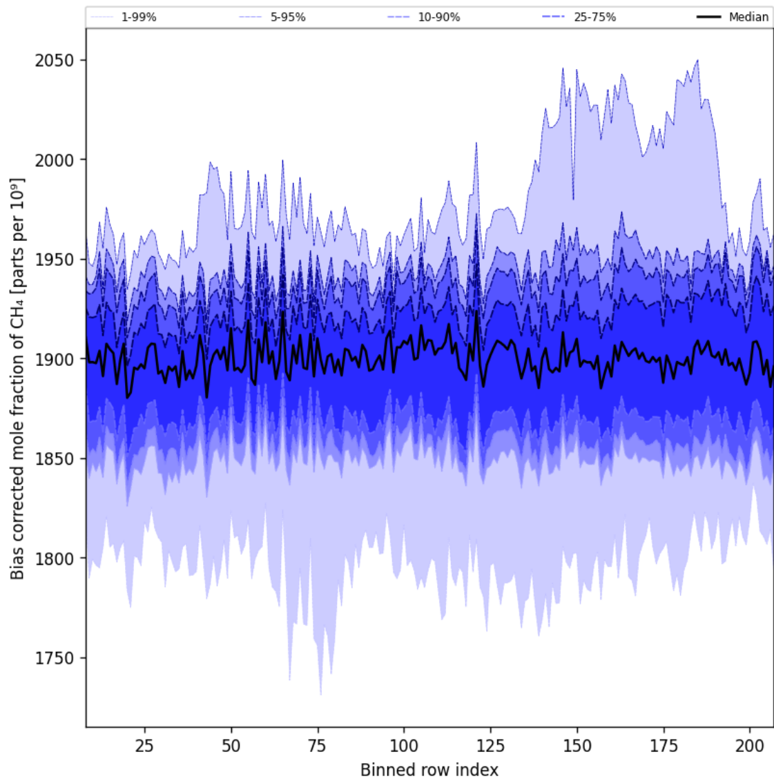
Figure 36: Along track statistics of “Bias corrected mole fraction of CH 4 ” for 2024-09-01 to 2024-09-02
