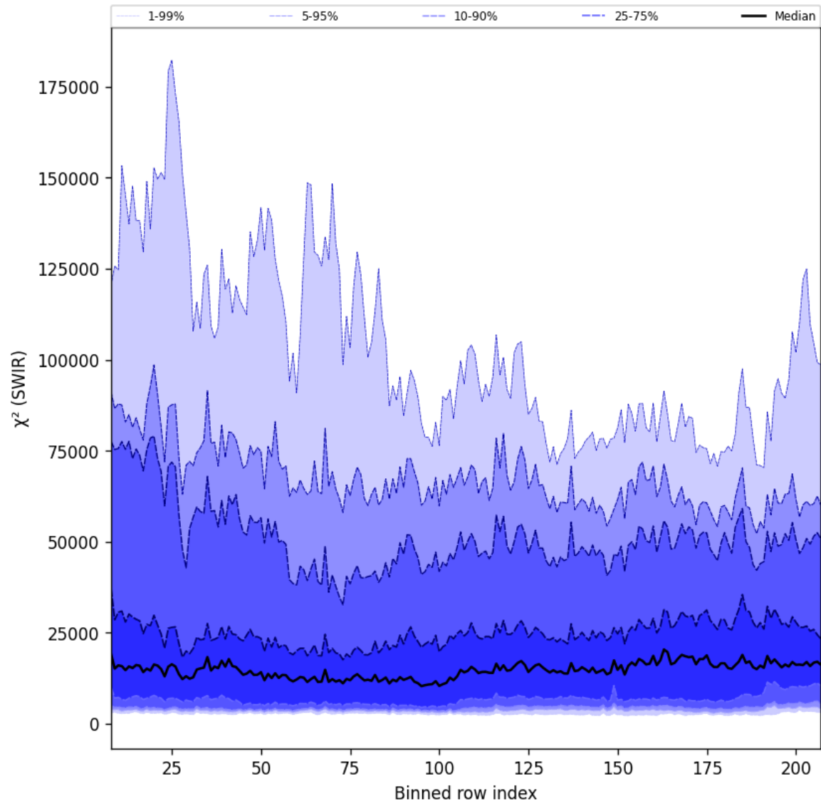
Figure 39: Along track statistics of “ \chi^2 (SWIR)” for 2024-09-01 to 2024-09-02
