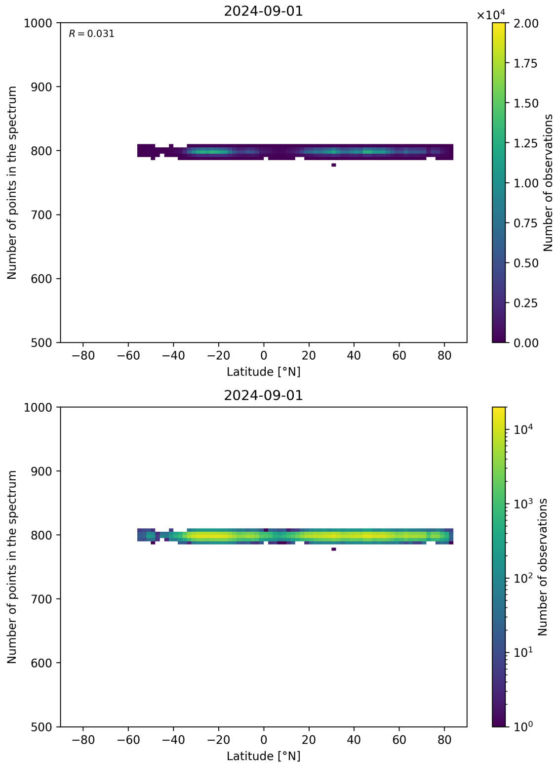
Figure 61: Scatter density plot of “Latitude” against “Number of points in the spectrum” for 2024-09-01 to 2024-09-02.
