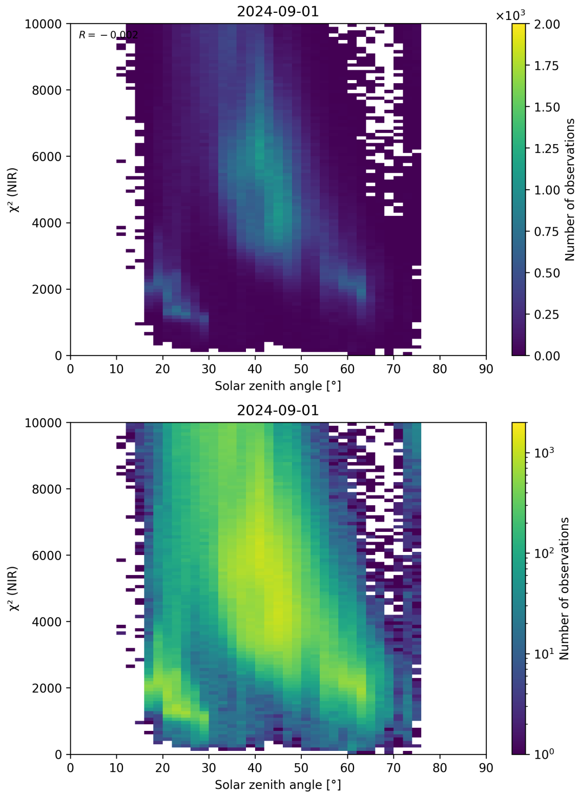
Figure 94: Scatter density plot of “Solar zenith angle” against “ \chi^2 (NIR)” for 2024-09-01 to 2024-09-02.
