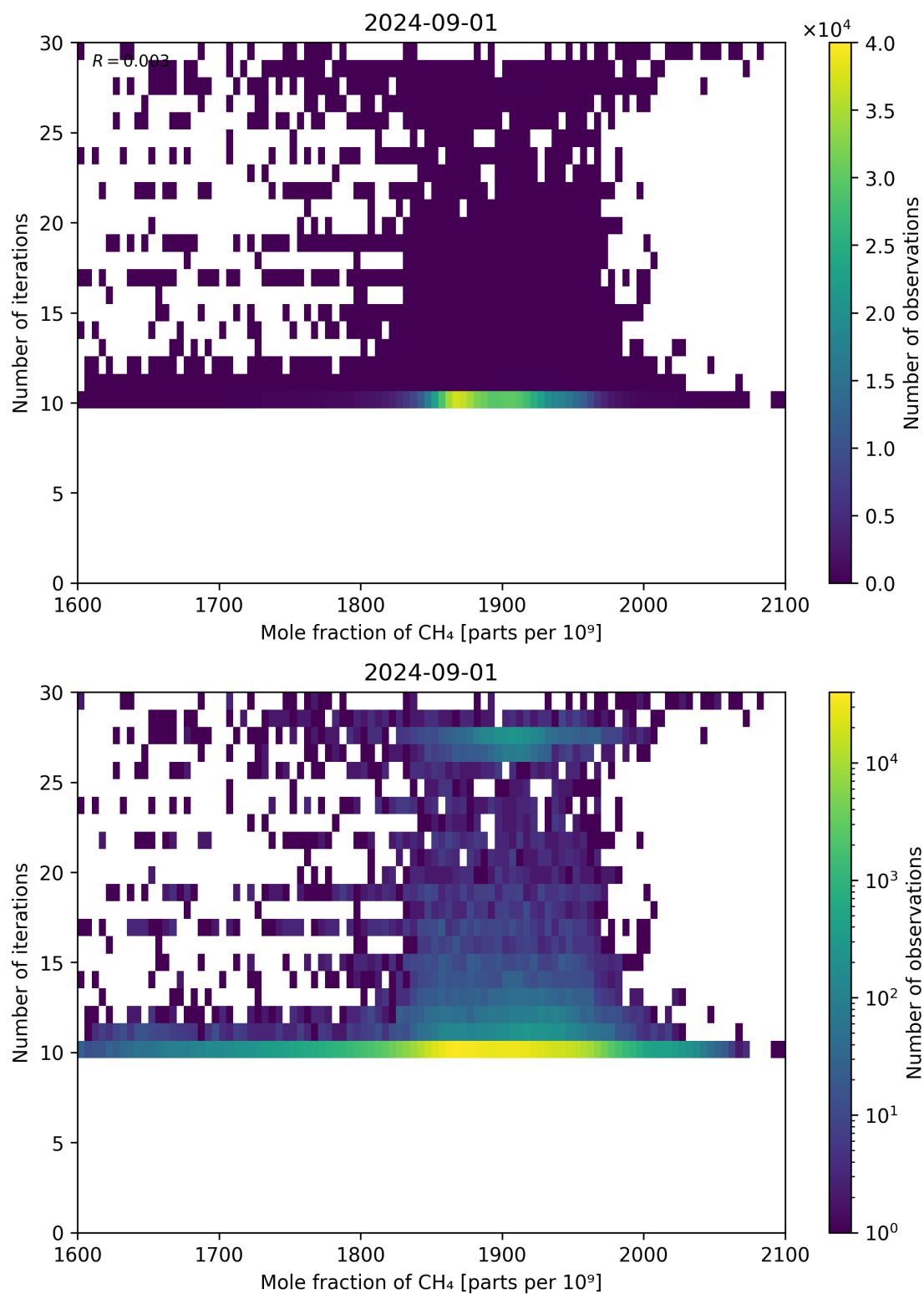
Figure 76: Scatter density plot of “Mole fraction of CH 4 ” against “Number of iterations” for 2024-09-01 to 2024-09-02.
