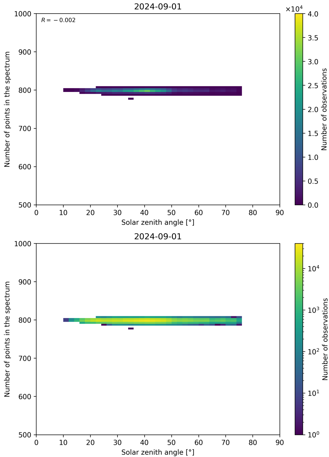
Figure 103: Scatter density plot of “Solar zenith angle” against “Number of points in the spectrum” for 2024-09-01 to 2024-09-02.
