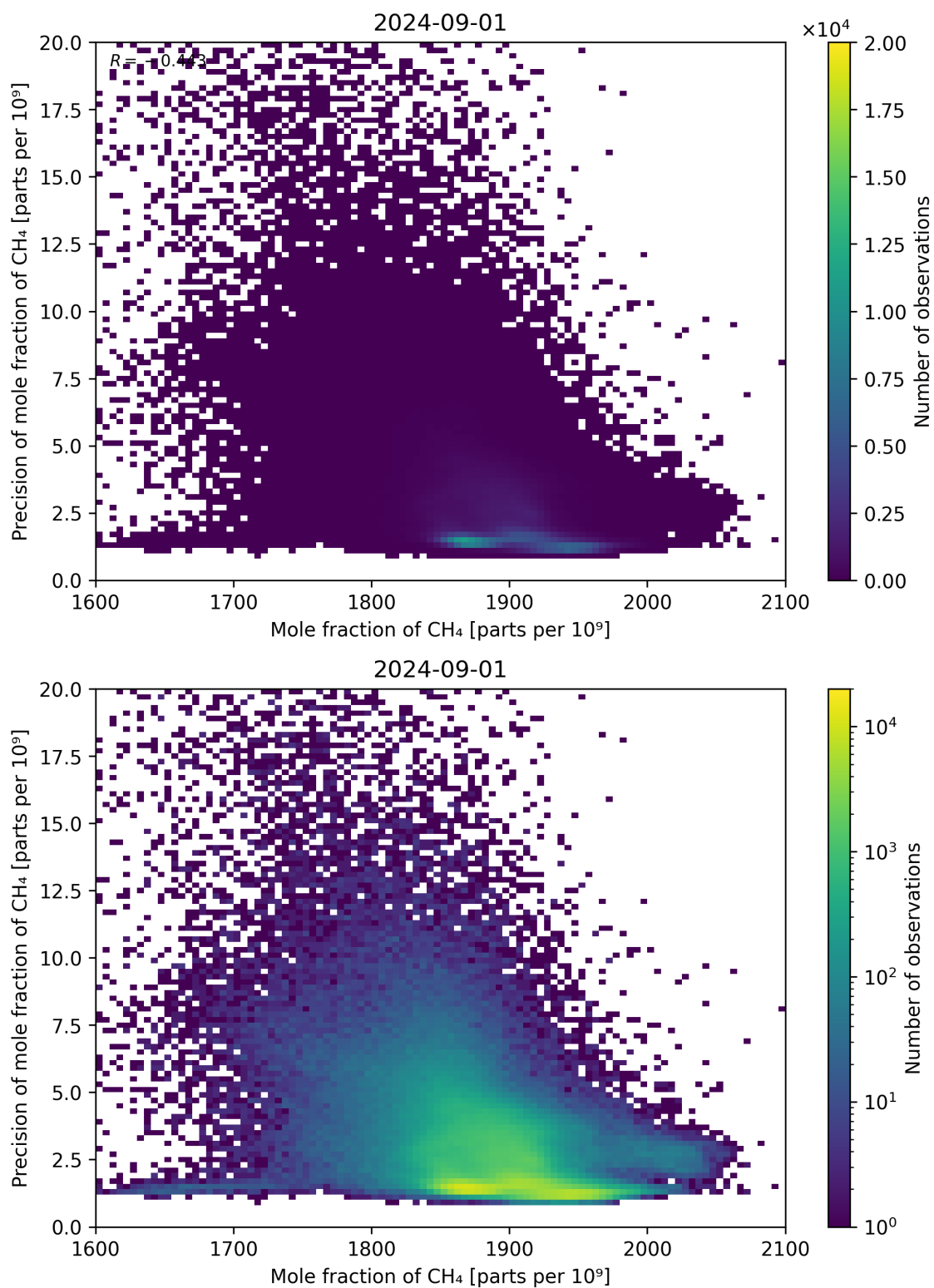
Figure 75: Scatter density plot of “Mole fraction of CH 4 ” against “Precision of mole fraction of CH 4 ” for 2024-09-01 to 2024-09-02.
