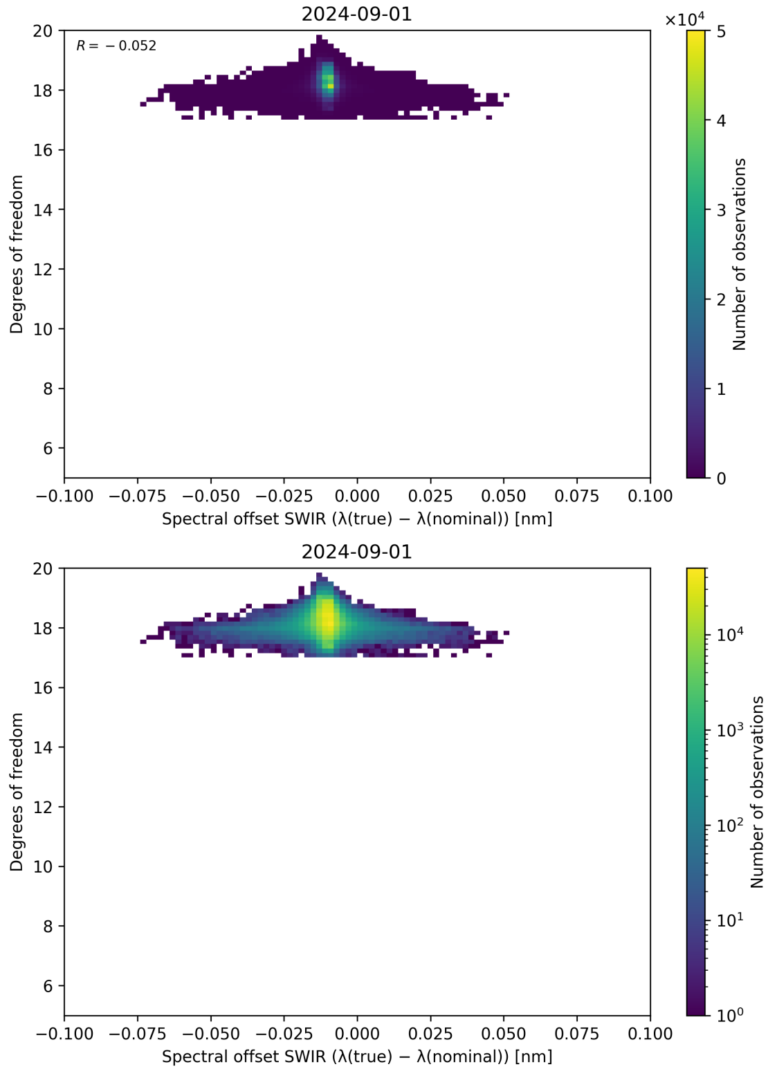
Figure 119: Scatter density plot of “Spectral offset SWIR ( \lambda_{\text{true}} - \lambda_{\text{nominal}} )” against “Degrees of freedom” for 2024-09-01 to 2024-09-02.
