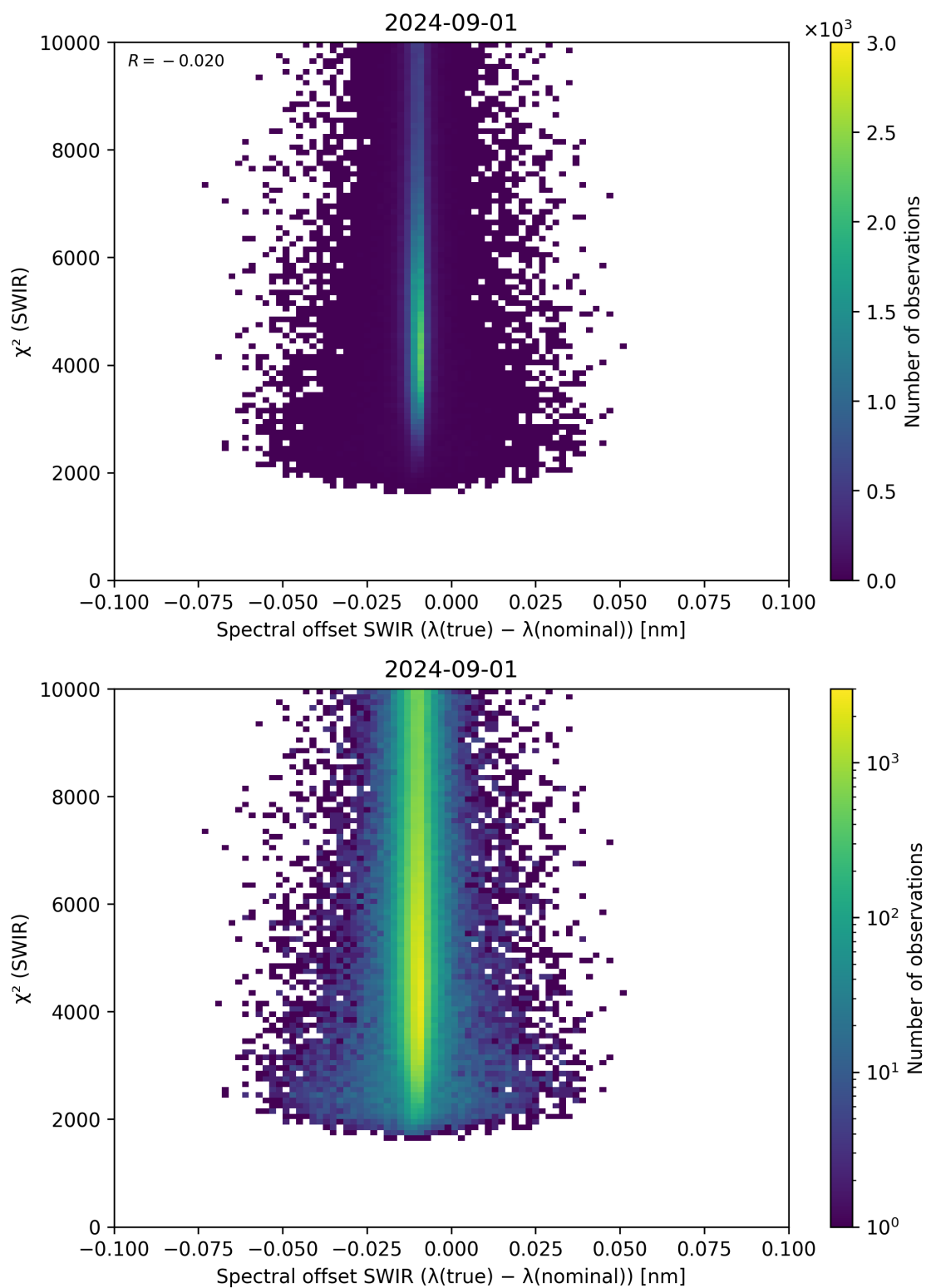
Figure 118: Scatter density plot of “Spectral offset SWIR ( \lambda_{\text{true}} - \lambda_{\text{nominal}} )” against “ \chi^2 (SWIR)” for 2024-09-01 to 2024-09-02.
