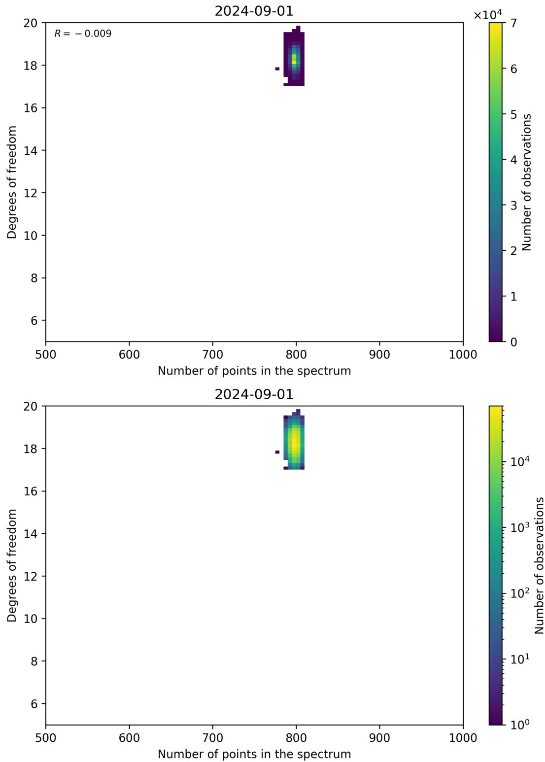
Figure 90: Scatter density plot of “Number of points in the spectrum” against “Degrees of freedom” for 2024-09-01 to 2024-09-02.
