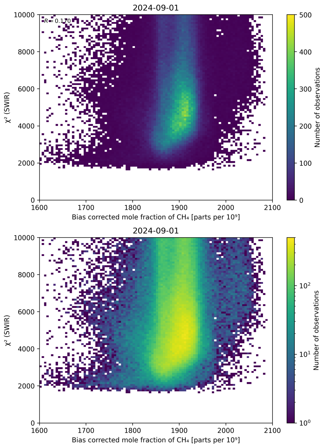
Figure 64: Scatter density plot of “Bias corrected mole fraction of \text{CH}_4 ” against “ \chi^2 (SWIR)” for 2024-09-01 to 2024-09-02.
