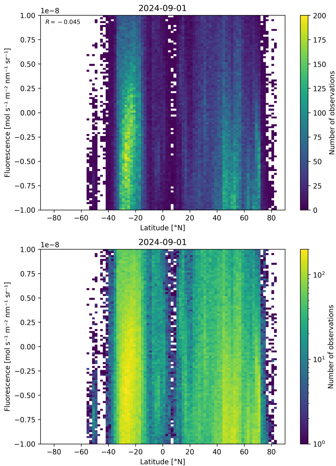
Figure 56: Scatter density plot of “Latitude” against “Fluorescence” for 2024-09-01 to 2024-09-02.
