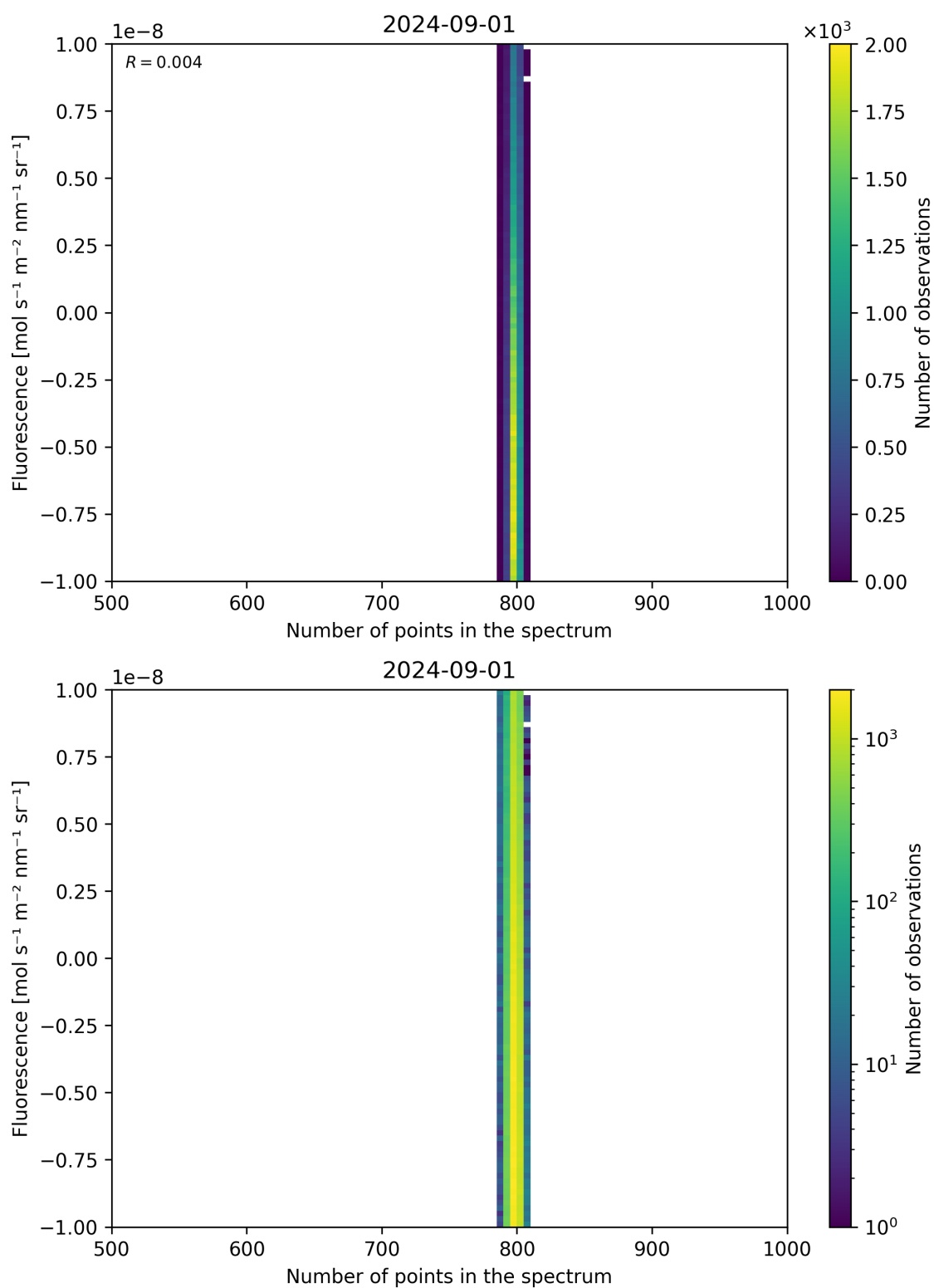
Figure 91: Scatter density plot of “Number of points in the spectrum” against “Fluorescence” for 2024-09-01 to 2024-09-02.
