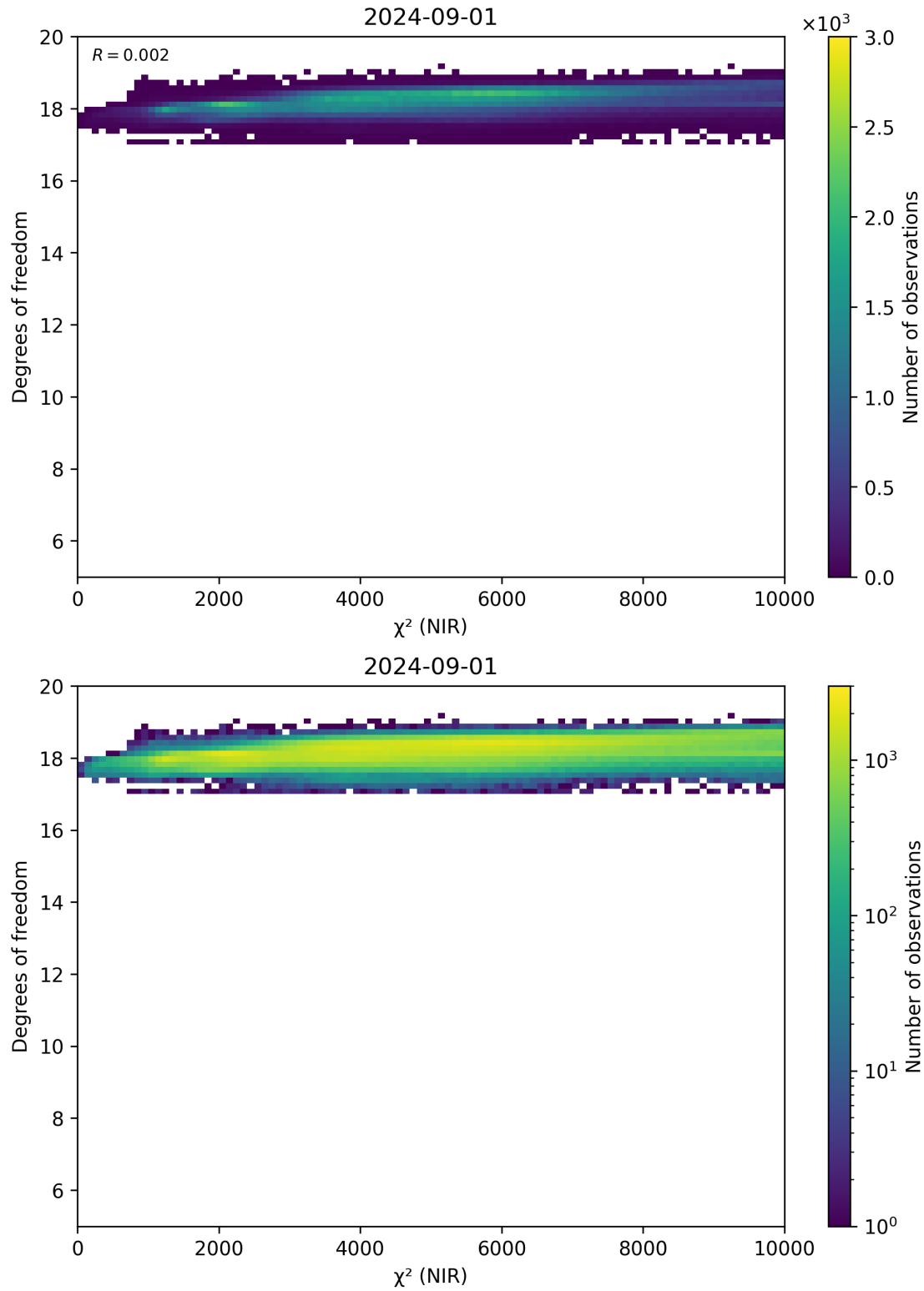
Figure 44: Scatter density plot of “ \chi^2 (NIR)” against “Degrees of freedom” for 2024-09-01 to 2024-09-02.
