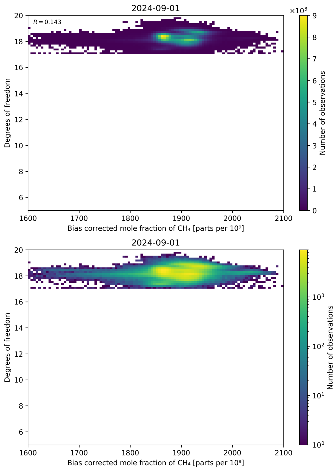
Figure 65: Scatter density plot of “Bias corrected mole fraction of CH 4 ” against “Degrees of freedom” for 2024-09-01 to 2024-09-02.
