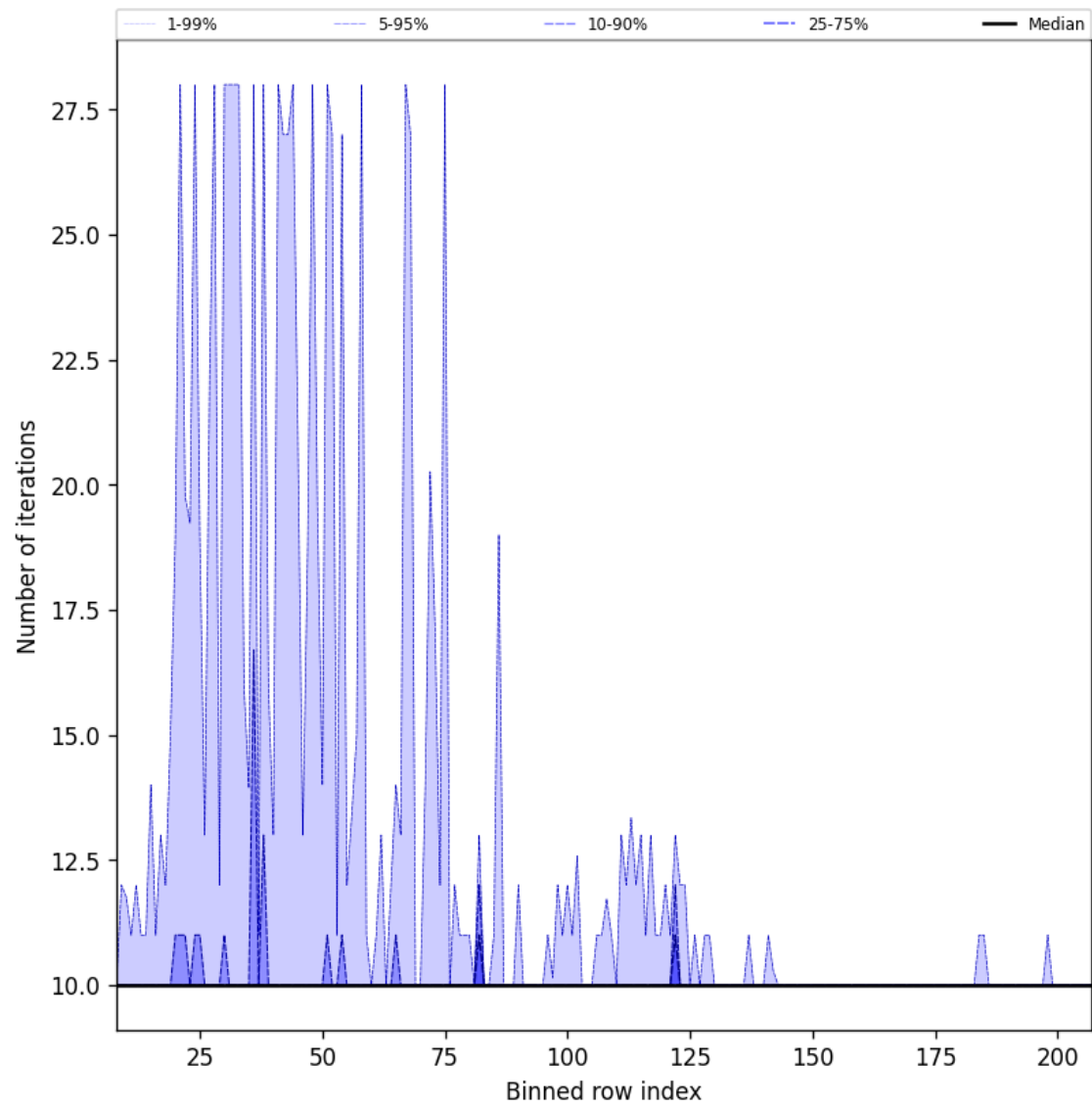
Figure 42: Along track statistics of “Number of iterations” for 2024-09-01 to 2024-09-02
