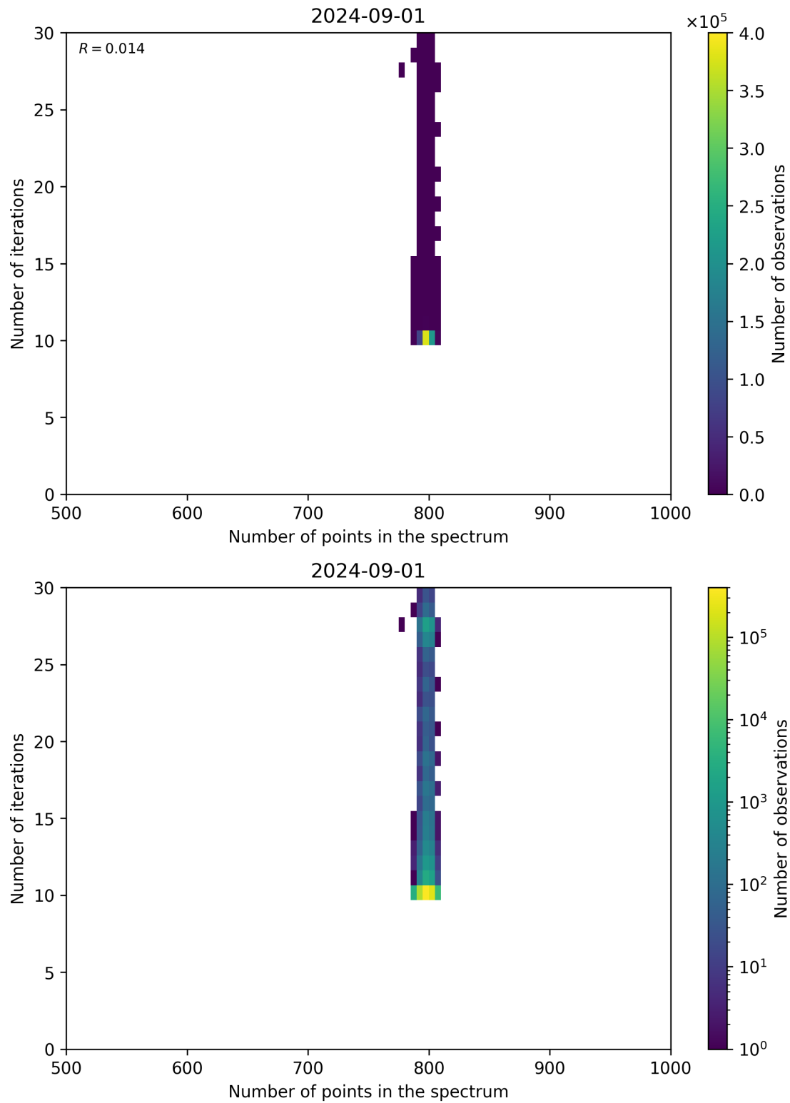
Figure 92: Scatter density plot of “Number of points in the spectrum” against “Number of iterations” for 2024-09-01 to 2024-09-02.
