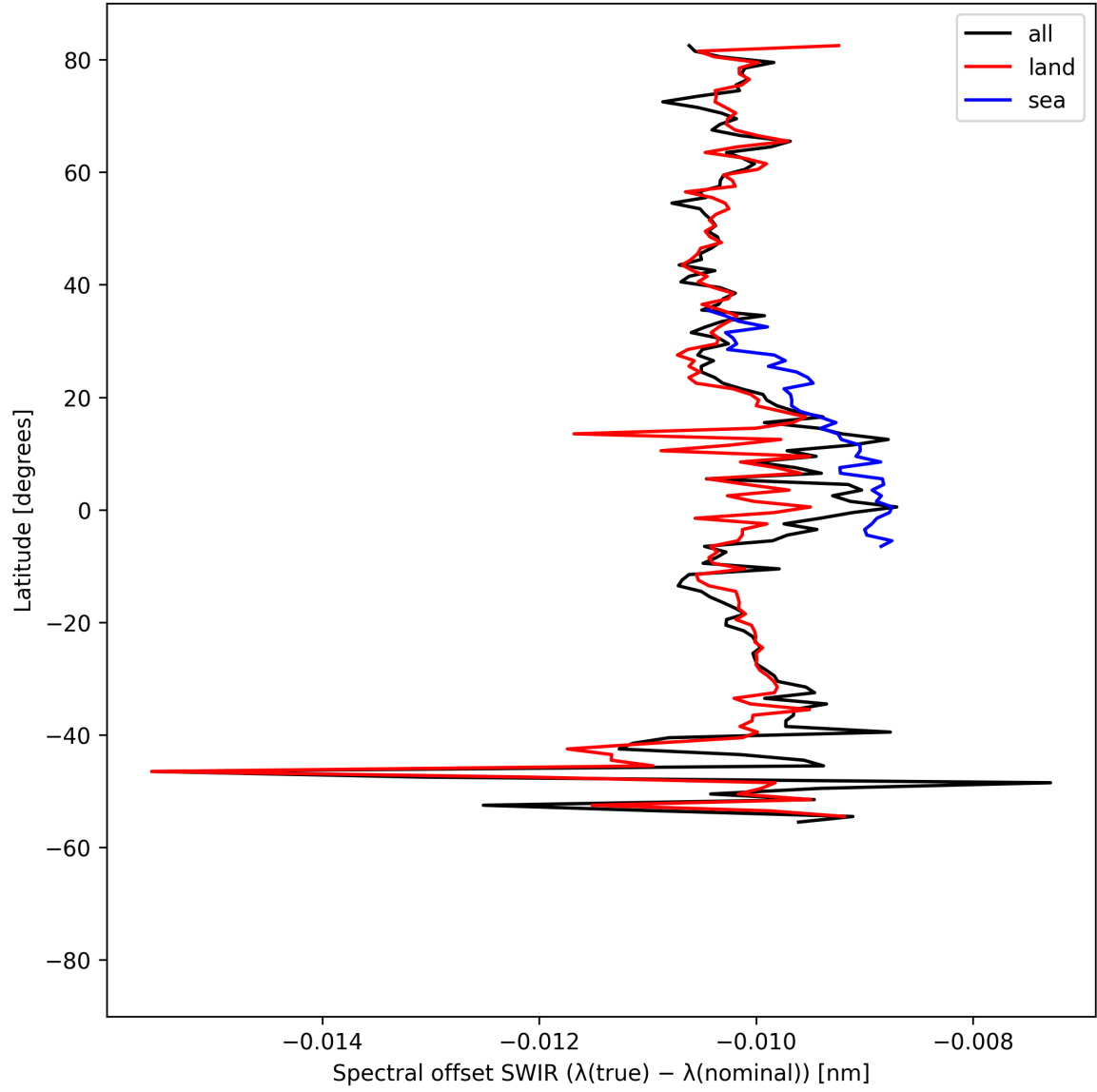
Figure 16: Zonal average of “Spectral offset SWIR ( \lambda_{\text{true}} - \lambda_{\text{nominal}} )” for 2024-09-01 to 2024-09-02.
