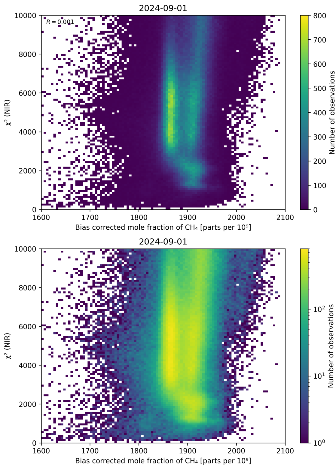
Figure 63: Scatter density plot of “Bias corrected mole fraction of CH 4 ” against “ \chi^2 (NIR)” for 2024-09-01 to 2024-09-02.
