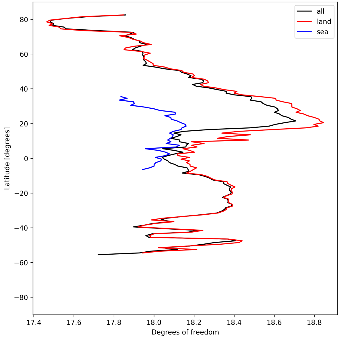
Figure 19: Zonal average of “Degrees of freedom” for 2024-09-01 to 2024-09-02.
