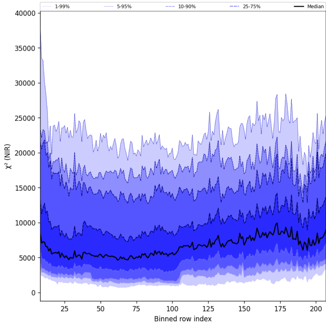
Figure 40: Along track statistics of “ \chi^2 (NIR)” for 2024-09-01 to 2024-09-02
