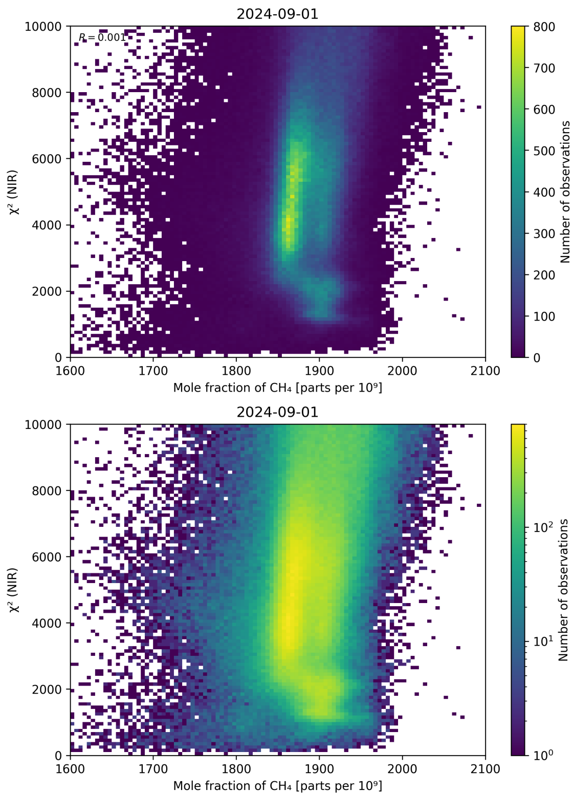
Figure 70: Scatter density plot of “Mole fraction of \text{CH}_4 ” against “ \chi^2 (NIR)” for 2024-09-01 to 2024-09-02.
