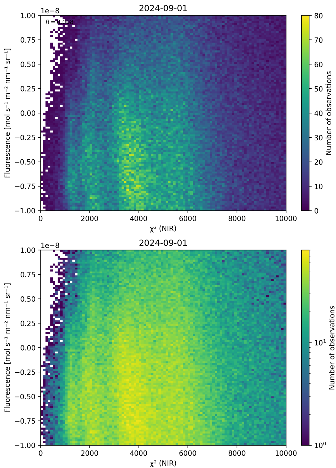
Figure 45: Scatter density plot of “ \chi^2 (NIR)” against “Fluorescence” for 2024-09-01 to 2024-09-02.
