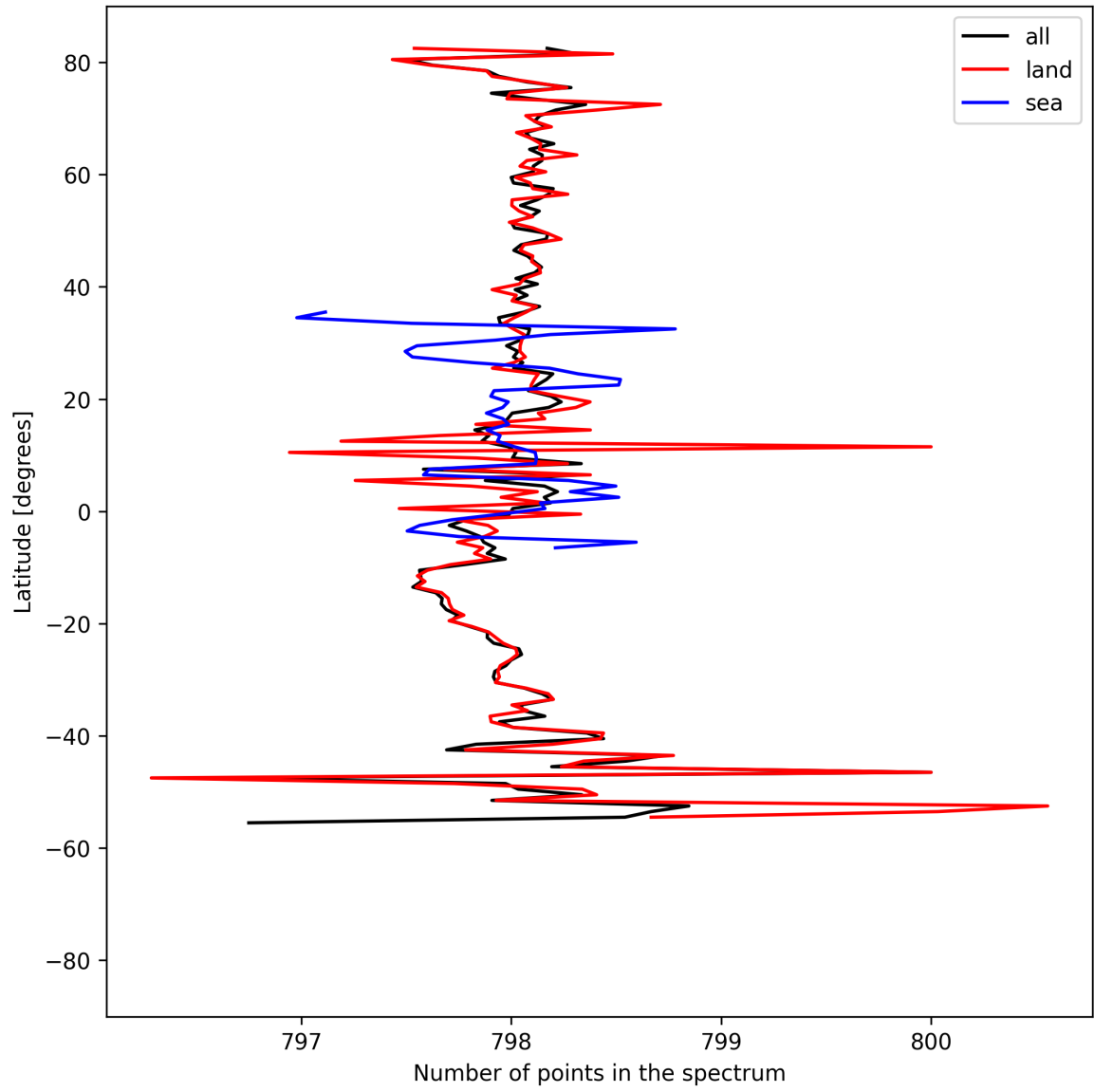
Figure 15: Zonal average of “Number of points in the spectrum” for 2024-09-01 to 2024-09-02.
