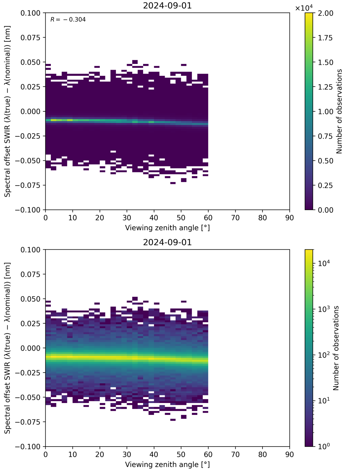
Figure 116: Scatter density plot of “Viewing zenith angle” against “Spectral offset SWIR ( \lambda_{\text{true}} - \lambda_{\text{nominal}} )” for 2024-09-01 to 2024-09-02.
