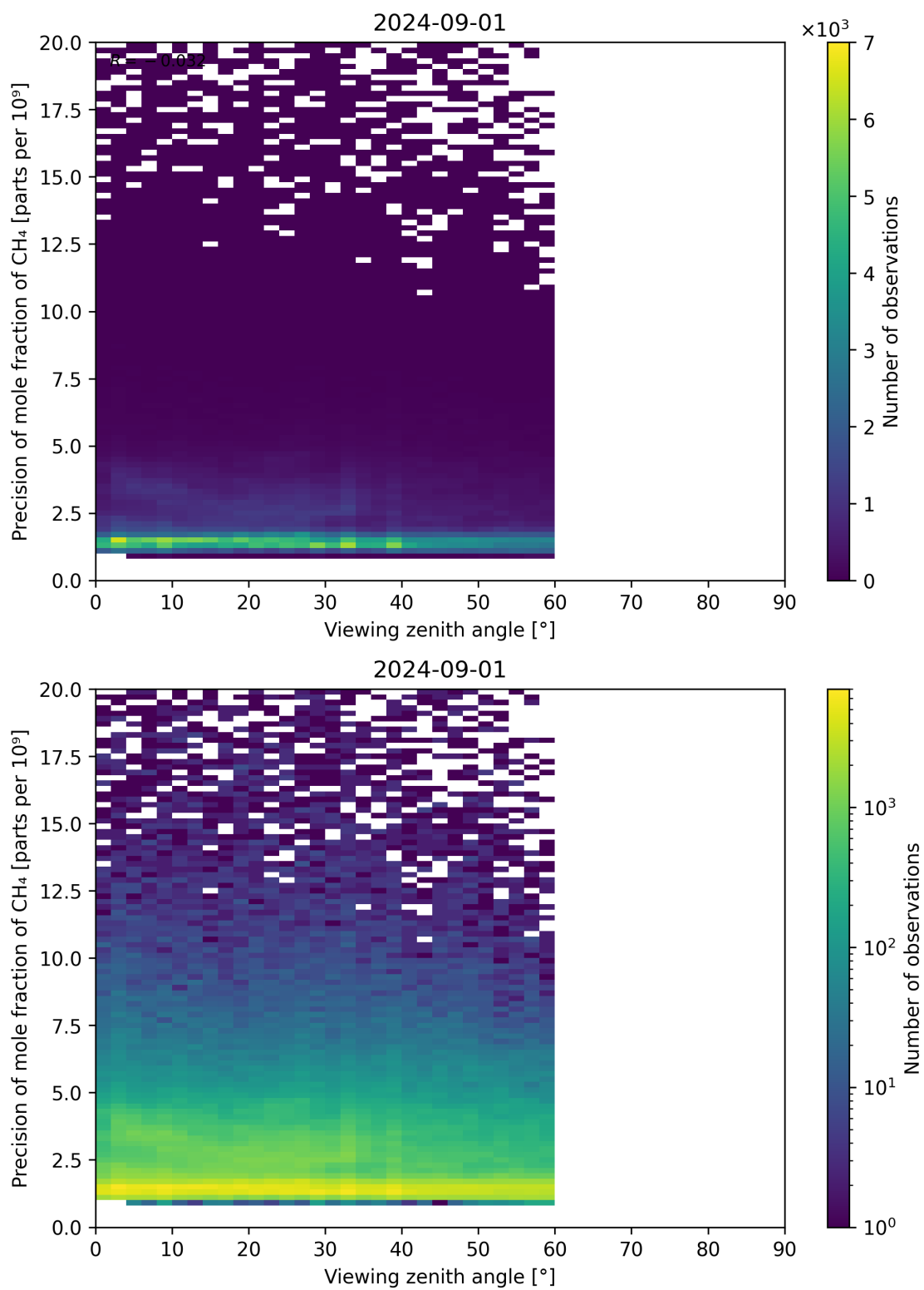
Figure 112: Scatter density plot of “Viewing zenith angle” against “Precision of mole fraction of CH 4 ” for 2024-09-01 to 2024-09-02.
