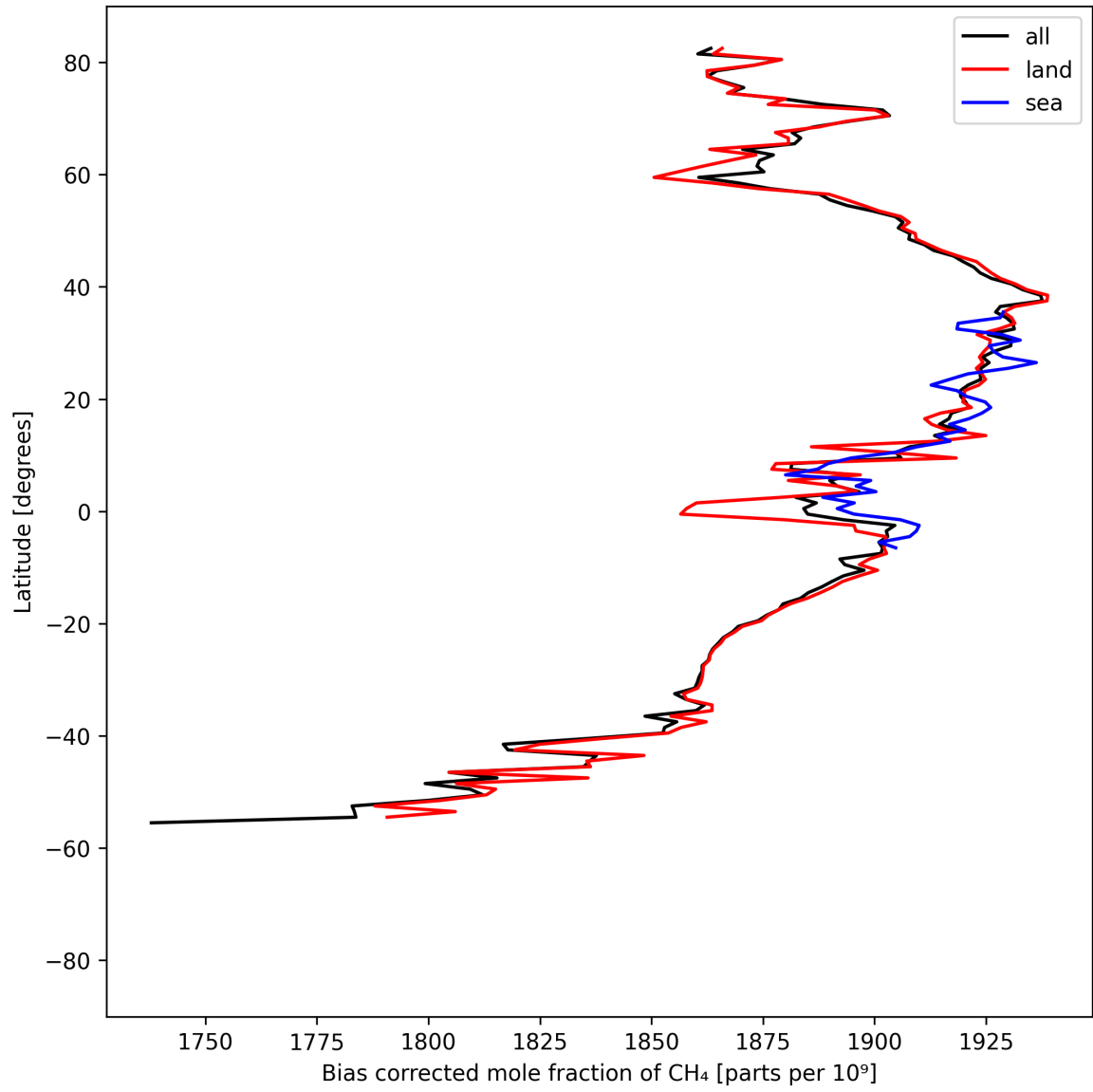
Figure 14: Zonal average of “Bias corrected mole fraction of CH 4 ” for 2024-09-01 to 2024-09-02.
