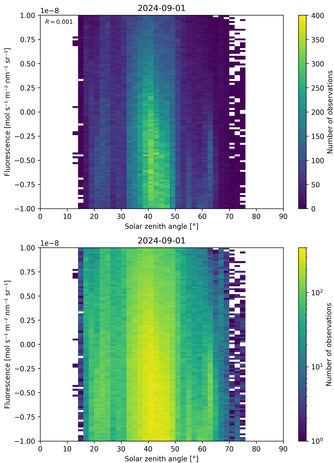
Figure 97: Scatter density plot of “Solar zenith angle” against “Fluorescence” for 2024-09-01 to 2024-09-02.
