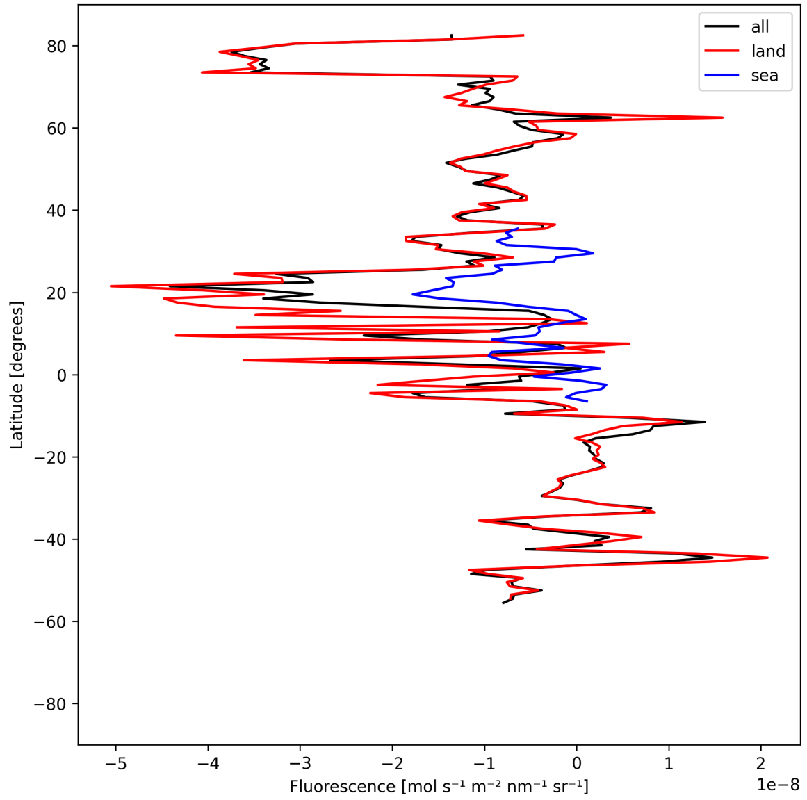
Figure 21: Zonal average of “Fluorescence” for 2024-09-01 to 2024-09-02.
