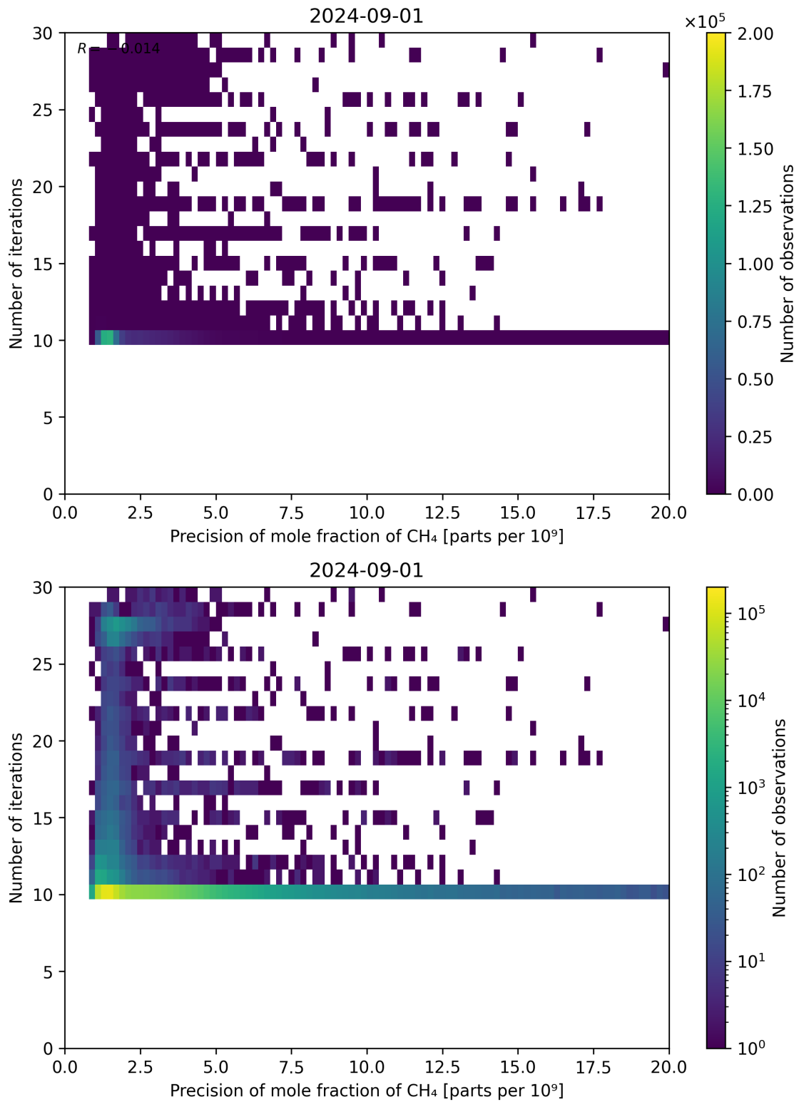
Figure 83: Scatter density plot of “Precision of mole fraction of CH 4 ” against “Number of iterations” for 2024-09-01 to 2024-09-02.
