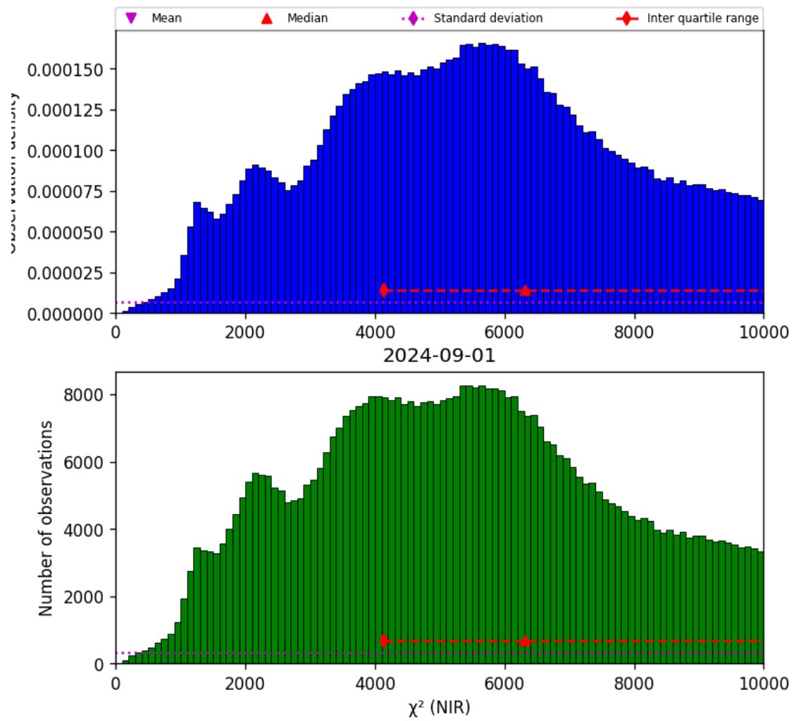
Figure 29: Histogram of “ \chi^2 (NIR)” for 2024-09-01 to 2024-09-02
