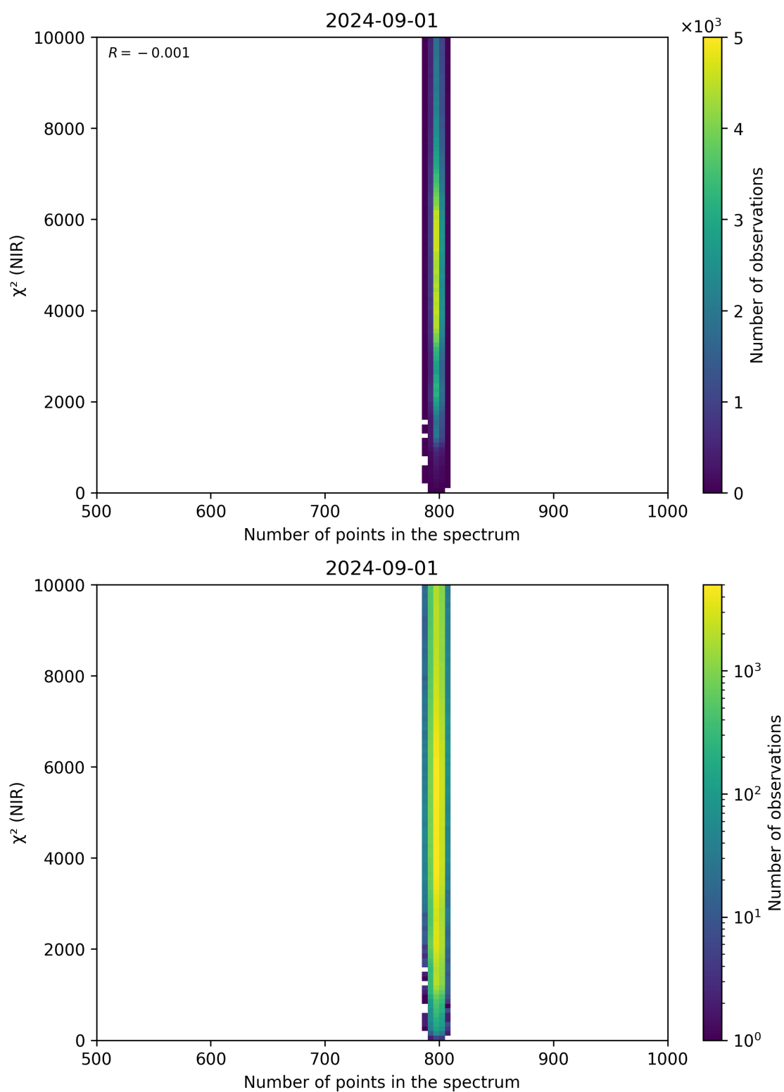
Figure 88: Scatter density plot of “Number of points in the spectrum” against “ \chi^2 (NIR)” for 2024-09-01 to 2024-09-02.
