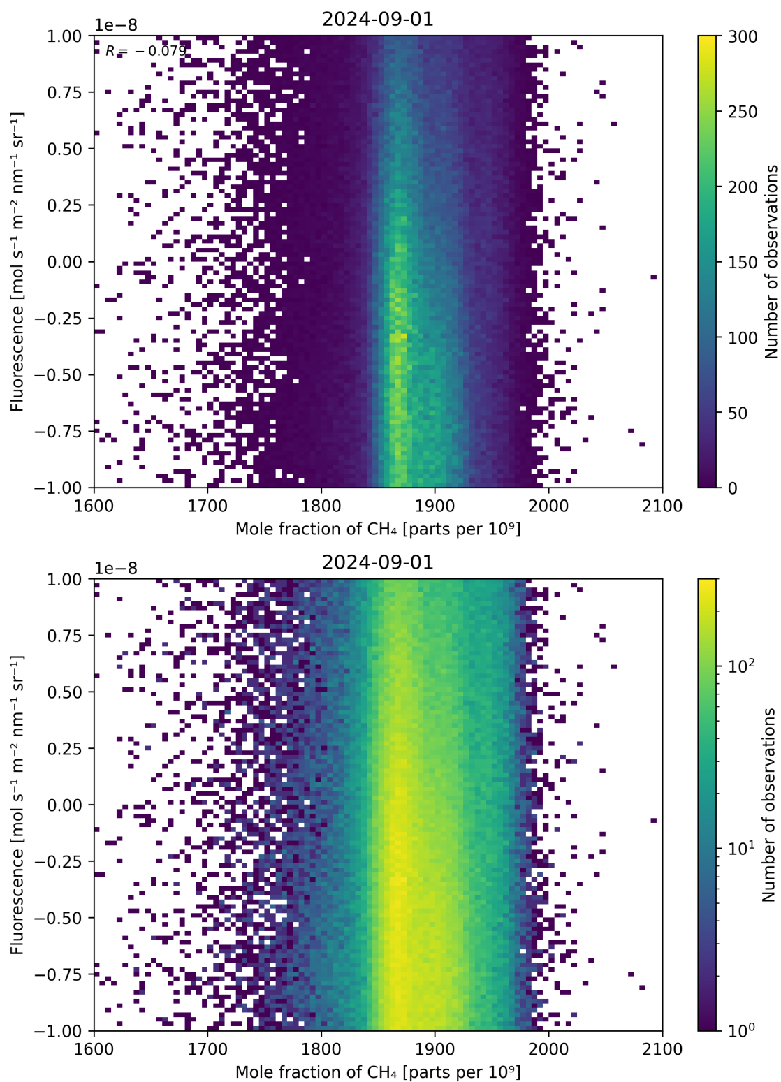
Figure 73: Scatter density plot of “Mole fraction of \text{CH}_4 ” against “Fluorescence” for 2024-09-01 to 2024-09-02.
