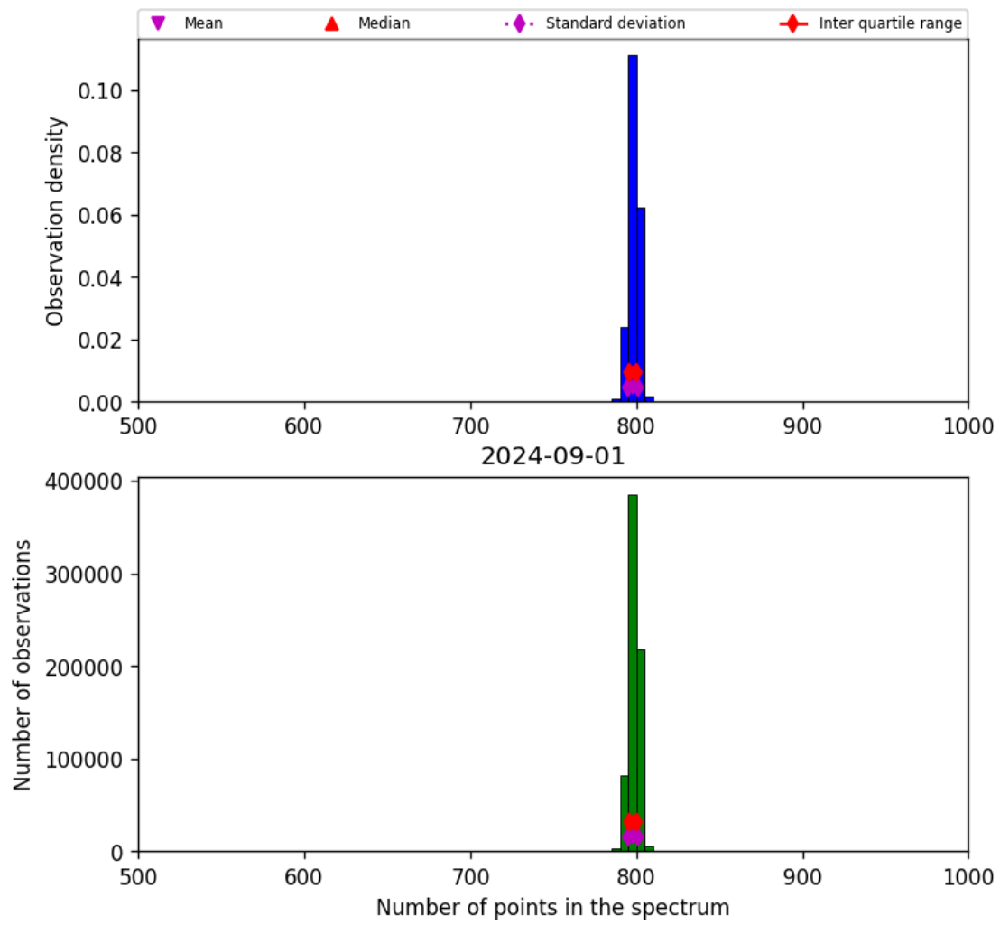
Figure 26: Histogram of “Number of points in the spectrum” for 2024-09-01 to 2024-09-02
