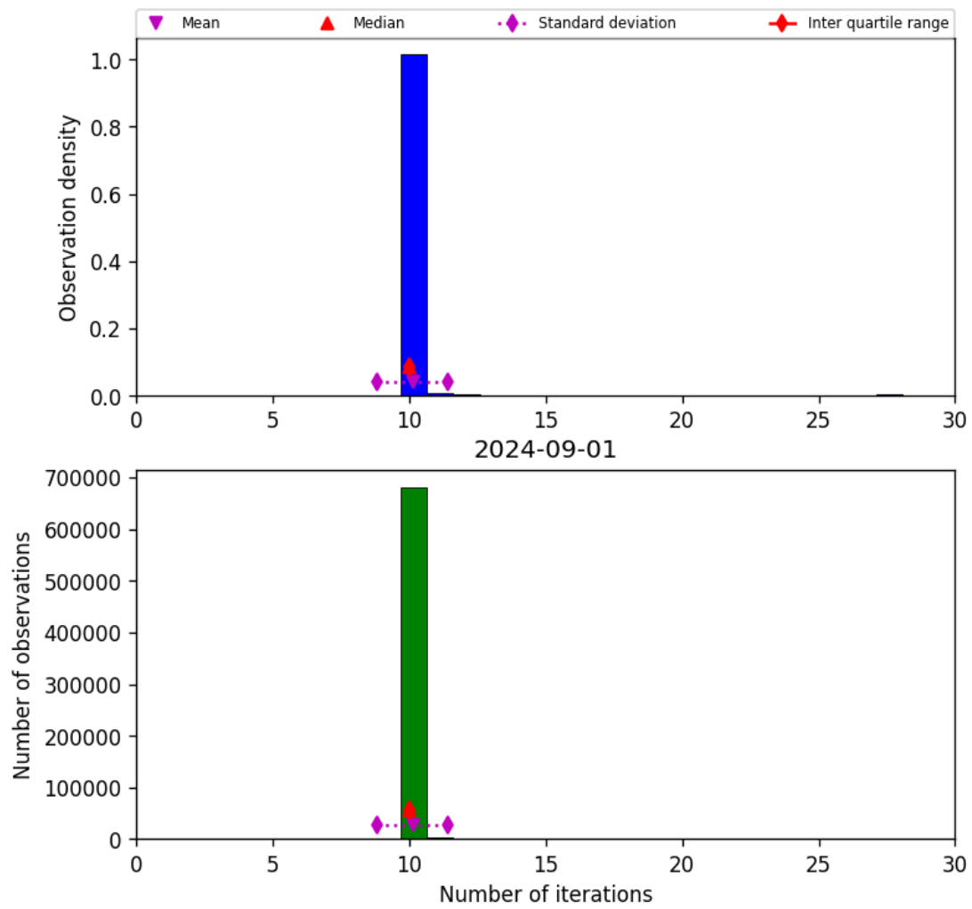
Figure 31: Histogram of “Number of iterations” for 2024-09-01 to 2024-09-02
