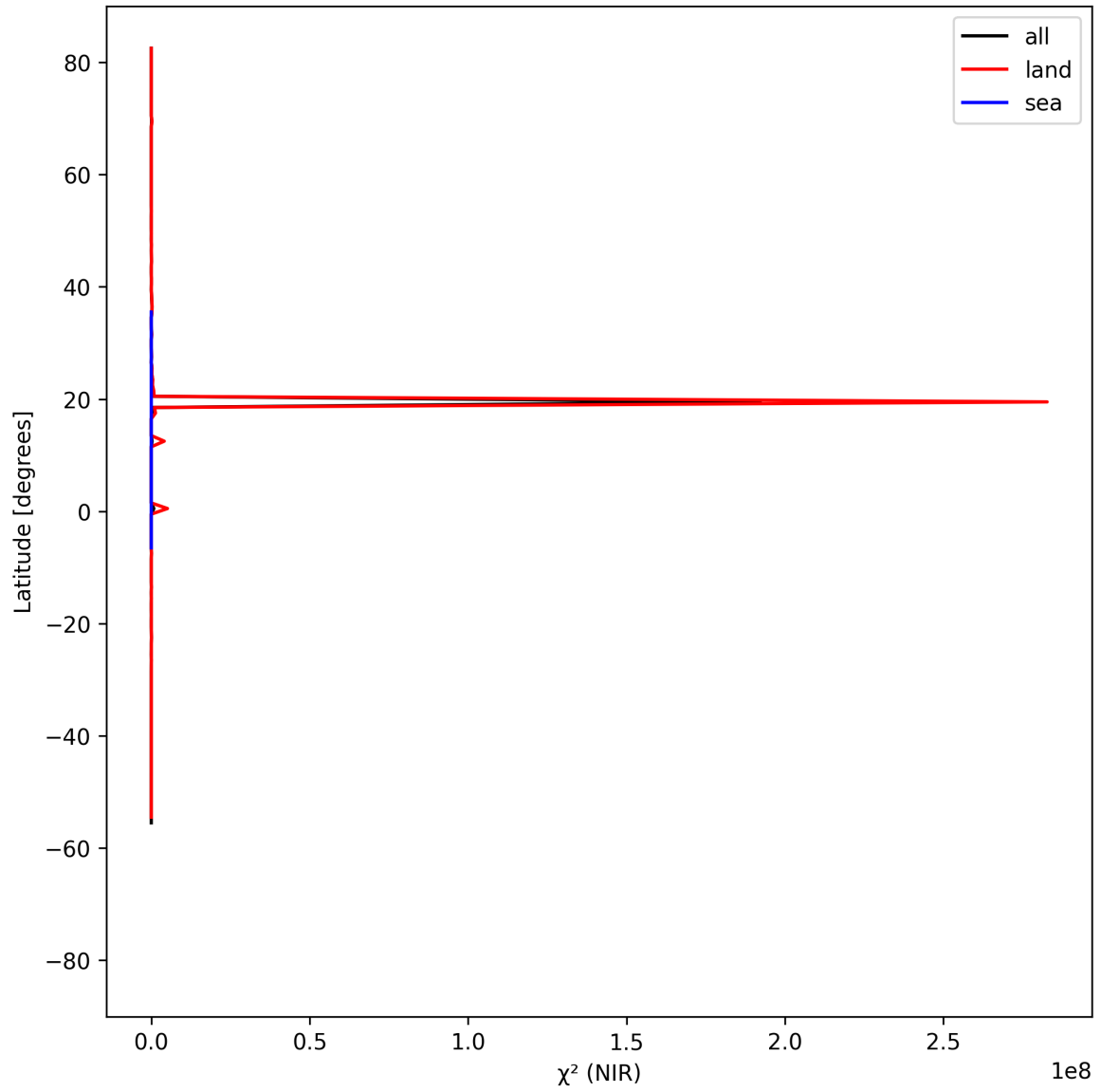
Figure 18: Zonal average of “ \chi^2 (NIR)” for 2024-09-01 to 2024-09-02.
