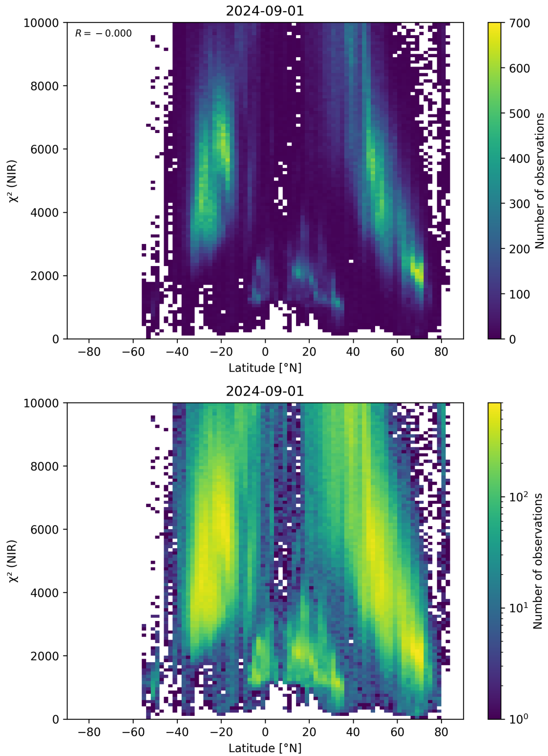
Figure 53: Scatter density plot of “Latitude” against “ \chi^2 (NIR)” for 2024-09-01 to 2024-09-02.
