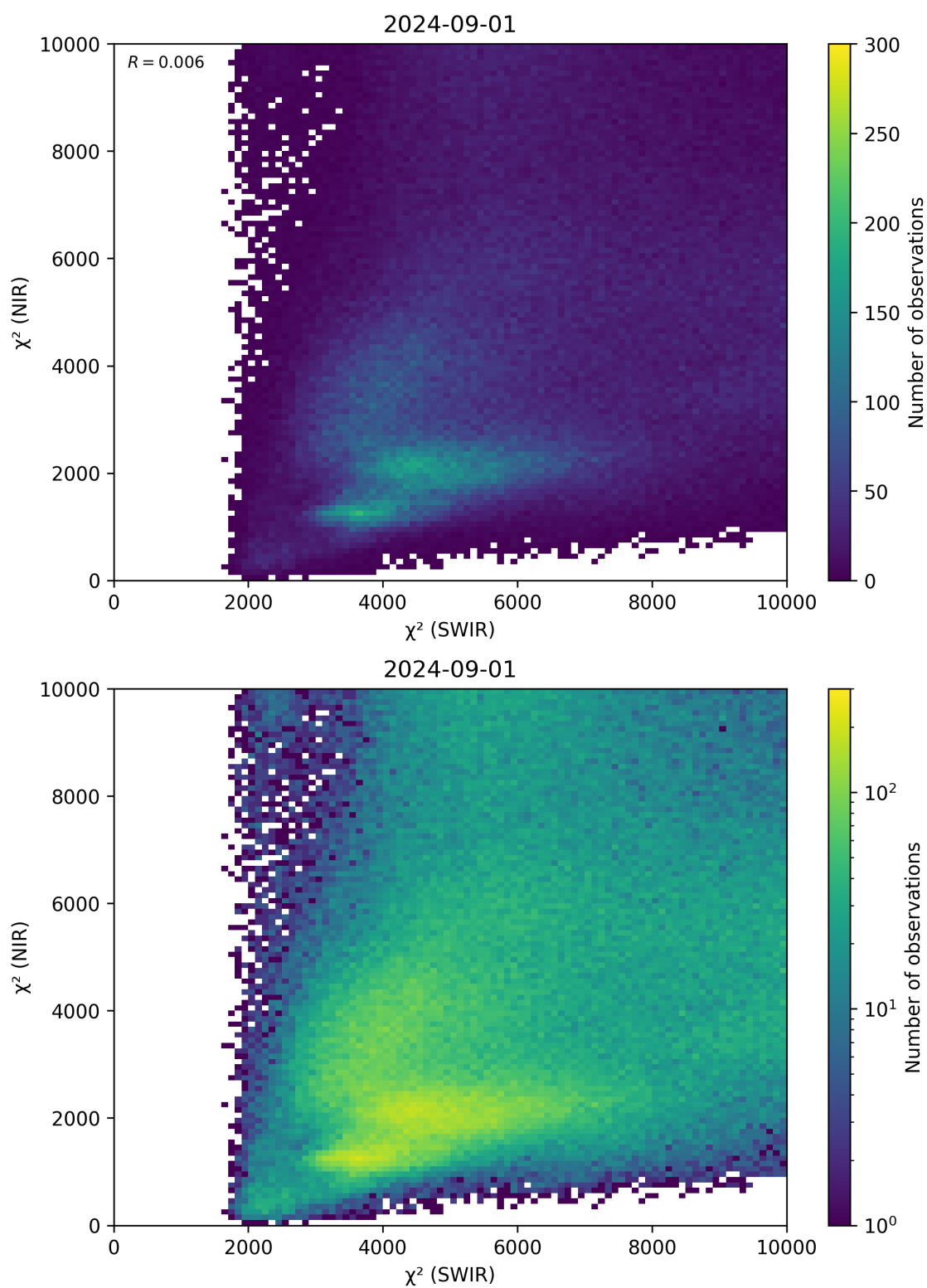
Figure 47: Scatter density plot of “ \chi^2 (SWIR)” against “ \chi^2 (NIR)” for 2024-09-01 to 2024-09-02.
