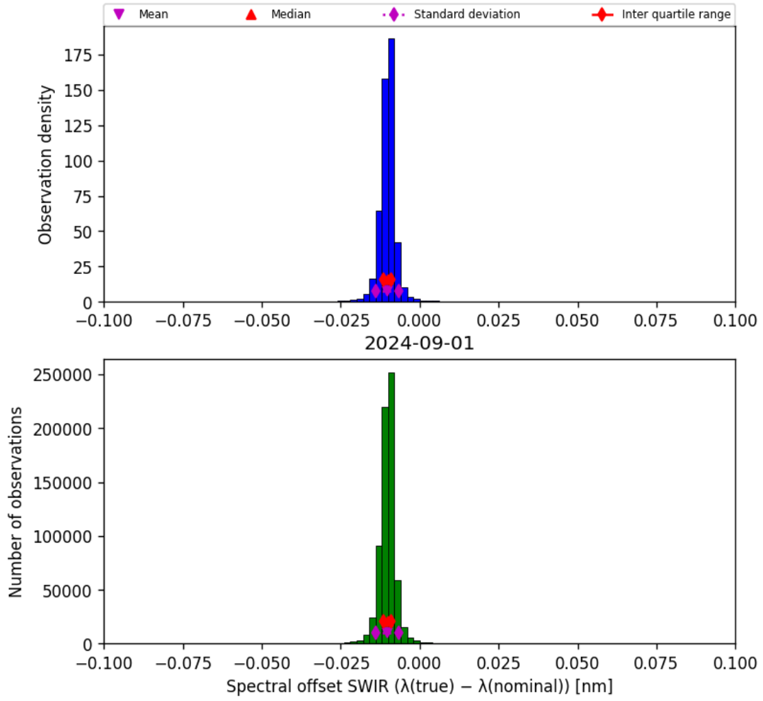
Figure 27: Histogram of “Spectral offset SWIR ( \lambda_{\text{true}} - \lambda_{\text{nominal}} )” for 2024-09-01 to 2024-09-02
