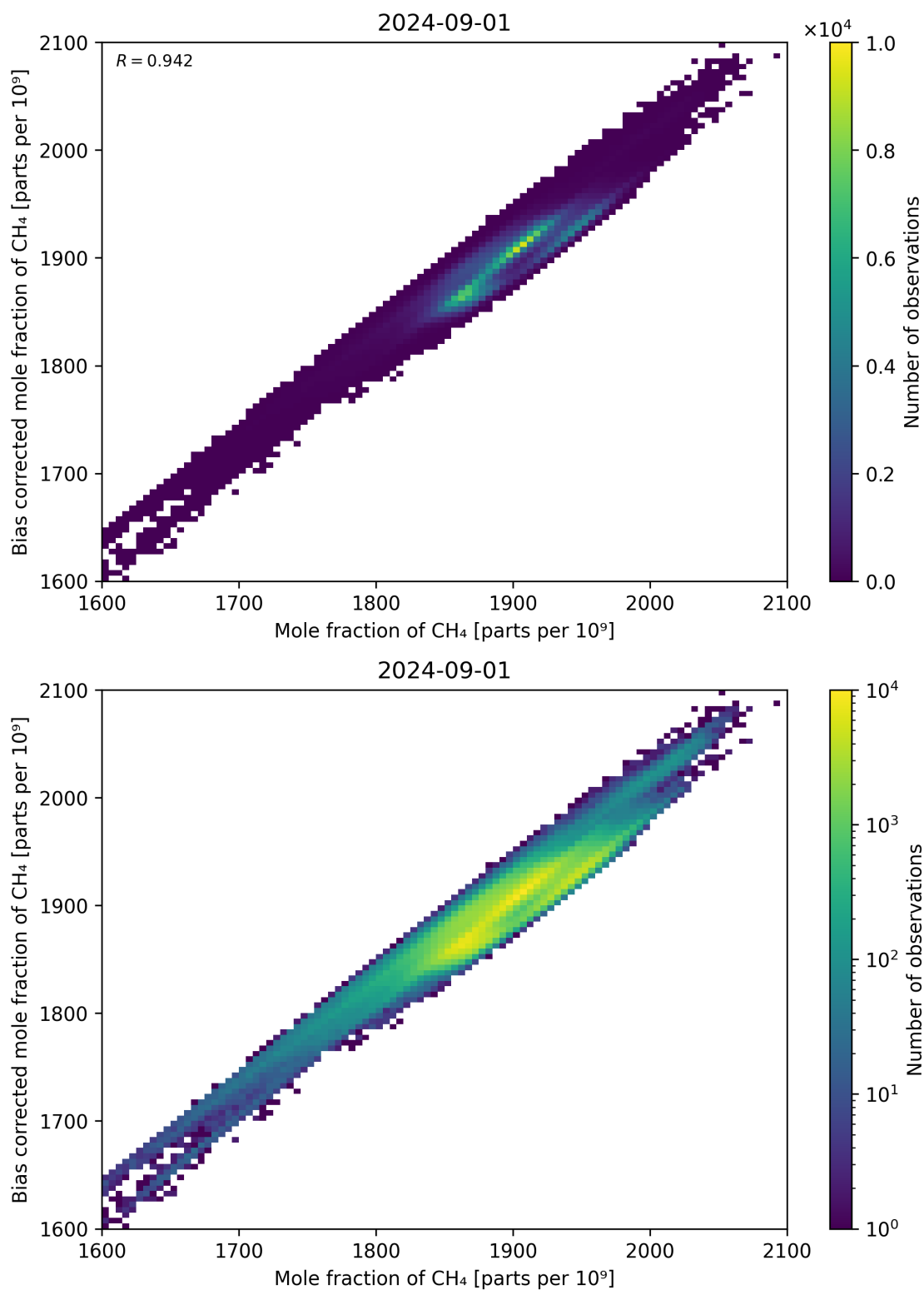
Figure 74: Scatter density plot of “Mole fraction of CH 4 ” against “Bias corrected mole fraction of CH 4 ” for 2024-09-01 to 2024-09-02.
