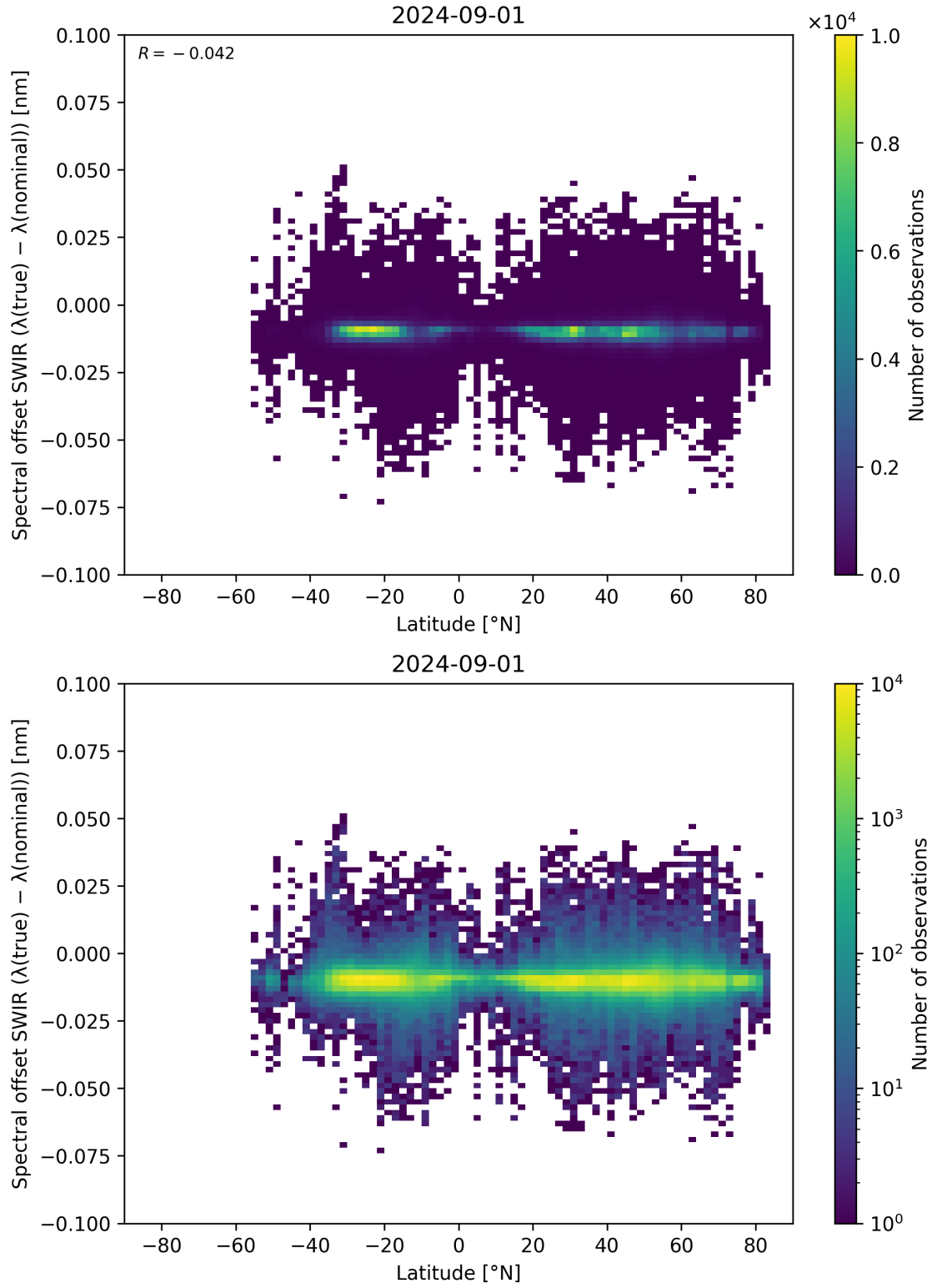
Figure 62: Scatter density plot of “Latitude” against “Spectral offset SWIR ( \lambda_{\text{true}} - \lambda_{\text{nominal}} )” for 2024-09-01 to 2024-09-02.
