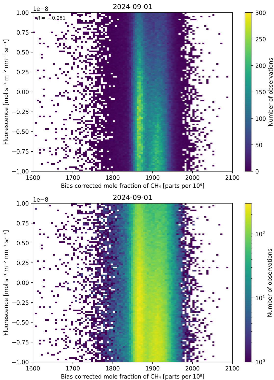
Figure 66: Scatter density plot of “Bias corrected mole fraction of CH 4 ” against “Fluorescence” for 2024-09-01 to 2024-09-02.
