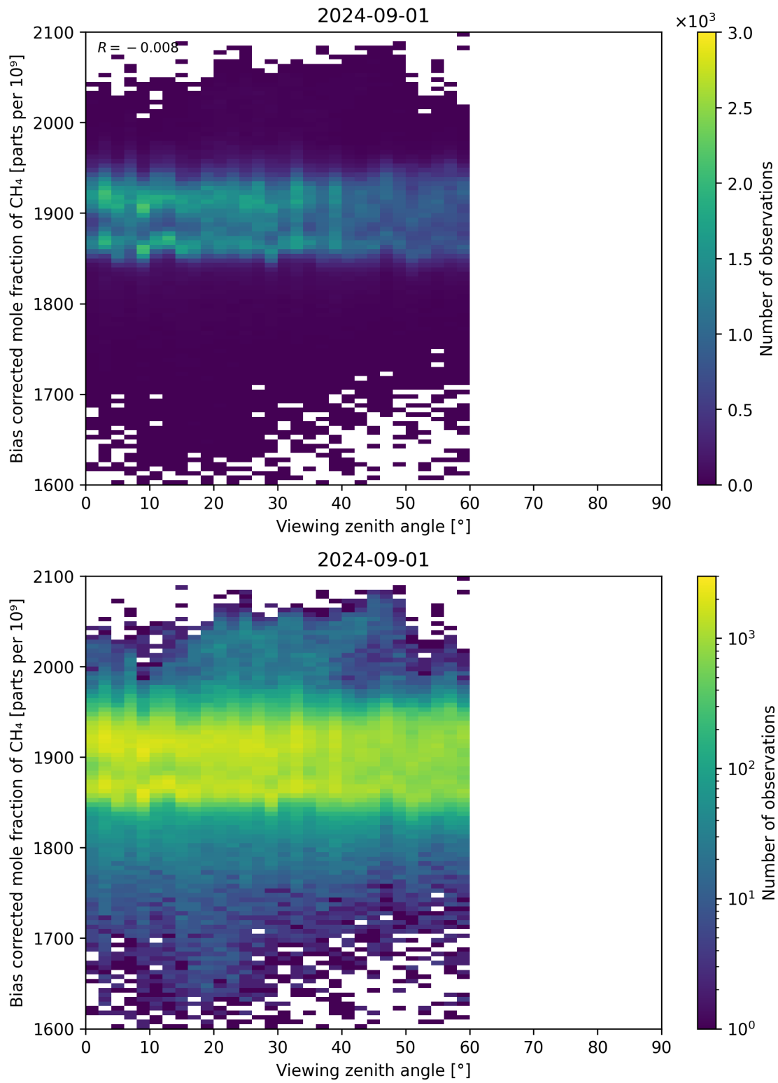
Figure 111: Scatter density plot of “Viewing zenith angle” against “Bias corrected mole fraction of CH 4 ” for 2024-09-01 to 2024-09-02.
