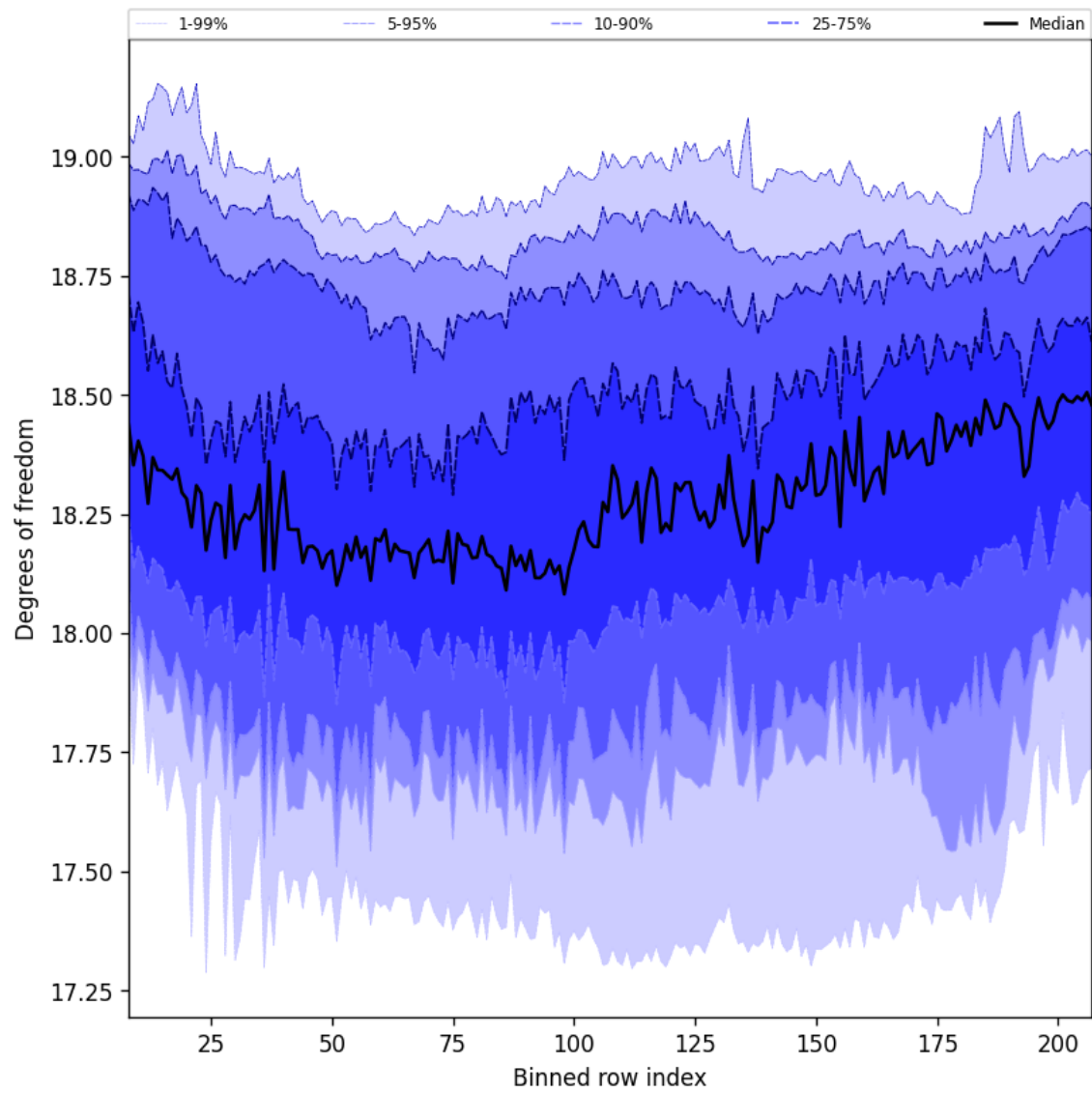
Figure 41: Along track statistics of “Degrees of freedom” for 2024-09-01 to 2024-09-02
