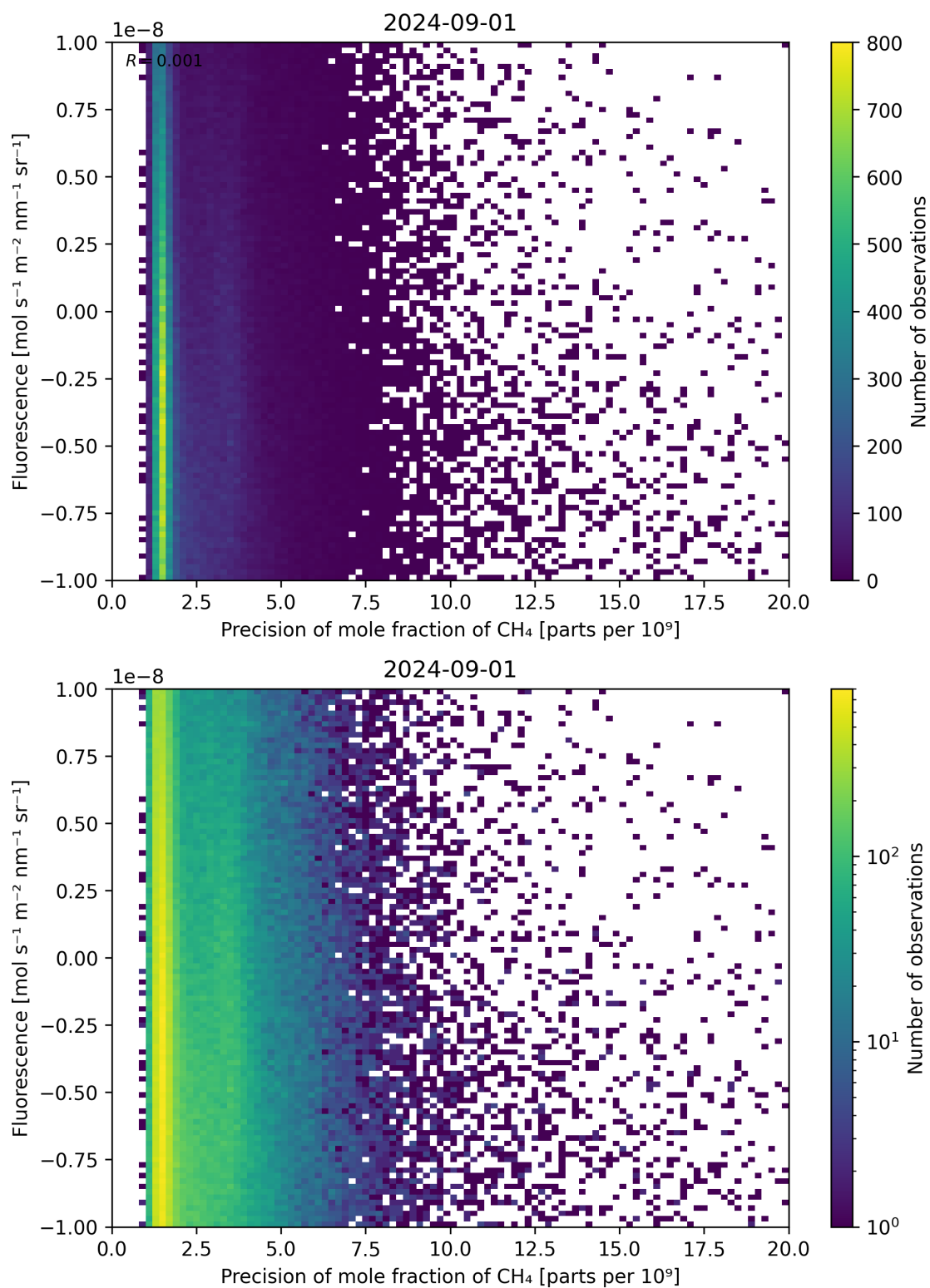
Figure 81: Scatter density plot of “Precision of mole fraction of \text{CH}_4 ” against “Fluorescence” for 2024-09-01 to 2024-09-02.
