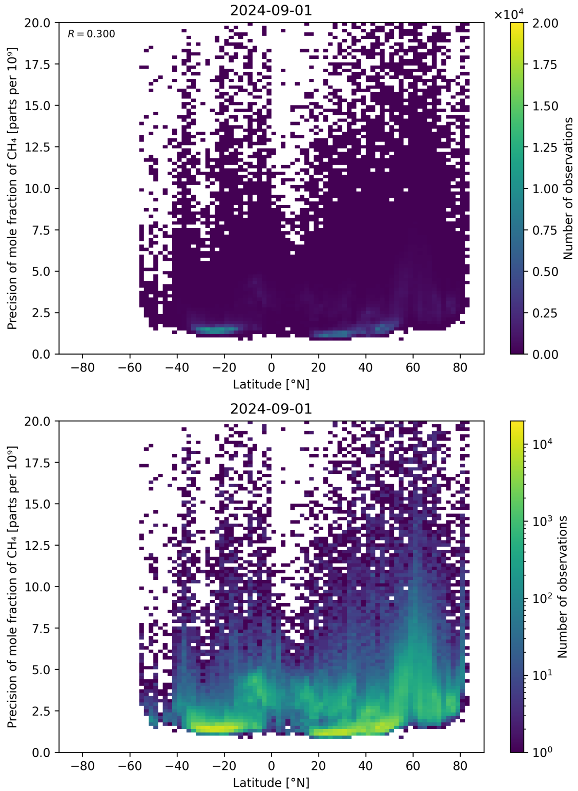
Figure 59: Scatter density plot of “Latitude” against “Precision of mole fraction of \text{CH}_4 ” for 2024-09-01 to 2024-09-02.
