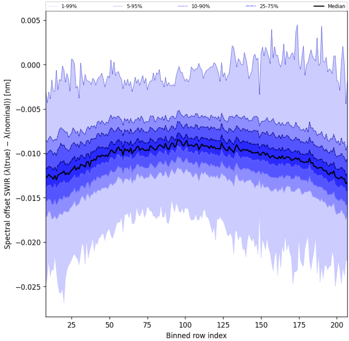
Figure 38: Along track statistics of “Spectral offset SWIR ( \lambda_{\text{true}} - \lambda_{\text{nominal}} )” for 2024-09-01 to 2024-09-02
