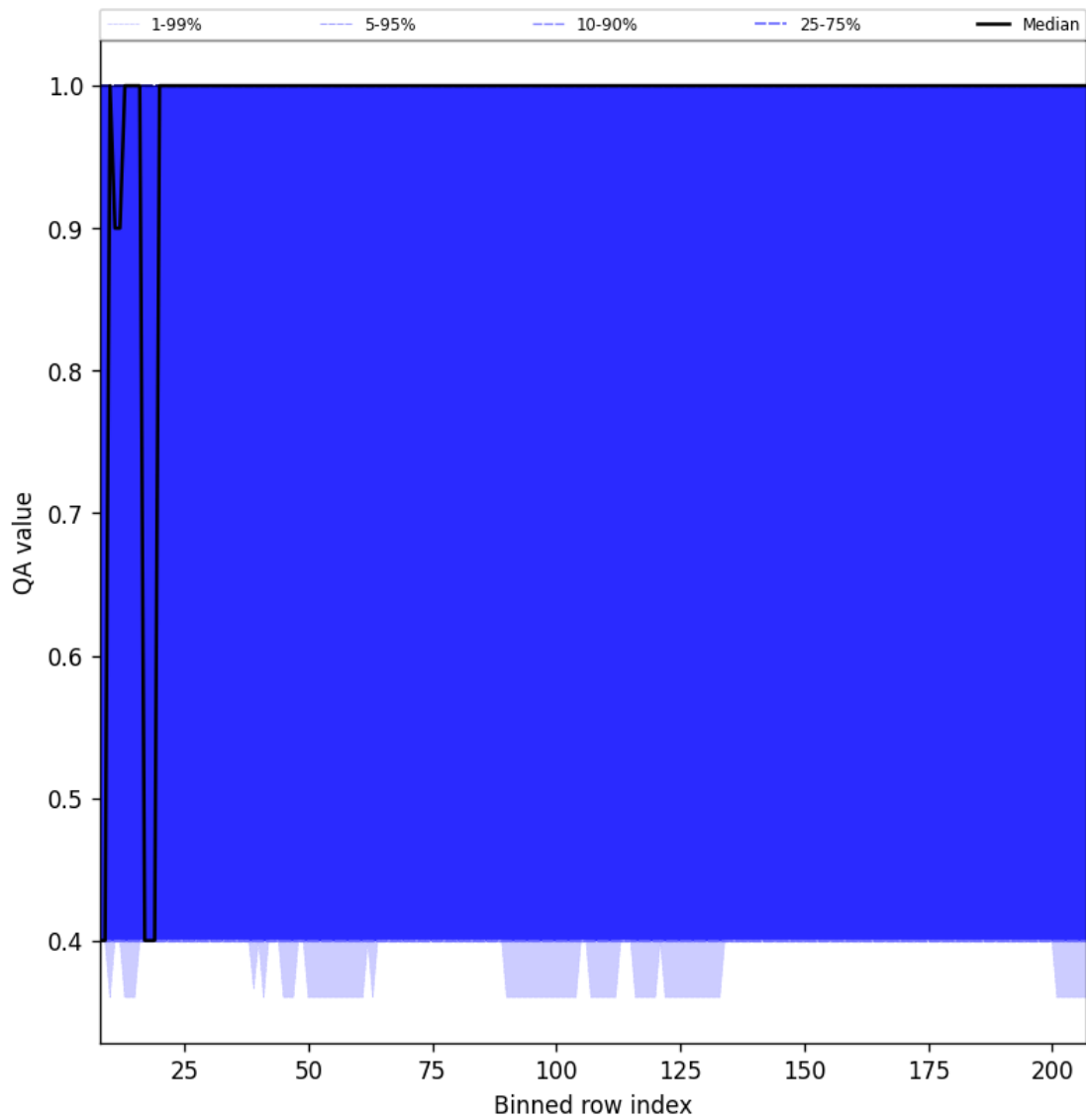
Figure 33: Along track statistics of “QA value” for 2024-09-01 to 2024-09-02
