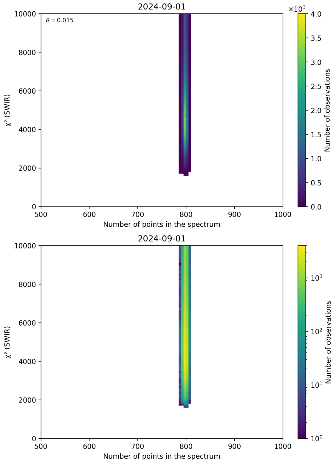
Figure 89: Scatter density plot of “Number of points in the spectrum” against “ \chi^2 (SWIR)” for 2024-09-01 to 2024-09-02.
