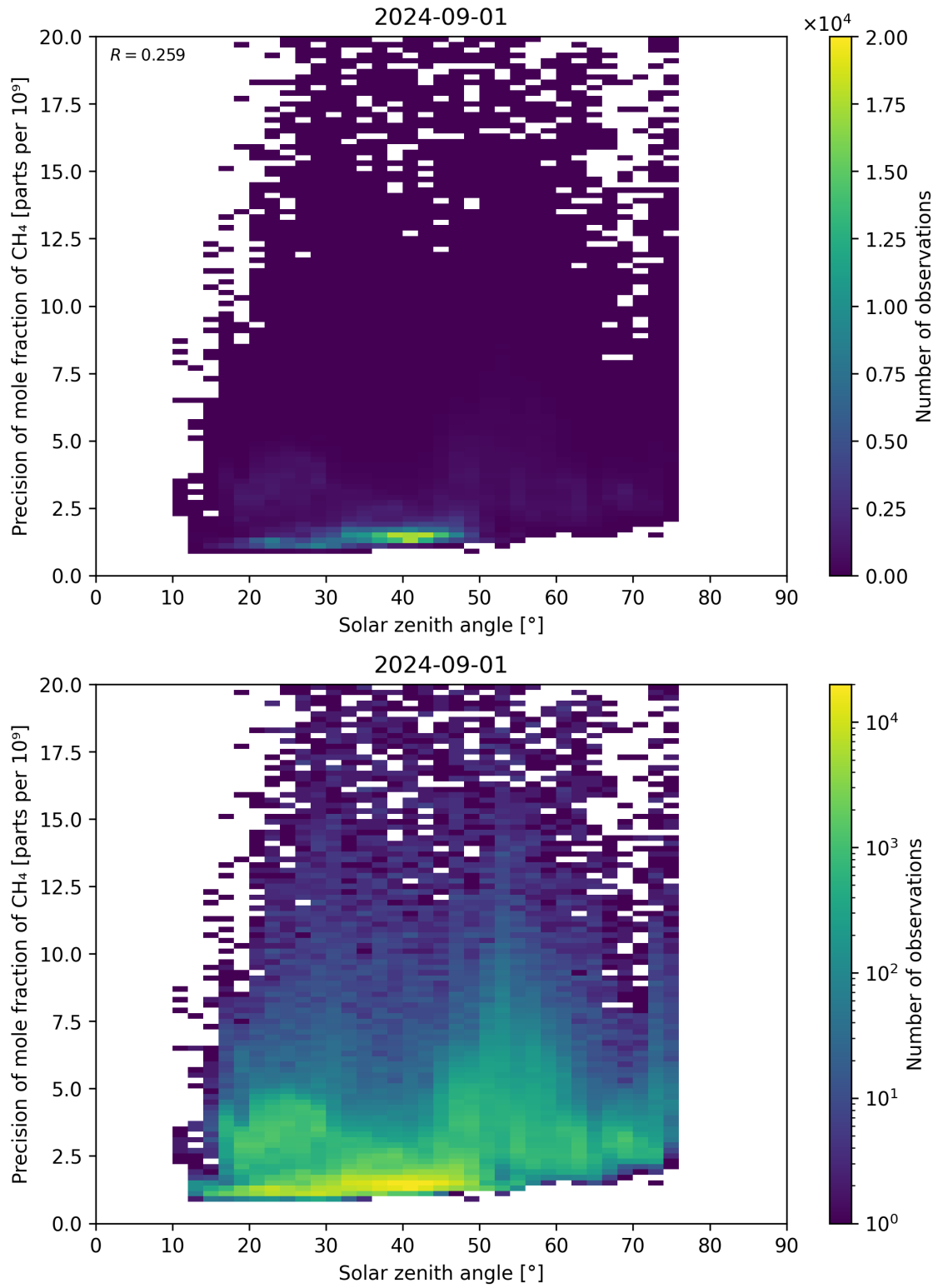
Figure 101: Scatter density plot of “Solar zenith angle” against “Precision of mole fraction of CH 4 ” for 2024-09-01 to 2024-09-02.
