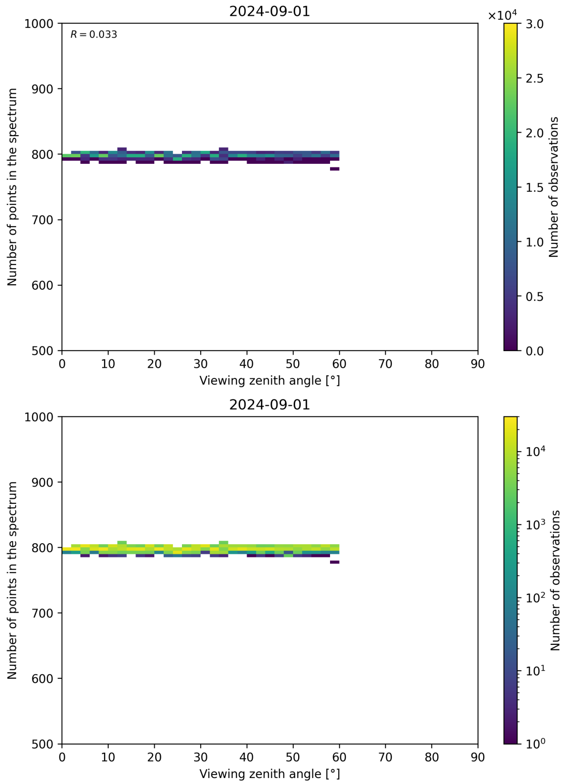
Figure 114: Scatter density plot of “Viewing zenith angle” against “Number of points in the spectrum” for 2024-09-01 to 2024-09-02.
