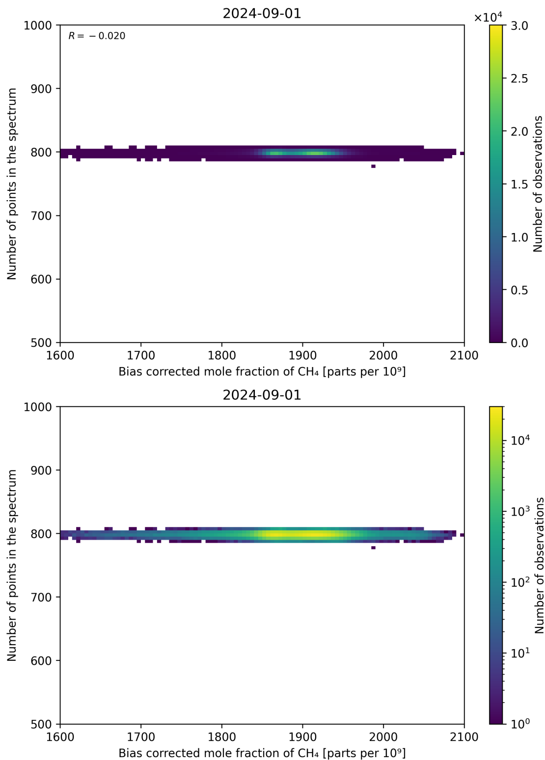
Figure 68: Scatter density plot of “Bias corrected mole fraction of CH 4 ” against “Number of points in the spectrum” for 2024-09-01 to 2024-09-02.
