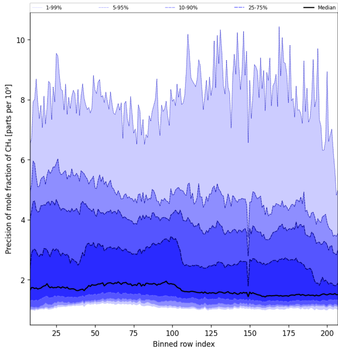
Figure 35: Along track statistics of “Precision of mole fraction of CH 4 ” for 2024-09-01 to 2024-09-02
