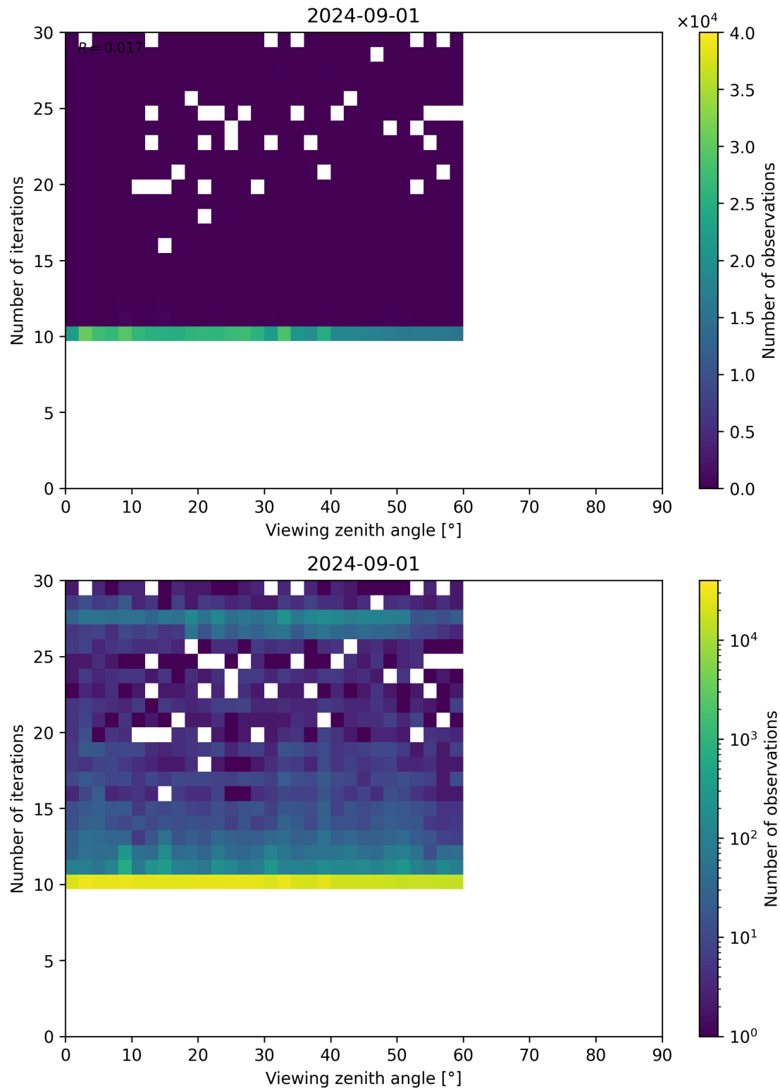
Figure 113: Scatter density plot of “Viewing zenith angle” against “Number of iterations” for 2024-09-01 to 2024-09-02.
