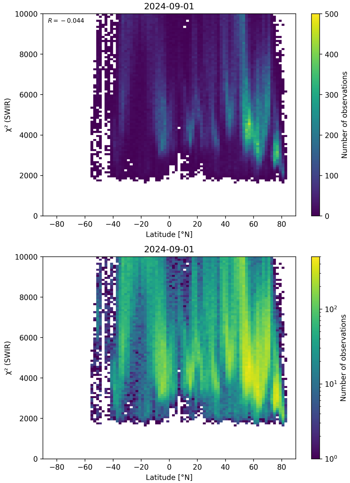
Figure 54: Scatter density plot of “Latitude” against “ \chi^2 (SWIR)” for 2024-09-01 to 2024-09-02.
