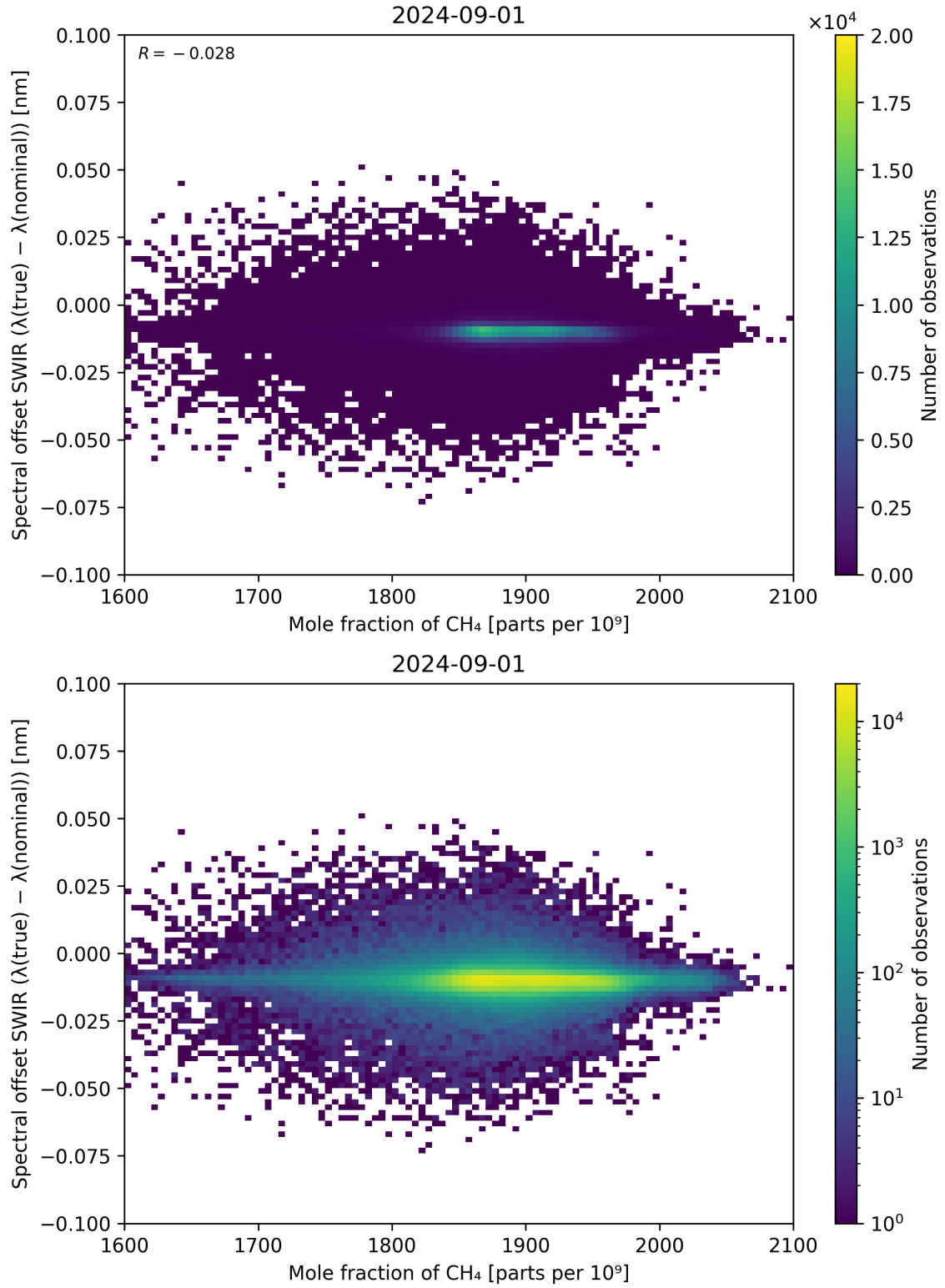
Figure 86: Scatter density plot of “Mole fraction of \text{CH}_4 ” against “Spectral offset SWIR ( \lambda_{\text{true}} - \lambda_{\text{nominal}} )” for 2024-09-01 to 2024-09-02.
