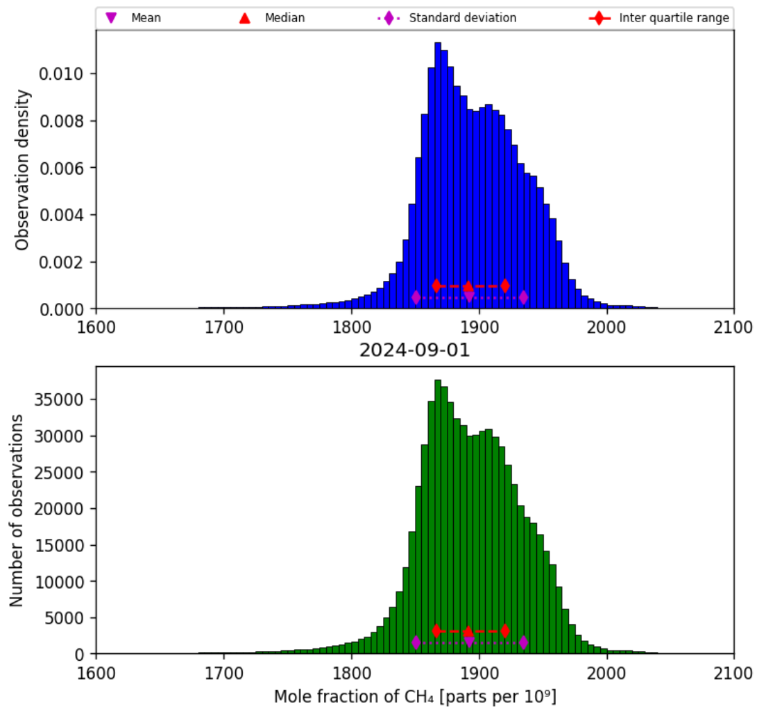
Figure 23: Histogram of “Mole fraction of CH 4 ” for 2024-09-01 to 2024-09-02
