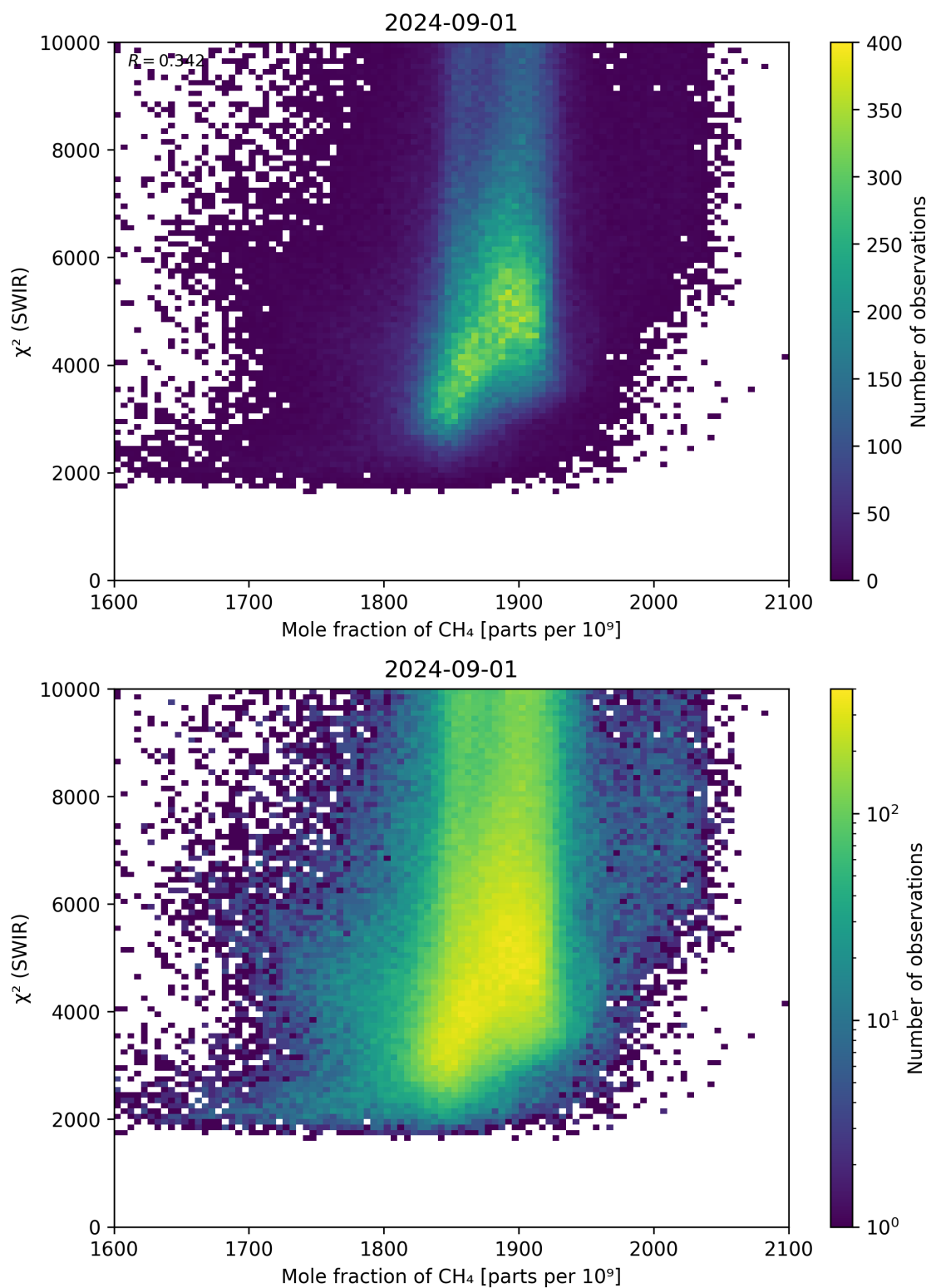
Figure 71: Scatter density plot of “Mole fraction of \text{CH}_4 ” against “ \chi^2 (SWIR)” for 2024-09-01 to 2024-09-02.
