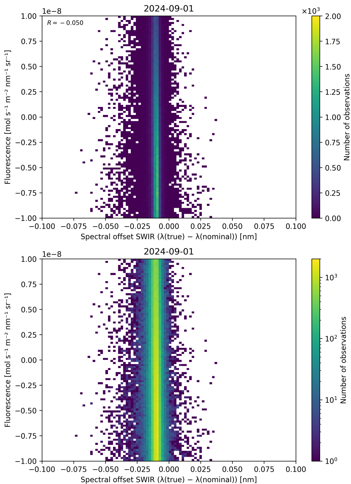
Figure 120: Scatter density plot of “Spectral offset SWIR ( \lambda_{\text{true}} - \lambda_{\text{nominal}} )” against “Fluorescence” for 2024-09-01 to 2024-09-02.
