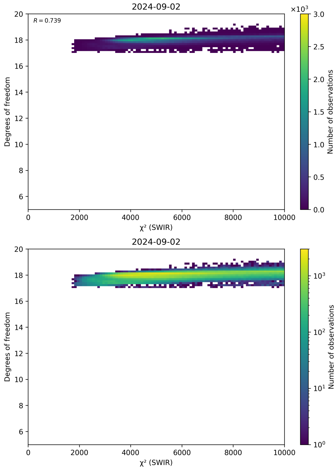
Figure 48: Scatter density plot of “ \chi^2 (SWIR)” against “Degrees of freedom” for 2024-09-01 to 2024-09-03.
