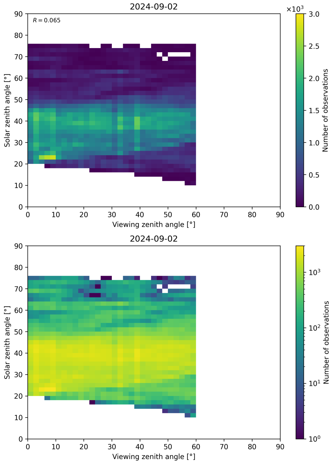
Figure 115: Scatter density plot of “Viewing zenith angle” against “Solar zenith angle” for 2024-09-01 to 2024-09-03.
