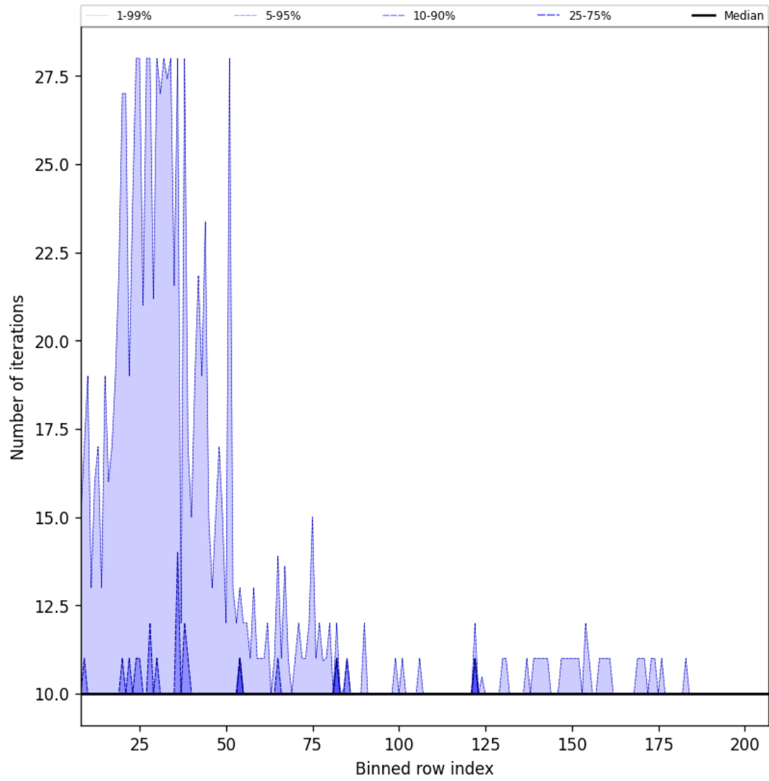
Figure 42: Along track statistics of “Number of iterations” for 2024-09-01 to 2024-09-03
