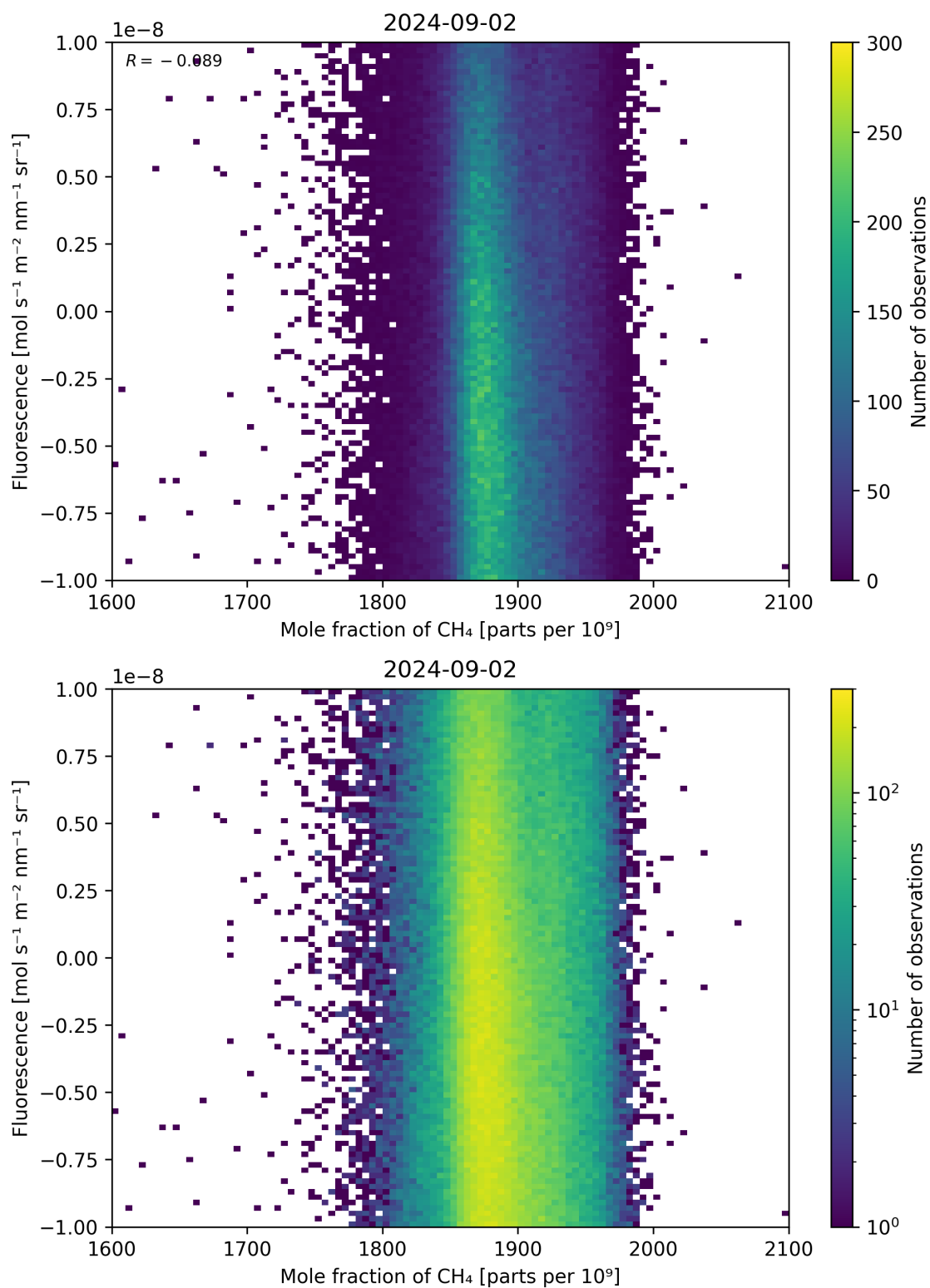
Figure 73: Scatter density plot of “Mole fraction of \text{CH}_4 ” against “Fluorescence” for 2024-09-01 to 2024-09-03.
