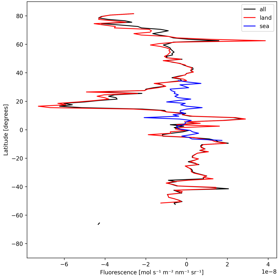
Figure 21: Zonal average of “Fluorescence” for 2024-09-01 to 2024-09-03.
