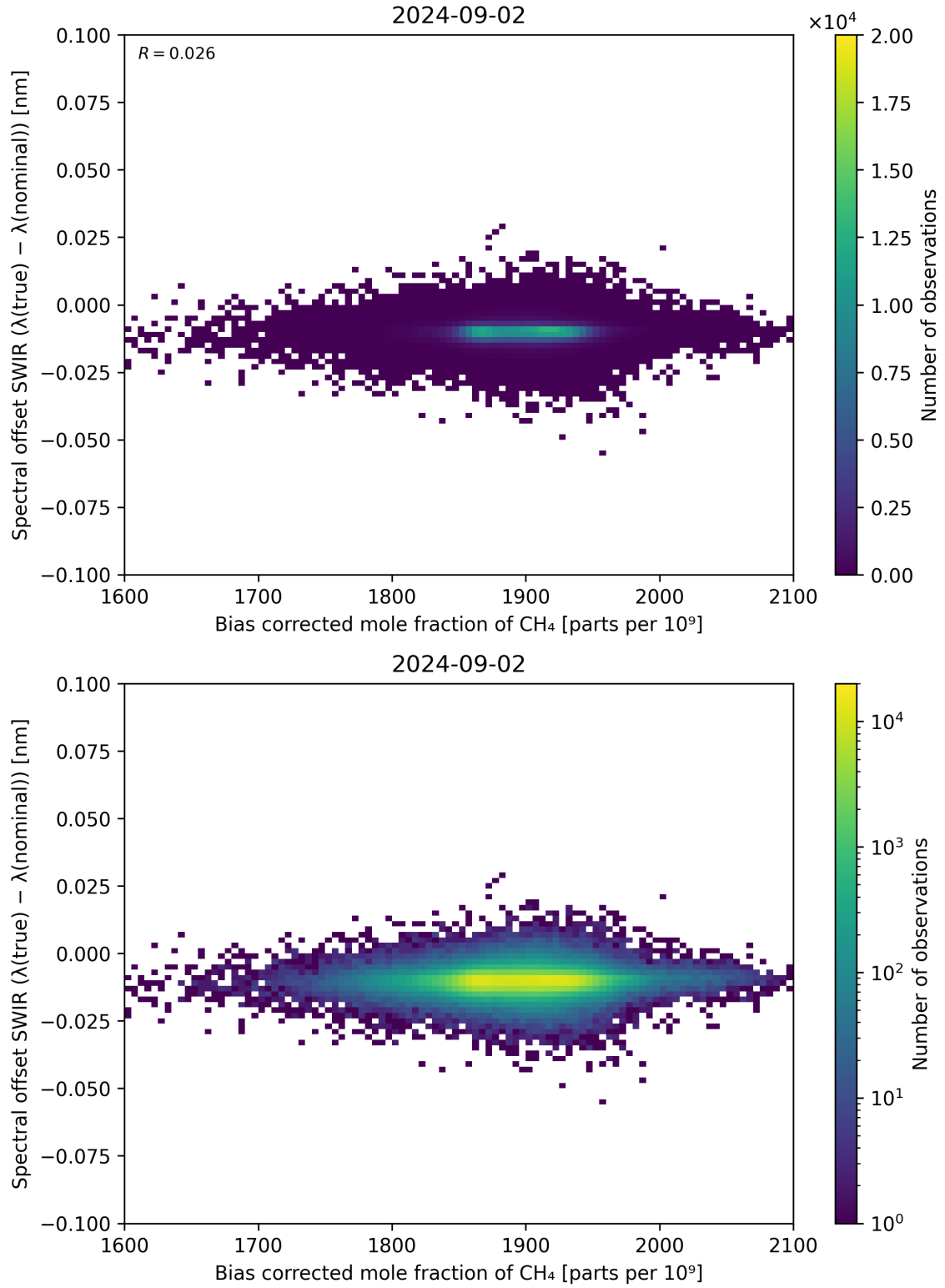
Figure 69: Scatter density plot of “Bias corrected mole fraction of \text{CH}_4 ” against “Spectral offset SWIR ( \lambda_{\text{true}} - \lambda_{\text{nominal}} )” for 2024-09-01 to 2024-09-03.
