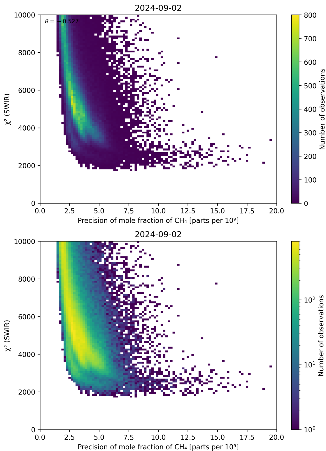
Figure 79: Scatter density plot of “Precision of mole fraction of CH 4 ” against “ \chi^2 (SWIR)” for 2024-09-01 to 2024-09-03.
