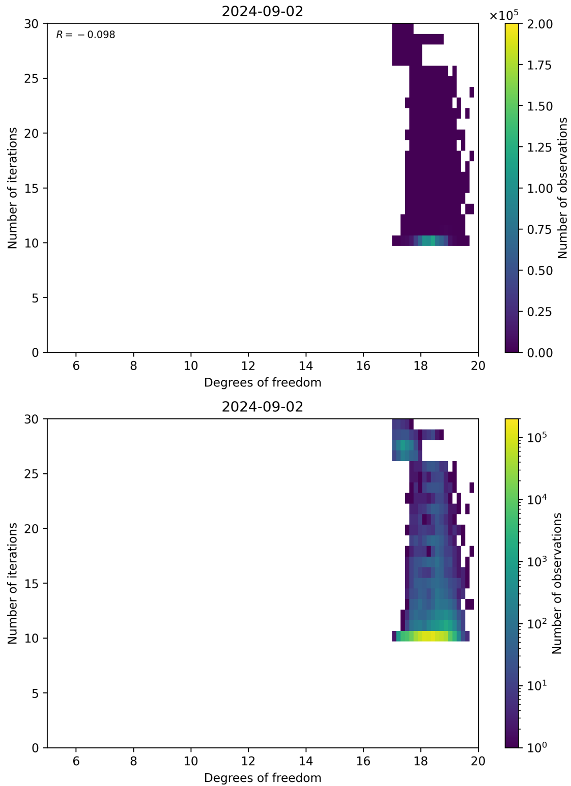
Figure 52: Scatter density plot of “Degrees of freedom” against “Number of iterations” for 2024-09-01 to 2024-09-03.
