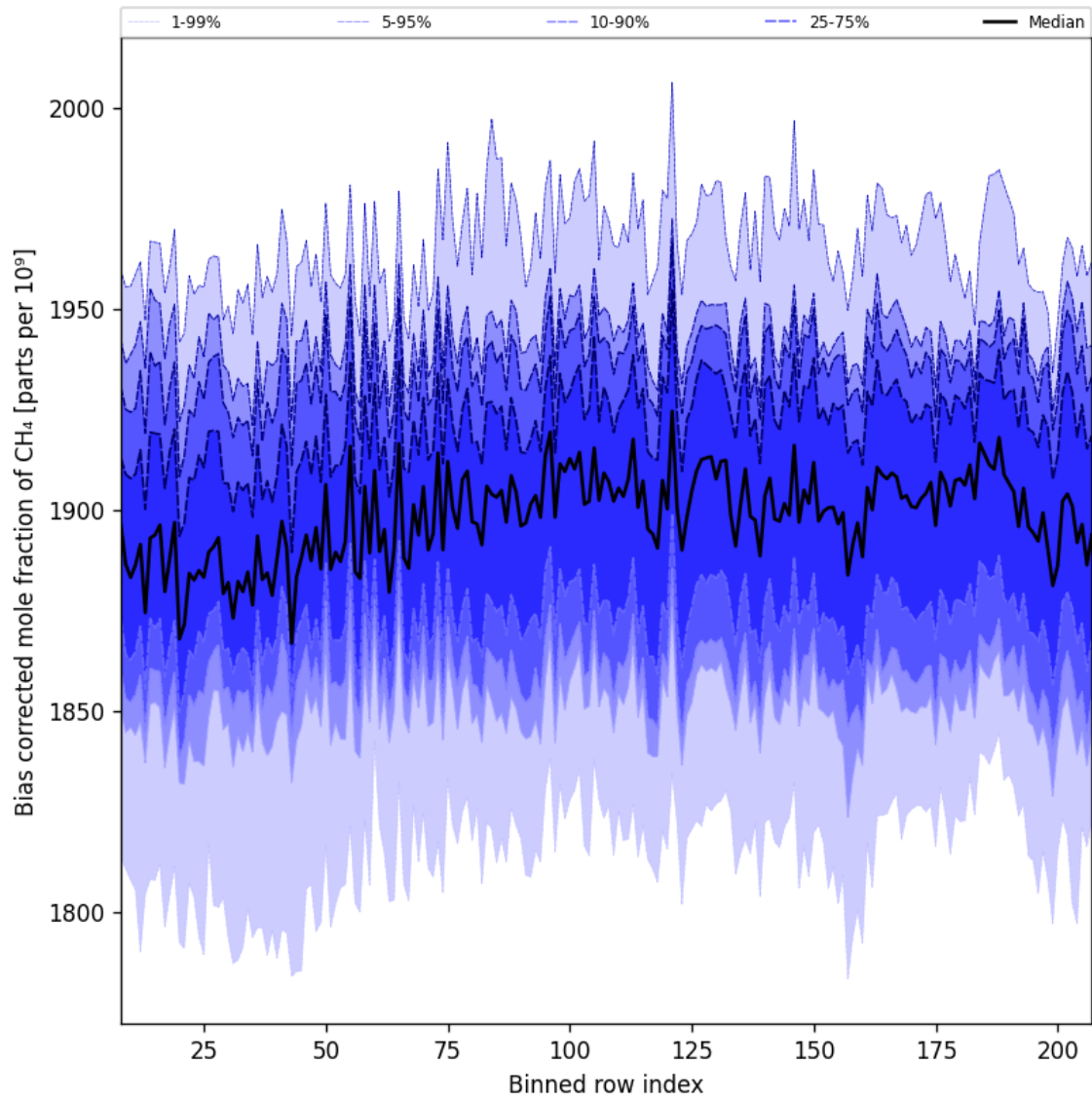
Figure 36: Along track statistics of “Bias corrected mole fraction of CH 4 ” for 2024-09-01 to 2024-09-03
