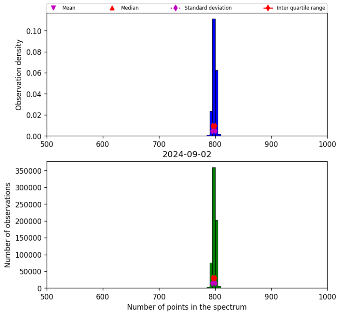
Figure 26: Histogram of “Number of points in the spectrum” for 2024-09-01 to 2024-09-03
