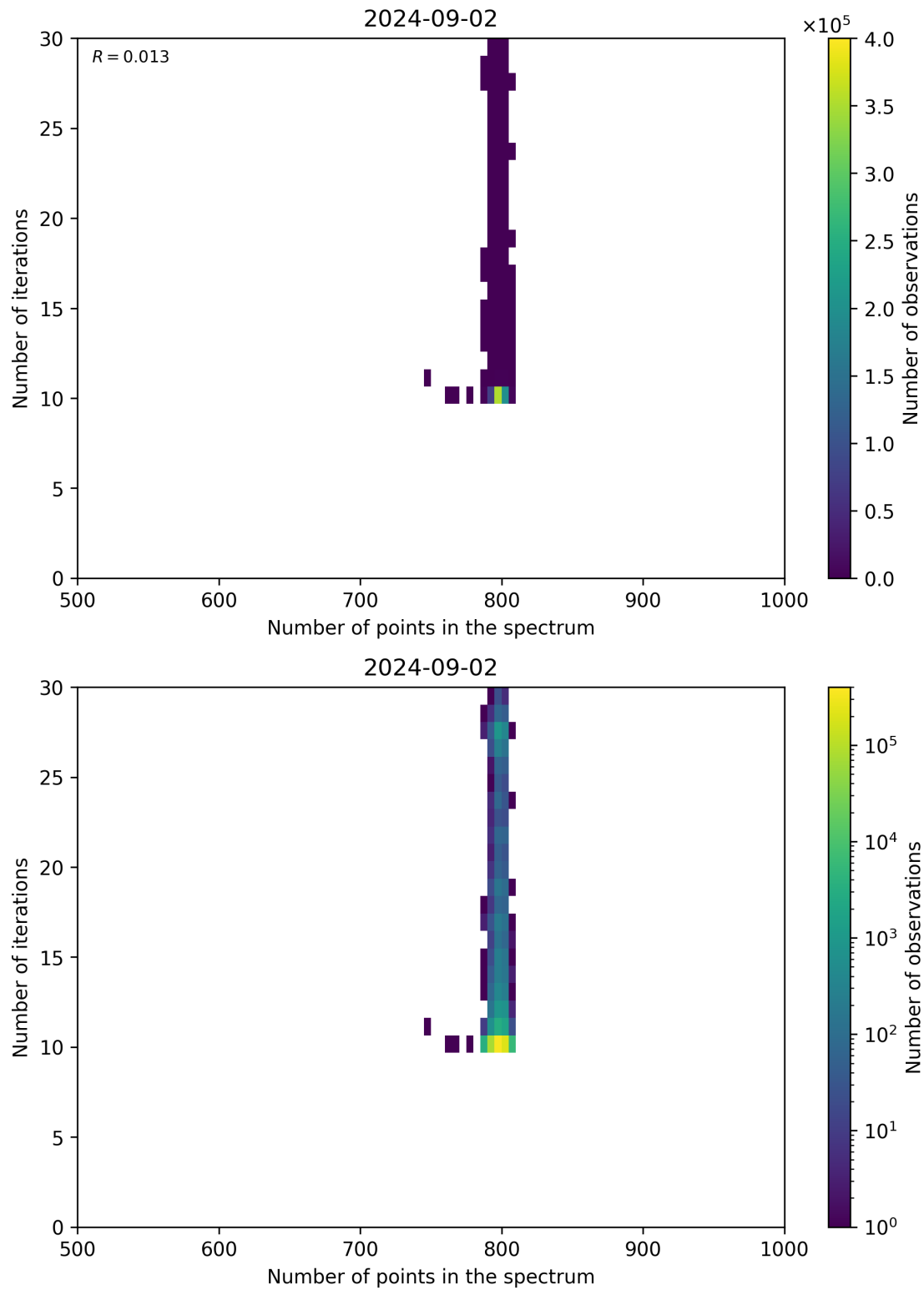
Figure 92: Scatter density plot of “Number of points in the spectrum” against “Number of iterations” for 2024-09-01 to 2024-09-03.
