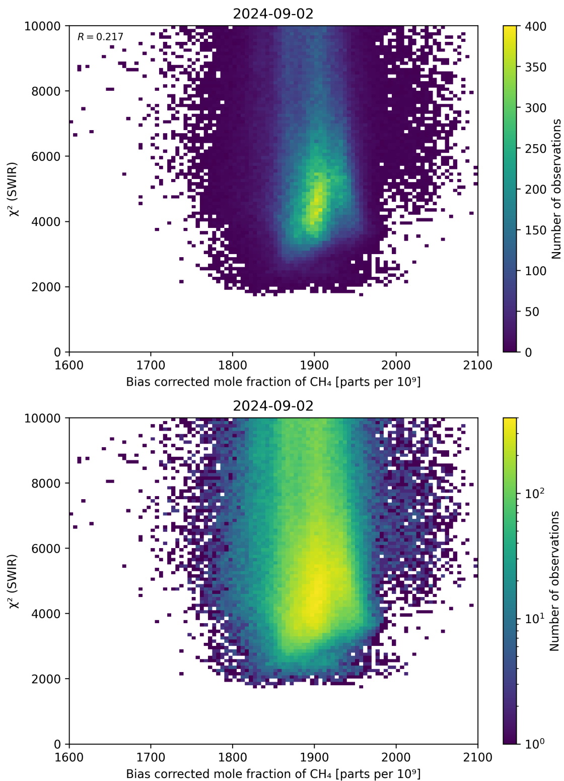
Figure 64: Scatter density plot of “Bias corrected mole fraction of \text{CH}_4 ” against “ \chi^2 (SWIR)” for 2024-09-01 to 2024-09-03.
