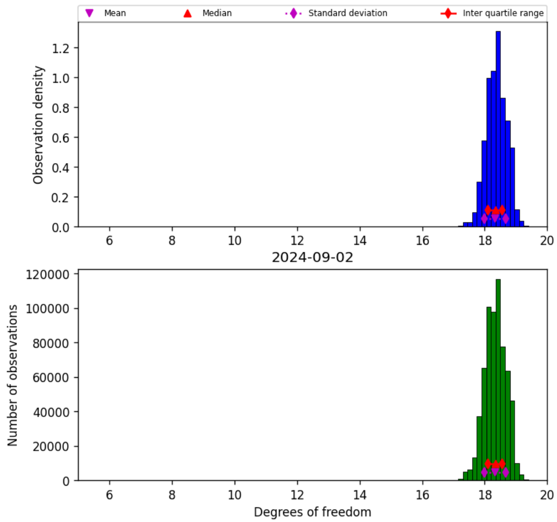
Figure 30: Histogram of “Degrees of freedom” for 2024-09-01 to 2024-09-03
