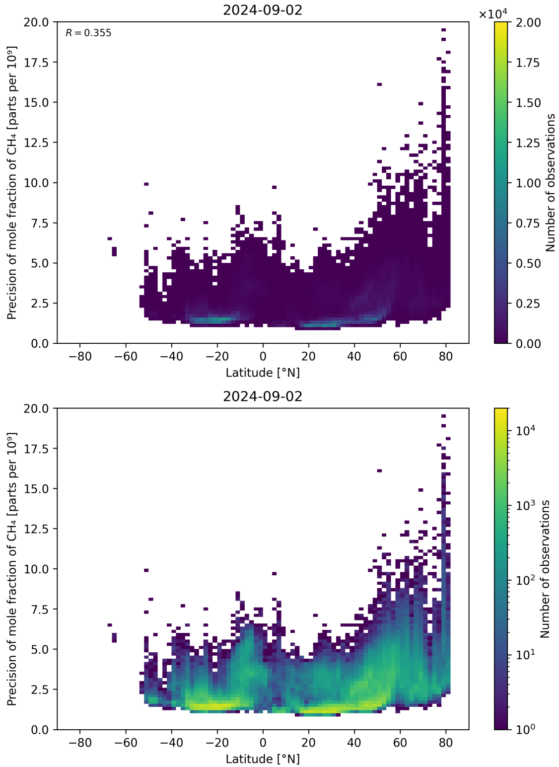
Figure 59: Scatter density plot of “Latitude” against “Precision of mole fraction of \text{CH}_4 ” for 2024-09-01 to 2024-09-03.
