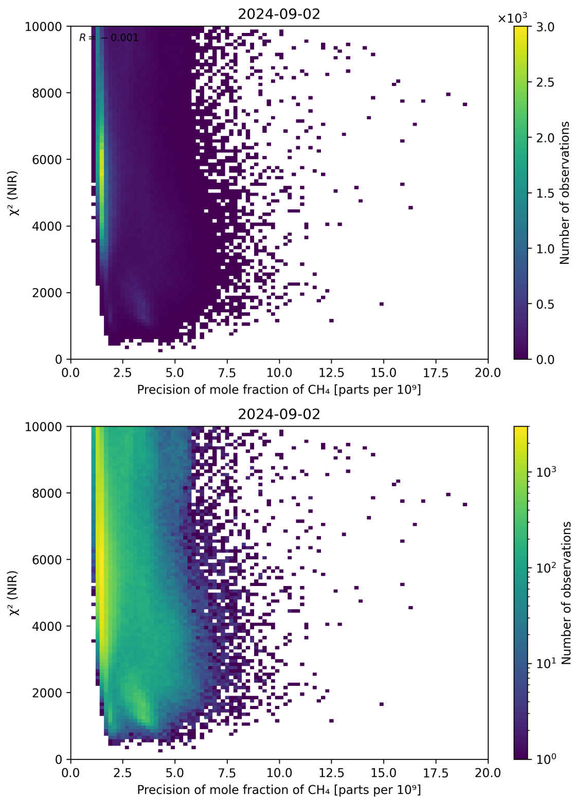
Figure 78: Scatter density plot of “Precision of mole fraction of CH 4 ” against “ \chi^2 (NIR)” for 2024-09-01 to 2024-09-03.
