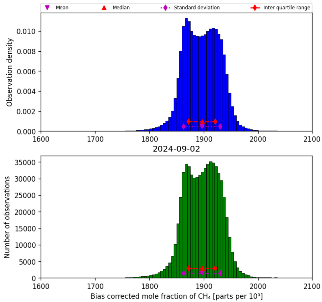
Figure 25: Histogram of “Bias corrected mole fraction of CH 4 ” for 2024-09-01 to 2024-09-03
