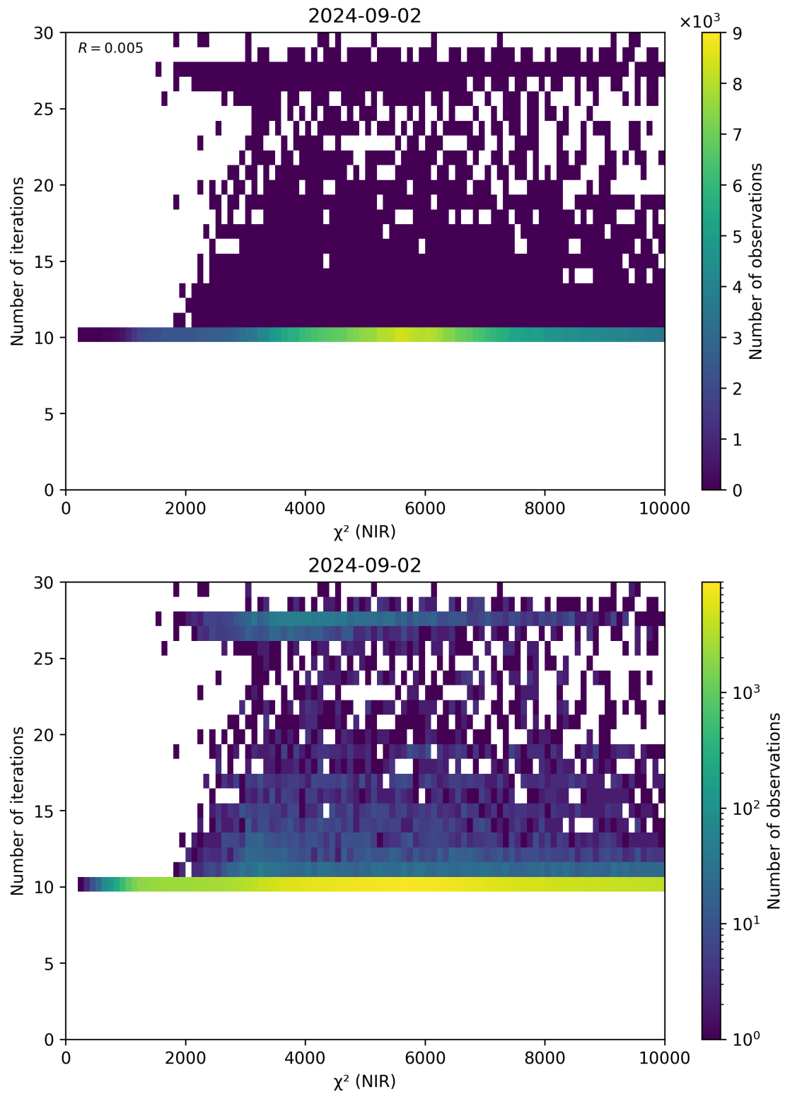
Figure 46: Scatter density plot of “ \chi^2 (NIR)” against “Number of iterations” for 2024-09-01 to 2024-09-03.
