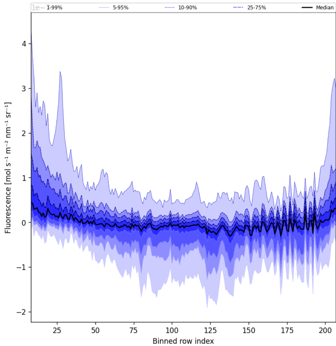
Figure 43: Along track statistics of “Fluorescence” for 2024-09-01 to 2024-09-03
