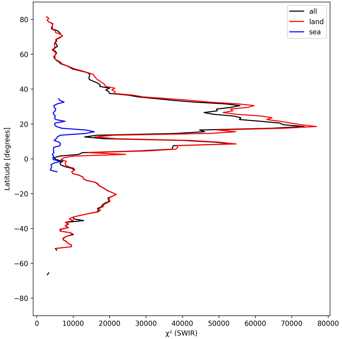
Figure 17: Zonal average of “ \chi^2 (SWIR)” for 2024-09-01 to 2024-09-03.
