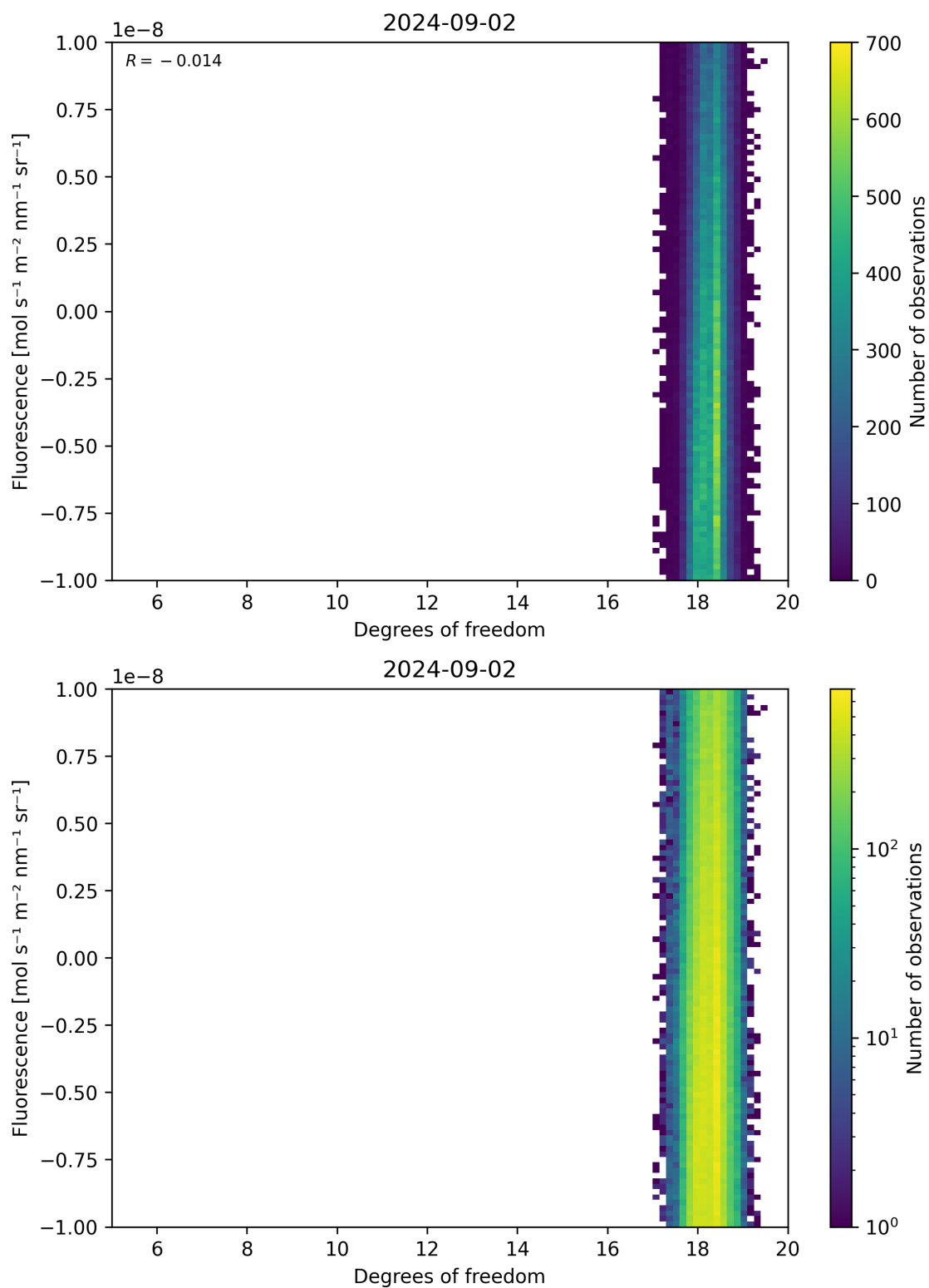
Figure 51: Scatter density plot of “Degrees of freedom” against “Fluorescence” for 2024-09-01 to 2024-09-03.
