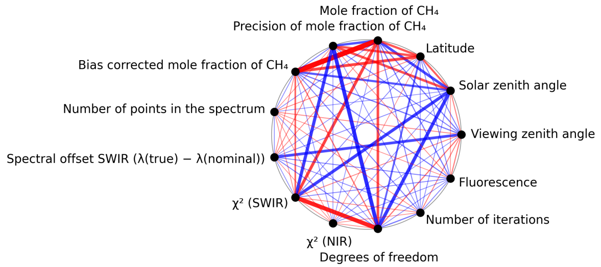
Figure 1: Map of correlation graph for 2024-09-01 to 2024-09-03.
