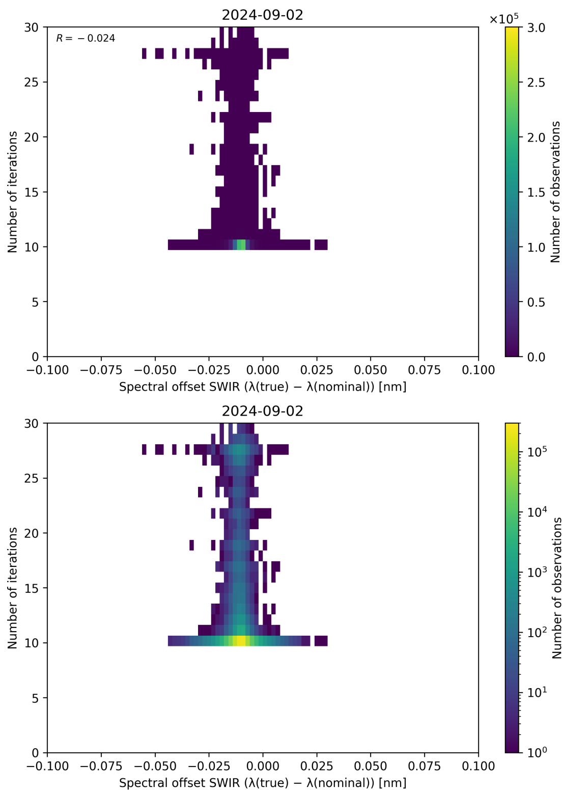
Figure 121: Scatter density plot of “Spectral offset SWIR ( \lambda_{\text{true}} - \lambda_{\text{nominal}} )” against “Number of iterations” for 2024-09-01 to 2024-09-03.
