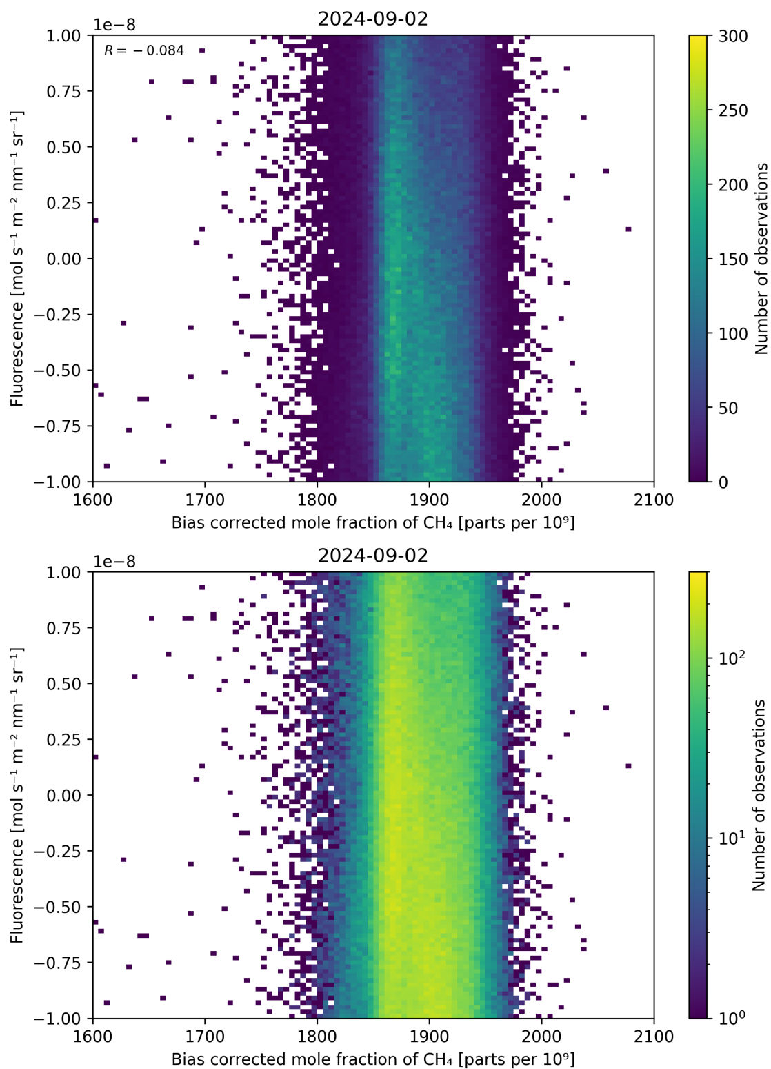
Figure 66: Scatter density plot of “Bias corrected mole fraction of \text{CH}_4 ” against “Fluorescence” for 2024-09-01 to 2024-09-03.
