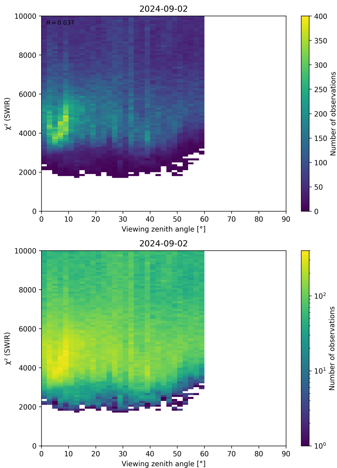
Figure 106: Scatter density plot of “Viewing zenith angle” against “ \chi^2 (SWIR)” for 2024-09-01 to 2024-09-03.
