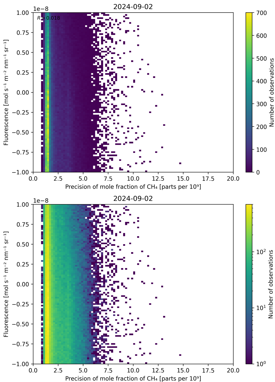
Figure 81: Scatter density plot of “Precision of mole fraction of \text{CH}_4 ” against “Fluorescence” for 2024-09-01 to 2024-09-03.
