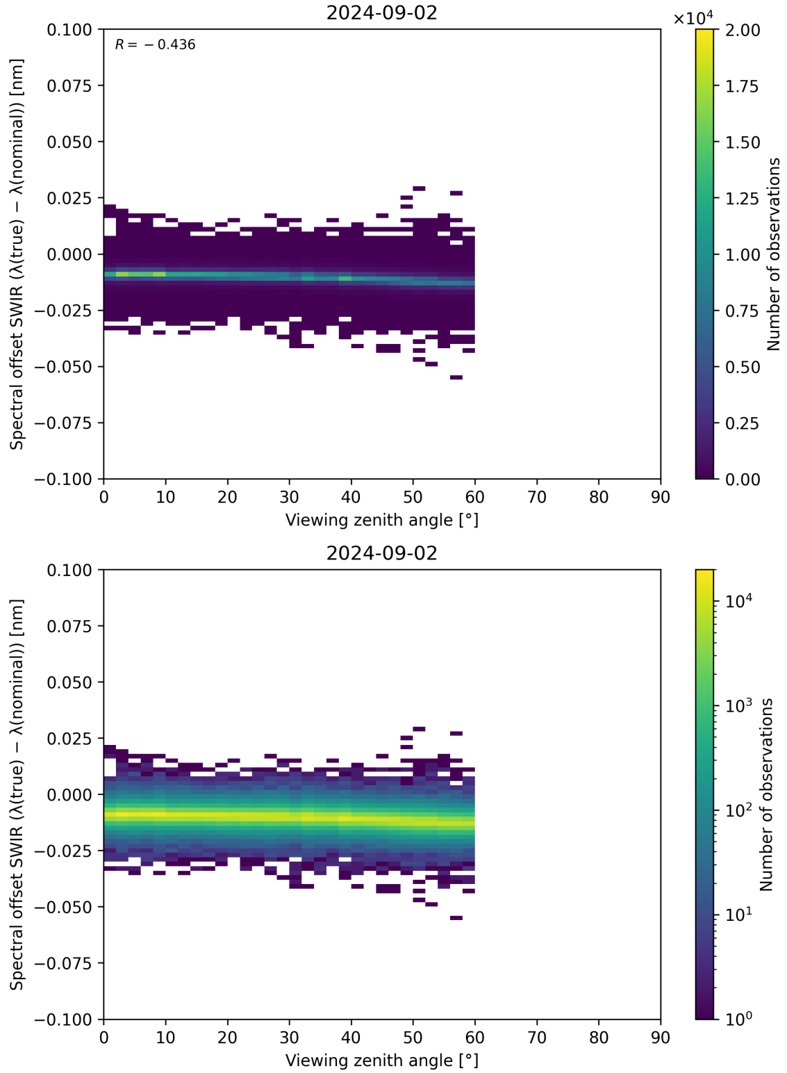
Figure 116: Scatter density plot of “Viewing zenith angle” against “Spectral offset SWIR ( \lambda_{\text{true}} - \lambda_{\text{nominal}} )” for 2024-09-01 to 2024-09-03.
