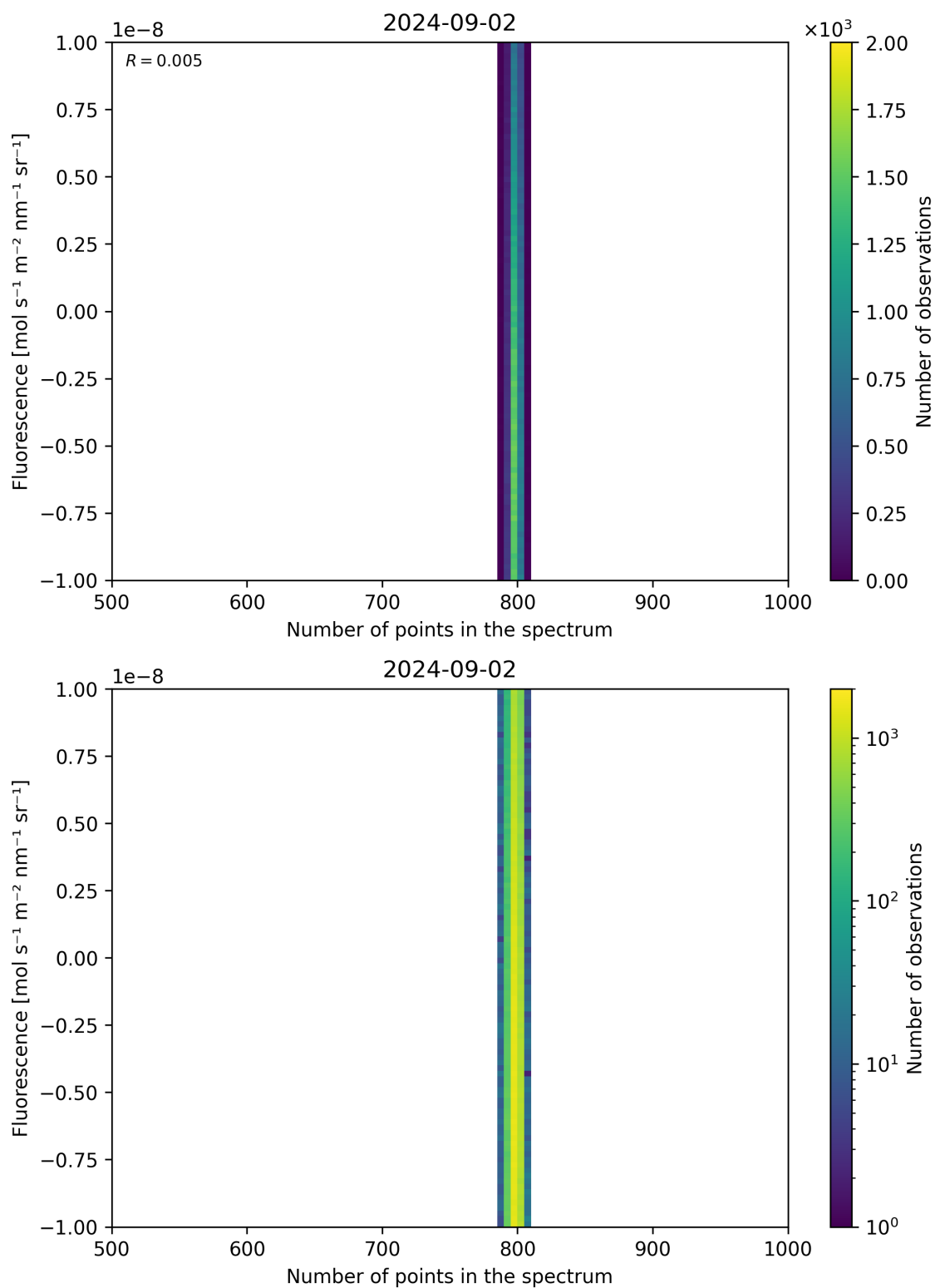
Figure 91: Scatter density plot of “Number of points in the spectrum” against “Fluorescence” for 2024-09-01 to 2024-09-03.
