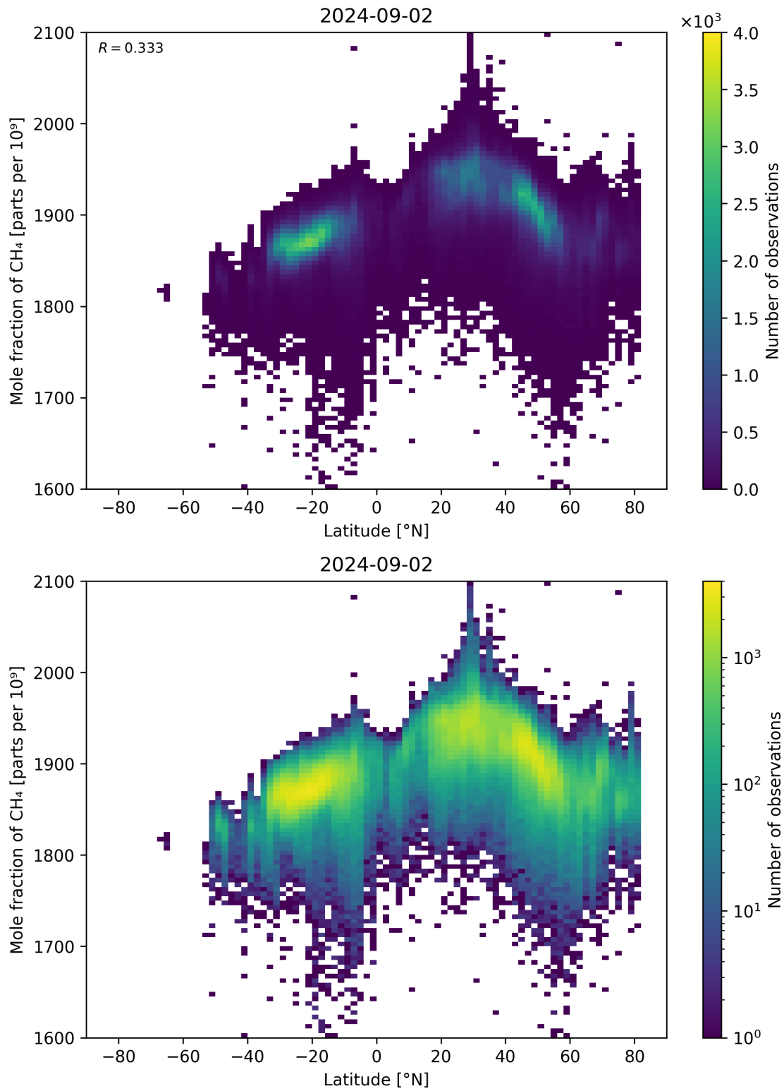
Figure 57: Scatter density plot of “Latitude” against “Mole fraction of CH 4 ” for 2024-09-01 to 2024-09-03.
