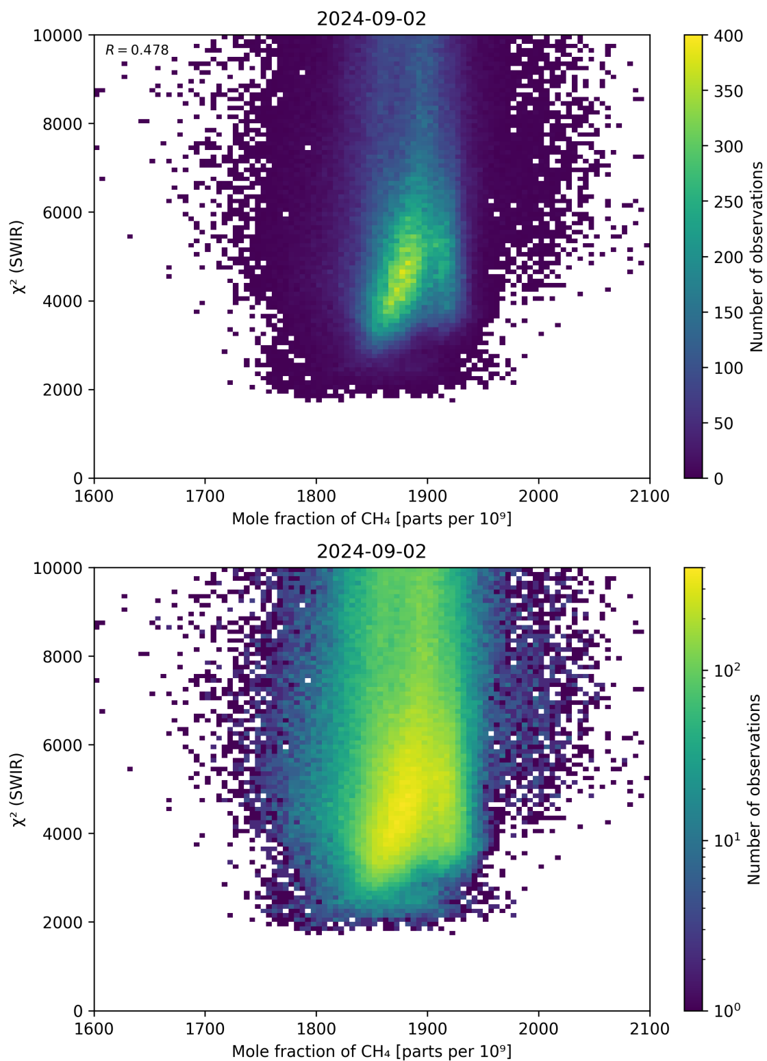
Figure 71: Scatter density plot of “Mole fraction of \text{CH}_4 ” against “ \chi^2 (SWIR)” for 2024-09-01 to 2024-09-03.
