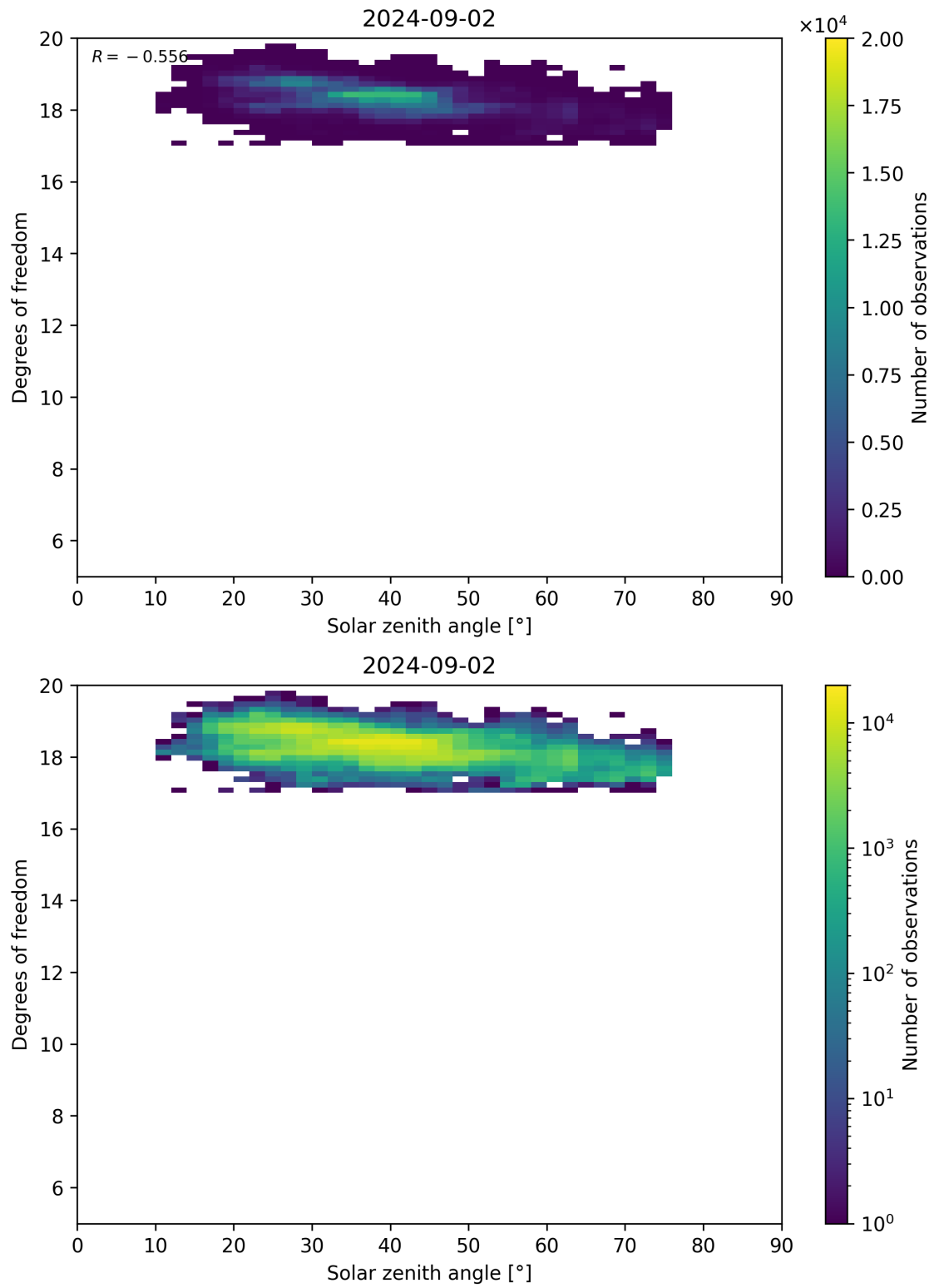
Figure 96: Scatter density plot of “Solar zenith angle” against “Degrees of freedom” for 2024-09-01 to 2024-09-03.
