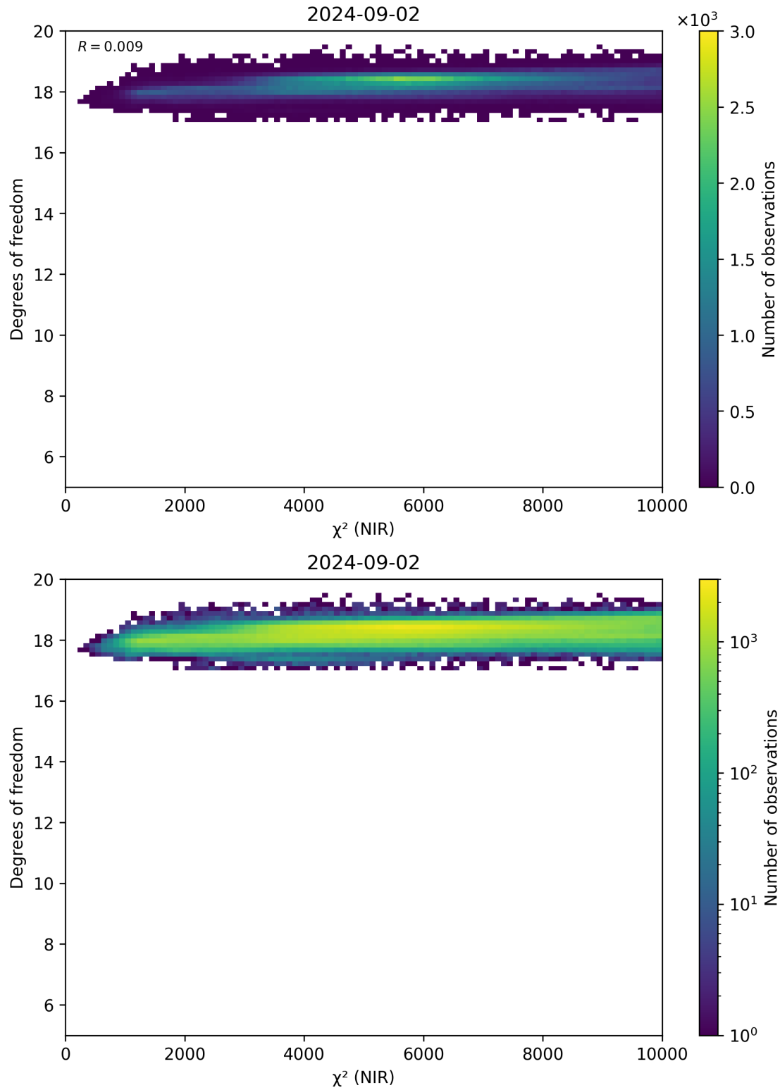
Figure 44: Scatter density plot of “ \chi^2 (NIR)” against “Degrees of freedom” for 2024-09-01 to 2024-09-03.
