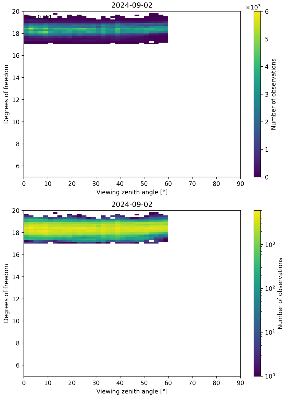
Figure 107: Scatter density plot of “Viewing zenith angle” against “Degrees of freedom” for 2024-09-01 to 2024-09-03.
