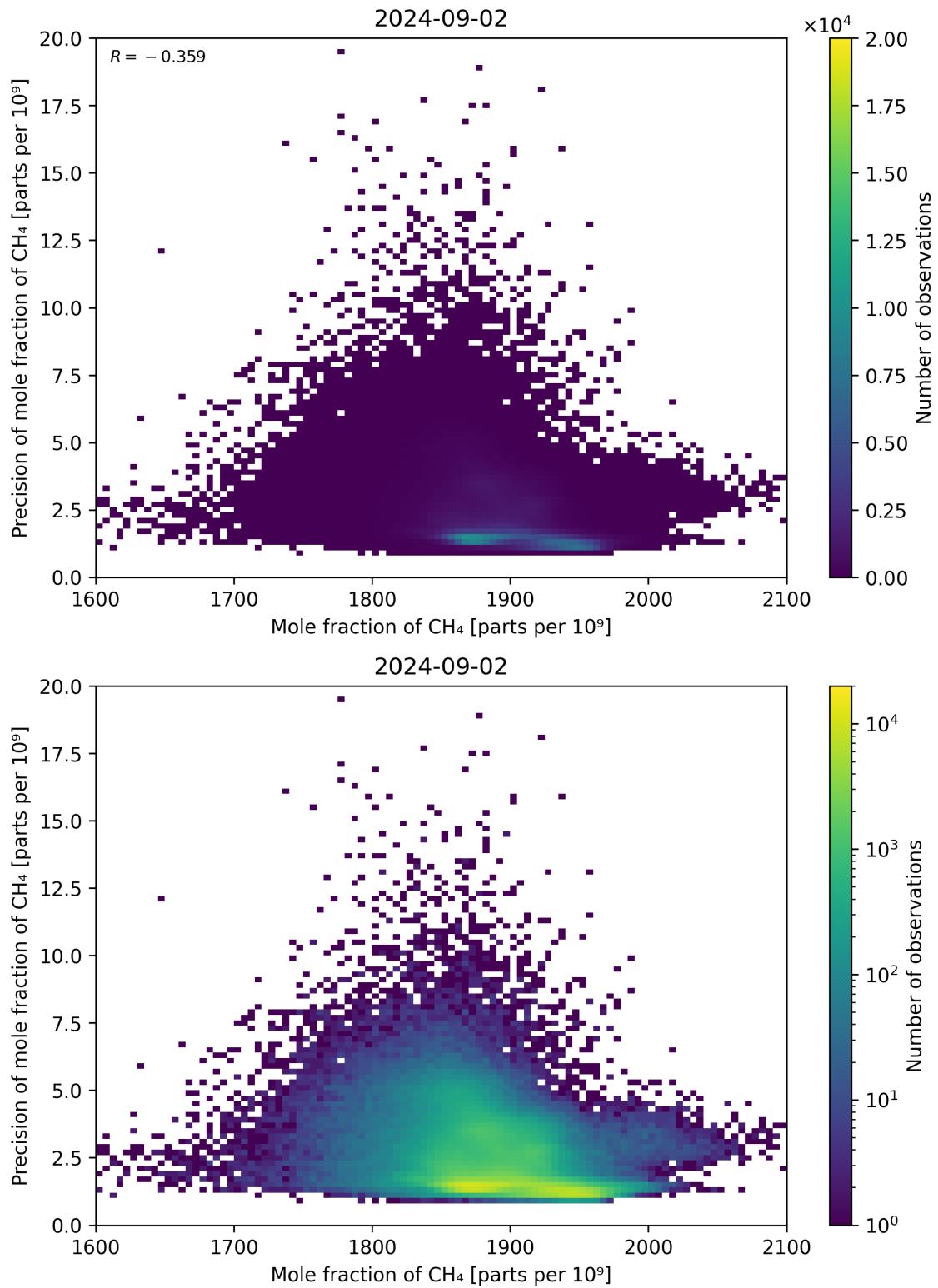
Figure 75: Scatter density plot of “Mole fraction of CH 4 ” against “Precision of mole fraction of CH 4 ” for 2024-09-01 to 2024-09-03.
