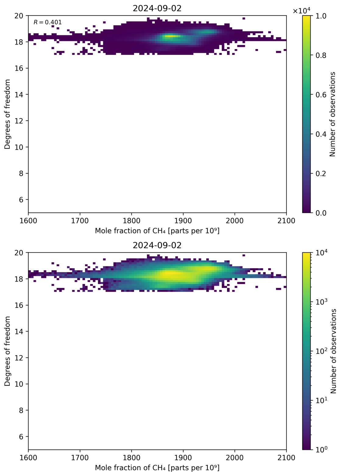
Figure 72: Scatter density plot of “Mole fraction of CH 4 ” against “Degrees of freedom” for 2024-09-01 to 2024-09-03.
