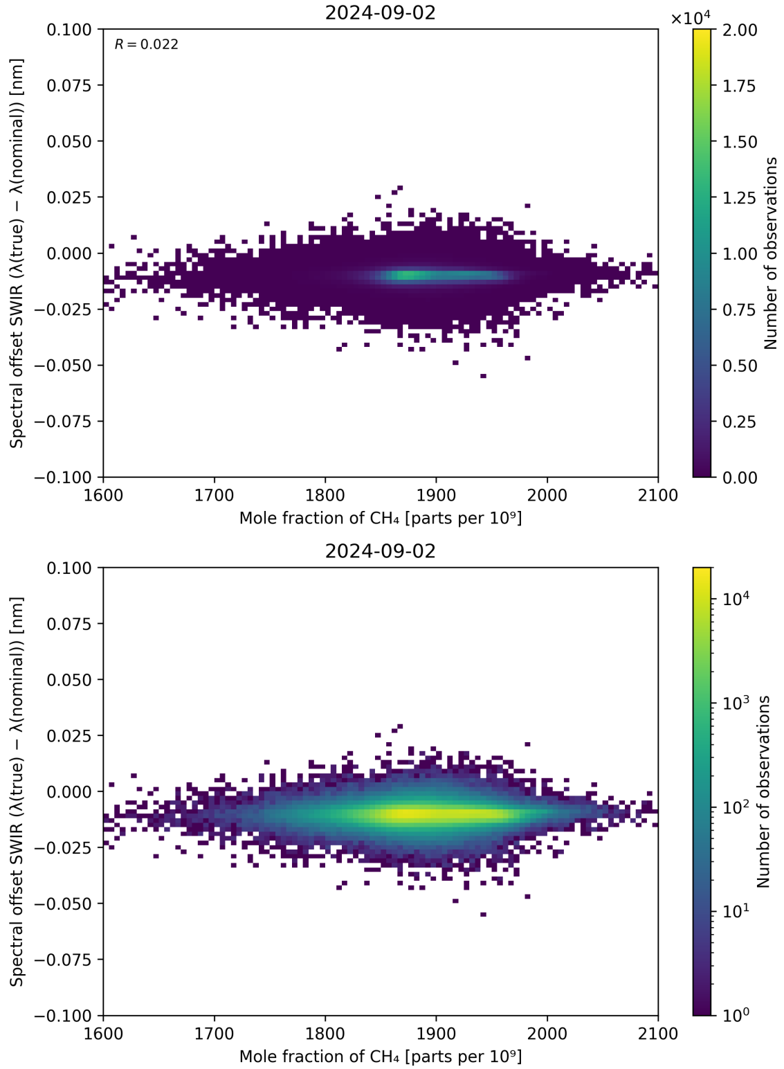
Figure 86: Scatter density plot of “Mole fraction of \text{CH}_4 ” against “Spectral offset SWIR ( \lambda_{\text{true}} - \lambda_{\text{nominal}} )” for 2024-09-01 to 2024-09-03.
