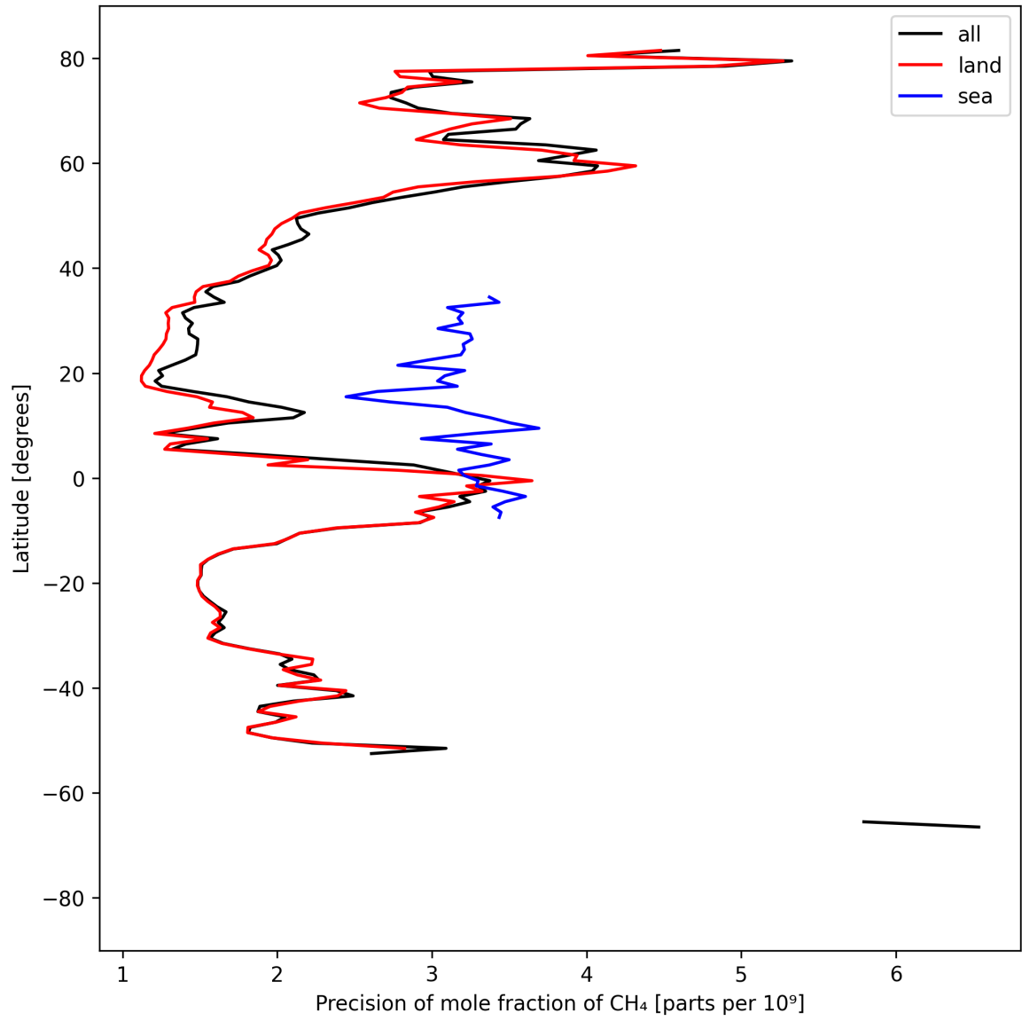
Figure 13: Zonal average of “Precision of mole fraction of CH 4 ” for 2024-09-01 to 2024-09-03.
