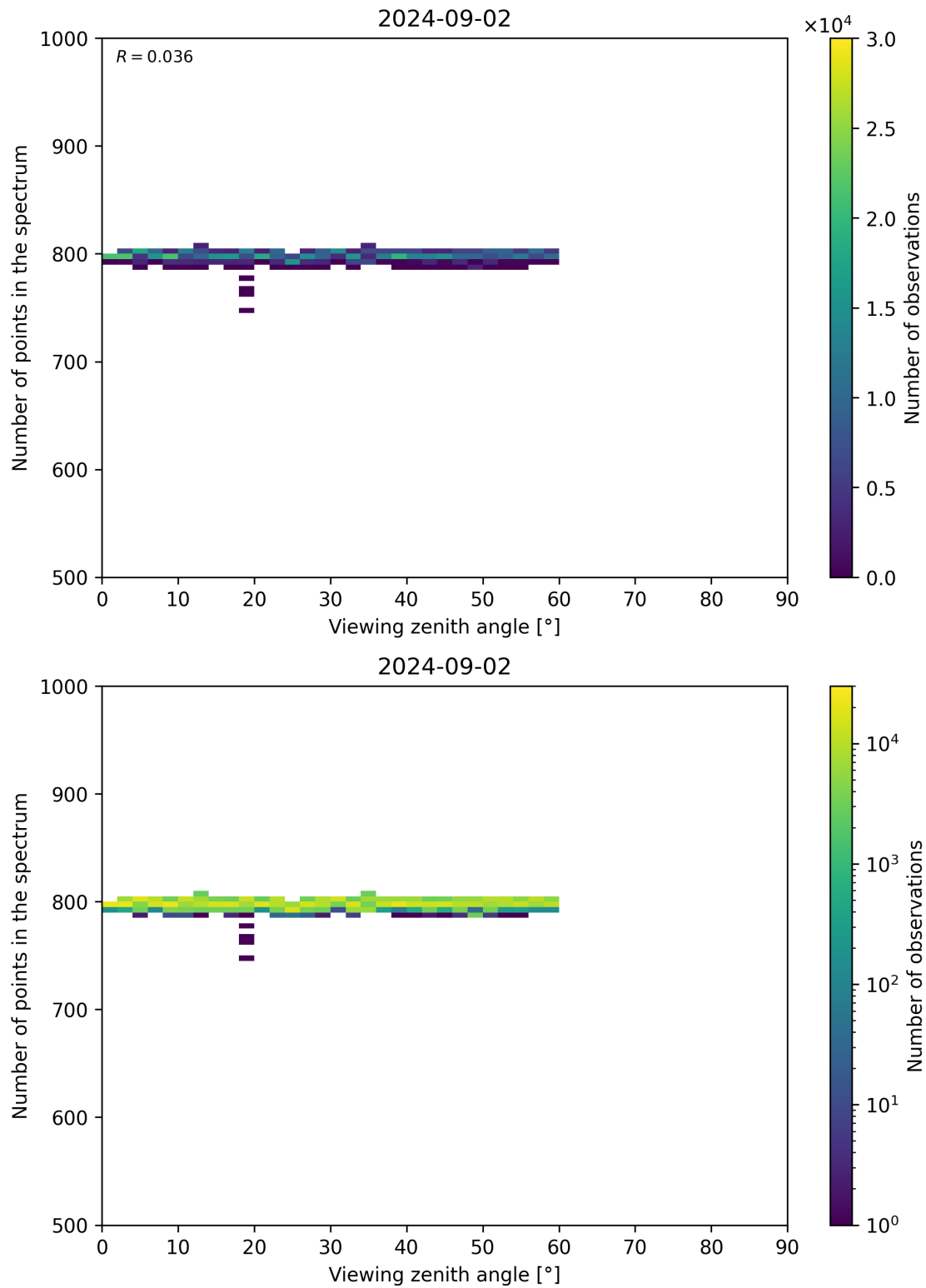
Figure 114: Scatter density plot of “Viewing zenith angle” against “Number of points in the spectrum” for 2024-09-01 to 2024-09-03.
