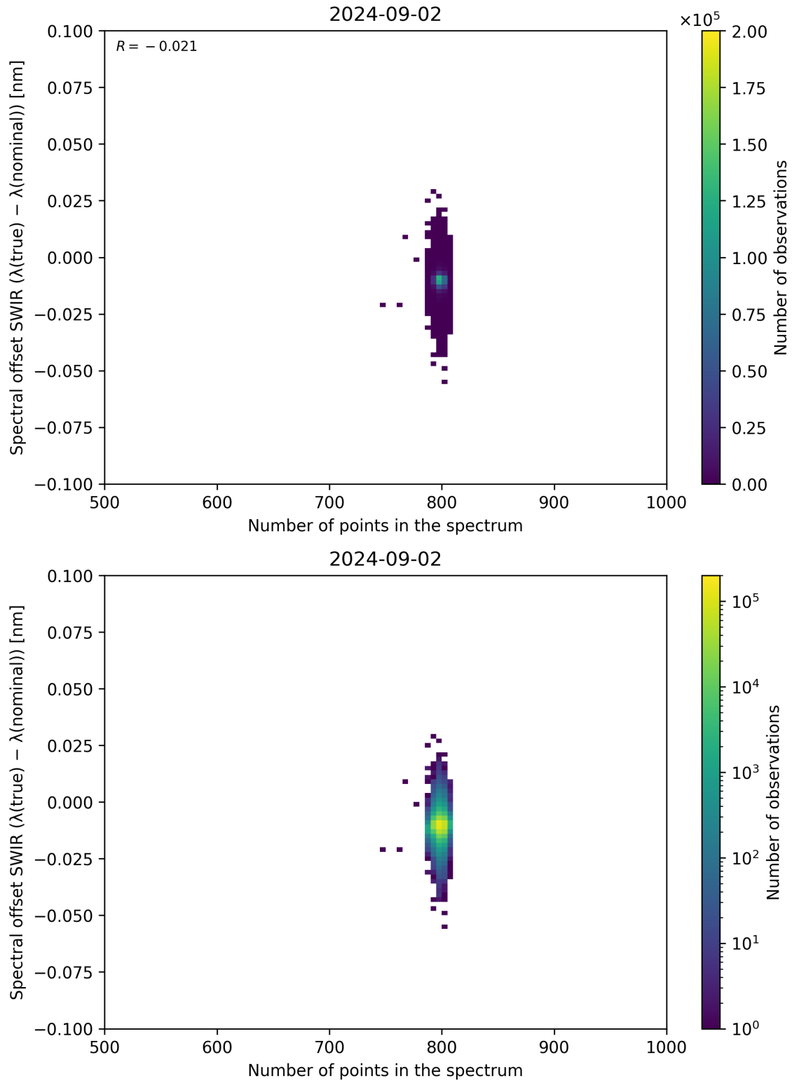
Figure 93: Scatter density plot of “Number of points in the spectrum” against “Spectral offset SWIR ( \lambda_{\text{true}} - \lambda_{\text{nominal}} )” for 2024-09-01 to 2024-09-03.
