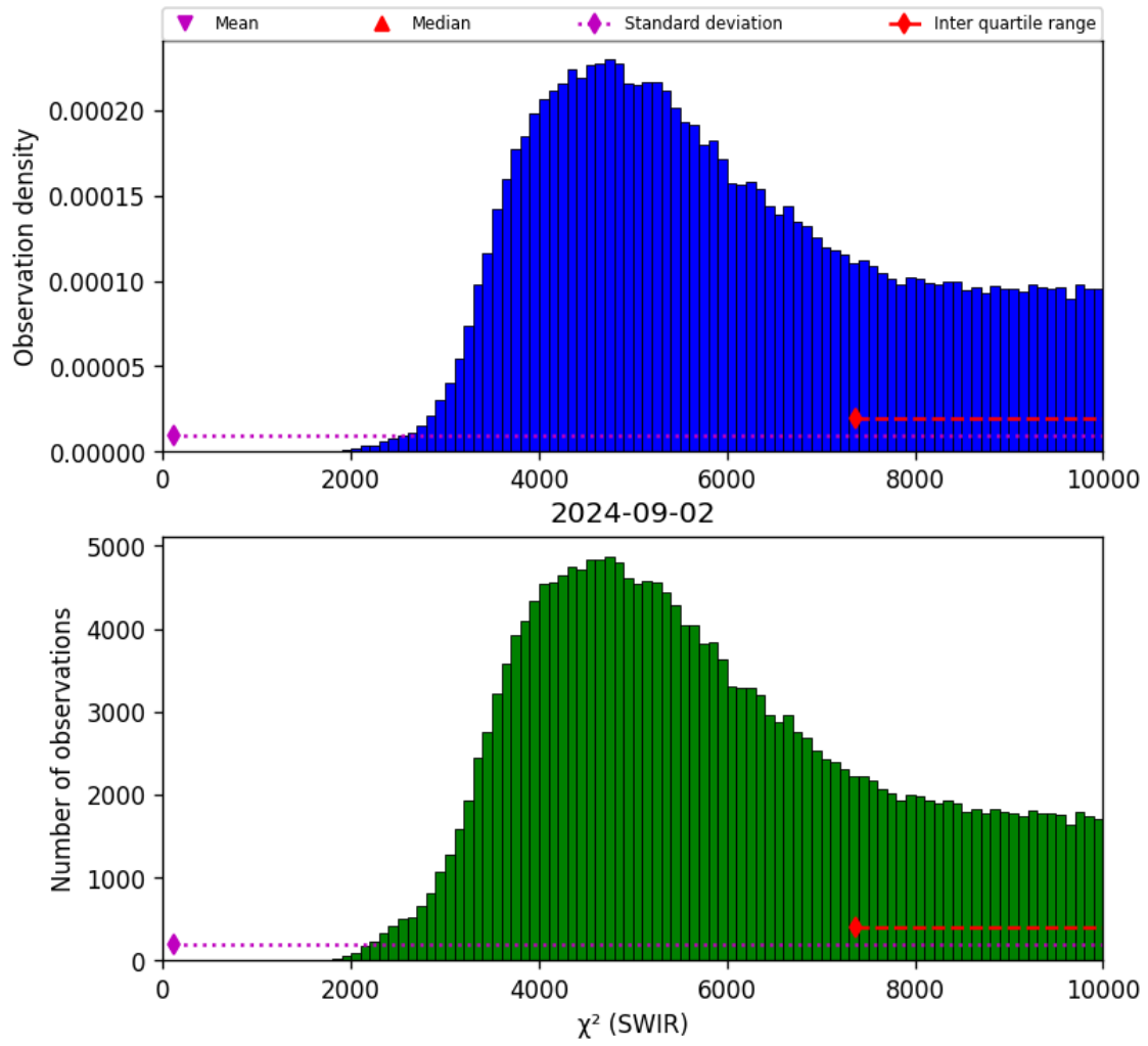
Figure 28: Histogram of “ \chi^2 (SWIR)” for 2024-09-01 to 2024-09-03
