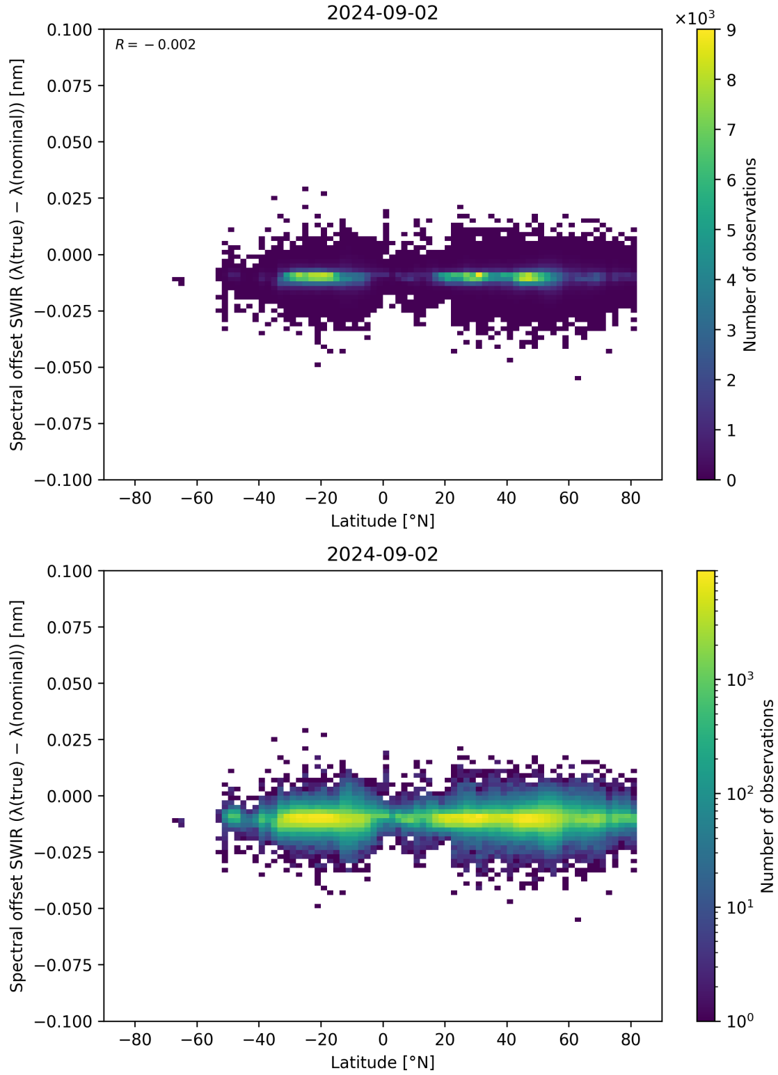
Figure 62: Scatter density plot of “Latitude” against “Spectral offset SWIR ( \lambda_{\text{true}} - \lambda_{\text{nominal}} )” for 2024-09-01 to 2024-09-03.
