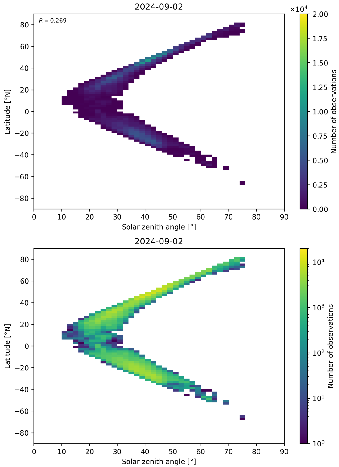
Figure 98: Scatter density plot of “Solar zenith angle” against “Latitude” for 2024-09-01 to 2024-09-03.
