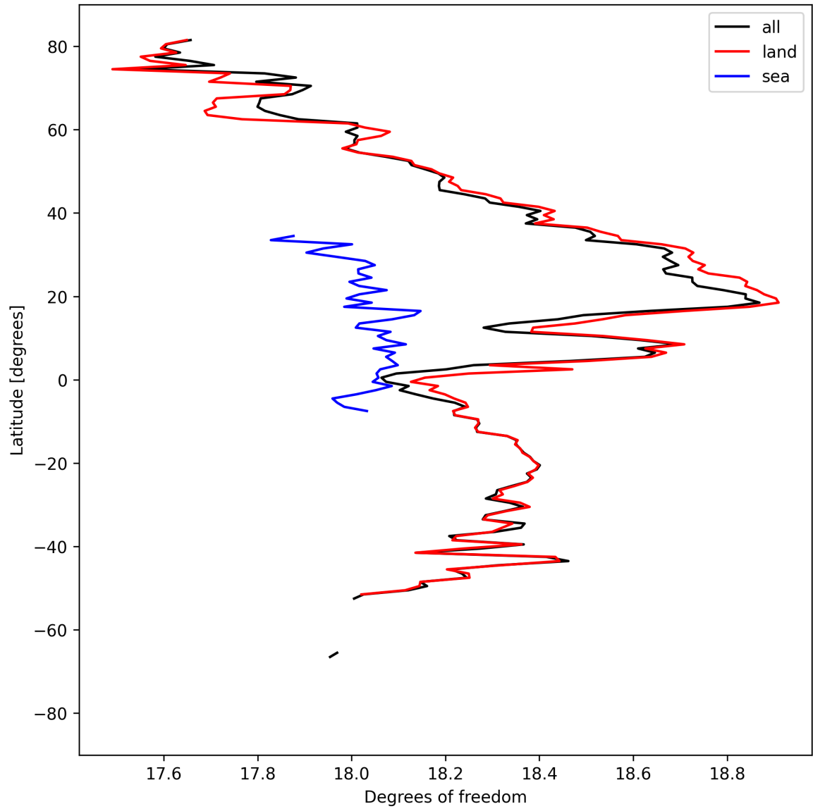
Figure 19: Zonal average of “Degrees of freedom” for 2024-09-01 to 2024-09-03.
