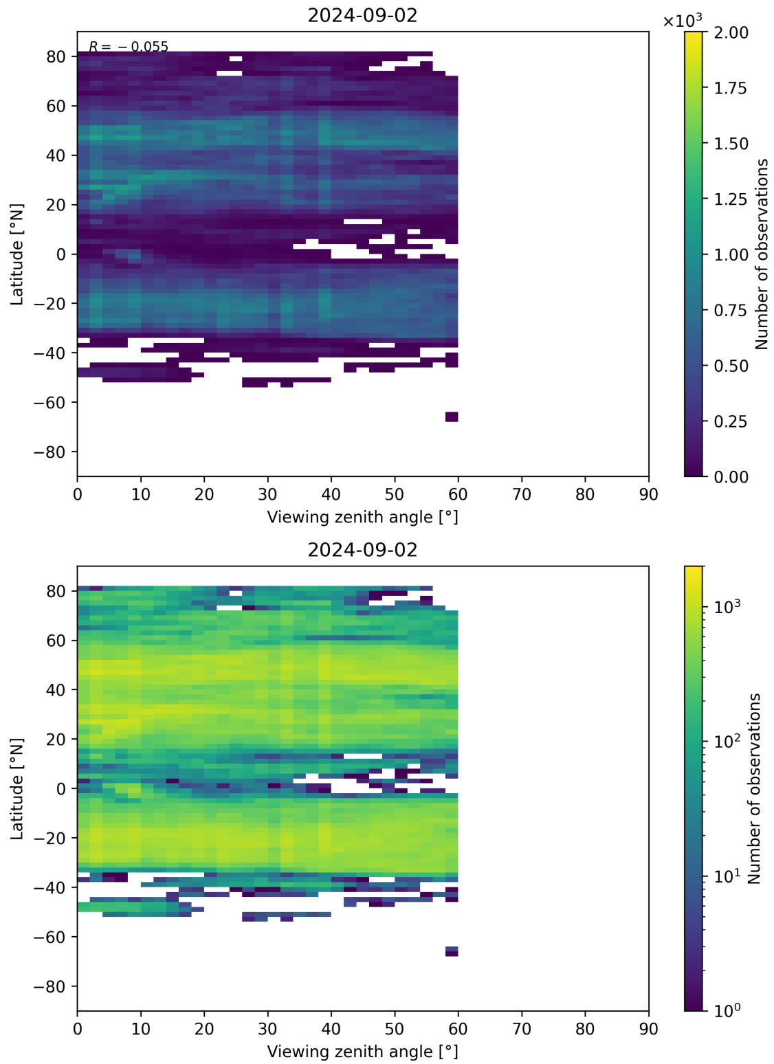
Figure 109: Scatter density plot of “Viewing zenith angle” against “Latitude” for 2024-09-01 to 2024-09-03.
