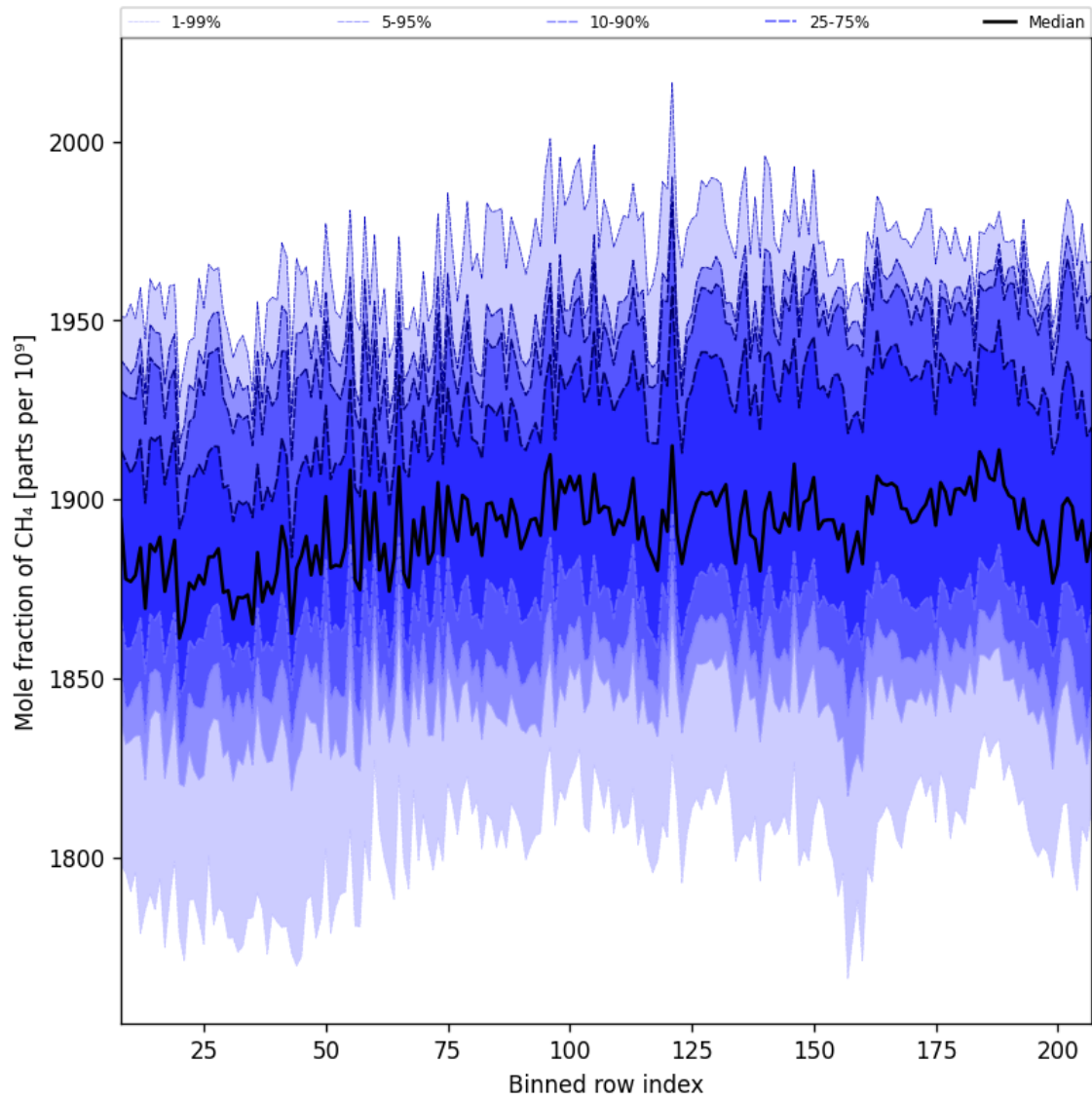
Figure 34: Along track statistics of “Mole fraction of CH 4 ” for 2024-09-01 to 2024-09-03
