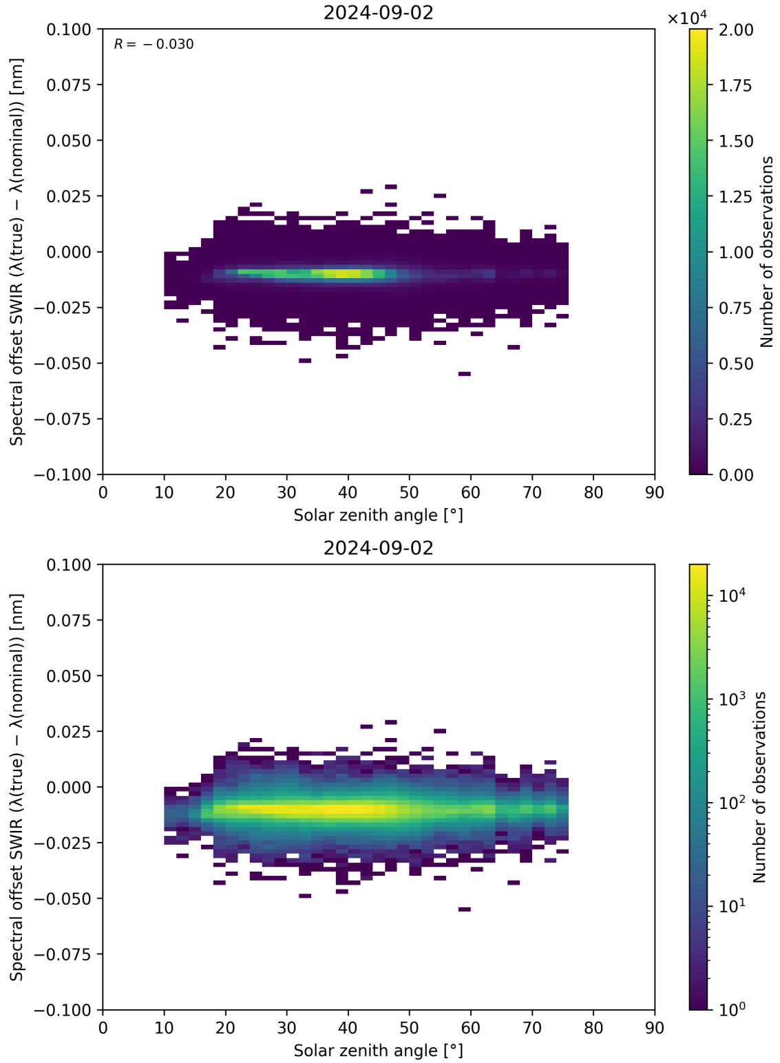
Figure 104: Scatter density plot of “Solar zenith angle” against “Spectral offset SWIR ( \lambda_{\text{true}} - \lambda_{\text{nominal}} )” for 2024-09-01 to 2024-09-03.
