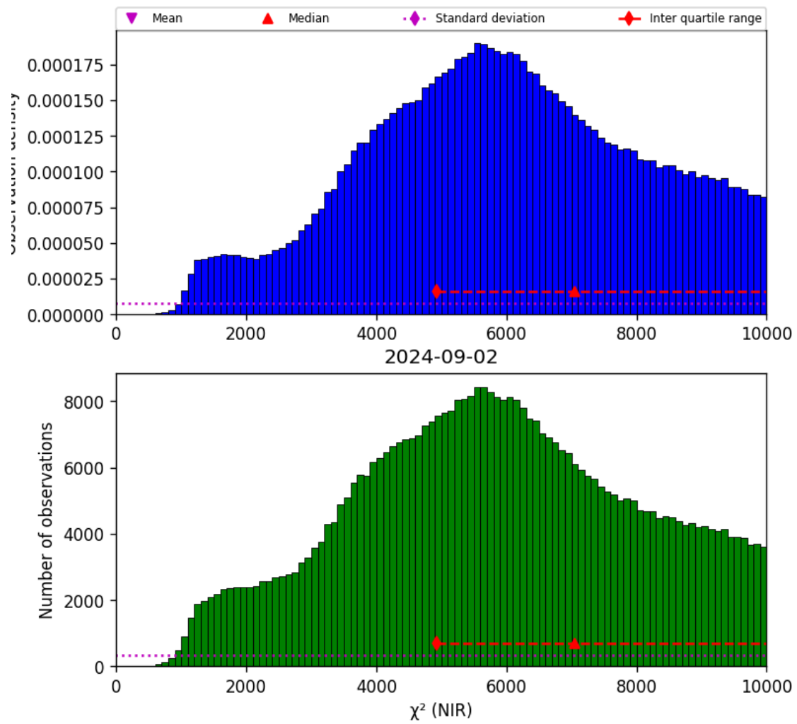
Figure 29: Histogram of “ \chi^2 (NIR)” for 2024-09-01 to 2024-09-03
