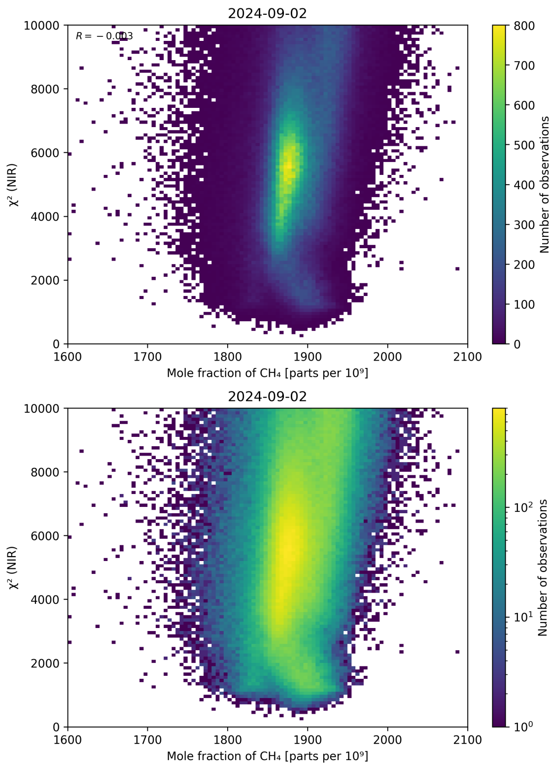
Figure 70: Scatter density plot of “Mole fraction of \text{CH}_4 ” against “ \chi^2 (NIR)” for 2024-09-01 to 2024-09-03.
