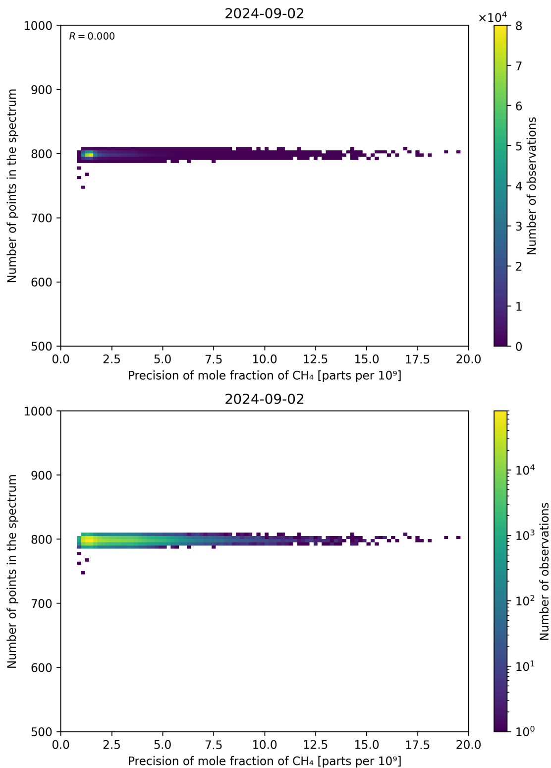
Figure 84: Scatter density plot of “Precision of mole fraction of CH 4 ” against “Number of points in the spectrum” for 2024-09-01 to 2024-09-03.
