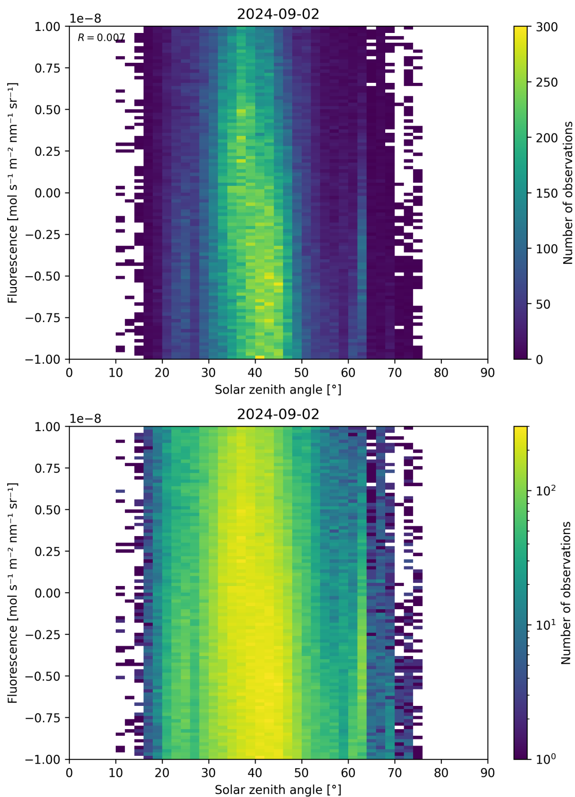
Figure 97: Scatter density plot of “Solar zenith angle” against “Fluorescence” for 2024-09-01 to 2024-09-03.
