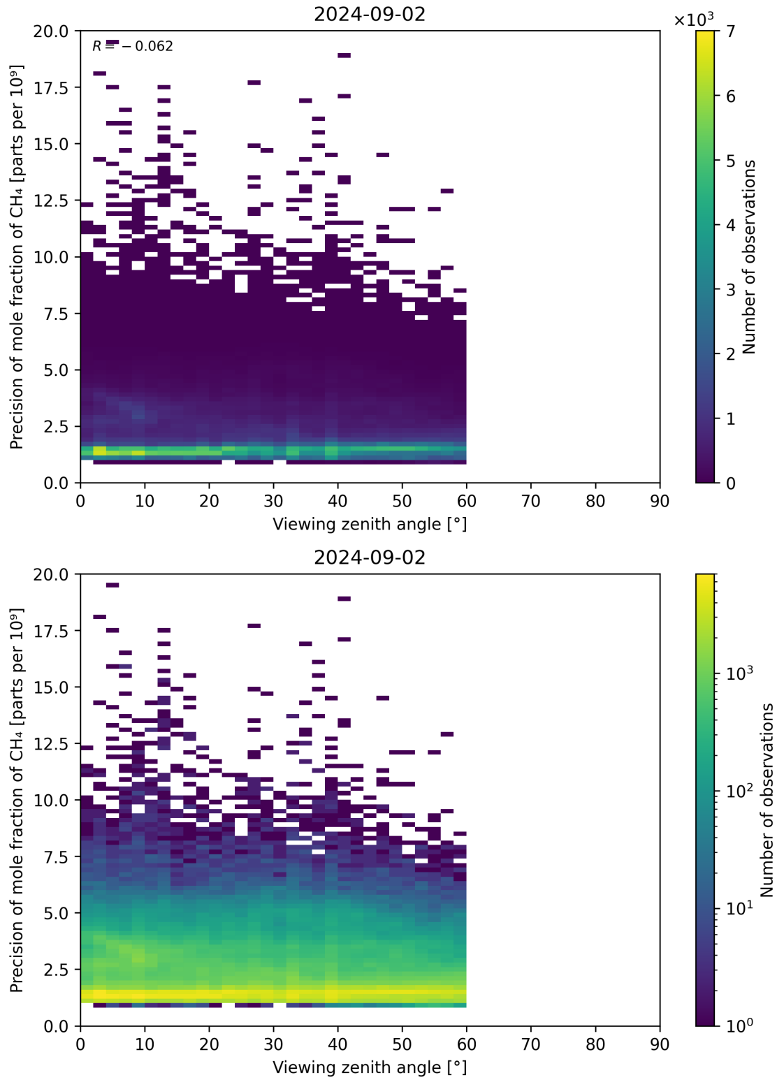
Figure 112: Scatter density plot of “Viewing zenith angle” against “Precision of mole fraction of CH 4 ” for 2024-09-01 to 2024-09-03.
