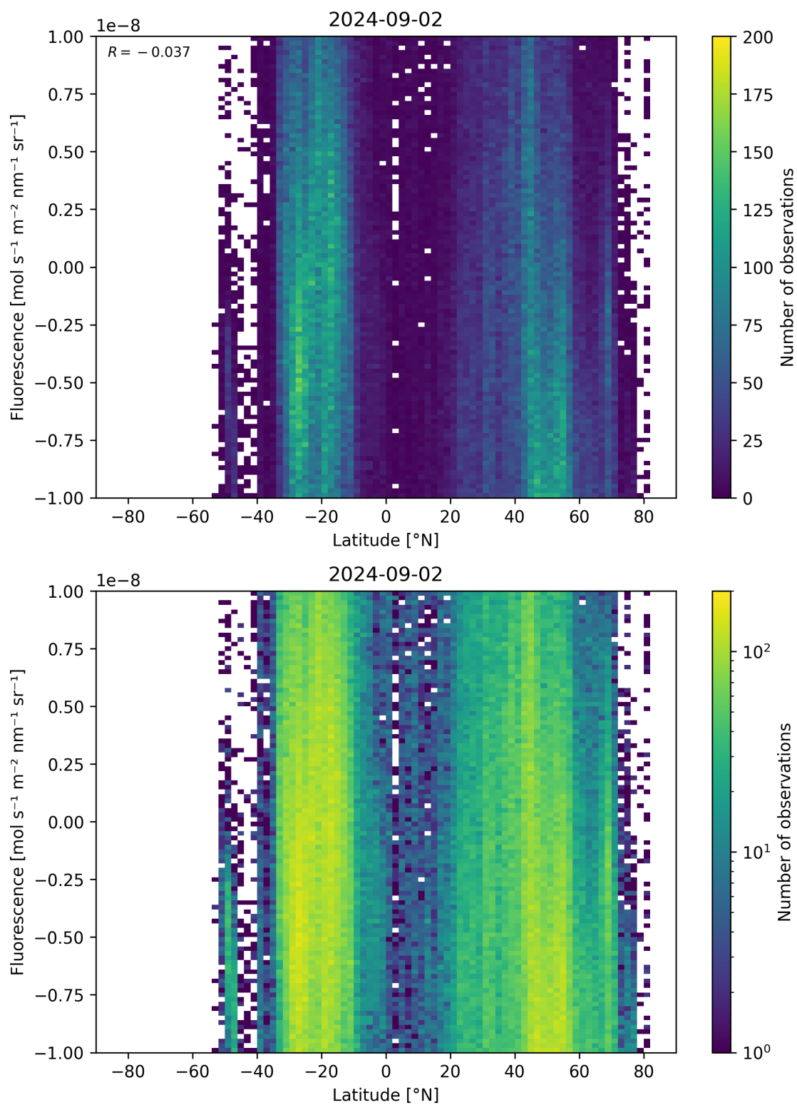
Figure 56: Scatter density plot of “Latitude” against “Fluorescence” for 2024-09-01 to 2024-09-03.
