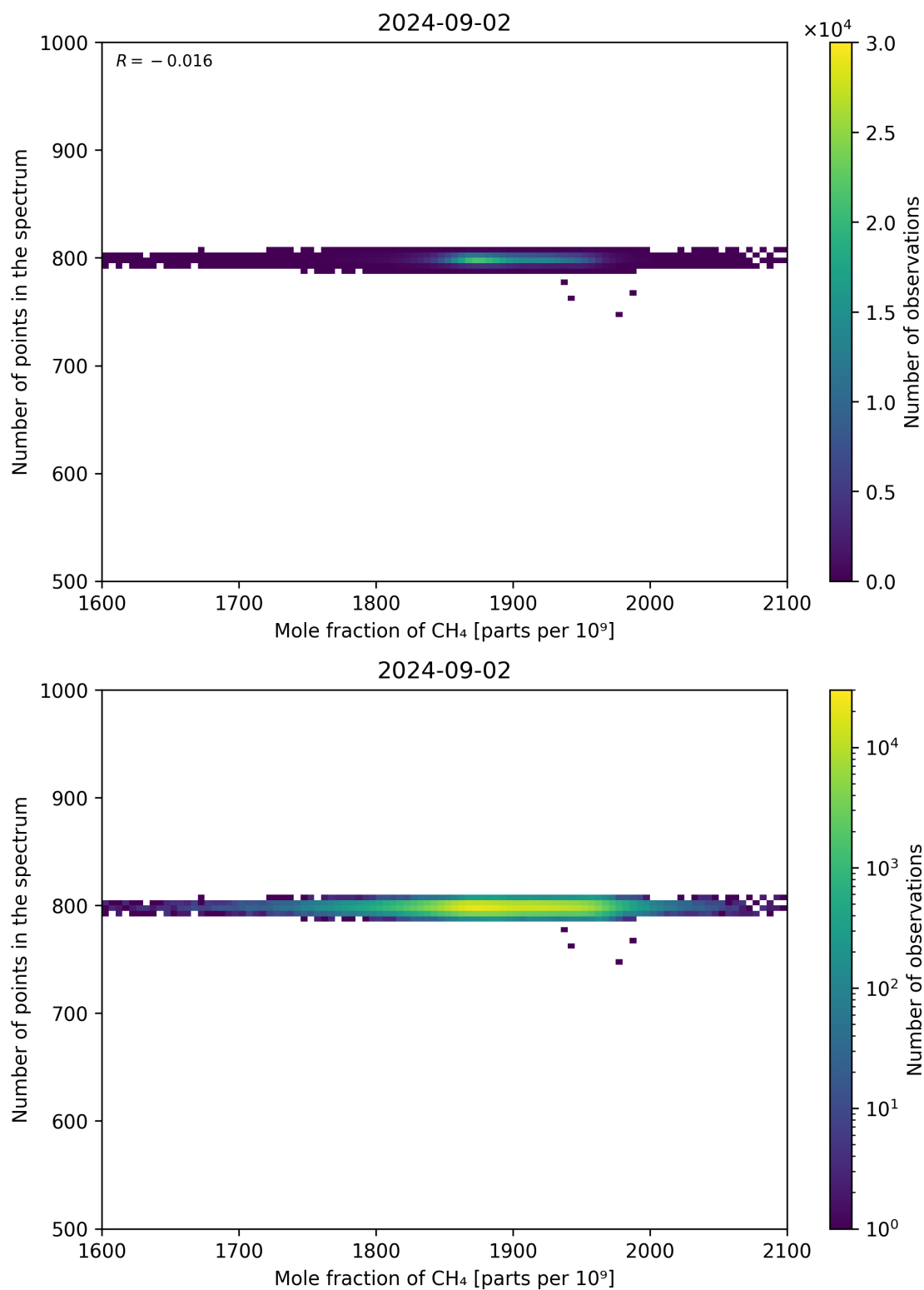
Figure 77: Scatter density plot of “Mole fraction of CH 4 ” against “Number of points in the spectrum” for 2024-09-01 to 2024-09-03.
