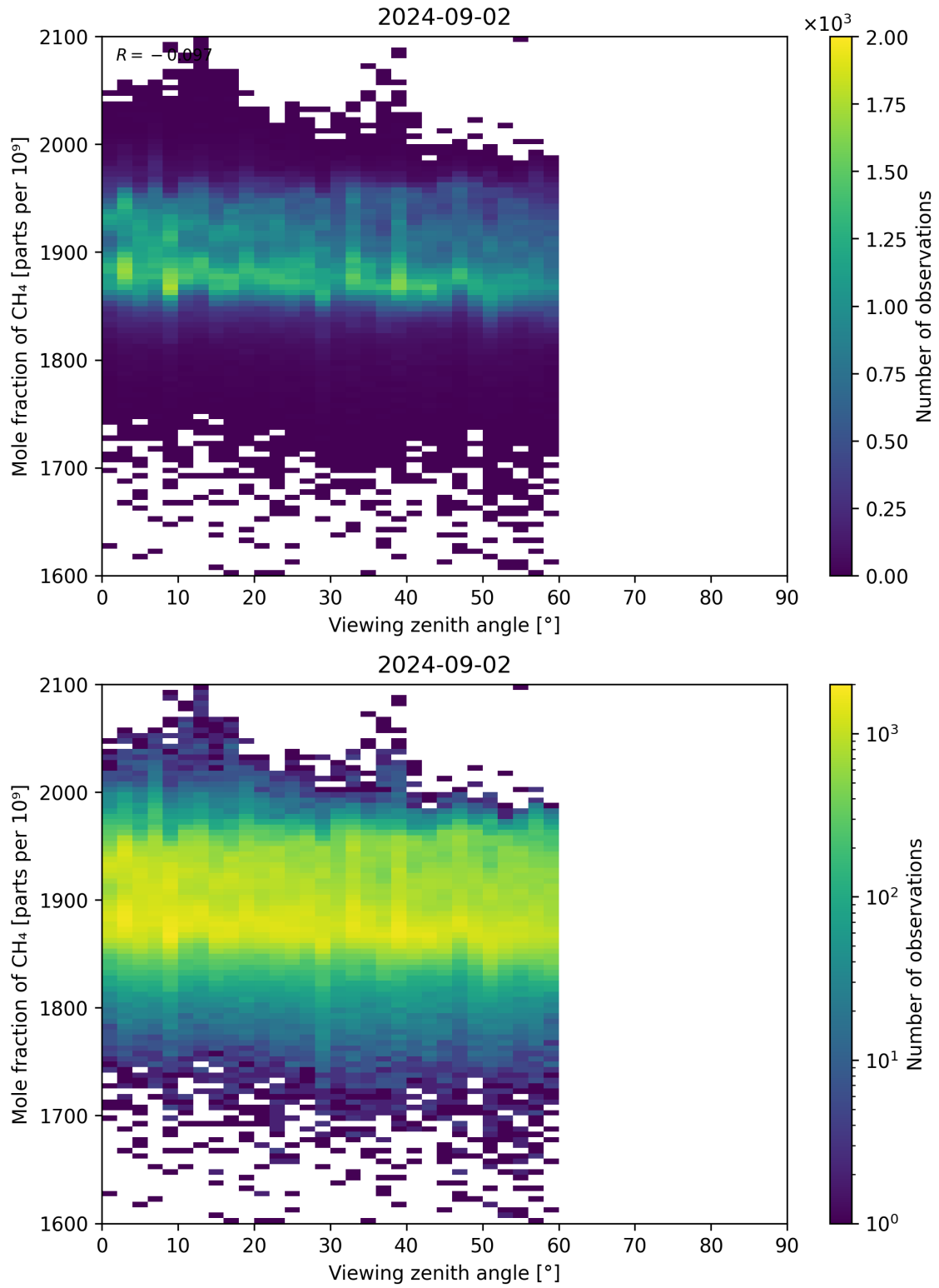
Figure 110: Scatter density plot of “Viewing zenith angle” against “Mole fraction of CH 4 ” for 2024-09-01 to 2024-09-03.
