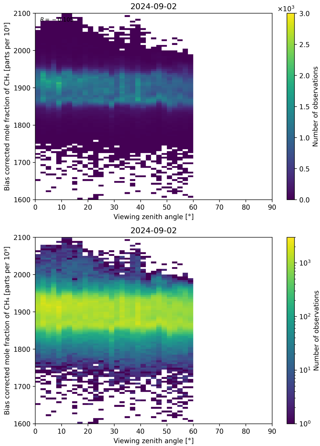
Figure 111: Scatter density plot of “Viewing zenith angle” against “Bias corrected mole fraction of CH 4 ” for 2024-09-01 to 2024-09-03.
