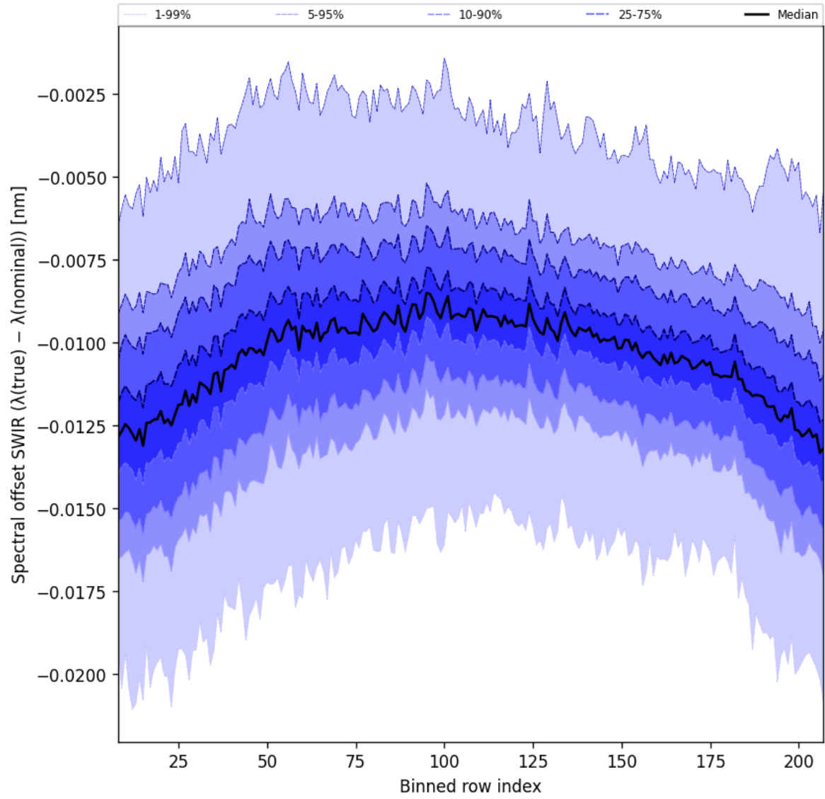
Figure 38: Along track statistics of “Spectral offset SWIR ( \lambda_{\text{true}} - \lambda_{\text{nominal}} )” for 2024-09-01 to 2024-09-03
