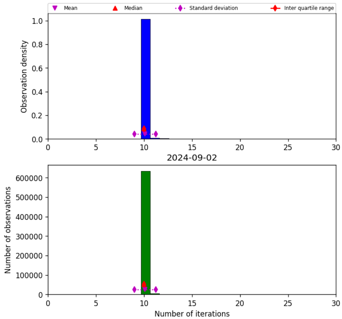
Figure 31: Histogram of “Number of iterations” for 2024-09-01 to 2024-09-03
