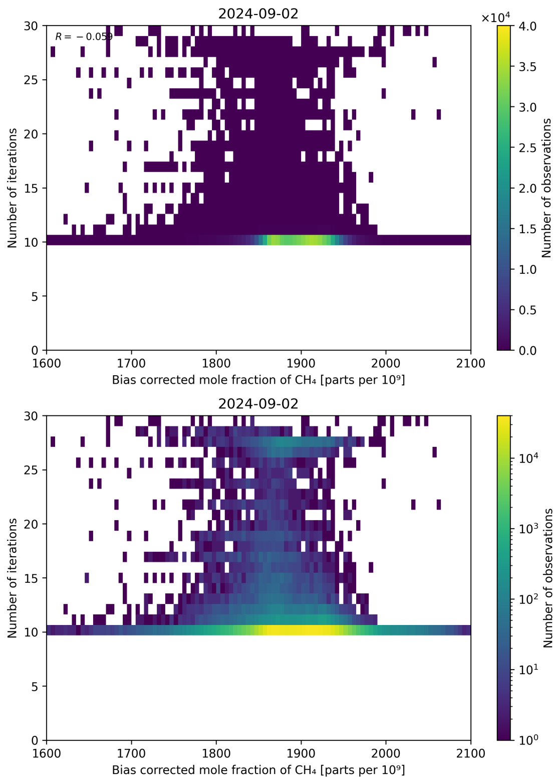
Figure 67: Scatter density plot of “Bias corrected mole fraction of \text{CH}_4 ” against “Number of iterations” for 2024-09-01 to 2024-09-03.
