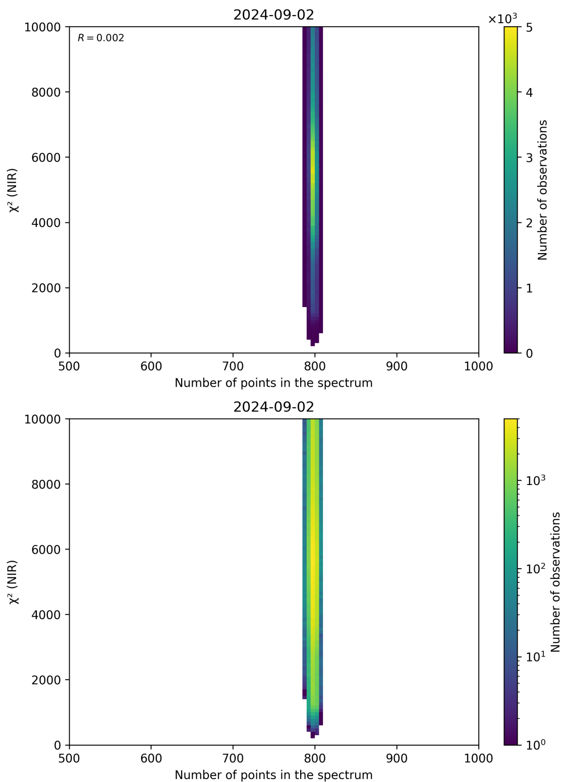
Figure 88: Scatter density plot of “Number of points in the spectrum” against “ \chi^2 (NIR)” for 2024-09-01 to 2024-09-03.
