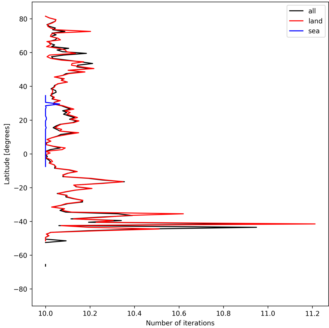
Figure 20: Zonal average of “Number of iterations” for 2024-09-01 to 2024-09-03.
