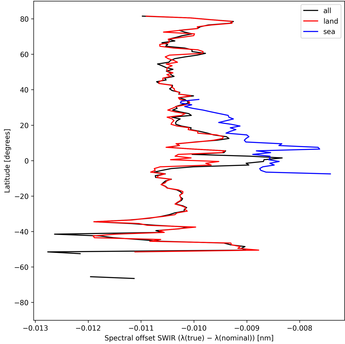
Figure 16: Zonal average of “Spectral offset SWIR ( \lambda_{\text{true}} - \lambda_{\text{nominal}} )” for 2024-09-01 to 2024-09-03.
