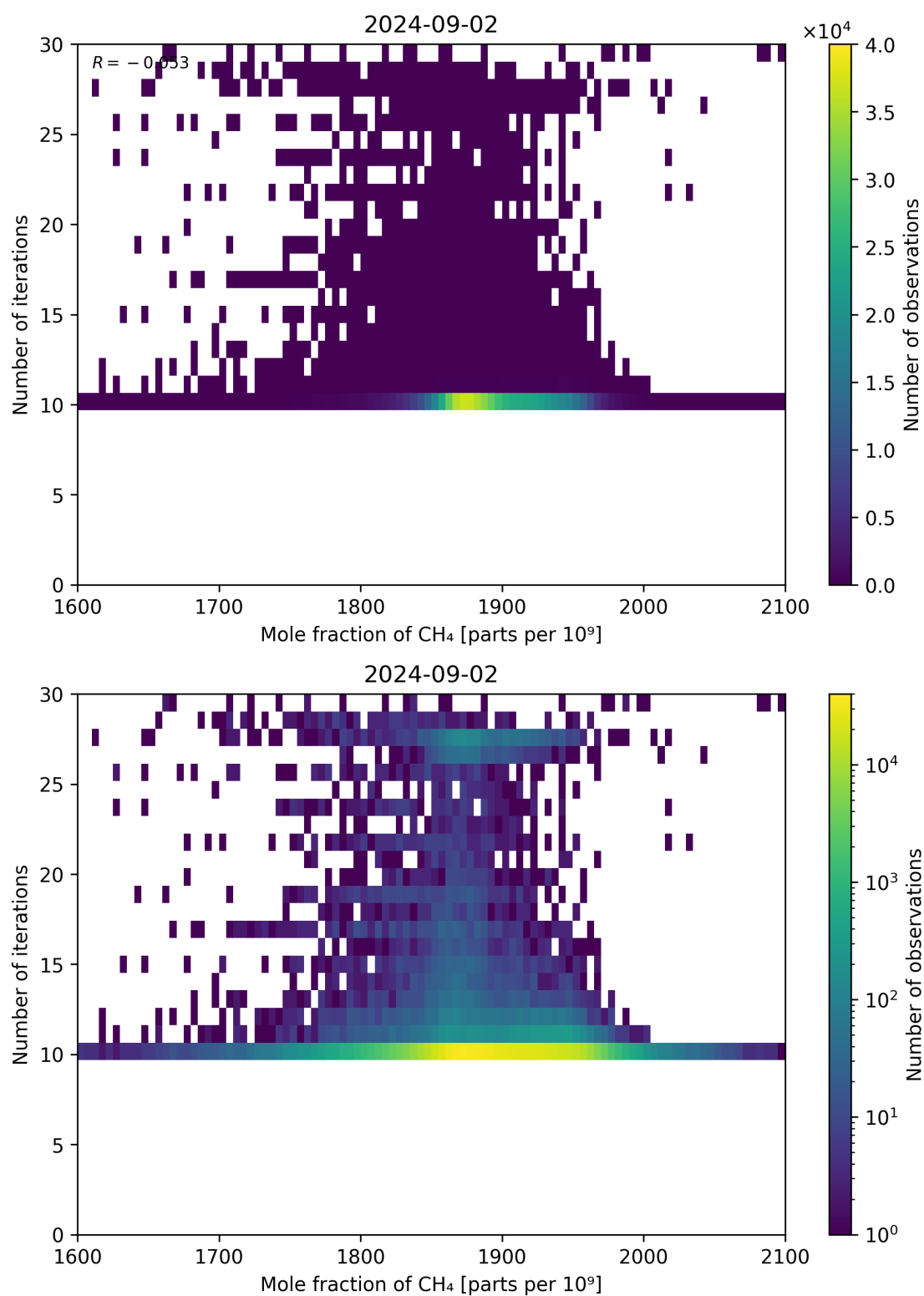
Figure 76: Scatter density plot of “Mole fraction of CH 4 ” against “Number of iterations” for 2024-09-01 to 2024-09-03.
