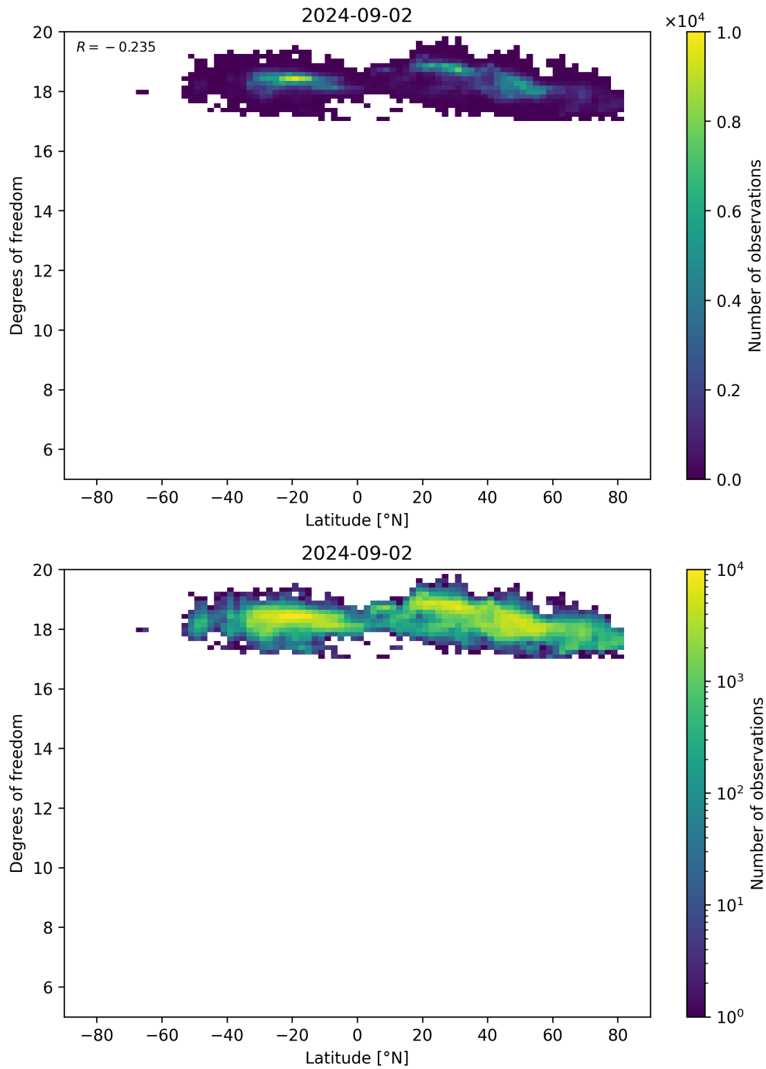
Figure 55: Scatter density plot of “Latitude” against “Degrees of freedom” for 2024-09-01 to 2024-09-03.
