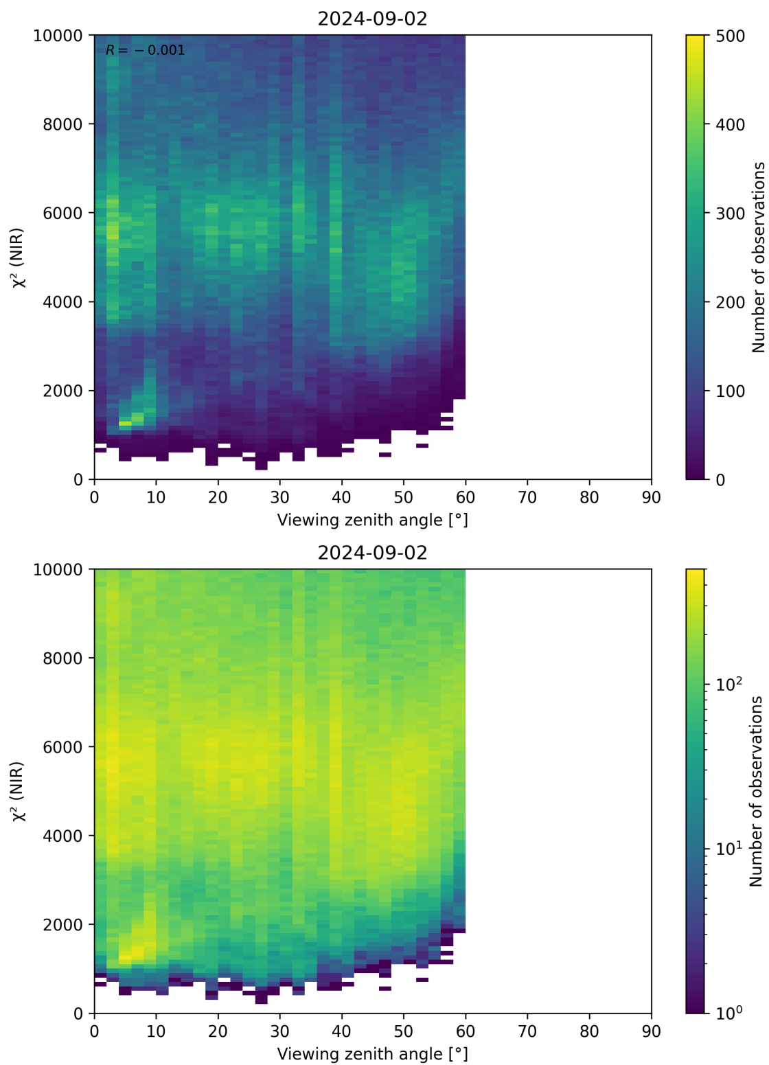
Figure 105: Scatter density plot of “Viewing zenith angle” against “ \chi^2 (NIR)” for 2024-09-01 to 2024-09-03.
