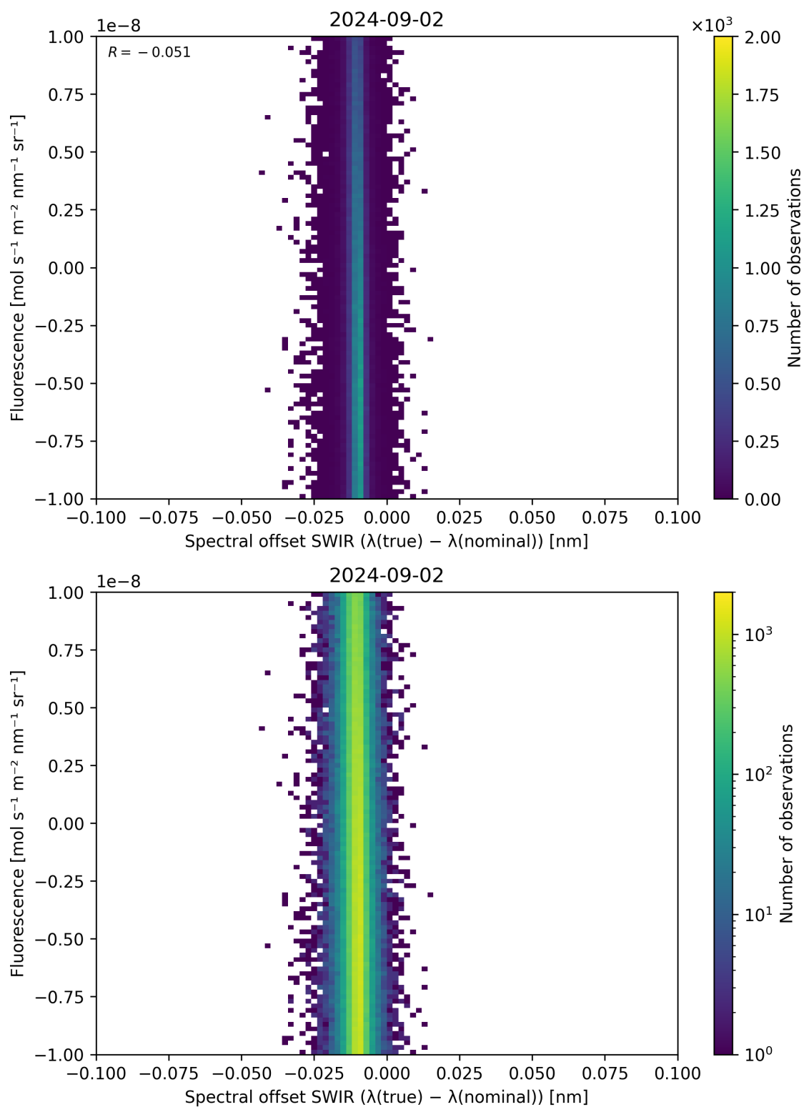
Figure 120: Scatter density plot of “Spectral offset SWIR ( \lambda_{\text{true}} - \lambda_{\text{nominal}} )” against “Fluorescence” for 2024-09-01 to 2024-09-03.
