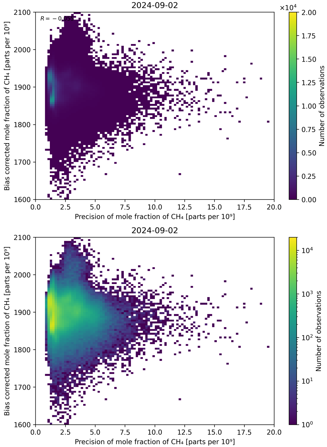
Figure 82: Scatter density plot of “Precision of mole fraction of CH 4 ” against “Bias corrected mole fraction of CH 4 ” for 2024-09-01 to 2024-09-03.
