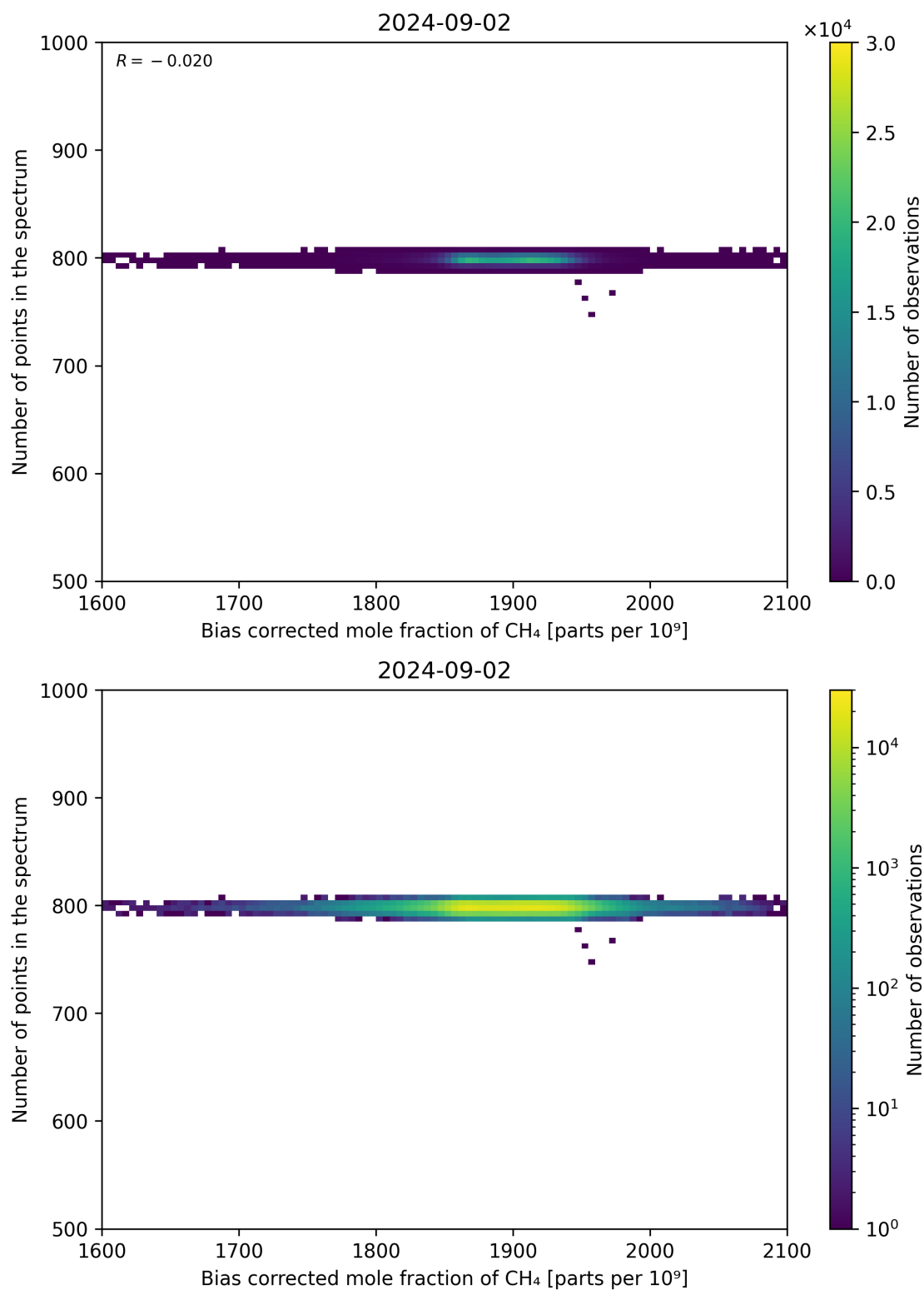
Figure 68: Scatter density plot of “Bias corrected mole fraction of CH 4 ” against “Number of points in the spectrum” for 2024-09-01 to 2024-09-03.
