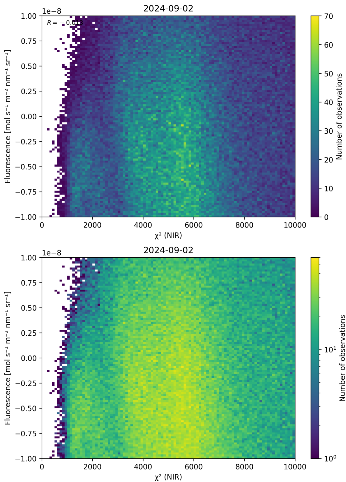
Figure 45: Scatter density plot of “ \chi^2 (NIR)” against “Fluorescence” for 2024-09-01 to 2024-09-03.
