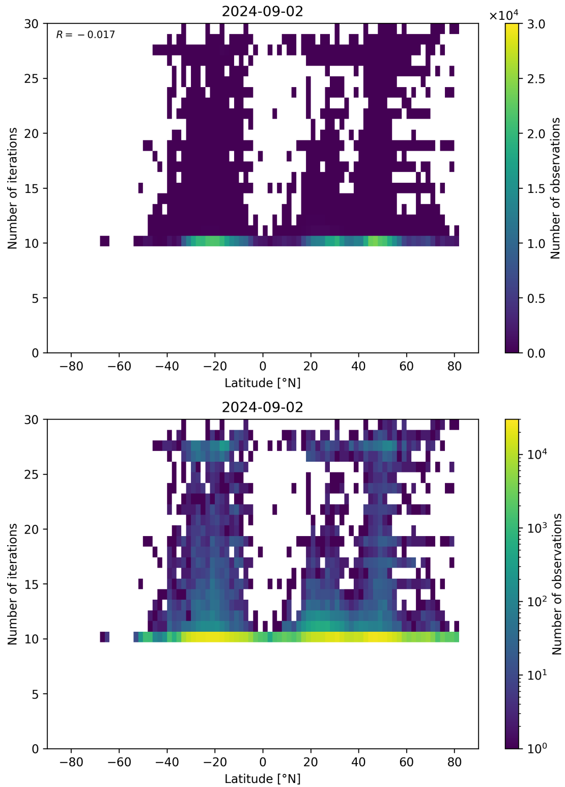
Figure 60: Scatter density plot of “Latitude” against “Number of iterations” for 2024-09-01 to 2024-09-03.
