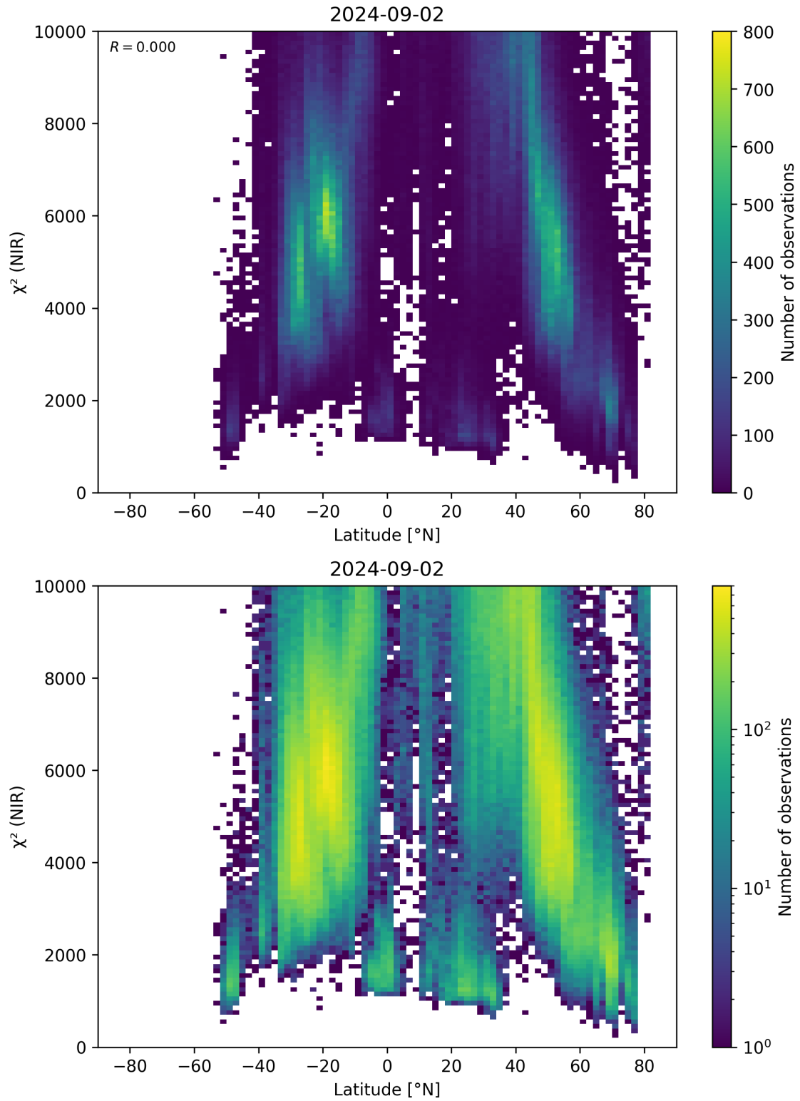
Figure 53: Scatter density plot of “Latitude” against “ \chi^2 (NIR)” for 2024-09-01 to 2024-09-03.
