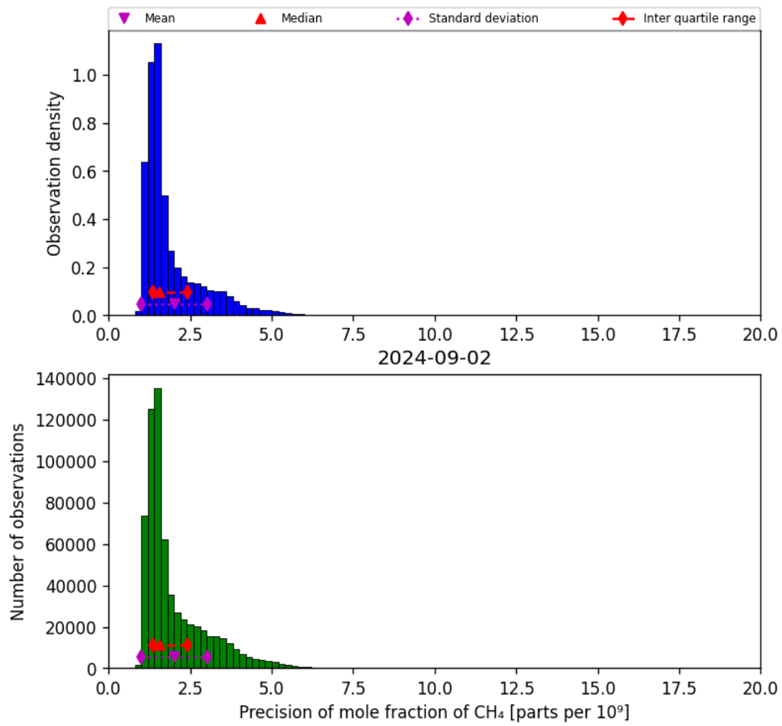
Figure 24: Histogram of “Precision of mole fraction of CH 4 ” for 2024-09-01 to 2024-09-03
