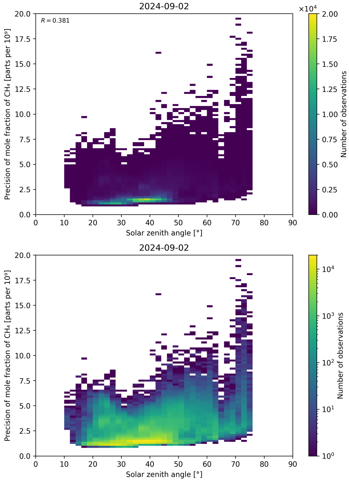
Figure 101: Scatter density plot of “Solar zenith angle” against “Precision of mole fraction of CH 4 ” for 2024-09-01 to 2024-09-03.
