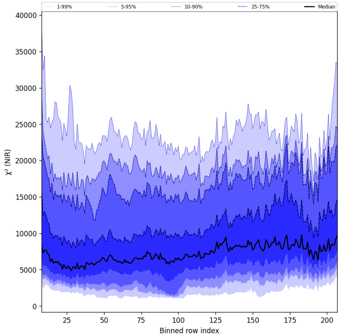
Figure 40: Along track statistics of “ \chi^2 (NIR)” for 2024-09-01 to 2024-09-03
