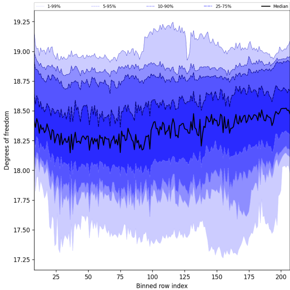
Figure 41: Along track statistics of “Degrees of freedom” for 2024-09-01 to 2024-09-03
