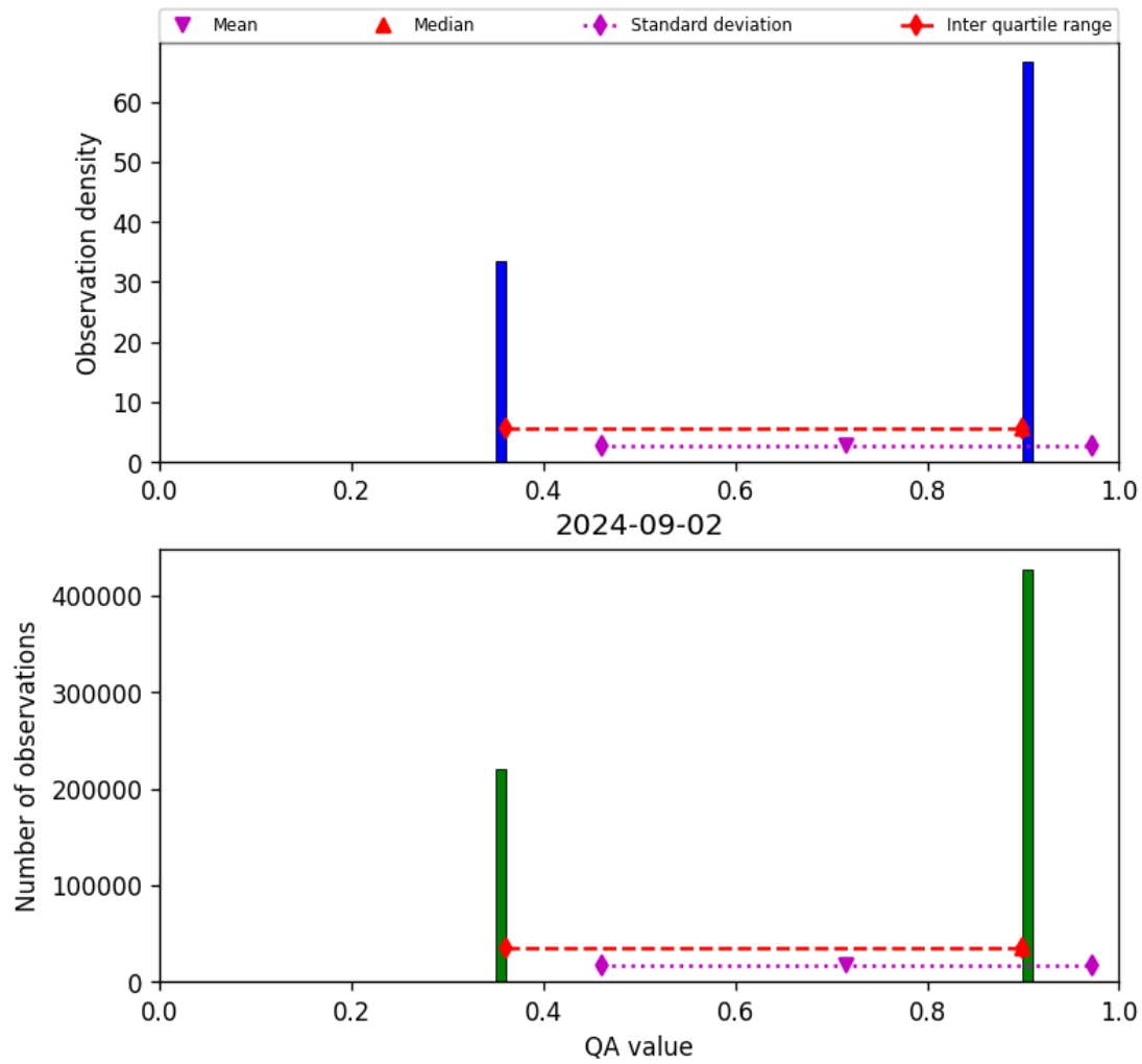
Figure 22: Histogram of “QA value” for 2024-09-01 to 2024-09-03
