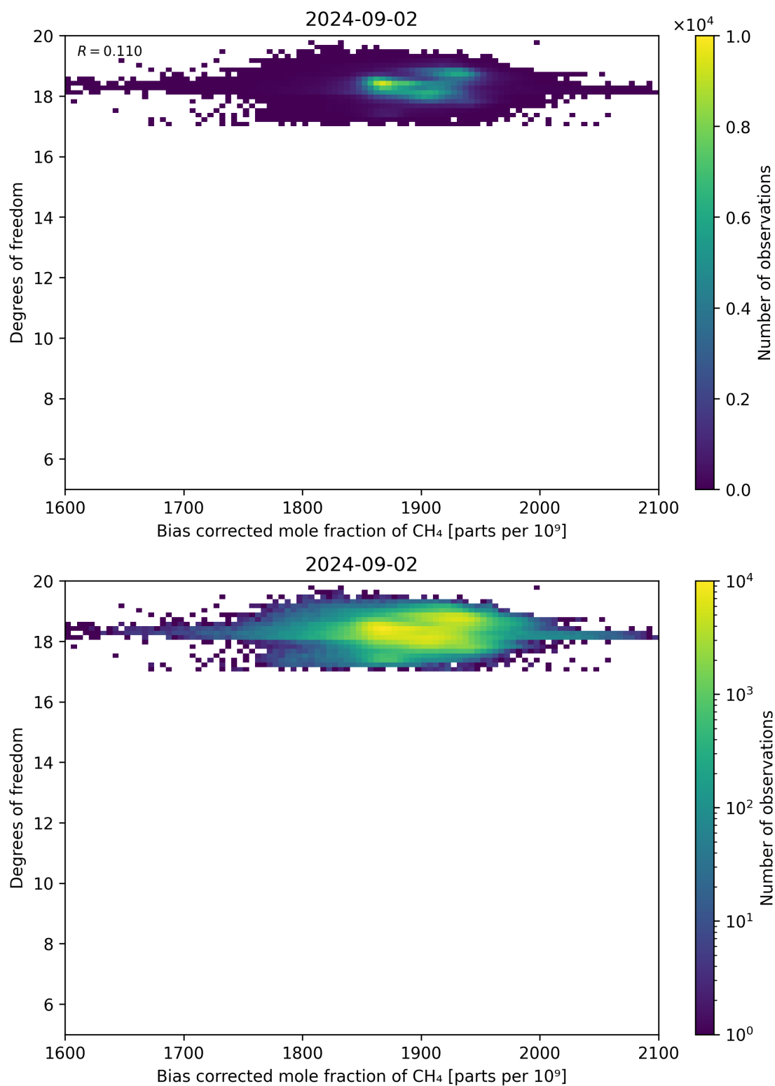
Figure 65: Scatter density plot of “Bias corrected mole fraction of \text{CH}_4 ” against “Degrees of freedom” for 2024-09-01 to 2024-09-03.
