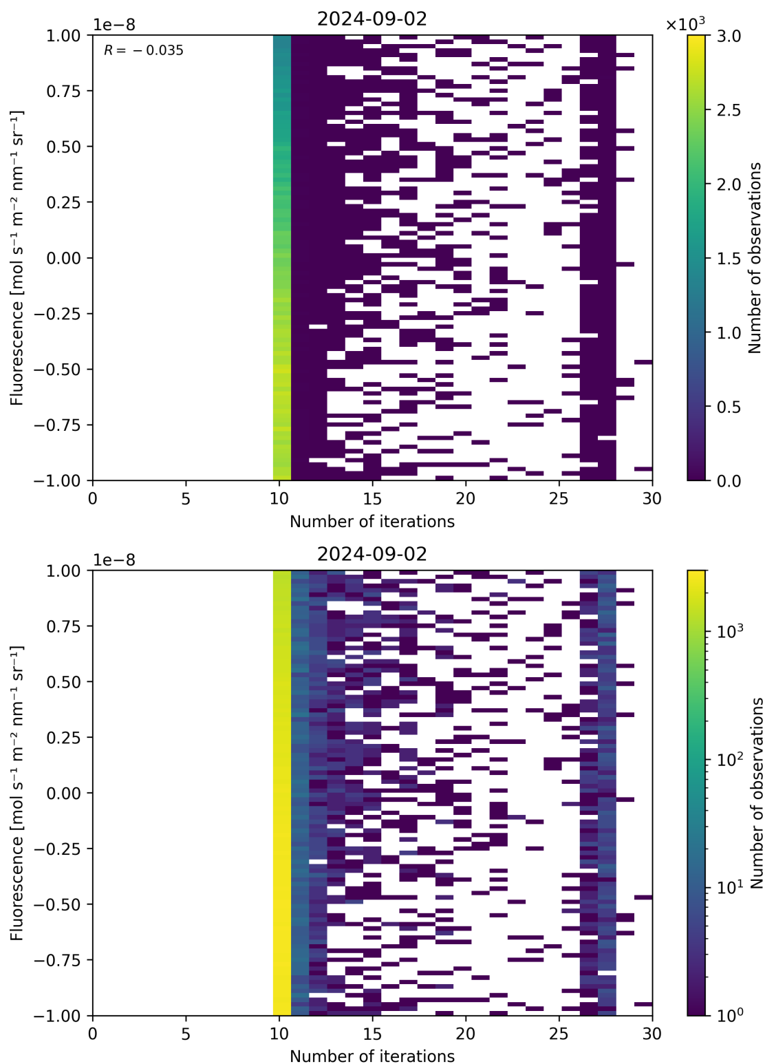
Figure 87: Scatter density plot of “Number of iterations” against “Fluorescence” for 2024-09-01 to 2024-09-03.
