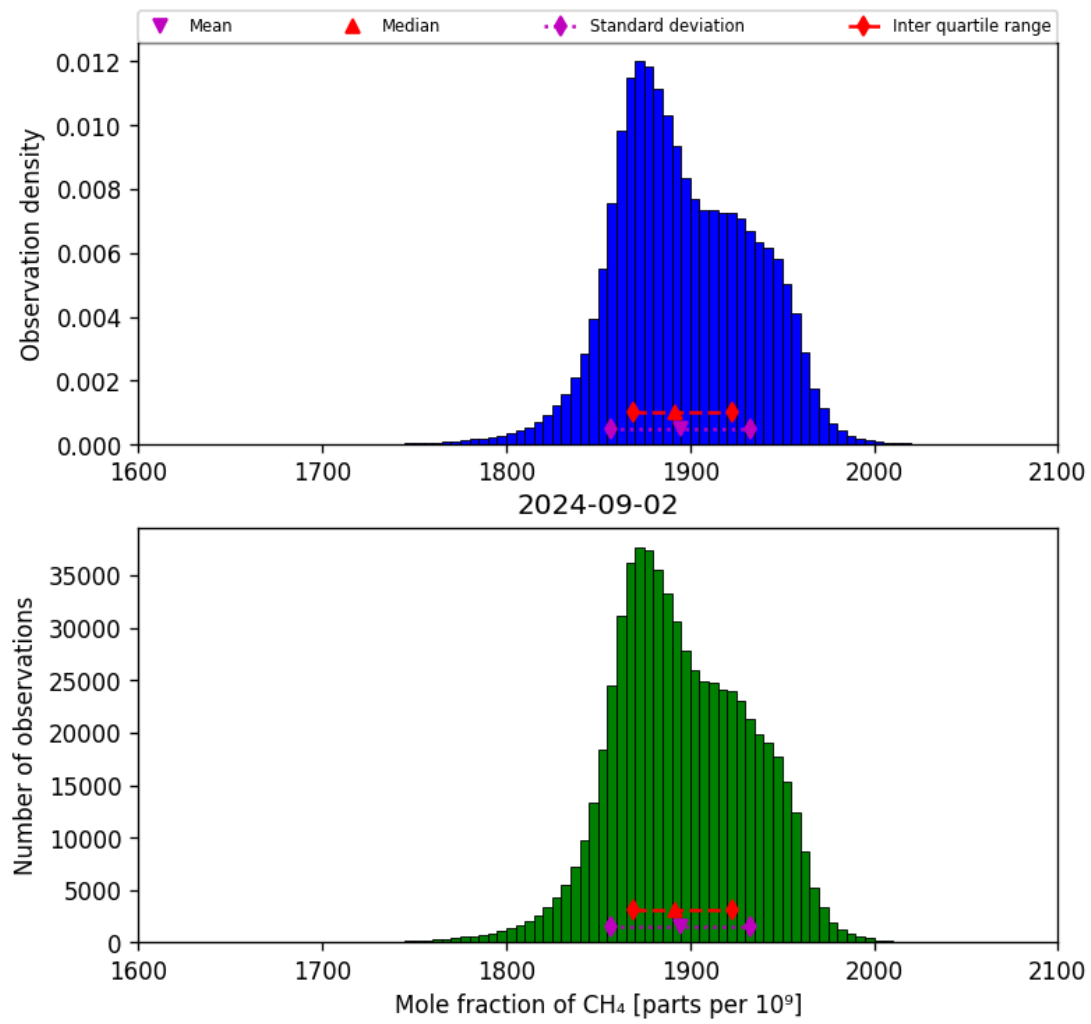
Figure 23: Histogram of “Mole fraction of CH 4 ” for 2024-09-01 to 2024-09-03
