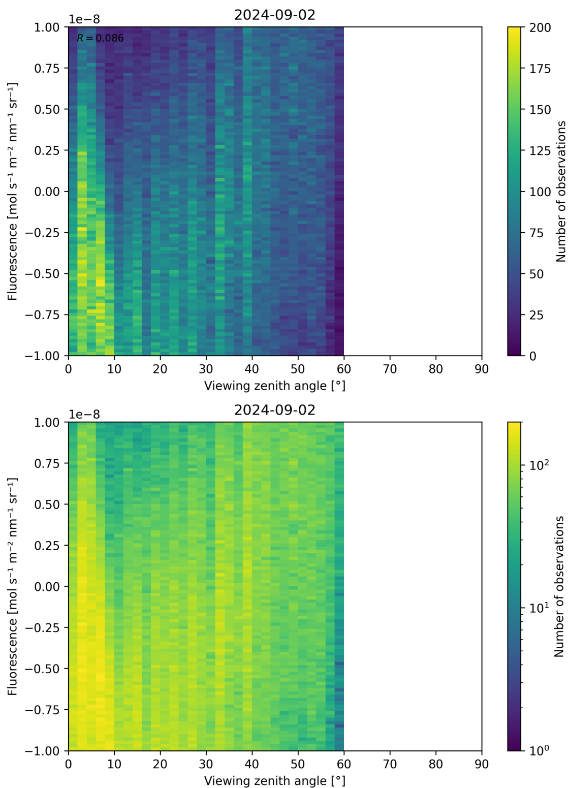
Figure 108: Scatter density plot of “Viewing zenith angle” against “Fluorescence” for 2024-09-01 to 2024-09-03.
