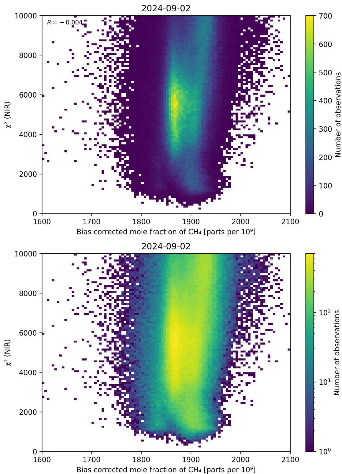
Figure 63: Scatter density plot of “Bias corrected mole fraction of CH 4 ” against “ \chi^2 (NIR)” for 2024-09-01 to 2024-09-03.
