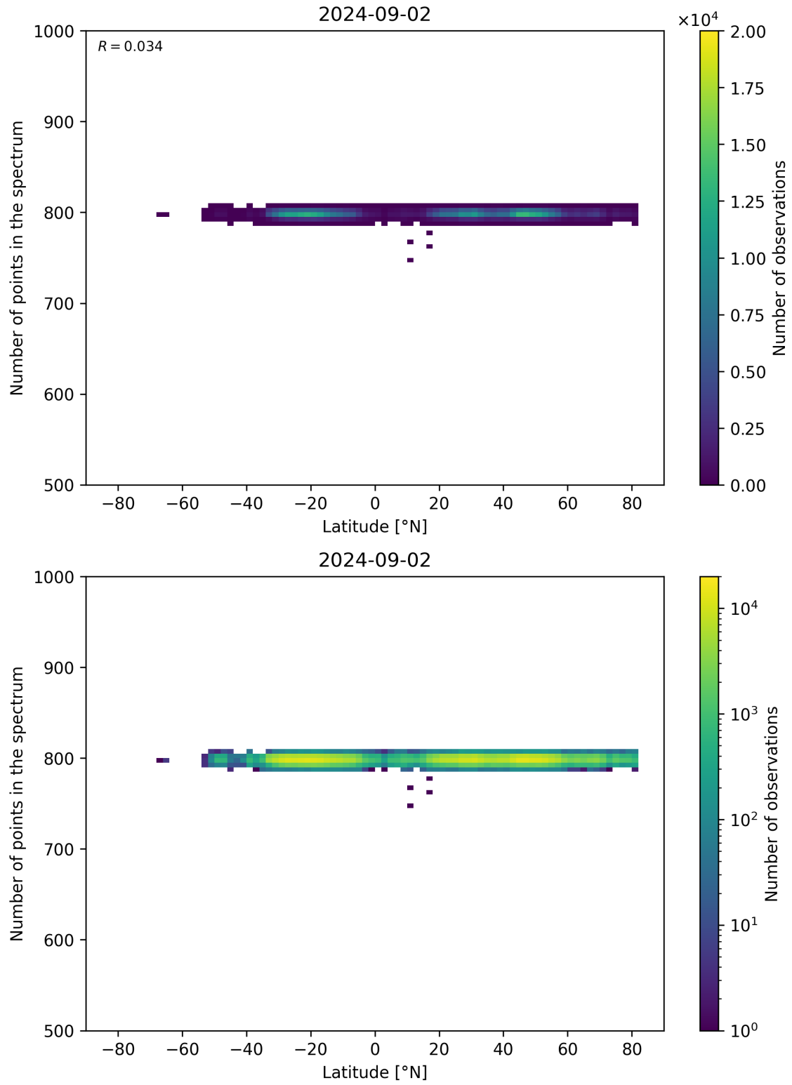
Figure 61: Scatter density plot of “Latitude” against “Number of points in the spectrum” for 2024-09-01 to 2024-09-03.
