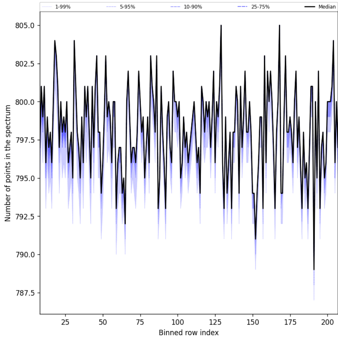
Figure 37: Along track statistics of “Number of points in the spectrum” for 2024-09-01 to 2024-09-03
