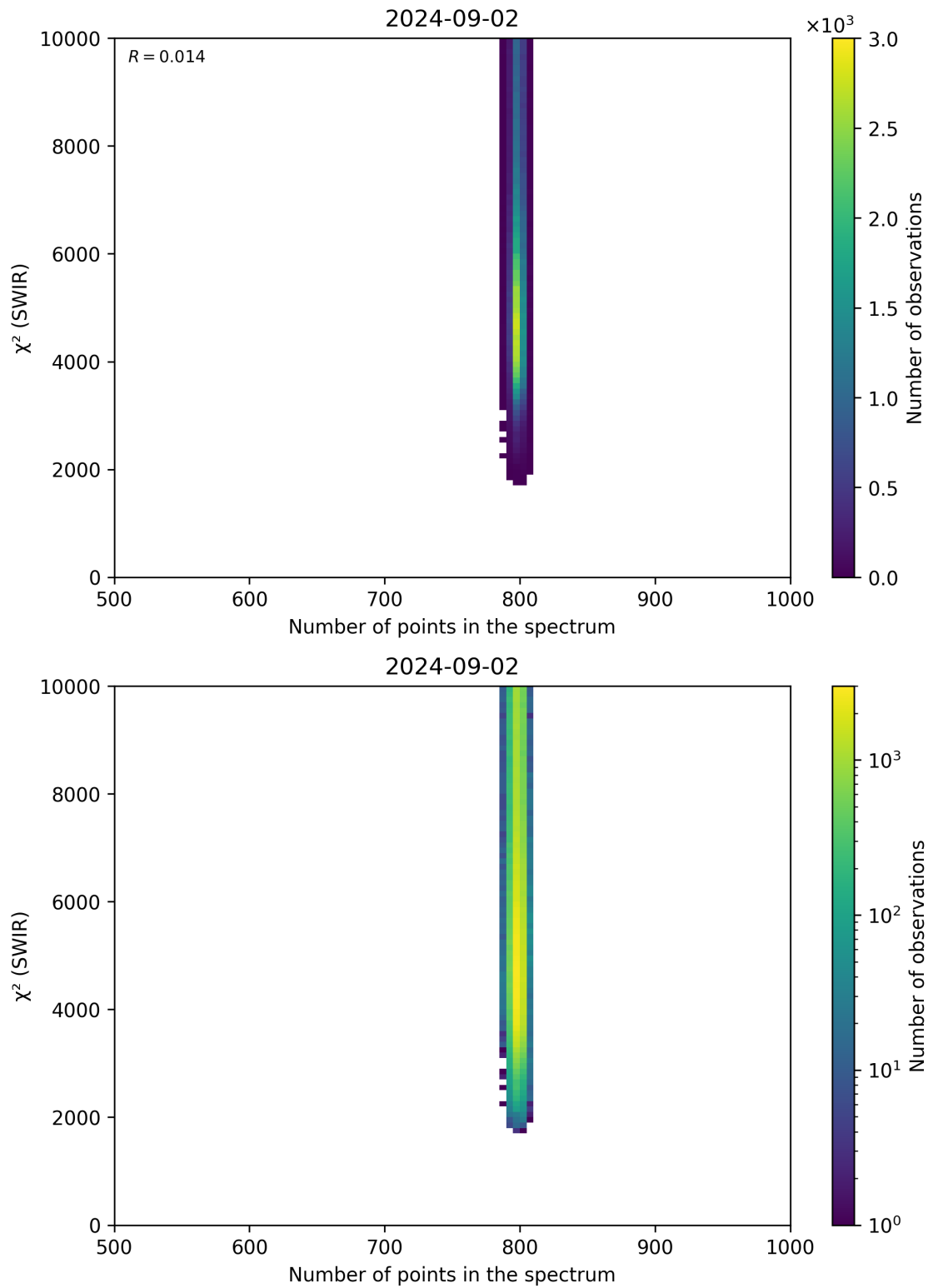
Figure 89: Scatter density plot of “Number of points in the spectrum” against “ \chi^2 (SWIR)” for 2024-09-01 to 2024-09-03.
