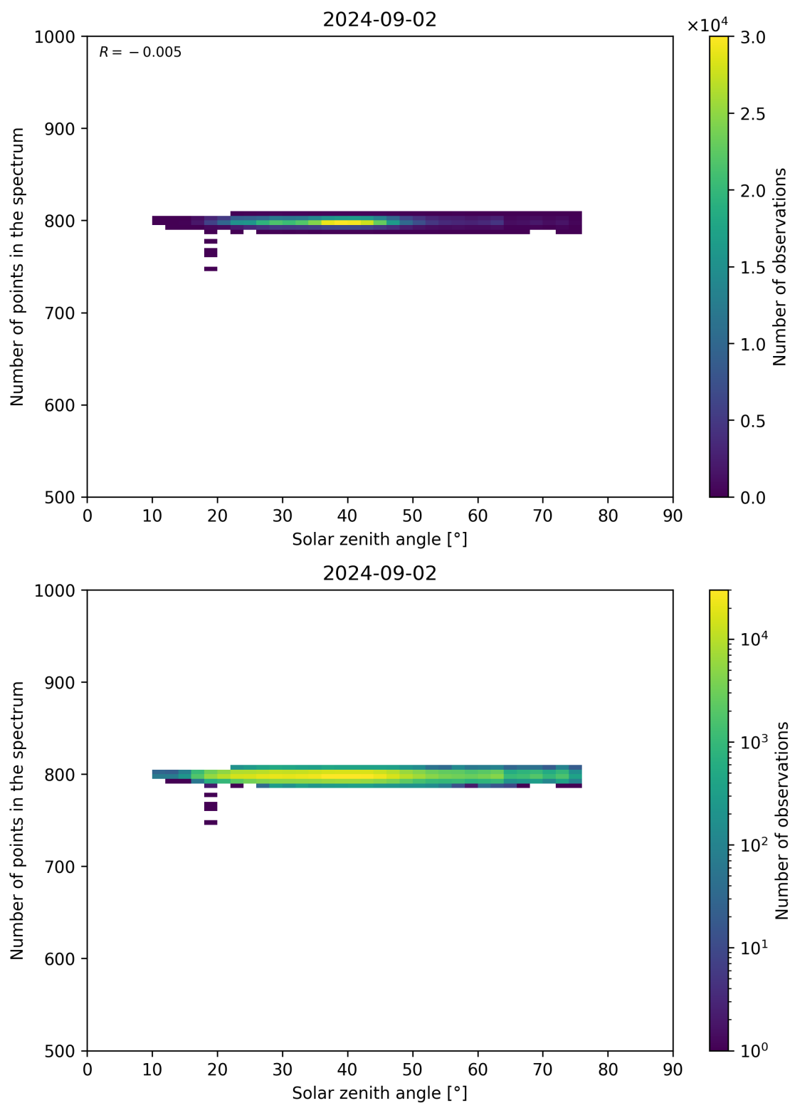
Figure 103: Scatter density plot of “Solar zenith angle” against “Number of points in the spectrum” for 2024-09-01 to 2024-09-03.
