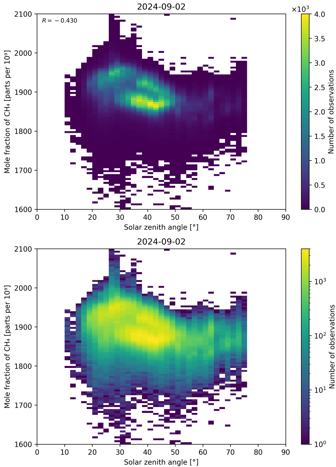
Figure 99: Scatter density plot of “Solar zenith angle” against “Mole fraction of CH 4 ” for 2024-09-01 to 2024-09-03.
