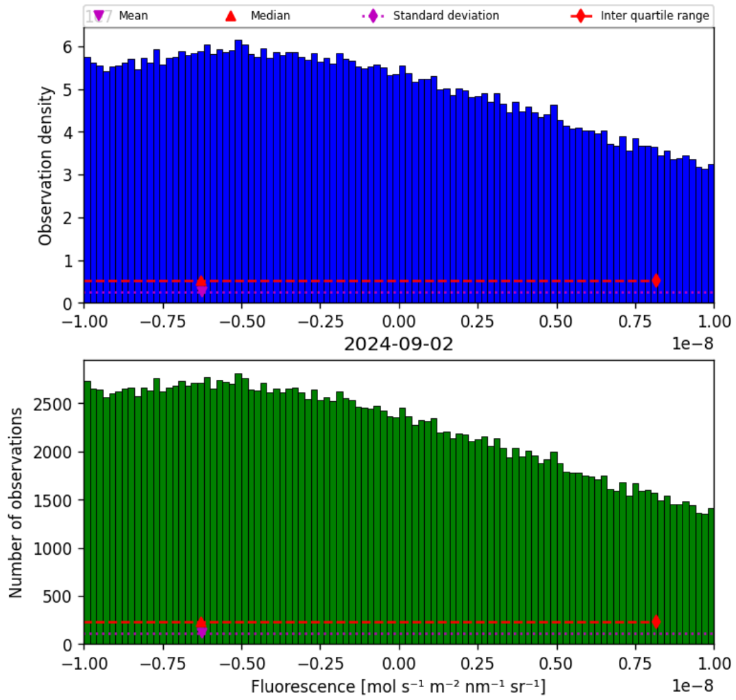
Figure 32: Histogram of “Fluorescence” for 2024-09-01 to 2024-09-03
