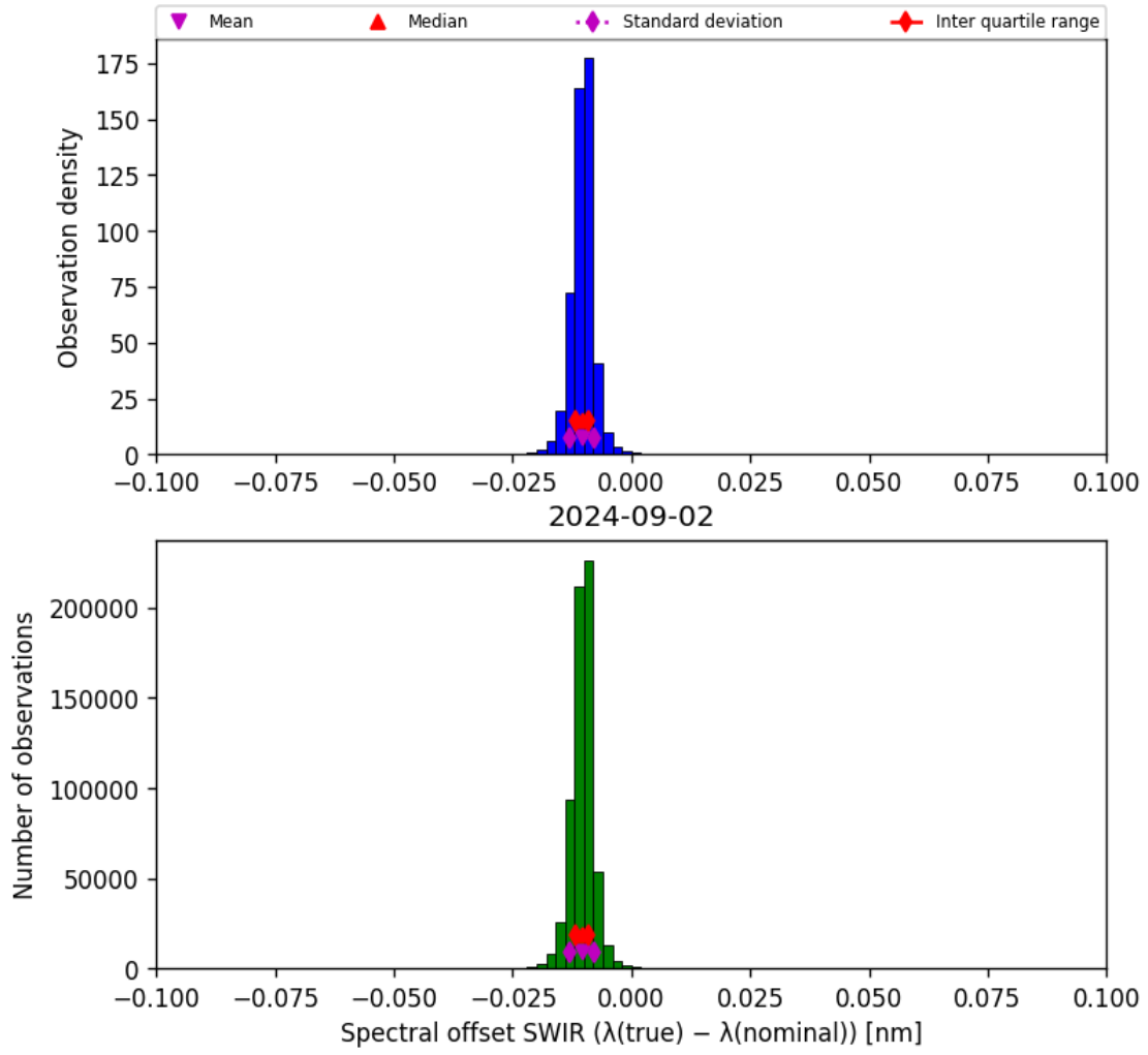
Figure 27: Histogram of “Spectral offset SWIR ( \lambda_{\text{true}} - \lambda_{\text{nominal}} )” for 2024-09-01 to 2024-09-03
