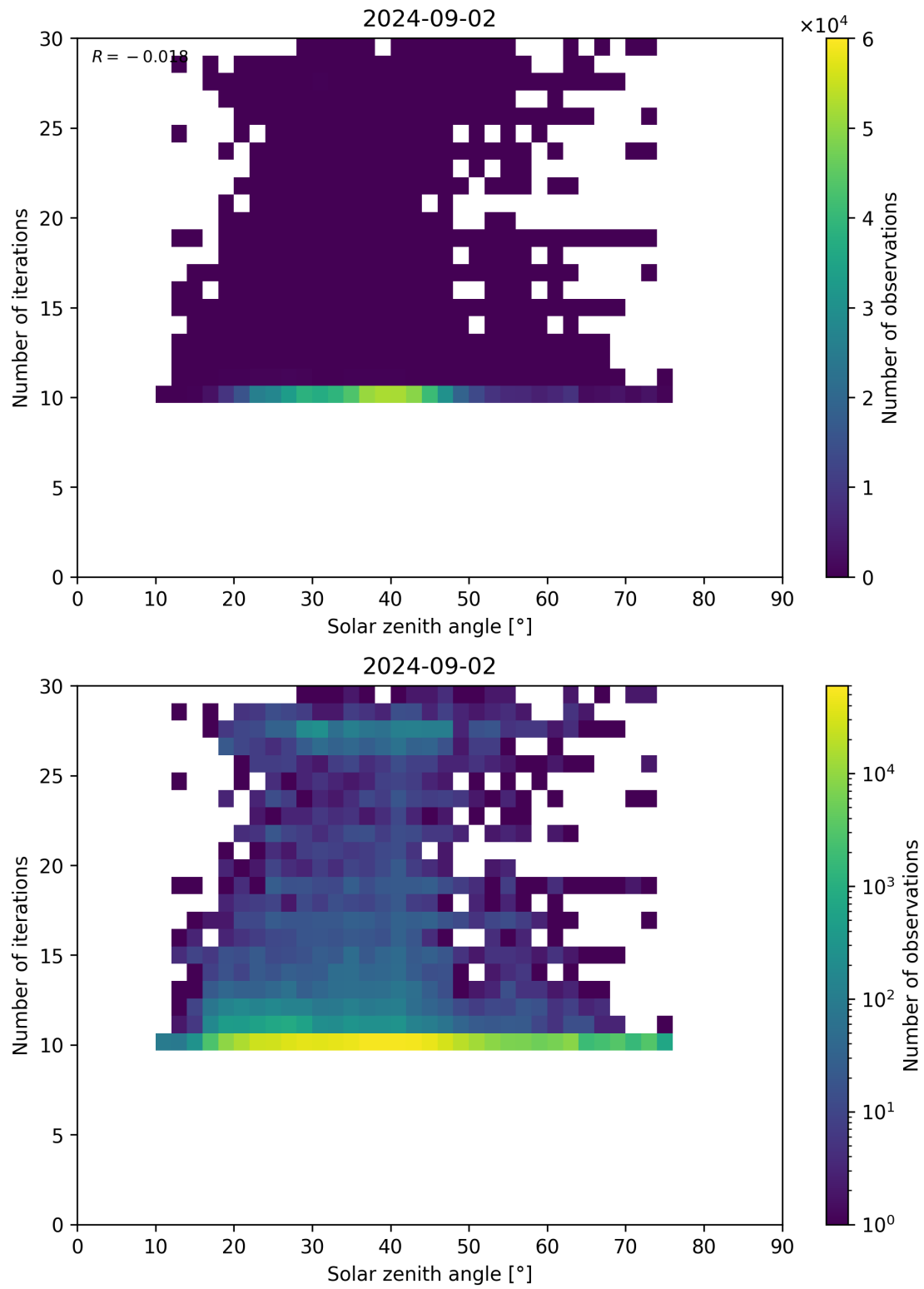
Figure 102: Scatter density plot of “Solar zenith angle” against “Number of iterations” for 2024-09-01 to 2024-09-03.
