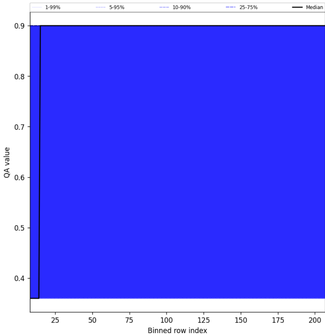
Figure 33: Along track statistics of “QA value” for 2024-09-01 to 2024-09-03
