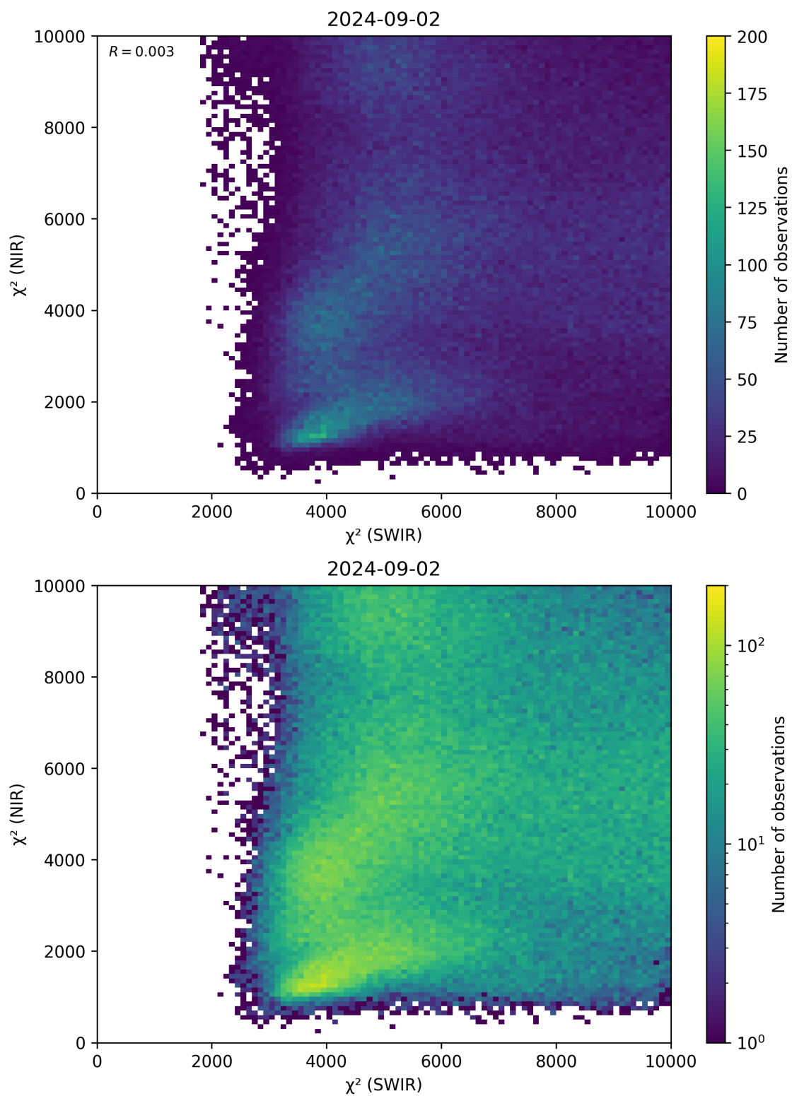
Figure 47: Scatter density plot of “ \chi^2 (SWIR)” against “ \chi^2 (NIR)” for 2024-09-01 to 2024-09-03.
