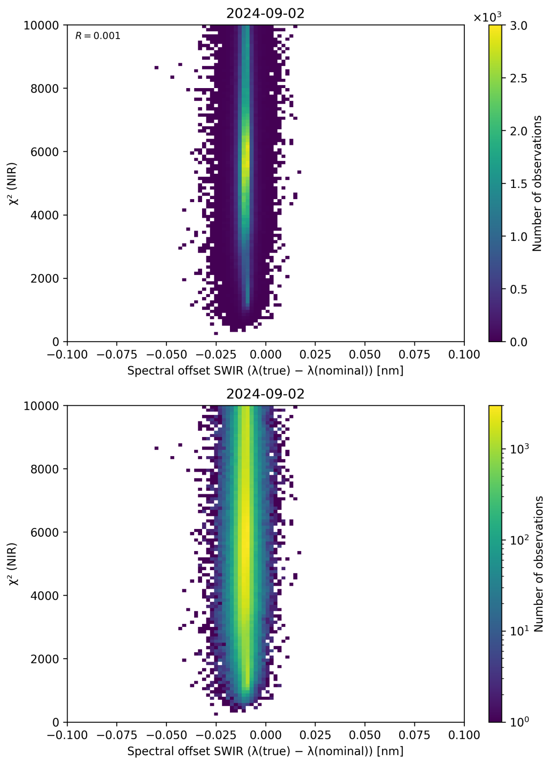
Figure 117: Scatter density plot of “Spectral offset SWIR ( \lambda_{\text{true}} - \lambda_{\text{nominal}} )” against “ \chi^2 (NIR)” for 2024-09-01 to 2024-09-03.
