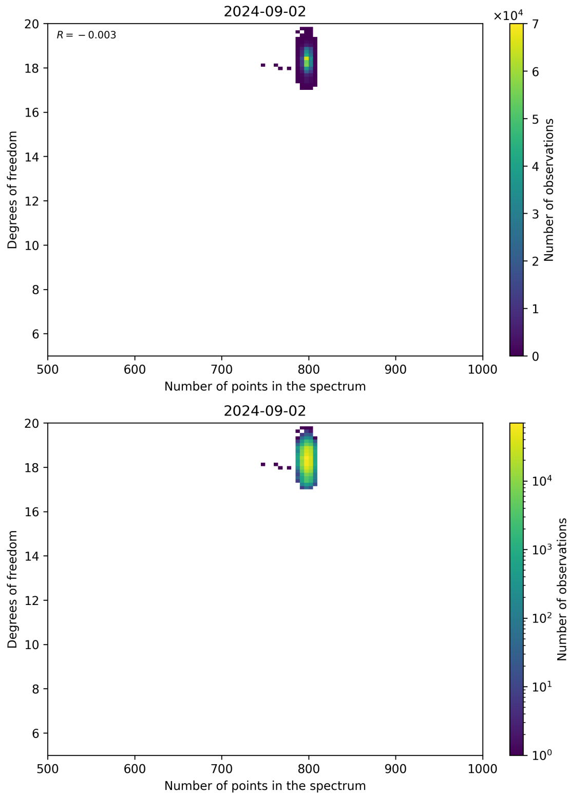
Figure 90: Scatter density plot of “Number of points in the spectrum” against “Degrees of freedom” for 2024-09-01 to 2024-09-03.
