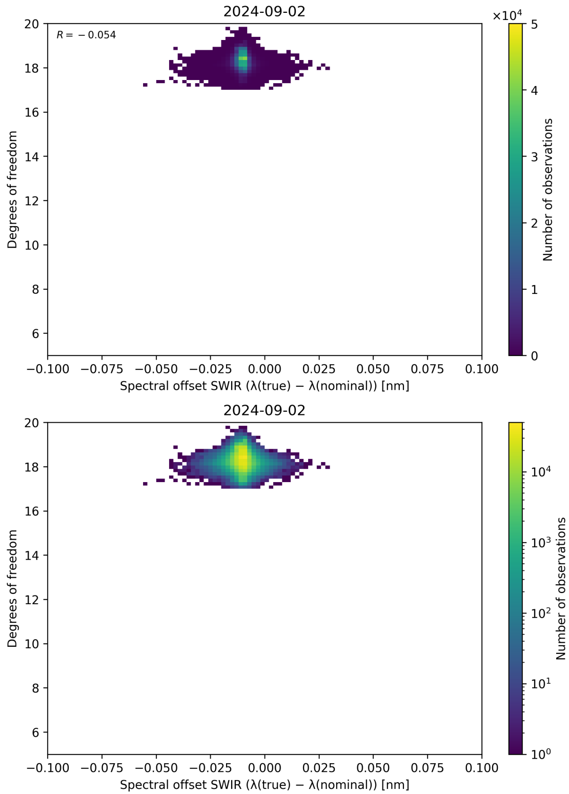
Figure 119: Scatter density plot of “Spectral offset SWIR ( \lambda_{\text{true}} - \lambda_{\text{nominal}} )” against “Degrees of freedom” for 2024-09-01 to 2024-09-03.
