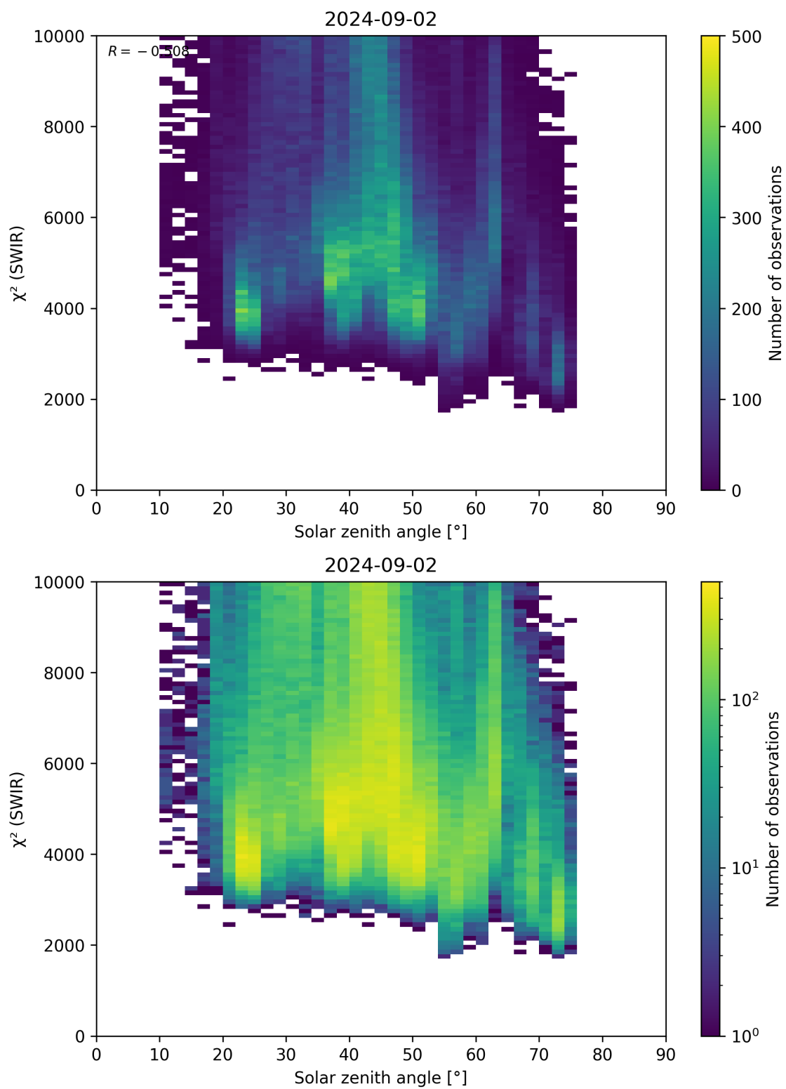
Figure 95: Scatter density plot of “Solar zenith angle” against “ \chi^2 (SWIR)” for 2024-09-01 to 2024-09-03.
