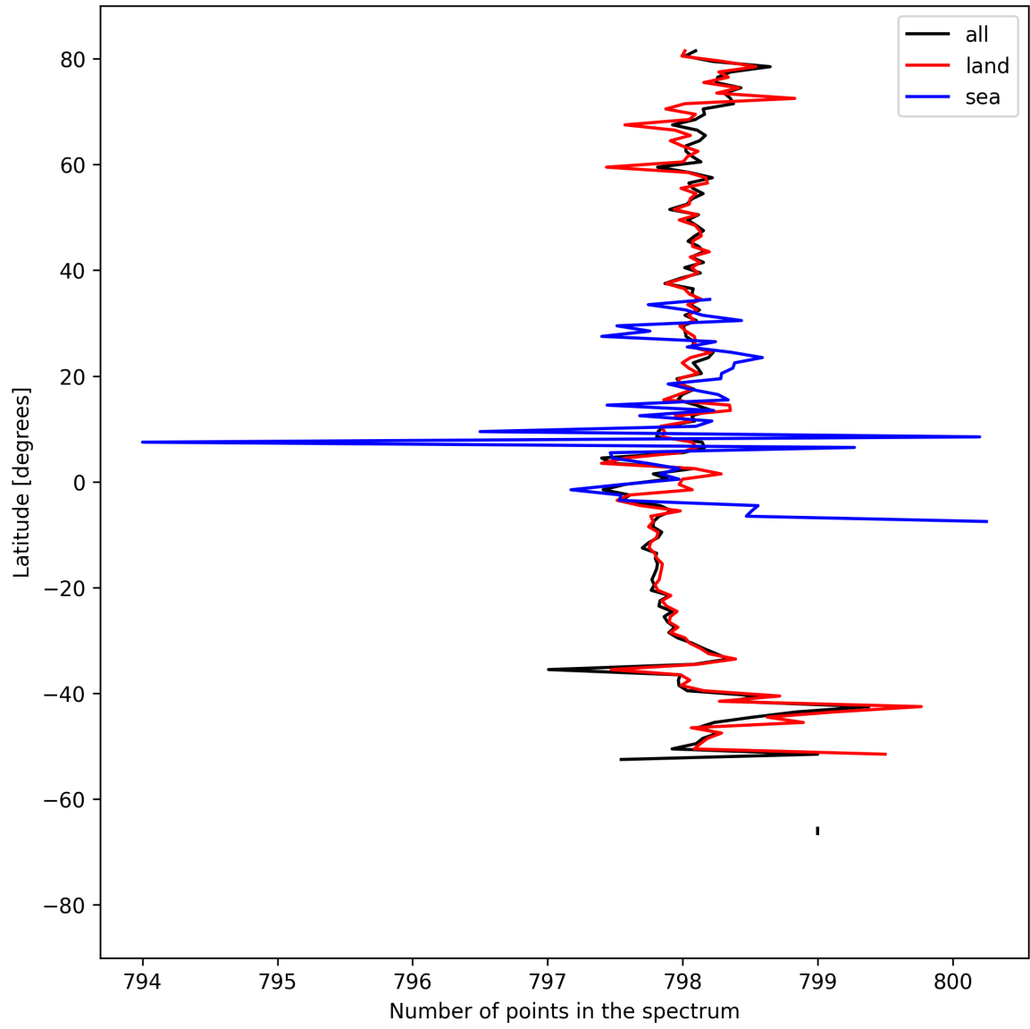
Figure 15: Zonal average of “Number of points in the spectrum” for 2024-09-01 to 2024-09-03.
