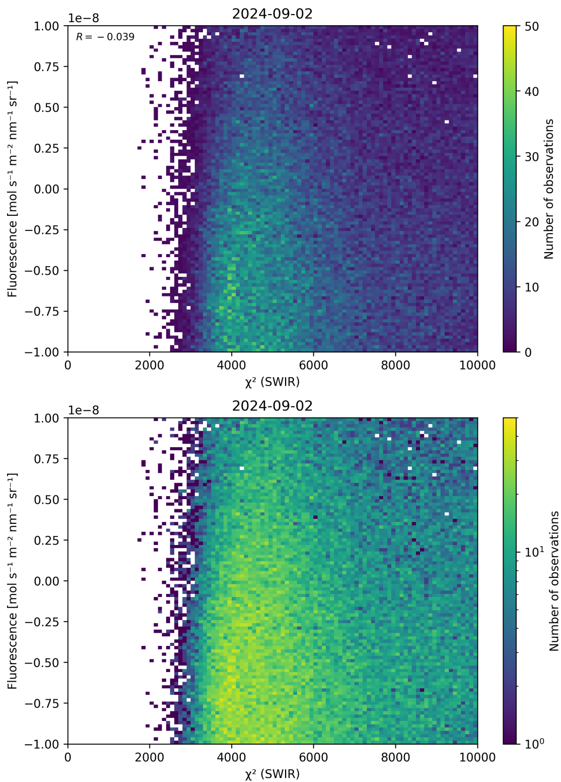
Figure 49: Scatter density plot of “ \chi^2 (SWIR)” against “Fluorescence” for 2024-09-01 to 2024-09-03.
