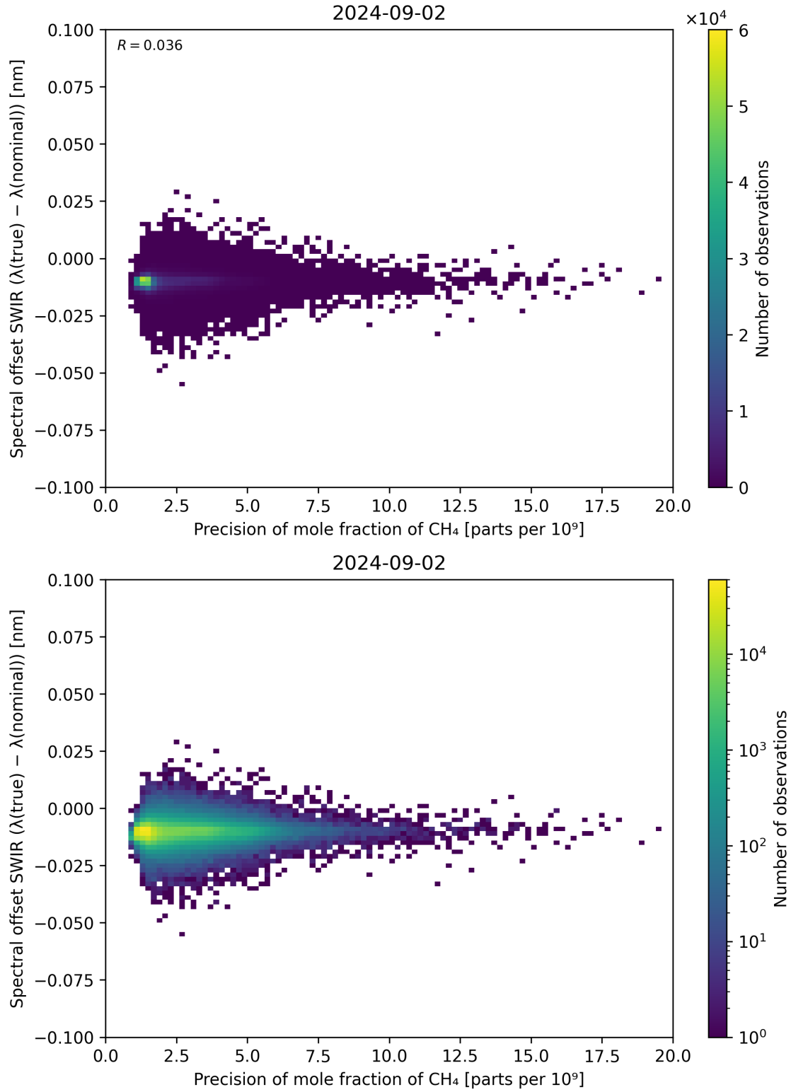
Figure 85: Scatter density plot of “Precision of mole fraction of \text{CH}_4 ” against “Spectral offset SWIR ( \lambda_{\text{true}} - \lambda_{\text{nominal}} )” for 2024-09-01 to 2024-09-03.
