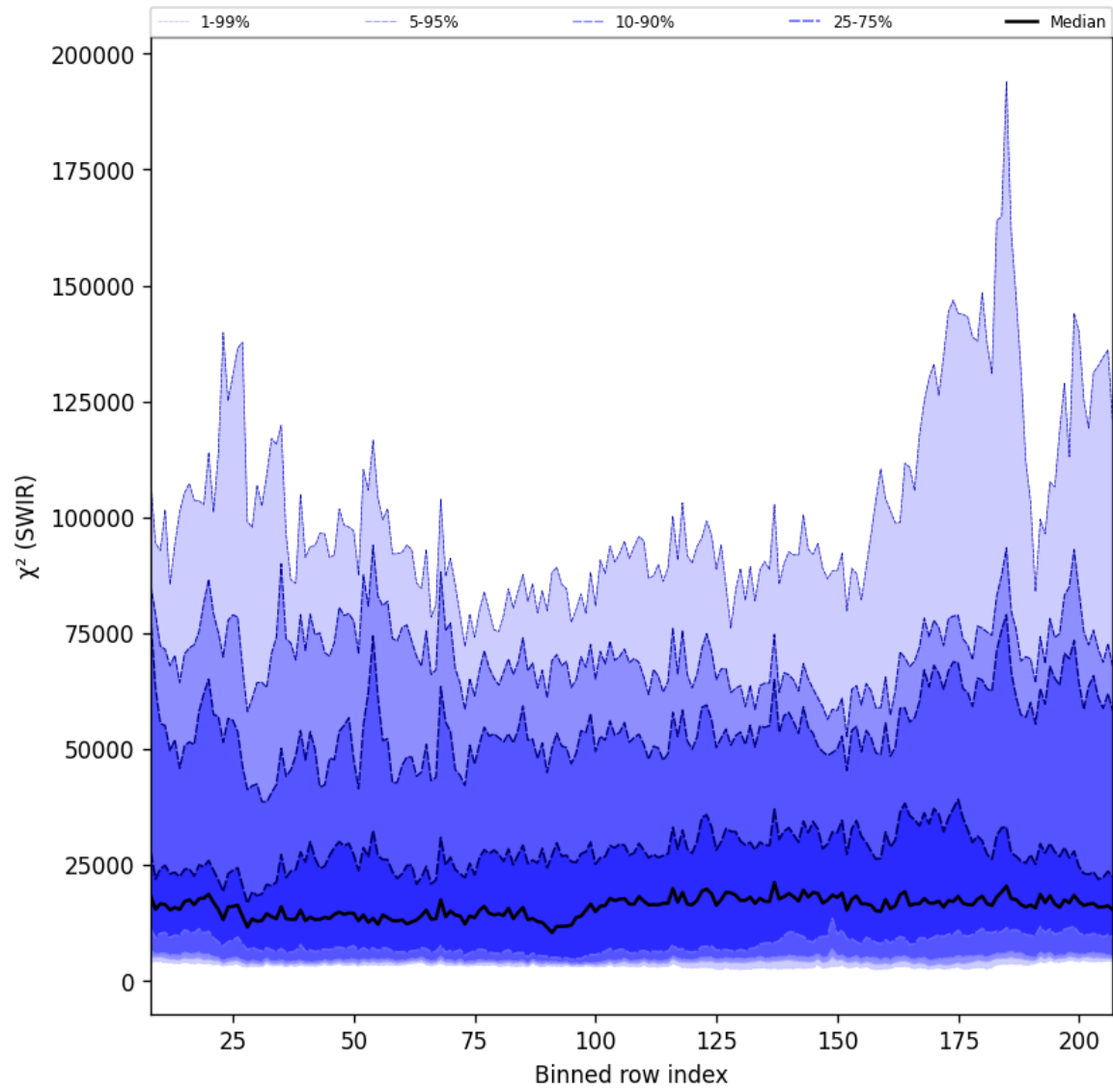
Figure 39: Along track statistics of " \chi^2 (SWIR)" for 2024-09-01 to 2024-09-03
