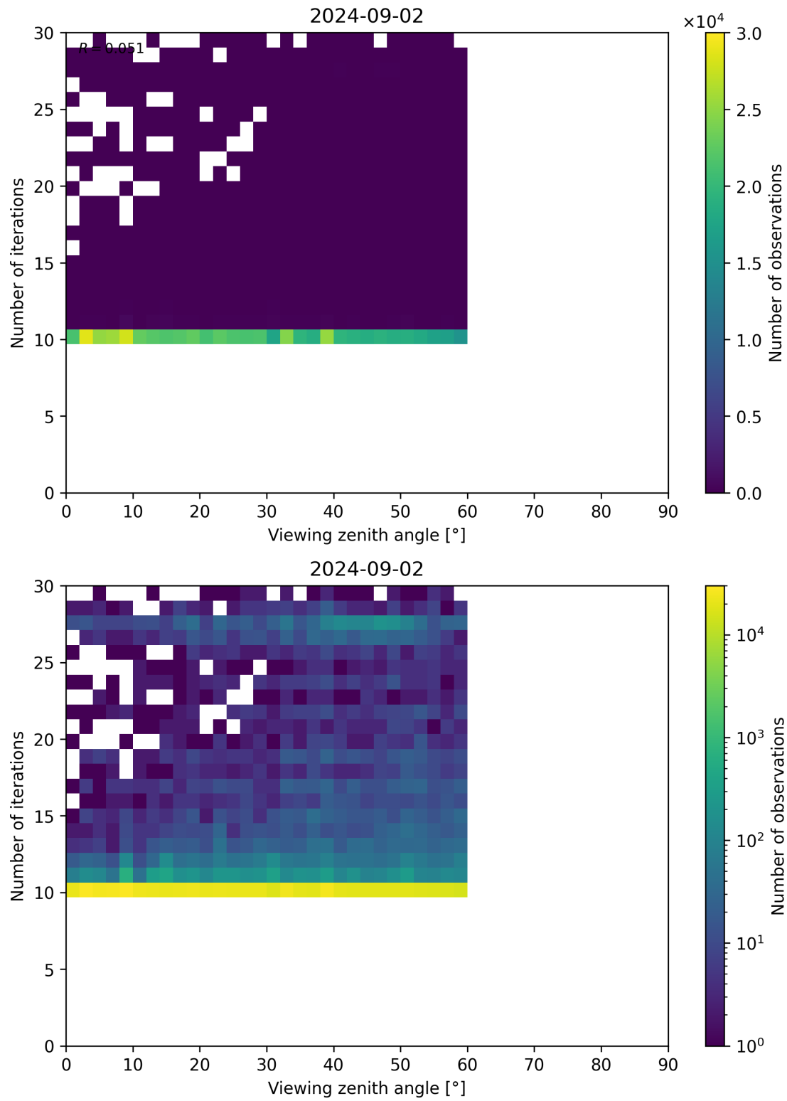
Figure 113: Scatter density plot of “Viewing zenith angle” against “Number of iterations” for 2024-09-01 to 2024-09-03.
