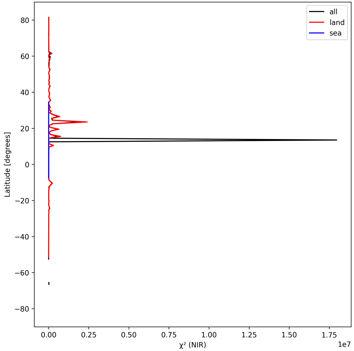
Figure 18: Zonal average of “ \chi^2 (NIR)” for 2024-09-01 to 2024-09-03.
