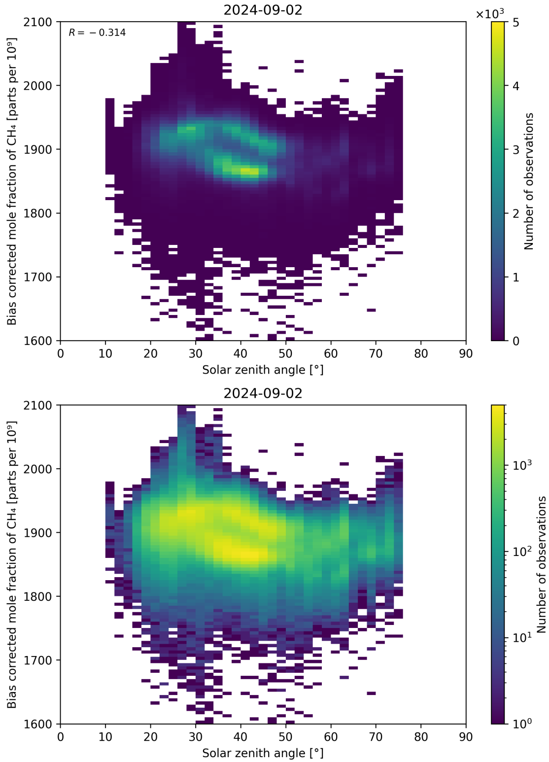
Figure 100: Scatter density plot of “Solar zenith angle” against “Bias corrected mole fraction of \text{CH}_4 ” for 2024-09-01 to 2024-09-03.
