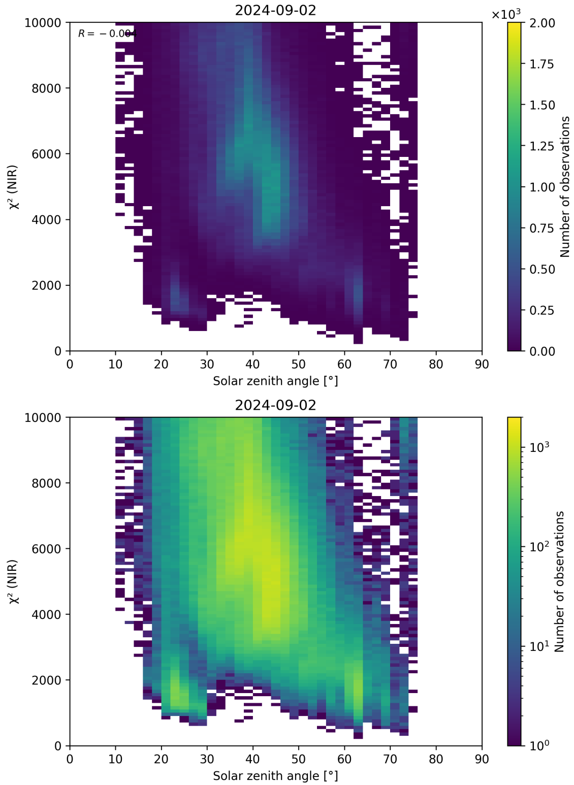
Figure 94: Scatter density plot of “Solar zenith angle” against “ \chi^2 (NIR)” for 2024-09-01 to 2024-09-03.
