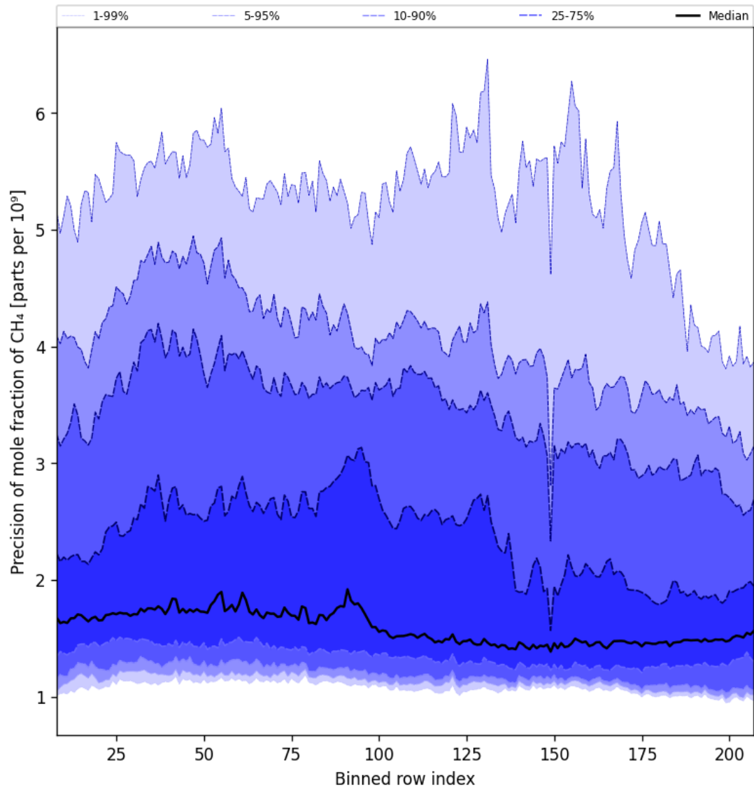
Figure 35: Along track statistics of “Precision of mole fraction of CH 4 ” for 2024-09-01 to 2024-09-03
