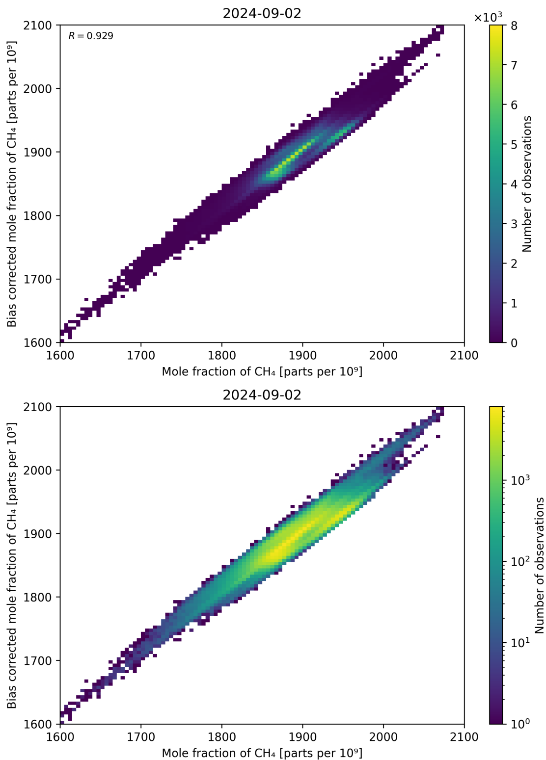
Figure 74: Scatter density plot of “Mole fraction of CH 4 ” against “Bias corrected mole fraction of CH 4 ” for 2024-09-01 to 2024-09-03.
