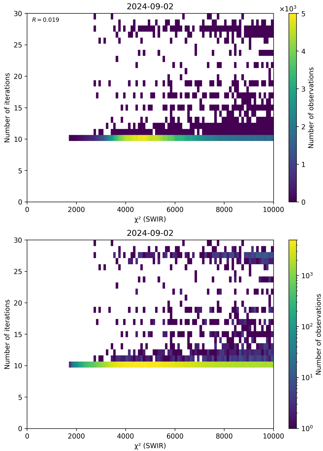
Figure 50: Scatter density plot of “ \chi^2 (SWIR)” against “Number of iterations” for 2024-09-01 to 2024-09-03.
