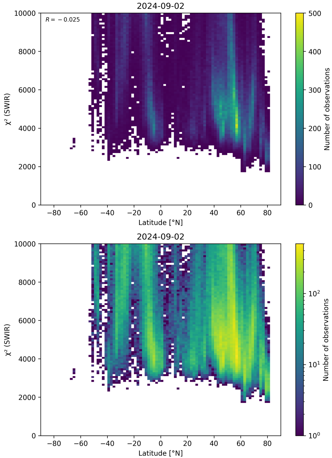
Figure 54: Scatter density plot of “Latitude” against “ \chi^2 (SWIR)” for 2024-09-01 to 2024-09-03.
