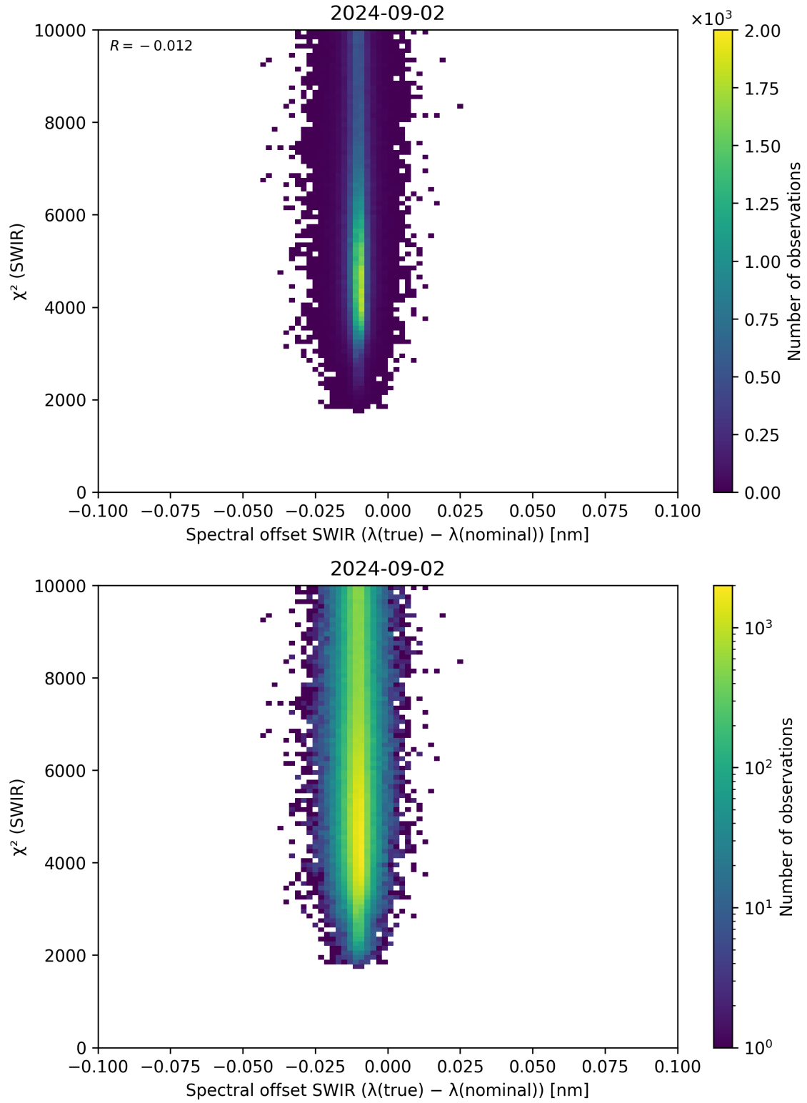
Figure 118: Scatter density plot of “Spectral offset SWIR ( \lambda_{\text{true}} - \lambda_{\text{nominal}} )” against “ \chi^2 (SWIR)” for 2024-09-01 to 2024-09-03.
