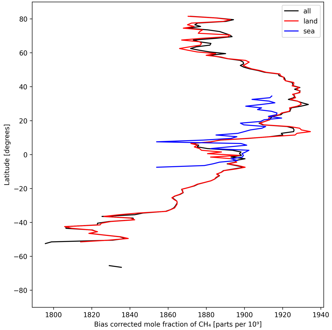
Figure 14: Zonal average of “Bias corrected mole fraction of CH 4 ” for 2024-09-01 to 2024-09-03.
