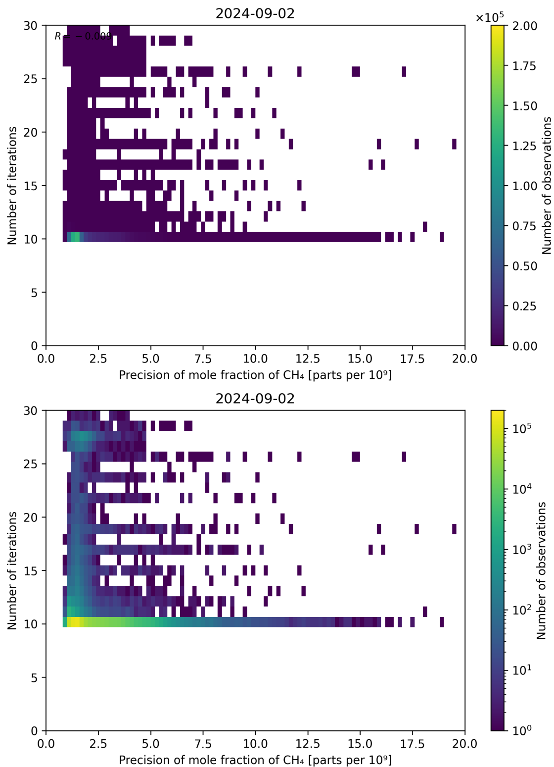
Figure 83: Scatter density plot of “Precision of mole fraction of CH 4 ” against “Number of iterations” for 2024-09-01 to 2024-09-03.
