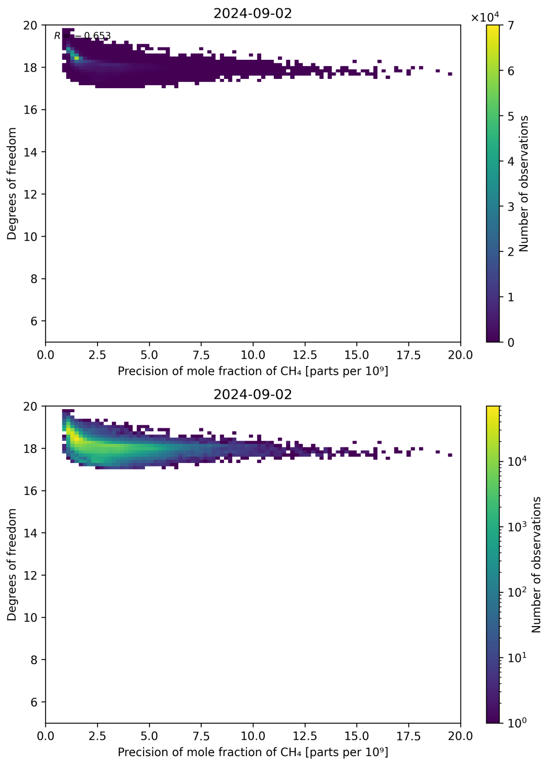
Figure 80: Scatter density plot of “Precision of mole fraction of CH 4 ” against “Degrees of freedom” for 2024-09-01 to 2024-09-03.
