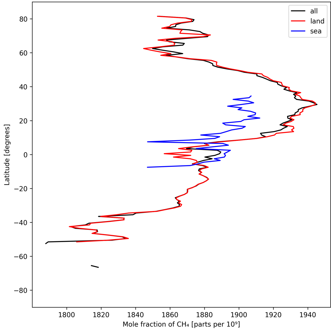
Figure 12: Zonal average of “Mole fraction of \text{CH}_4 ” for 2024-09-01 to 2024-09-03.
