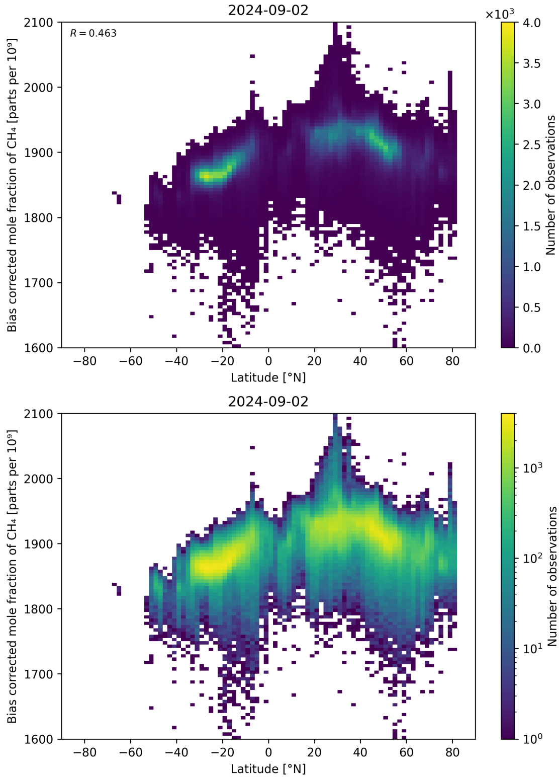
Figure 58: Scatter density plot of “Latitude” against “Bias corrected mole fraction of CH 4 ” for 2024-09-01 to 2024-09-03.
