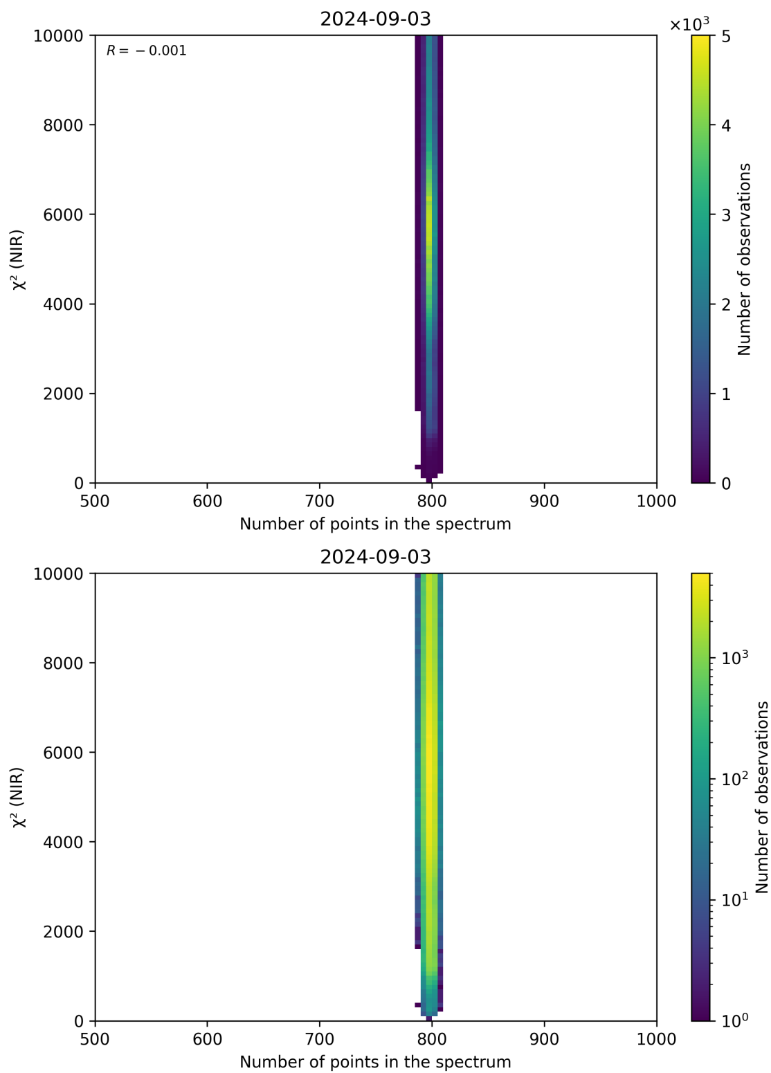
Figure 88: Scatter density plot of “Number of points in the spectrum” against “ \chi^2 (NIR)” for 2024-09-02 to 2024-09-04.
