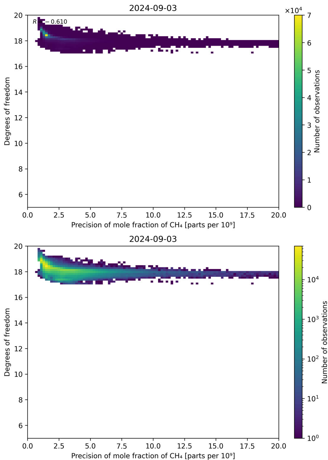
Figure 80: Scatter density plot of “Precision of mole fraction of CH 4 ” against “Degrees of freedom” for 2024-09-02 to 2024-09-04.
