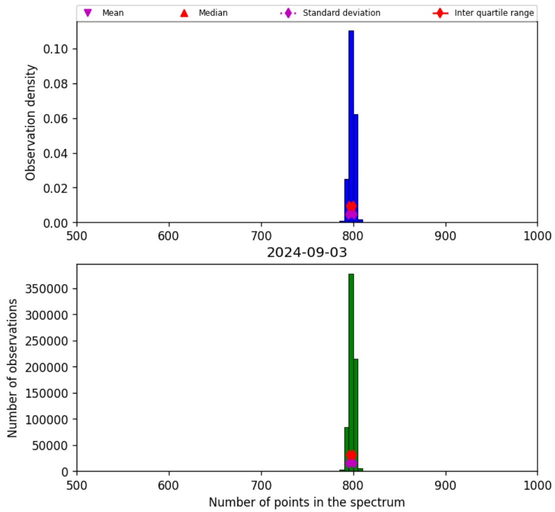
Figure 26: Histogram of “Number of points in the spectrum” for 2024-09-02 to 2024-09-04
