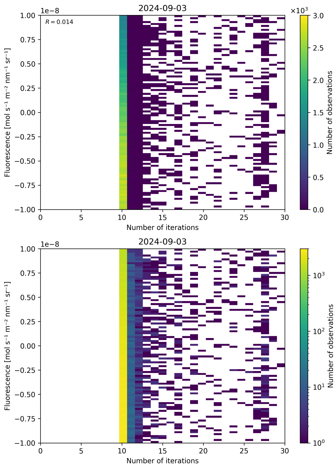
Figure 87: Scatter density plot of “Number of iterations” against “Fluorescence” for 2024-09-02 to 2024-09-04.
