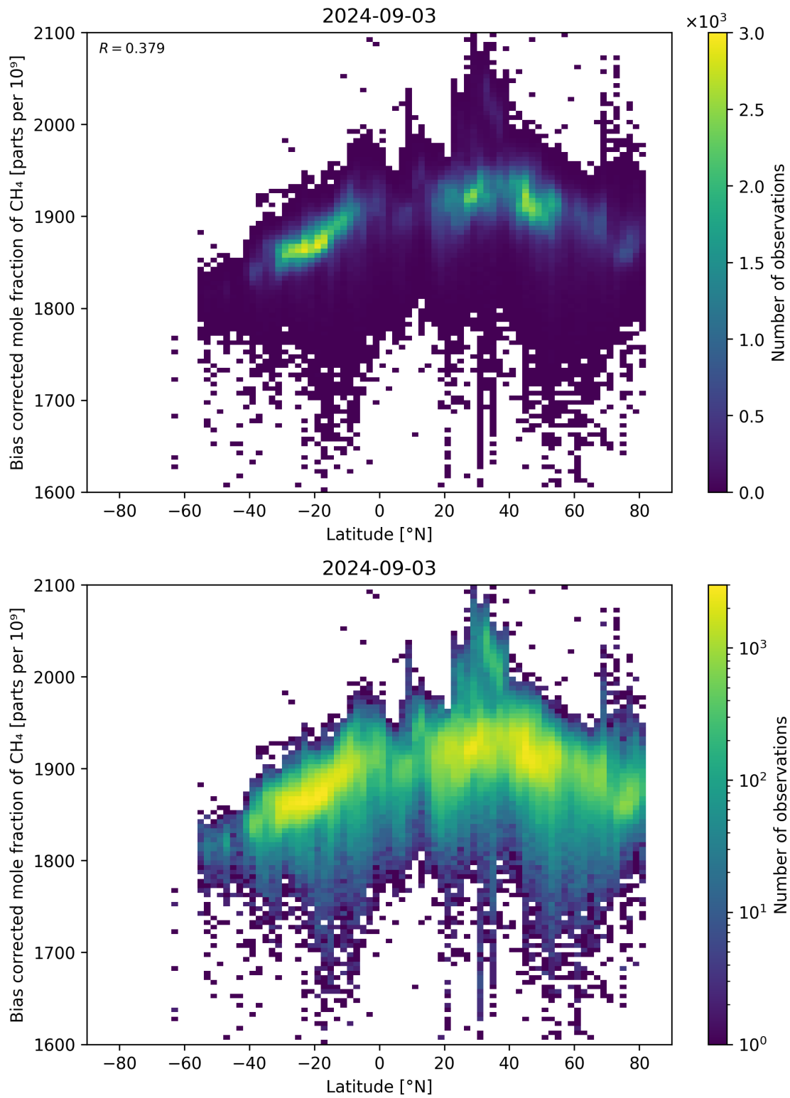
Figure 58: Scatter density plot of “Latitude” against “Bias corrected mole fraction of CH 4 ” for 2024-09-02 to 2024-09-04.
