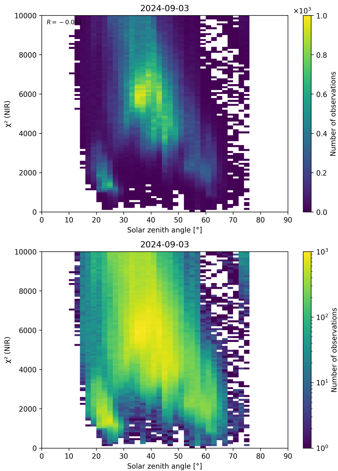
Figure 94: Scatter density plot of “Solar zenith angle” against “ \chi^2 (NIR)” for 2024-09-02 to 2024-09-04.
