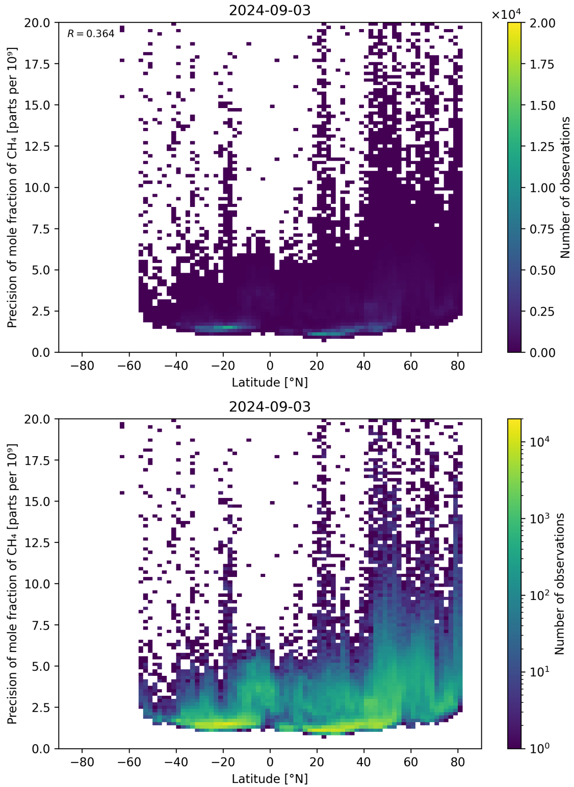
Figure 59: Scatter density plot of “Latitude” against “Precision of mole fraction of \text{CH}_4 ” for 2024-09-02 to 2024-09-04.
