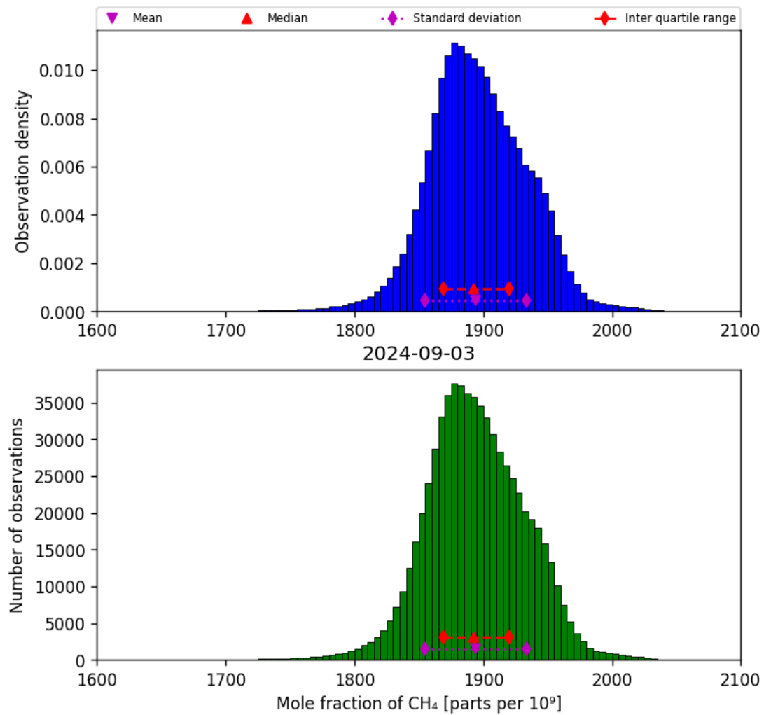
Figure 23: Histogram of “Mole fraction of CH 4 ” for 2024-09-02 to 2024-09-04
