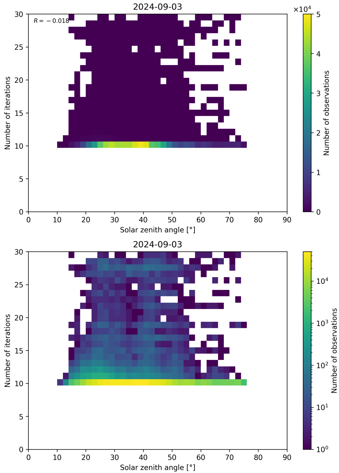
Figure 102: Scatter density plot of “Solar zenith angle” against “Number of iterations” for 2024-09-02 to 2024-09-04.
