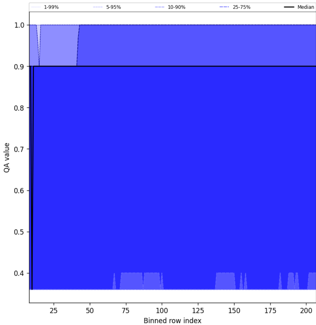
Figure 33: Along track statistics of “QA value” for 2024-09-02 to 2024-09-04
