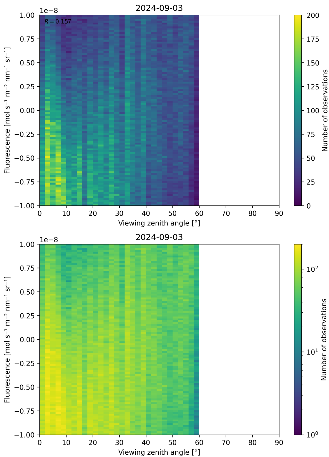
Figure 108: Scatter density plot of “Viewing zenith angle” against “Fluorescence” for 2024-09-02 to 2024-09-04.
