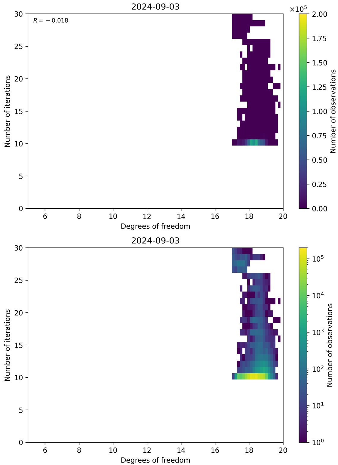
Figure 52: Scatter density plot of “Degrees of freedom” against “Number of iterations” for 2024-09-02 to 2024-09-04.
