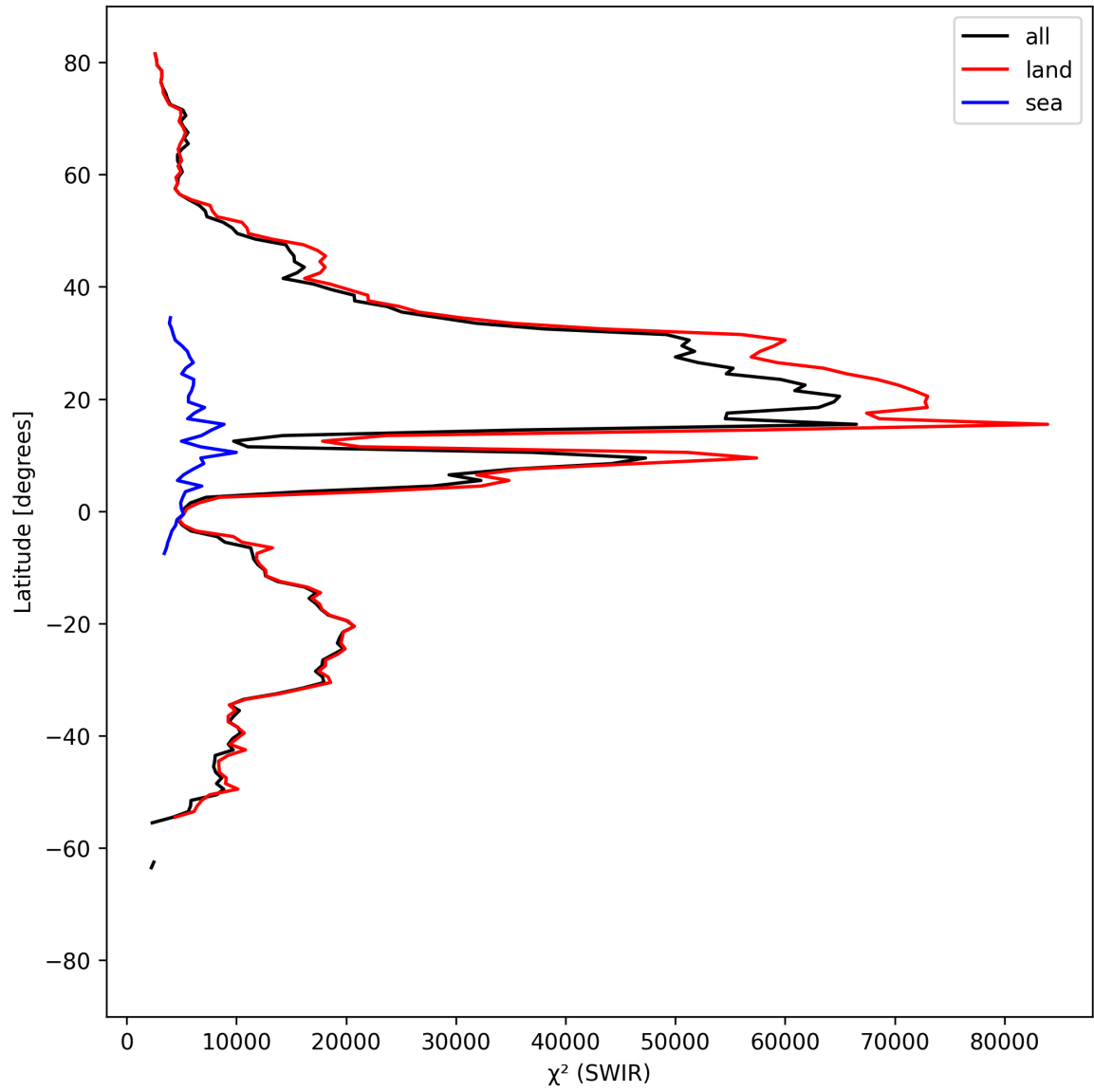
Figure 17: Zonal average of “ \chi^2 (SWIR)” for 2024-09-02 to 2024-09-04.
