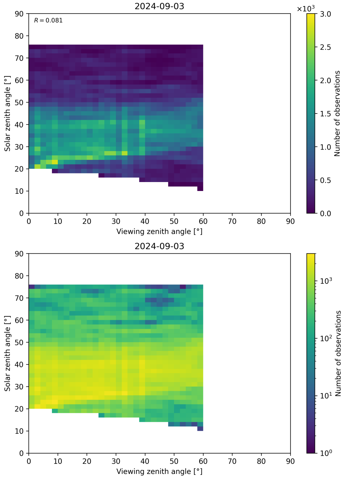
Figure 115: Scatter density plot of “Viewing zenith angle” against “Solar zenith angle” for 2024-09-02 to 2024-09-04.
