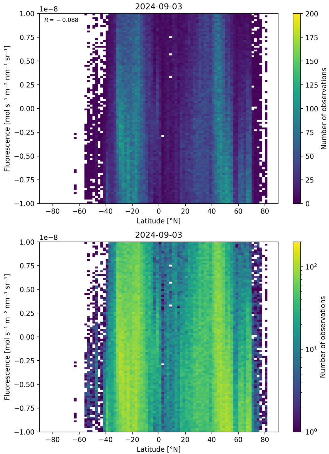
Figure 56: Scatter density plot of “Latitude” against “Fluorescence” for 2024-09-02 to 2024-09-04.
