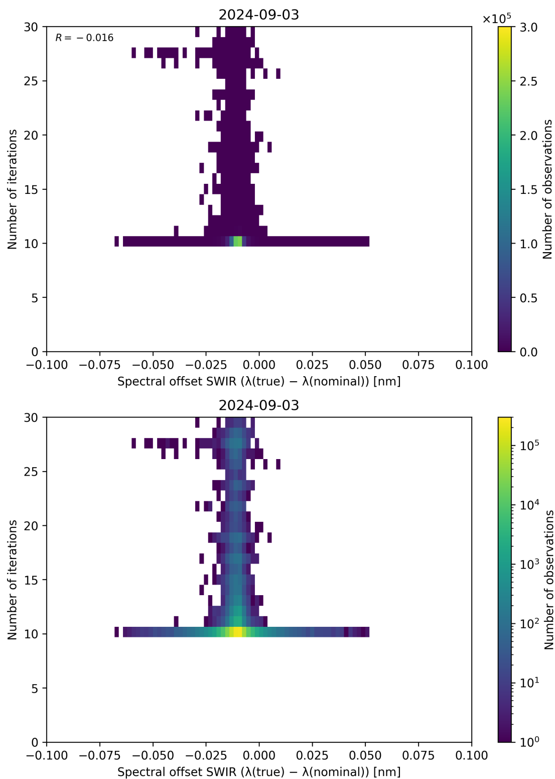
Figure 121: Scatter density plot of “Spectral offset SWIR ( \lambda_{\text{true}} - \lambda_{\text{nominal}} )” against “Number of iterations” for 2024-09-02 to 2024-09-04.
