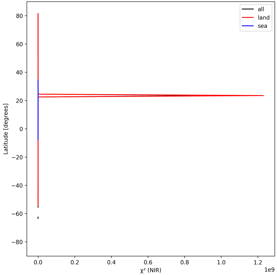
Figure 18: Zonal average of “ \chi^2 (NIR)” for 2024-09-02 to 2024-09-04.
