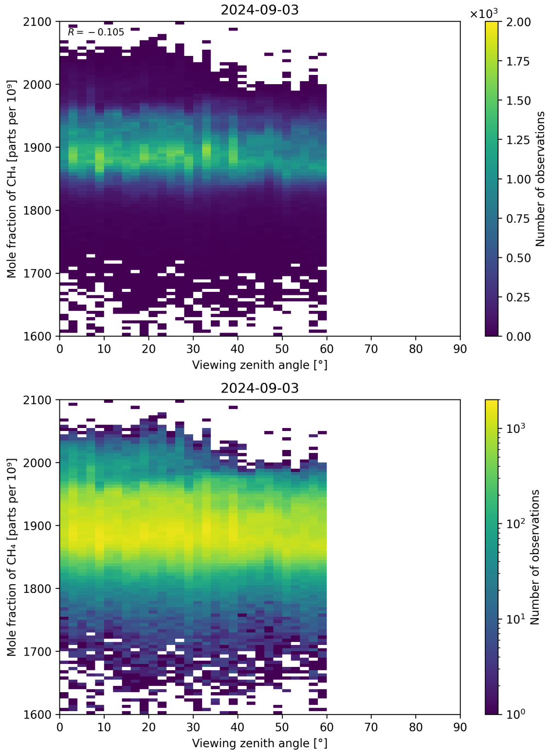
Figure 110: Scatter density plot of “Viewing zenith angle” against “Mole fraction of CH 4 ” for 2024-09-02 to 2024-09-04.
