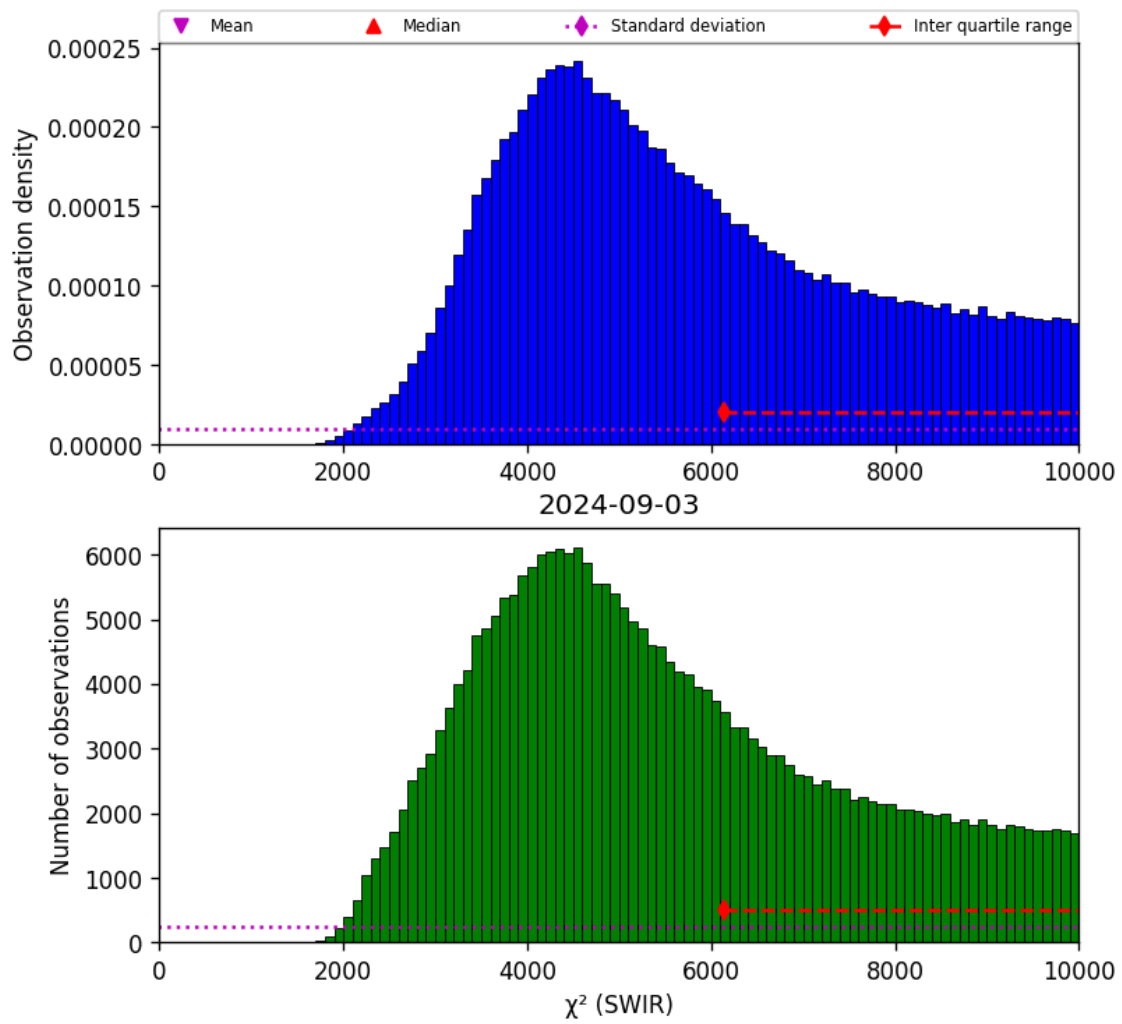
Figure 28: Histogram of " \chi^2 (SWIR)" for 2024-09-02 to 2024-09-04
