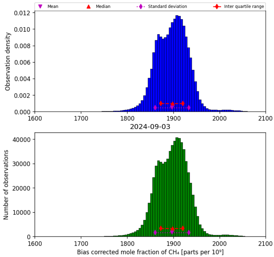
Figure 25: Histogram of “Bias corrected mole fraction of CH 4 ” for 2024-09-02 to 2024-09-04
