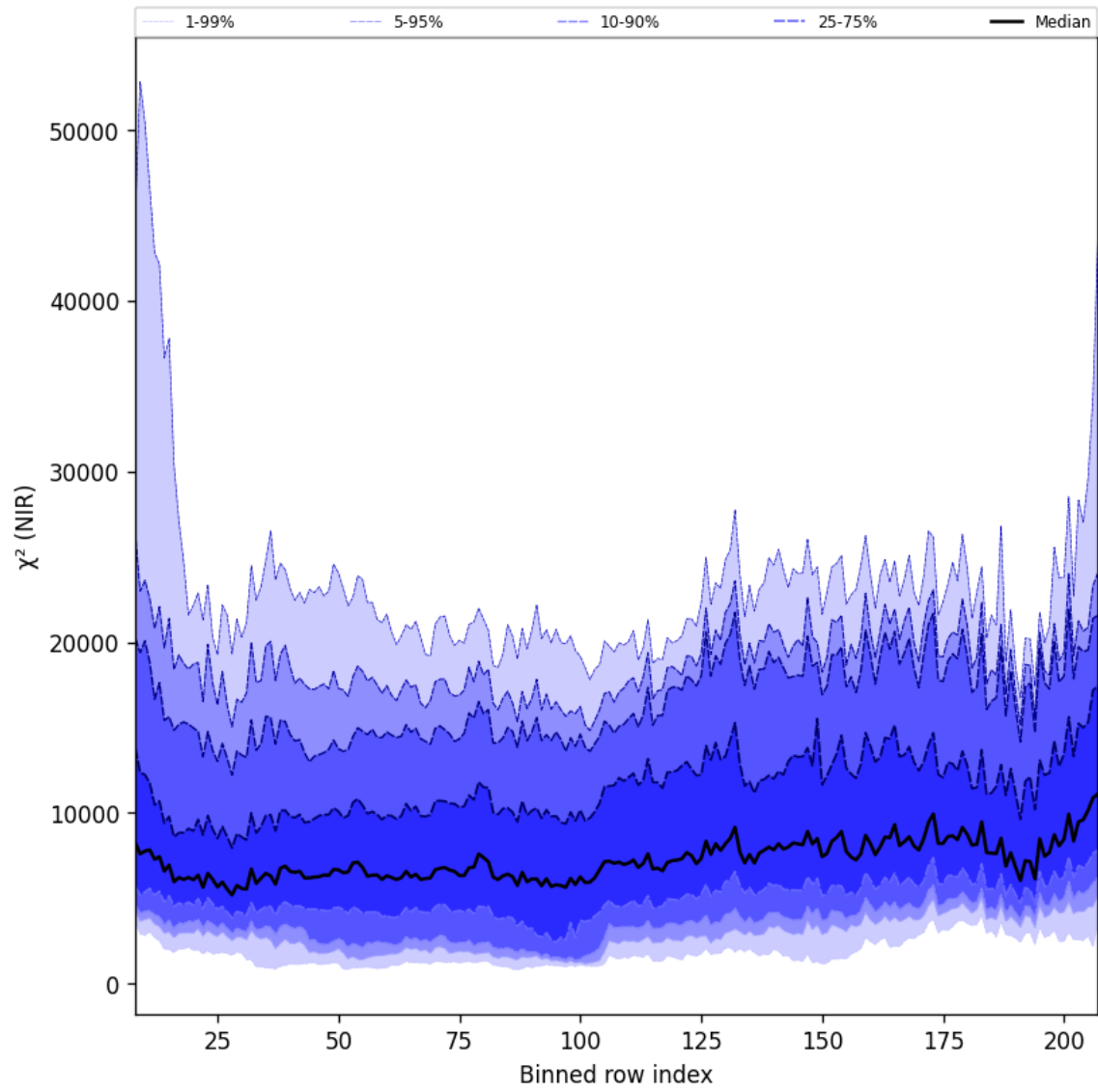
Figure 40: Along track statistics of “ \chi^2 (NIR)” for 2024-09-02 to 2024-09-04
