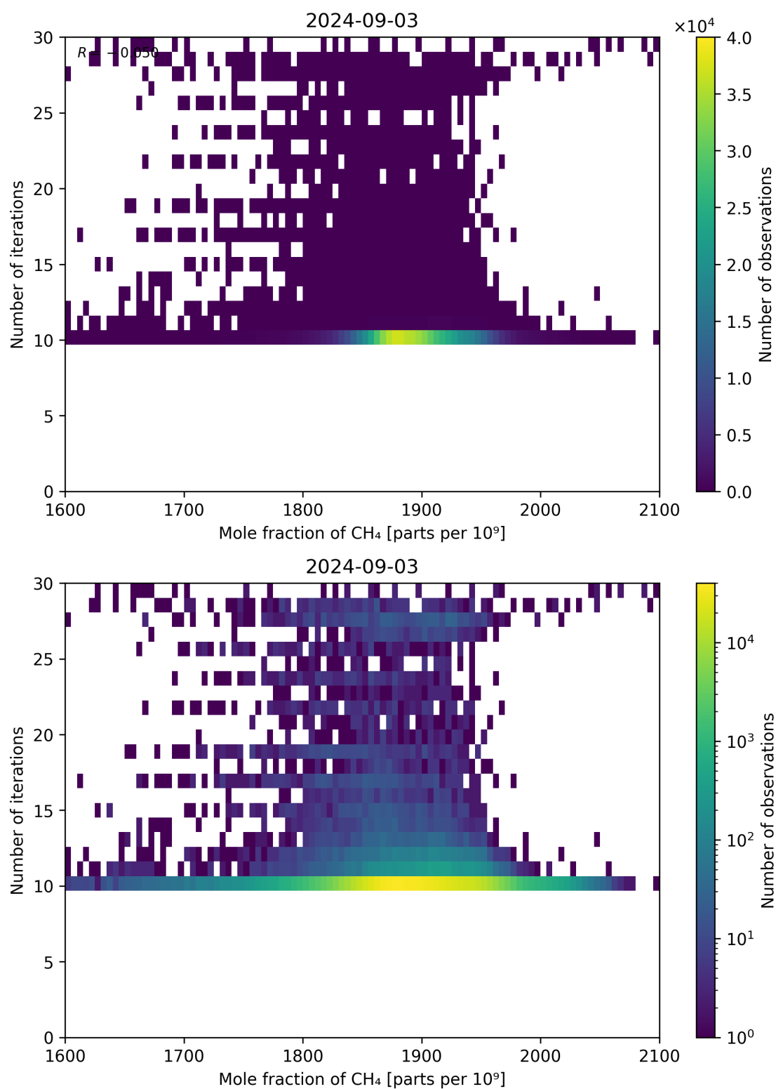
Figure 76: Scatter density plot of “Mole fraction of CH 4 ” against “Number of iterations” for 2024-09-02 to 2024-09-04.
