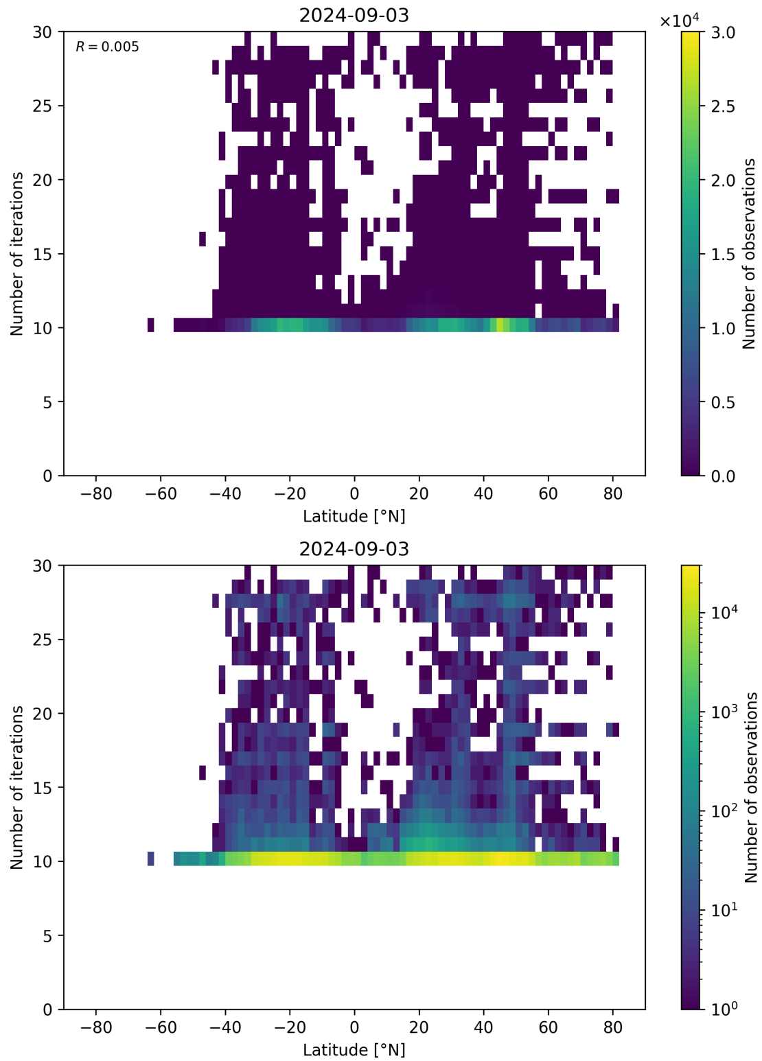
Figure 60: Scatter density plot of “Latitude” against “Number of iterations” for 2024-09-02 to 2024-09-04.
