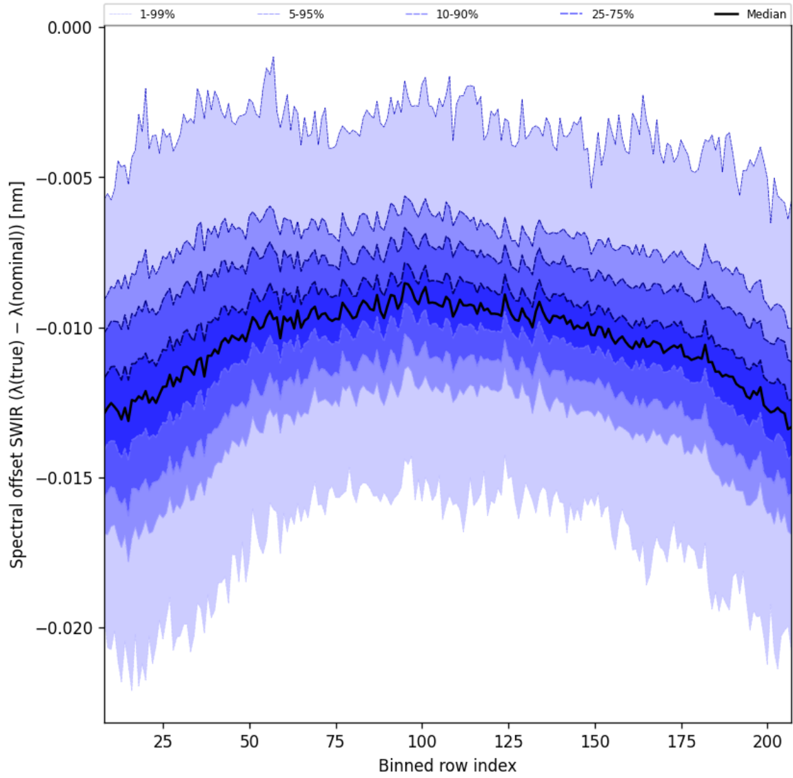
Figure 38: Along track statistics of “Spectral offset SWIR ( \lambda_{\text{true}} - \lambda_{\text{nominal}} )” for 2024-09-02 to 2024-09-04
