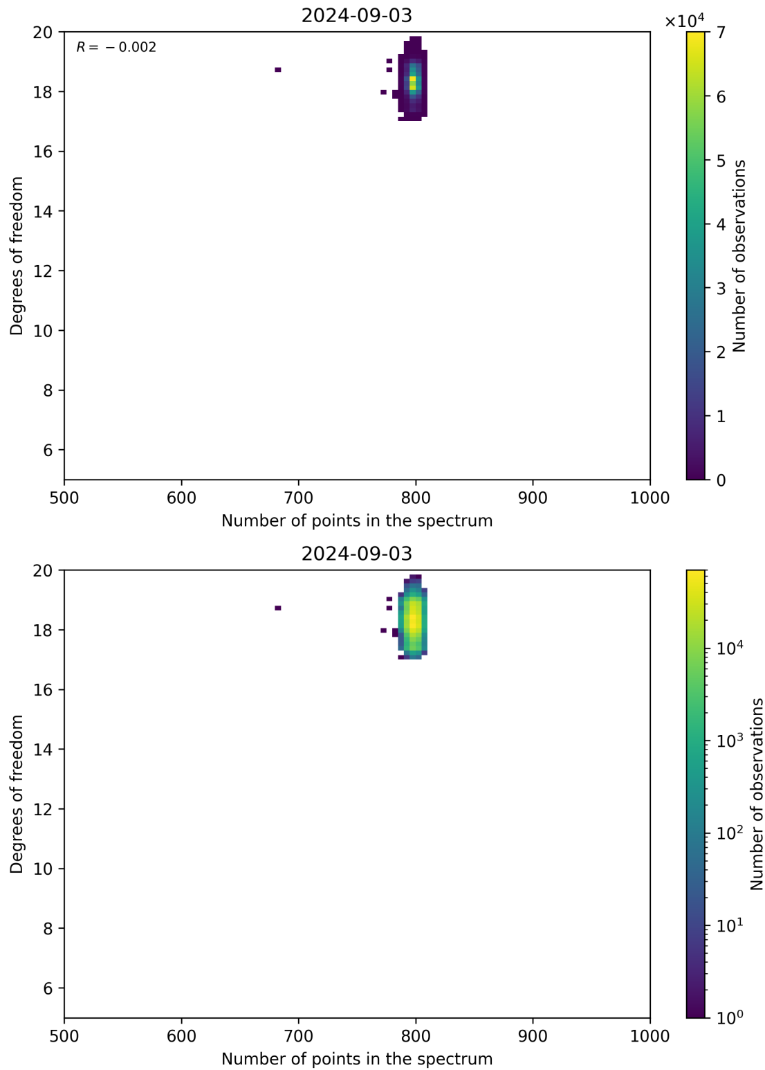
Figure 90: Scatter density plot of “Number of points in the spectrum” against “Degrees of freedom” for 2024-09-02 to 2024-09-04.
