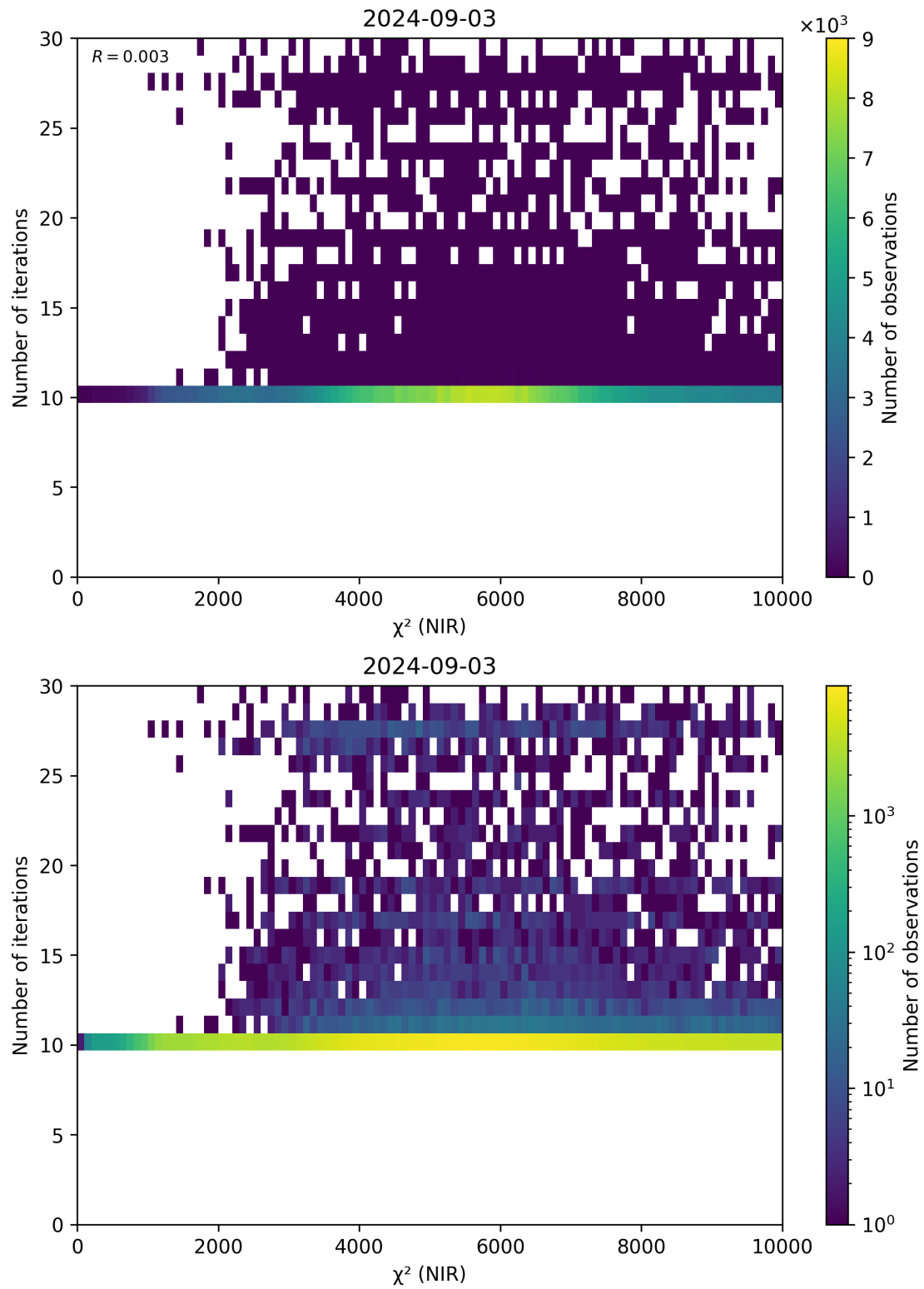
Figure 46: Scatter density plot of “ \chi^2 (NIR)” against “Number of iterations” for 2024-09-02 to 2024-09-04.
