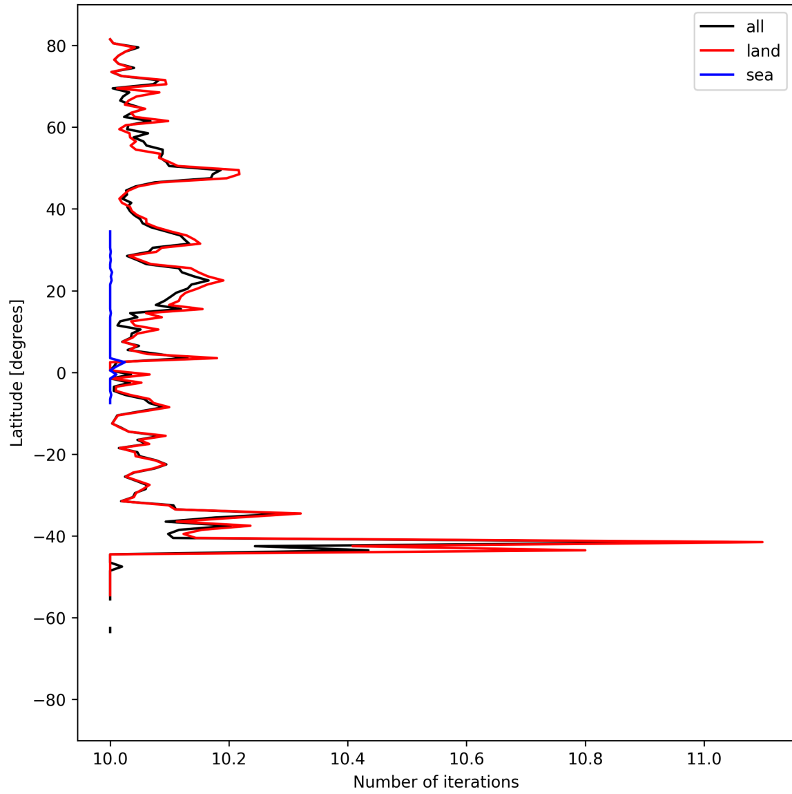
Figure 20: Zonal average of “Number of iterations” for 2024-09-02 to 2024-09-04.
