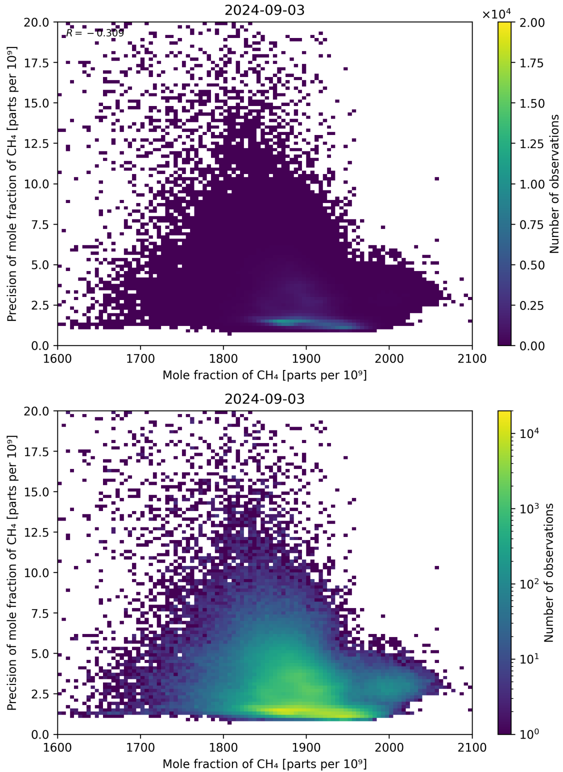
Figure 75: Scatter density plot of “Mole fraction of CH 4 ” against “Precision of mole fraction of CH 4 ” for 2024-09-02 to 2024-09-04.
