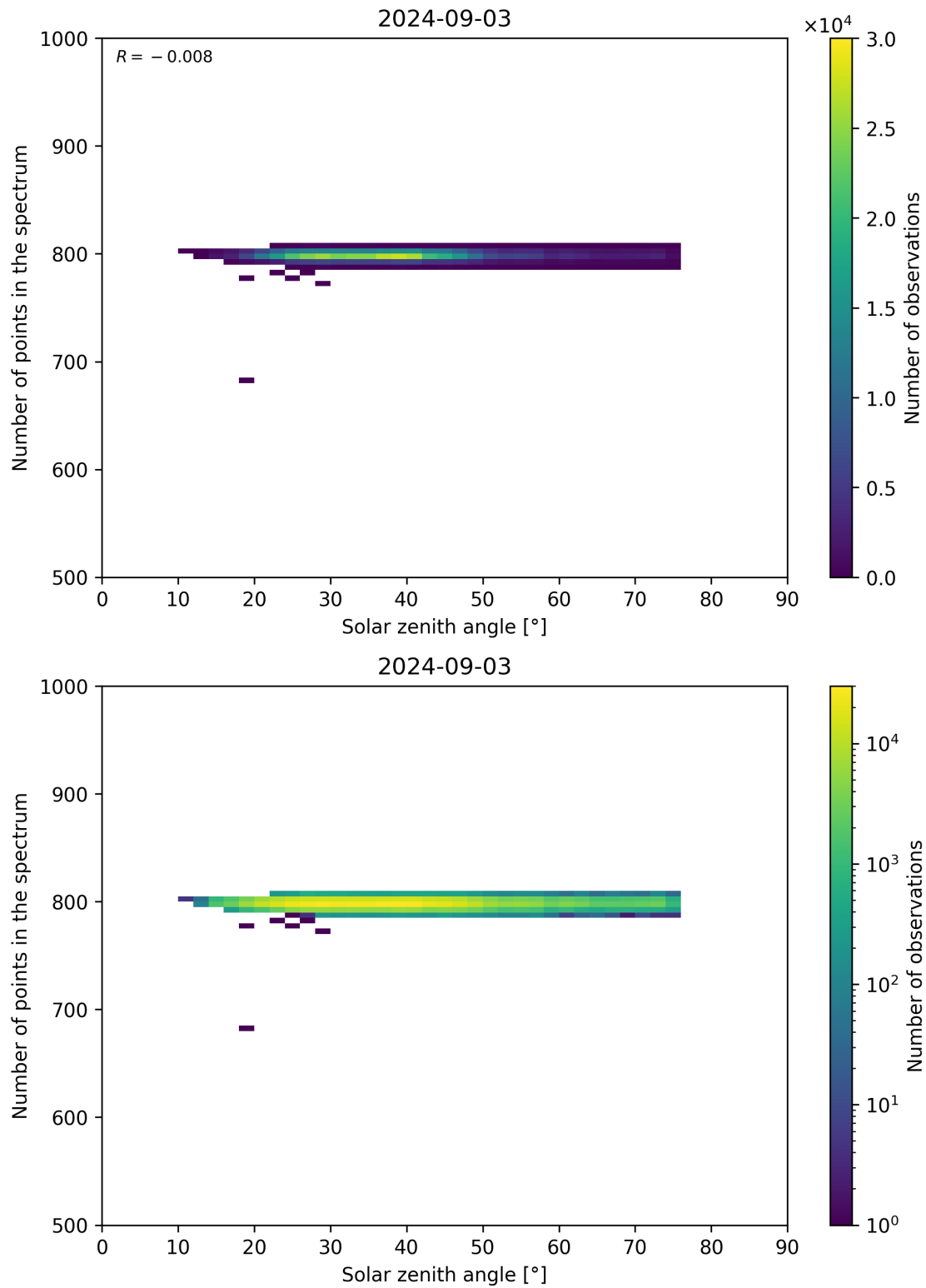
Figure 103: Scatter density plot of “Solar zenith angle” against “Number of points in the spectrum” for 2024-09-02 to 2024-09-04.
