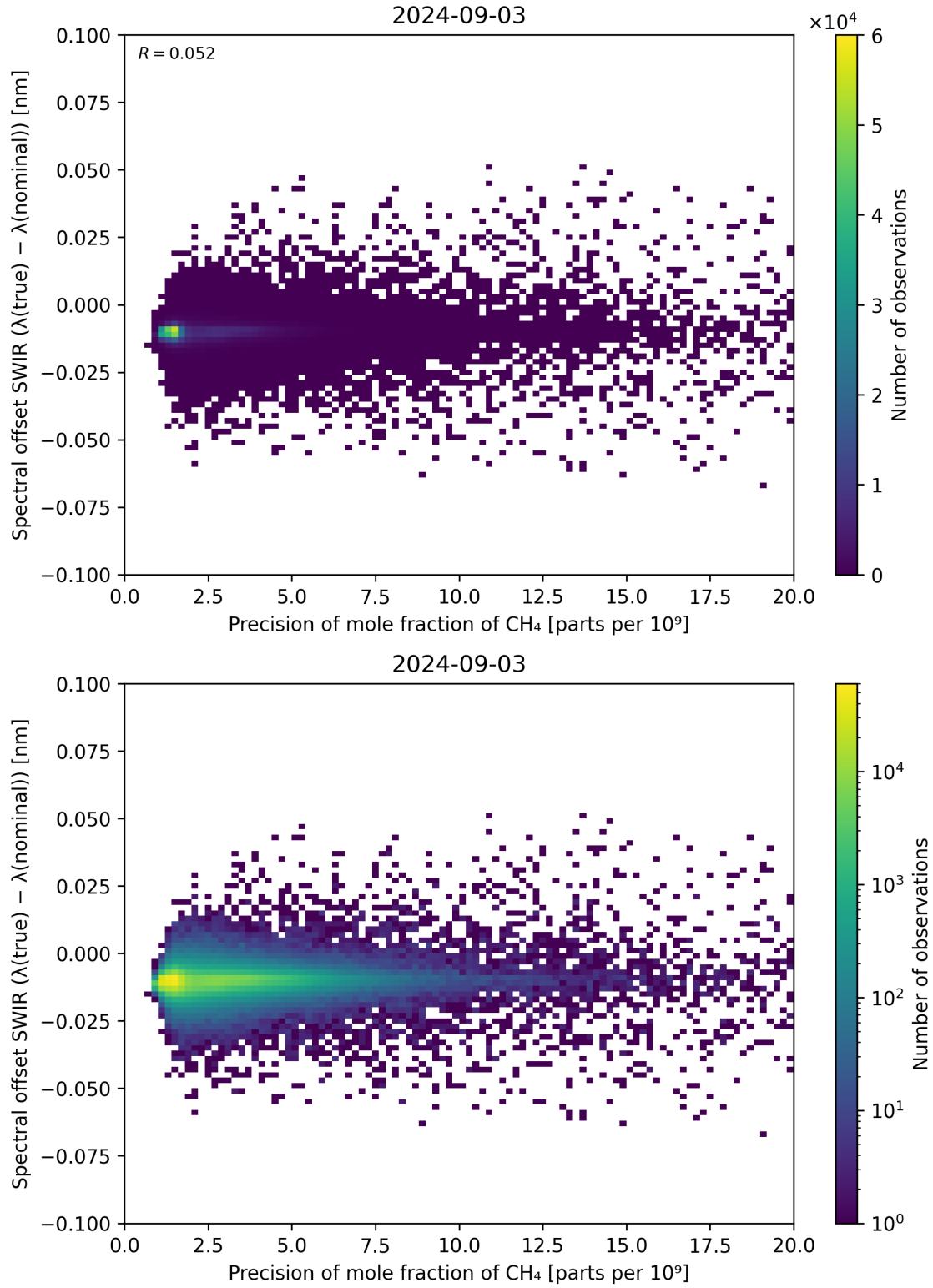
Figure 85: Scatter density plot of “Precision of mole fraction of \text{CH}_4 ” against “Spectral offset SWIR ( \lambda_{\text{true}} - \lambda_{\text{nominal}} )” for 2024-09-02 to 2024-09-04.
