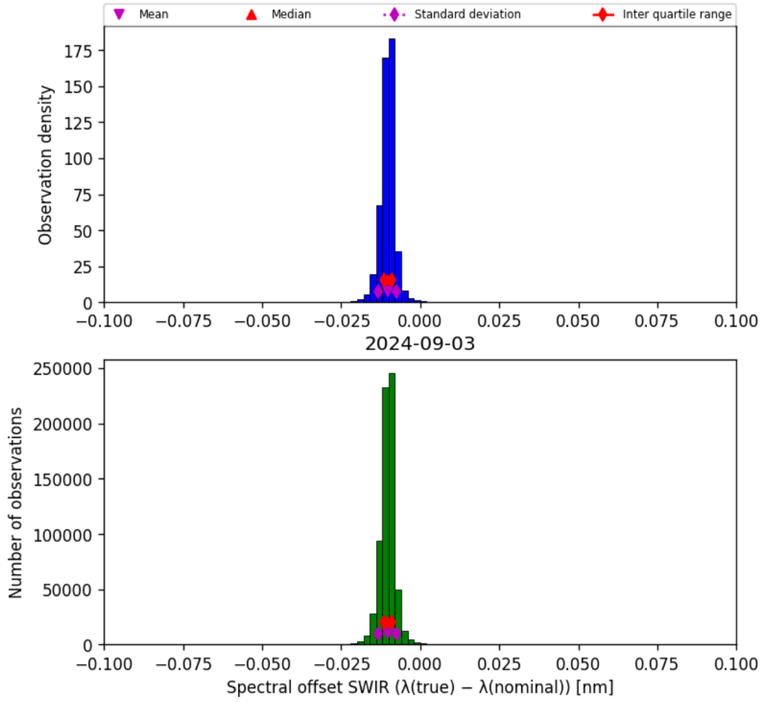
Figure 27: Histogram of “Spectral offset SWIR ( \lambda_{\text{true}} - \lambda_{\text{nominal}} )” for 2024-09-02 to 2024-09-04
