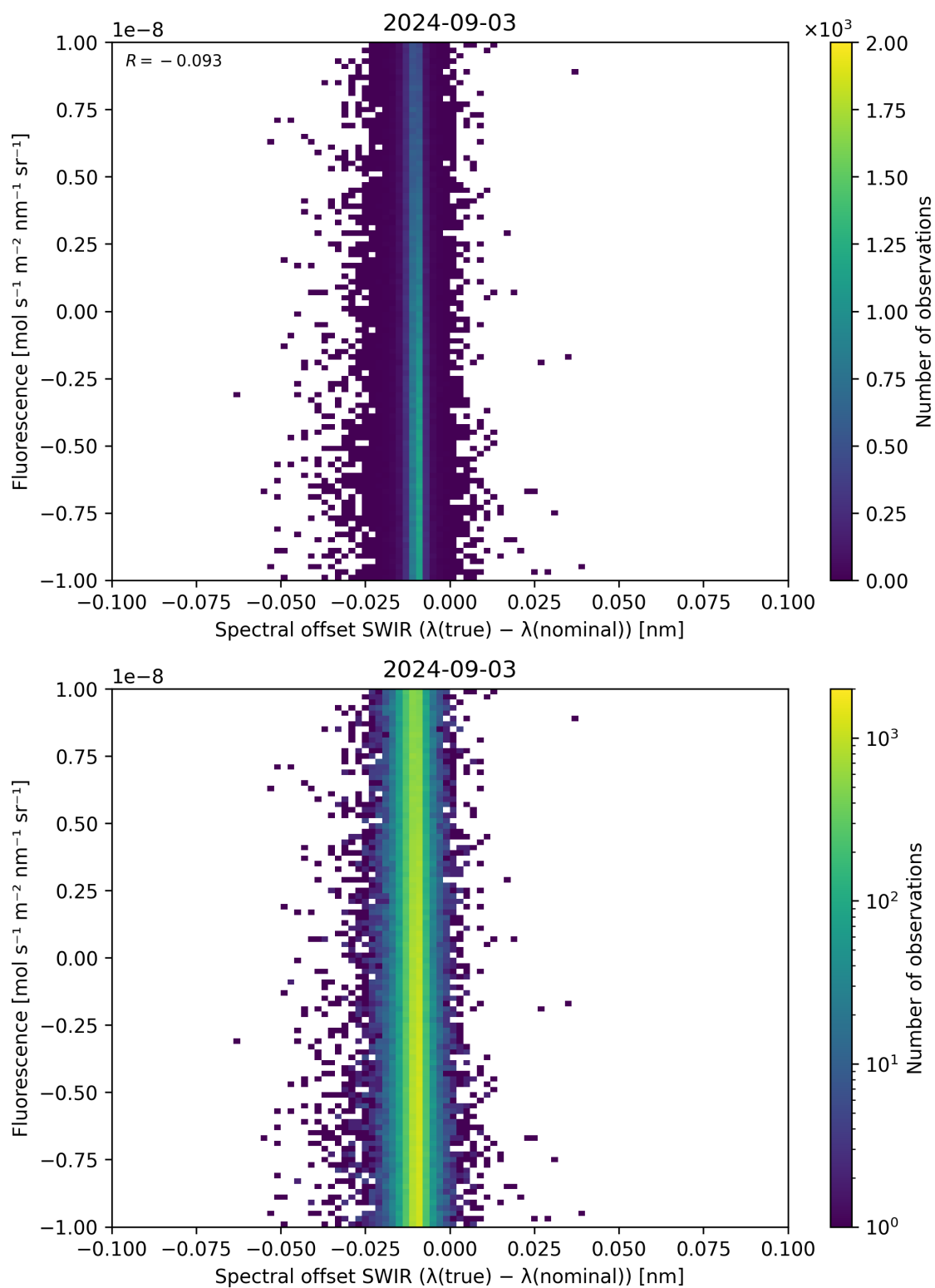
Figure 120: Scatter density plot of “Spectral offset SWIR ( \lambda_{\text{true}} - \lambda_{\text{nominal}} )” against “Fluorescence” for 2024-09-02 to 2024-09-04.
