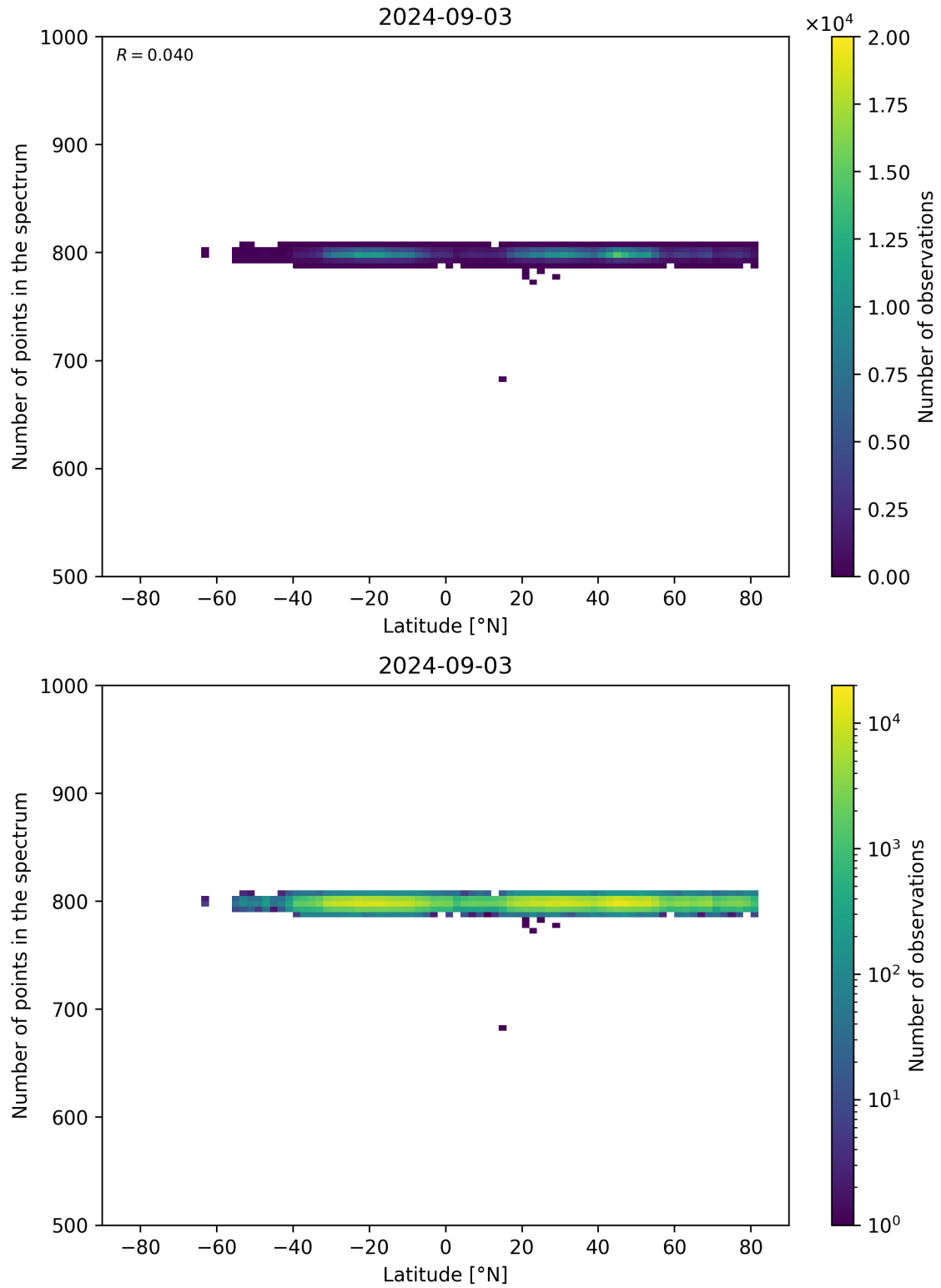
Figure 61: Scatter density plot of “Latitude” against “Number of points in the spectrum” for 2024-09-02 to 2024-09-04.
