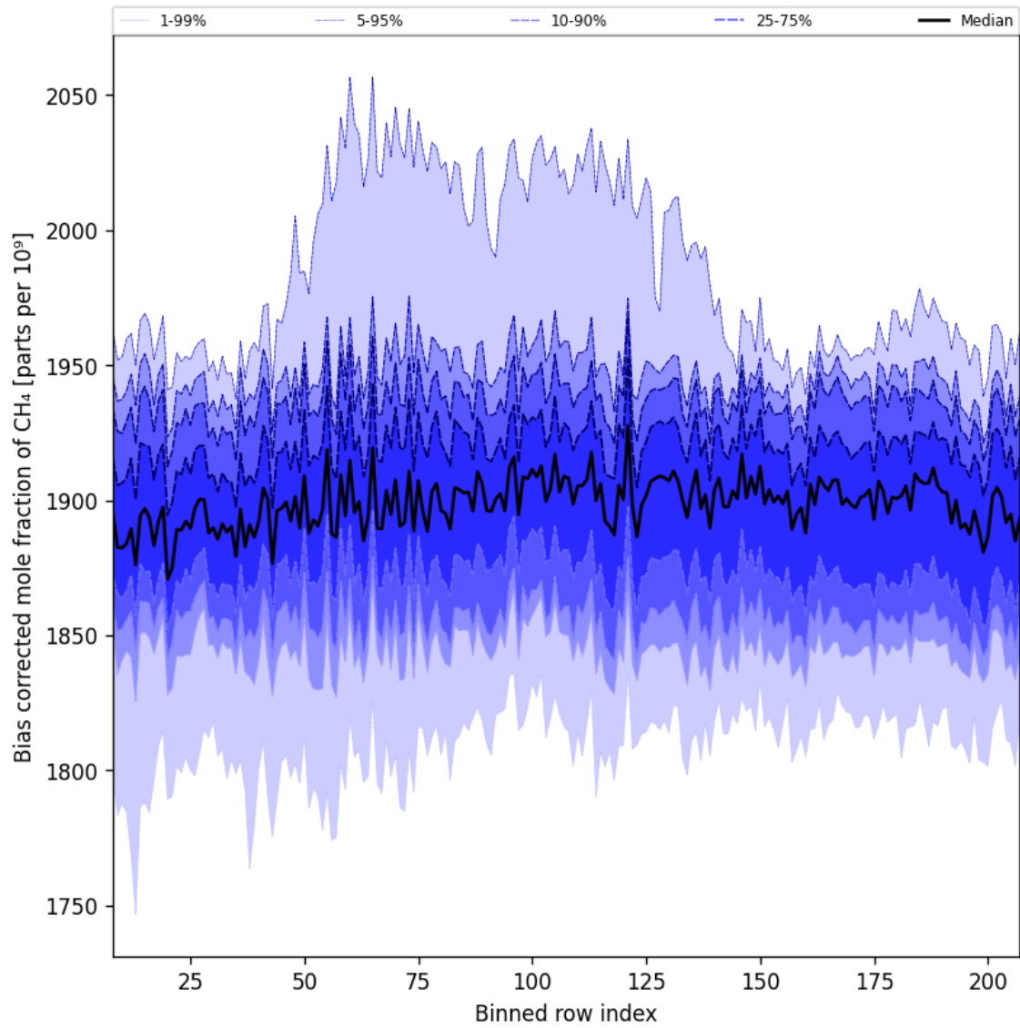
Figure 36: Along track statistics of “Bias corrected mole fraction of CH 4 ” for 2024-09-02 to 2024-09-04
