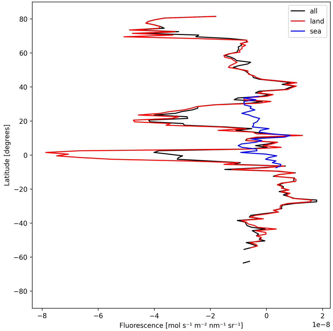
Figure 21: Zonal average of “Fluorescence” for 2024-09-02 to 2024-09-04.
