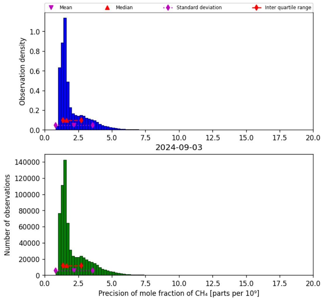
Figure 24: Histogram of “Precision of mole fraction of CH 4 ” for 2024-09-02 to 2024-09-04
