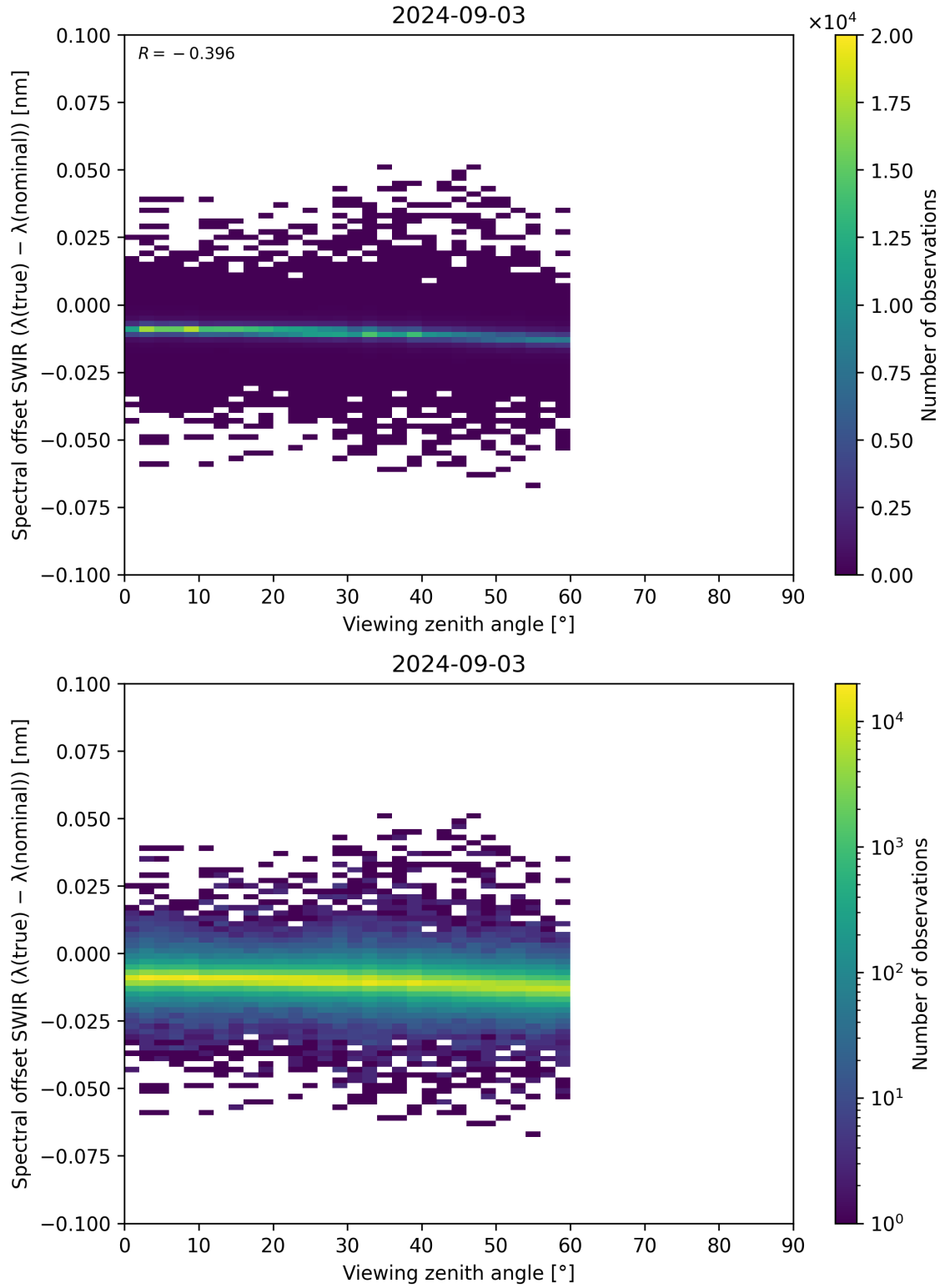
Figure 116: Scatter density plot of “Viewing zenith angle” against “Spectral offset SWIR ( \lambda_{\text{true}} - \lambda_{\text{nominal}} )” for 2024-09-02 to 2024-09-04.
