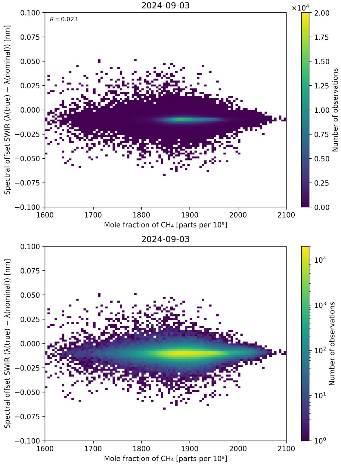
Figure 86: Scatter density plot of “Mole fraction of CH 4 ” against “Spectral offset SWIR ( \lambda_{\text{true}} - \lambda_{\text{nominal}} )” for 2024-09-02 to 2024-09-04.
