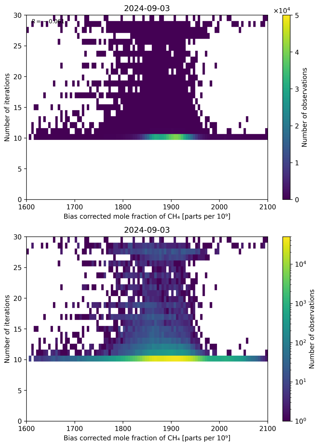
Figure 67: Scatter density plot of “Bias corrected mole fraction of CH 4 ” against “Number of iterations” for 2024-09-02 to 2024-09-04.
