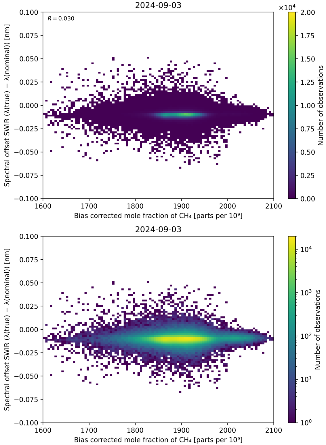
Figure 69: Scatter density plot of “Bias corrected mole fraction of \text{CH}_4 ” against “Spectral offset SWIR ( \lambda_{\text{true}} - \lambda_{\text{nominal}} )” for 2024-09-02 to 2024-09-04.
