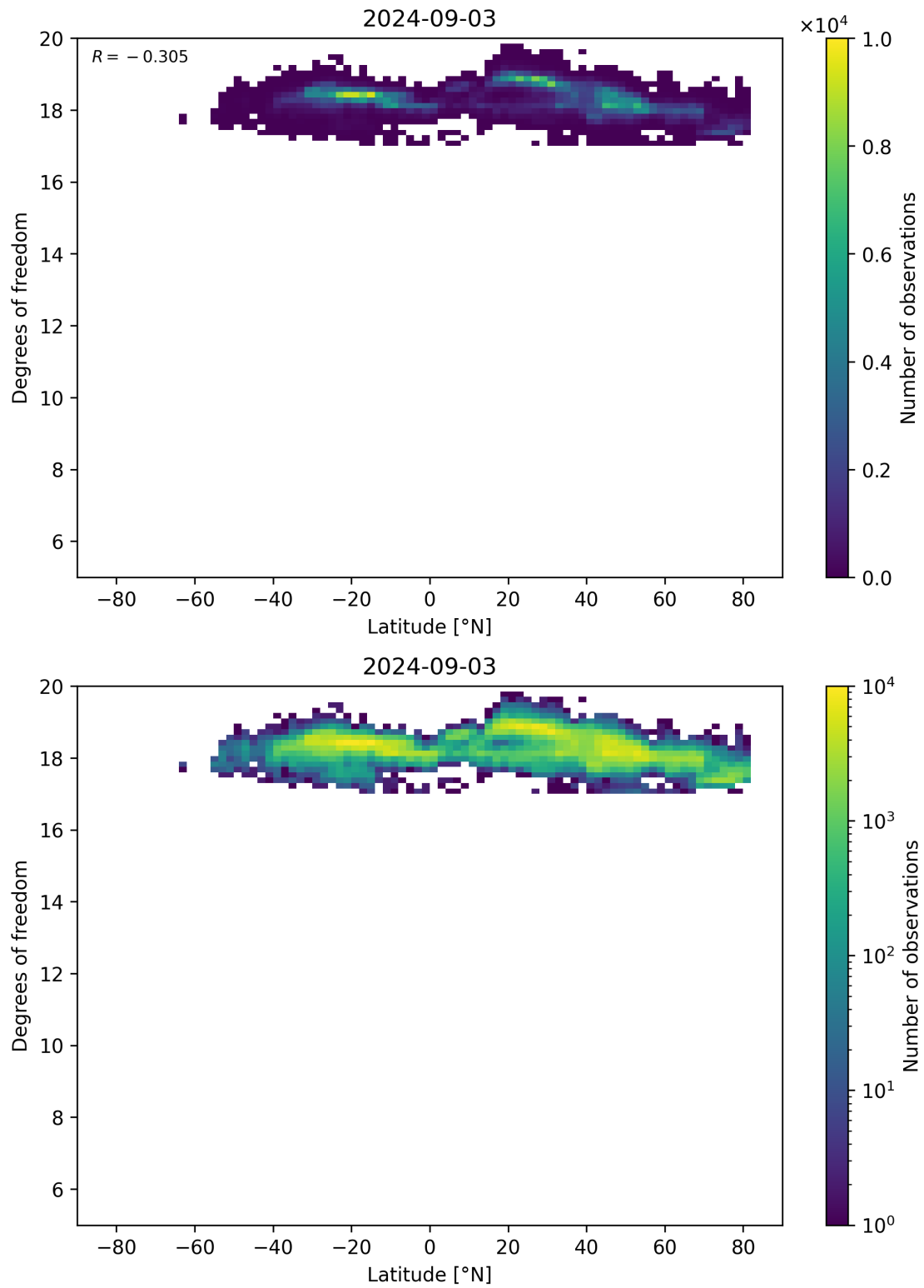
Figure 55: Scatter density plot of “Latitude” against “Degrees of freedom” for 2024-09-02 to 2024-09-04.
