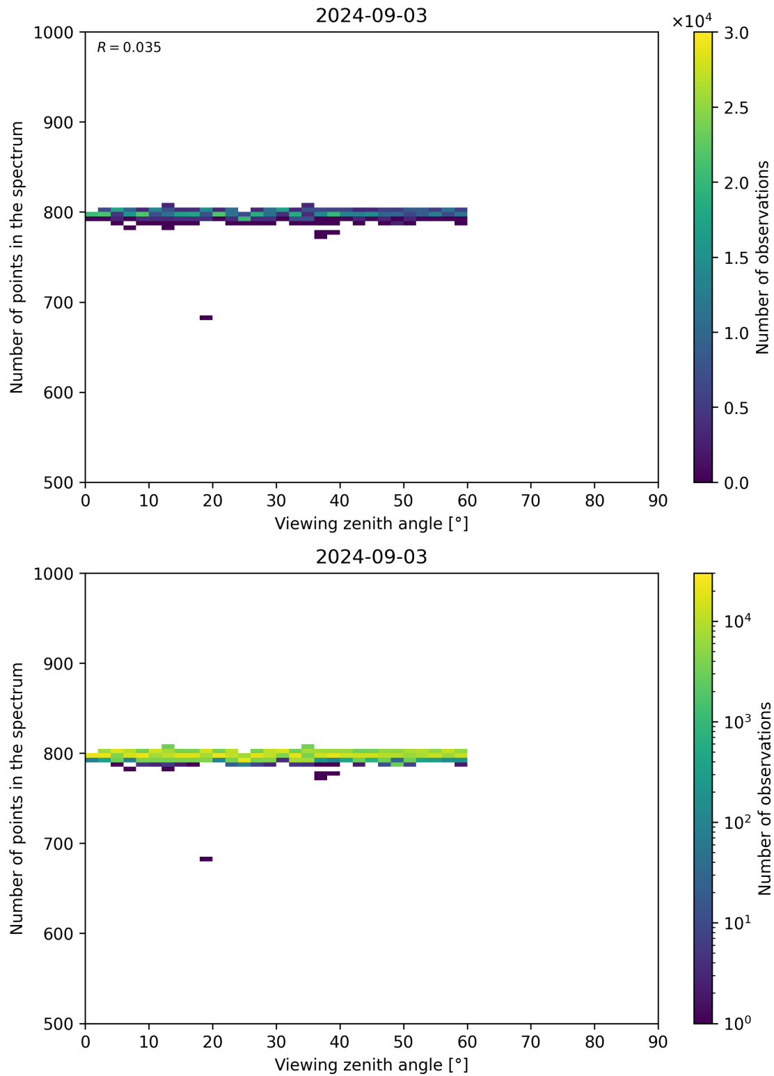
Figure 114: Scatter density plot of “Viewing zenith angle” against “Number of points in the spectrum” for 2024-09-02 to 2024-09-04.
