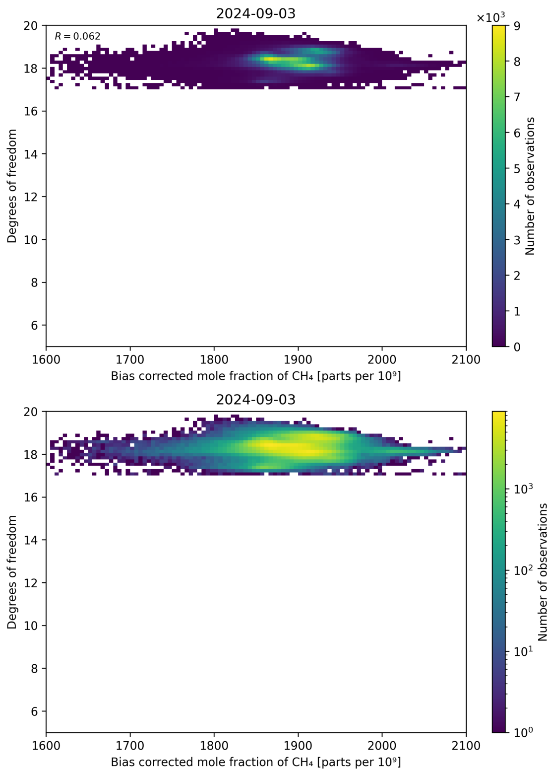
Figure 65: Scatter density plot of “Bias corrected mole fraction of CH 4 ” against “Degrees of freedom” for 2024-09-02 to 2024-09-04.
