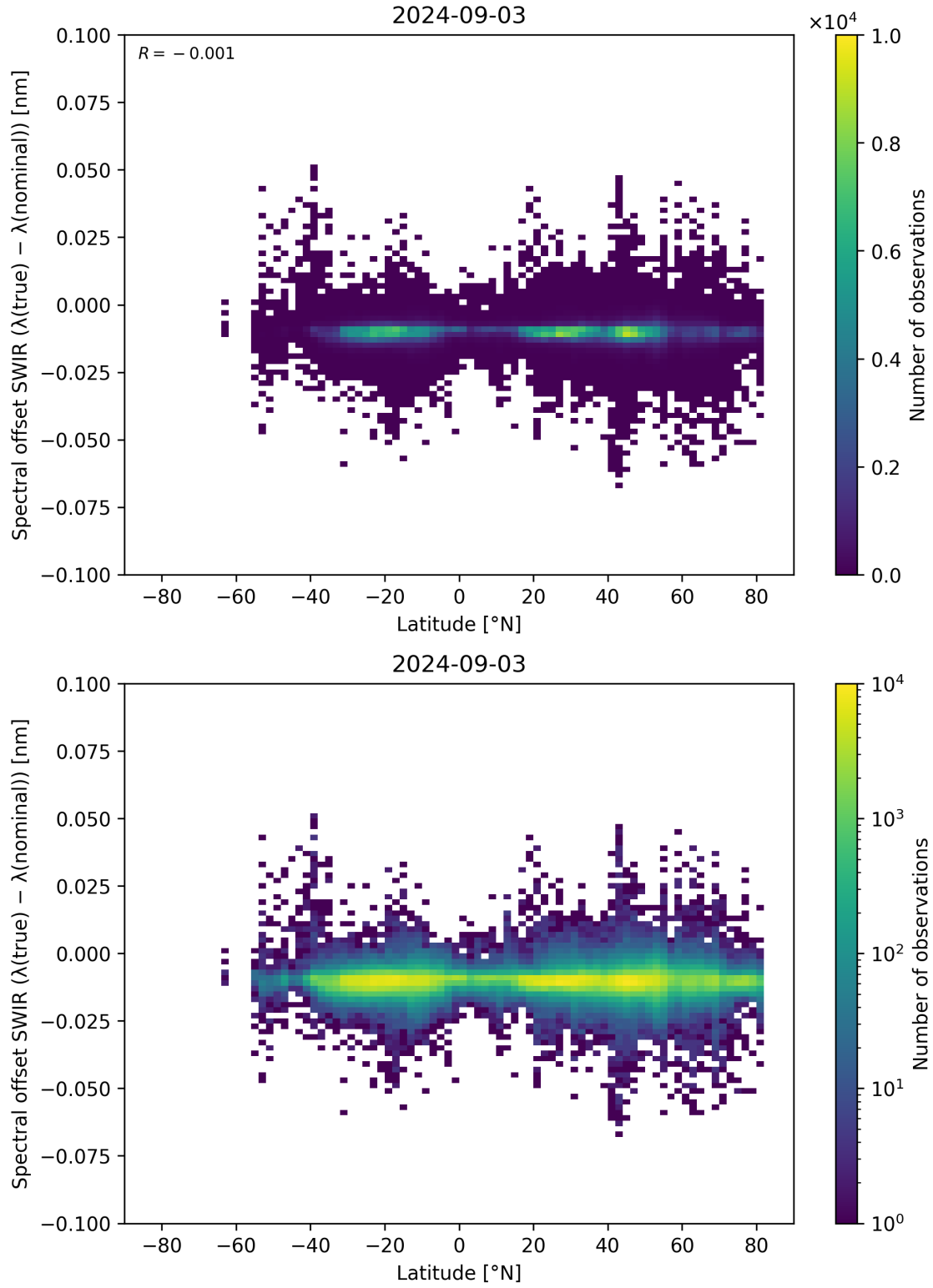
Figure 62: Scatter density plot of “Latitude” against “Spectral offset SWIR ( \lambda_{\text{true}} - \lambda_{\text{nominal}} )” for 2024-09-02 to 2024-09-04.
