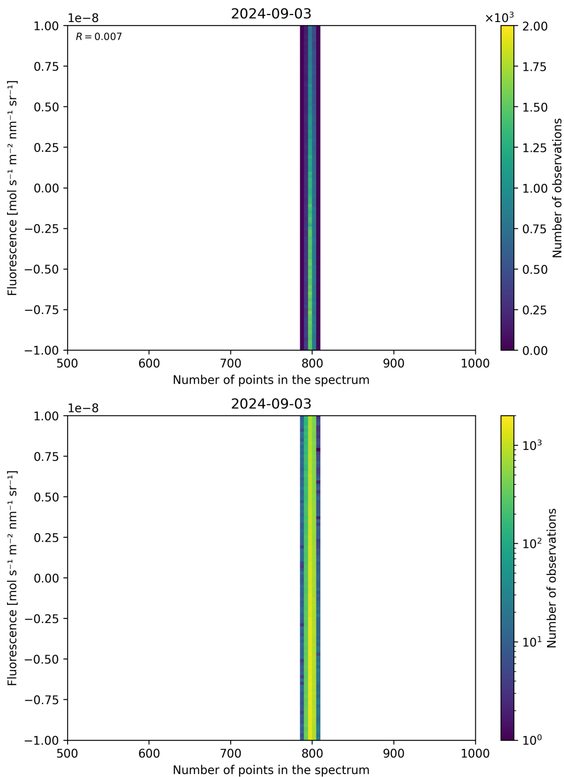
Figure 91: Scatter density plot of “Number of points in the spectrum” against “Fluorescence” for 2024-09-02 to 2024-09-04.
