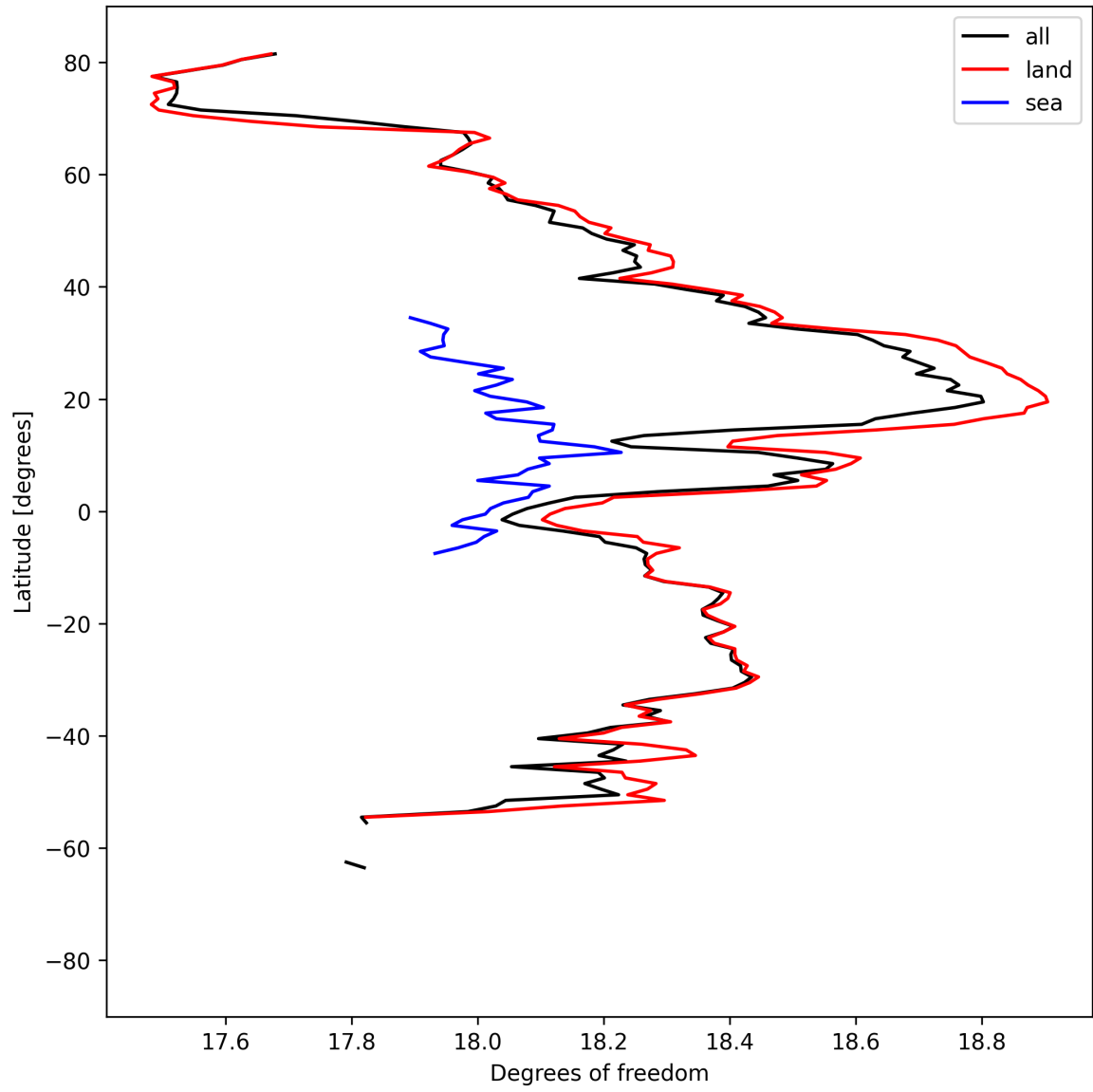
Figure 19: Zonal average of “Degrees of freedom” for 2024-09-02 to 2024-09-04.
