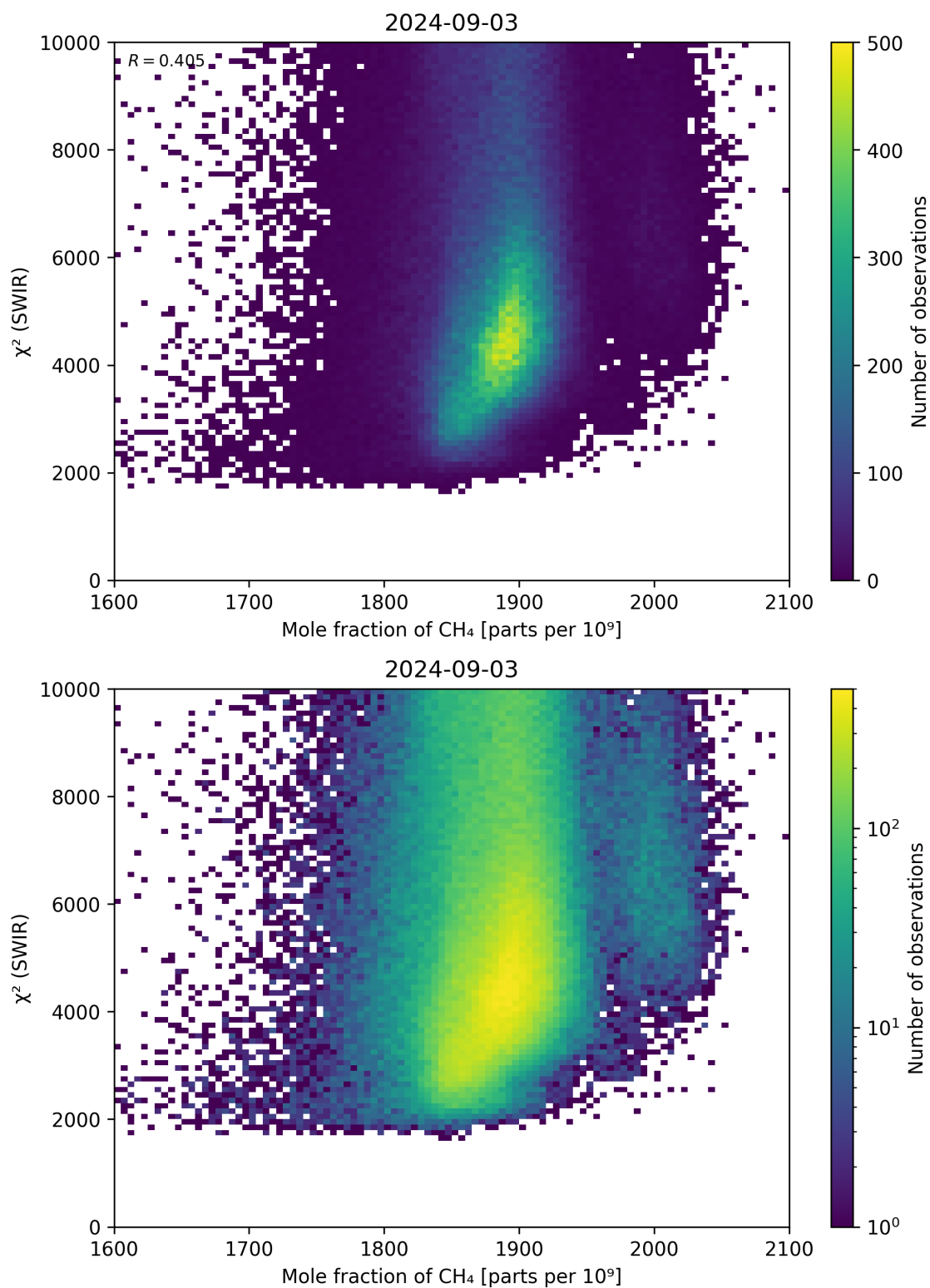
Figure 71: Scatter density plot of “Mole fraction of \text{CH}_4 ” against “ \chi^2 (SWIR)” for 2024-09-02 to 2024-09-04.
