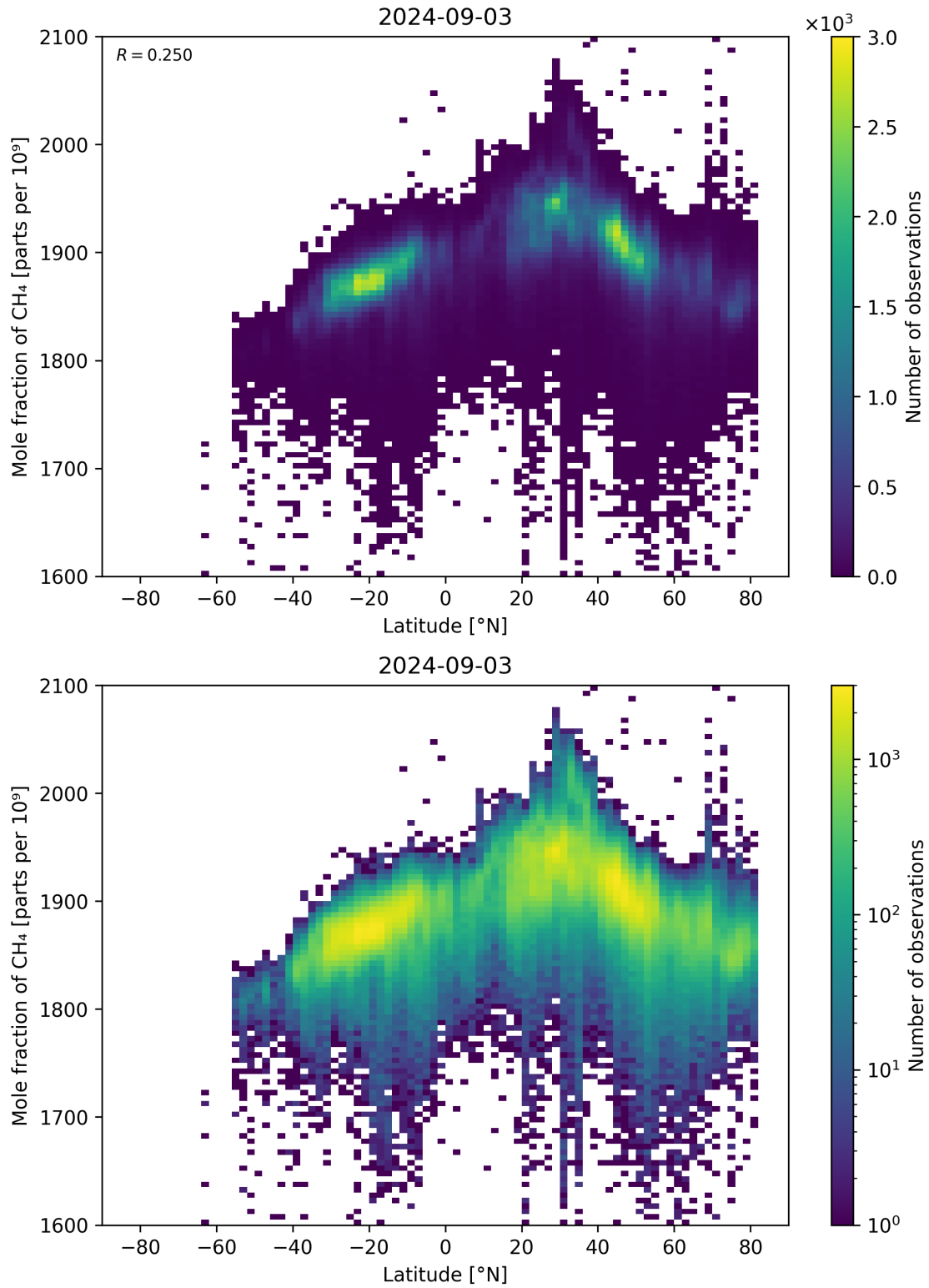
Figure 57: Scatter density plot of “Latitude” against “Mole fraction of CH 4 ” for 2024-09-02 to 2024-09-04.
