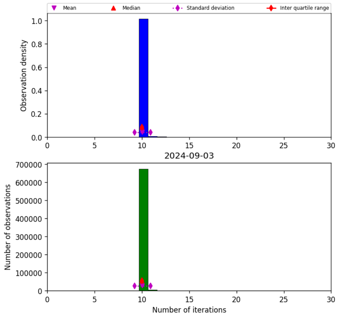
Figure 31: Histogram of “Number of iterations” for 2024-09-02 to 2024-09-04
