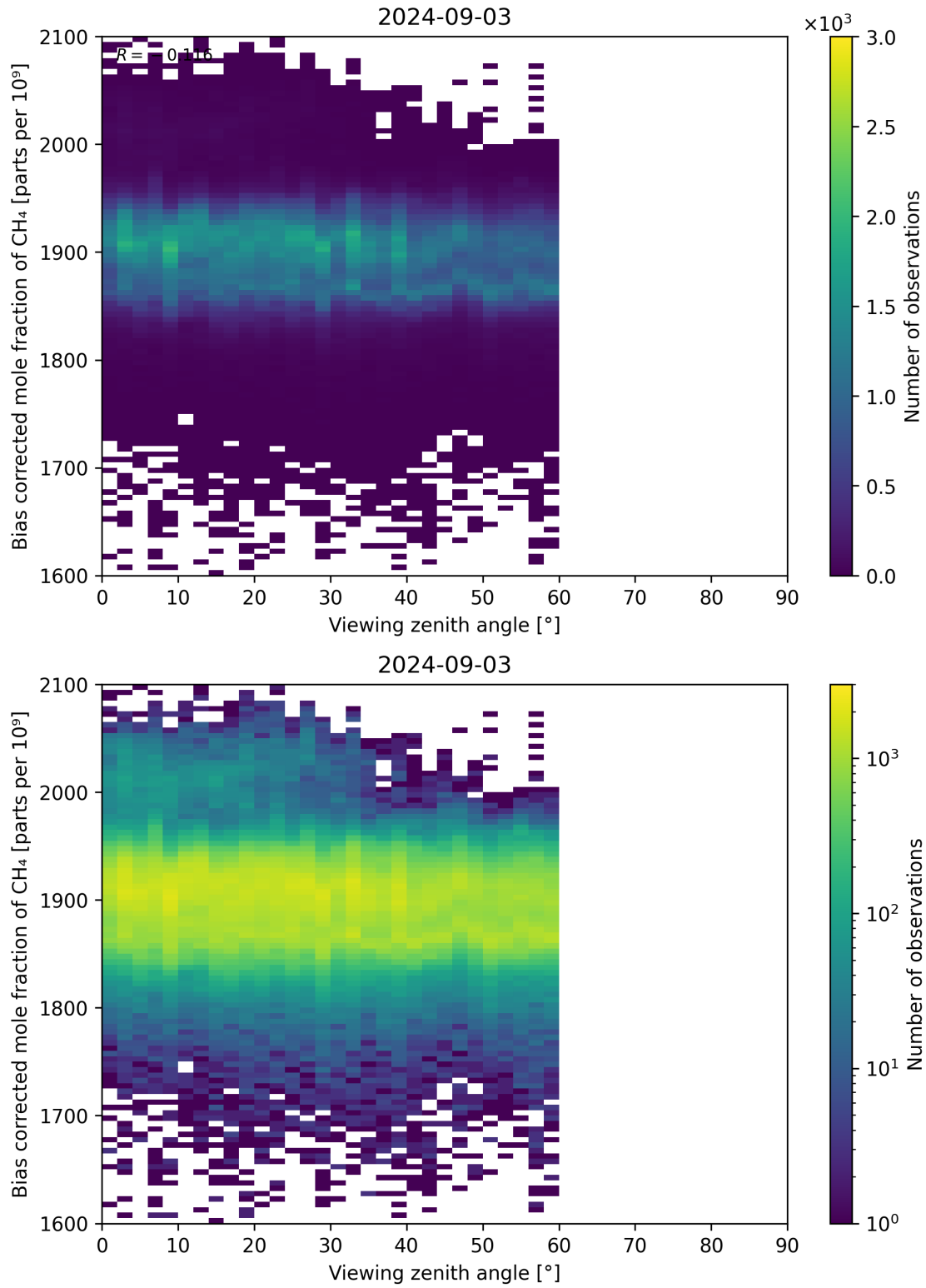
Figure 111: Scatter density plot of “Viewing zenith angle” against “Bias corrected mole fraction of CH 4 ” for 2024-09-02 to 2024-09-04.
