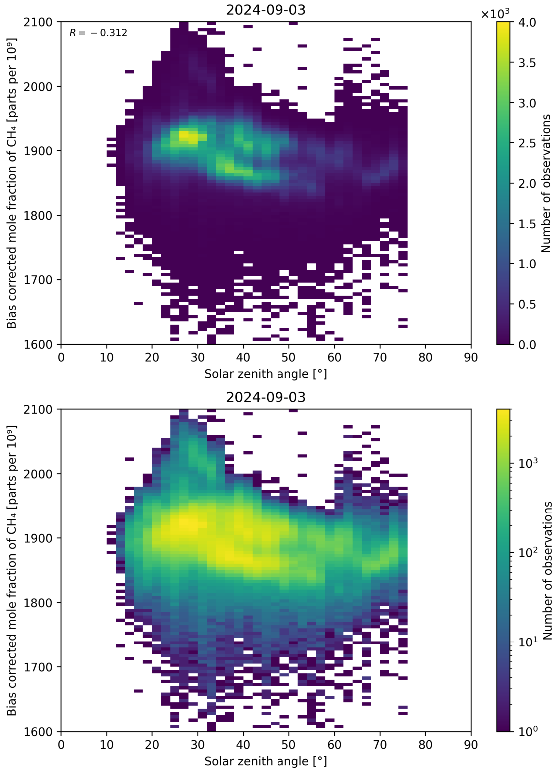
Figure 100: Scatter density plot of “Solar zenith angle” against “Bias corrected mole fraction of \text{CH}_4 ” for 2024-09-02 to 2024-09-04.
