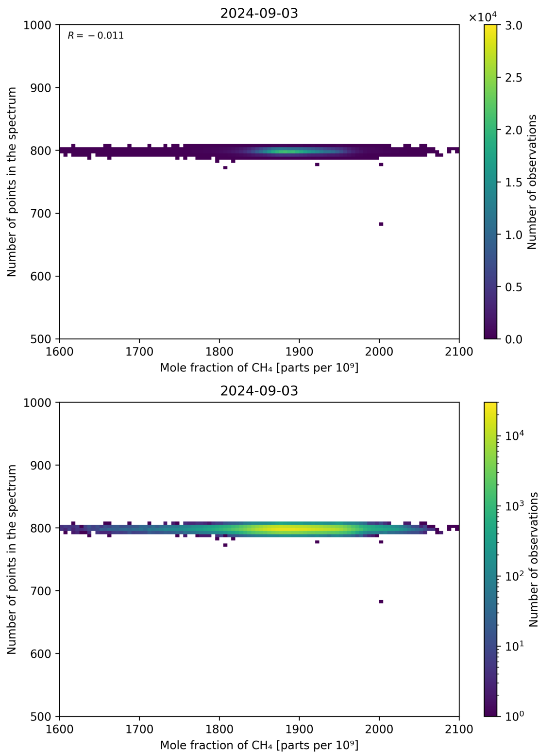
Figure 77: Scatter density plot of “Mole fraction of CH 4 ” against “Number of points in the spectrum” for 2024-09-02 to 2024-09-04.
