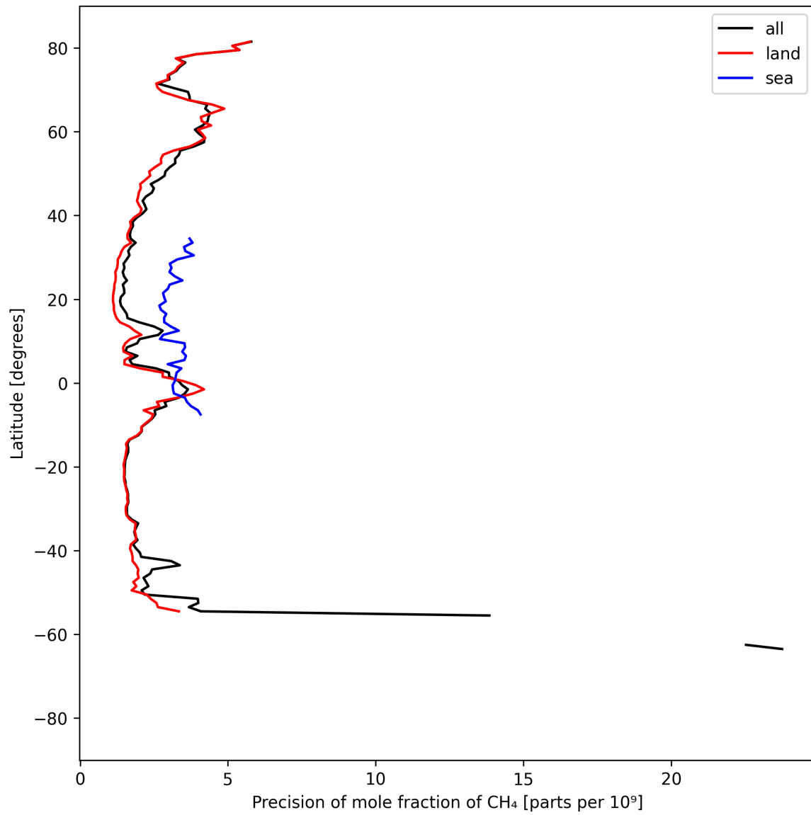
Figure 13: Zonal average of “Precision of mole fraction of CH 4 ” for 2024-09-02 to 2024-09-04.
