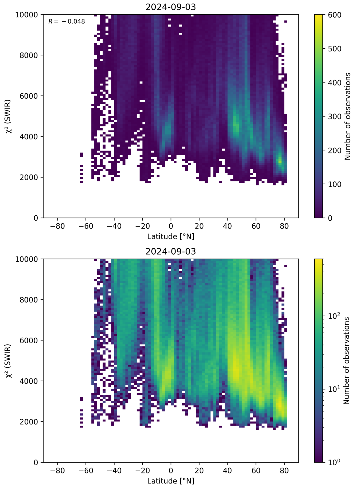
Figure 54: Scatter density plot of “Latitude” against “ \chi^2 (SWIR)” for 2024-09-02 to 2024-09-04.
