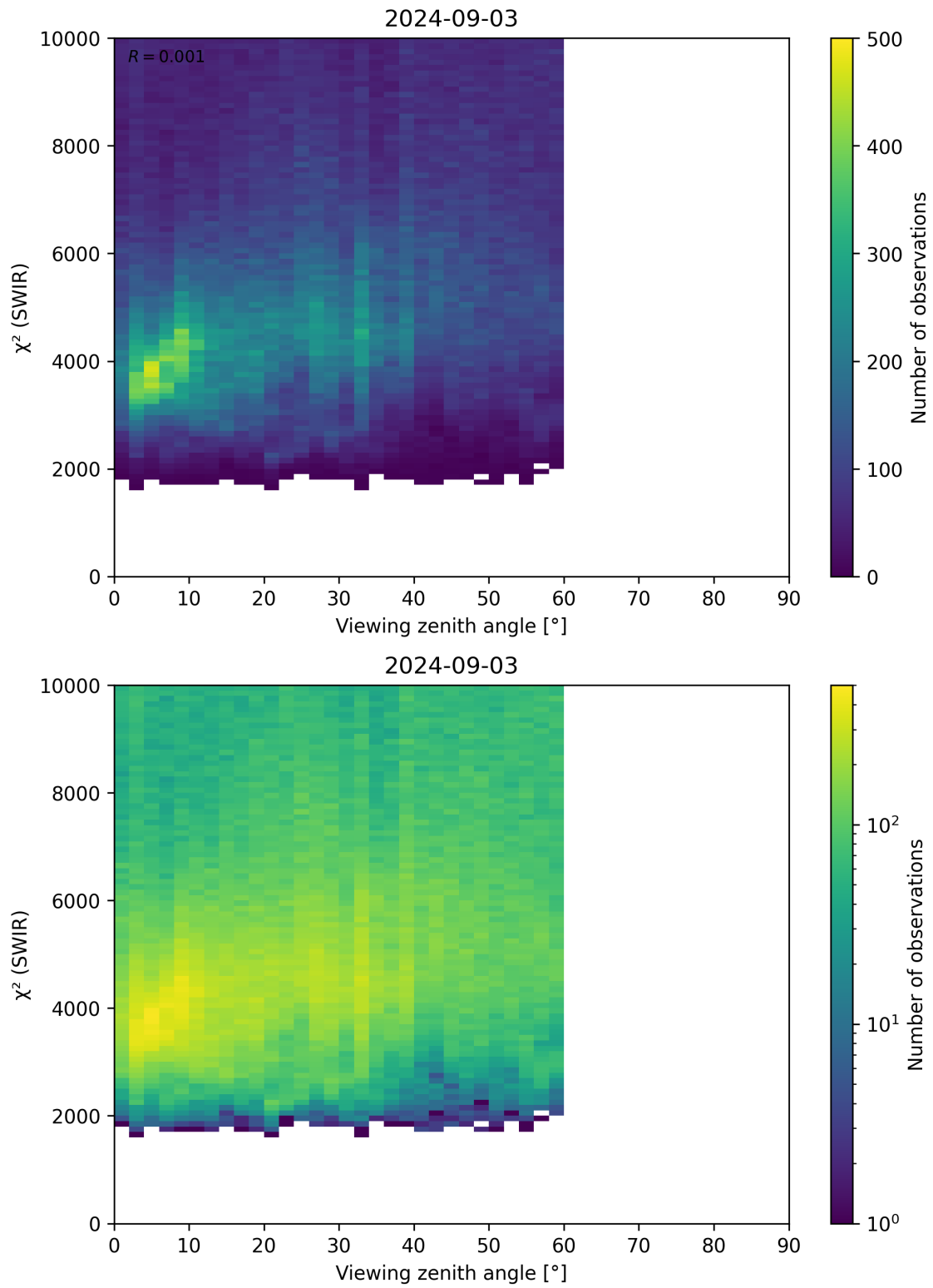
Figure 106: Scatter density plot of “Viewing zenith angle” against “ \chi^2 (SWIR)” for 2024-09-02 to 2024-09-04.
