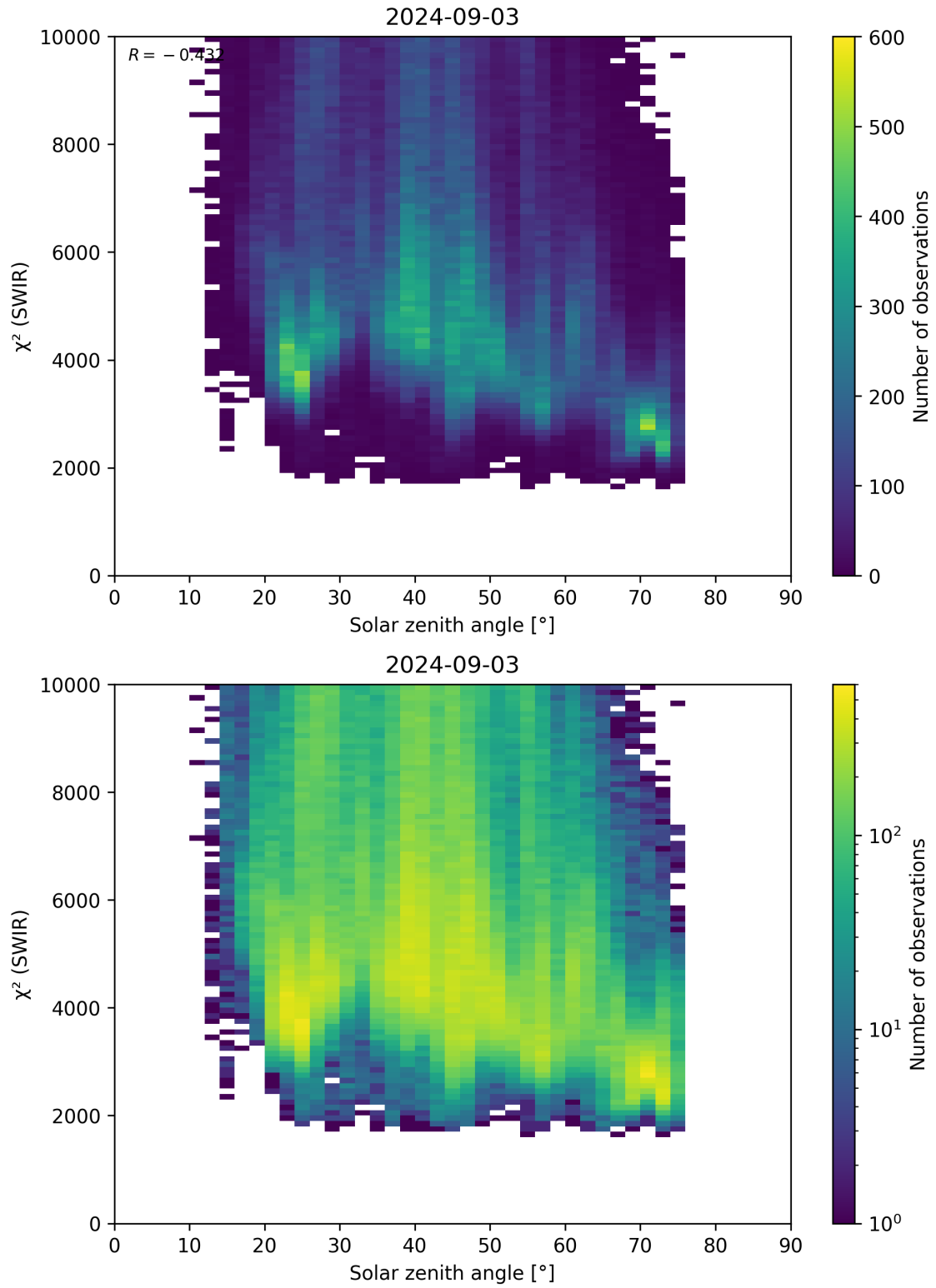
Figure 95: Scatter density plot of “Solar zenith angle” against “ \chi^2 (SWIR)” for 2024-09-02 to 2024-09-04.
