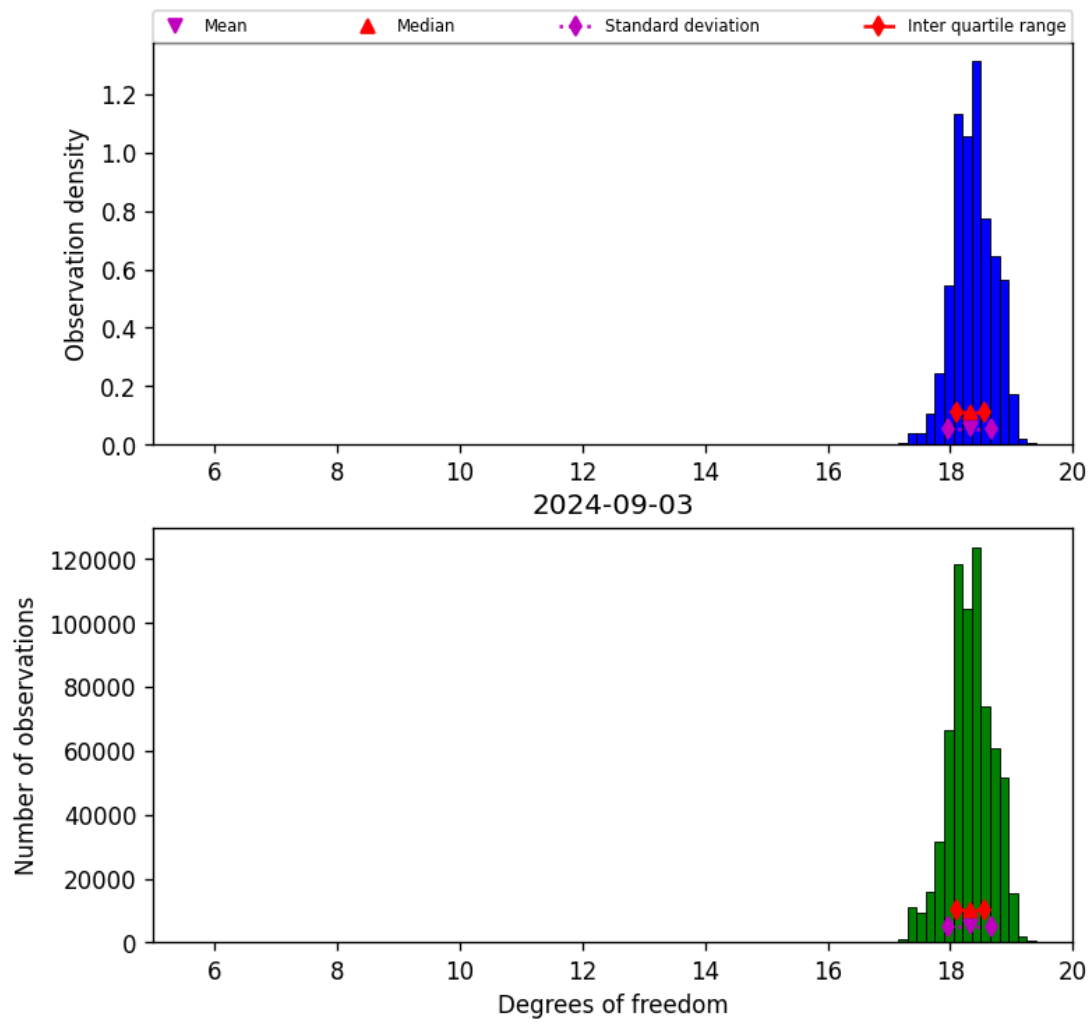
Figure 30: Histogram of "Degrees of freedom" for 2024-09-02 to 2024-09-04
