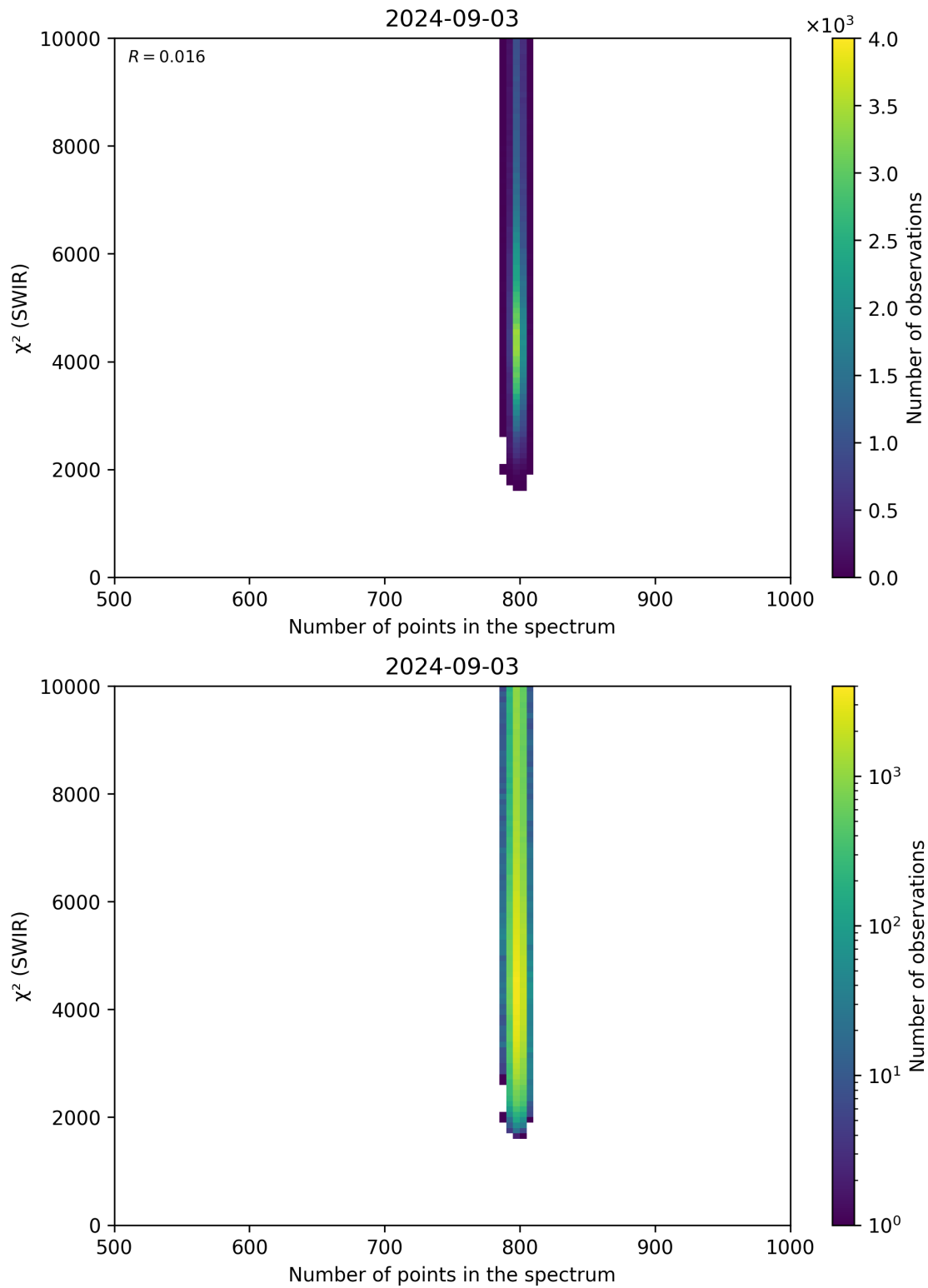
Figure 89: Scatter density plot of “Number of points in the spectrum” against “ \chi^2 (SWIR)” for 2024-09-02 to 2024-09-04.
