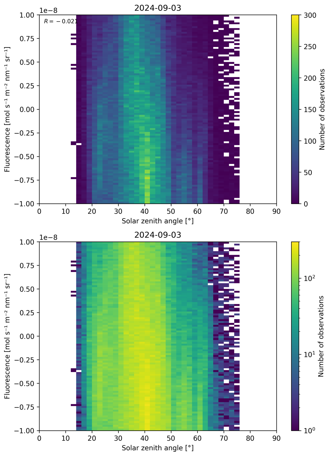
Figure 97: Scatter density plot of “Solar zenith angle” against “Fluorescence” for 2024-09-02 to 2024-09-04.
