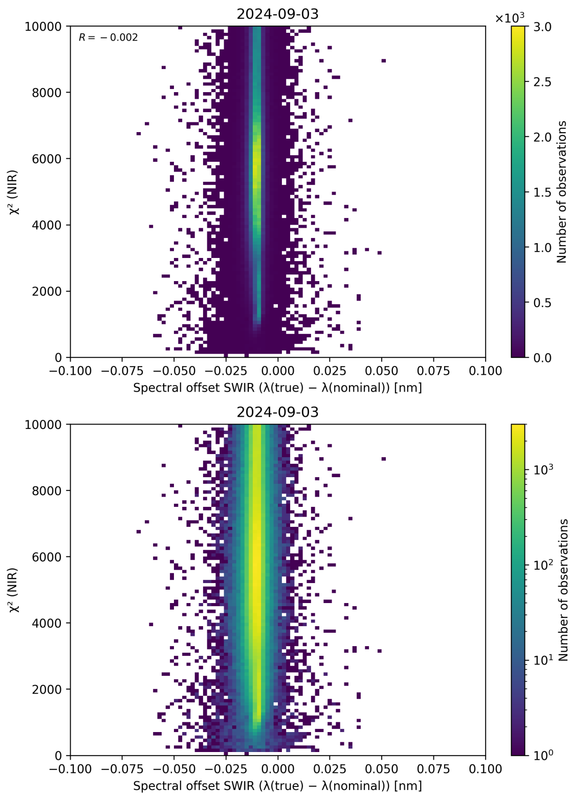
Figure 117: Scatter density plot of “Spectral offset SWIR ( \lambda_{\text{true}} - \lambda_{\text{nominal}} )” against “ \chi^2 (NIR)” for 2024-09-02 to 2024-09-04.
