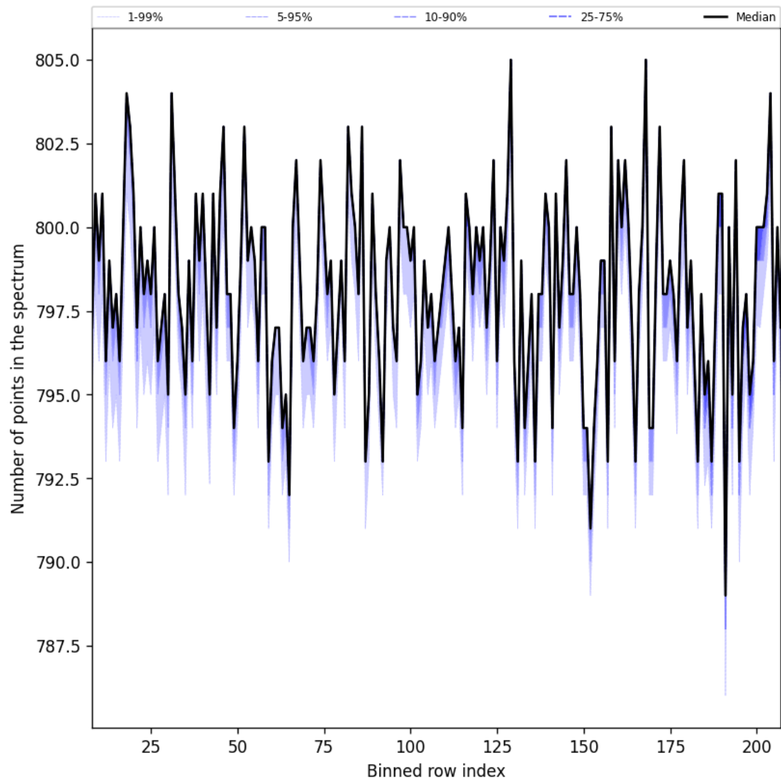
Figure 37: Along track statistics of “Number of points in the spectrum” for 2024-09-02 to 2024-09-04
