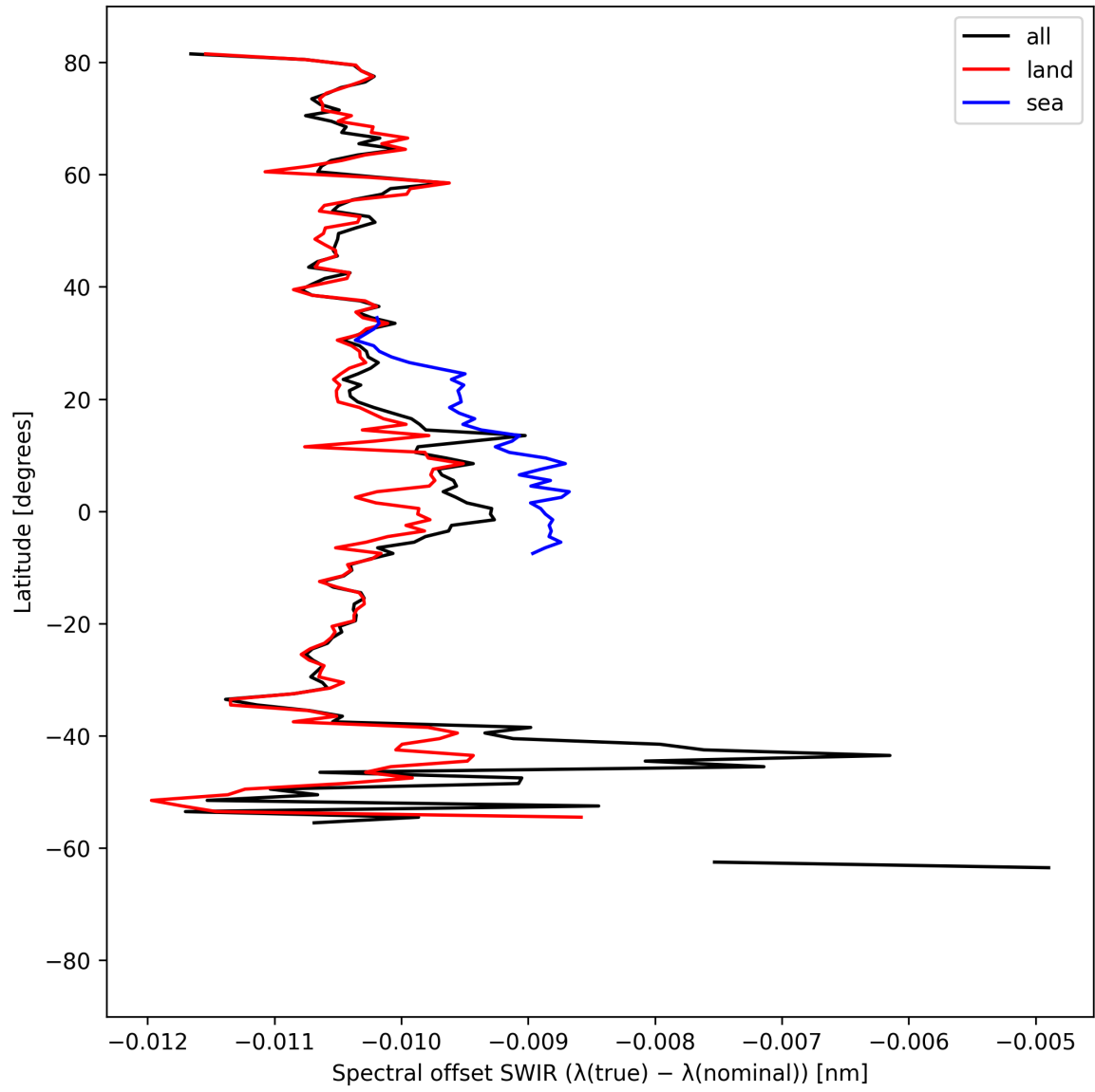
Figure 16: Zonal average of “Spectral offset SWIR ( \lambda_{\text{true}} - \lambda_{\text{nominal}} )” for 2024-09-02 to 2024-09-04.
