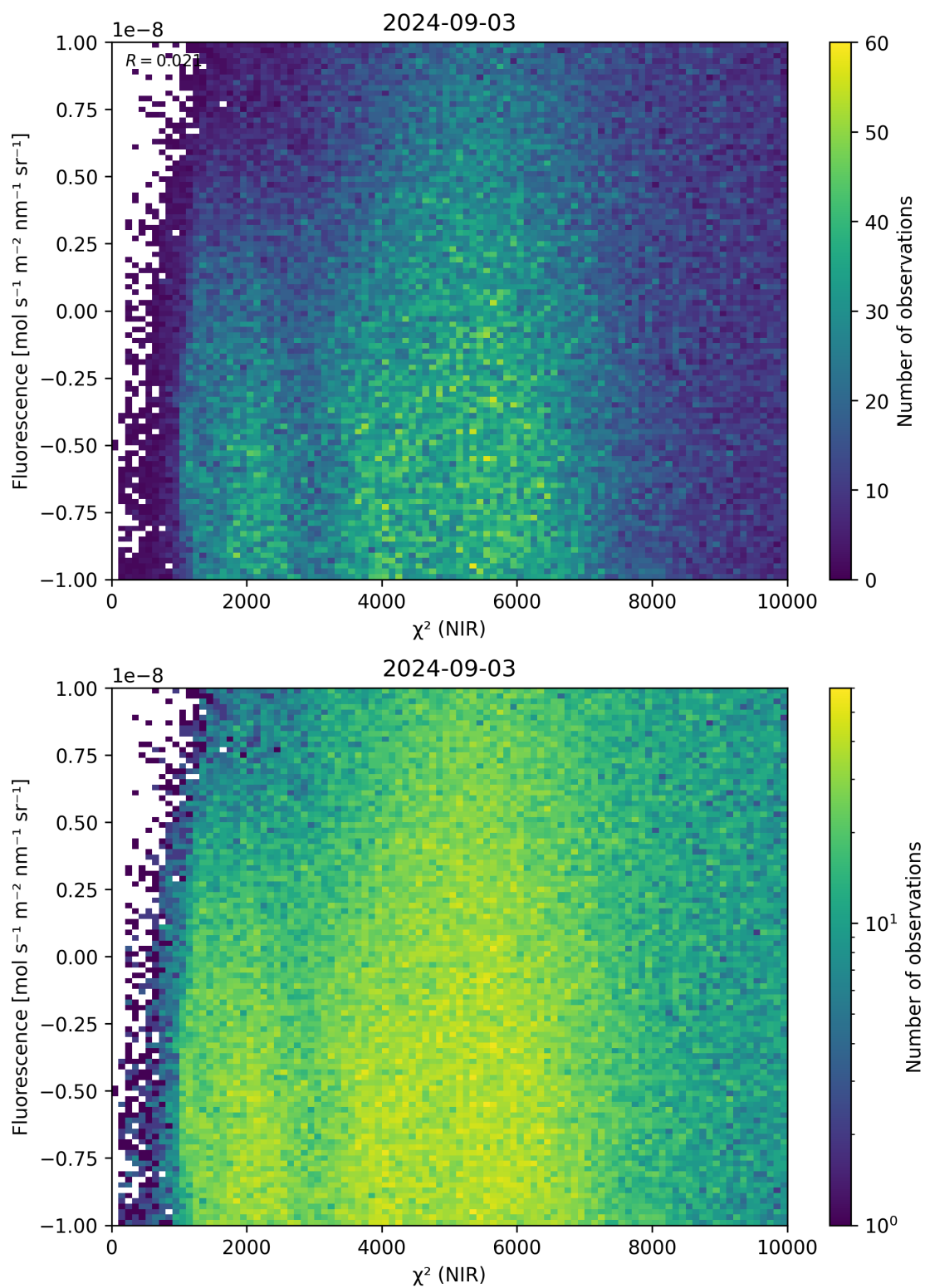
Figure 45: Scatter density plot of “ \chi^2 (NIR)” against “Fluorescence” for 2024-09-02 to 2024-09-04.
