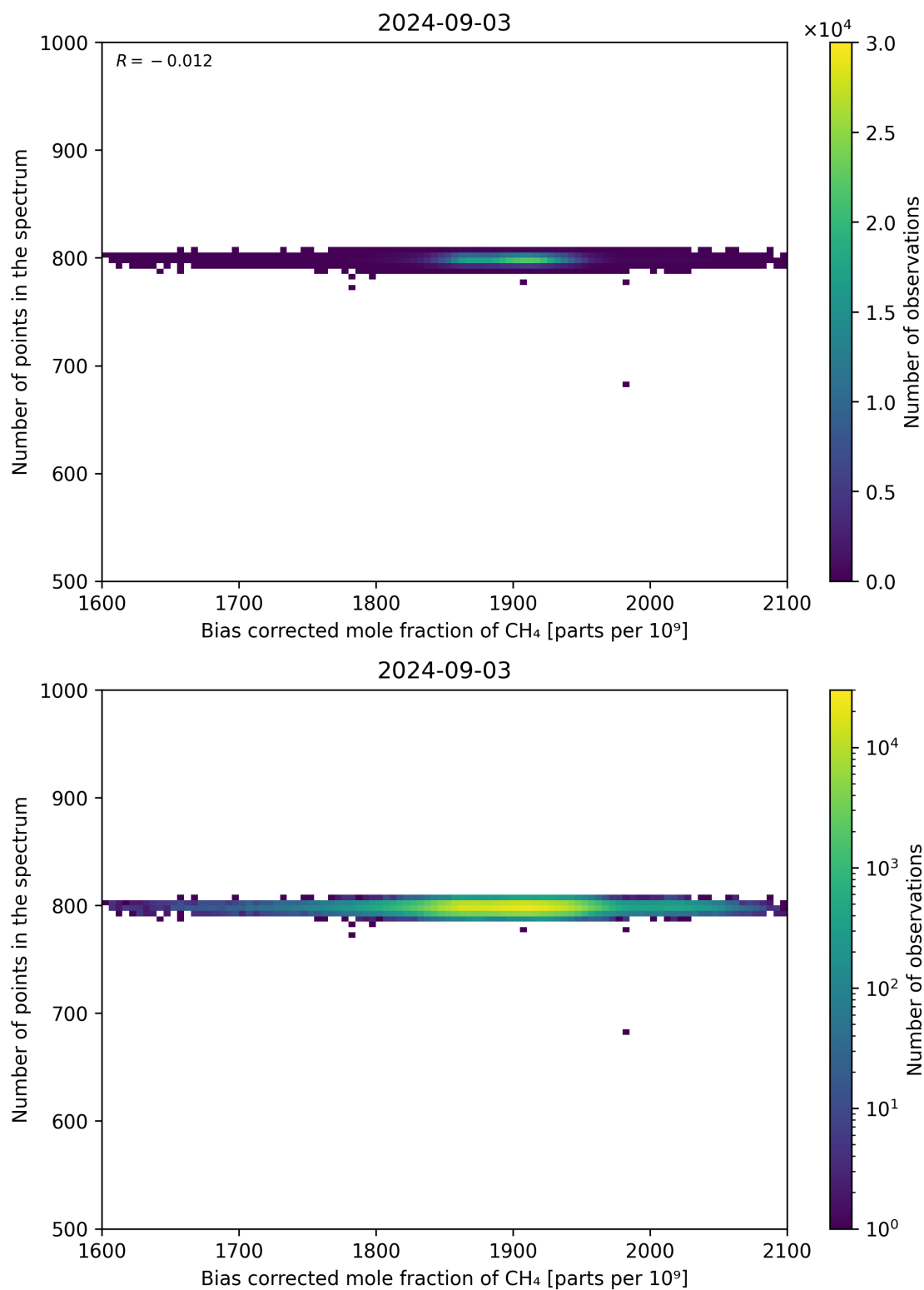
Figure 68: Scatter density plot of “Bias corrected mole fraction of CH 4 ” against “Number of points in the spectrum” for 2024-09-02 to 2024-09-04.
