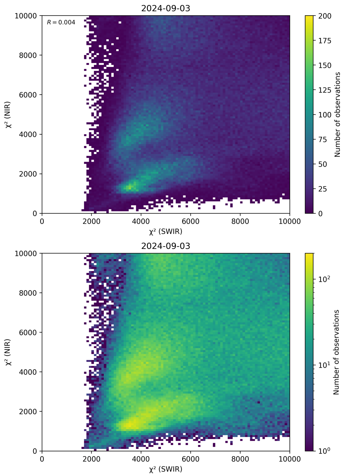
Figure 47: Scatter density plot of “ \chi^2 (SWIR)” against “ \chi^2 (NIR)” for 2024-09-02 to 2024-09-04.
