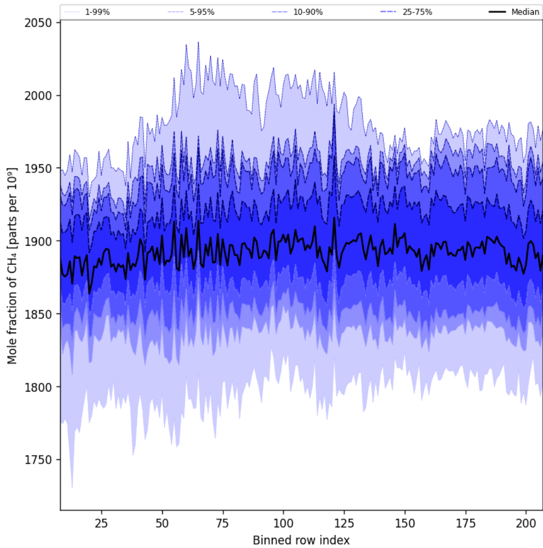
Figure 34: Along track statistics of “Mole fraction of CH 4 ” for 2024-09-02 to 2024-09-04
