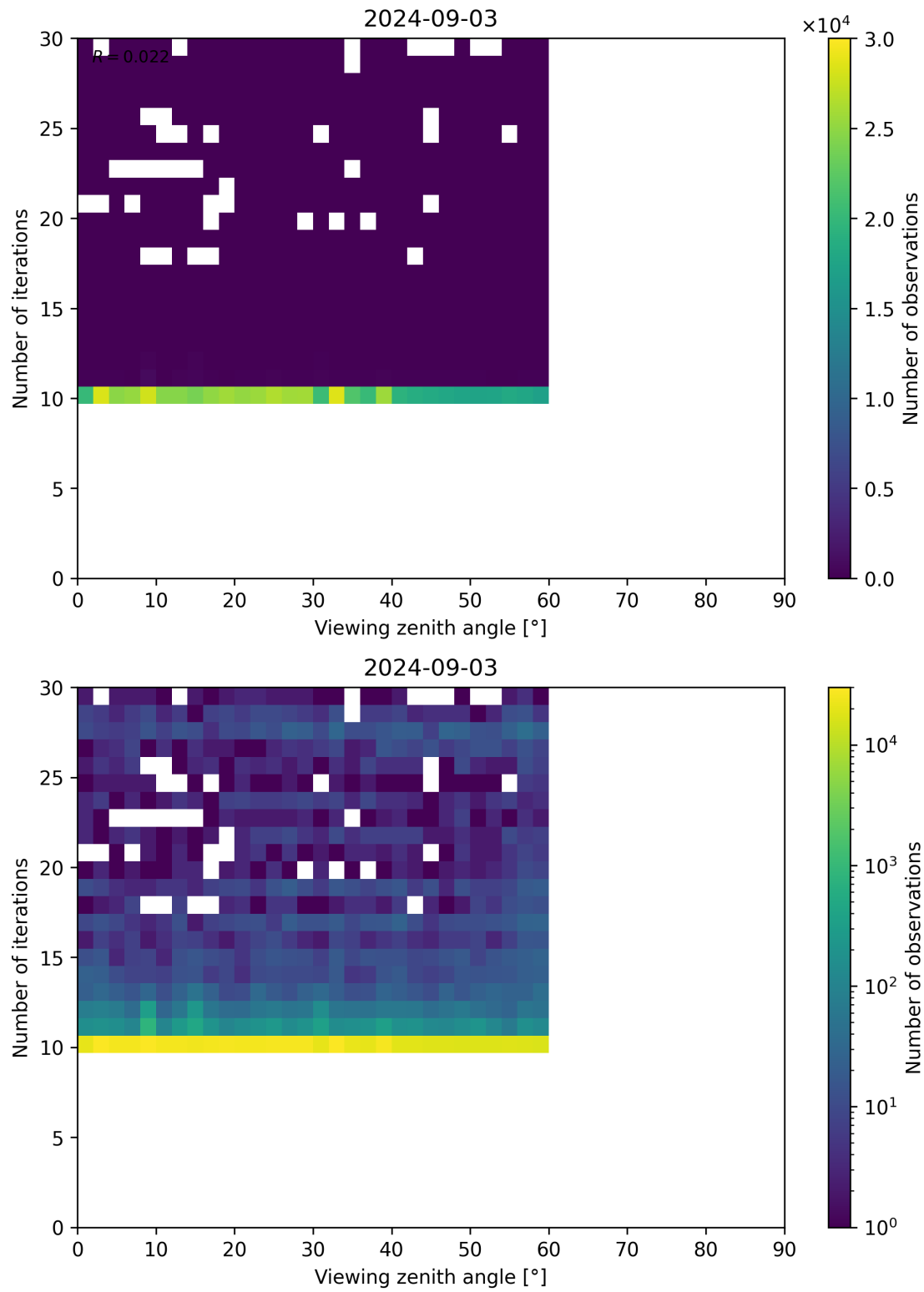
Figure 113: Scatter density plot of “Viewing zenith angle” against “Number of iterations” for 2024-09-02 to 2024-09-04.
