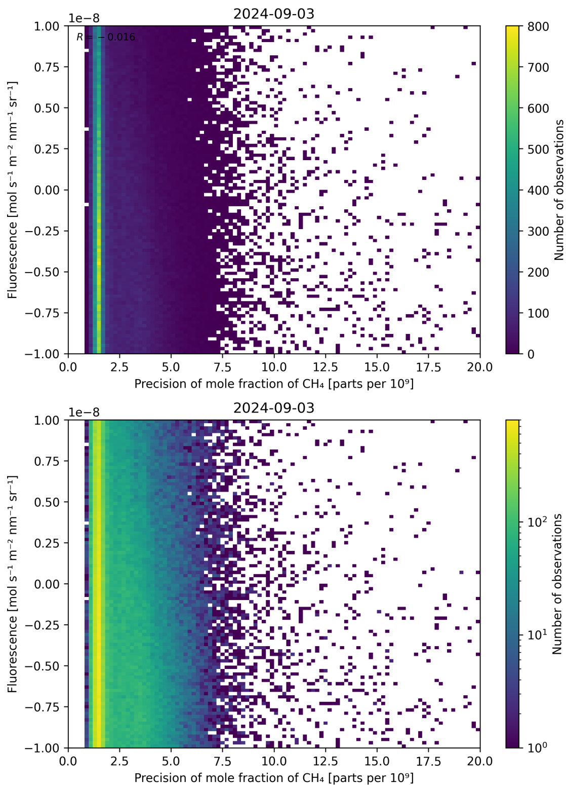
Figure 81: Scatter density plot of “Precision of mole fraction of \text{CH}_4 ” against “Fluorescence” for 2024-09-02 to 2024-09-04.
