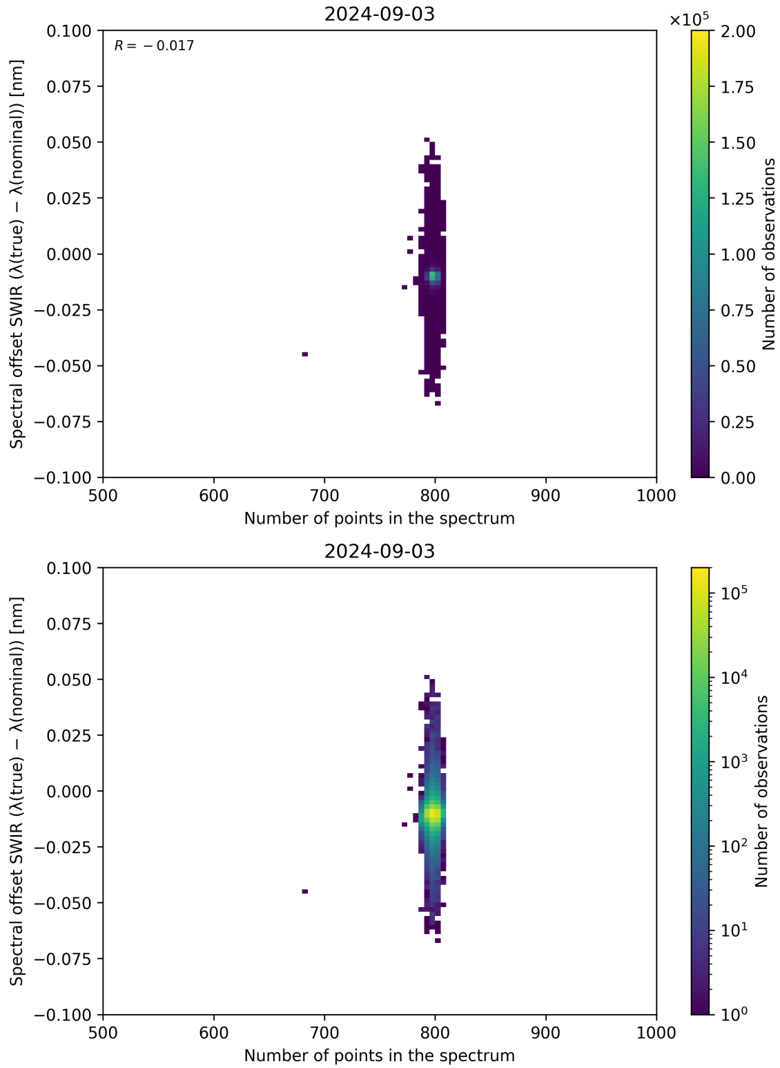
Figure 93: Scatter density plot of “Number of points in the spectrum” against “Spectral offset SWIR ( \lambda_{\text{true}} - \lambda_{\text{nominal}} )” for 2024-09-02 to 2024-09-04.
