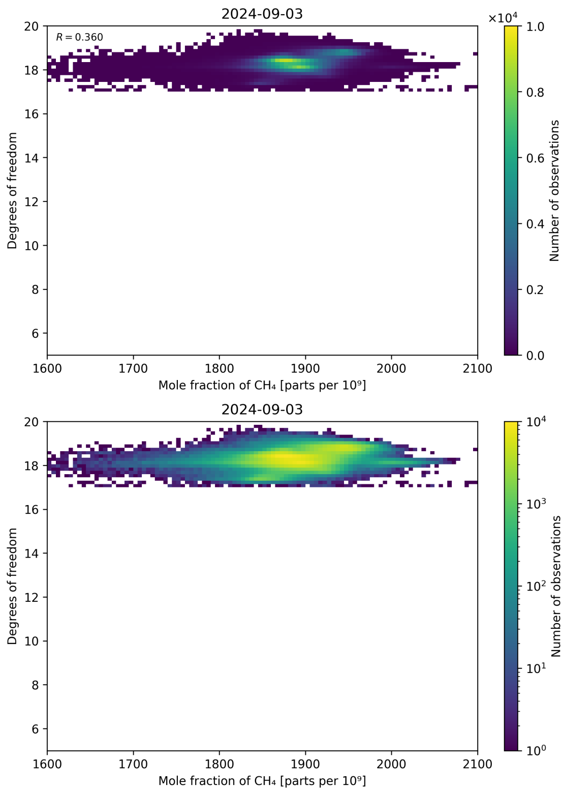
Figure 72: Scatter density plot of “Mole fraction of CH 4 ” against “Degrees of freedom” for 2024-09-02 to 2024-09-04.
