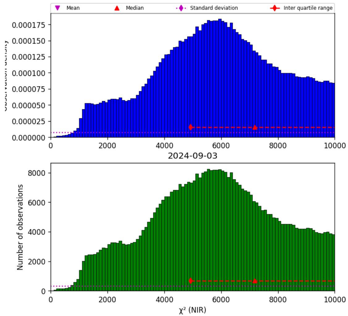
Figure 29: Histogram of “ \chi^2 (NIR)” for 2024-09-02 to 2024-09-04
