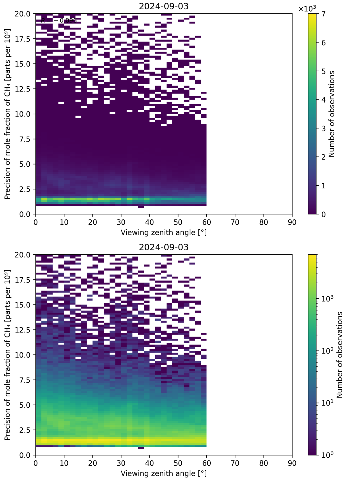
Figure 112: Scatter density plot of “Viewing zenith angle” against “Precision of mole fraction of CH 4 ” for 2024-09-02 to 2024-09-04.
