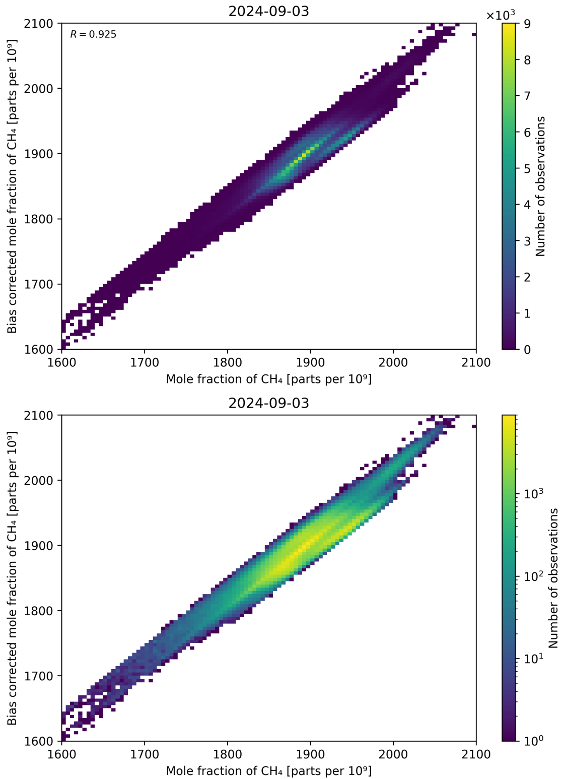
Figure 74: Scatter density plot of “Mole fraction of CH 4 ” against “Bias corrected mole fraction of CH 4 ” for 2024-09-02 to 2024-09-04.
