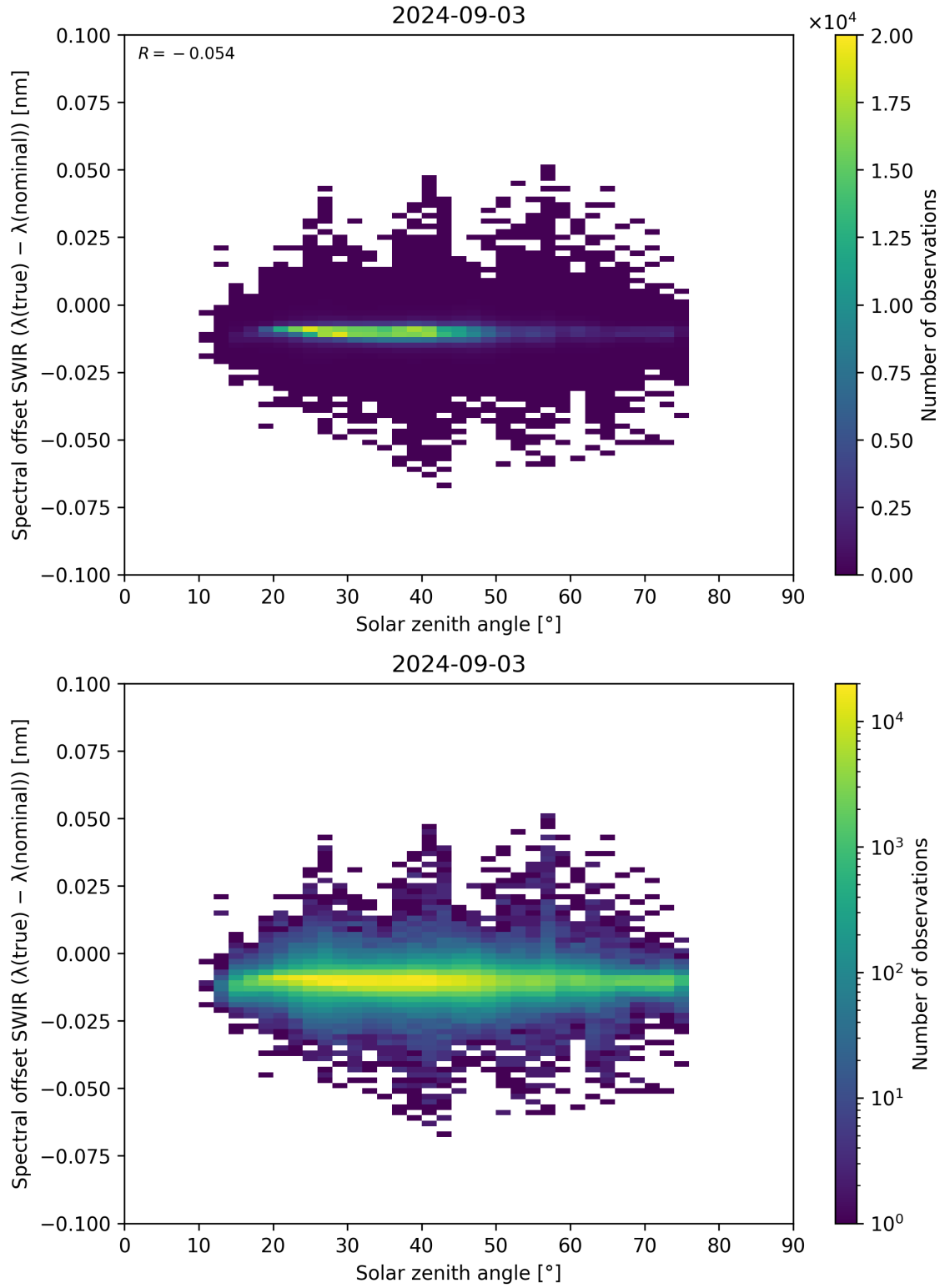
Figure 104: Scatter density plot of “Solar zenith angle” against “Spectral offset SWIR ( \lambda_{\text{true}} - \lambda_{\text{nominal}} )” for 2024-09-02 to 2024-09-04.
