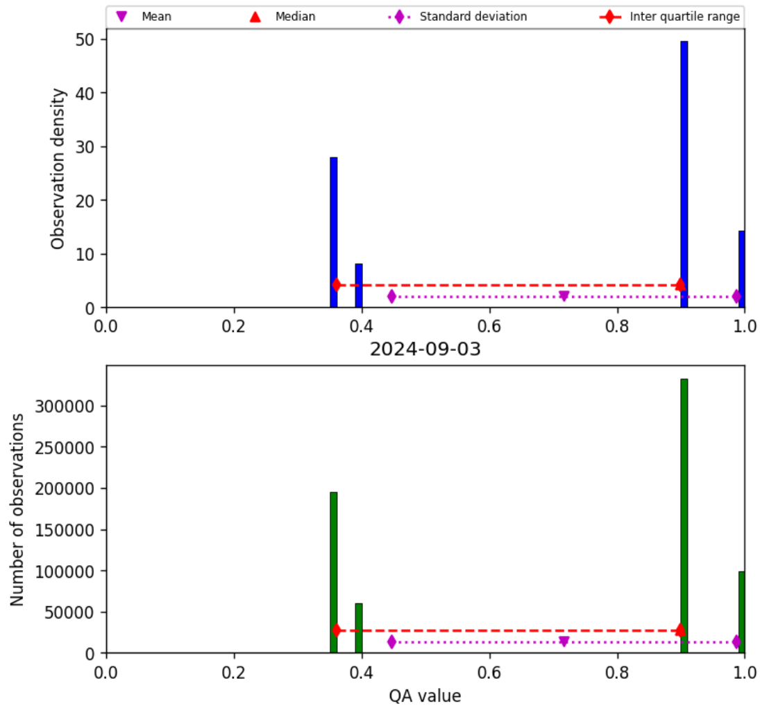
Figure 22: Histogram of “QA value” for 2024-09-02 to 2024-09-04
