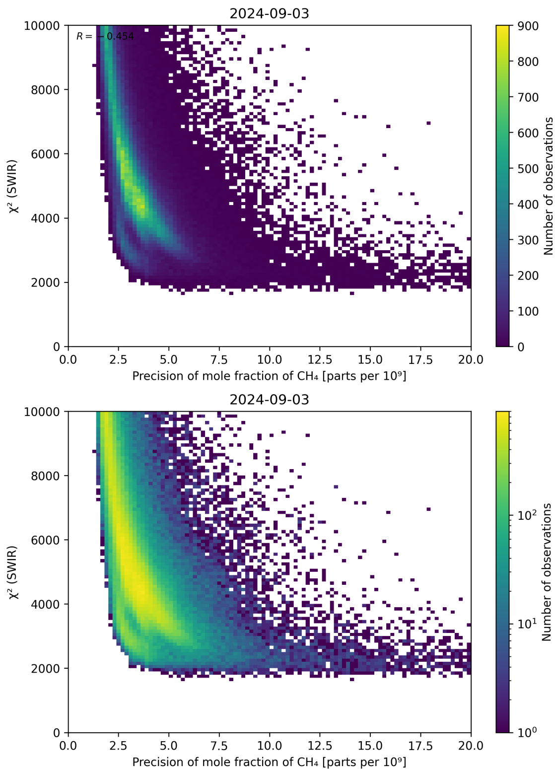
Figure 79: Scatter density plot of “Precision of mole fraction of \text{CH}_4 ” against “ \chi^2 (SWIR)” for 2024-09-02 to 2024-09-04.
