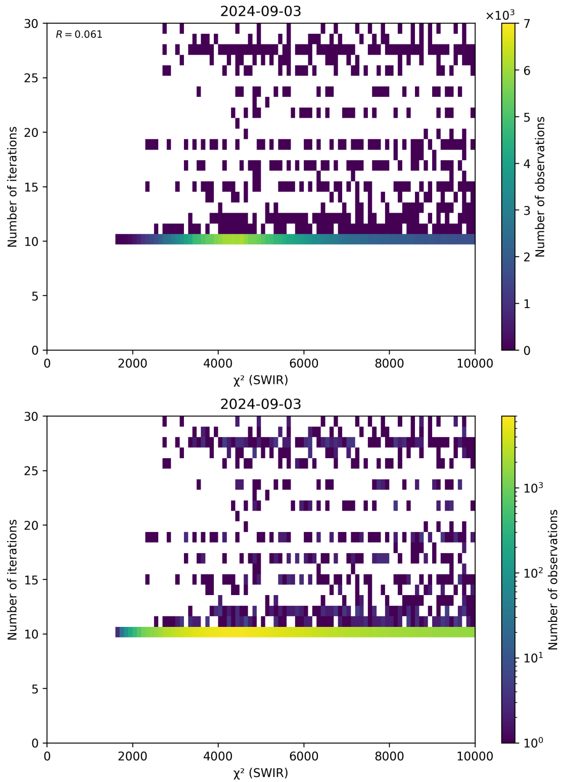
Figure 50: Scatter density plot of “ \chi^2 (SWIR)” against “Number of iterations” for 2024-09-02 to 2024-09-04.
