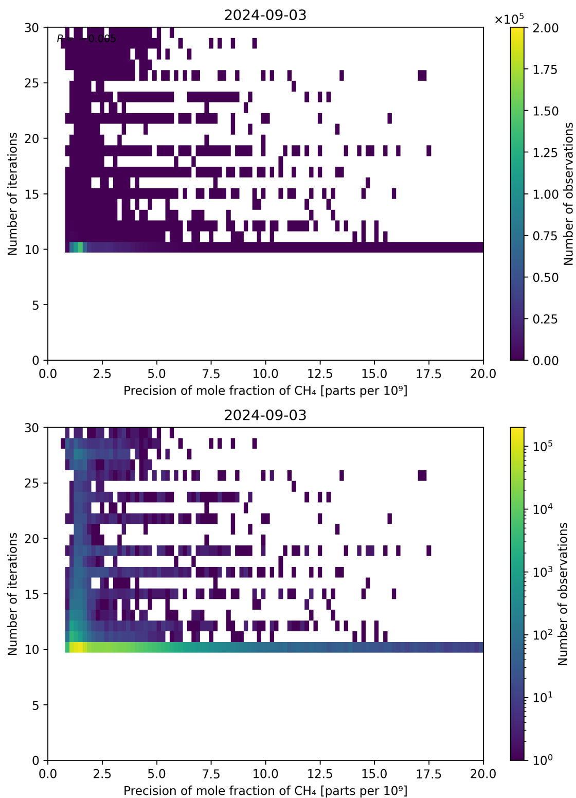
Figure 83: Scatter density plot of “Precision of mole fraction of CH 4 ” against “Number of iterations” for 2024-09-02 to 2024-09-04.
