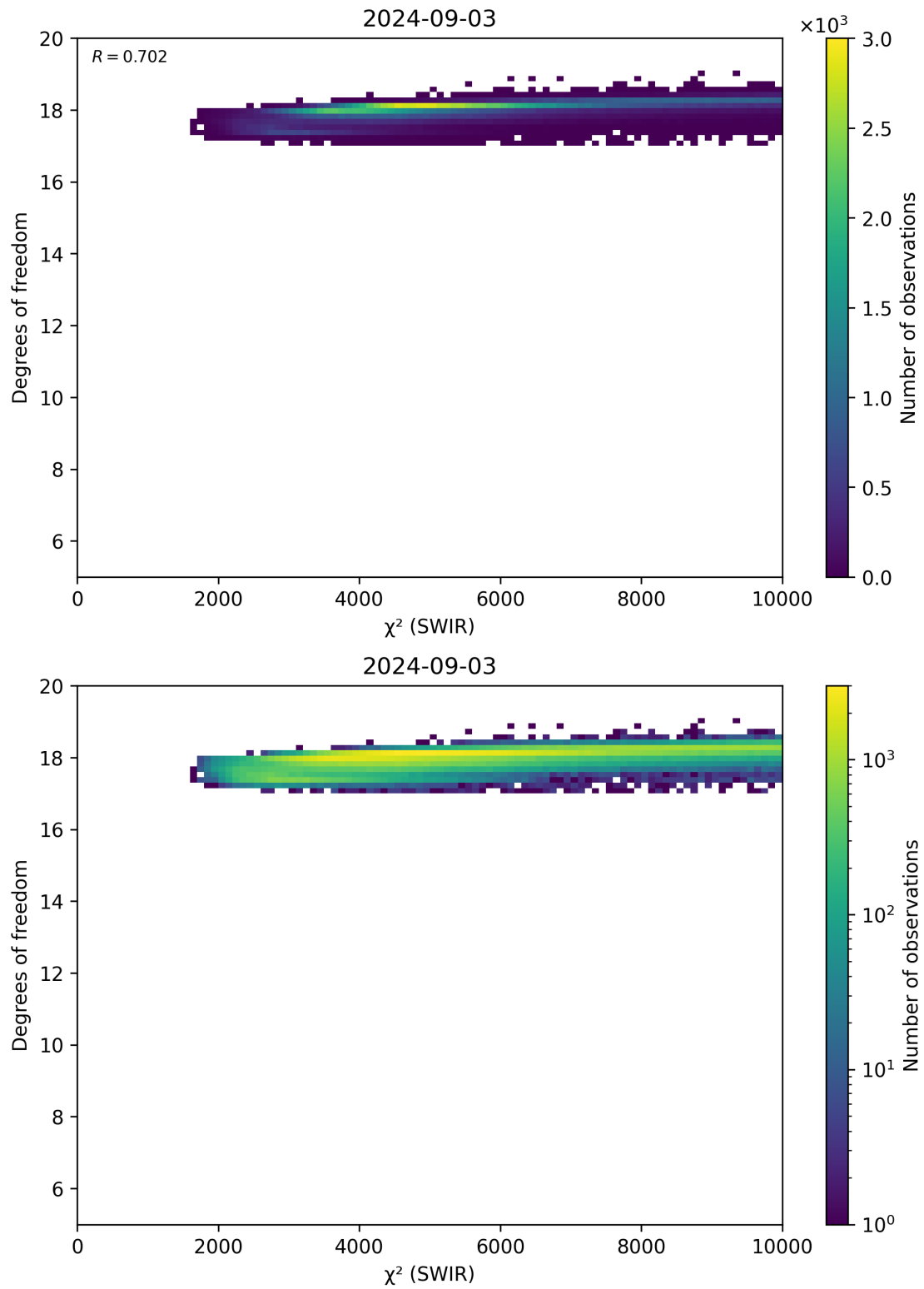
Figure 48: Scatter density plot of “ \chi^2 (SWIR)” against “Degrees of freedom” for 2024-09-02 to 2024-09-04.
