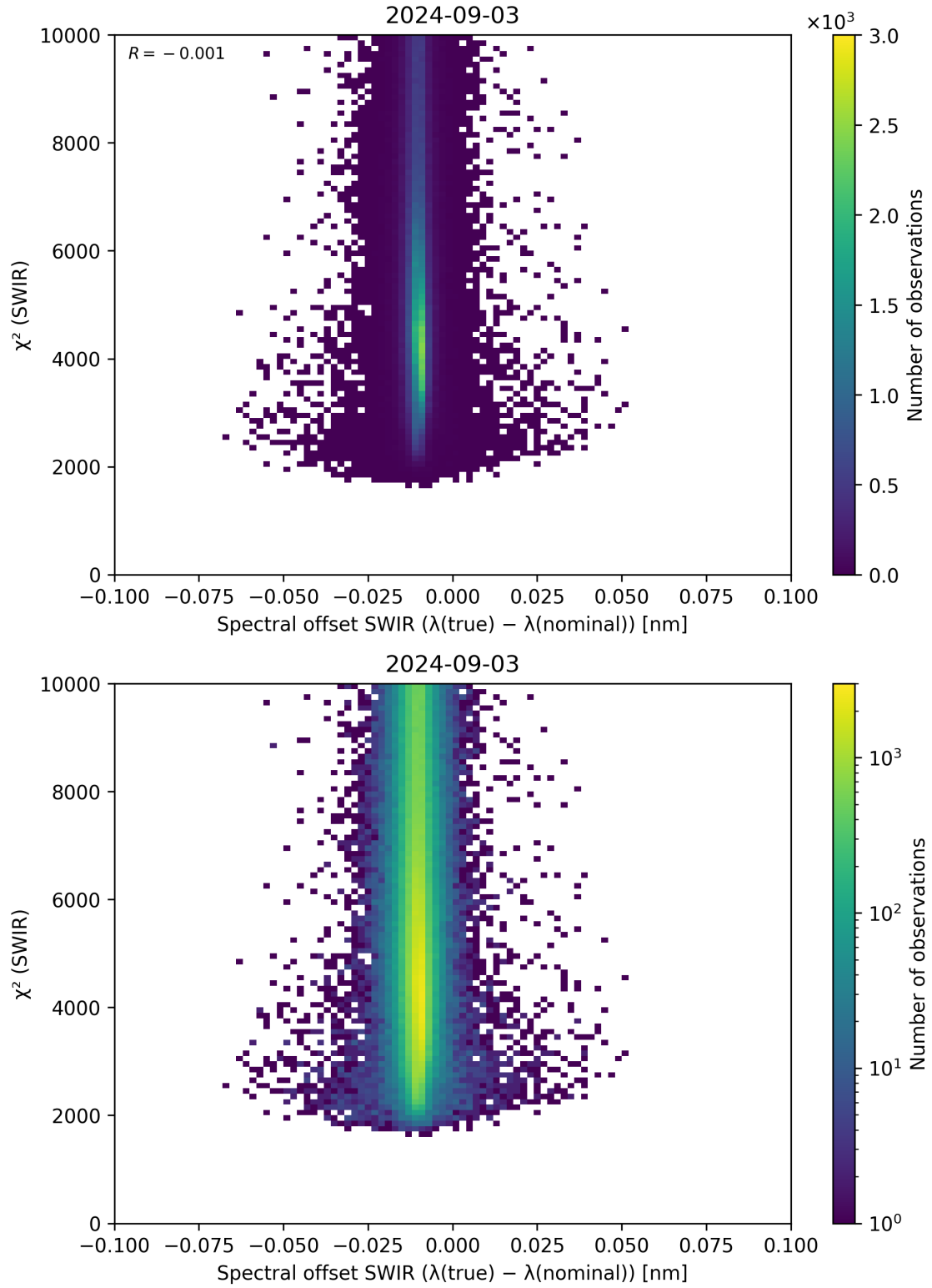
Figure 118: Scatter density plot of “Spectral offset SWIR ( \lambda_{\text{true}} - \lambda_{\text{nominal}} )” against “ \chi^2 (SWIR)” for 2024-09-02 to 2024-09-04.
