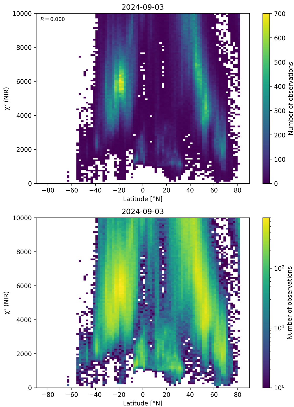
Figure 53: Scatter density plot of “Latitude” against “ \chi^2 (NIR)” for 2024-09-02 to 2024-09-04.
