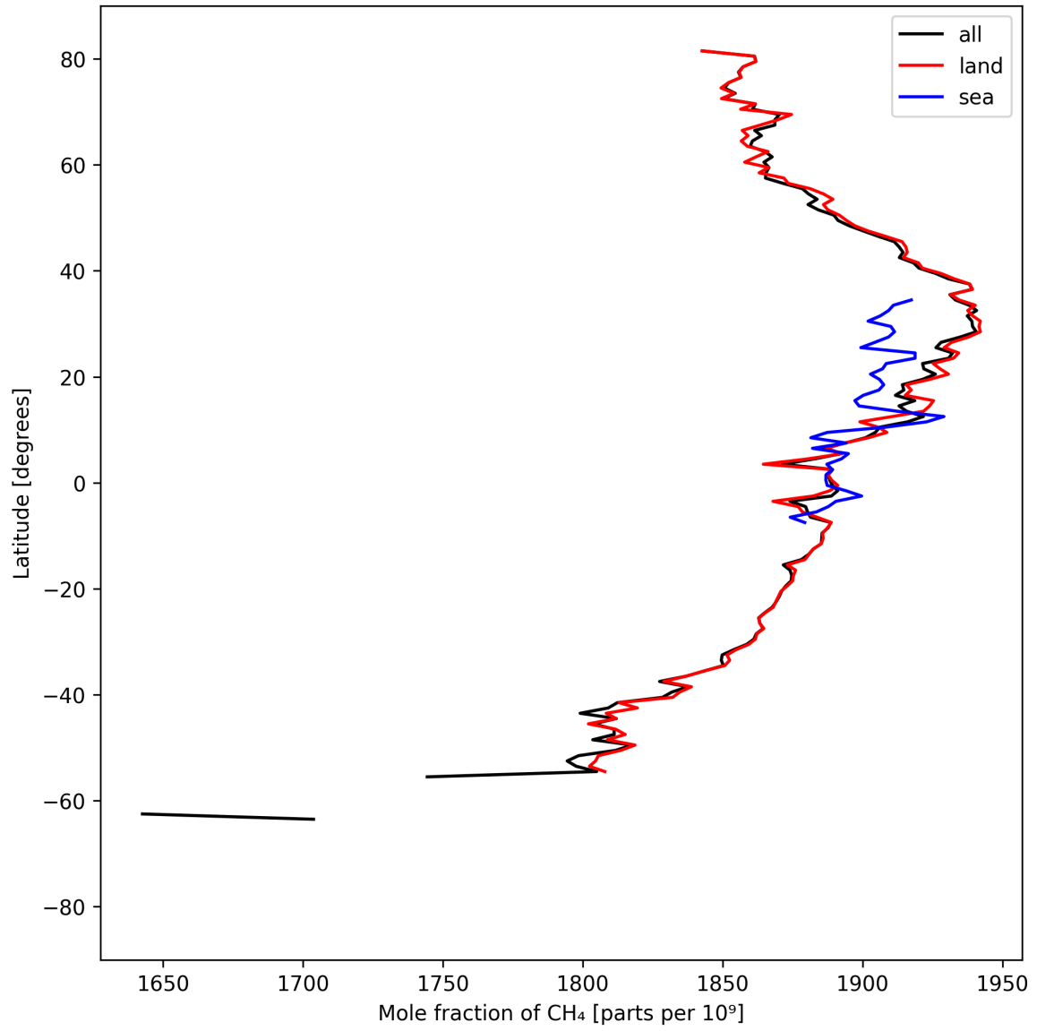
Figure 12: Zonal average of “Mole fraction of \text{CH}_4 ” for 2024-09-02 to 2024-09-04.
