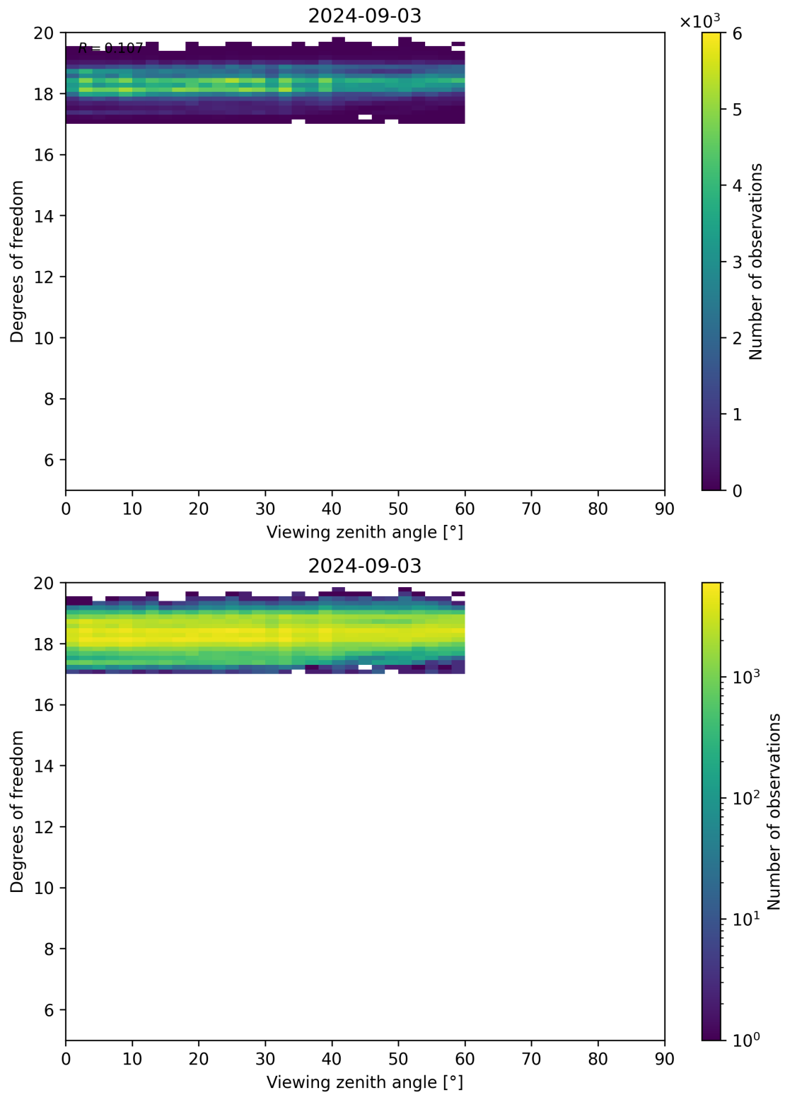
Figure 107: Scatter density plot of “Viewing zenith angle” against “Degrees of freedom” for 2024-09-02 to 2024-09-04.
