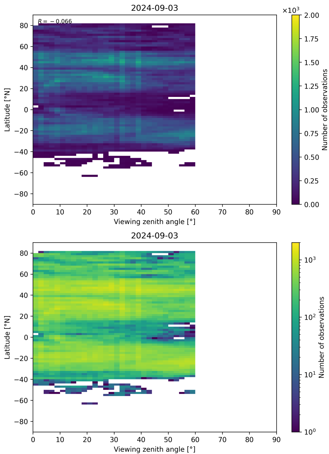
Figure 109: Scatter density plot of “Viewing zenith angle” against “Latitude” for 2024-09-02 to 2024-09-04.
