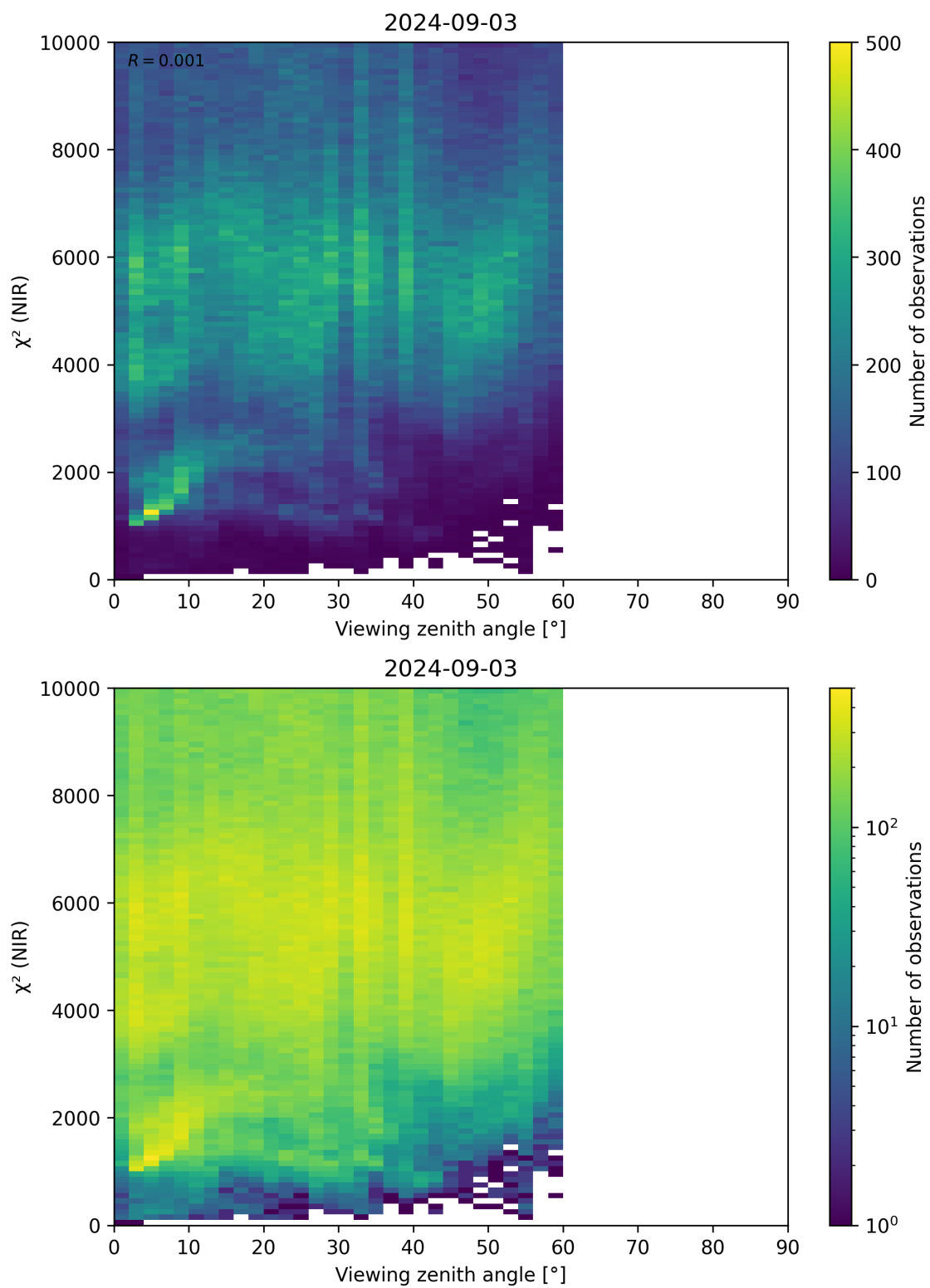
Figure 105: Scatter density plot of “Viewing zenith angle” against “ \chi^2 (NIR)” for 2024-09-02 to 2024-09-04.
