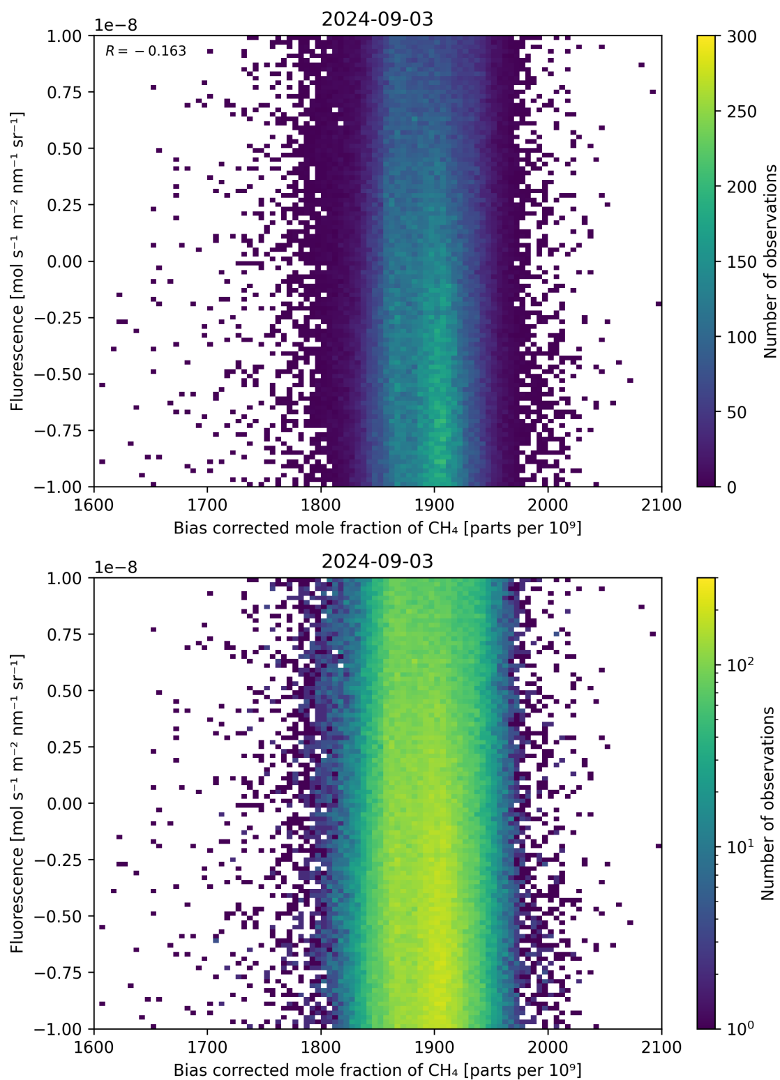
Figure 66: Scatter density plot of “Bias corrected mole fraction of \text{CH}_4 ” against “Fluorescence” for 2024-09-02 to 2024-09-04.
