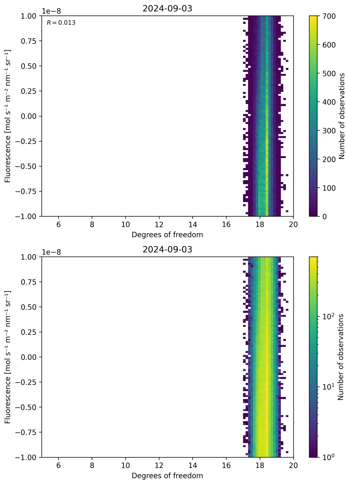
Figure 51: Scatter density plot of “Degrees of freedom” against “Fluorescence” for 2024-09-02 to 2024-09-04.
