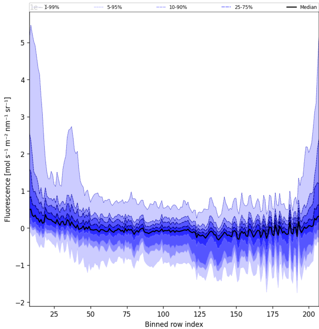
Figure 43: Along track statistics of “Fluorescence” for 2024-09-02 to 2024-09-04
