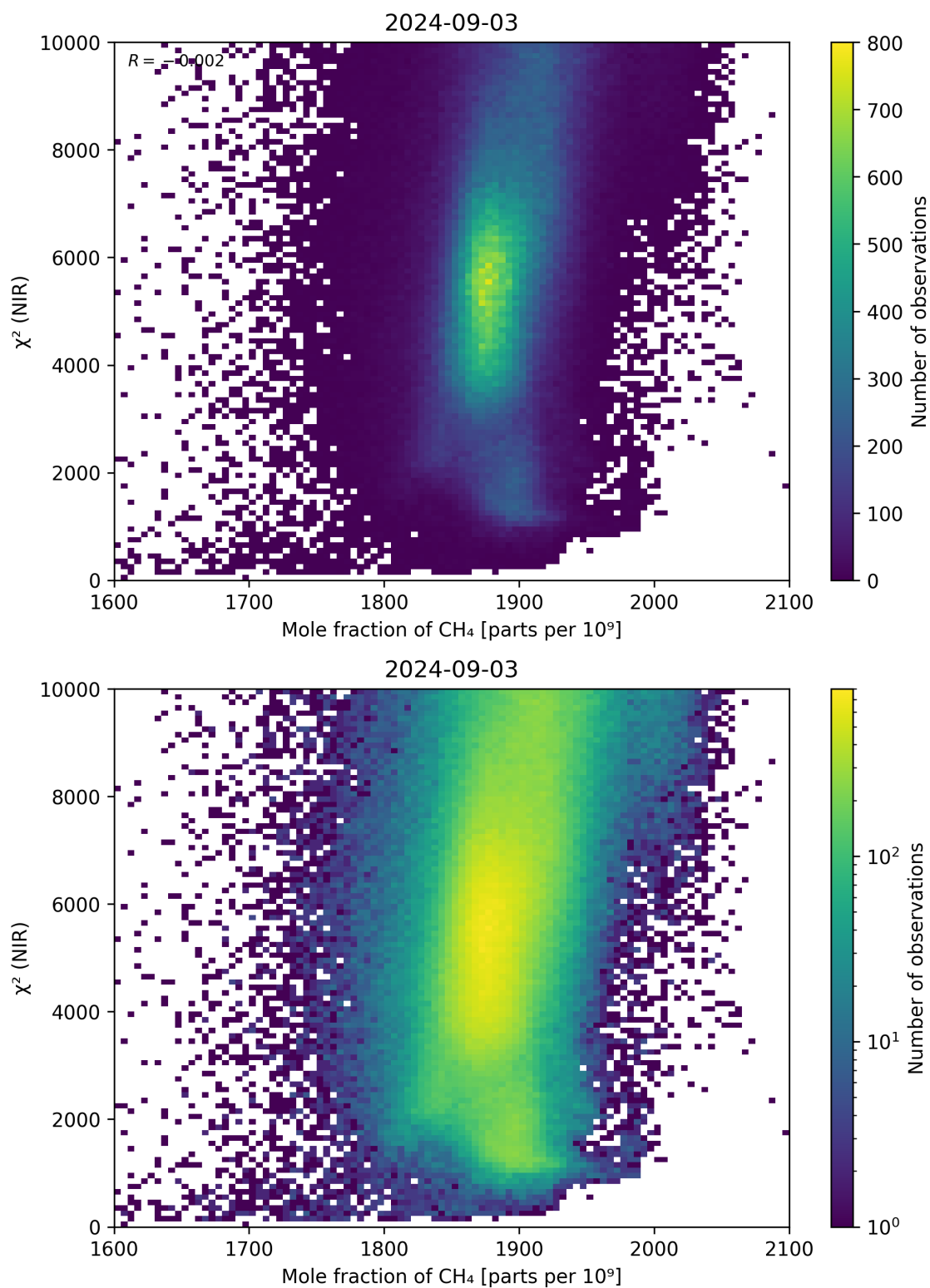
Figure 70: Scatter density plot of “Mole fraction of \text{CH}_4 ” against “ \chi^2 (NIR)” for 2024-09-02 to 2024-09-04.
