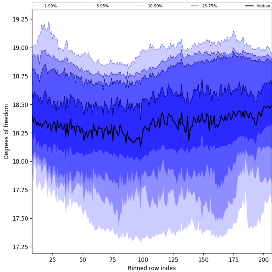
Figure 41: Along track statistics of “Degrees of freedom” for 2024-09-02 to 2024-09-04
