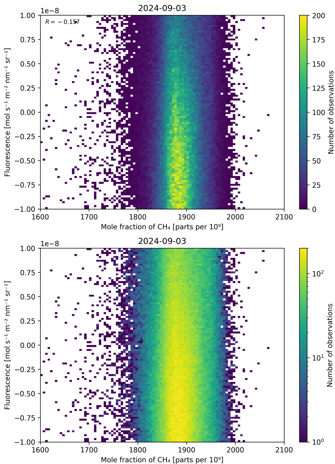
Figure 73: Scatter density plot of “Mole fraction of \text{CH}_4 ” against “Fluorescence” for 2024-09-02 to 2024-09-04.
