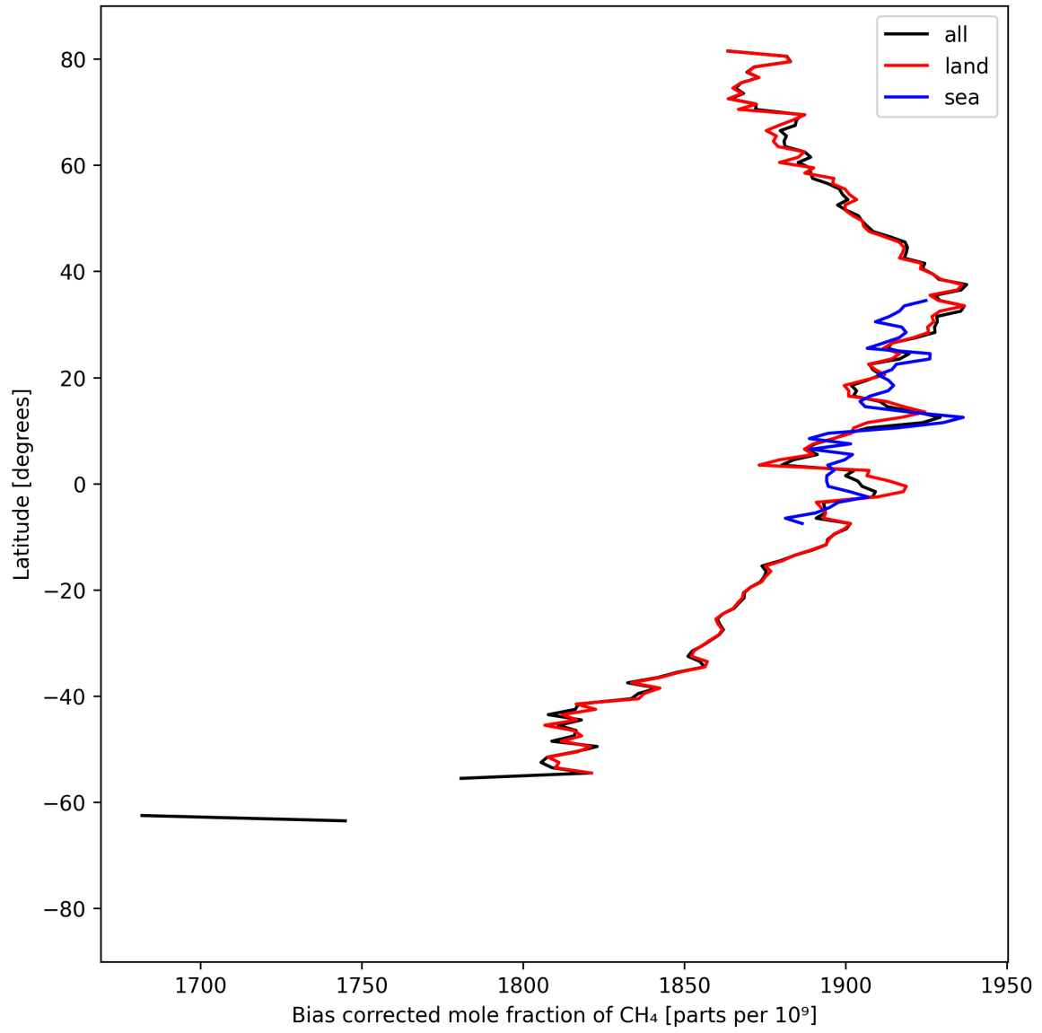
Figure 14: Zonal average of “Bias corrected mole fraction of CH 4 ” for 2024-09-02 to 2024-09-04.
