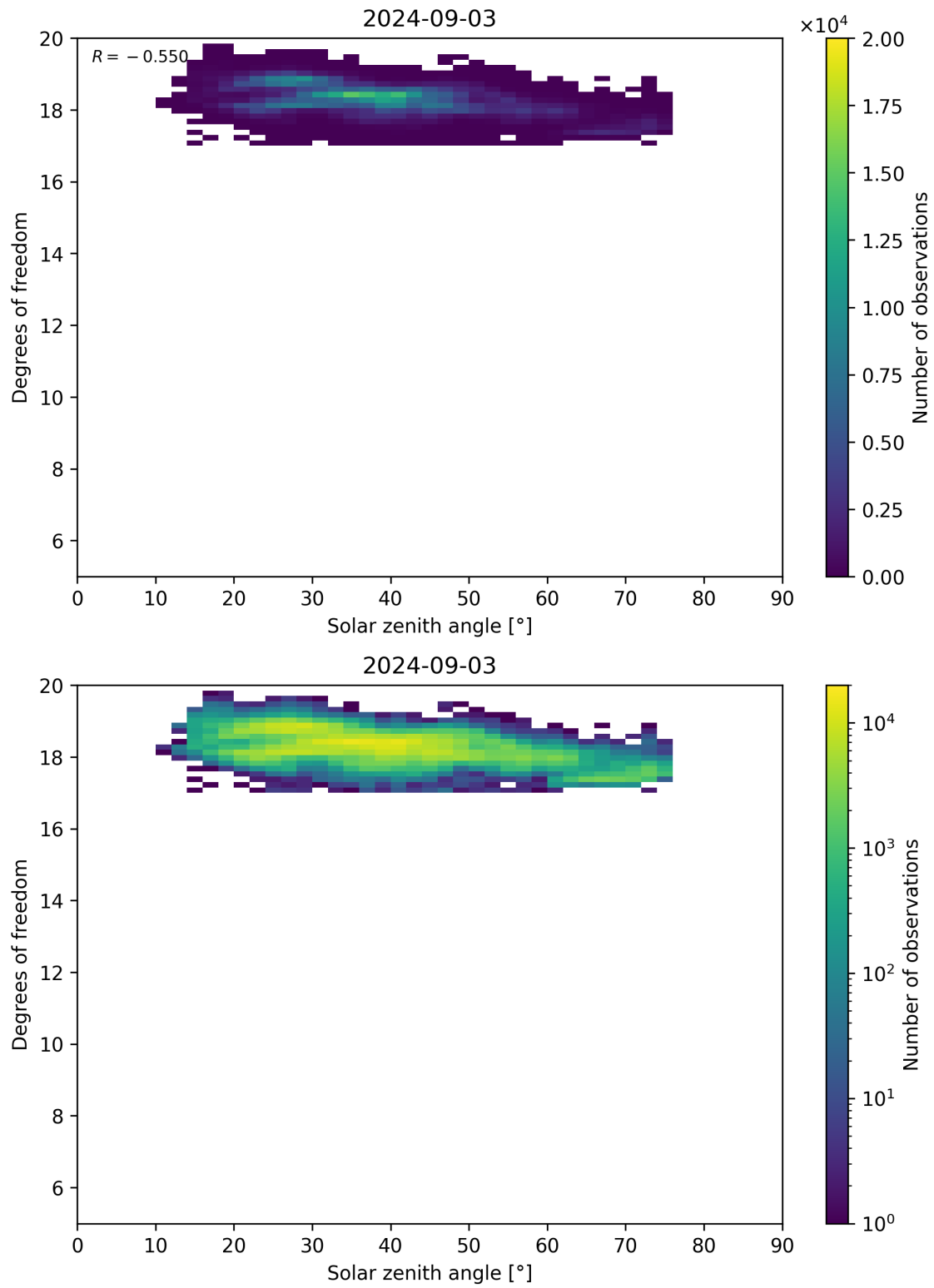
Figure 96: Scatter density plot of “Solar zenith angle” against “Degrees of freedom” for 2024-09-02 to 2024-09-04.
