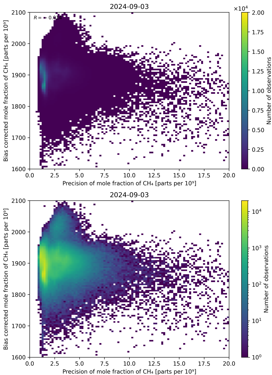
Figure 82: Scatter density plot of “Precision of mole fraction of CH 4 ” against “Bias corrected mole fraction of CH 4 ” for 2024-09-02 to 2024-09-04.
