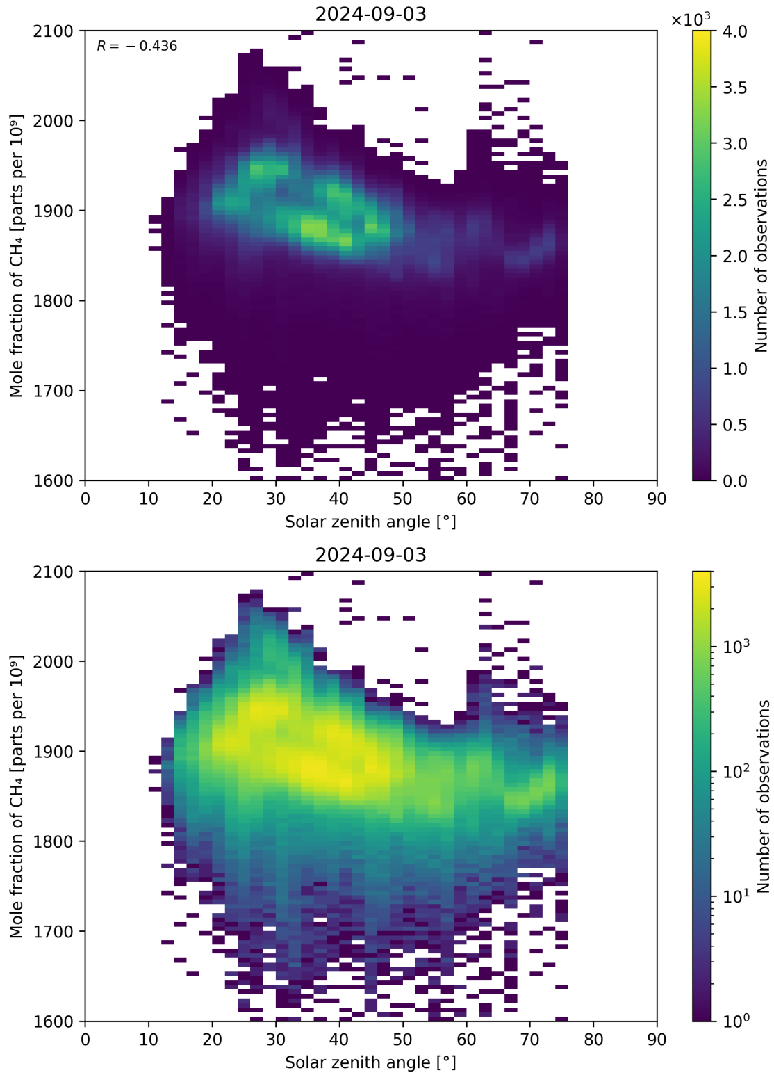
Figure 99: Scatter density plot of “Solar zenith angle” against “Mole fraction of \text{CH}_4 ” for 2024-09-02 to 2024-09-04.
