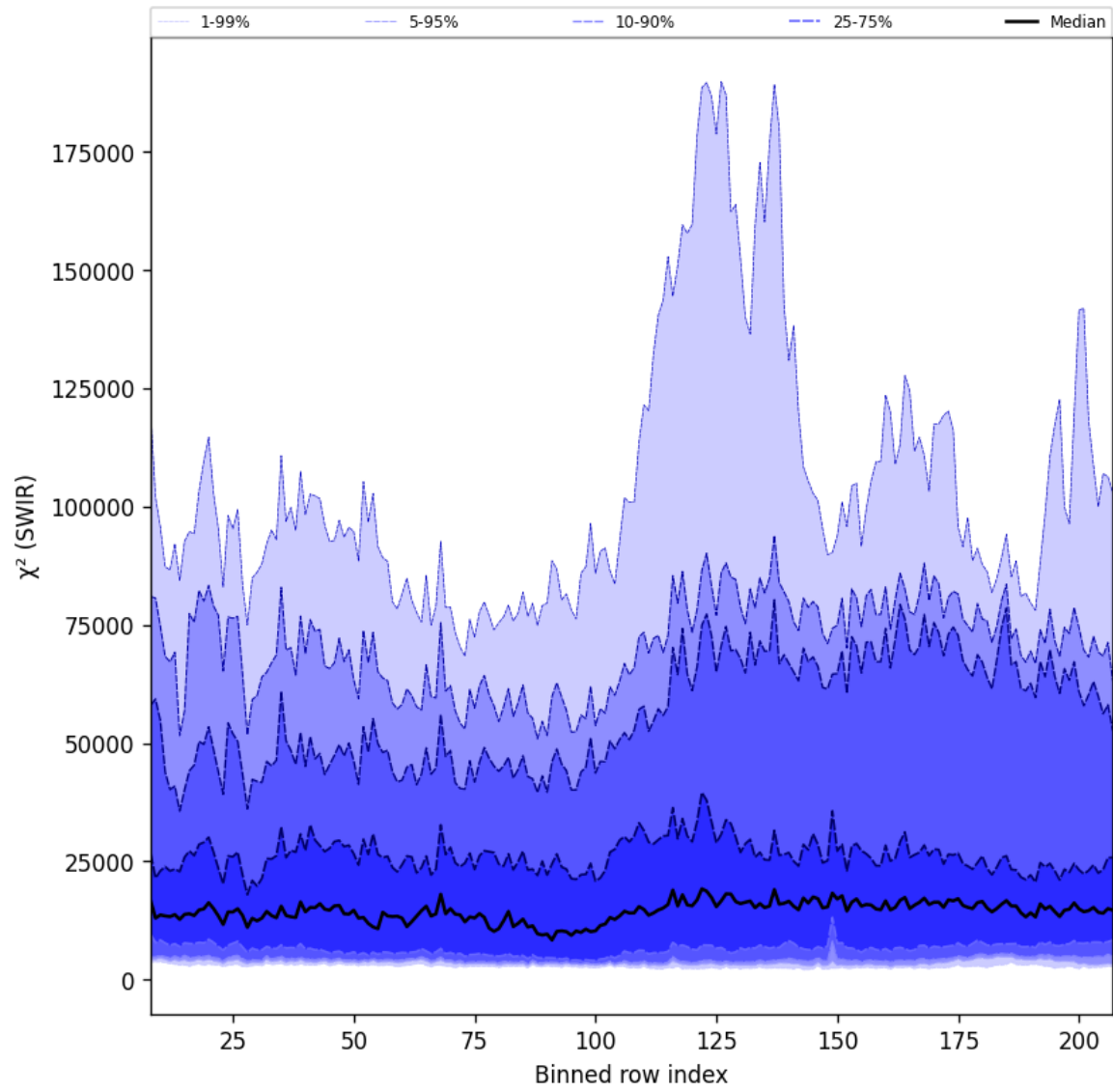
Figure 39: Along track statistics of “ \chi^2 (SWIR)” for 2024-09-02 to 2024-09-04
