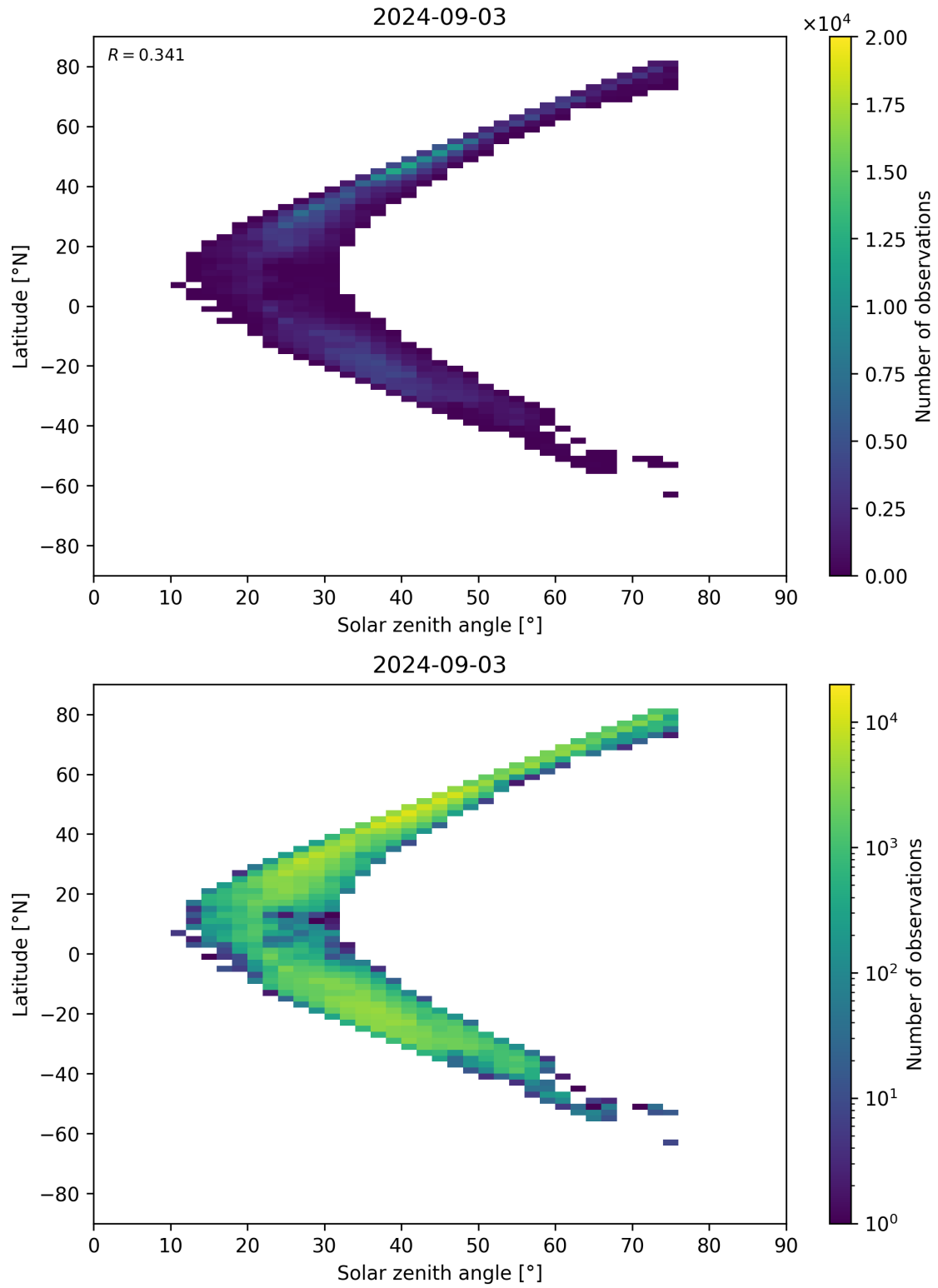
Figure 98: Scatter density plot of “Solar zenith angle” against “Latitude” for 2024-09-02 to 2024-09-04.
