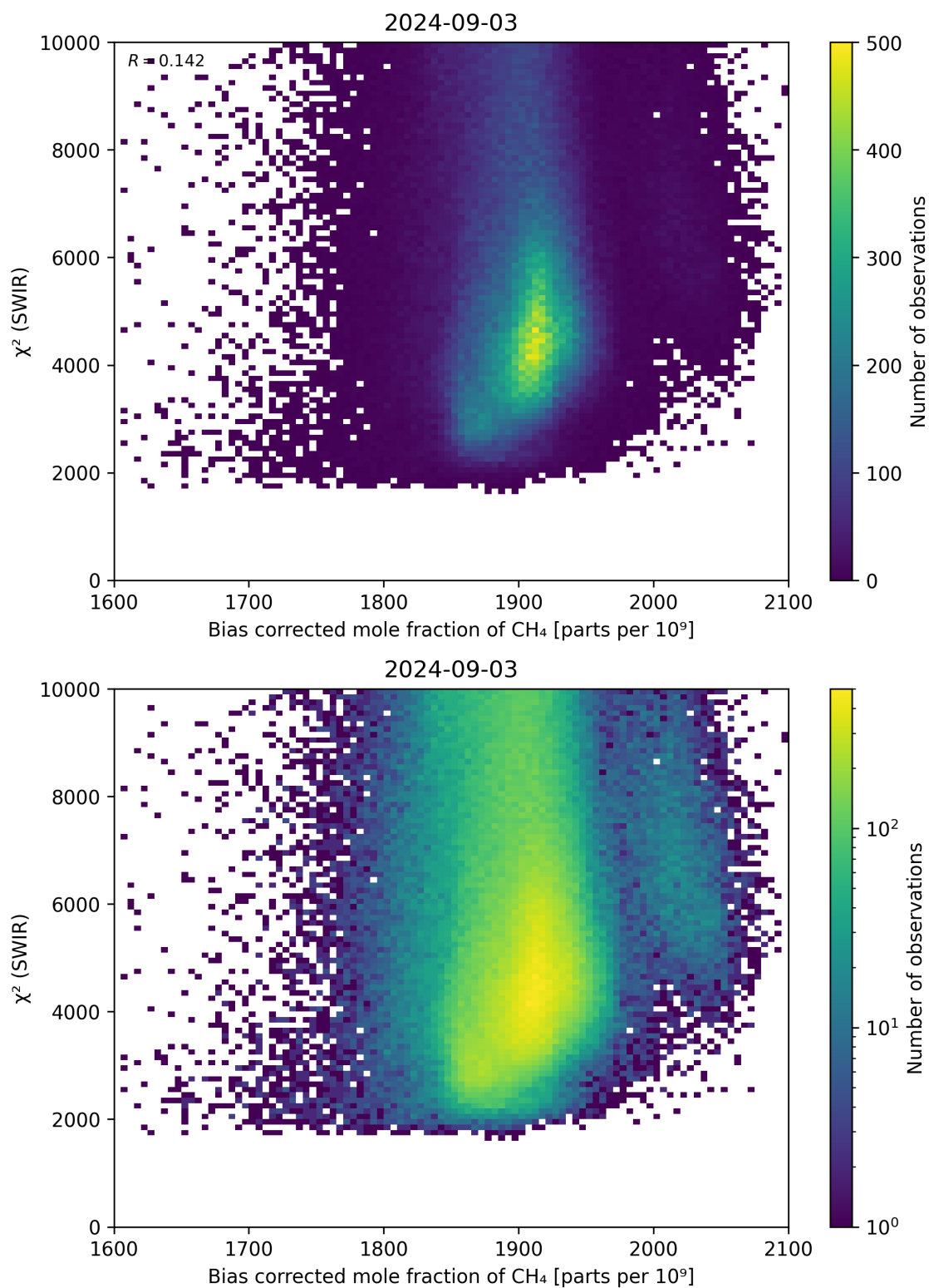
Figure 64: Scatter density plot of “Bias corrected mole fraction of \text{CH}_4 ” against “ \chi^2 (SWIR)” for 2024-09-02 to 2024-09-04.
