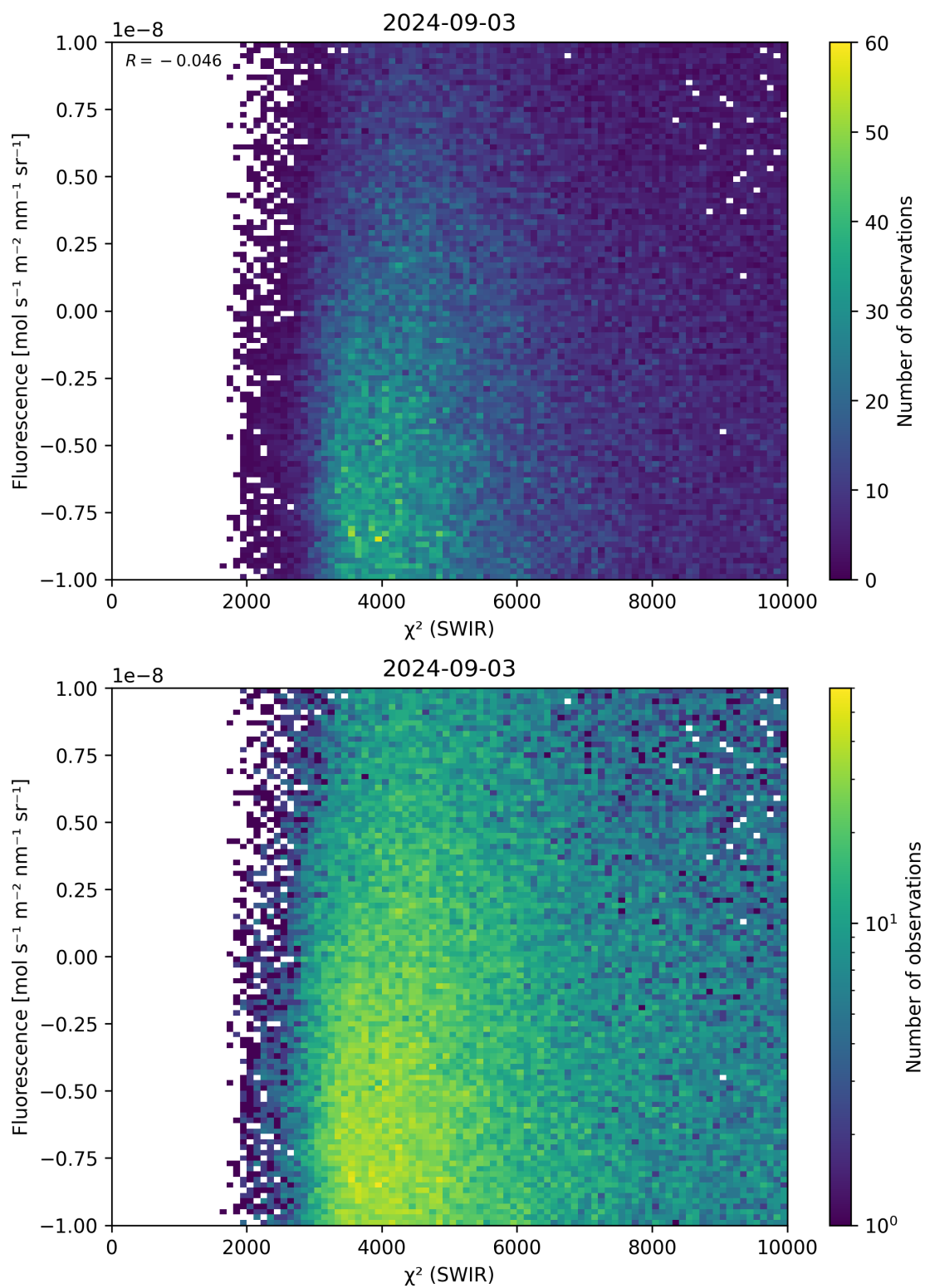
Figure 49: Scatter density plot of “ \chi^2 (SWIR)” against “Fluorescence” for 2024-09-02 to 2024-09-04.
