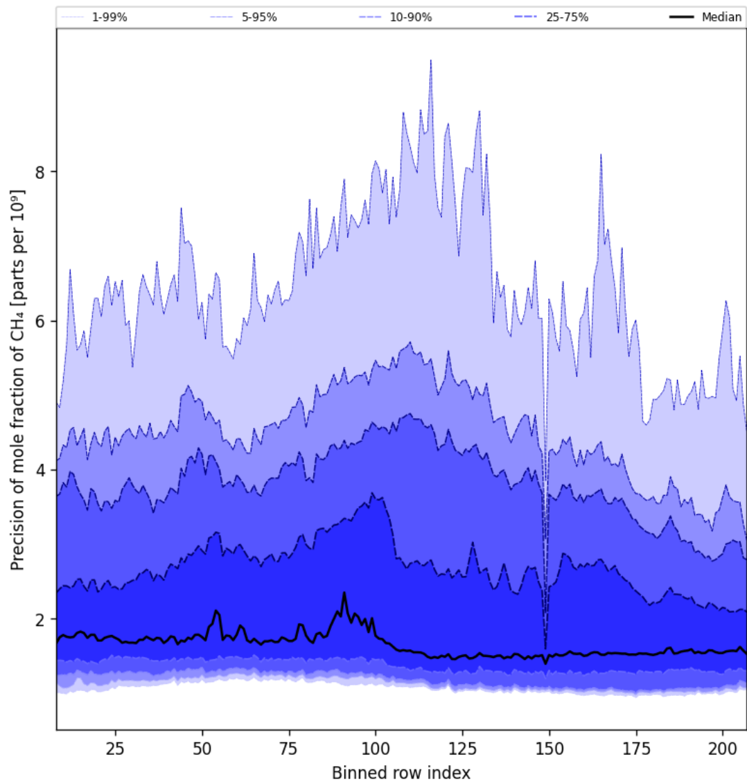
Figure 35: Along track statistics of “Precision of mole fraction of CH 4 ” for 2024-09-02 to 2024-09-04
