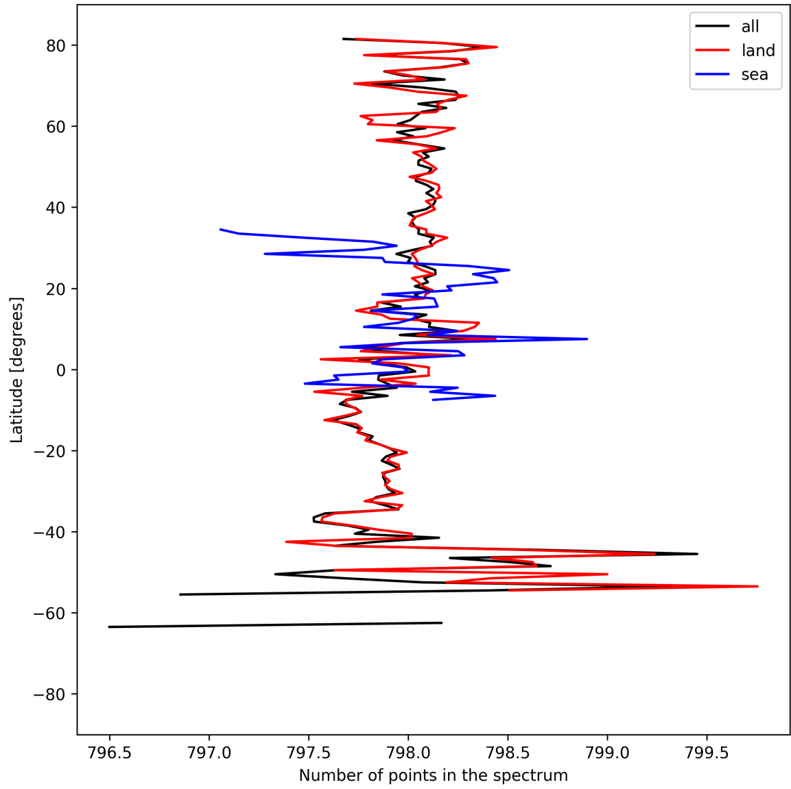
Figure 15: Zonal average of “Number of points in the spectrum” for 2024-09-02 to 2024-09-04.
