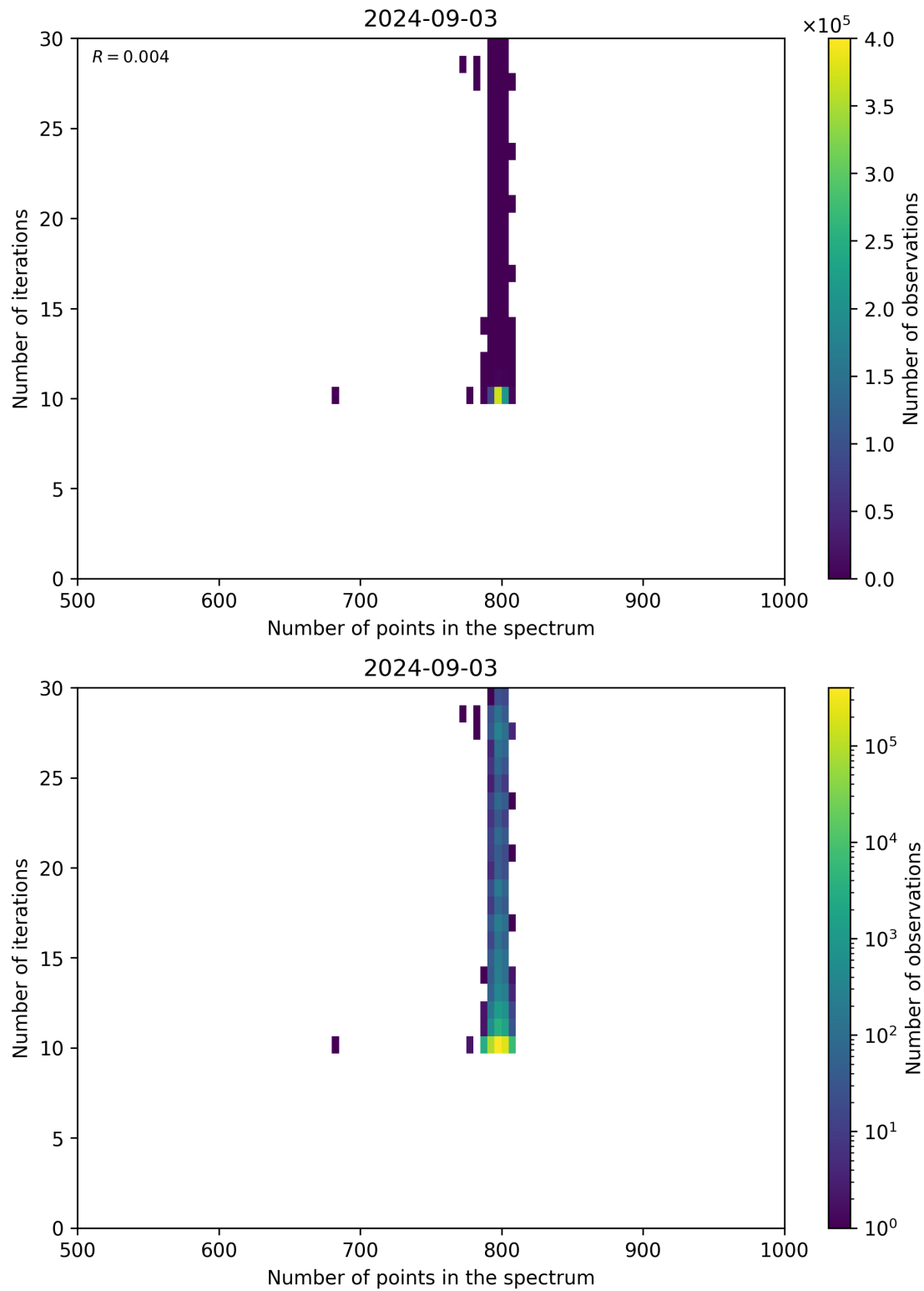
Figure 92: Scatter density plot of “Number of points in the spectrum” against “Number of iterations” for 2024-09-02 to 2024-09-04.
