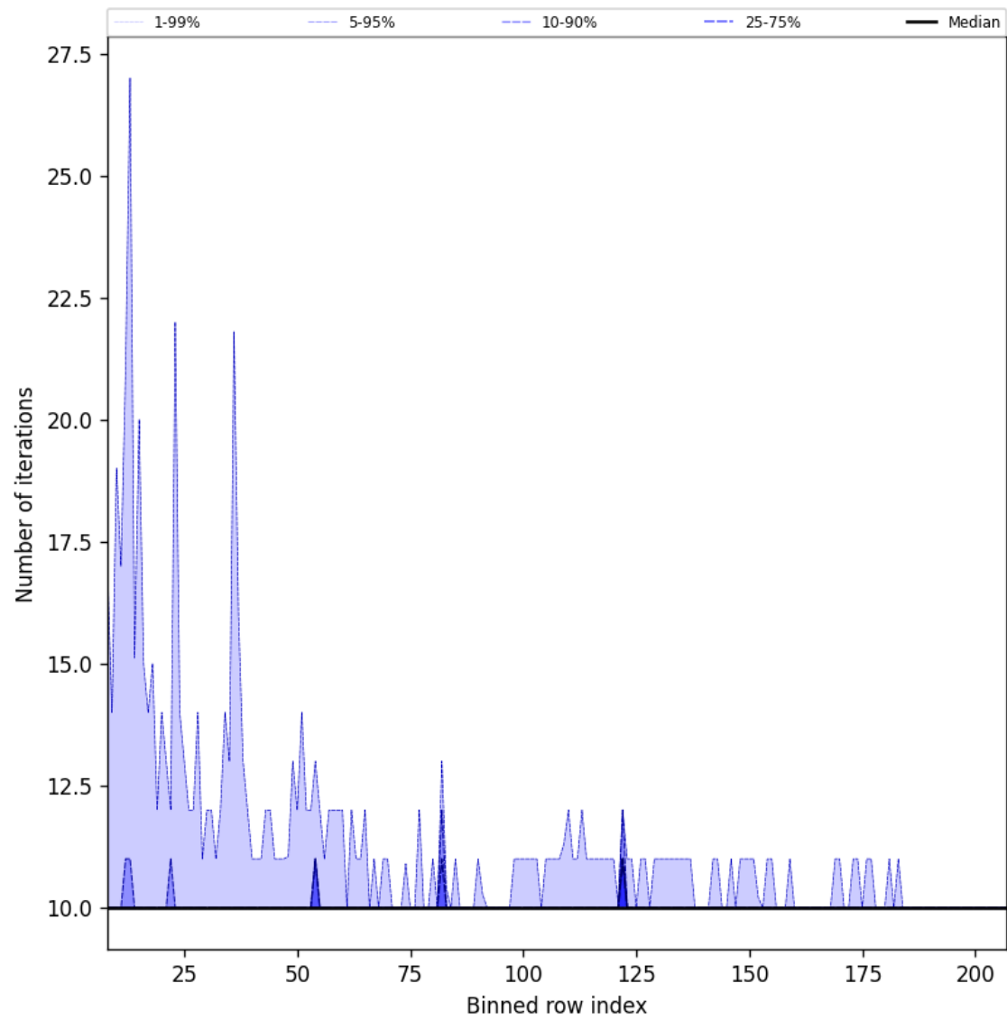
Figure 42: Along track statistics of “Number of iterations” for 2024-09-02 to 2024-09-04
