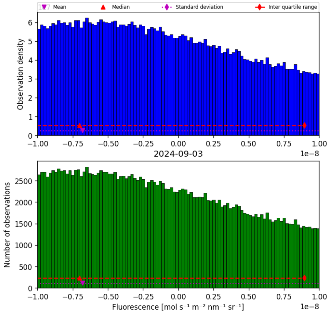
Figure 32: Histogram of “Fluorescence” for 2024-09-02 to 2024-09-04
