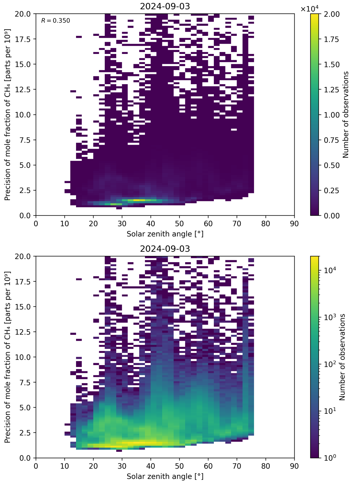
Figure 101: Scatter density plot of “Solar zenith angle” against “Precision of mole fraction of \text{CH}_4 ” for 2024-09-02 to 2024-09-04.
