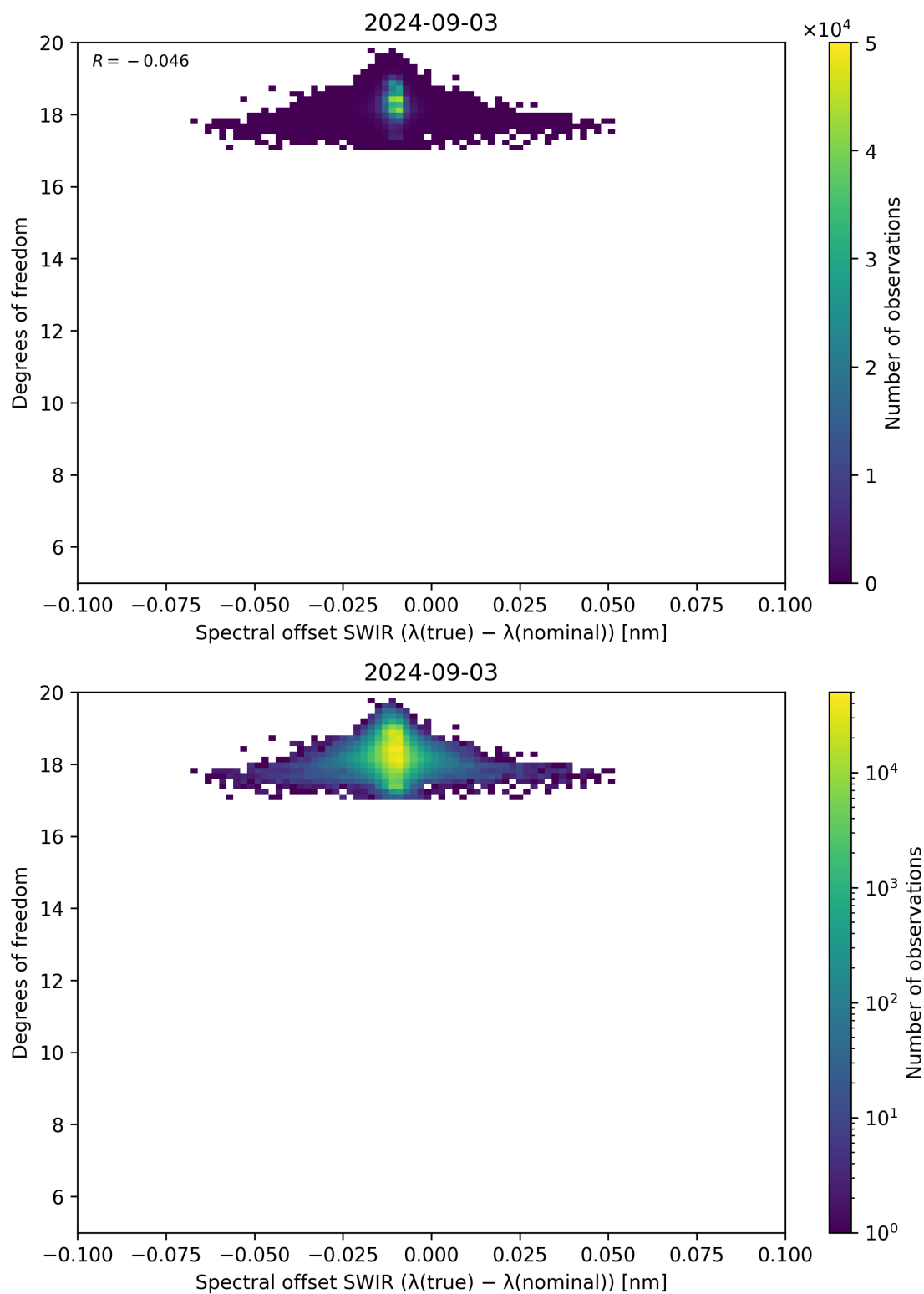
Figure 119: Scatter density plot of “Spectral offset SWIR ( \lambda_{\text{true}} - \lambda_{\text{nominal}} )” against “Degrees of freedom” for 2024-09-02 to 2024-09-04.
