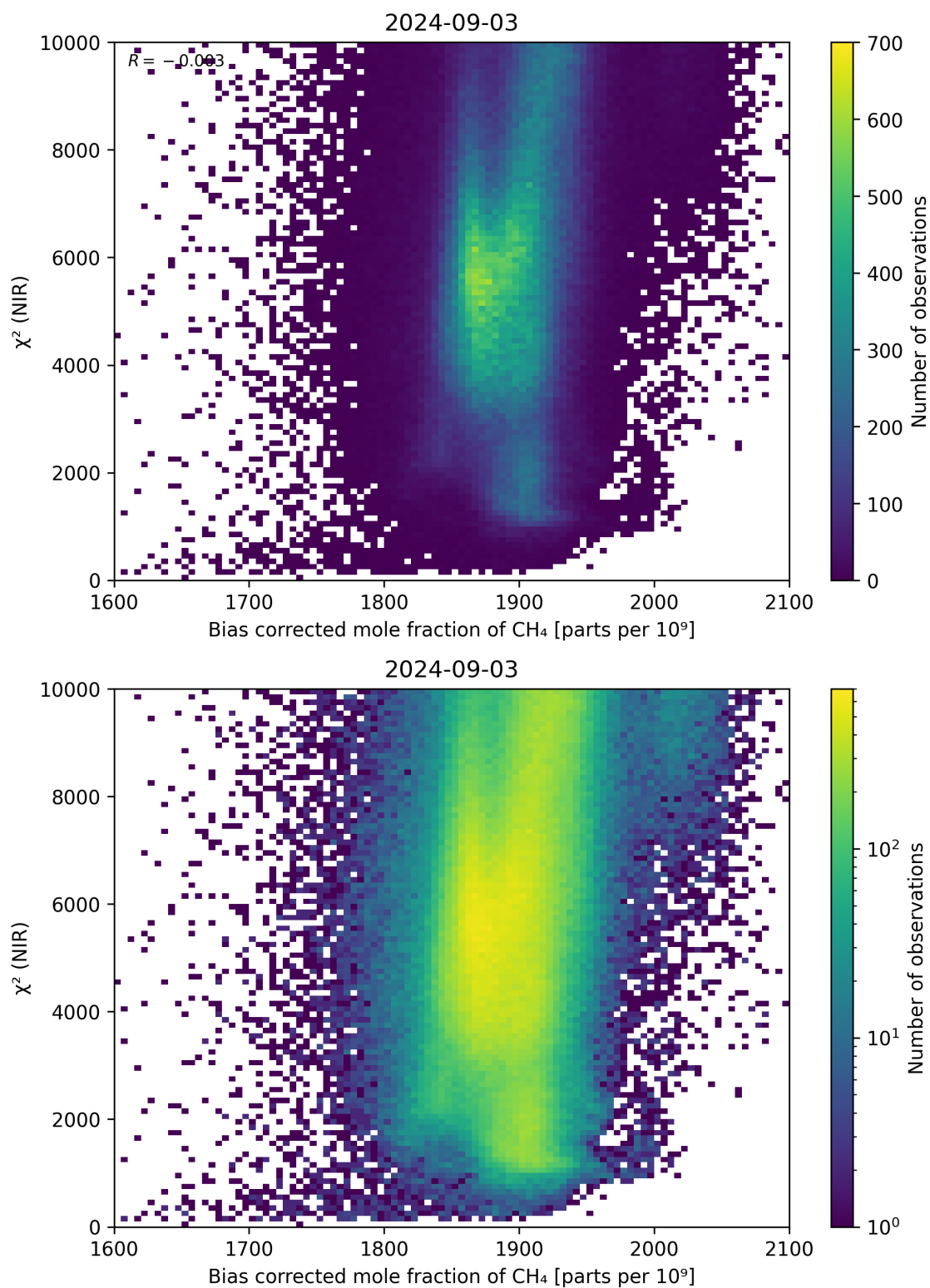
Figure 63: Scatter density plot of “Bias corrected mole fraction of CH 4 ” against “ \chi^2 (NIR)” for 2024-09-02 to 2024-09-04.
