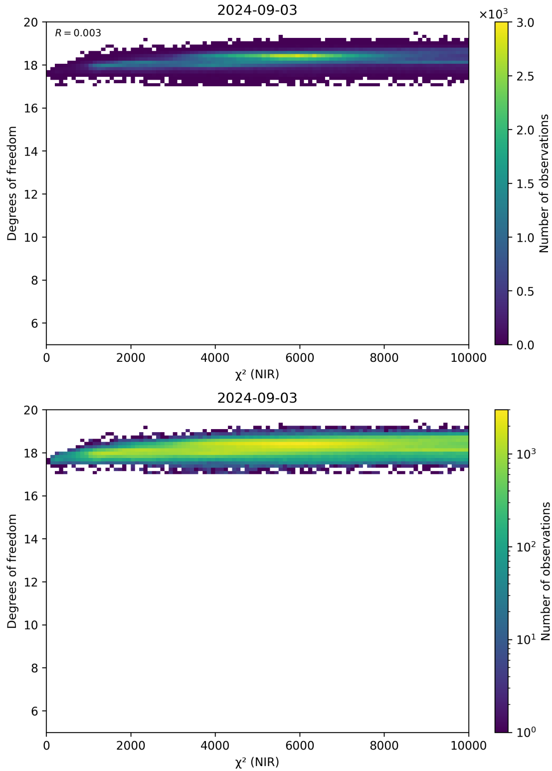
Figure 44: Scatter density plot of “ \chi^2 (NIR)” against “Degrees of freedom” for 2024-09-02 to 2024-09-04.
