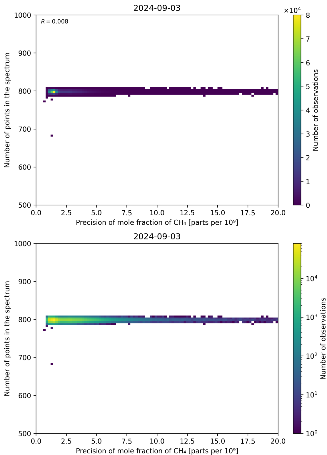
Figure 84: Scatter density plot of “Precision of mole fraction of CH 4 ” against “Number of points in the spectrum” for 2024-09-02 to 2024-09-04.
