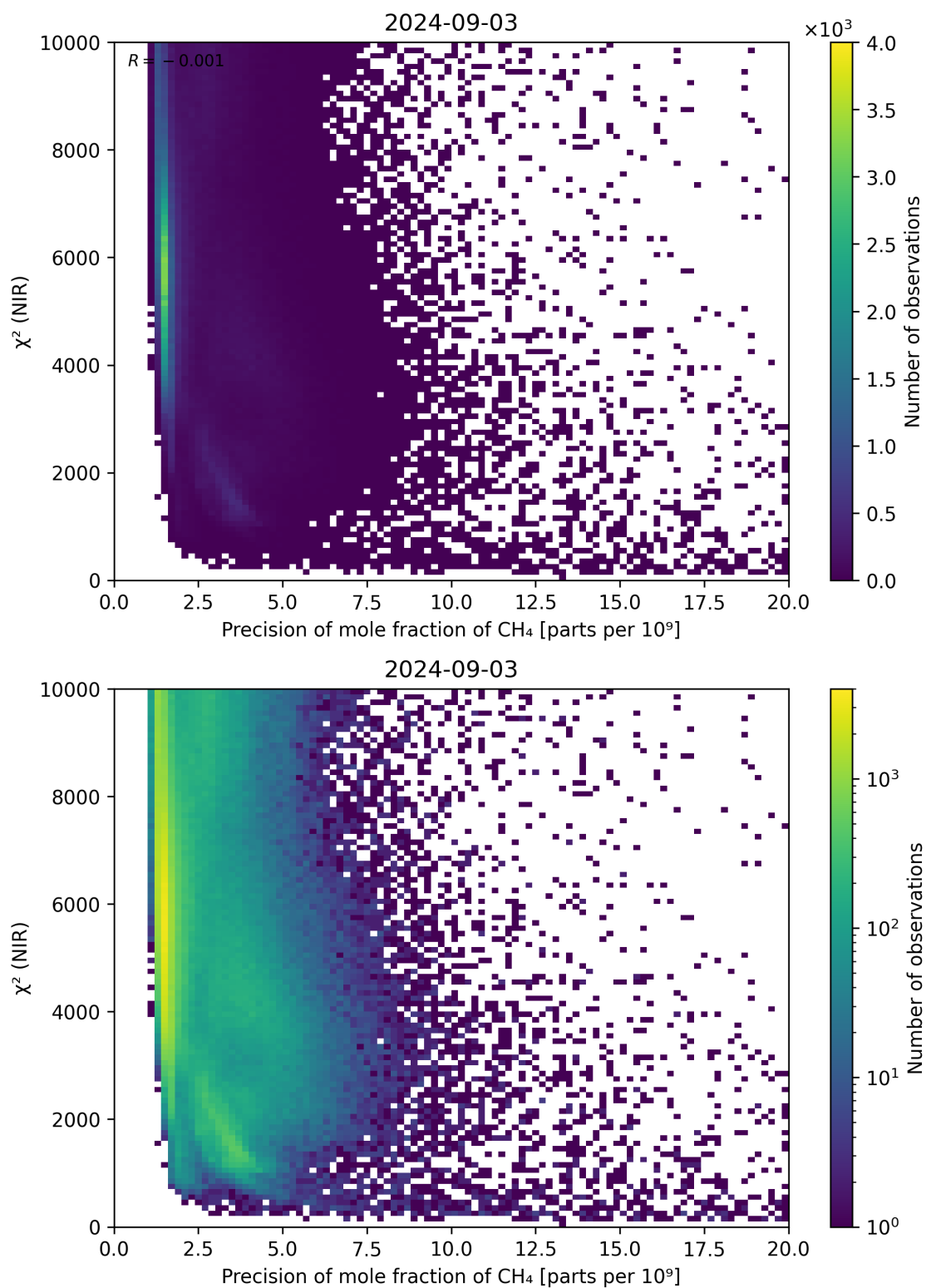
Figure 78: Scatter density plot of “Precision of mole fraction of CH 4 ” against “ \chi^2 (NIR)” for 2024-09-02 to 2024-09-04.
