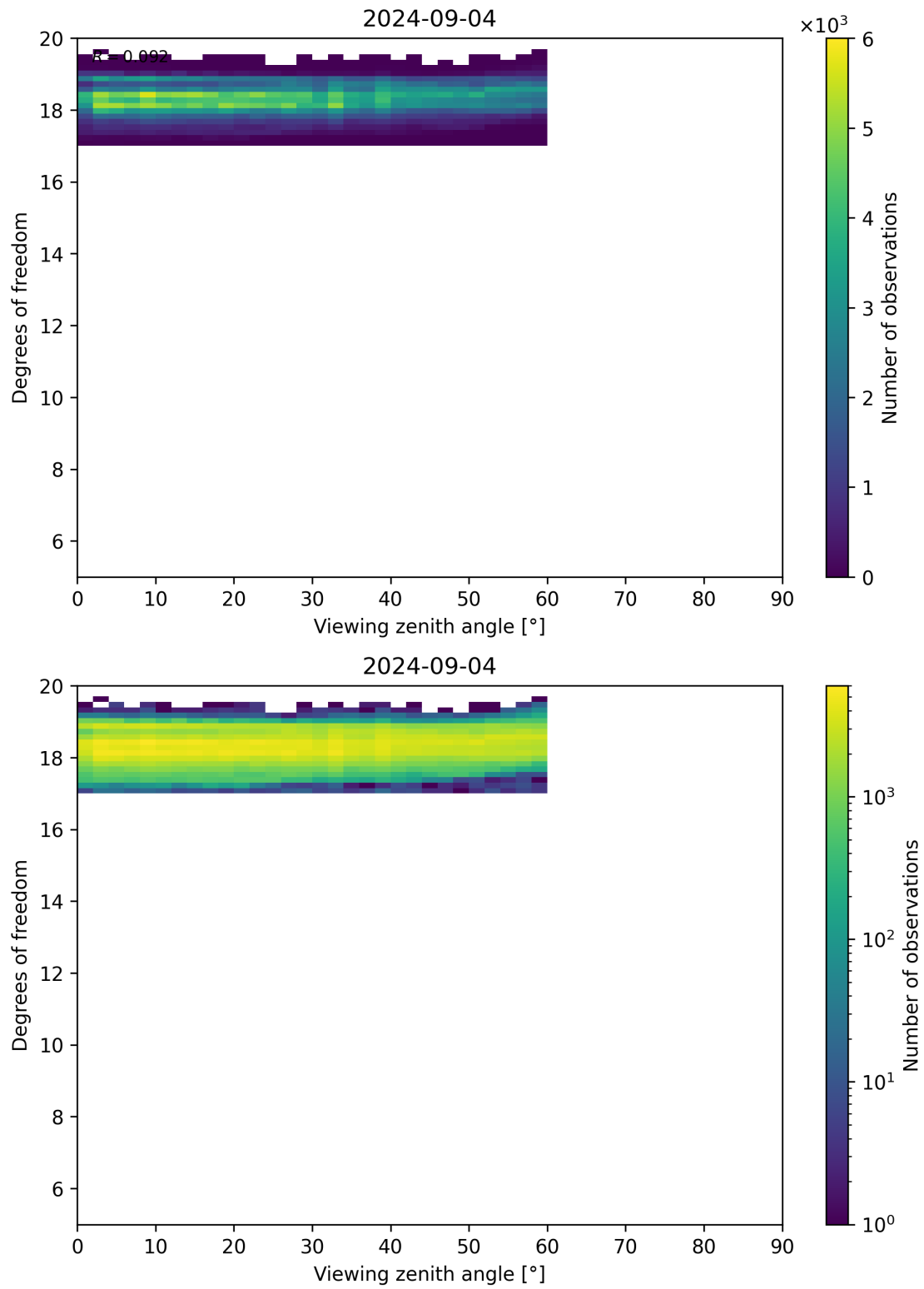
Figure 107: Scatter density plot of “Viewing zenith angle” against “Degrees of freedom” for 2024-09-03 to 2024-09-05.
