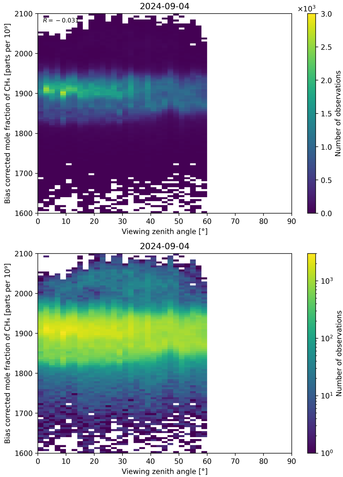
Figure 111: Scatter density plot of “Viewing zenith angle” against “Bias corrected mole fraction of CH 4 ” for 2024-09-03 to 2024-09-05.
