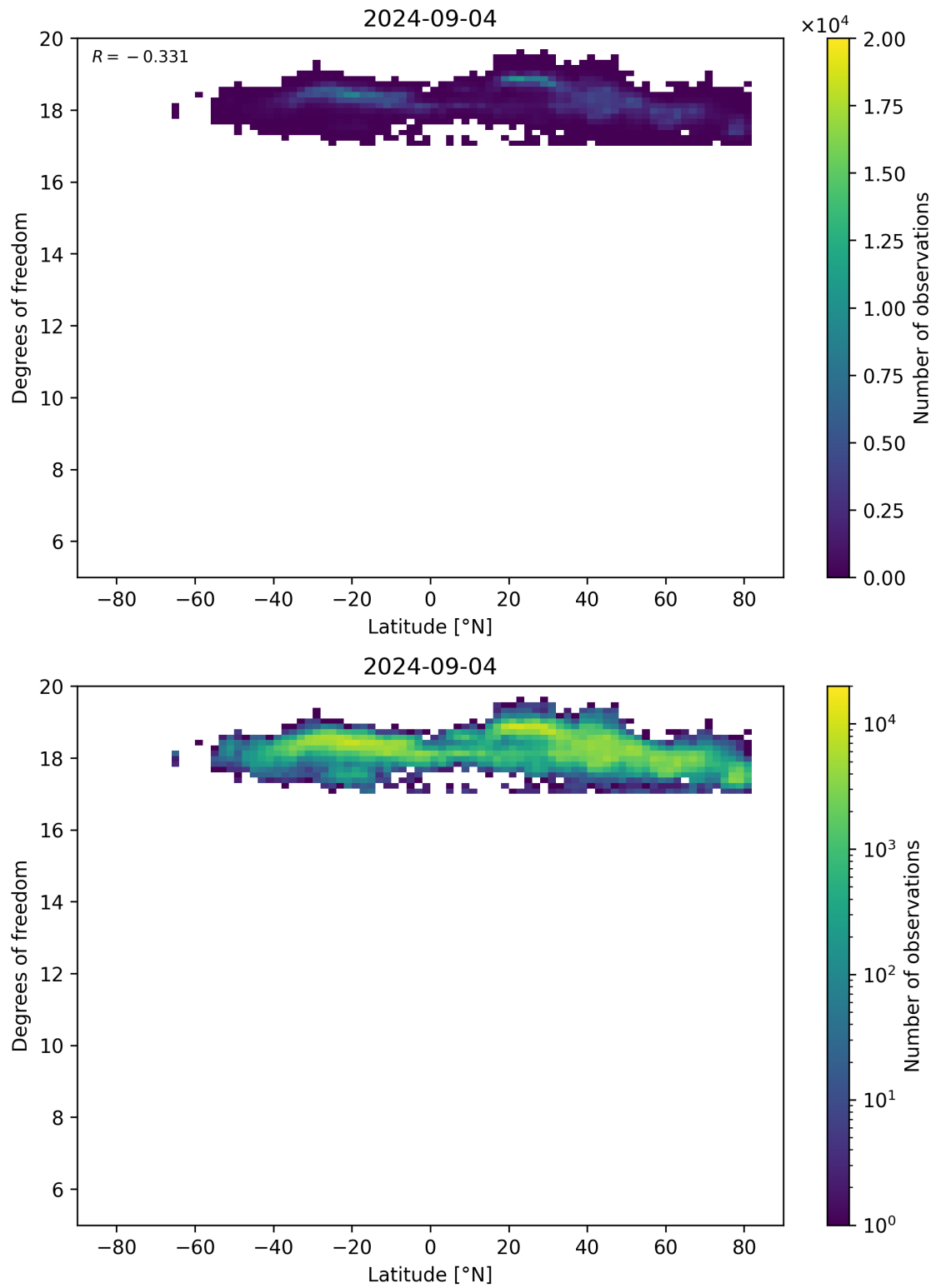
Figure 55: Scatter density plot of “Latitude” against “Degrees of freedom” for 2024-09-03 to 2024-09-05.
