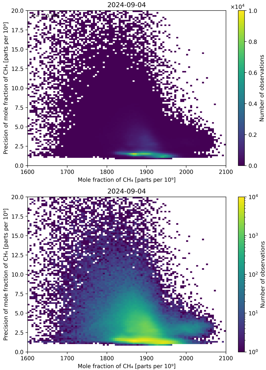
Figure 75: Scatter density plot of “Mole fraction of CH 4 ” against “Precision of mole fraction of CH 4 ” for 2024-09-03 to 2024-09-05.
