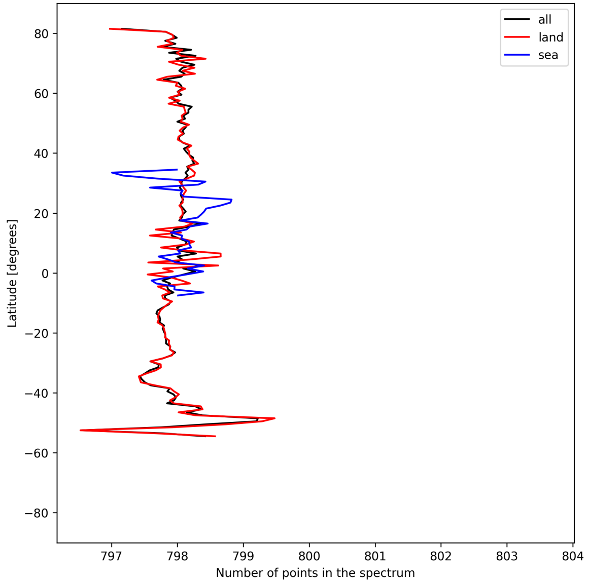
Figure 15: Zonal average of “Number of points in the spectrum” for 2024-09-03 to 2024-09-05.
