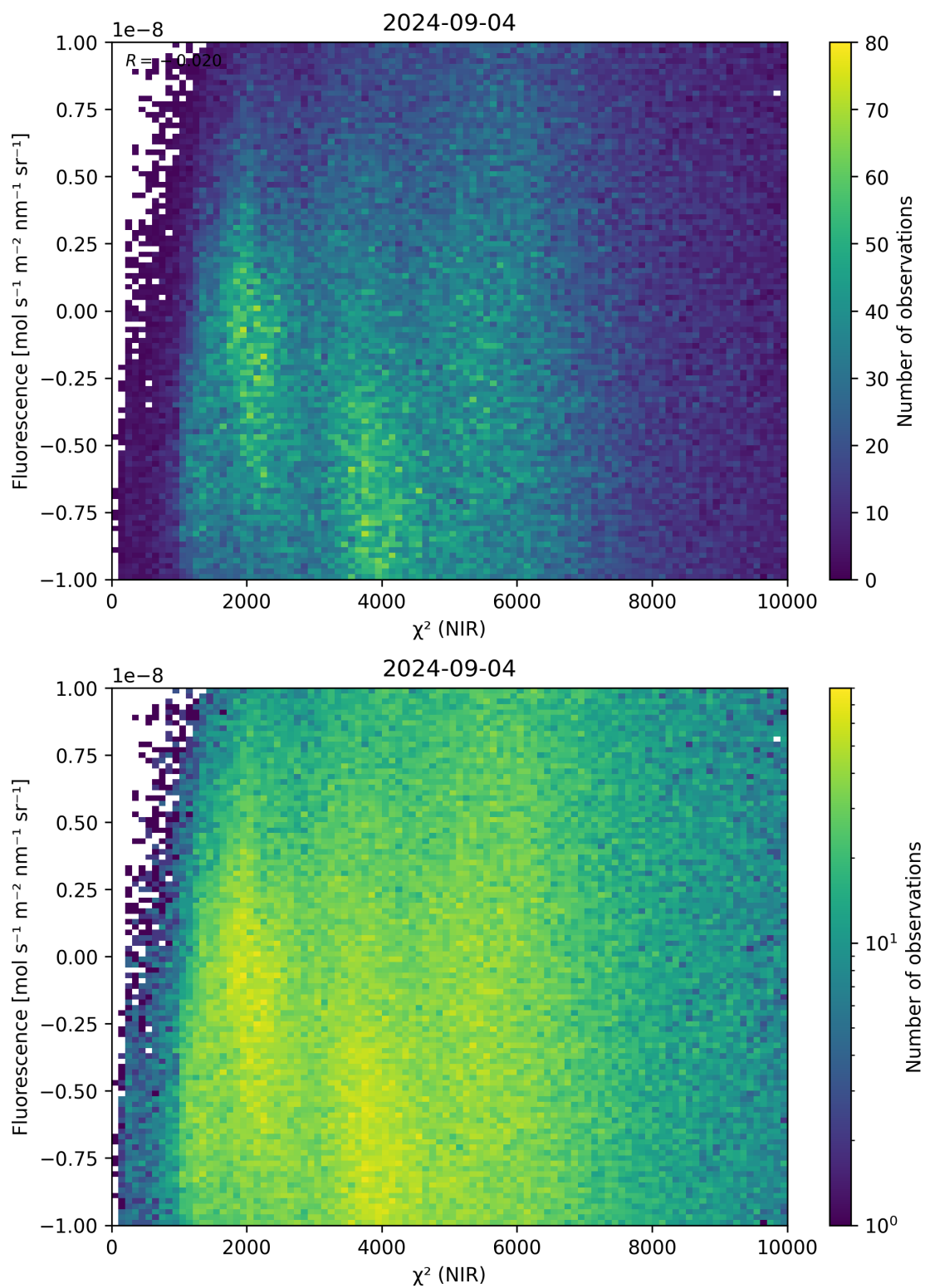
Figure 45: Scatter density plot of “ \chi^2 (NIR)” against “Fluorescence” for 2024-09-03 to 2024-09-05.
