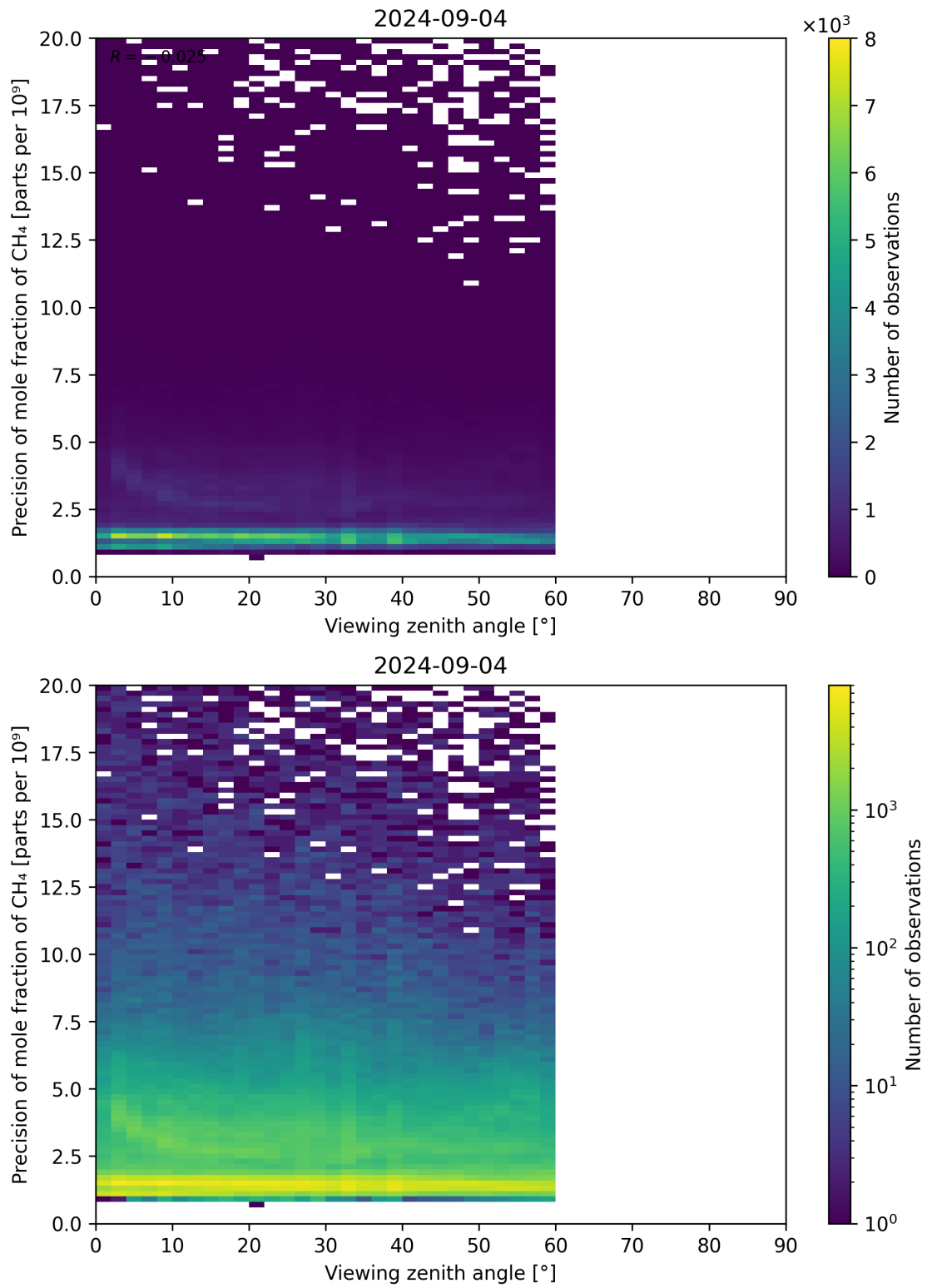
Figure 112: Scatter density plot of “Viewing zenith angle” against “Precision of mole fraction of CH 4 ” for 2024-09-03 to 2024-09-05.
