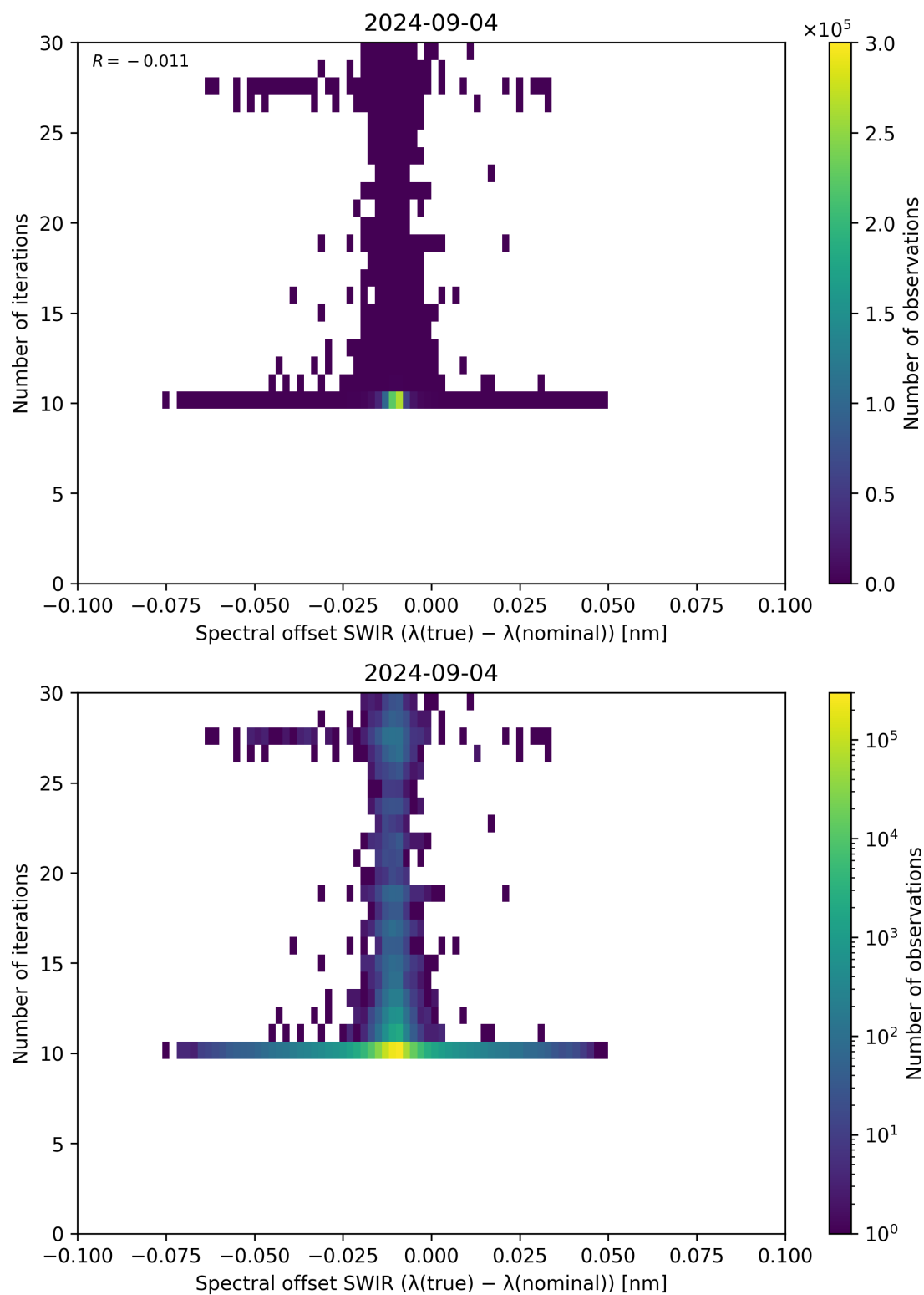
Figure 121: Scatter density plot of “Spectral offset SWIR ( \lambda_{\text{true}} - \lambda_{\text{nominal}} )” against “Number of iterations” for 2024-09-03 to 2024-09-05.
