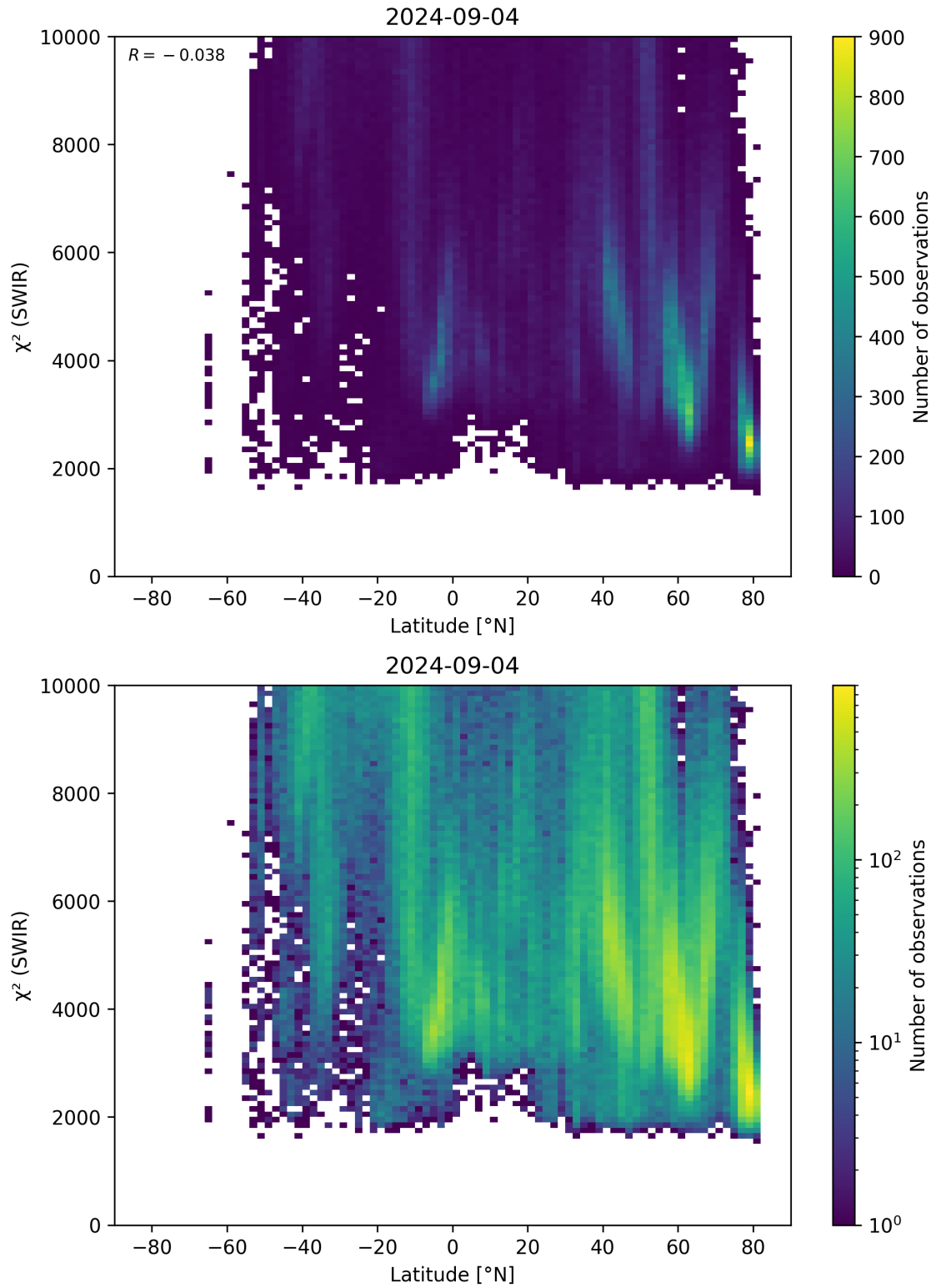
Figure 54: Scatter density plot of “Latitude” against “ \chi^2 (SWIR)” for 2024-09-03 to 2024-09-05.
