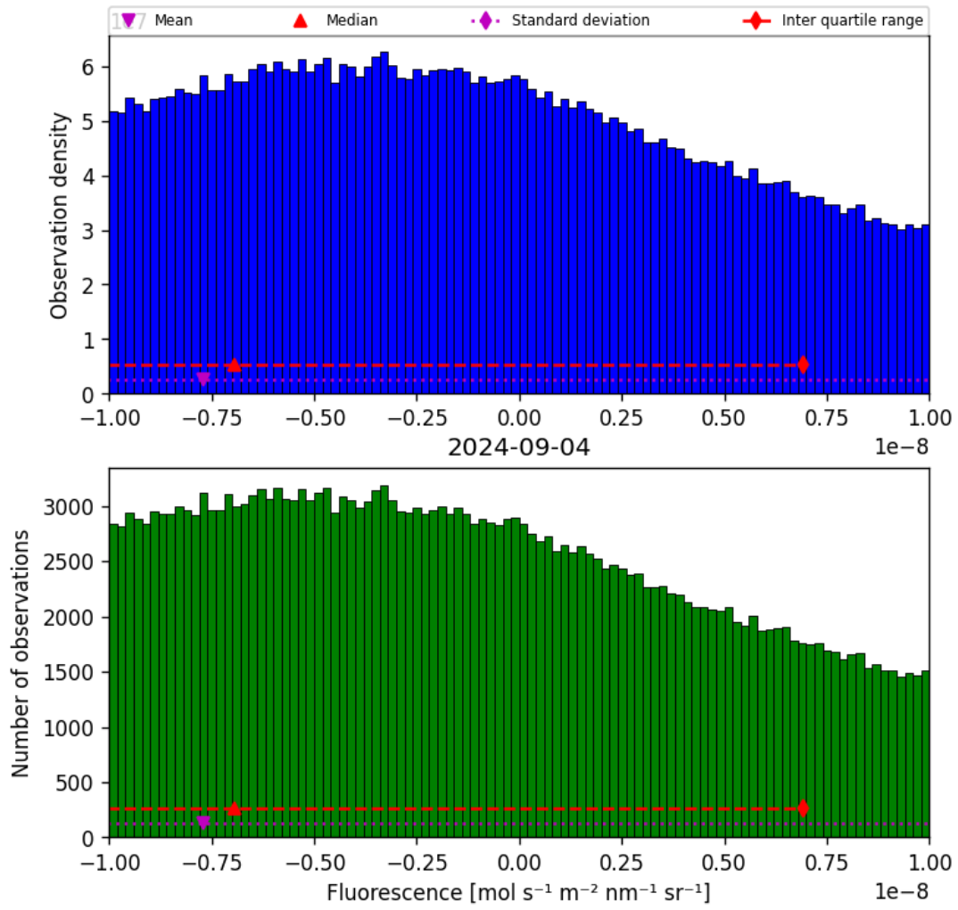
Figure 32: Histogram of “Fluorescence” for 2024-09-03 to 2024-09-05
