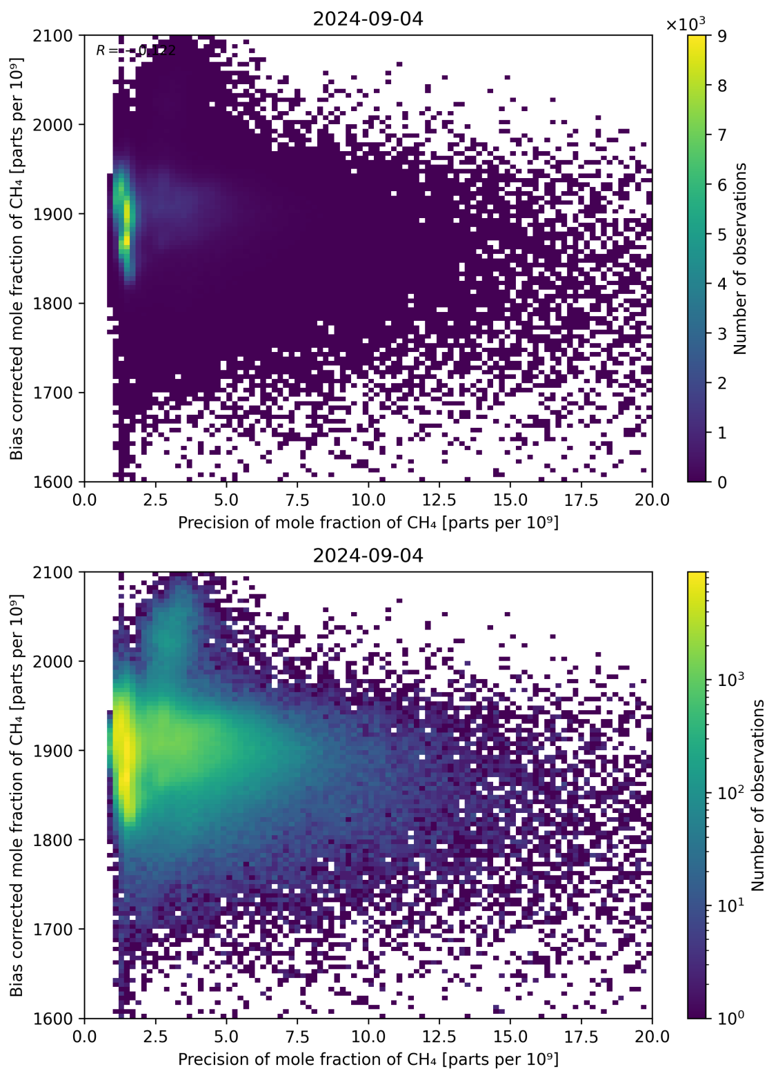
Figure 82: Scatter density plot of “Precision of mole fraction of CH 4 ” against “Bias corrected mole fraction of CH 4 ” for 2024-09-03 to 2024-09-05.
