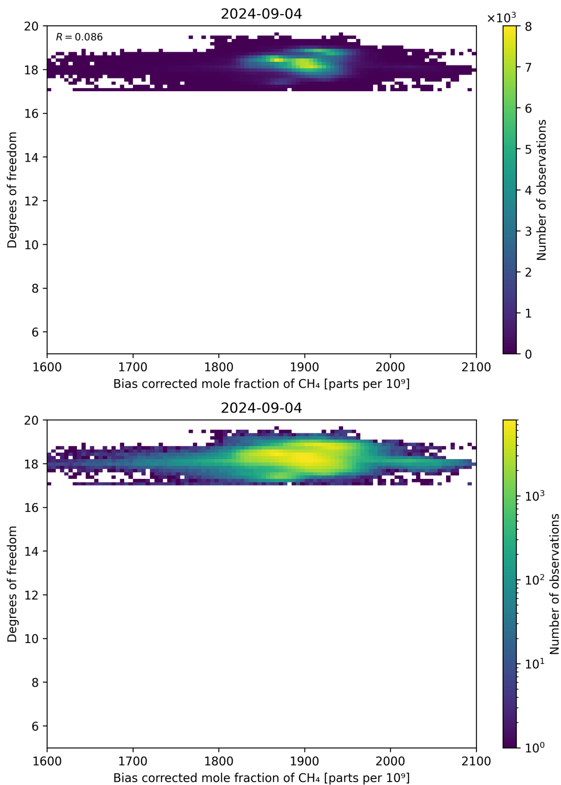
Figure 65: Scatter density plot of “Bias corrected mole fraction of CH 4 ” against “Degrees of freedom” for 2024-09-03 to 2024-09-05.
