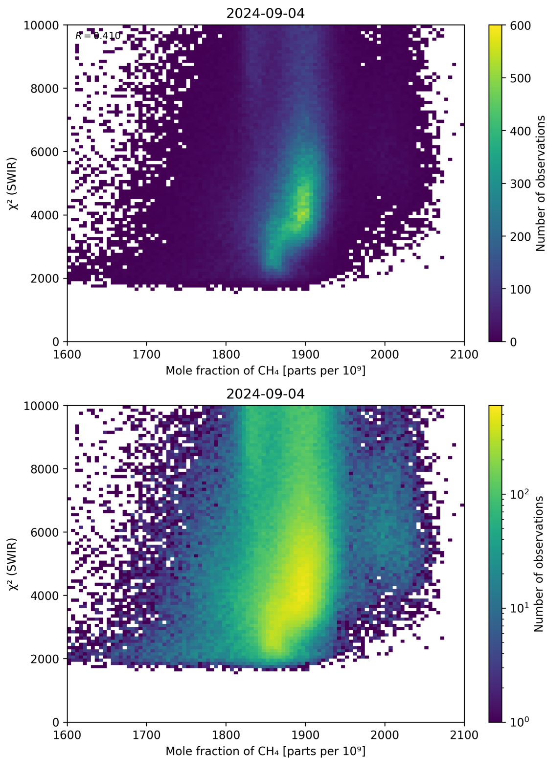
Figure 71: Scatter density plot of “Mole fraction of \text{CH}_4 ” against “ \chi^2 (SWIR)” for 2024-09-03 to 2024-09-05.
