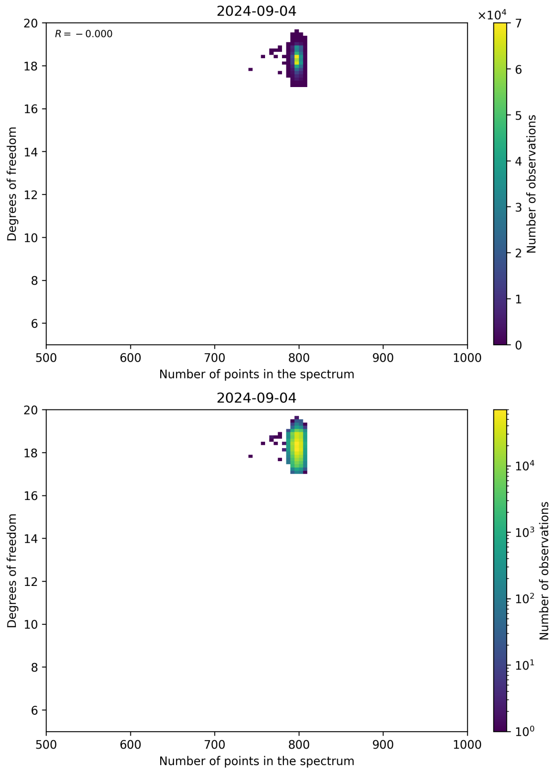
Figure 90: Scatter density plot of “Number of points in the spectrum” against “Degrees of freedom” for 2024-09-03 to 2024-09-05.
