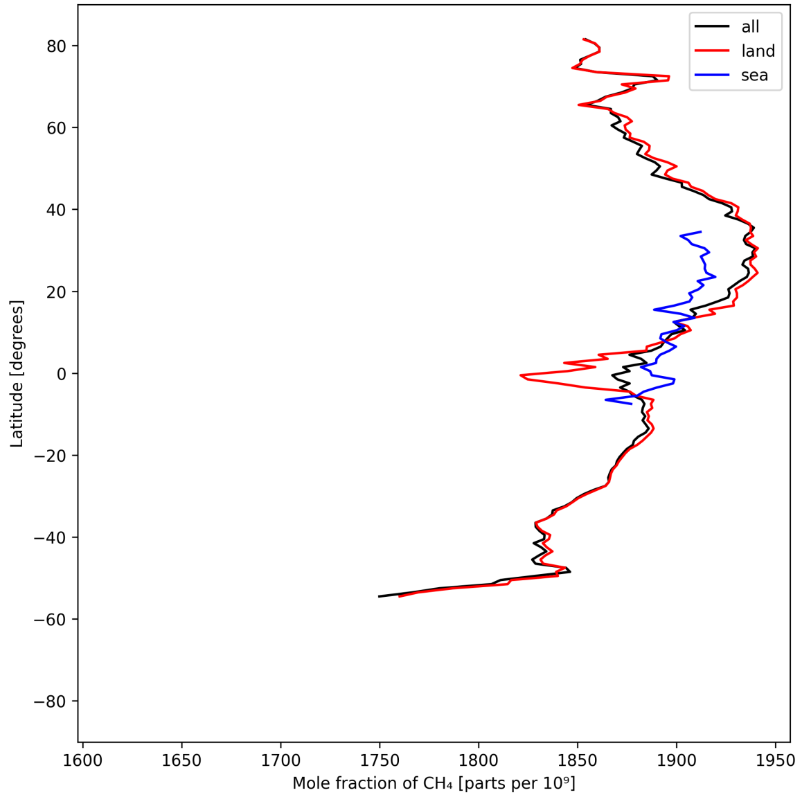
Figure 12: Zonal average of “Mole fraction of CH 4 ” for 2024-09-03 to 2024-09-05.
