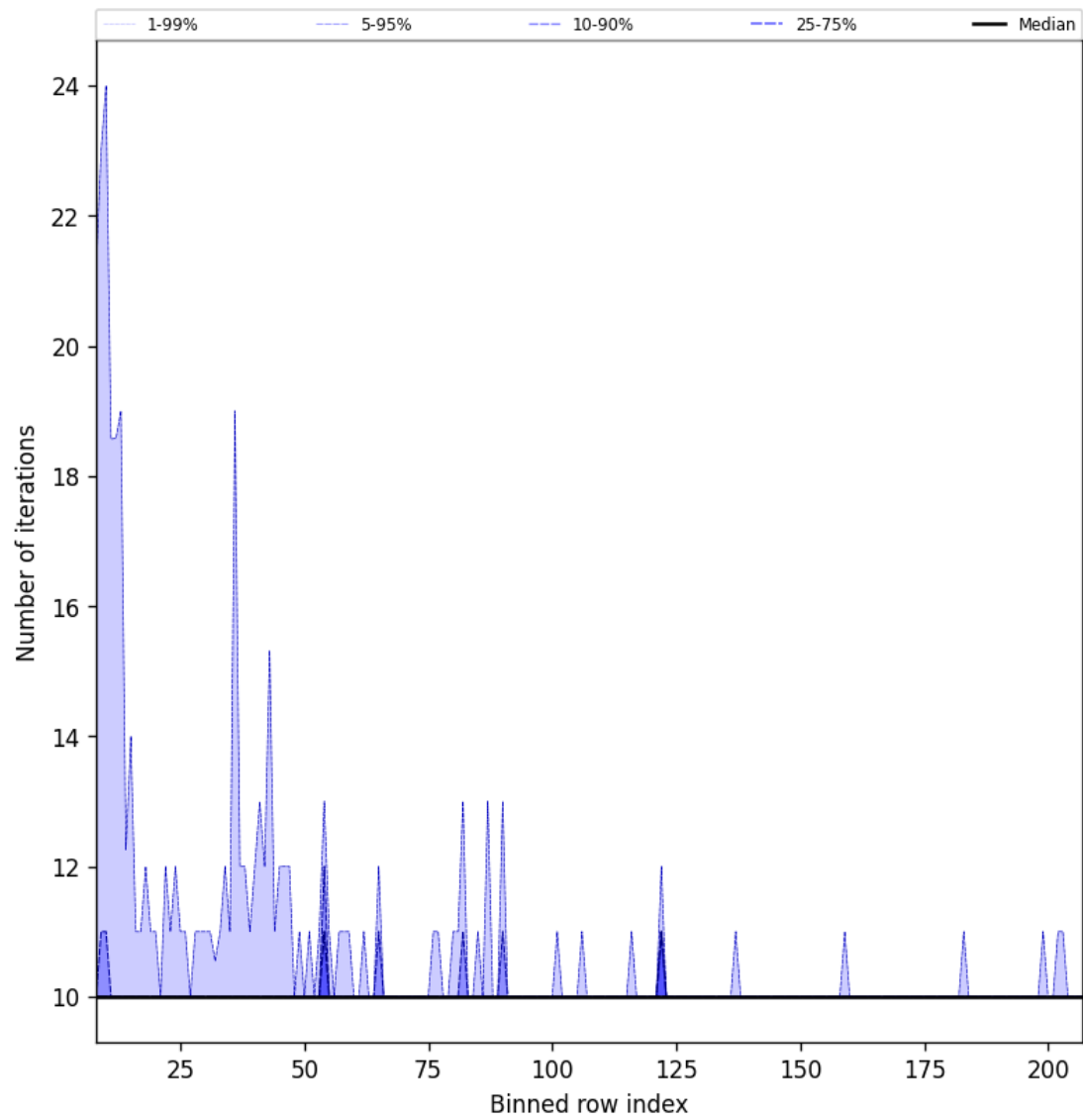
Figure 42: Along track statistics of “Number of iterations” for 2024-09-03 to 2024-09-05
