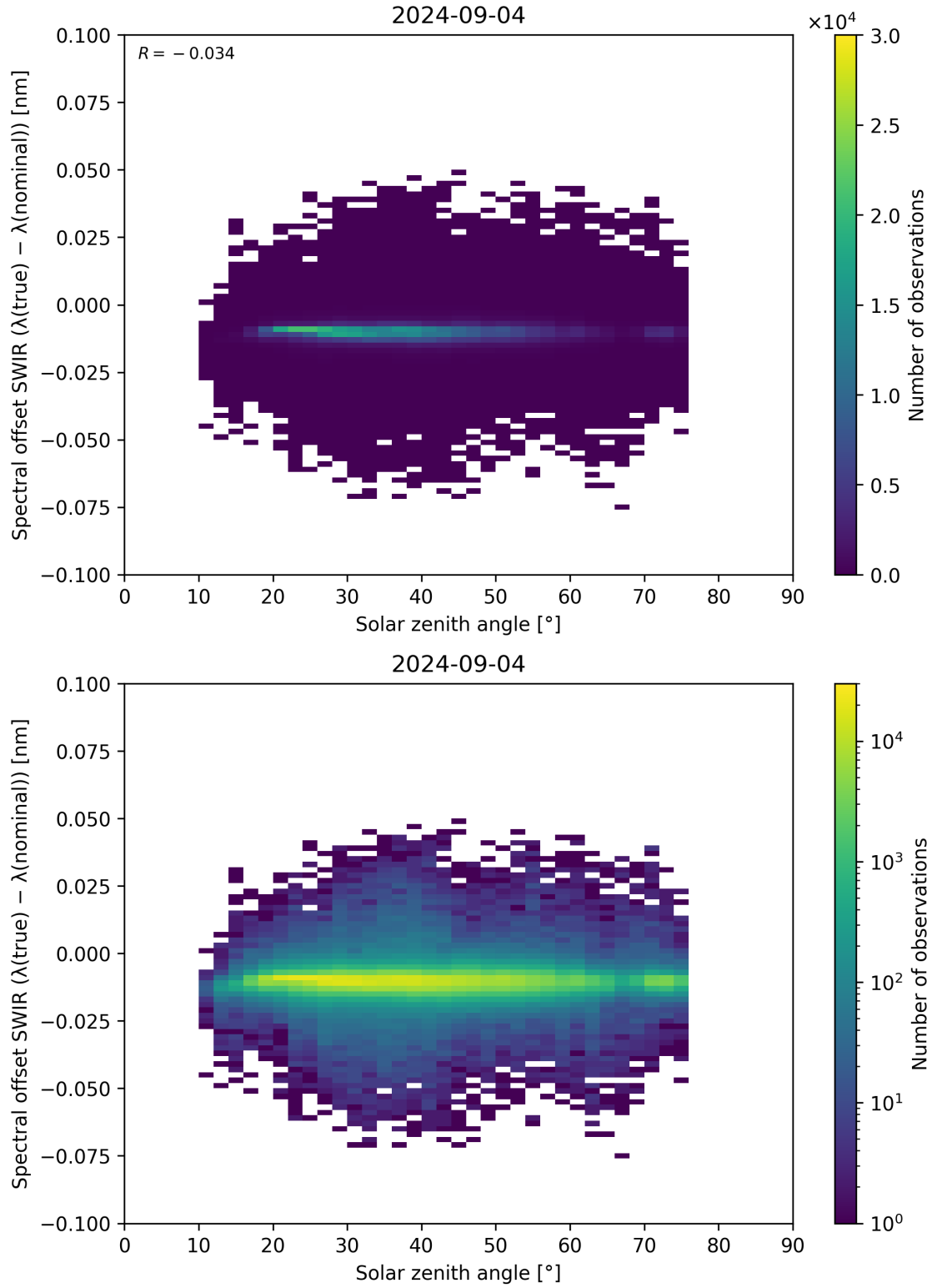
Figure 104: Scatter density plot of “Solar zenith angle” against “Spectral offset SWIR ( \lambda_{\text{true}} - \lambda_{\text{nominal}} )” for 2024-09-03 to 2024-09-05.
