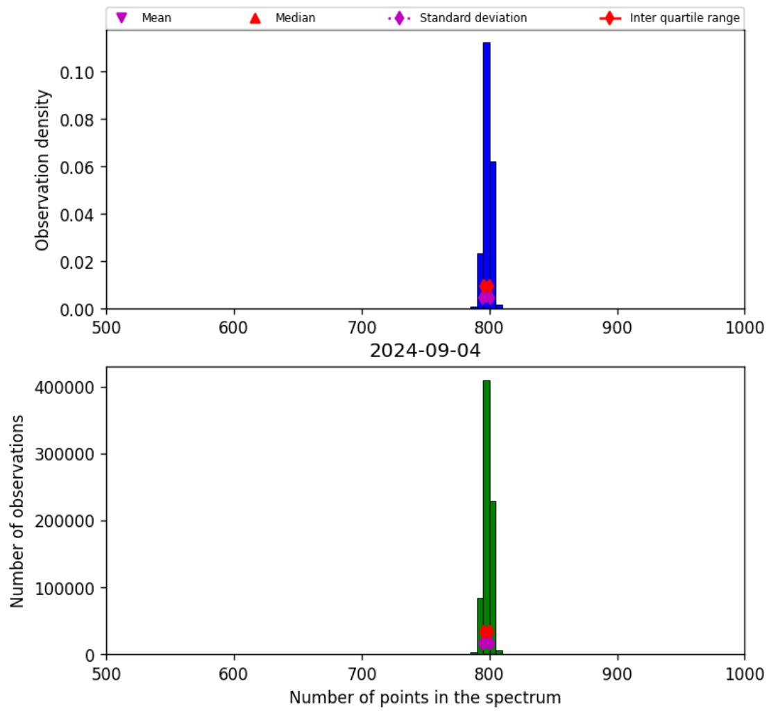
Figure 26: Histogram of “Number of points in the spectrum” for 2024-09-03 to 2024-09-05
