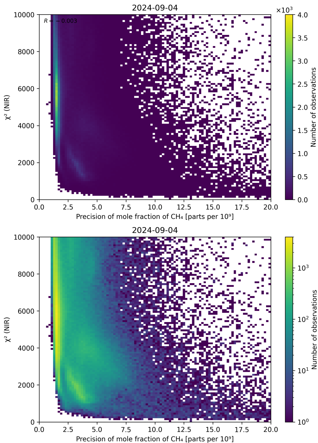
Figure 78: Scatter density plot of “Precision of mole fraction of \text{CH}_4 ” against “ \chi^2 (NIR)” for 2024-09-03 to 2024-09-05.
