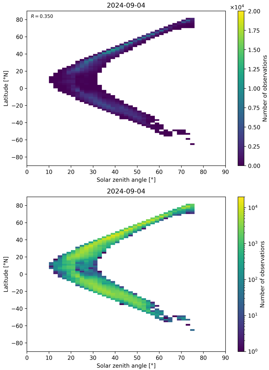
Figure 98: Scatter density plot of “Solar zenith angle” against “Latitude” for 2024-09-03 to 2024-09-05.
