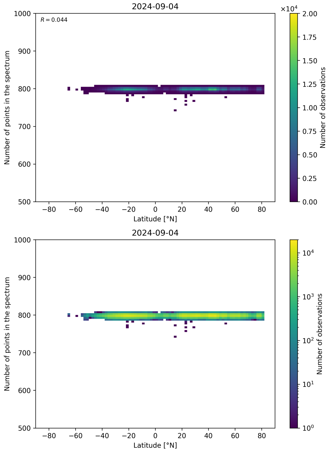
Figure 61: Scatter density plot of “Latitude” against “Number of points in the spectrum” for 2024-09-03 to 2024-09-05.
