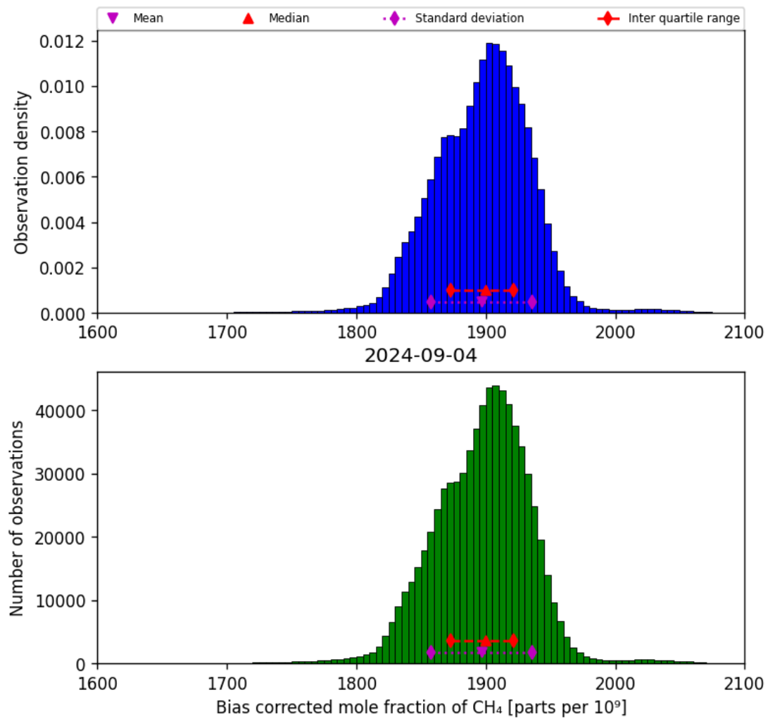
Figure 25: Histogram of “Bias corrected mole fraction of CH 4 ” for 2024-09-03 to 2024-09-05
