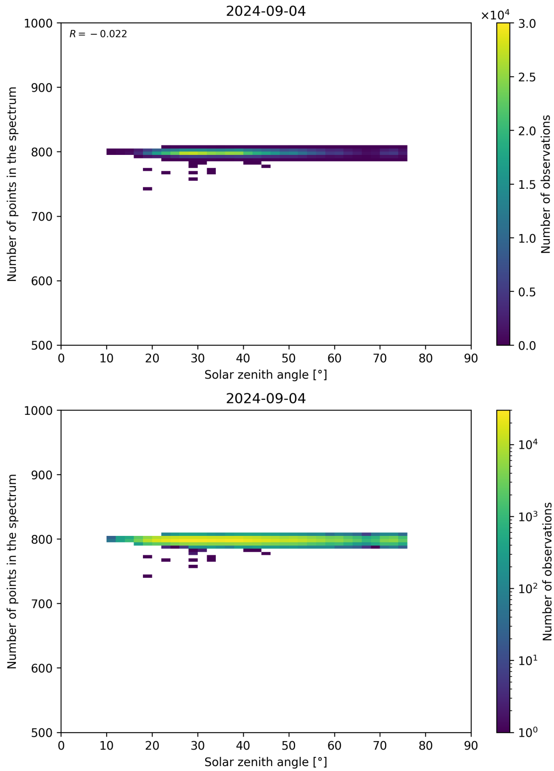
Figure 103: Scatter density plot of “Solar zenith angle” against “Number of points in the spectrum” for 2024-09-03 to 2024-09-05.
