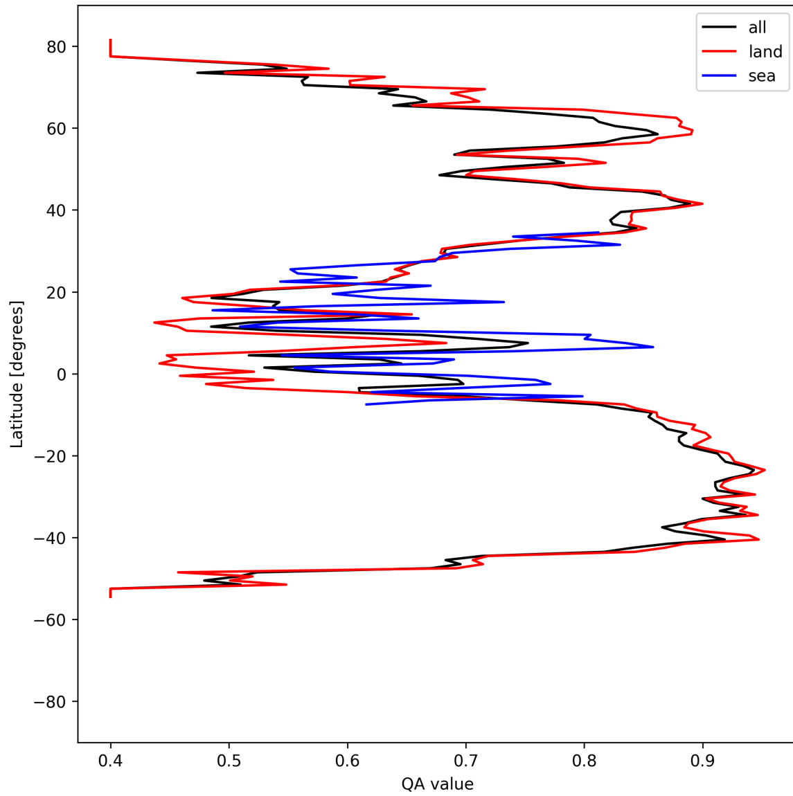
Figure 11: Zonal average of “QA value” for 2024-09-03 to 2024-09-05.
