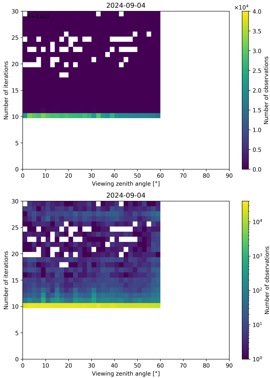
Figure 113: Scatter density plot of “Viewing zenith angle” against “Number of iterations” for 2024-09-03 to 2024-09-05.
