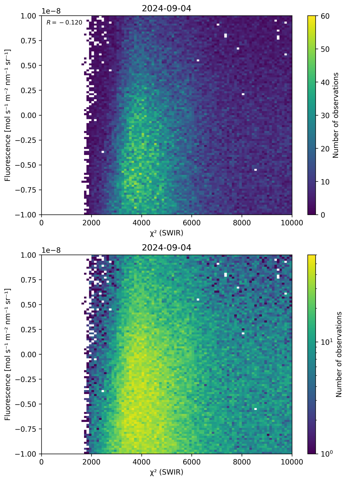
Figure 49: Scatter density plot of “ \chi^2 (SWIR)” against “Fluorescence” for 2024-09-03 to 2024-09-05.
