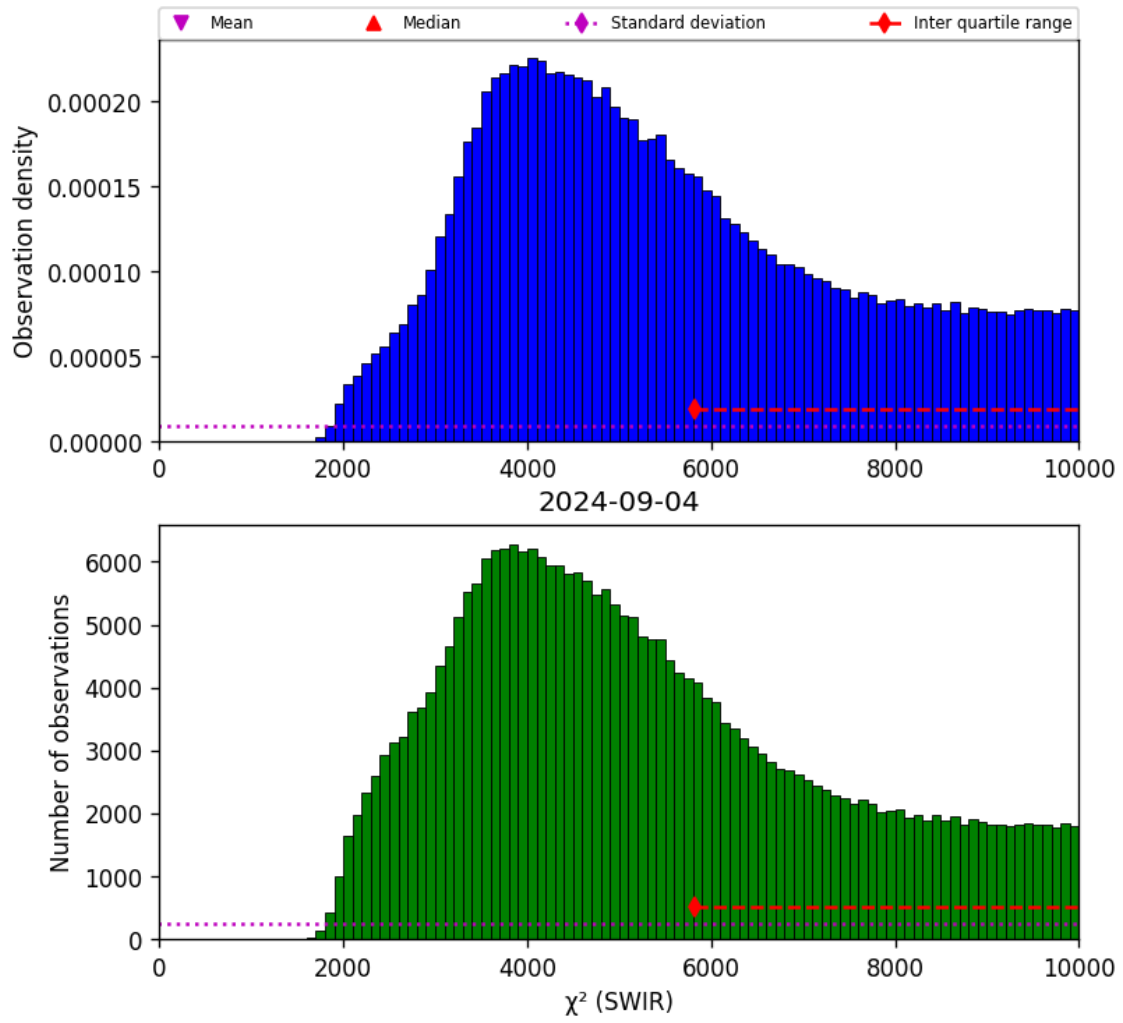
Figure 28: Histogram of " \chi^2 (SWIR)" for 2024-09-03 to 2024-09-05
