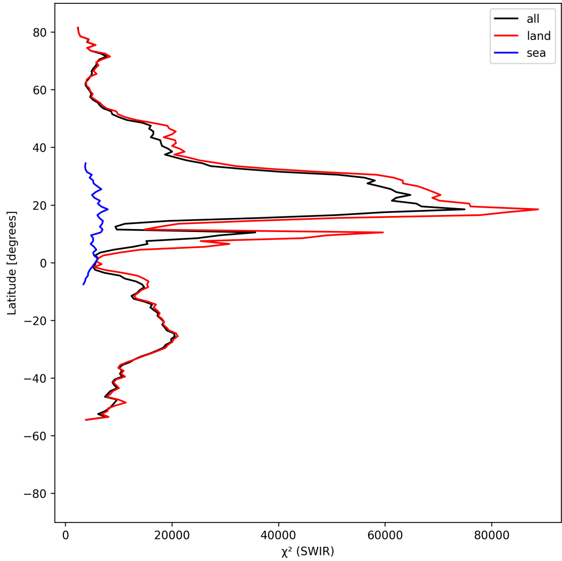
Figure 17: Zonal average of “ \chi^2 (SWIR)” for 2024-09-03 to 2024-09-05.
