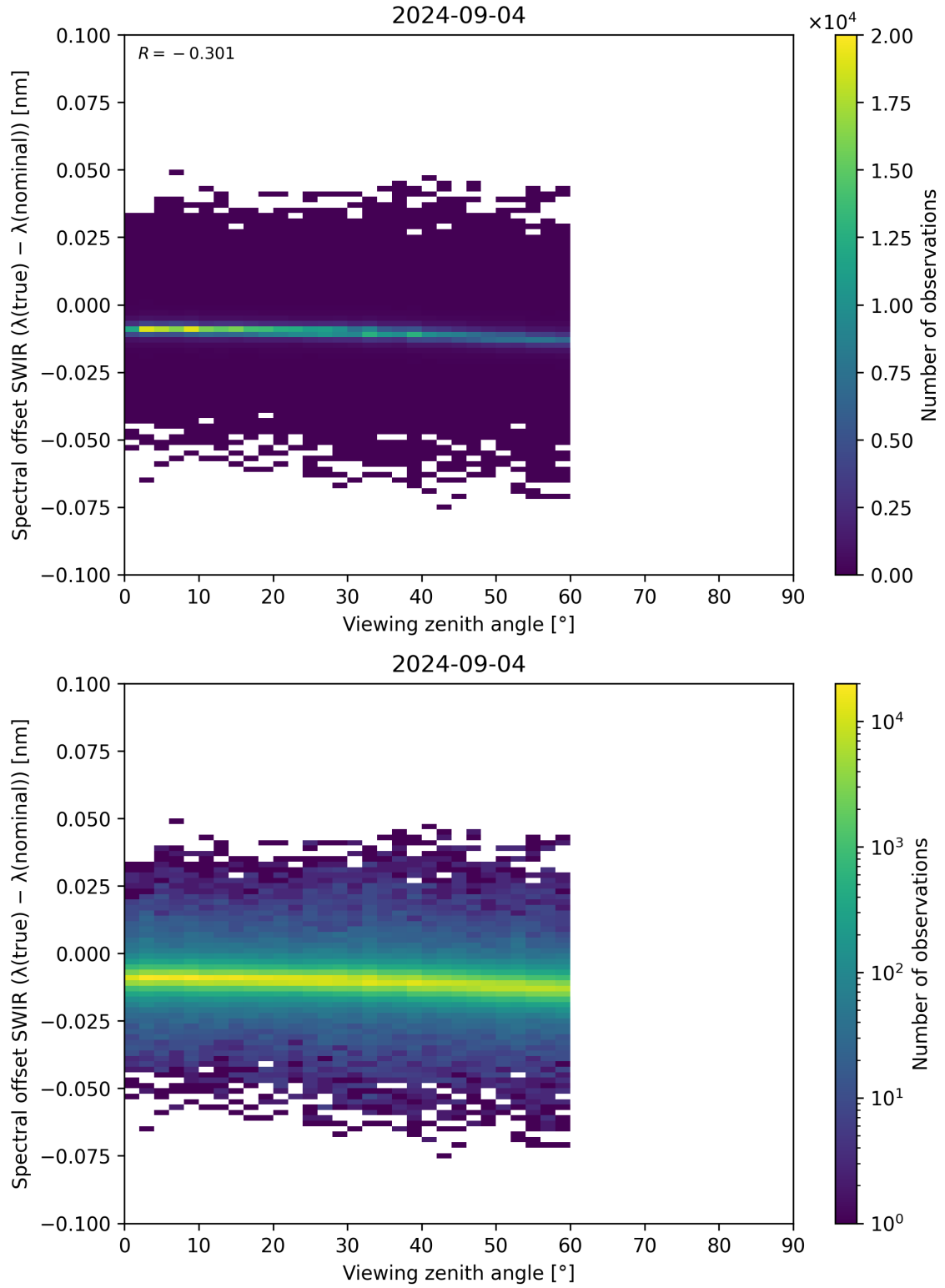
Figure 116: Scatter density plot of “Viewing zenith angle” against “Spectral offset SWIR ( \lambda_{\text{true}} - \lambda_{\text{nominal}} )” for 2024-09-03 to 2024-09-05.
