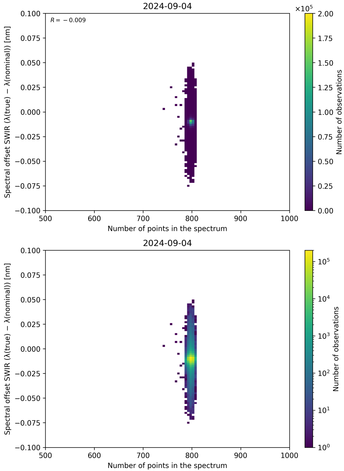
Figure 93: Scatter density plot of “Number of points in the spectrum” against “Spectral offset SWIR ( \lambda_{\text{true}} - \lambda_{\text{nominal}} )” for 2024-09-03 to 2024-09-05.
