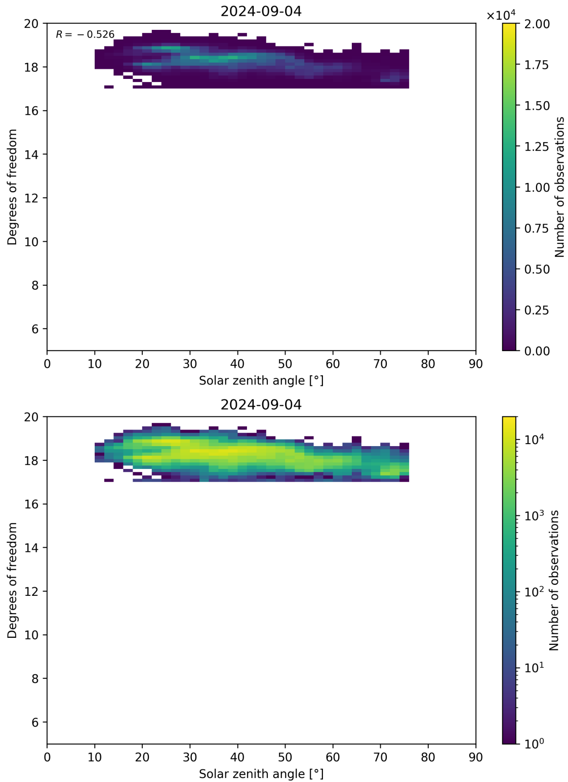
Figure 96: Scatter density plot of “Solar zenith angle” against “Degrees of freedom” for 2024-09-03 to 2024-09-05.
