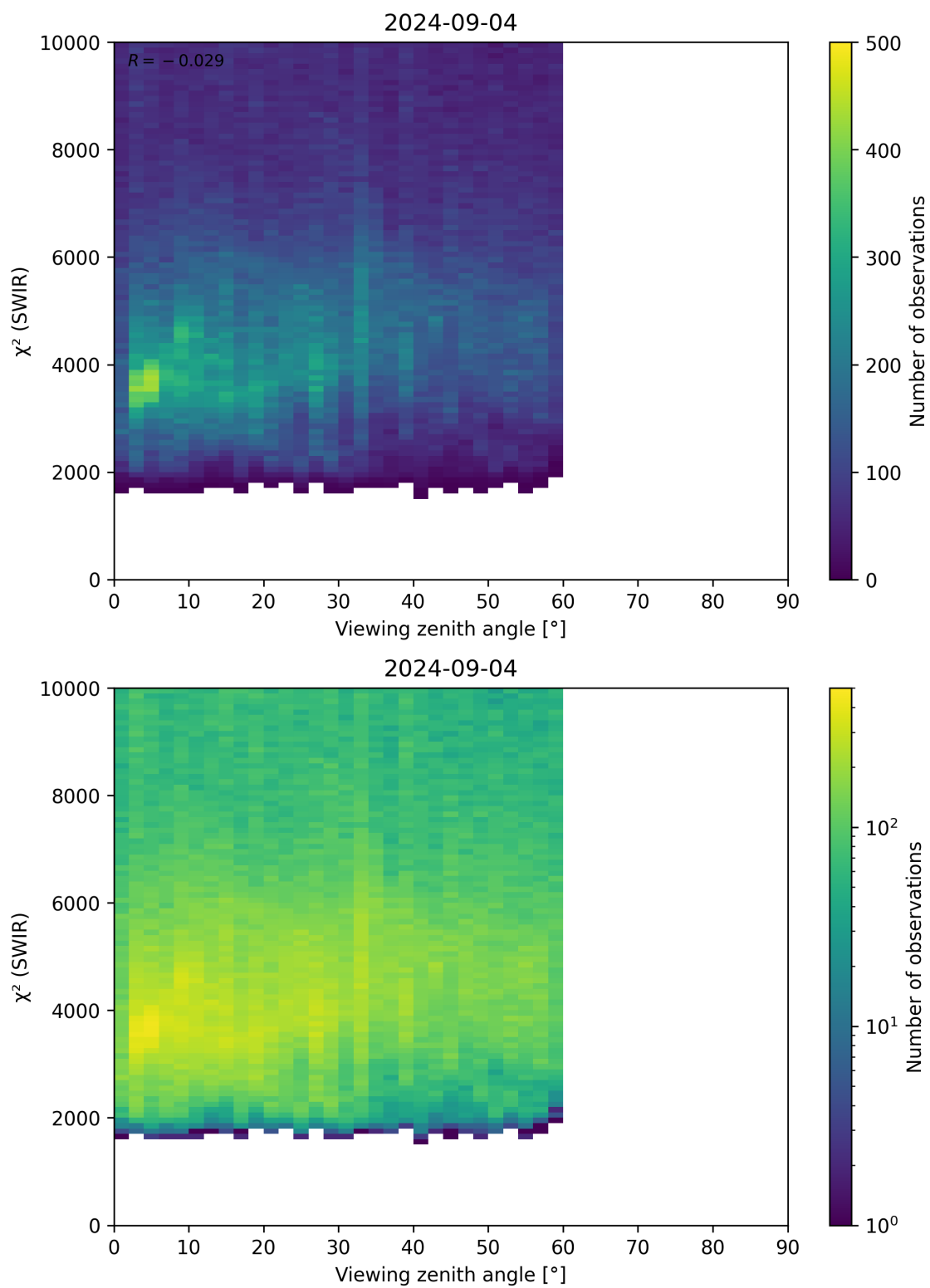
Figure 106: Scatter density plot of “Viewing zenith angle” against “ \chi^2 (SWIR)” for 2024-09-03 to 2024-09-05.
