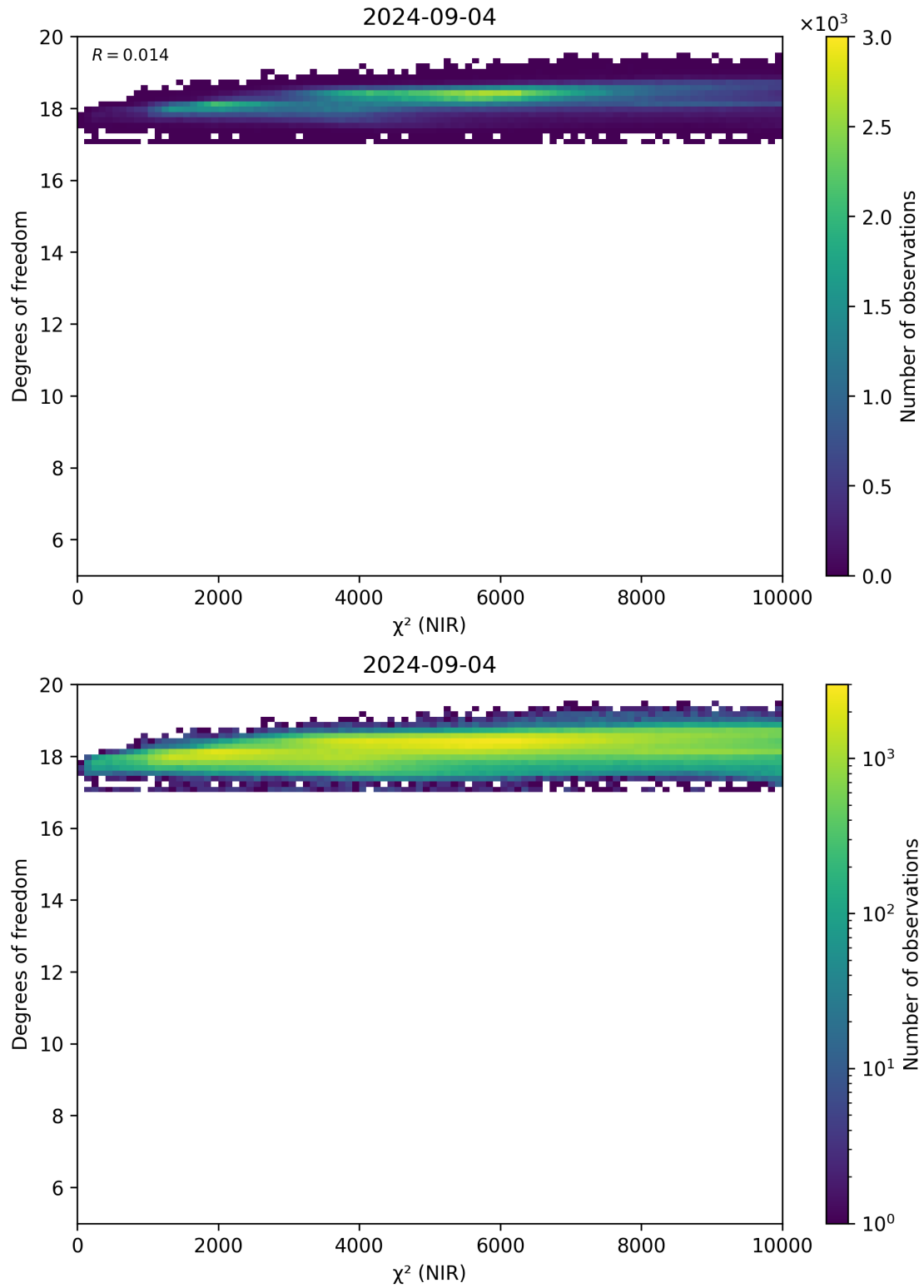
Figure 44: Scatter density plot of “ \chi^2 (NIR)” against “Degrees of freedom” for 2024-09-03 to 2024-09-05.
