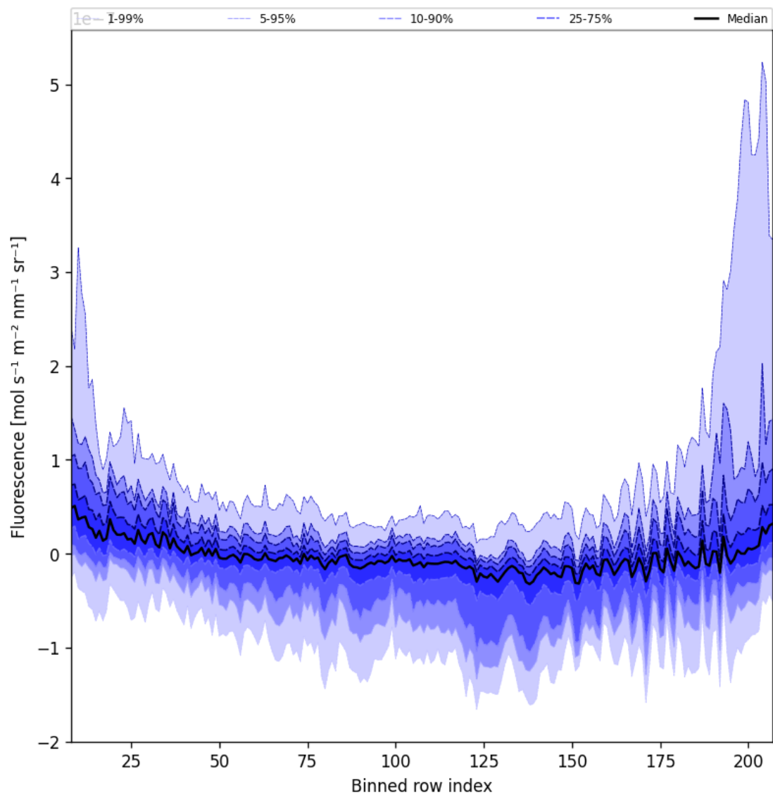
Figure 43: Along track statistics of “Fluorescence” for 2024-09-03 to 2024-09-05
