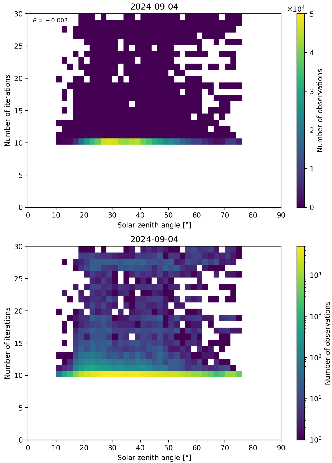
Figure 102: Scatter density plot of “Solar zenith angle” against “Number of iterations” for 2024-09-03 to 2024-09-05.
