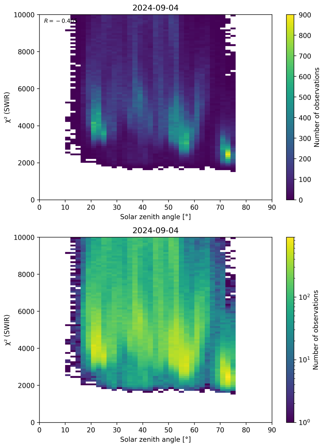
Figure 95: Scatter density plot of “Solar zenith angle” against “ \chi^2 (SWIR)” for 2024-09-03 to 2024-09-05.
