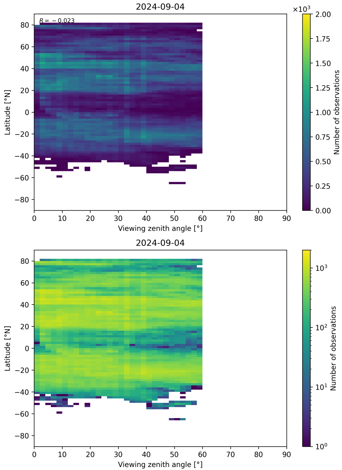
Figure 109: Scatter density plot of “Viewing zenith angle” against “Latitude” for 2024-09-03 to 2024-09-05.
