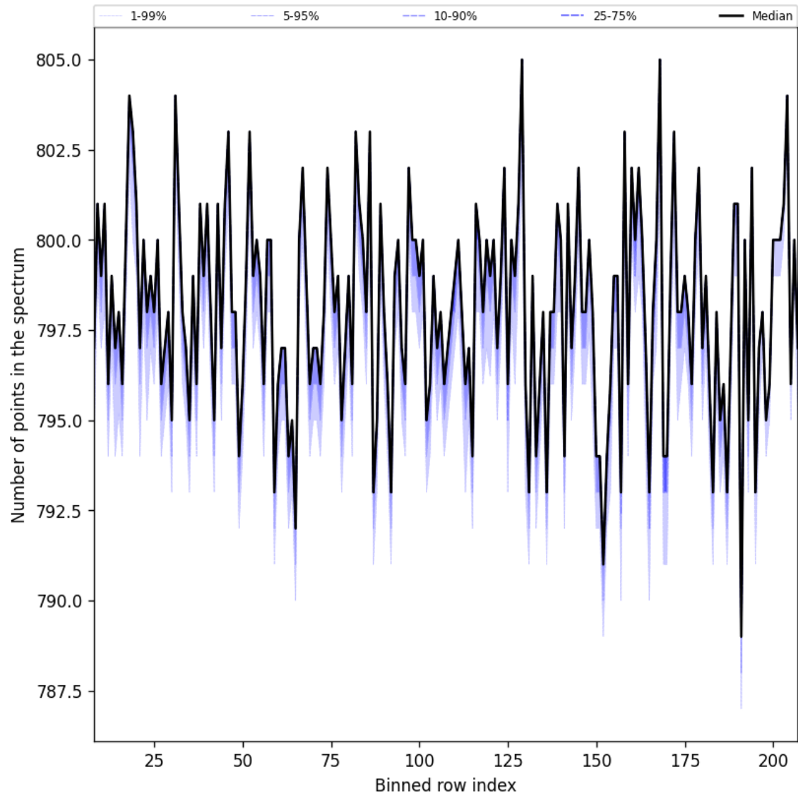
Figure 37: Along track statistics of “Number of points in the spectrum” for 2024-09-03 to 2024-09-05
