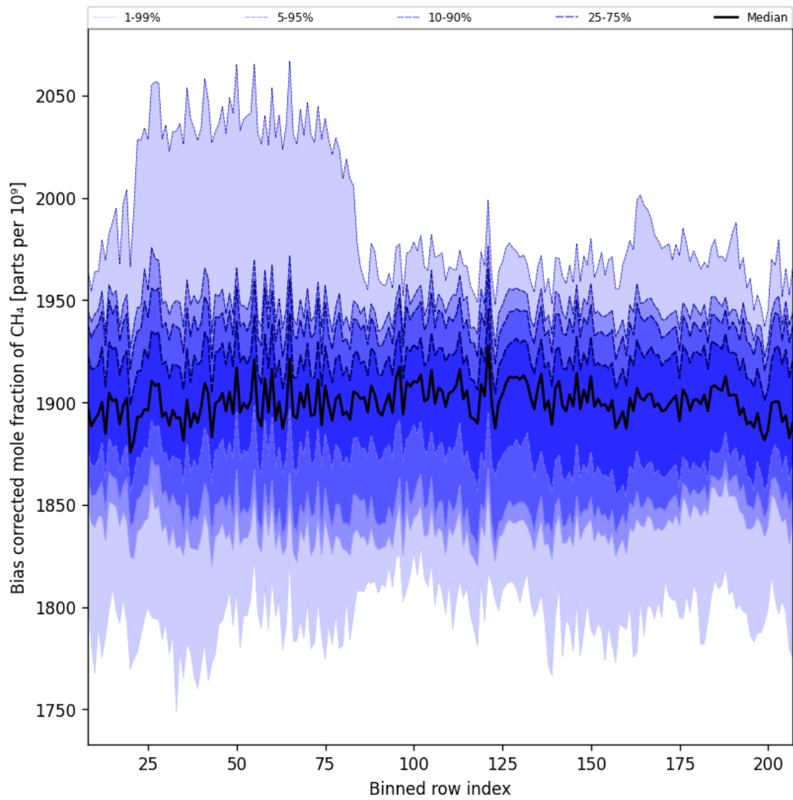
Figure 36: Along track statistics of “Bias corrected mole fraction of CH 4 ” for 2024-09-03 to 2024-09-05
