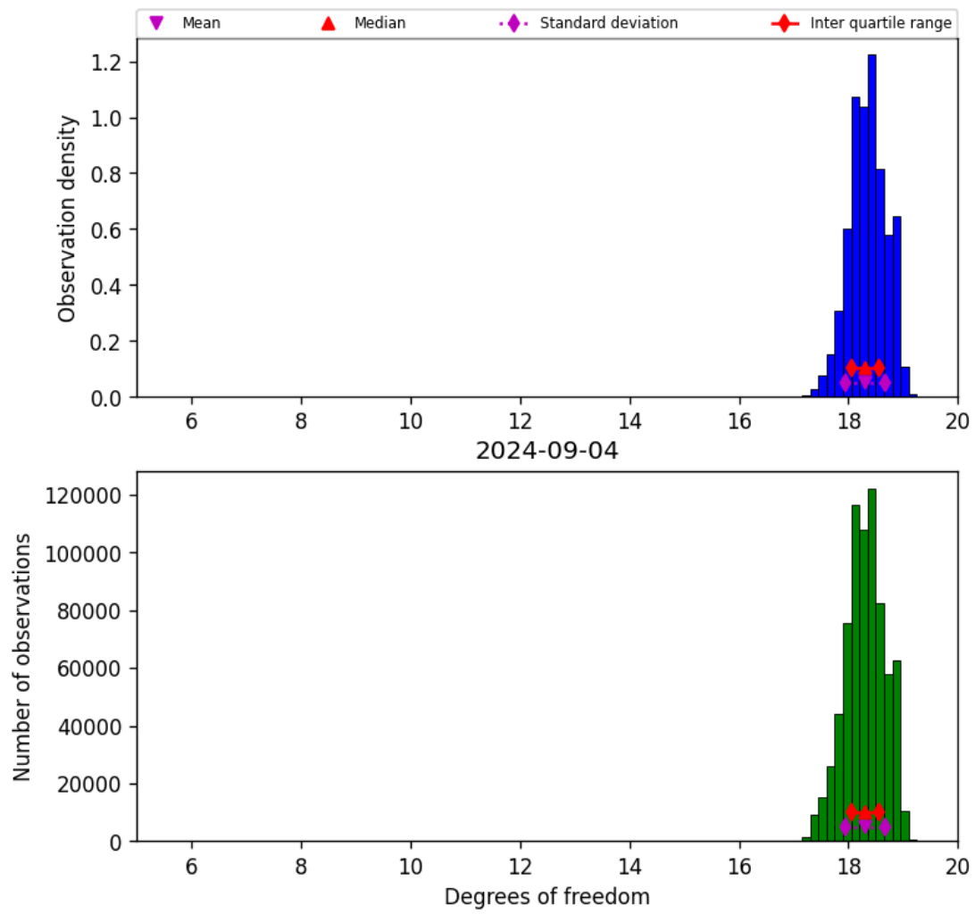
Figure 30: Histogram of “Degrees of freedom” for 2024-09-03 to 2024-09-05
