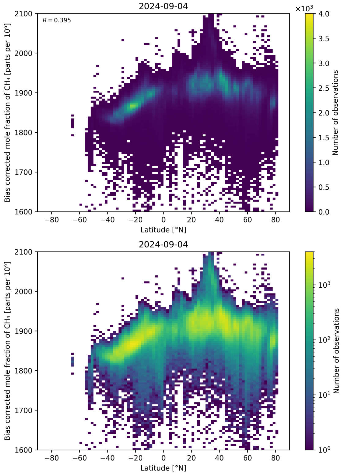
Figure 58: Scatter density plot of “Latitude” against “Bias corrected mole fraction of \text{CH}_4 ” for 2024-09-03 to 2024-09-05.
