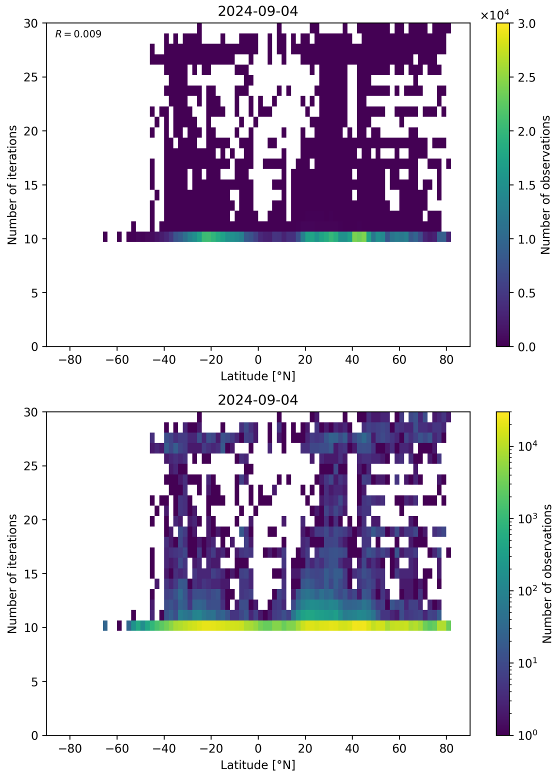
Figure 60: Scatter density plot of “Latitude” against “Number of iterations” for 2024-09-03 to 2024-09-05.
