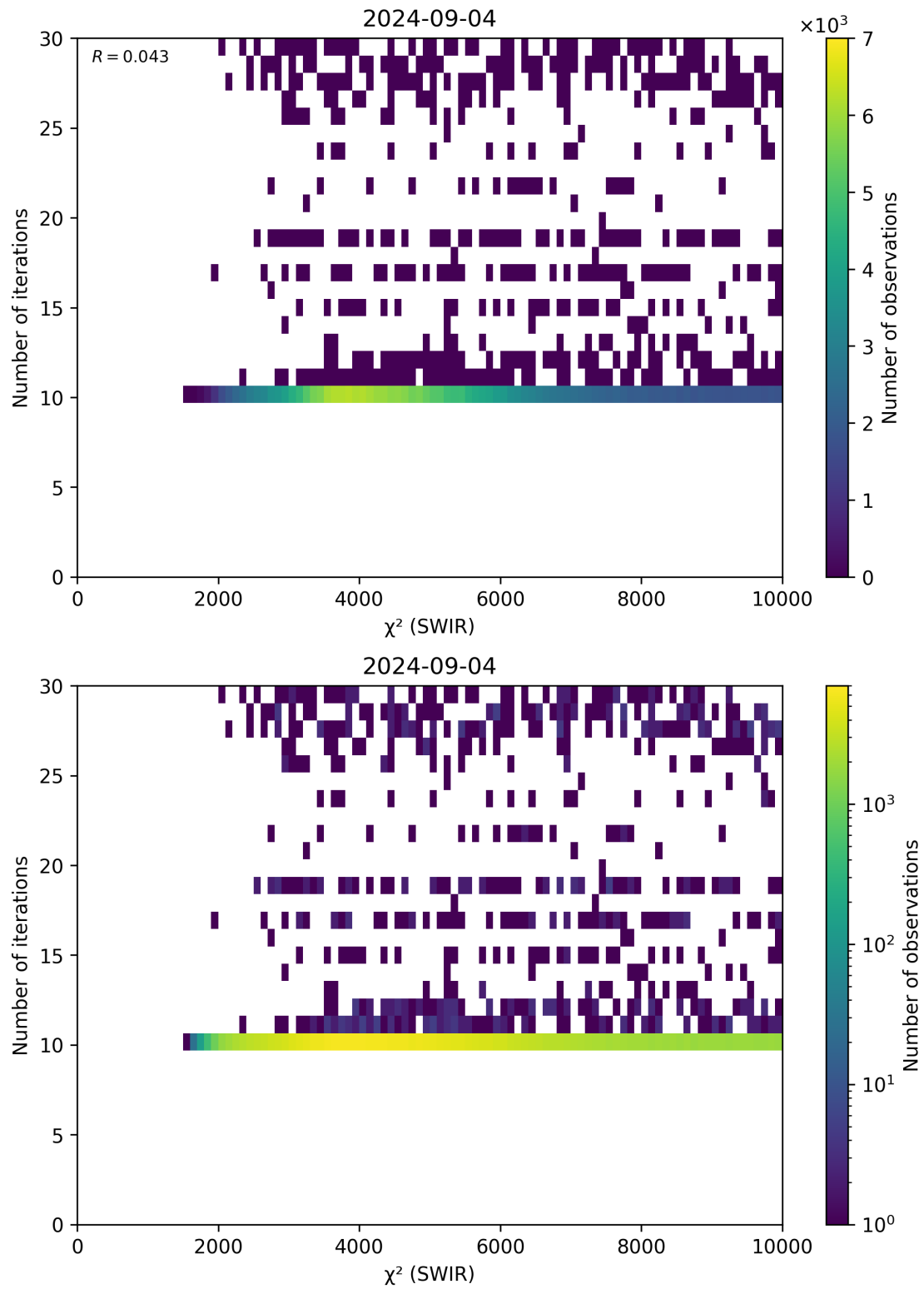
Figure 50: Scatter density plot of “ \chi^2 (SWIR)” against “Number of iterations” for 2024-09-03 to 2024-09-05.
