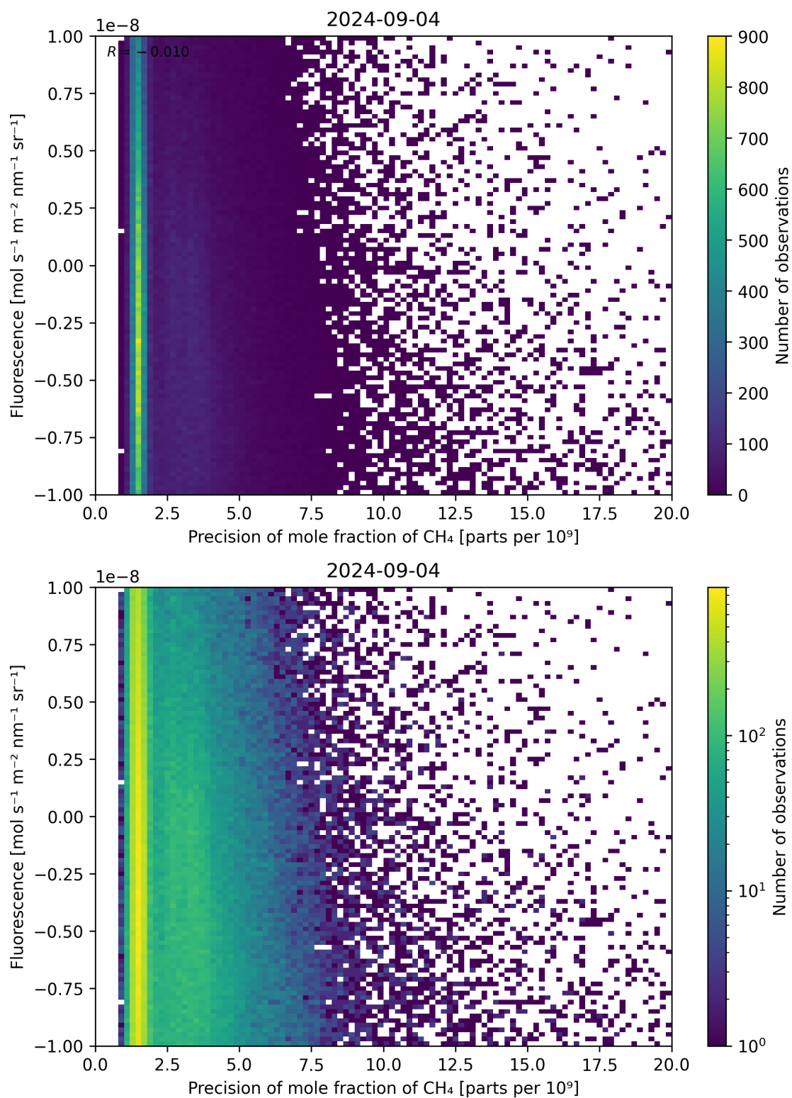
Figure 81: Scatter density plot of “Precision of mole fraction of \text{CH}_4 ” against “Fluorescence” for 2024-09-03 to 2024-09-05.
