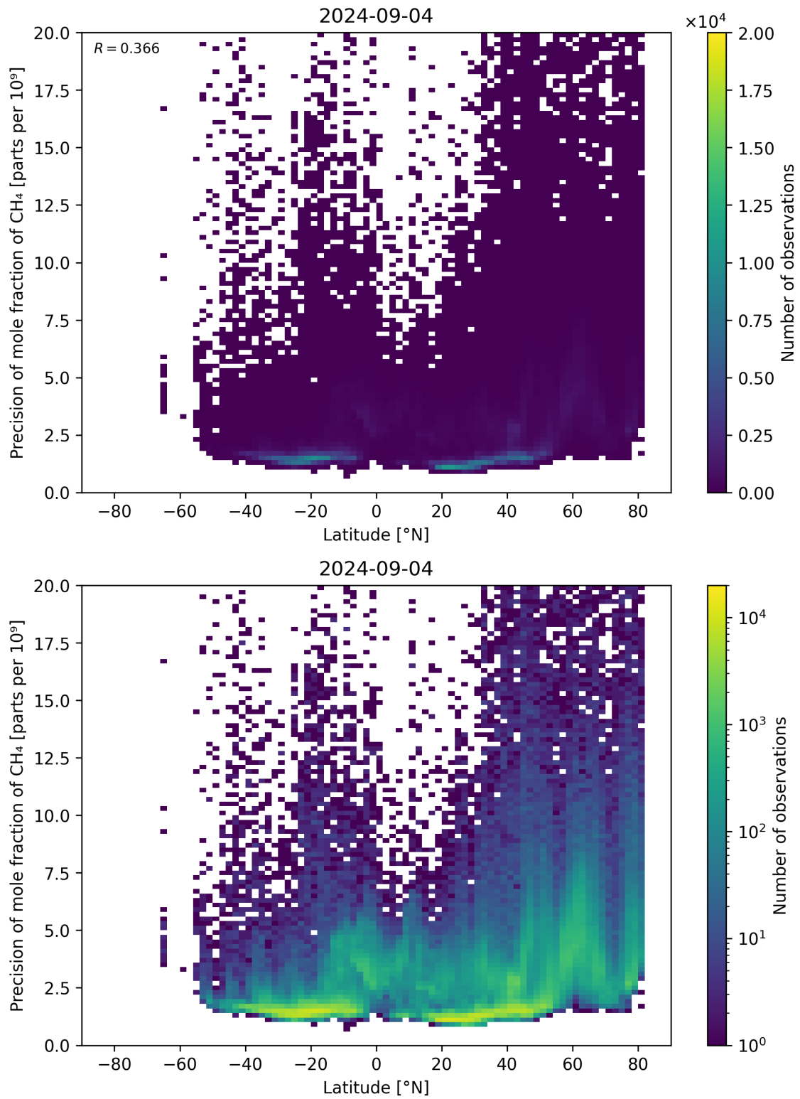
Figure 59: Scatter density plot of “Latitude” against “Precision of mole fraction of \text{CH}_4 ” for 2024-09-03 to 2024-09-05.
