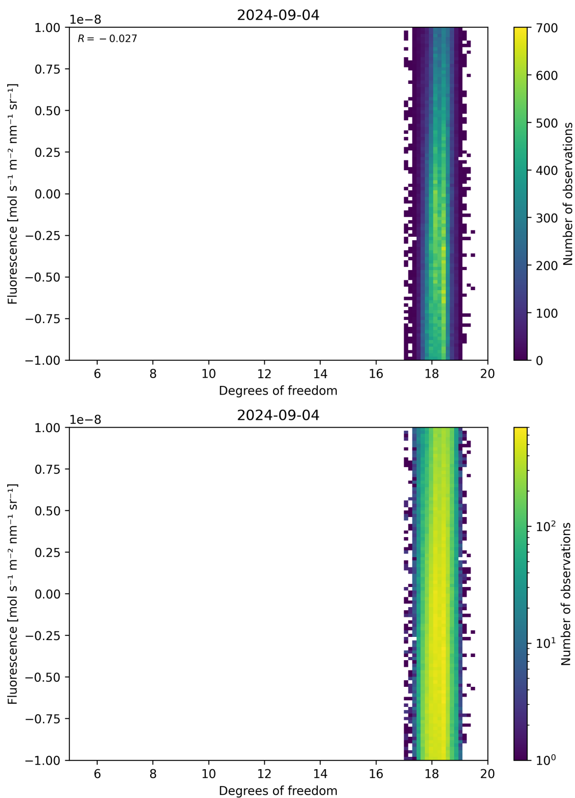
Figure 51: Scatter density plot of “Degrees of freedom” against “Fluorescence” for 2024-09-03 to 2024-09-05.
