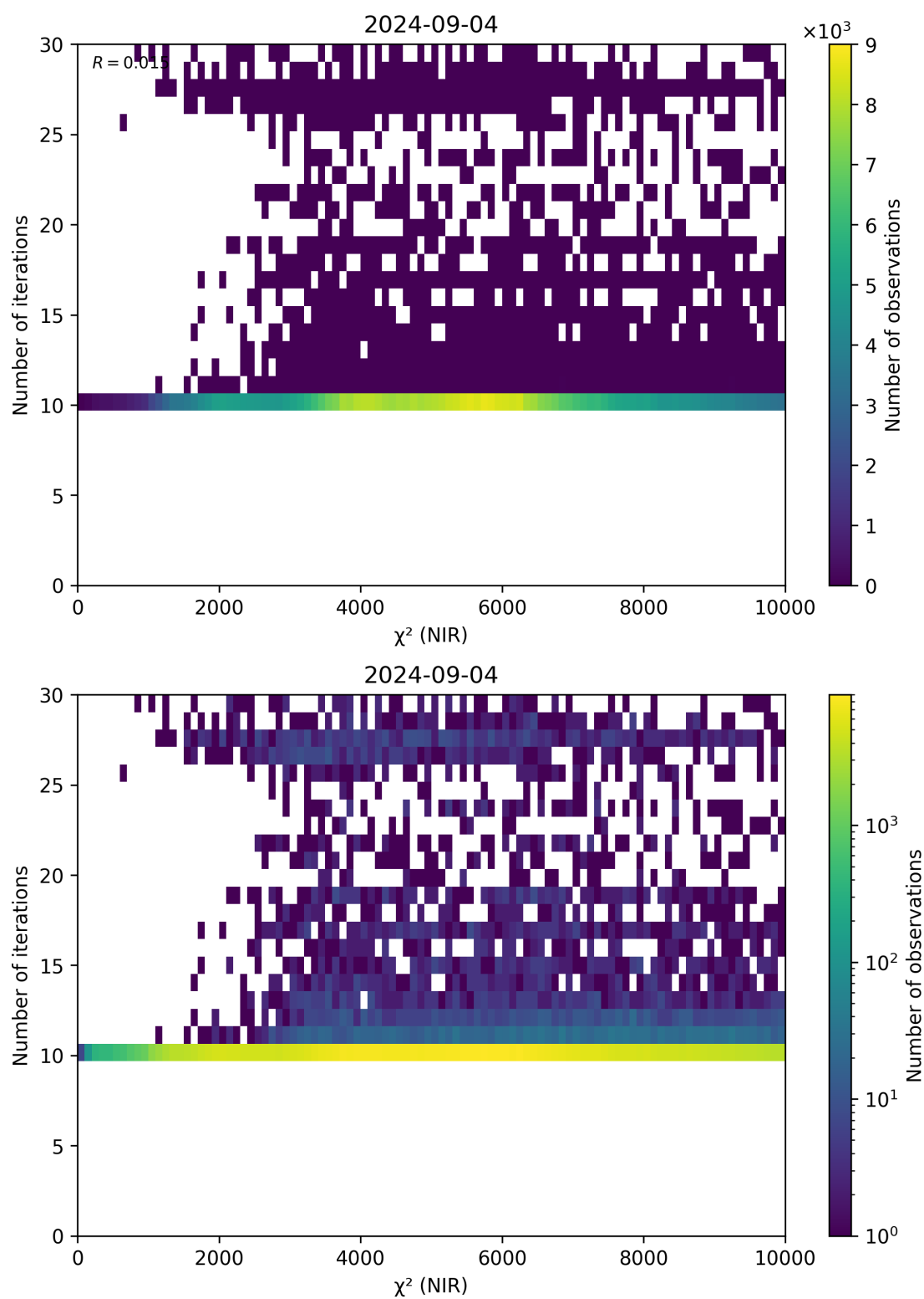
Figure 46: Scatter density plot of “ \chi^2 (NIR)” against “Number of iterations” for 2024-09-03 to 2024-09-05.
