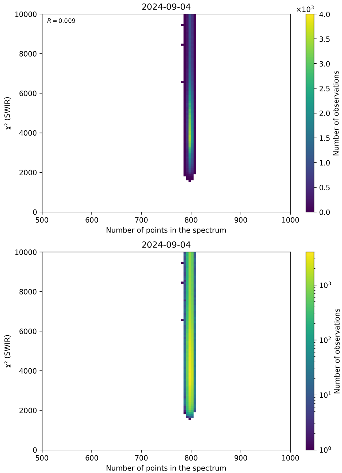
Figure 89: Scatter density plot of “Number of points in the spectrum” against “ \chi^2 (SWIR)” for 2024-09-03 to 2024-09-05.
