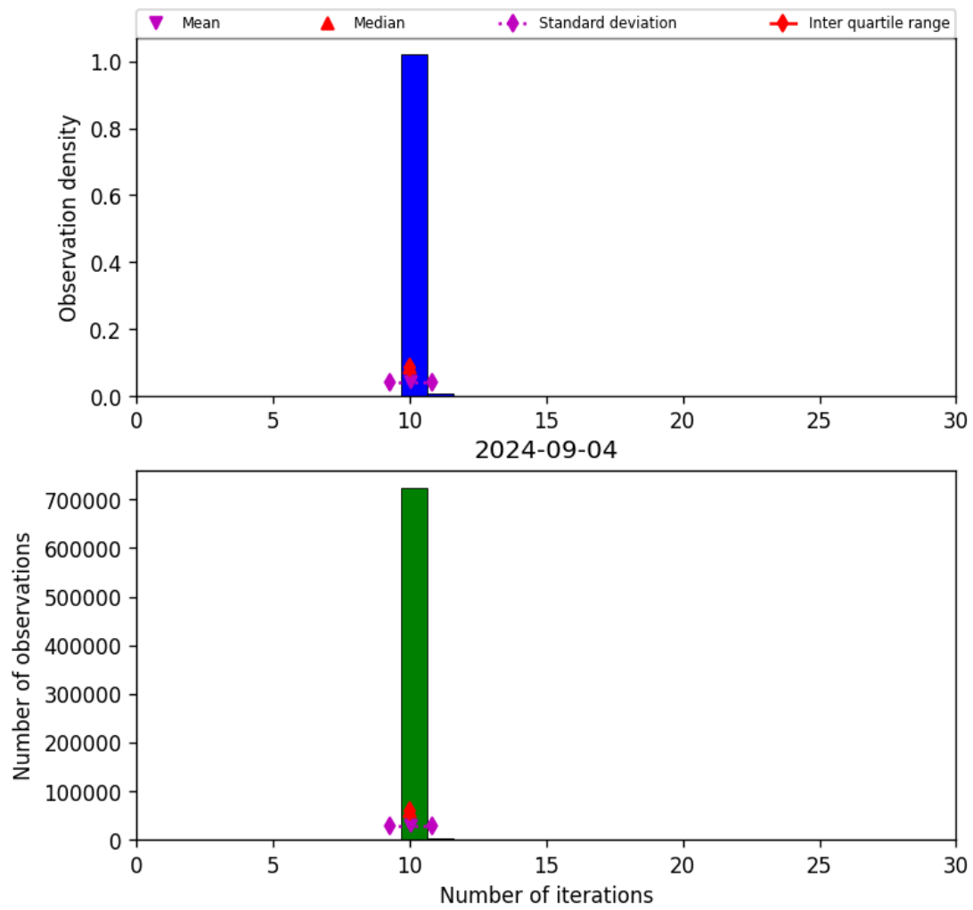
Figure 31: Histogram of “Number of iterations” for 2024-09-03 to 2024-09-05
