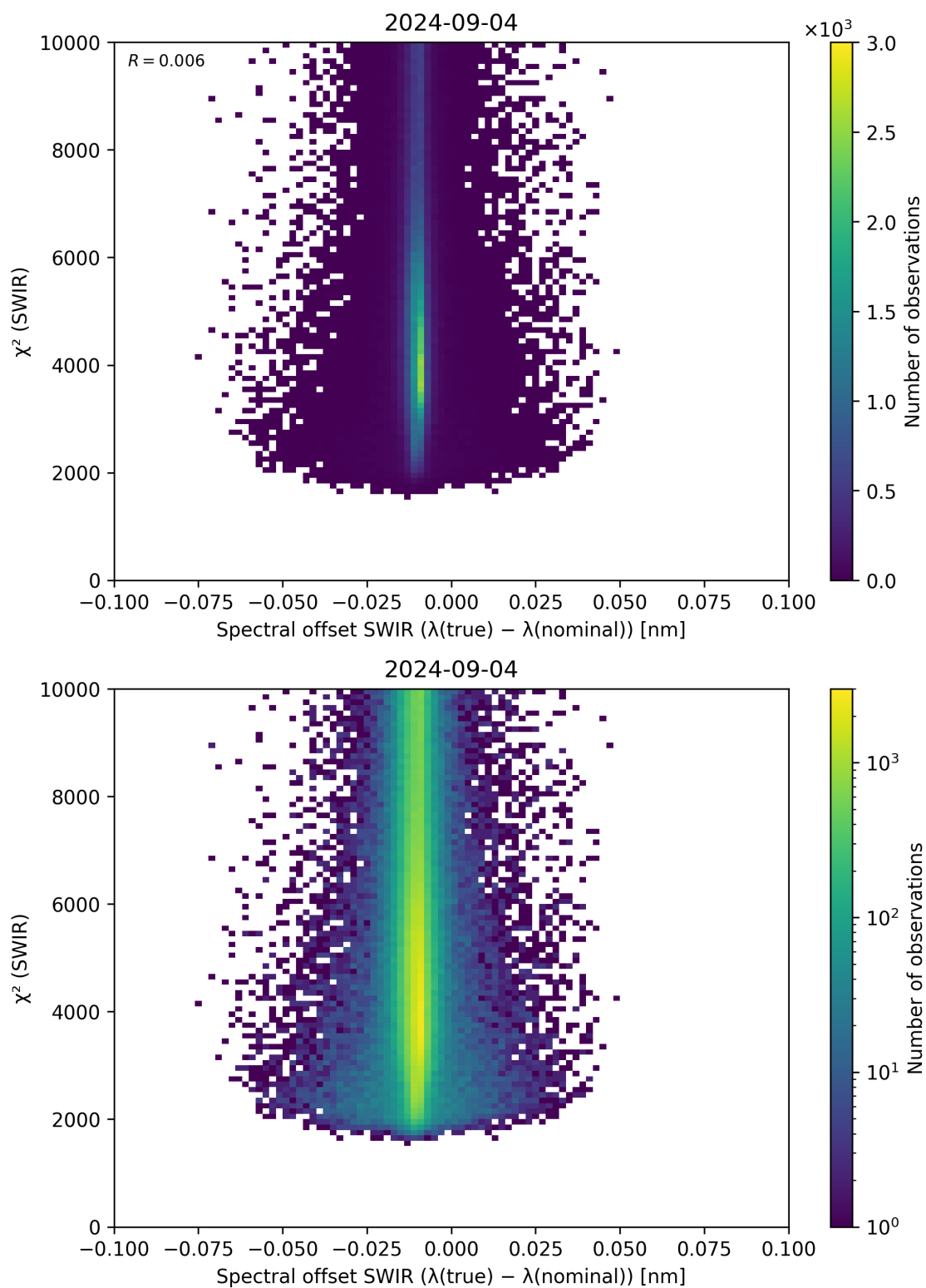
Figure 118: Scatter density plot of “Spectral offset SWIR ( \lambda_{\text{true}} - \lambda_{\text{nominal}} )” against “ \chi^2 (SWIR)” for 2024-09-03 to 2024-09-05.
