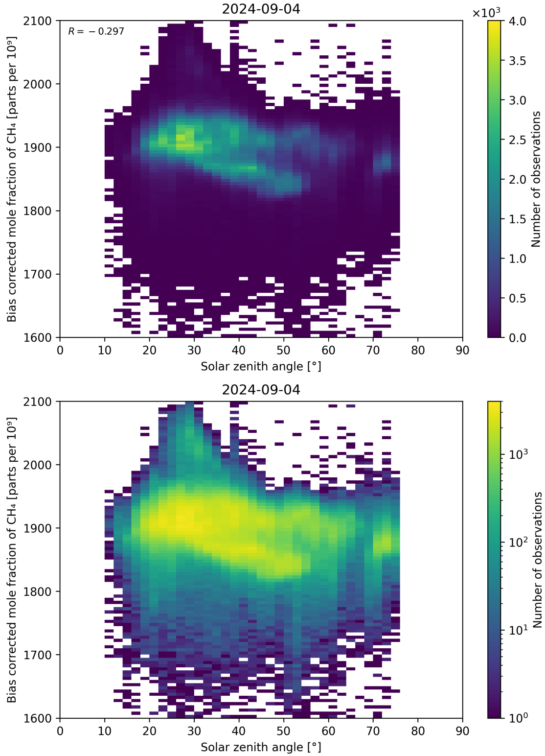
Figure 100: Scatter density plot of “Solar zenith angle” against “Bias corrected mole fraction of \text{CH}_4 ” for 2024-09-03 to 2024-09-05.
