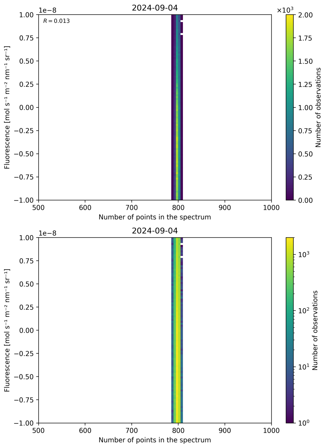
Figure 91: Scatter density plot of “Number of points in the spectrum” against “Fluorescence” for 2024-09-03 to 2024-09-05.
