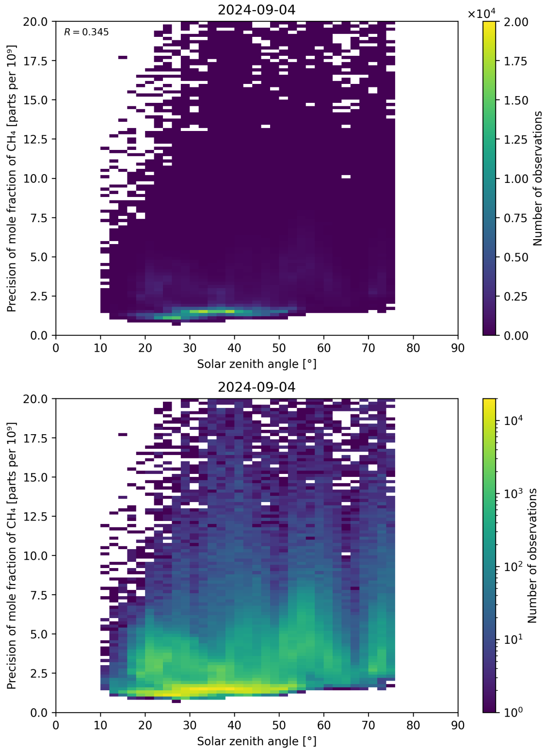
Figure 101: Scatter density plot of “Solar zenith angle” against “Precision of mole fraction of \text{CH}_4 ” for 2024-09-03 to 2024-09-05.
