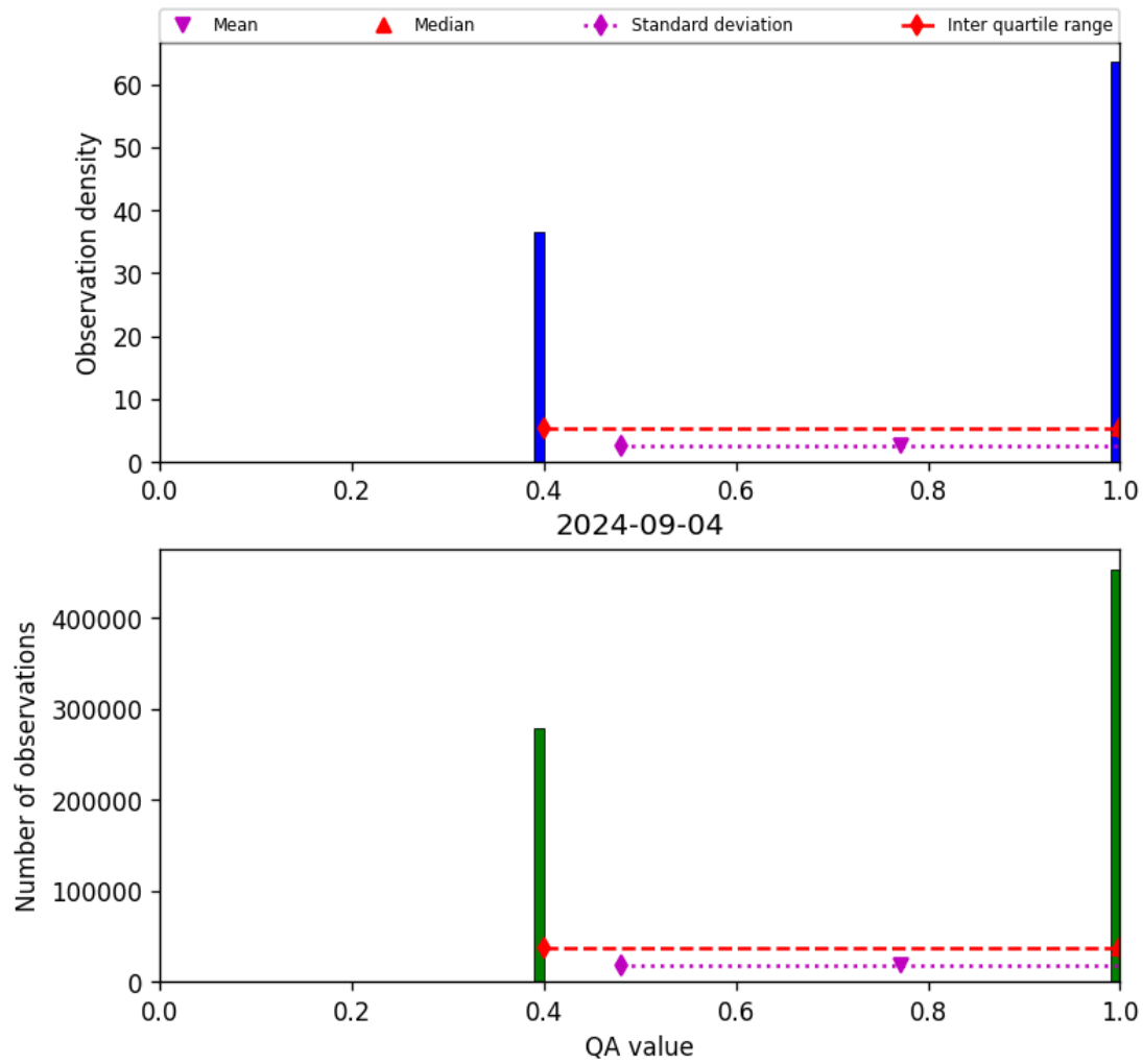
Figure 22: Histogram of “QA value” for 2024-09-03 to 2024-09-05
