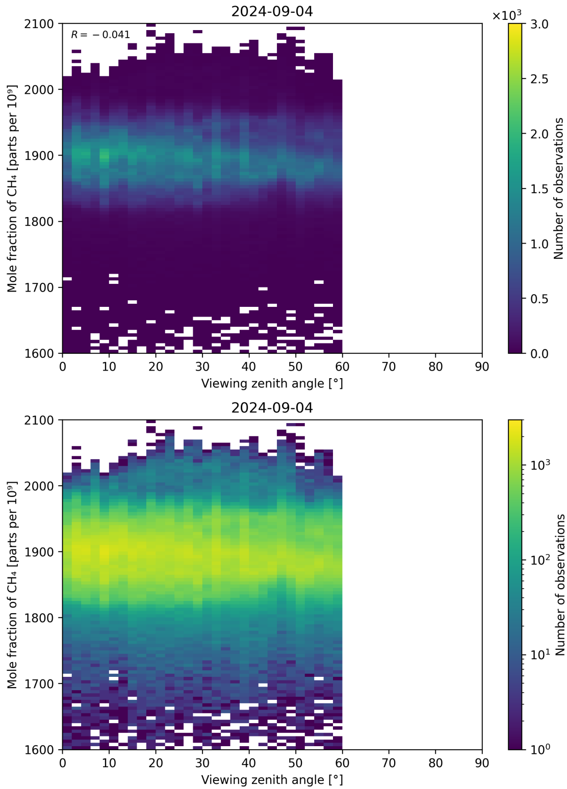
Figure 110: Scatter density plot of “Viewing zenith angle” against “Mole fraction of CH 4 ” for 2024-09-03 to 2024-09-05.
