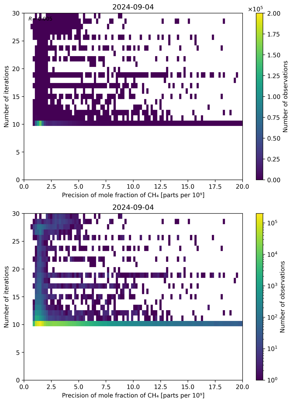
Figure 83: Scatter density plot of “Precision of mole fraction of CH 4 ” against “Number of iterations” for 2024-09-03 to 2024-09-05.
