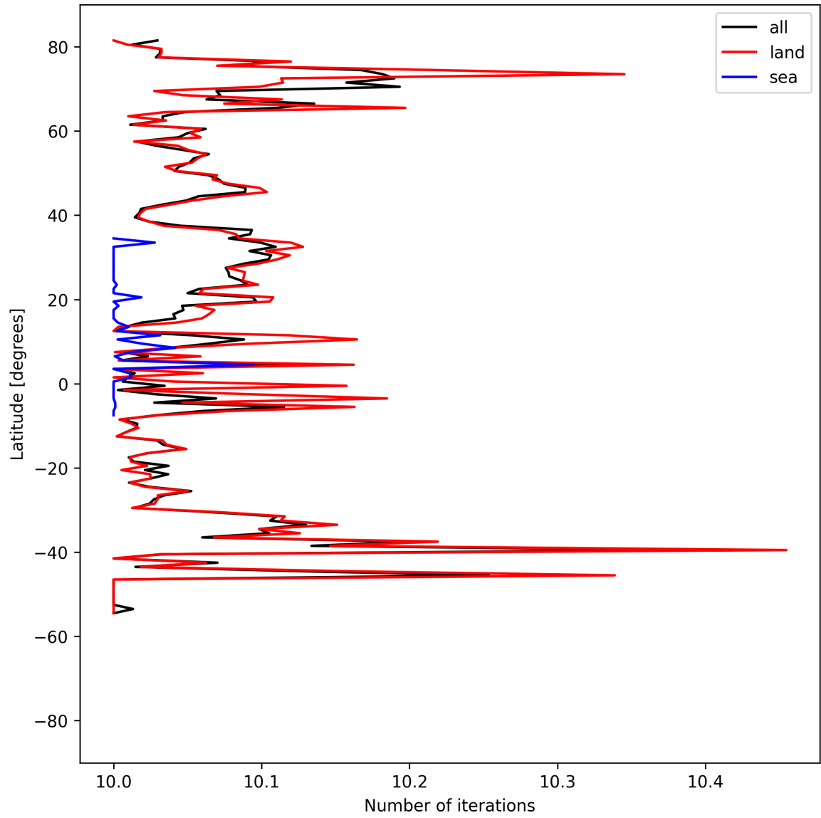
Figure 20: Zonal average of “Number of iterations” for 2024-09-03 to 2024-09-05.
