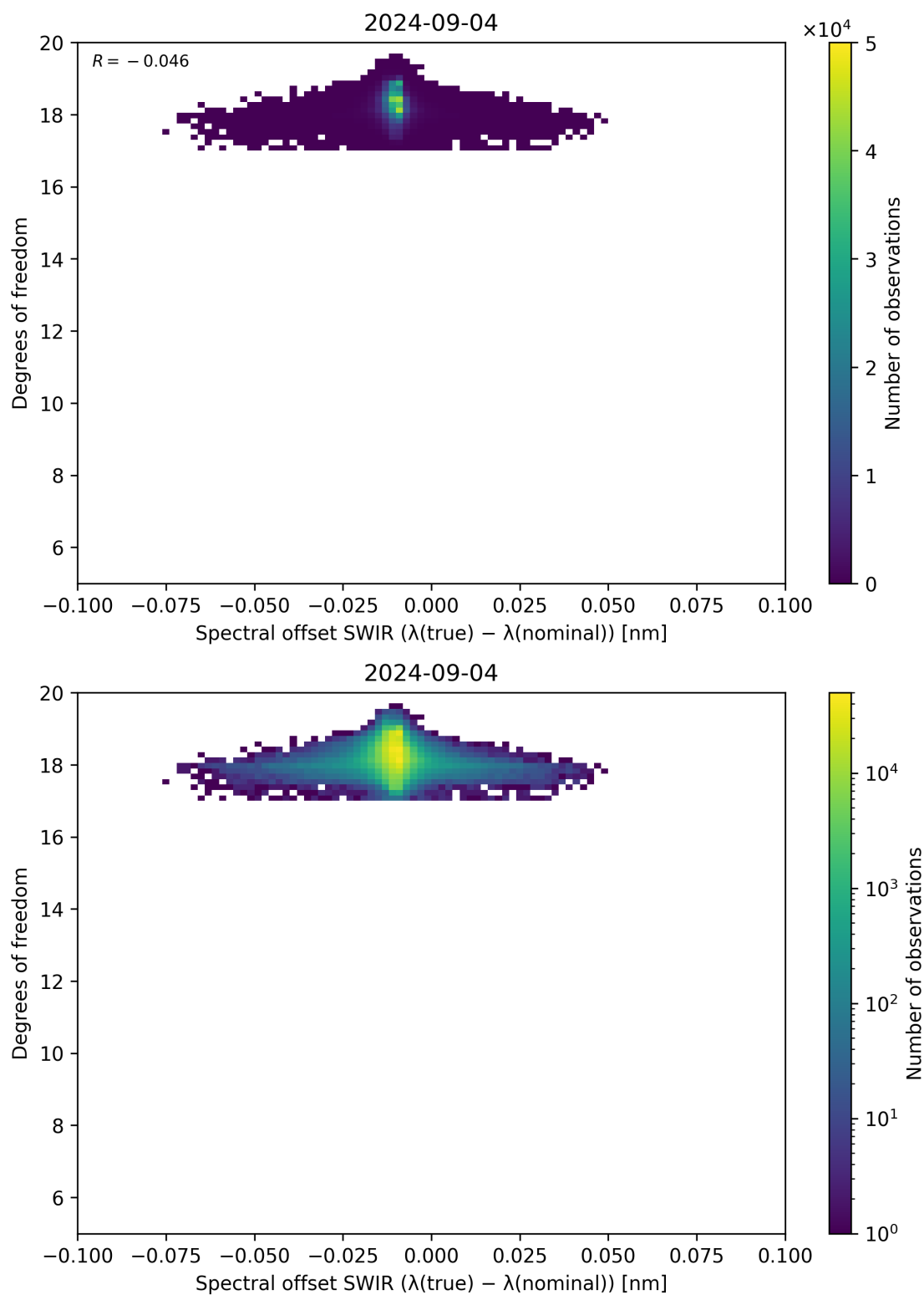
Figure 119: Scatter density plot of “Spectral offset SWIR ( \lambda_{\text{true}} - \lambda_{\text{nominal}} )” against “Degrees of freedom” for 2024-09-03 to 2024-09-05.
