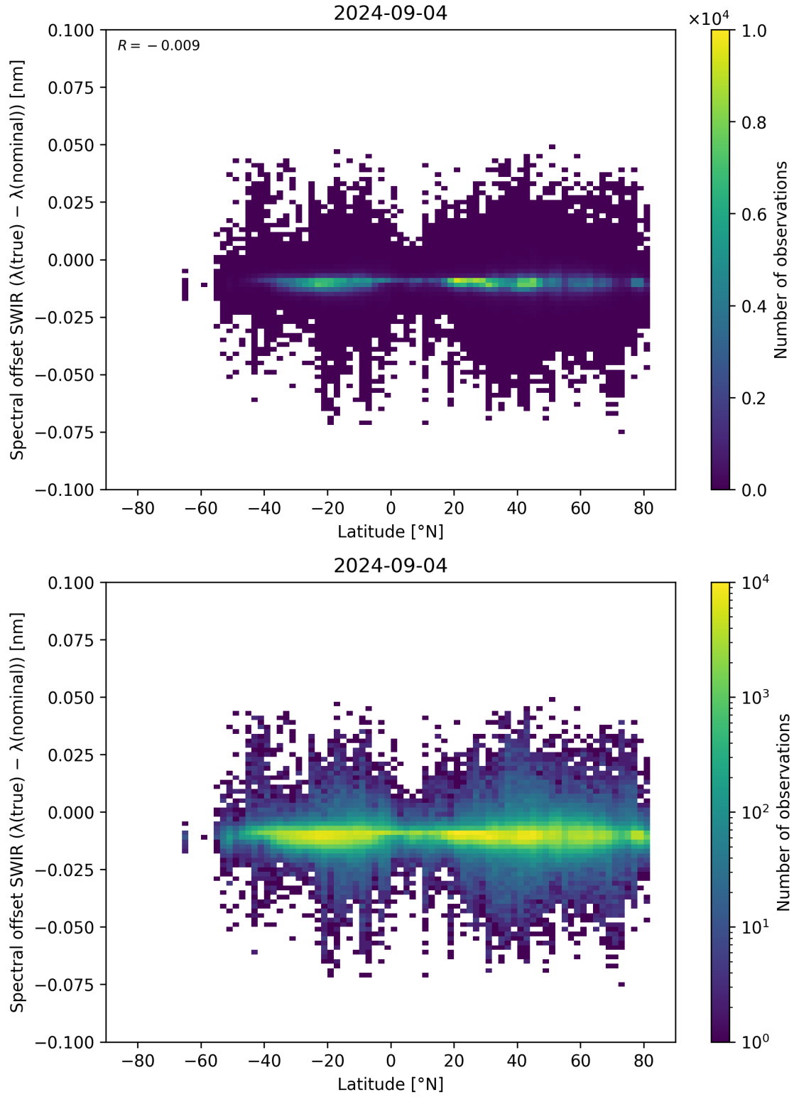
Figure 62: Scatter density plot of “Latitude” against “Spectral offset SWIR ( \lambda_{\text{true}} - \lambda_{\text{nominal}} )” for 2024-09-03 to 2024-09-05.
