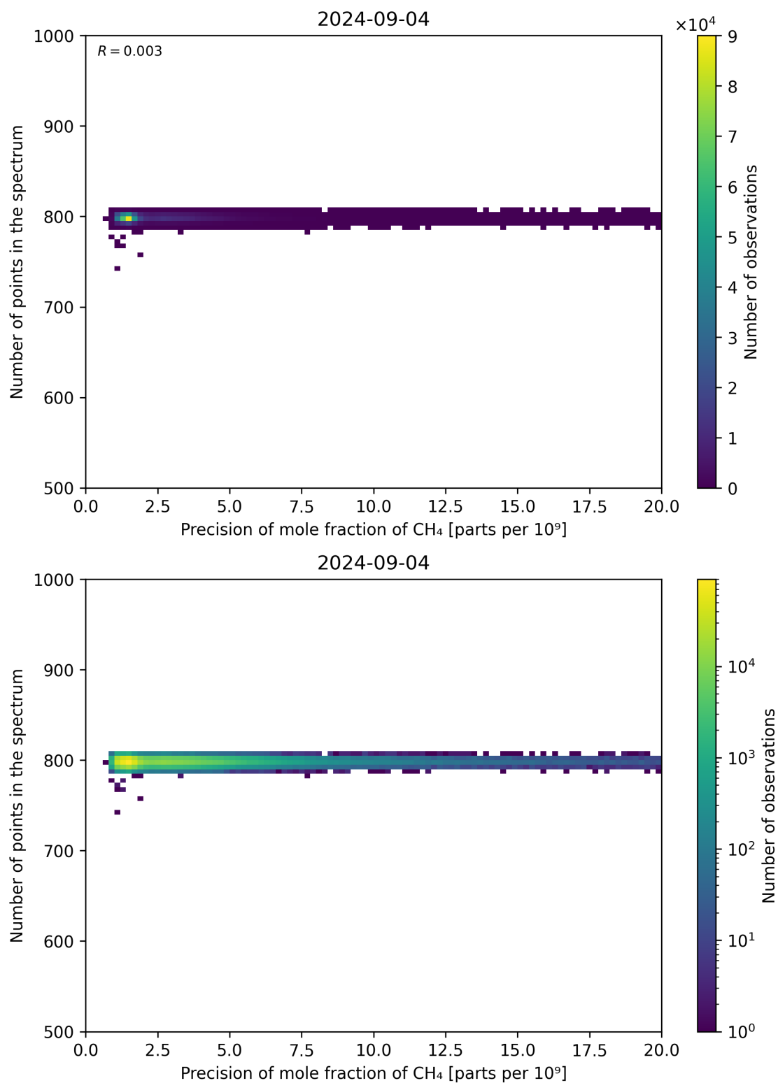
Figure 84: Scatter density plot of “Precision of mole fraction of CH 4 ” against “Number of points in the spectrum” for 2024-09-03 to 2024-09-05.
