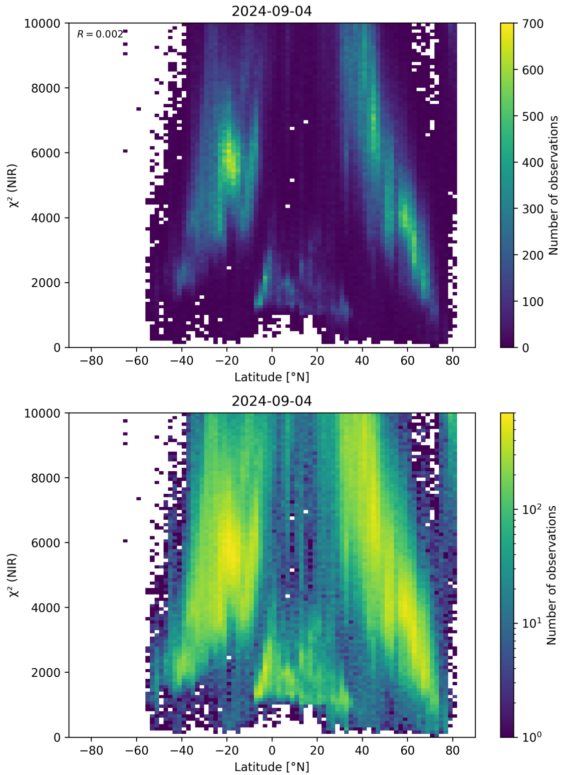
Figure 53: Scatter density plot of “Latitude” against “ \chi^2 (NIR)” for 2024-09-03 to 2024-09-05.
