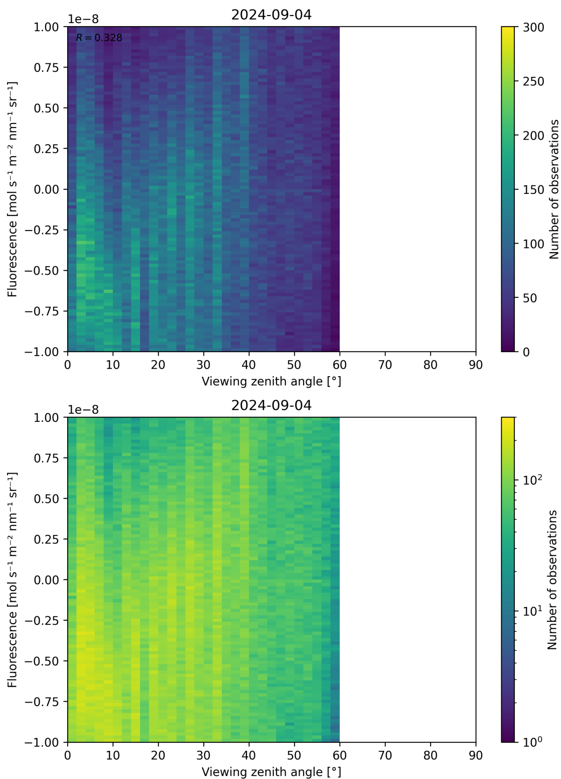
Figure 108: Scatter density plot of “Viewing zenith angle” against “Fluorescence” for 2024-09-03 to 2024-09-05.
