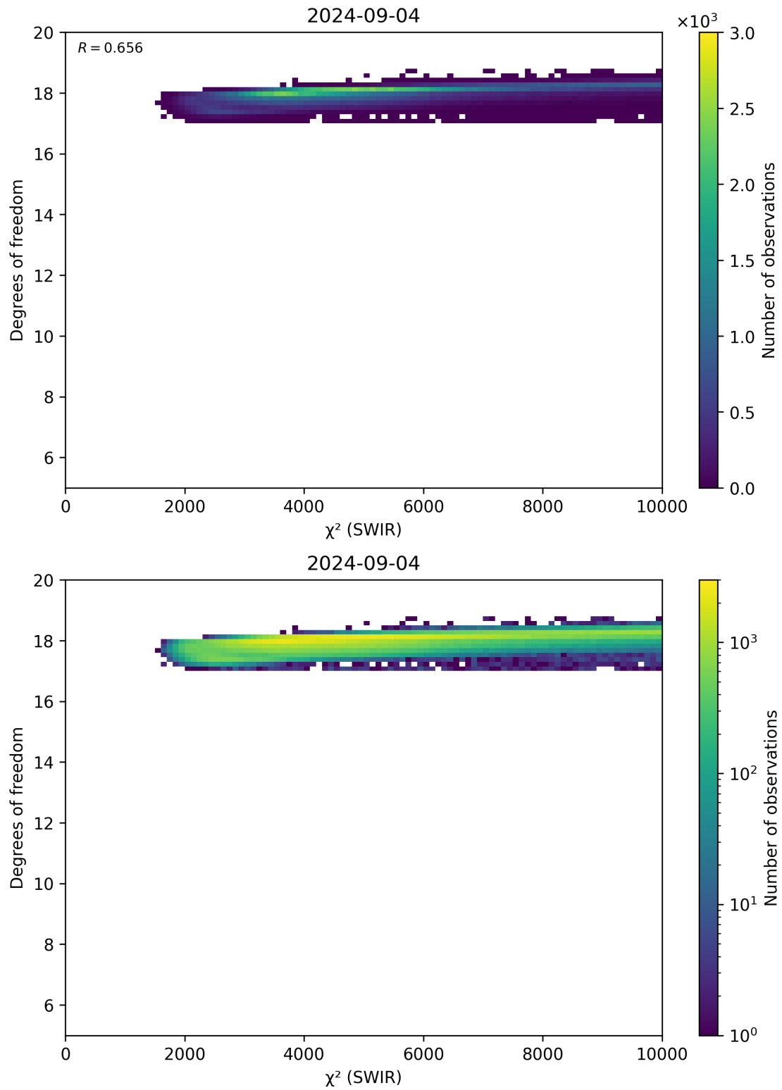
Figure 48: Scatter density plot of “ \chi^2 (SWIR)” against “Degrees of freedom” for 2024-09-03 to 2024-09-05.
