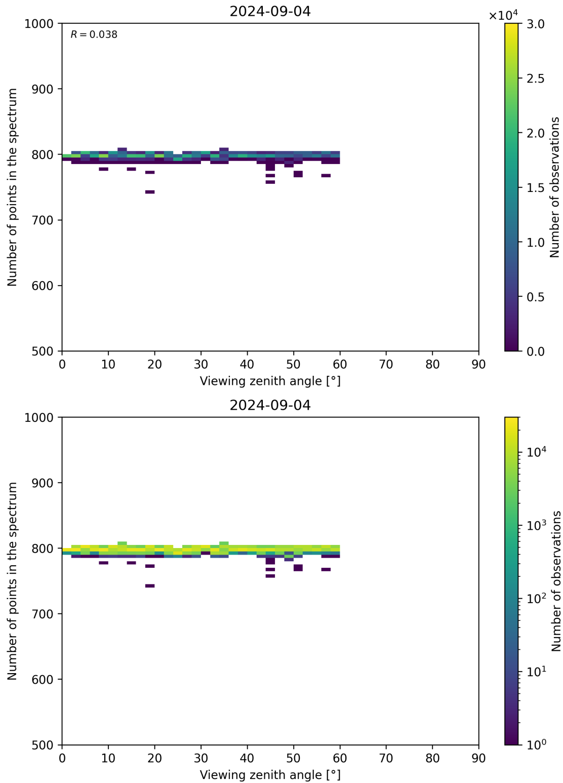
Figure 114: Scatter density plot of “Viewing zenith angle” against “Number of points in the spectrum” for 2024-09-03 to 2024-09-05.
