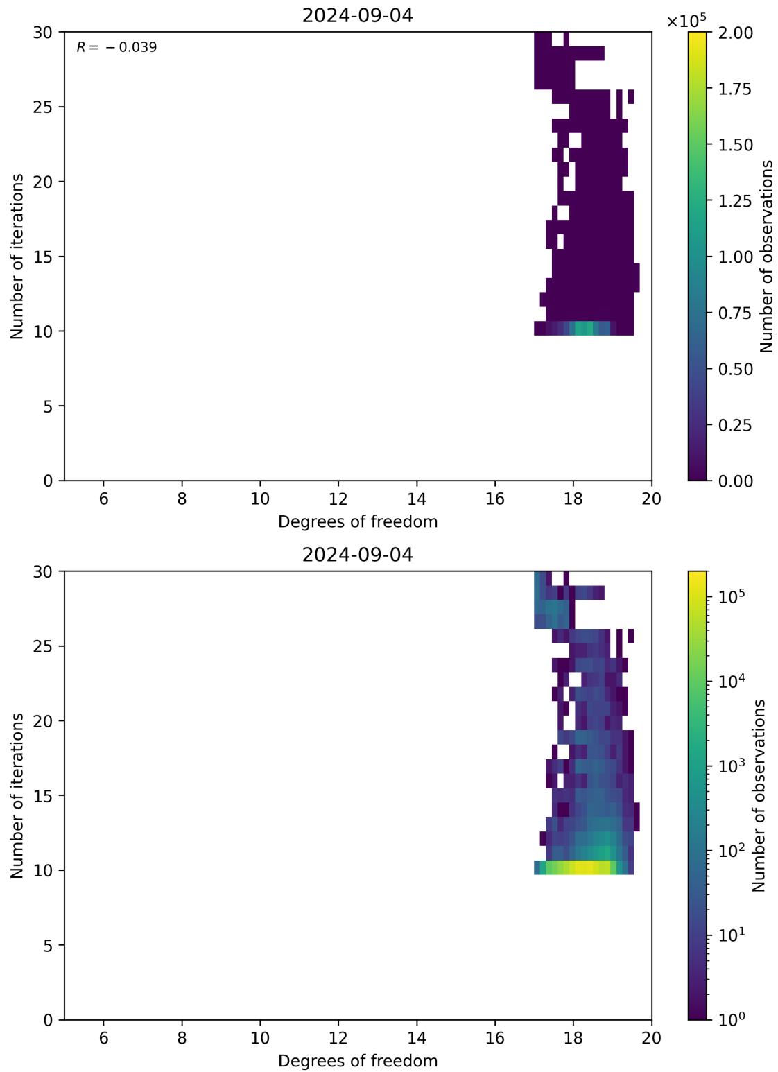
Figure 52: Scatter density plot of “Degrees of freedom” against “Number of iterations” for 2024-09-03 to 2024-09-05.
