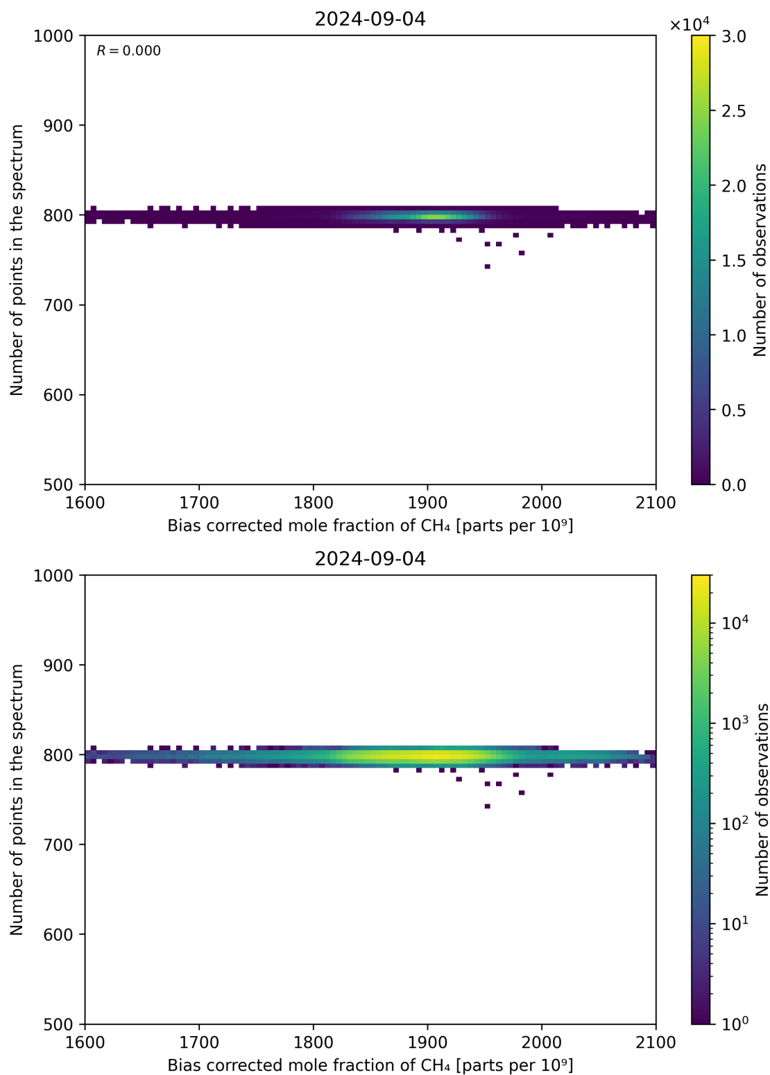
Figure 68: Scatter density plot of “Bias corrected mole fraction of CH 4 ” against “Number of points in the spectrum” for 2024-09-03 to 2024-09-05.
