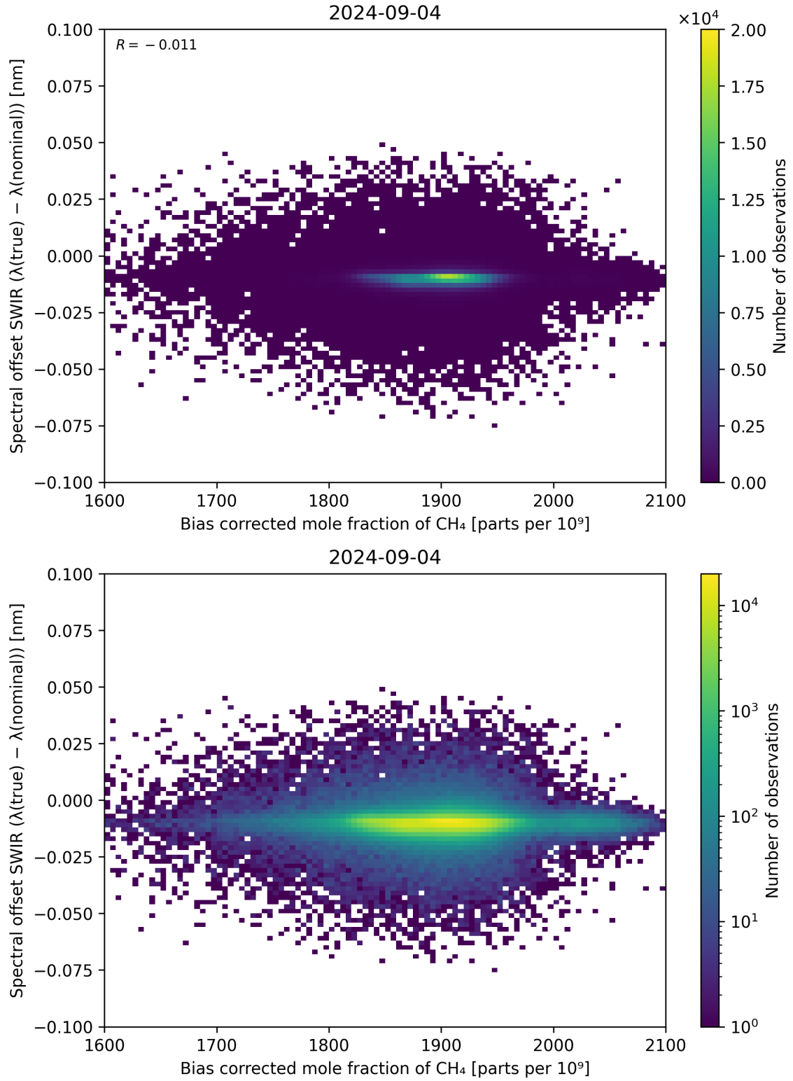
Figure 69: Scatter density plot of “Bias corrected mole fraction of \text{CH}_4 ” against “Spectral offset SWIR ( \lambda_{\text{true}} - \lambda_{\text{nominal}} )” for 2024-09-03 to 2024-09-05.
