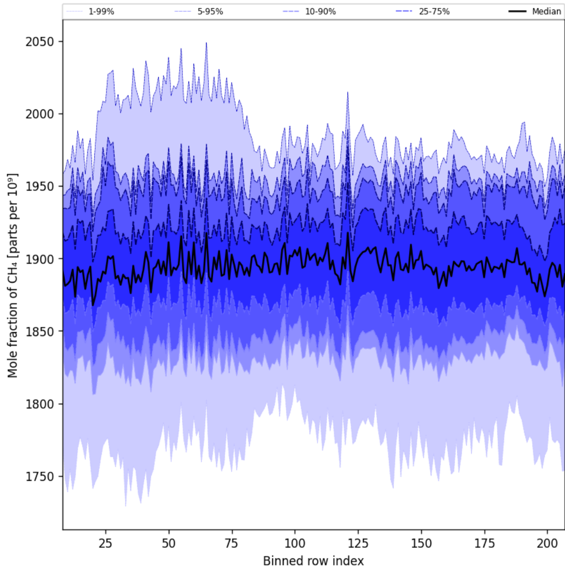
Figure 34: Along track statistics of “Mole fraction of CH 4 ” for 2024-09-03 to 2024-09-05
