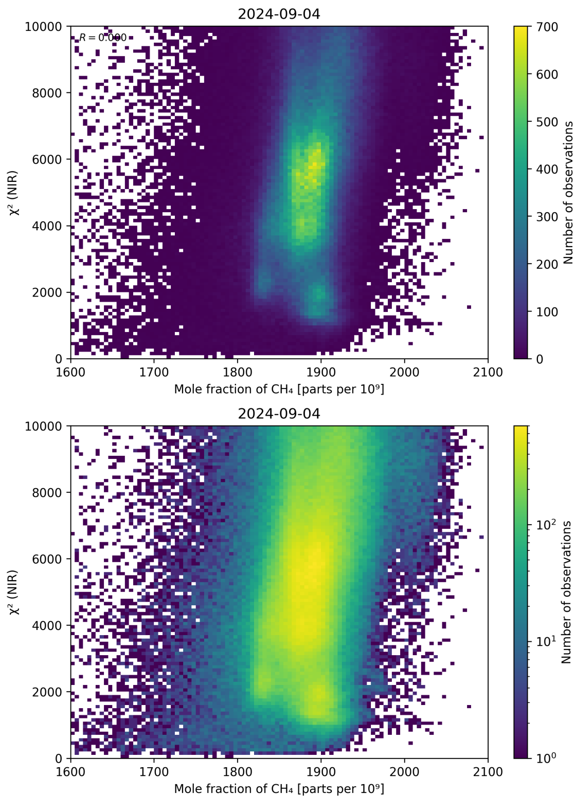
Figure 70: Scatter density plot of “Mole fraction of \text{CH}_4 ” against “ \chi^2 (NIR)” for 2024-09-03 to 2024-09-05.
