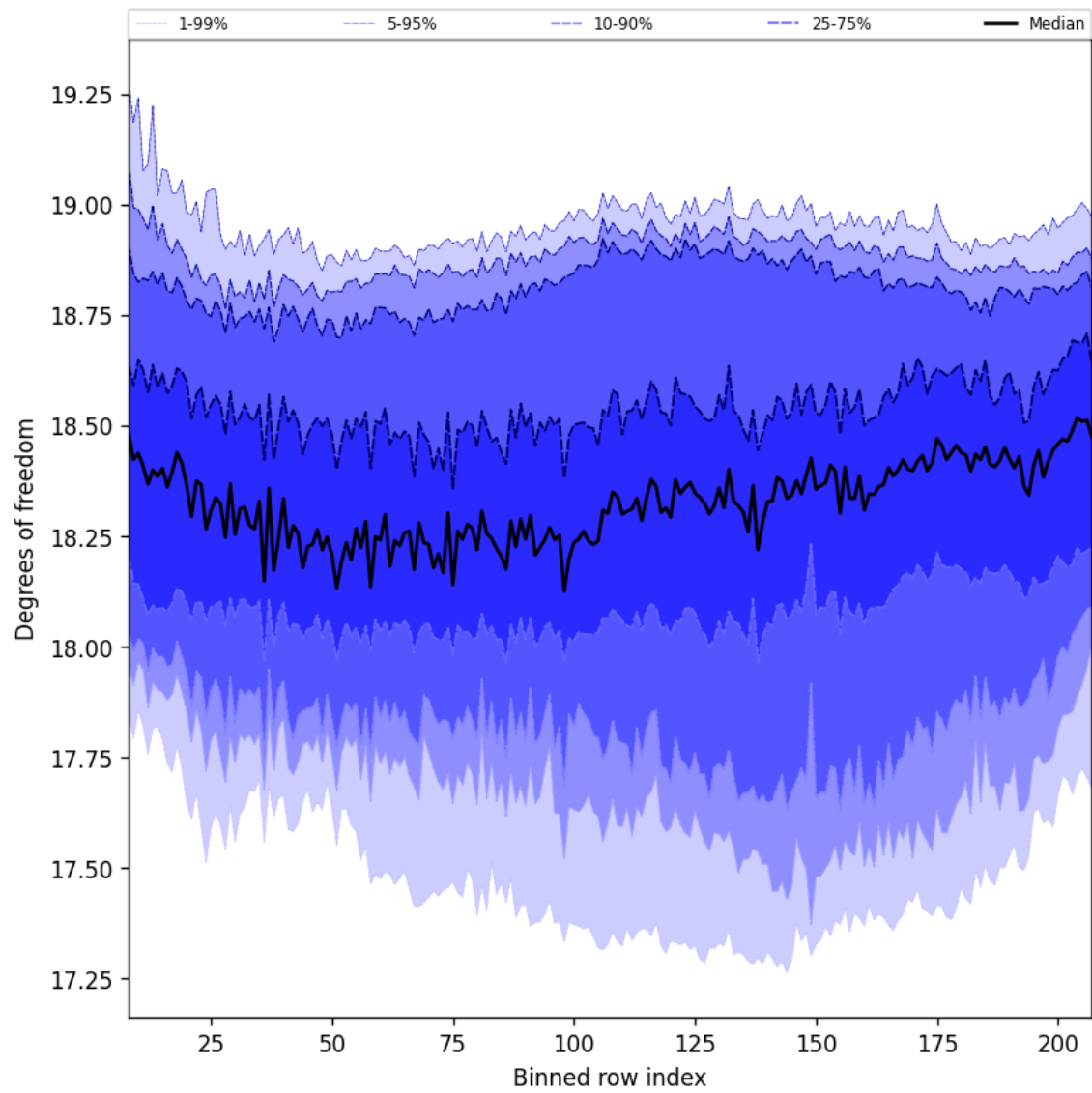
Figure 41: Along track statistics of “Degrees of freedom” for 2024-09-03 to 2024-09-05
