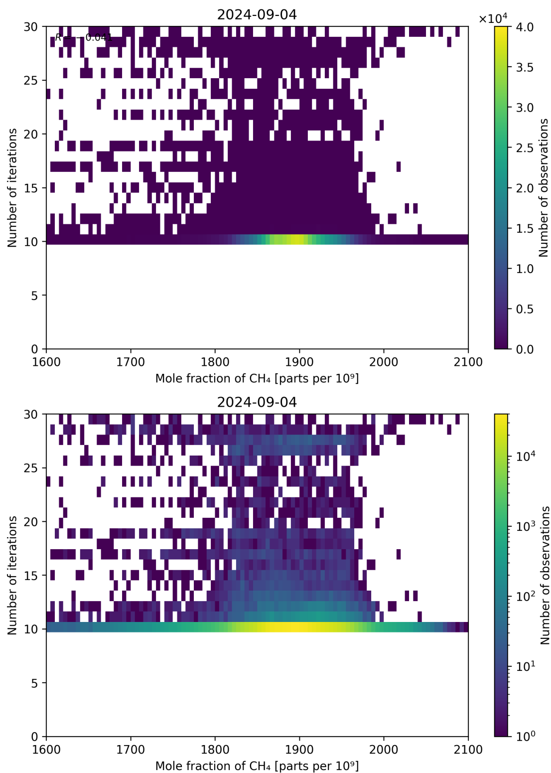
Figure 76: Scatter density plot of “Mole fraction of CH 4 ” against “Number of iterations” for 2024-09-03 to 2024-09-05.
