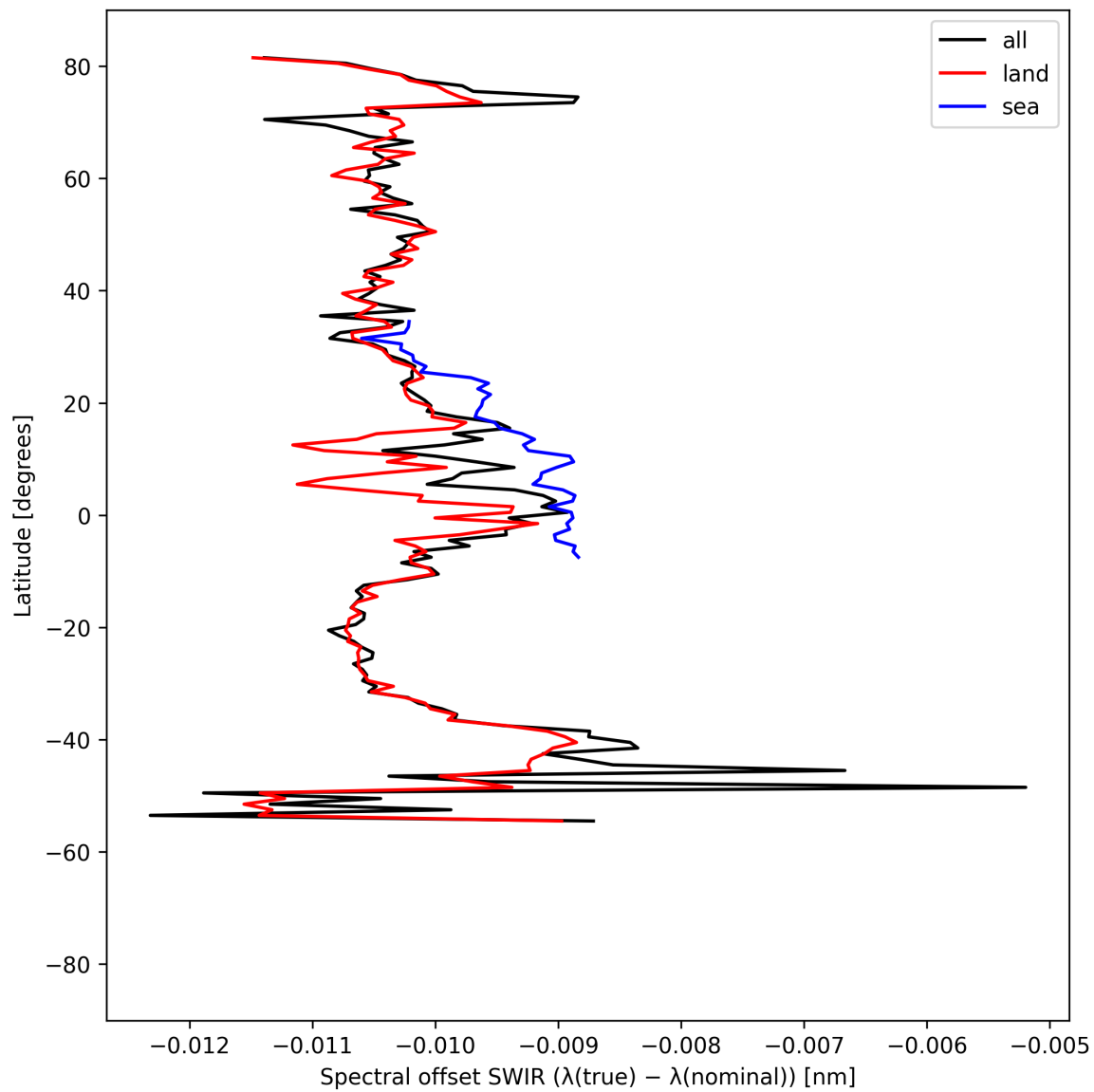
Figure 16: Zonal average of “Spectral offset SWIR ( \lambda_{\text{true}} - \lambda_{\text{nominal}} )” for 2024-09-03 to 2024-09-05.
