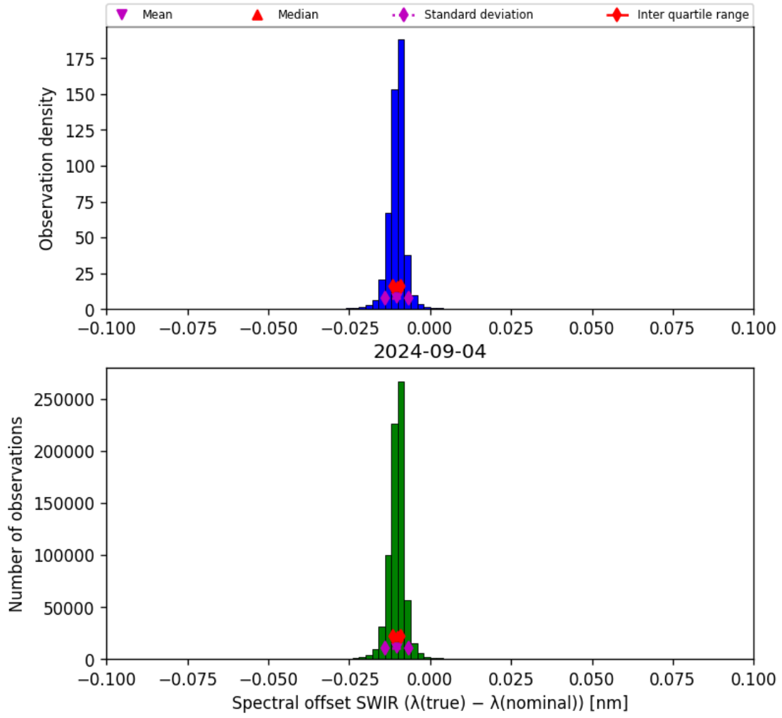
Figure 27: Histogram of “Spectral offset SWIR ( \lambda_{\text{true}} - \lambda_{\text{nominal}} )” for 2024-09-03 to 2024-09-05
