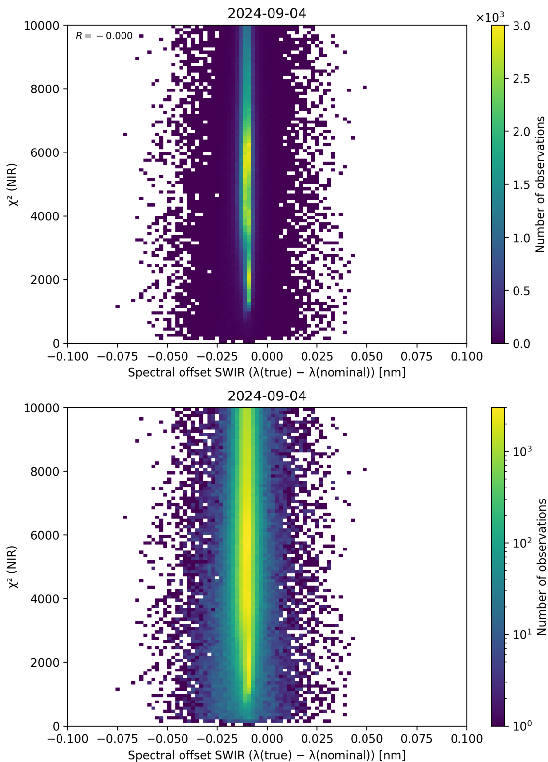
Figure 117: Scatter density plot of “Spectral offset SWIR ( \lambda_{\text{true}} - \lambda_{\text{nominal}} )” against “ \chi^2 (NIR)” for 2024-09-03 to 2024-09-05.
