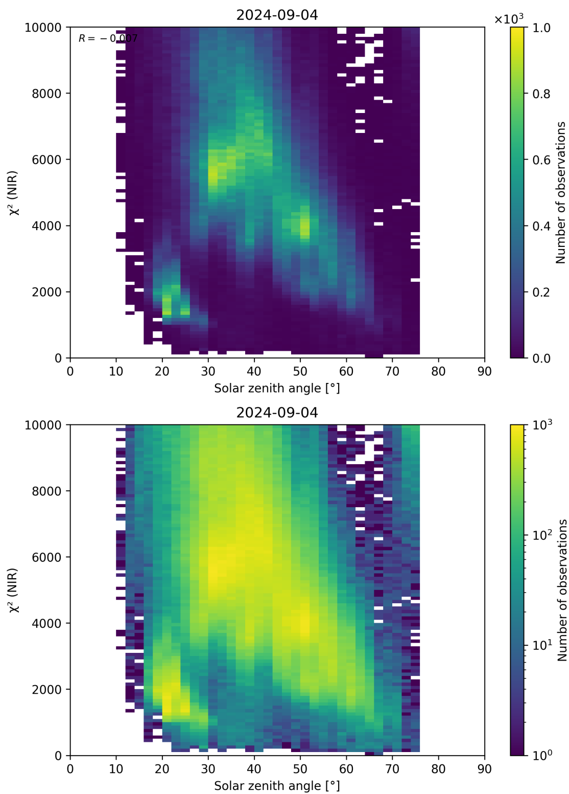
Figure 94: Scatter density plot of “Solar zenith angle” against “ \chi^2 (NIR)” for 2024-09-03 to 2024-09-05.
