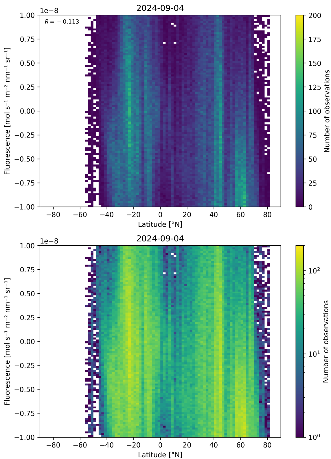
Figure 56: Scatter density plot of “Latitude” against “Fluorescence” for 2024-09-03 to 2024-09-05.
