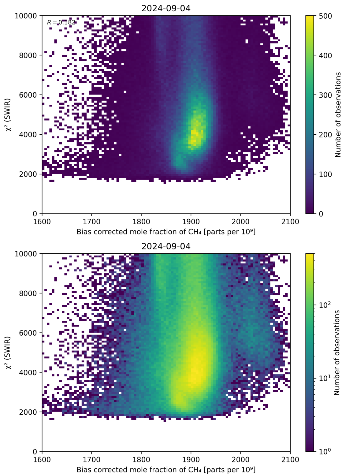
Figure 64: Scatter density plot of “Bias corrected mole fraction of \text{CH}_4 ” against “ \chi^2 (SWIR)” for 2024-09-03 to 2024-09-05.
