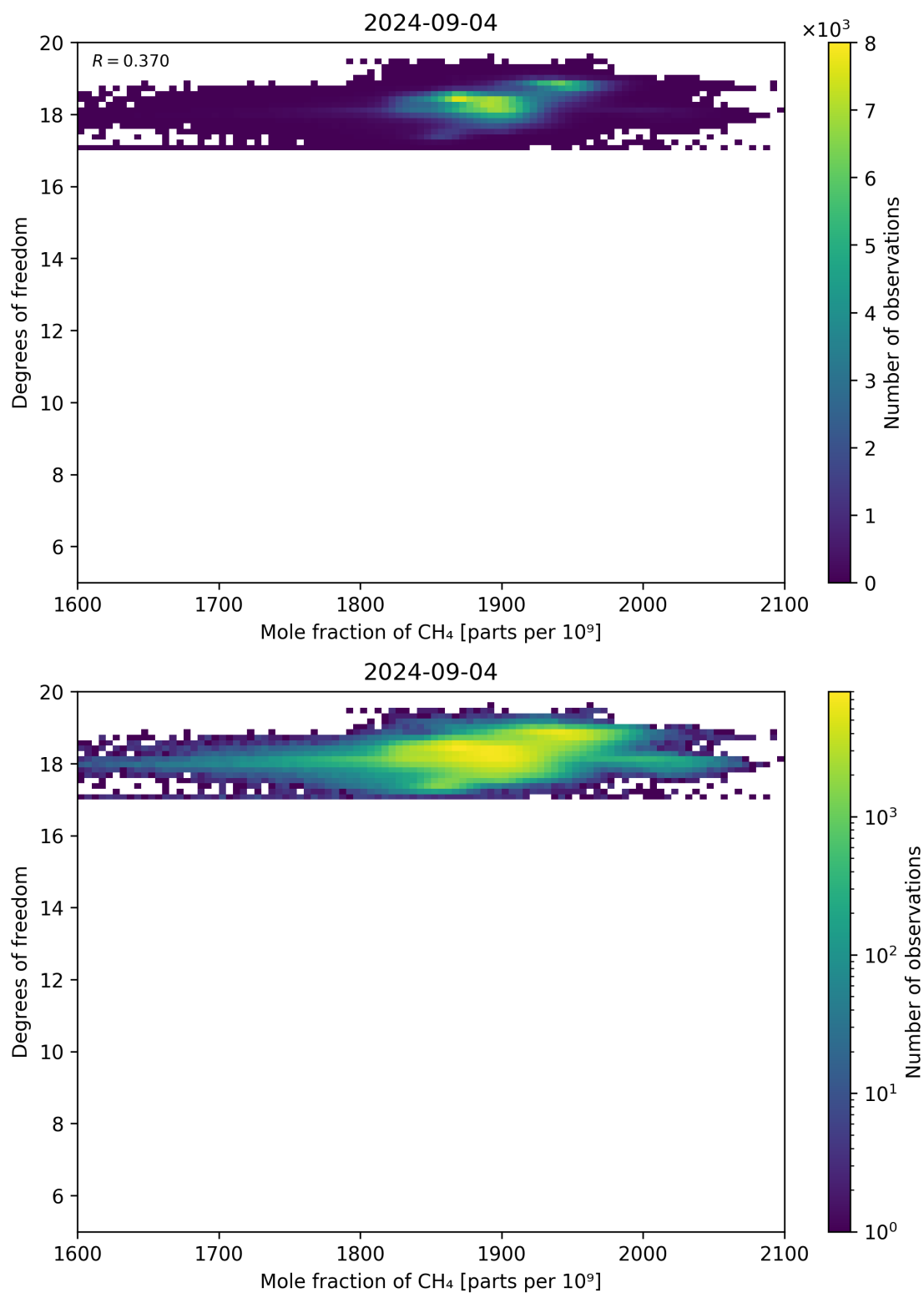
Figure 72: Scatter density plot of “Mole fraction of CH 4 ” against “Degrees of freedom” for 2024-09-03 to 2024-09-05.
