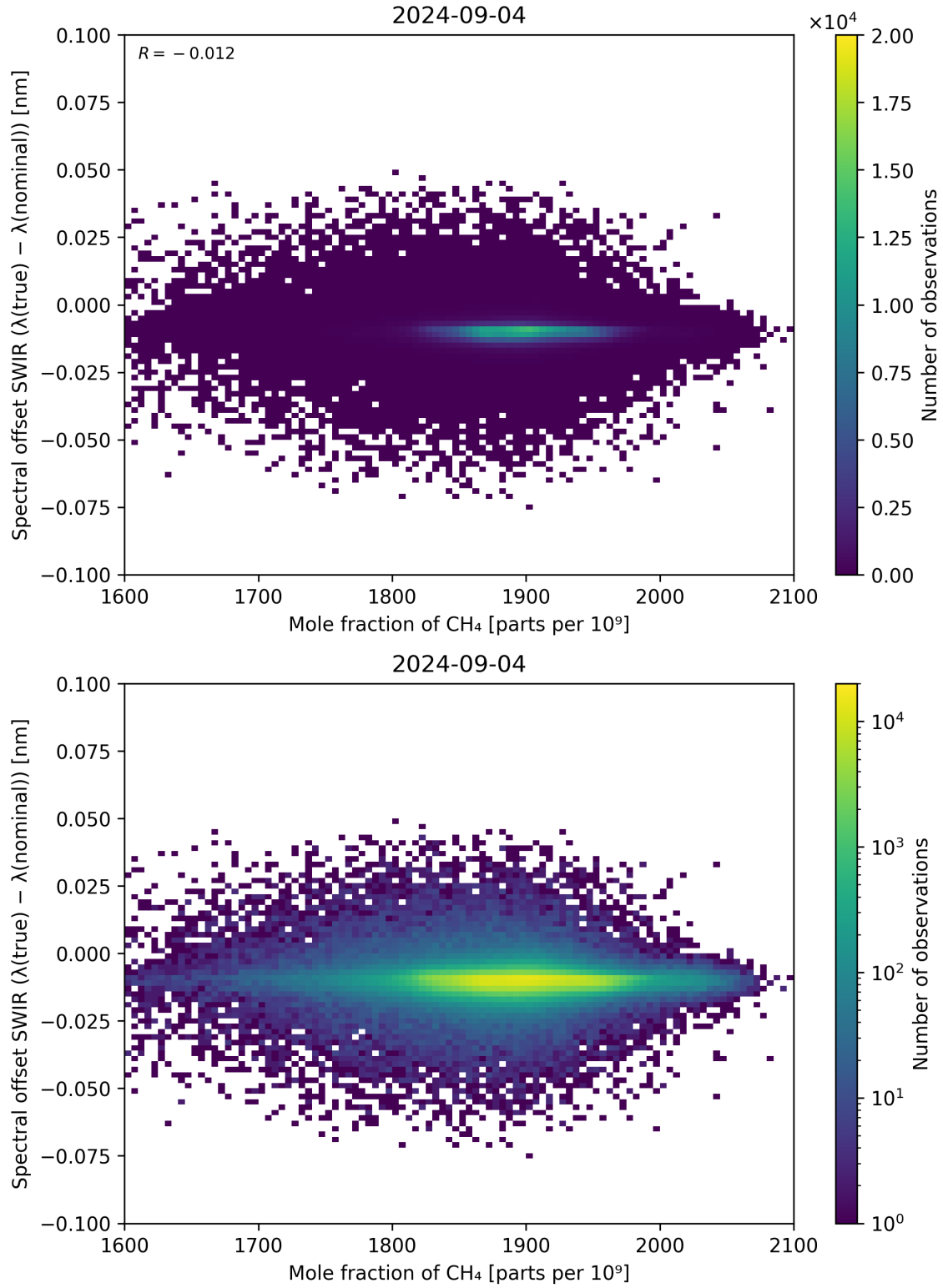
Figure 86: Scatter density plot of “Mole fraction of CH 4 ” against “Spectral offset SWIR ( \lambda_{\text{true}} - \lambda_{\text{nominal}} )” for 2024-09-03 to 2024-09-05.
