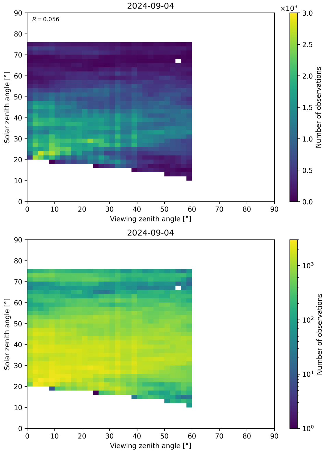
Figure 115: Scatter density plot of “Viewing zenith angle” against “Solar zenith angle” for 2024-09-03 to 2024-09-05.
