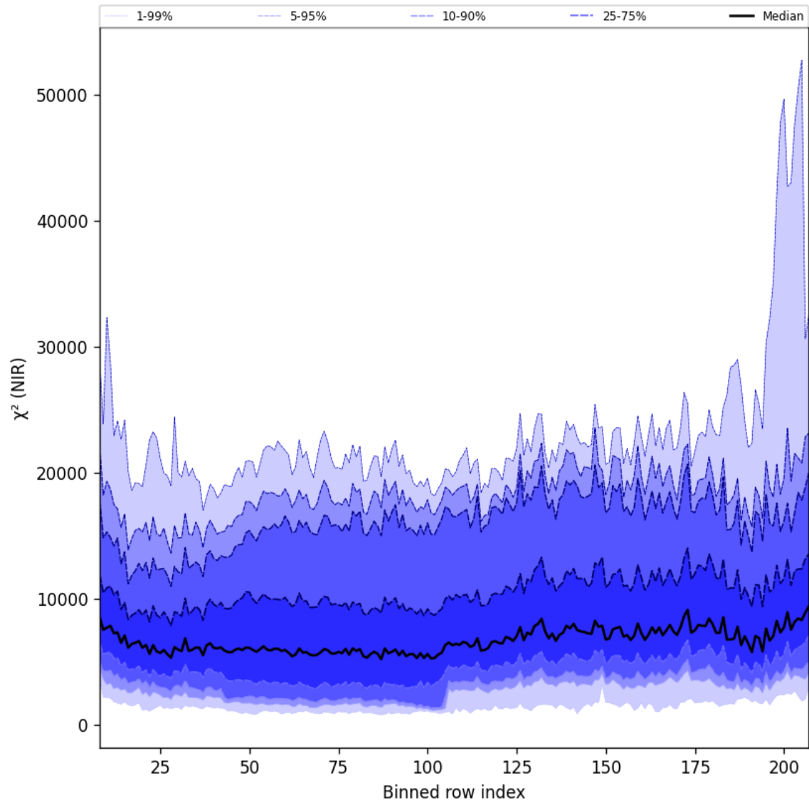
Figure 40: Along track statistics of “ \chi^2 (NIR)” for 2024-09-03 to 2024-09-05
