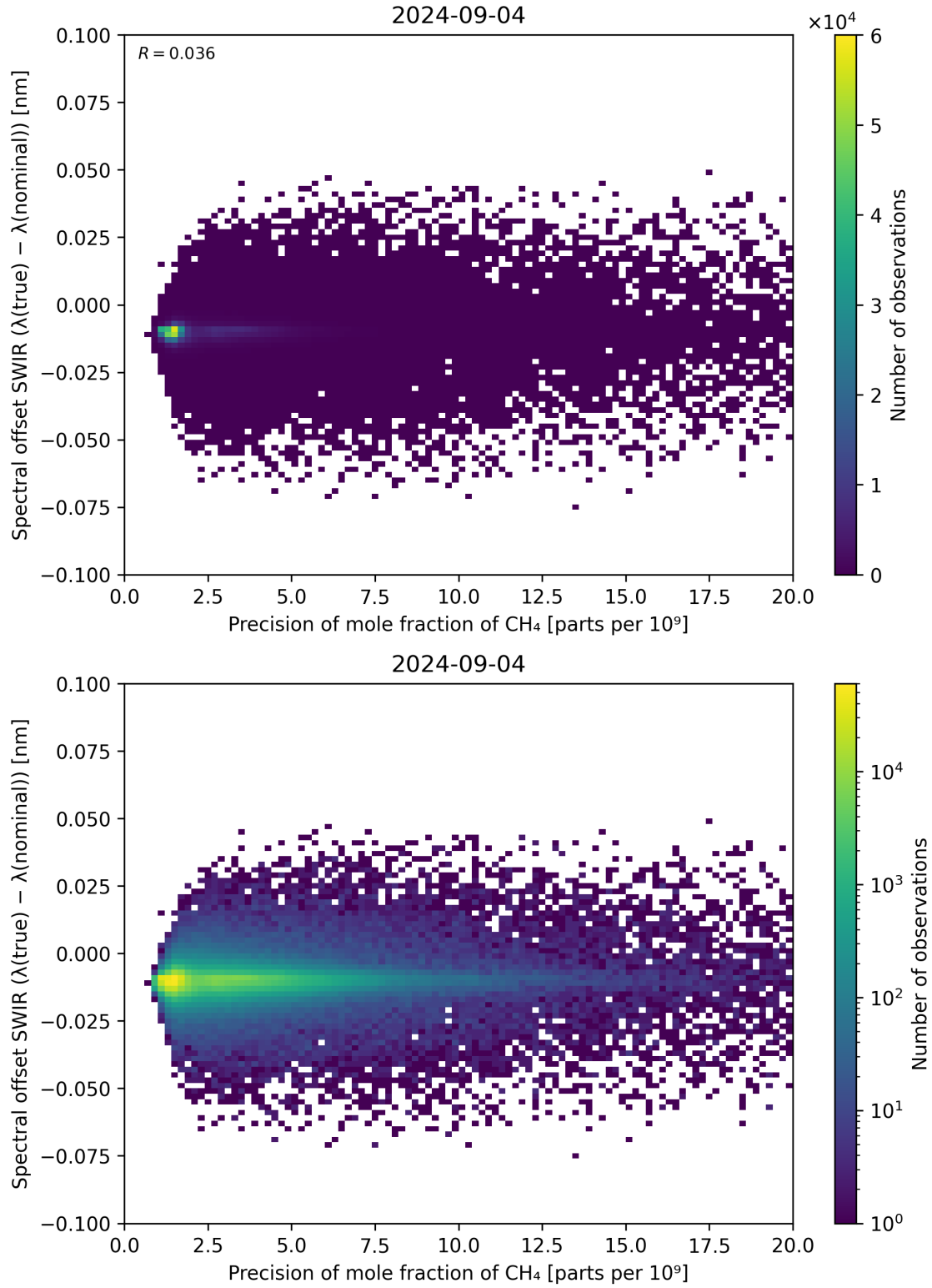
Figure 85: Scatter density plot of “Precision of mole fraction of CH 4 ” against “Spectral offset SWIR ( \lambda_{\text{true}} - \lambda_{\text{nominal}} )” for 2024-09-03 to 2024-09-05.
