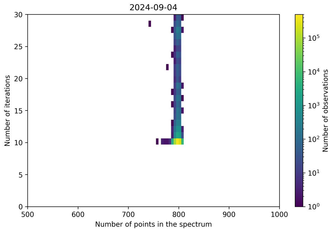
Figure 92: Scatter density plot of “Number of points in the spectrum” against “Number of iterations” for 2024-09-03 to 2024-09-05.
