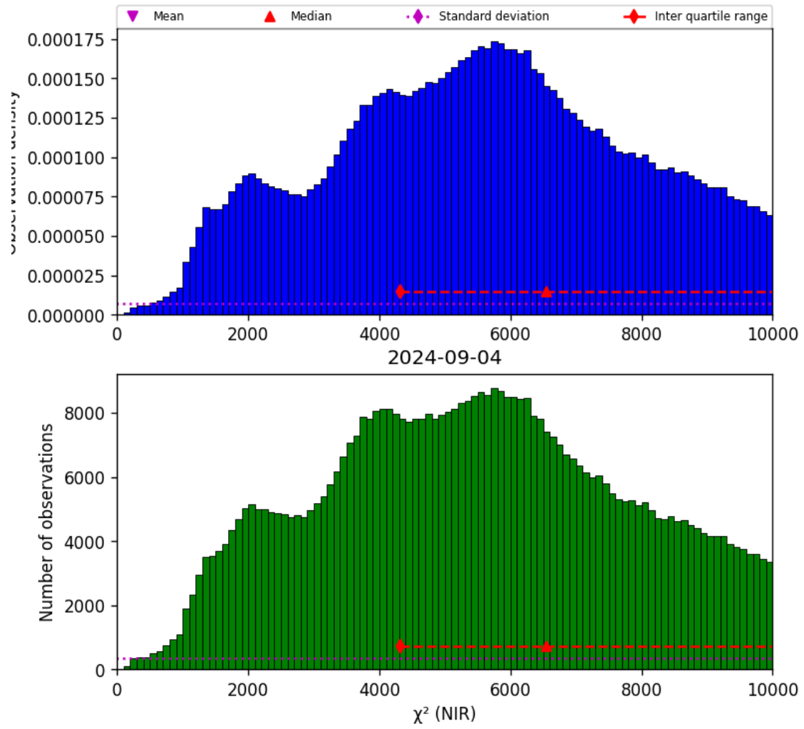
Figure 29: Histogram of “ \chi^2 (NIR)” for 2024-09-03 to 2024-09-05
