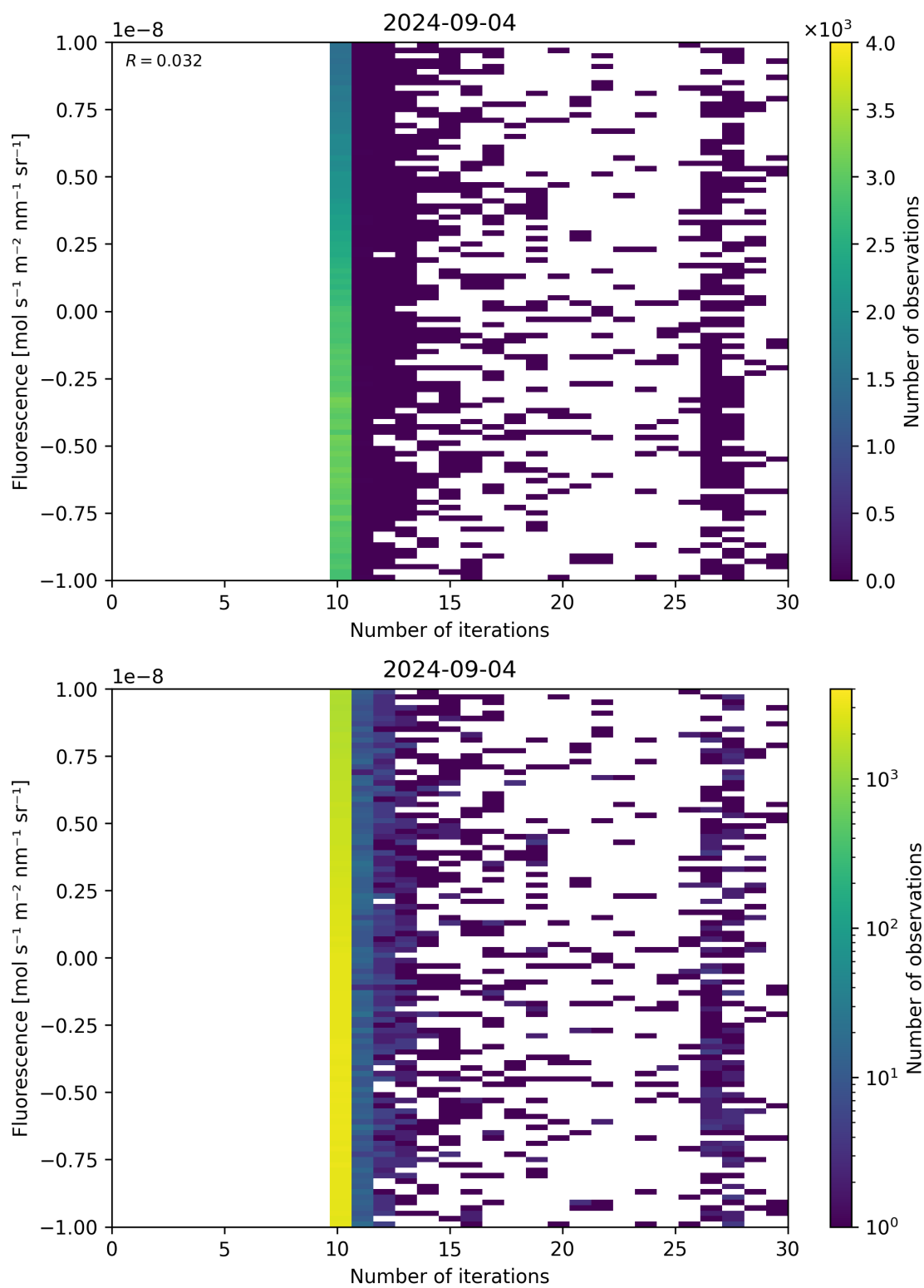
Figure 87: Scatter density plot of “Number of iterations” against “Fluorescence” for 2024-09-03 to 2024-09-05.
