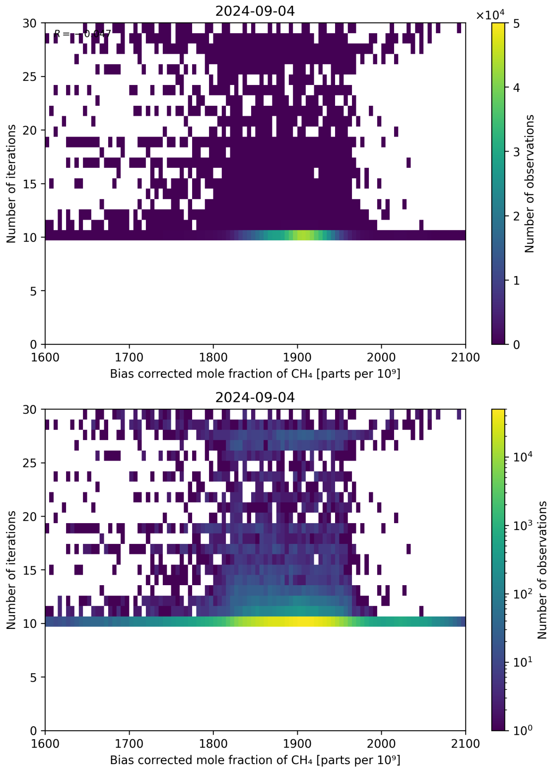
Figure 67: Scatter density plot of “Bias corrected mole fraction of CH 4 ” against “Number of iterations” for 2024-09-03 to 2024-09-05.
