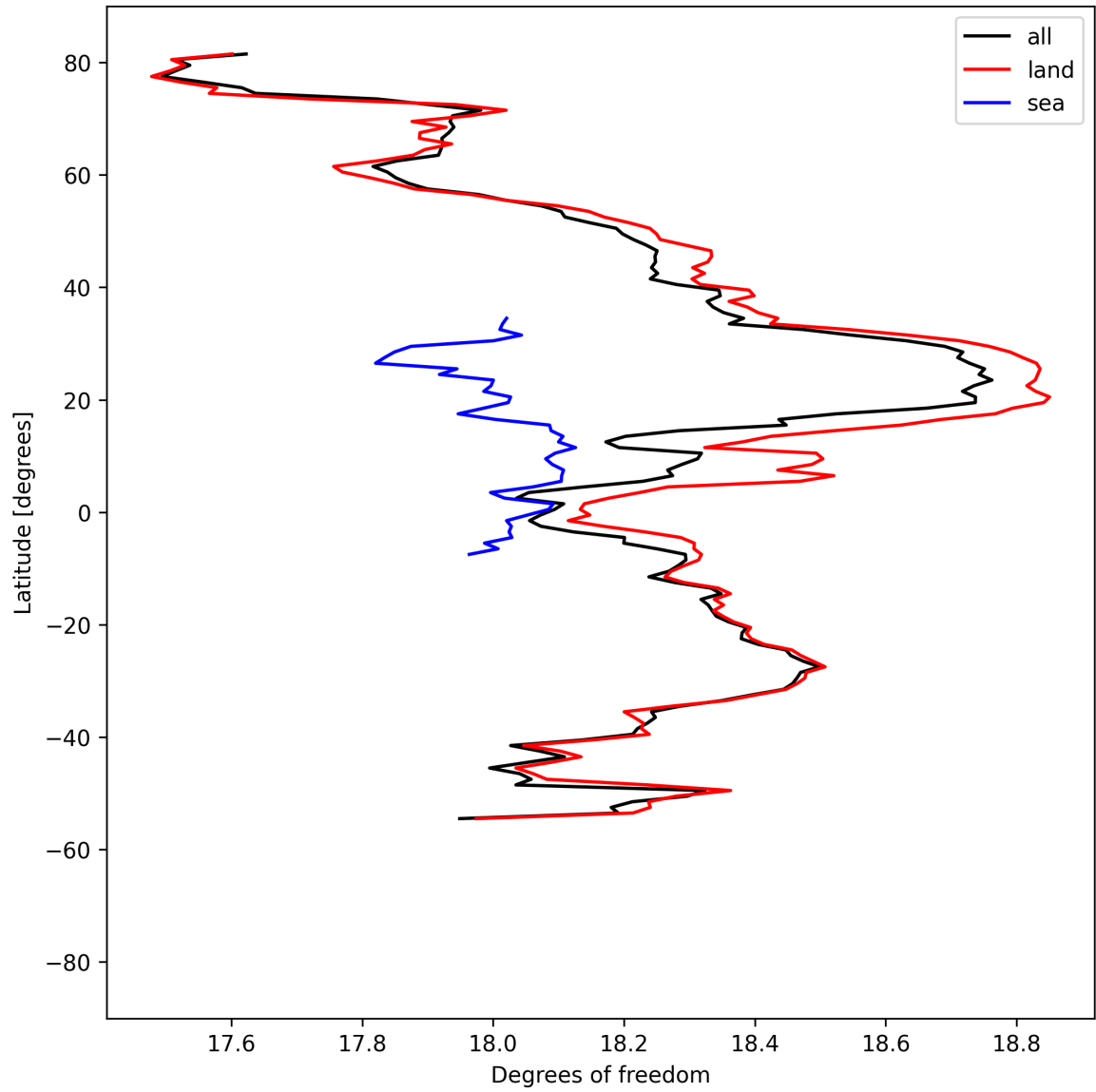
Figure 19: Zonal average of “Degrees of freedom” for 2024-09-03 to 2024-09-05.
