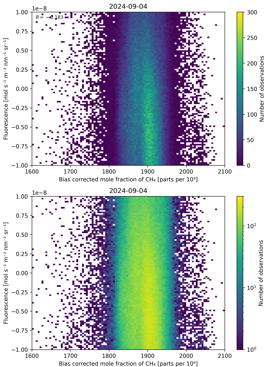
Figure 66: Scatter density plot of “Bias corrected mole fraction of \text{CH}_4 ” against “Fluorescence” for 2024-09-03 to 2024-09-05.
