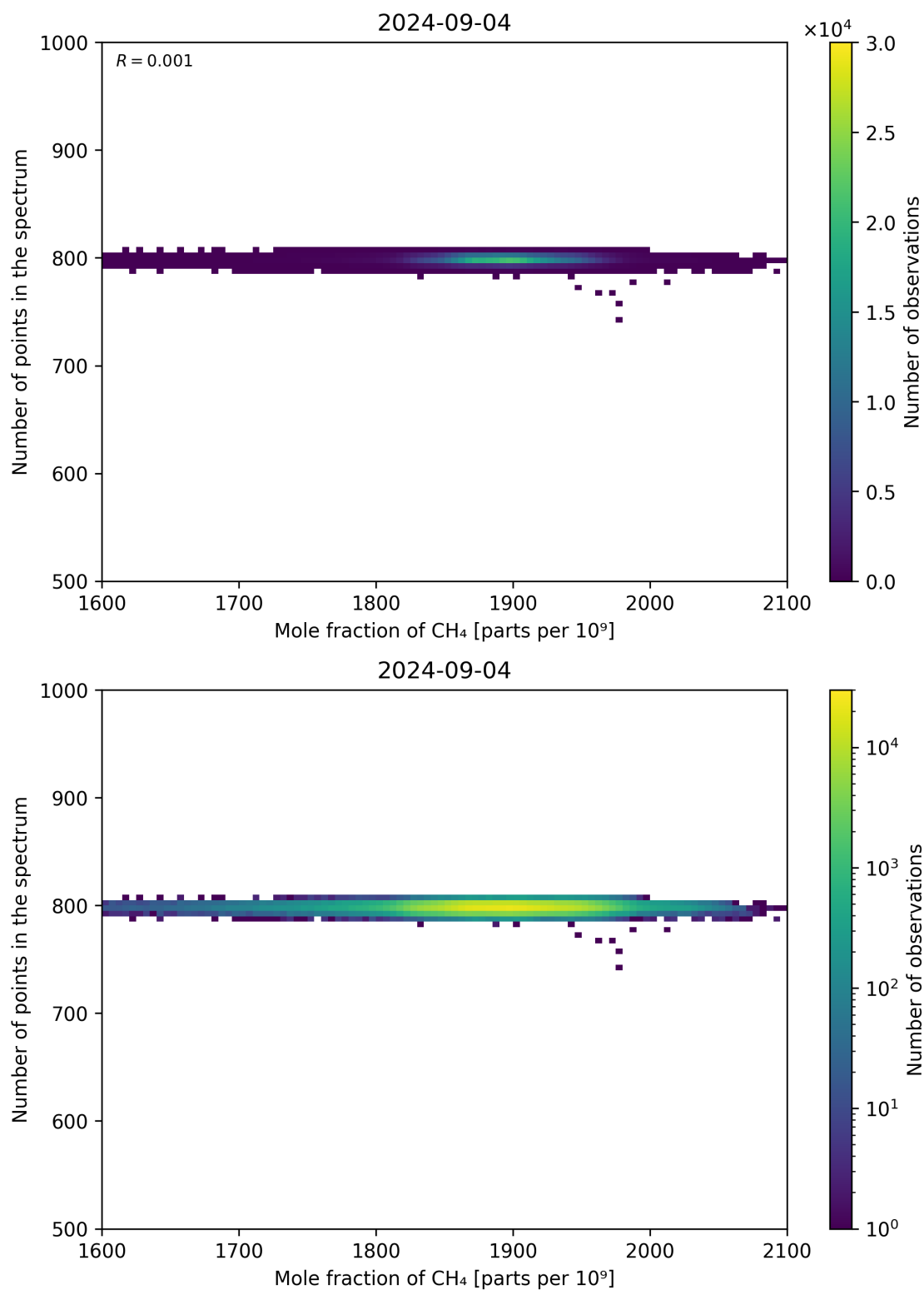
Figure 77: Scatter density plot of “Mole fraction of CH 4 ” against “Number of points in the spectrum” for 2024-09-03 to 2024-09-05.
