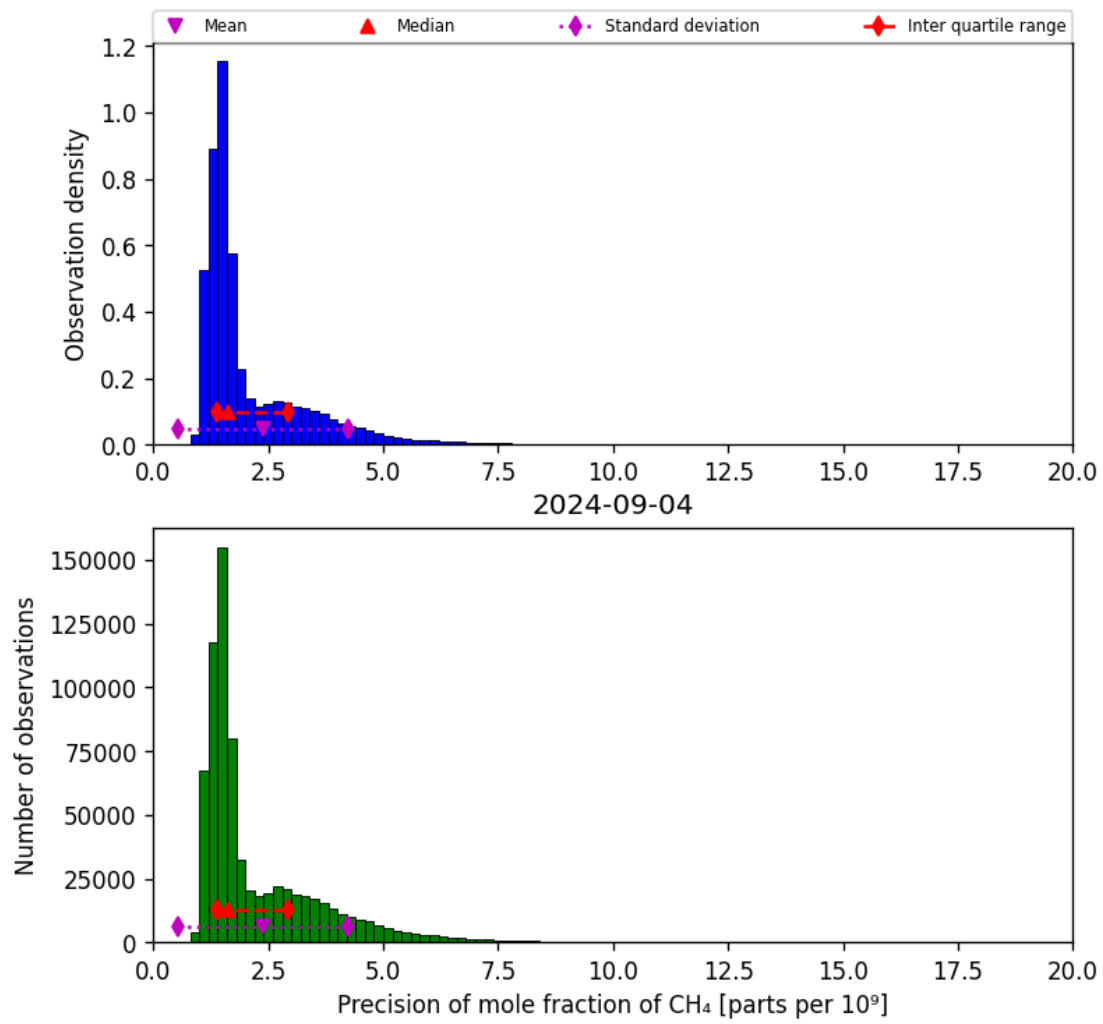
Figure 24: Histogram of “Precision of mole fraction of CH 4 ” for 2024-09-03 to 2024-09-05
