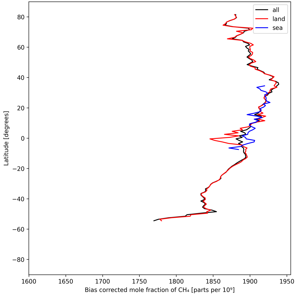
Figure 14: Zonal average of “Bias corrected mole fraction of CH 4 ” for 2024-09-03 to 2024-09-05.
