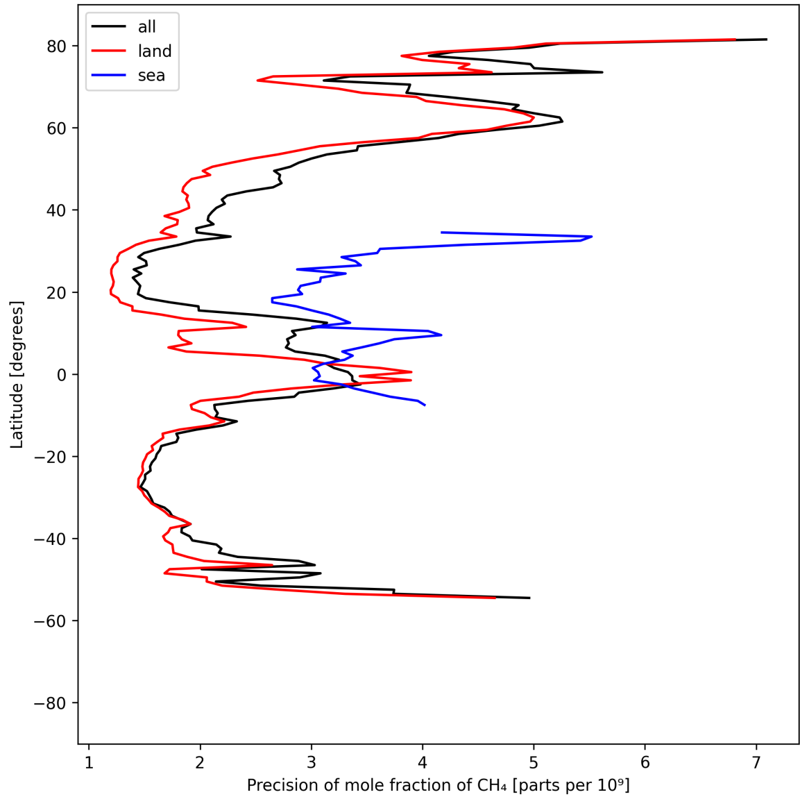
Figure 13: Zonal average of “Precision of mole fraction of CH 4 ” for 2024-09-03 to 2024-09-05.
