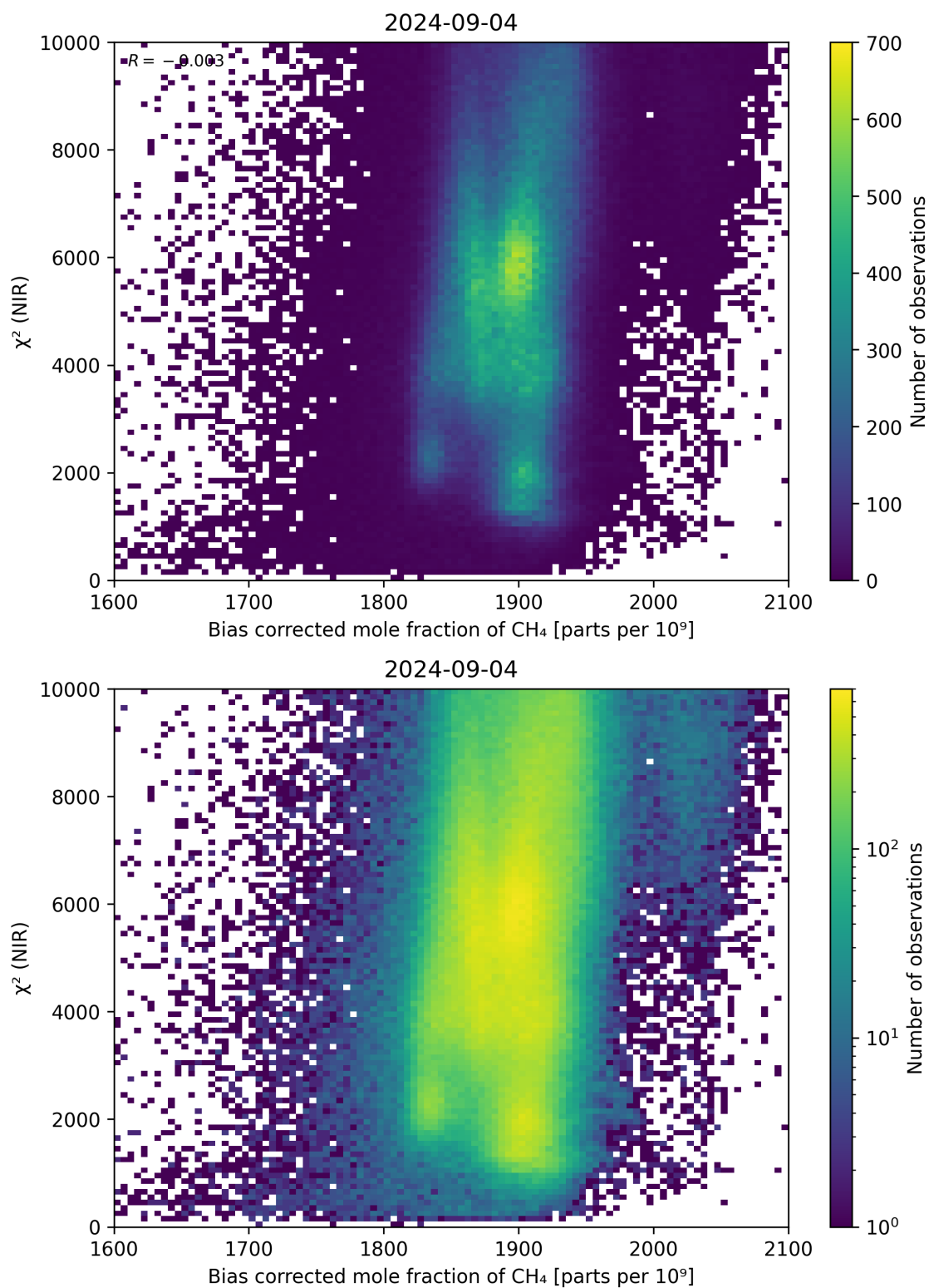
Figure 63: Scatter density plot of “Bias corrected mole fraction of CH 4 ” against “ \chi^2 (NIR)” for 2024-09-03 to 2024-09-05.
