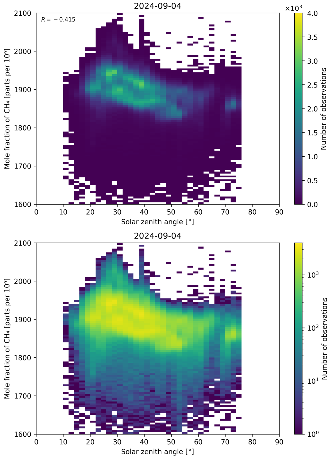
Figure 99: Scatter density plot of “Solar zenith angle” against “Mole fraction of \text{CH}_4 ” for 2024-09-03 to 2024-09-05.
