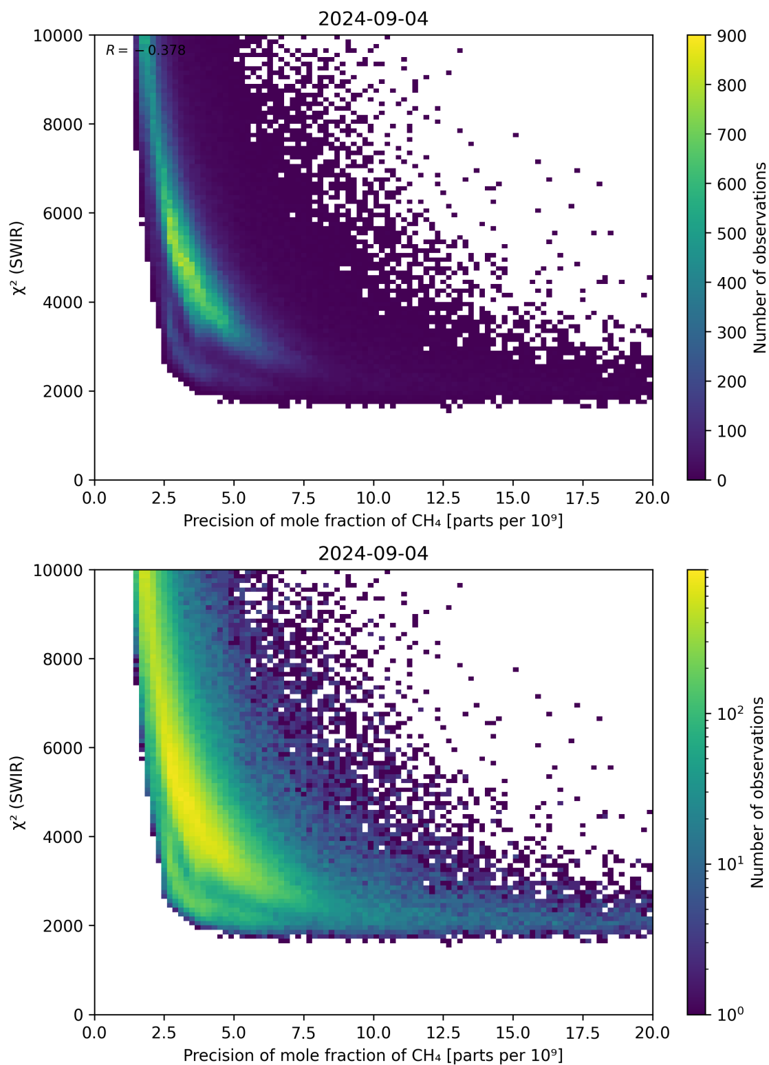
Figure 79: Scatter density plot of “Precision of mole fraction of \text{CH}_4 ” against “ \chi^2 (SWIR)” for 2024-09-03 to 2024-09-05.
