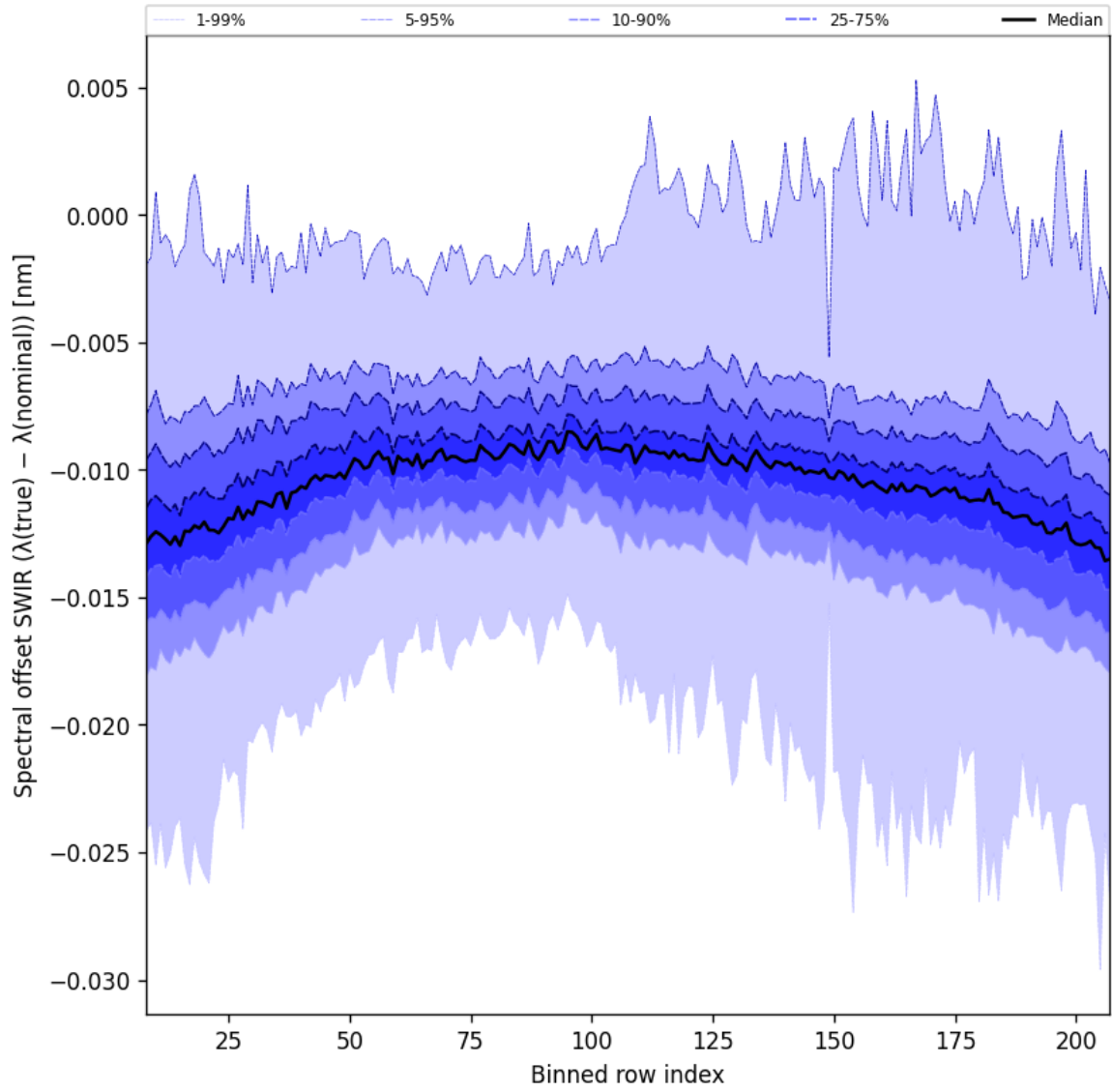
Figure 38: Along track statistics of “Spectral offset SWIR ( \lambda_{\text{true}} - \lambda_{\text{nominal}} )” for 2024-09-03 to 2024-09-05
