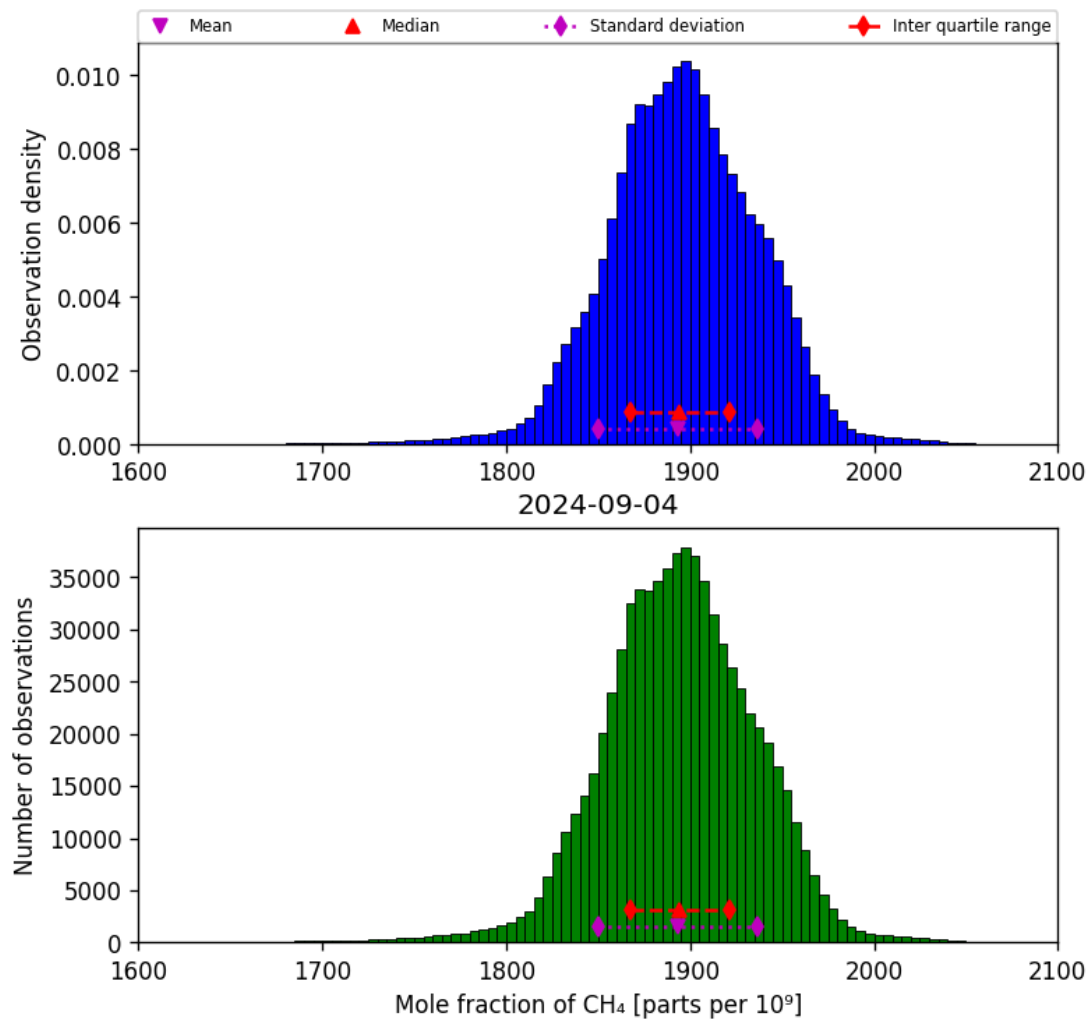
Figure 23: Histogram of “Mole fraction of CH 4 ” for 2024-09-03 to 2024-09-05
