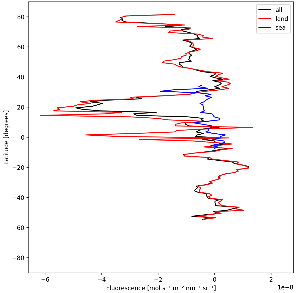
Figure 21: Zonal average of “Fluorescence” for 2024-09-03 to 2024-09-05.
