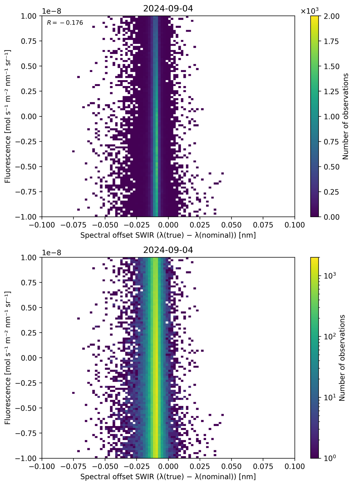
Figure 120: Scatter density plot of “Spectral offset SWIR ( \lambda_{\text{true}} - \lambda_{\text{nominal}} )” against “Fluorescence” for 2024-09-03 to 2024-09-05.
