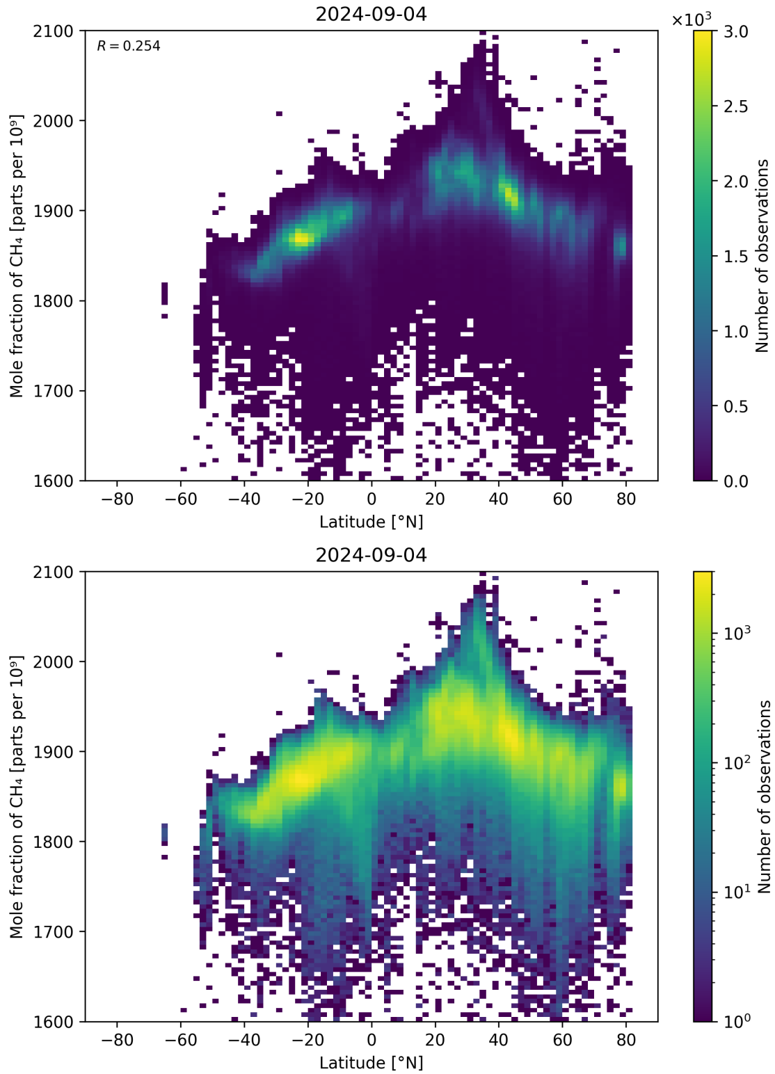
Figure 57: Scatter density plot of “Latitude” against “Mole fraction of CH 4 ” for 2024-09-03 to 2024-09-05.
