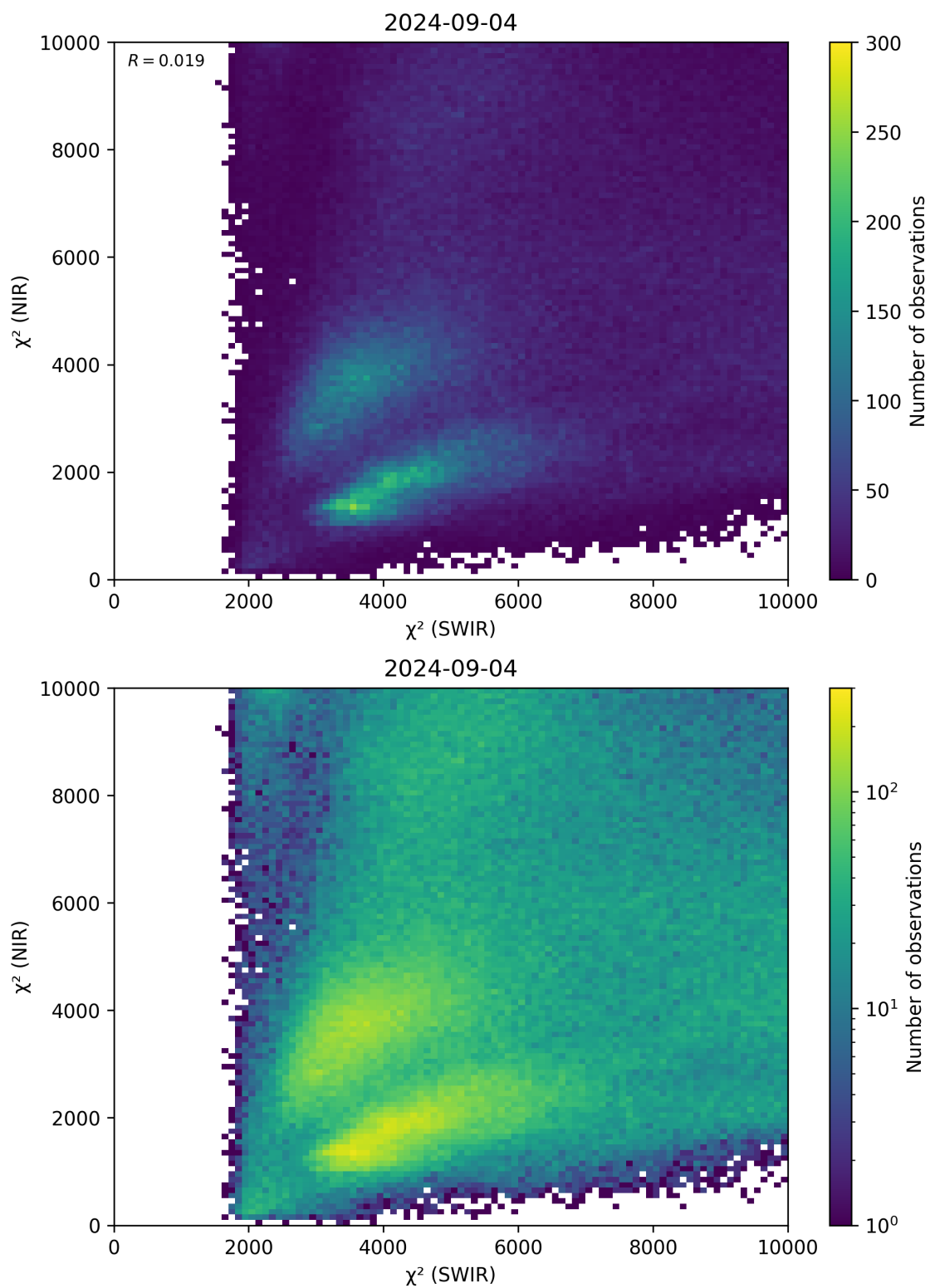
Figure 47: Scatter density plot of “ \chi^2 (SWIR)” against “ \chi^2 (NIR)” for 2024-09-03 to 2024-09-05.
