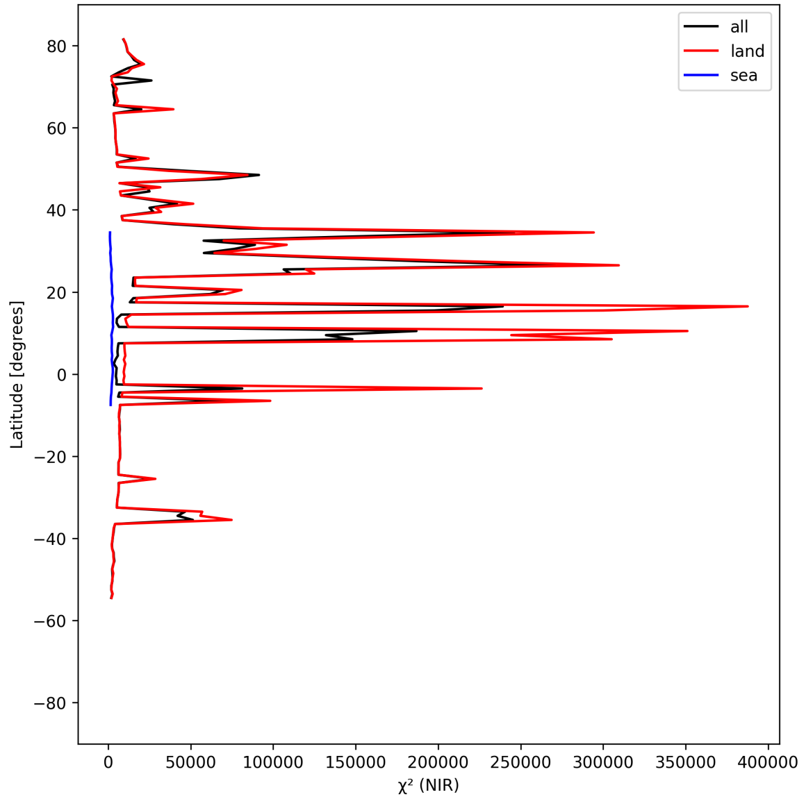
Figure 18: Zonal average of “ \chi^2 (NIR)” for 2024-09-03 to 2024-09-05.
