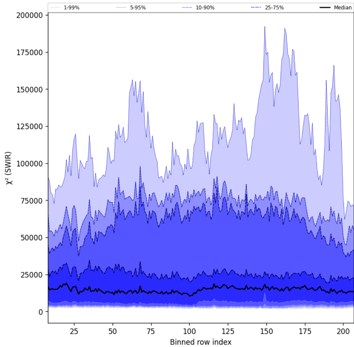
Figure 39: Along track statistics of “ \chi^2 (SWIR)” for 2024-09-03 to 2024-09-05
