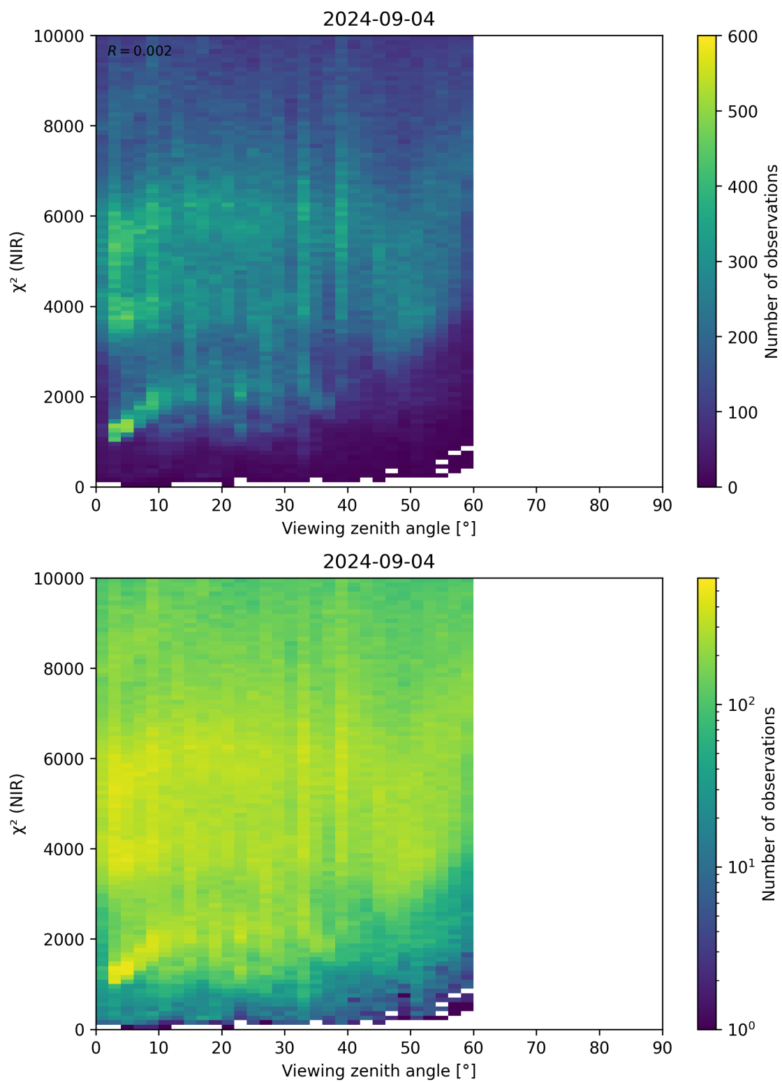
Figure 105: Scatter density plot of “Viewing zenith angle” against “ \chi^2 (NIR)” for 2024-09-03 to 2024-09-05.
