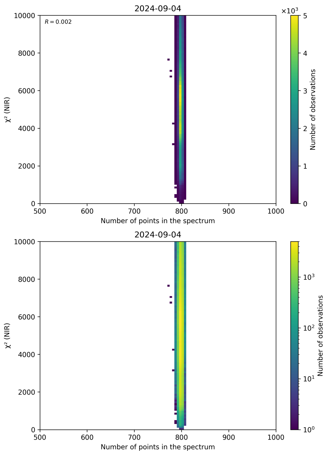
Figure 88: Scatter density plot of “Number of points in the spectrum” against “ \chi^2 (NIR)” for 2024-09-03 to 2024-09-05.
