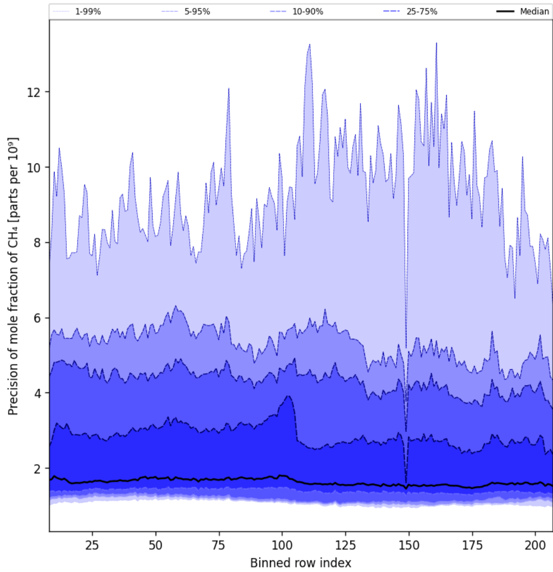
Figure 35: Along track statistics of “Precision of mole fraction of CH 4 ” for 2024-09-03 to 2024-09-05
