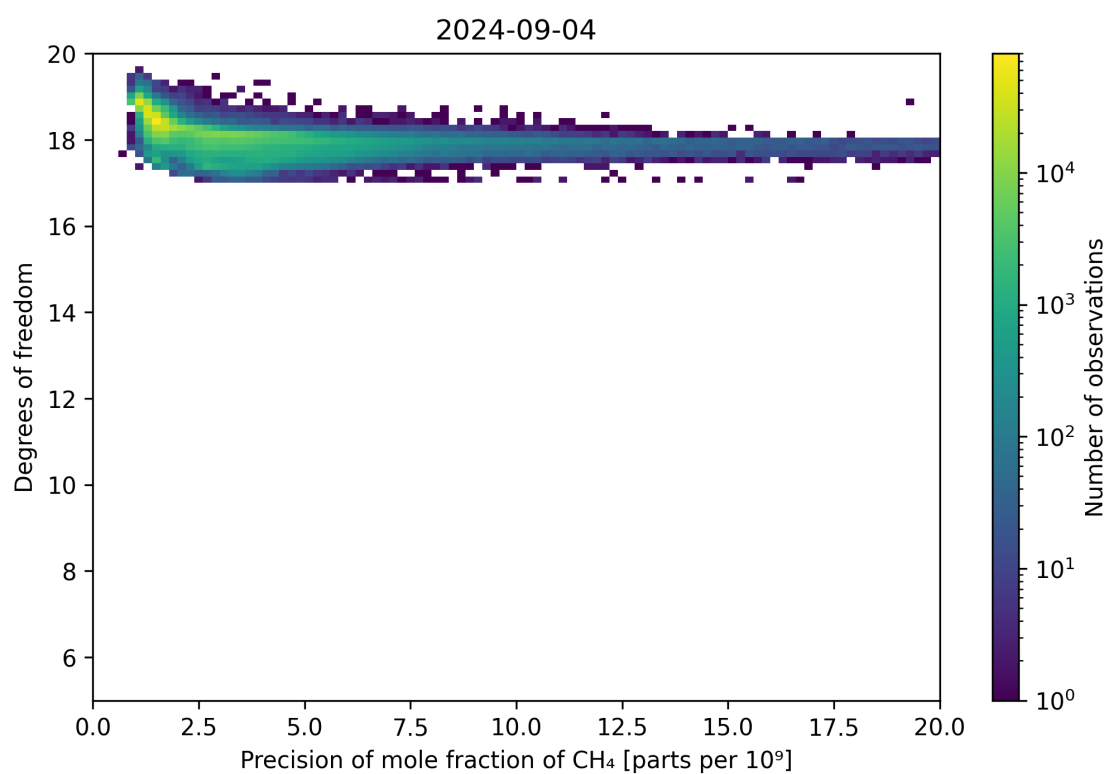
Figure 80: Scatter density plot of “Precision of mole fraction of CH 4 ” against “Degrees of freedom” for 2024-09-03 to 2024-09-05.
