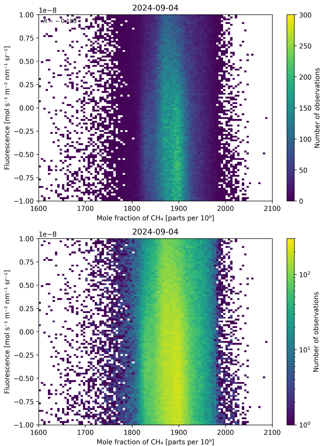
Figure 73: Scatter density plot of “Mole fraction of \text{CH}_4 ” against “Fluorescence” for 2024-09-03 to 2024-09-05.
