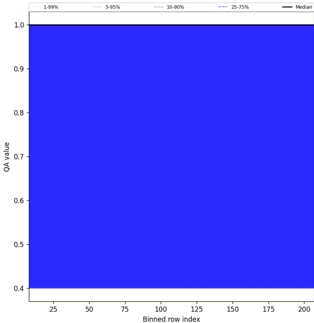
Figure 33: Along track statistics of “QA value” for 2024-09-03 to 2024-09-05
