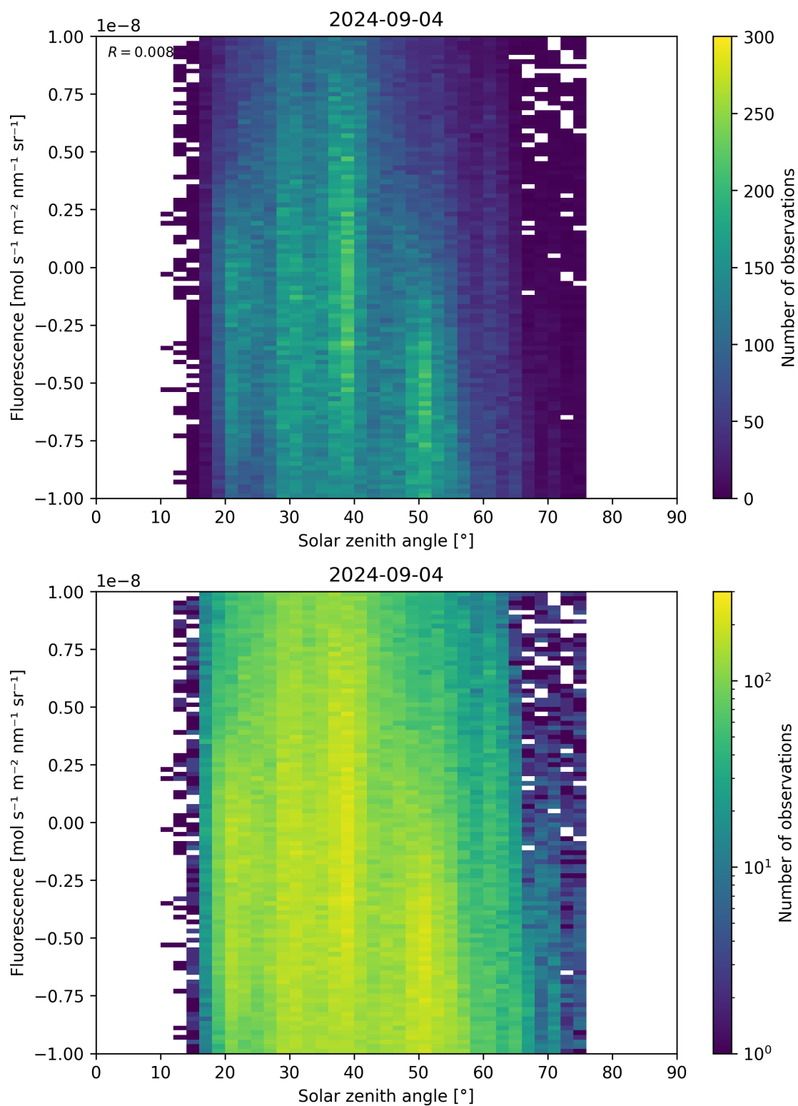
Figure 97: Scatter density plot of “Solar zenith angle” against “Fluorescence” for 2024-09-03 to 2024-09-05.
