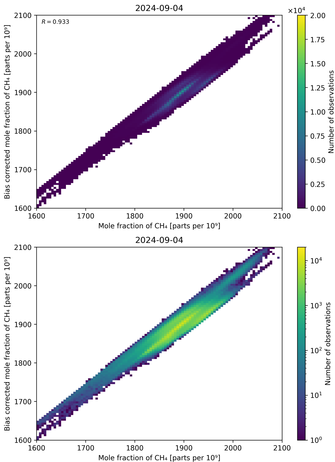
Figure 74: Scatter density plot of “Mole fraction of CH 4 ” against “Bias corrected mole fraction of CH 4 ” for 2024-09-03 to 2024-09-05.
