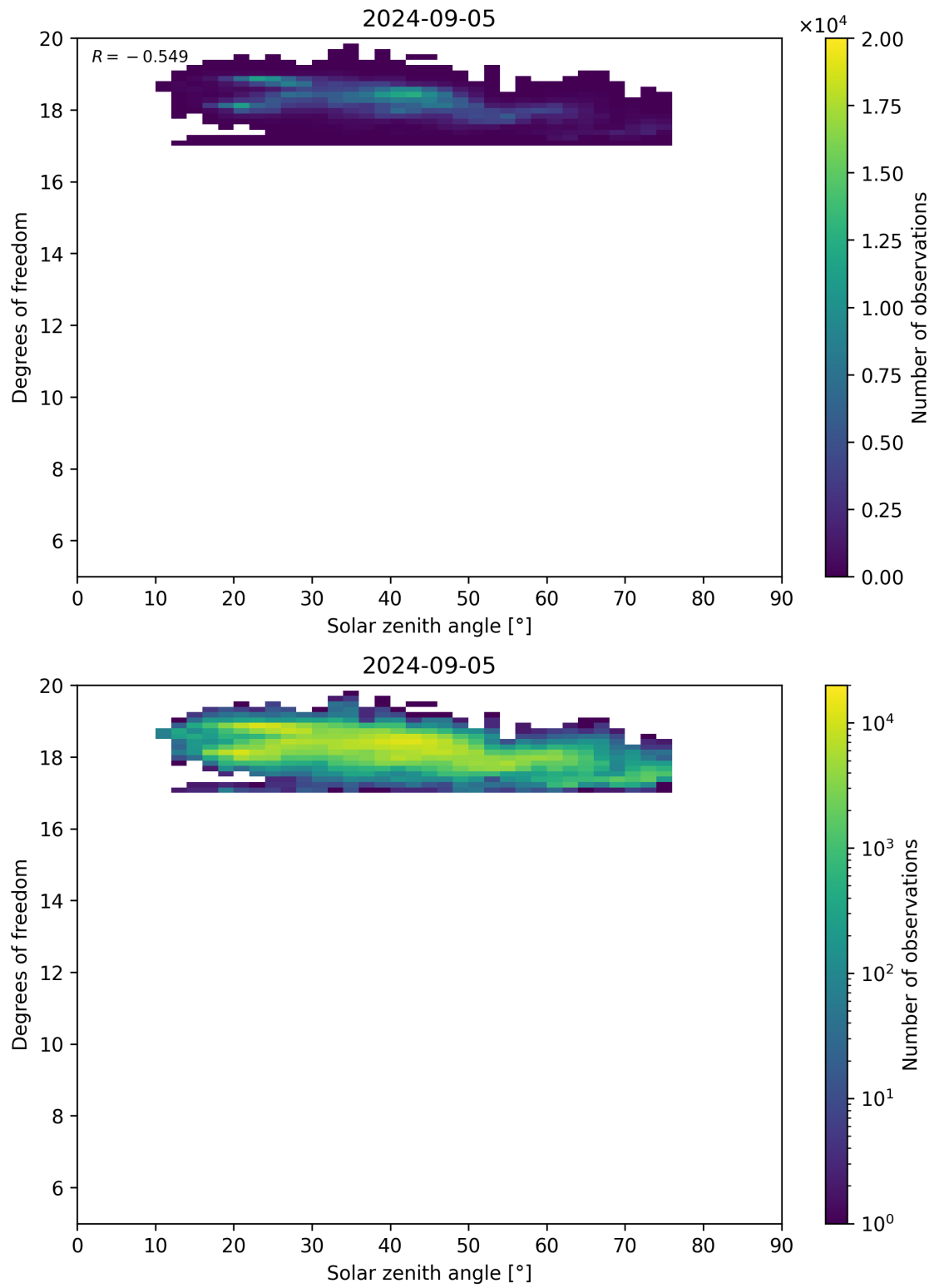
Figure 96: Scatter density plot of “Solar zenith angle” against “Degrees of freedom” for 2024-09-04 to 2024-09-06.
