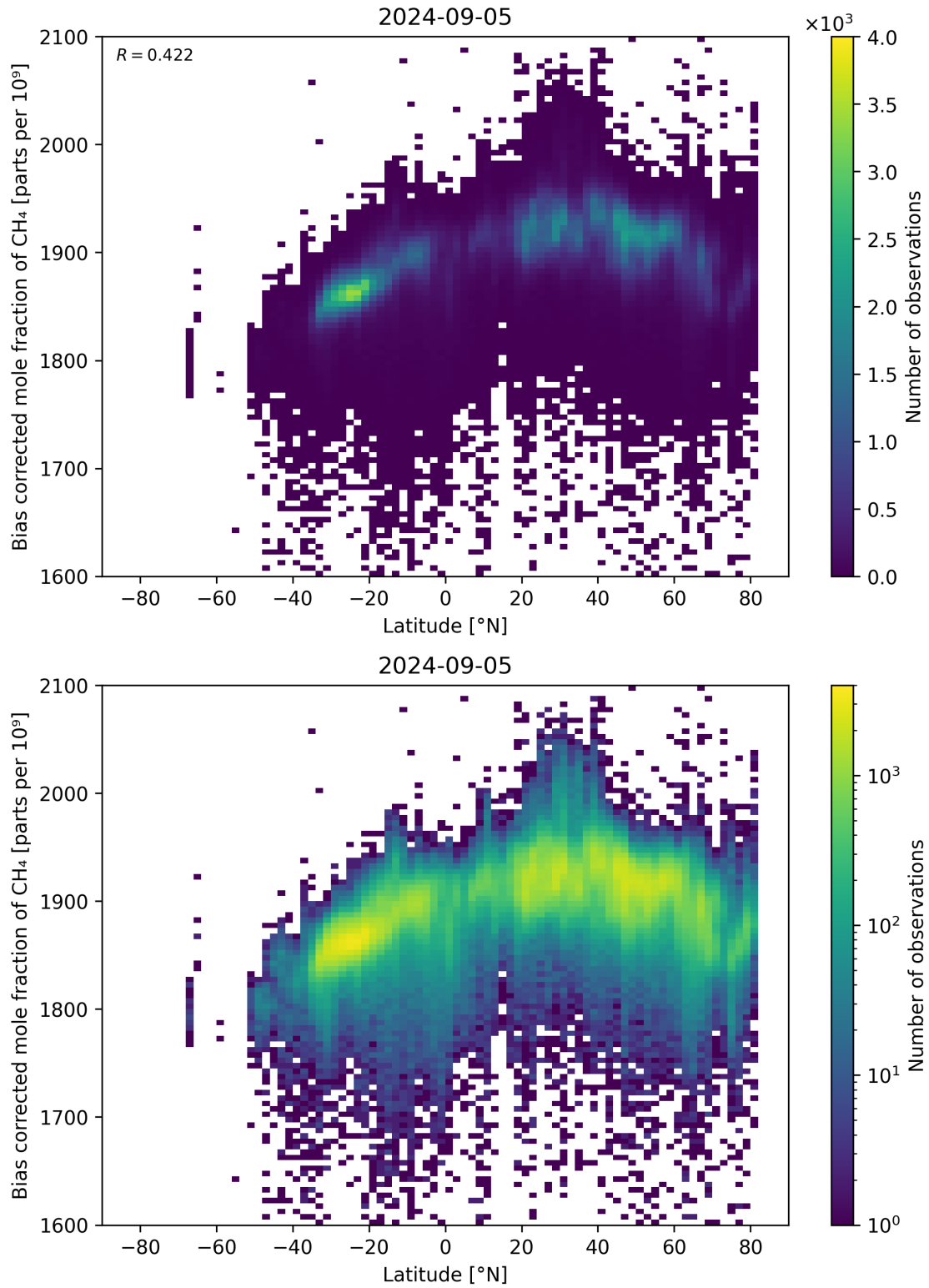
Figure 58: Scatter density plot of “Latitude” against “Bias corrected mole fraction of CH 4 ” for 2024-09-04 to 2024-09-06.
