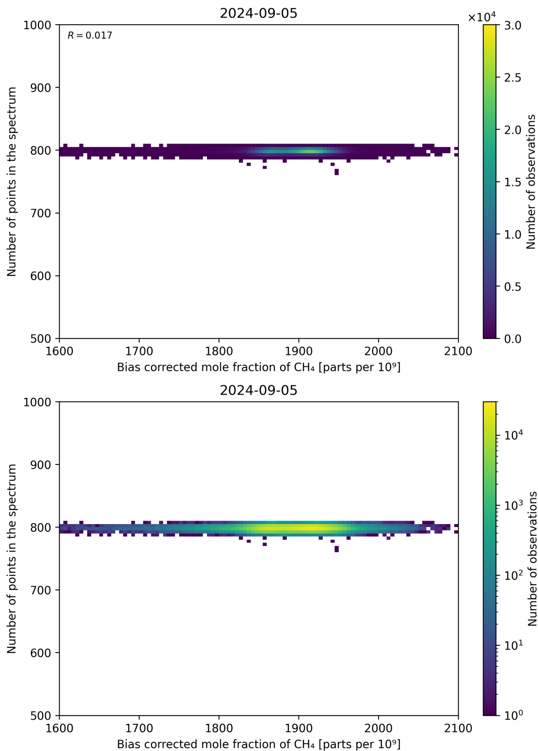
Figure 68: Scatter density plot of “Bias corrected mole fraction of CH 4 ” against “Number of points in the spectrum” for 2024-09-04 to 2024-09-06.
