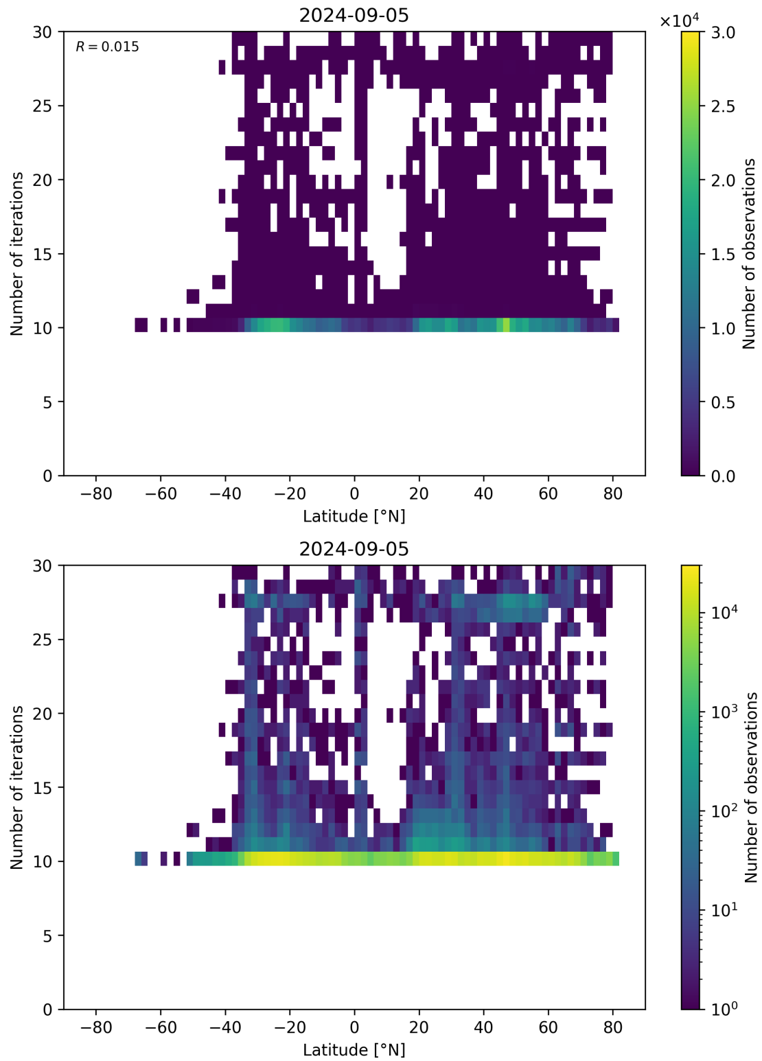
Figure 60: Scatter density plot of “Latitude” against “Number of iterations” for 2024-09-04 to 2024-09-06.
