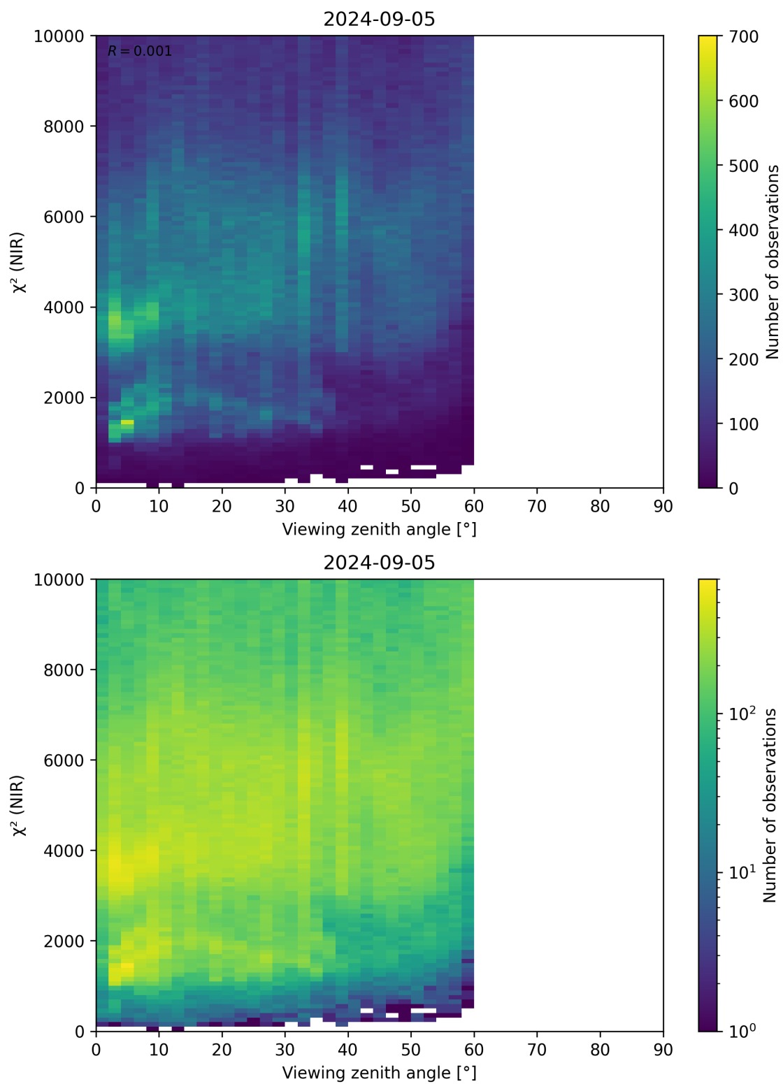
Figure 105: Scatter density plot of “Viewing zenith angle” against “ \chi^2 (NIR)” for 2024-09-04 to 2024-09-06.
