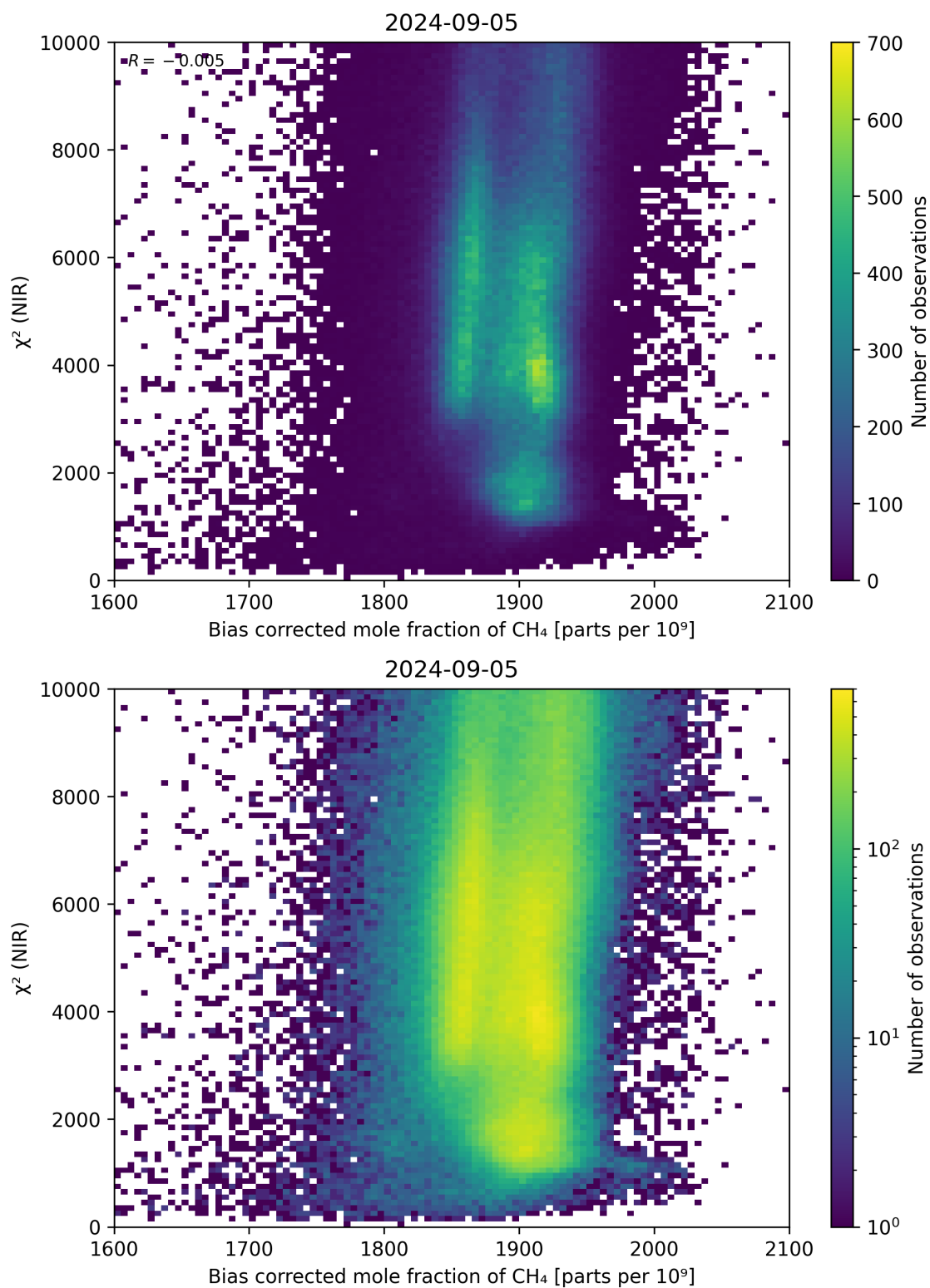
Figure 63: Scatter density plot of “Bias corrected mole fraction of CH 4 ” against “ \chi^2 (NIR)” for 2024-09-04 to 2024-09-06.
