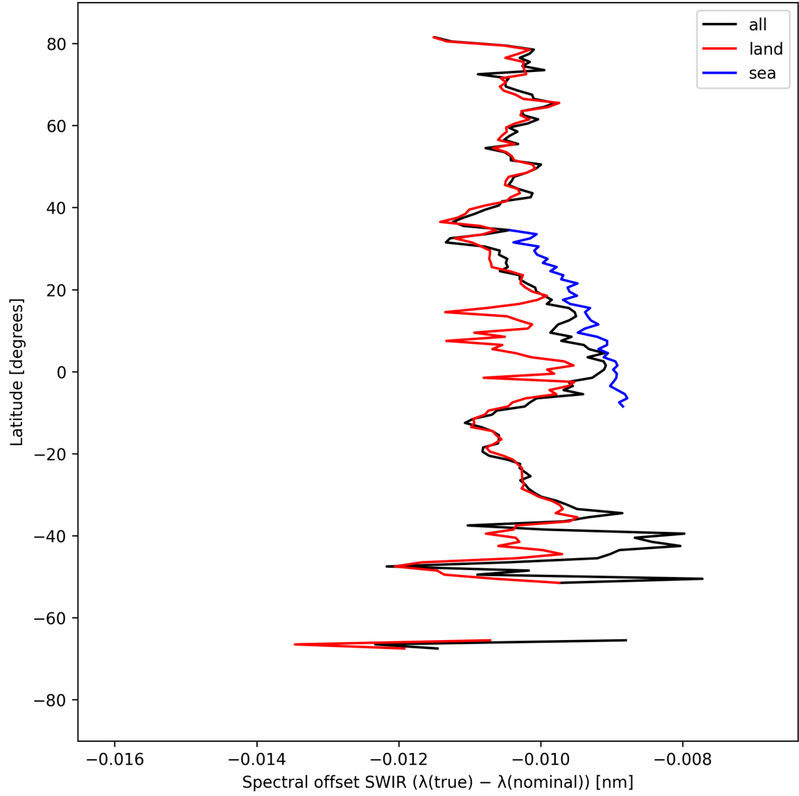
Figure 16: Zonal average of “Spectral offset SWIR ( \lambda_{\text{true}} - \lambda_{\text{nominal}} )” for 2024-09-04 to 2024-09-06.
