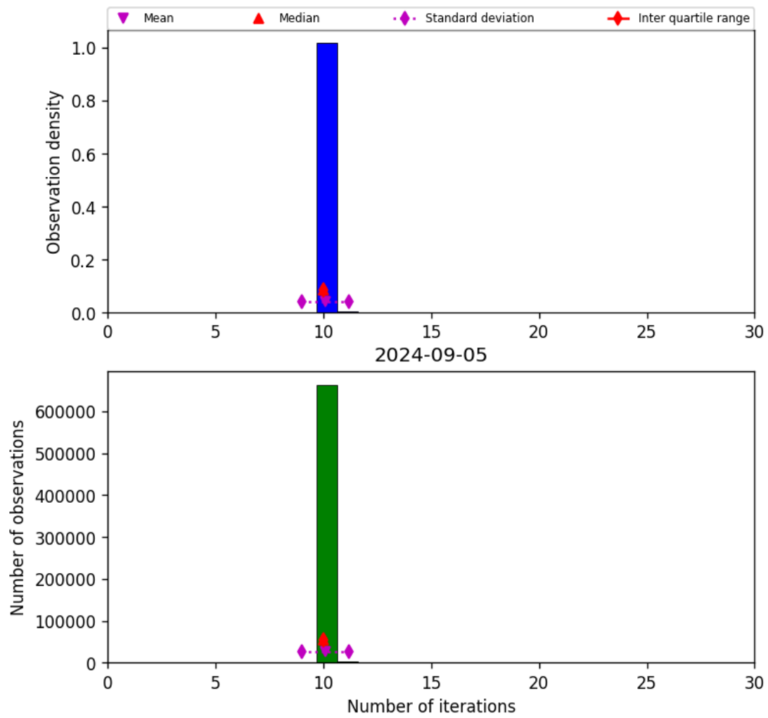
Figure 31: Histogram of “Number of iterations” for 2024-09-04 to 2024-09-06
