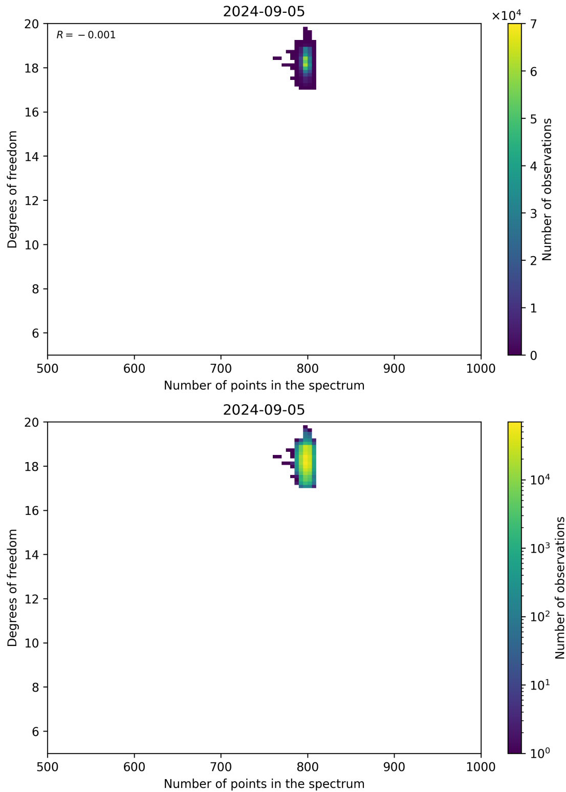
Figure 90: Scatter density plot of “Number of points in the spectrum” against “Degrees of freedom” for 2024-09-04 to 2024-09-06.
