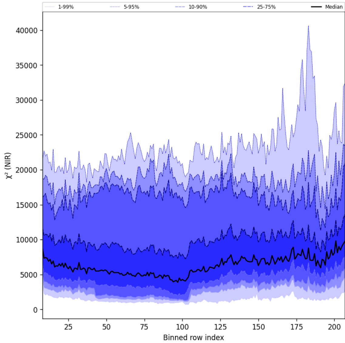
Figure 40: Along track statistics of “ \chi^2 (NIR)” for 2024-09-04 to 2024-09-06
