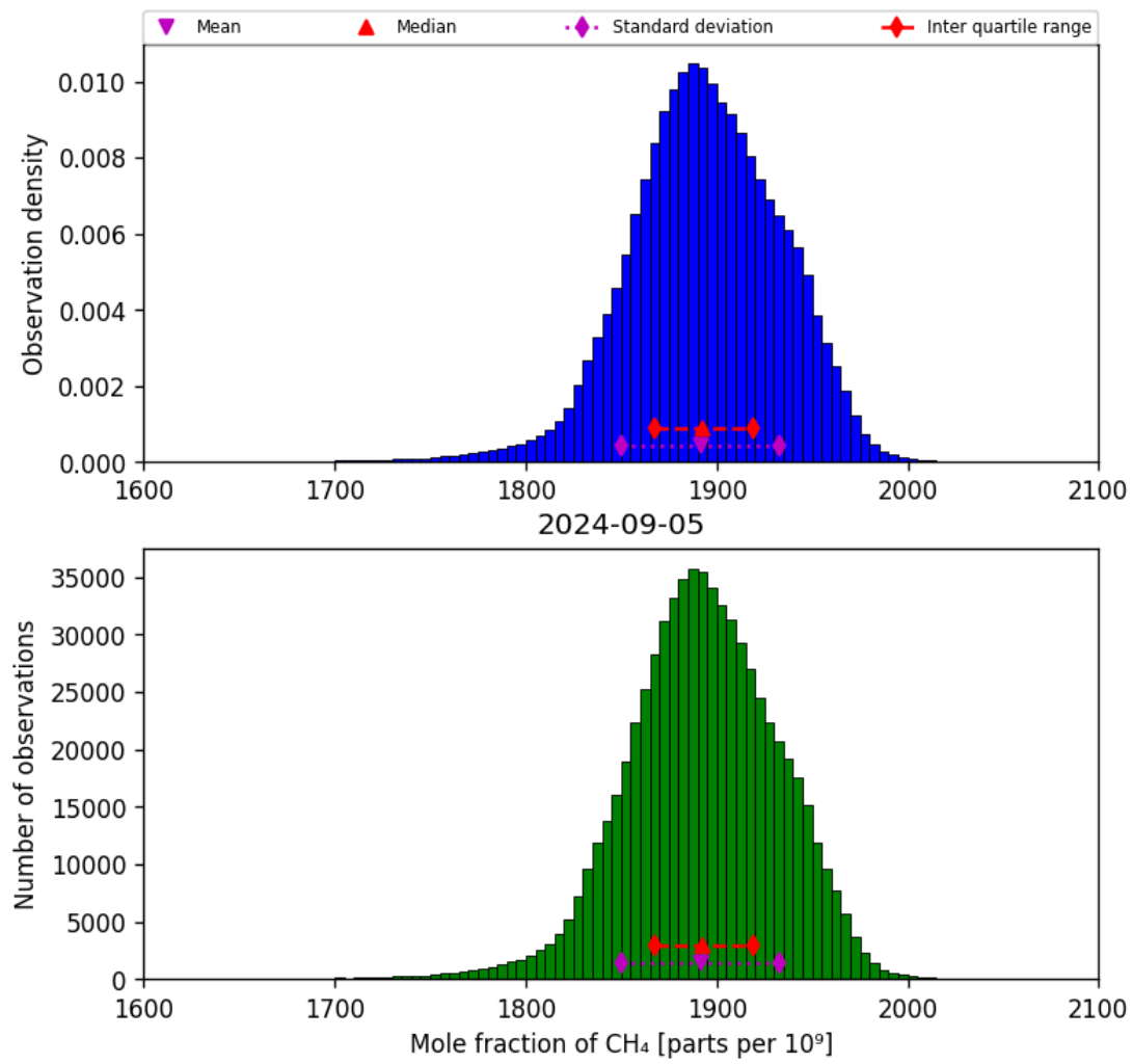
Figure 23: Histogram of “Mole fraction of CH 4 ” for 2024-09-04 to 2024-09-06
