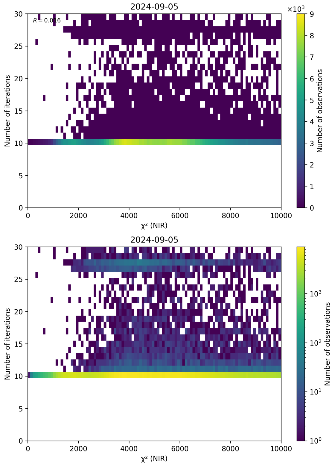
Figure 46: Scatter density plot of “ \chi^2 (NIR)” against “Number of iterations” for 2024-09-04 to 2024-09-06.
