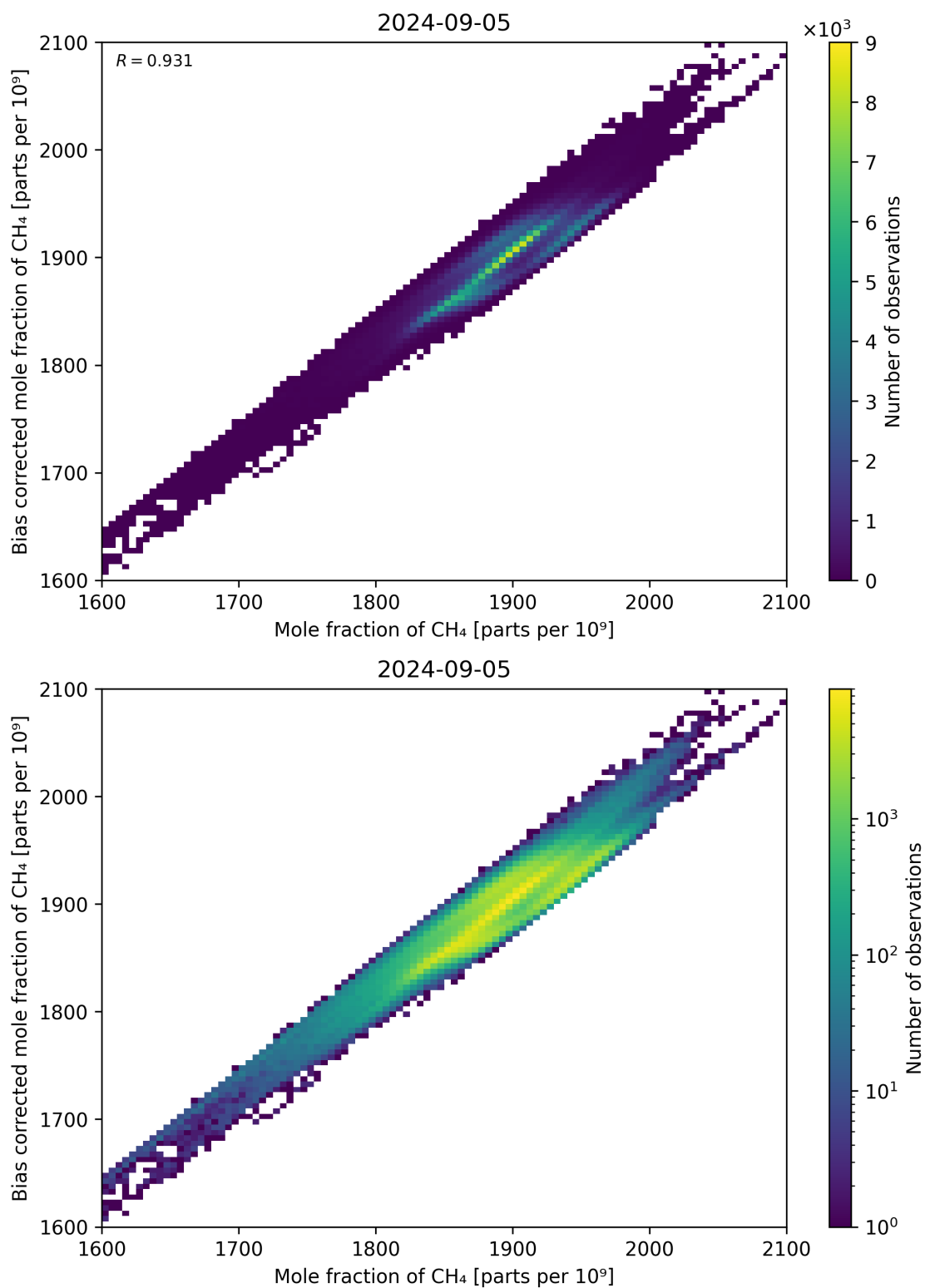
Figure 74: Scatter density plot of “Mole fraction of CH 4 ” against “Bias corrected mole fraction of CH 4 ” for 2024-09-04 to 2024-09-06.
