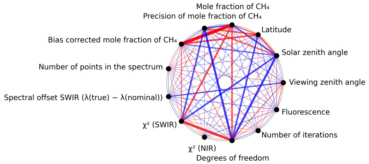
Figure 1: Map of correlation graph for 2024-09-04 to 2024-09-06.
