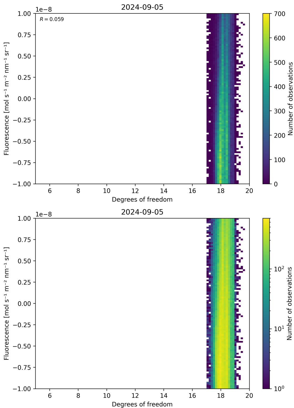
Figure 51: Scatter density plot of “Degrees of freedom” against “Fluorescence” for 2024-09-04 to 2024-09-06.
