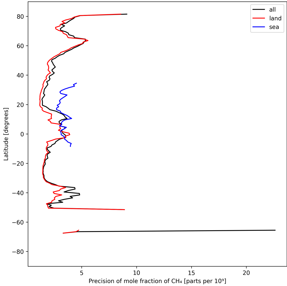
Figure 13: Zonal average of “Precision of mole fraction of CH 4 ” for 2024-09-04 to 2024-09-06.
