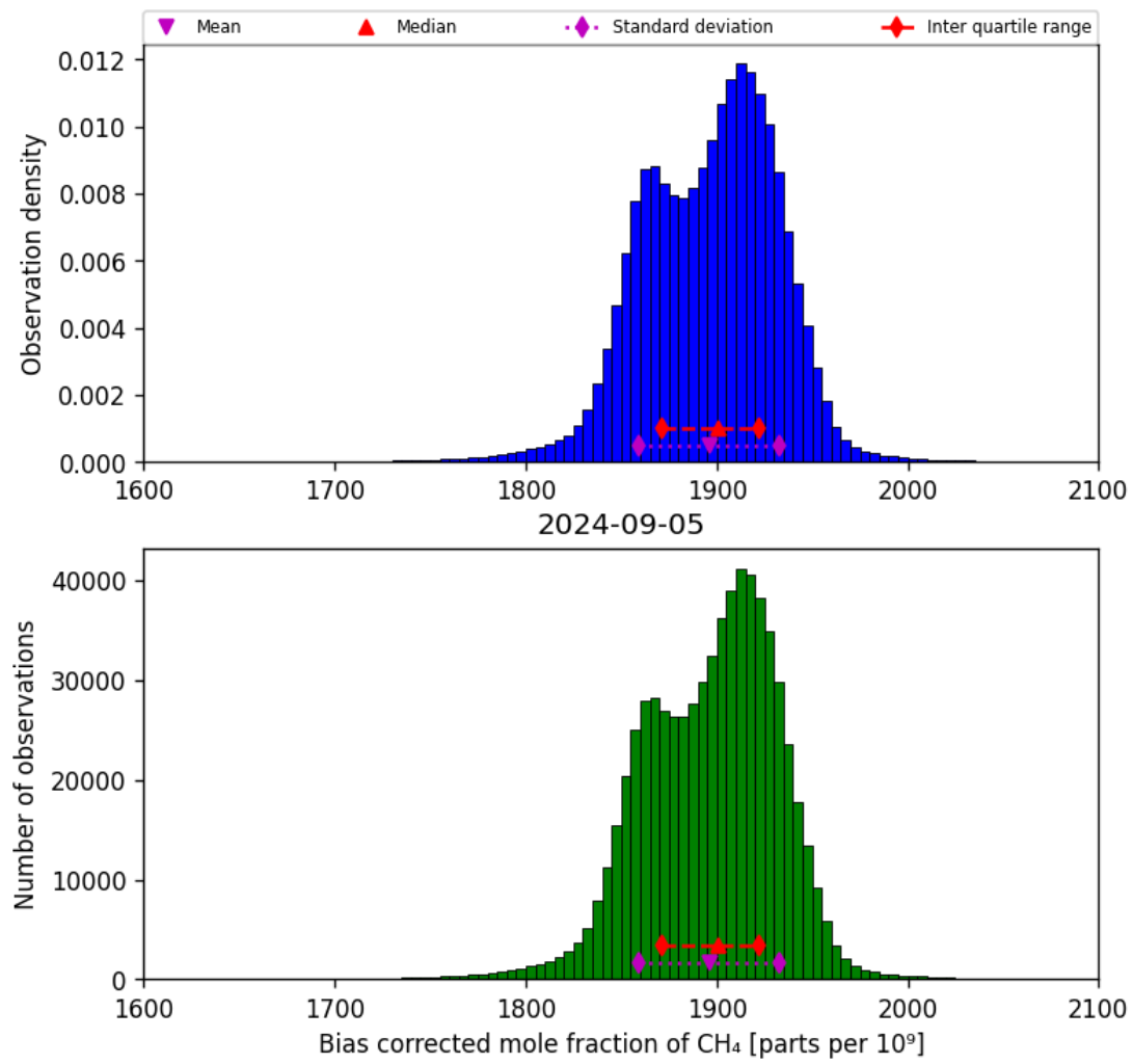
Figure 25: Histogram of “Bias corrected mole fraction of CH 4 ” for 2024-09-04 to 2024-09-06
