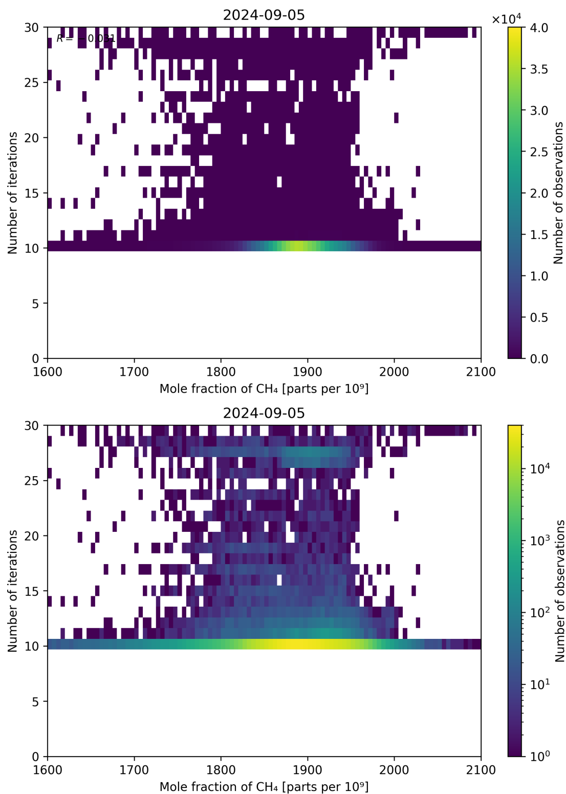
Figure 76: Scatter density plot of “Mole fraction of CH 4 ” against “Number of iterations” for 2024-09-04 to 2024-09-06.
