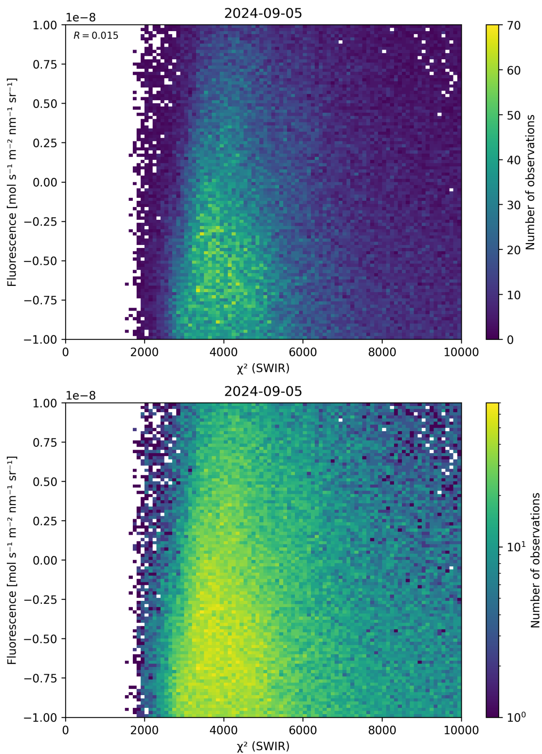
Figure 49: Scatter density plot of “ \chi^2 (SWIR)” against “Fluorescence” for 2024-09-04 to 2024-09-06.
