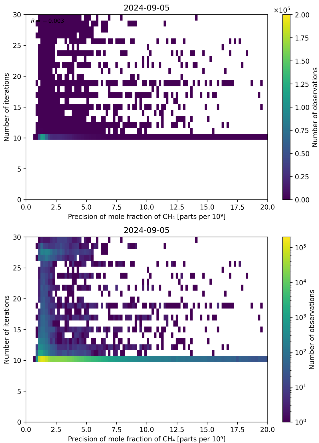
Figure 83: Scatter density plot of “Precision of mole fraction of CH 4 ” against “Number of iterations” for 2024-09-04 to 2024-09-06.
