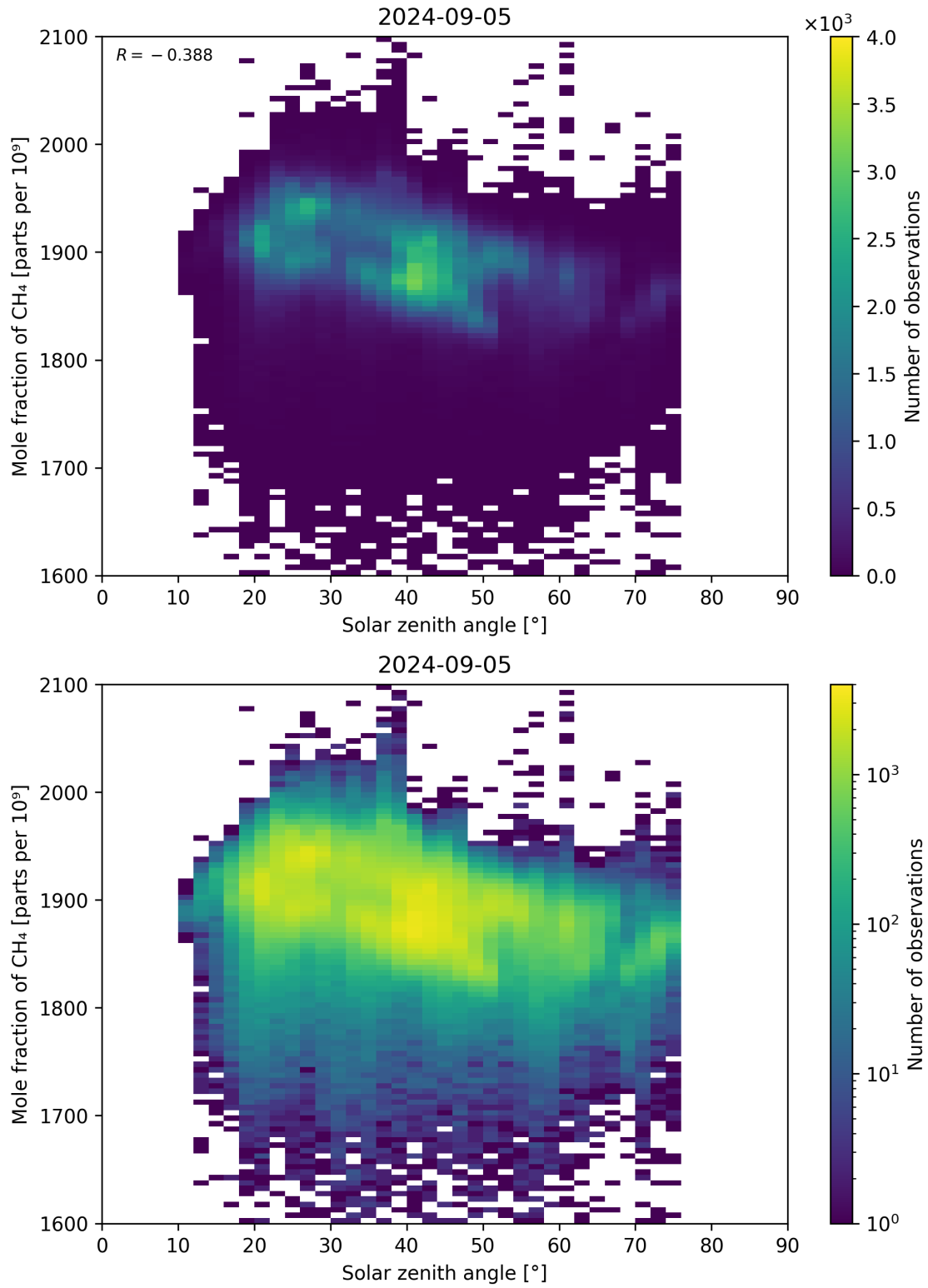
Figure 99: Scatter density plot of “Solar zenith angle” against “Mole fraction of \text{CH}_4 ” for 2024-09-04 to 2024-09-06.
