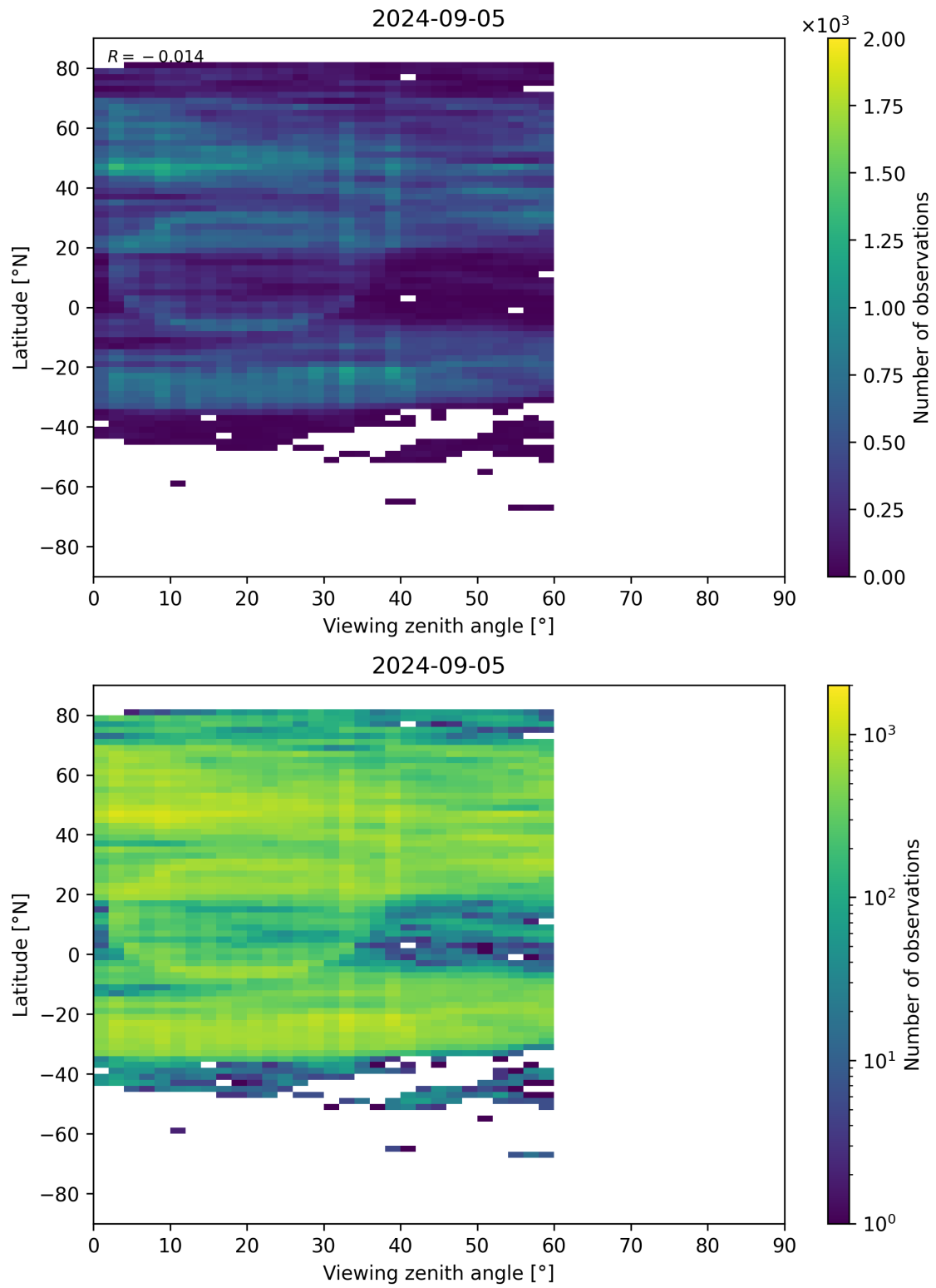
Figure 109: Scatter density plot of “Viewing zenith angle” against “Latitude” for 2024-09-04 to 2024-09-06.
