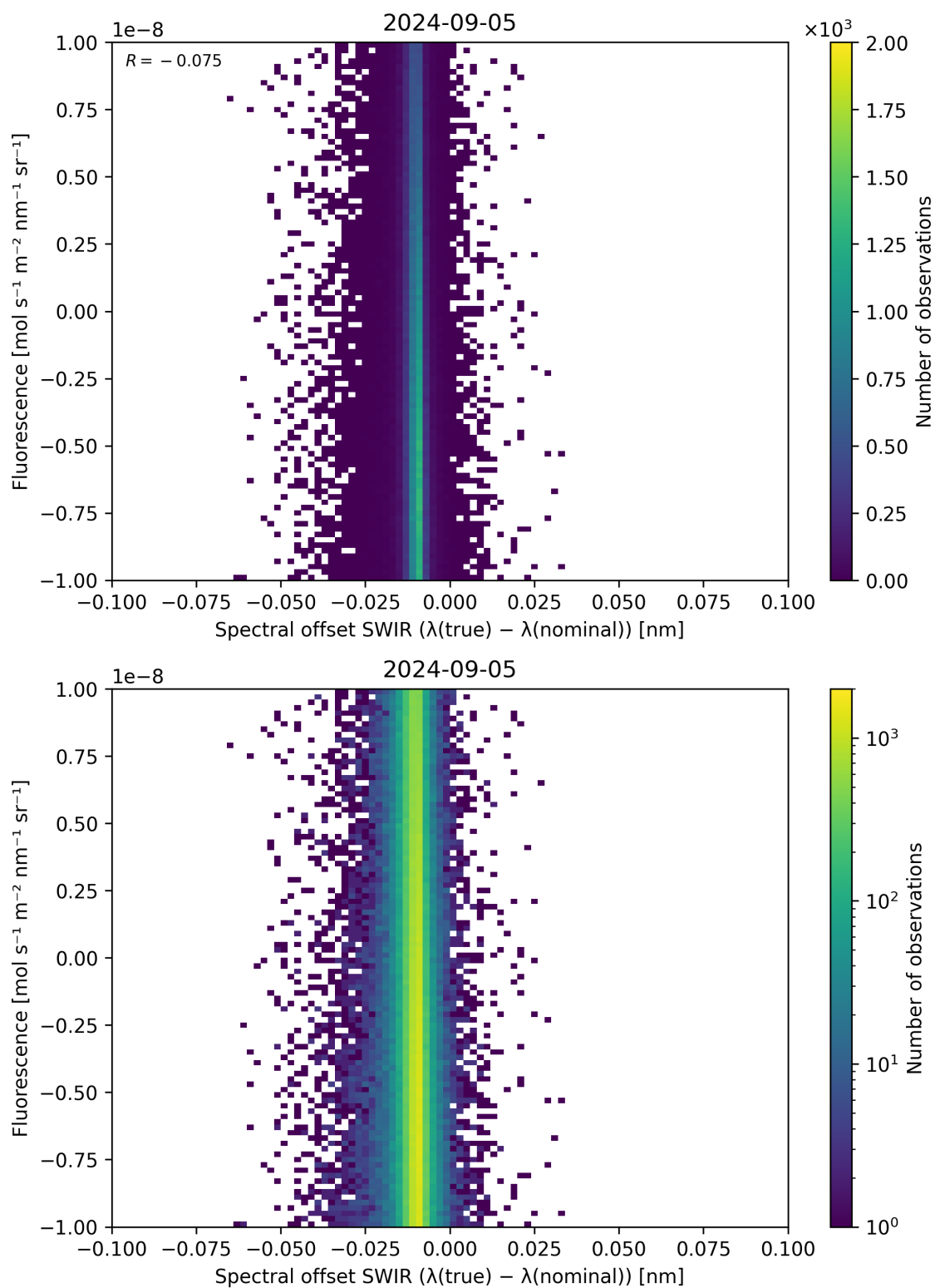
Figure 120: Scatter density plot of “Spectral offset SWIR ( \lambda_{\text{true}} - \lambda_{\text{nominal}} )” against “Fluorescence” for 2024-09-04 to 2024-09-06.
