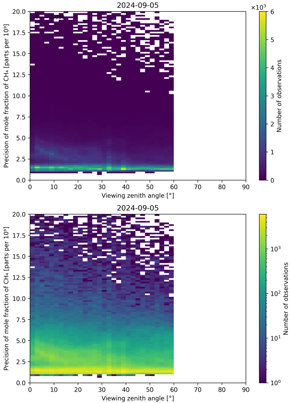
Figure 112: Scatter density plot of “Viewing zenith angle” against “Precision of mole fraction of CH 4 ” for 2024-09-04 to 2024-09-06.
