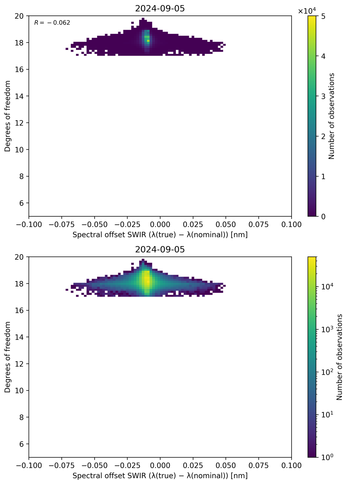
Figure 119: Scatter density plot of “Spectral offset SWIR ( \lambda_{\text{true}} - \lambda_{\text{nominal}} )” against “Degrees of freedom” for 2024-09-04 to 2024-09-06.
