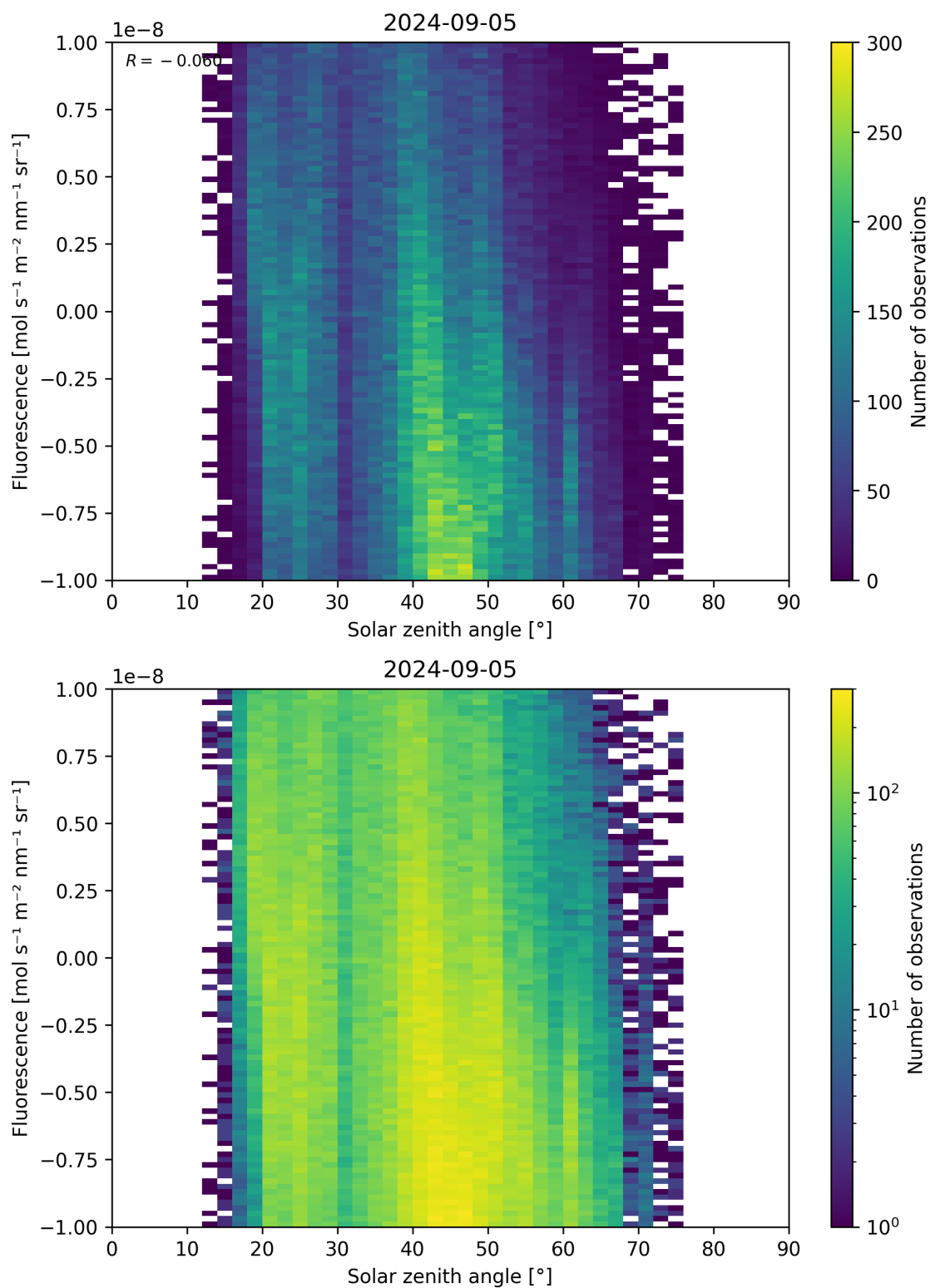
Figure 97: Scatter density plot of “Solar zenith angle” against “Fluorescence” for 2024-09-04 to 2024-09-06.
