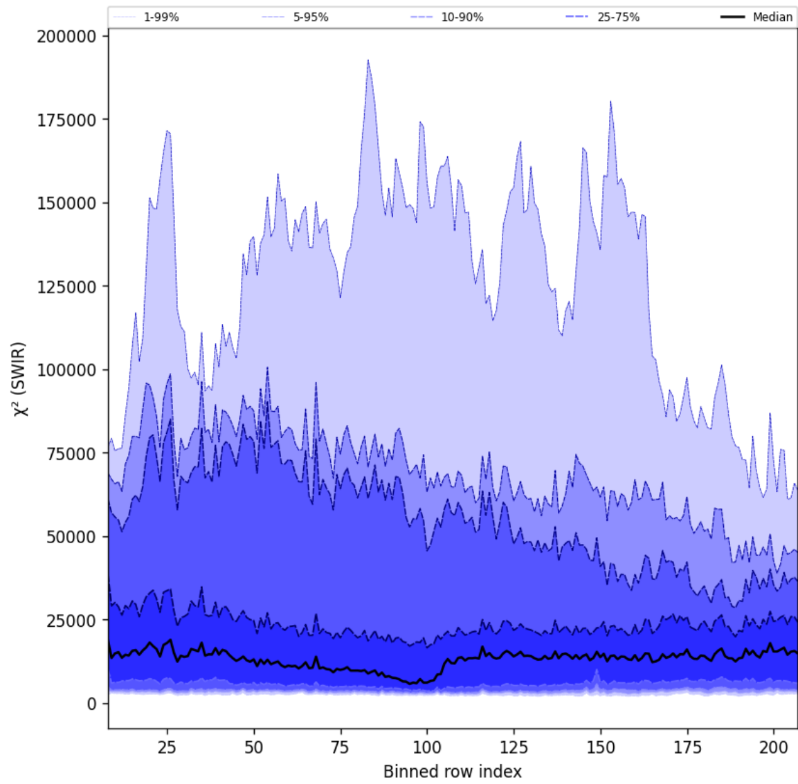
Figure 39: Along track statistics of “ \chi^2 (SWIR)” for 2024-09-04 to 2024-09-06
