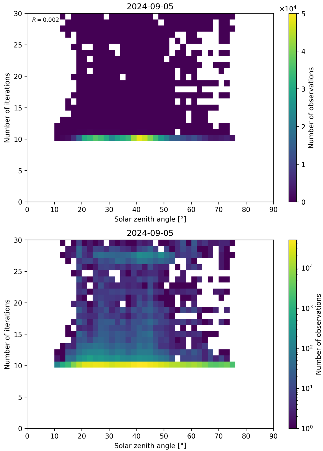
Figure 102: Scatter density plot of “Solar zenith angle” against “Number of iterations” for 2024-09-04 to 2024-09-06.
