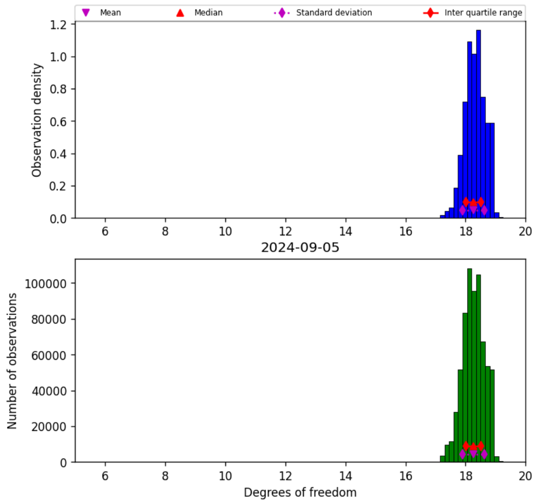
Figure 30: Histogram of “Degrees of freedom” for 2024-09-04 to 2024-09-06
