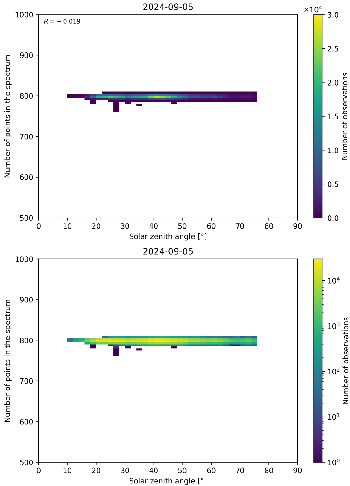
Figure 103: Scatter density plot of “Solar zenith angle” against “Number of points in the spectrum” for 2024-09-04 to 2024-09-06.
