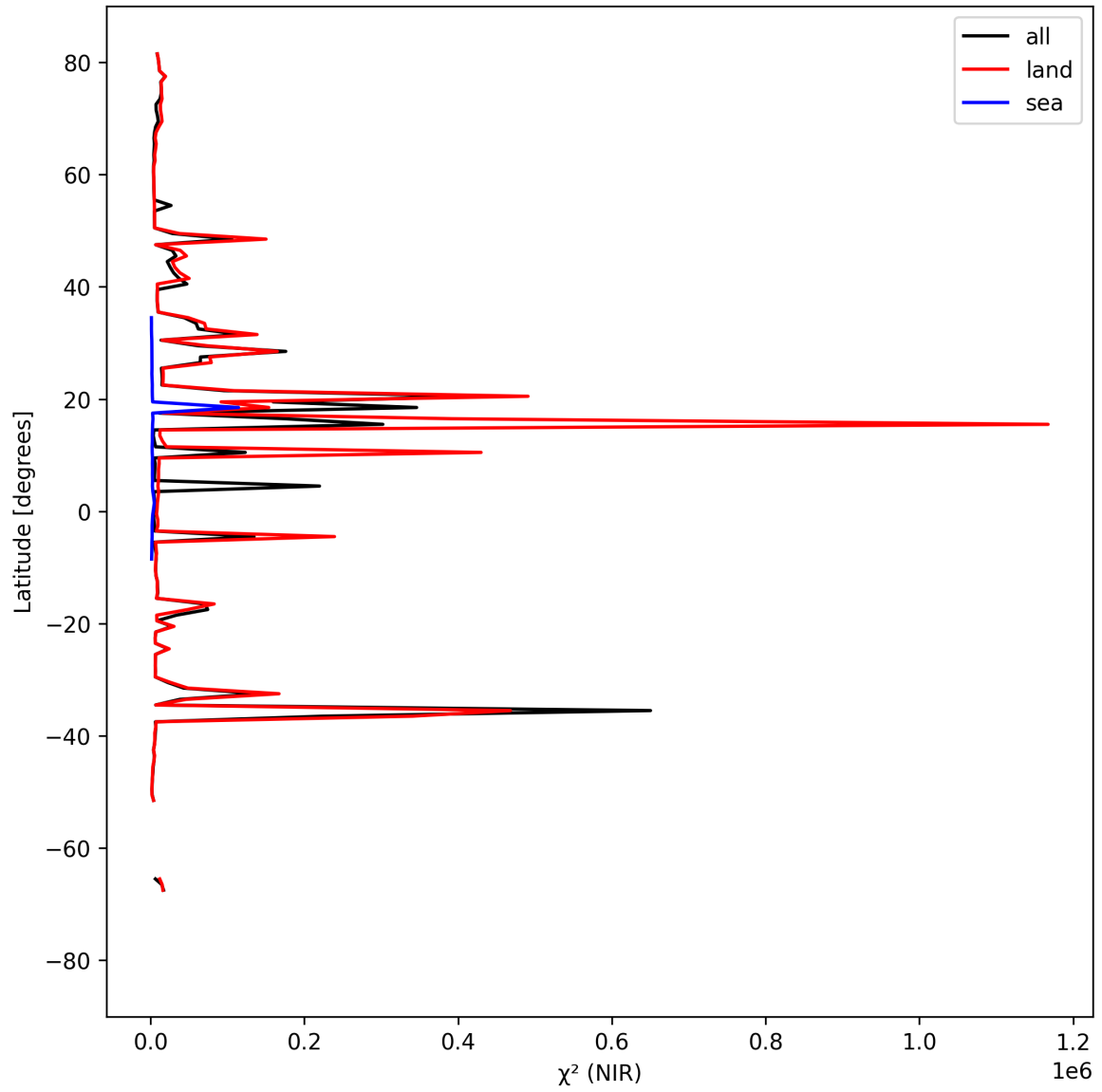
Figure 18: Zonal average of “ \chi^2 (NIR)” for 2024-09-04 to 2024-09-06.
