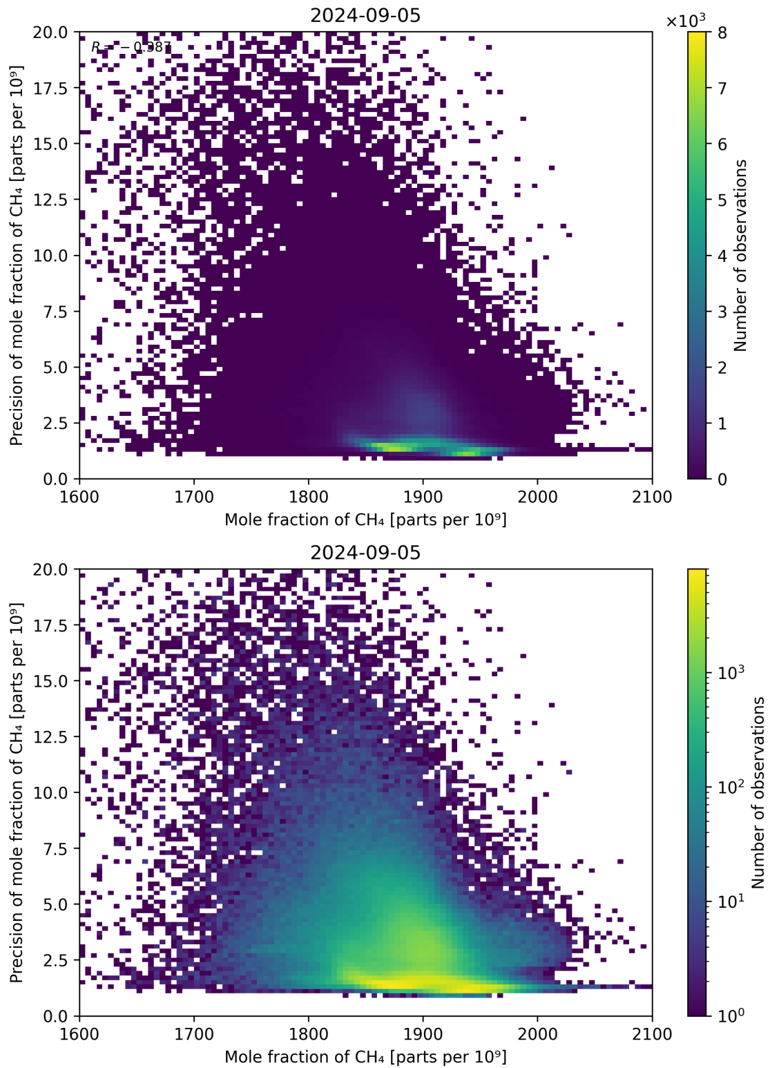
Figure 75: Scatter density plot of “Mole fraction of CH 4 ” against “Precision of mole fraction of CH 4 ” for 2024-09-04 to 2024-09-06.
