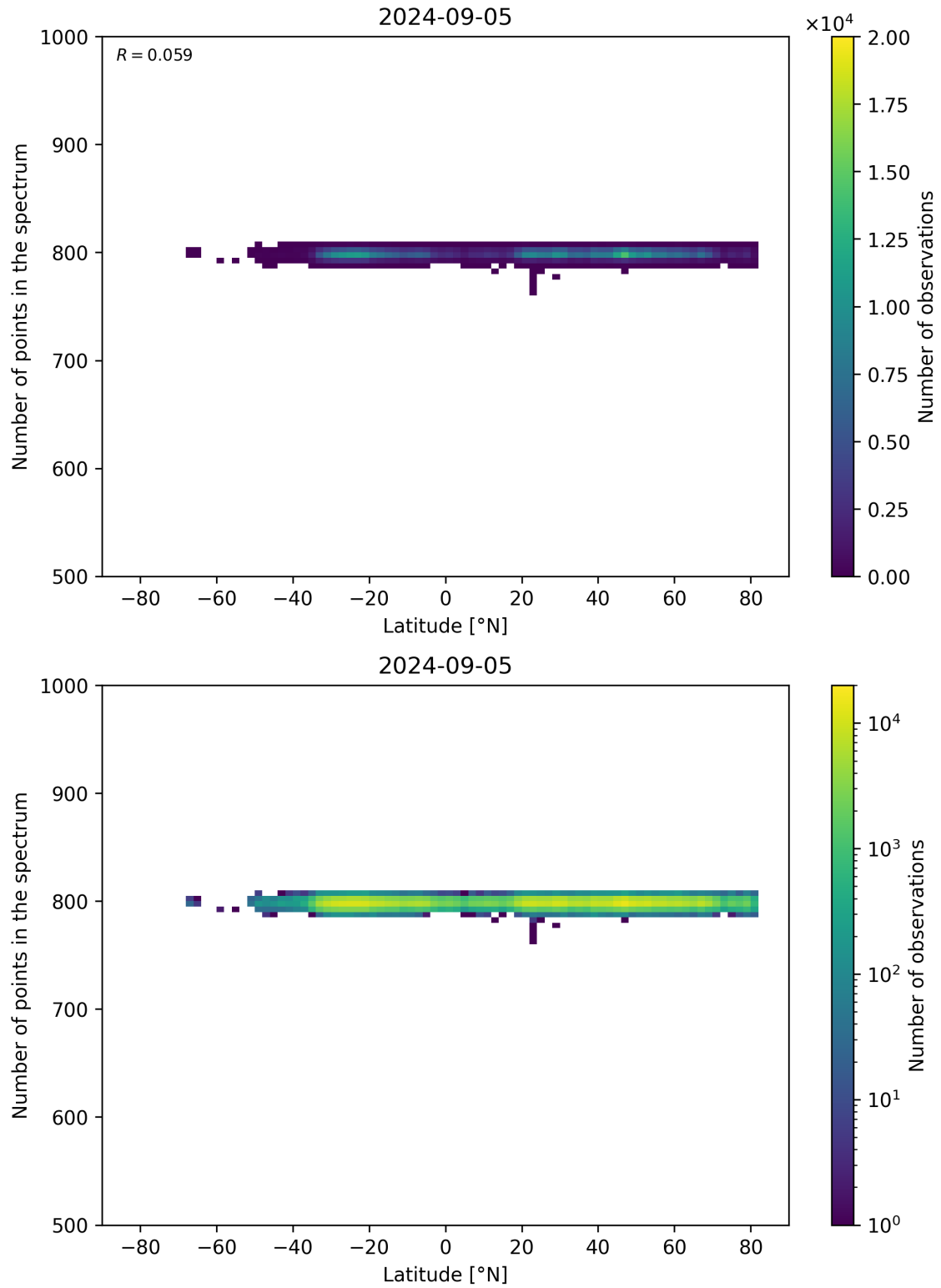
Figure 61: Scatter density plot of “Latitude” against “Number of points in the spectrum” for 2024-09-04 to 2024-09-06.
