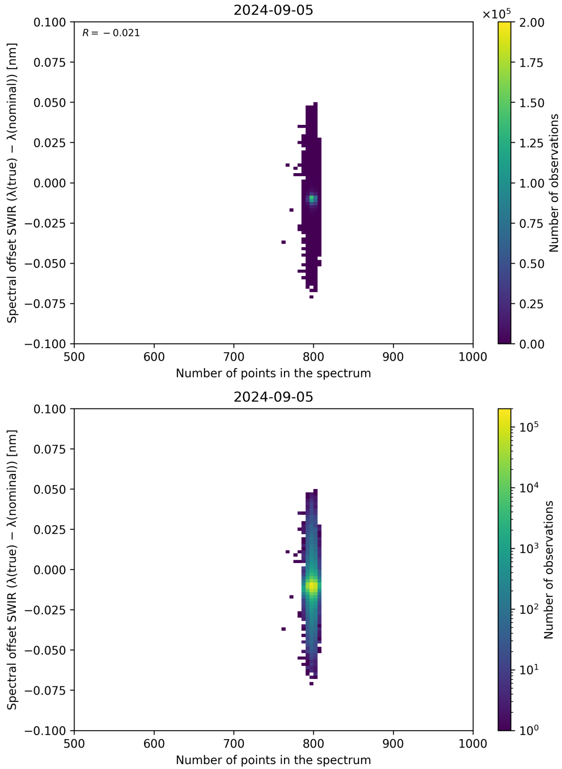
Figure 93: Scatter density plot of “Number of points in the spectrum” against “Spectral offset SWIR ( \lambda_{\text{true}} - \lambda_{\text{nominal}} )” for 2024-09-04 to 2024-09-06.
