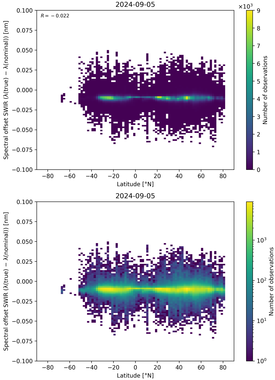
Figure 62: Scatter density plot of “Latitude” against “Spectral offset SWIR ( \lambda_{\text{true}} - \lambda_{\text{nominal}} )” for 2024-09-04 to 2024-09-06.
