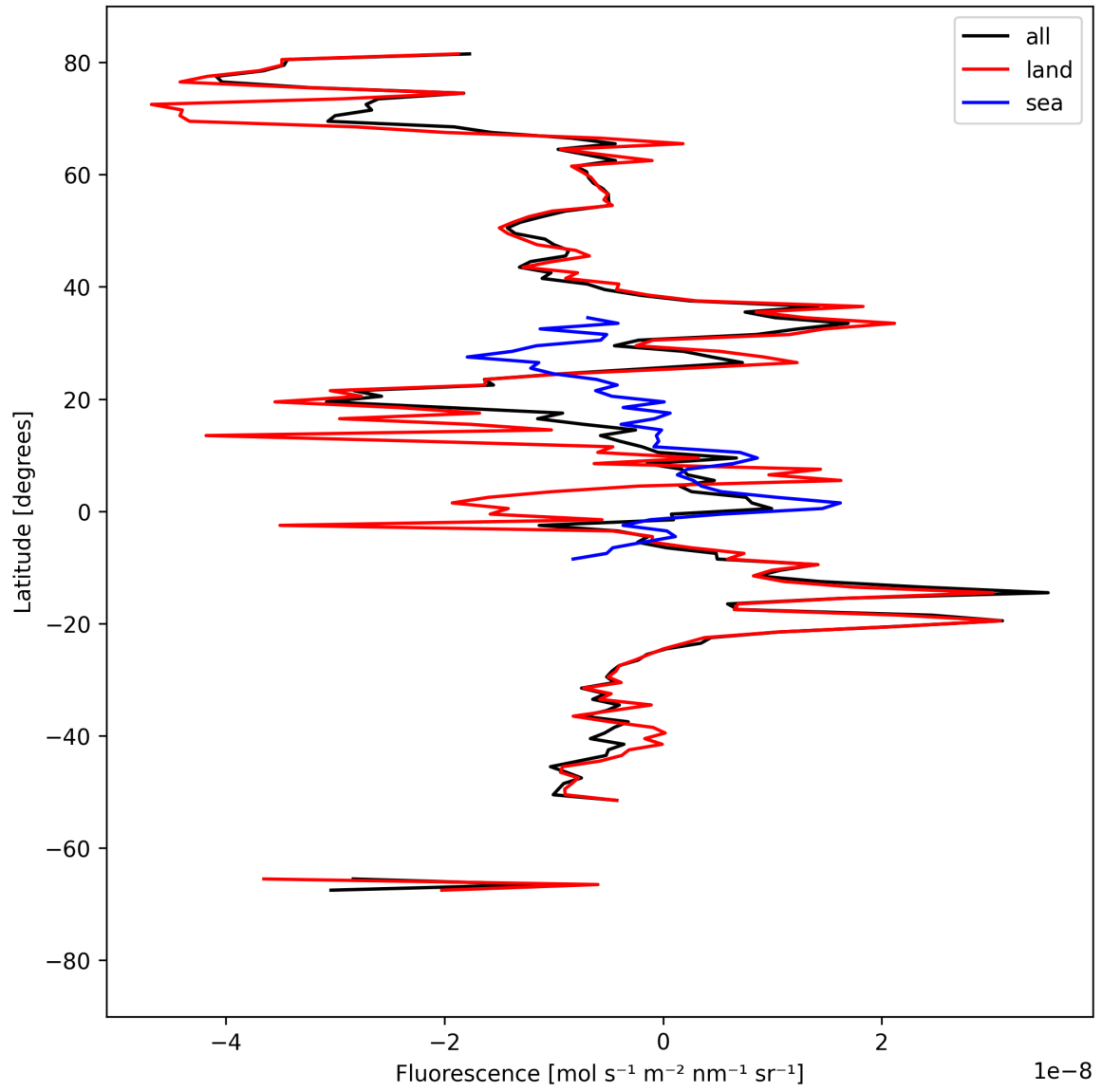
Figure 21: Zonal average of “Fluorescence” for 2024-09-04 to 2024-09-06.
