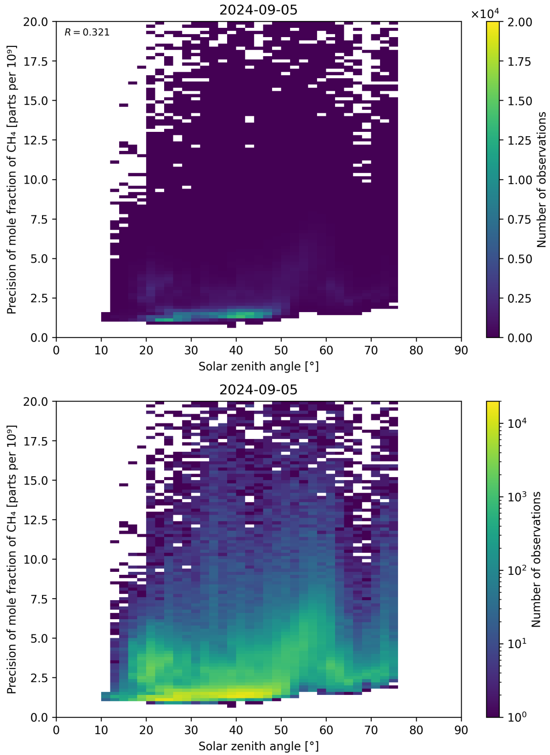
Figure 101: Scatter density plot of “Solar zenith angle” against “Precision of mole fraction of CH 4 ” for 2024-09-04 to 2024-09-06.
