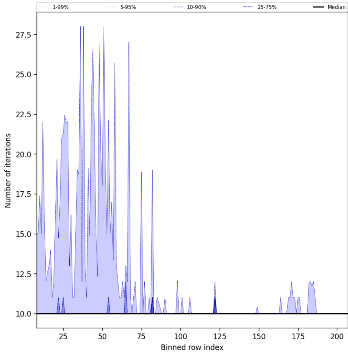
Figure 42: Along track statistics of “Number of iterations” for 2024-09-04 to 2024-09-06
