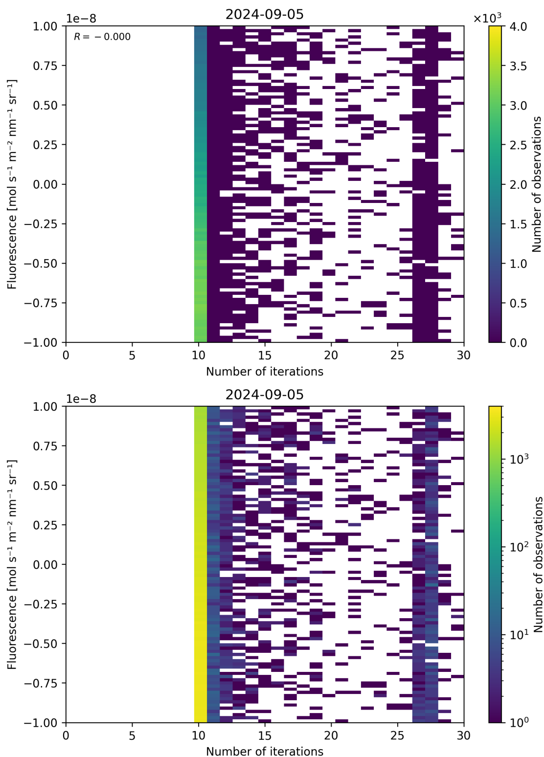
Figure 87: Scatter density plot of “Number of iterations” against “Fluorescence” for 2024-09-04 to 2024-09-06.
