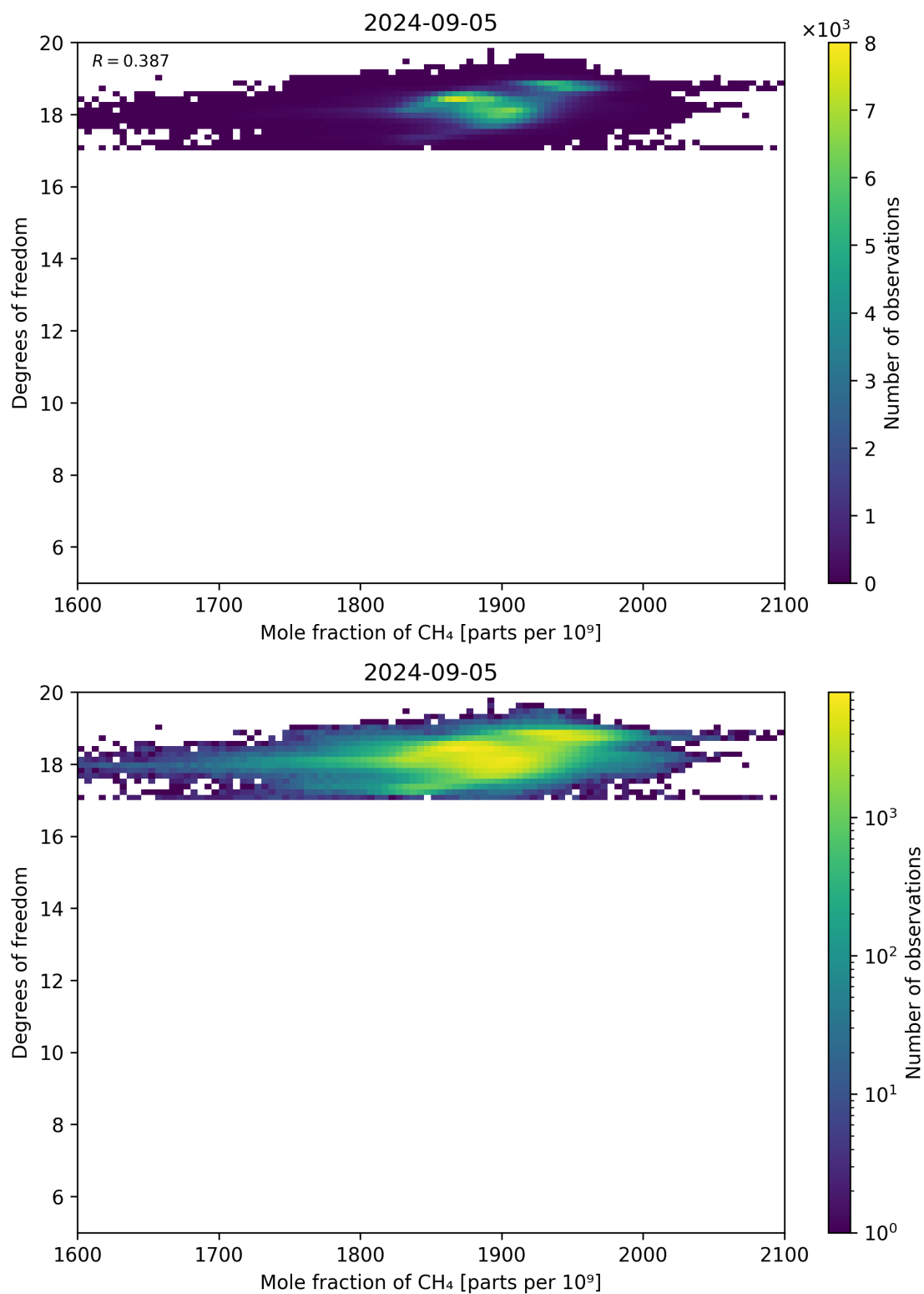
Figure 72: Scatter density plot of “Mole fraction of CH 4 ” against “Degrees of freedom” for 2024-09-04 to 2024-09-06.
