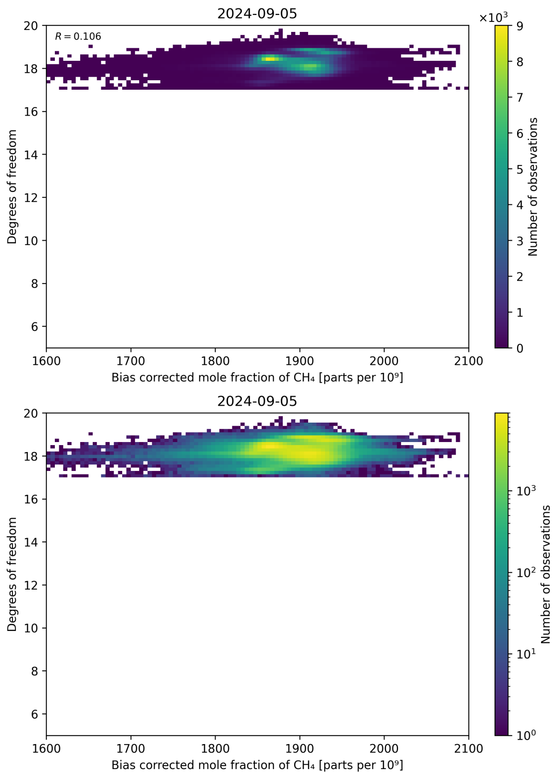
Figure 65: Scatter density plot of “Bias corrected mole fraction of CH 4 ” against “Degrees of freedom” for 2024-09-04 to 2024-09-06.
