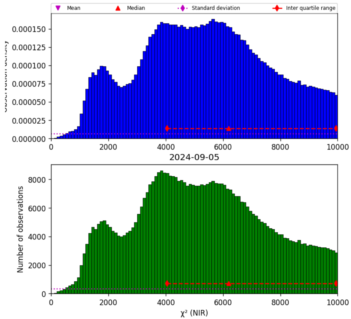
Figure 29: Histogram of “ \chi^2 (NIR)” for 2024-09-04 to 2024-09-06
