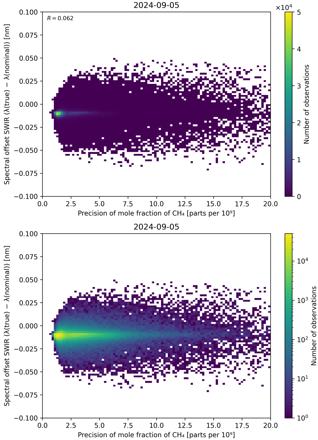
Figure 85: Scatter density plot of “Precision of mole fraction of CH 4 ” against “Spectral offset SWIR ( \lambda_{\text{true}} - \lambda_{\text{nominal}} )” for 2024-09-04 to 2024-09-06.
