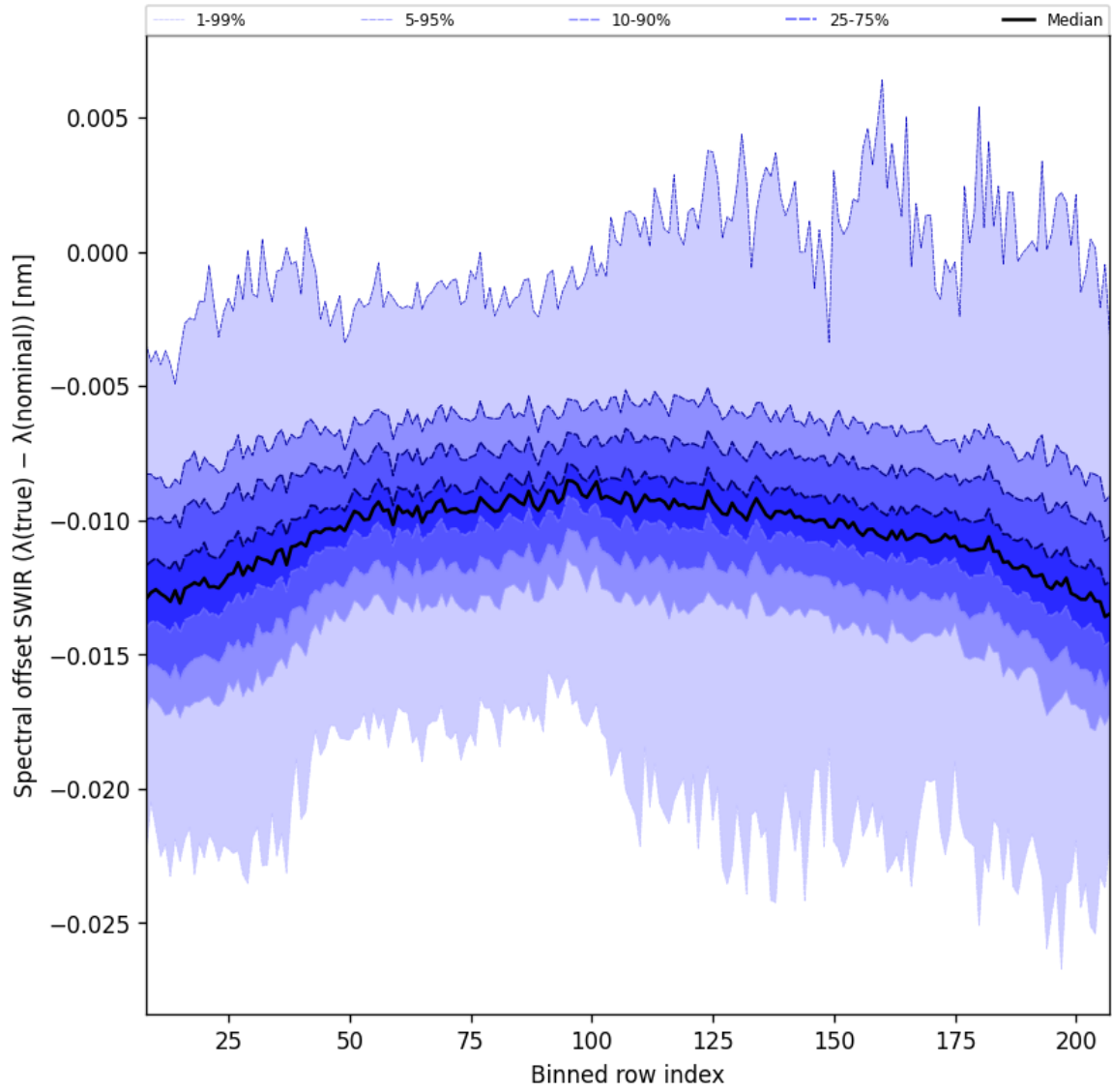
Figure 38: Along track statistics of “Spectral offset SWIR ( \lambda_{\text{true}} - \lambda_{\text{nominal}} )” for 2024-09-04 to 2024-09-06
