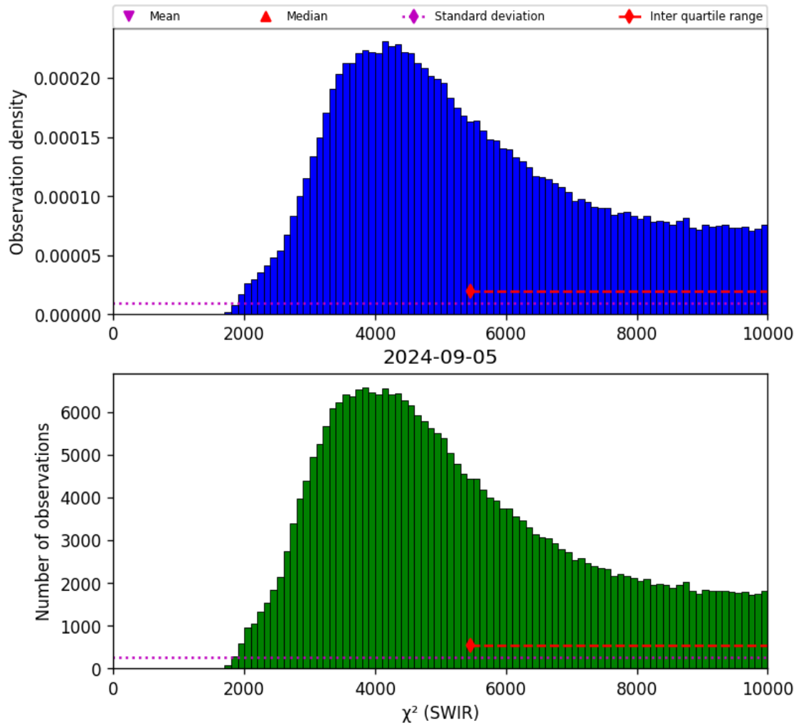
Figure 28: Histogram of “ \chi^2 (SWIR)” for 2024-09-04 to 2024-09-06
