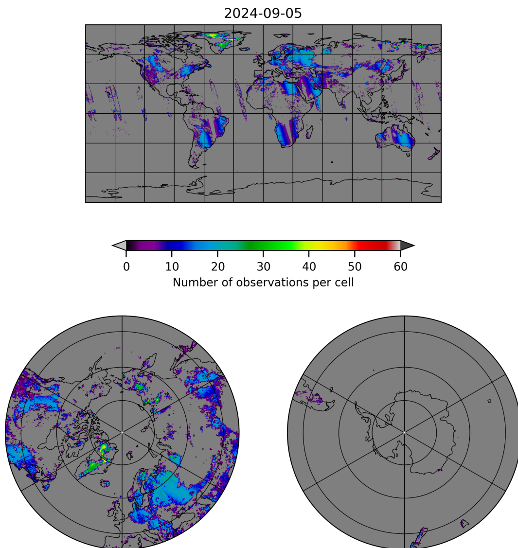
Figure 10: Map of the number of observations for 2024-09-04 to 2024-09-06
