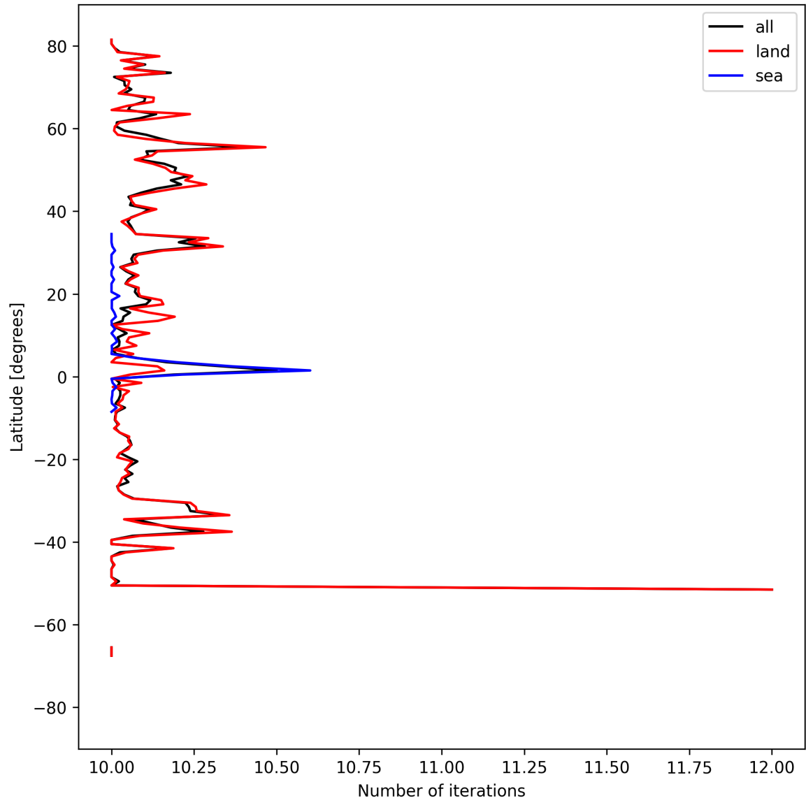
Figure 20: Zonal average of “Number of iterations” for 2024-09-04 to 2024-09-06.
