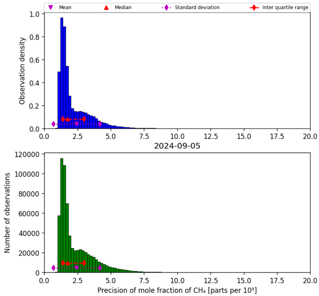
Figure 24: Histogram of “Precision of mole fraction of CH 4 ” for 2024-09-04 to 2024-09-06
