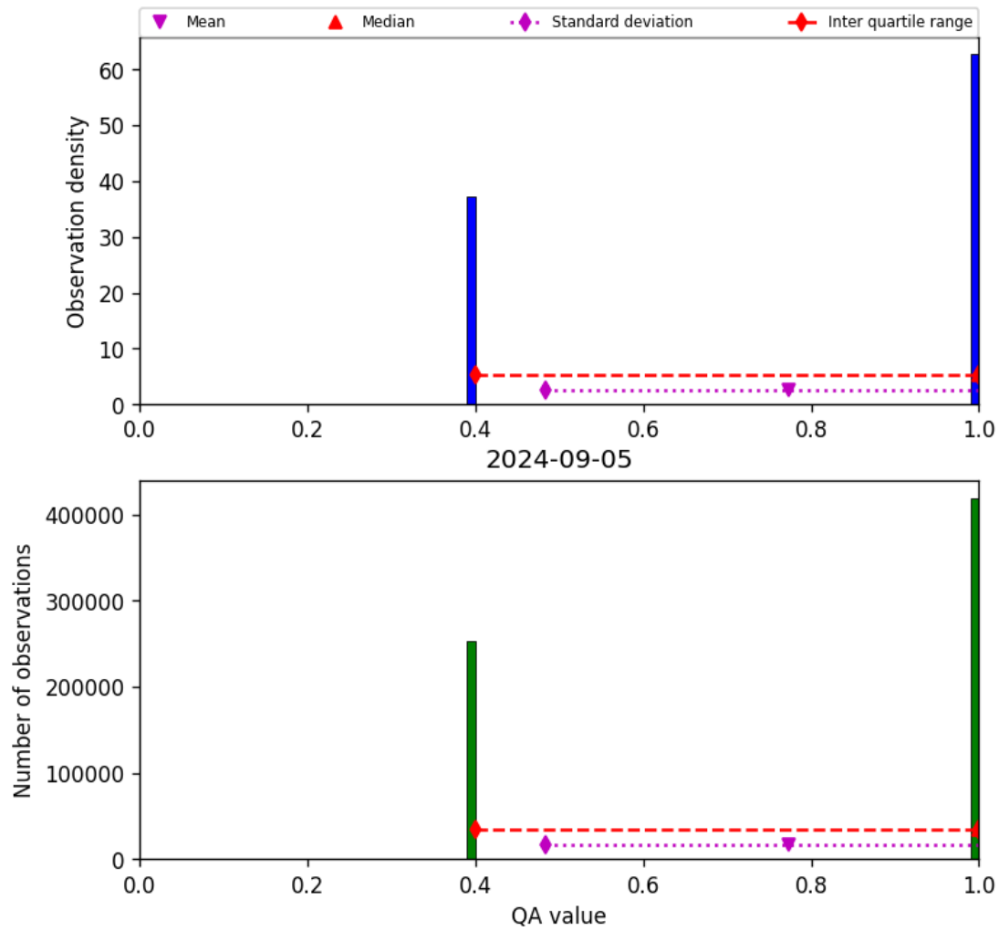
Figure 22: Histogram of “QA value” for 2024-09-04 to 2024-09-06
