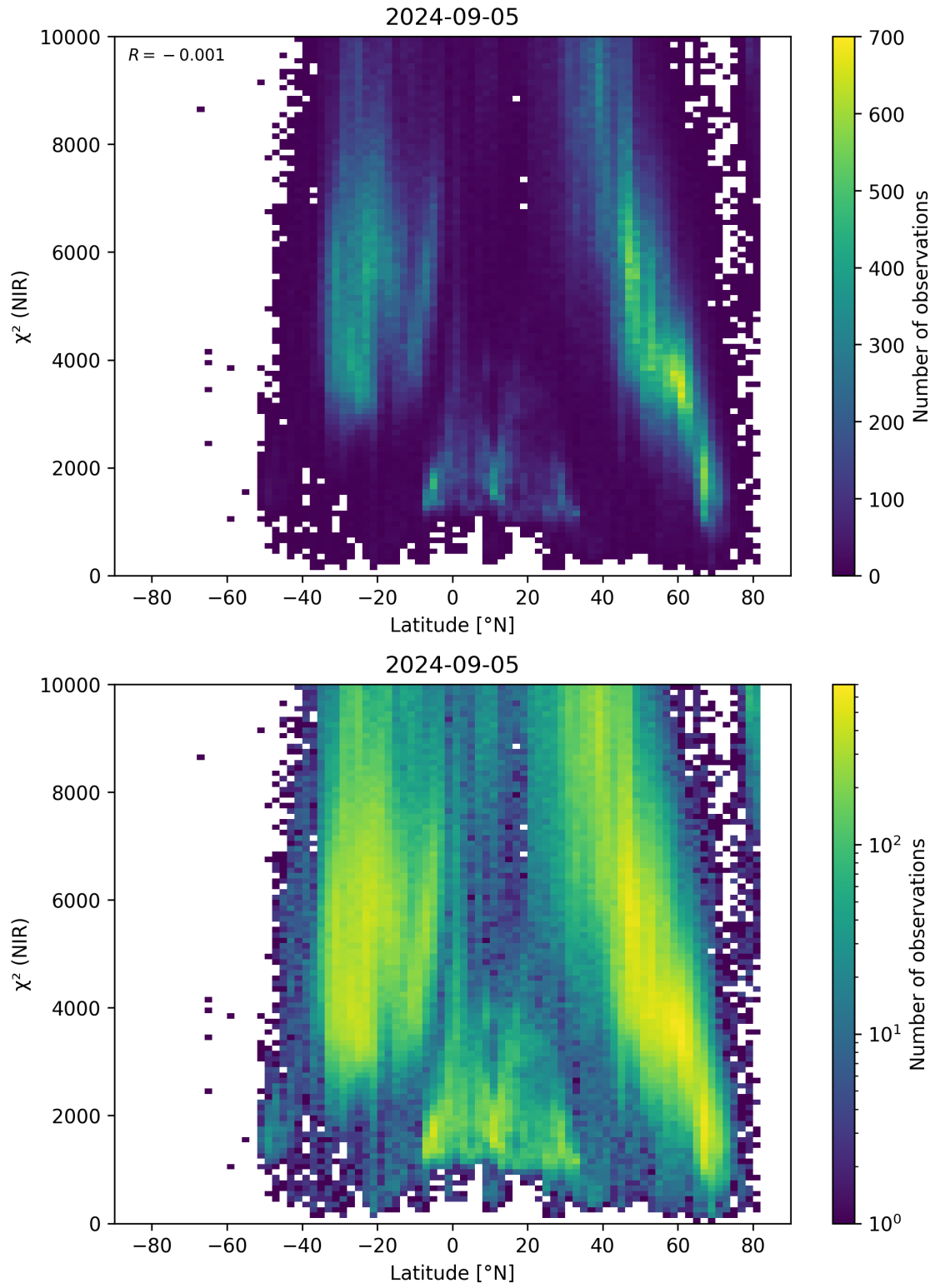
Figure 53: Scatter density plot of “Latitude” against “ \chi^2 (NIR)” for 2024-09-04 to 2024-09-06.
