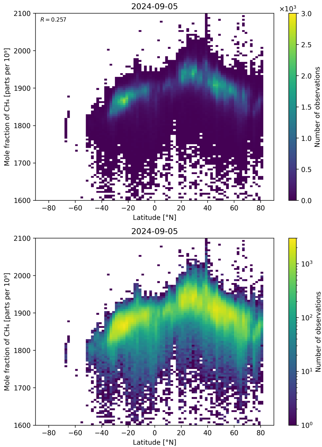
Figure 57: Scatter density plot of “Latitude” against “Mole fraction of CH 4 ” for 2024-09-04 to 2024-09-06.
