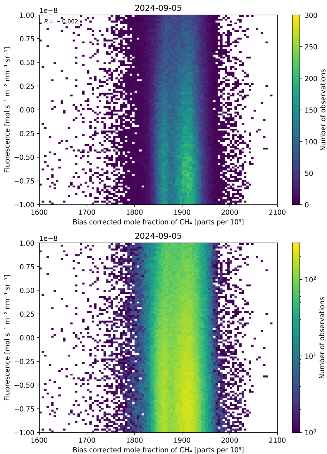
Figure 66: Scatter density plot of “Bias corrected mole fraction of \text{CH}_4 ” against “Fluorescence” for 2024-09-04 to 2024-09-06.
