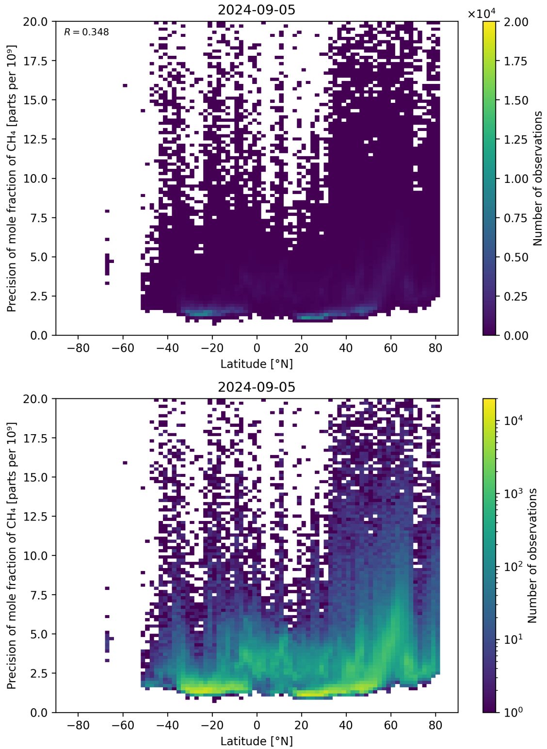
Figure 59: Scatter density plot of “Latitude” against “Precision of mole fraction of \text{CH}_4 ” for 2024-09-04 to 2024-09-06.
