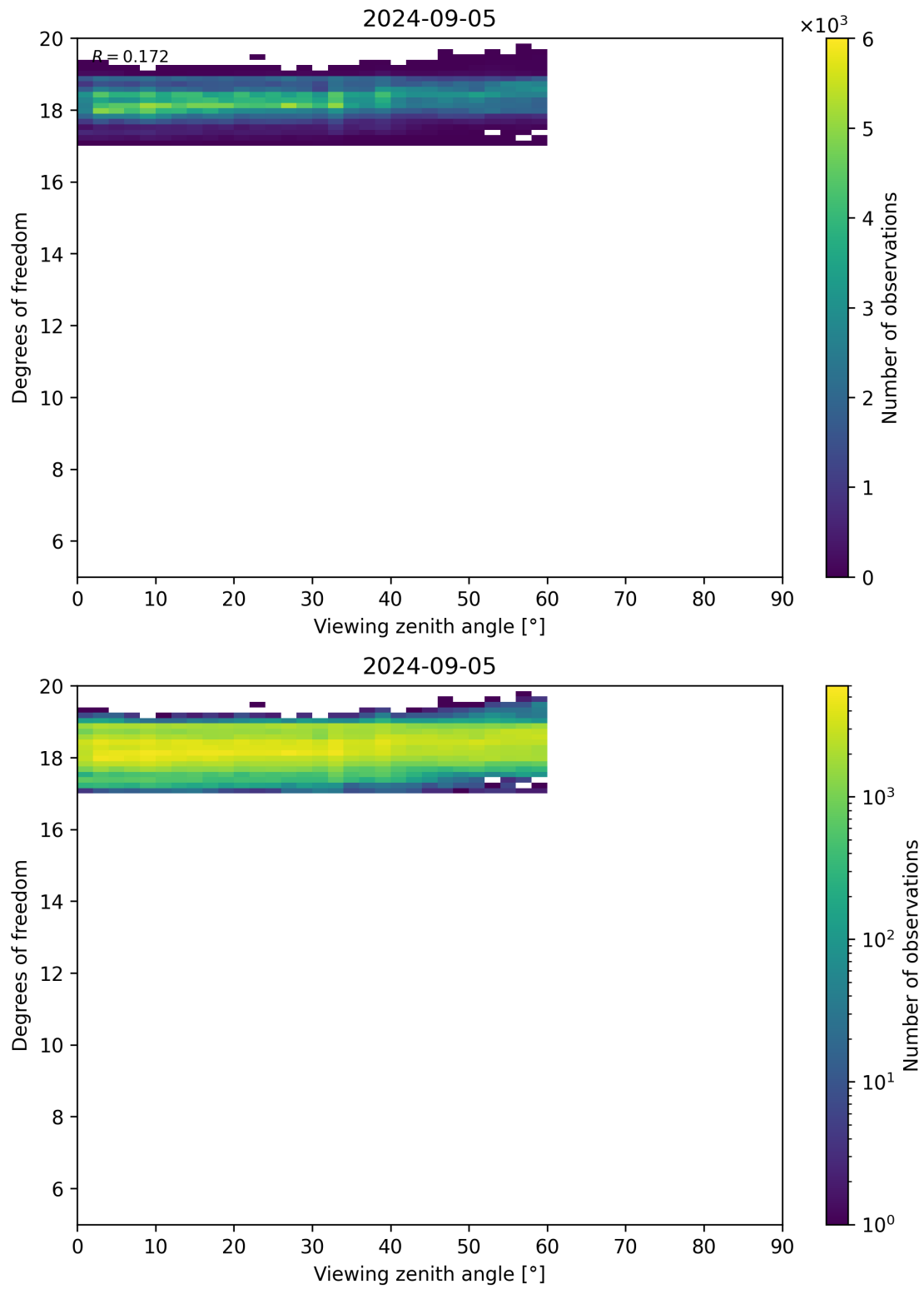
Figure 107: Scatter density plot of “Viewing zenith angle” against “Degrees of freedom” for 2024-09-04 to 2024-09-06.
