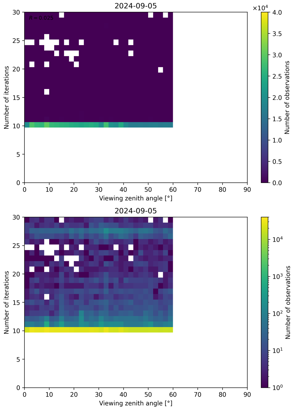
Figure 113: Scatter density plot of “Viewing zenith angle” against “Number of iterations” for 2024-09-04 to 2024-09-06.
