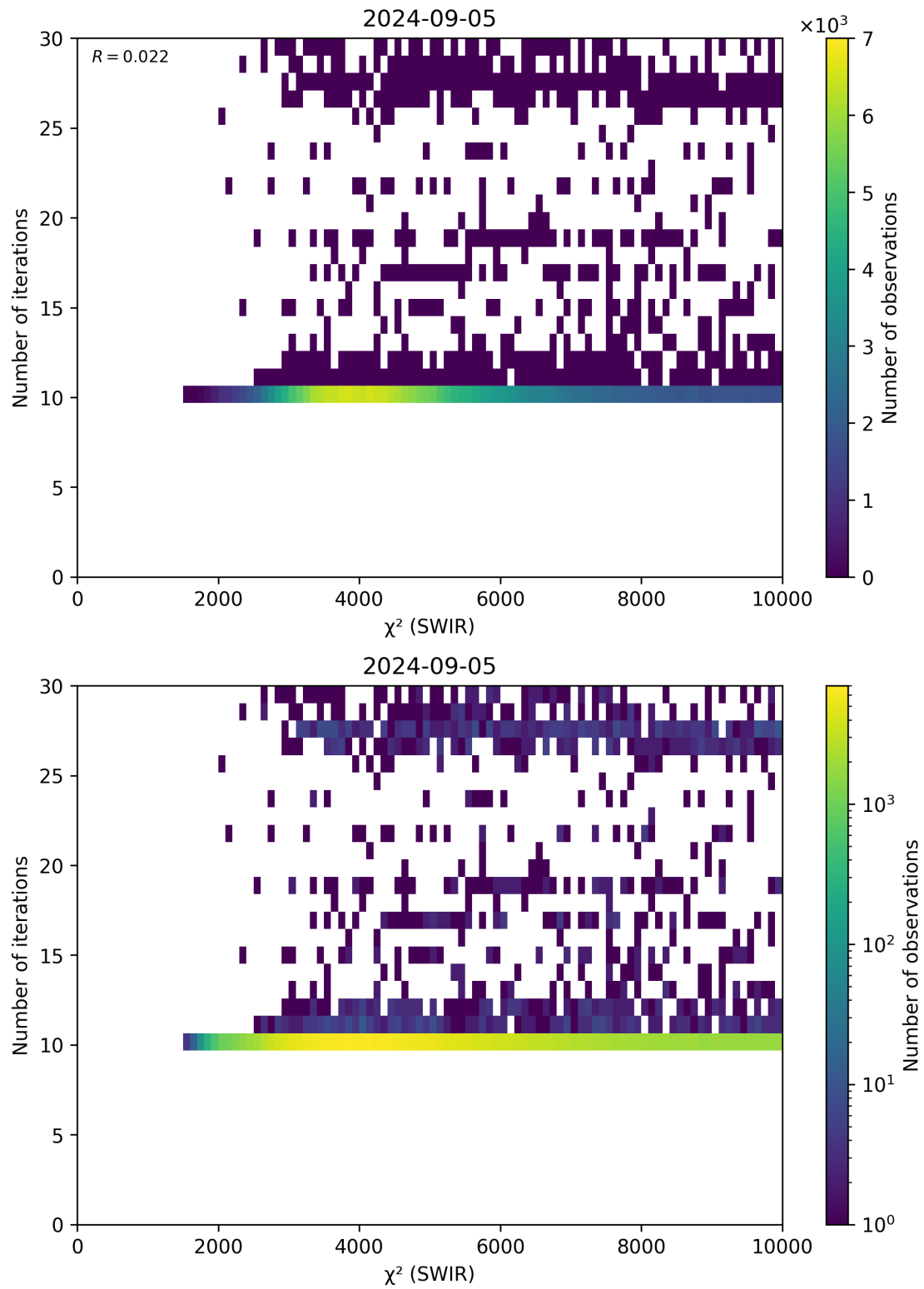
Figure 50: Scatter density plot of “ \chi^2 (SWIR)” against “Number of iterations” for 2024-09-04 to 2024-09-06.
