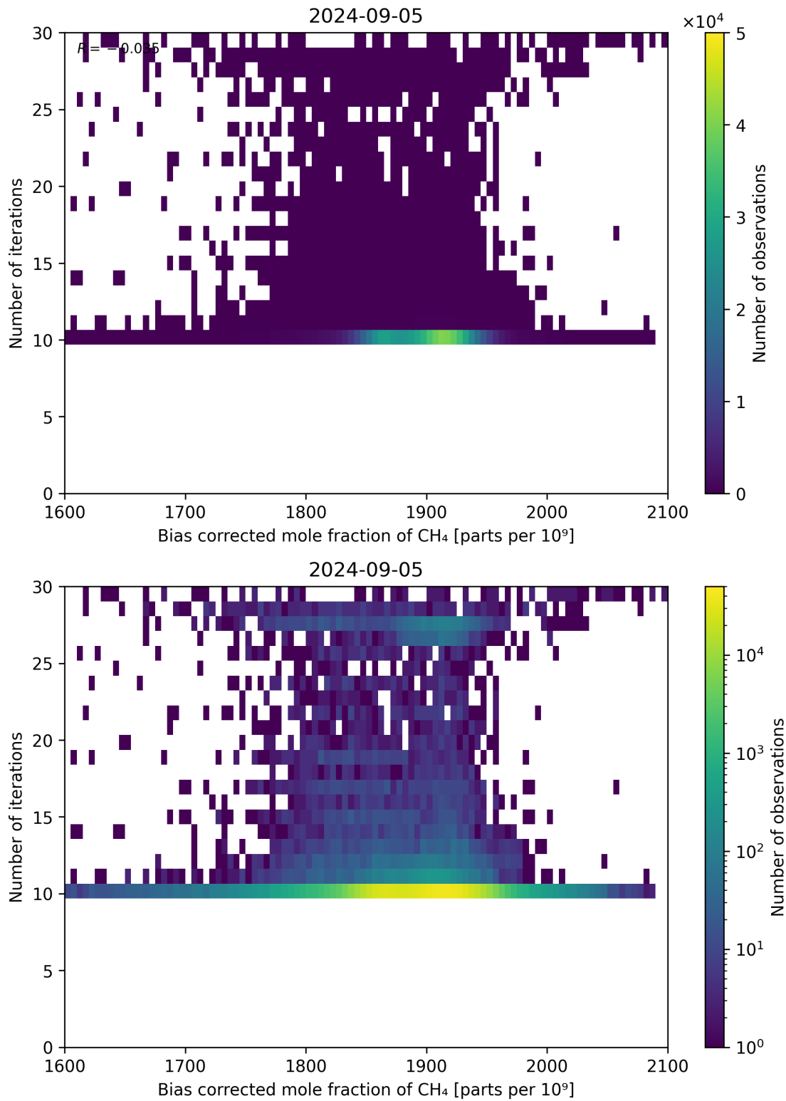
Figure 67: Scatter density plot of “Bias corrected mole fraction of CH 4 ” against “Number of iterations” for 2024-09-04 to 2024-09-06.
