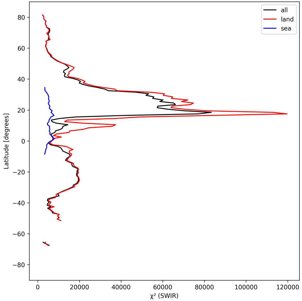
Figure 17: Zonal average of “ \chi^2 (SWIR)” for 2024-09-04 to 2024-09-06.
