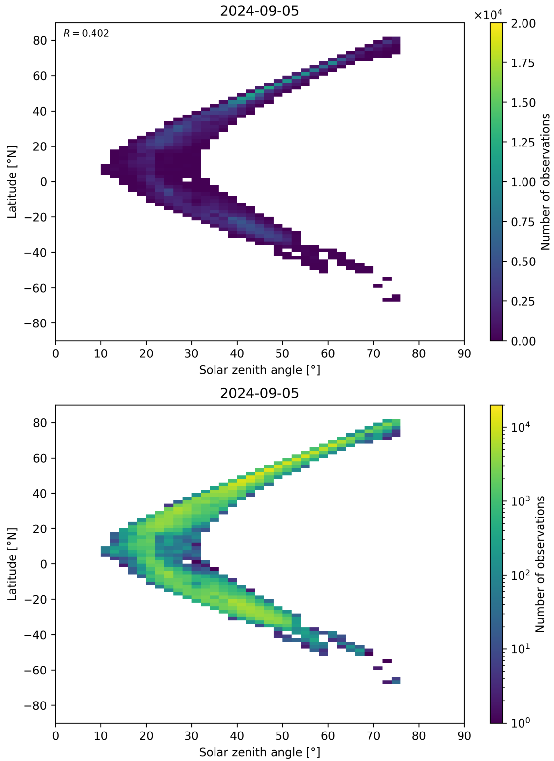
Figure 98: Scatter density plot of “Solar zenith angle” against “Latitude” for 2024-09-04 to 2024-09-06.
