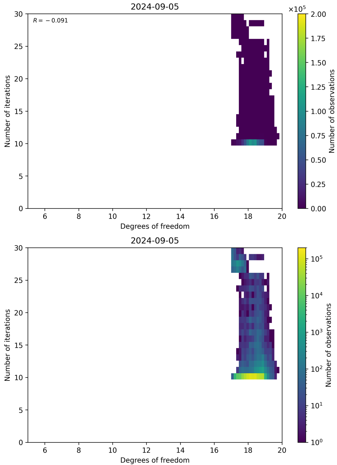
Figure 52: Scatter density plot of “Degrees of freedom” against “Number of iterations” for 2024-09-04 to 2024-09-06.
