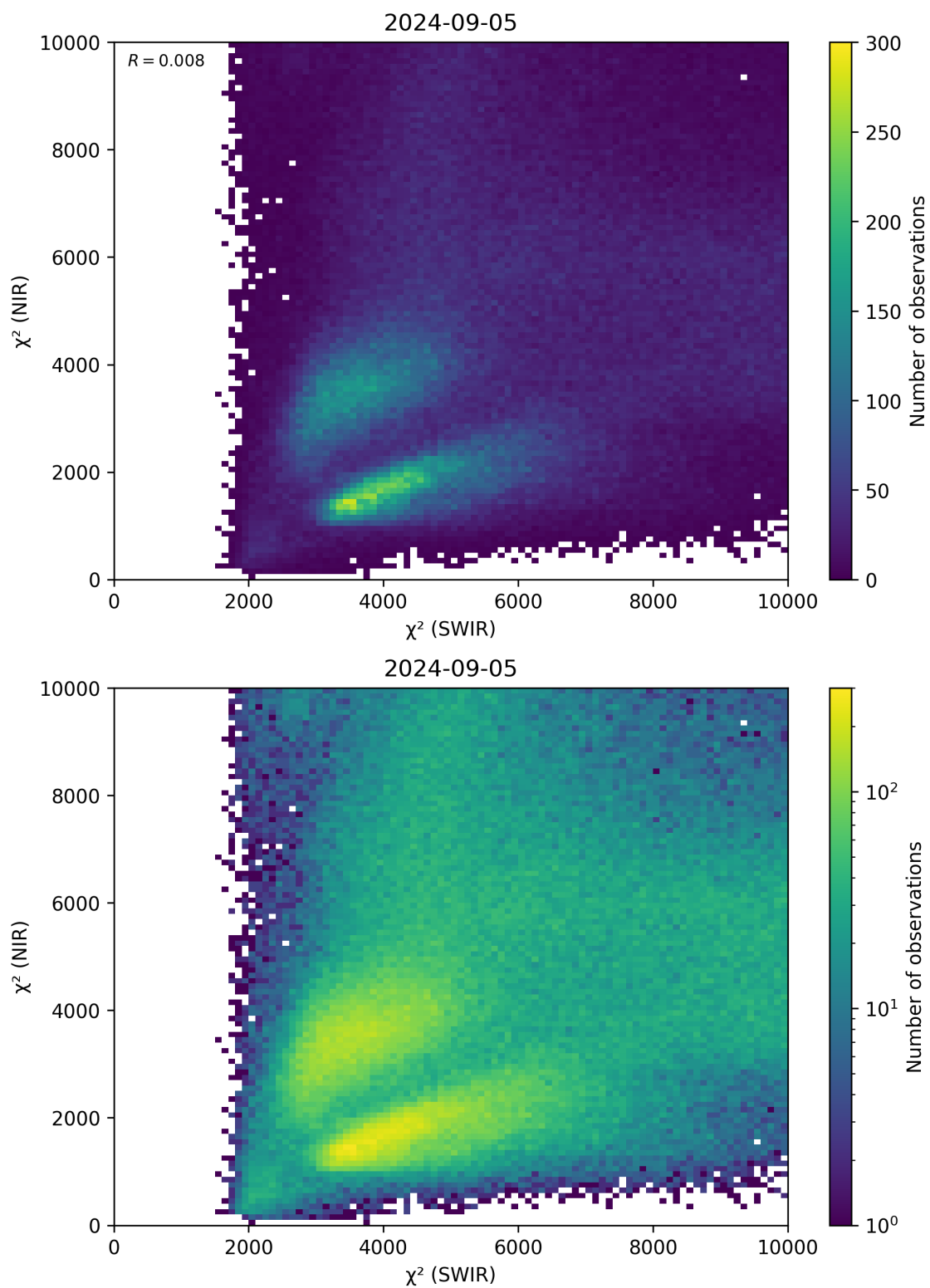
Figure 47: Scatter density plot of “ \chi^2 (SWIR)” against “ \chi^2 (NIR)” for 2024-09-04 to 2024-09-06.
