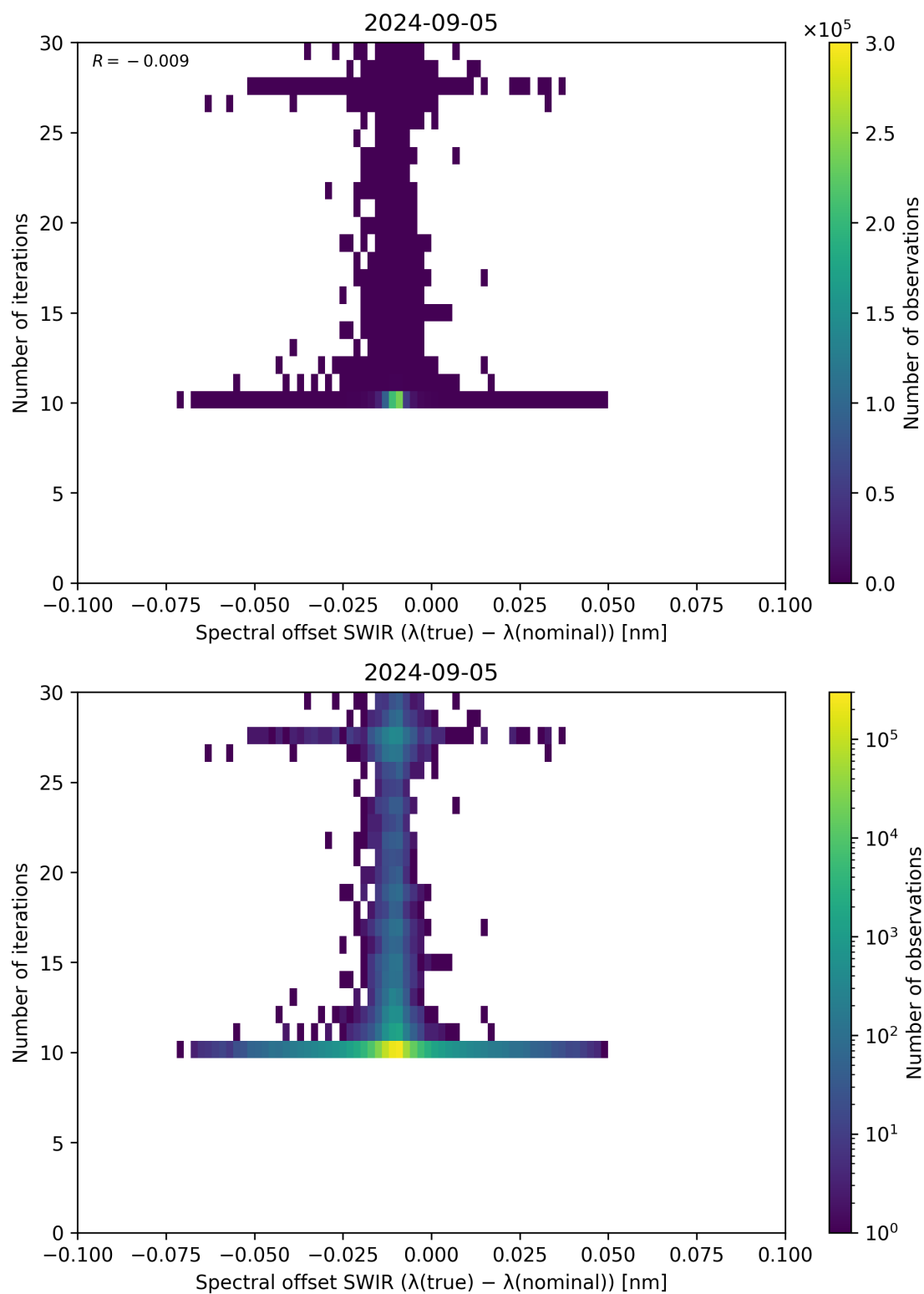
Figure 121: Scatter density plot of “Spectral offset SWIR ( \lambda_{\text{true}} - \lambda_{\text{nominal}} )” against “Number of iterations” for 2024-09-04 to 2024-09-06.
