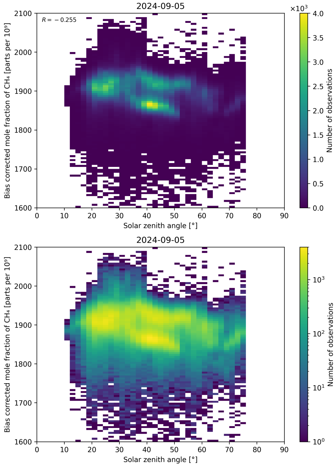
Figure 100: Scatter density plot of “Solar zenith angle” against “Bias corrected mole fraction of CH 4 ” for 2024-09-04 to 2024-09-06.
