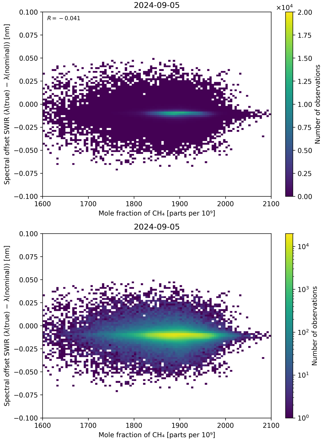
Figure 86: Scatter density plot of “Mole fraction of \text{CH}_4 ” against “Spectral offset SWIR ( \lambda_{\text{true}} - \lambda_{\text{nominal}} )” for 2024-09-04 to 2024-09-06.
