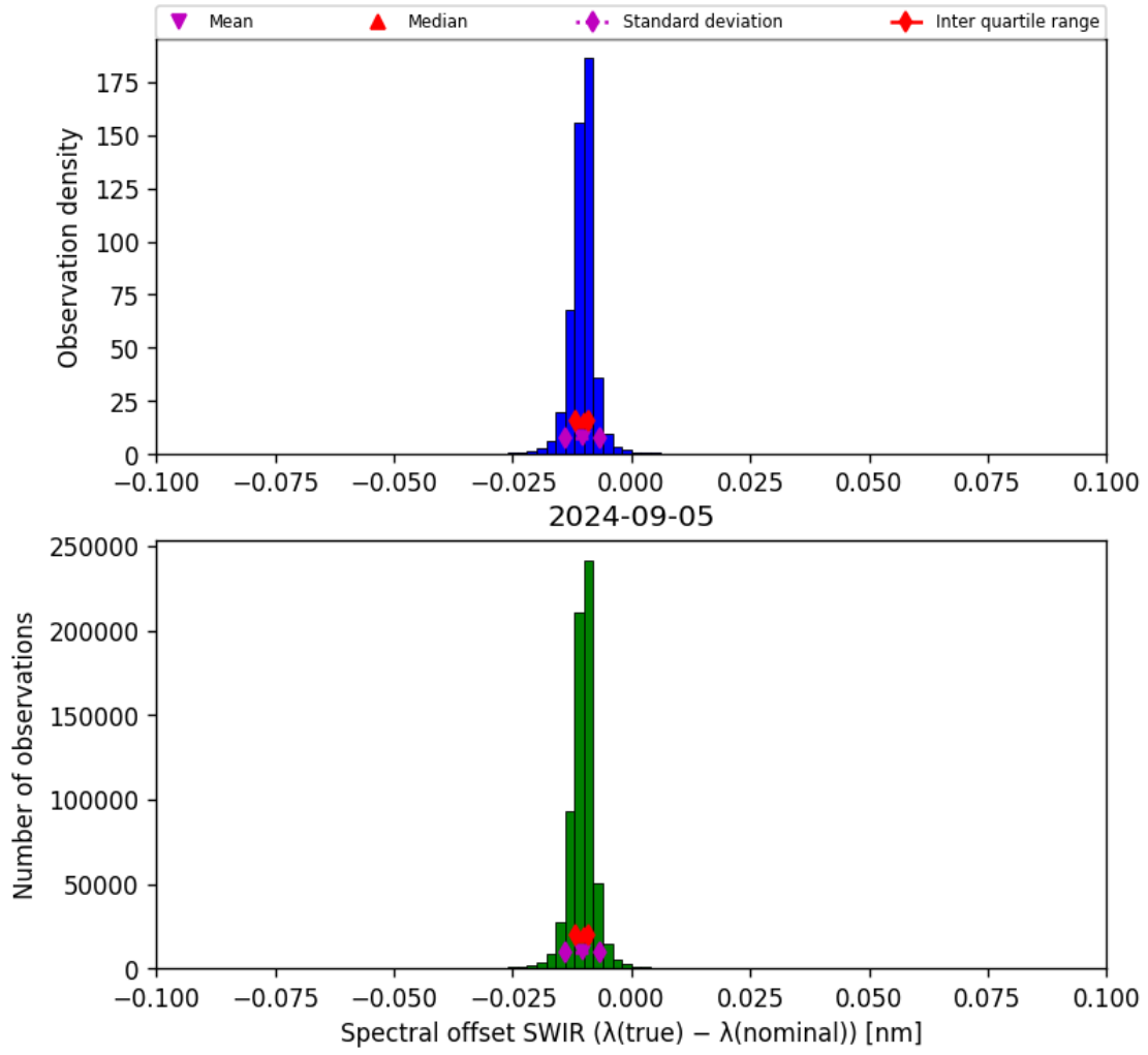
Figure 27: Histogram of “Spectral offset SWIR ( \lambda_{\text{true}} - \lambda_{\text{nominal}} )” for 2024-09-04 to 2024-09-06
