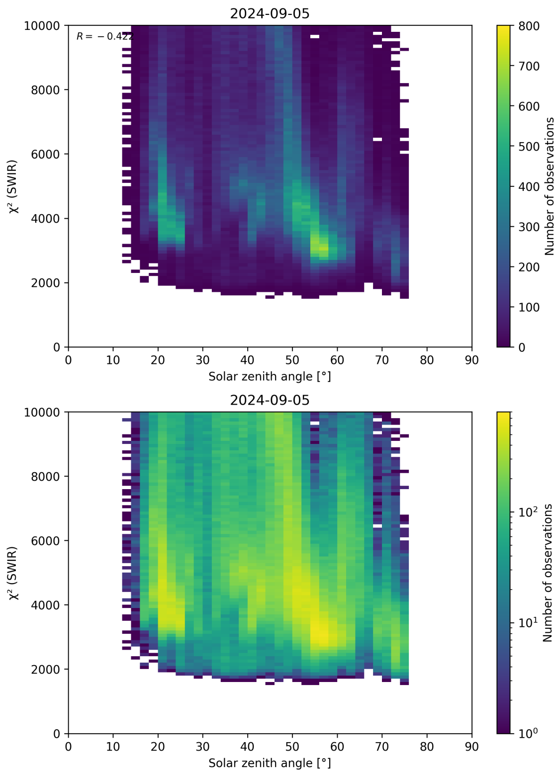
Figure 95: Scatter density plot of “Solar zenith angle” against “ \chi^2 (SWIR)” for 2024-09-04 to 2024-09-06.
