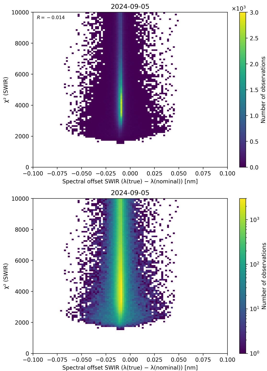
Figure 118: Scatter density plot of “Spectral offset SWIR ( \lambda_{\text{true}} - \lambda_{\text{nominal}} )” against “ \chi^2 (SWIR)” for 2024-09-04 to 2024-09-06.
