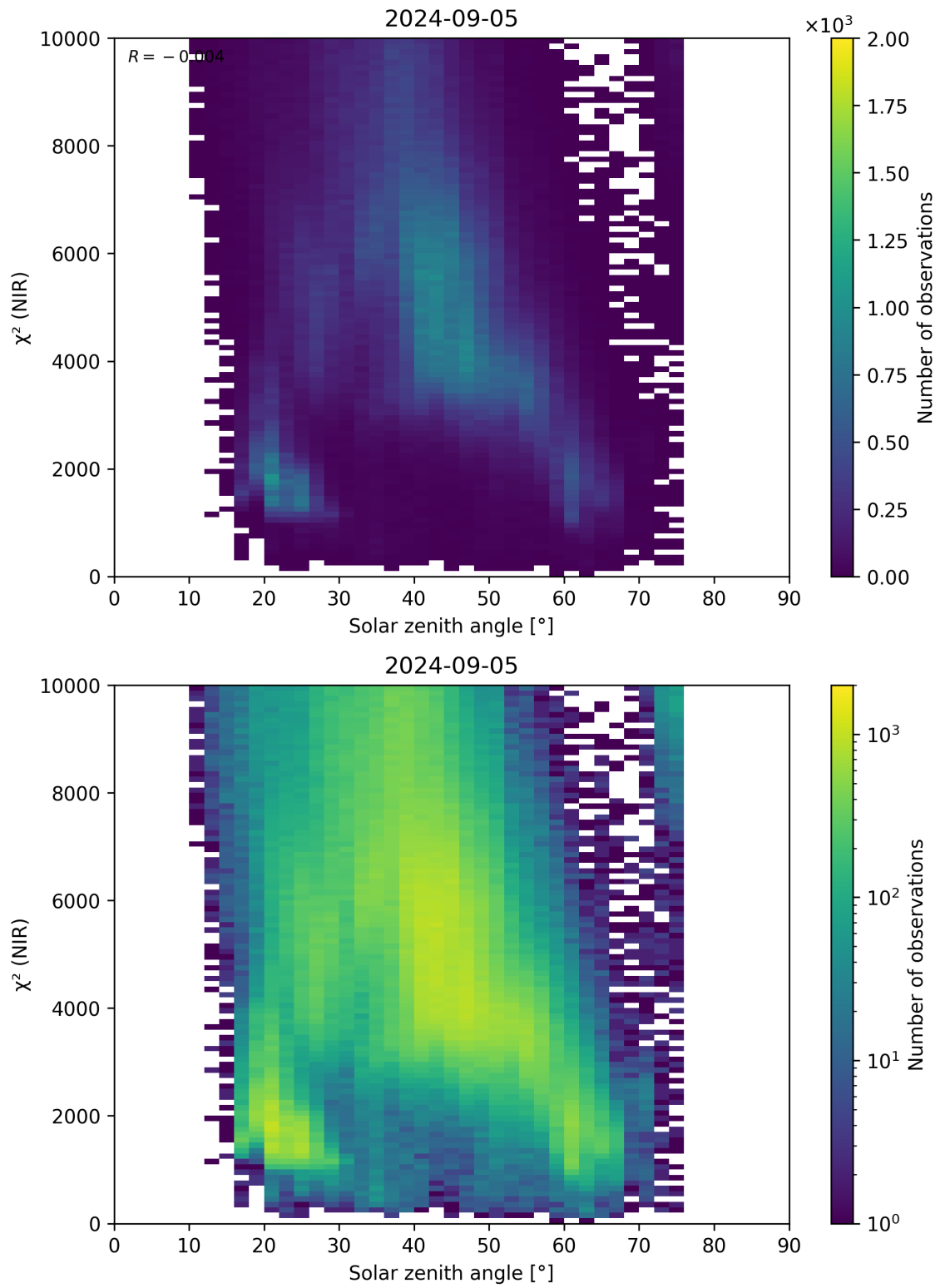
Figure 94: Scatter density plot of “Solar zenith angle” against “ \chi^2 (NIR)” for 2024-09-04 to 2024-09-06.
