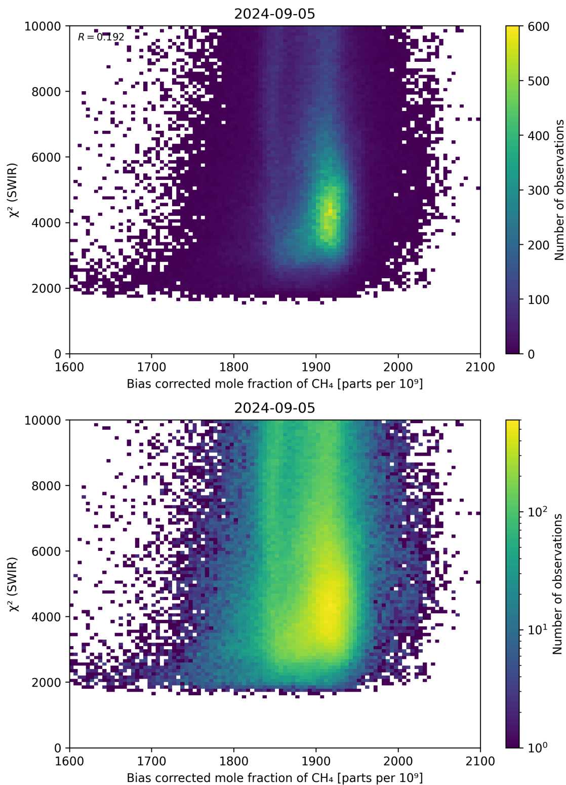
Figure 64: Scatter density plot of “Bias corrected mole fraction of \text{CH}_4 ” against “ \chi^2 (SWIR)” for 2024-09-04 to 2024-09-06.
