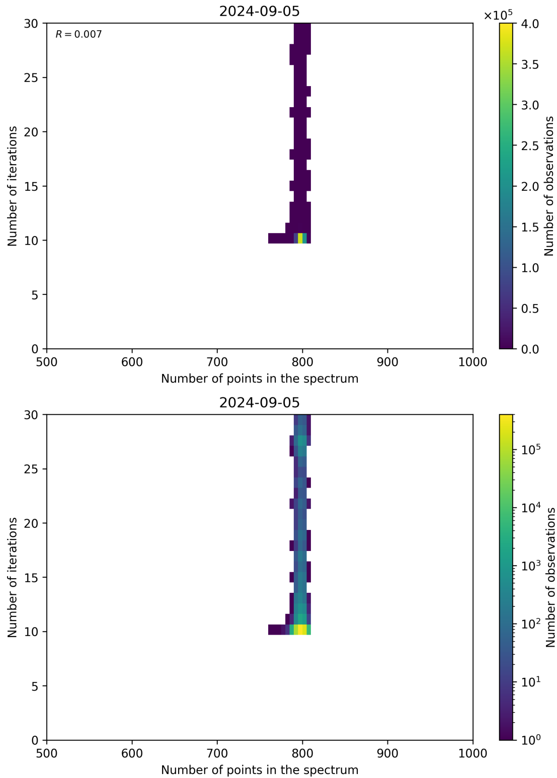
Figure 92: Scatter density plot of “Number of points in the spectrum” against “Number of iterations” for 2024-09-04 to 2024-09-06.
