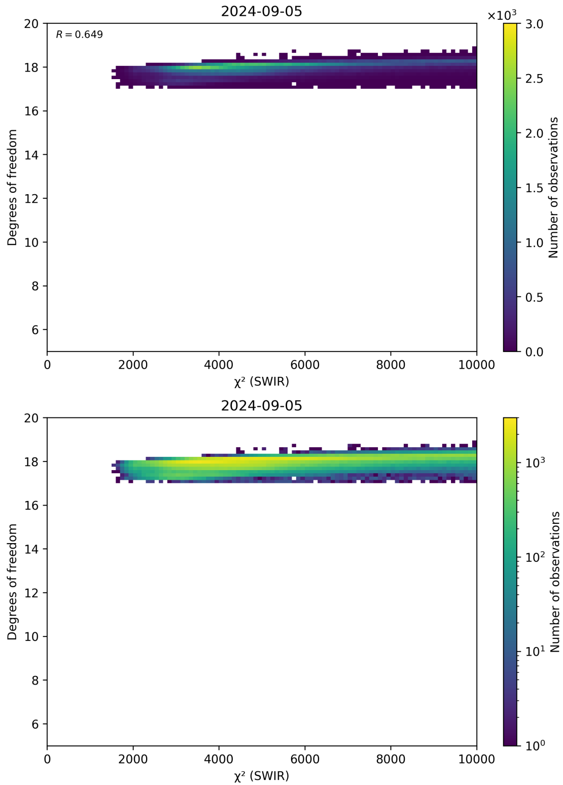
Figure 48: Scatter density plot of “ \chi^2 (SWIR)” against “Degrees of freedom” for 2024-09-04 to 2024-09-06.
