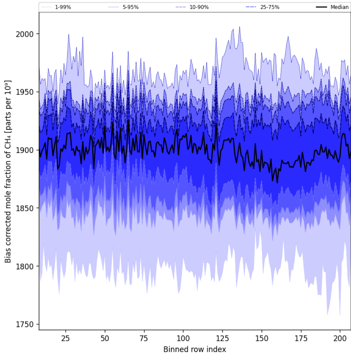
Figure 36: Along track statistics of “Bias corrected mole fraction of CH 4 ” for 2024-09-04 to 2024-09-06
