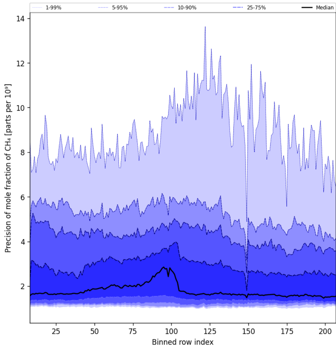
Figure 35: Along track statistics of “Precision of mole fraction of CH 4 ” for 2024-09-04 to 2024-09-06
