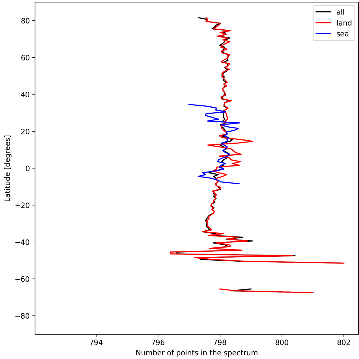
Figure 15: Zonal average of “Number of points in the spectrum” for 2024-09-04 to 2024-09-06.
