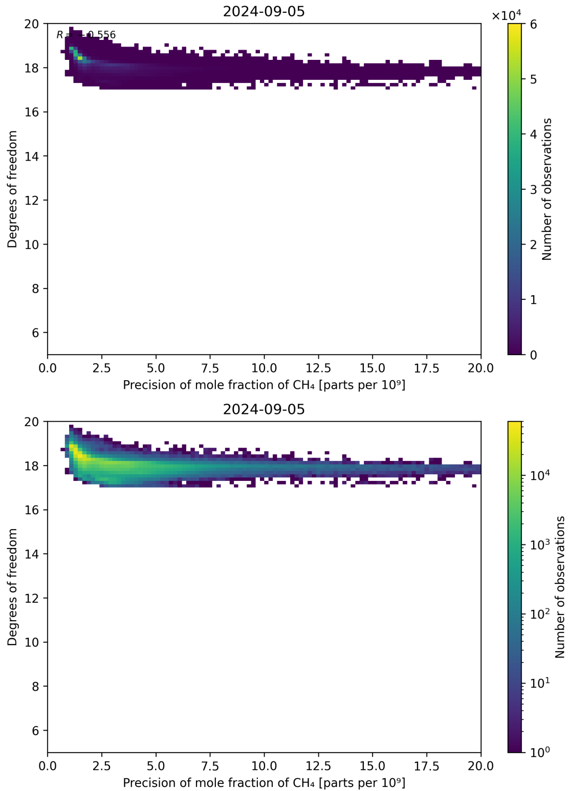
Figure 80: Scatter density plot of “Precision of mole fraction of CH 4 ” against “Degrees of freedom” for 2024-09-04 to 2024-09-06.
