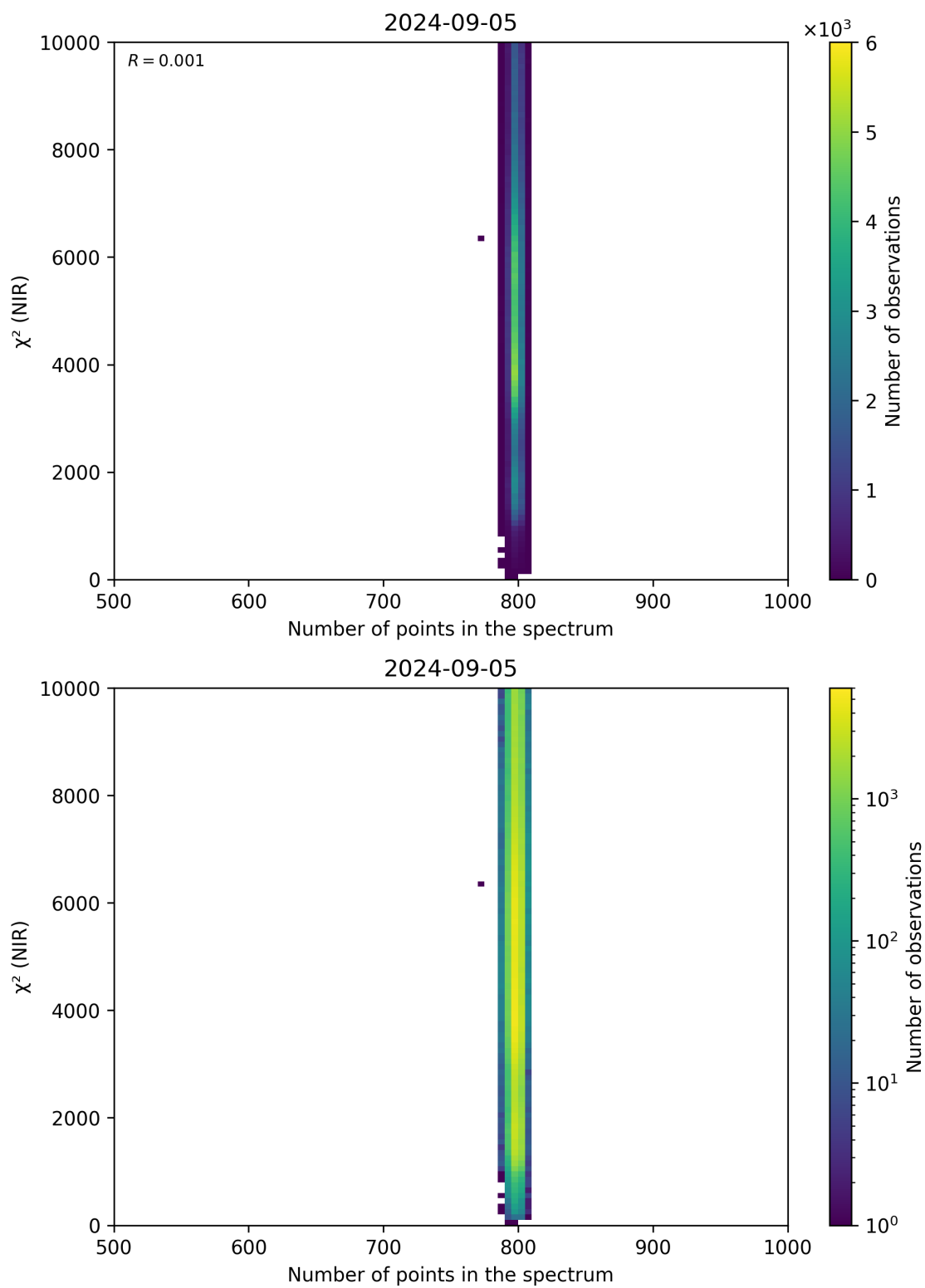
Figure 88: Scatter density plot of “Number of points in the spectrum” against “ \chi^2 (NIR)” for 2024-09-04 to 2024-09-06.
