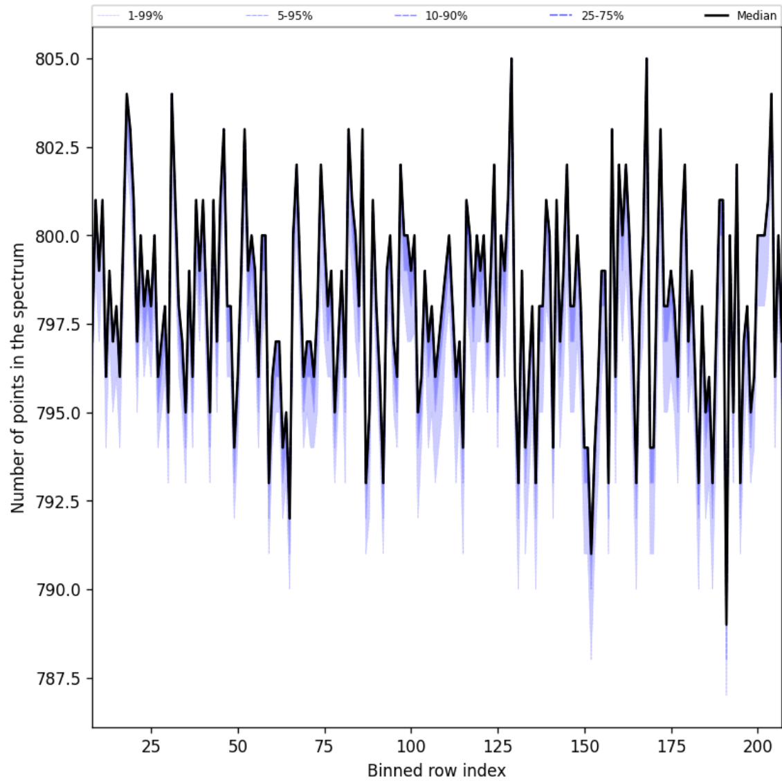
Figure 37: Along track statistics of “Number of points in the spectrum” for 2024-09-04 to 2024-09-06
