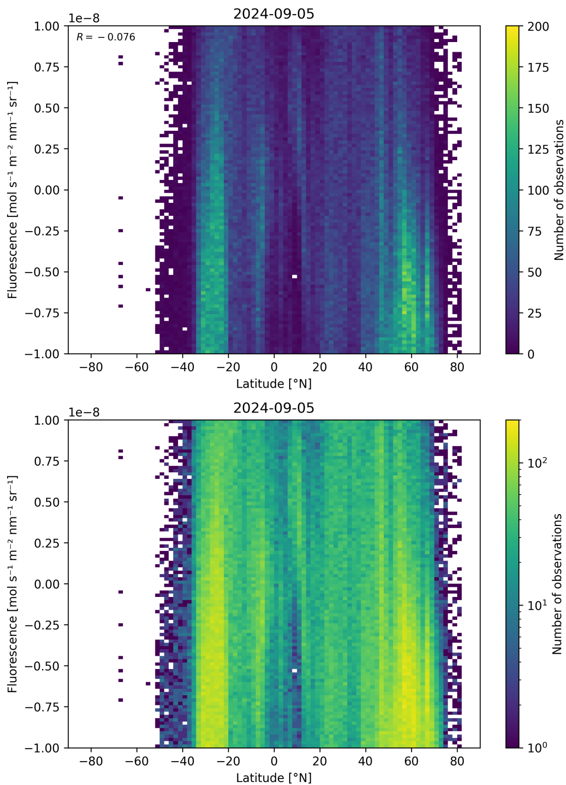
Figure 56: Scatter density plot of “Latitude” against “Fluorescence” for 2024-09-04 to 2024-09-06.
