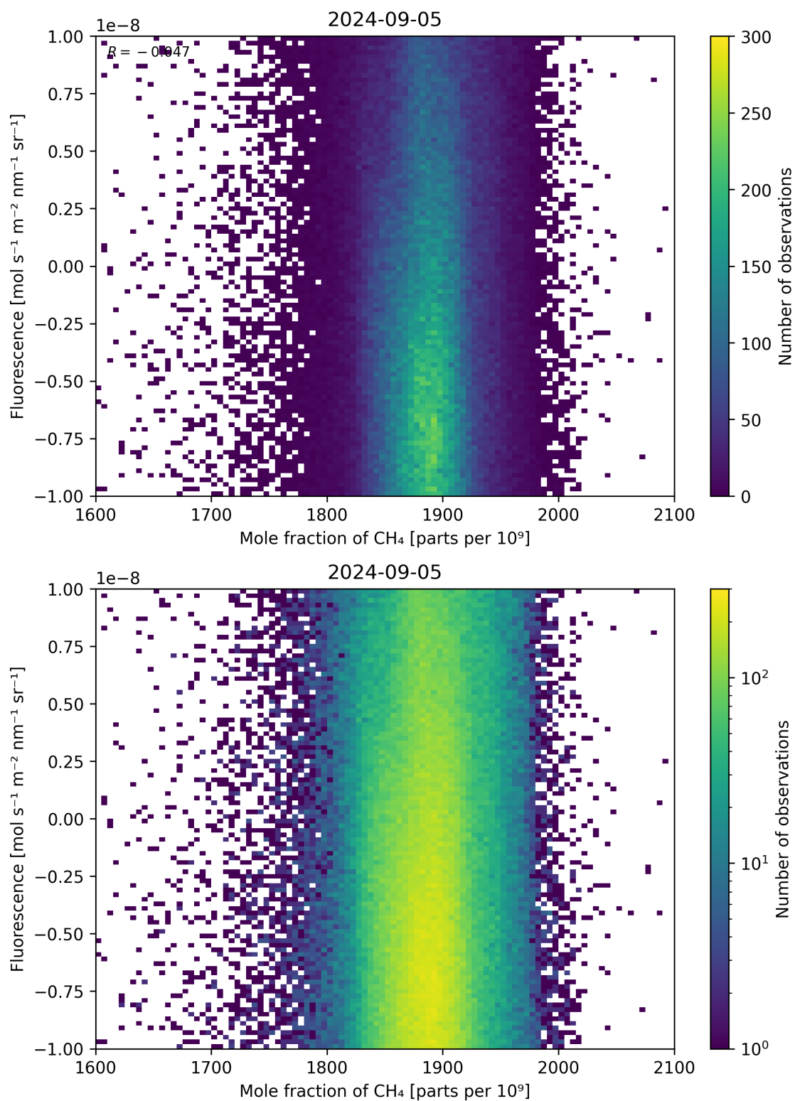
Figure 73: Scatter density plot of “Mole fraction of CH 4 ” against “Fluorescence” for 2024-09-04 to 2024-09-06.
