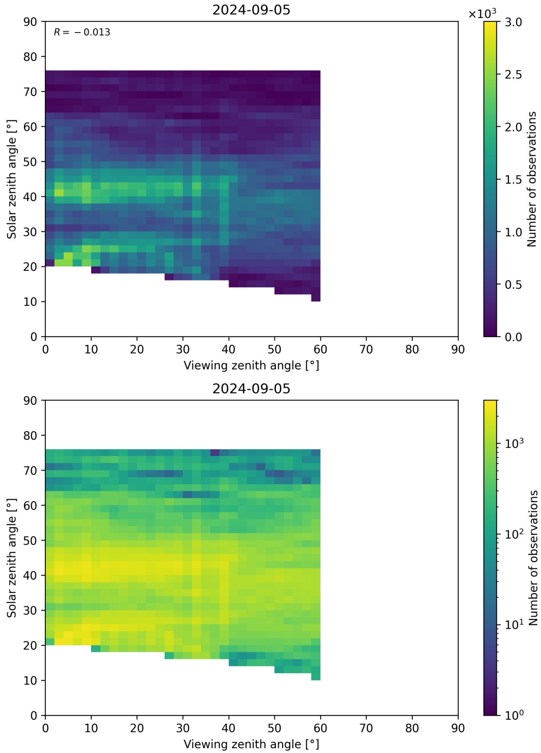
Figure 115: Scatter density plot of “Viewing zenith angle” against “Solar zenith angle” for 2024-09-04 to 2024-09-06.
