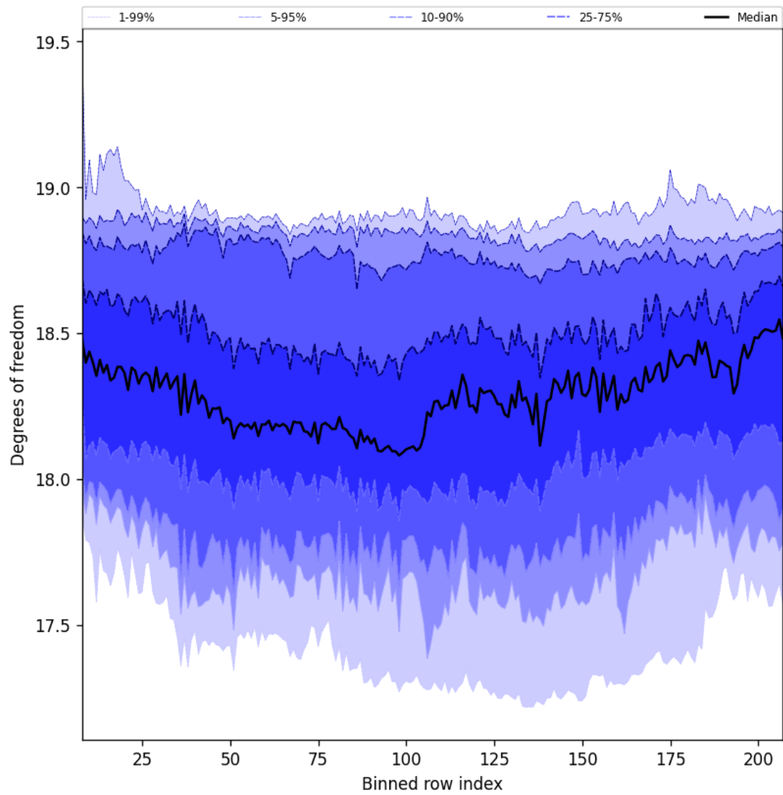
Figure 41: Along track statistics of “Degrees of freedom” for 2024-09-04 to 2024-09-06
