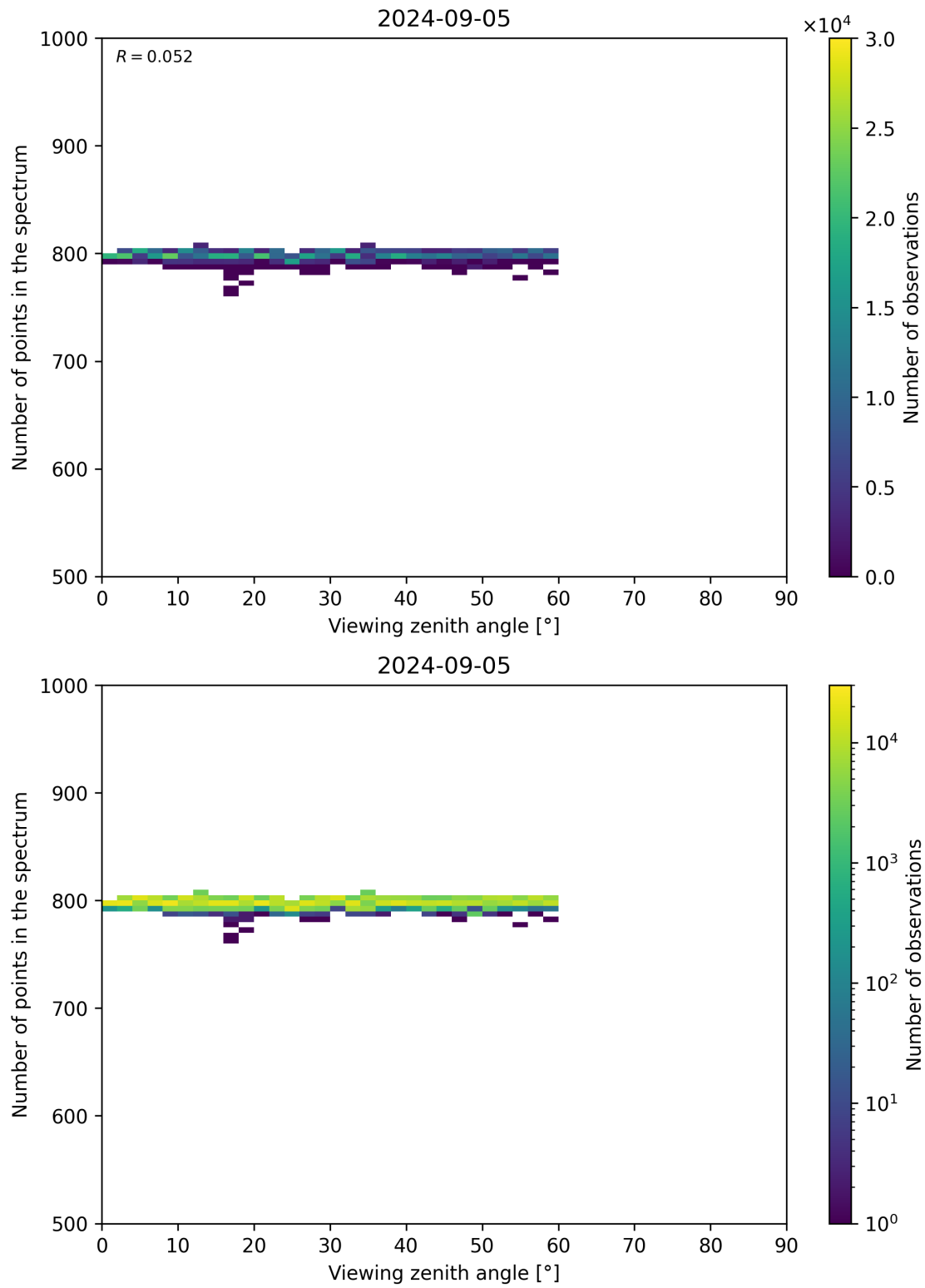
Figure 114: Scatter density plot of “Viewing zenith angle” against “Number of points in the spectrum” for 2024-09-04 to 2024-09-06.
