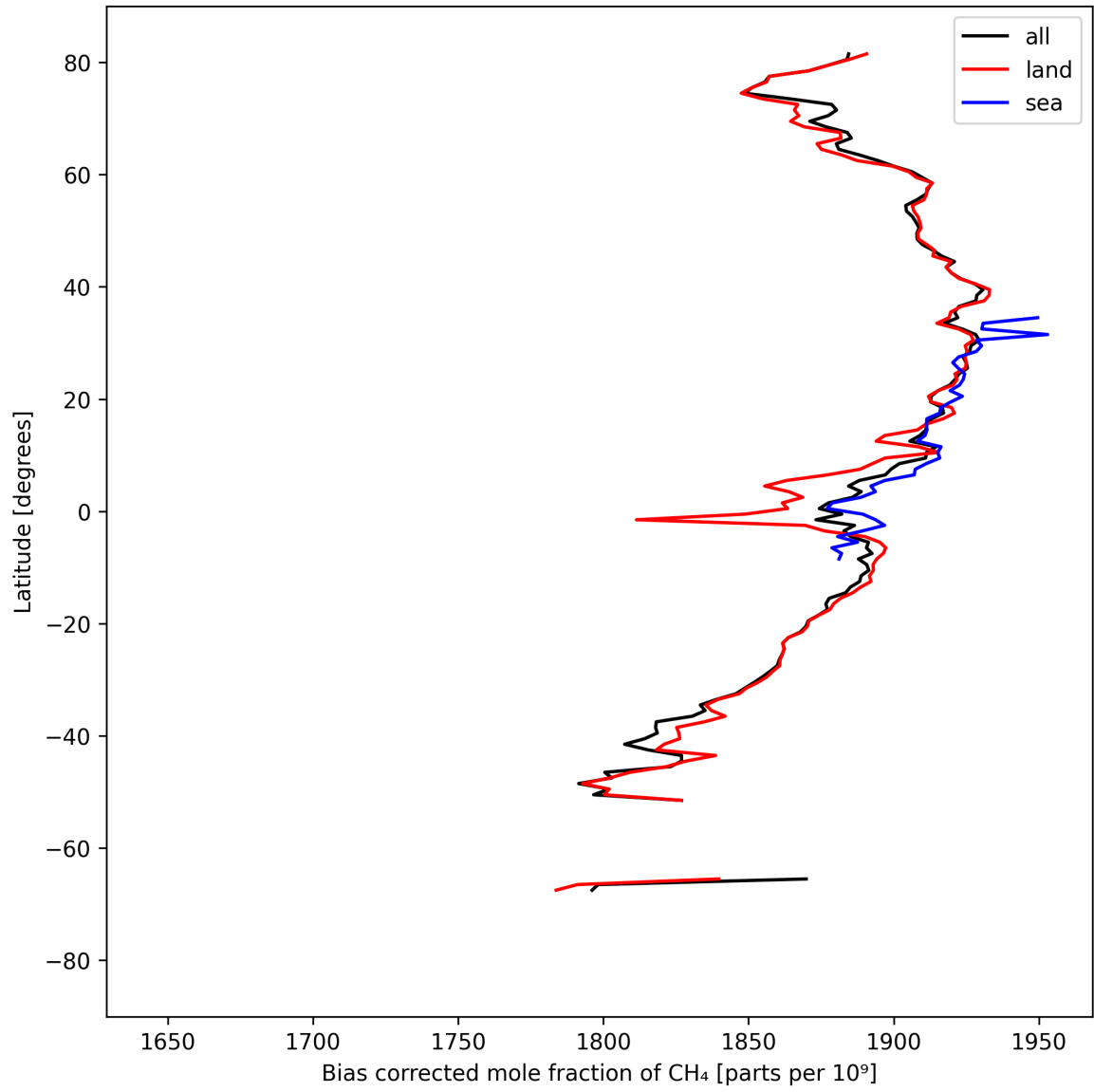
Figure 14: Zonal average of “Bias corrected mole fraction of CH 4 ” for 2024-09-04 to 2024-09-06.
