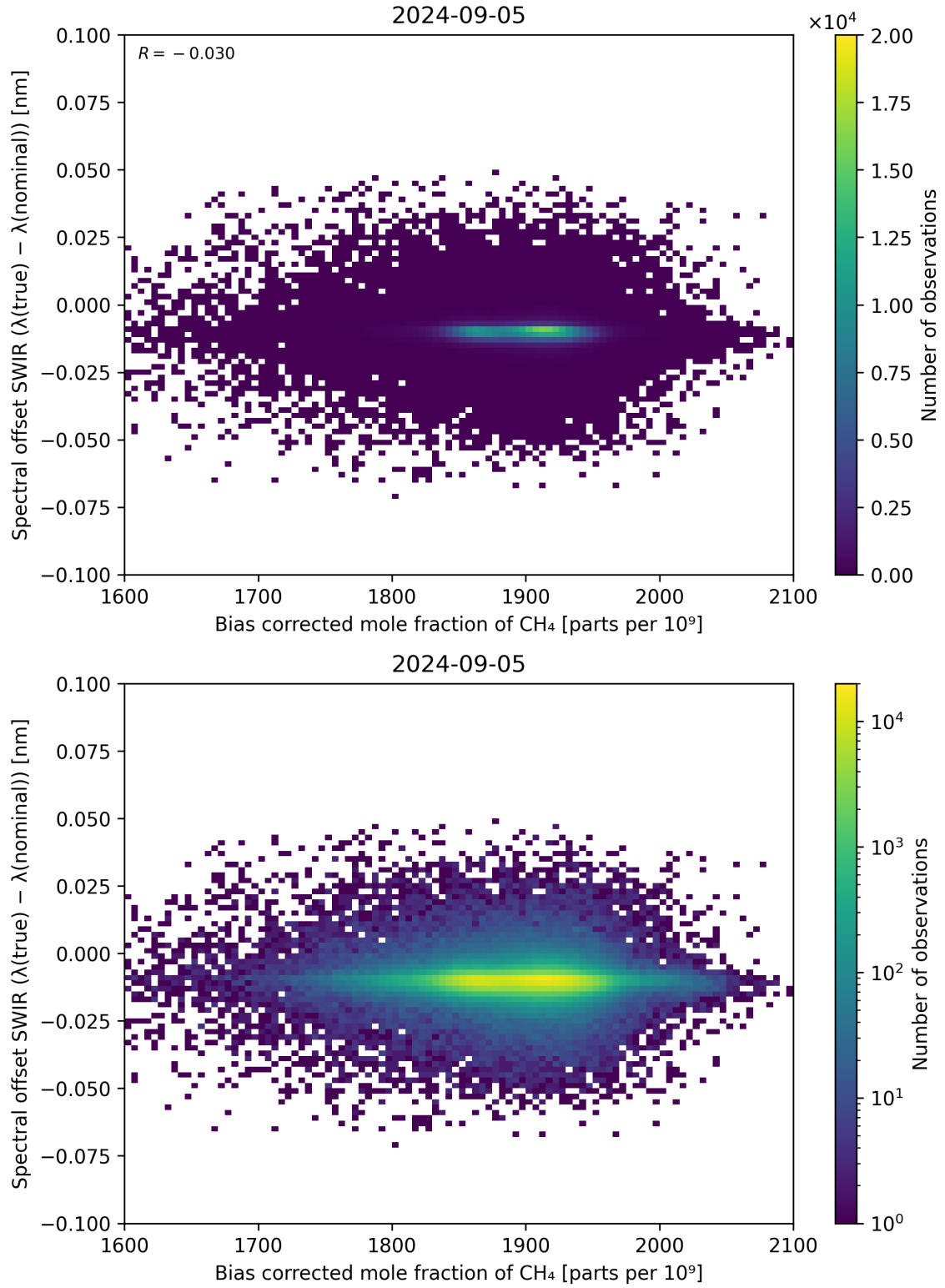
Figure 69: Scatter density plot of “Bias corrected mole fraction of CH 4 ” against “Spectral offset SWIR ( \lambda_{\text{true}} - \lambda_{\text{nominal}} )” for 2024-09-04 to 2024-09-06.
