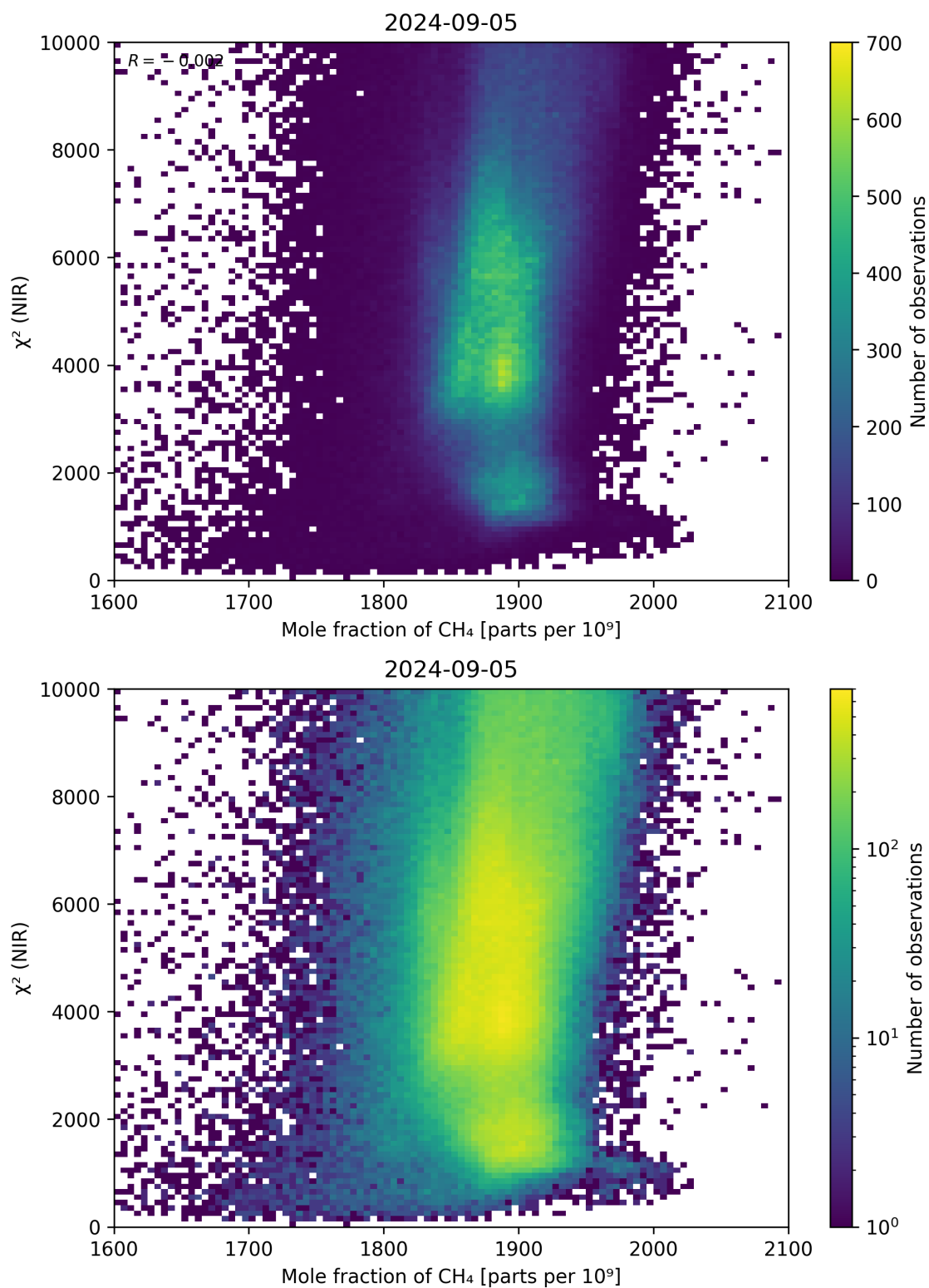
Figure 70: Scatter density plot of “Mole fraction of CH 4 ” against “ \chi^2 (NIR)” for 2024-09-04 to 2024-09-06.
