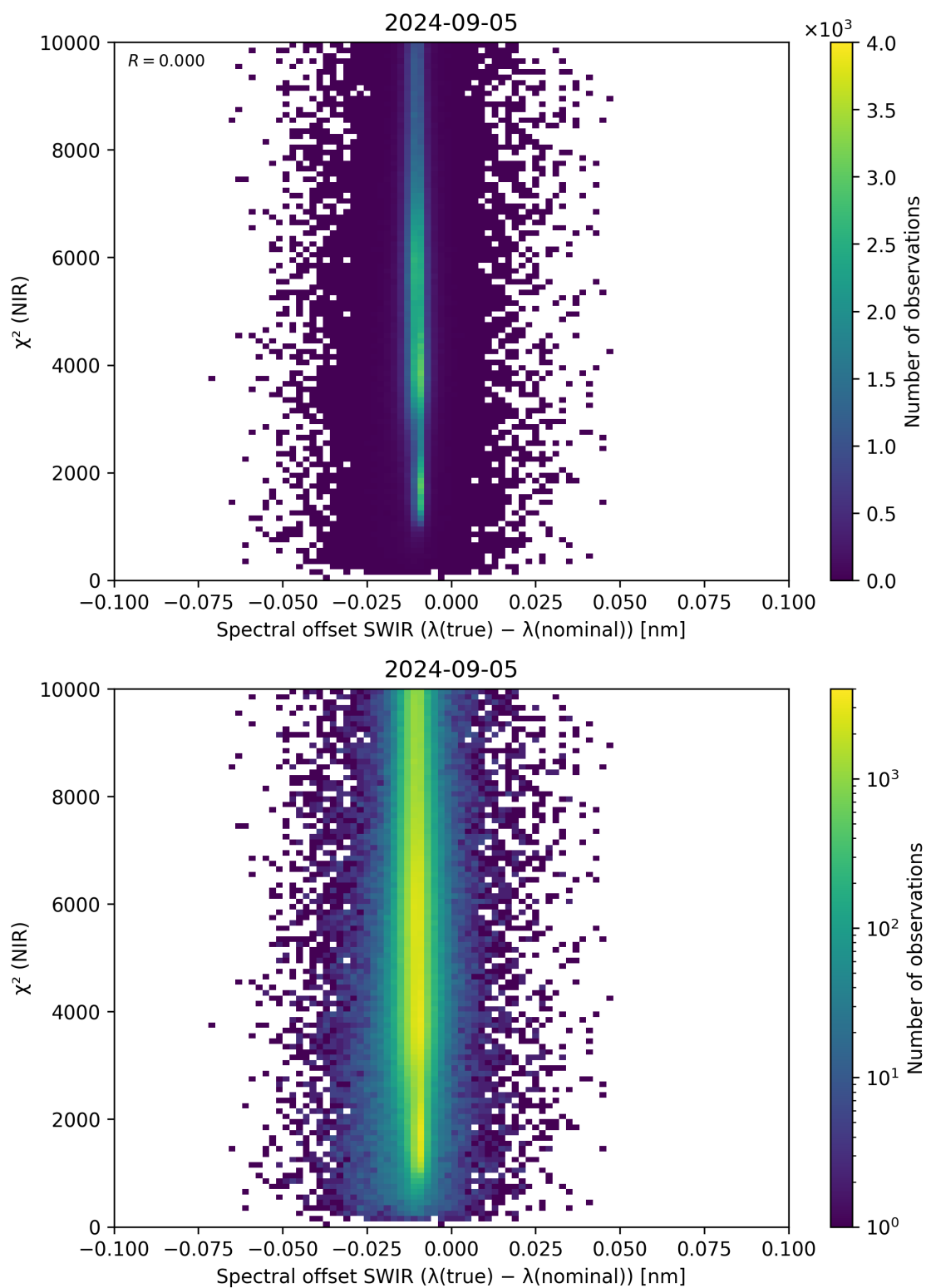
Figure 117: Scatter density plot of “Spectral offset SWIR ( \lambda_{\text{true}} - \lambda_{\text{nominal}} )” against “ \chi^2 (NIR)” for 2024-09-04 to 2024-09-06.
