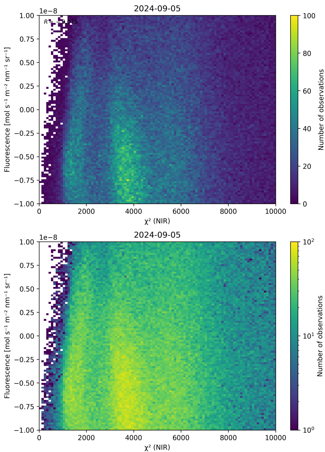
Figure 45: Scatter density plot of “ \chi^2 (NIR)” against “Fluorescence” for 2024-09-04 to 2024-09-06.
