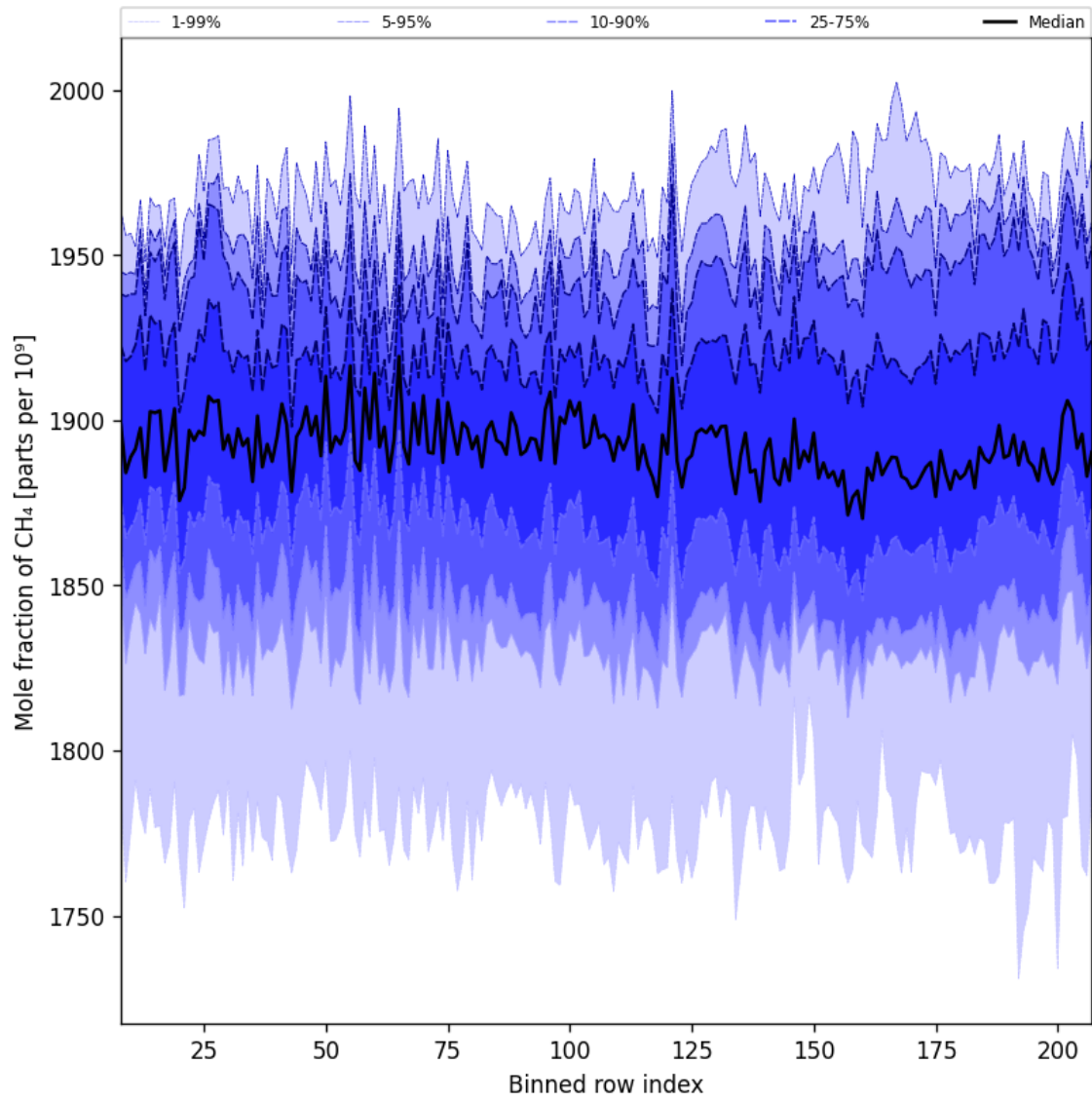
Figure 34: Along track statistics of “Mole fraction of CH 4 ” for 2024-09-04 to 2024-09-06
