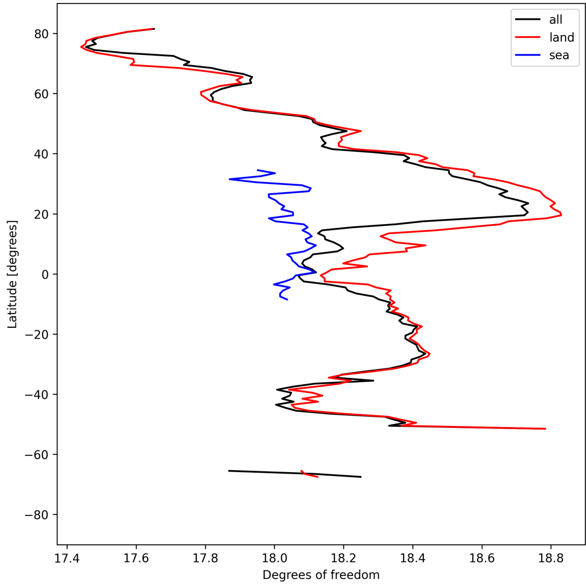
Figure 19: Zonal average of “Degrees of freedom” for 2024-09-04 to 2024-09-06.
