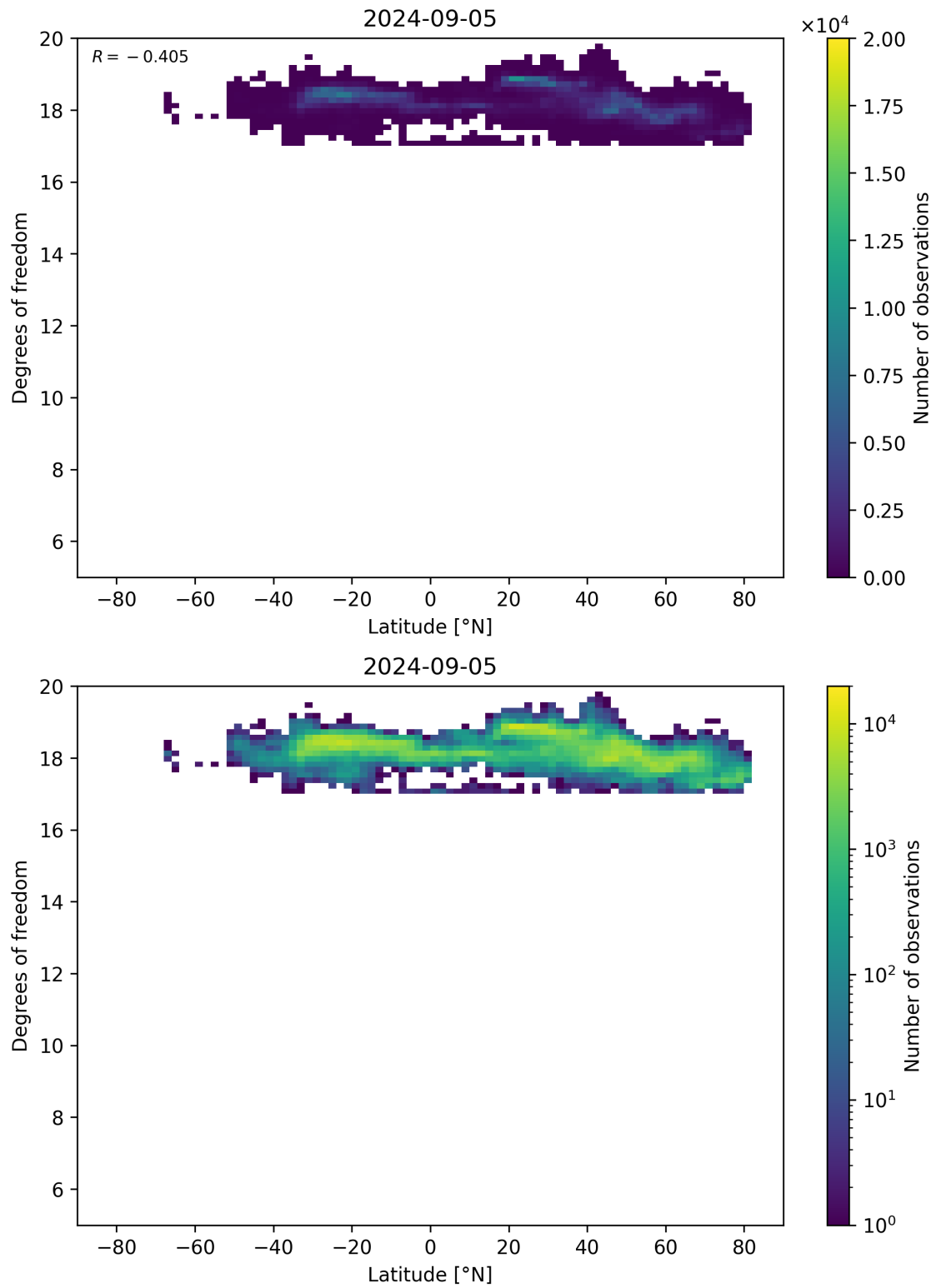
Figure 55: Scatter density plot of “Latitude” against “Degrees of freedom” for 2024-09-04 to 2024-09-06.
