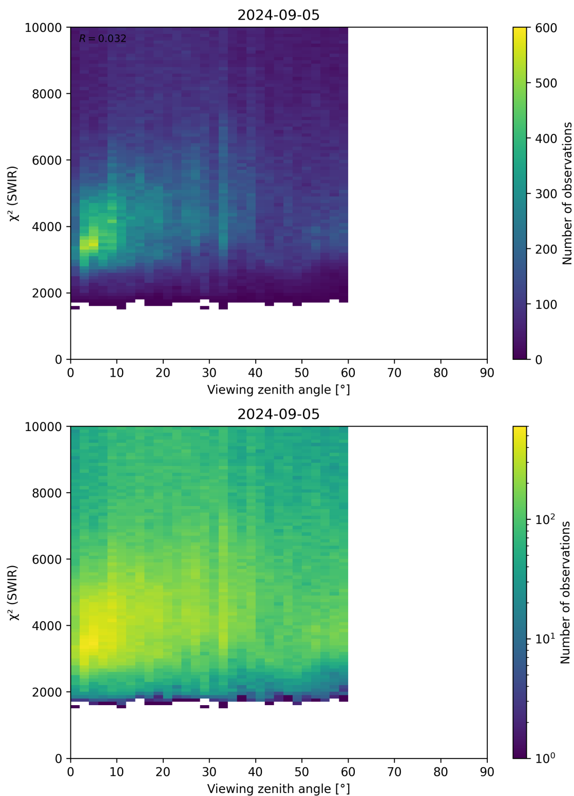
Figure 106: Scatter density plot of “Viewing zenith angle” against “ \chi^2 (SWIR)” for 2024-09-04 to 2024-09-06.
