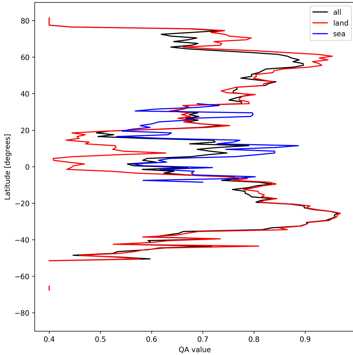
Figure 11: Zonal average of “QA value” for 2024-09-04 to 2024-09-06.
