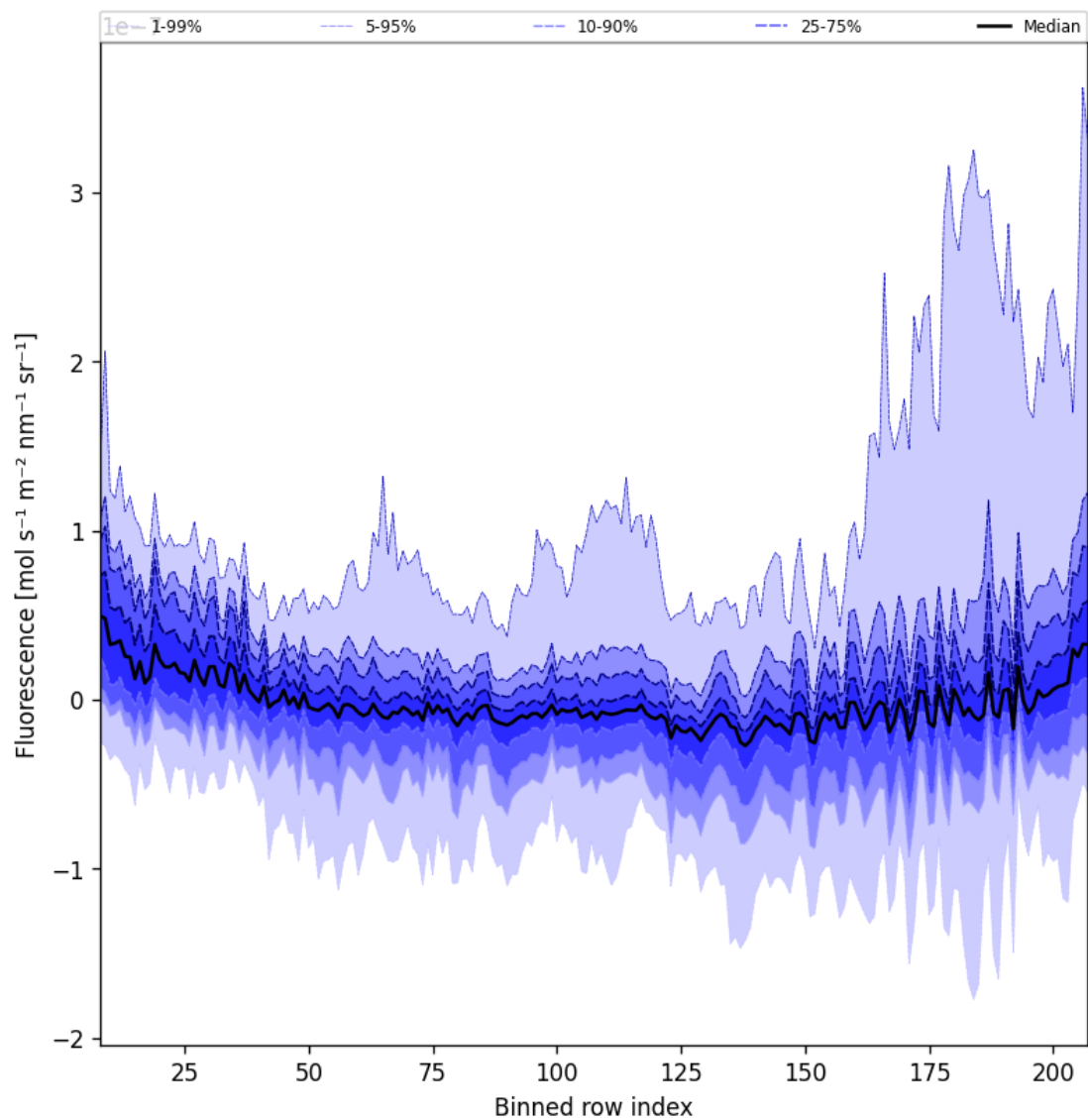
Figure 43: Along track statistics of “Fluorescence” for 2024-09-04 to 2024-09-06
