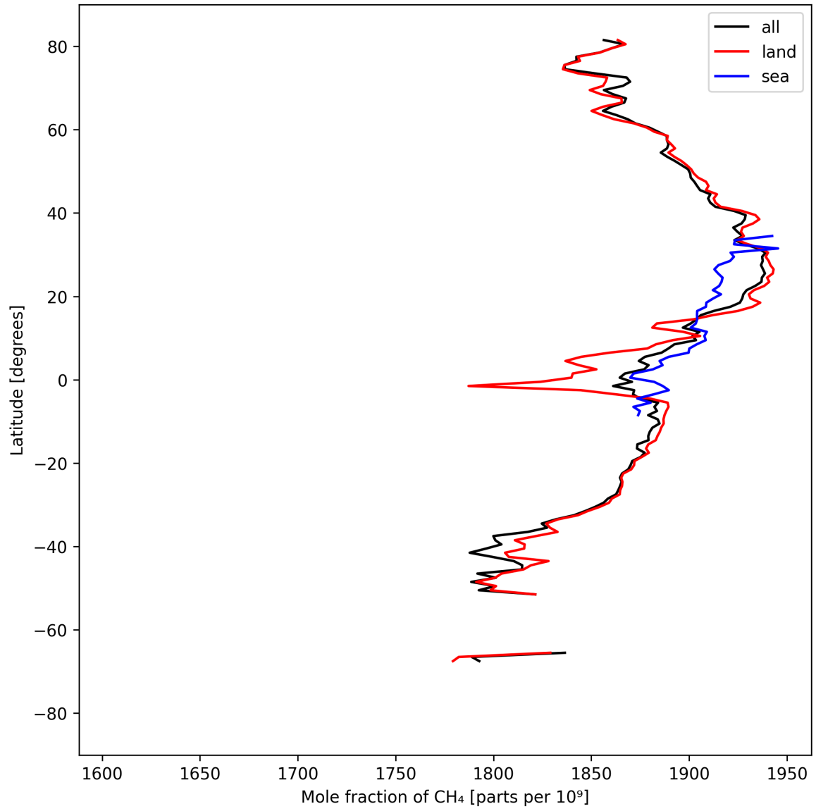
Figure 12: Zonal average of “Mole fraction of CH 4 ” for 2024-09-04 to 2024-09-06.
