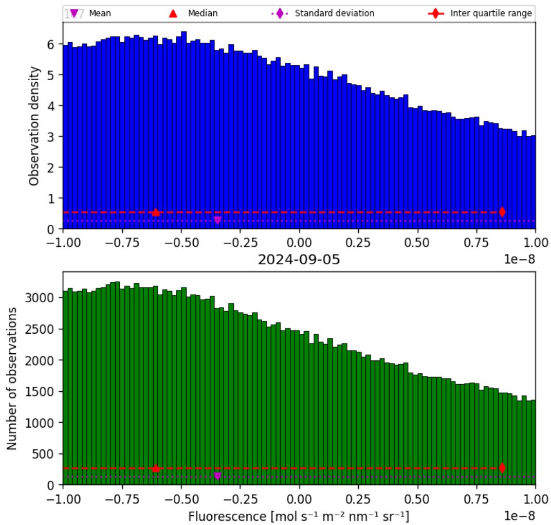
Figure 32: Histogram of “Fluorescence” for 2024-09-04 to 2024-09-06
