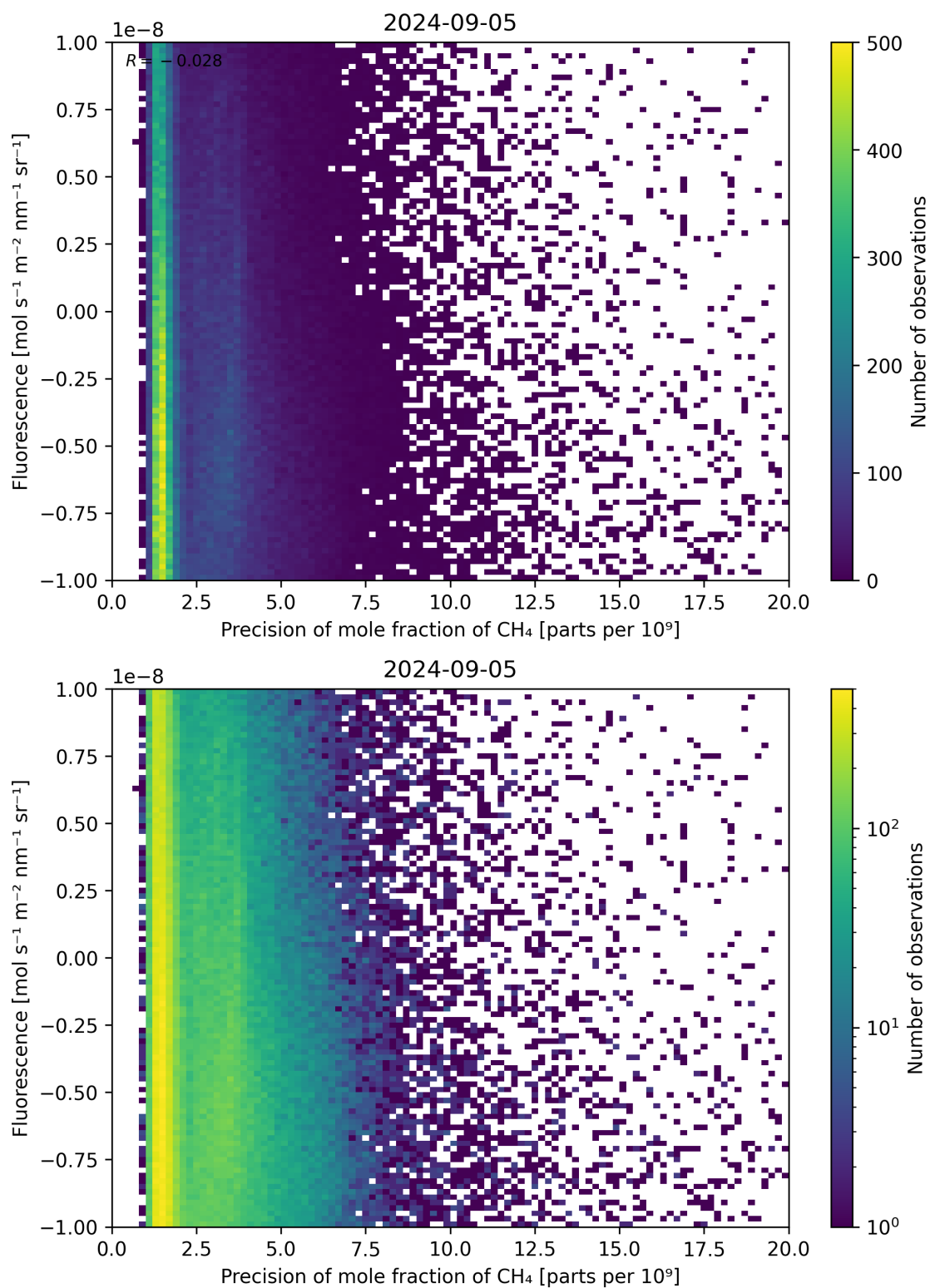
Figure 81: Scatter density plot of “Precision of mole fraction of \text{CH}_4 ” against “Fluorescence” for 2024-09-04 to 2024-09-06.
