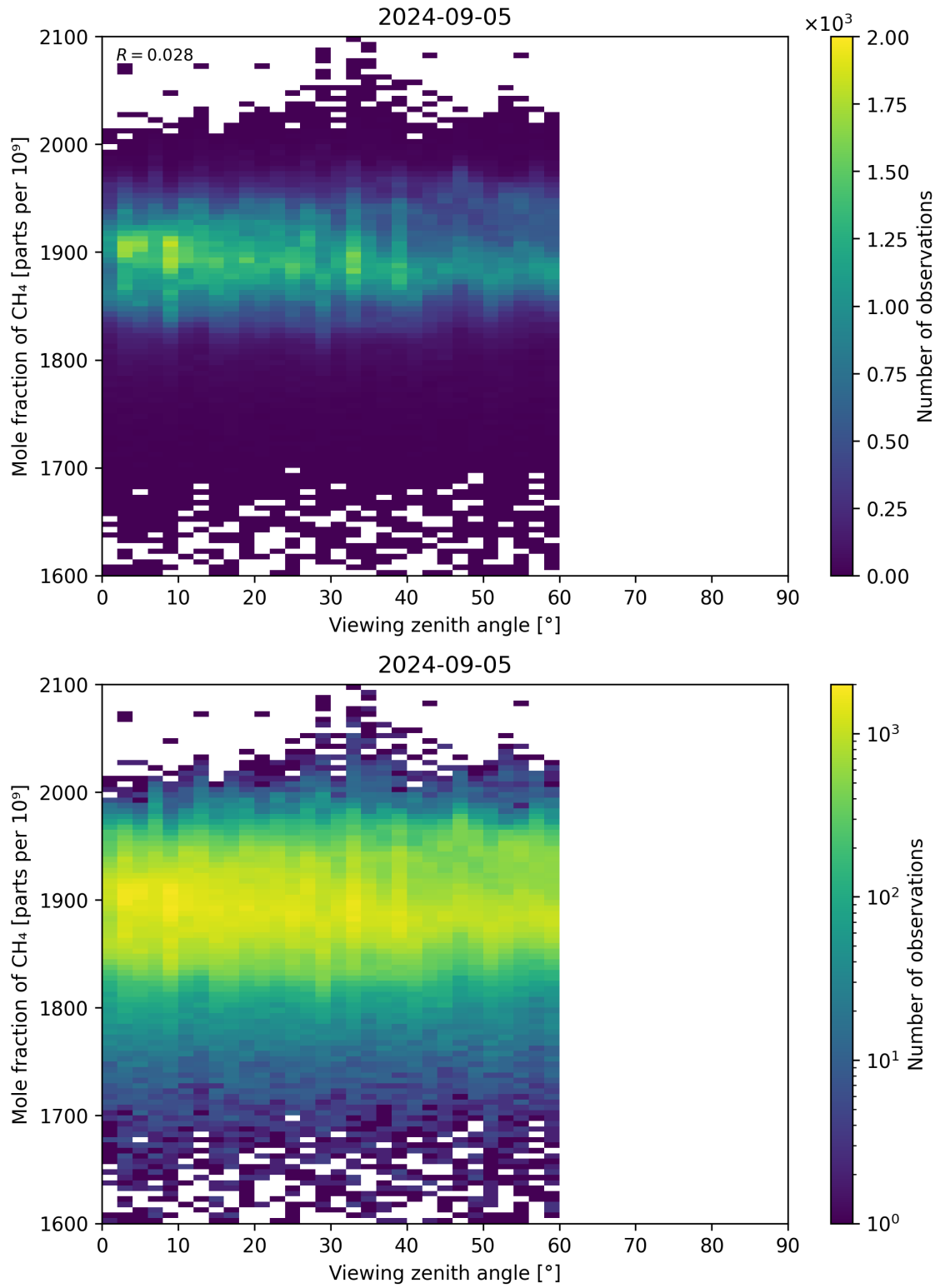
Figure 110: Scatter density plot of “Viewing zenith angle” against “Mole fraction of CH 4 ” for 2024-09-04 to 2024-09-06.
