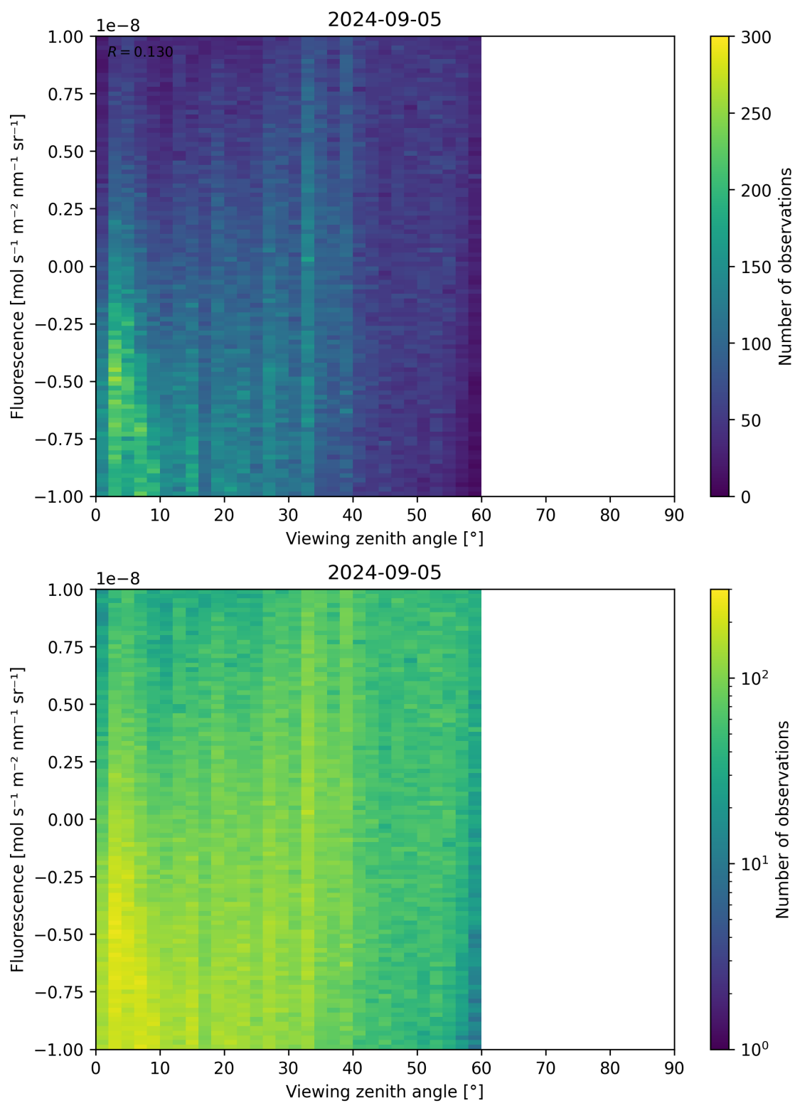
Figure 108: Scatter density plot of “Viewing zenith angle” against “Fluorescence” for 2024-09-04 to 2024-09-06.
