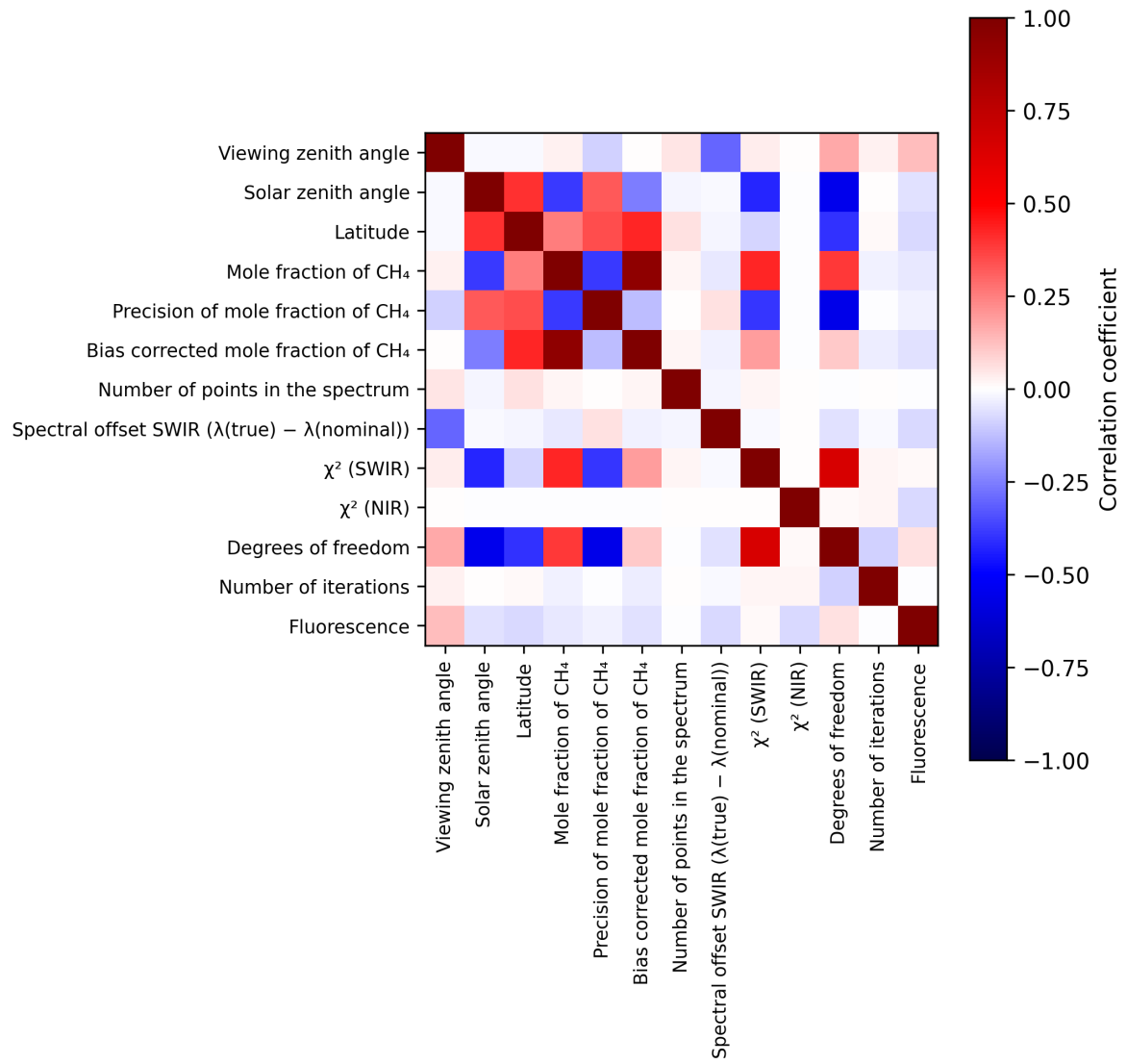
Figure 2: Map of correlation matrix for 2024-09-04 to 2024-09-06.
