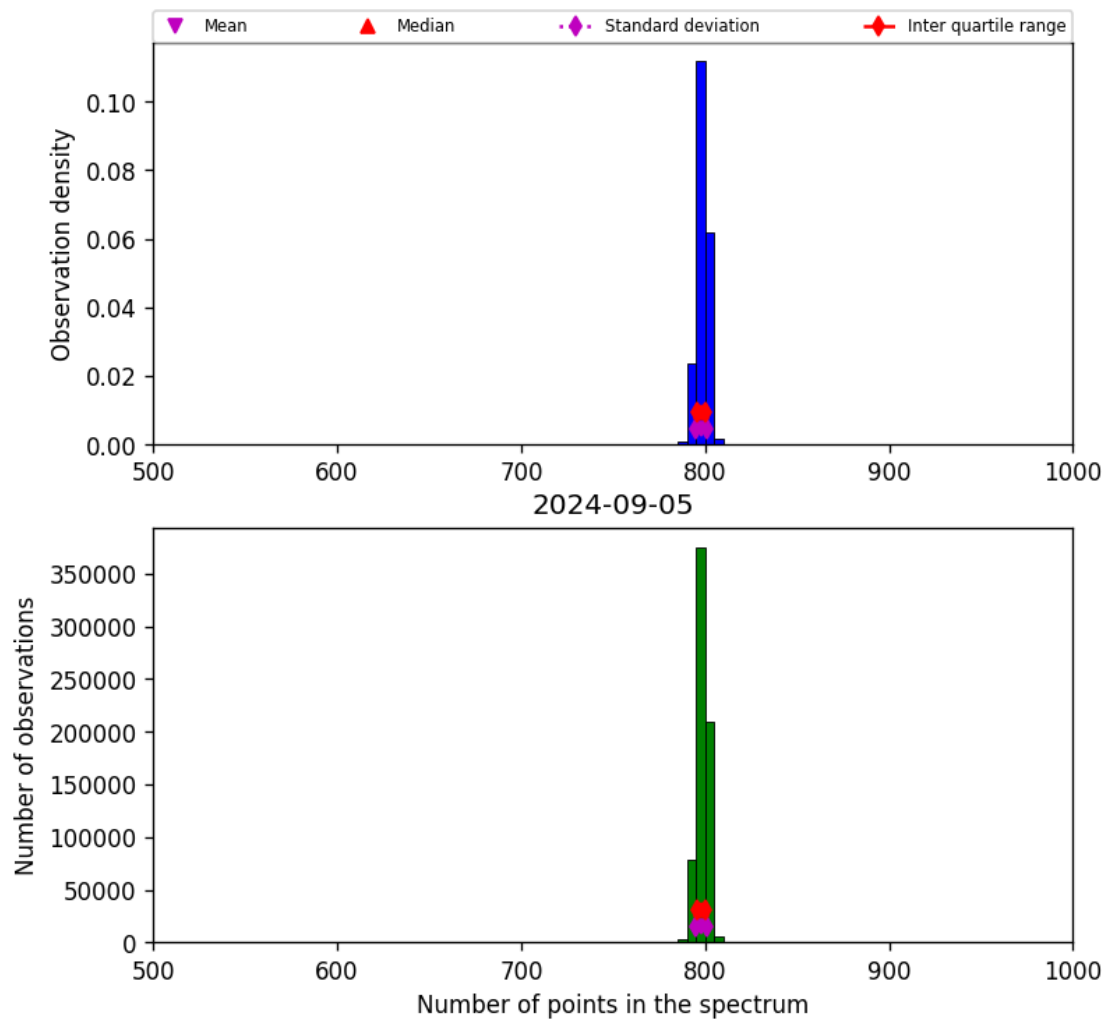
Figure 26: Histogram of “Number of points in the spectrum” for 2024-09-04 to 2024-09-06
