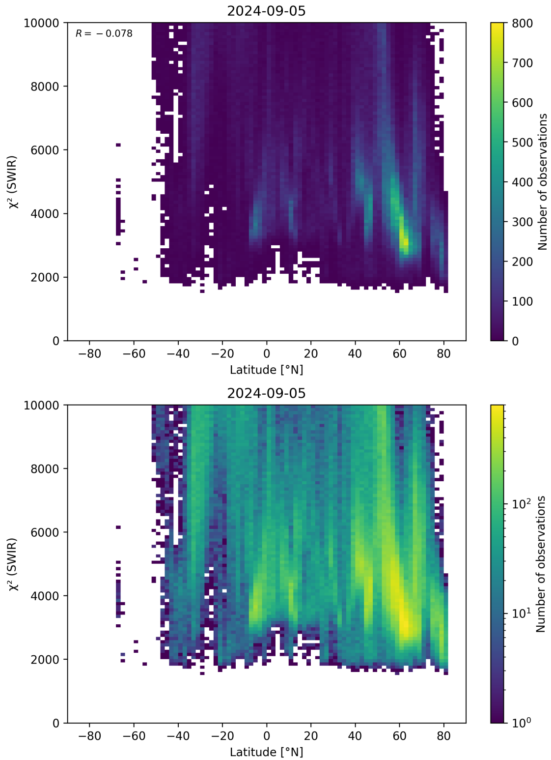
Figure 54: Scatter density plot of “Latitude” against “ \chi^2 (SWIR)” for 2024-09-04 to 2024-09-06.
