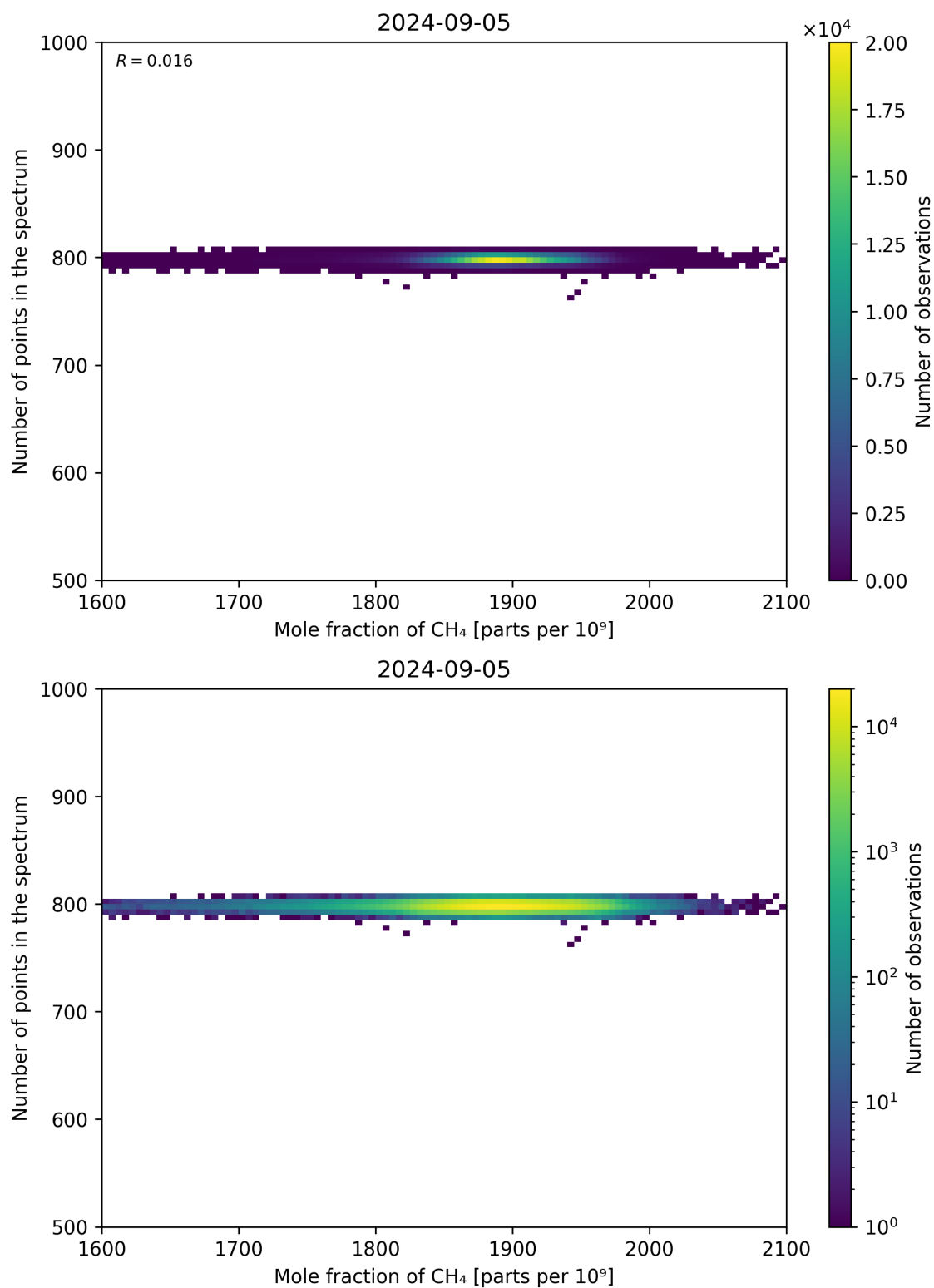
Figure 77: Scatter density plot of “Mole fraction of CH 4 ” against “Number of points in the spectrum” for 2024-09-04 to 2024-09-06.
