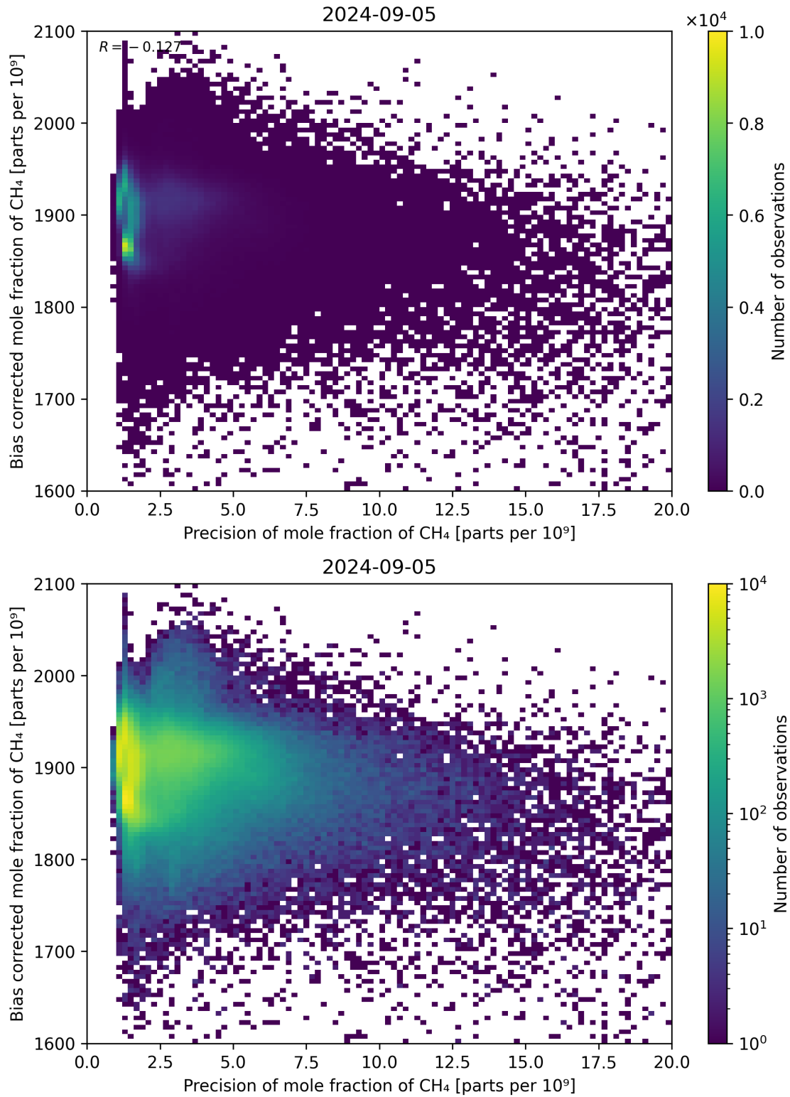
Figure 82: Scatter density plot of “Precision of mole fraction of \text{CH}_4 ” against “Bias corrected mole fraction of \text{CH}_4 ” for 2024-09-04 to 2024-09-06.
