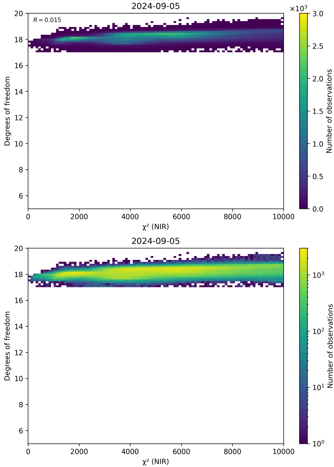
Figure 44: Scatter density plot of “ \chi^2 (NIR)” against “Degrees of freedom” for 2024-09-04 to 2024-09-06.
