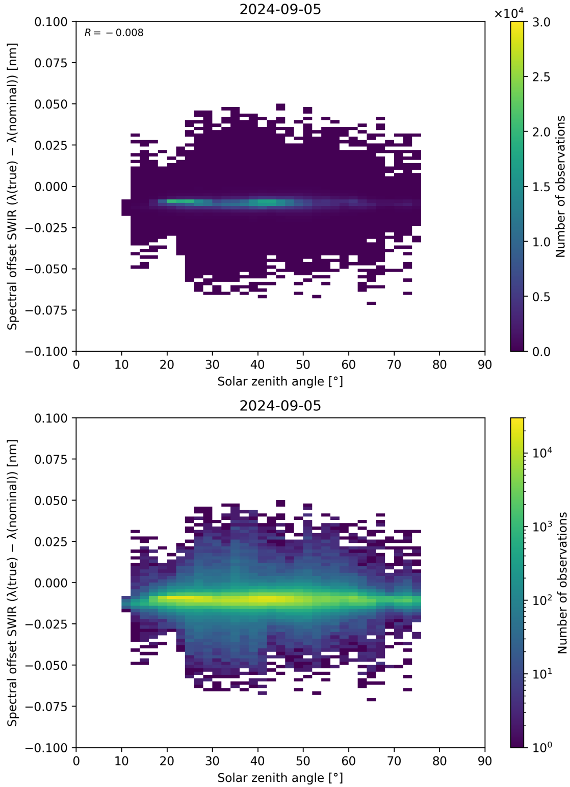
Figure 104: Scatter density plot of “Solar zenith angle” against “Spectral offset SWIR ( \lambda_{\text{true}} - \lambda_{\text{nominal}} )” for 2024-09-04 to 2024-09-06.
