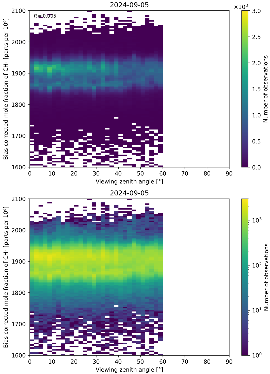
Figure 111: Scatter density plot of “Viewing zenith angle” against “Bias corrected mole fraction of CH 4 ” for 2024-09-04 to 2024-09-06.
