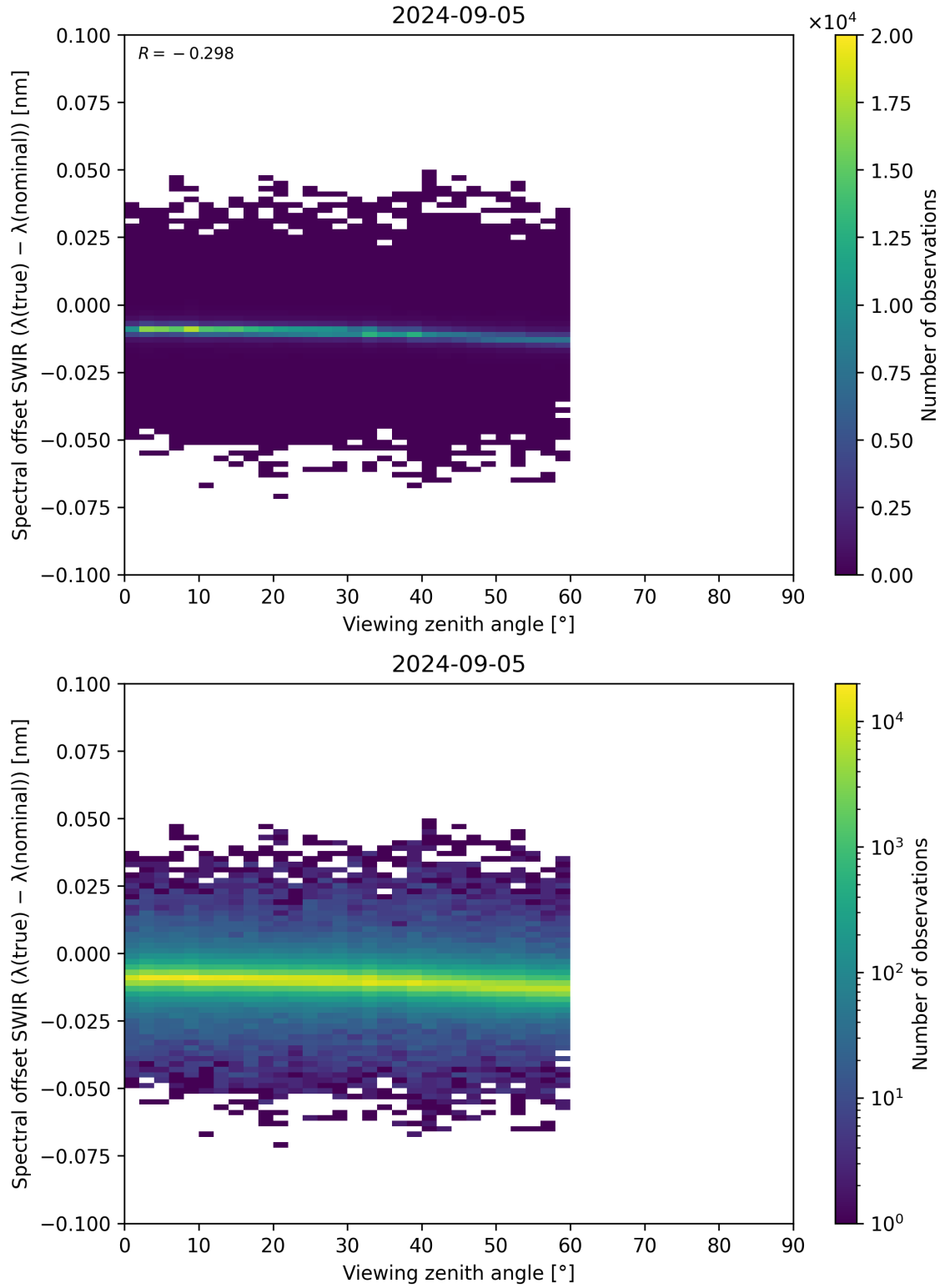
Figure 116: Scatter density plot of “Viewing zenith angle” against “Spectral offset SWIR ( \lambda_{\text{true}} - \lambda_{\text{nominal}} )” for 2024-09-04 to 2024-09-06.
