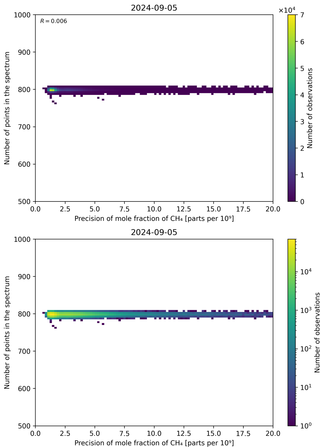
Figure 84: Scatter density plot of “Precision of mole fraction of CH 4 ” against “Number of points in the spectrum” for 2024-09-04 to 2024-09-06.
