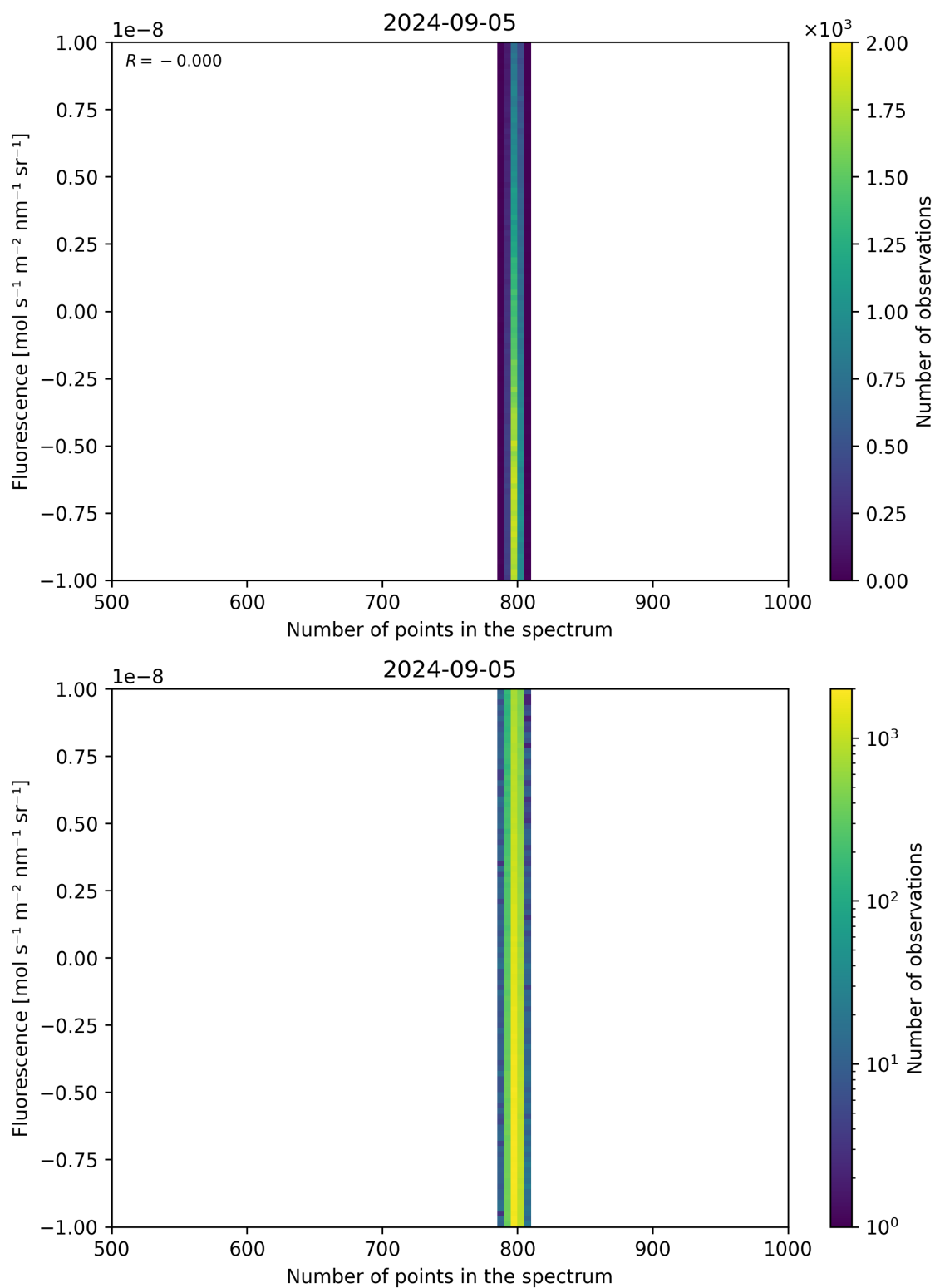
Figure 91: Scatter density plot of “Number of points in the spectrum” against “Fluorescence” for 2024-09-04 to 2024-09-06.
