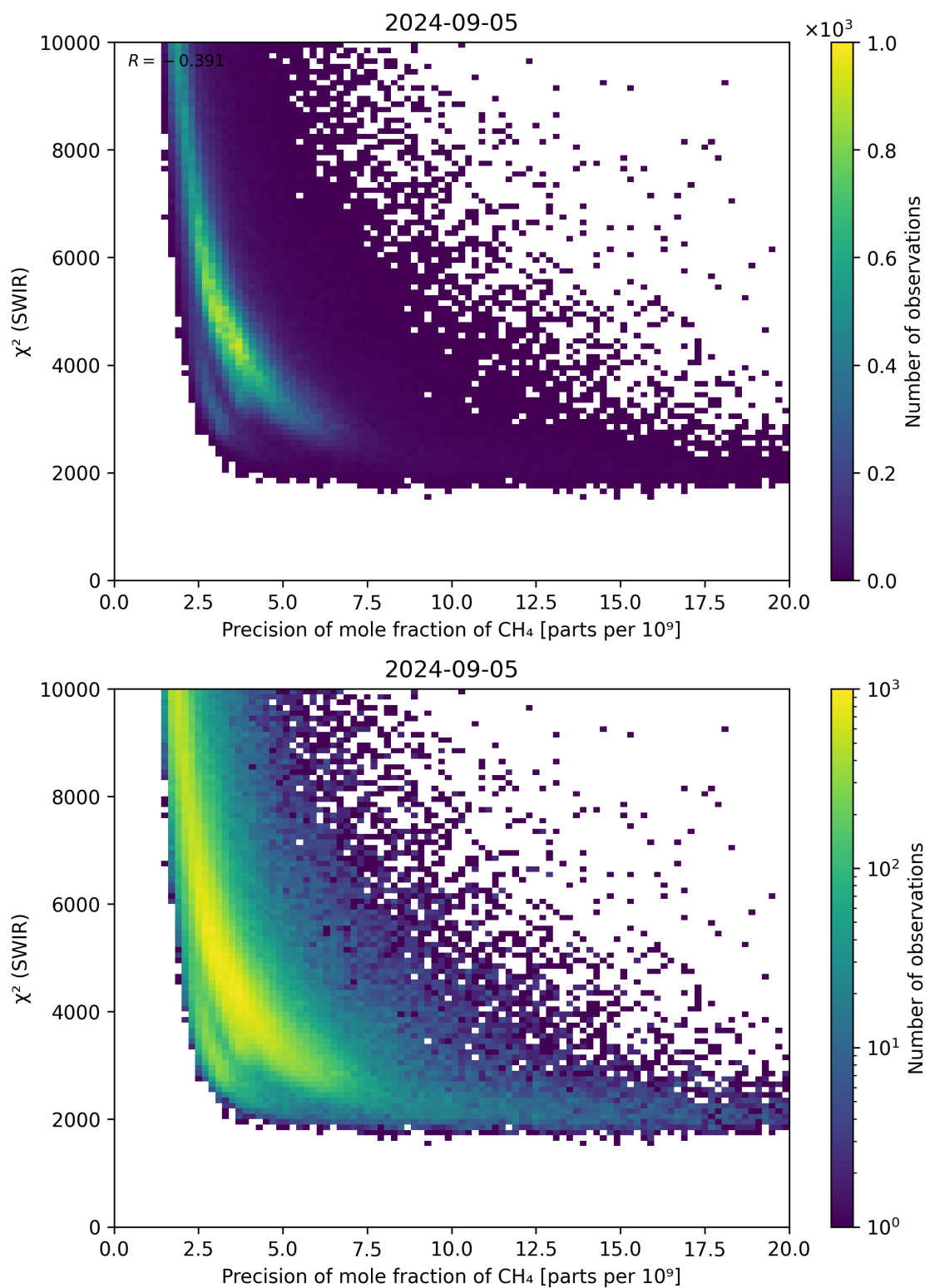
Figure 79: Scatter density plot of “Precision of mole fraction of \text{CH}_4 ” against “ \chi^2 (SWIR)” for 2024-09-04 to 2024-09-06.
