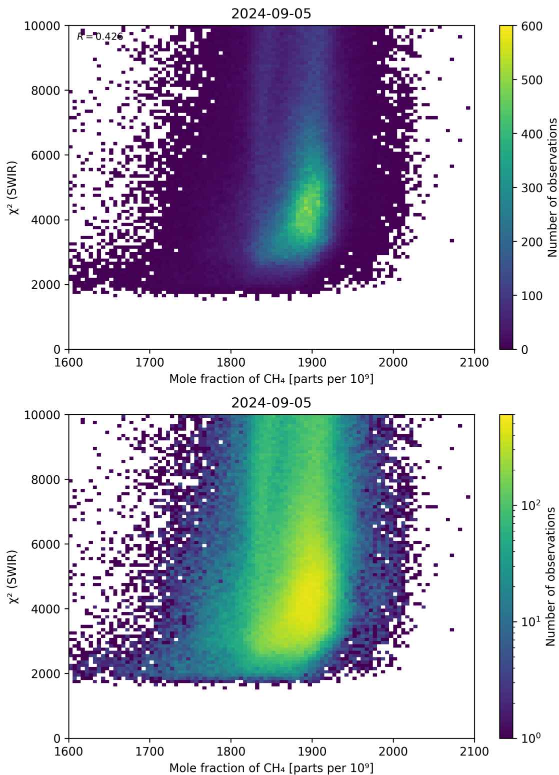
Figure 71: Scatter density plot of “Mole fraction of \text{CH}_4 ” against “ \chi^2 (SWIR)” for 2024-09-04 to 2024-09-06.
