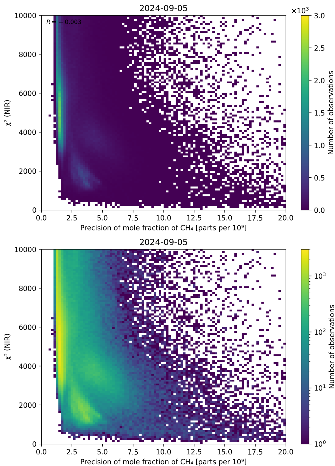
Figure 78: Scatter density plot of “Precision of mole fraction of \text{CH}_4 ” against “ \chi^2 (NIR)” for 2024-09-04 to 2024-09-06.
