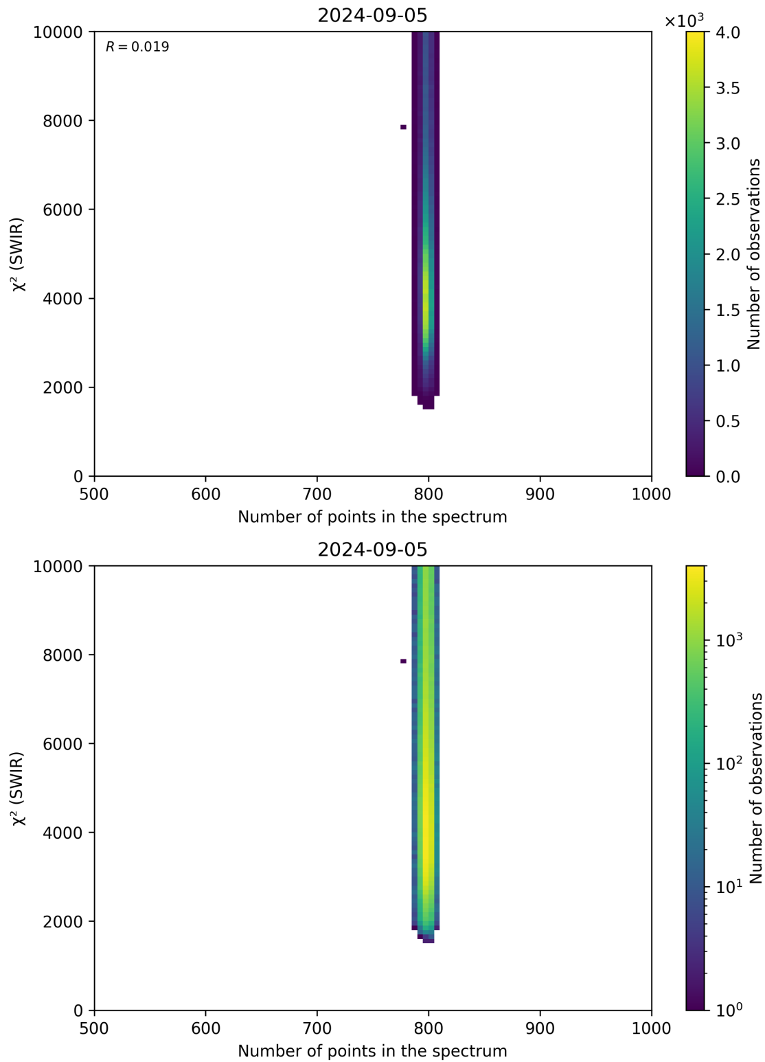
Figure 89: Scatter density plot of “Number of points in the spectrum” against “ \chi^2 (SWIR)” for 2024-09-04 to 2024-09-06.
