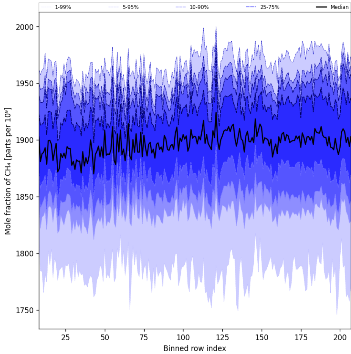
Figure 34: Along track statistics of “Mole fraction of CH 4 ” for 2024-09-06 to 2024-09-08
