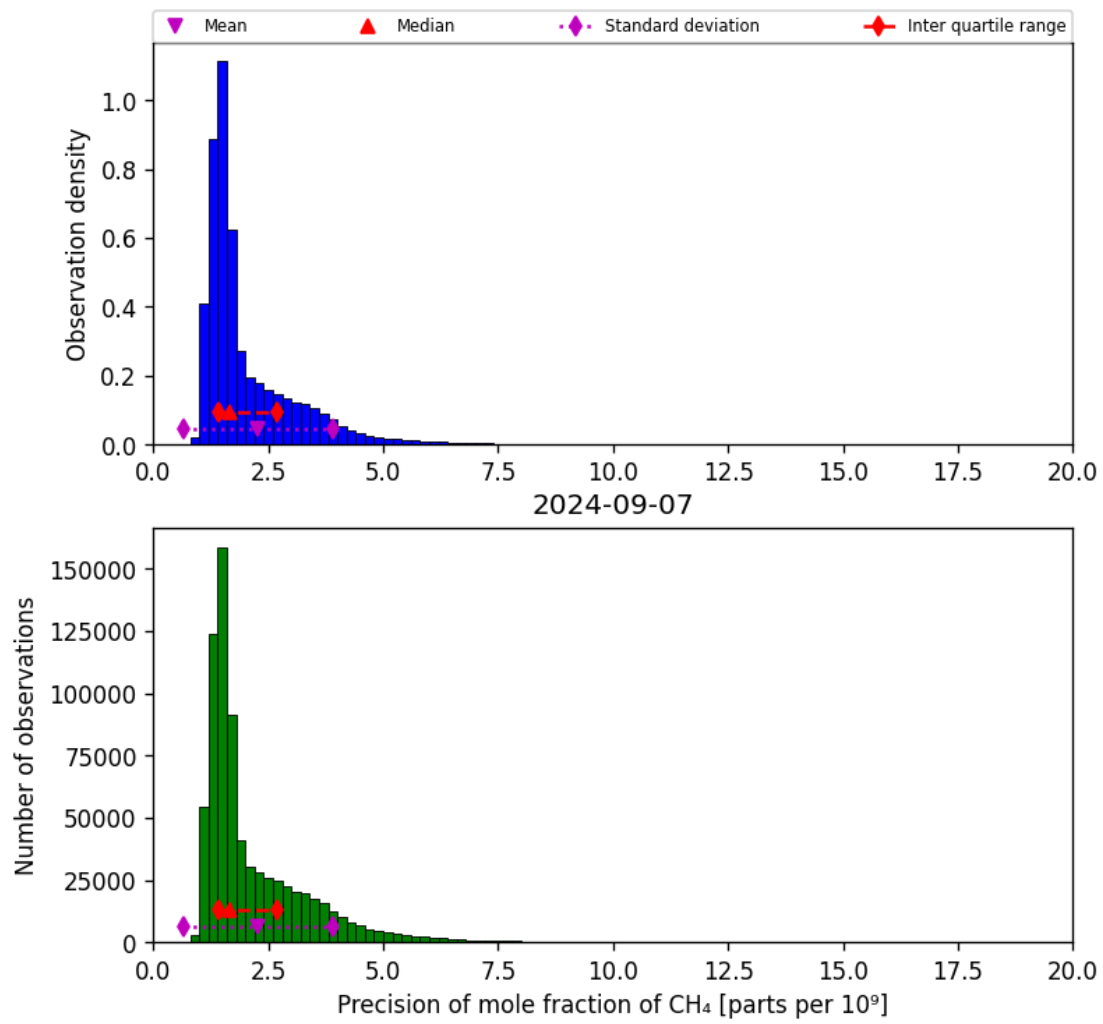
Figure 24: Histogram of “Precision of mole fraction of CH 4 ” for 2024-09-06 to 2024-09-08
