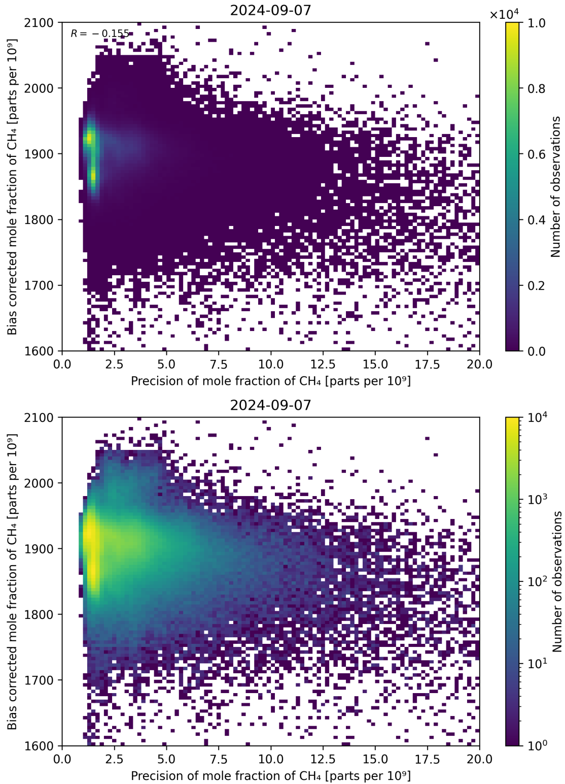
Figure 82: Scatter density plot of “Precision of mole fraction of \text{CH}_4 ” against “Bias corrected mole fraction of \text{CH}_4 ” for 2024-09-06 to 2024-09-08.
