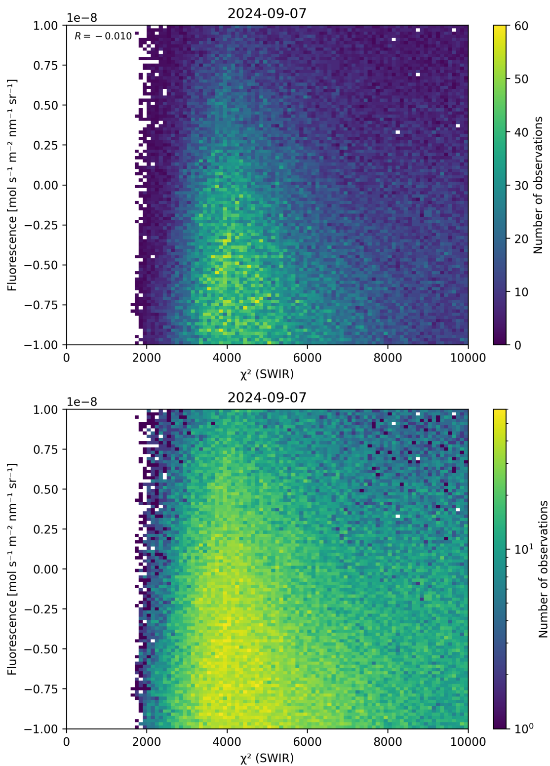
Figure 49: Scatter density plot of “ \chi^2 (SWIR)” against “Fluorescence” for 2024-09-06 to 2024-09-08.
