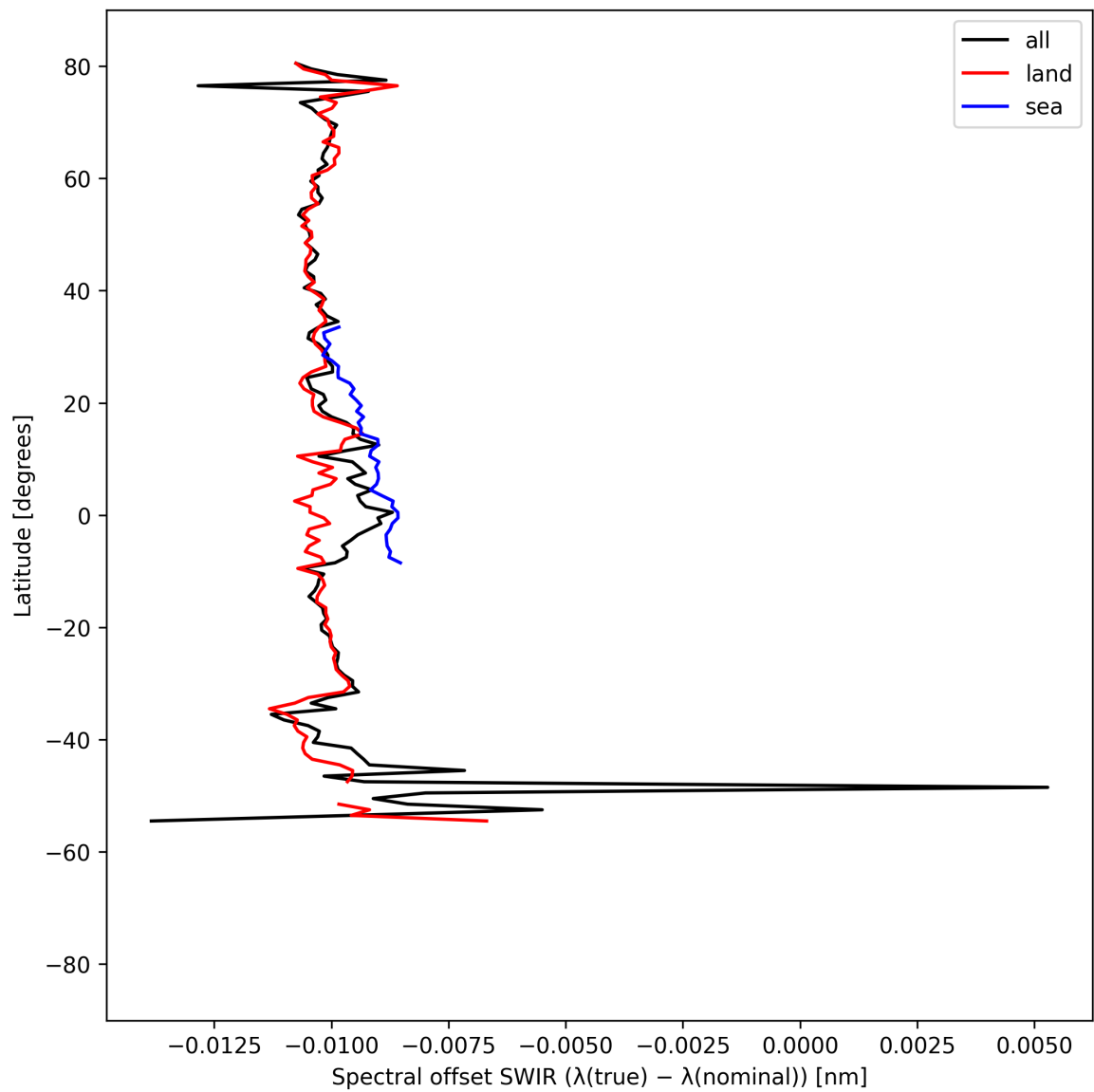
Figure 16: Zonal average of “Spectral offset SWIR ( \lambda_{\text{true}} - \lambda_{\text{nominal}} )” for 2024-09-06 to 2024-09-08.
