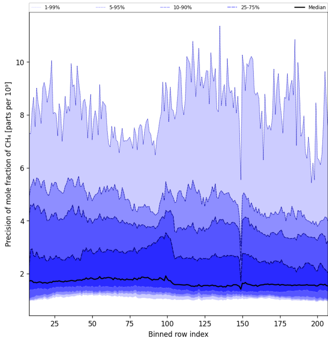
Figure 35: Along track statistics of “Precision of mole fraction of CH 4 ” for 2024-09-06 to 2024-09-08
