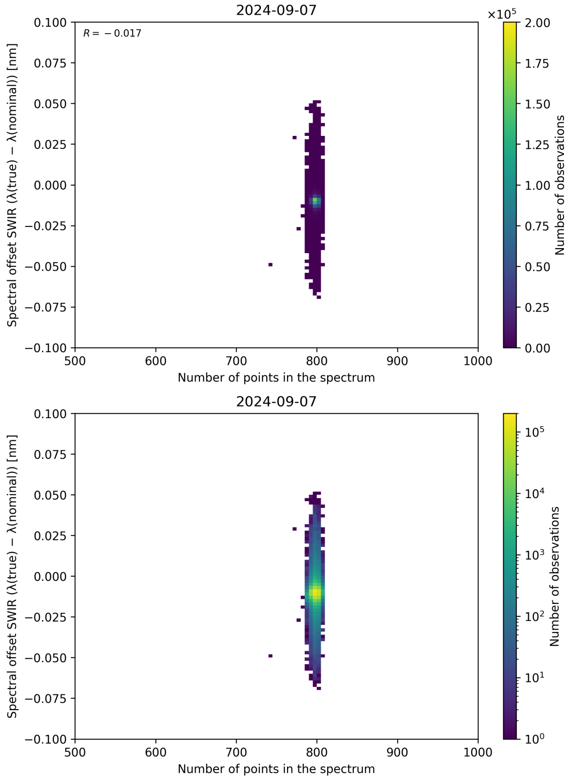
Figure 93: Scatter density plot of “Number of points in the spectrum” against “Spectral offset SWIR ( \lambda_{\text{true}} - \lambda_{\text{nominal}} )” for 2024-09-06 to 2024-09-08.
