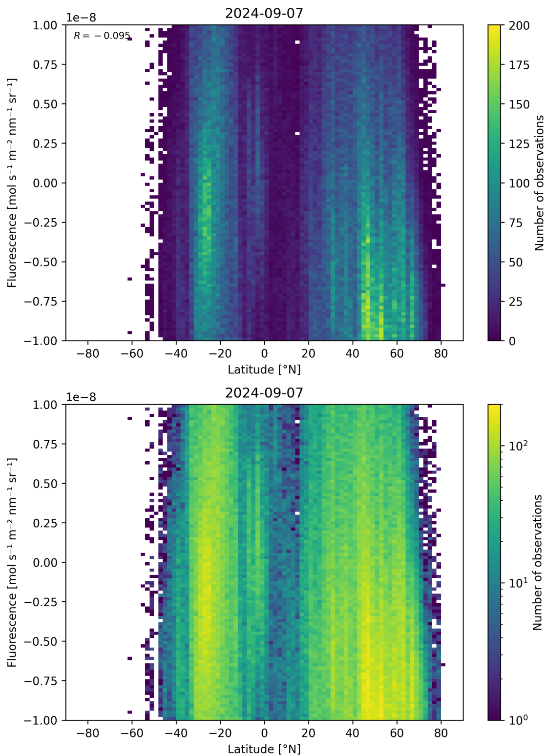
Figure 56: Scatter density plot of “Latitude” against “Fluorescence” for 2024-09-06 to 2024-09-08.
