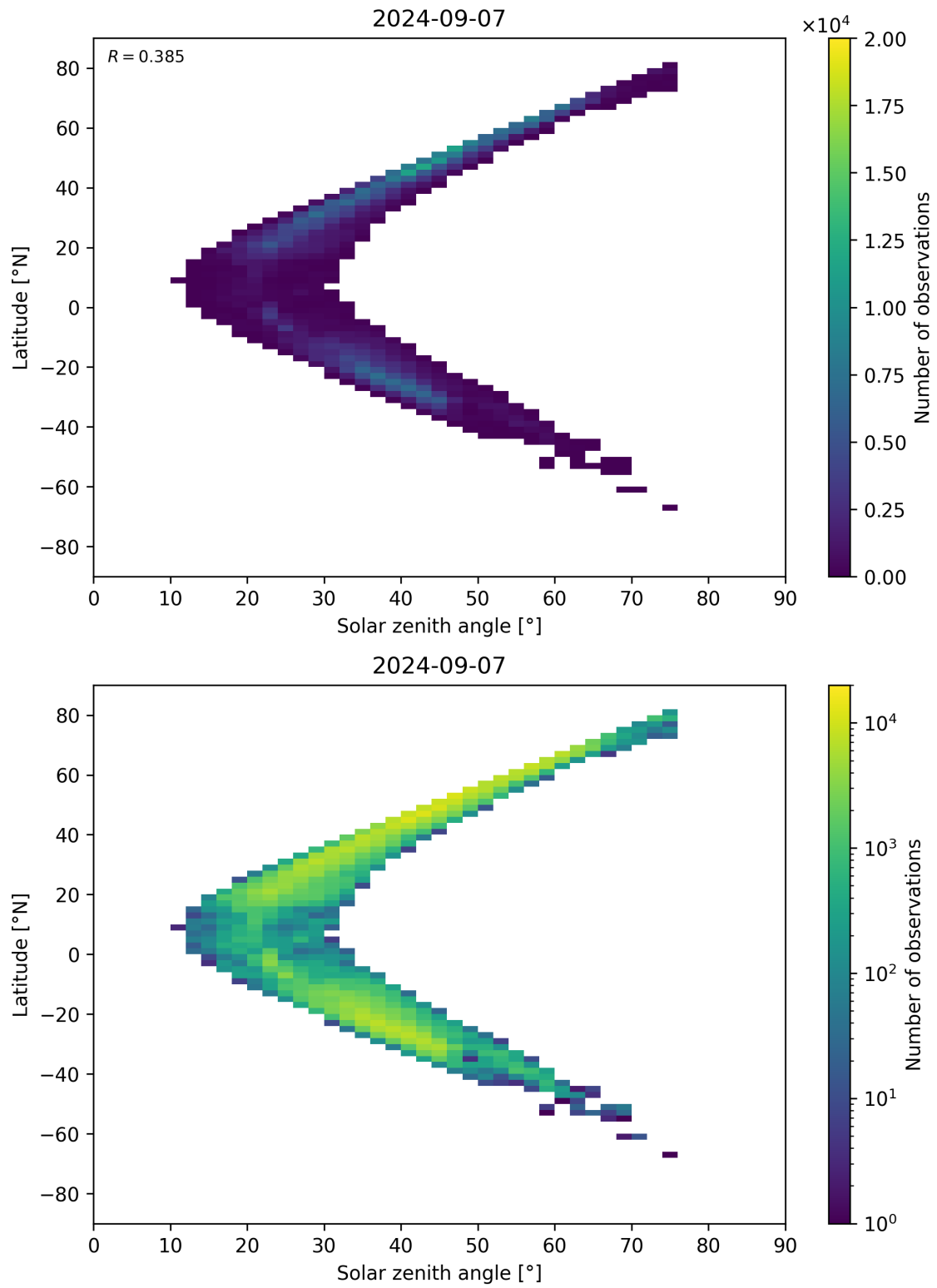
Figure 98: Scatter density plot of “Solar zenith angle” against “Latitude” for 2024-09-06 to 2024-09-08.
