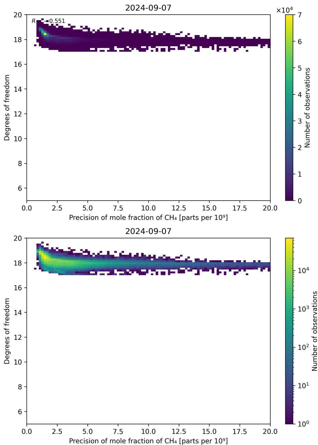
Figure 80: Scatter density plot of “Precision of mole fraction of CH 4 ” against “Degrees of freedom” for 2024-09-06 to 2024-09-08.
