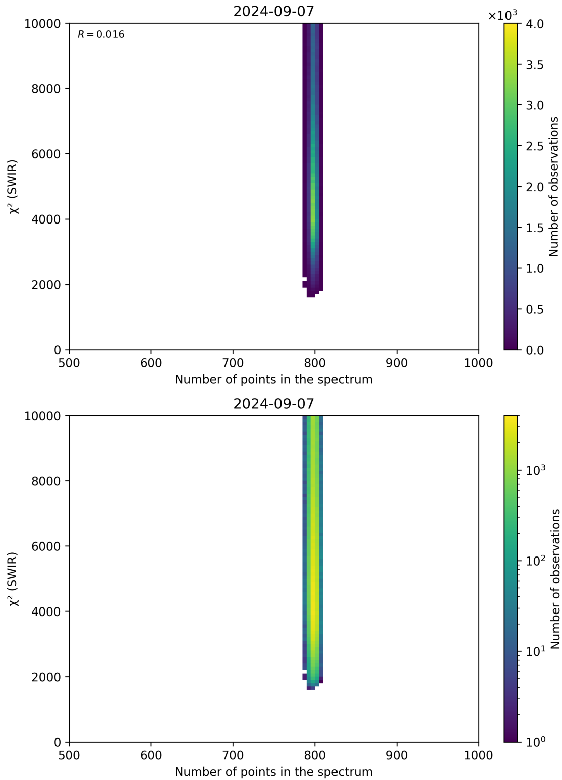
Figure 89: Scatter density plot of “Number of points in the spectrum” against “ \chi^2 (SWIR)” for 2024-09-06 to 2024-09-08.
