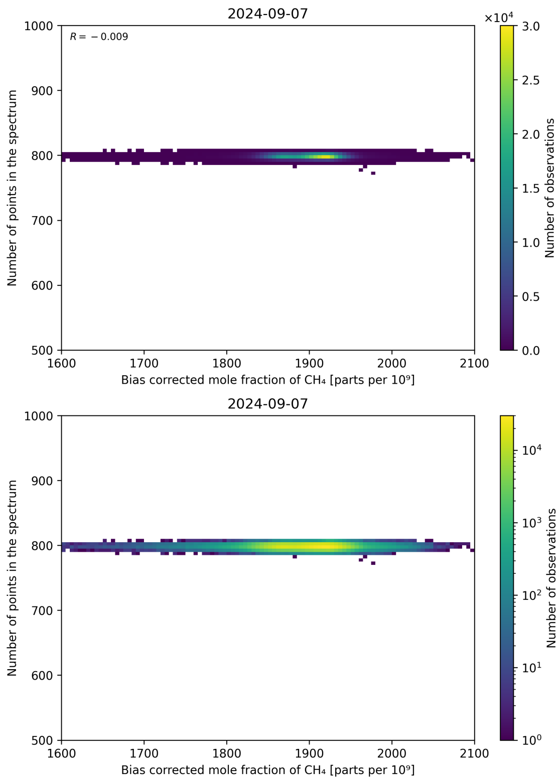
Figure 68: Scatter density plot of “Bias corrected mole fraction of CH 4 ” against “Number of points in the spectrum” for 2024-09-06 to 2024-09-08.
