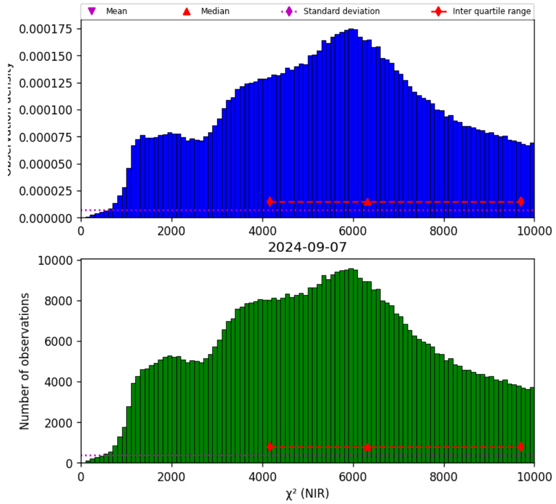
Figure 29: Histogram of “ \chi^2 (NIR)” for 2024-09-06 to 2024-09-08
