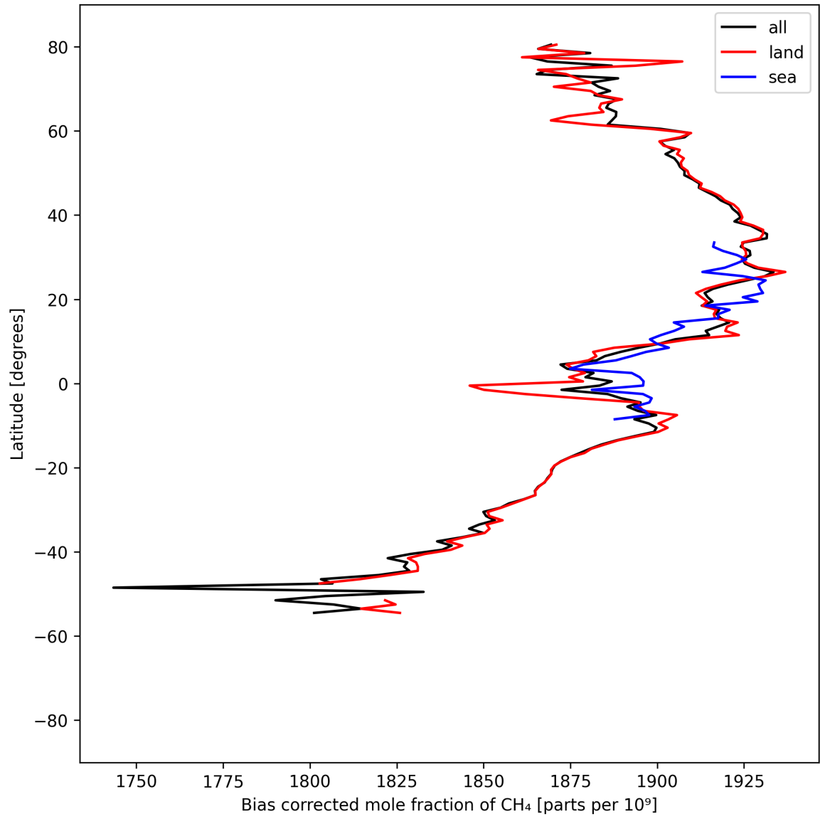
Figure 14: Zonal average of “Bias corrected mole fraction of CH 4 ” for 2024-09-06 to 2024-09-08.
