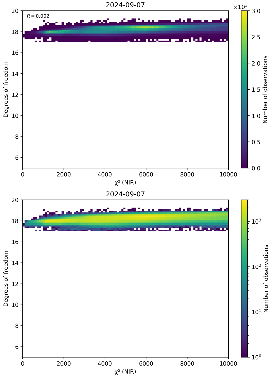
Figure 44: Scatter density plot of “ \chi^2 (NIR)” against “Degrees of freedom” for 2024-09-06 to 2024-09-08.
