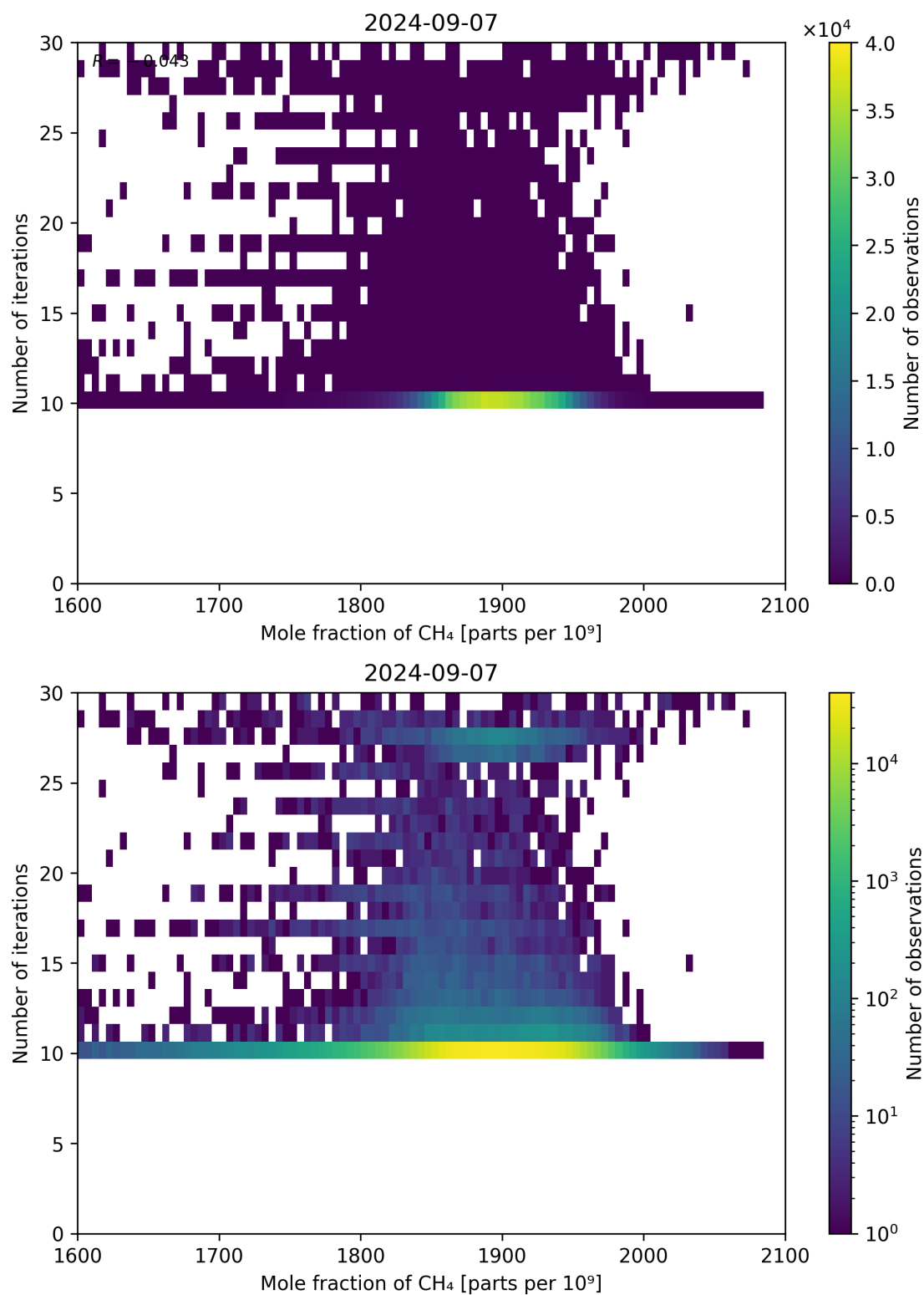
Figure 76: Scatter density plot of “Mole fraction of CH 4 ” against “Number of iterations” for 2024-09-06 to 2024-09-08.
