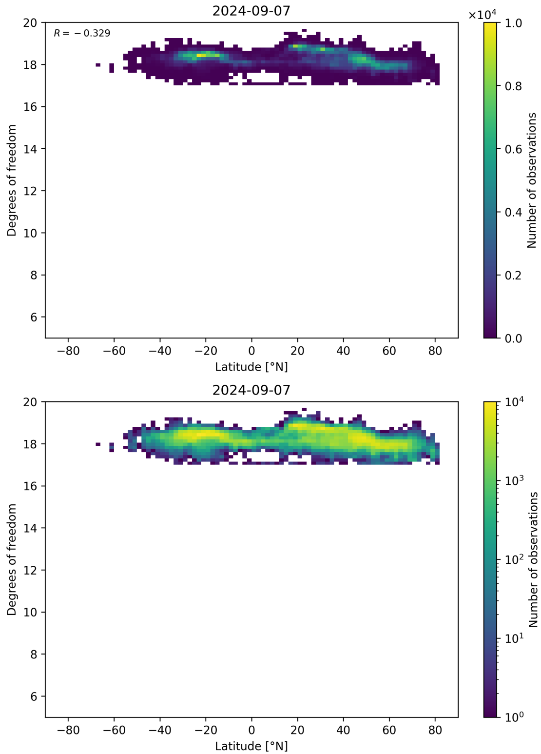
Figure 55: Scatter density plot of “Latitude” against “Degrees of freedom” for 2024-09-06 to 2024-09-08.
