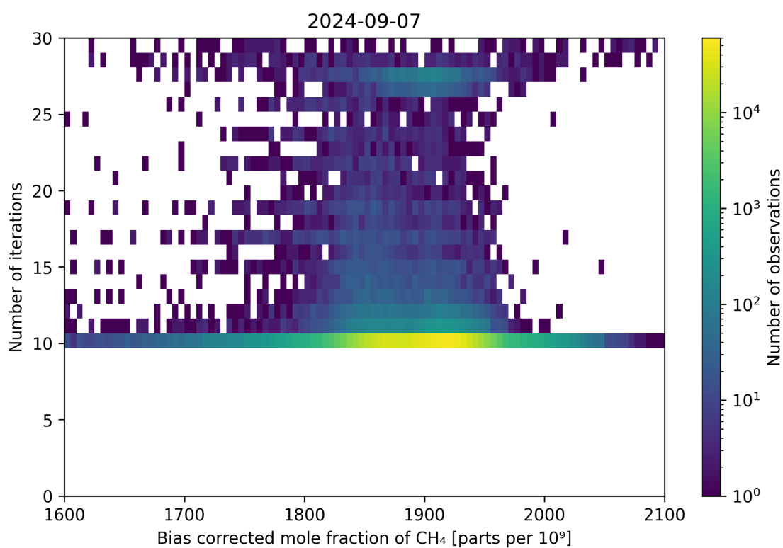
Figure 67: Scatter density plot of “Bias corrected mole fraction of CH 4 ” against “Number of iterations” for 2024-09-06 to 2024-09-08.
