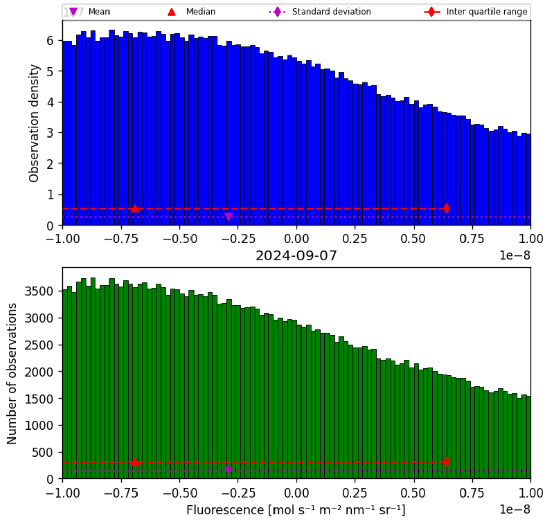
Figure 32: Histogram of “Fluorescence” for 2024-09-06 to 2024-09-08
