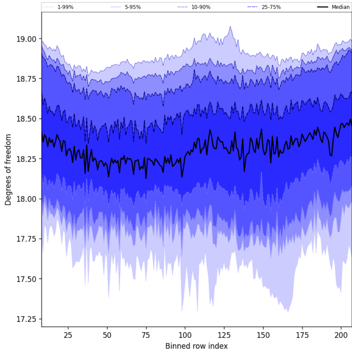
Figure 41: Along track statistics of “Degrees of freedom” for 2024-09-06 to 2024-09-08
