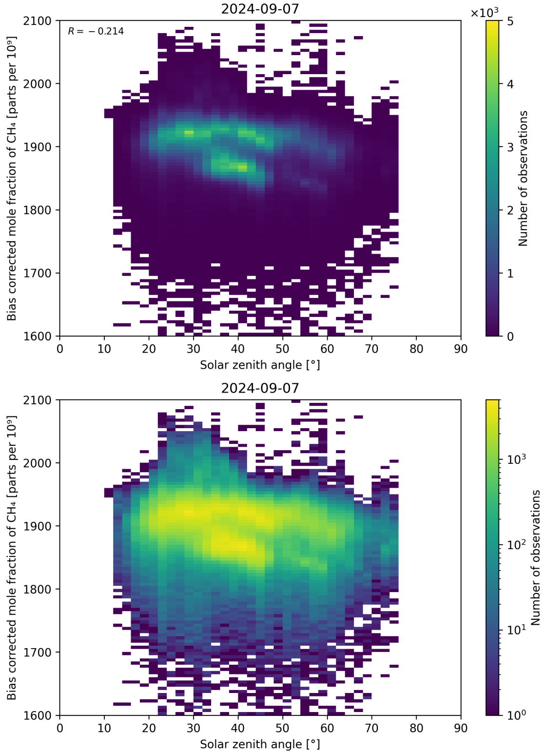
Figure 100: Scatter density plot of “Solar zenith angle” against “Bias corrected mole fraction of CH 4 ” for 2024-09-06 to 2024-09-08.
