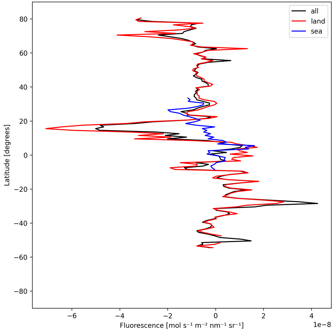
Figure 21: Zonal average of “Fluorescence” for 2024-09-06 to 2024-09-08.
