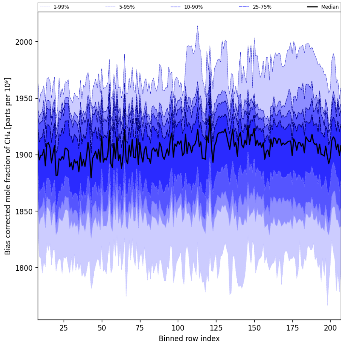
Figure 36: Along track statistics of “Bias corrected mole fraction of CH 4 ” for 2024-09-06 to 2024-09-08
