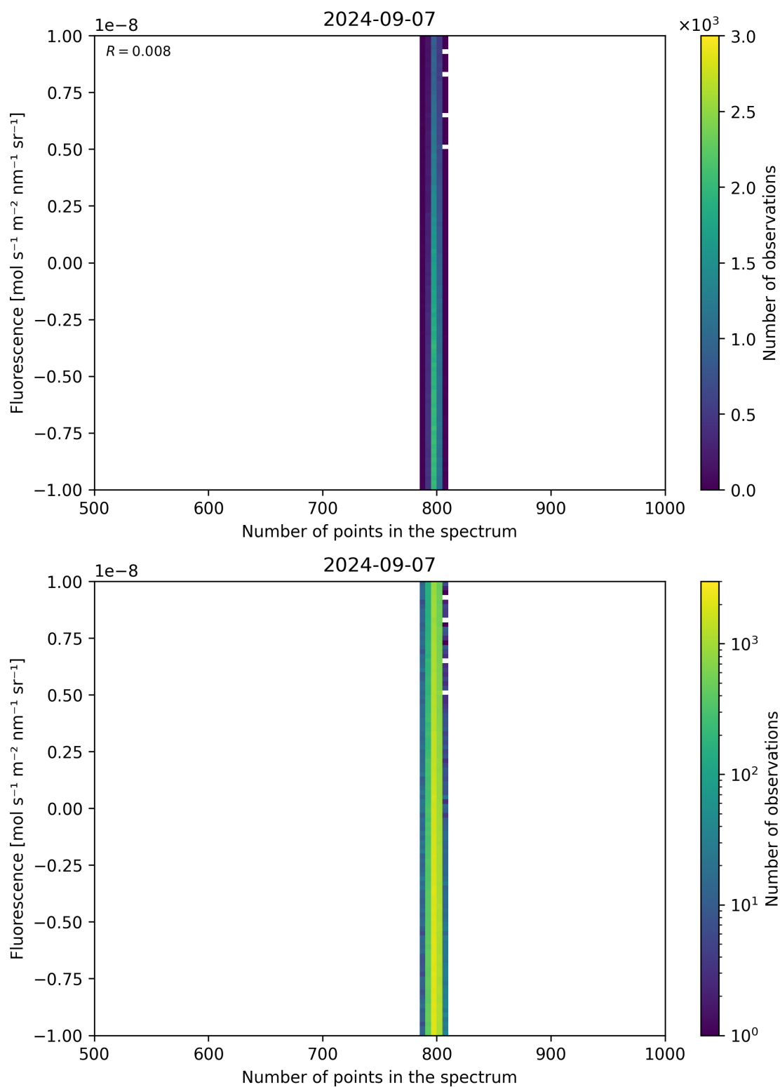
Figure 91: Scatter density plot of “Number of points in the spectrum” against “Fluorescence” for 2024-09-06 to 2024-09-08.
