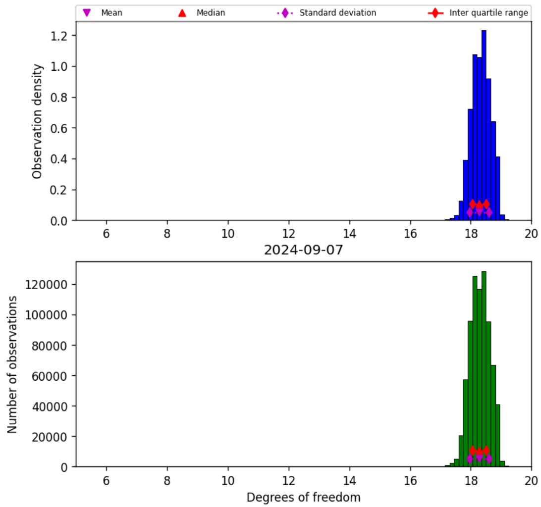
Figure 30: Histogram of “Degrees of freedom” for 2024-09-06 to 2024-09-08
