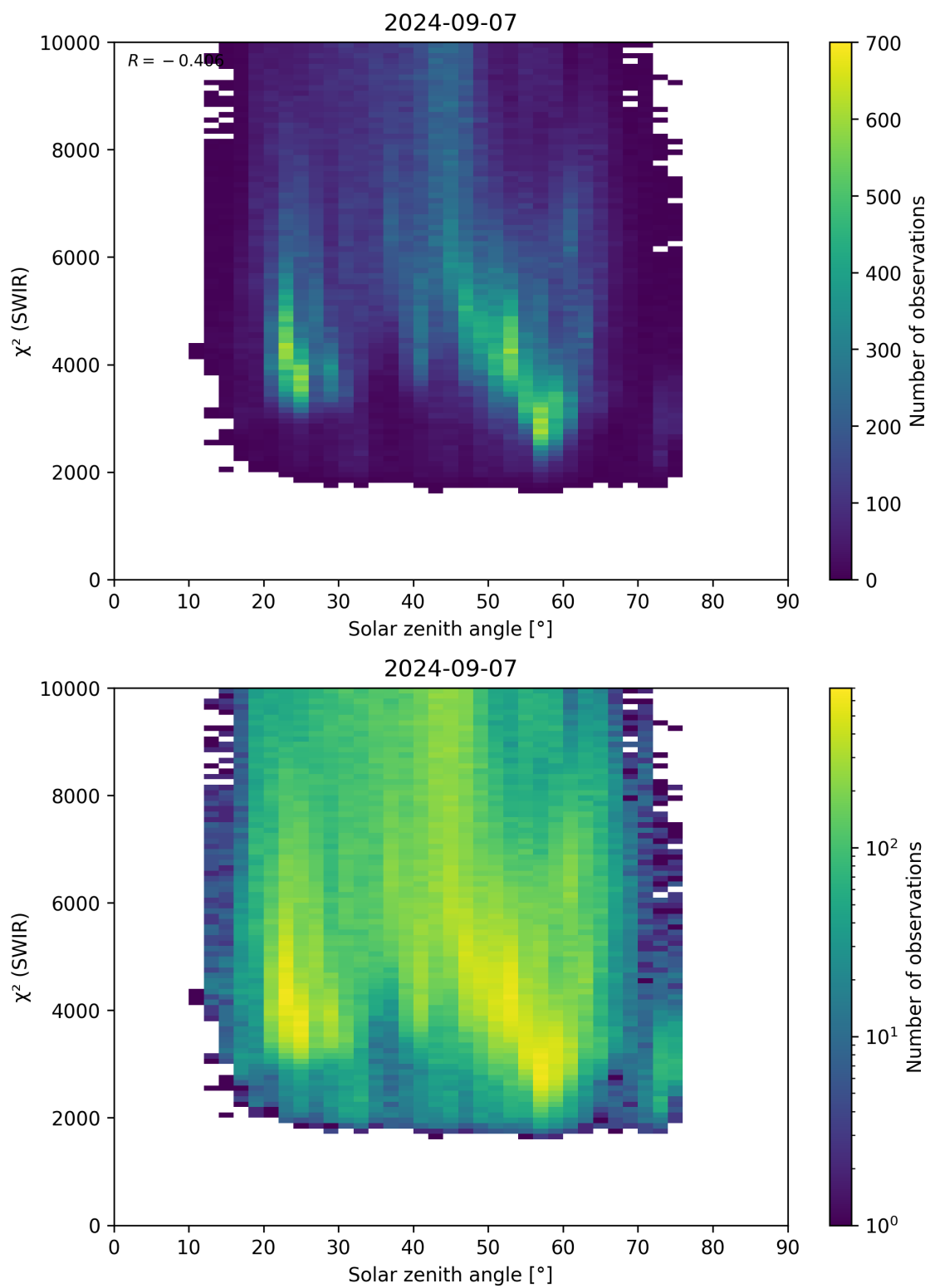
Figure 95: Scatter density plot of “Solar zenith angle” against “ \chi^2 (SWIR)” for 2024-09-06 to 2024-09-08.
