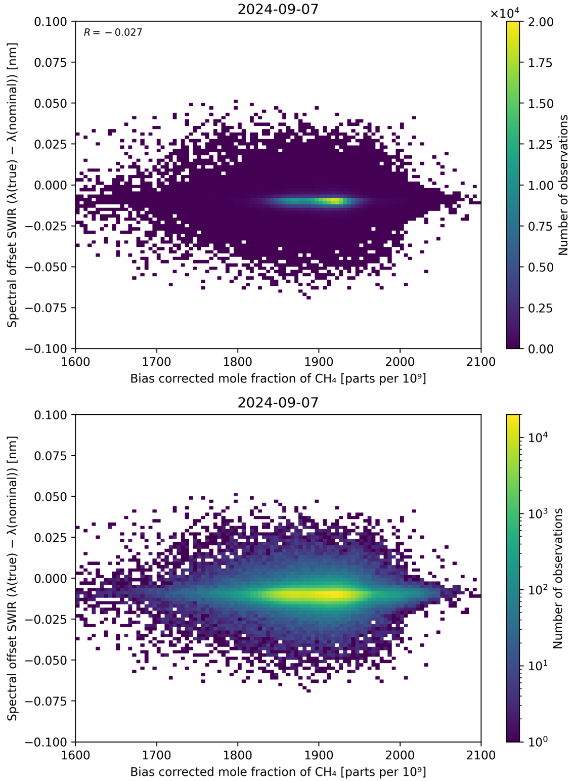
Figure 69: Scatter density plot of “Bias corrected mole fraction of \text{CH}_4 ” against “Spectral offset SWIR ( \lambda_{\text{true}} - \lambda_{\text{nominal}} )” for 2024-09-06 to 2024-09-08.
