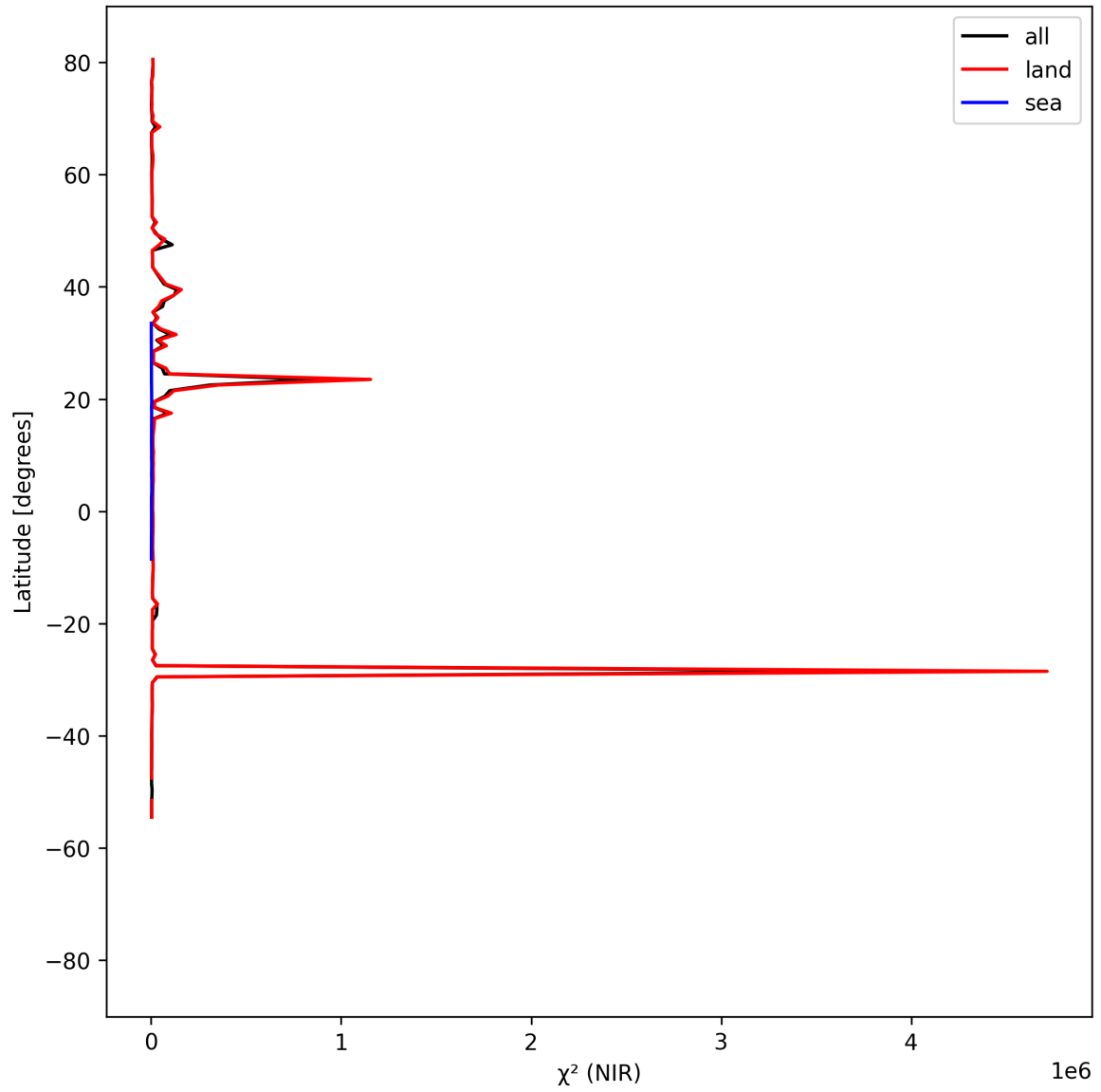
Figure 18: Zonal average of “ \chi^2 (NIR)” for 2024-09-06 to 2024-09-08.
