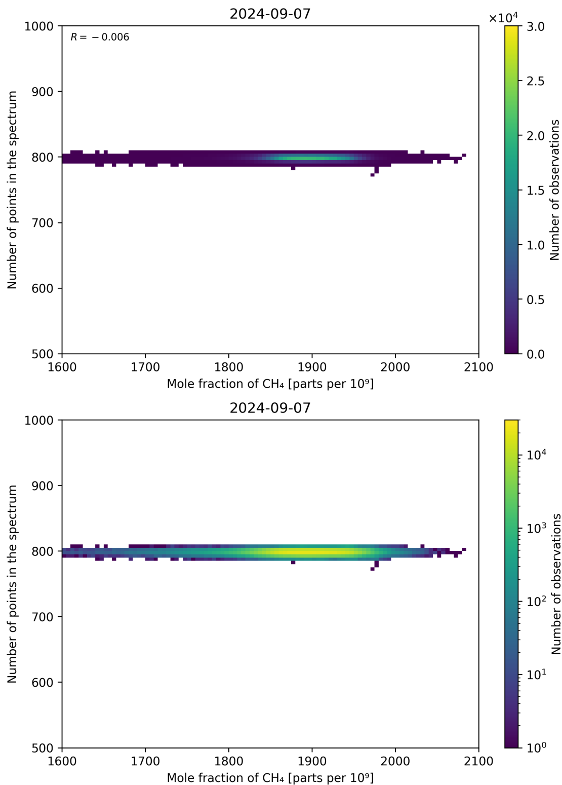
Figure 77: Scatter density plot of “Mole fraction of CH 4 ” against “Number of points in the spectrum” for 2024-09-06 to 2024-09-08.
