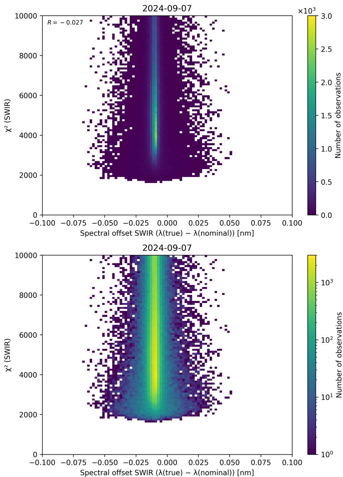
Figure 118: Scatter density plot of “Spectral offset SWIR ( \lambda_{\text{true}} - \lambda_{\text{nominal}} )” against “ \chi^2 (SWIR)” for 2024-09-06 to 2024-09-08.
