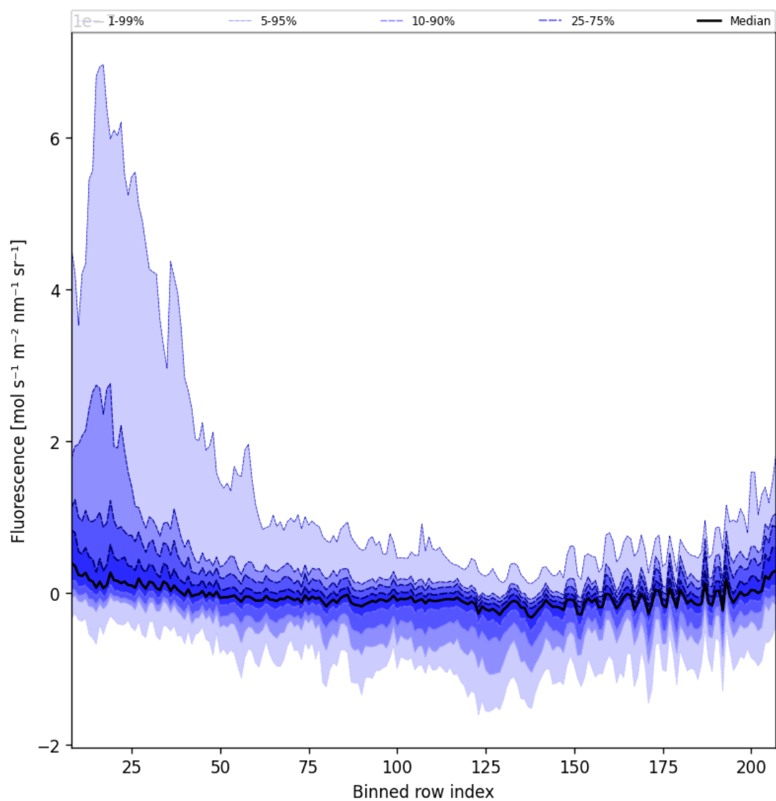
Figure 43: Along track statistics of “Fluorescence” for 2024-09-06 to 2024-09-08
