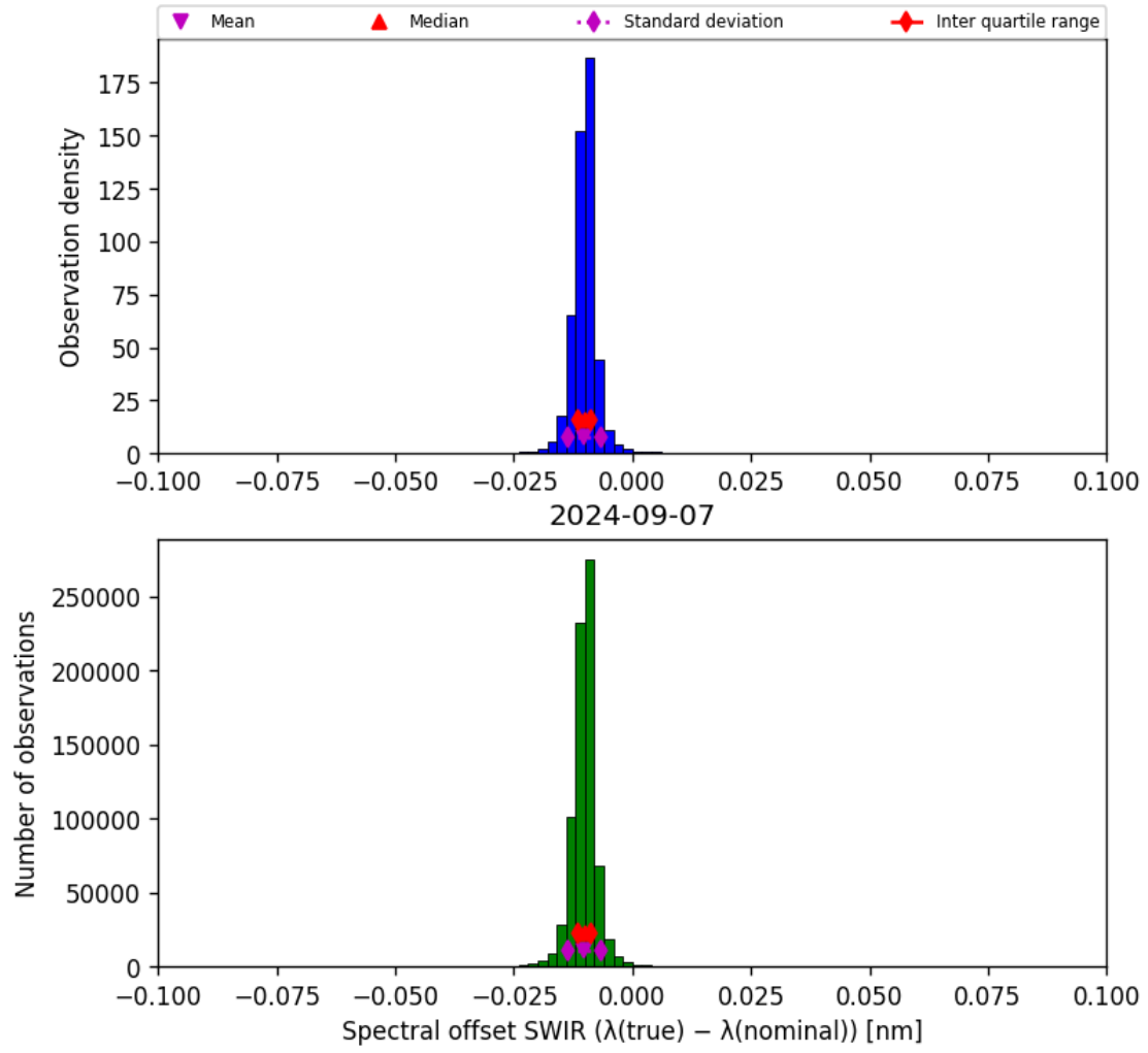
Figure 27: Histogram of “Spectral offset SWIR ( \lambda_{\text{true}} - \lambda_{\text{nominal}} )” for 2024-09-06 to 2024-09-08
