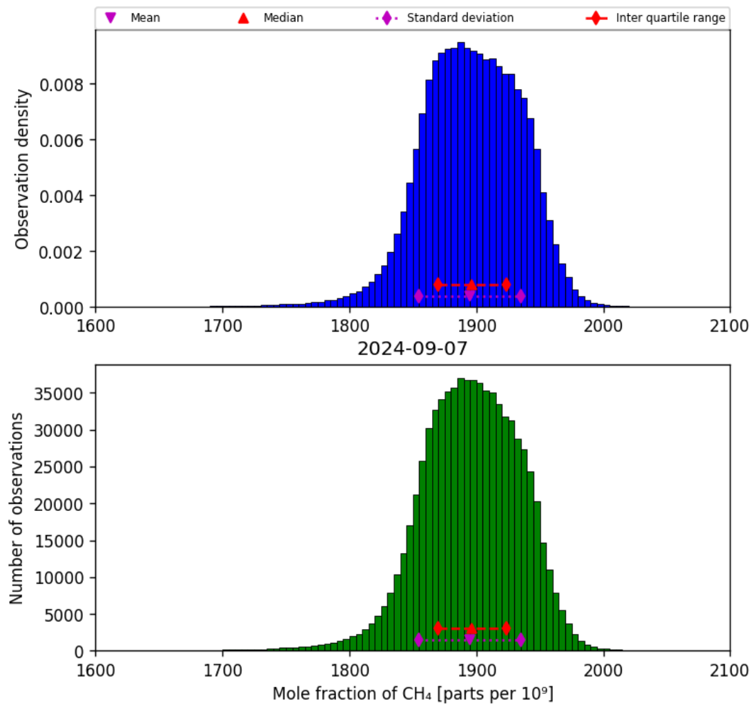
Figure 23: Histogram of “Mole fraction of CH 4 ” for 2024-09-06 to 2024-09-08
