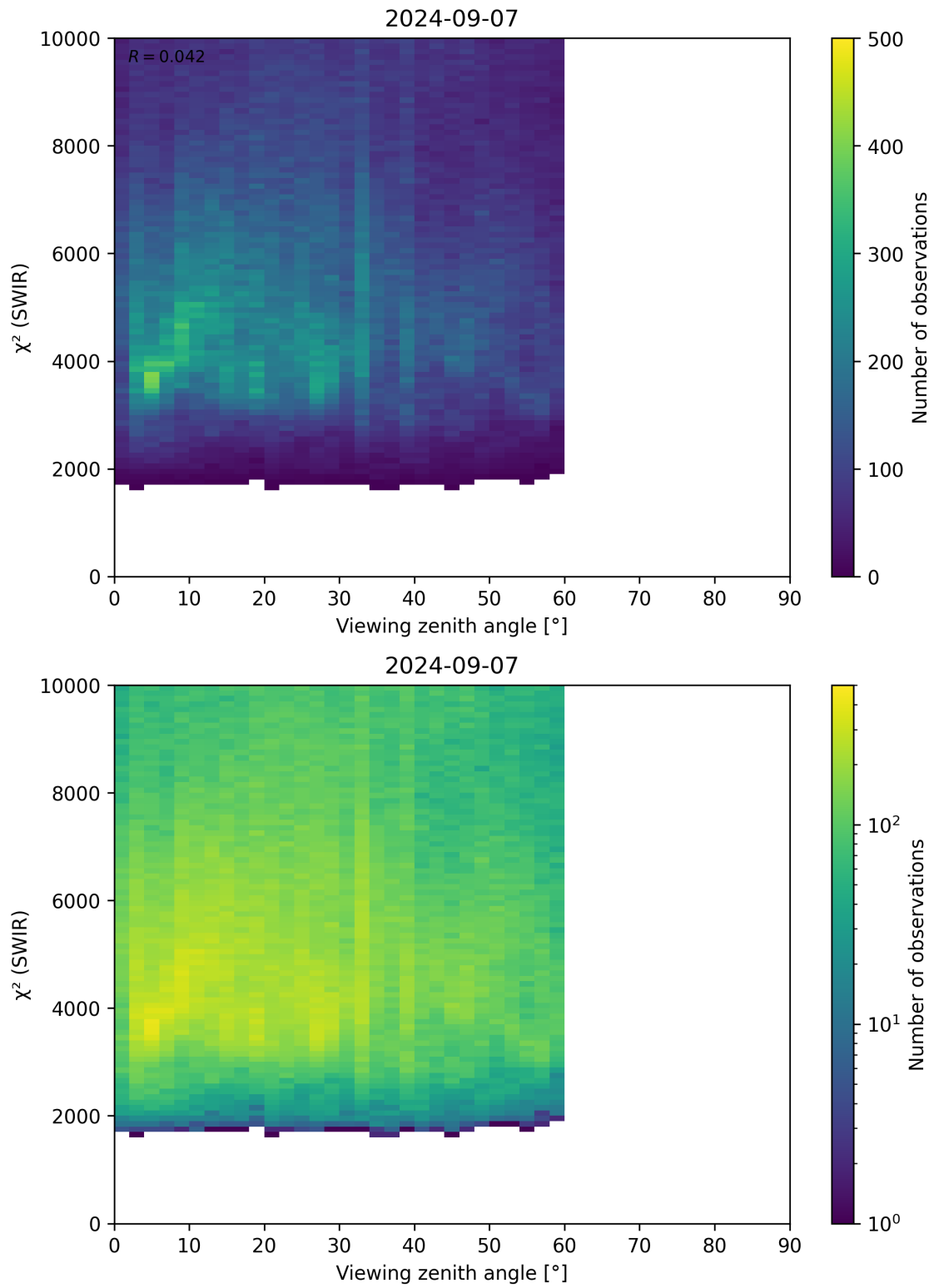
Figure 106: Scatter density plot of “Viewing zenith angle” against “ \chi^2 (SWIR)” for 2024-09-06 to 2024-09-08.
