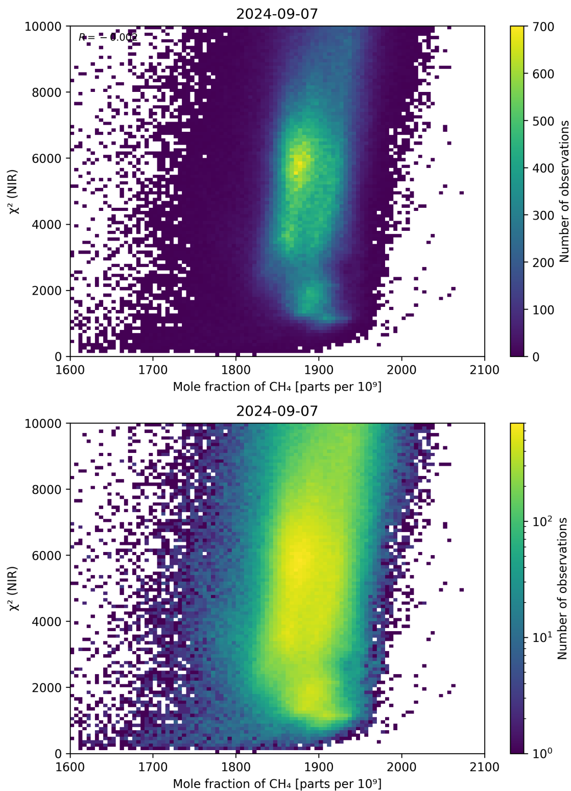
Figure 70: Scatter density plot of “Mole fraction of CH 4 ” against “ \chi^2 (NIR)” for 2024-09-06 to 2024-09-08.
