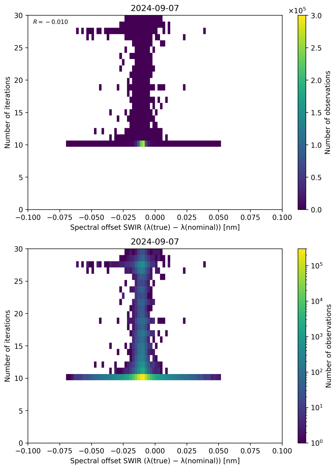
Figure 121: Scatter density plot of “Spectral offset SWIR ( \lambda_{\text{true}} - \lambda_{\text{nominal}} )” against “Number of iterations” for 2024-09-06 to 2024-09-08.
