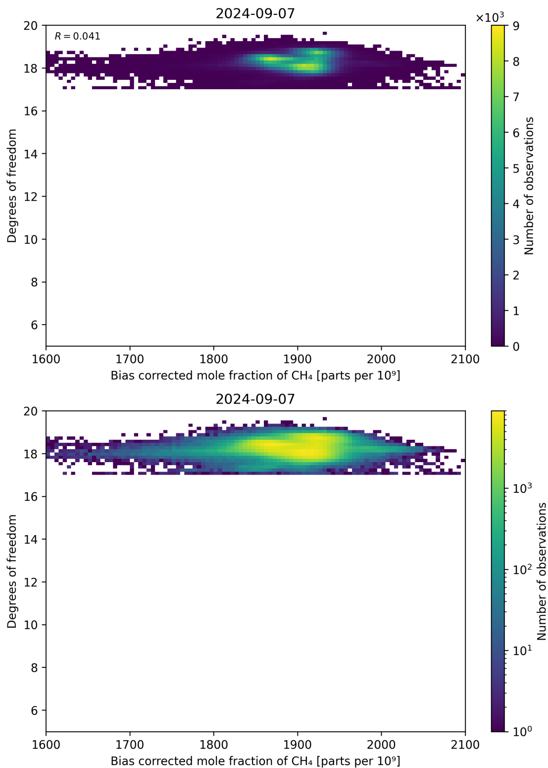
Figure 65: Scatter density plot of “Bias corrected mole fraction of CH 4 ” against “Degrees of freedom” for 2024-09-06 to 2024-09-08.
