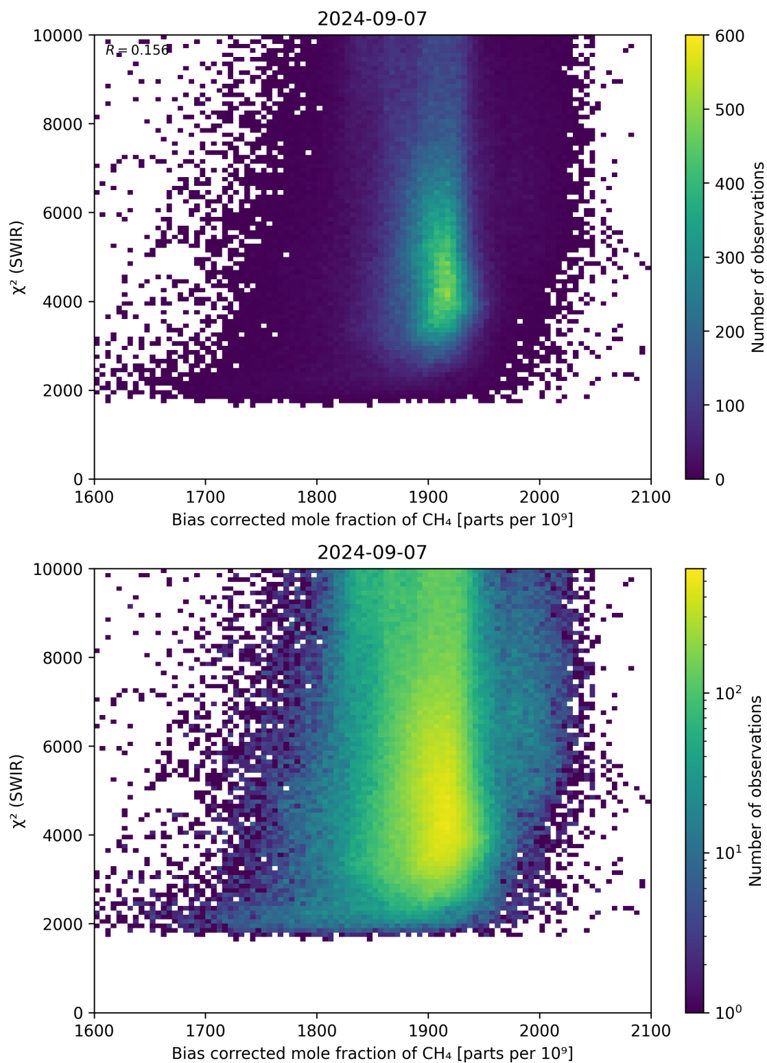
Figure 64: Scatter density plot of “Bias corrected mole fraction of \text{CH}_4 ” against “ \chi^2 (SWIR)” for 2024-09-06 to 2024-09-08.
