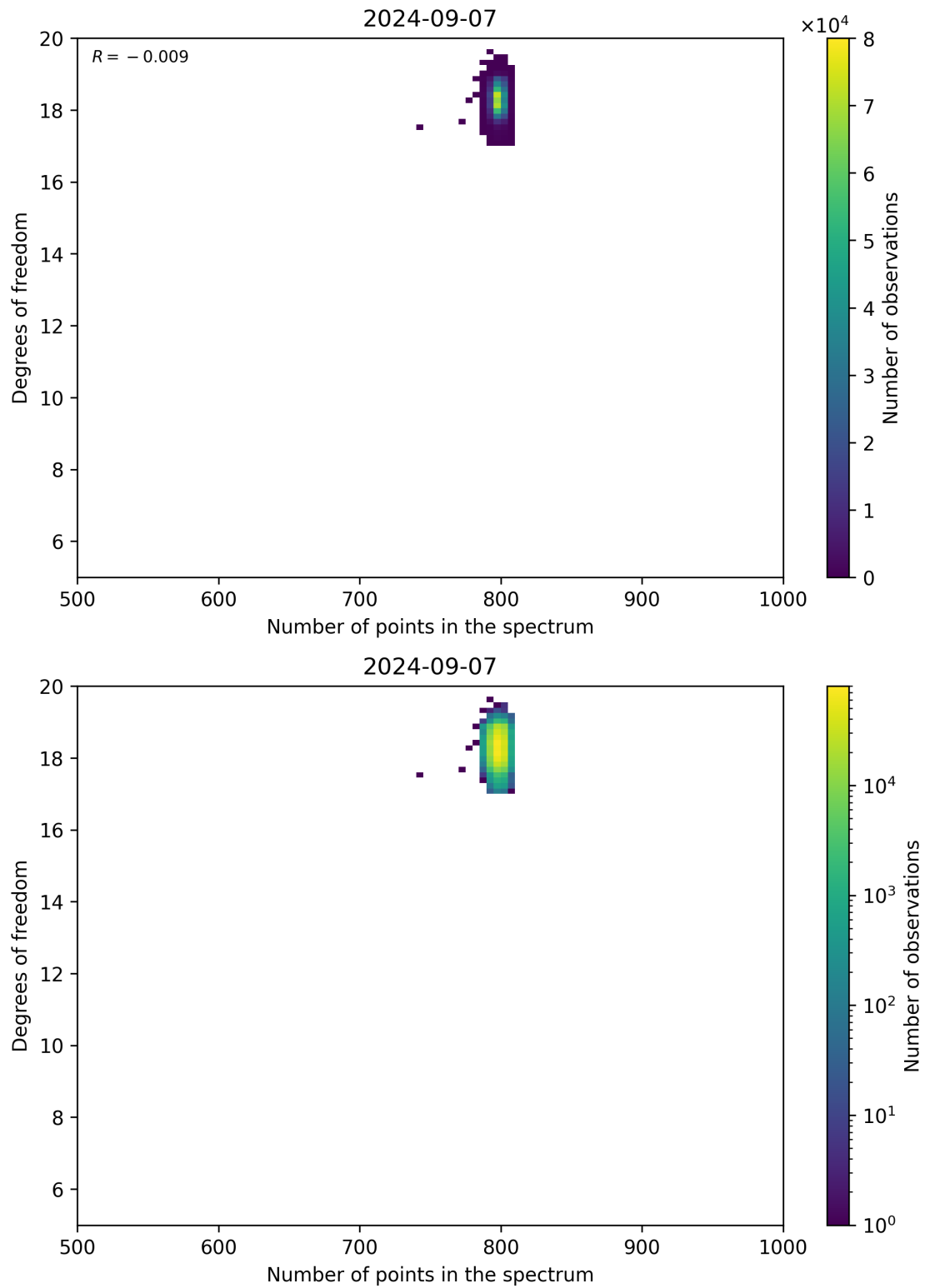
Figure 90: Scatter density plot of “Number of points in the spectrum” against “Degrees of freedom” for 2024-09-06 to 2024-09-08.
