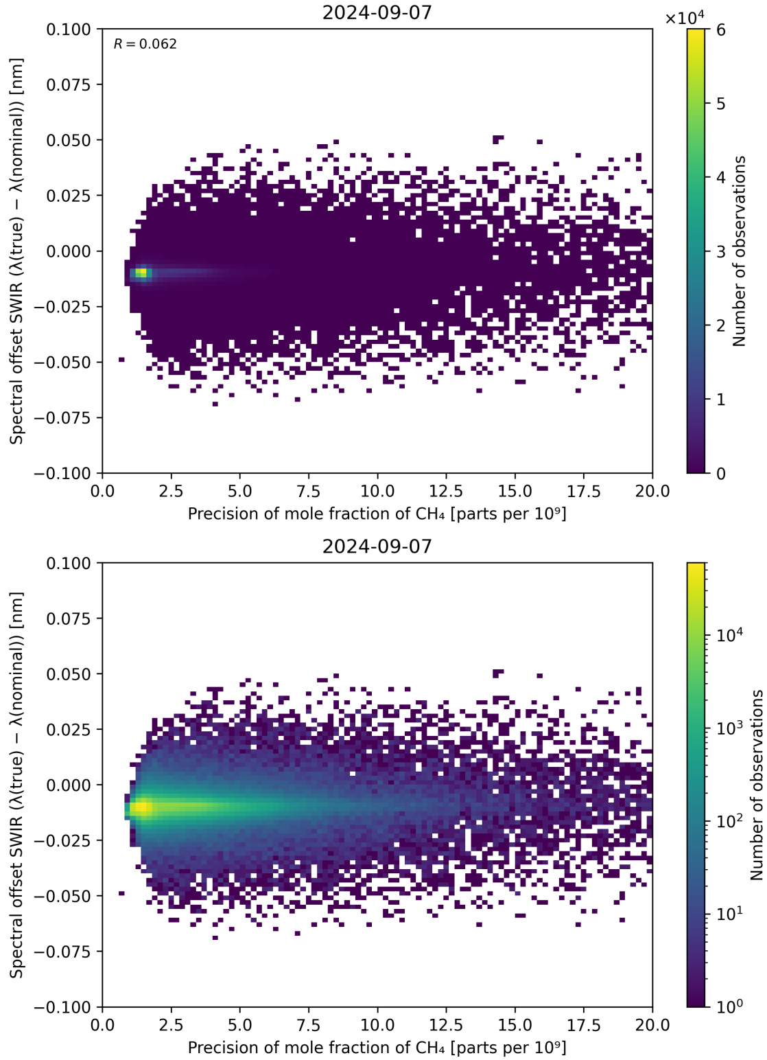
Figure 85: Scatter density plot of “Precision of mole fraction of \text{CH}_4 ” against “Spectral offset SWIR ( \lambda_{\text{true}} - \lambda_{\text{nominal}} )” for 2024-09-06 to 2024-09-08.
