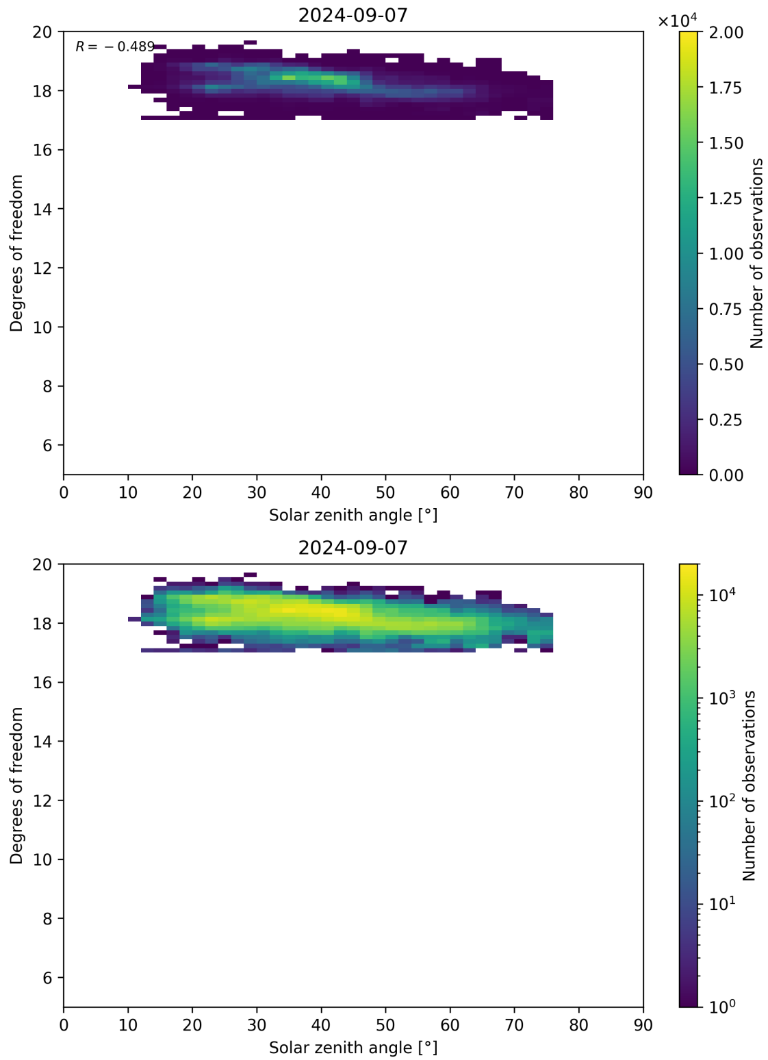
Figure 96: Scatter density plot of “Solar zenith angle” against “Degrees of freedom” for 2024-09-06 to 2024-09-08.
