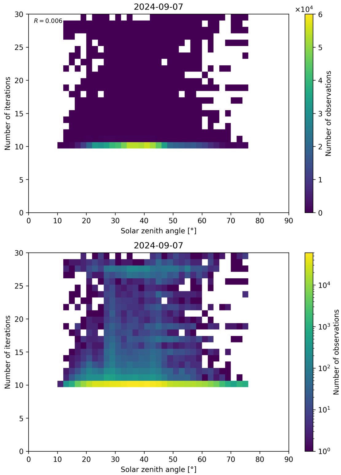
Figure 102: Scatter density plot of “Solar zenith angle” against “Number of iterations” for 2024-09-06 to 2024-09-08.
