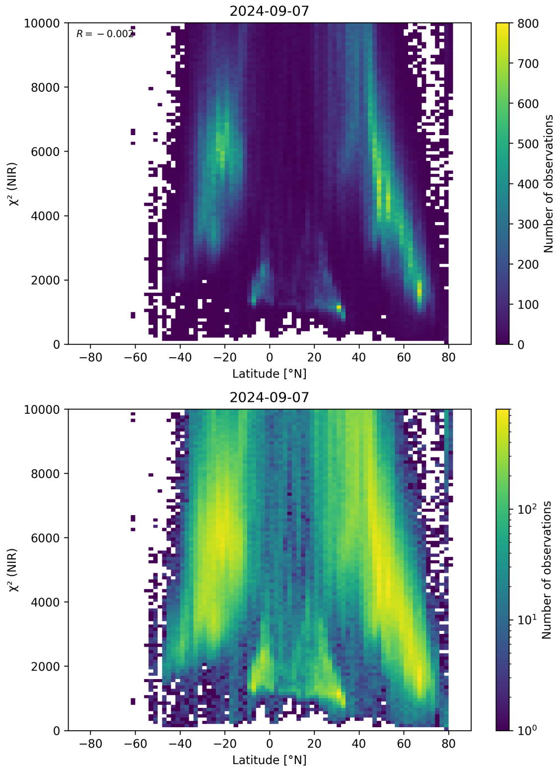
Figure 53: Scatter density plot of “Latitude” against “ \chi^2 (NIR)” for 2024-09-06 to 2024-09-08.
