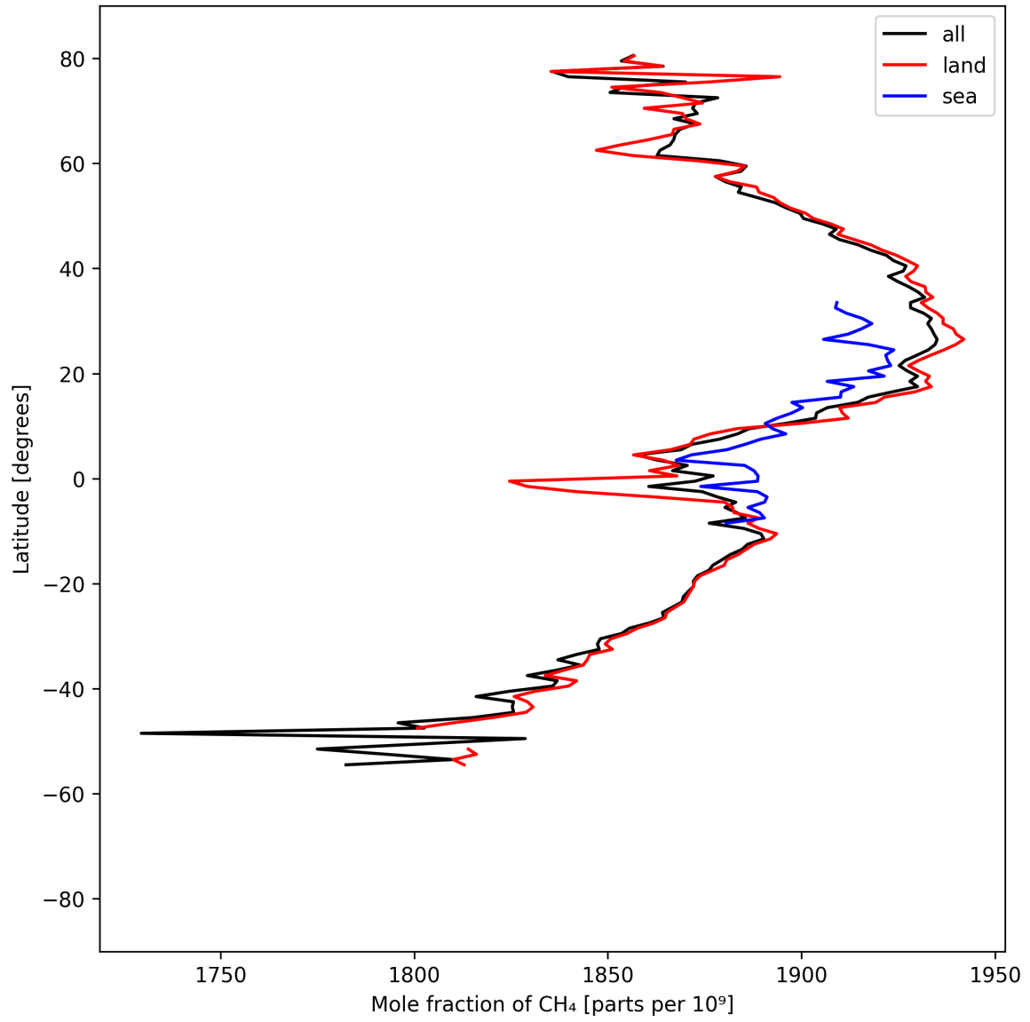
Figure 12: Zonal average of “Mole fraction of \text{CH}_4 ” for 2024-09-06 to 2024-09-08.
