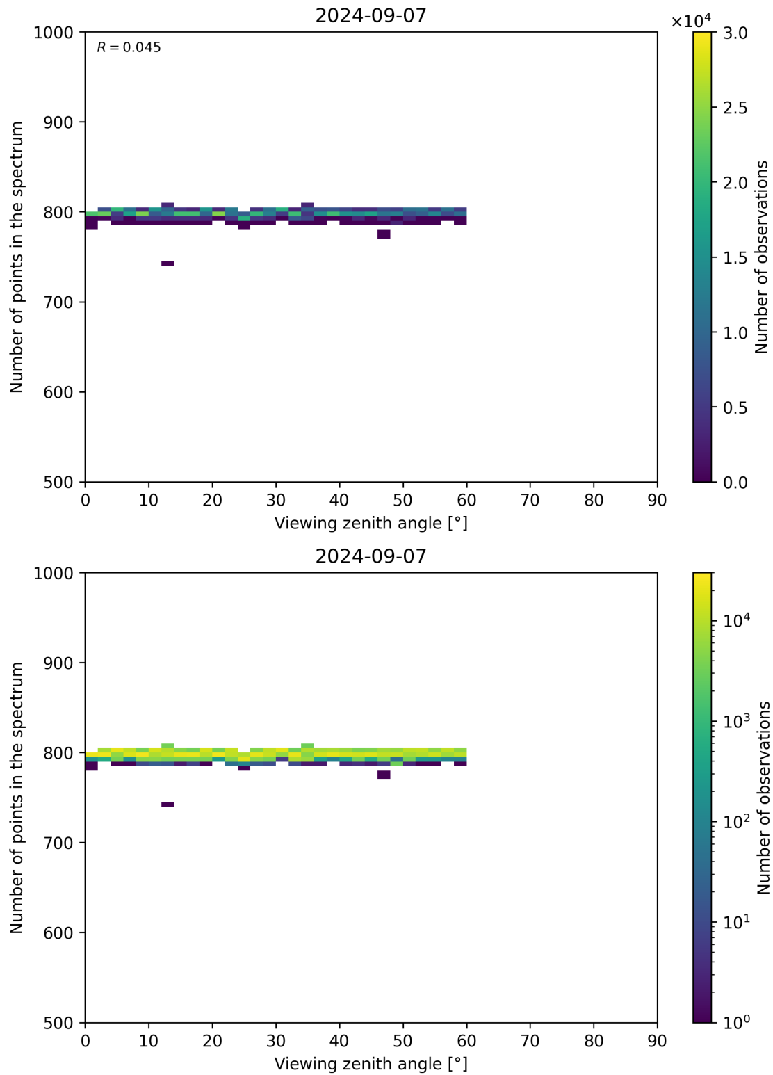
Figure 114: Scatter density plot of “Viewing zenith angle” against “Number of points in the spectrum” for 2024-09-06 to 2024-09-08.
