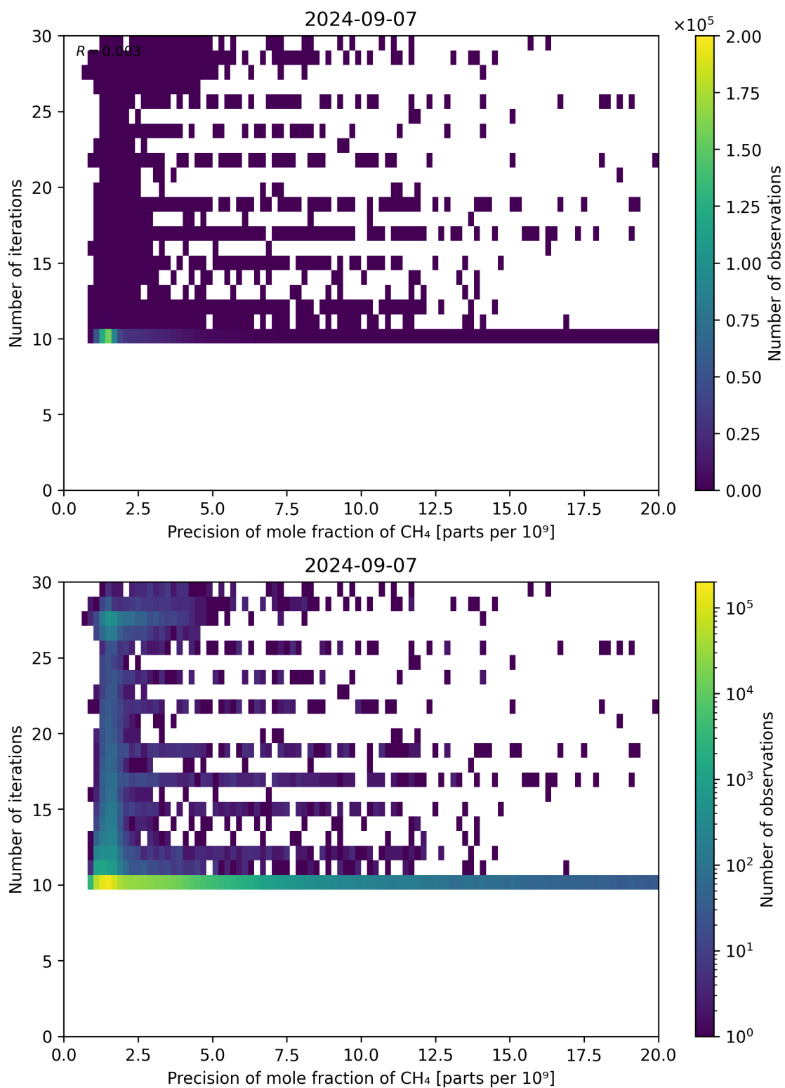
Figure 83: Scatter density plot of “Precision of mole fraction of CH 4 ” against “Number of iterations” for 2024-09-06 to 2024-09-08.
