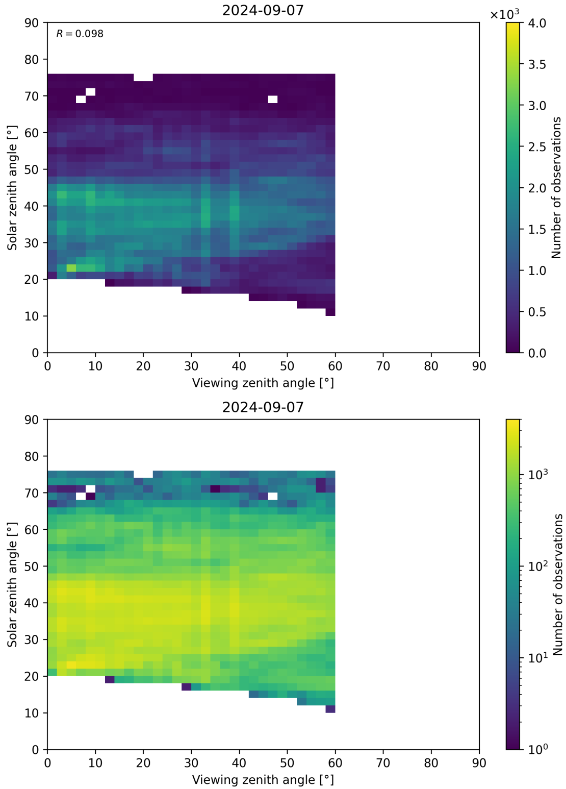
Figure 115: Scatter density plot of “Viewing zenith angle” against “Solar zenith angle” for 2024-09-06 to 2024-09-08.
