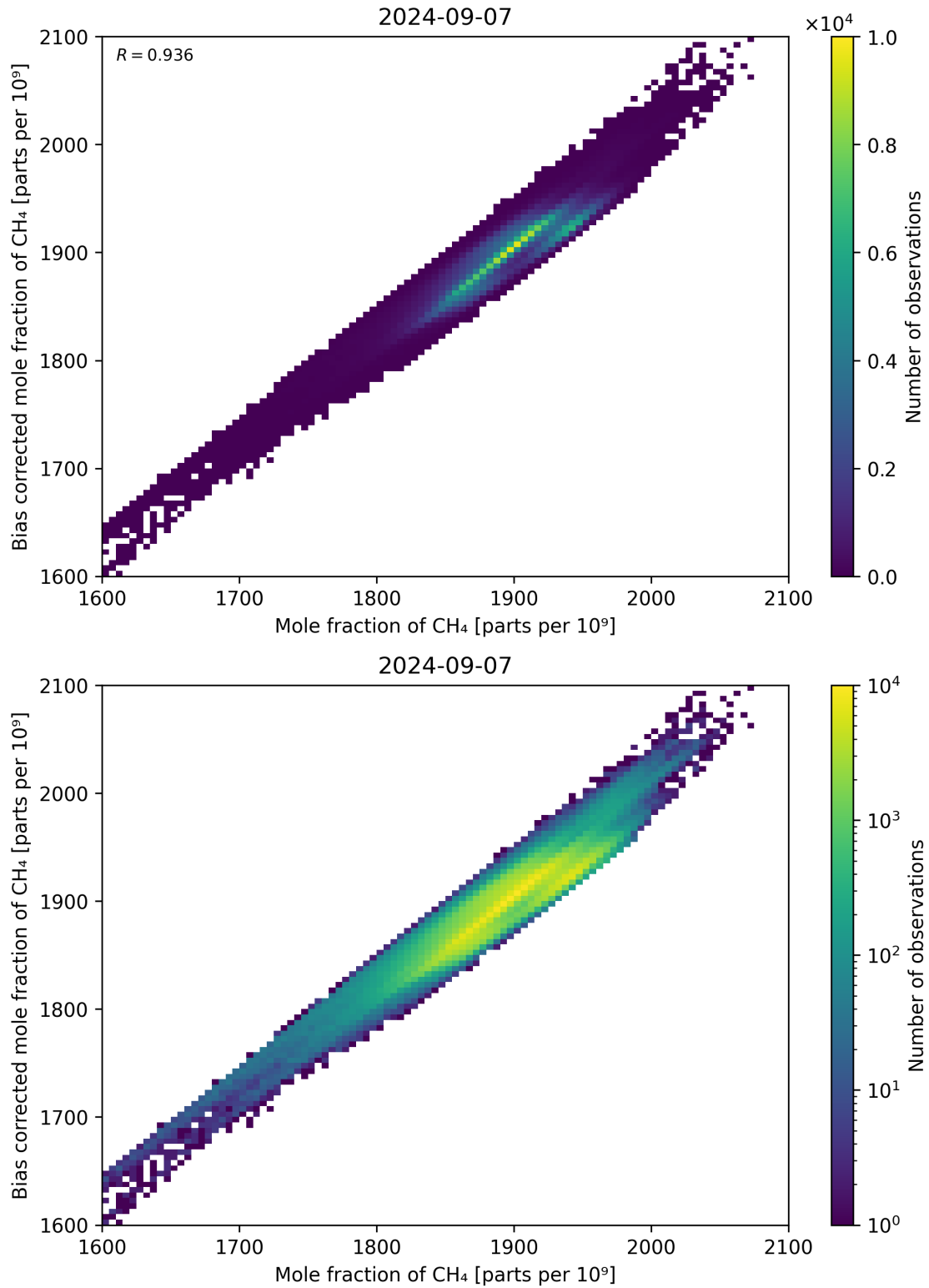
Figure 74: Scatter density plot of “Mole fraction of \text{CH}_4 ” against “Bias corrected mole fraction of \text{CH}_4 ” for 2024-09-06 to 2024-09-08.
