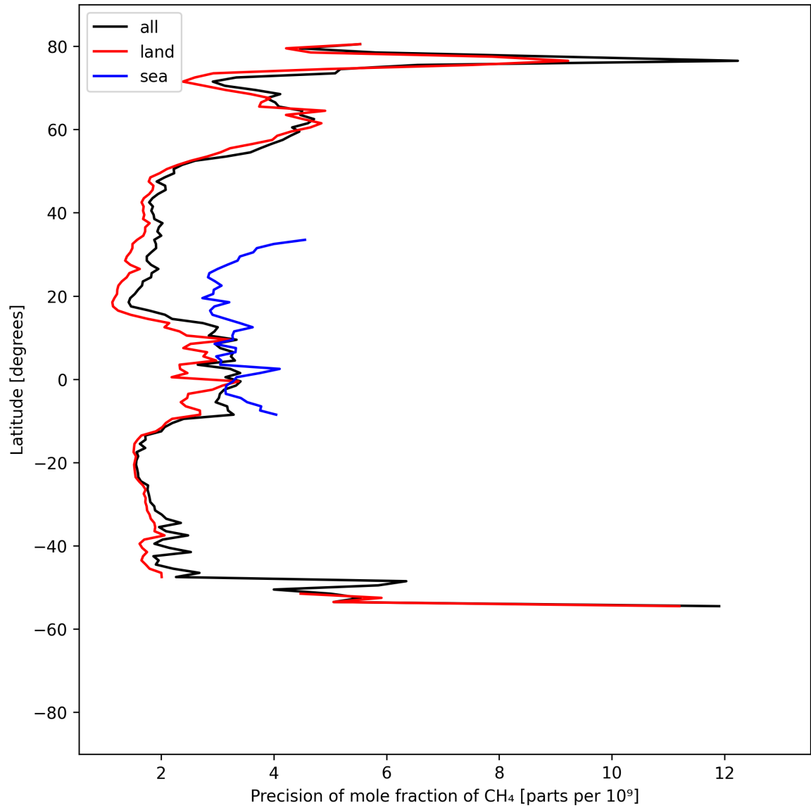
Figure 13: Zonal average of “Precision of mole fraction of CH 4 ” for 2024-09-06 to 2024-09-08.
