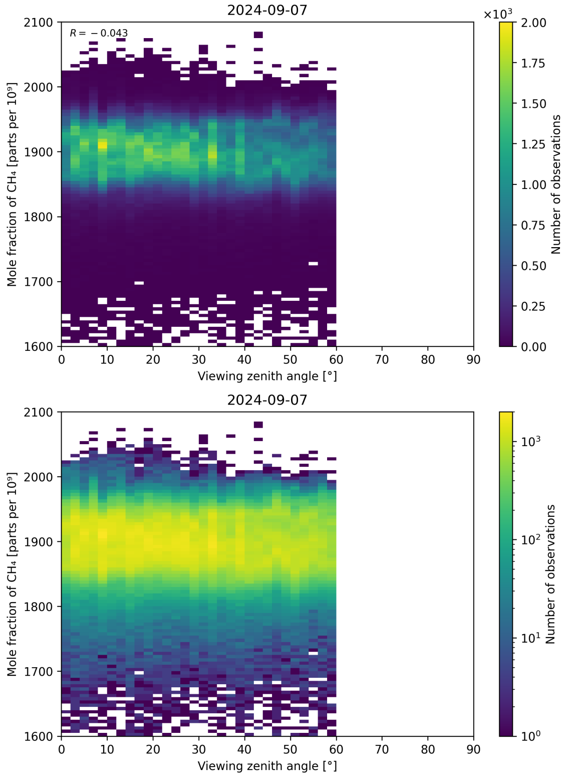
Figure 110: Scatter density plot of “Viewing zenith angle” against “Mole fraction of CH 4 ” for 2024-09-06 to 2024-09-08.
