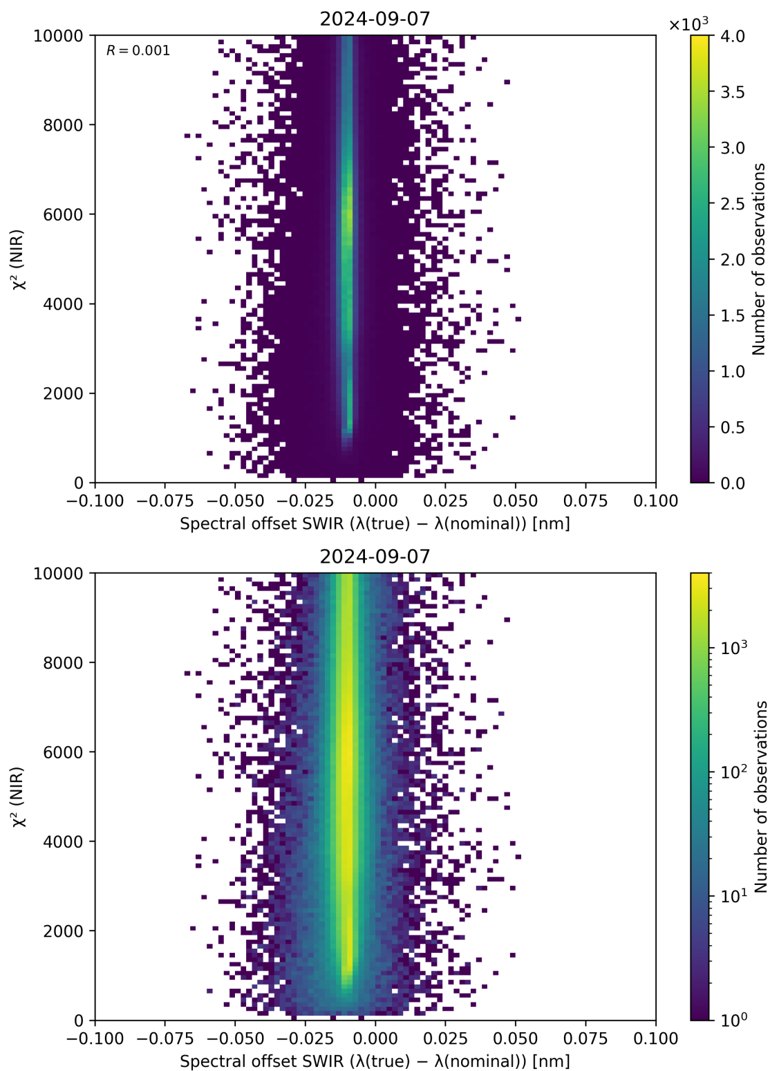
Figure 117: Scatter density plot of “Spectral offset SWIR ( \lambda_{\text{true}} - \lambda_{\text{nominal}} )” against “ \chi^2 (NIR)” for 2024-09-06 to 2024-09-08.
