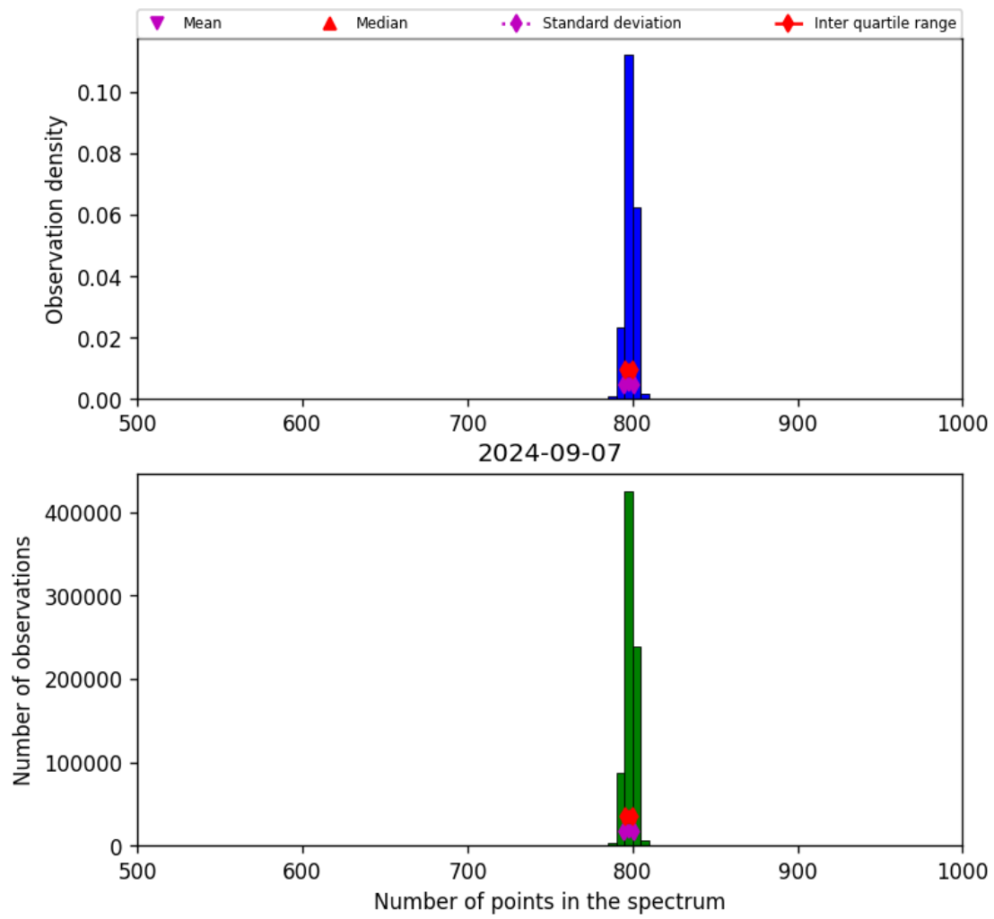
Figure 26: Histogram of “Number of points in the spectrum” for 2024-09-06 to 2024-09-08
