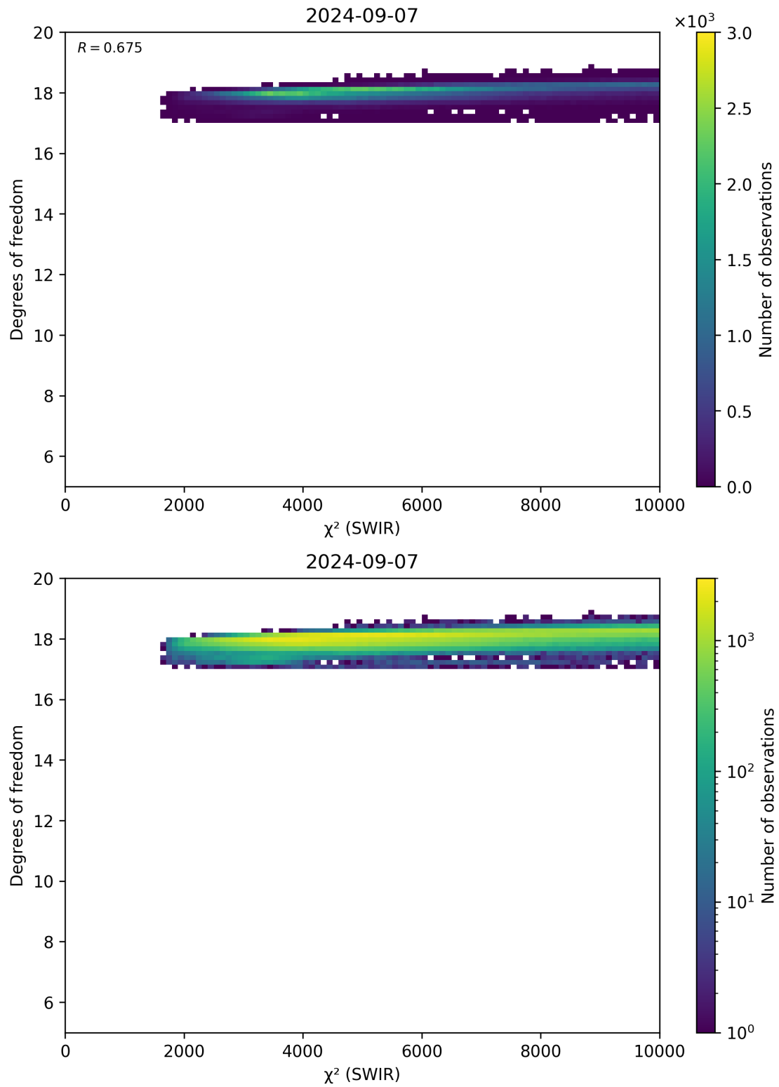
Figure 48: Scatter density plot of “ \chi^2 (SWIR)” against “Degrees of freedom” for 2024-09-06 to 2024-09-08.
