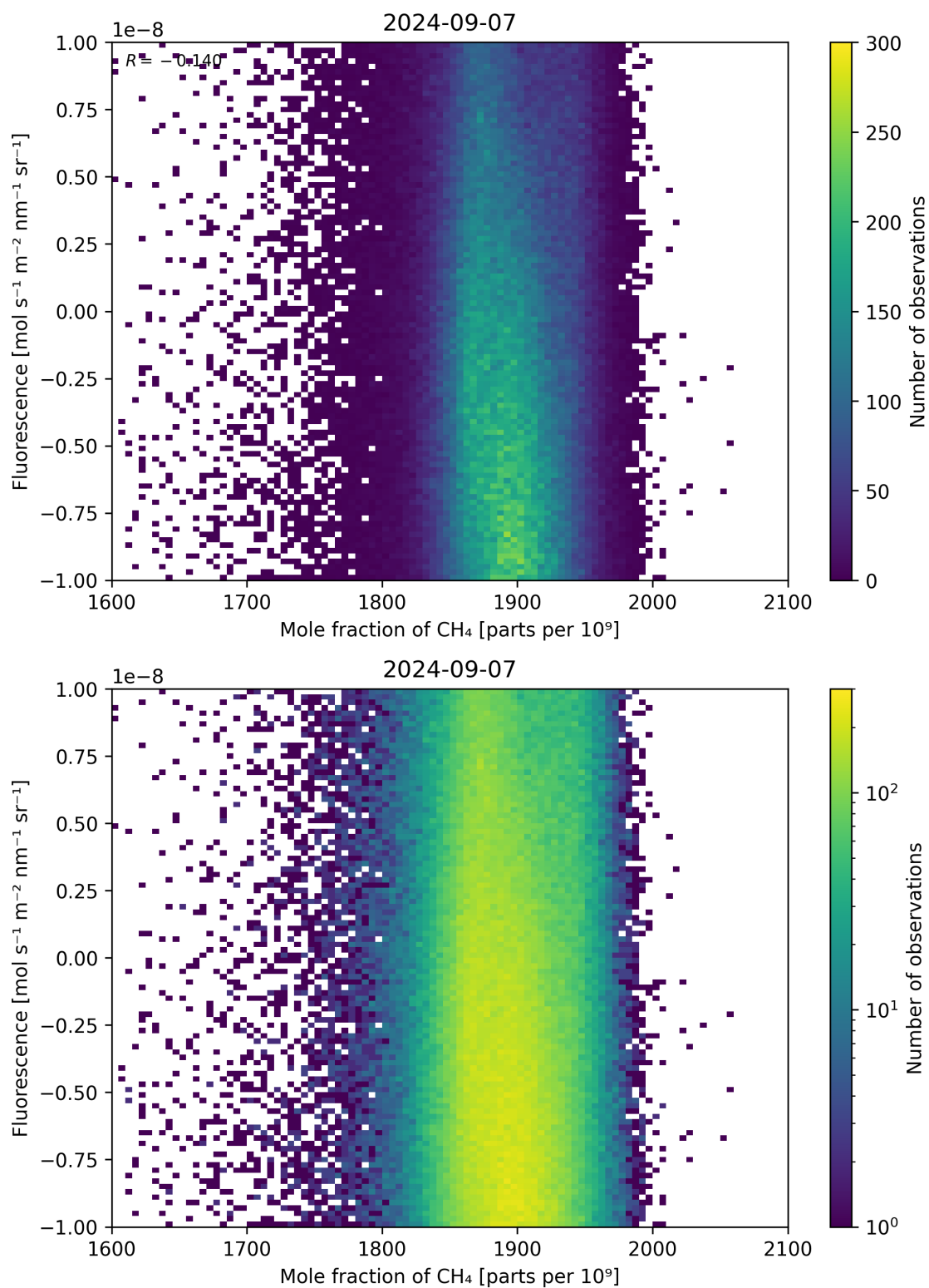
Figure 73: Scatter density plot of “Mole fraction of \text{CH}_4 ” against “Fluorescence” for 2024-09-06 to 2024-09-08.
