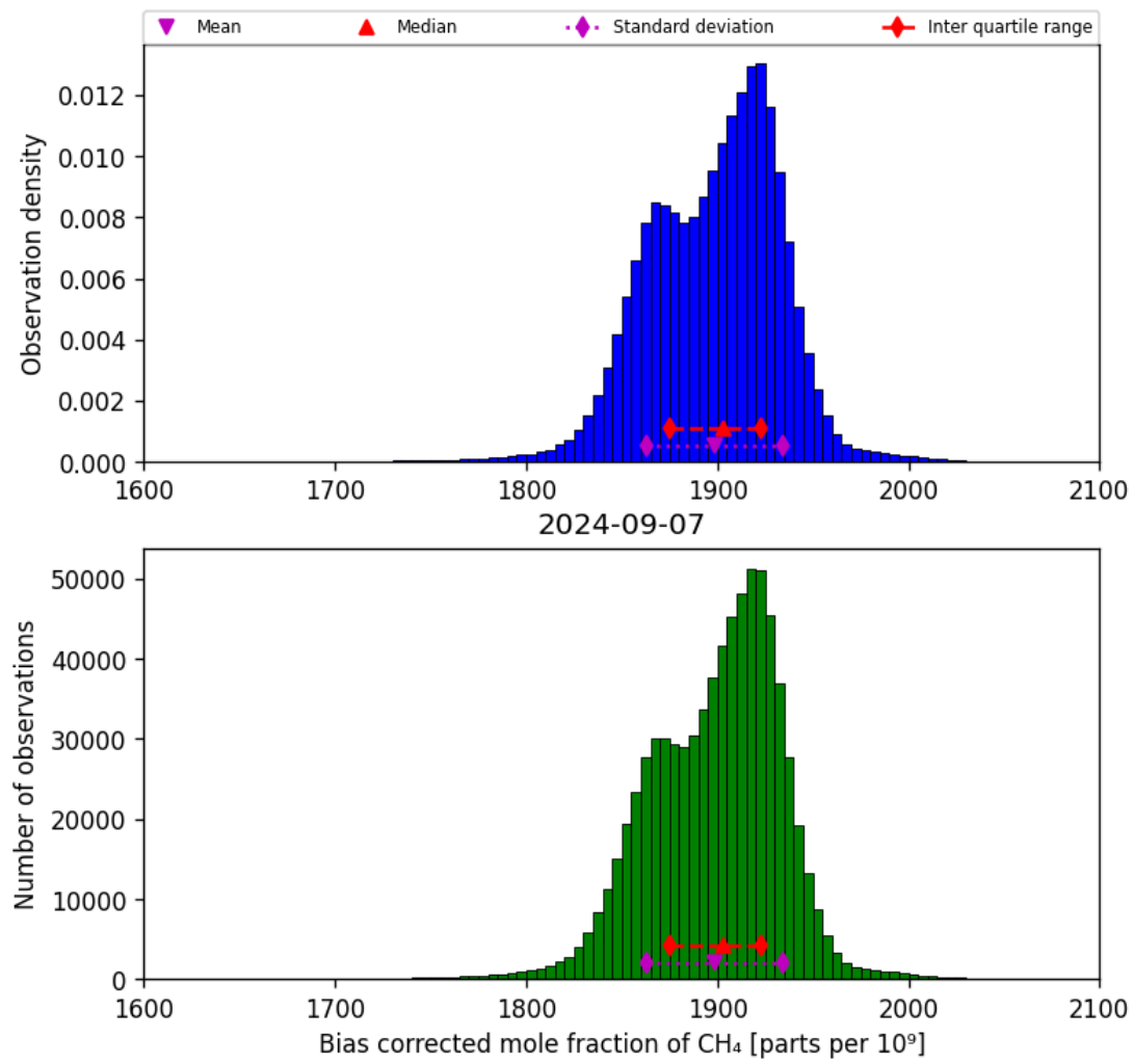
Figure 25: Histogram of “Bias corrected mole fraction of CH 4 ” for 2024-09-06 to 2024-09-08
