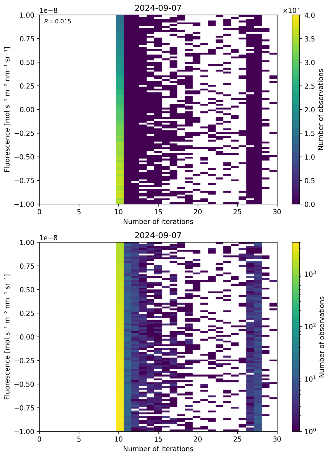
Figure 87: Scatter density plot of “Number of iterations” against “Fluorescence” for 2024-09-06 to 2024-09-08.
