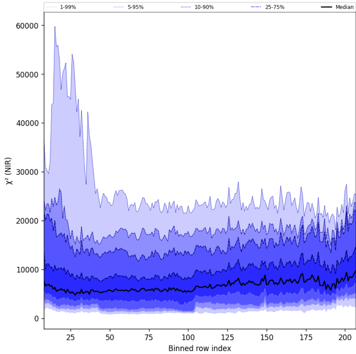
Figure 40: Along track statistics of “ \chi^2 (NIR)” for 2024-09-06 to 2024-09-08
