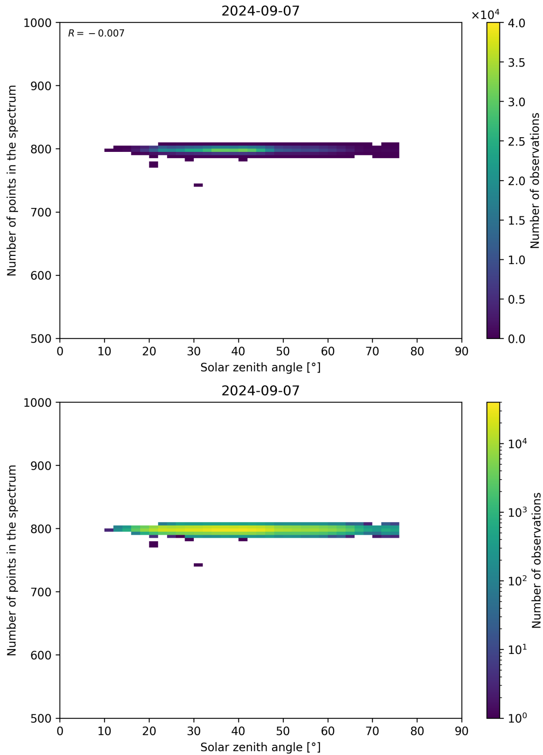
Figure 103: Scatter density plot of “Solar zenith angle” against “Number of points in the spectrum” for 2024-09-06 to 2024-09-08.
