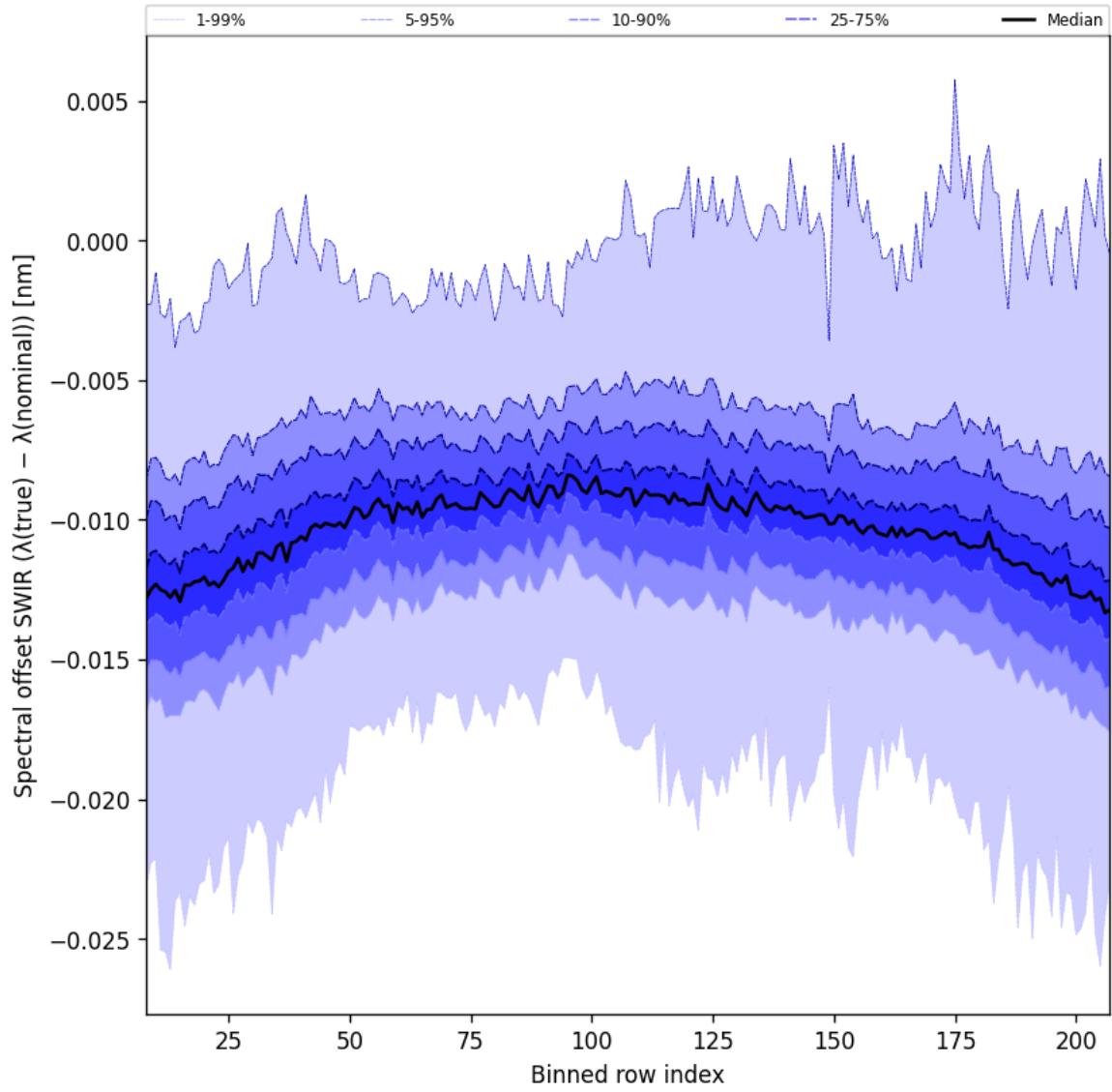
Figure 38: Along track statistics of “Spectral offset SWIR ( \lambda_{\text{true}} - \lambda_{\text{nominal}} )” for 2024-09-06 to 2024-09-08
