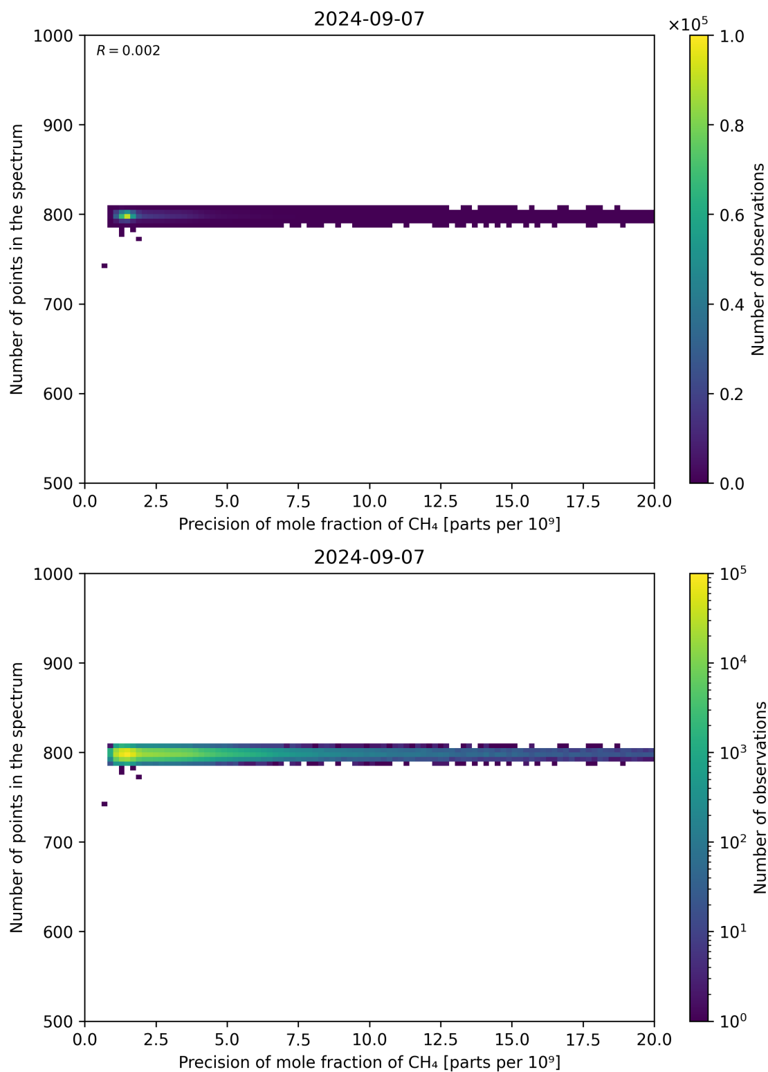
Figure 84: Scatter density plot of “Precision of mole fraction of CH 4 ” against “Number of points in the spectrum” for 2024-09-06 to 2024-09-08.
