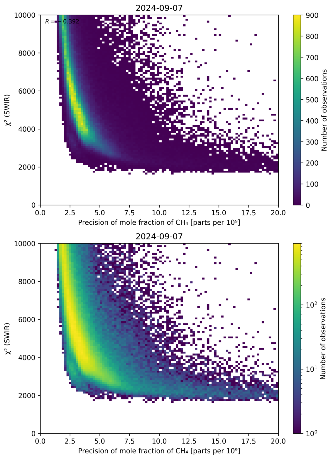
Figure 79: Scatter density plot of “Precision of mole fraction of \text{CH}_4 ” against “ \chi^2 (SWIR)” for 2024-09-06 to 2024-09-08.
