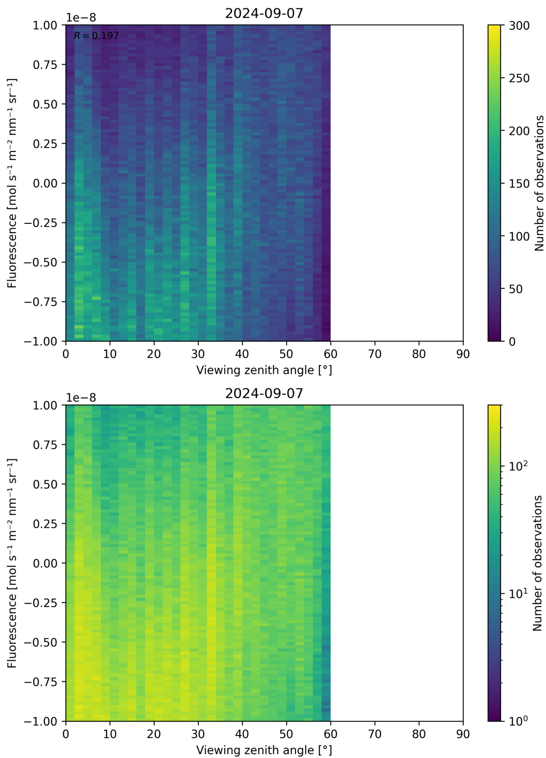
Figure 108: Scatter density plot of “Viewing zenith angle” against “Fluorescence” for 2024-09-06 to 2024-09-08.
