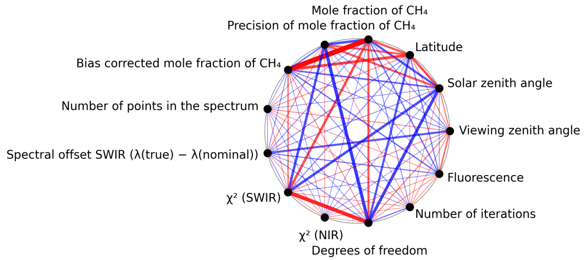
Figure 1: Map of correlation graph for 2024-09-06 to 2024-09-08.
