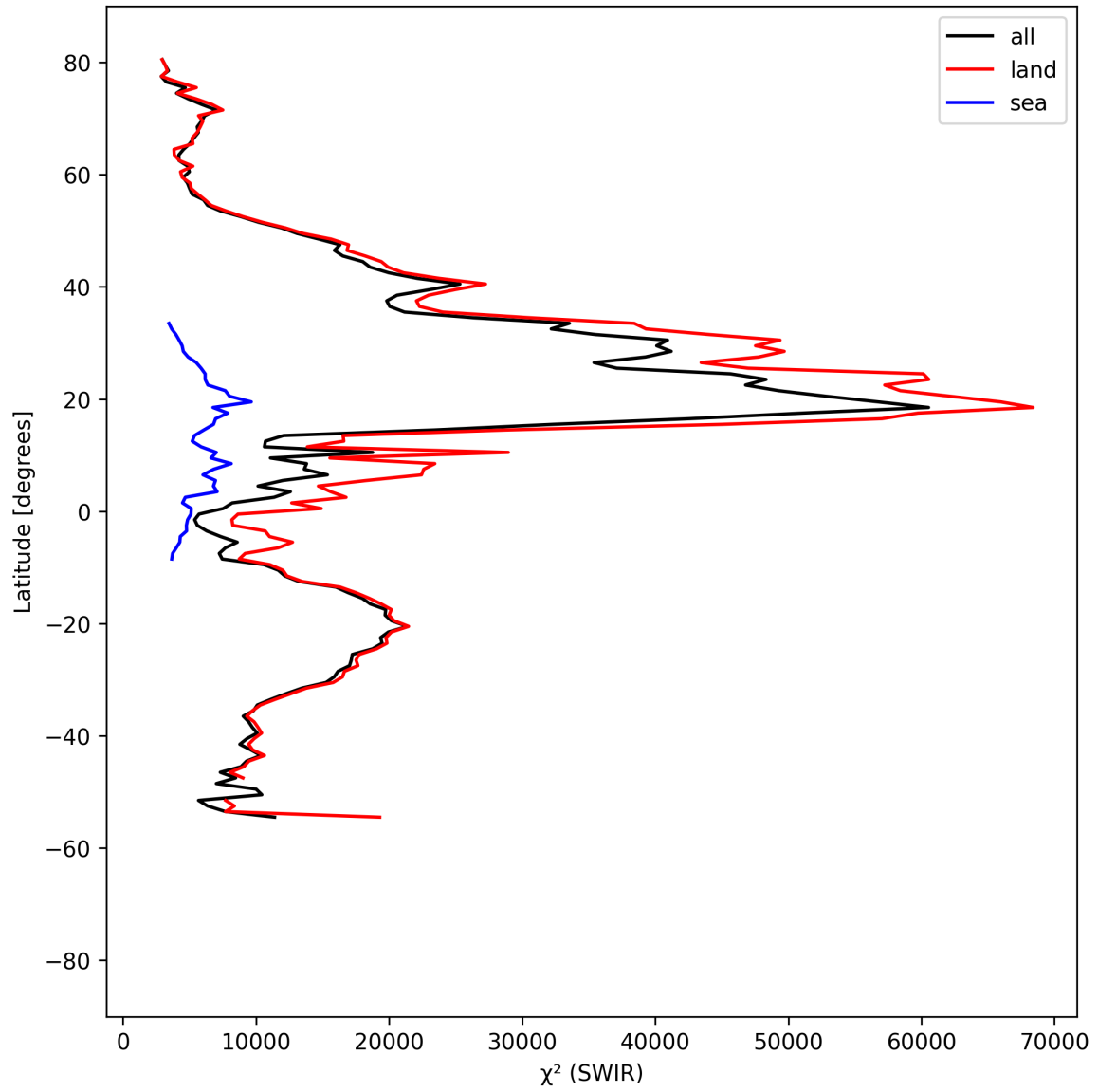
Figure 17: Zonal average of “ \chi^2 (SWIR)” for 2024-09-06 to 2024-09-08.
