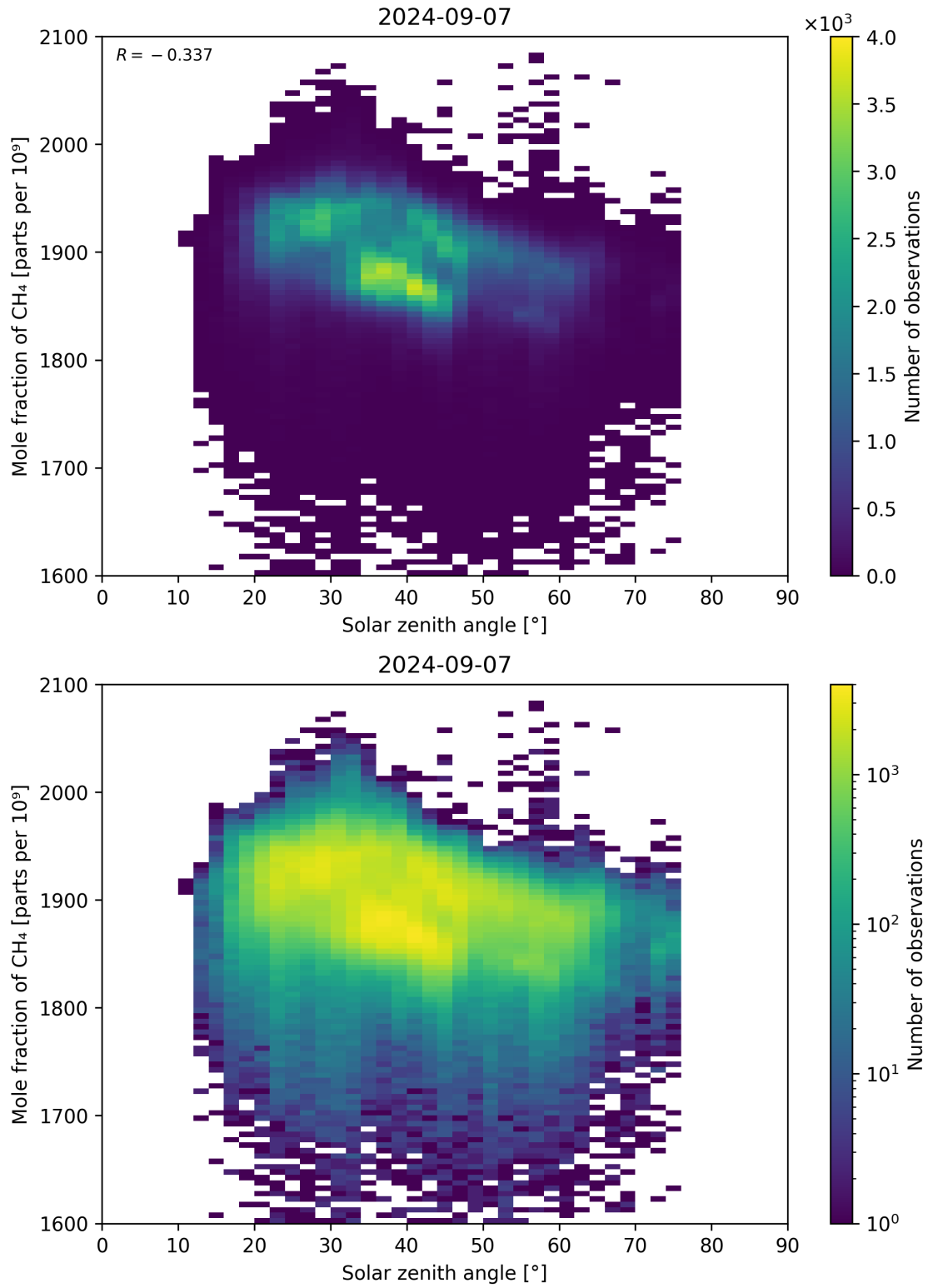
Figure 99: Scatter density plot of “Solar zenith angle” against “Mole fraction of CH 4 ” for 2024-09-06 to 2024-09-08.
