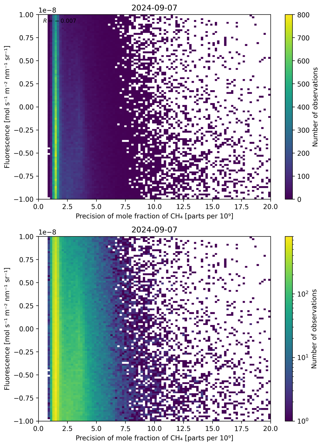
Figure 81: Scatter density plot of “Precision of mole fraction of \text{CH}_4 ” against “Fluorescence” for 2024-09-06 to 2024-09-08.
