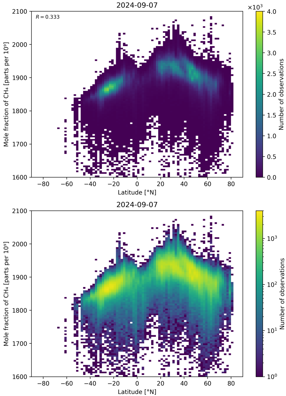
Figure 57: Scatter density plot of “Latitude” against “Mole fraction of CH 4 ” for 2024-09-06 to 2024-09-08.
