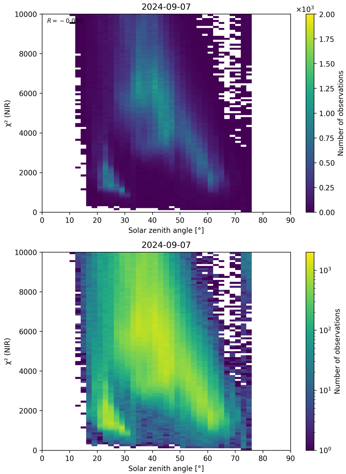
Figure 94: Scatter density plot of “Solar zenith angle” against “ \chi^2 (NIR)” for 2024-09-06 to 2024-09-08.
