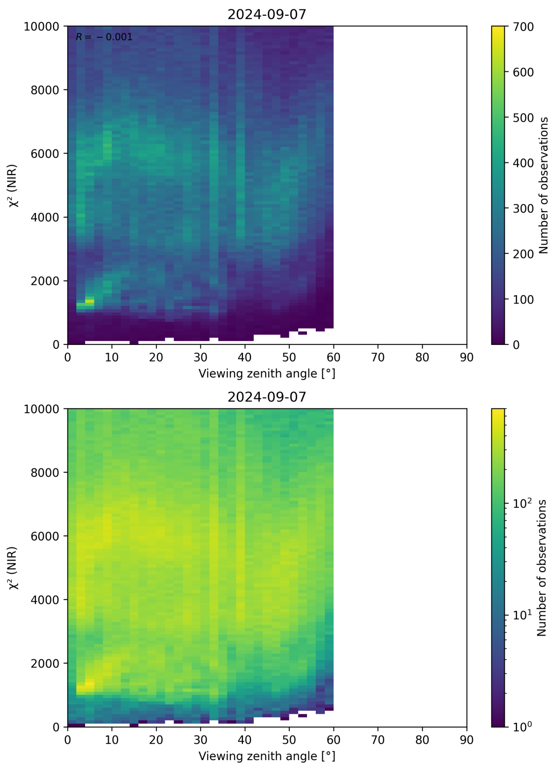
Figure 105: Scatter density plot of “Viewing zenith angle” against “ \chi^2 (NIR)” for 2024-09-06 to 2024-09-08.
