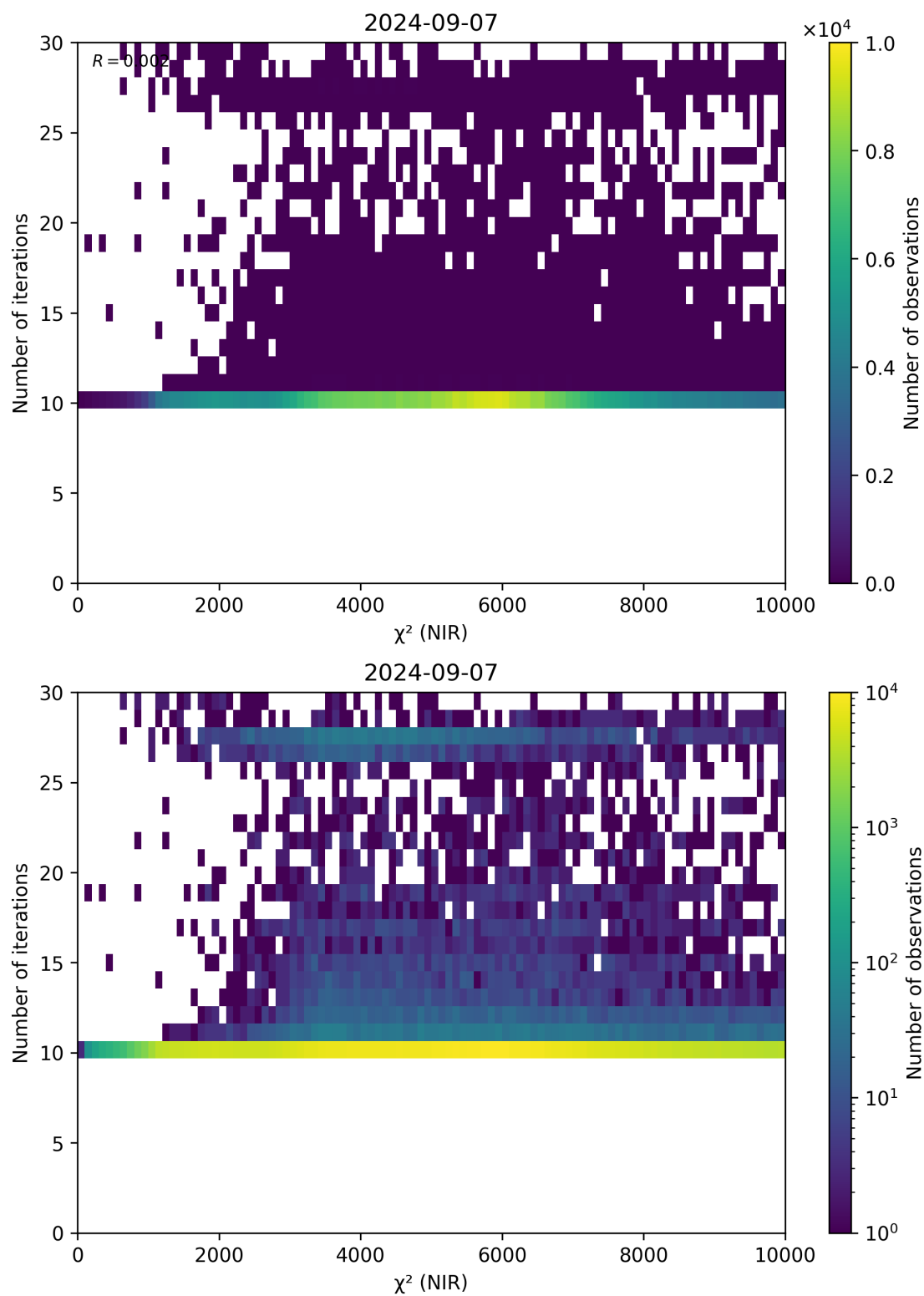
Figure 46: Scatter density plot of “ \chi^2 (NIR)” against “Number of iterations” for 2024-09-06 to 2024-09-08.
