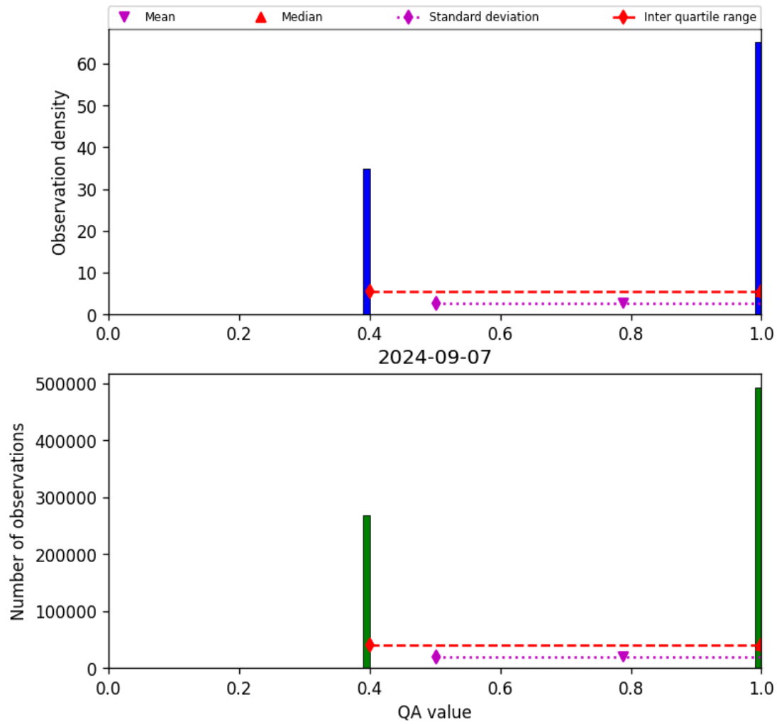
Figure 22: Histogram of “QA value” for 2024-09-06 to 2024-09-08
