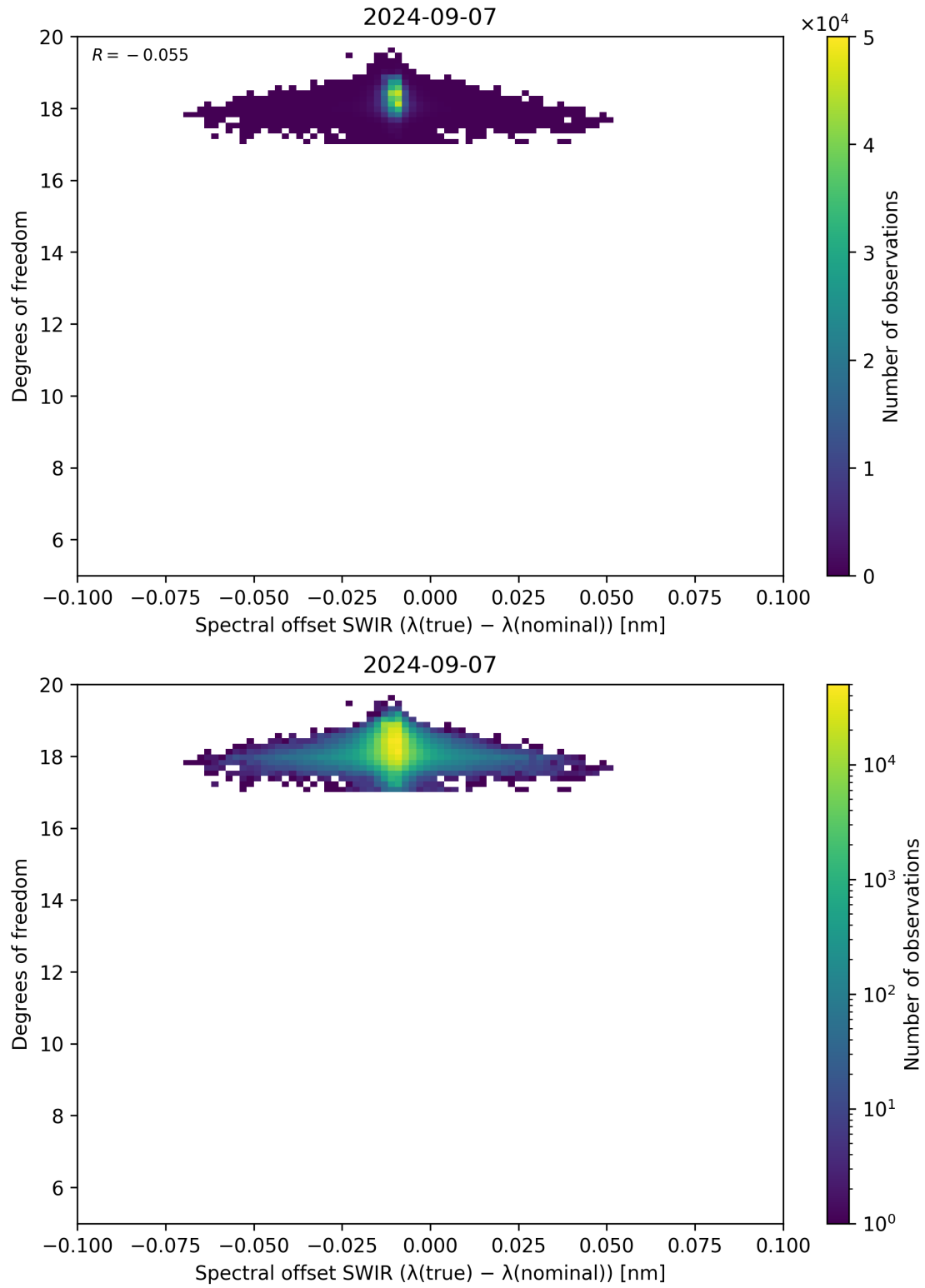
Figure 119: Scatter density plot of “Spectral offset SWIR ( \lambda_{\text{true}} - \lambda_{\text{nominal}} )” against “Degrees of freedom” for 2024-09-06 to 2024-09-08.
