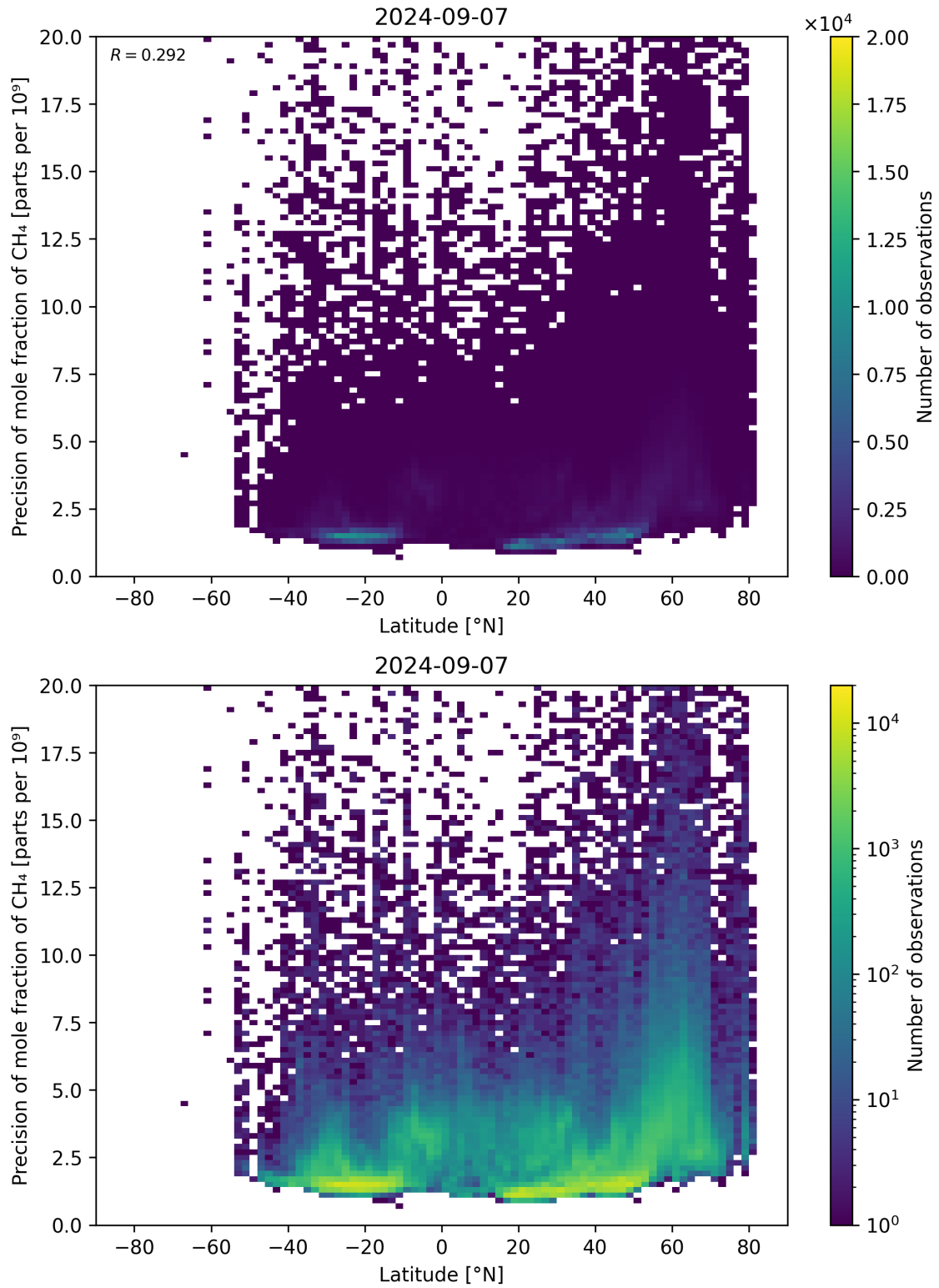
Figure 59: Scatter density plot of “Latitude” against “Precision of mole fraction of CH 4 ” for 2024-09-06 to 2024-09-08.
