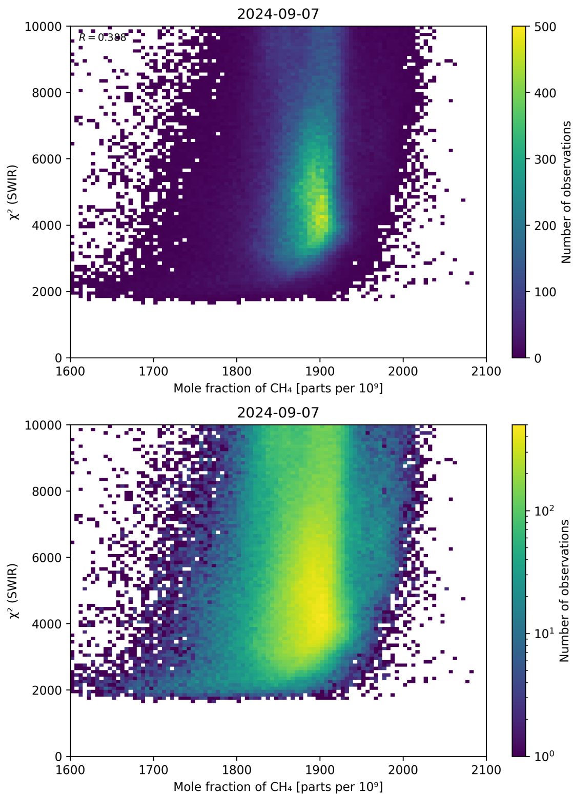
Figure 71: Scatter density plot of “Mole fraction of \text{CH}_4 ” against “ \chi^2 (SWIR)” for 2024-09-06 to 2024-09-08.
