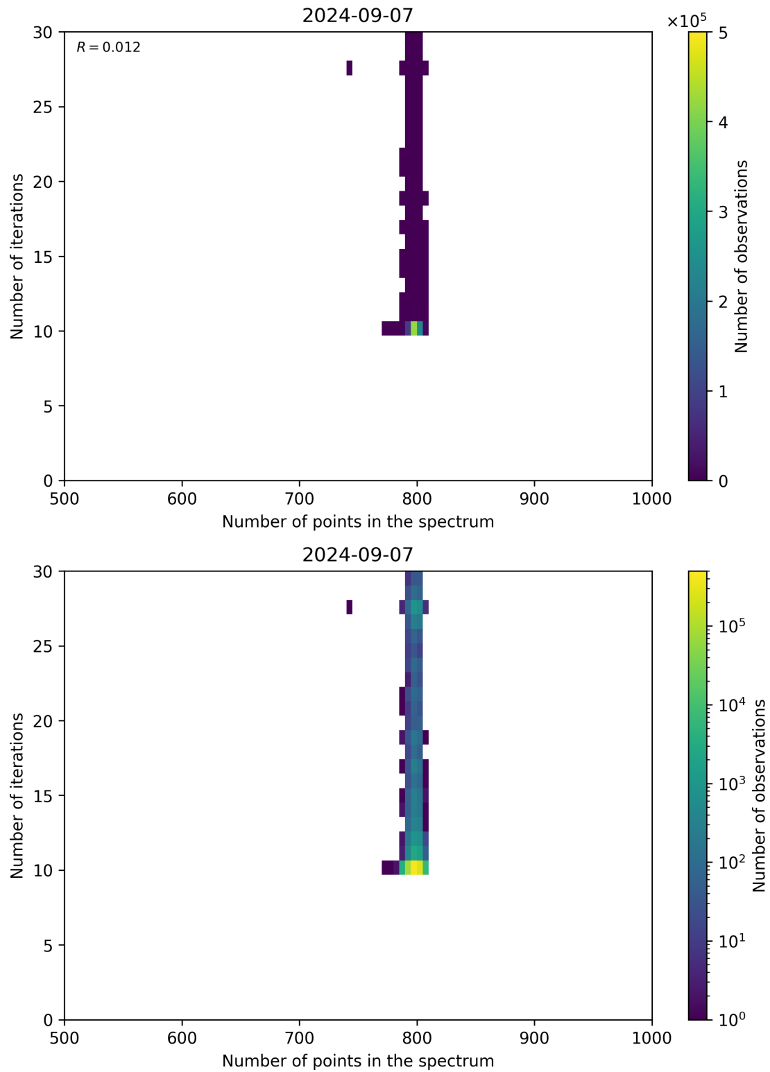
Figure 92: Scatter density plot of “Number of points in the spectrum” against “Number of iterations” for 2024-09-06 to 2024-09-08.
