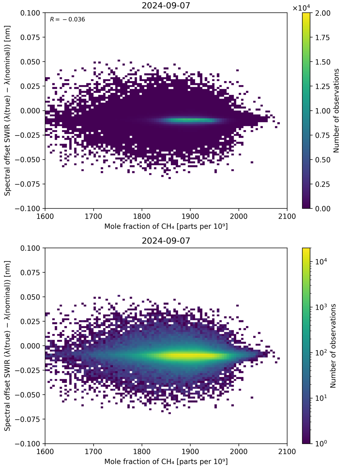
Figure 86: Scatter density plot of “Mole fraction of CH 4 ” against “Spectral offset SWIR ( \lambda_{\text{true}} - \lambda_{\text{nominal}} )” for 2024-09-06 to 2024-09-08.
