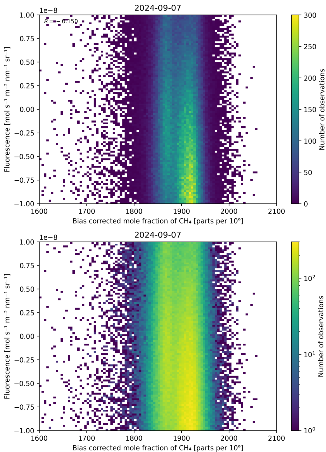
Figure 66: Scatter density plot of “Bias corrected mole fraction of \text{CH}_4 ” against “Fluorescence” for 2024-09-06 to 2024-09-08.
