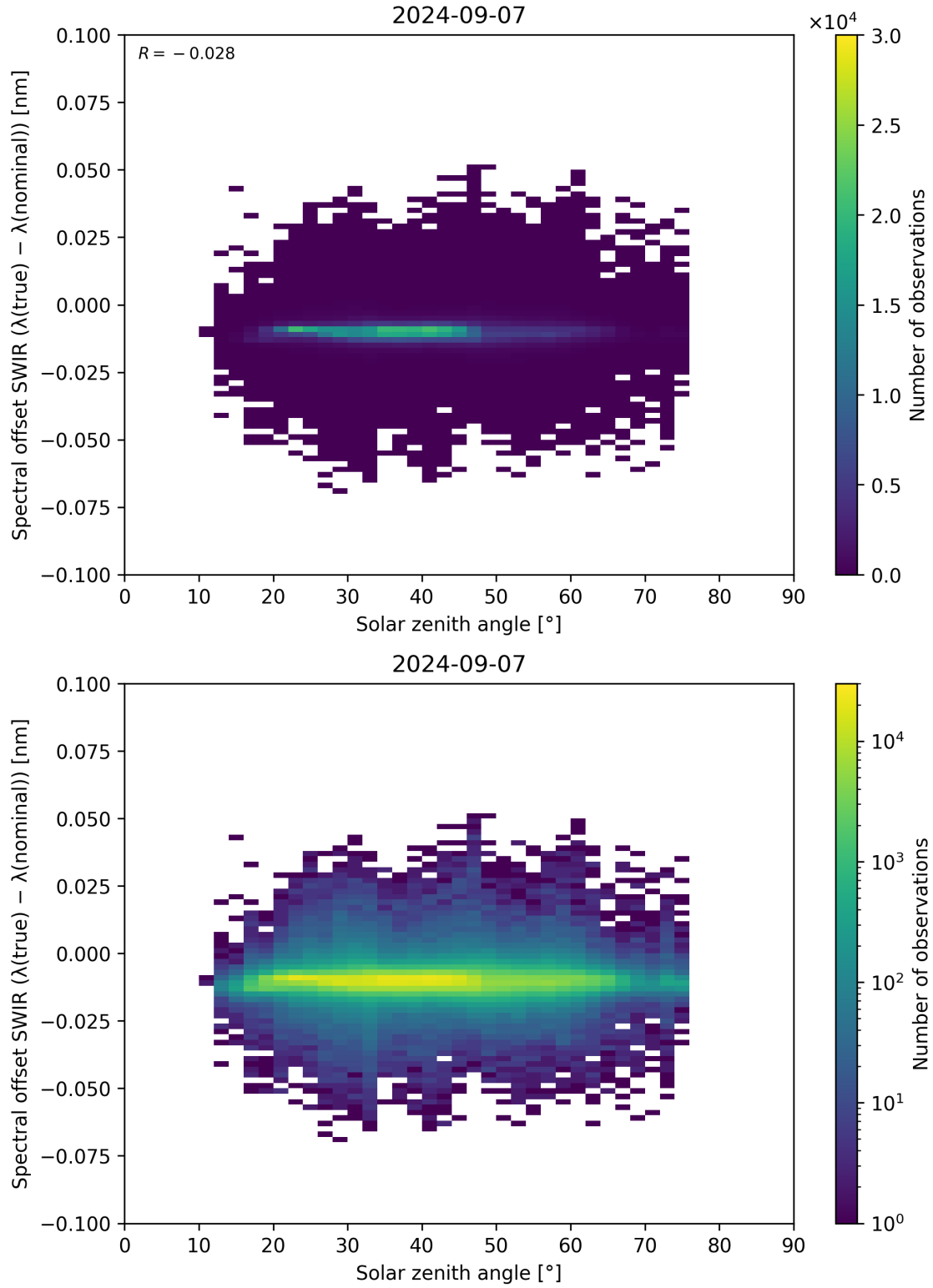
Figure 104: Scatter density plot of “Solar zenith angle” against “Spectral offset SWIR ( \lambda_{\text{true}} - \lambda_{\text{nominal}} )” for 2024-09-06 to 2024-09-08.
