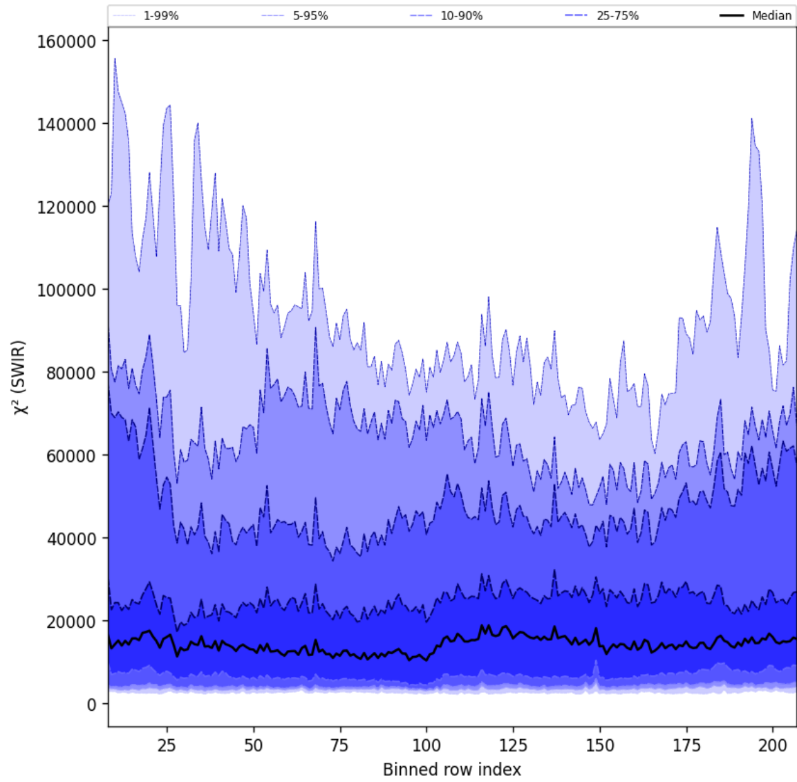
Figure 39: Along track statistics of “ \chi^2 (SWIR)” for 2024-09-06 to 2024-09-08
