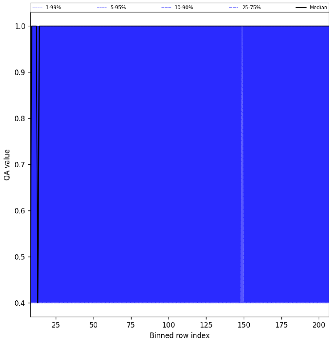
Figure 33: Along track statistics of “QA value” for 2024-09-06 to 2024-09-08
