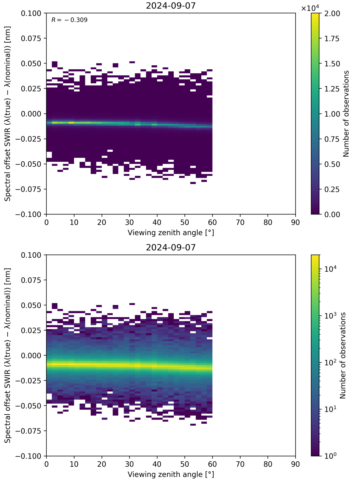
Figure 116: Scatter density plot of “Viewing zenith angle” against “Spectral offset SWIR ( \lambda_{\text{true}} - \lambda_{\text{nominal}} )” for 2024-09-06 to 2024-09-08.
