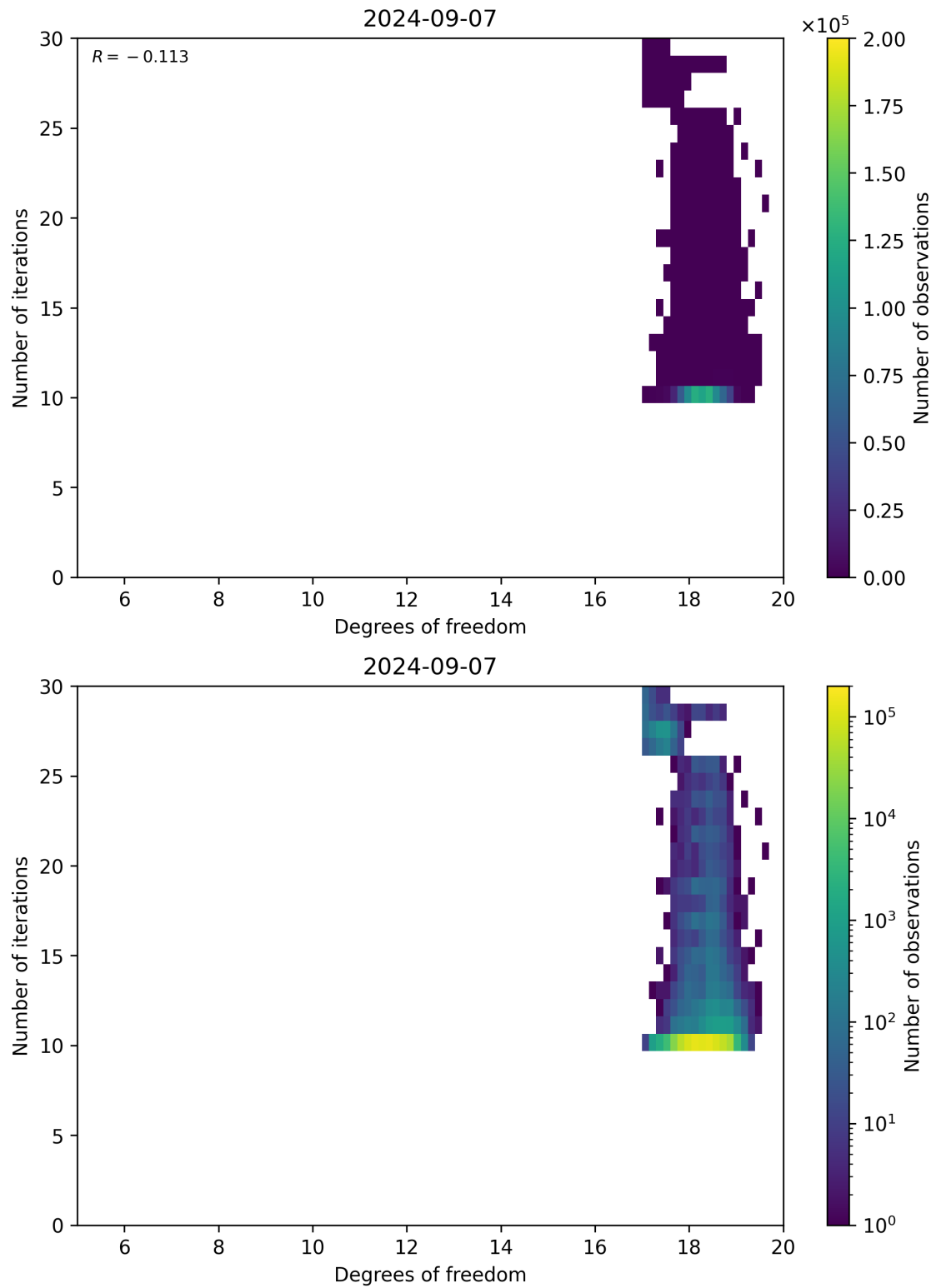
Figure 52: Scatter density plot of “Degrees of freedom” against “Number of iterations” for 2024-09-06 to 2024-09-08.
