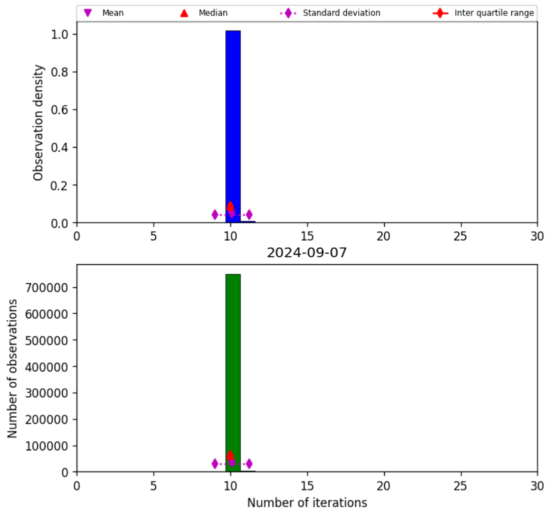
Figure 31: Histogram of “Number of iterations” for 2024-09-06 to 2024-09-08
