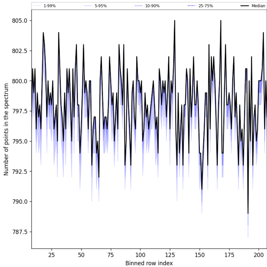
Figure 37: Along track statistics of “Number of points in the spectrum” for 2024-09-06 to 2024-09-08
