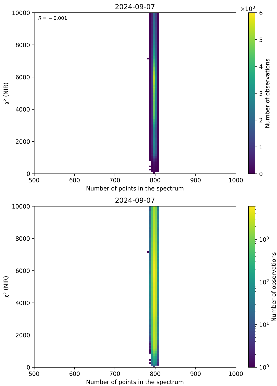
Figure 88: Scatter density plot of “Number of points in the spectrum” against “ \chi^2 (NIR)” for 2024-09-06 to 2024-09-08.
