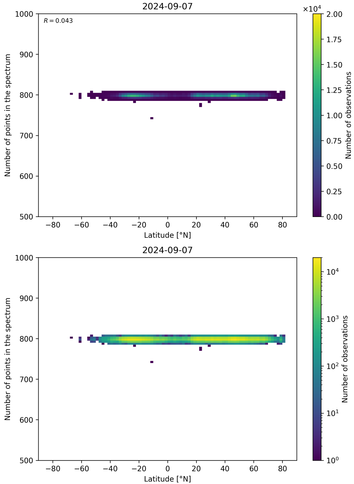
Figure 61: Scatter density plot of “Latitude” against “Number of points in the spectrum” for 2024-09-06 to 2024-09-08.
