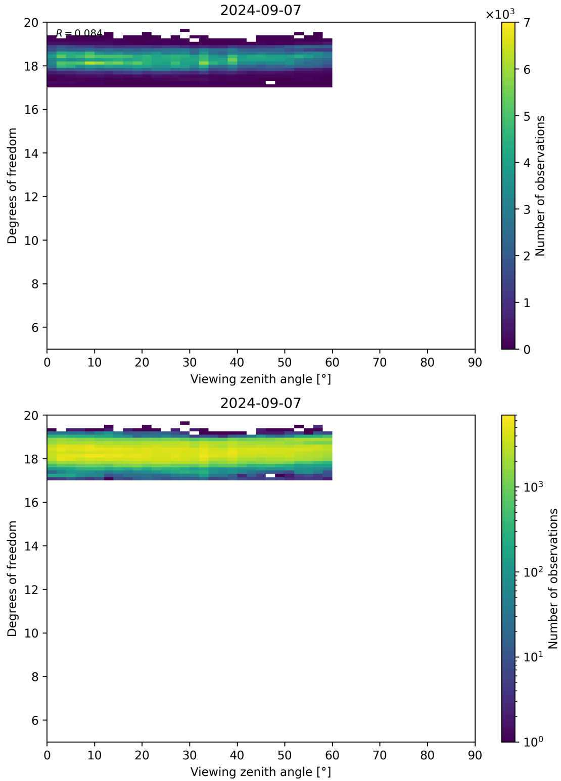
Figure 107: Scatter density plot of “Viewing zenith angle” against “Degrees of freedom” for 2024-09-06 to 2024-09-08.
