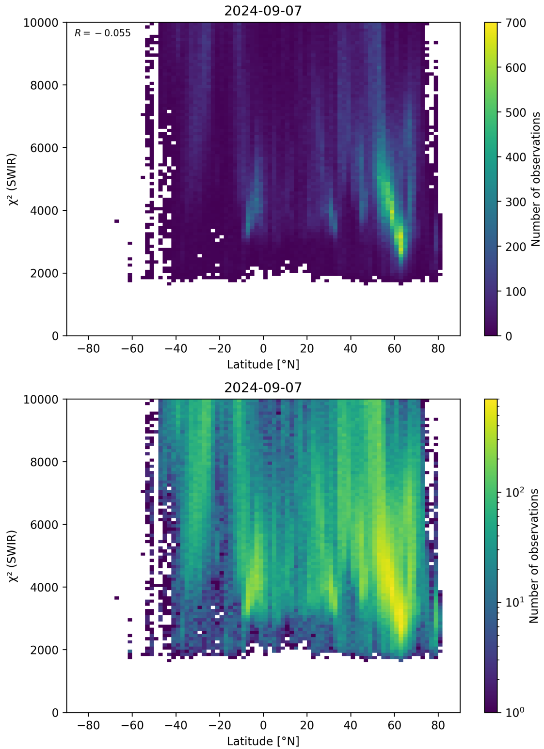
Figure 54: Scatter density plot of “Latitude” against “ \chi^2 (SWIR)” for 2024-09-06 to 2024-09-08.
