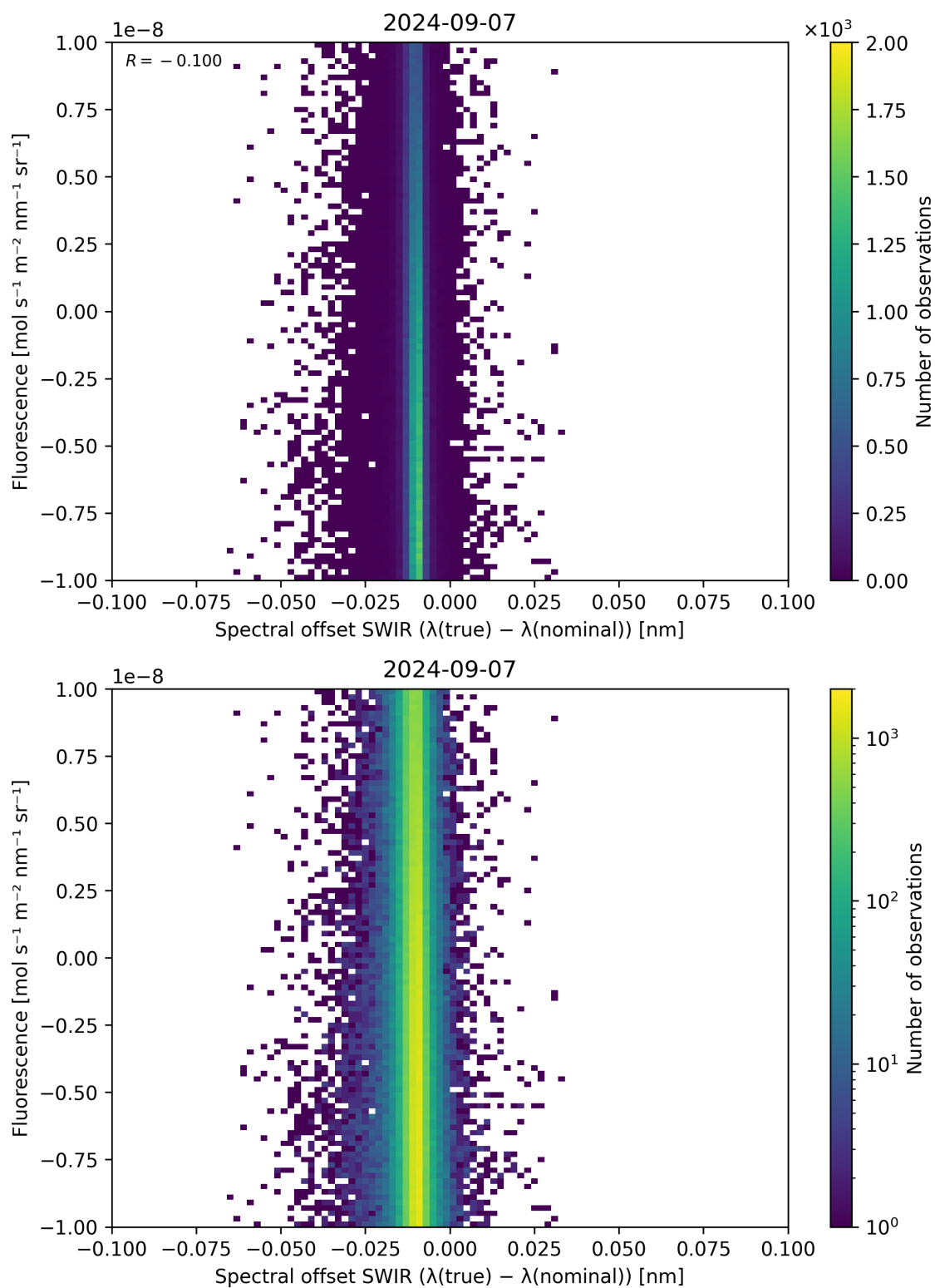
Figure 120: Scatter density plot of “Spectral offset SWIR ( \lambda_{\text{true}} - \lambda_{\text{nominal}} )” against “Fluorescence” for 2024-09-06 to 2024-09-08.
