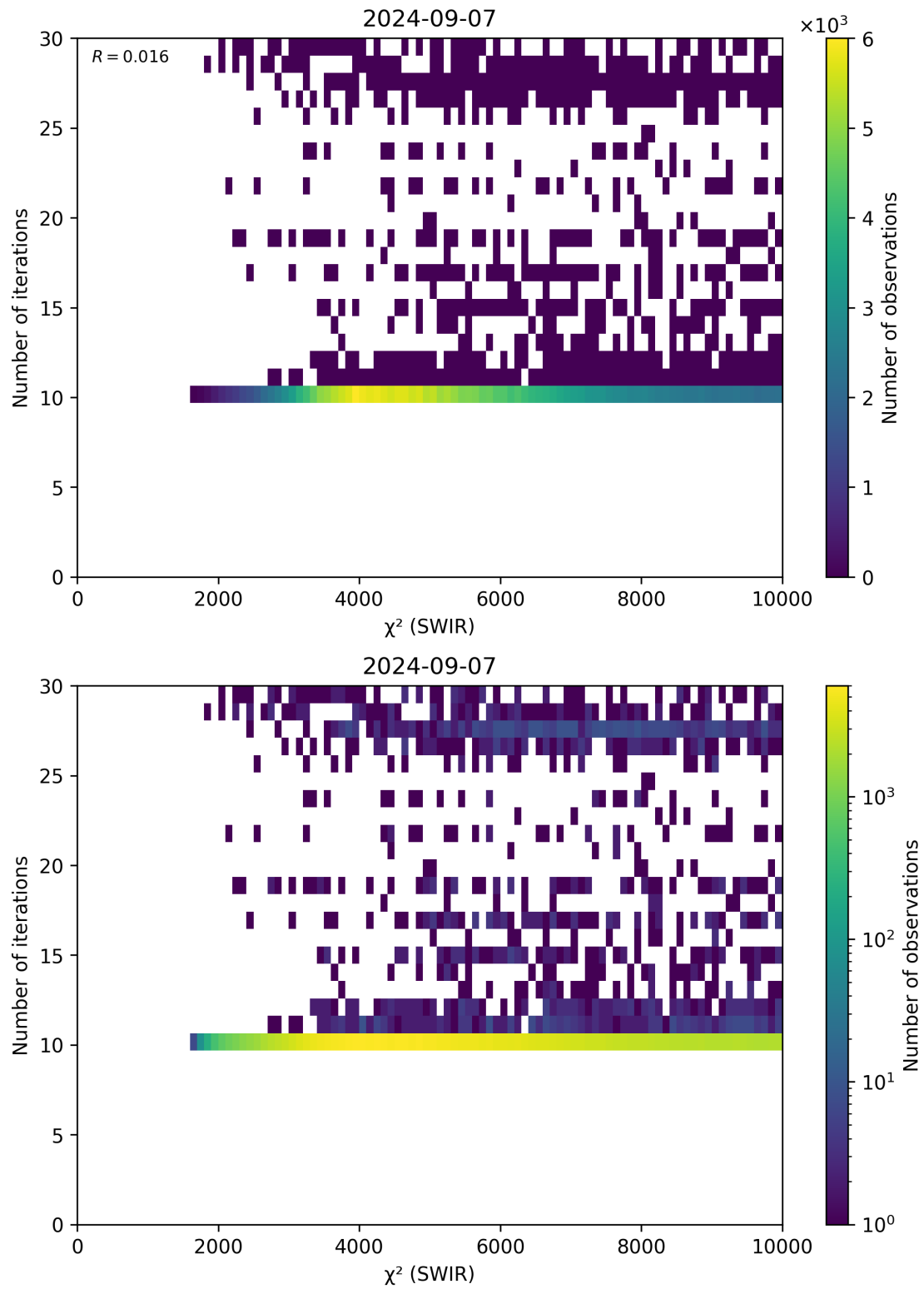
Figure 50: Scatter density plot of “ \chi^2 (SWIR)” against “Number of iterations” for 2024-09-06 to 2024-09-08.
