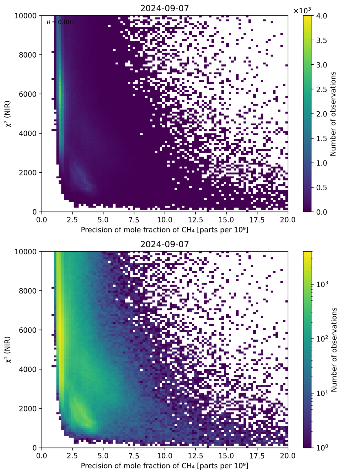
Figure 78: Scatter density plot of “Precision of mole fraction of \text{CH}_4 ” against “ \chi^2 (NIR)” for 2024-09-06 to 2024-09-08.
