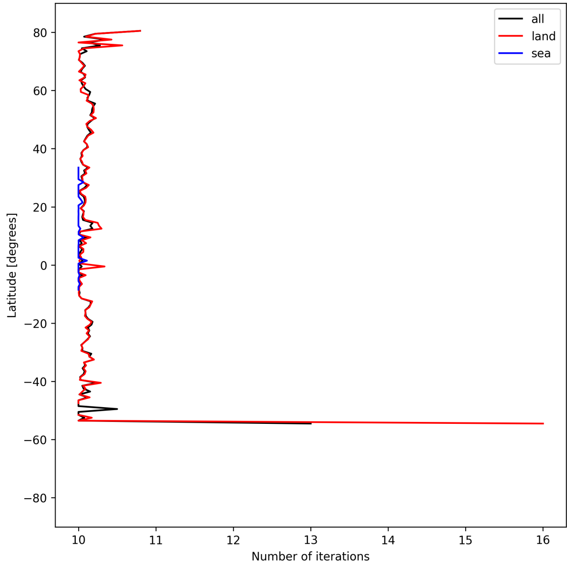
Figure 20: Zonal average of “Number of iterations” for 2024-09-06 to 2024-09-08.
