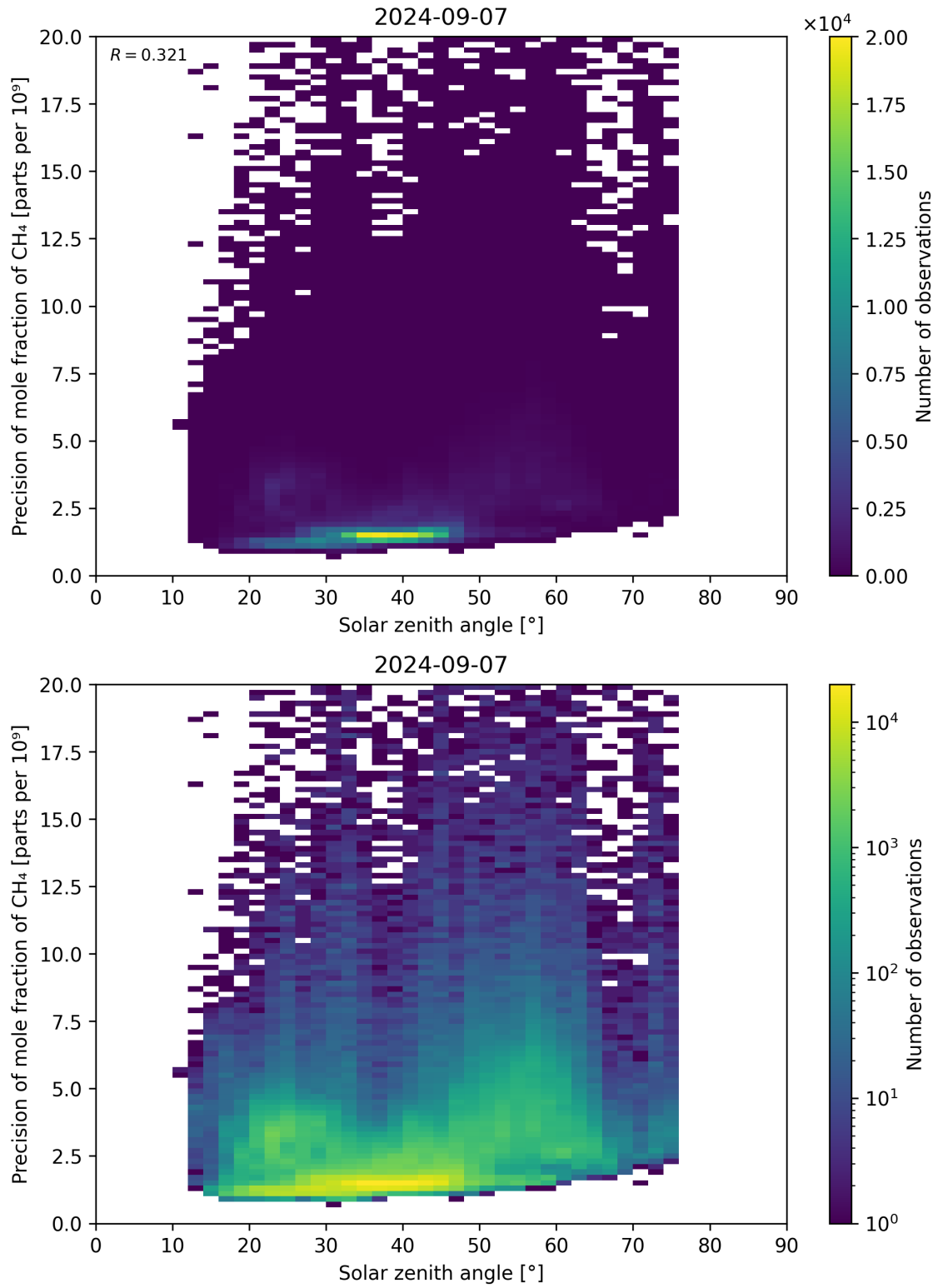
Figure 101: Scatter density plot of “Solar zenith angle” against “Precision of mole fraction of CH 4 ” for 2024-09-06 to 2024-09-08.
