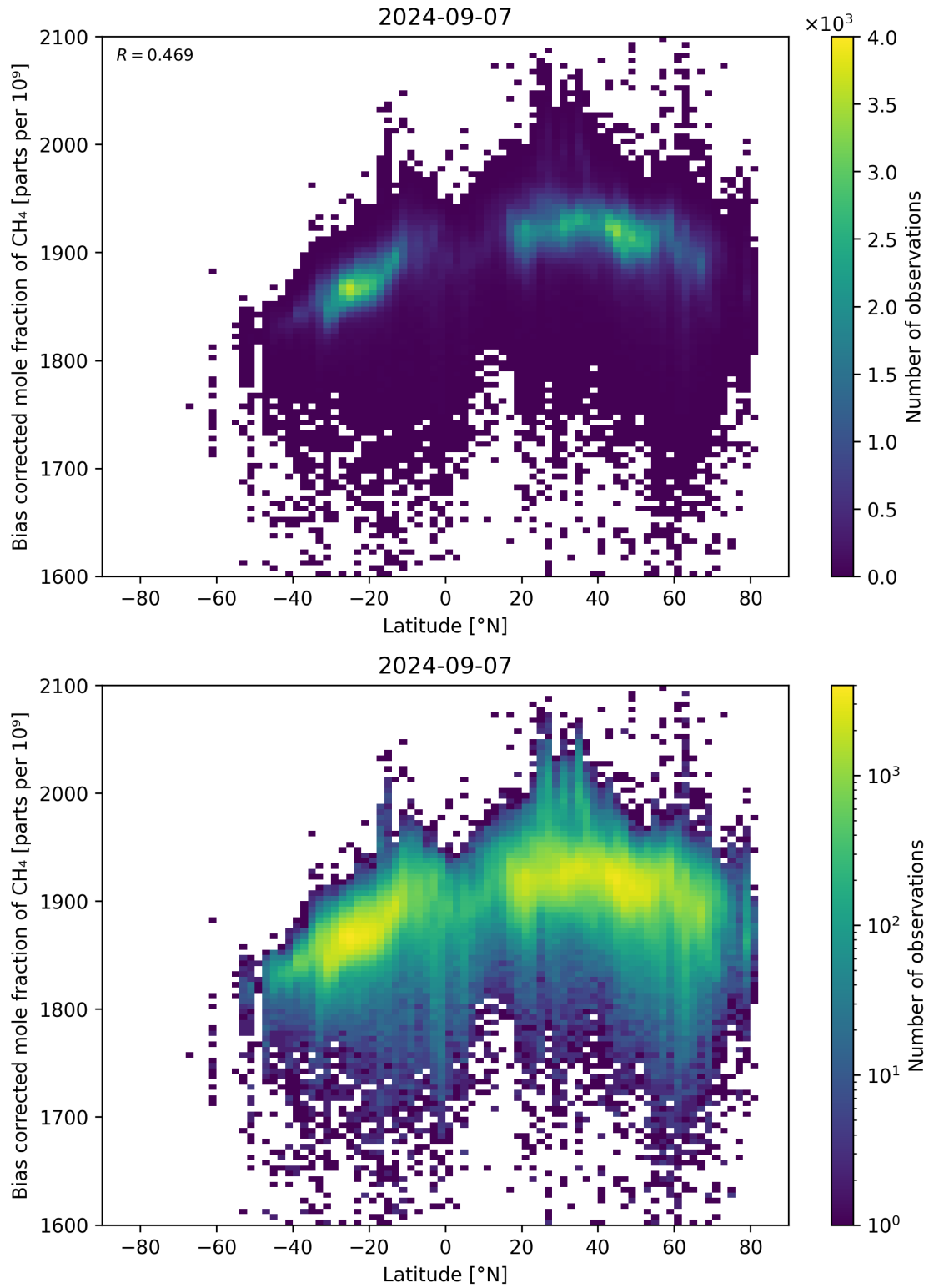
Figure 58: Scatter density plot of “Latitude” against “Bias corrected mole fraction of CH 4 ” for 2024-09-06 to 2024-09-08.
