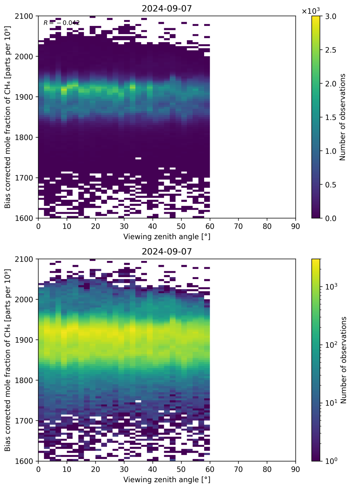
Figure 111: Scatter density plot of “Viewing zenith angle” against “Bias corrected mole fraction of CH 4 ” for 2024-09-06 to 2024-09-08.
