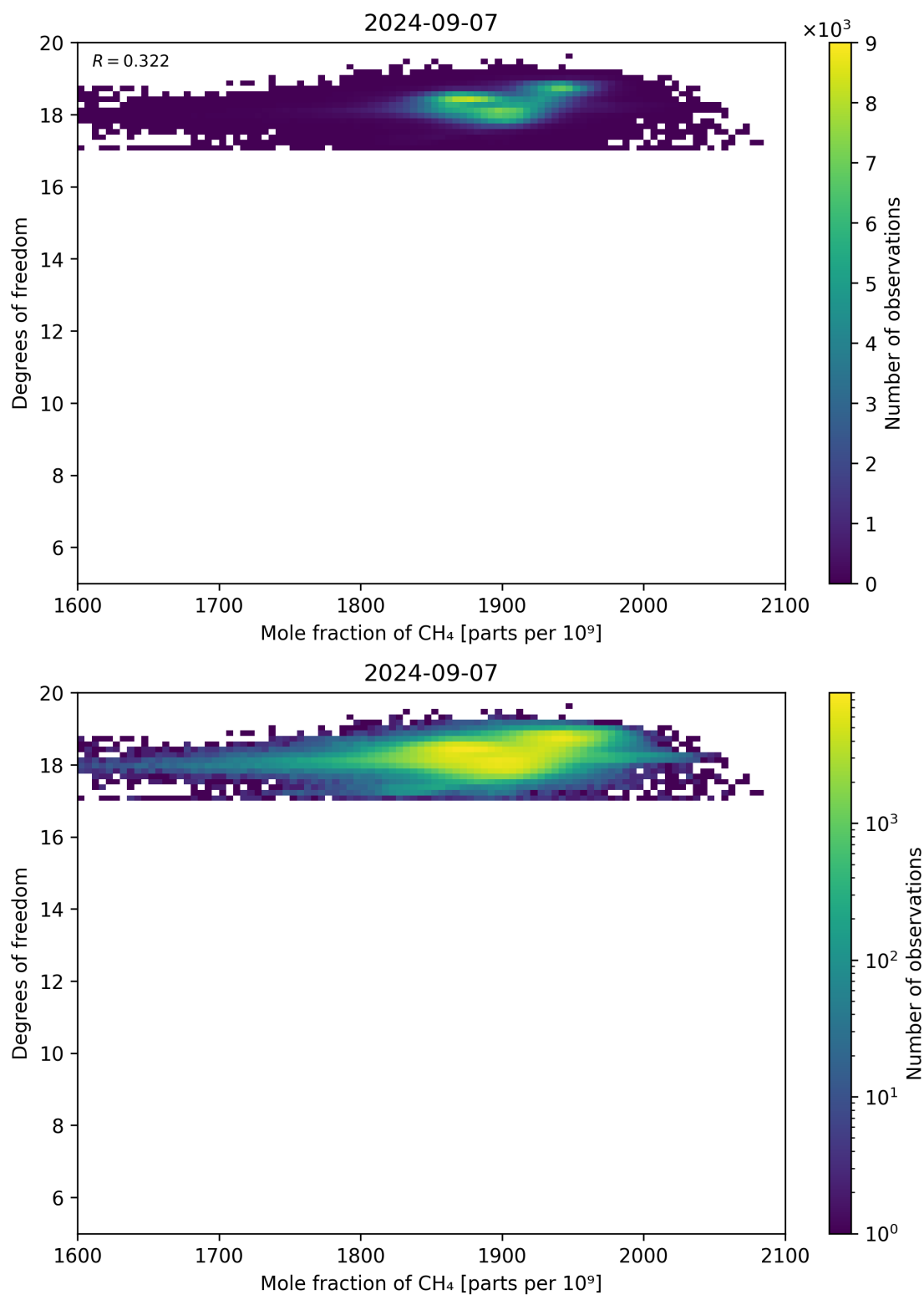
Figure 72: Scatter density plot of “Mole fraction of CH 4 ” against “Degrees of freedom” for 2024-09-06 to 2024-09-08.
