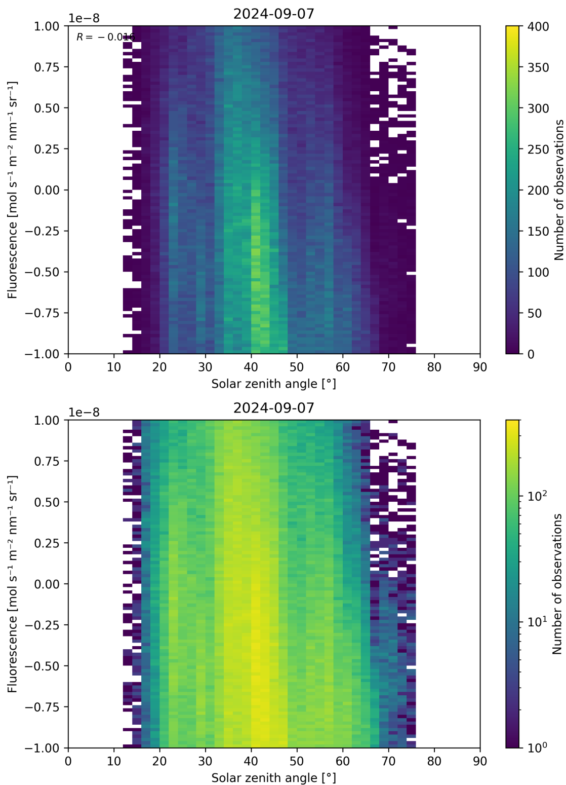
Figure 97: Scatter density plot of “Solar zenith angle” against “Fluorescence” for 2024-09-06 to 2024-09-08.
