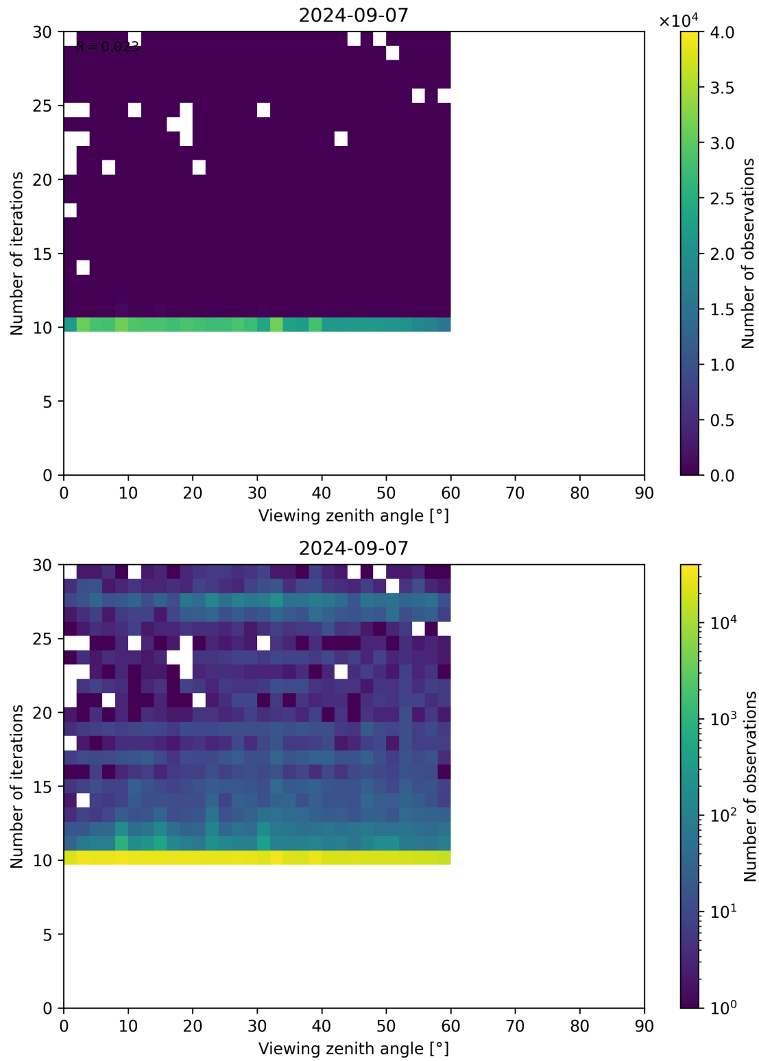
Figure 113: Scatter density plot of “Viewing zenith angle” against “Number of iterations” for 2024-09-06 to 2024-09-08.
