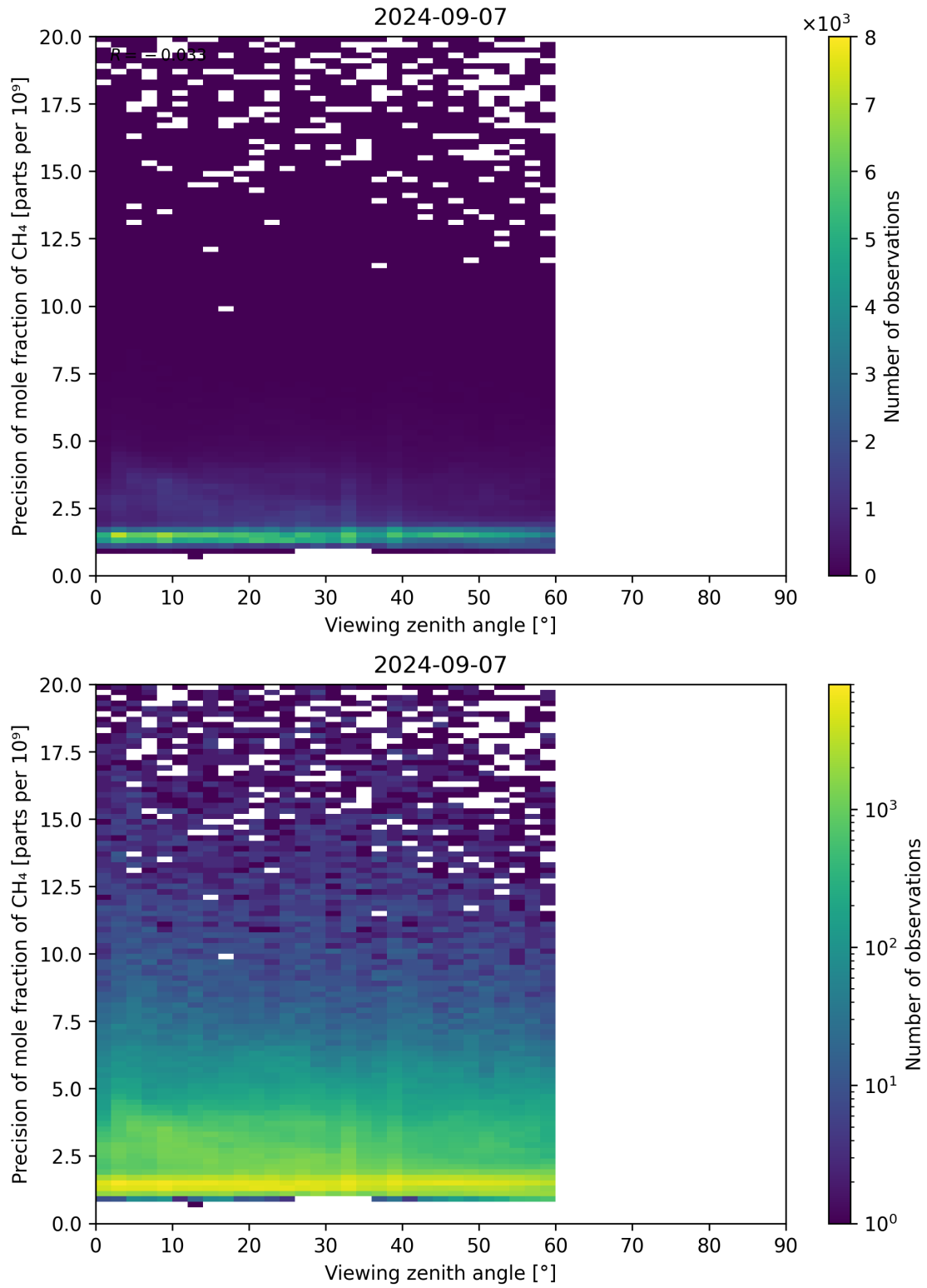
Figure 112: Scatter density plot of “Viewing zenith angle” against “Precision of mole fraction of CH 4 ” for 2024-09-06 to 2024-09-08.
