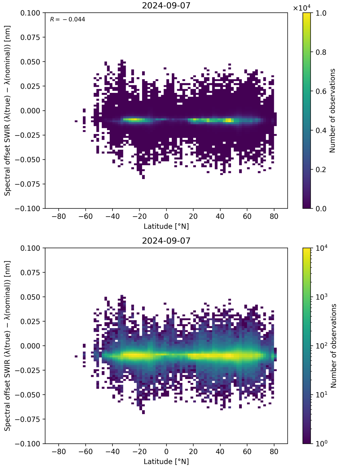
Figure 62: Scatter density plot of “Latitude” against “Spectral offset SWIR ( \lambda_{\text{true}} - \lambda_{\text{nominal}} )” for 2024-09-06 to 2024-09-08.
