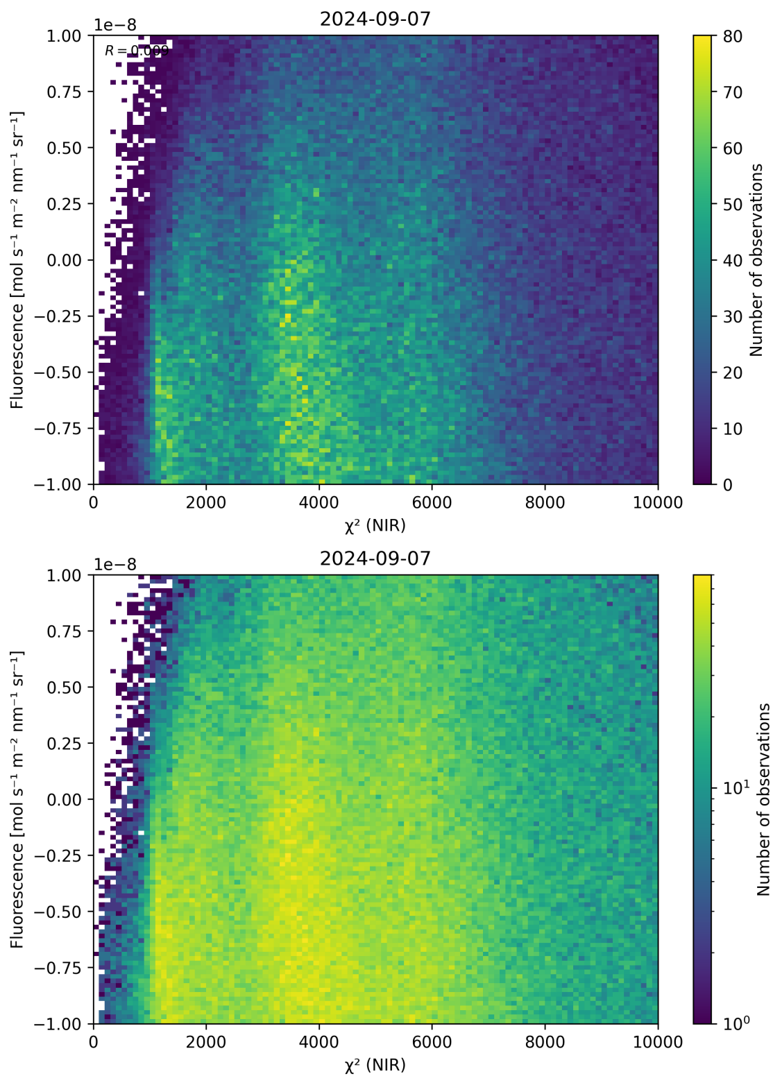
Figure 45: Scatter density plot of “ \chi^2 (NIR)” against “Fluorescence” for 2024-09-06 to 2024-09-08.
