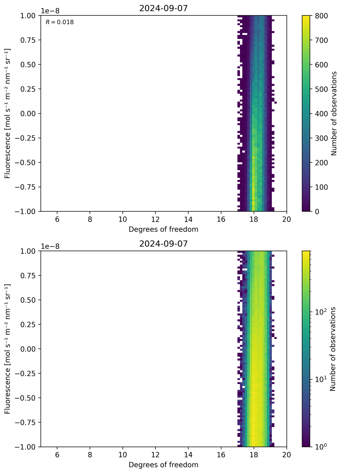
Figure 51: Scatter density plot of “Degrees of freedom” against “Fluorescence” for 2024-09-06 to 2024-09-08.
