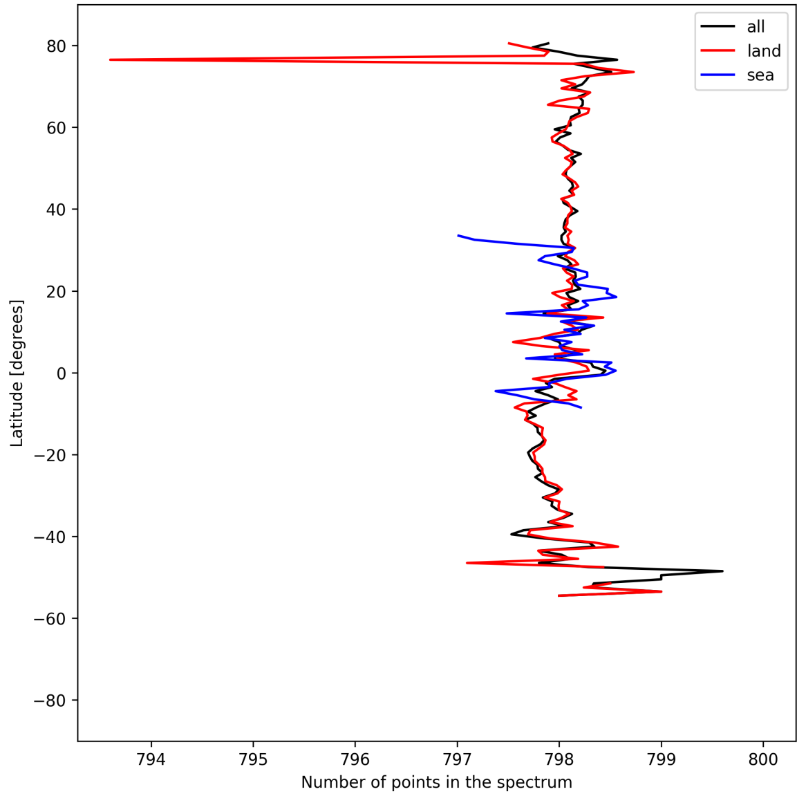
Figure 15: Zonal average of “Number of points in the spectrum” for 2024-09-06 to 2024-09-08.
