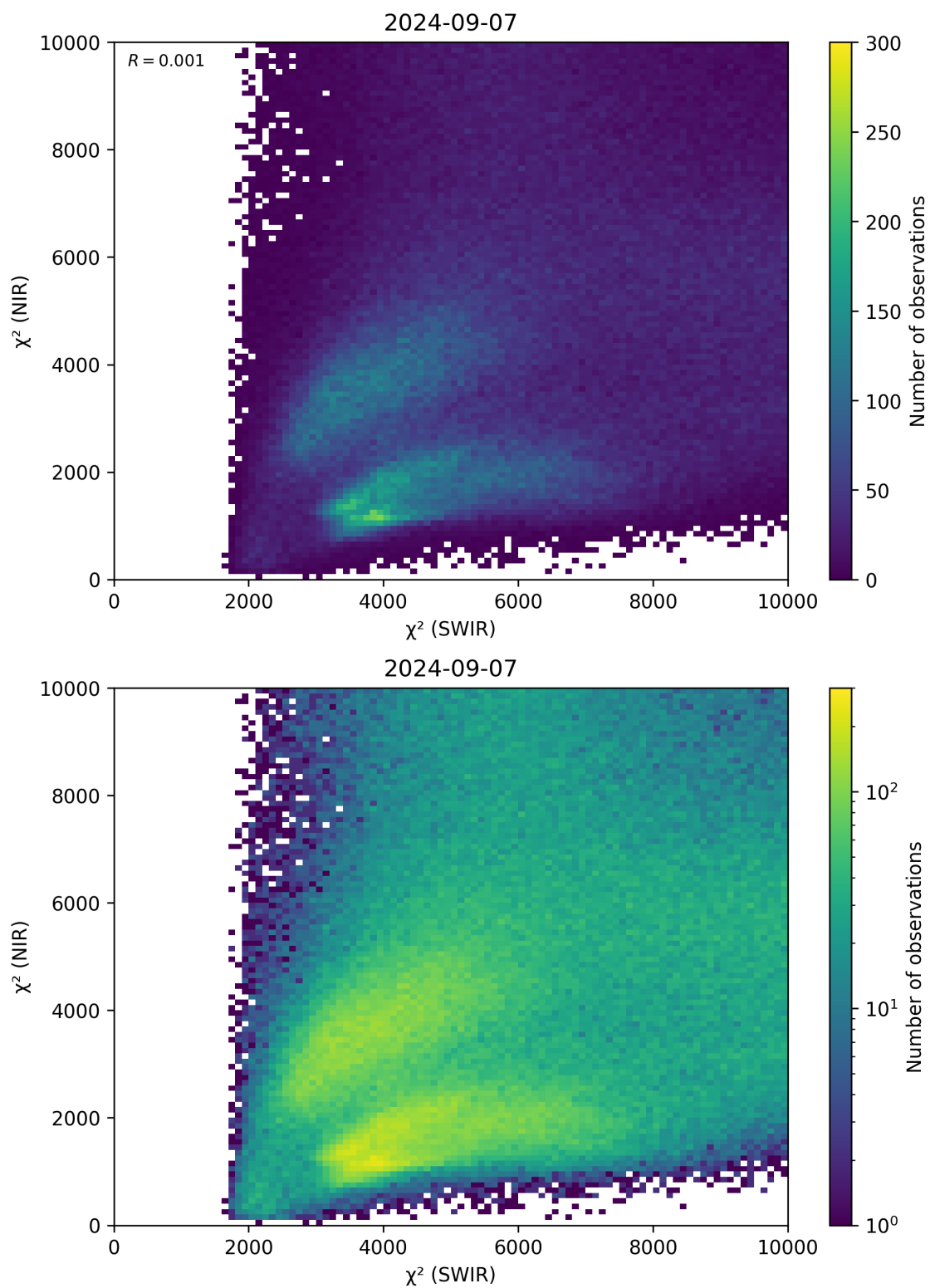
Figure 47: Scatter density plot of “ \chi^2 (SWIR)” against “ \chi^2 (NIR)” for 2024-09-06 to 2024-09-08.
