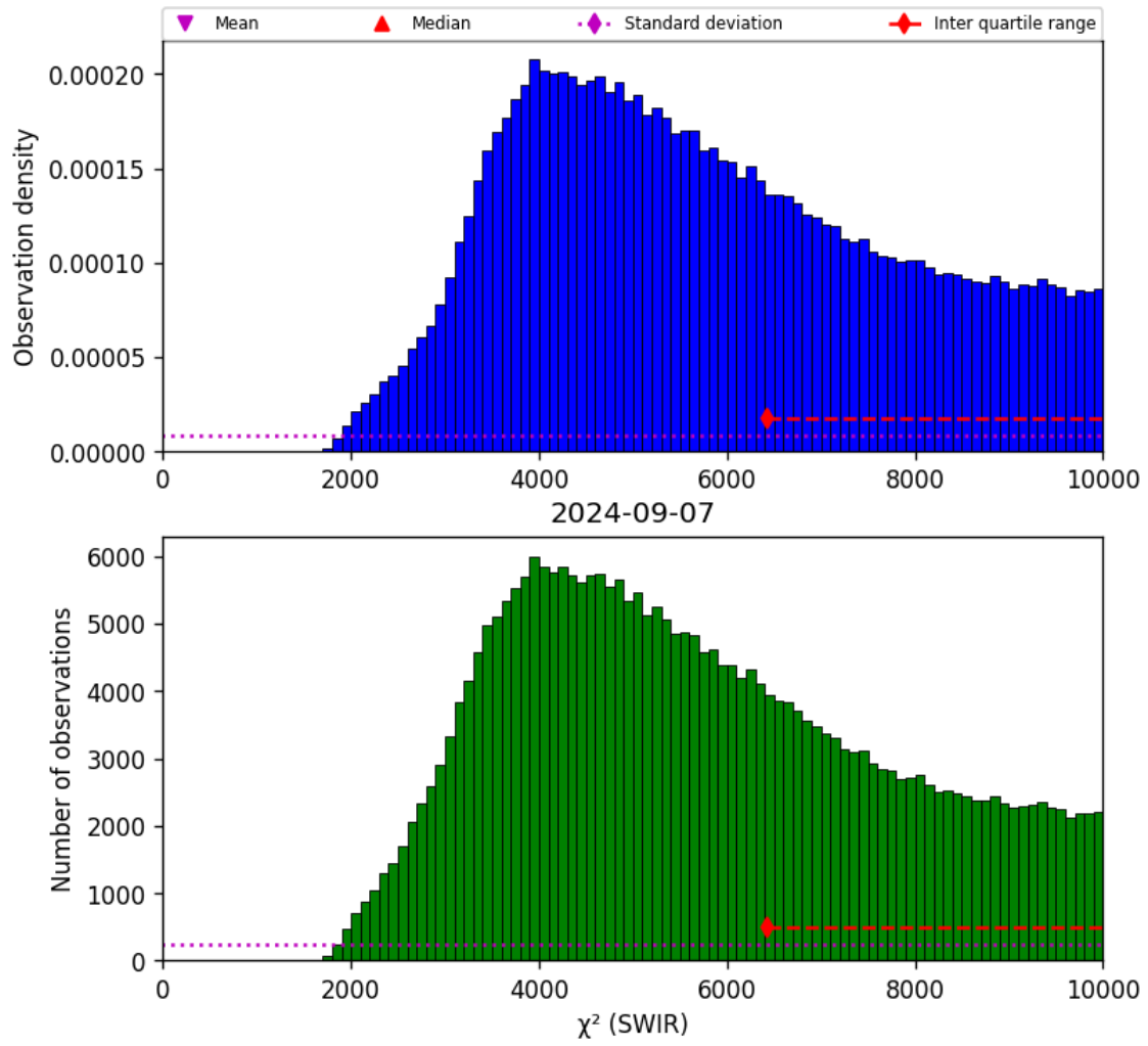
Figure 28: Histogram of “ \chi^2 (SWIR)” for 2024-09-06 to 2024-09-08
