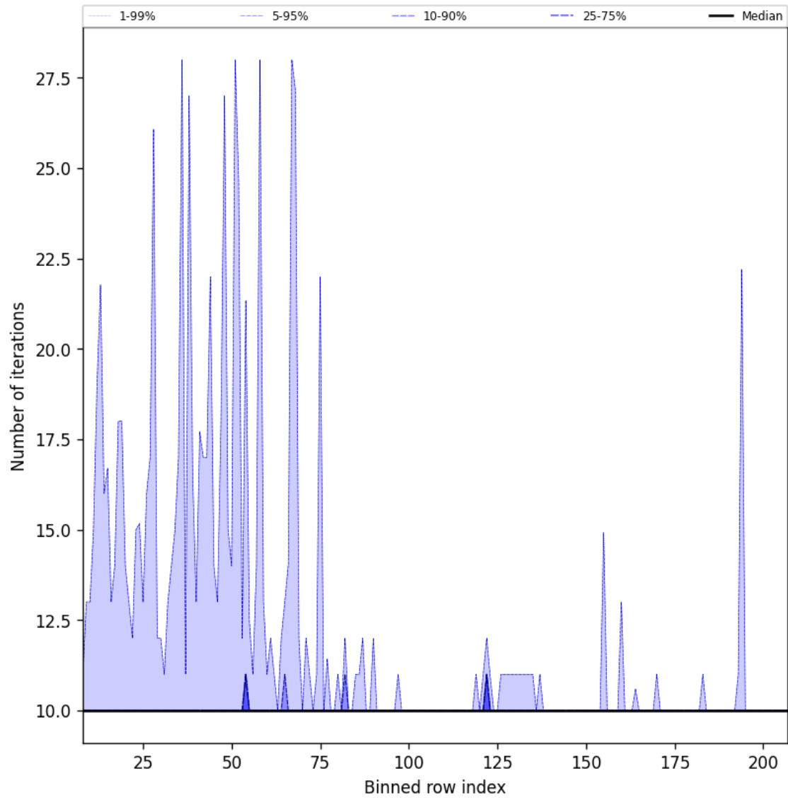
Figure 42: Along track statistics of “Number of iterations” for 2024-09-06 to 2024-09-08
