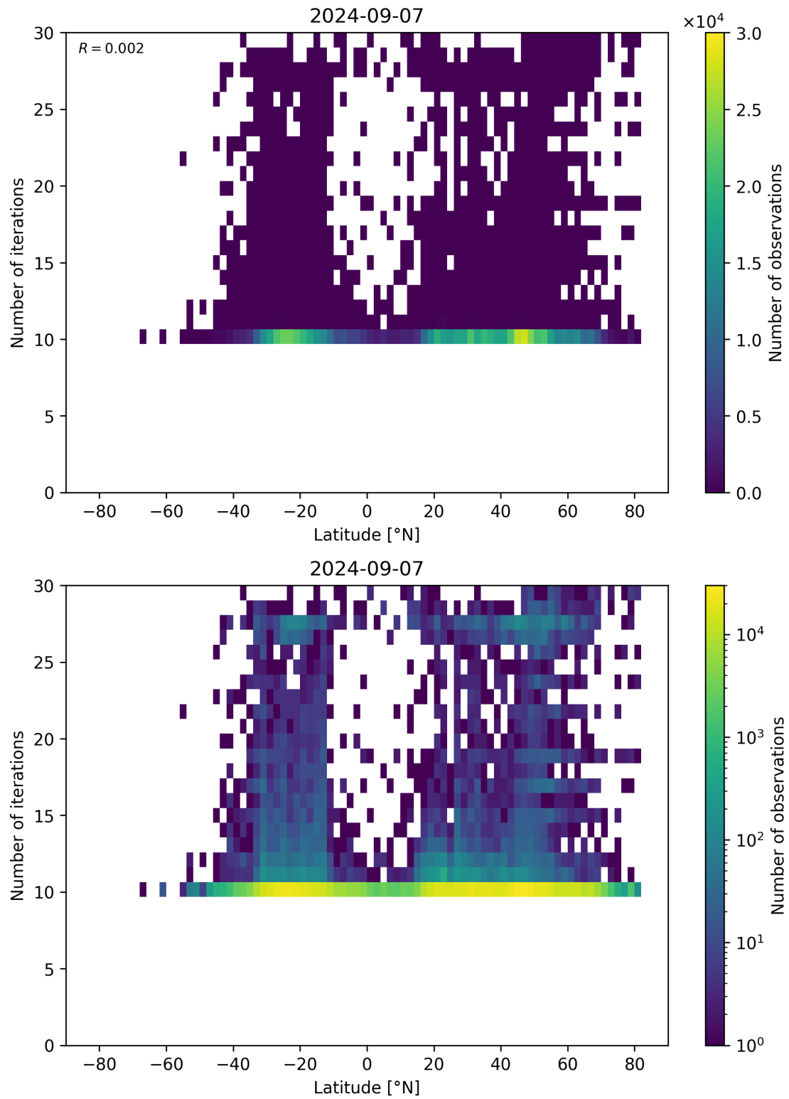
Figure 60: Scatter density plot of “Latitude” against “Number of iterations” for 2024-09-06 to 2024-09-08.
