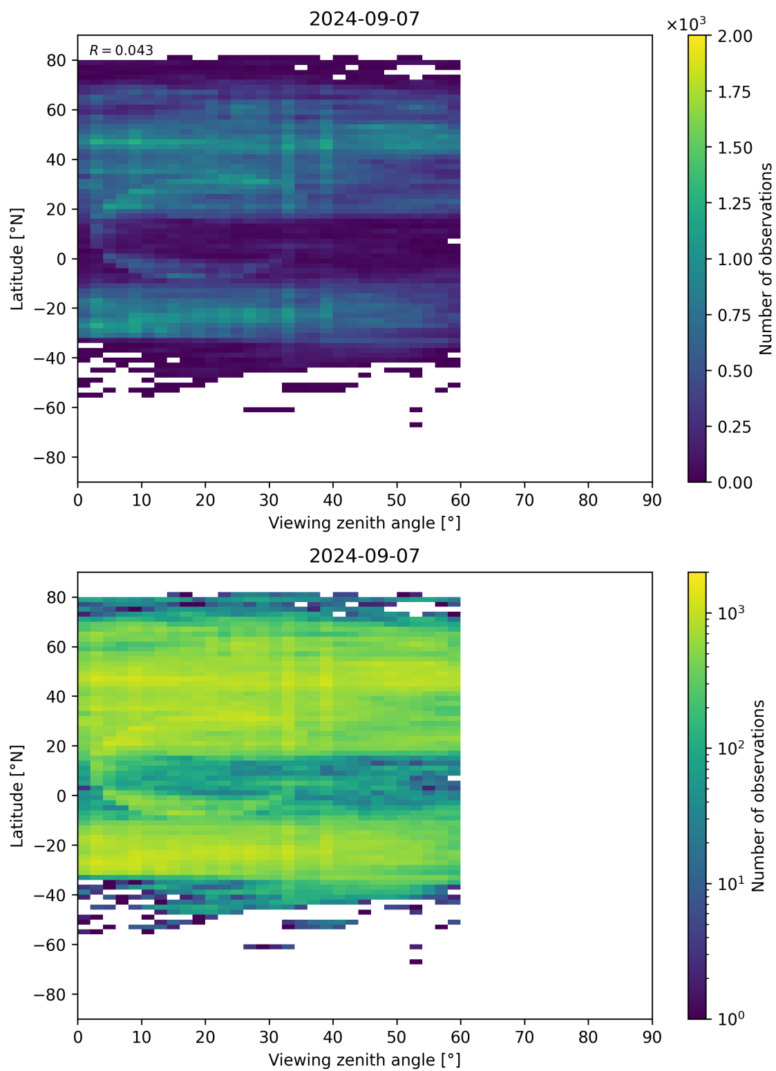
Figure 109: Scatter density plot of “Viewing zenith angle” against “Latitude” for 2024-09-06 to 2024-09-08.
