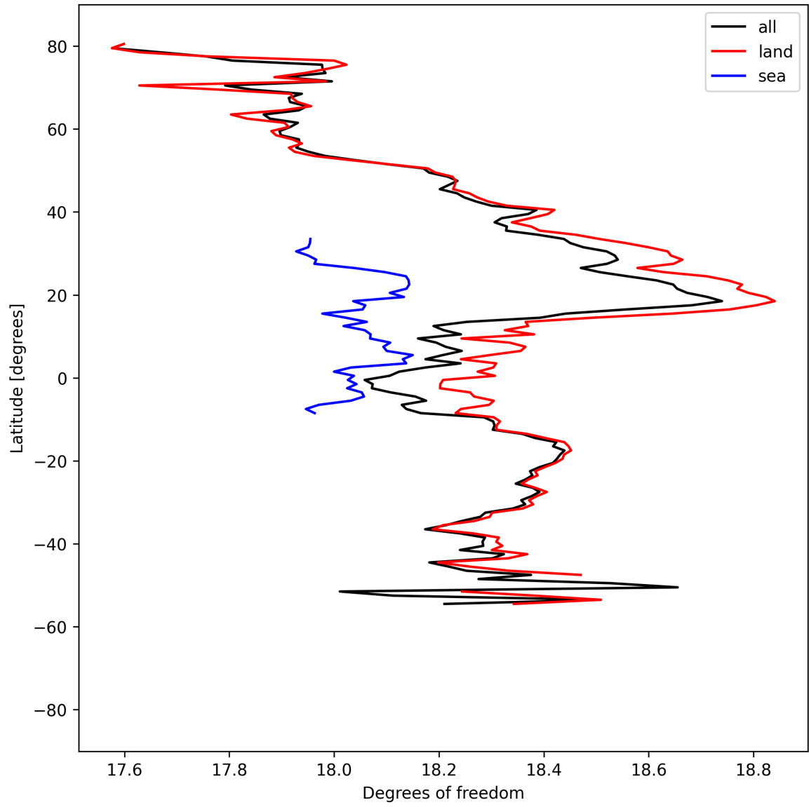
Figure 19: Zonal average of “Degrees of freedom” for 2024-09-06 to 2024-09-08.
