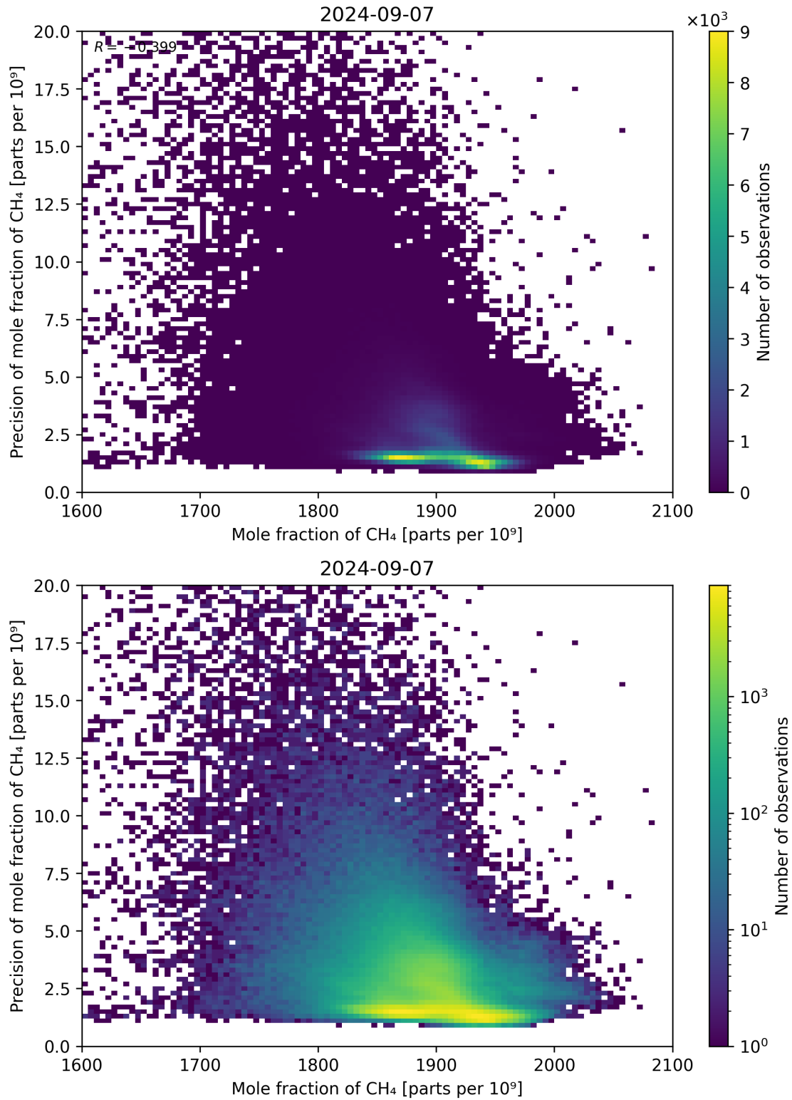
Figure 75: Scatter density plot of “Mole fraction of CH 4 ” against “Precision of mole fraction of CH 4 ” for 2024-09-06 to 2024-09-08.
