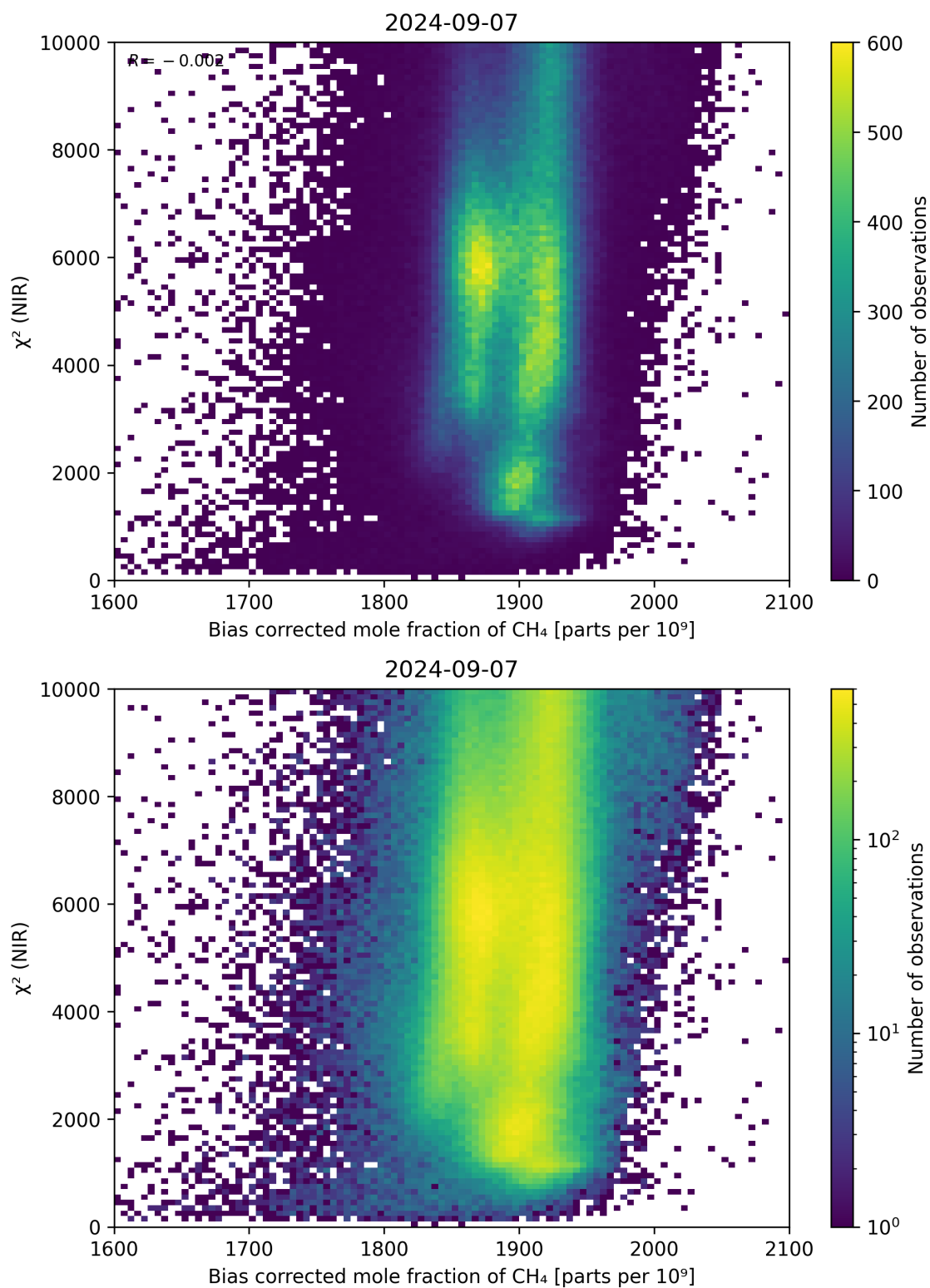
Figure 63: Scatter density plot of “Bias corrected mole fraction of \text{CH}_4 ” against “ \chi^2 (NIR)” for 2024-09-06 to 2024-09-08.
