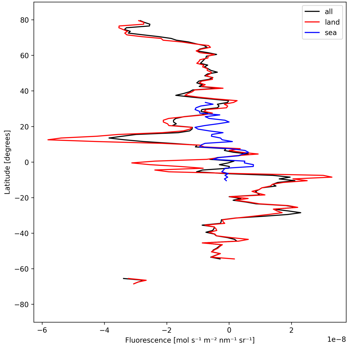
Figure 21: Zonal average of “Fluorescence” for 2024-09-07 to 2024-09-09.
