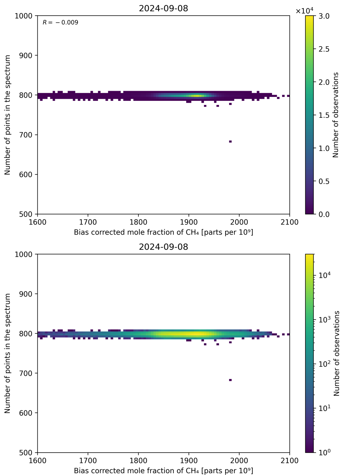
Figure 68: Scatter density plot of “Bias corrected mole fraction of CH 4 ” against “Number of points in the spectrum” for 2024-09-07 to 2024-09-09.
