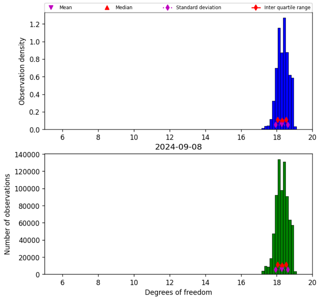
Figure 30: Histogram of “Degrees of freedom” for 2024-09-07 to 2024-09-09
