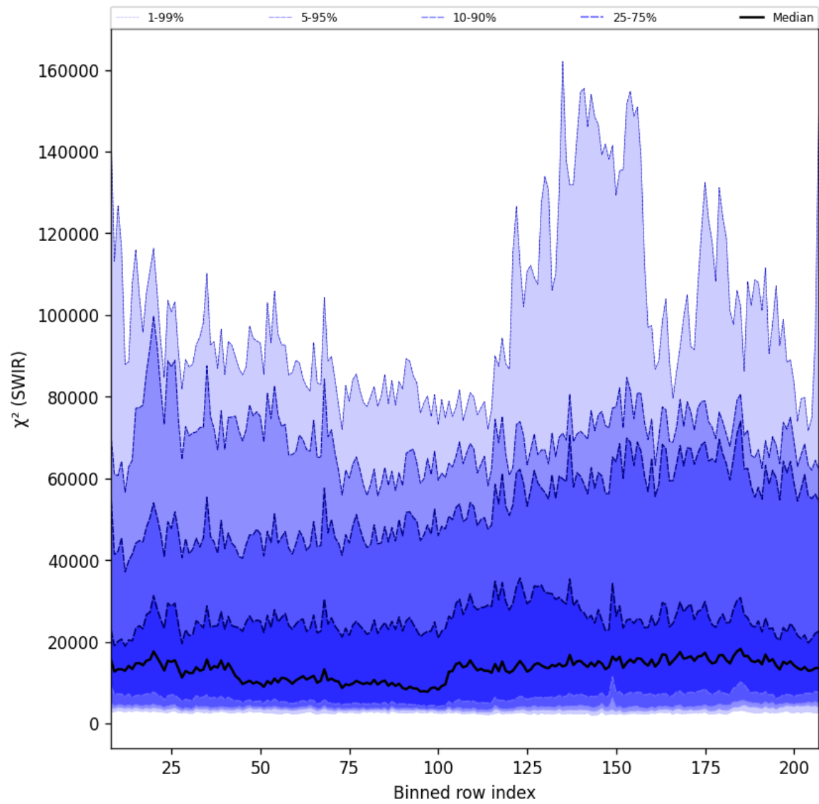
Figure 39: Along track statistics of “ \chi^2 (SWIR)” for 2024-09-07 to 2024-09-09
