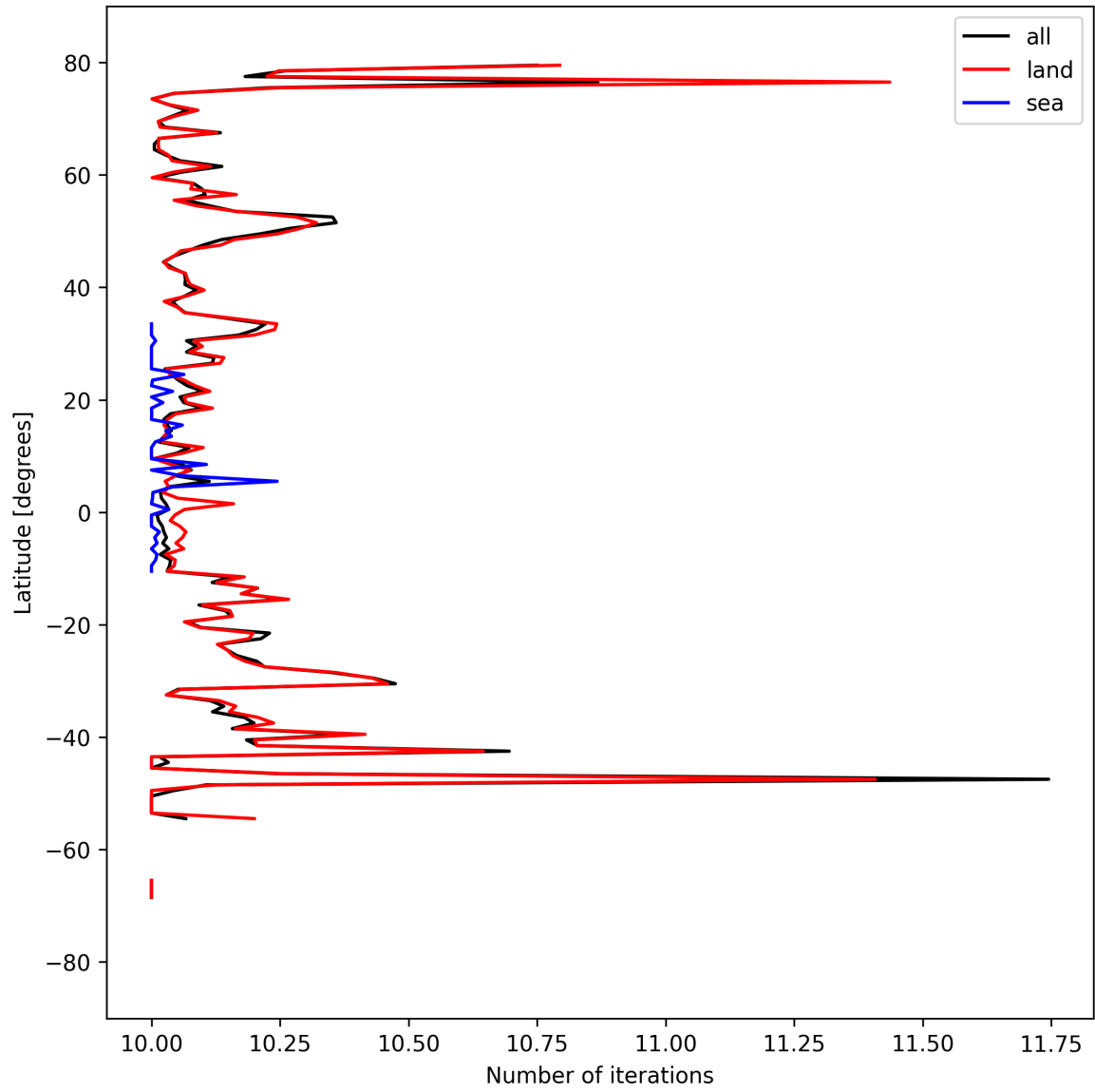
Figure 20: Zonal average of “Number of iterations” for 2024-09-07 to 2024-09-09.
