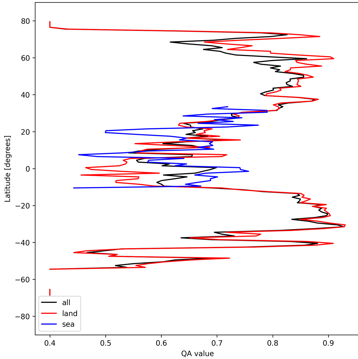
Figure 11: Zonal average of “QA value” for 2024-09-07 to 2024-09-09.
