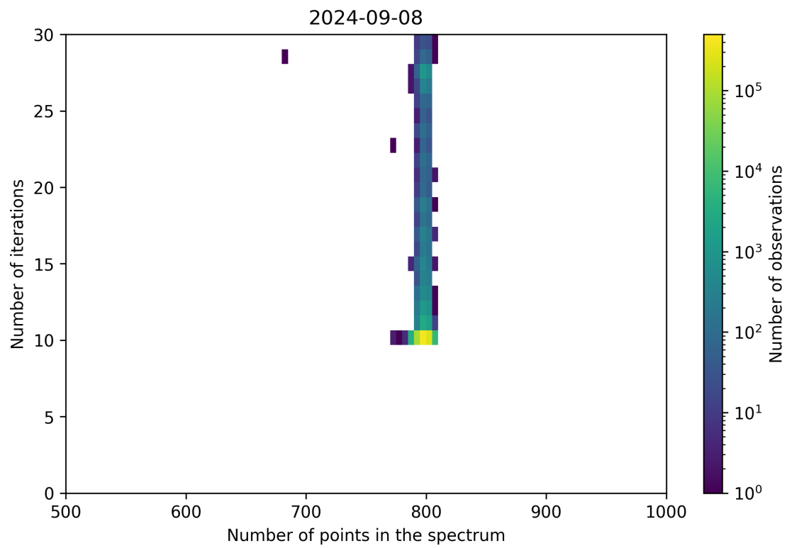
Figure 92: Scatter density plot of “Number of points in the spectrum” against “Number of iterations” for 2024-09-07 to 2024-09-09.
