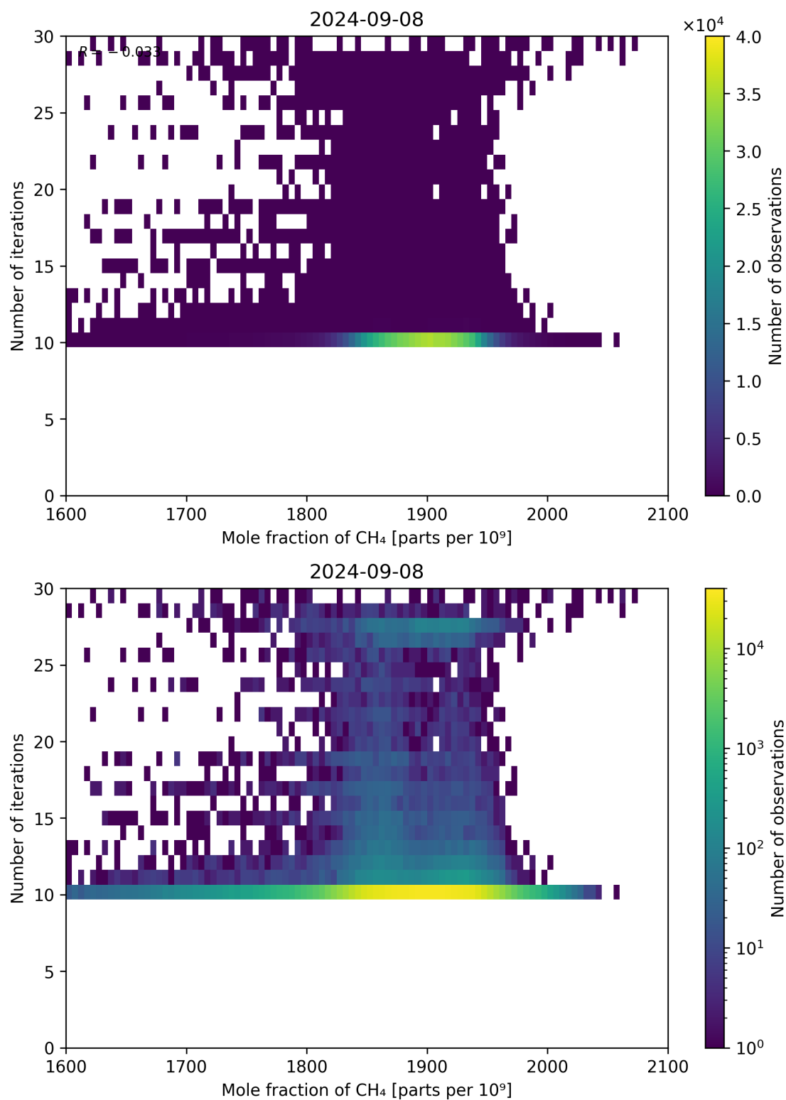
Figure 76: Scatter density plot of “Mole fraction of CH 4 ” against “Number of iterations” for 2024-09-07 to 2024-09-09.
