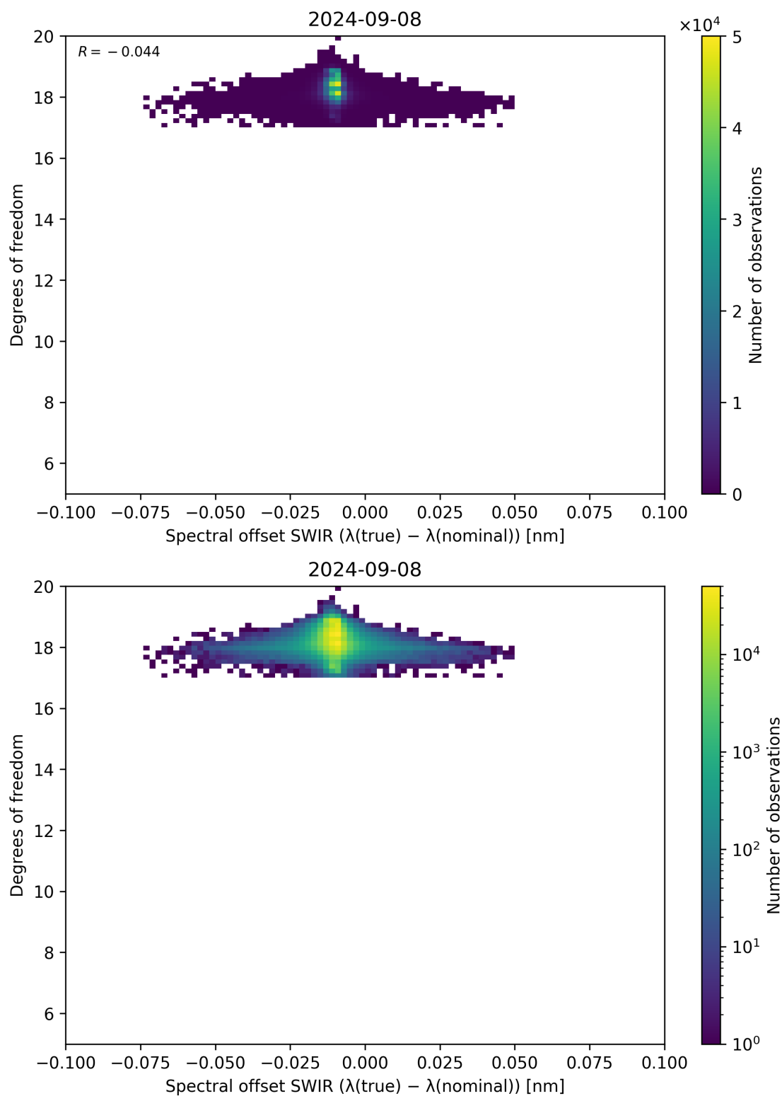
Figure 119: Scatter density plot of “Spectral offset SWIR ( \lambda_{\text{true}} - \lambda_{\text{nominal}} )” against “Degrees of freedom” for 2024-09-07 to 2024-09-09.
