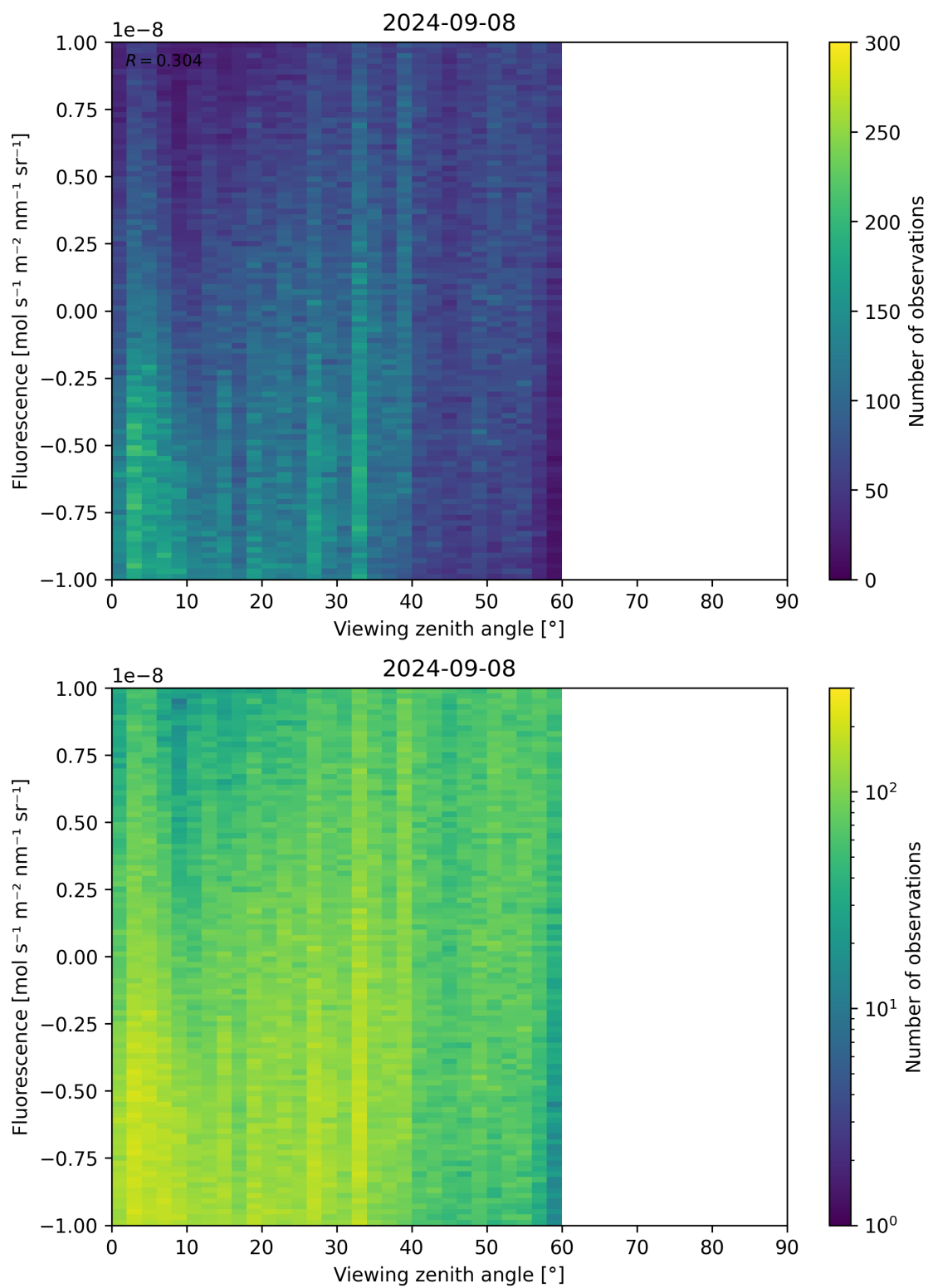
Figure 108: Scatter density plot of “Viewing zenith angle” against “Fluorescence” for 2024-09-07 to 2024-09-09.
