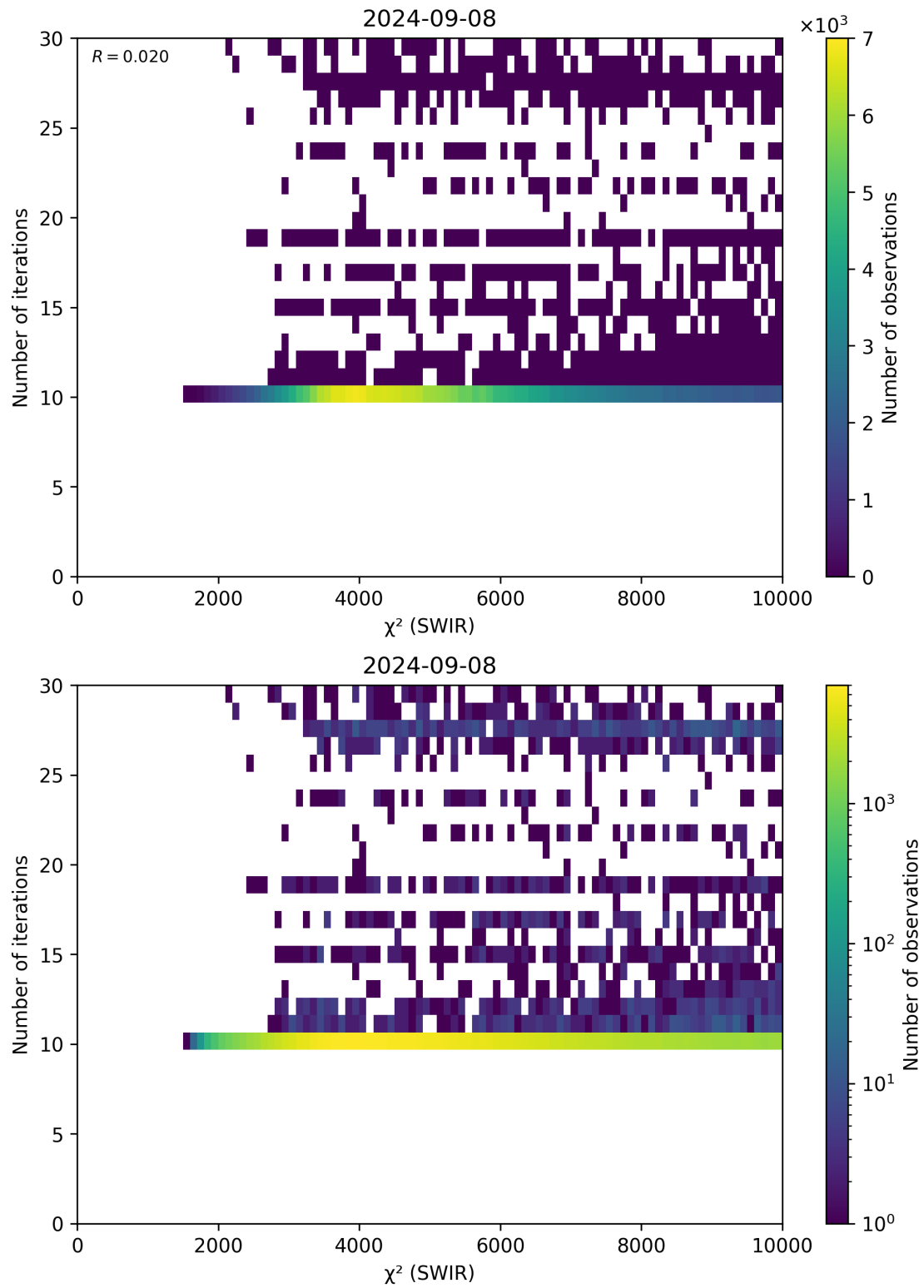
Figure 50: Scatter density plot of “ \chi^2 (SWIR)” against “Number of iterations” for 2024-09-07 to 2024-09-09.
