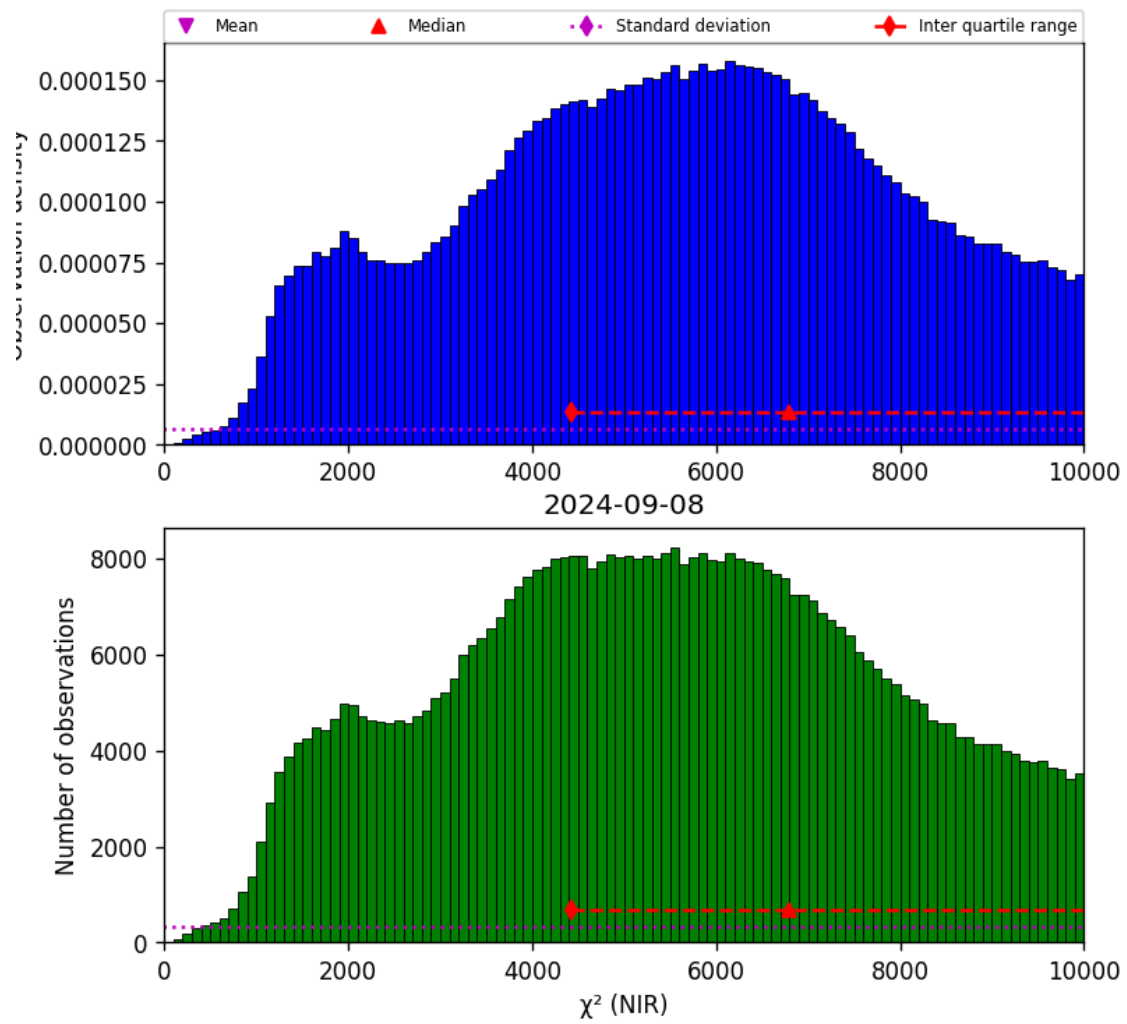
Figure 29: Histogram of “ \chi^2 (NIR)” for 2024-09-07 to 2024-09-09
