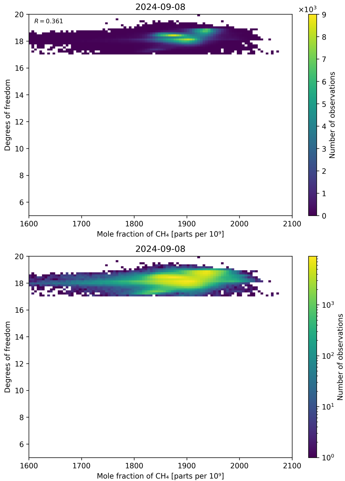
Figure 72: Scatter density plot of “Mole fraction of CH 4 ” against “Degrees of freedom” for 2024-09-07 to 2024-09-09.
