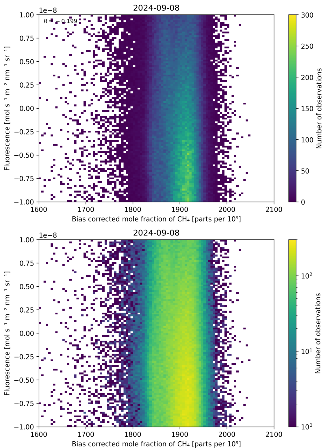
Figure 66: Scatter density plot of “Bias corrected mole fraction of \text{CH}_4 ” against “Fluorescence” for 2024-09-07 to 2024-09-09.
