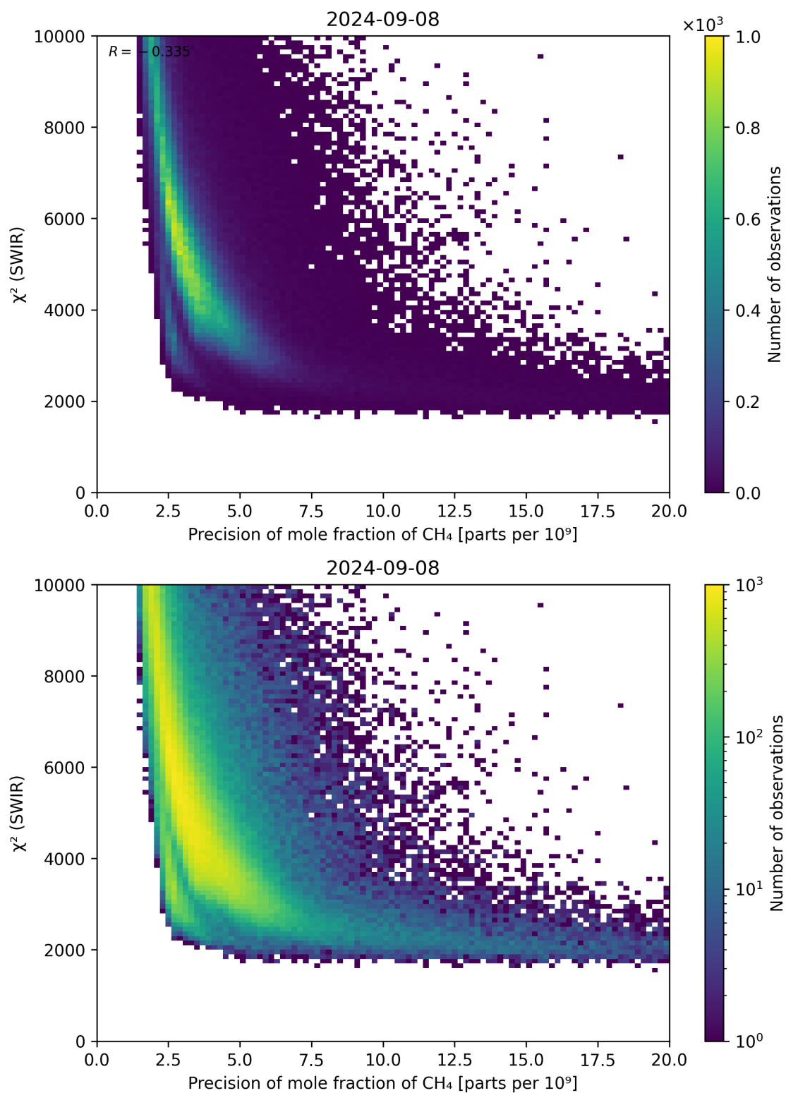
Figure 79: Scatter density plot of “Precision of mole fraction of \text{CH}_4 ” against “ \chi^2 (SWIR)” for 2024-09-07 to 2024-09-09.
