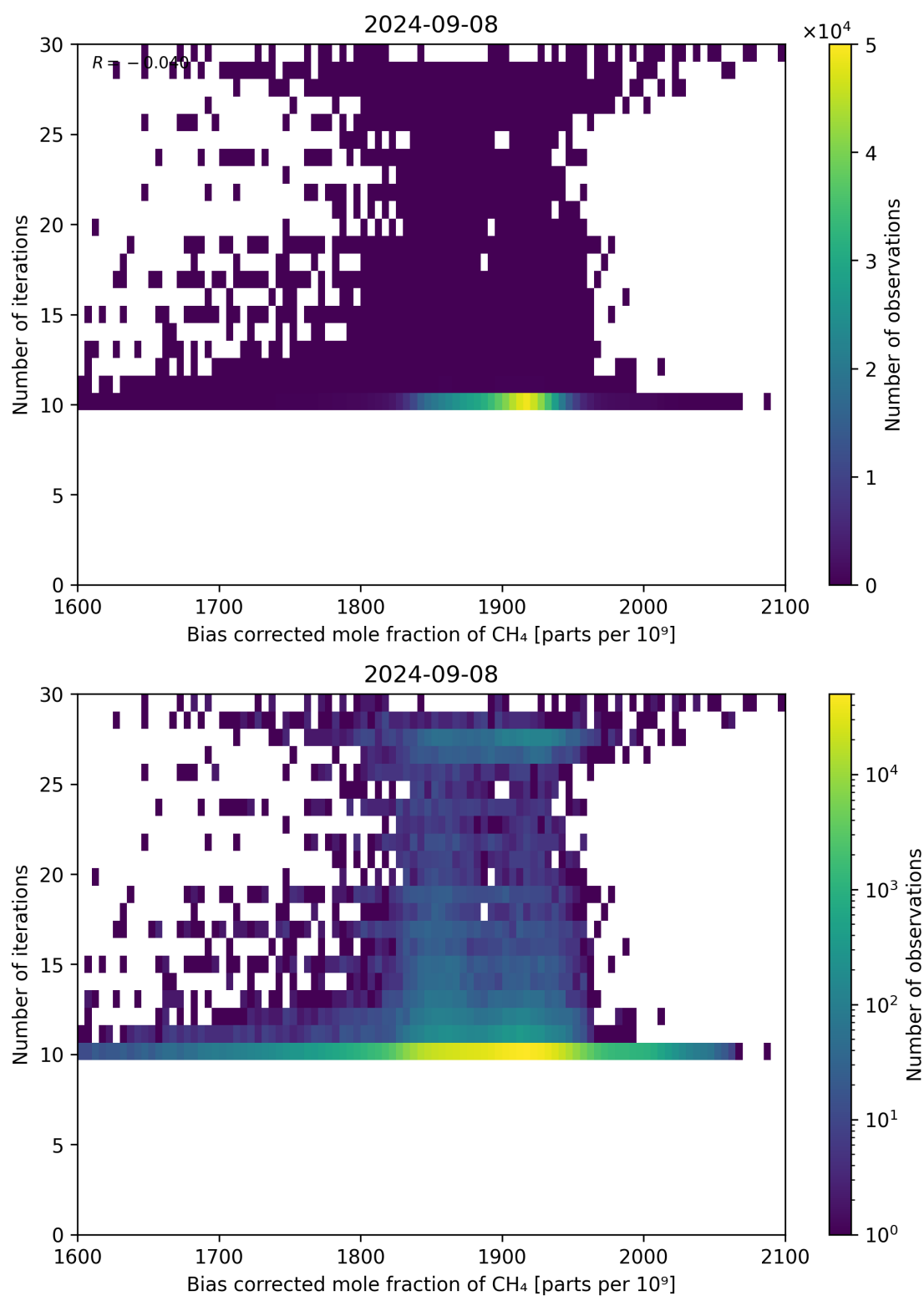
Figure 67: Scatter density plot of “Bias corrected mole fraction of CH 4 ” against “Number of iterations” for 2024-09-07 to 2024-09-09.
