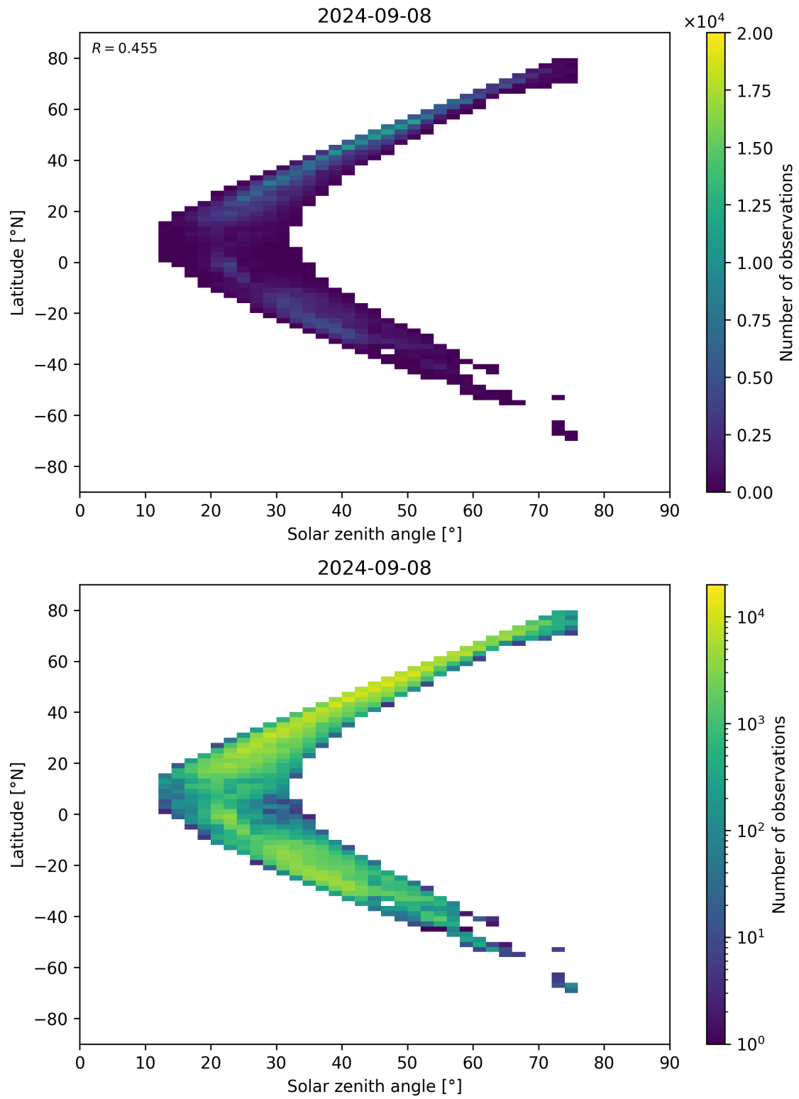
Figure 98: Scatter density plot of “Solar zenith angle” against “Latitude” for 2024-09-07 to 2024-09-09.
