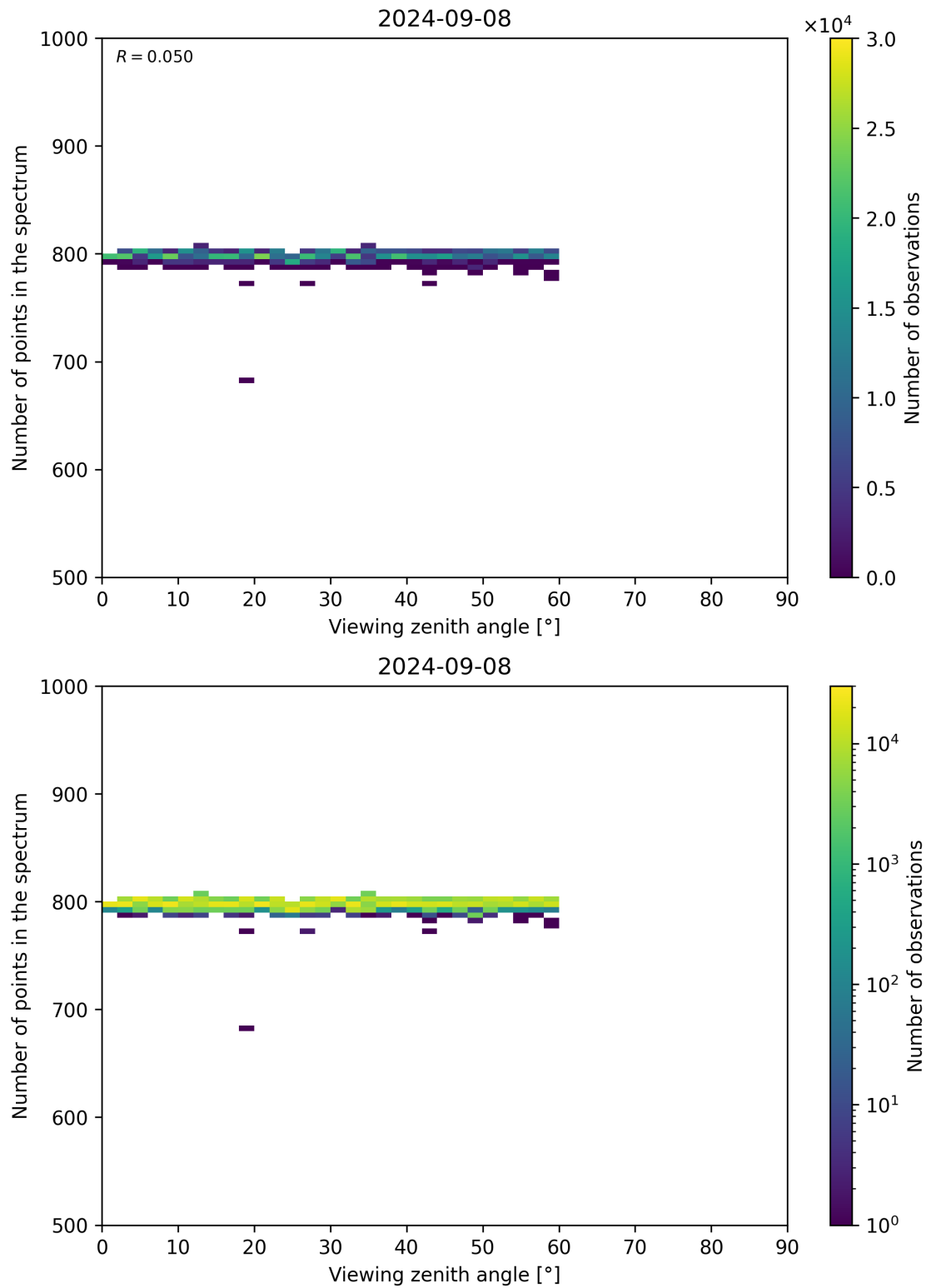
Figure 114: Scatter density plot of “Viewing zenith angle” against “Number of points in the spectrum” for 2024-09-07 to 2024-09-09.
