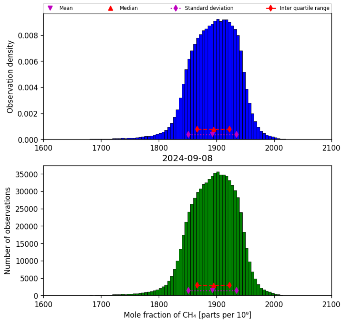
Figure 23: Histogram of “Mole fraction of CH 4 ” for 2024-09-07 to 2024-09-09
