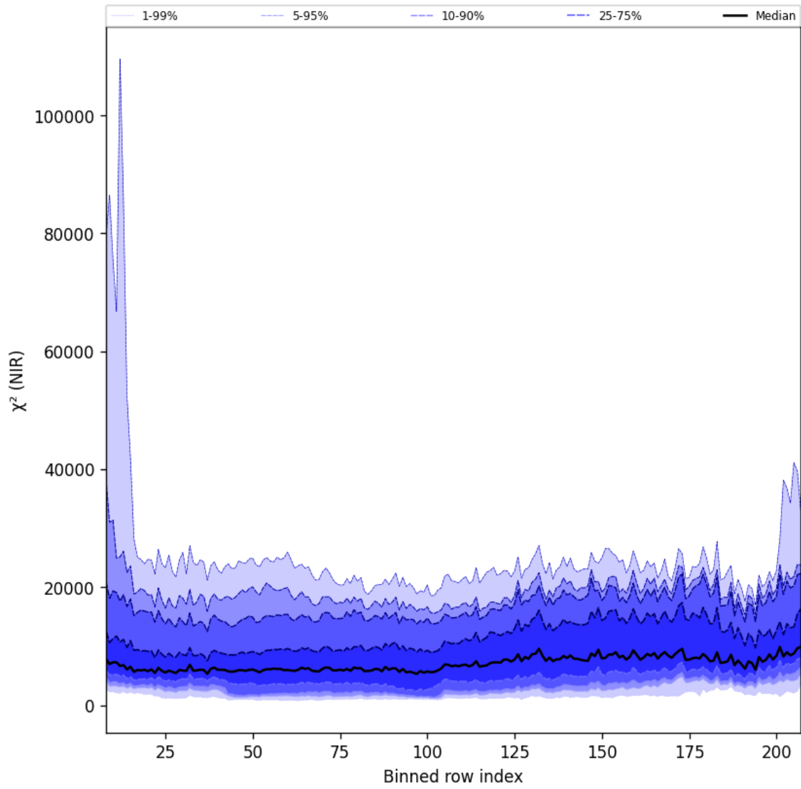
Figure 40: Along track statistics of “ \chi^2 (NIR)” for 2024-09-07 to 2024-09-09
