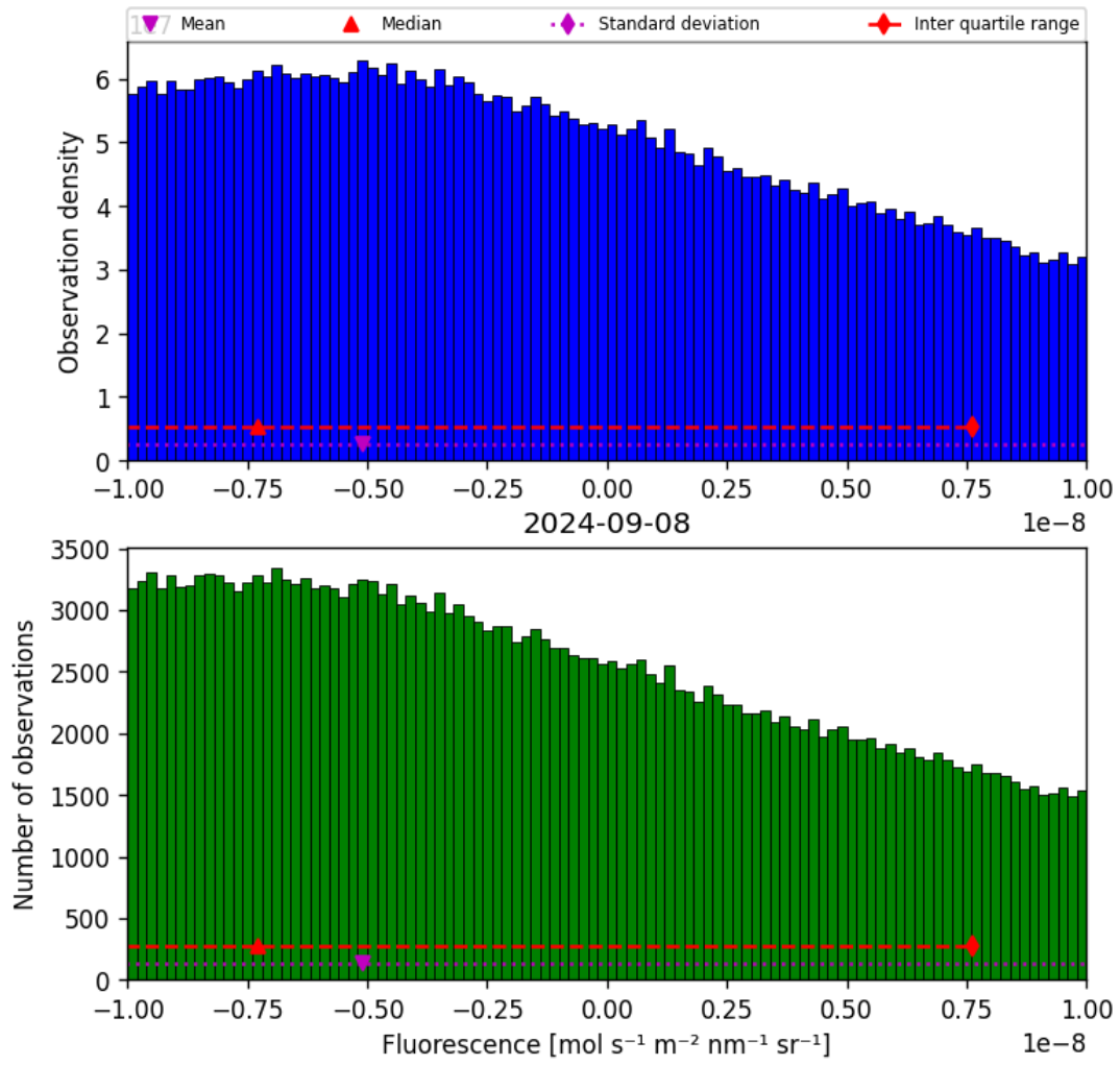
Figure 32: Histogram of “Fluorescence” for 2024-09-07 to 2024-09-09
