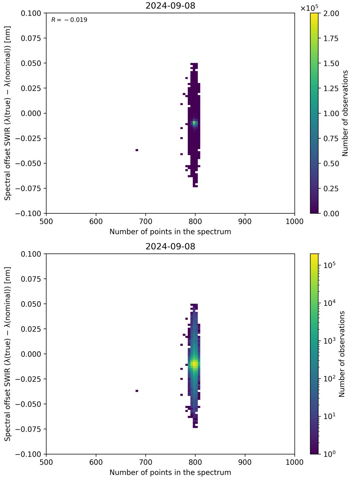
Figure 93: Scatter density plot of “Number of points in the spectrum” against “Spectral offset SWIR ( \lambda_{\text{true}} - \lambda_{\text{nominal}} )” for 2024-09-07 to 2024-09-09.
