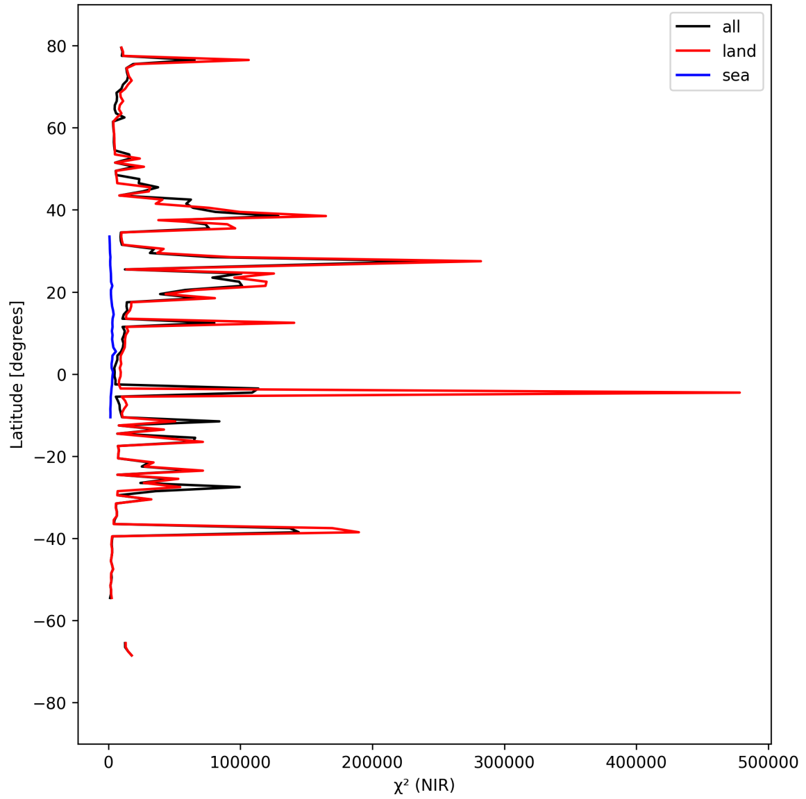
Figure 18: Zonal average of “ \chi^2 (NIR)” for 2024-09-07 to 2024-09-09.
