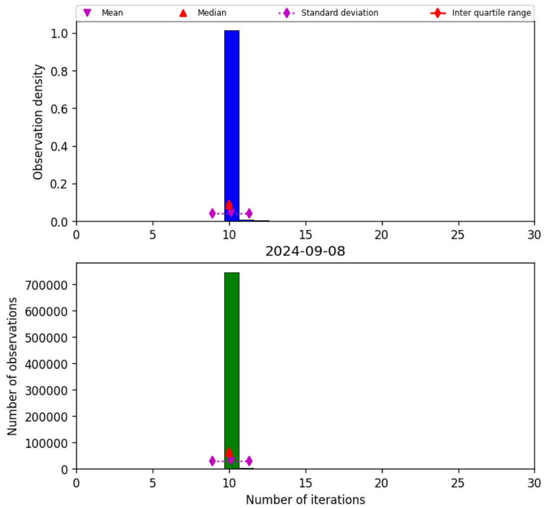
Figure 31: Histogram of “Number of iterations” for 2024-09-07 to 2024-09-09
