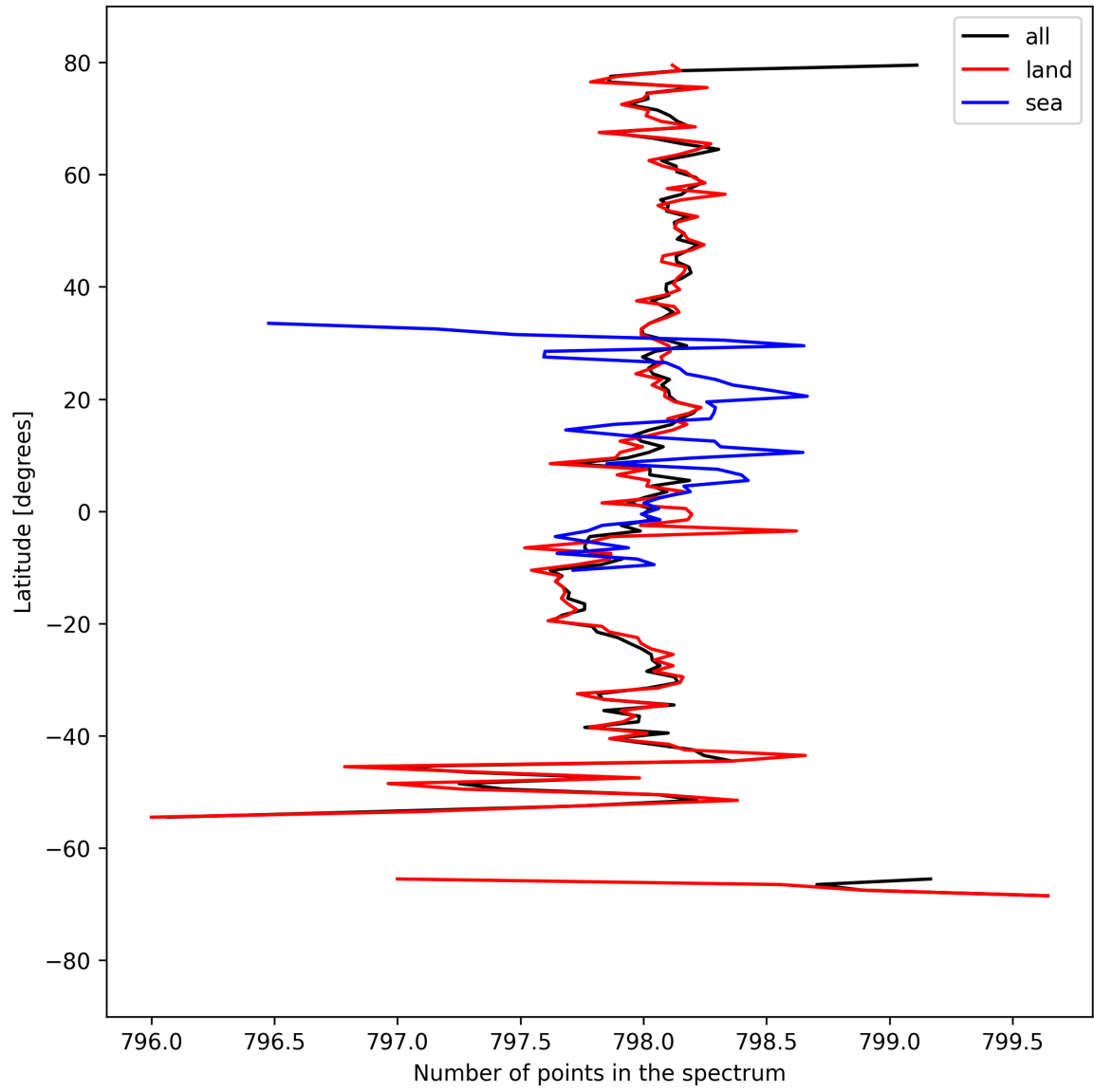
Figure 15: Zonal average of “Number of points in the spectrum” for 2024-09-07 to 2024-09-09.
