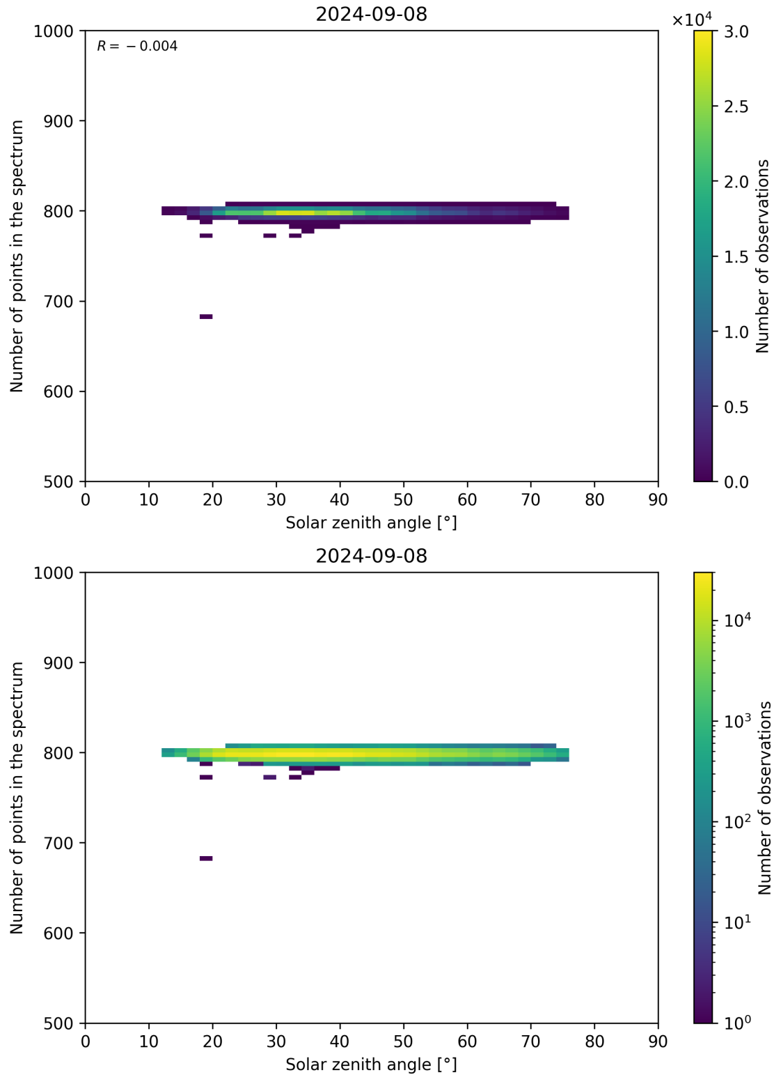
Figure 103: Scatter density plot of “Solar zenith angle” against “Number of points in the spectrum” for 2024-09-07 to 2024-09-09.
