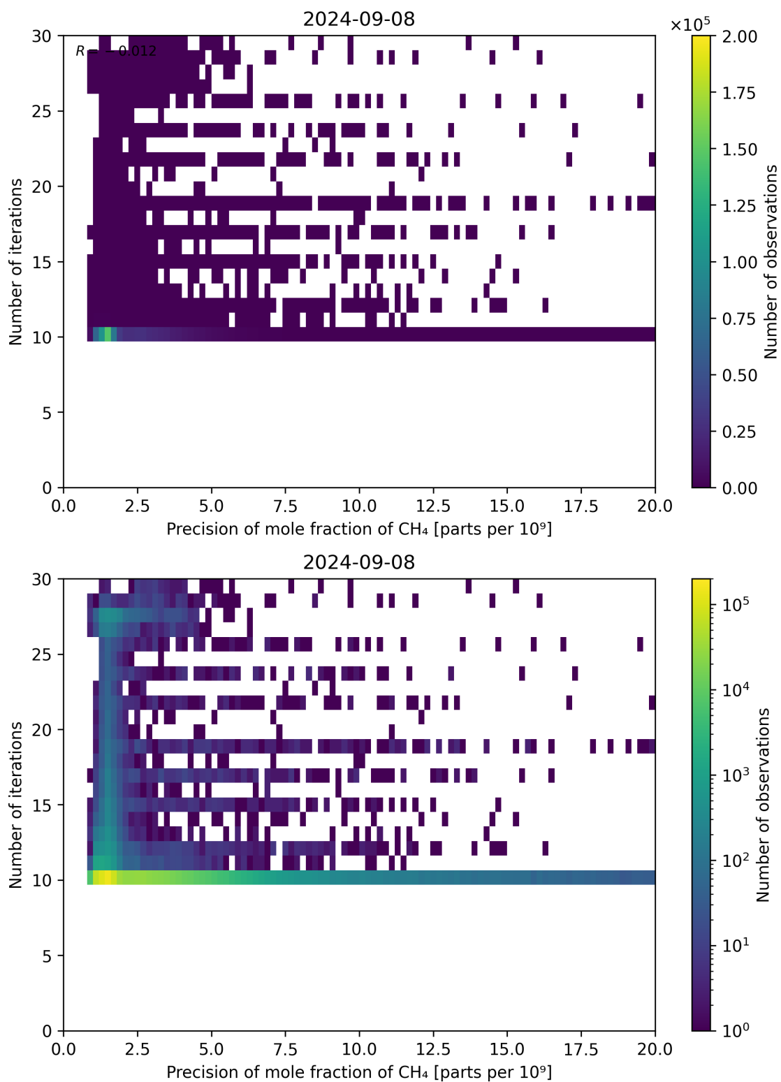
Figure 83: Scatter density plot of “Precision of mole fraction of CH 4 ” against “Number of iterations” for 2024-09-07 to 2024-09-09.
