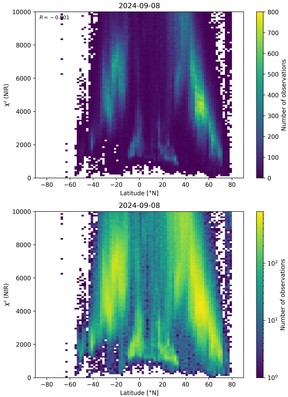
Figure 53: Scatter density plot of “Latitude” against “ \chi^2 (NIR)” for 2024-09-07 to 2024-09-09.
