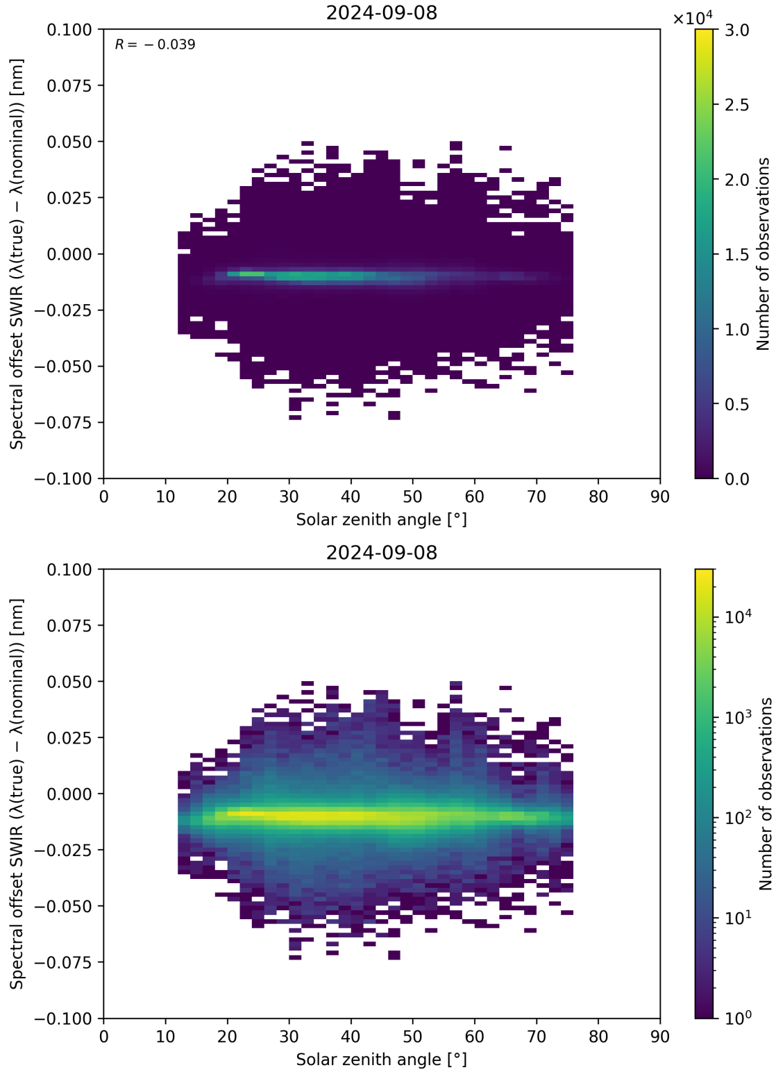
Figure 104: Scatter density plot of “Solar zenith angle” against “Spectral offset SWIR ( \lambda_{\text{true}} - \lambda_{\text{nominal}} )” for 2024-09-07 to 2024-09-09.
