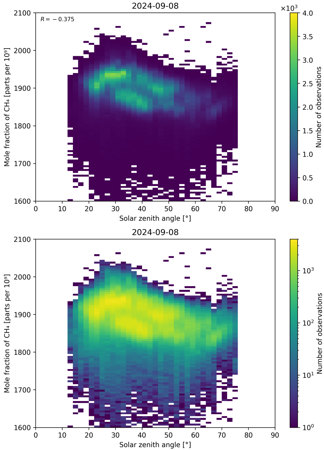
Figure 99: Scatter density plot of “Solar zenith angle” against “Mole fraction of \text{CH}_4 ” for 2024-09-07 to 2024-09-09.
