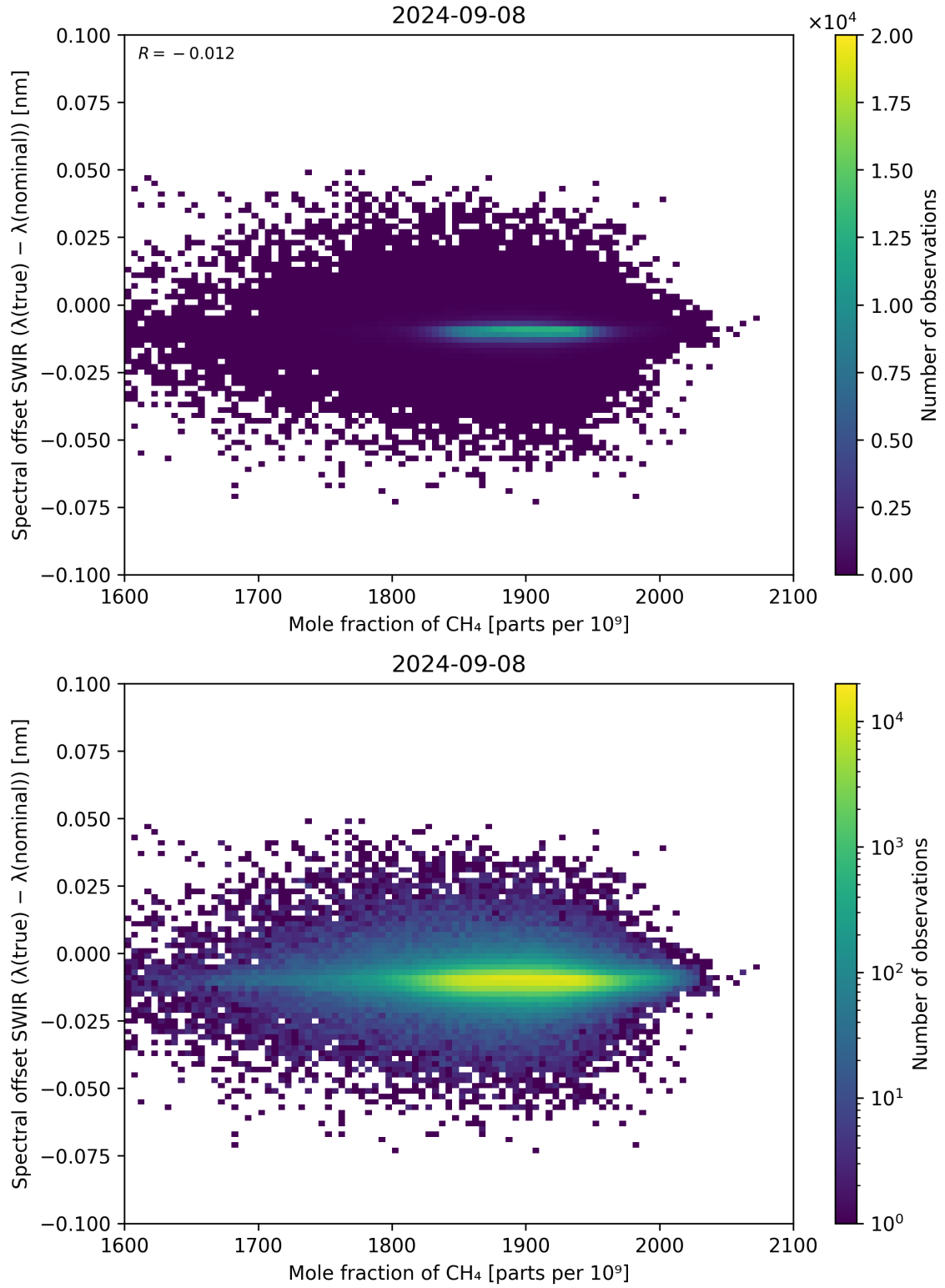
Figure 86: Scatter density plot of “Mole fraction of \text{CH}_4 ” against “Spectral offset SWIR ( \lambda_{\text{true}} - \lambda_{\text{nominal}} )” for 2024-09-07 to 2024-09-09.
