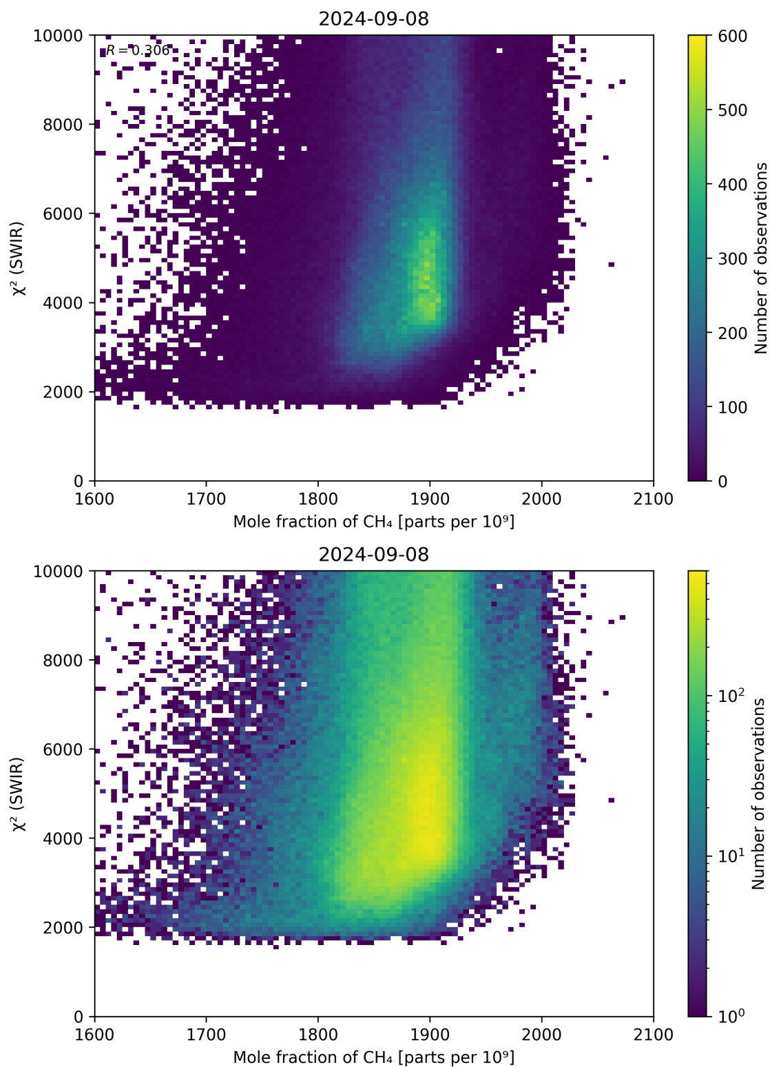
Figure 71: Scatter density plot of “Mole fraction of \text{CH}_4 ” against “ \chi^2 (SWIR)” for 2024-09-07 to 2024-09-09.
