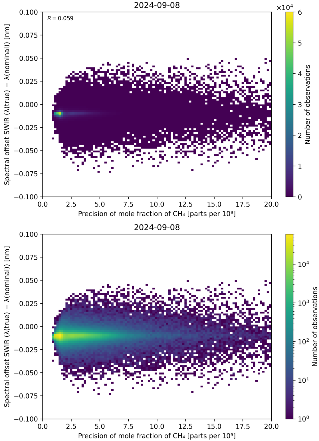
Figure 85: Scatter density plot of “Precision of mole fraction of \text{CH}_4 ” against “Spectral offset SWIR ( \lambda_{\text{true}} - \lambda_{\text{nominal}} )” for 2024-09-07 to 2024-09-09.
