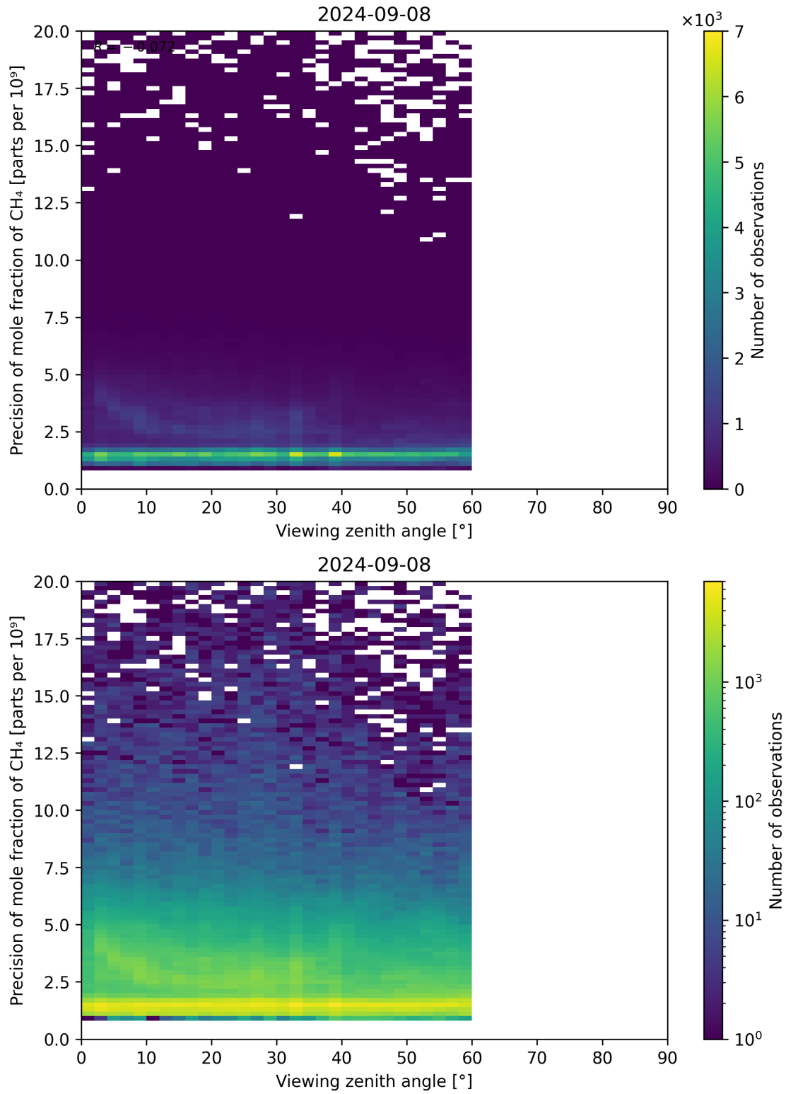
Figure 112: Scatter density plot of “Viewing zenith angle” against “Precision of mole fraction of CH 4 ” for 2024-09-07 to 2024-09-09.
