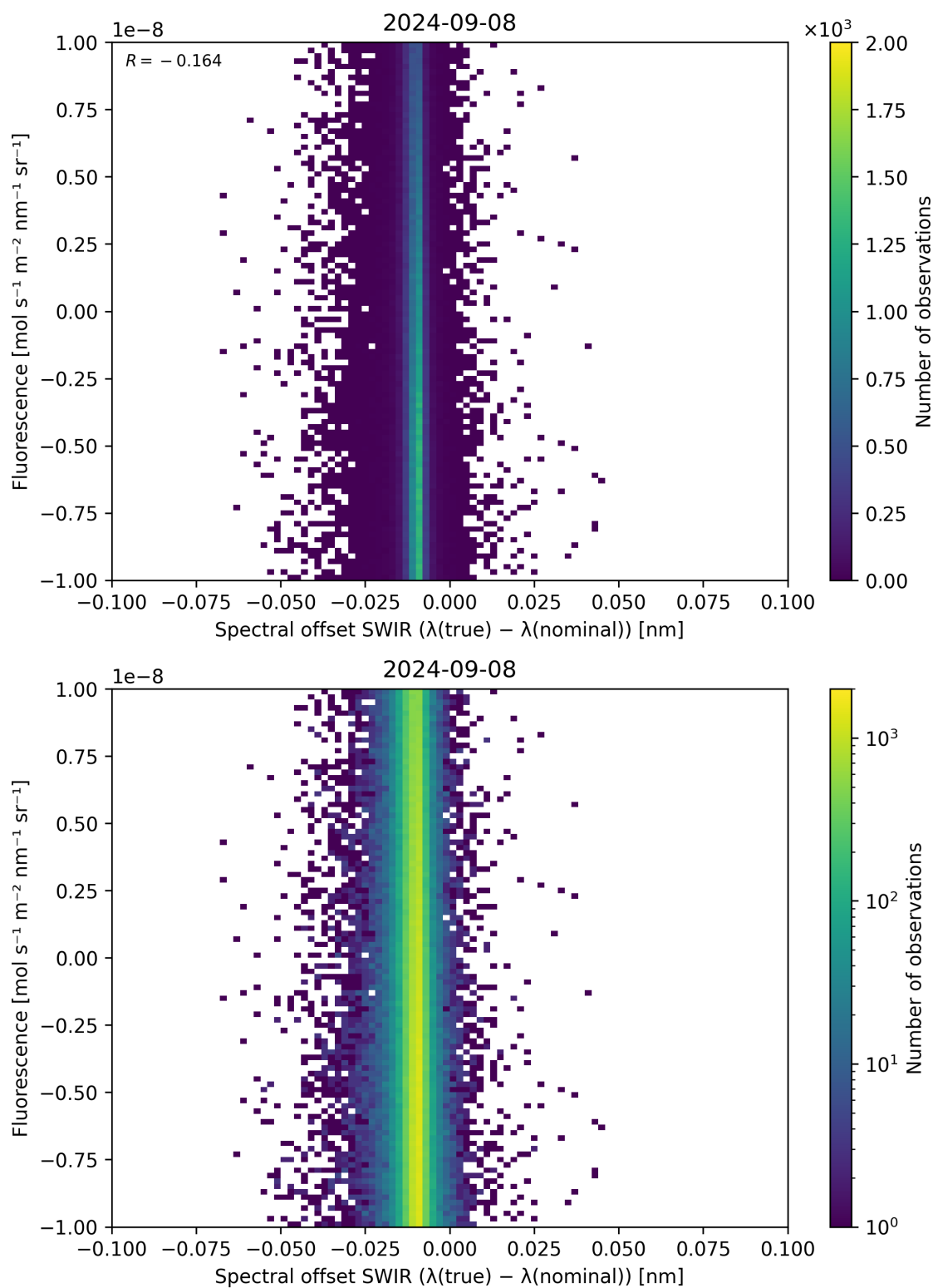
Figure 120: Scatter density plot of “Spectral offset SWIR ( \lambda_{\text{true}} - \lambda_{\text{nominal}} )” against “Fluorescence” for 2024-09-07 to 2024-09-09.
