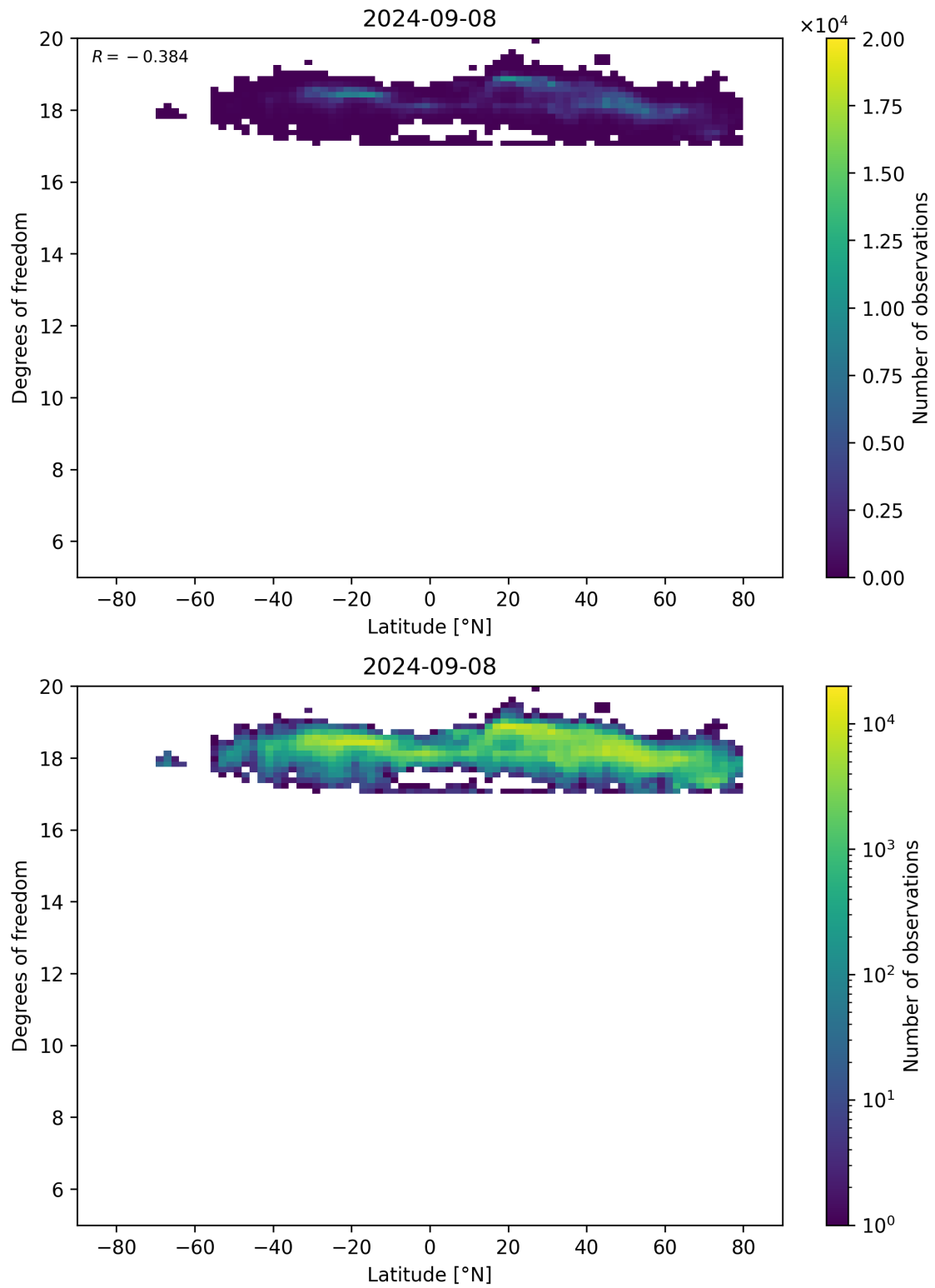
Figure 55: Scatter density plot of “Latitude” against “Degrees of freedom” for 2024-09-07 to 2024-09-09.
