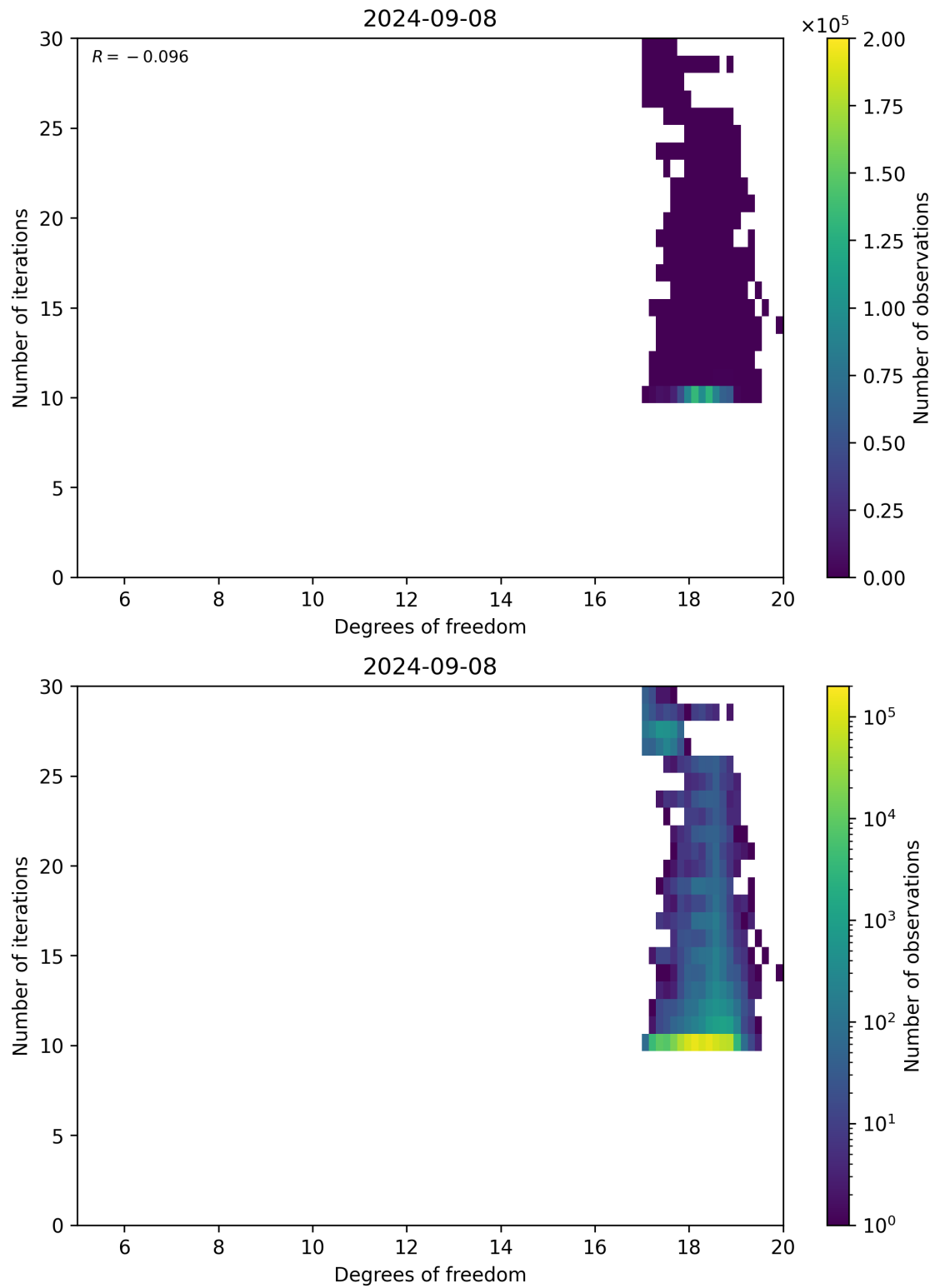
Figure 52: Scatter density plot of “Degrees of freedom” against “Number of iterations” for 2024-09-07 to 2024-09-09.
