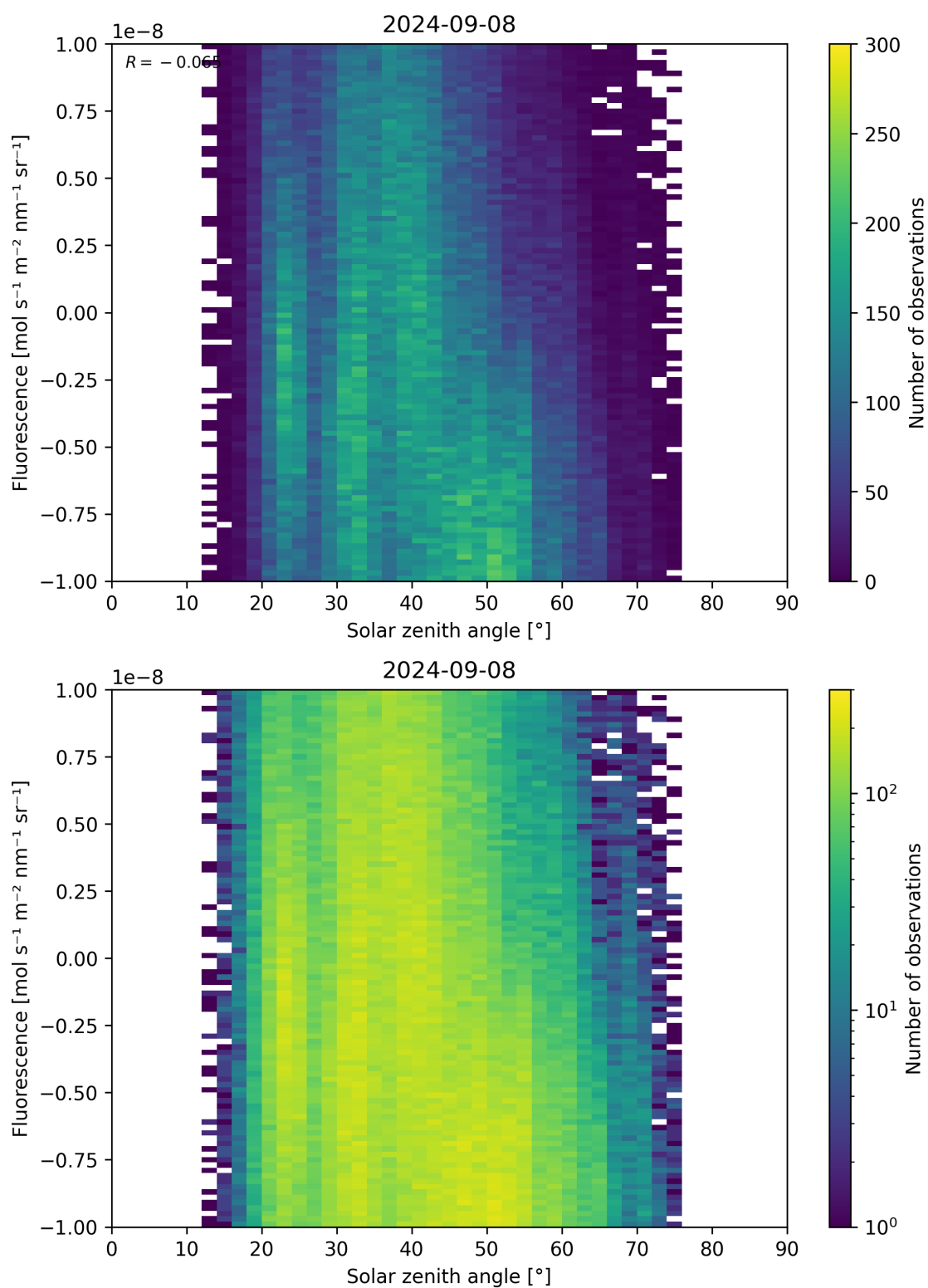
Figure 97: Scatter density plot of “Solar zenith angle” against “Fluorescence” for 2024-09-07 to 2024-09-09.
