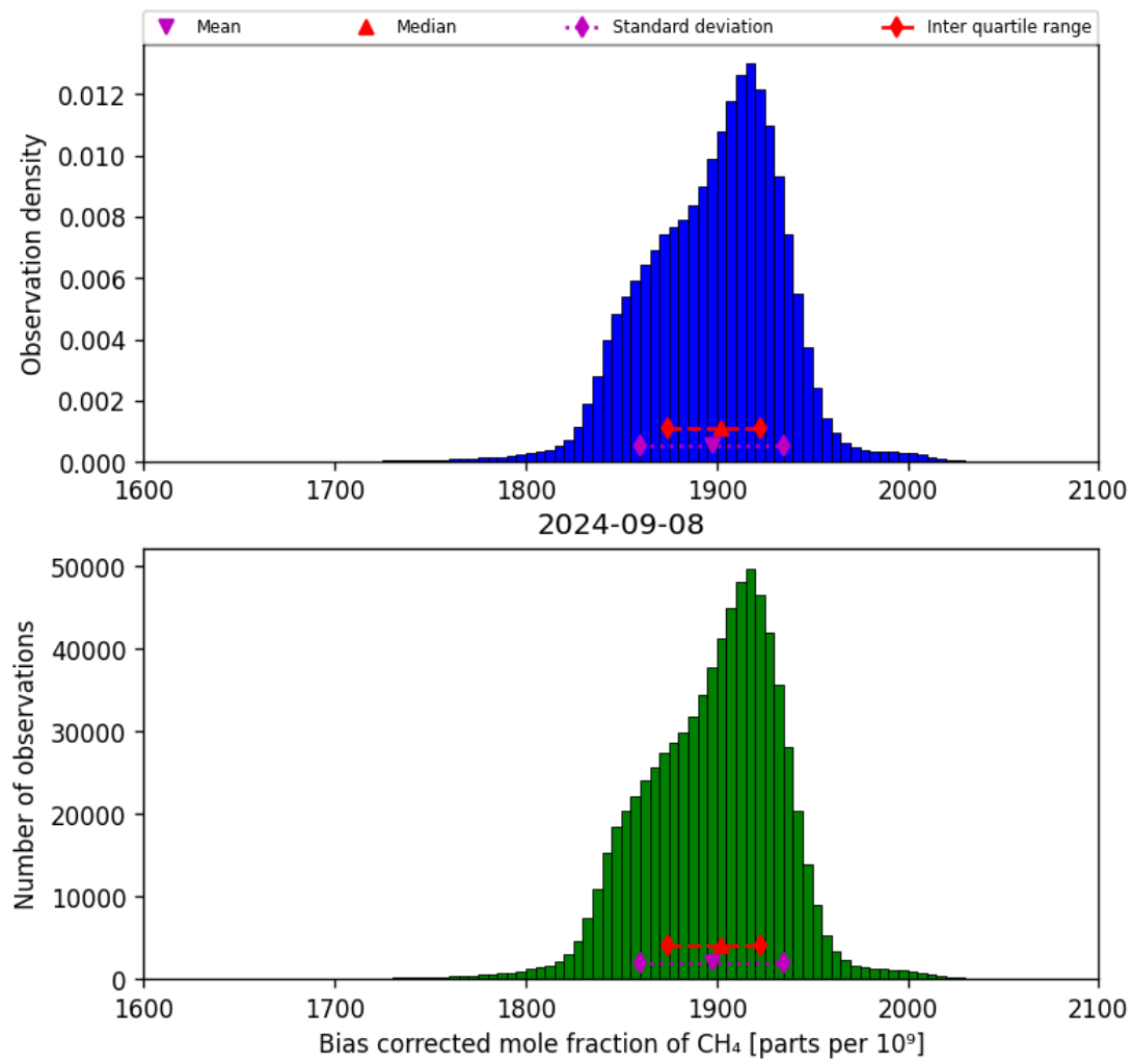
Figure 25: Histogram of “Bias corrected mole fraction of CH 4 ” for 2024-09-07 to 2024-09-09
