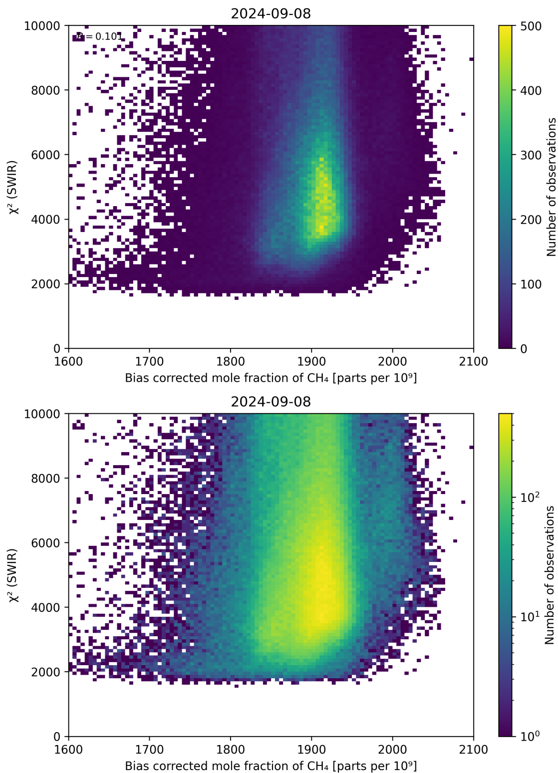
Figure 64: Scatter density plot of “Bias corrected mole fraction of \text{CH}_4 ” against “ \chi^2 (SWIR)” for 2024-09-07 to 2024-09-09.
