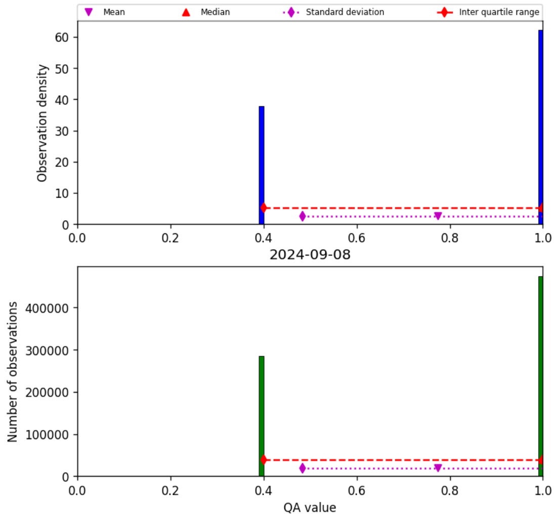
Figure 22: Histogram of “QA value” for 2024-09-07 to 2024-09-09
