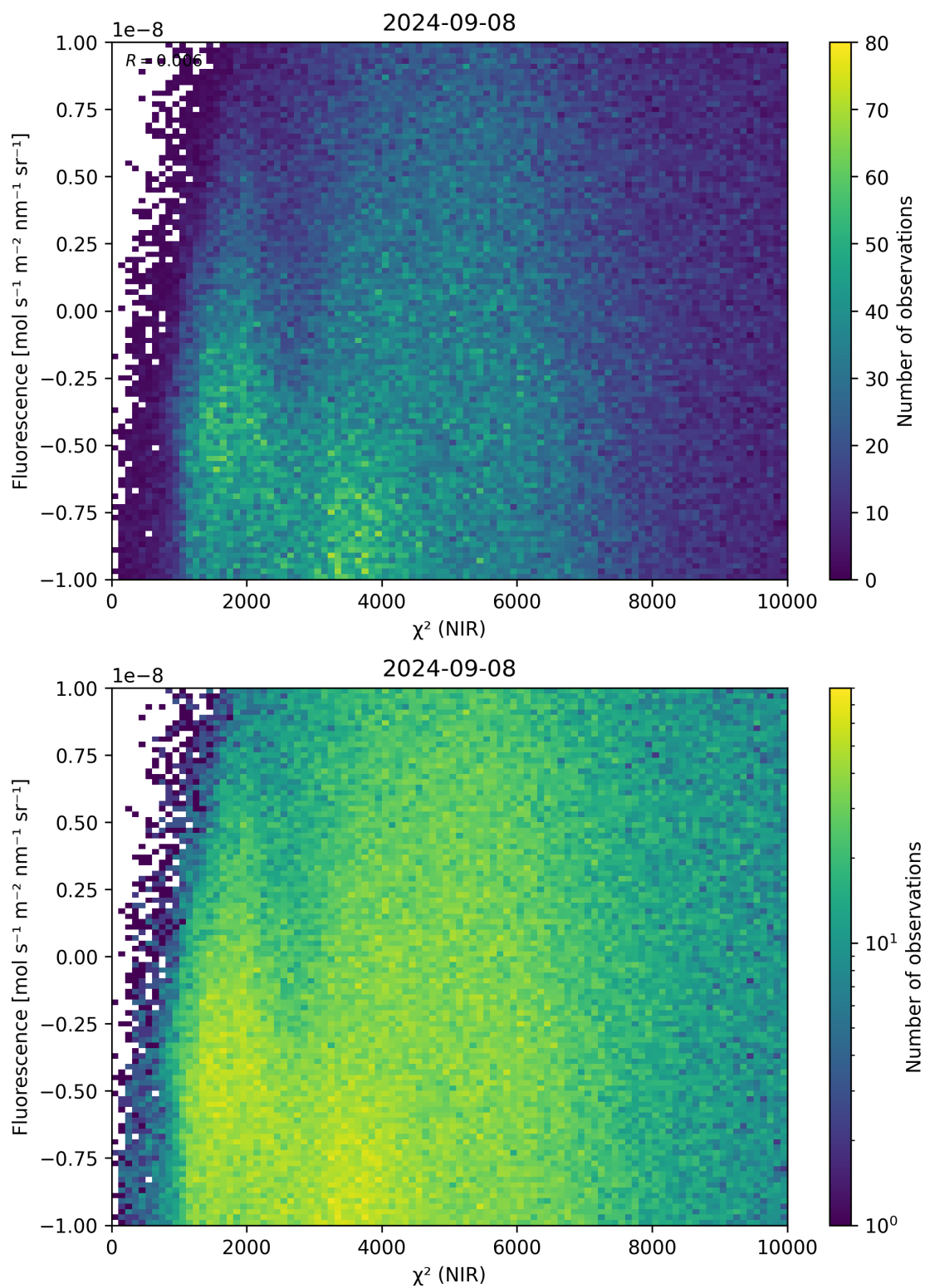
Figure 45: Scatter density plot of “ \chi^2 (NIR)” against “Fluorescence” for 2024-09-07 to 2024-09-09.
