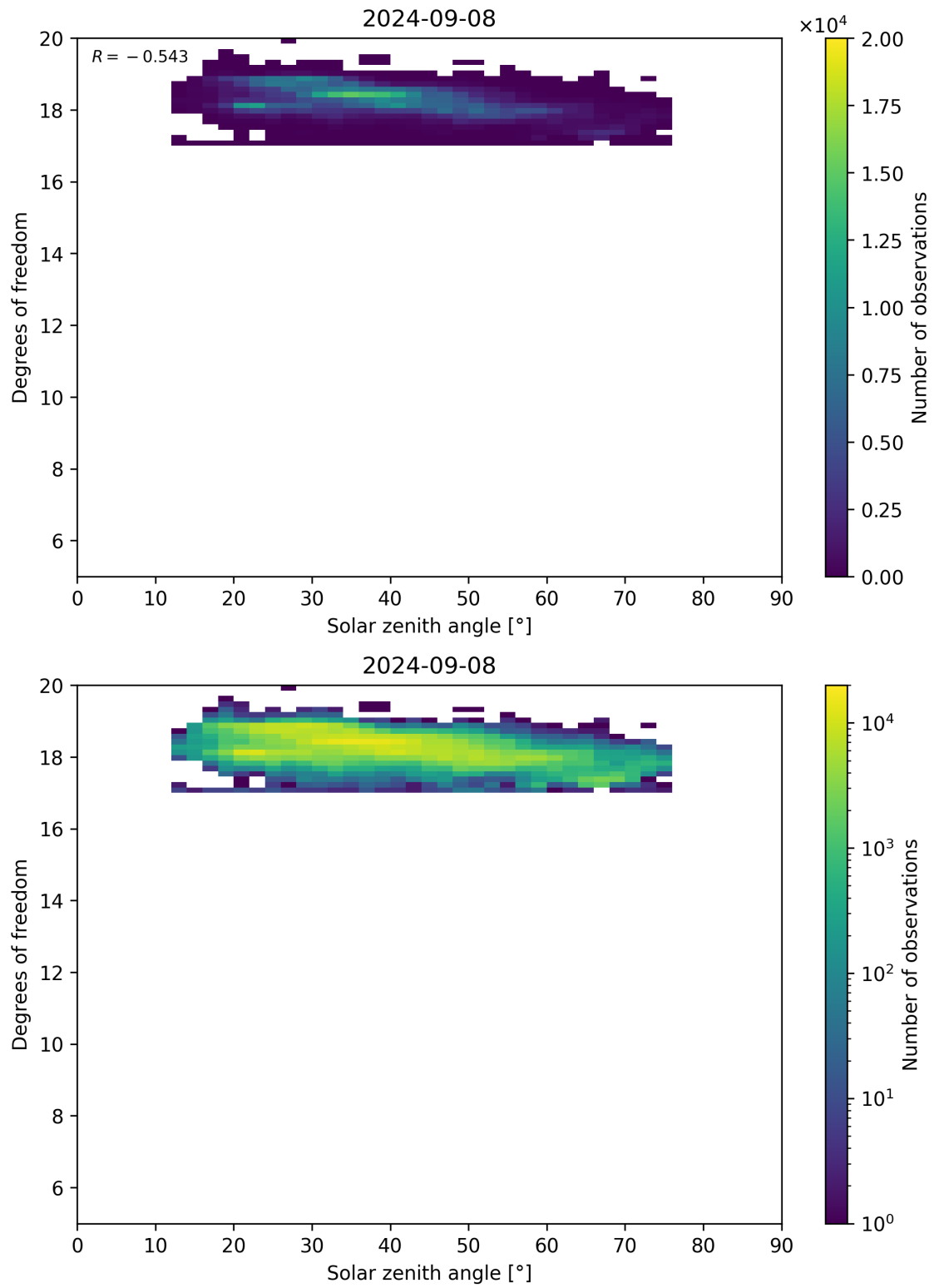
Figure 96: Scatter density plot of “Solar zenith angle” against “Degrees of freedom” for 2024-09-07 to 2024-09-09.
