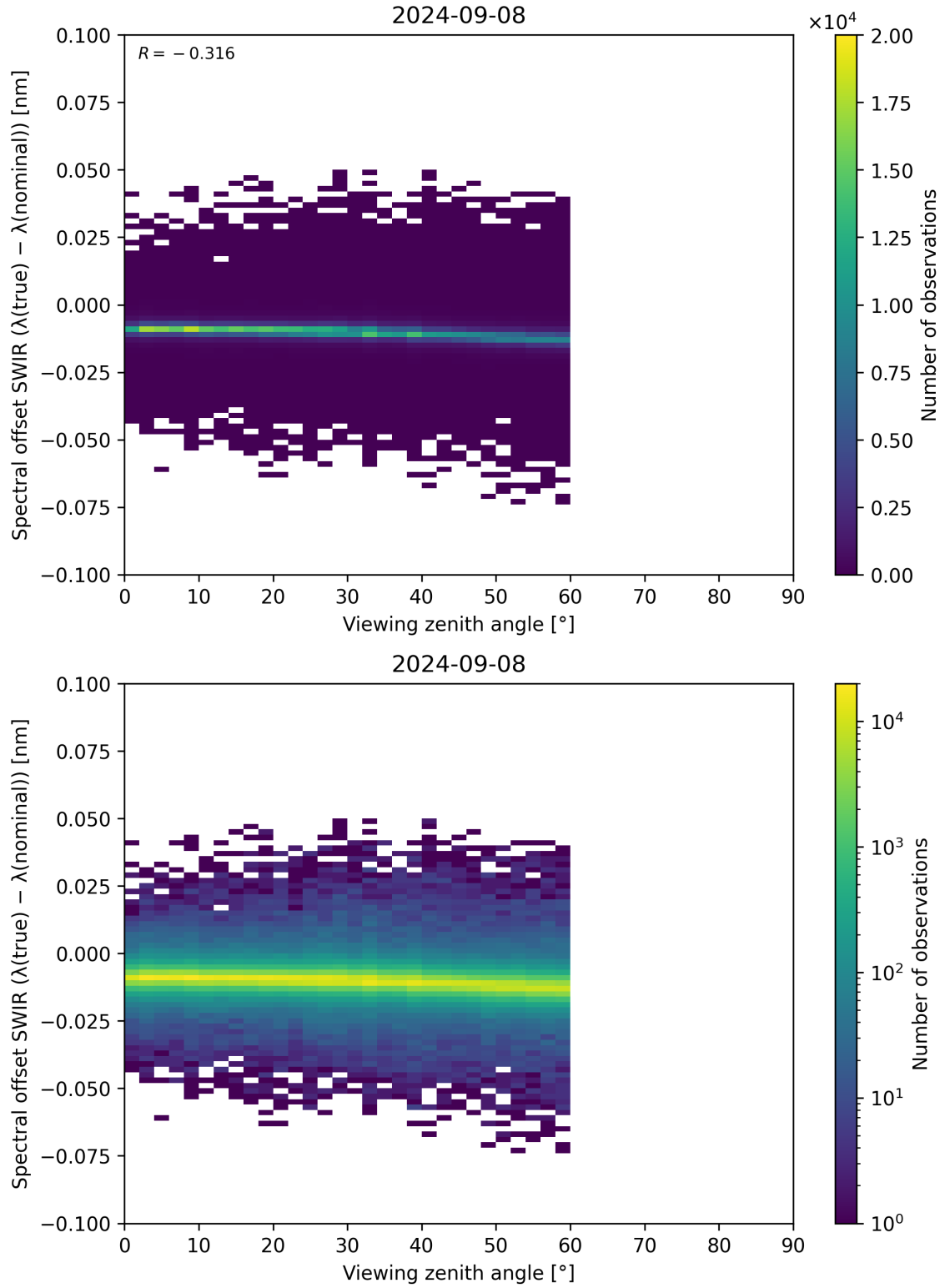
Figure 116: Scatter density plot of “Viewing zenith angle” against “Spectral offset SWIR ( \lambda_{\text{true}} - \lambda_{\text{nominal}} )” for 2024-09-07 to 2024-09-09.
