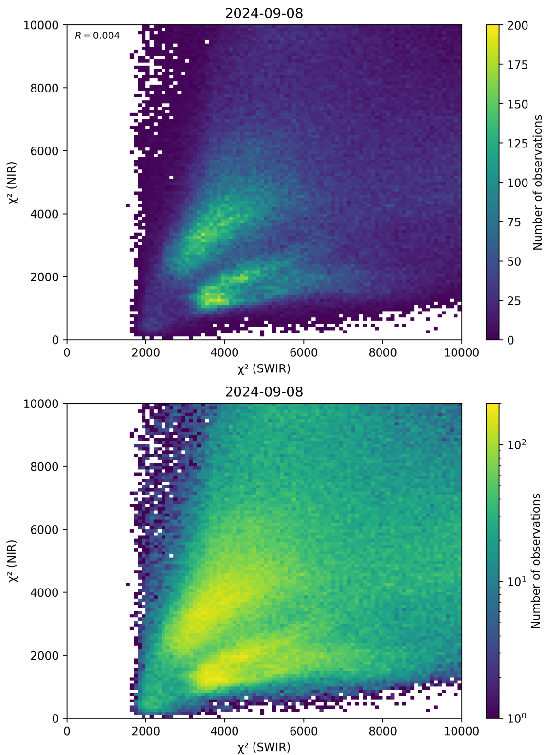
Figure 47: Scatter density plot of “ \chi^2 (SWIR)” against “ \chi^2 (NIR)” for 2024-09-07 to 2024-09-09.
