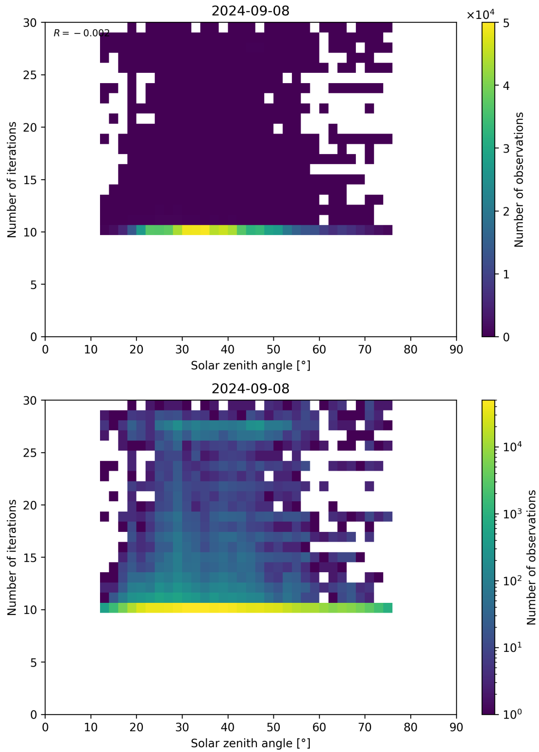
Figure 102: Scatter density plot of “Solar zenith angle” against “Number of iterations” for 2024-09-07 to 2024-09-09.
