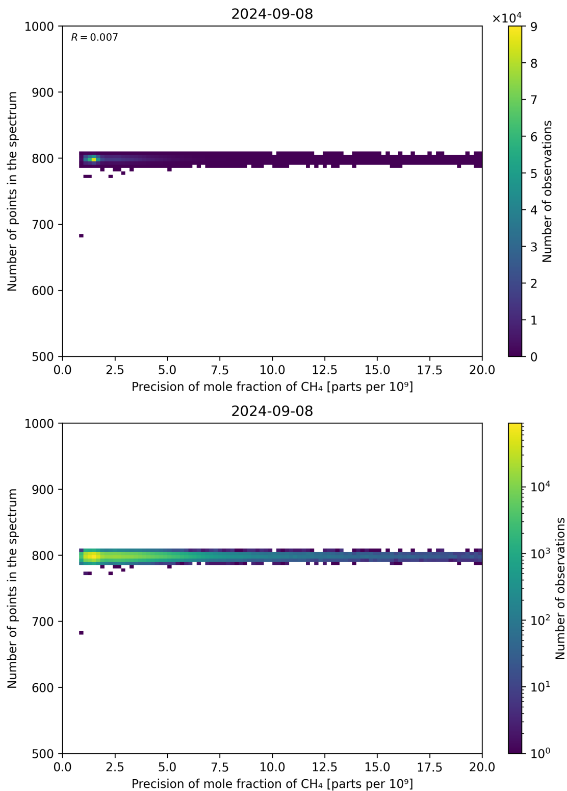
Figure 84: Scatter density plot of “Precision of mole fraction of CH 4 ” against “Number of points in the spectrum” for 2024-09-07 to 2024-09-09.
