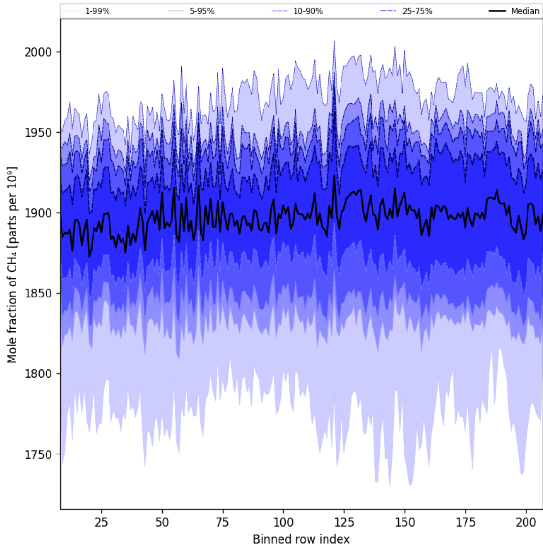
Figure 34: Along track statistics of “Mole fraction of CH 4 ” for 2024-09-07 to 2024-09-09
