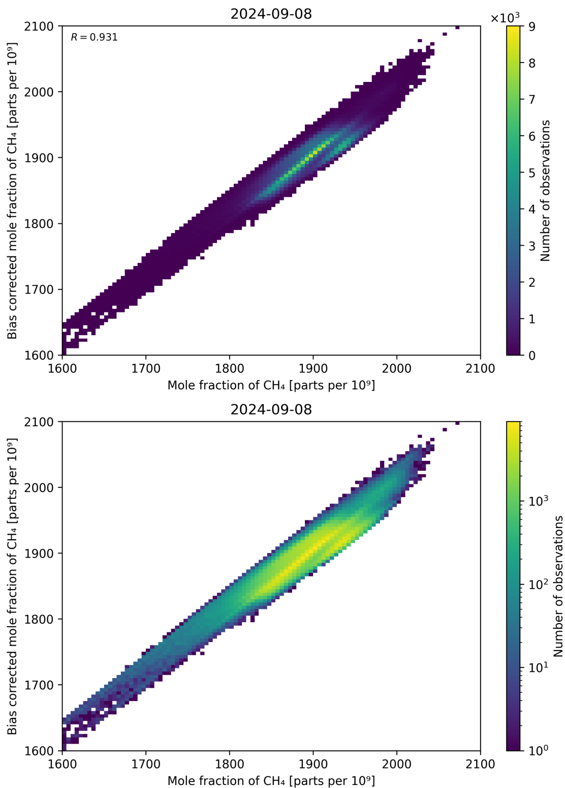
Figure 74: Scatter density plot of “Mole fraction of CH 4 ” against “Bias corrected mole fraction of CH 4 ” for 2024-09-07 to 2024-09-09.
