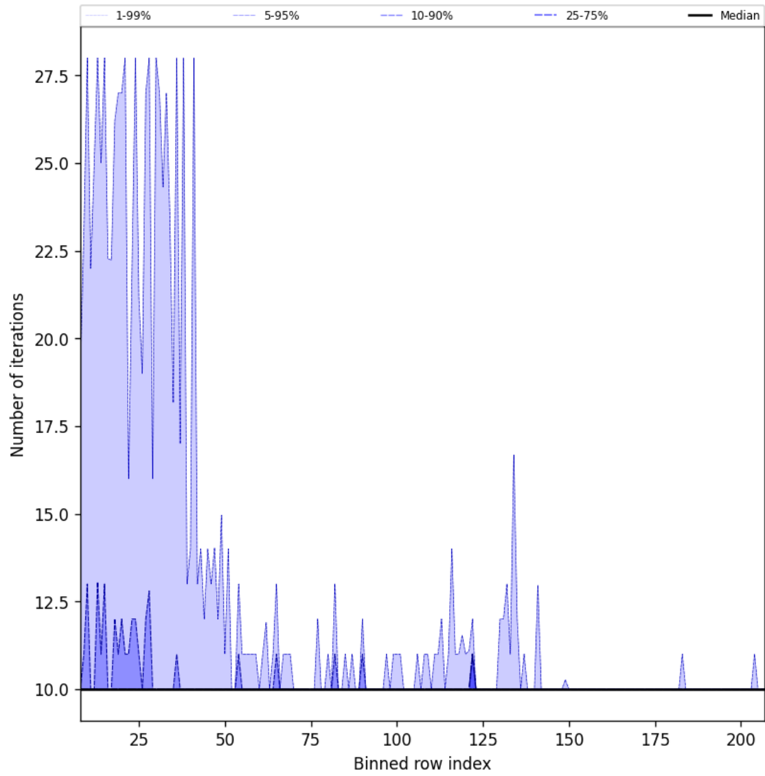
Figure 42: Along track statistics of “Number of iterations” for 2024-09-07 to 2024-09-09
