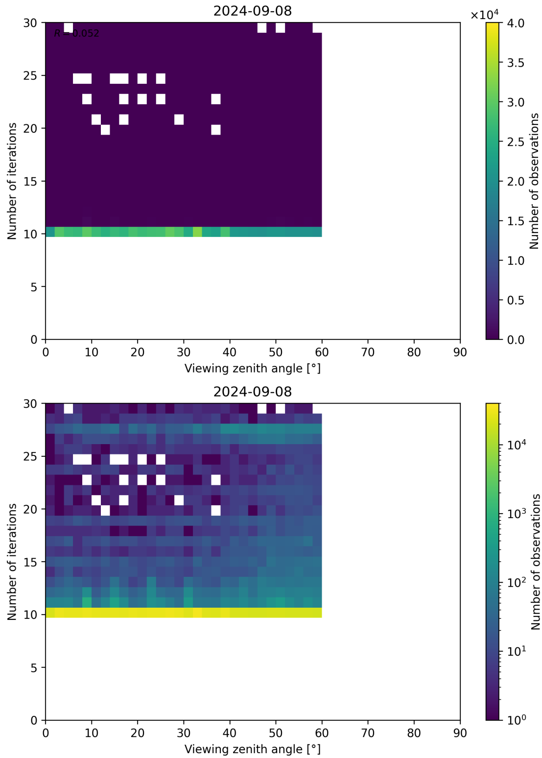
Figure 113: Scatter density plot of “Viewing zenith angle” against “Number of iterations” for 2024-09-07 to 2024-09-09.
