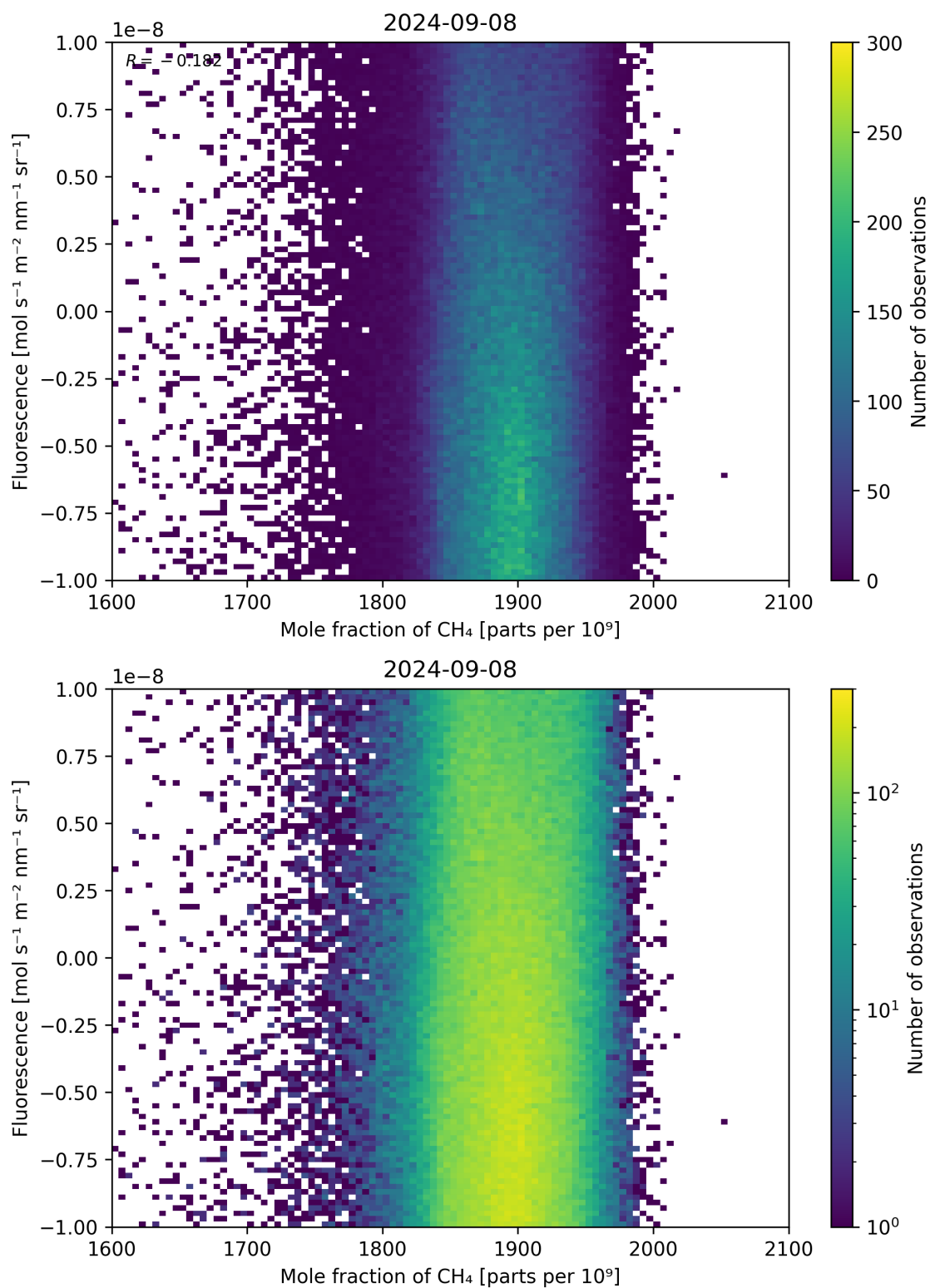
Figure 73: Scatter density plot of “Mole fraction of \text{CH}_4 ” against “Fluorescence” for 2024-09-07 to 2024-09-09.
