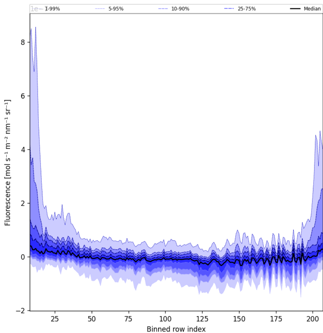
Figure 43: Along track statistics of “Fluorescence” for 2024-09-07 to 2024-09-09
