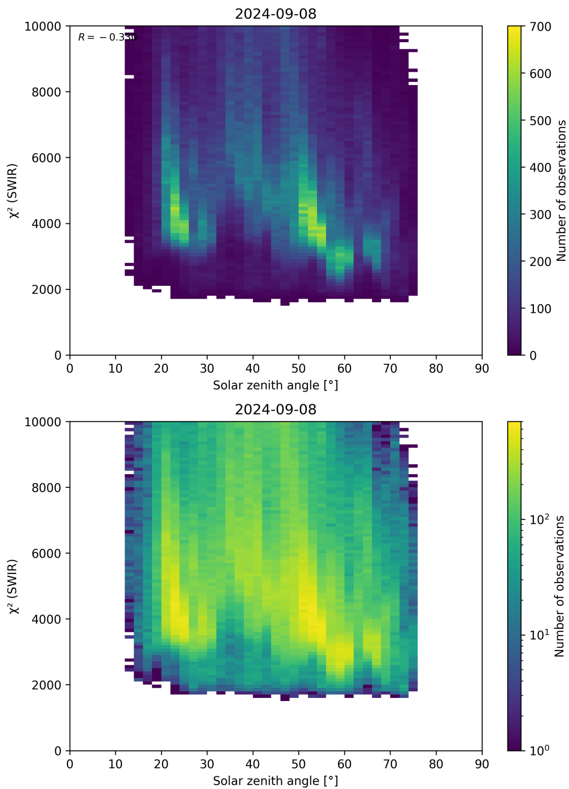
Figure 95: Scatter density plot of “Solar zenith angle” against “ \chi^2 (SWIR)” for 2024-09-07 to 2024-09-09.
