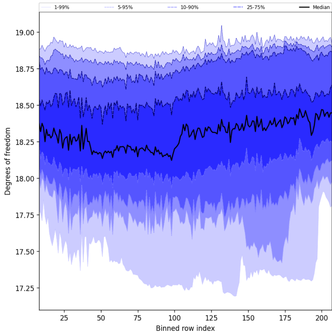
Figure 41: Along track statistics of “Degrees of freedom” for 2024-09-07 to 2024-09-09
