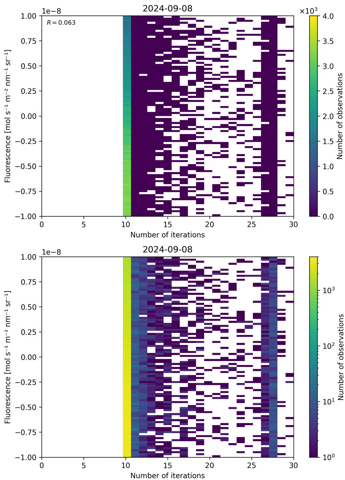
Figure 87: Scatter density plot of “Number of iterations” against “Fluorescence” for 2024-09-07 to 2024-09-09.
