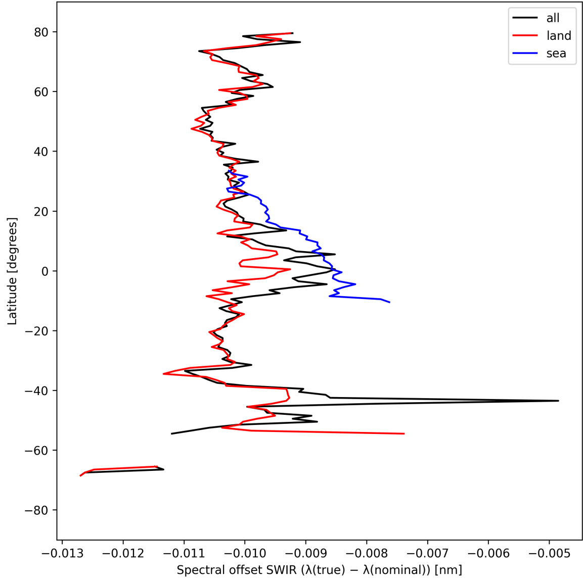
Figure 16: Zonal average of “Spectral offset SWIR ( \lambda_{\text{true}} - \lambda_{\text{nominal}} )” for 2024-09-07 to 2024-09-09.
