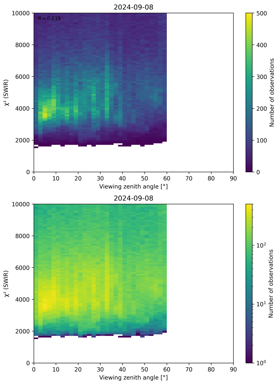
Figure 106: Scatter density plot of “Viewing zenith angle” against “ \chi^2 (SWIR)” for 2024-09-07 to 2024-09-09.
