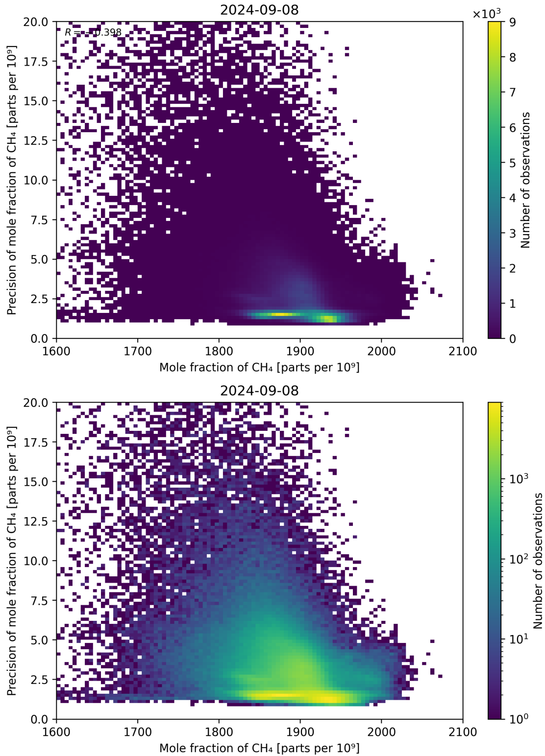
Figure 75: Scatter density plot of “Mole fraction of CH 4 ” against “Precision of mole fraction of CH 4 ” for 2024-09-07 to 2024-09-09.
