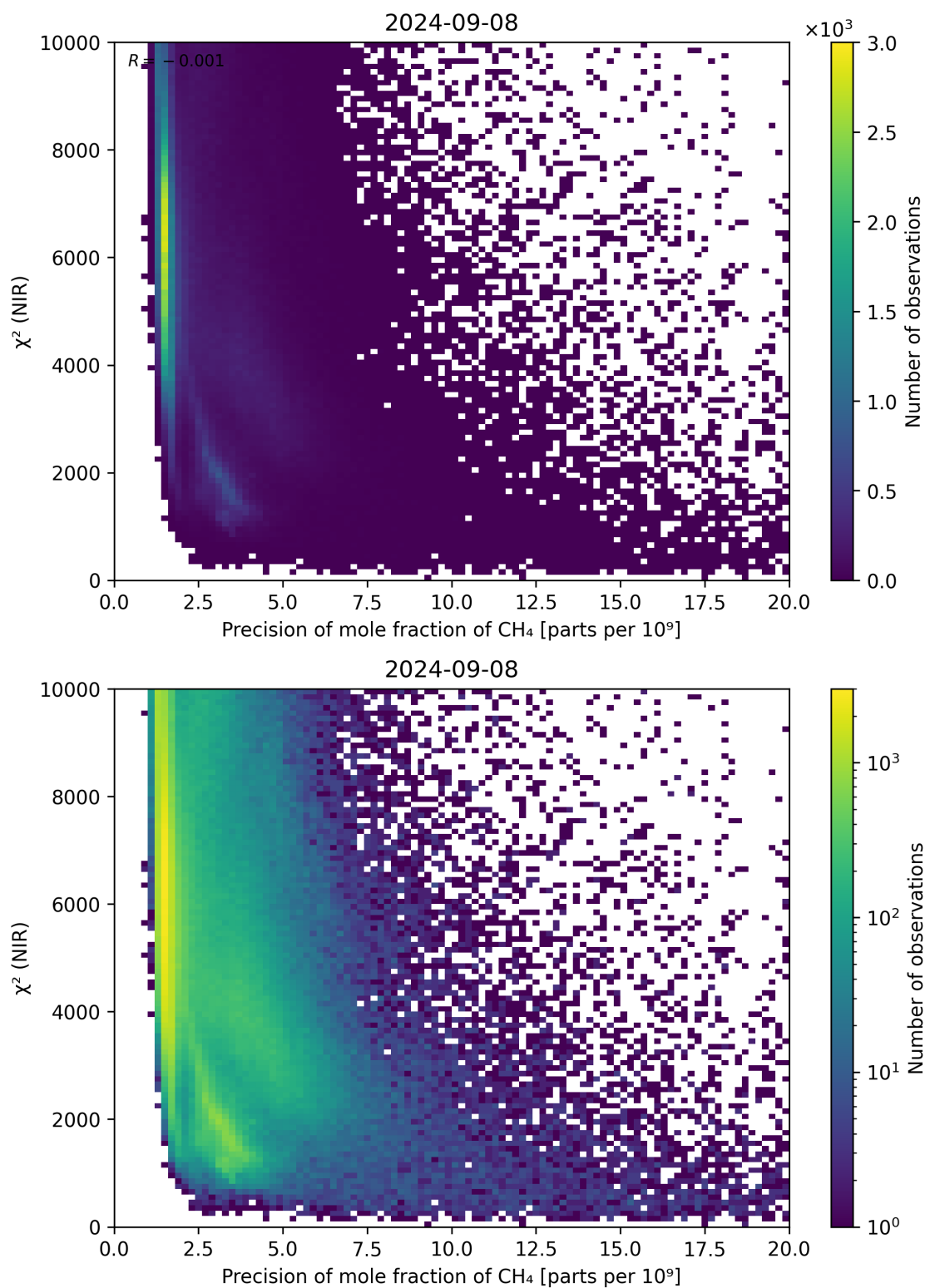
Figure 78: Scatter density plot of “Precision of mole fraction of CH 4 ” against “ \chi^2 (NIR)” for 2024-09-07 to 2024-09-09.
