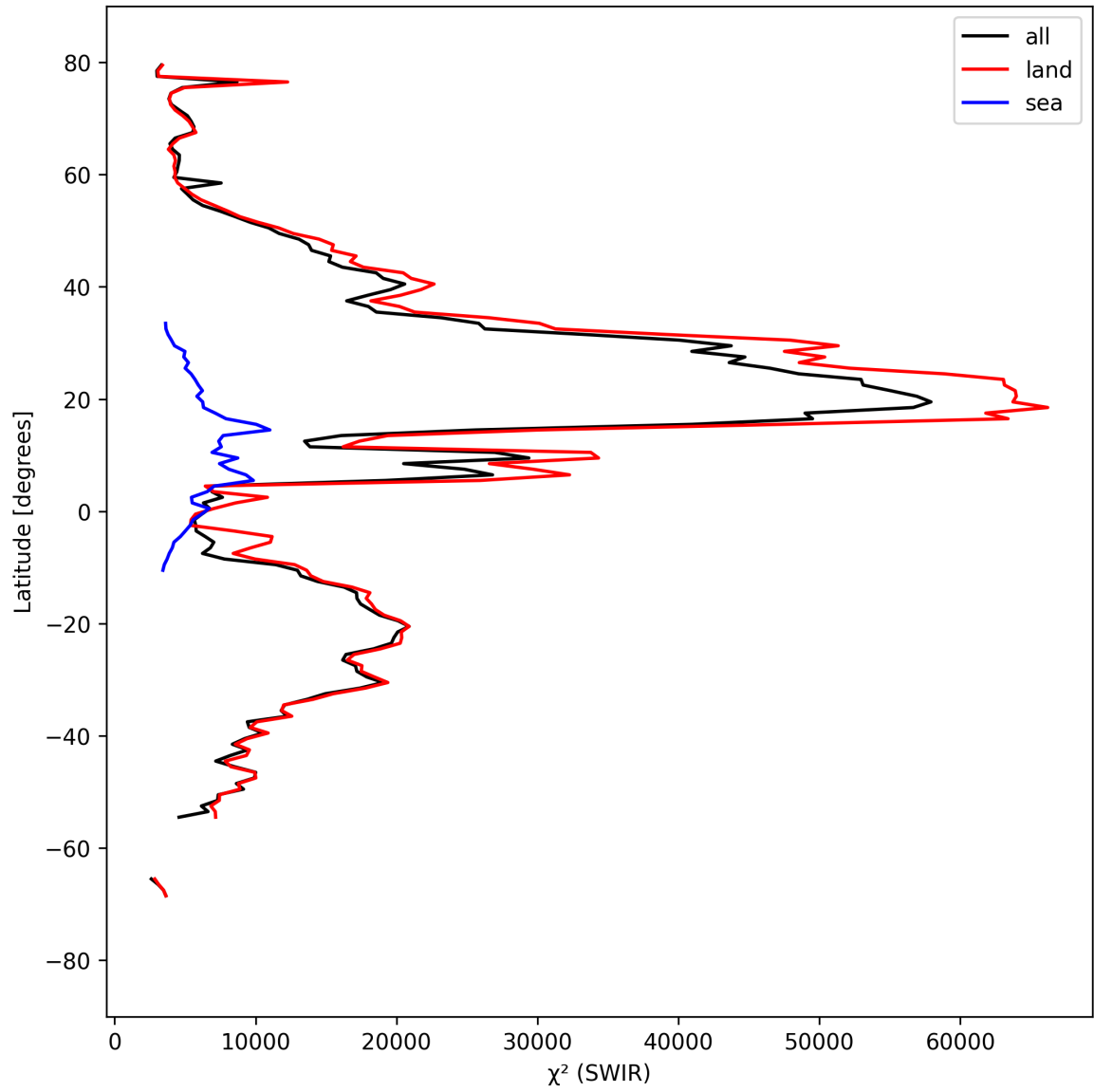
Figure 17: Zonal average of “ \chi^2 (SWIR)” for 2024-09-07 to 2024-09-09.
