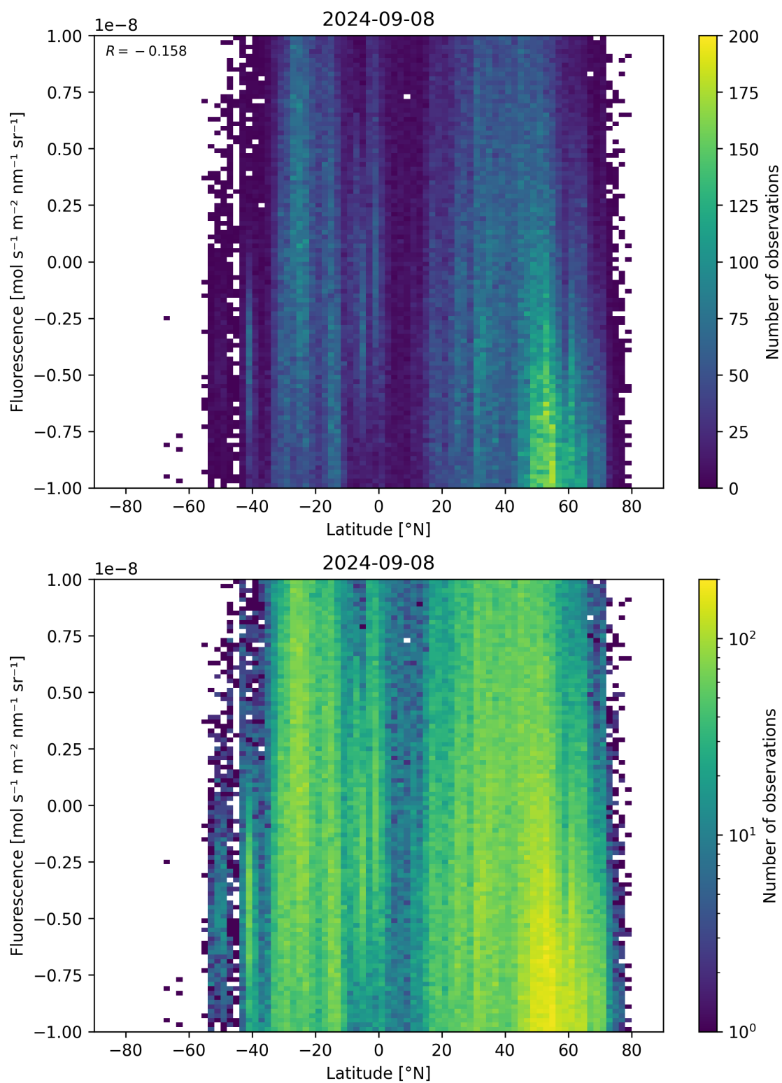
Figure 56: Scatter density plot of “Latitude” against “Fluorescence” for 2024-09-07 to 2024-09-09.
