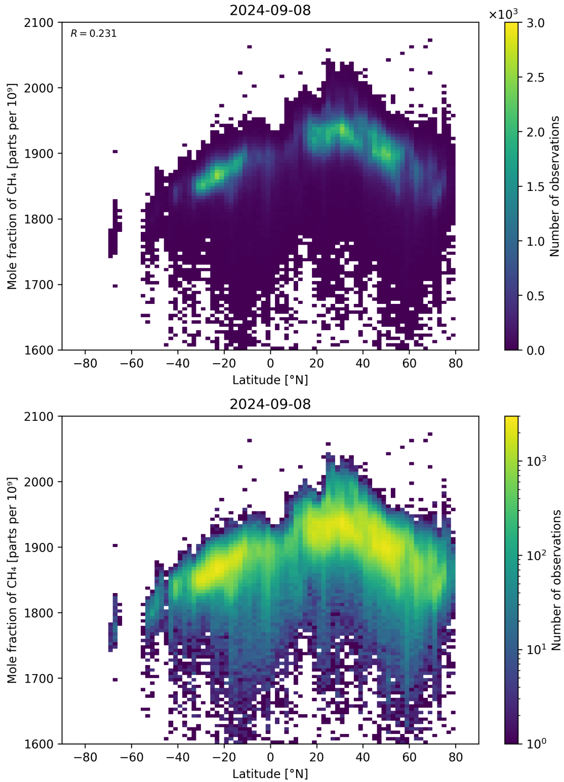
Figure 57: Scatter density plot of “Latitude” against “Mole fraction of CH 4 ” for 2024-09-07 to 2024-09-09.
