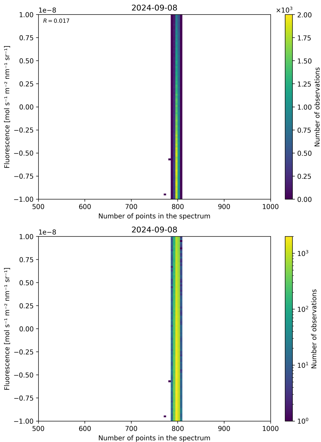
Figure 91: Scatter density plot of “Number of points in the spectrum” against “Fluorescence” for 2024-09-07 to 2024-09-09.
