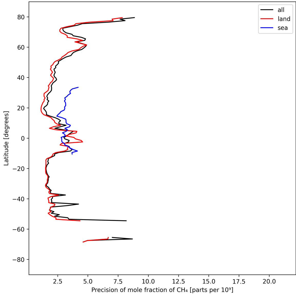
Figure 13: Zonal average of “Precision of mole fraction of \text{CH}_4 ” for 2024-09-07 to 2024-09-09.
