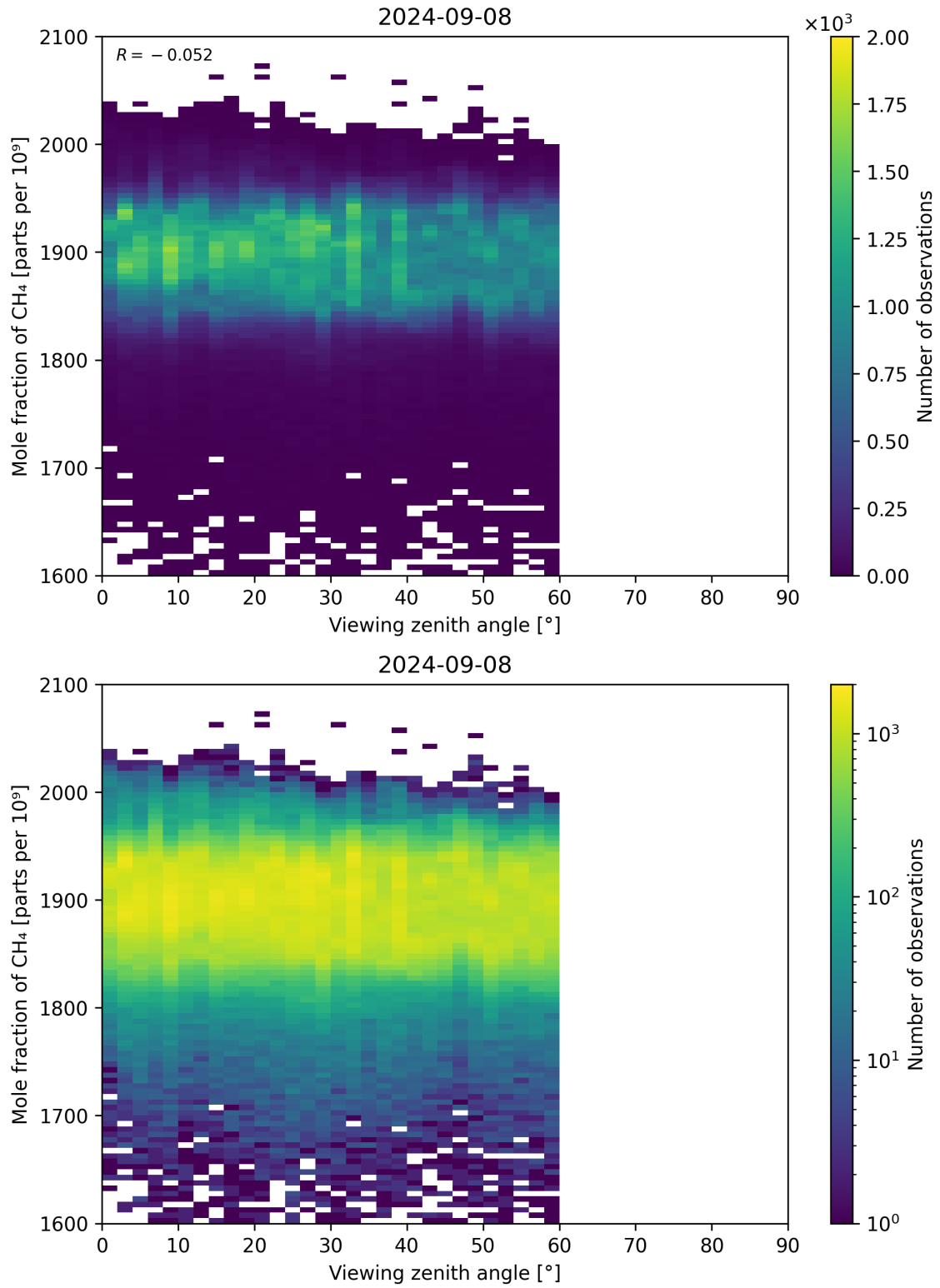
Figure 110: Scatter density plot of “Viewing zenith angle” against “Mole fraction of CH 4 ” for 2024-09-07 to 2024-09-09.
