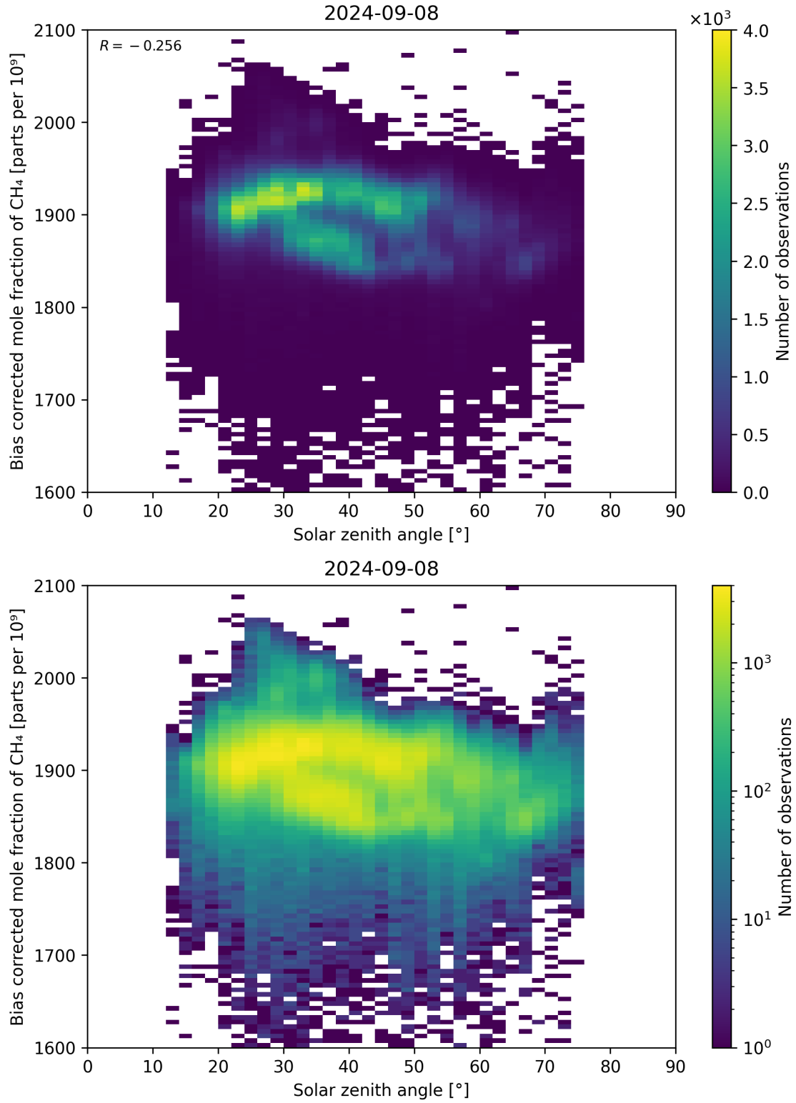
Figure 100: Scatter density plot of “Solar zenith angle” against “Bias corrected mole fraction of CH 4 ” for 2024-09-07 to 2024-09-09.
