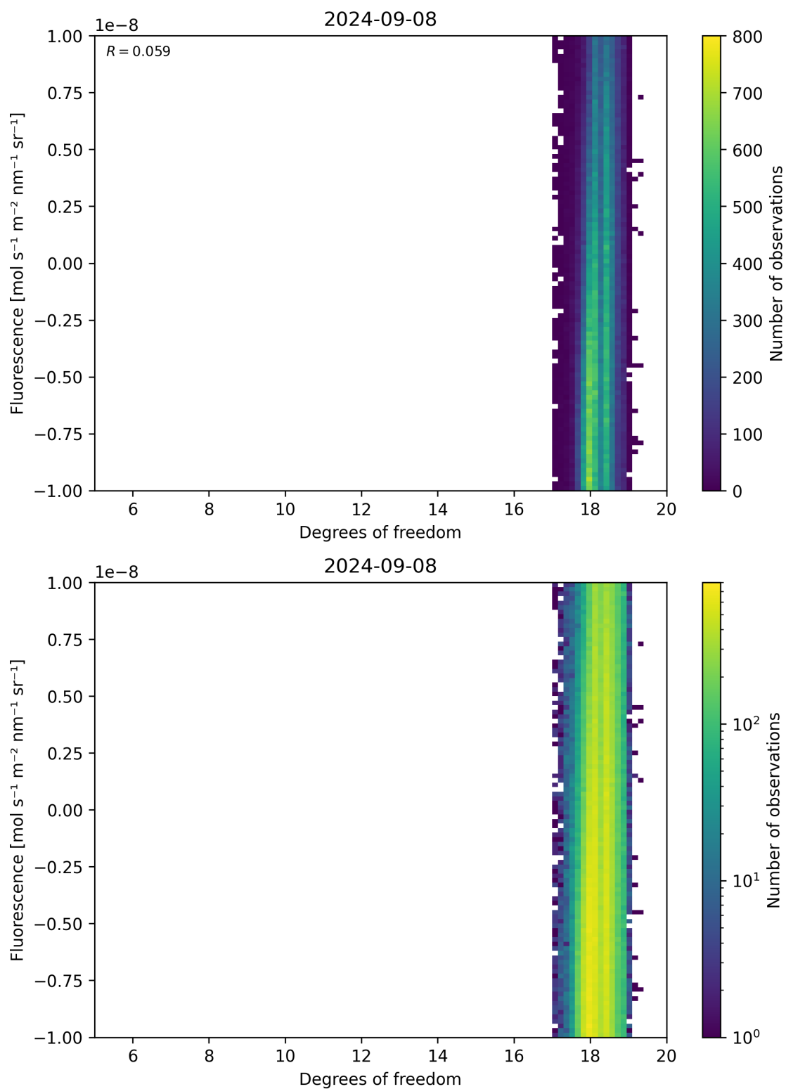
Figure 51: Scatter density plot of “Degrees of freedom” against “Fluorescence” for 2024-09-07 to 2024-09-09.
