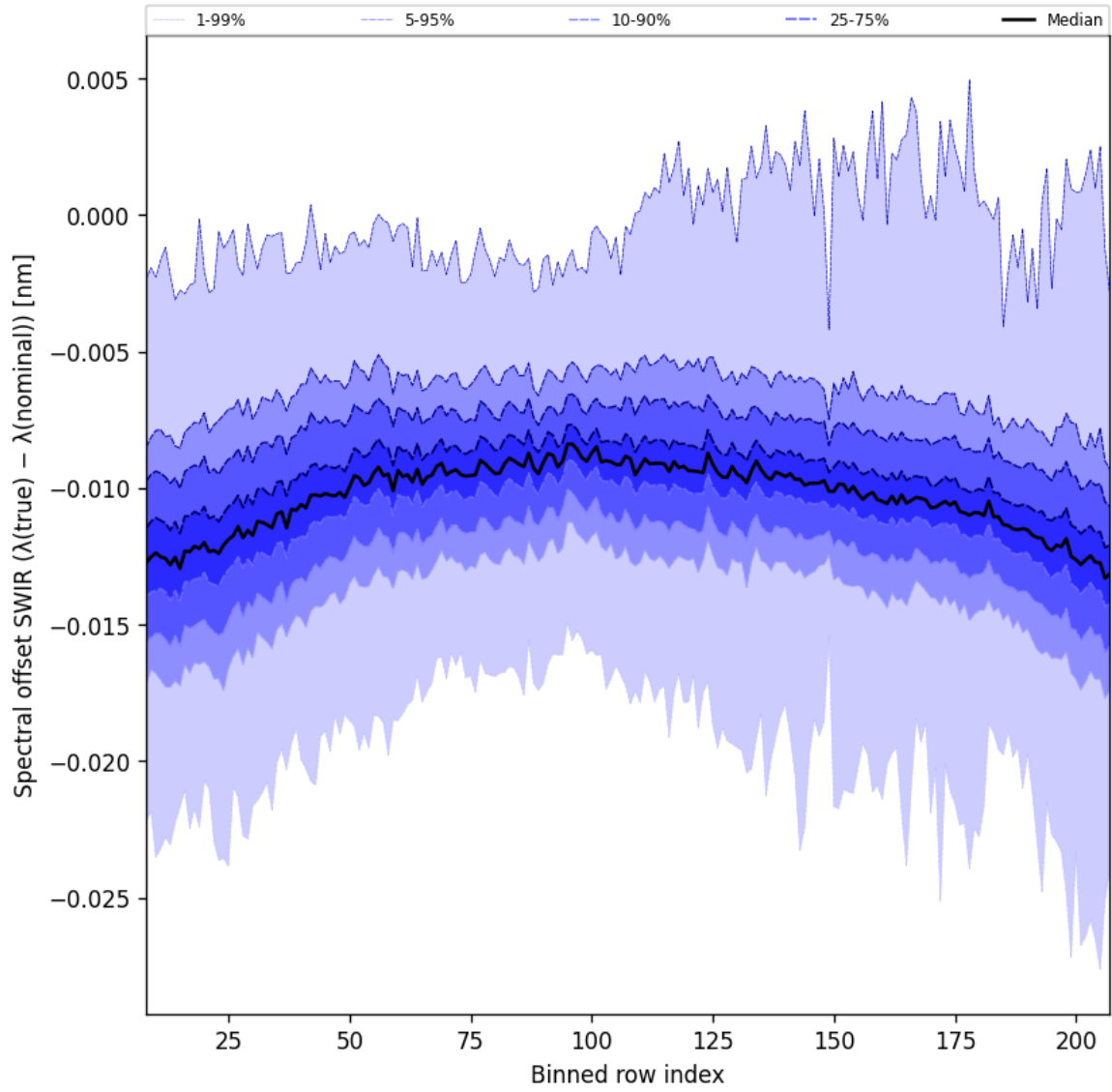
Figure 38: Along track statistics of “Spectral offset SWIR ( \lambda_{\text{true}} - \lambda_{\text{nominal}} )” for 2024-09-07 to 2024-09-09
