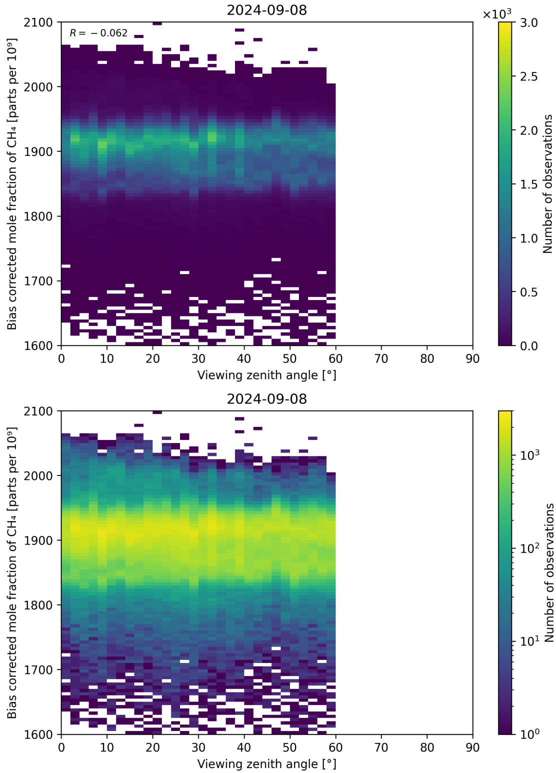
Figure 111: Scatter density plot of “Viewing zenith angle” against “Bias corrected mole fraction of CH 4 ” for 2024-09-07 to 2024-09-09.
