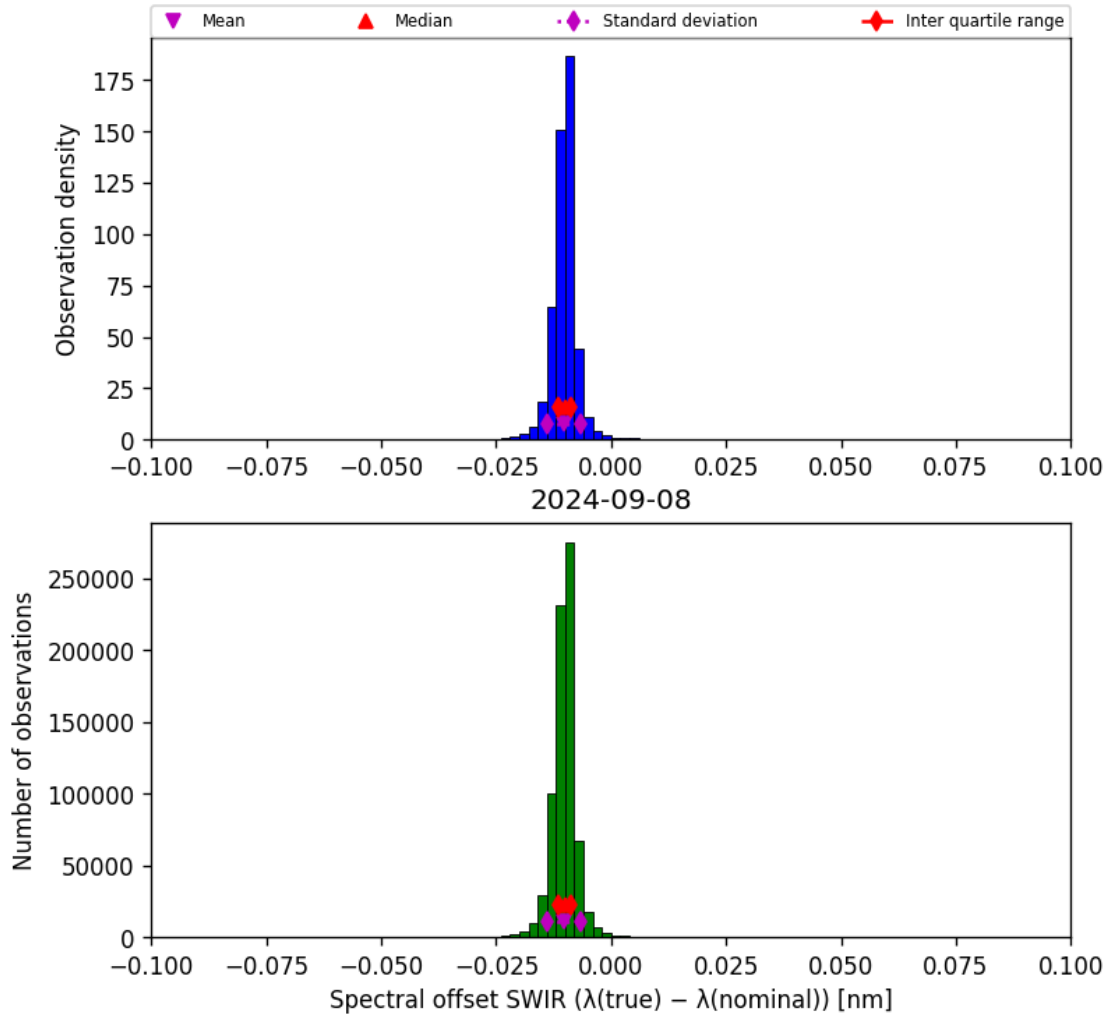
Figure 27: Histogram of “Spectral offset SWIR ( \lambda_{\text{true}} - \lambda_{\text{nominal}} )” for 2024-09-07 to 2024-09-09
