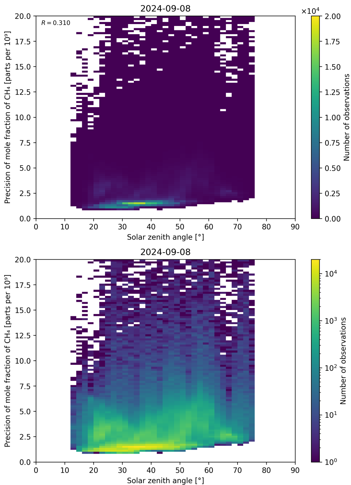
Figure 101: Scatter density plot of “Solar zenith angle” against “Precision of mole fraction of CH 4 ” for 2024-09-07 to 2024-09-09.
