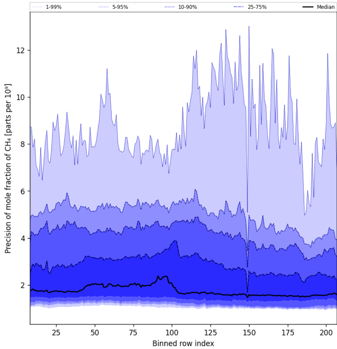
Figure 35: Along track statistics of “Precision of mole fraction of CH 4 ” for 2024-09-07 to 2024-09-09
