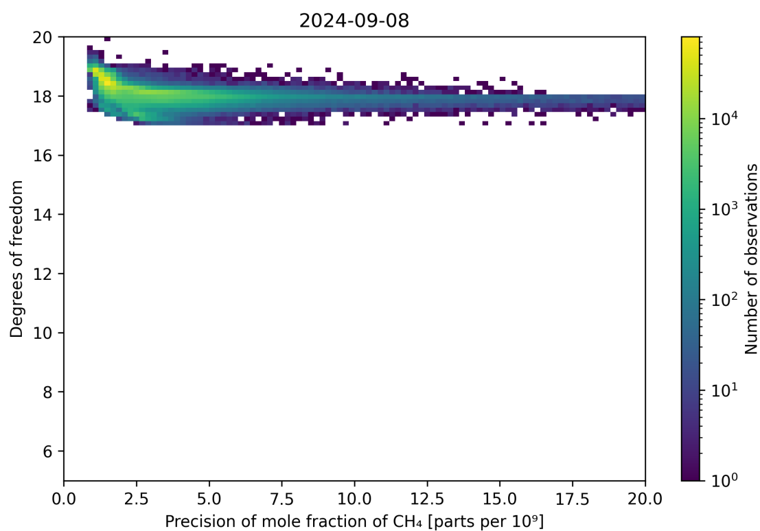
Figure 80: Scatter density plot of “Precision of mole fraction of CH 4 ” against “Degrees of freedom” for 2024-09-07 to 2024-09-09.
