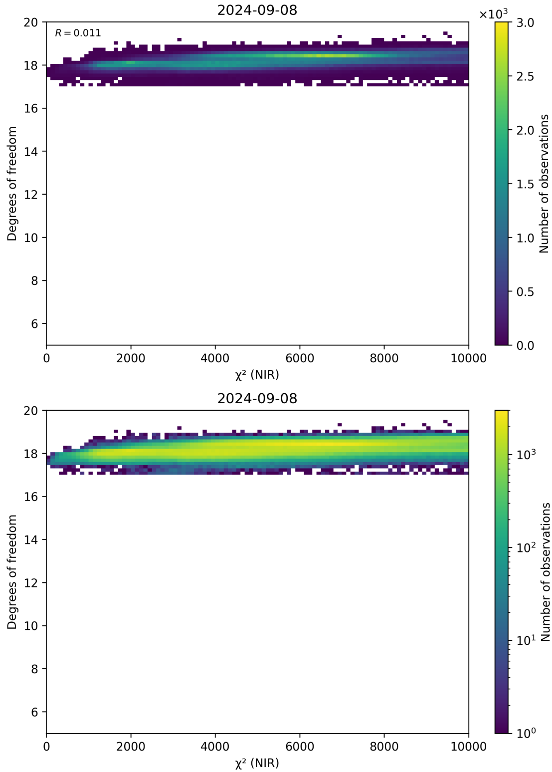
Figure 44: Scatter density plot of “ \chi^2 (NIR)” against “Degrees of freedom” for 2024-09-07 to 2024-09-09.
