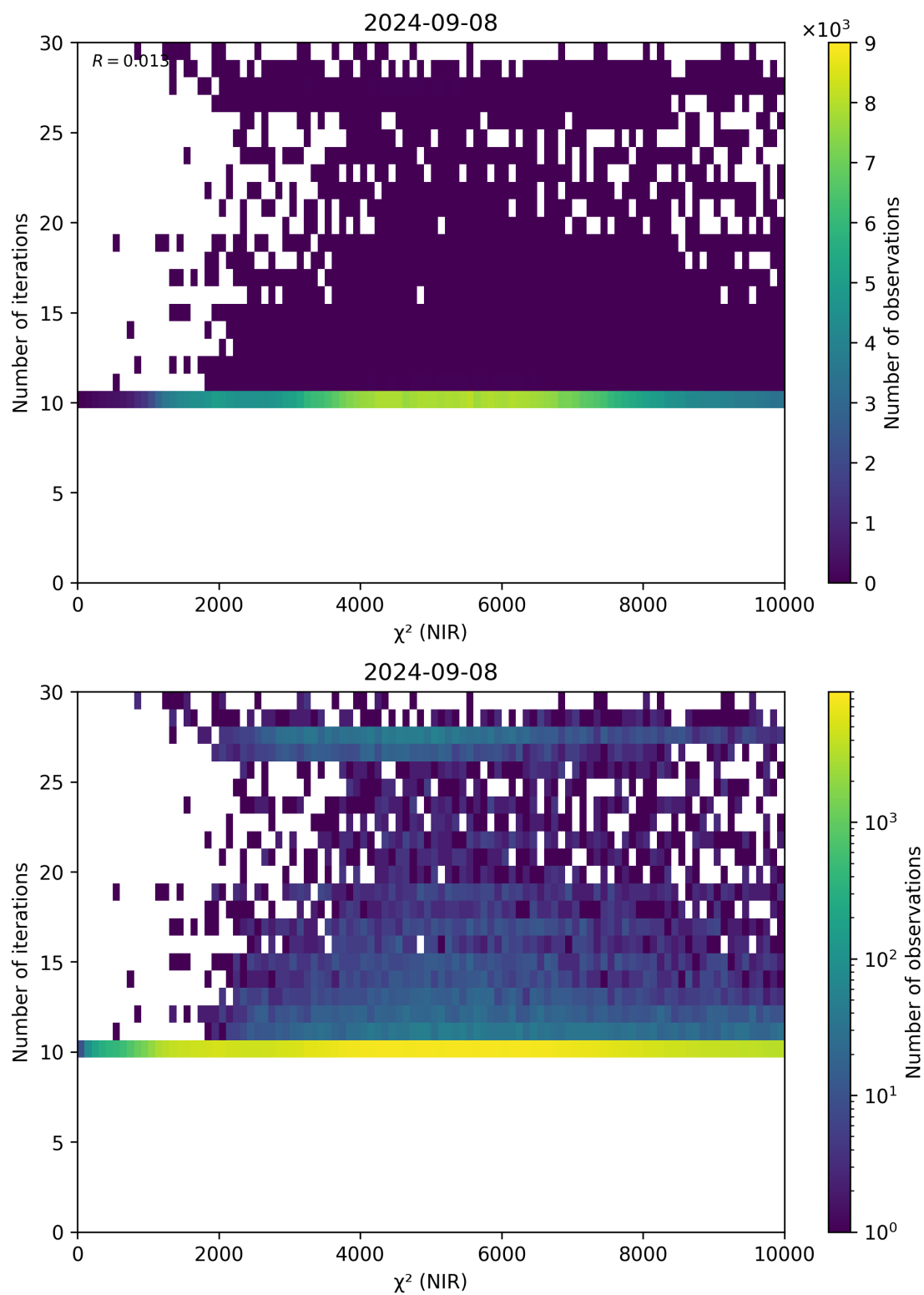
Figure 46: Scatter density plot of “ \chi^2 (NIR)” against “Number of iterations” for 2024-09-07 to 2024-09-09.
