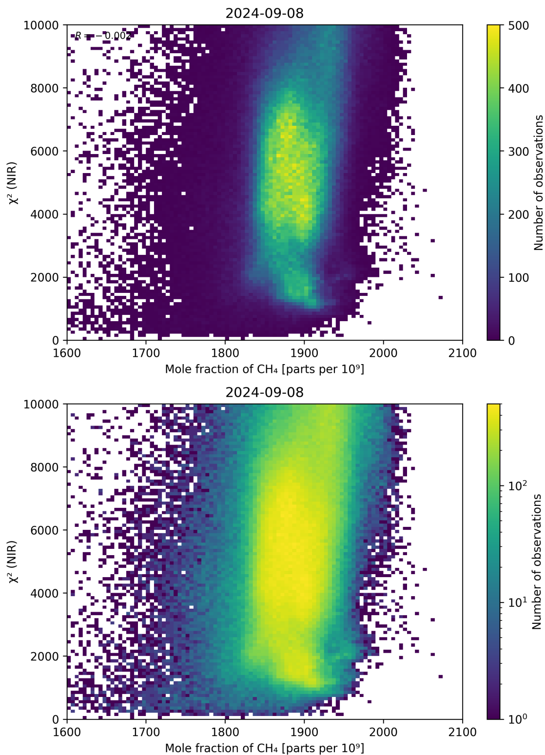
Figure 70: Scatter density plot of “Mole fraction of CH 4 ” against “ \chi^2 (NIR)” for 2024-09-07 to 2024-09-09.
