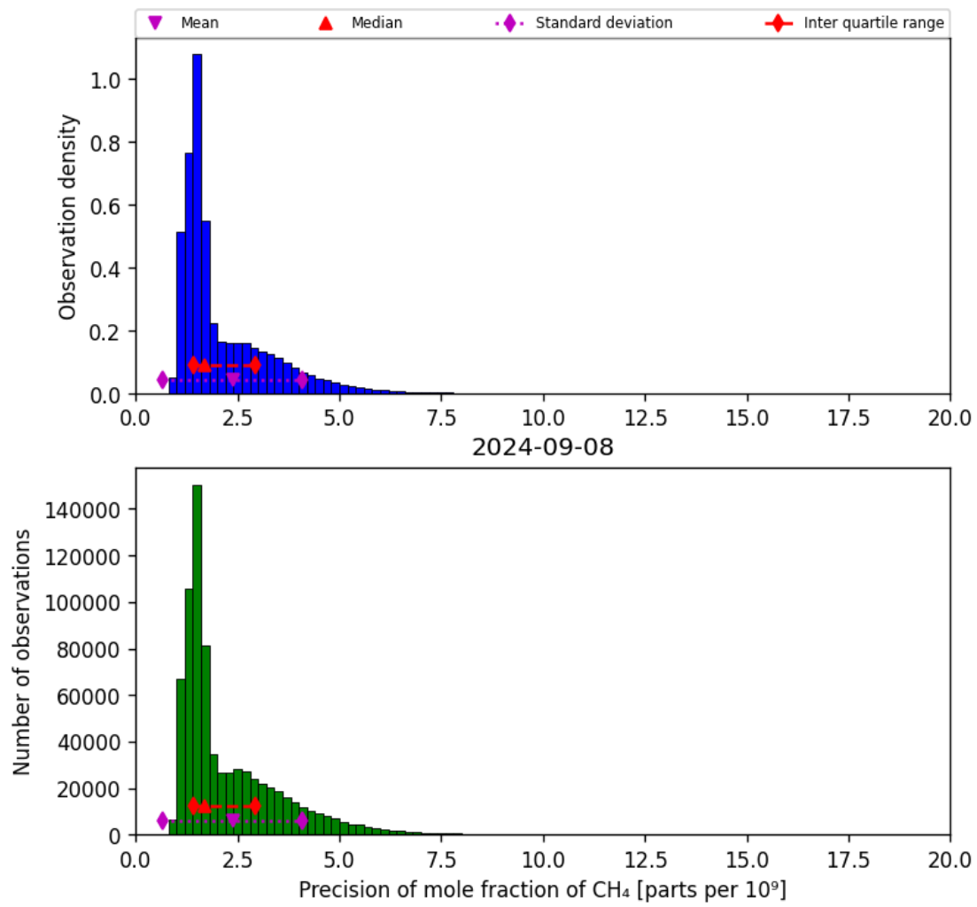
Figure 24: Histogram of “Precision of mole fraction of CH 4 ” for 2024-09-07 to 2024-09-09
