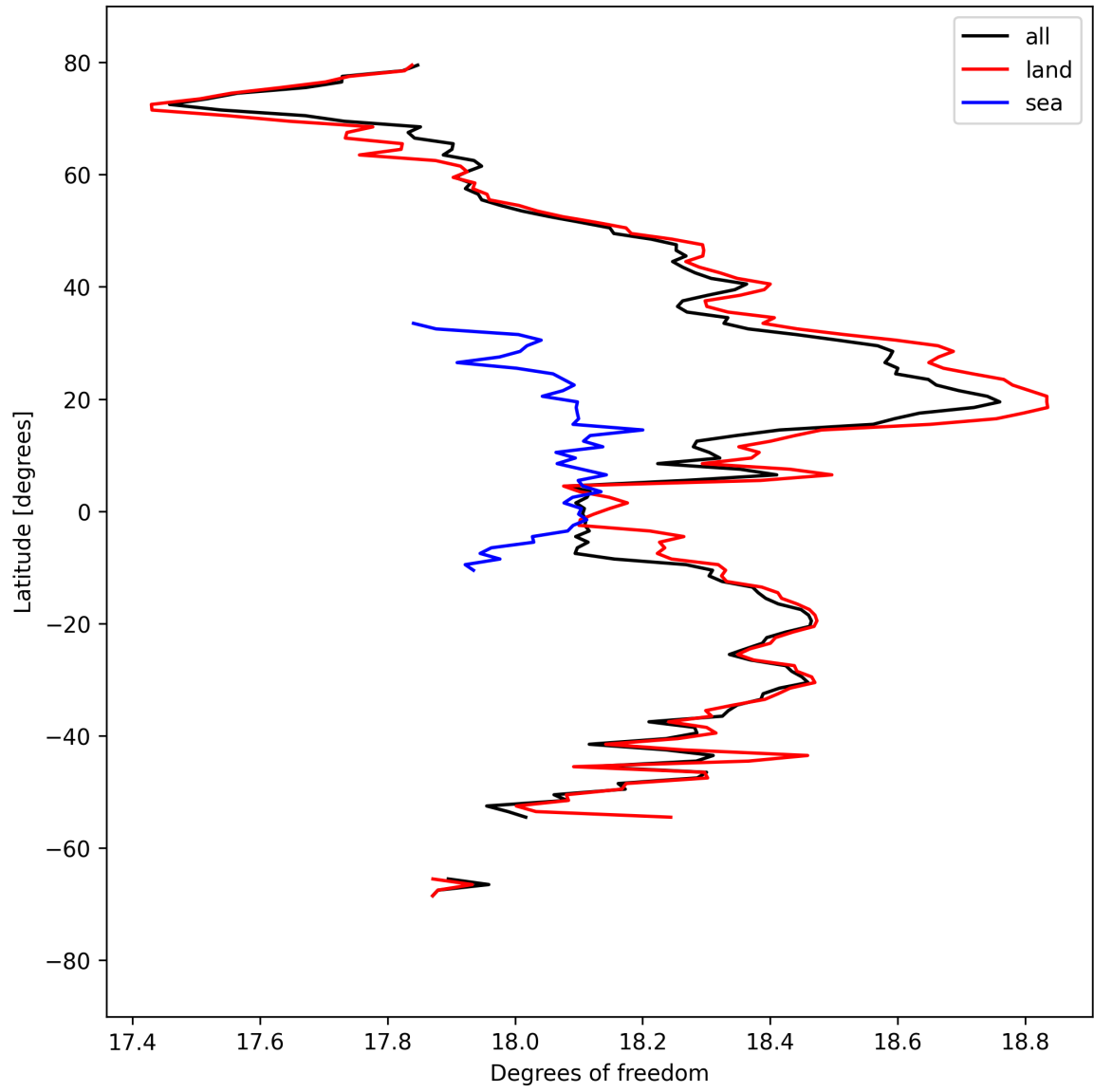
Figure 19: Zonal average of “Degrees of freedom” for 2024-09-07 to 2024-09-09.
