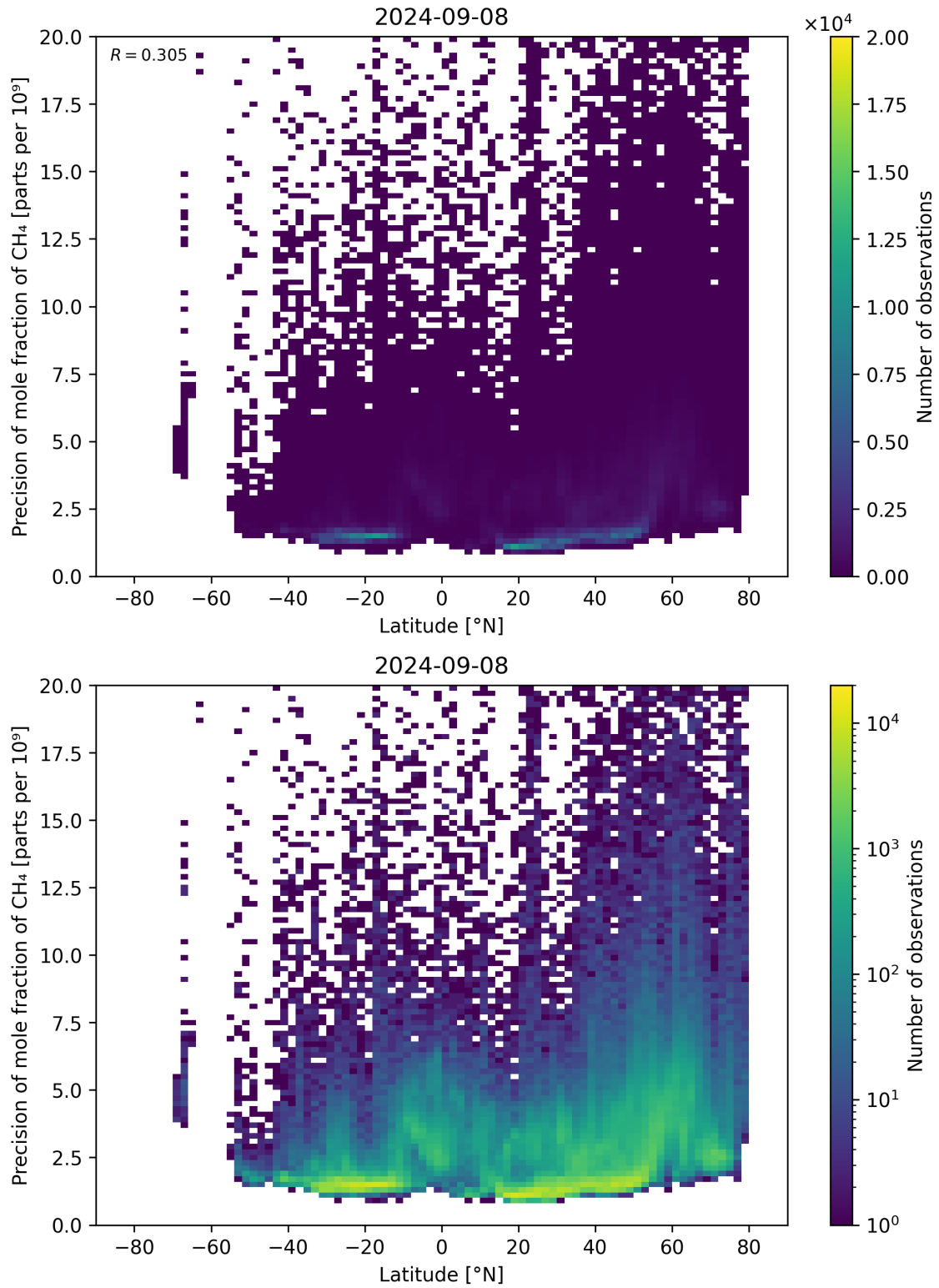
Figure 59: Scatter density plot of “Latitude” against “Precision of mole fraction of \text{CH}_4 ” for 2024-09-07 to 2024-09-09.
