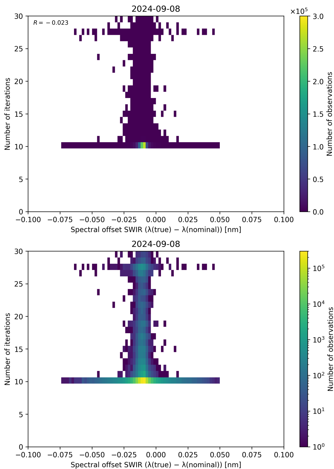
Figure 121: Scatter density plot of “Spectral offset SWIR ( \lambda_{\text{true}} - \lambda_{\text{nominal}} )” against “Number of iterations” for 2024-09-07 to 2024-09-09.
