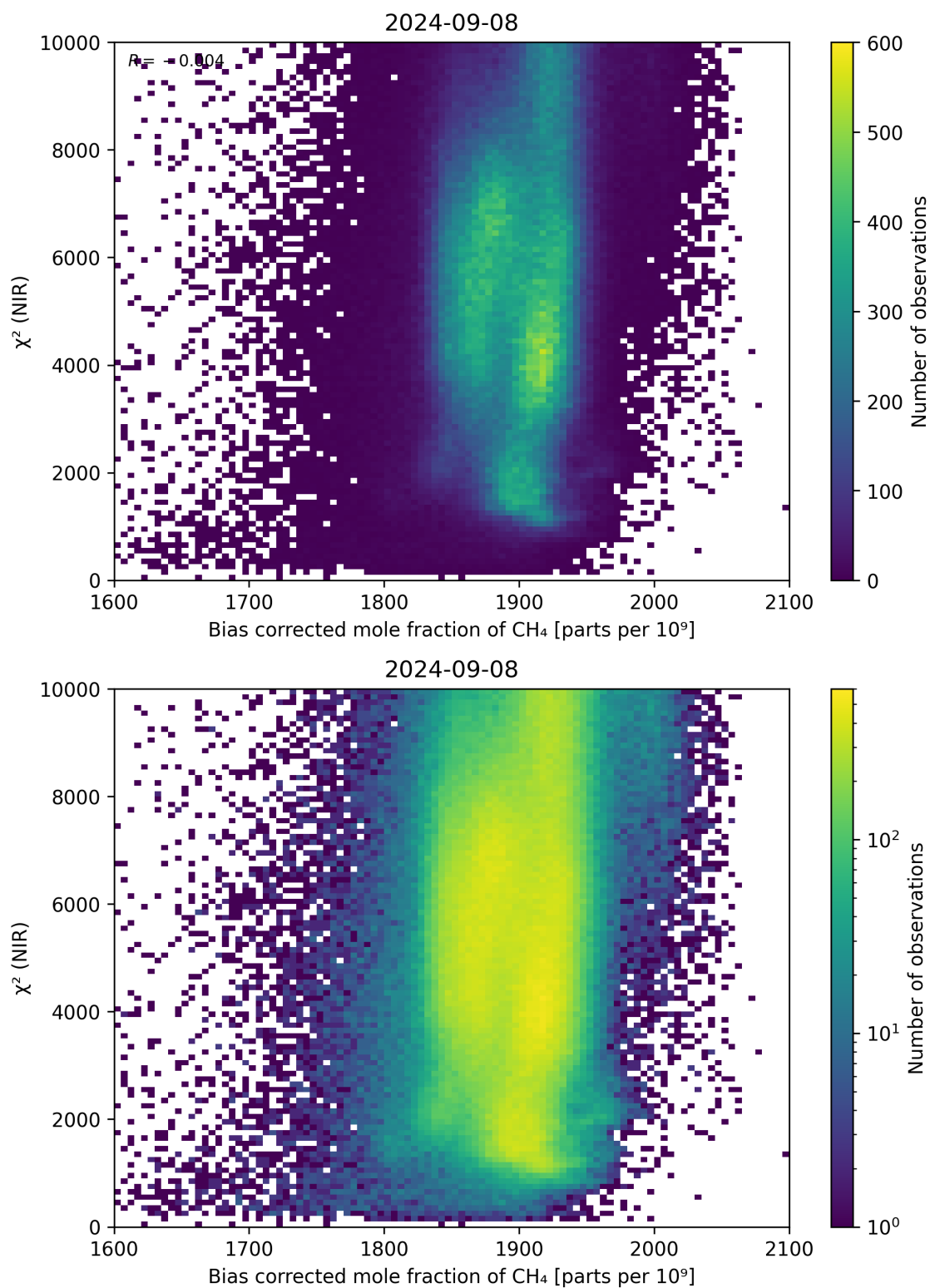
Figure 63: Scatter density plot of “Bias corrected mole fraction of CH 4 ” against “ \chi^2 (NIR)” for 2024-09-07 to 2024-09-09.
