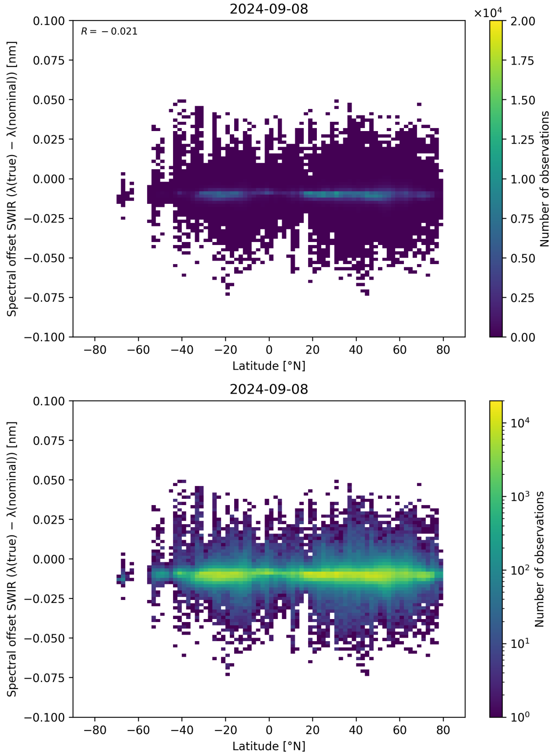
Figure 62: Scatter density plot of “Latitude” against “Spectral offset SWIR ( \lambda_{\text{true}} - \lambda_{\text{nominal}} )” for 2024-09-07 to 2024-09-09.
