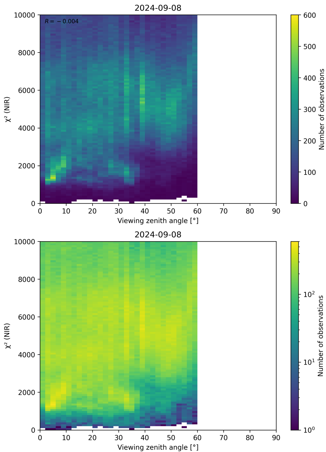
Figure 105: Scatter density plot of “Viewing zenith angle” against “ \chi^2 (NIR)” for 2024-09-07 to 2024-09-09.
