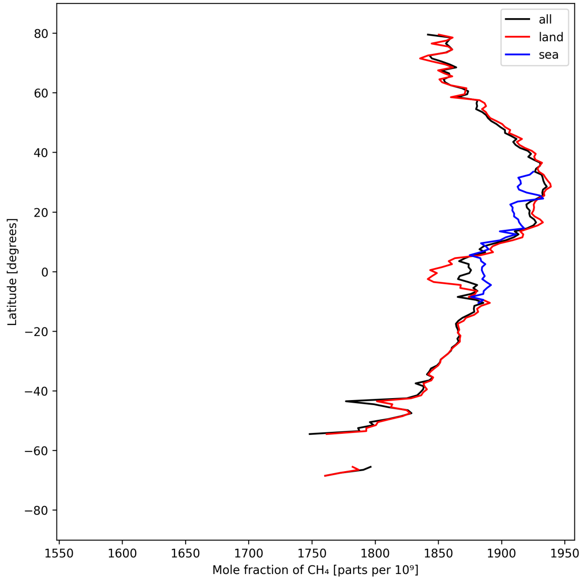
Figure 12: Zonal average of “Mole fraction of CH 4 ” for 2024-09-07 to 2024-09-09.
