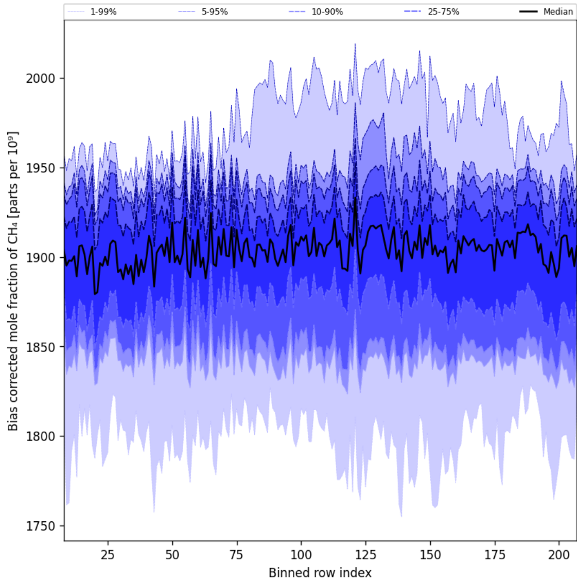
Figure 36: Along track statistics of “Bias corrected mole fraction of CH 4 ” for 2024-09-07 to 2024-09-09
