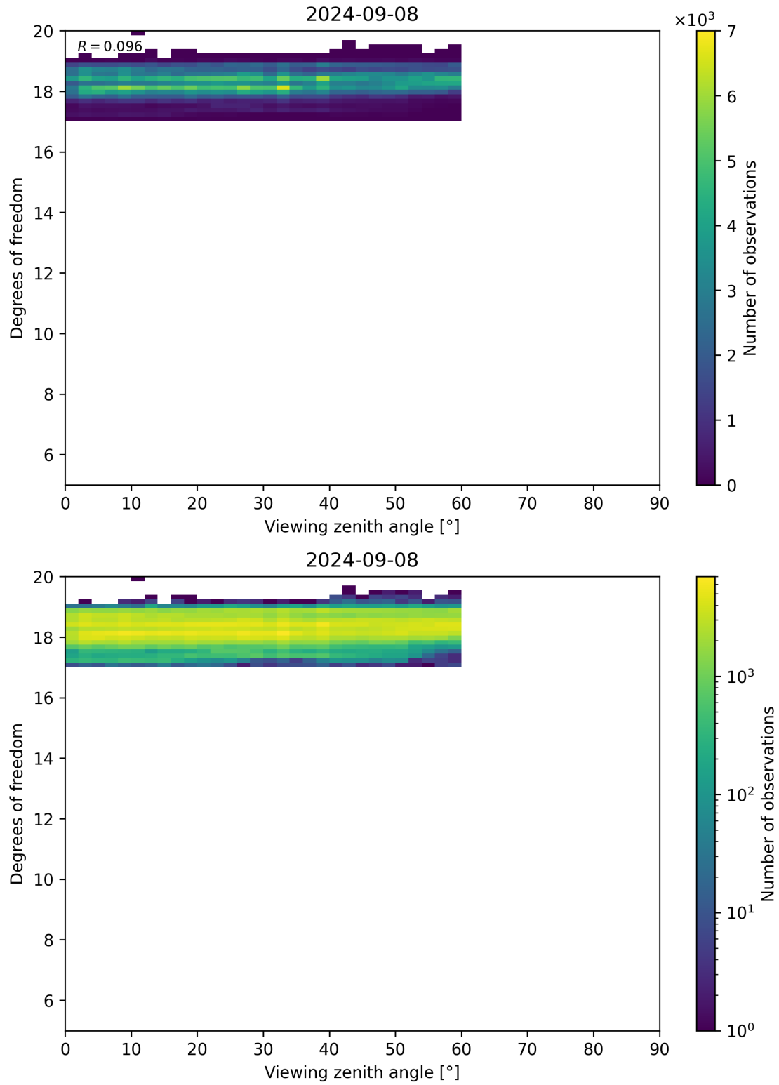
Figure 107: Scatter density plot of “Viewing zenith angle” against “Degrees of freedom” for 2024-09-07 to 2024-09-09.
