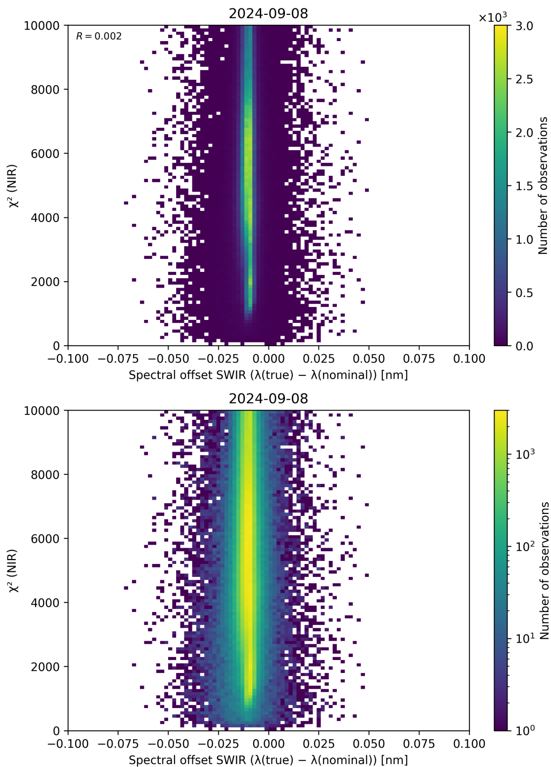
Figure 117: Scatter density plot of “Spectral offset SWIR ( \lambda_{\text{true}} - \lambda_{\text{nominal}} )” against “ \chi^2 (NIR)” for 2024-09-07 to 2024-09-09.
