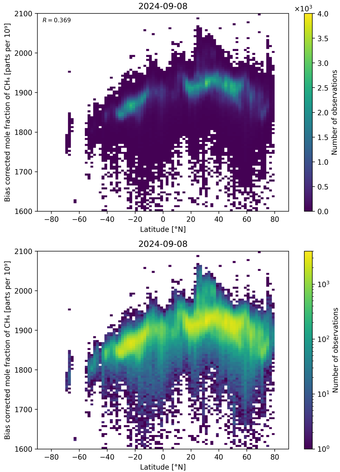
Figure 58: Scatter density plot of “Latitude” against “Bias corrected mole fraction of \text{CH}_4 ” for 2024-09-07 to 2024-09-09.
