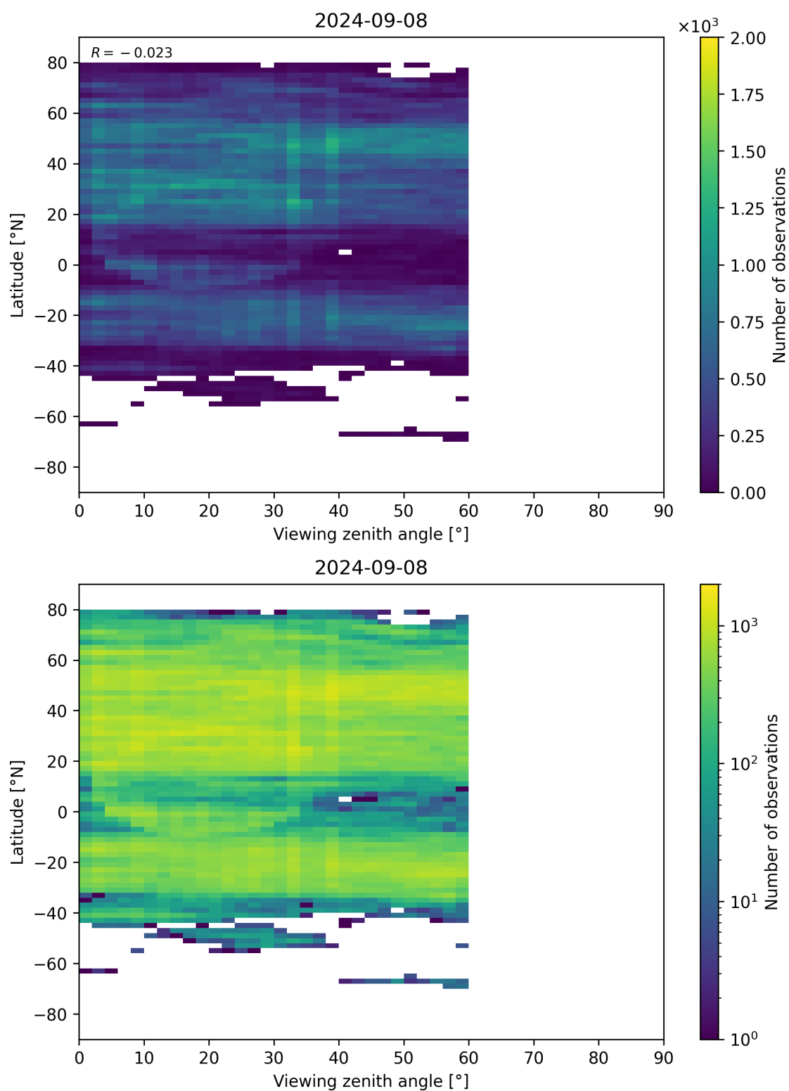
Figure 109: Scatter density plot of “Viewing zenith angle” against “Latitude” for 2024-09-07 to 2024-09-09.
