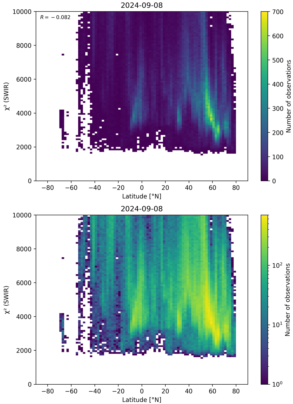
Figure 54: Scatter density plot of “Latitude” against “ \chi^2 (SWIR)” for 2024-09-07 to 2024-09-09.
