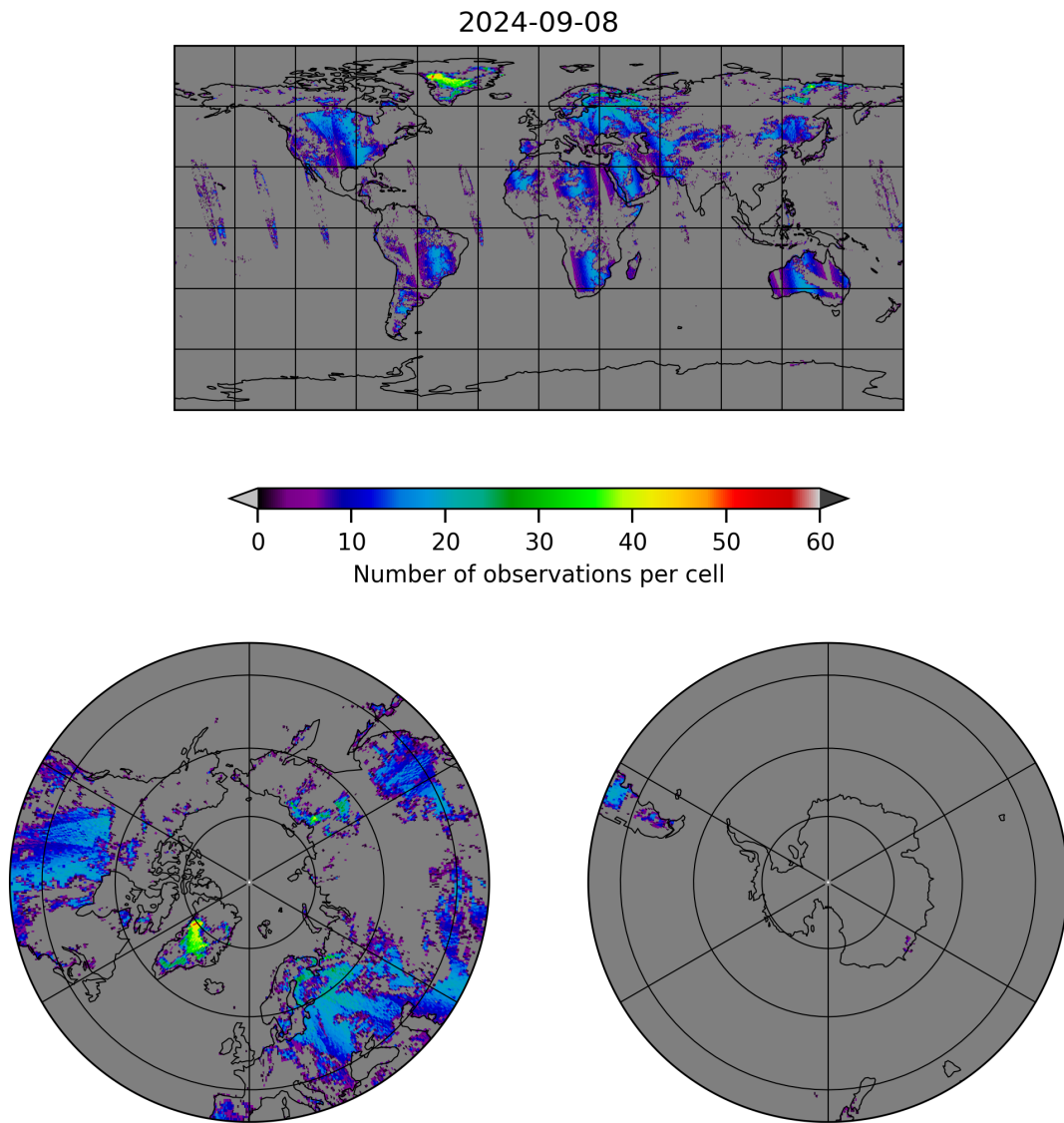
Figure 10: Map of the number of observations for 2024-09-07 to 2024-09-09
