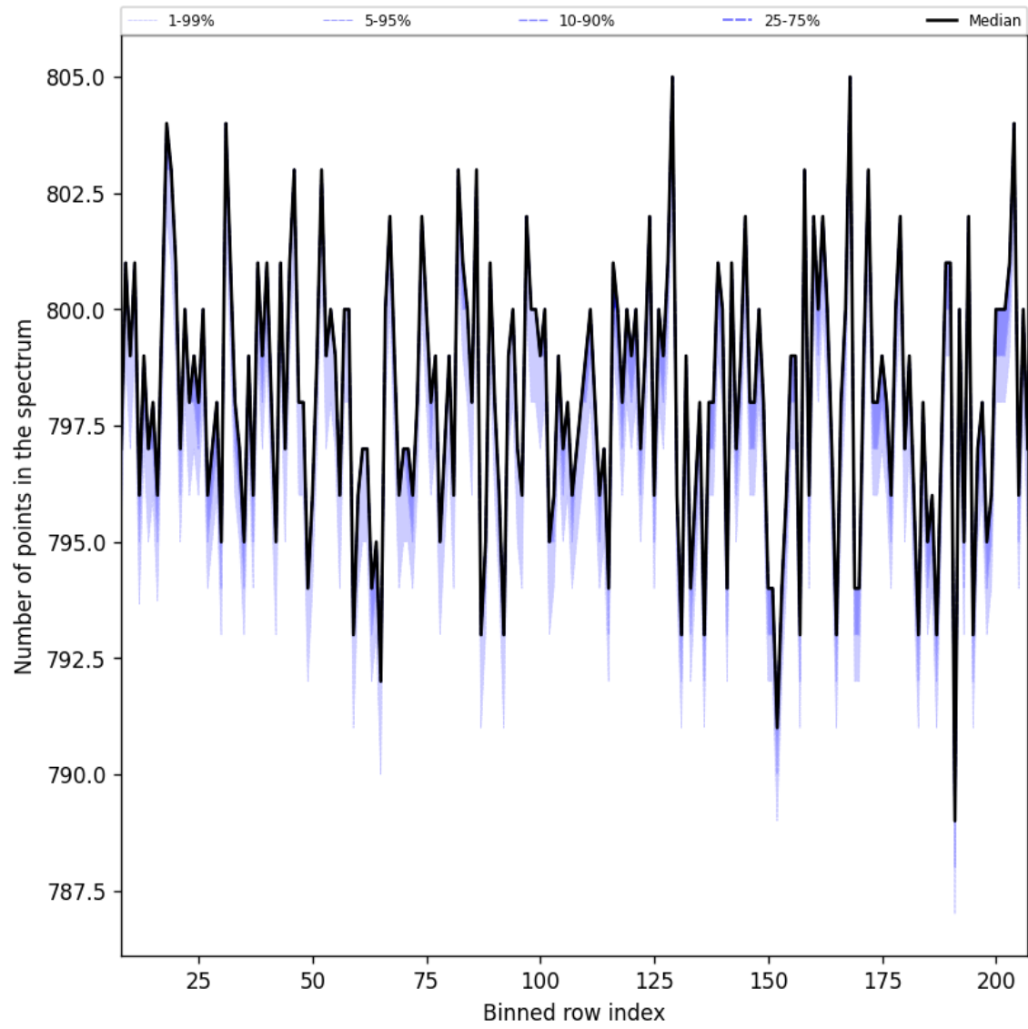
Figure 37: Along track statistics of “Number of points in the spectrum” for 2024-09-07 to 2024-09-09
