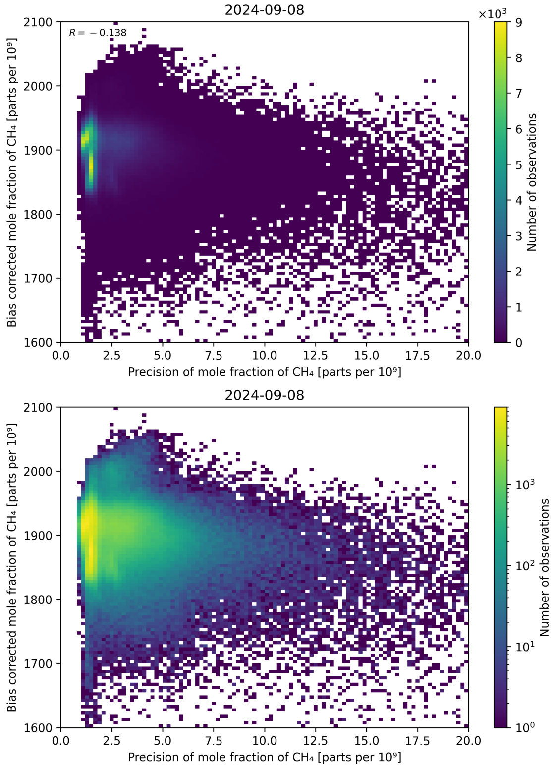
Figure 82: Scatter density plot of “Precision of mole fraction of CH 4 ” against “Bias corrected mole fraction of CH 4 ” for 2024-09-07 to 2024-09-09.
