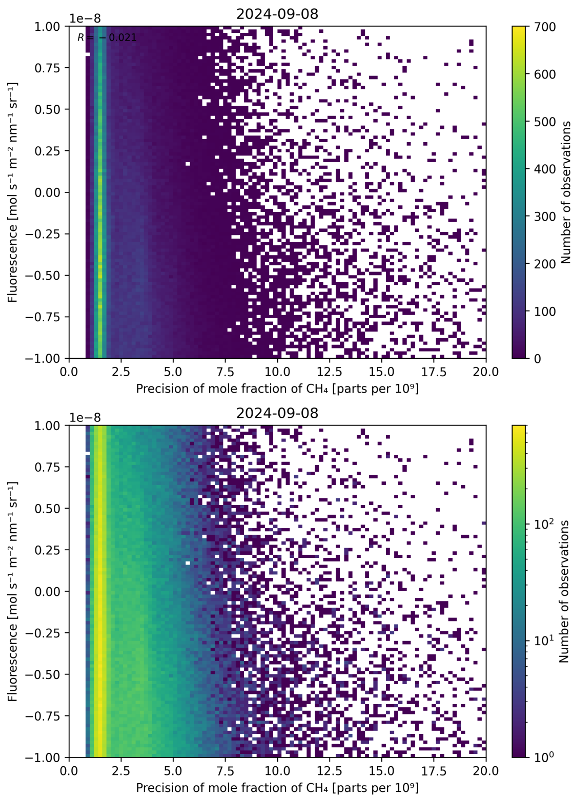
Figure 81: Scatter density plot of “Precision of mole fraction of \text{CH}_4 ” against “Fluorescence” for 2024-09-07 to 2024-09-09.
