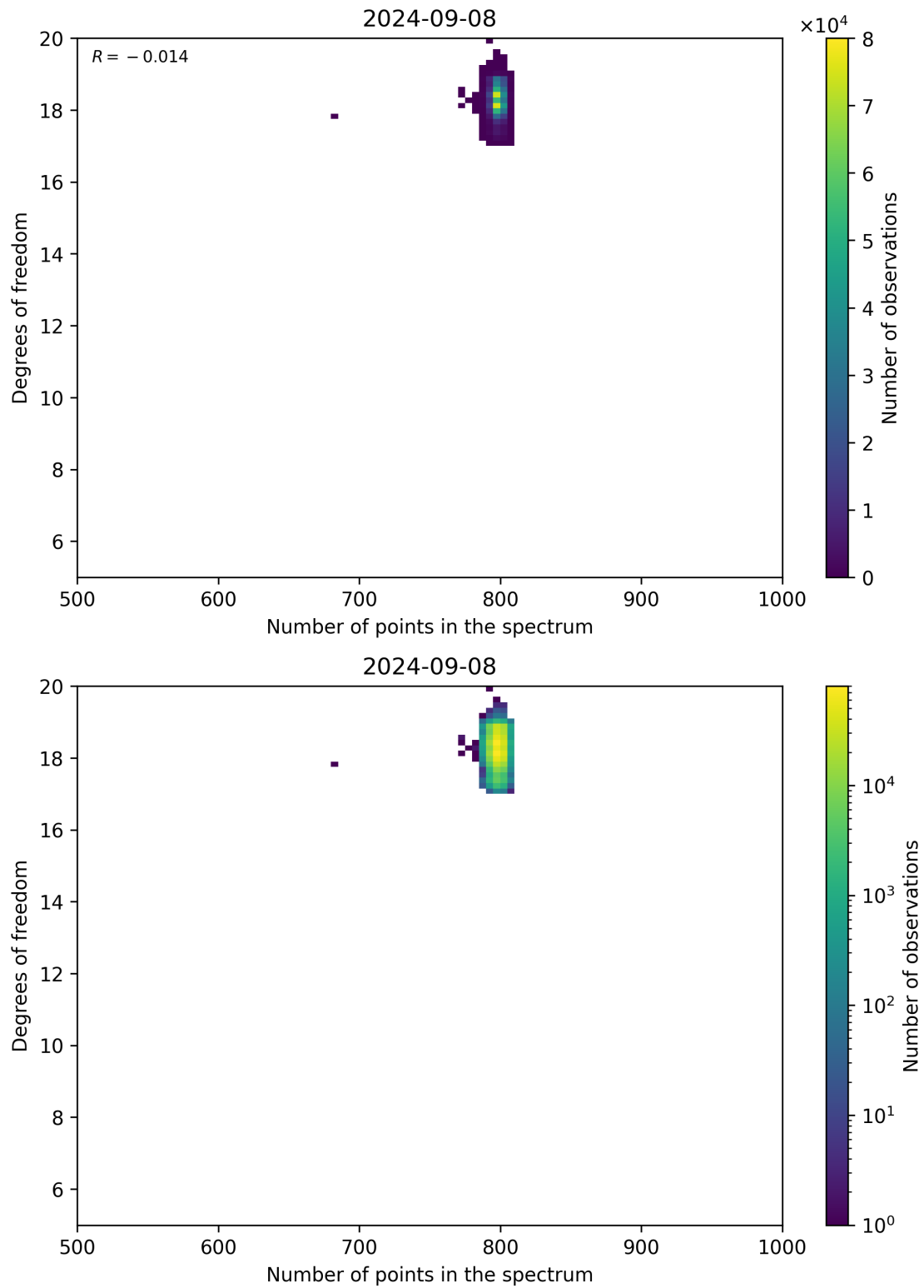
Figure 90: Scatter density plot of “Number of points in the spectrum” against “Degrees of freedom” for 2024-09-07 to 2024-09-09.
