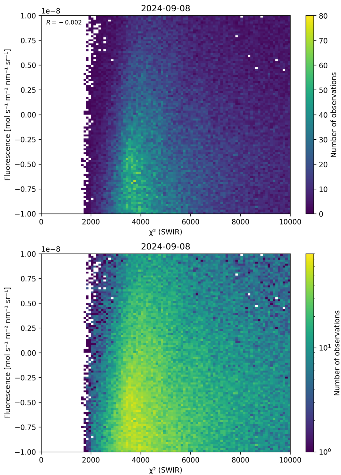
Figure 49: Scatter density plot of “ \chi^2 (SWIR)” against “Fluorescence” for 2024-09-07 to 2024-09-09.
