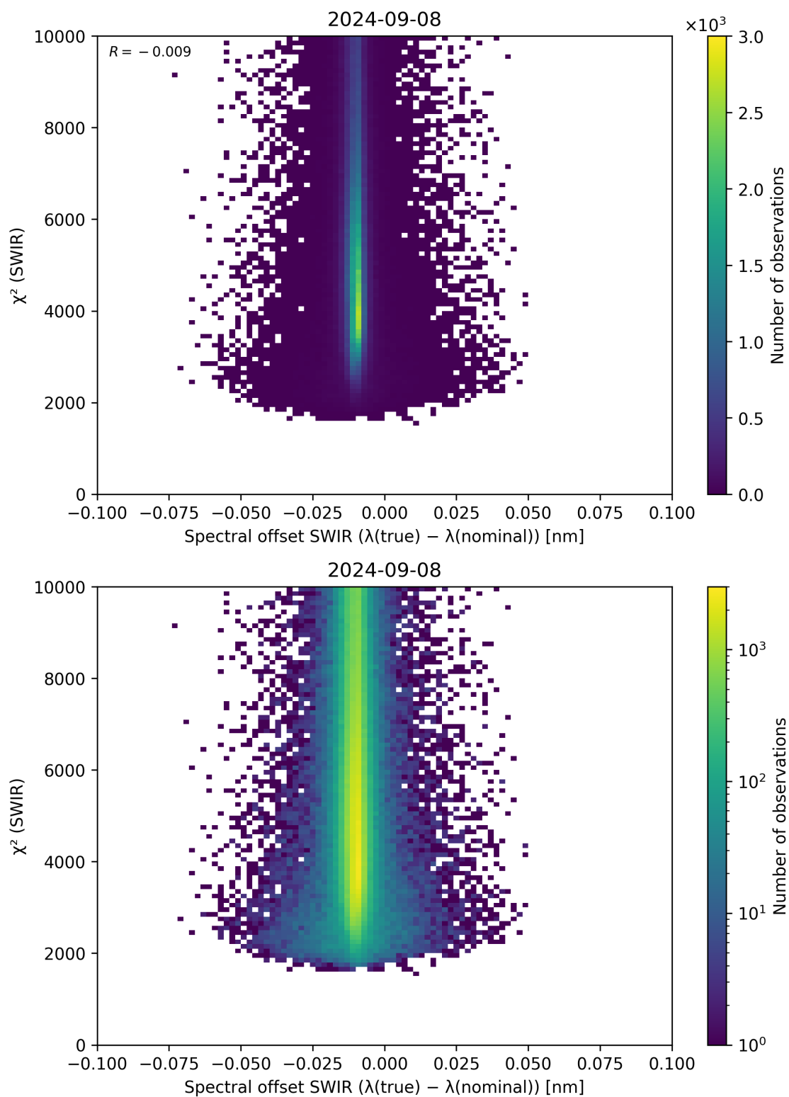
Figure 118: Scatter density plot of “Spectral offset SWIR ( \lambda_{\text{true}} - \lambda_{\text{nominal}} )” against “ \chi^2 (SWIR)” for 2024-09-07 to 2024-09-09.
