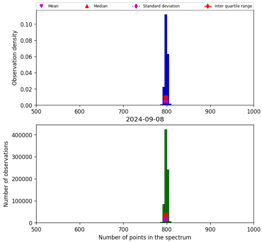
Figure 26: Histogram of “Number of points in the spectrum” for 2024-09-07 to 2024-09-09
