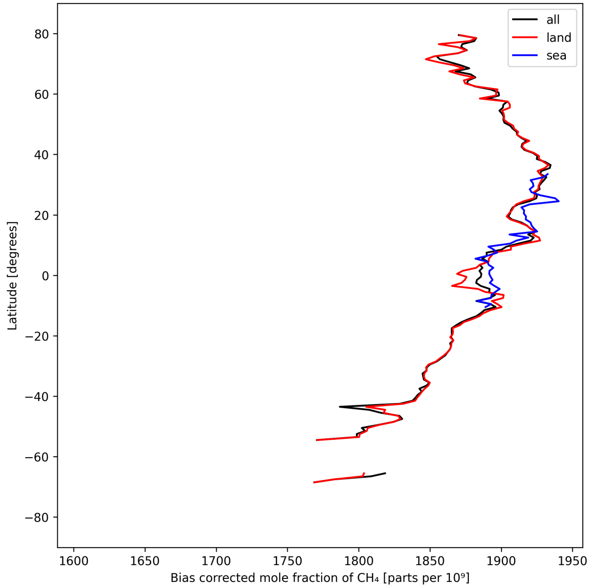
Figure 14: Zonal average of “Bias corrected mole fraction of \text{CH}_4 ” for 2024-09-07 to 2024-09-09.
