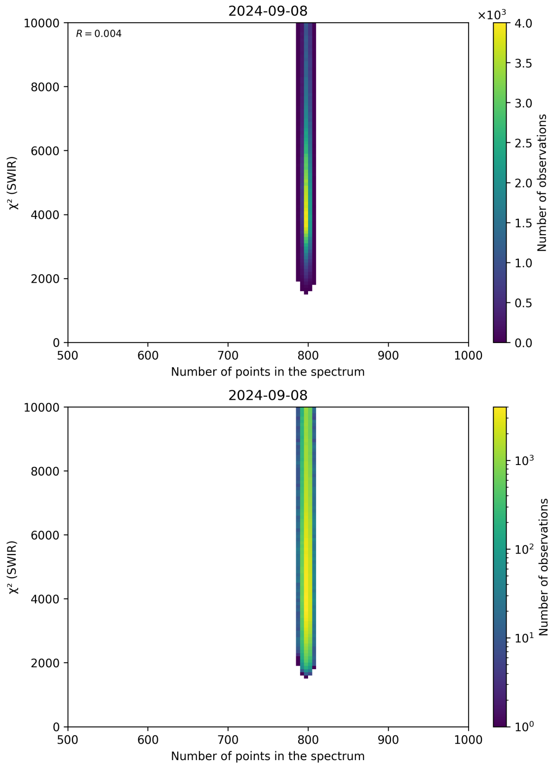
Figure 89: Scatter density plot of “Number of points in the spectrum” against “ \chi^2 (SWIR)” for 2024-09-07 to 2024-09-09.
