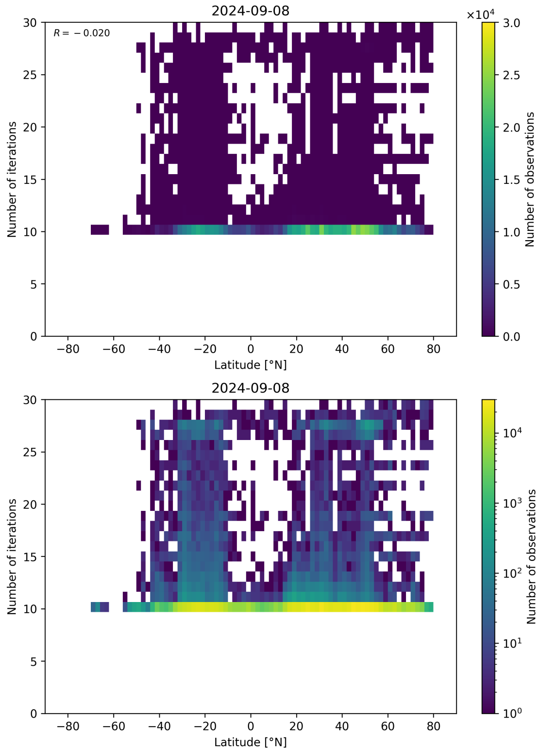
Figure 60: Scatter density plot of “Latitude” against “Number of iterations” for 2024-09-07 to 2024-09-09.
