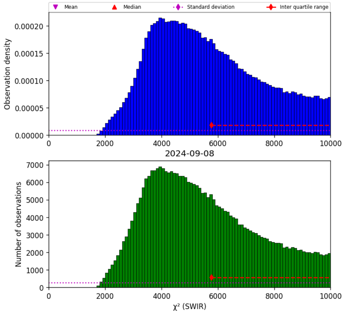
Figure 28: Histogram of “ \chi^2 (SWIR)” for 2024-09-07 to 2024-09-09
