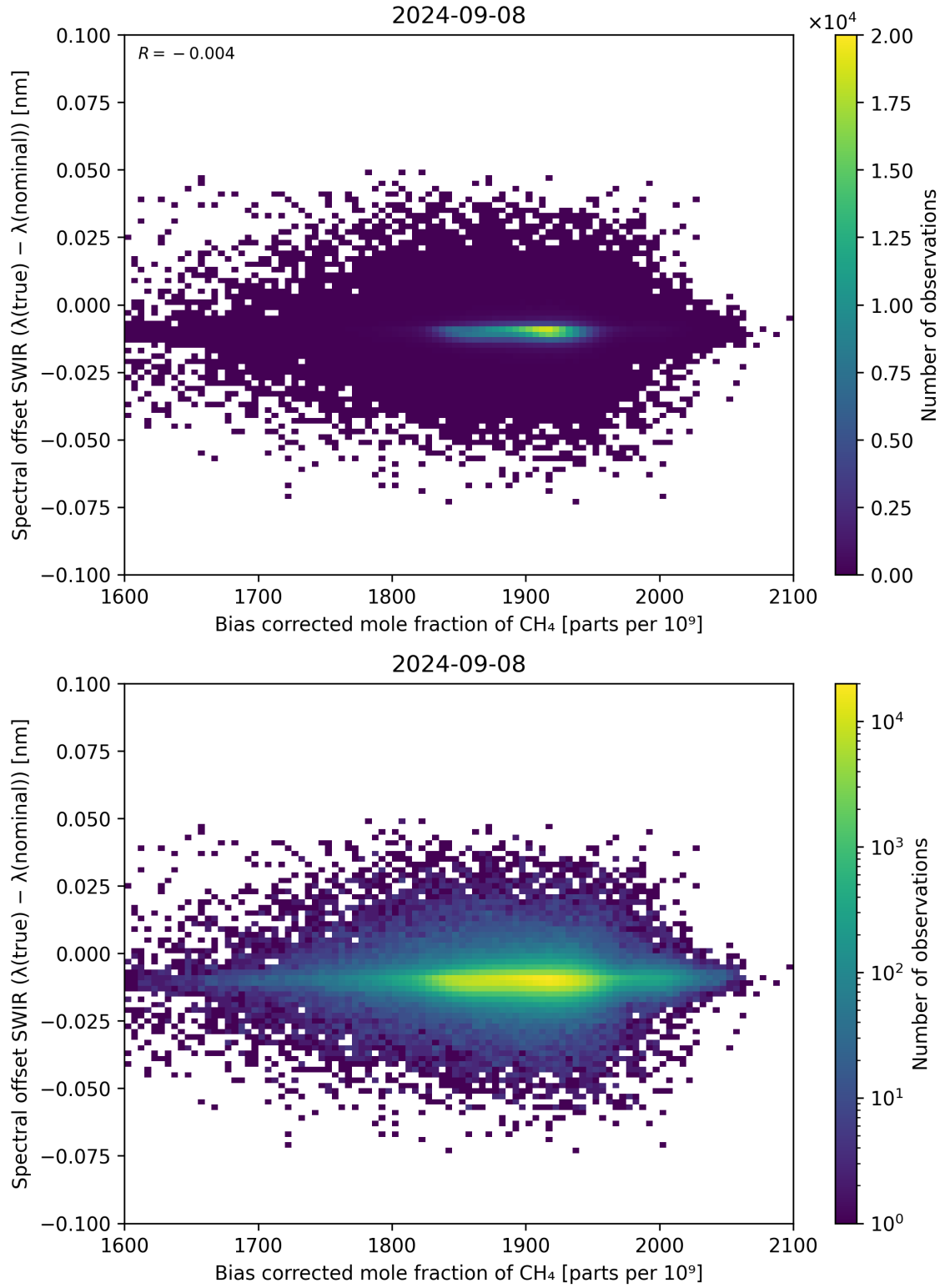
Figure 69: Scatter density plot of “Bias corrected mole fraction of CH 4 ” against “Spectral offset SWIR ( \lambda_{\text{true}} - \lambda_{\text{nominal}} )” for 2024-09-07 to 2024-09-09.
