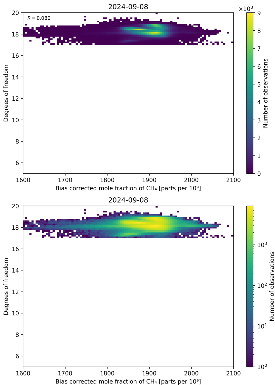
Figure 65: Scatter density plot of “Bias corrected mole fraction of CH 4 ” against “Degrees of freedom” for 2024-09-07 to 2024-09-09.
