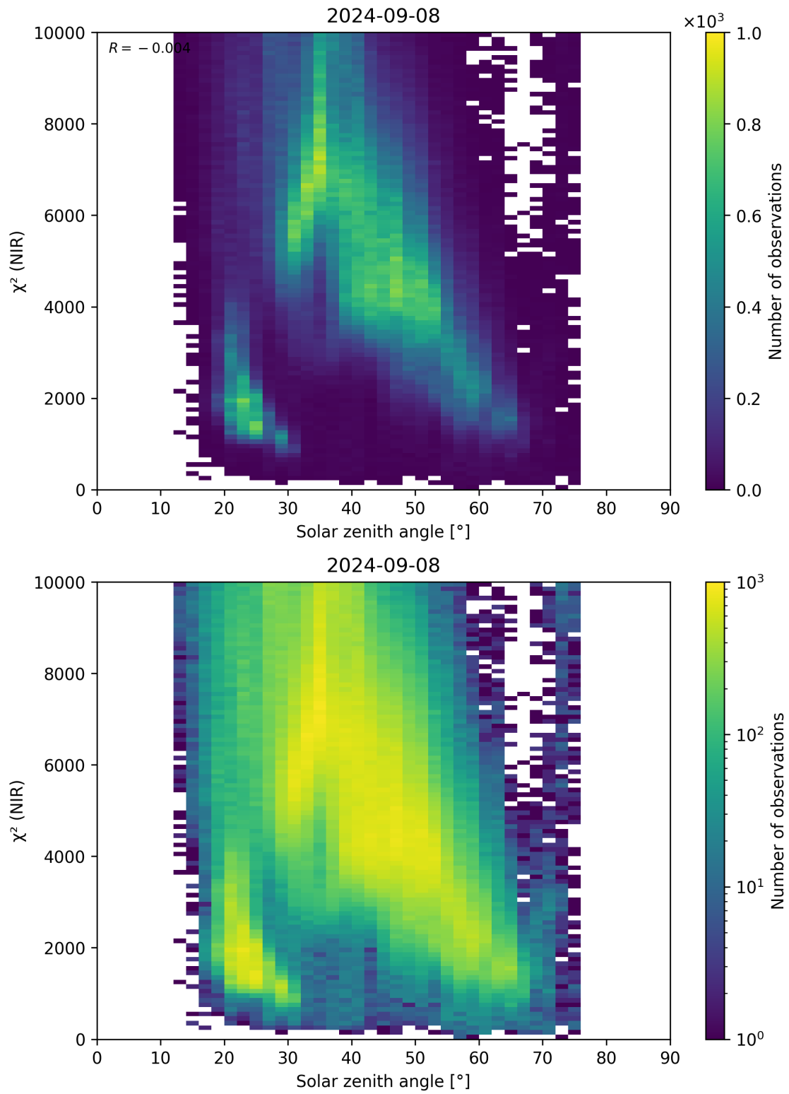
Figure 94: Scatter density plot of “Solar zenith angle” against “ \chi^2 (NIR)” for 2024-09-07 to 2024-09-09.
