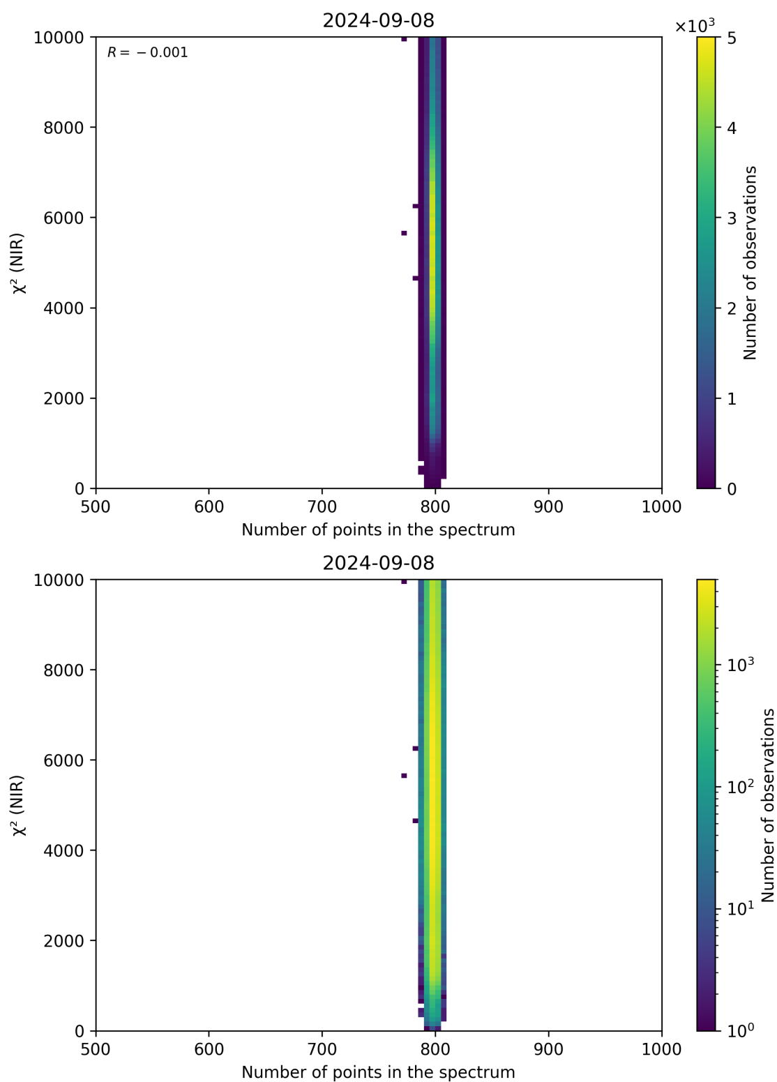
Figure 88: Scatter density plot of “Number of points in the spectrum” against “ \chi^2 (NIR)” for 2024-09-07 to 2024-09-09.
