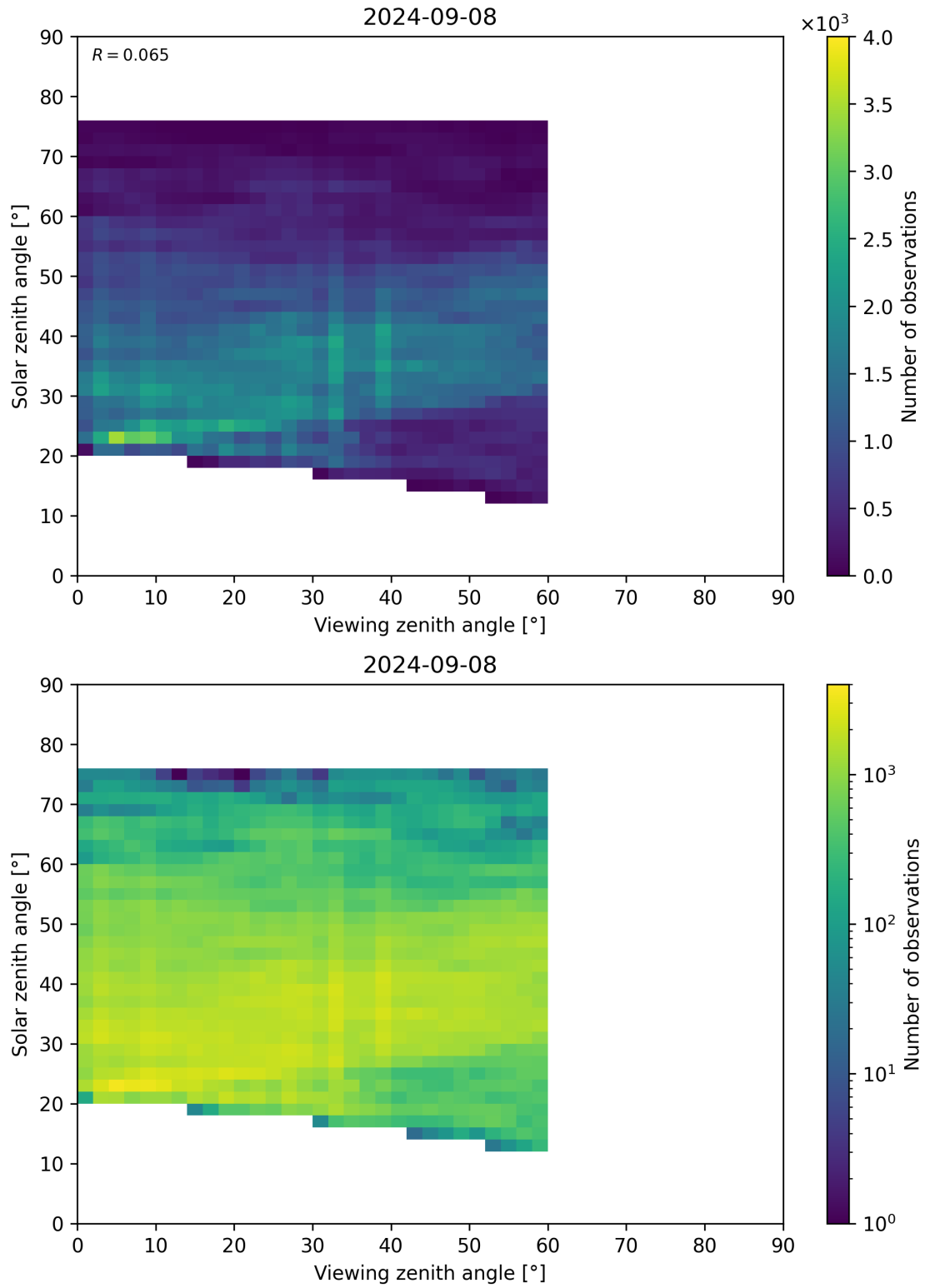
Figure 115: Scatter density plot of “Viewing zenith angle” against “Solar zenith angle” for 2024-09-07 to 2024-09-09.
