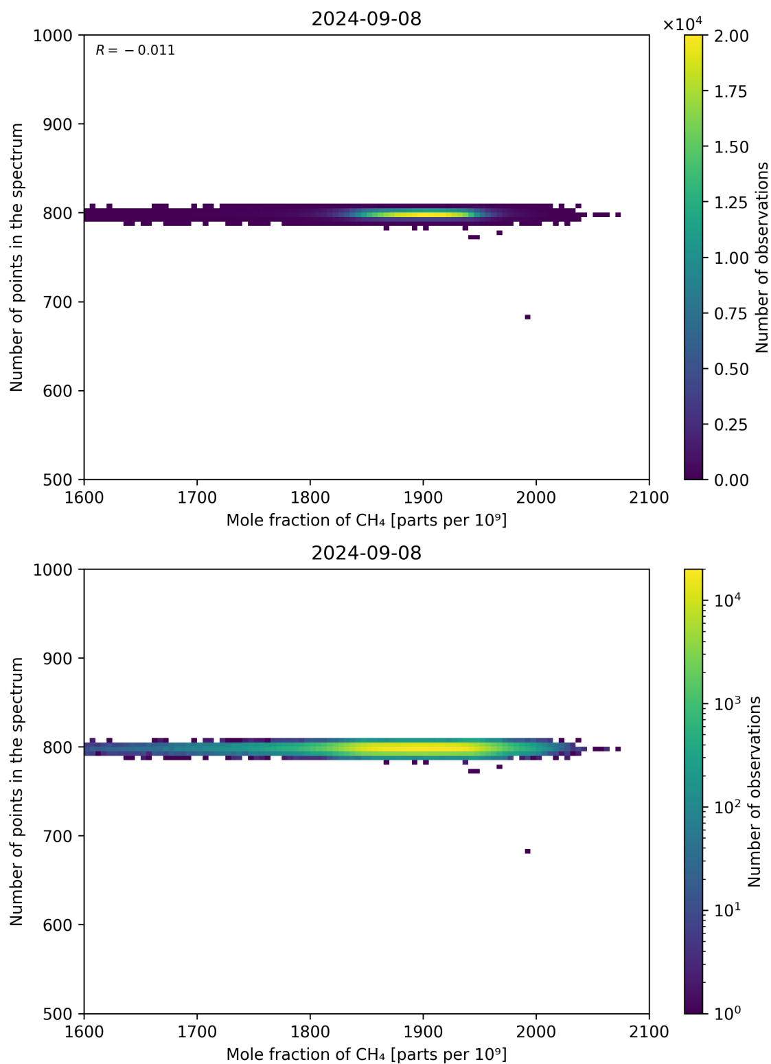
Figure 77: Scatter density plot of “Mole fraction of CH 4 ” against “Number of points in the spectrum” for 2024-09-07 to 2024-09-09.
