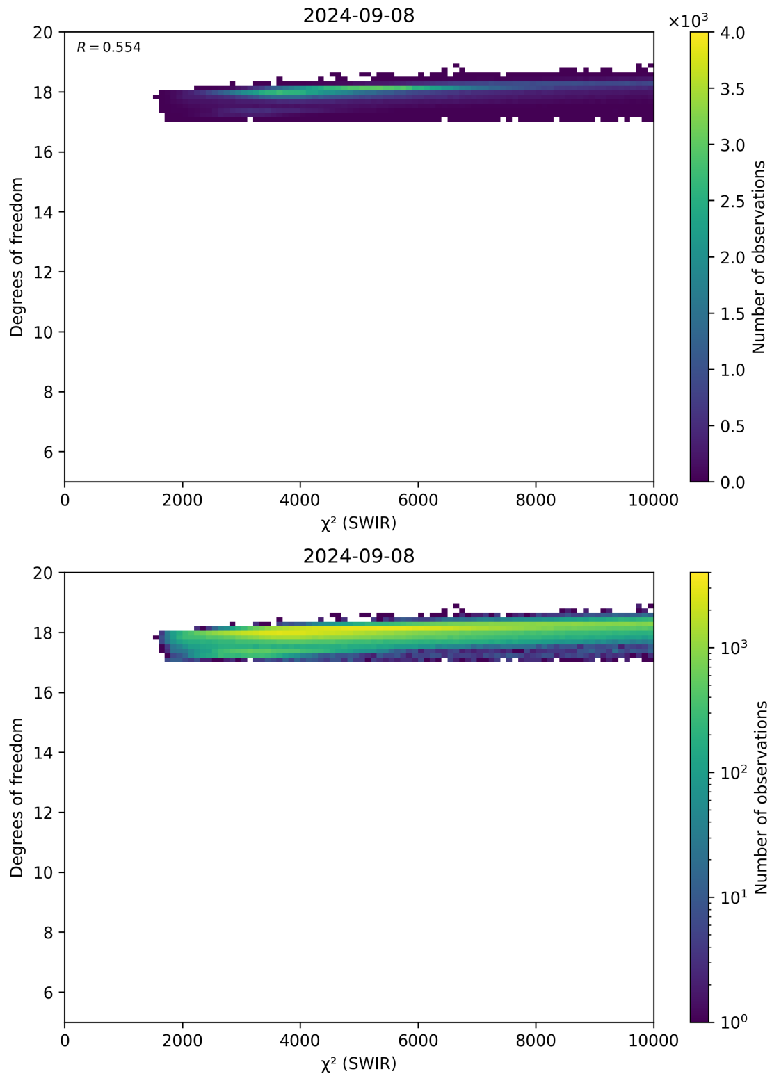
Figure 48: Scatter density plot of “ \chi^2 (SWIR)” against “Degrees of freedom” for 2024-09-07 to 2024-09-09.
