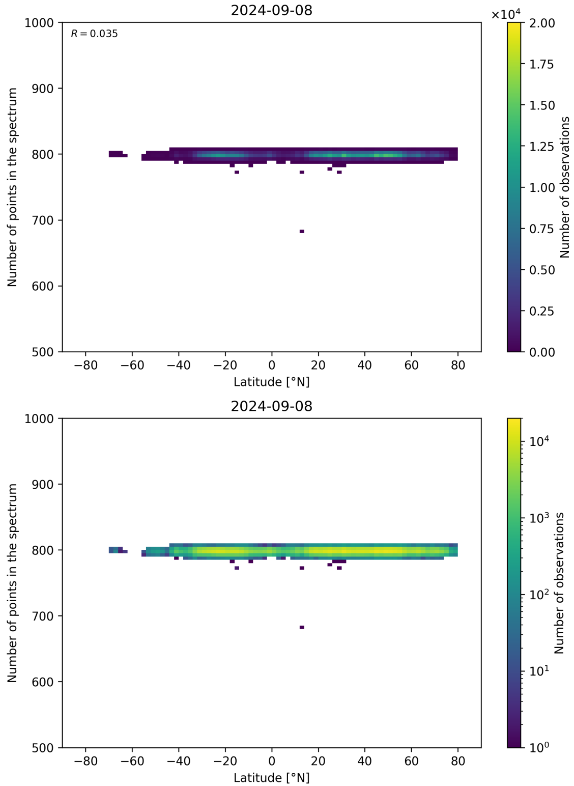
Figure 61: Scatter density plot of “Latitude” against “Number of points in the spectrum” for 2024-09-07 to 2024-09-09.
