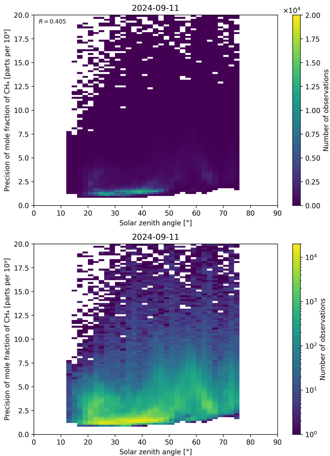
Figure 101: Scatter density plot of “Solar zenith angle” against “Precision of mole fraction of \text{CH}_4 ” for 2024-09-10 to 2024-09-12.
