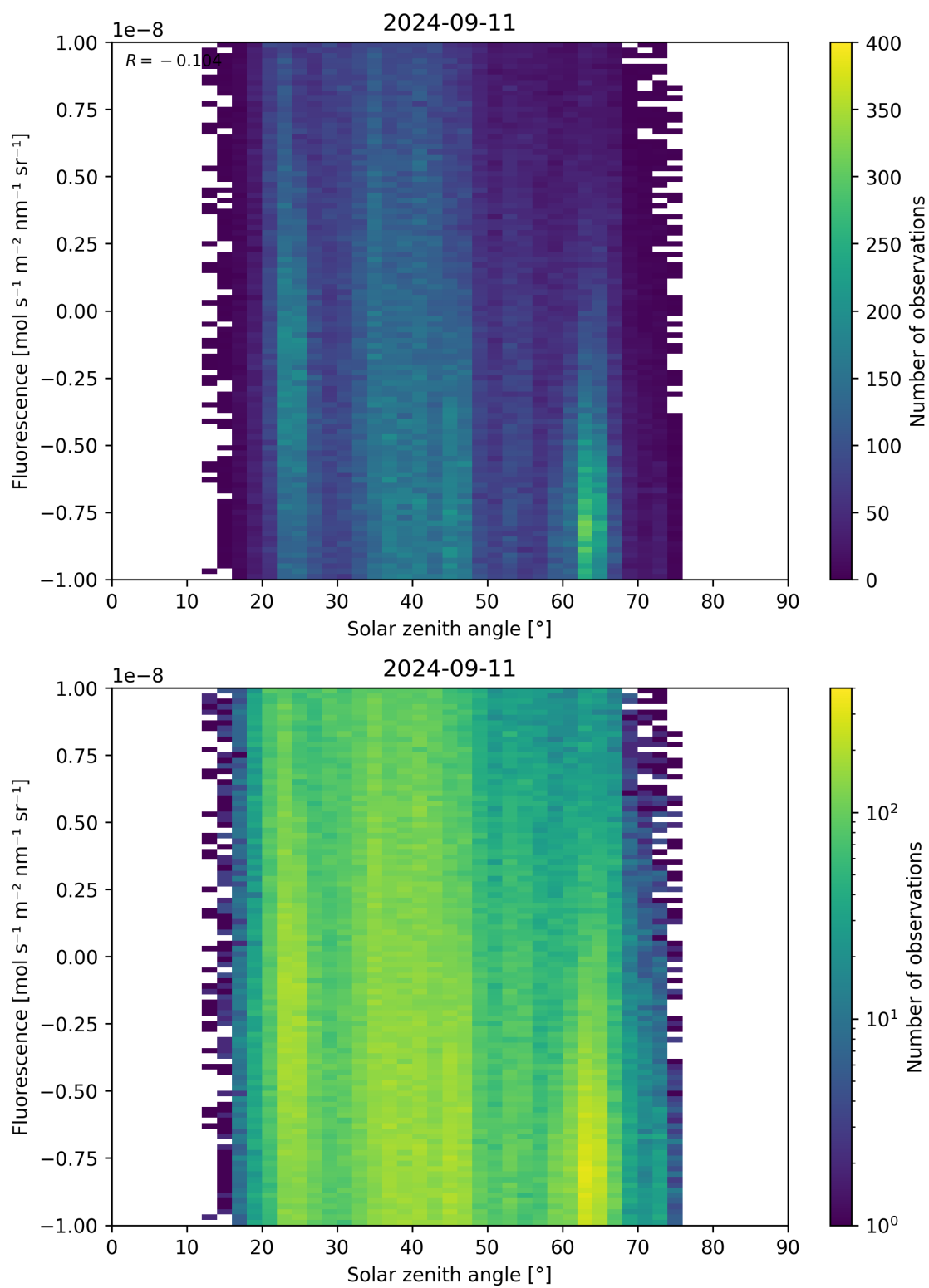
Figure 97: Scatter density plot of “Solar zenith angle” against “Fluorescence” for 2024-09-10 to 2024-09-12.
