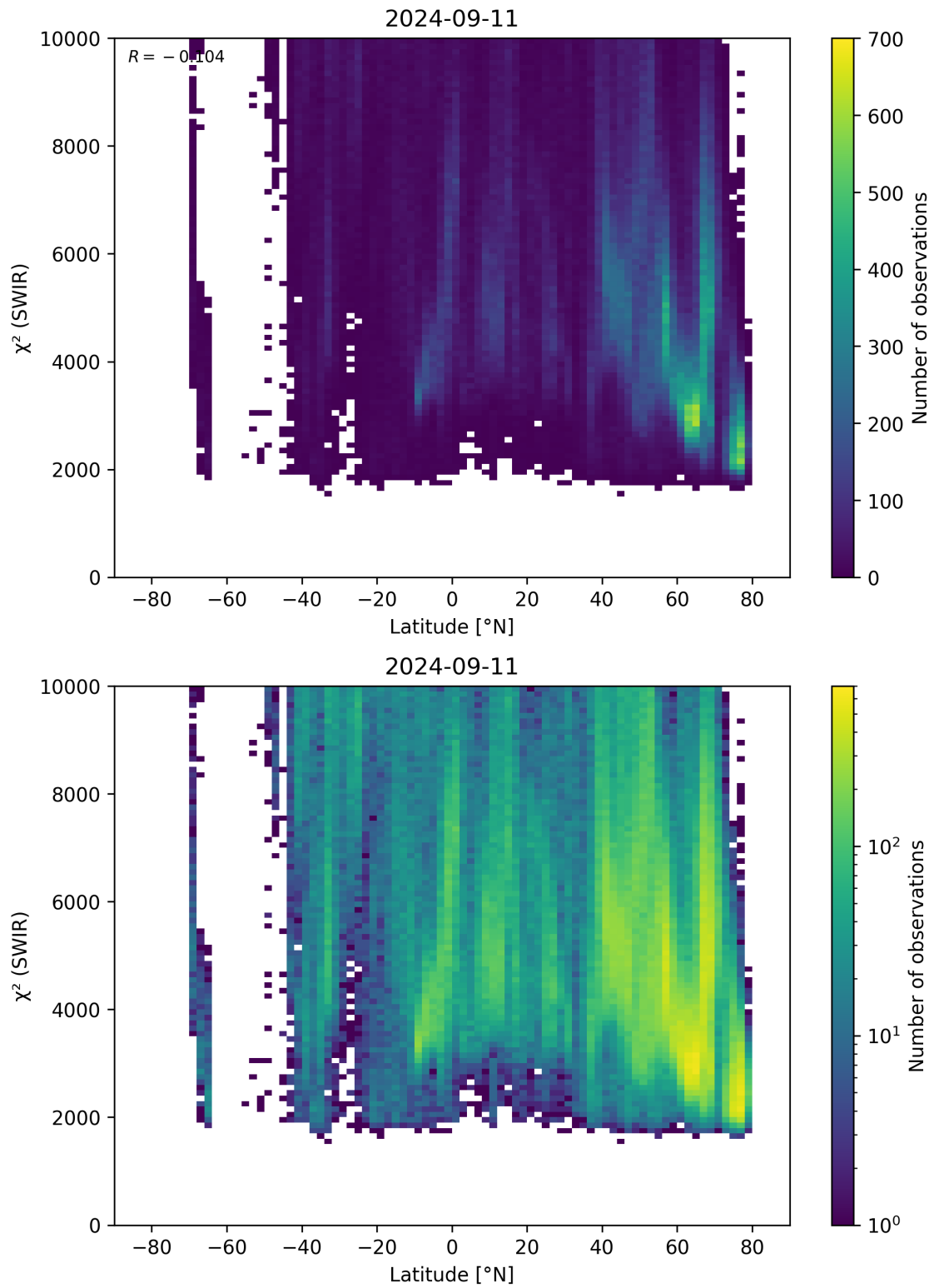
Figure 54: Scatter density plot of “Latitude” against “ \chi^2 (SWIR)” for 2024-09-10 to 2024-09-12.
