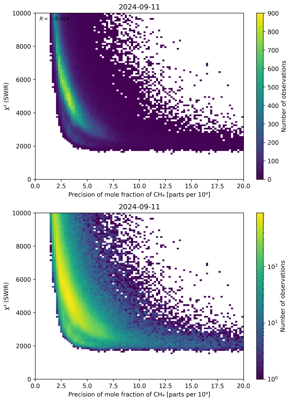
Figure 79: Scatter density plot of “Precision of mole fraction of CH 4 ” against “ \chi^2 (SWIR)” for 2024-09-10 to 2024-09-12.
