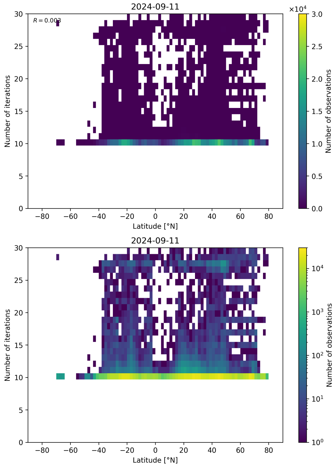
Figure 60: Scatter density plot of “Latitude” against “Number of iterations” for 2024-09-10 to 2024-09-12.
