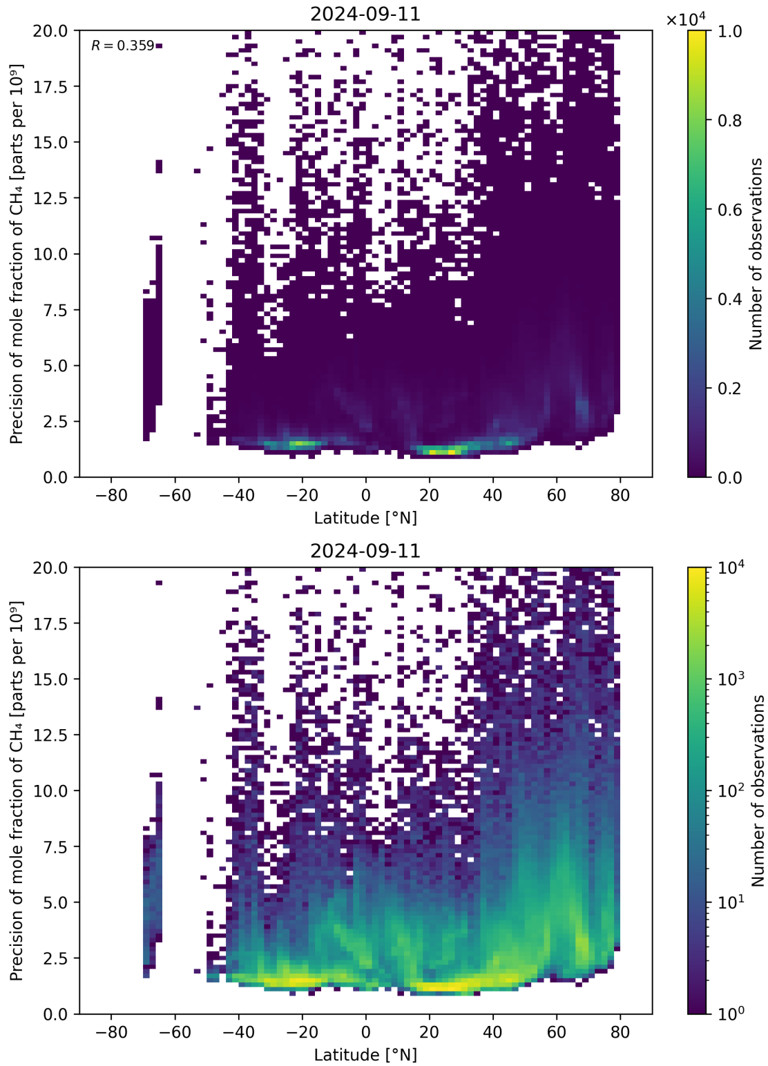
Figure 59: Scatter density plot of “Latitude” against “Precision of mole fraction of \text{CH}_4 ” for 2024-09-10 to 2024-09-12.
