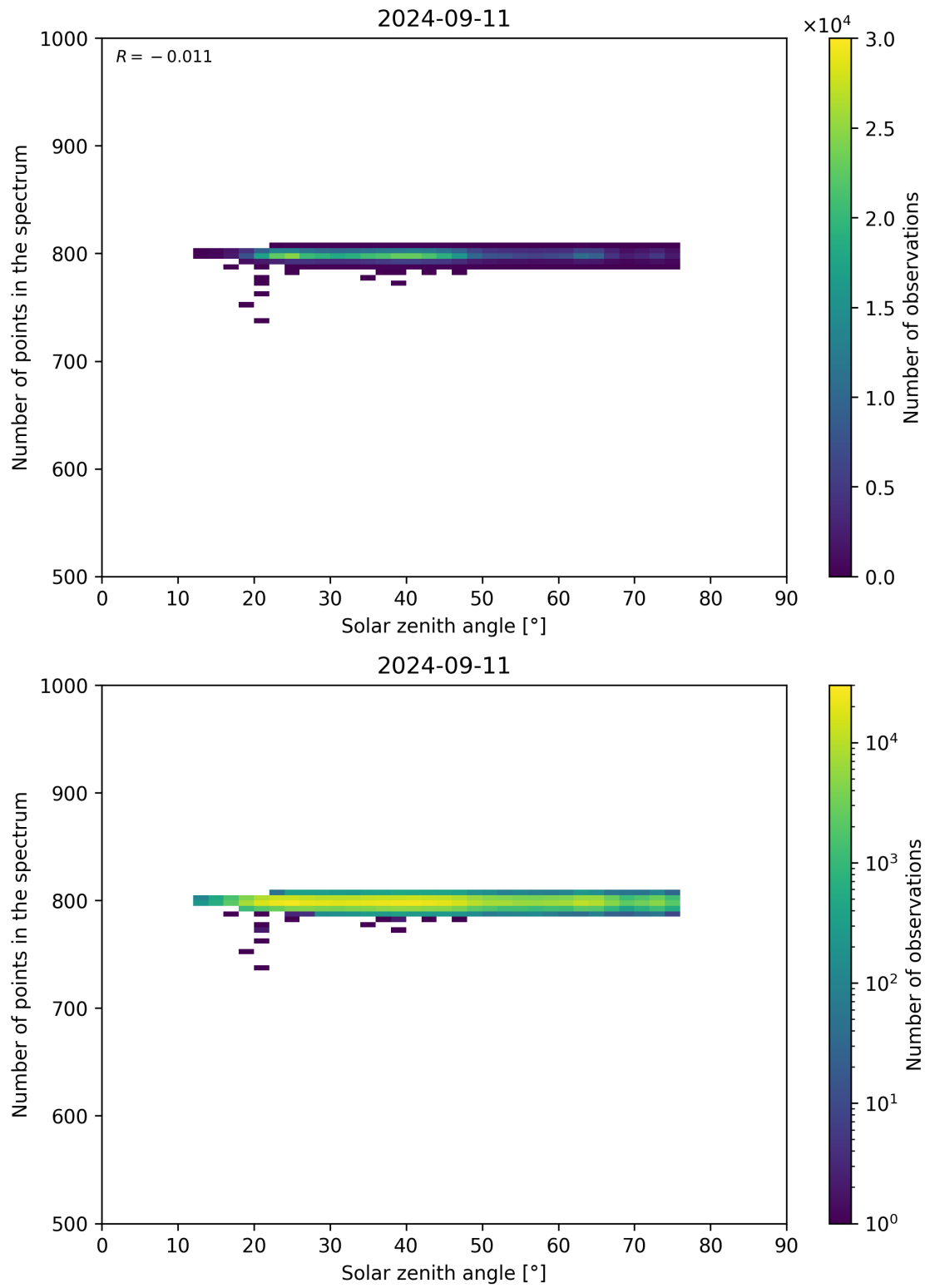
Figure 103: Scatter density plot of “Solar zenith angle” against “Number of points in the spectrum” for 2024-09-10 to 2024-09-12.
