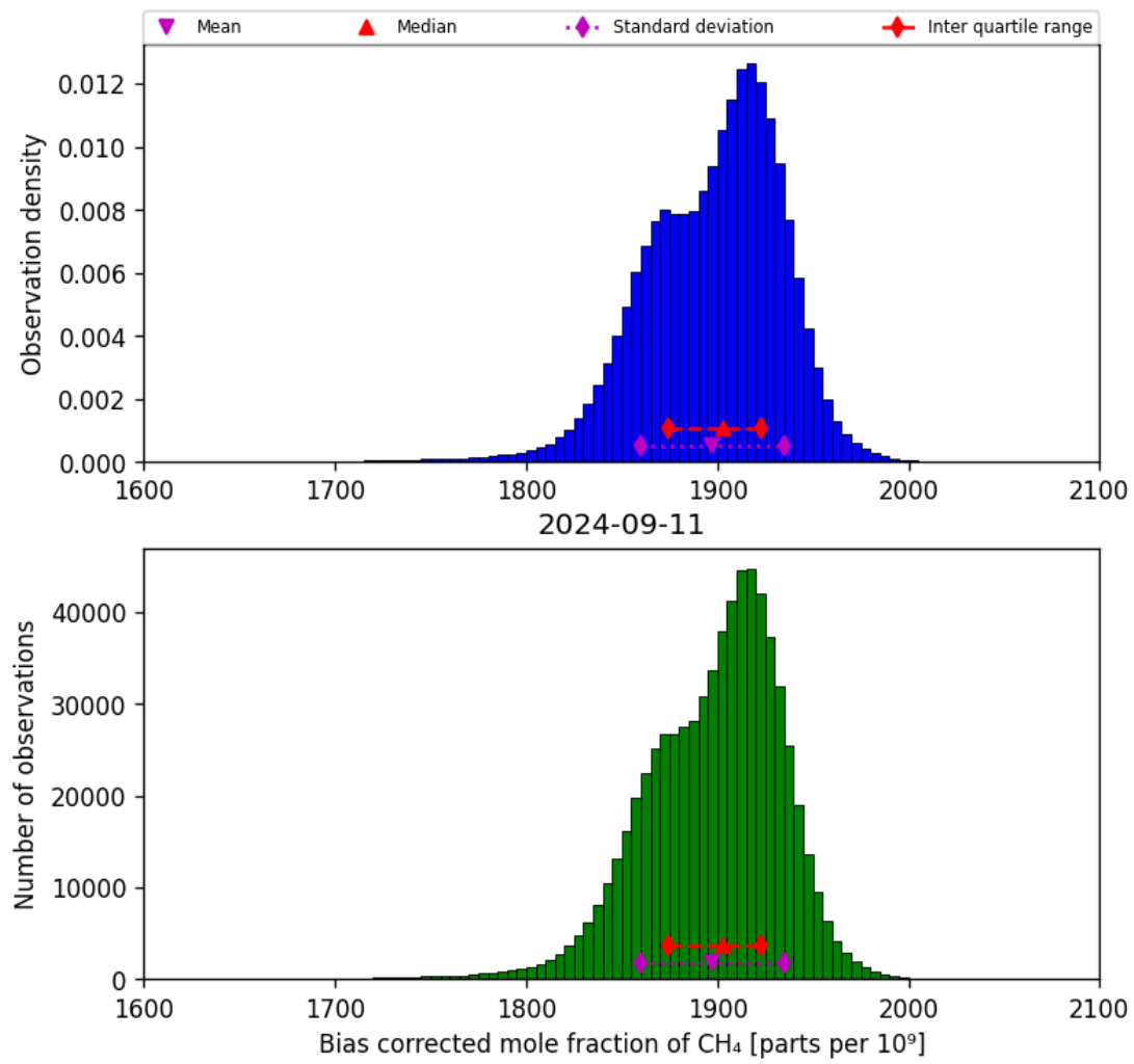
Figure 25: Histogram of “Bias corrected mole fraction of CH 4 ” for 2024-09-10 to 2024-09-12
