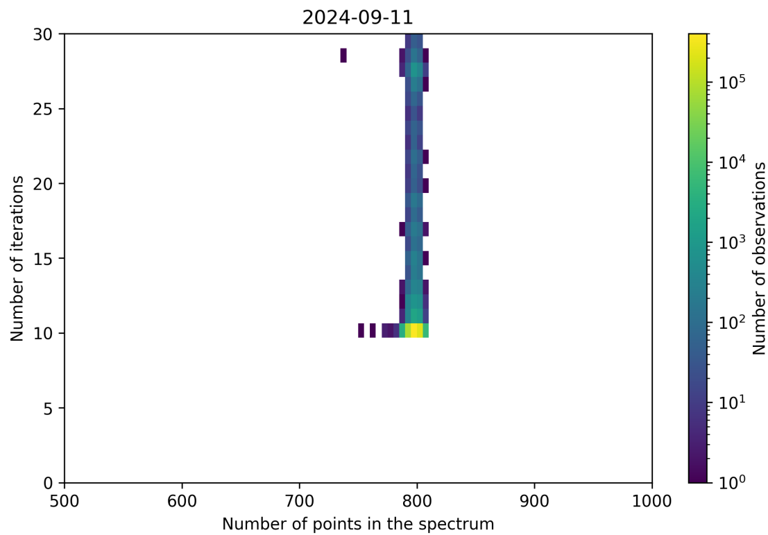
Figure 92: Scatter density plot of “Number of points in the spectrum” against “Number of iterations” for 2024-09-10 to 2024-09-12.
