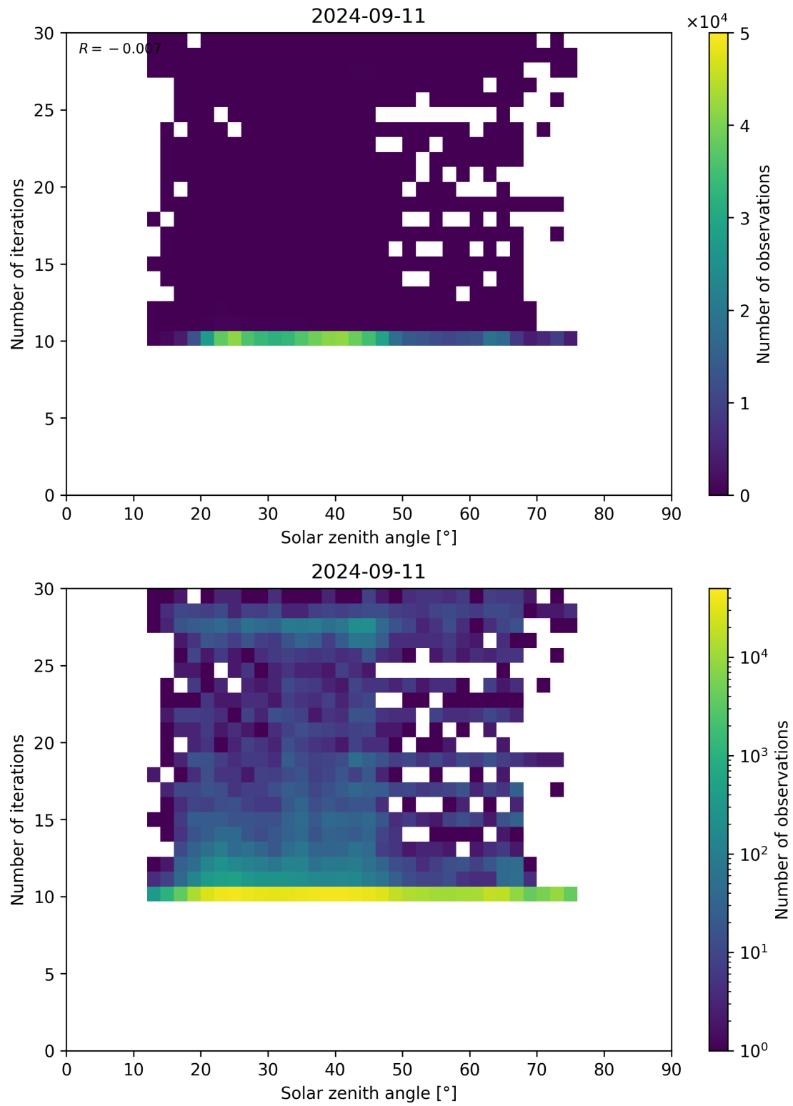
Figure 102: Scatter density plot of “Solar zenith angle” against “Number of iterations” for 2024-09-10 to 2024-09-12.
