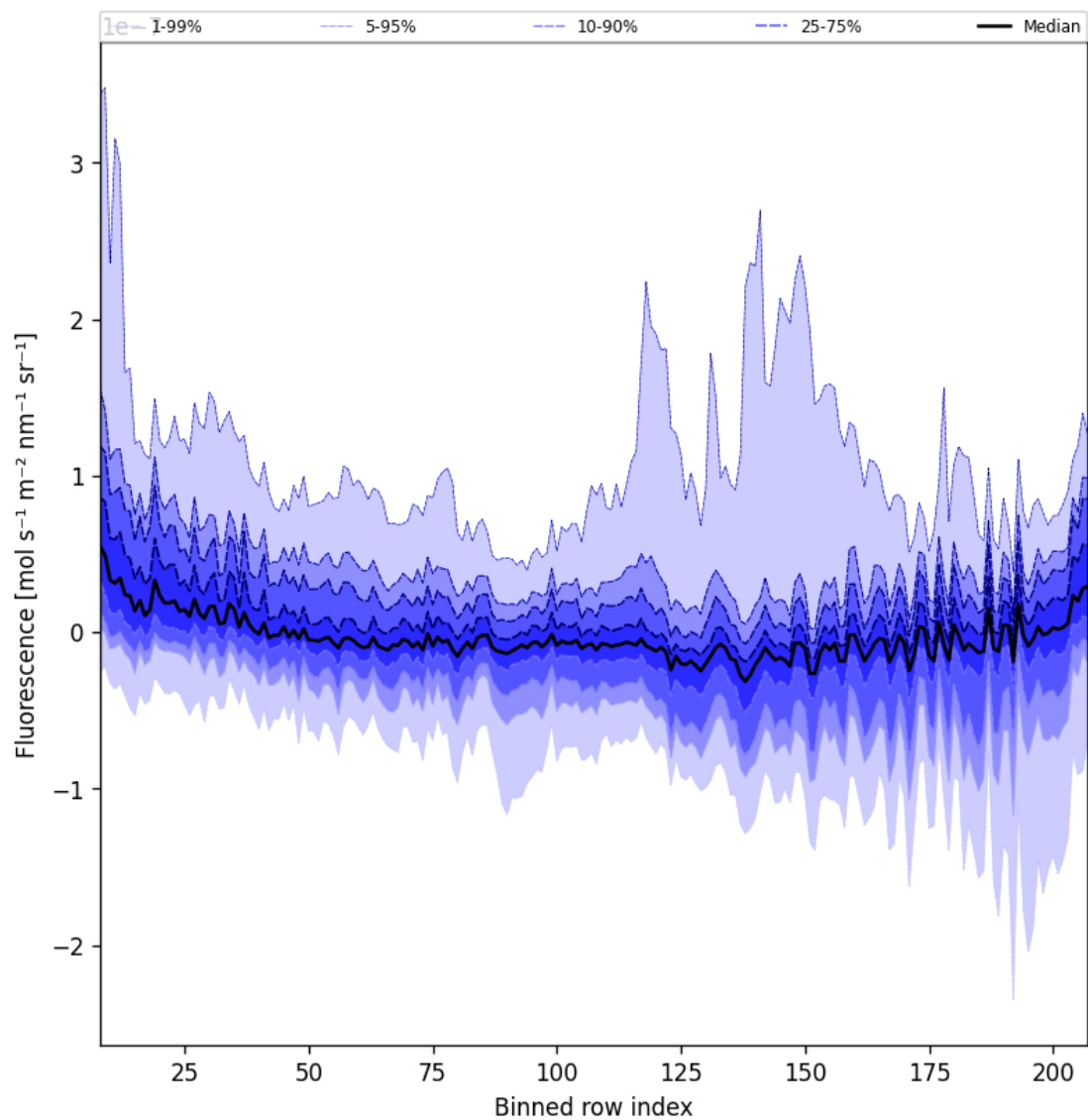
Figure 43: Along track statistics of “Fluorescence” for 2024-09-10 to 2024-09-12
