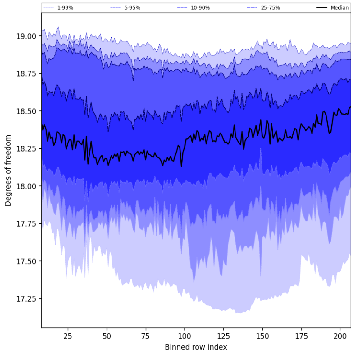
Figure 41: Along track statistics of “Degrees of freedom” for 2024-09-10 to 2024-09-12
