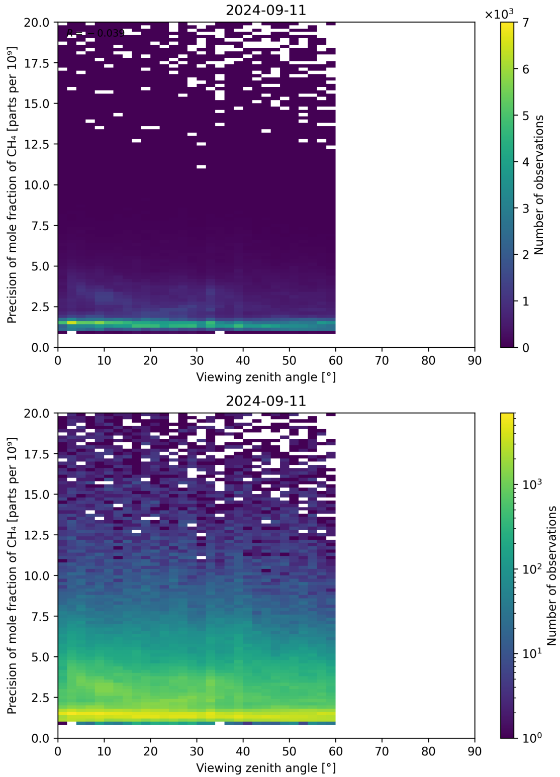
Figure 112: Scatter density plot of “Viewing zenith angle” against “Precision of mole fraction of CH 4 ” for 2024-09-10 to 2024-09-12.
