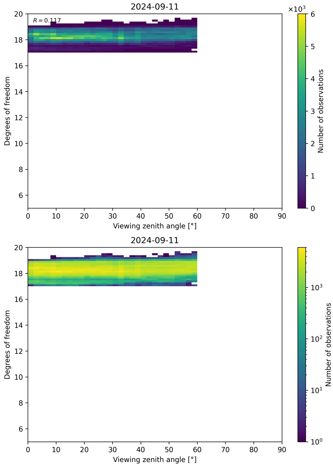
Figure 107: Scatter density plot of “Viewing zenith angle” against “Degrees of freedom” for 2024-09-10 to 2024-09-12.
