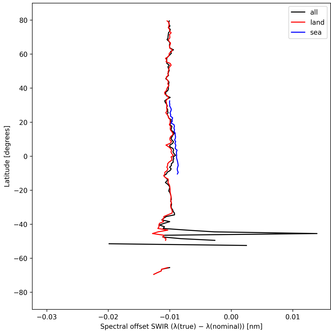
Figure 16: Zonal average of “Spectral offset SWIR ( \lambda_{\text{true}} - \lambda_{\text{nominal}} )” for 2024-09-10 to 2024-09-12.
