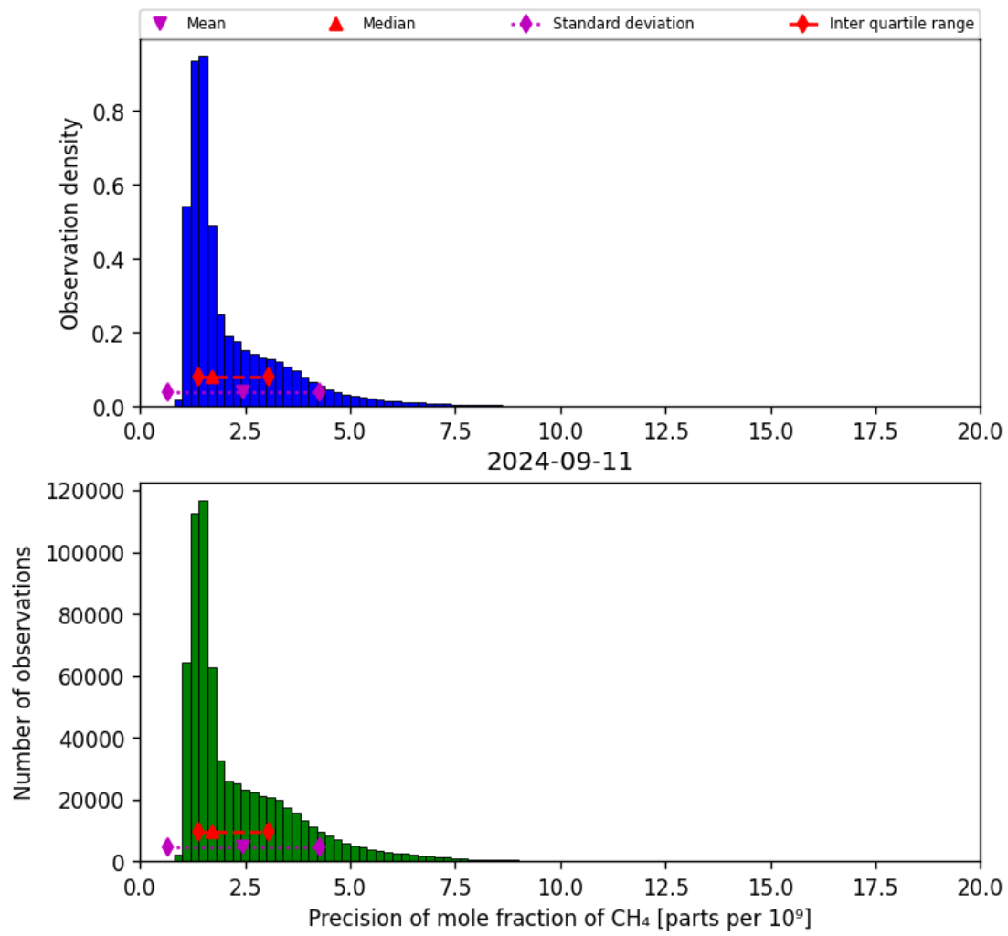
Figure 24: Histogram of “Precision of mole fraction of CH 4 ” for 2024-09-10 to 2024-09-12
