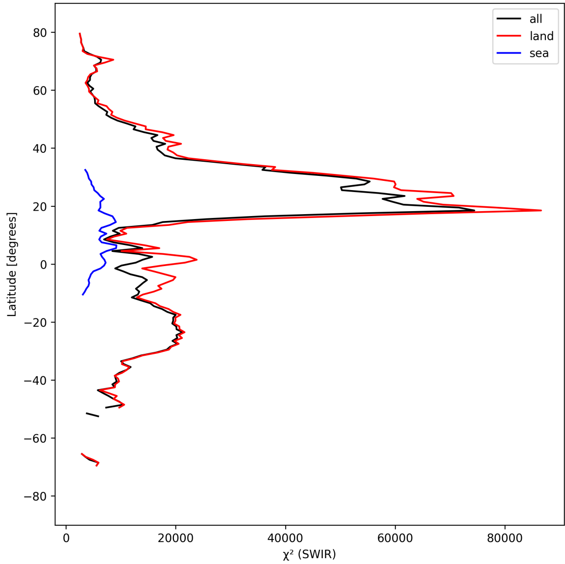
Figure 17: Zonal average of “ \chi^2 (SWIR)” for 2024-09-10 to 2024-09-12.
