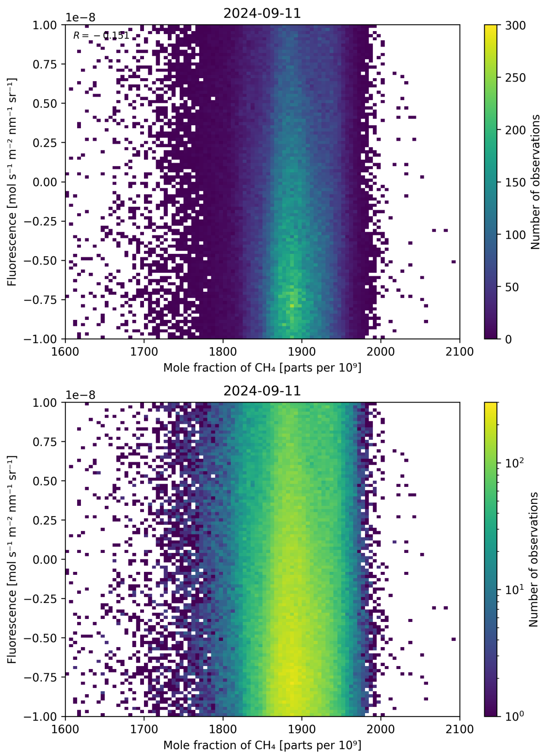
Figure 73: Scatter density plot of “Mole fraction of \text{CH}_4 ” against “Fluorescence” for 2024-09-10 to 2024-09-12.
