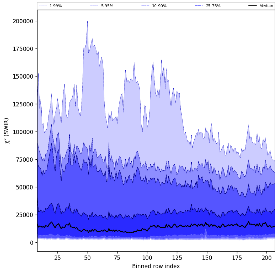
Figure 39: Along track statistics of “ \chi^2 (SWIR)” for 2024-09-10 to 2024-09-12
