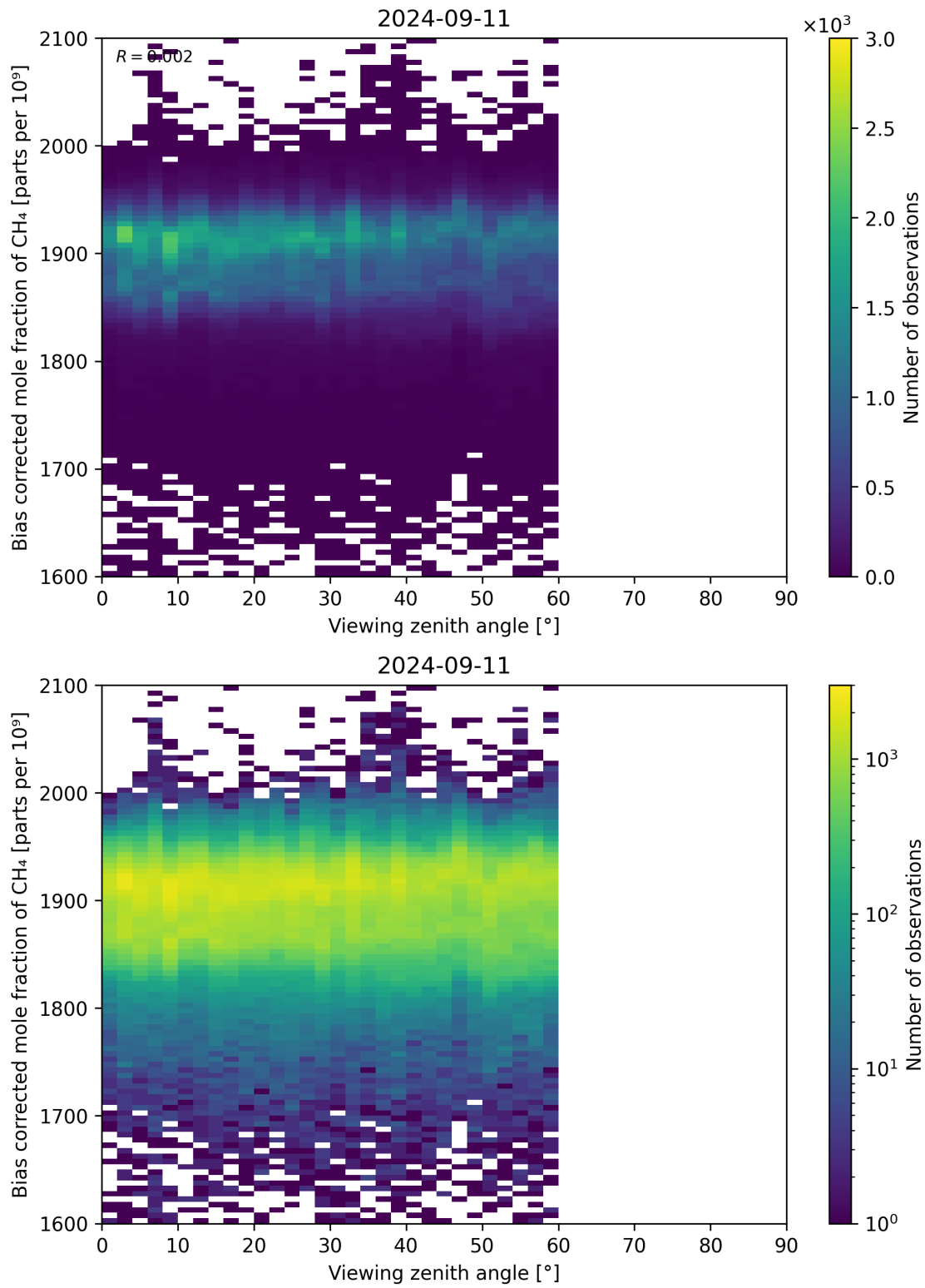
Figure 111: Scatter density plot of “Viewing zenith angle” against “Bias corrected mole fraction of CH 4 ” for 2024-09-10 to 2024-09-12.
