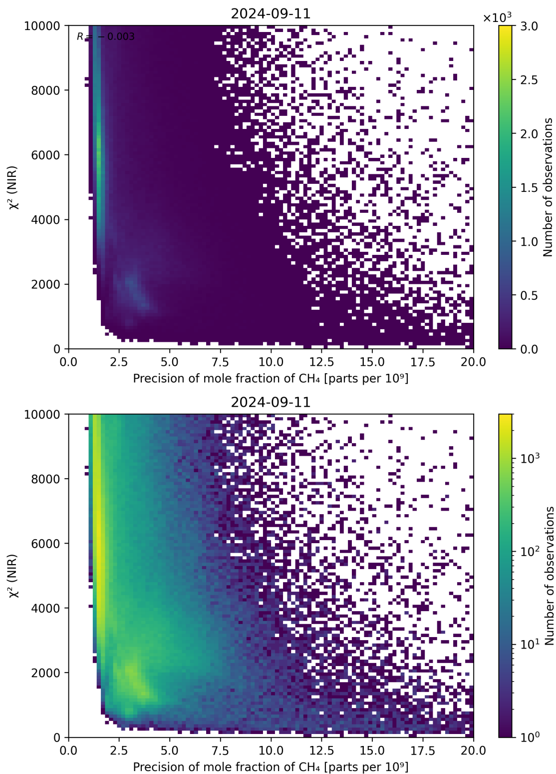
Figure 78: Scatter density plot of “Precision of mole fraction of CH 4 ” against “ \chi^2 (NIR)” for 2024-09-10 to 2024-09-12.
