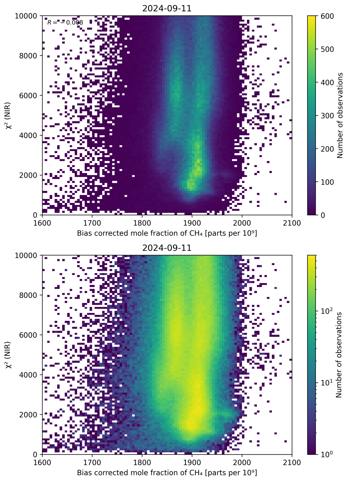
Figure 63: Scatter density plot of “Bias corrected mole fraction of CH 4 ” against “ \chi^2 (NIR)” for 2024-09-10 to 2024-09-12.
