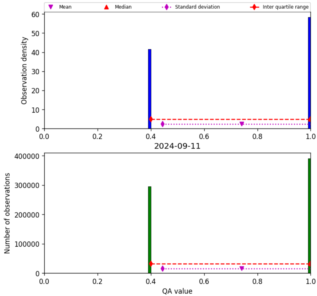
Figure 22: Histogram of “QA value” for 2024-09-10 to 2024-09-12
