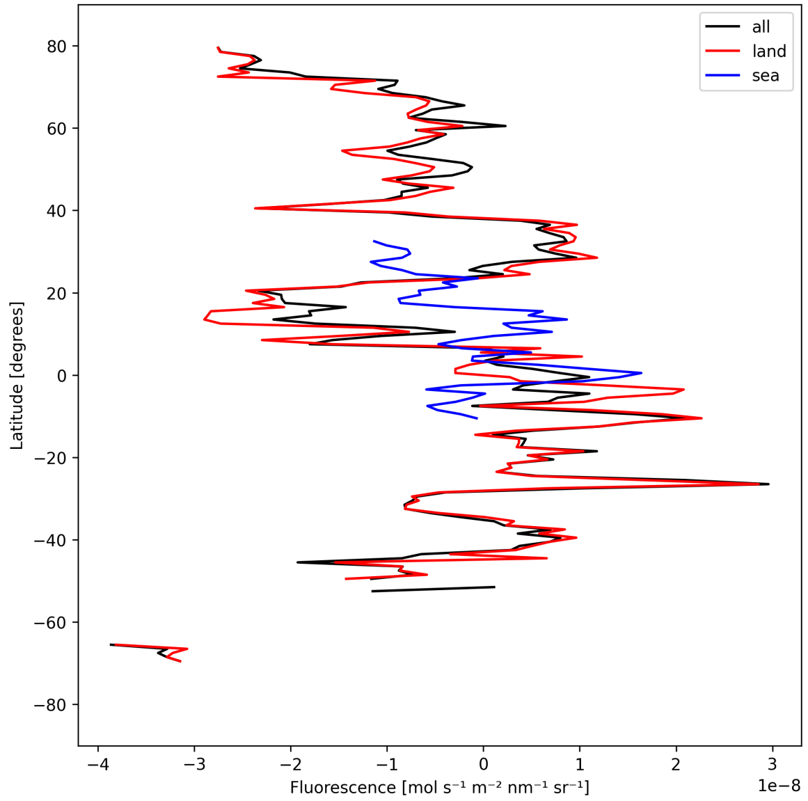
Figure 21: Zonal average of “Fluorescence” for 2024-09-10 to 2024-09-12.
