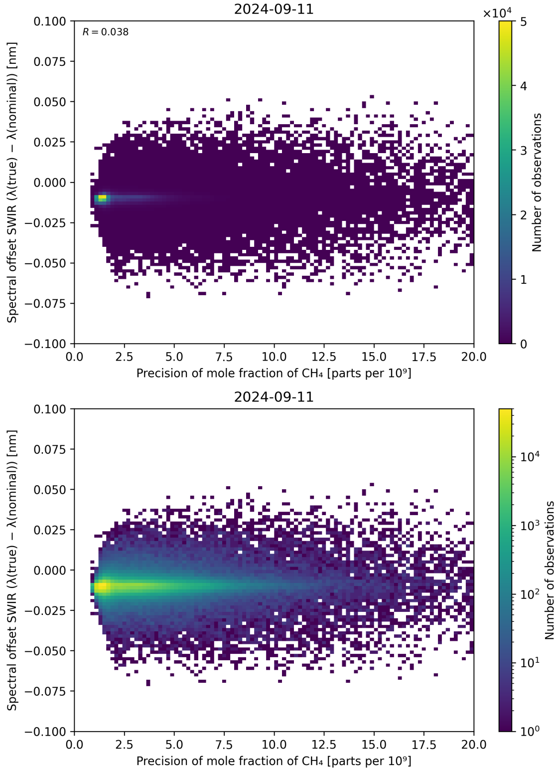
Figure 85: Scatter density plot of “Precision of mole fraction of \text{CH}_4 ” against “Spectral offset SWIR ( \lambda_{\text{true}} - \lambda_{\text{nominal}} )” for 2024-09-10 to 2024-09-12.
