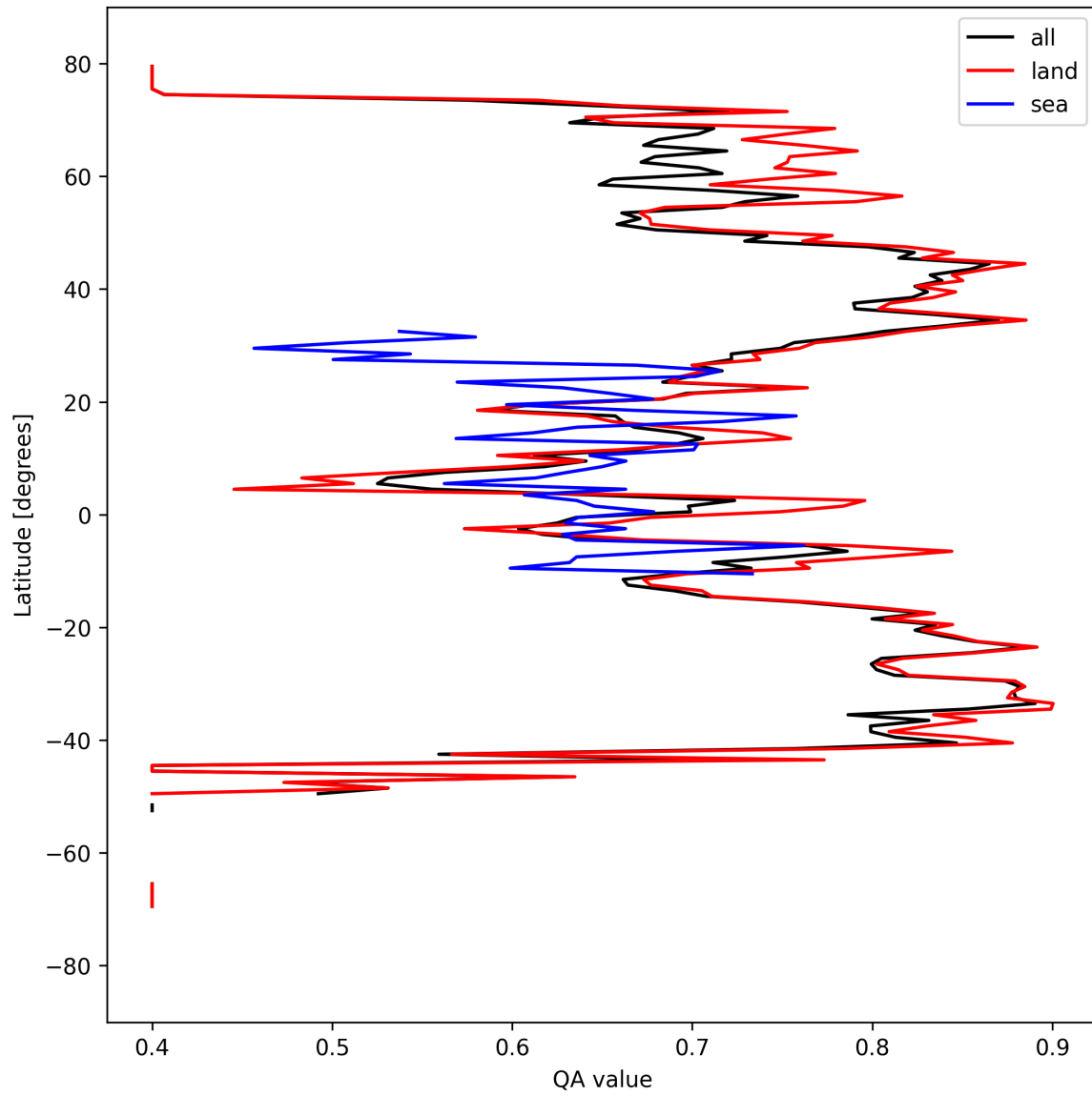
Figure 11: Zonal average of “QA value” for 2024-09-10 to 2024-09-12.
