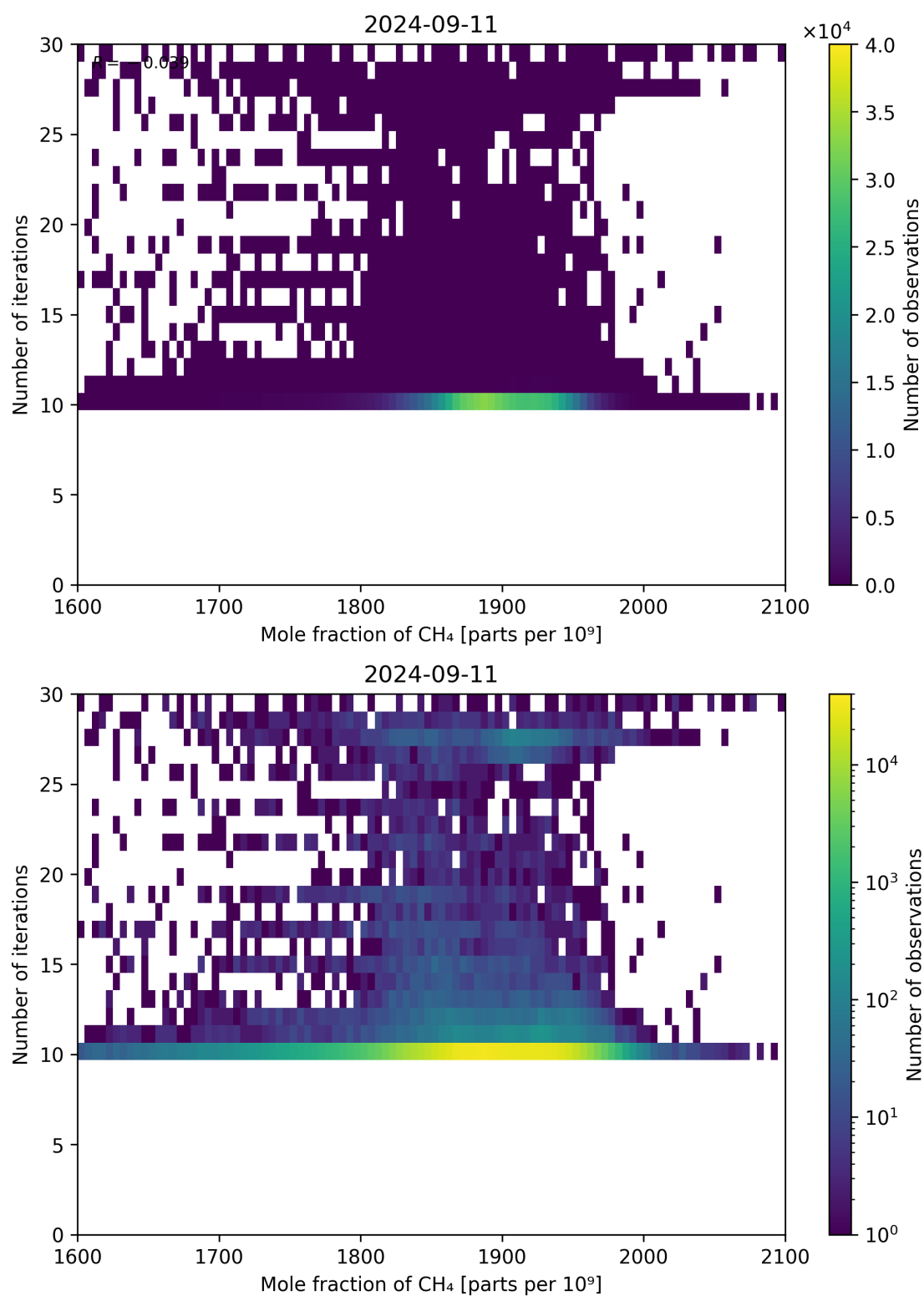
Figure 76: Scatter density plot of “Mole fraction of CH 4 ” against “Number of iterations” for 2024-09-10 to 2024-09-12.
