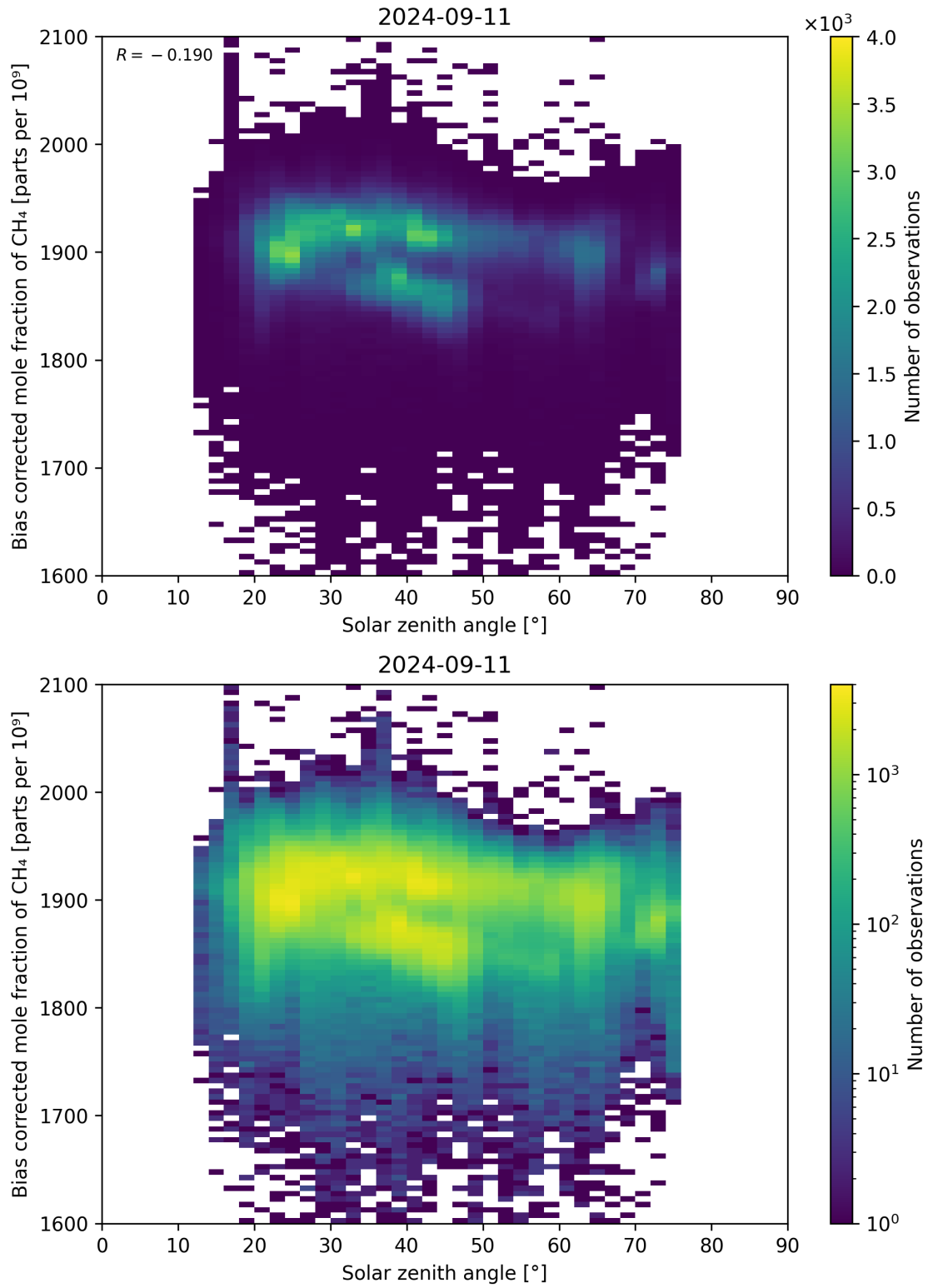
Figure 100: Scatter density plot of “Solar zenith angle” against “Bias corrected mole fraction of CH 4 ” for 2024-09-10 to 2024-09-12.
