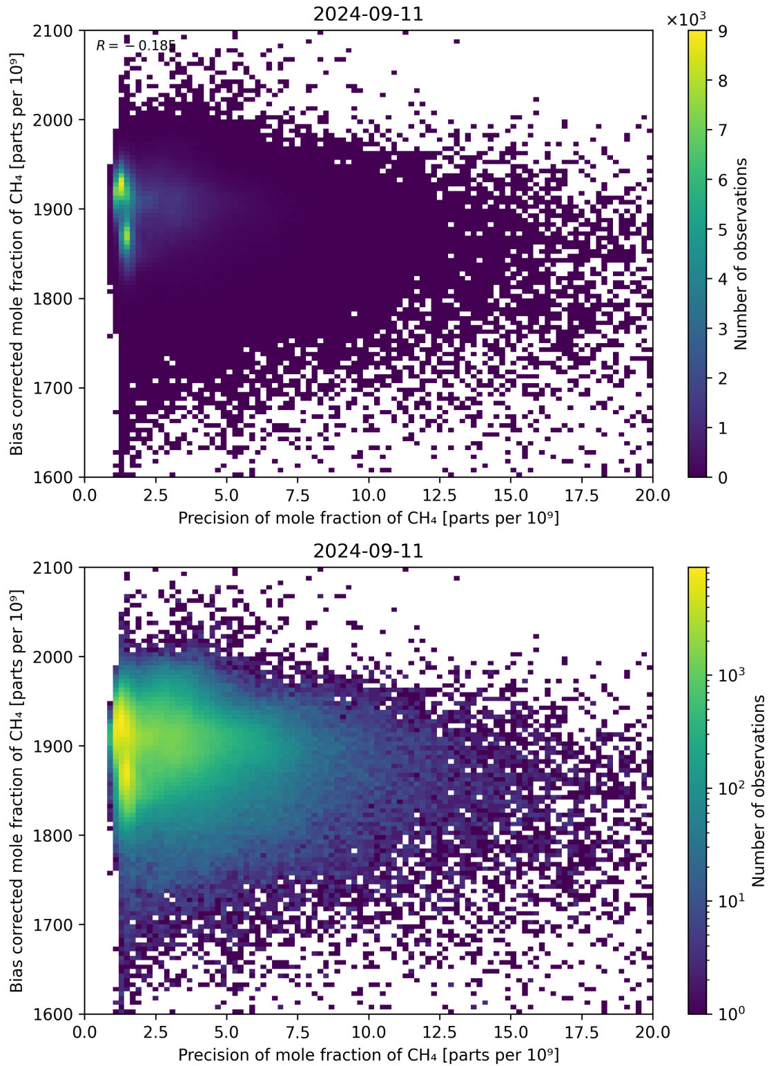
Figure 82: Scatter density plot of “Precision of mole fraction of CH 4 ” against “Bias corrected mole fraction of CH 4 ” for 2024-09-10 to 2024-09-12.
