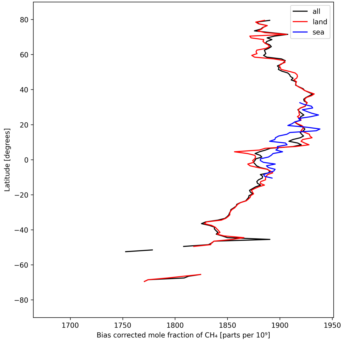
Figure 14: Zonal average of “Bias corrected mole fraction of \text{CH}_4 ” for 2024-09-10 to 2024-09-12.
