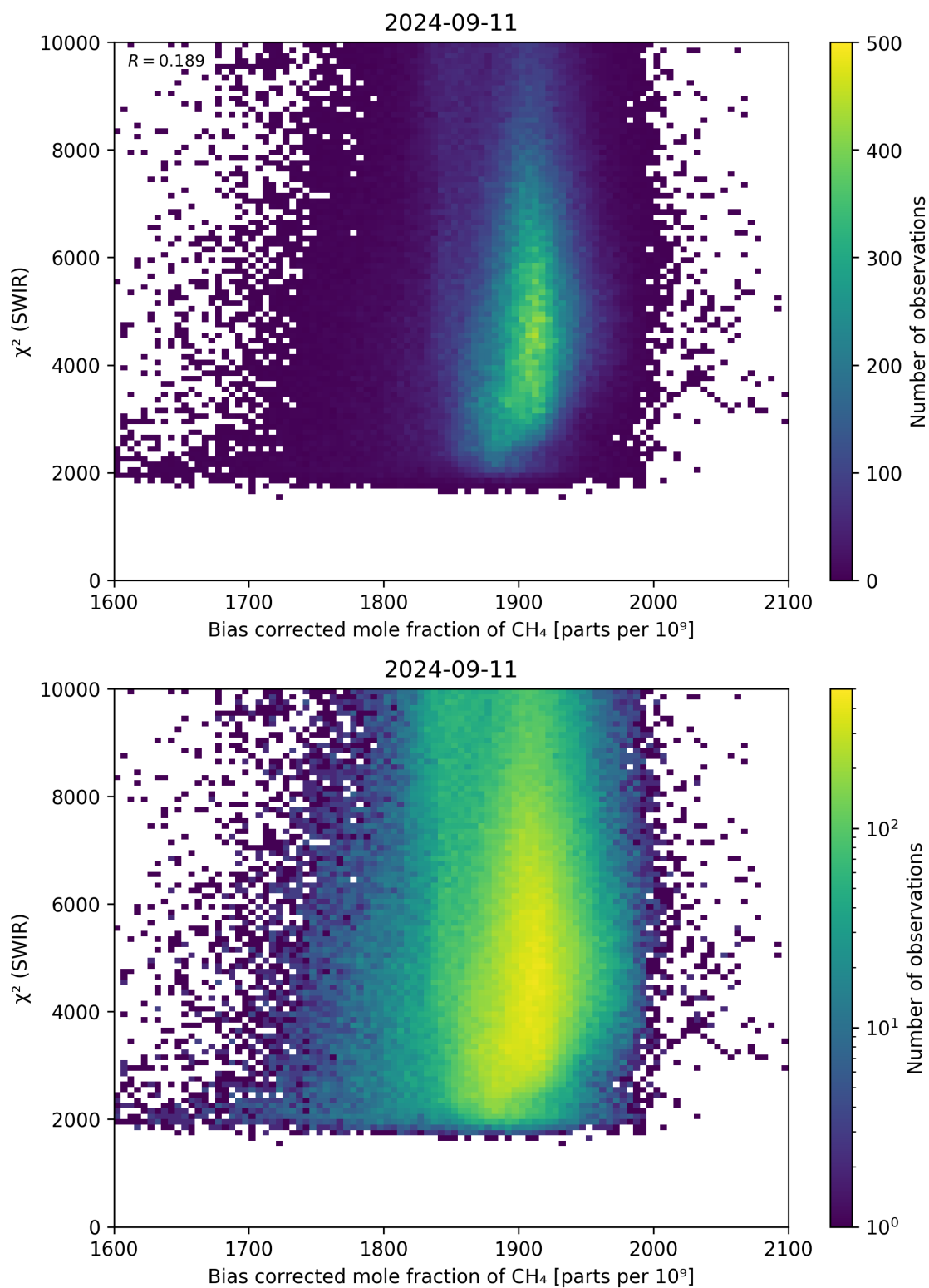
Figure 64: Scatter density plot of “Bias corrected mole fraction of \text{CH}_4 ” against “ \chi^2 (SWIR)” for 2024-09-10 to 2024-09-12.
