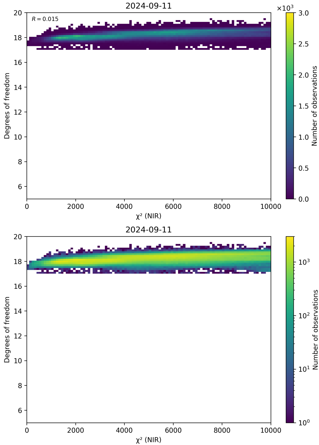
Figure 44: Scatter density plot of “ \chi^2 (NIR)” against “Degrees of freedom” for 2024-09-10 to 2024-09-12.
