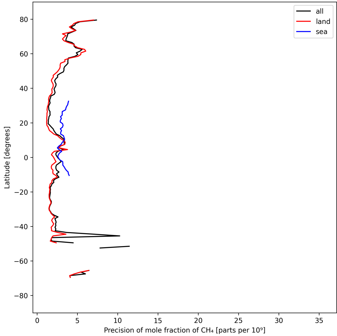
Figure 13: Zonal average of “Precision of mole fraction of CH 4 ” for 2024-09-10 to 2024-09-12.
