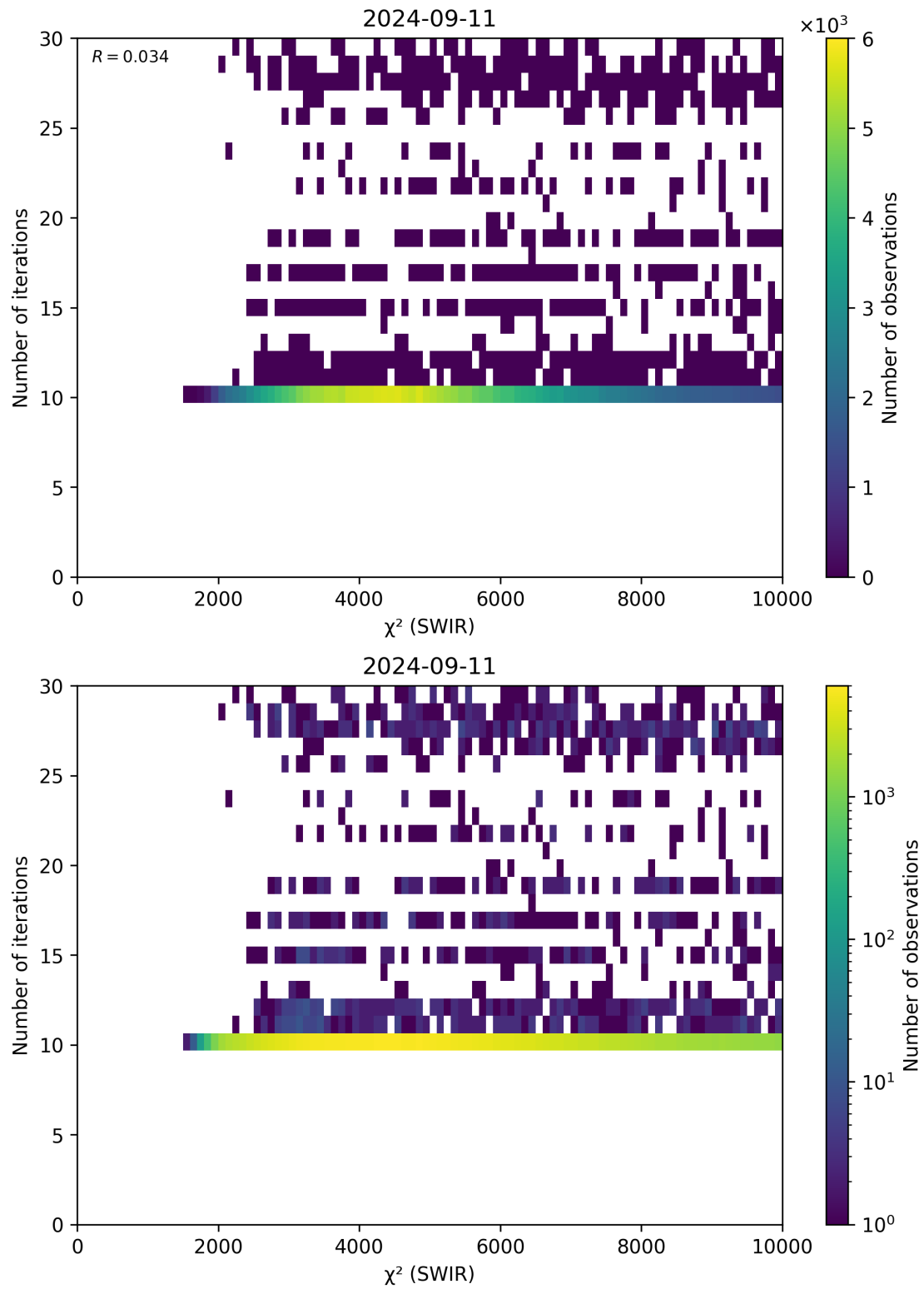
Figure 50: Scatter density plot of “ \chi^2 (SWIR)” against “Number of iterations” for 2024-09-10 to 2024-09-12.
