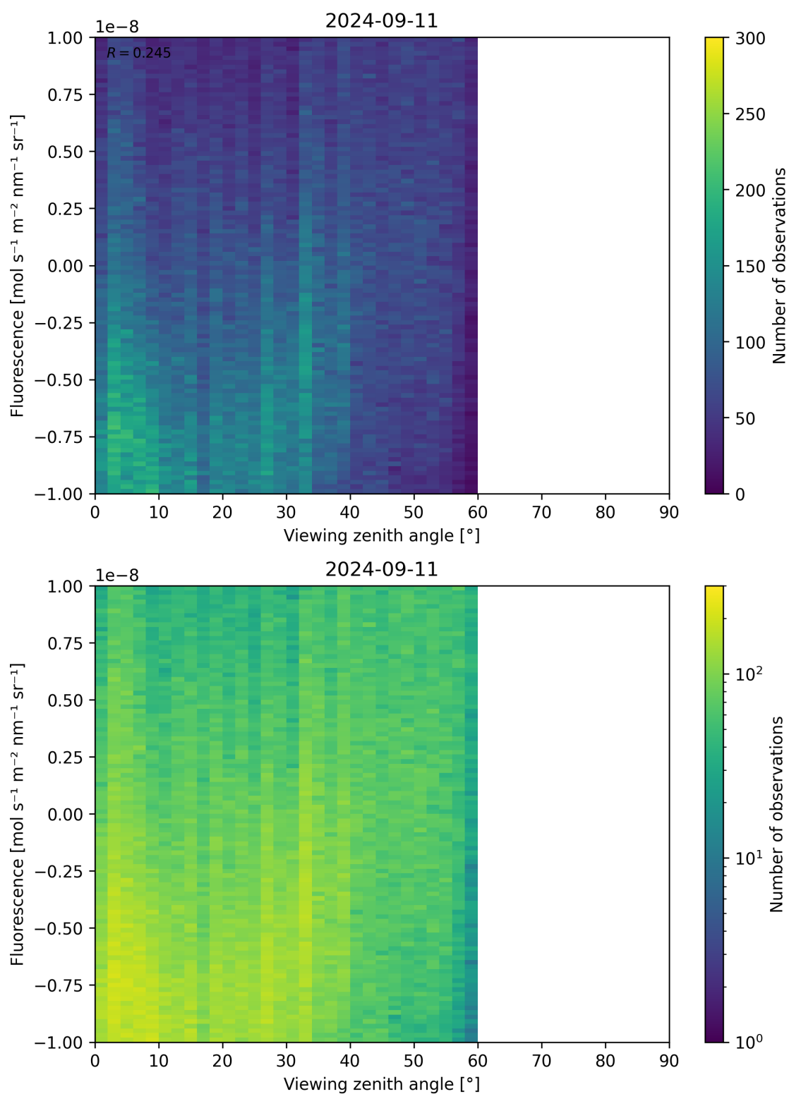
Figure 108: Scatter density plot of “Viewing zenith angle” against “Fluorescence” for 2024-09-10 to 2024-09-12.
