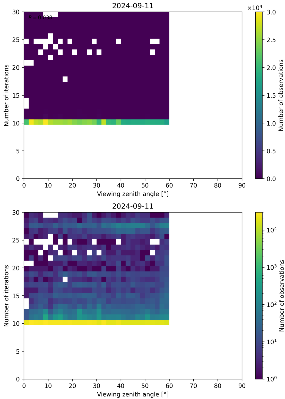
Figure 113: Scatter density plot of “Viewing zenith angle” against “Number of iterations” for 2024-09-10 to 2024-09-12.
