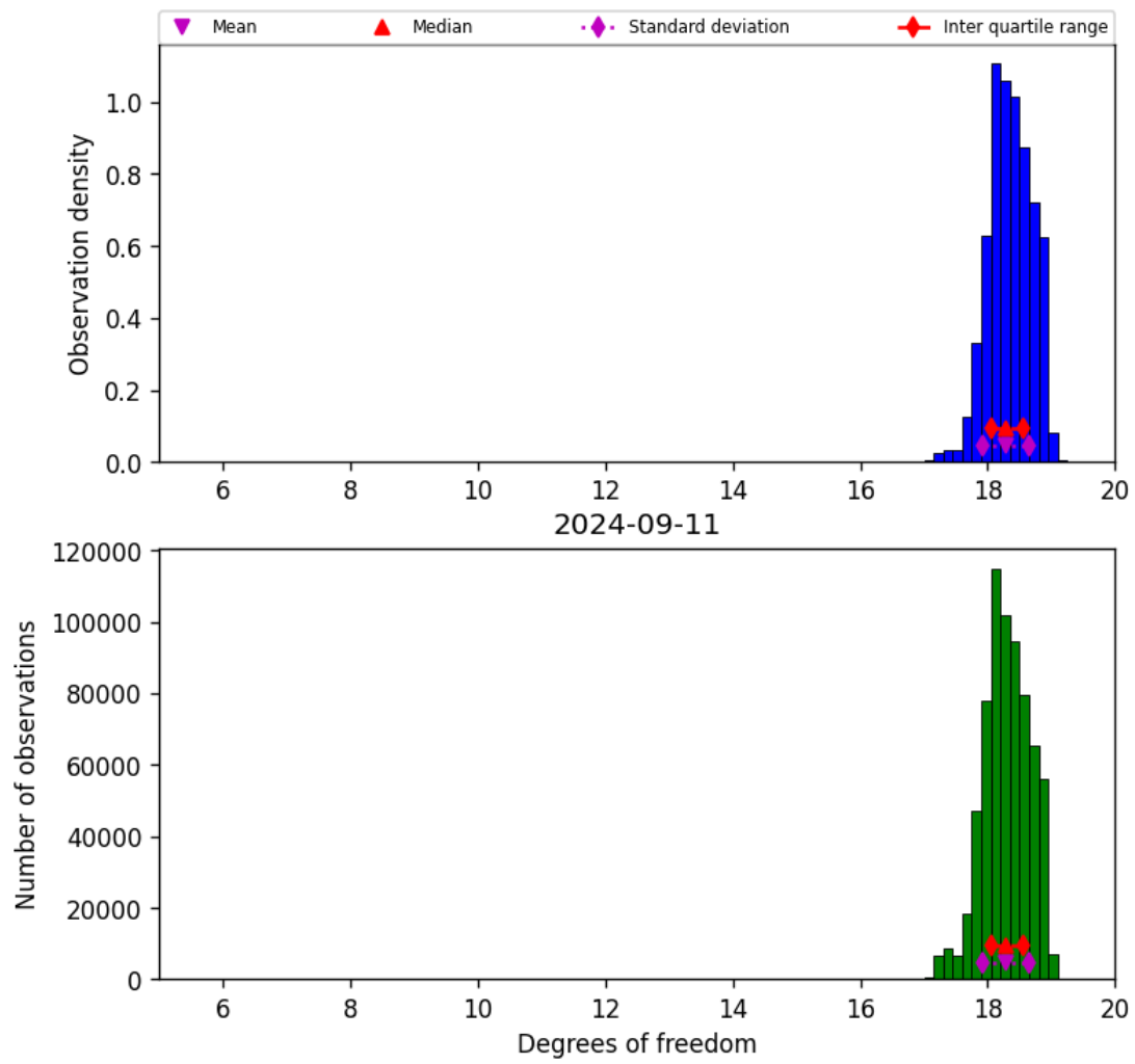
Figure 30: Histogram of “Degrees of freedom” for 2024-09-10 to 2024-09-12
