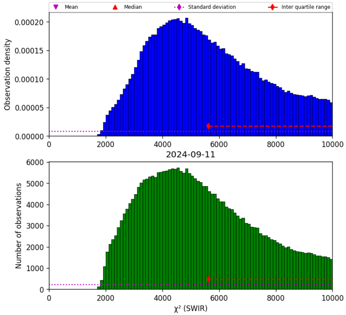
Figure 28: Histogram of “ \chi^2 (SWIR)” for 2024-09-10 to 2024-09-12
