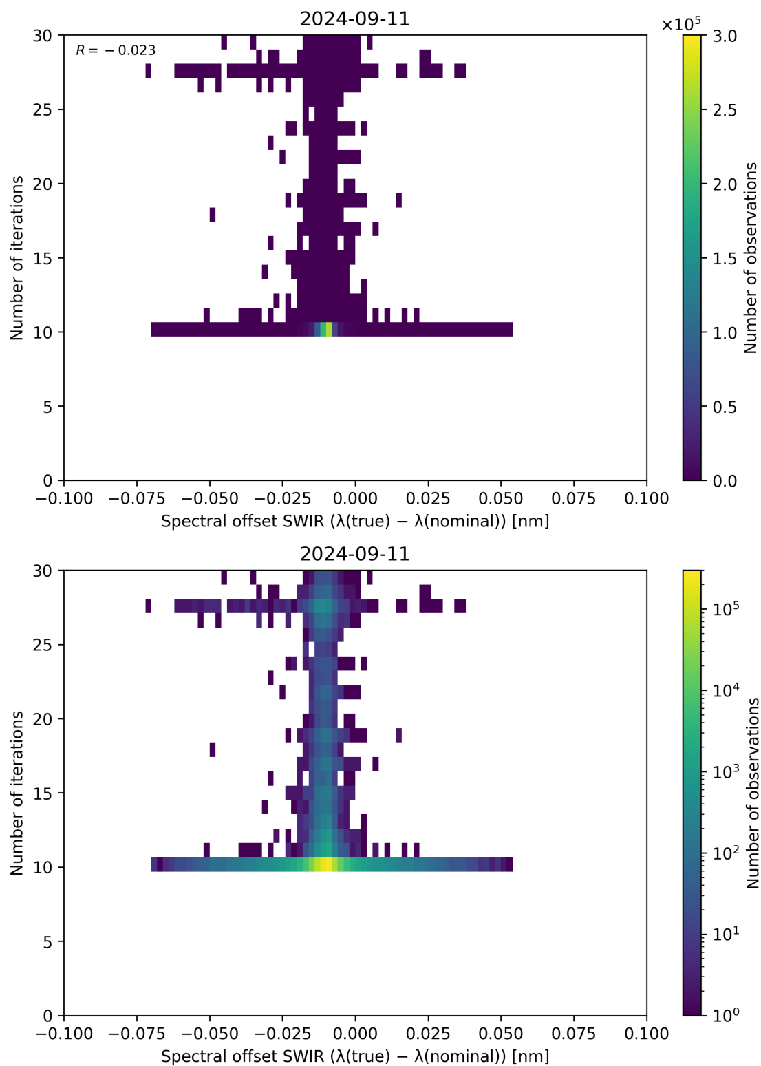
Figure 121: Scatter density plot of “Spectral offset SWIR ( \lambda_{\text{true}} - \lambda_{\text{nominal}} )” against “Number of iterations” for 2024-09-10 to 2024-09-12.
