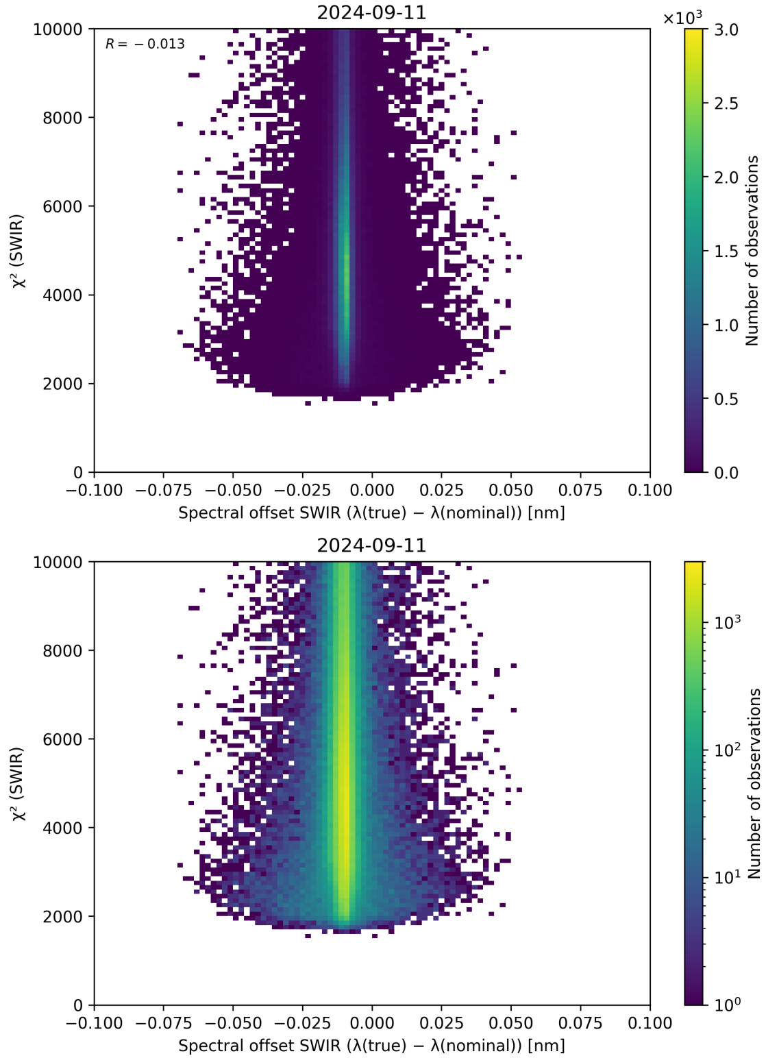
Figure 118: Scatter density plot of “Spectral offset SWIR ( \lambda_{\text{true}} - \lambda_{\text{nominal}} )” against “ \chi^2 (SWIR)” for 2024-09-10 to 2024-09-12.
