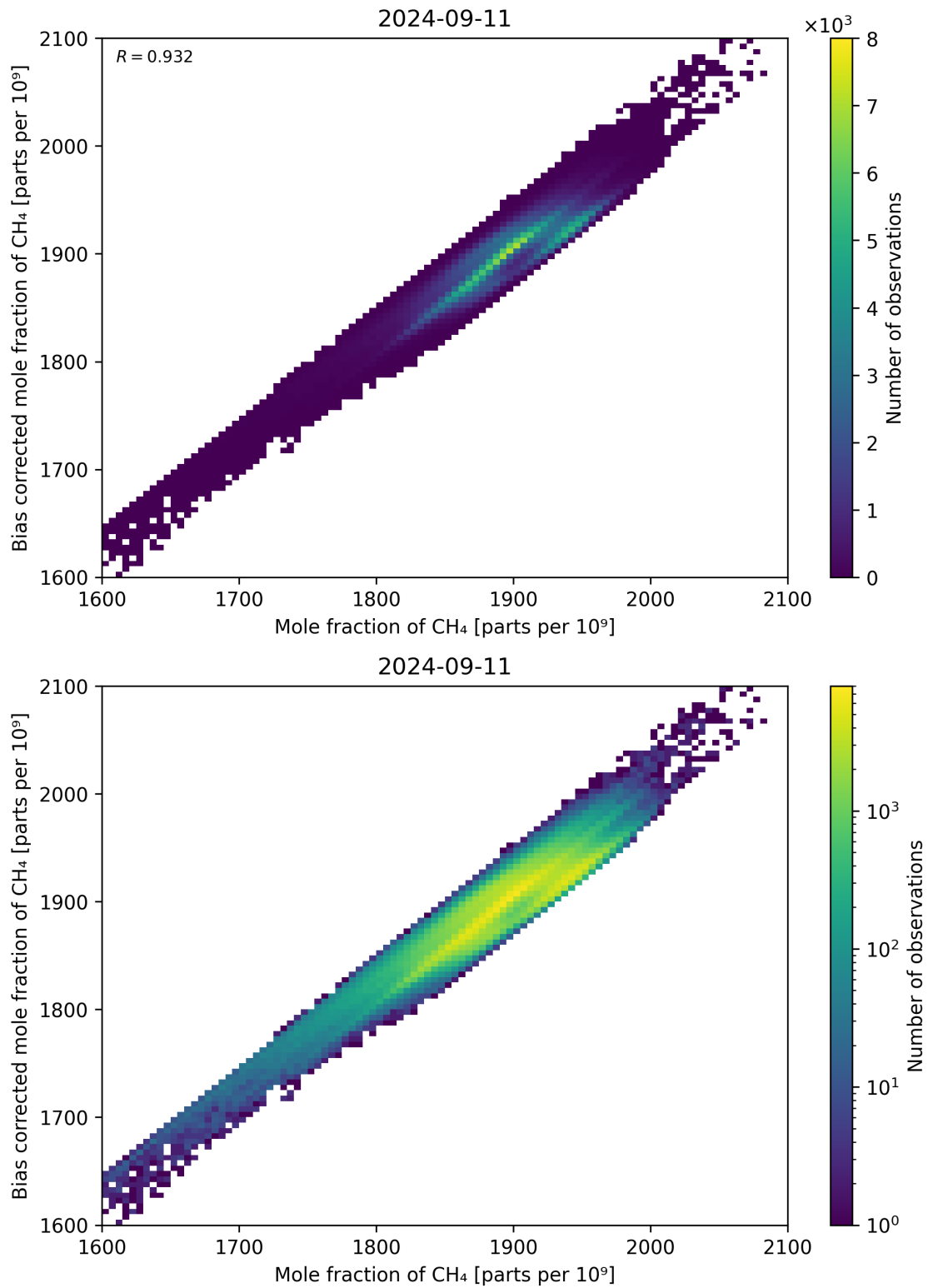
Figure 74: Scatter density plot of “Mole fraction of CH 4 ” against “Bias corrected mole fraction of CH 4 ” for 2024-09-10 to 2024-09-12.
