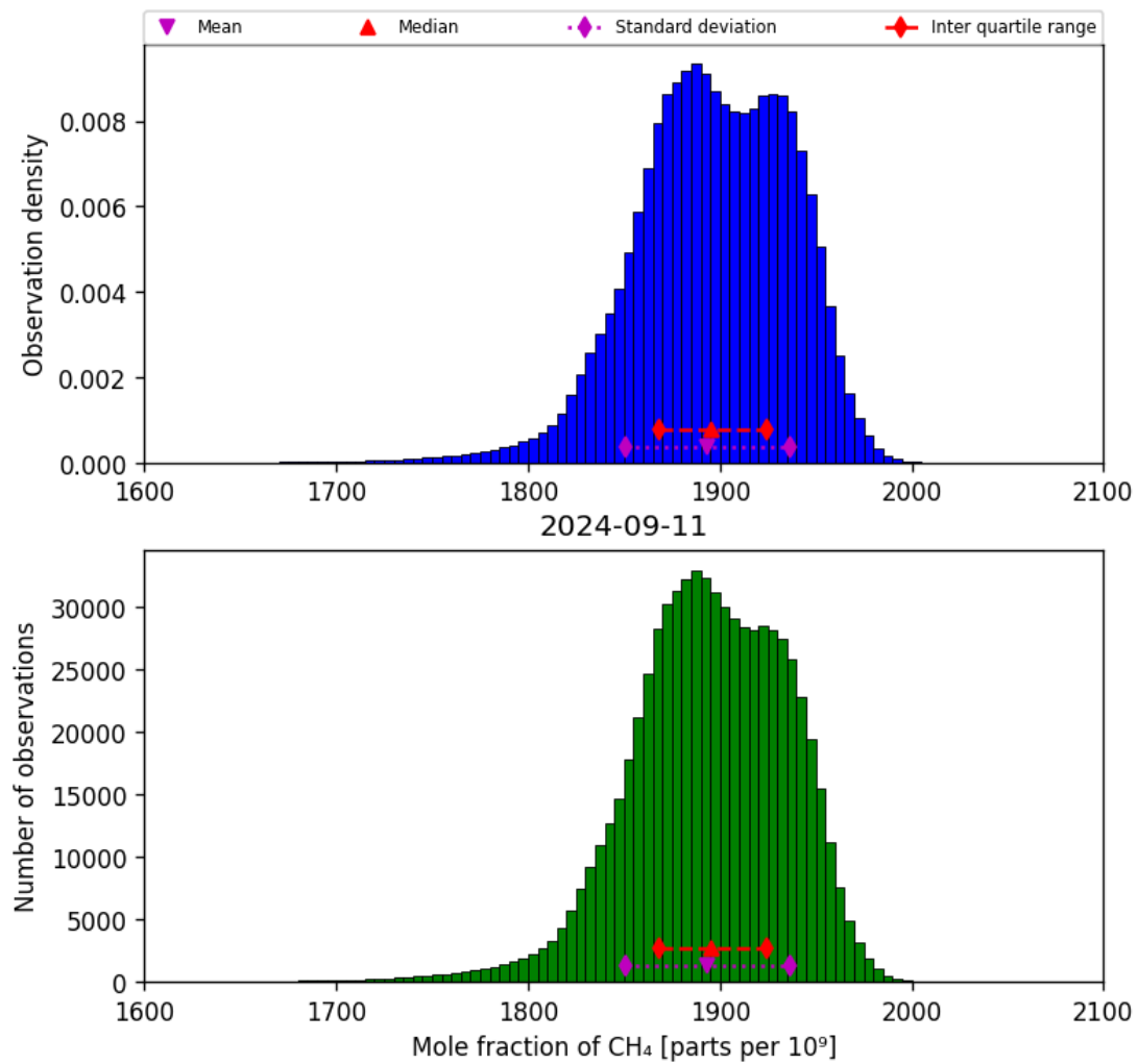
Figure 23: Histogram of “Mole fraction of CH 4 ” for 2024-09-10 to 2024-09-12
