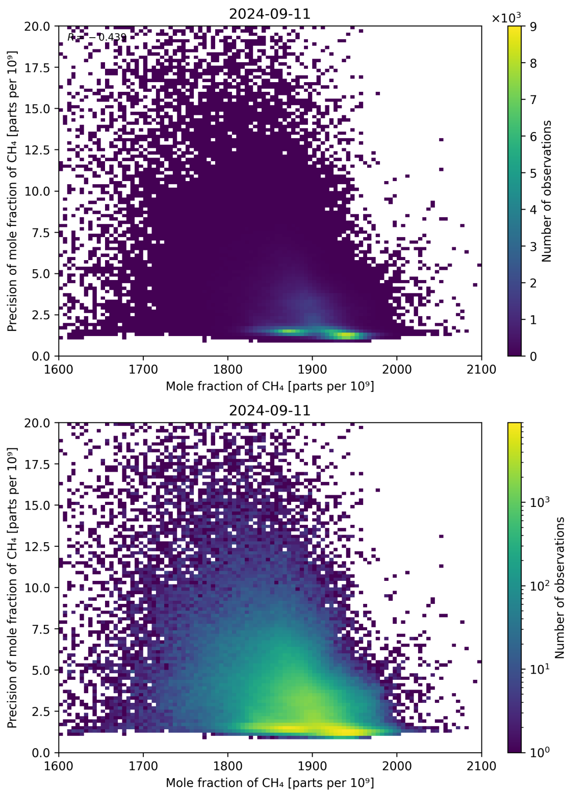
Figure 75: Scatter density plot of “Mole fraction of CH 4 ” against “Precision of mole fraction of CH 4 ” for 2024-09-10 to 2024-09-12.
