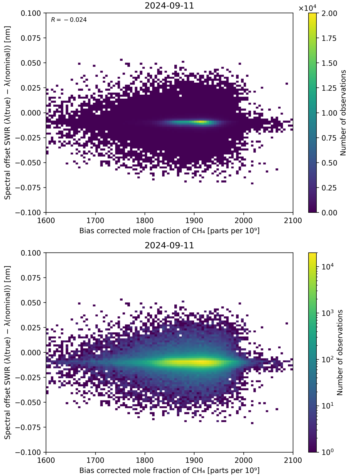
Figure 69: Scatter density plot of “Bias corrected mole fraction of \text{CH}_4 ” against “Spectral offset SWIR ( \lambda_{\text{true}} - \lambda_{\text{nominal}} )” for 2024-09-10 to 2024-09-12.
