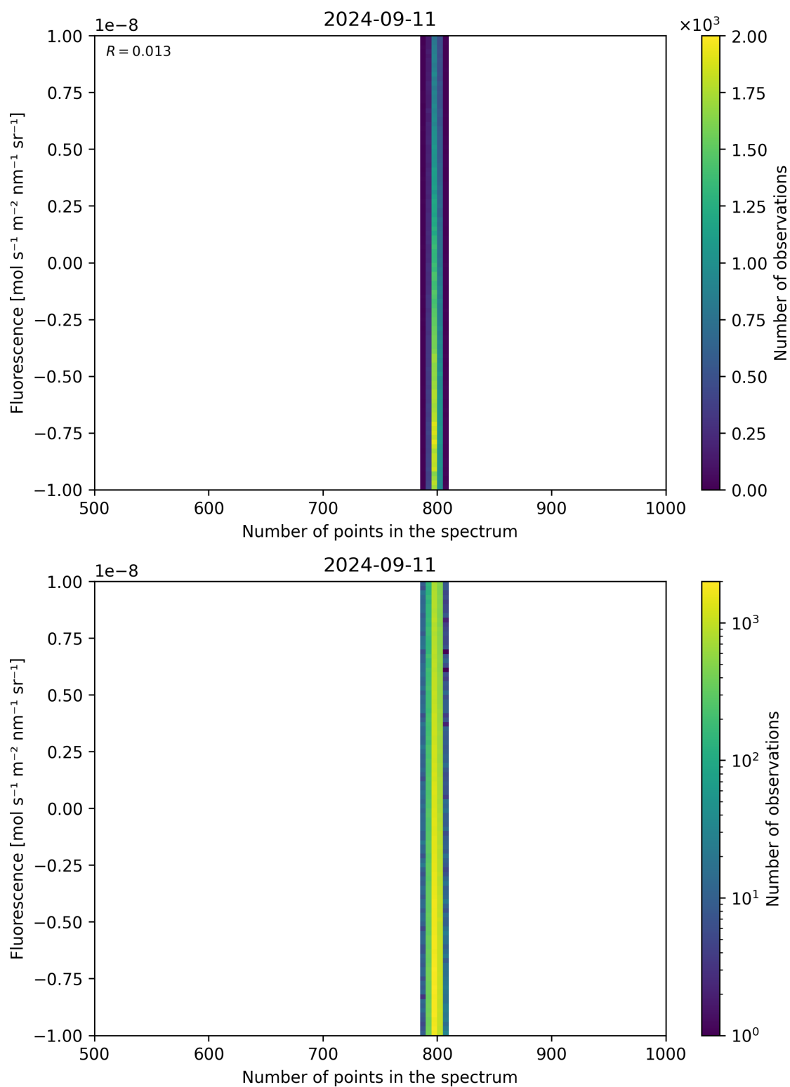
Figure 91: Scatter density plot of “Number of points in the spectrum” against “Fluorescence” for 2024-09-10 to 2024-09-12.
