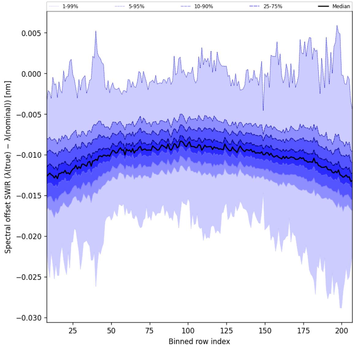
Figure 38: Along track statistics of “Spectral offset SWIR ( \lambda_{\text{true}} - \lambda_{\text{nominal}} )” for 2024-09-10 to 2024-09-12
