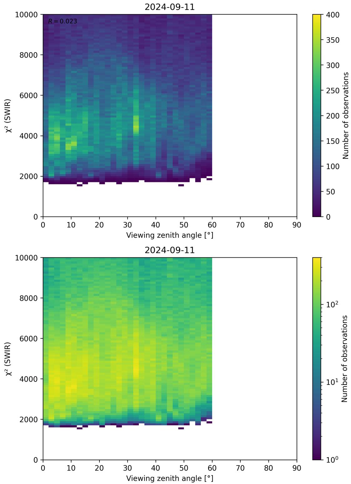
Figure 106: Scatter density plot of “Viewing zenith angle” against “ \chi^2 (SWIR)” for 2024-09-10 to 2024-09-12.
