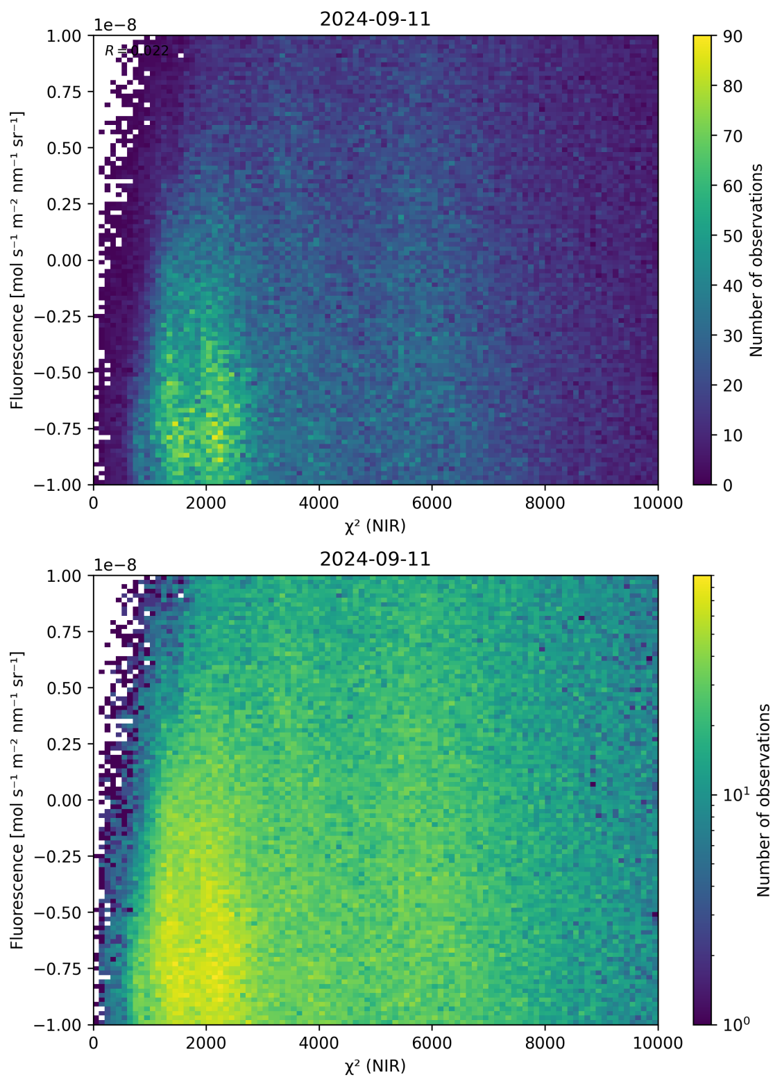
Figure 45: Scatter density plot of “ \chi^2 (NIR)” against “Fluorescence” for 2024-09-10 to 2024-09-12.
