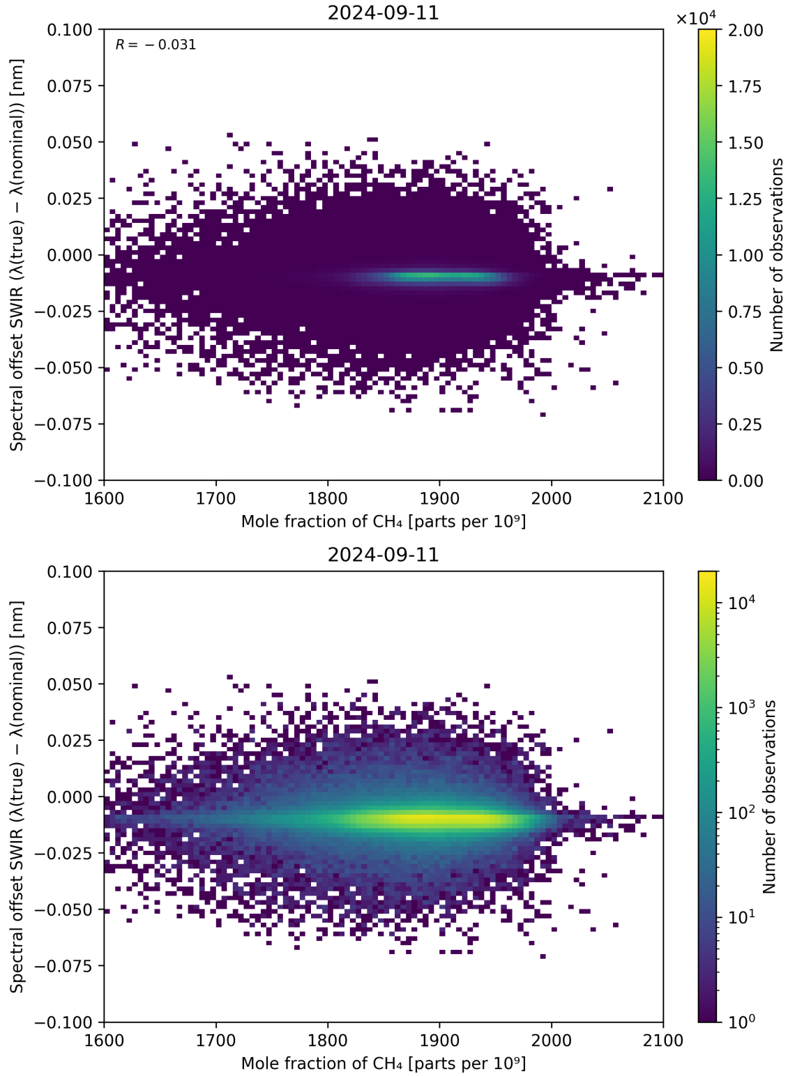
Figure 86: Scatter density plot of “Mole fraction of CH 4 ” against “Spectral offset SWIR ( \lambda_{\text{true}} - \lambda_{\text{nominal}} )” for 2024-09-10 to 2024-09-12.
