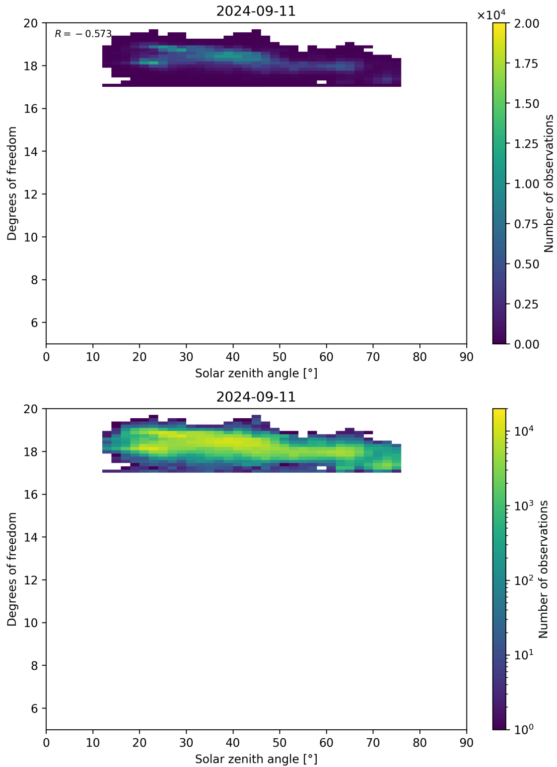
Figure 96: Scatter density plot of “Solar zenith angle” against “Degrees of freedom” for 2024-09-10 to 2024-09-12.
