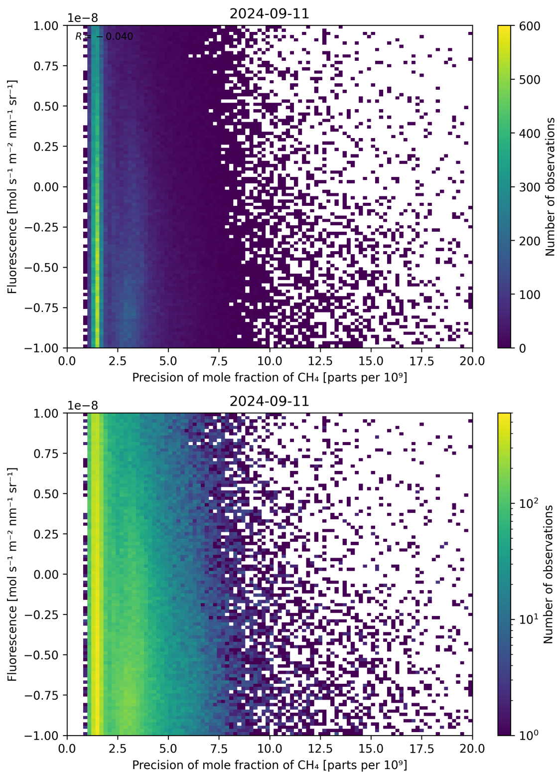
Figure 81: Scatter density plot of “Precision of mole fraction of \text{CH}_4 ” against “Fluorescence” for 2024-09-10 to 2024-09-12.
