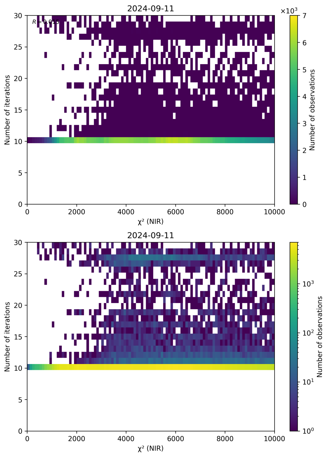
Figure 46: Scatter density plot of “ \chi^2 (NIR)” against “Number of iterations” for 2024-09-10 to 2024-09-12.
