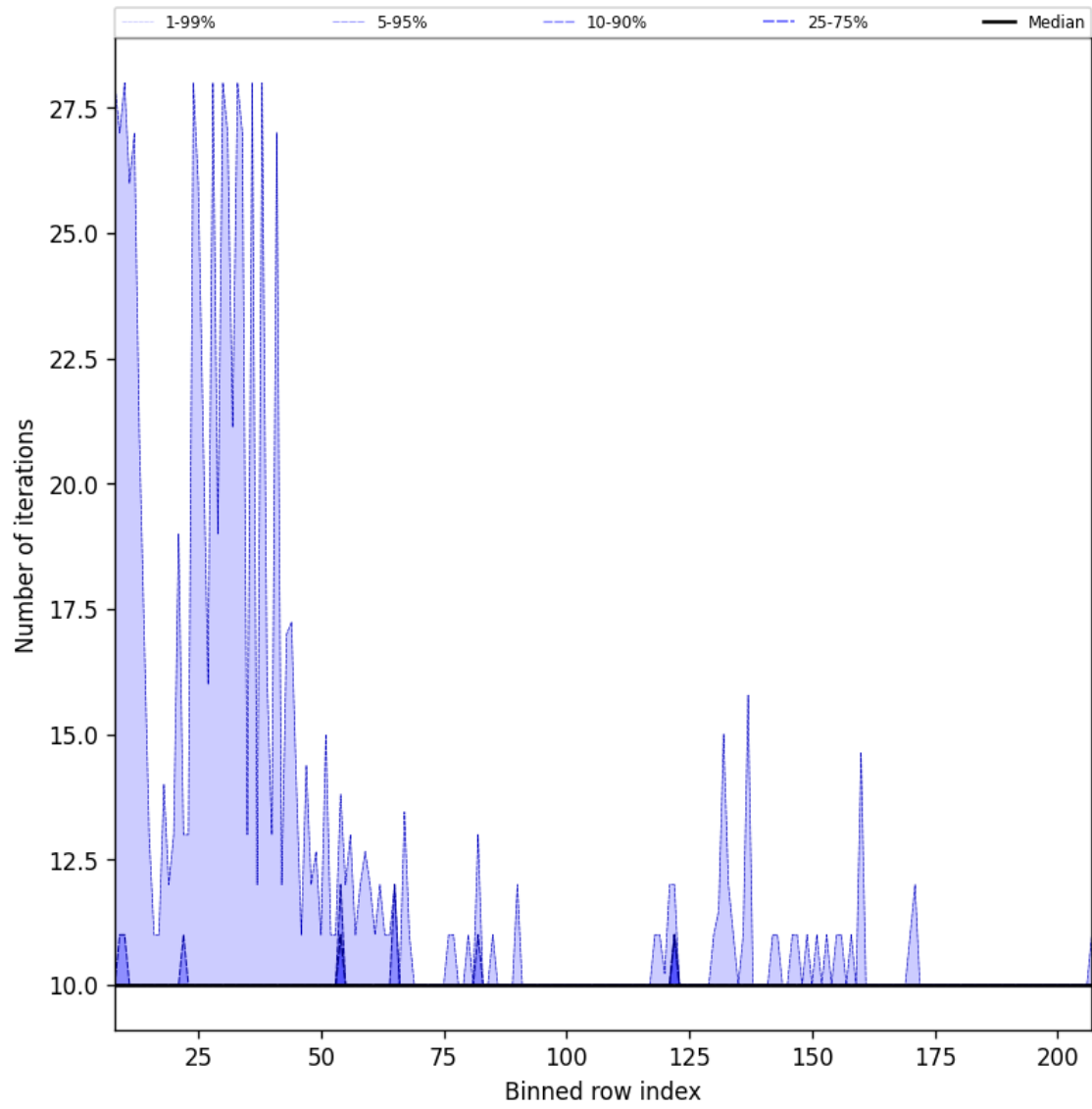
Figure 42: Along track statistics of “Number of iterations” for 2024-09-10 to 2024-09-12
