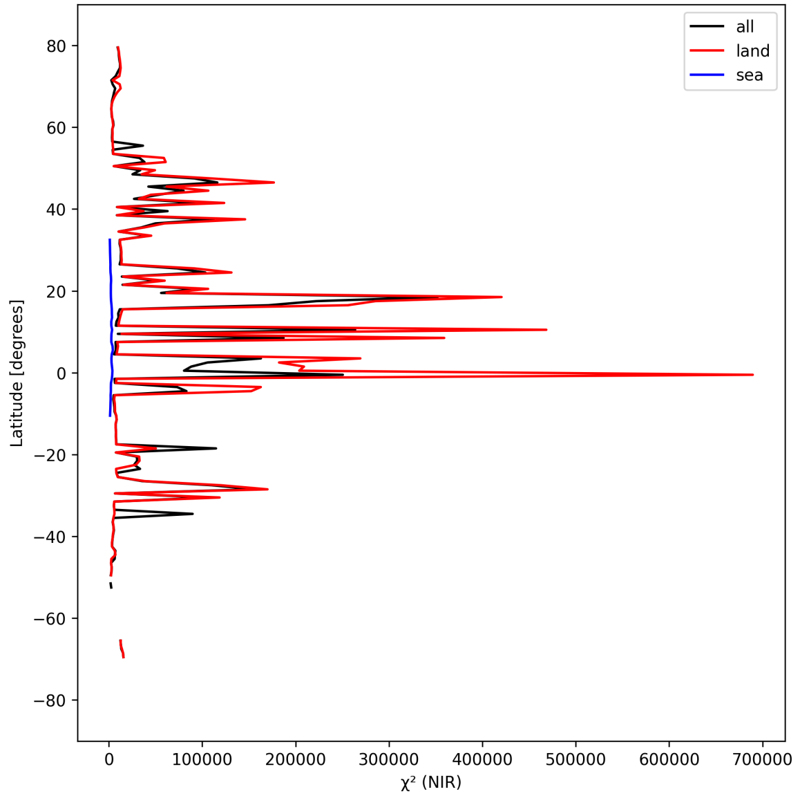
Figure 18: Zonal average of “ \chi^2 (NIR)” for 2024-09-10 to 2024-09-12.
