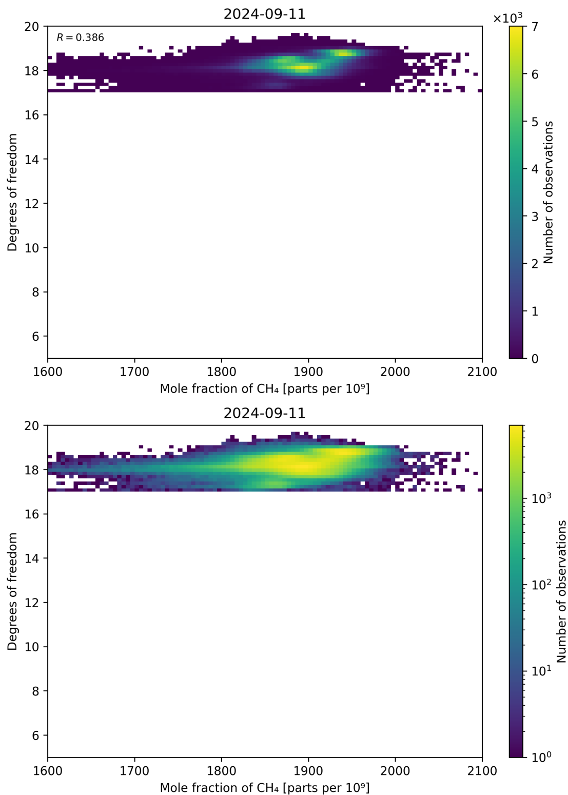
Figure 72: Scatter density plot of “Mole fraction of CH 4 ” against “Degrees of freedom” for 2024-09-10 to 2024-09-12.
