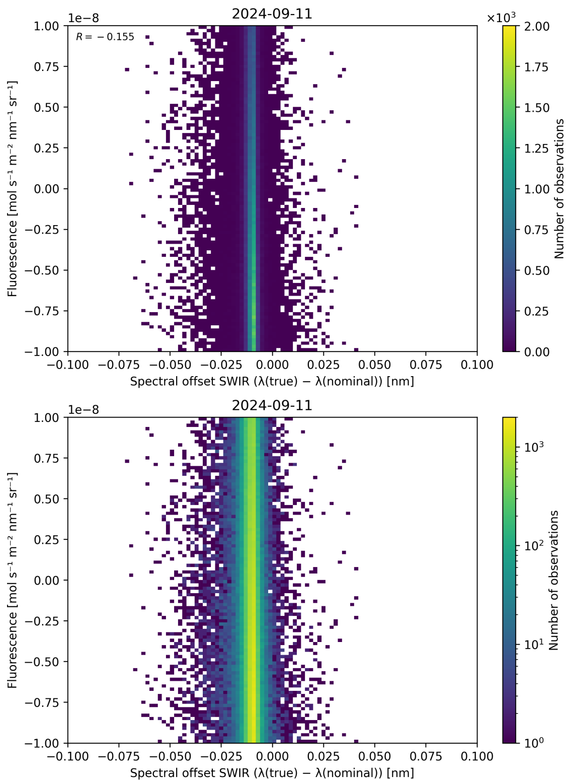
Figure 120: Scatter density plot of “Spectral offset SWIR ( \lambda_{\text{true}} - \lambda_{\text{nominal}} )” against “Fluorescence” for 2024-09-10 to 2024-09-12.
