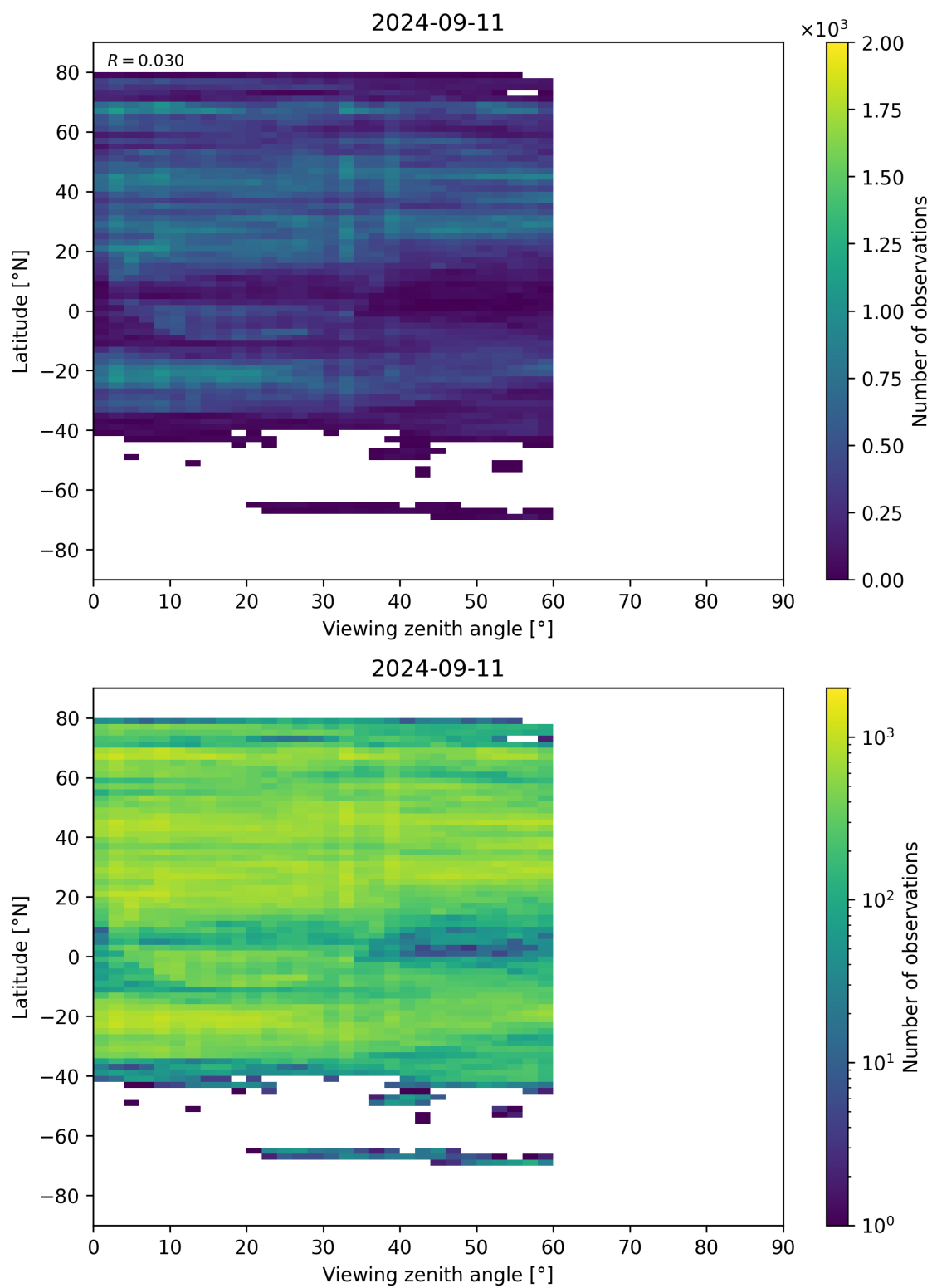
Figure 109: Scatter density plot of “Viewing zenith angle” against “Latitude” for 2024-09-10 to 2024-09-12.
