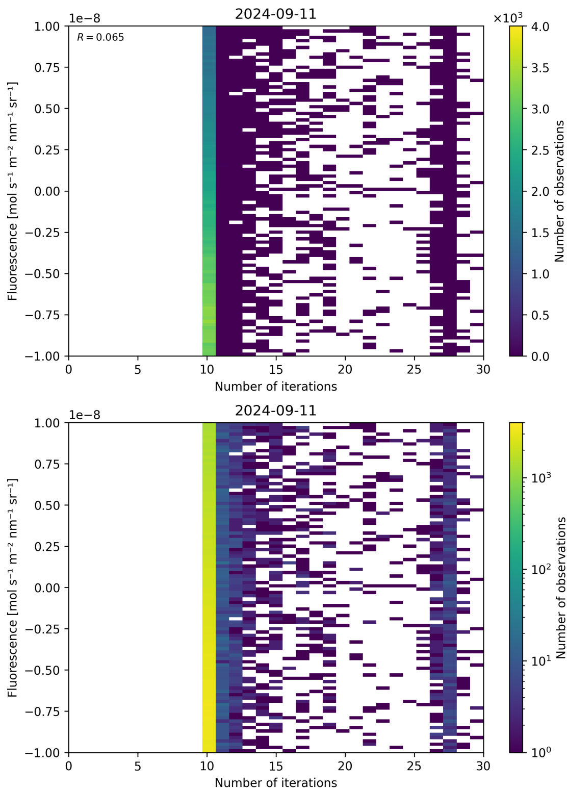
Figure 87: Scatter density plot of “Number of iterations” against “Fluorescence” for 2024-09-10 to 2024-09-12.
