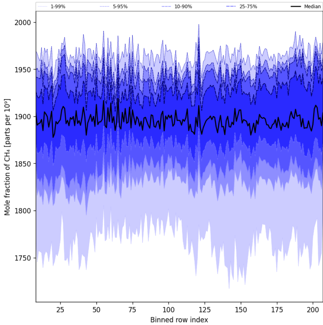
Figure 34: Along track statistics of “Mole fraction of CH 4 ” for 2024-09-10 to 2024-09-12
