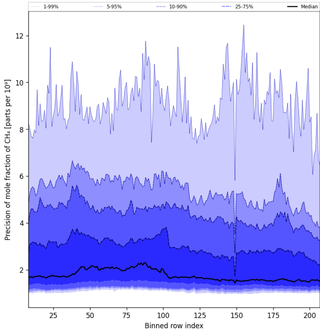
Figure 35: Along track statistics of “Precision of mole fraction of CH 4 ” for 2024-09-10 to 2024-09-12
