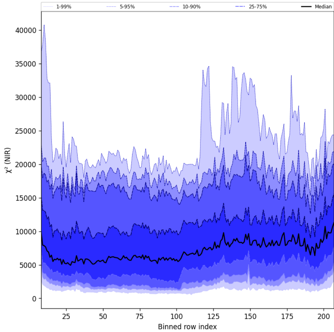
Figure 40: Along track statistics of “ \chi^2 (NIR)” for 2024-09-10 to 2024-09-12
