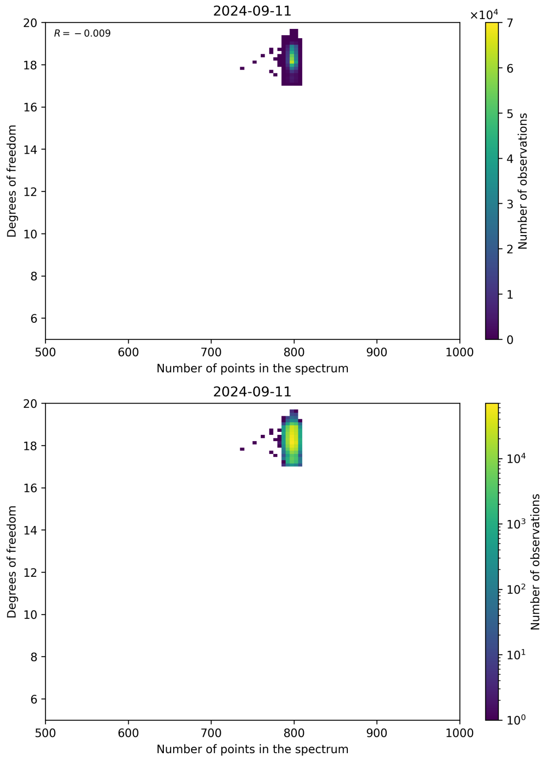
Figure 90: Scatter density plot of “Number of points in the spectrum” against “Degrees of freedom” for 2024-09-10 to 2024-09-12.
