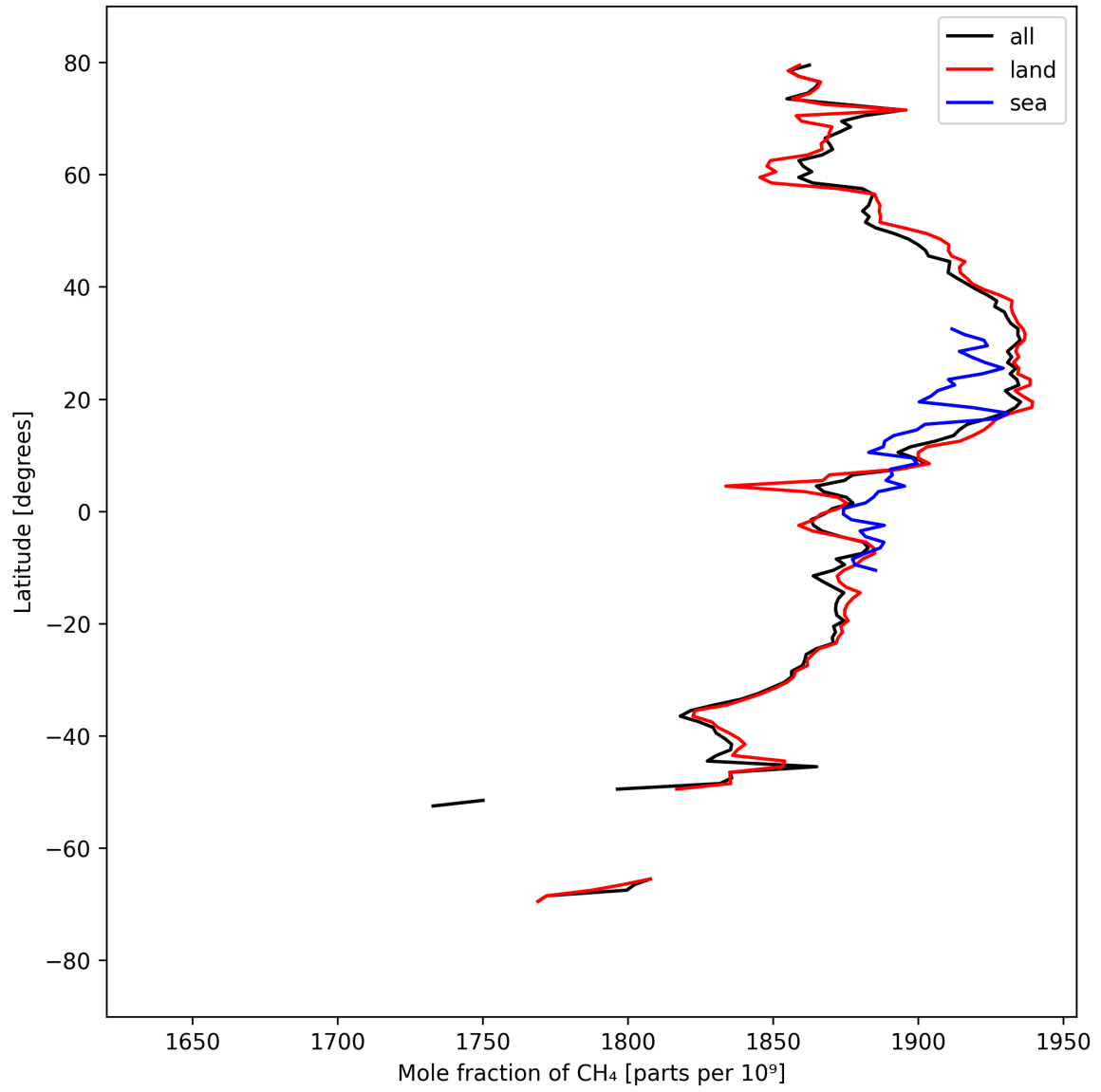
Figure 12: Zonal average of “Mole fraction of \text{CH}_4 ” for 2024-09-10 to 2024-09-12.
