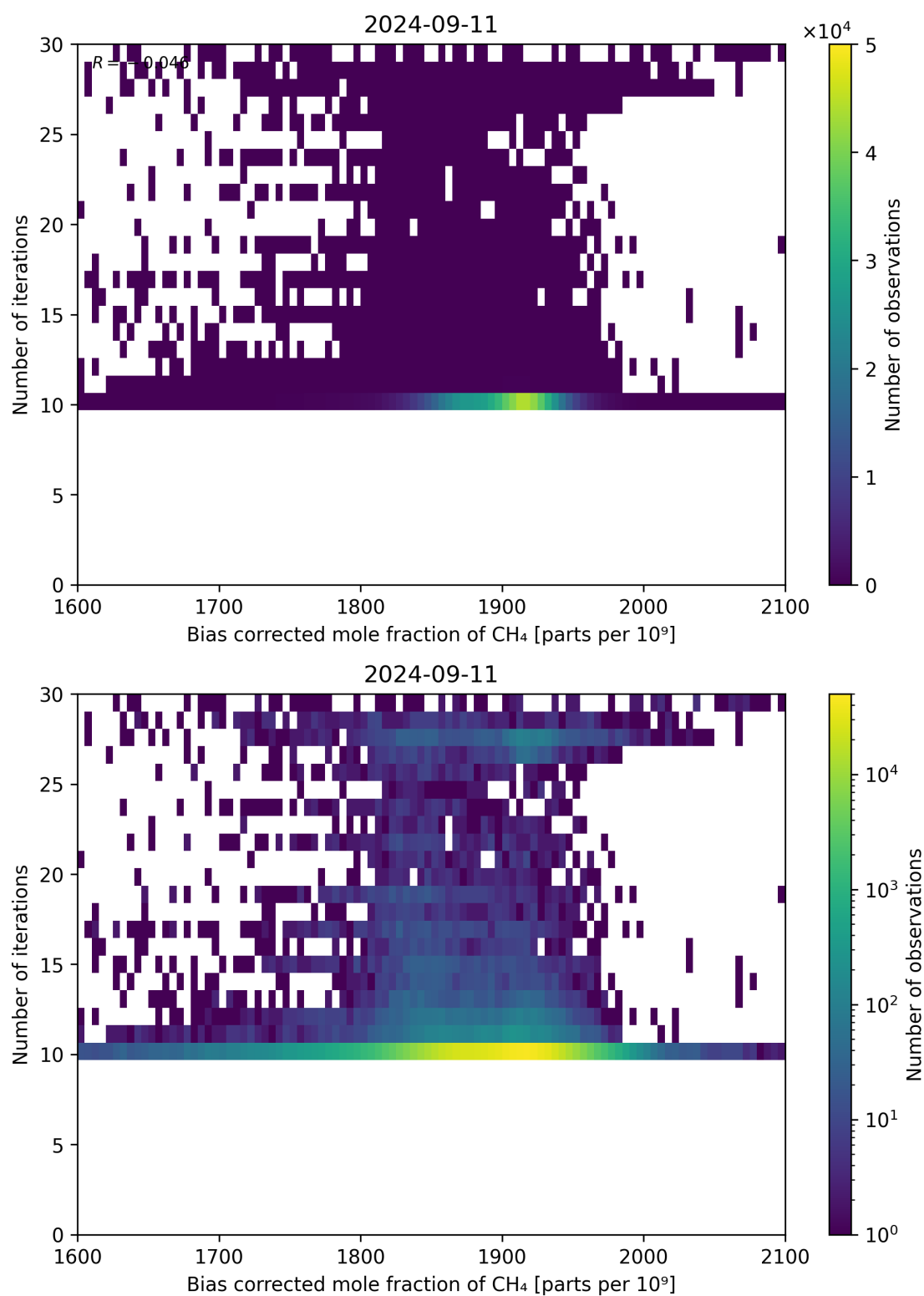
Figure 67: Scatter density plot of “Bias corrected mole fraction of CH 4 ” against “Number of iterations” for 2024-09-10 to 2024-09-12.
