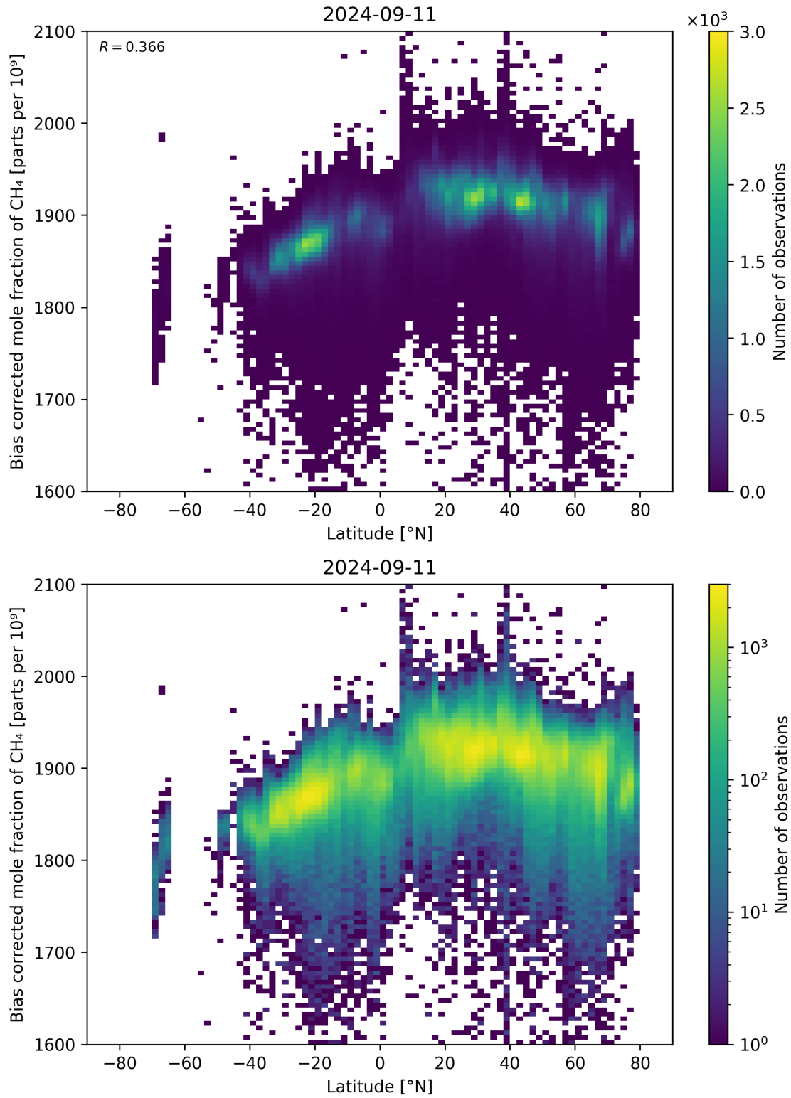
Figure 58: Scatter density plot of “Latitude” against “Bias corrected mole fraction of CH 4 ” for 2024-09-10 to 2024-09-12.
