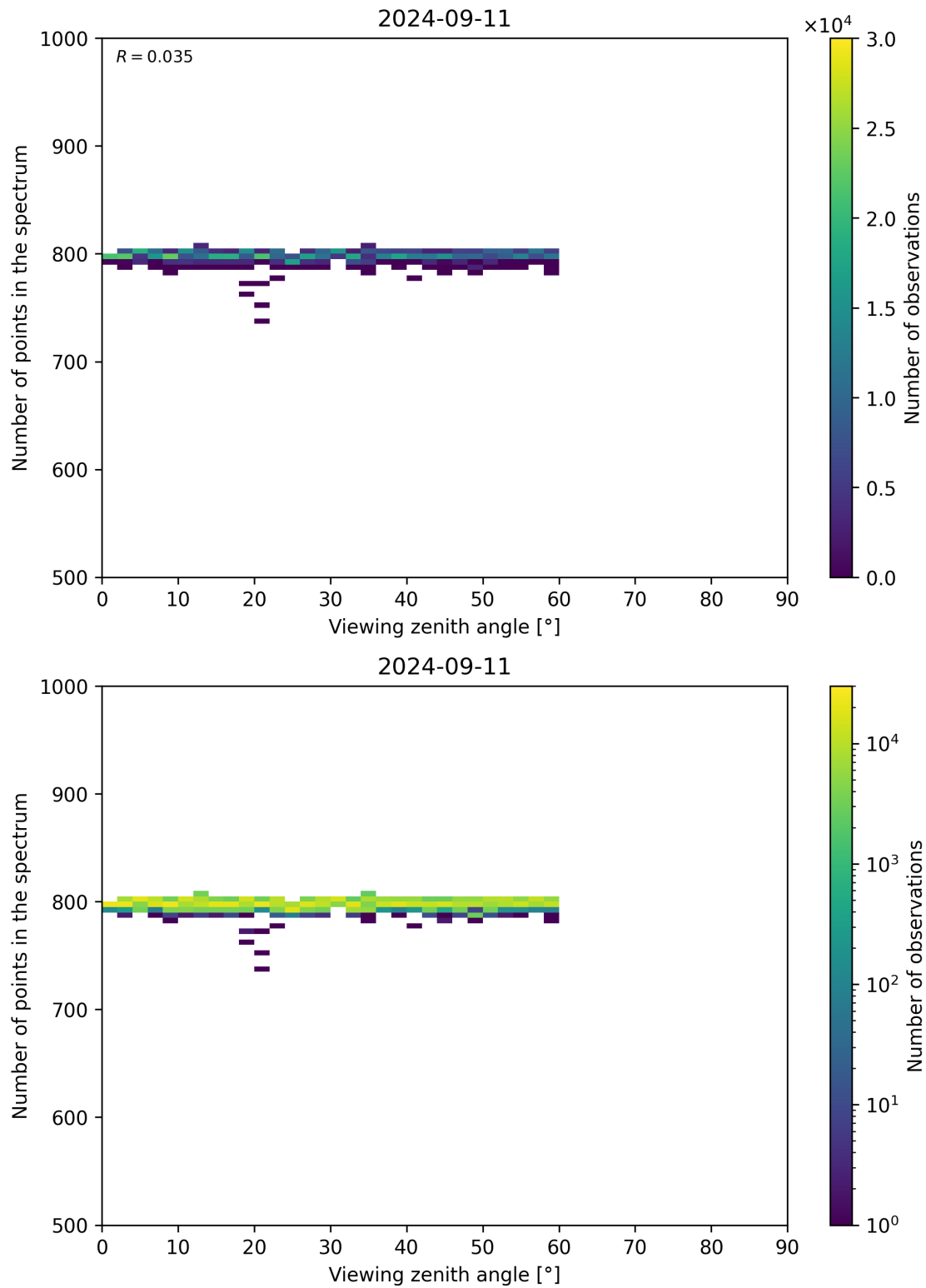
Figure 114: Scatter density plot of “Viewing zenith angle” against “Number of points in the spectrum” for 2024-09-10 to 2024-09-12.
