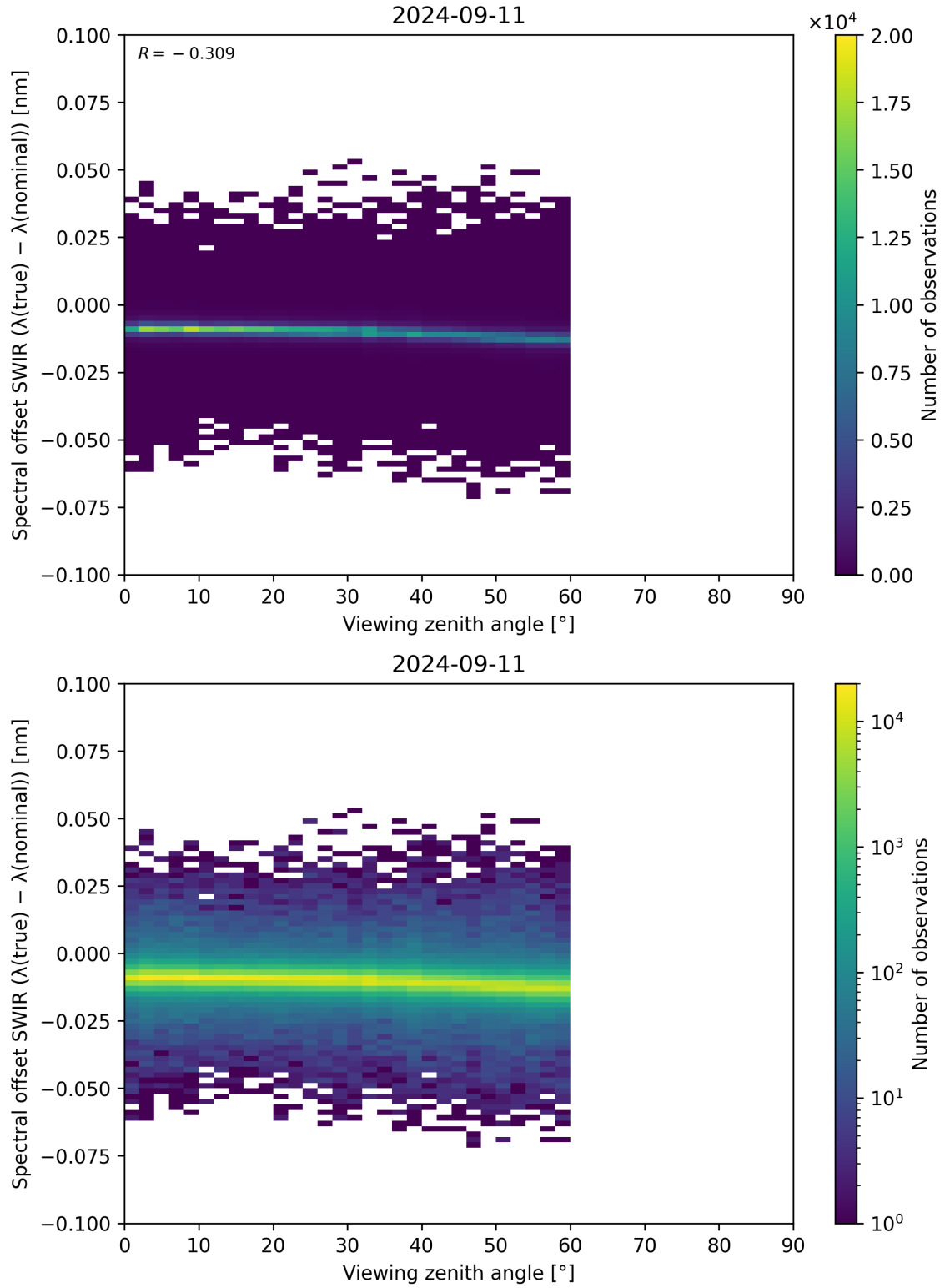
Figure 116: Scatter density plot of “Viewing zenith angle” against “Spectral offset SWIR ( \lambda_{\text{true}} - \lambda_{\text{nominal}} )” for 2024-09-10 to 2024-09-12.
