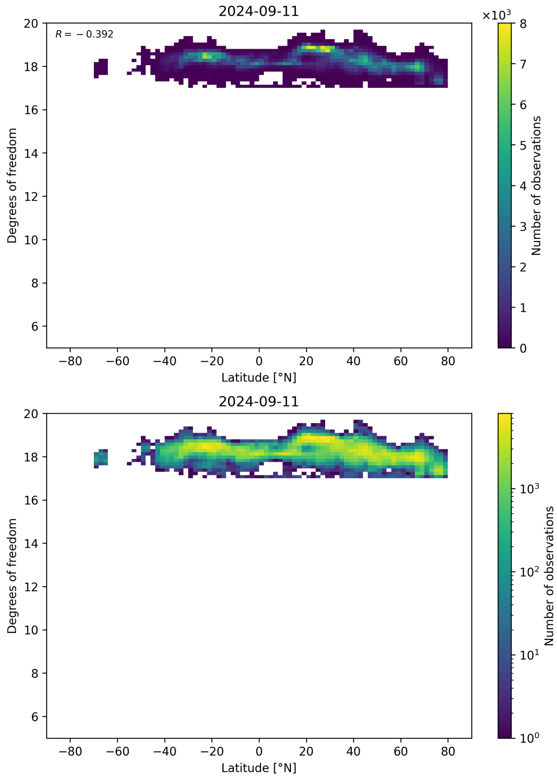
Figure 55: Scatter density plot of “Latitude” against “Degrees of freedom” for 2024-09-10 to 2024-09-12.
