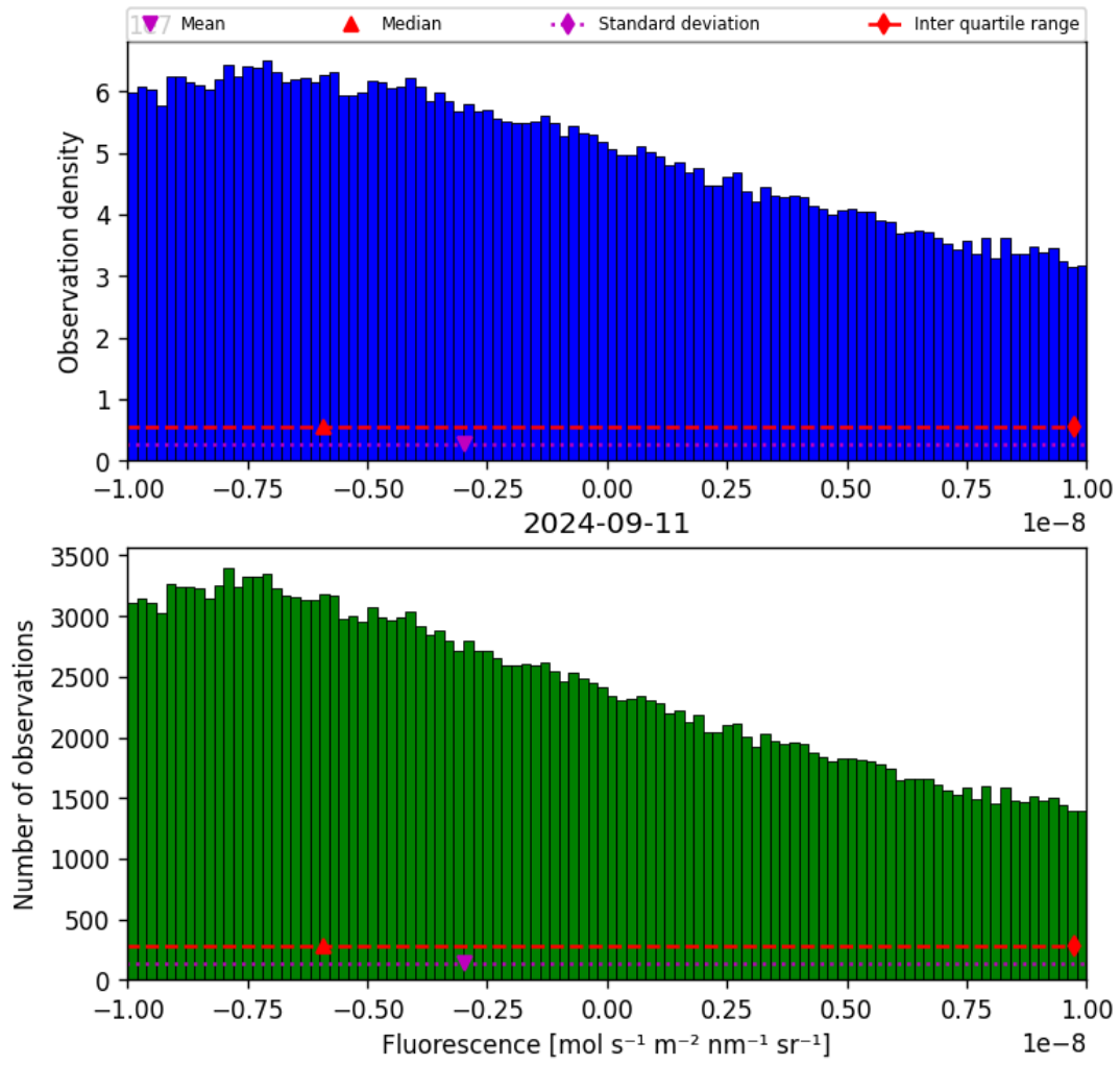
Figure 32: Histogram of “Fluorescence” for 2024-09-10 to 2024-09-12
