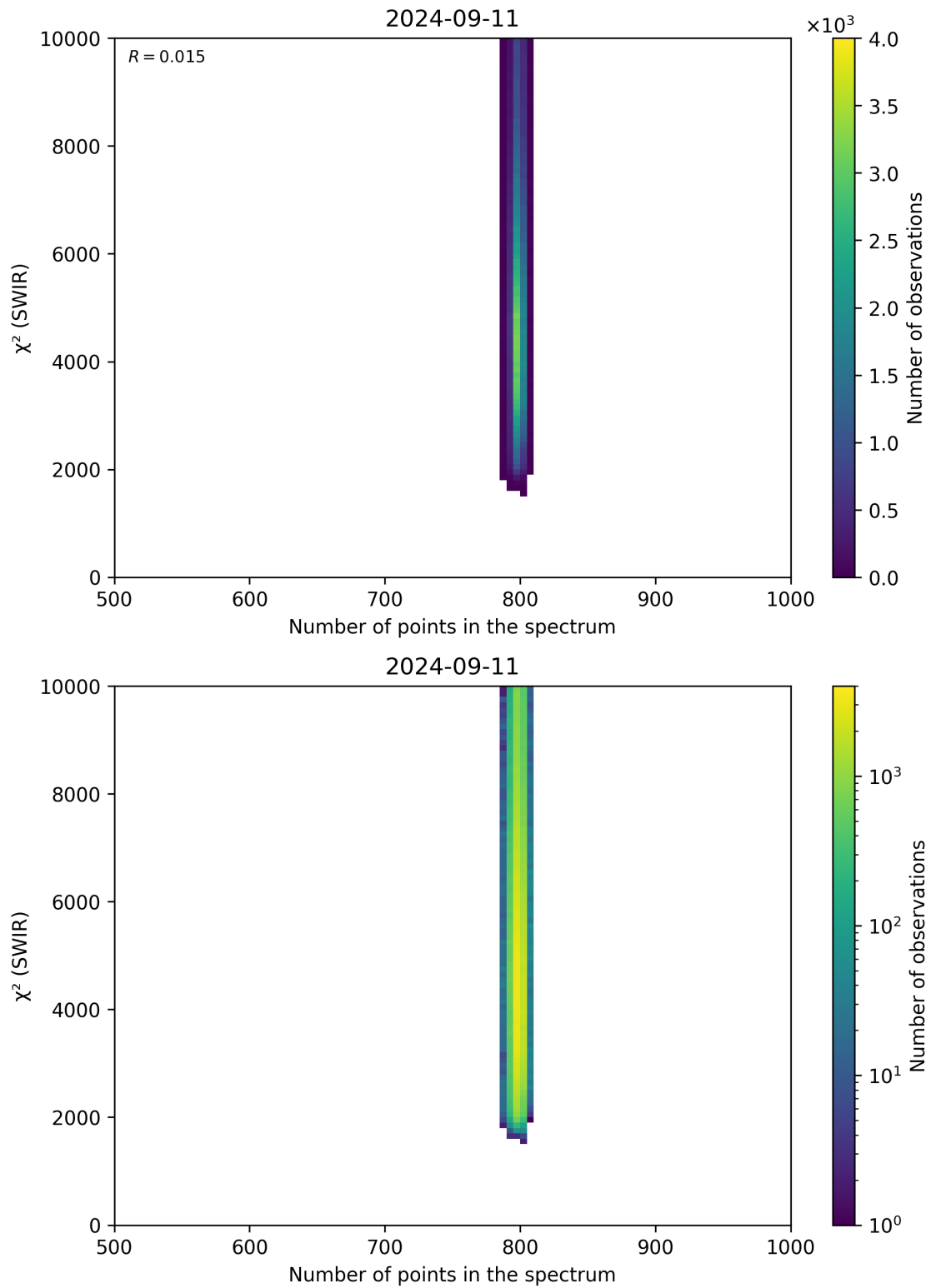
Figure 89: Scatter density plot of “Number of points in the spectrum” against “ \chi^2 (SWIR)” for 2024-09-10 to 2024-09-12.
