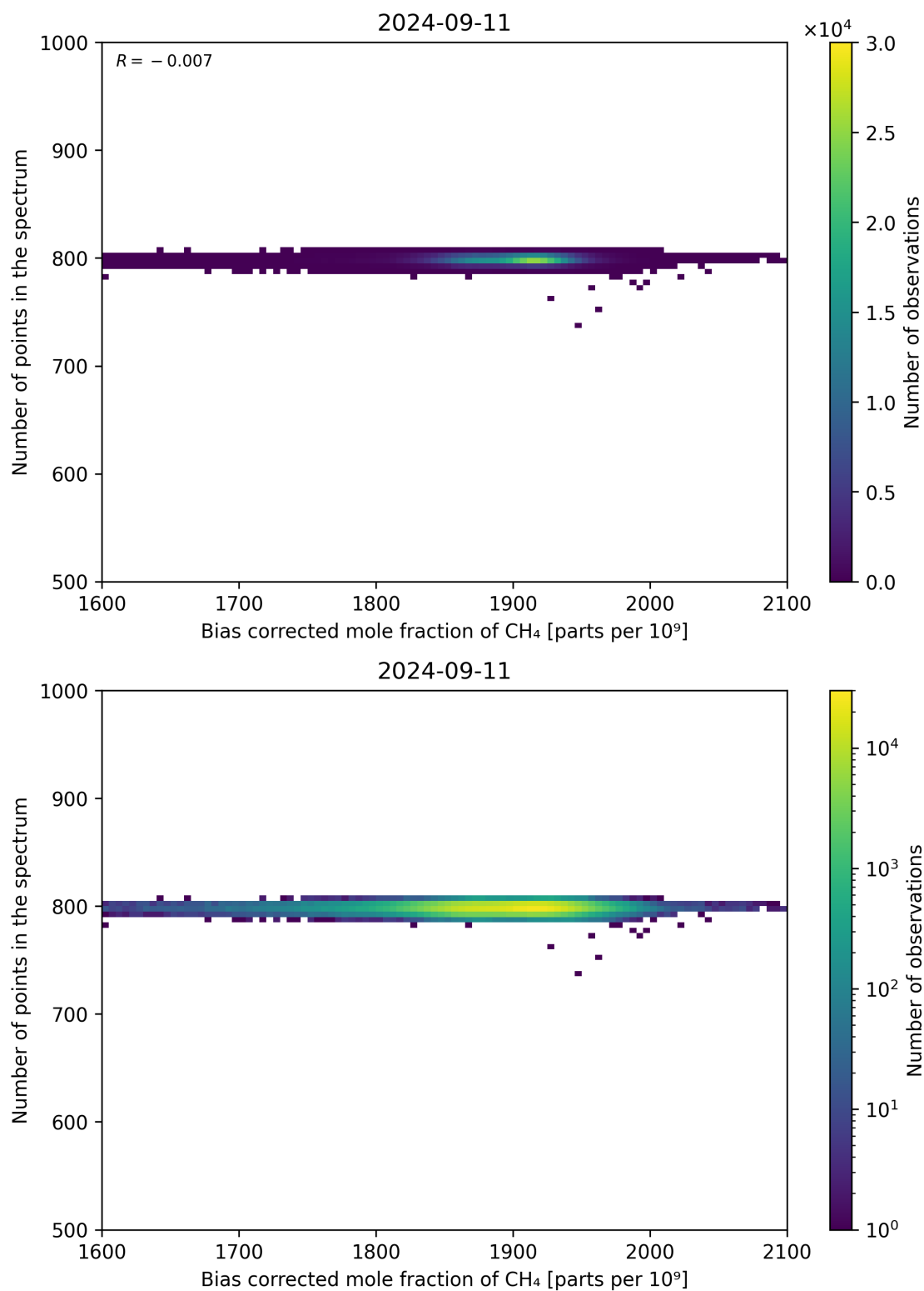
Figure 68: Scatter density plot of “Bias corrected mole fraction of CH 4 ” against “Number of points in the spectrum” for 2024-09-10 to 2024-09-12.
