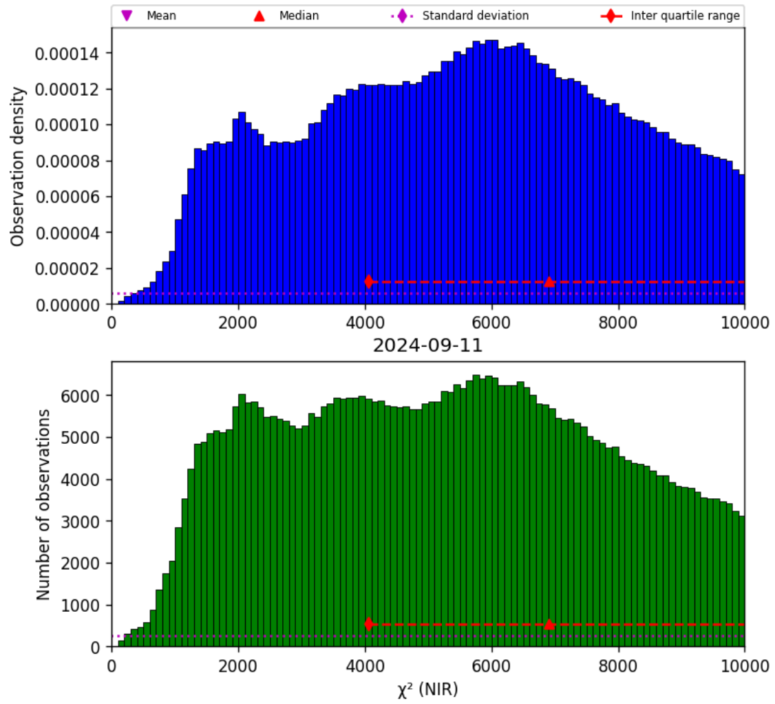
Figure 29: Histogram of “ \chi^2 (NIR)” for 2024-09-10 to 2024-09-12
