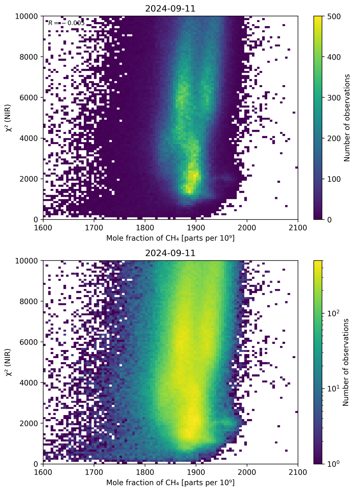
Figure 70: Scatter density plot of “Mole fraction of \text{CH}_4 ” against “ \chi^2 (NIR)” for 2024-09-10 to 2024-09-12.
