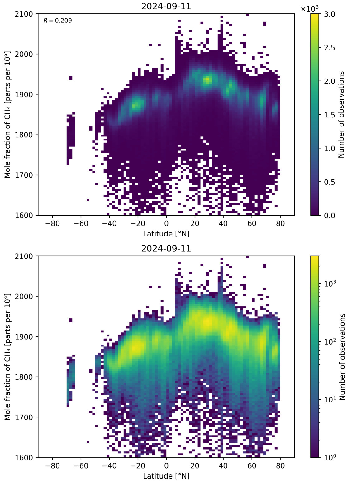
Figure 57: Scatter density plot of “Latitude” against “Mole fraction of \text{CH}_4 ” for 2024-09-10 to 2024-09-12.
