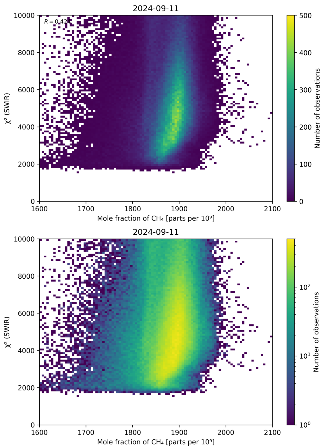
Figure 71: Scatter density plot of “Mole fraction of \text{CH}_4 ” against “ \chi^2 (SWIR)” for 2024-09-10 to 2024-09-12.
