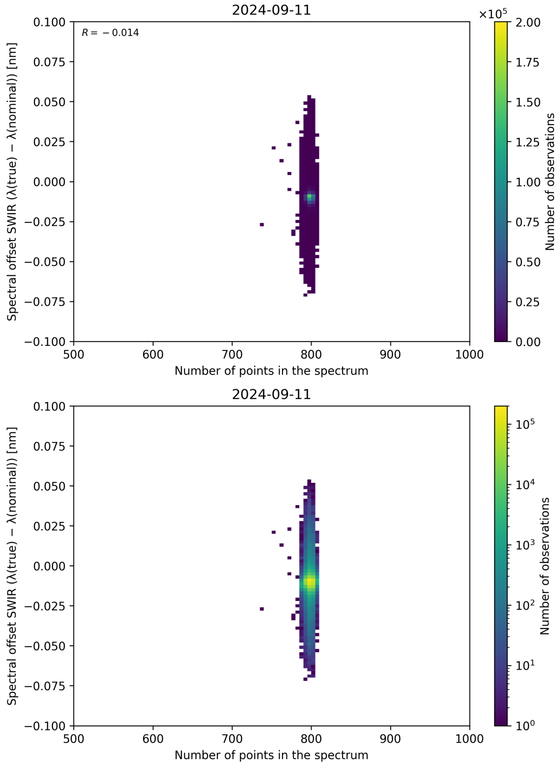
Figure 93: Scatter density plot of “Number of points in the spectrum” against “Spectral offset SWIR ( \lambda_{\text{true}} - \lambda_{\text{nominal}} )” for 2024-09-10 to 2024-09-12.
