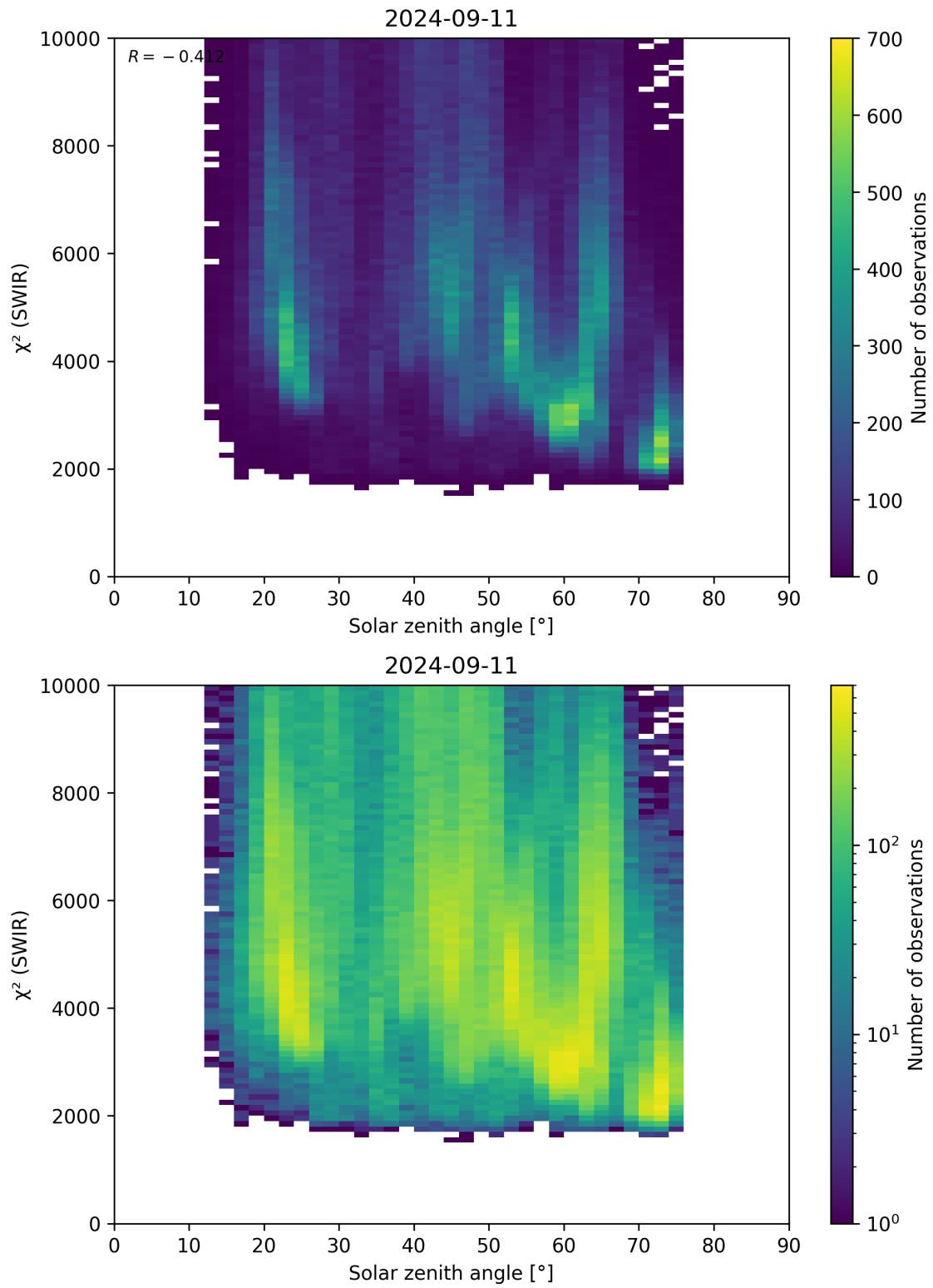
Figure 95: Scatter density plot of “Solar zenith angle” against “ \chi^2 (SWIR)” for 2024-09-10 to 2024-09-12.
