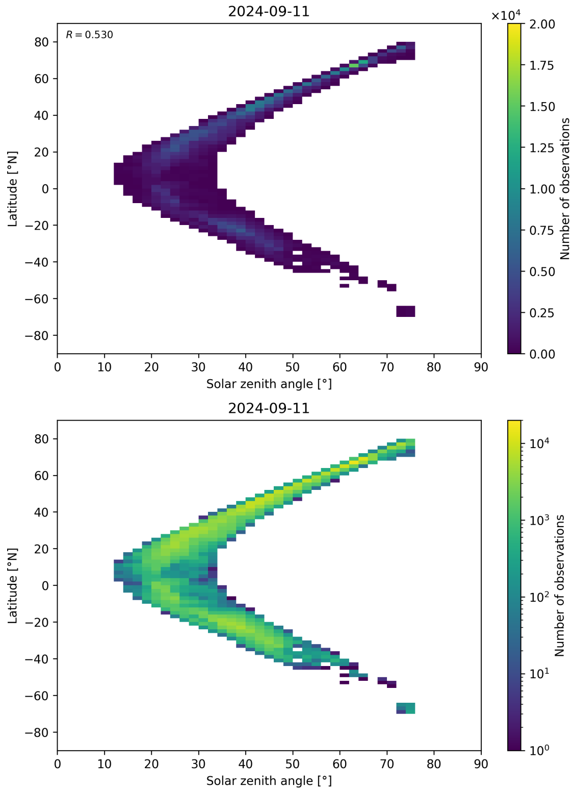
Figure 98: Scatter density plot of “Solar zenith angle” against “Latitude” for 2024-09-10 to 2024-09-12.
