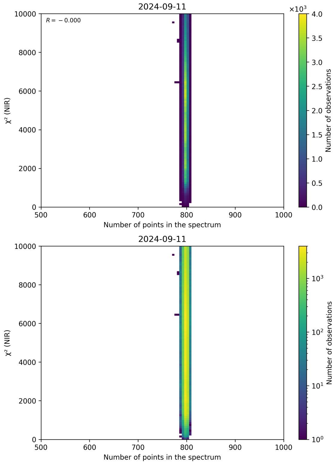
Figure 88: Scatter density plot of “Number of points in the spectrum” against “ \chi^2 (NIR)” for 2024-09-10 to 2024-09-12.
