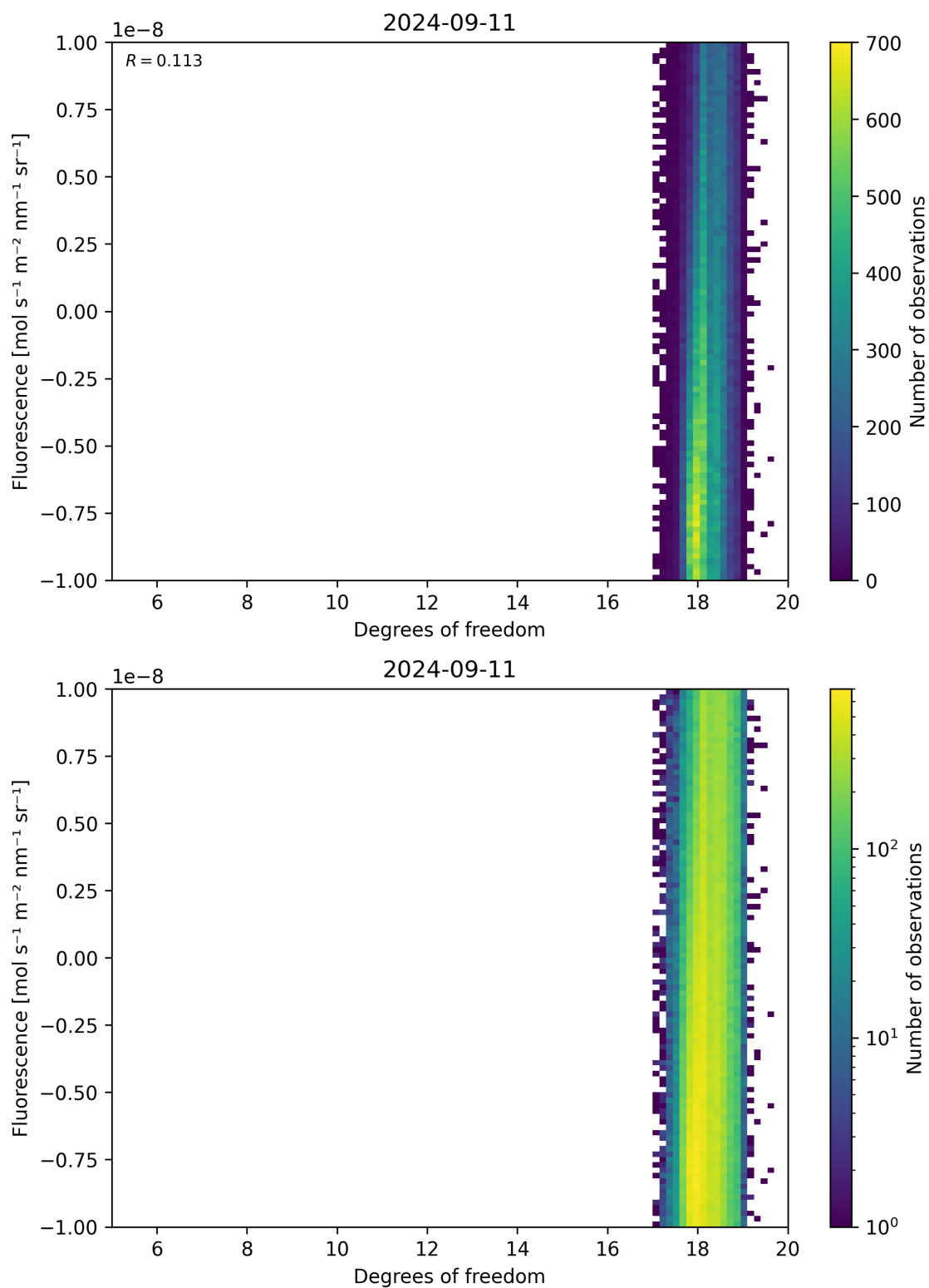
Figure 51: Scatter density plot of “Degrees of freedom” against “Fluorescence” for 2024-09-10 to 2024-09-12.
