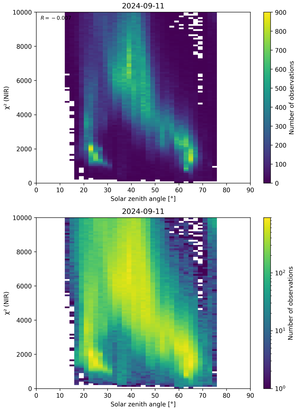
Figure 94: Scatter density plot of “Solar zenith angle” against “ \chi^2 (NIR)” for 2024-09-10 to 2024-09-12.
