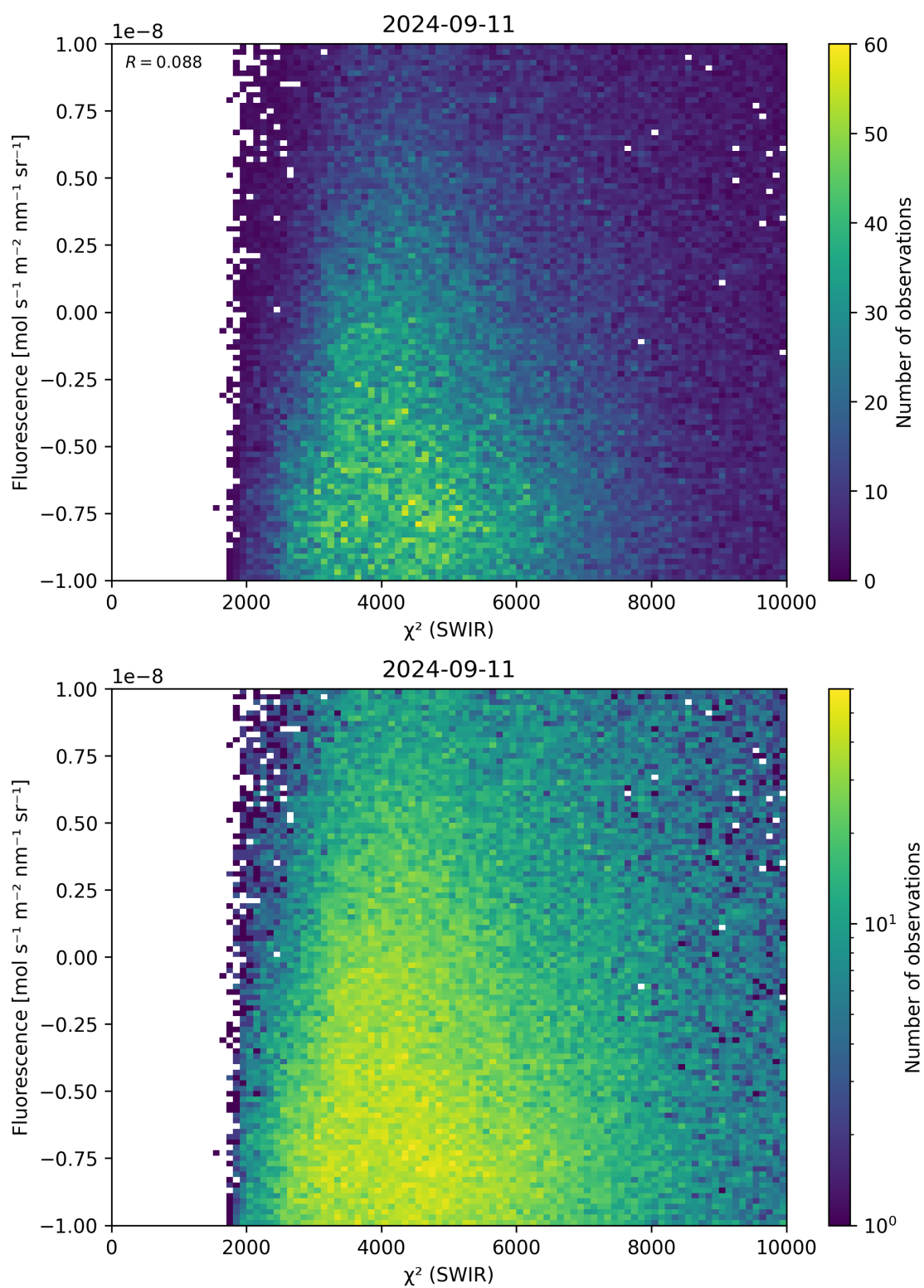
Figure 49: Scatter density plot of “ \chi^2 (SWIR)” against “Fluorescence” for 2024-09-10 to 2024-09-12.
