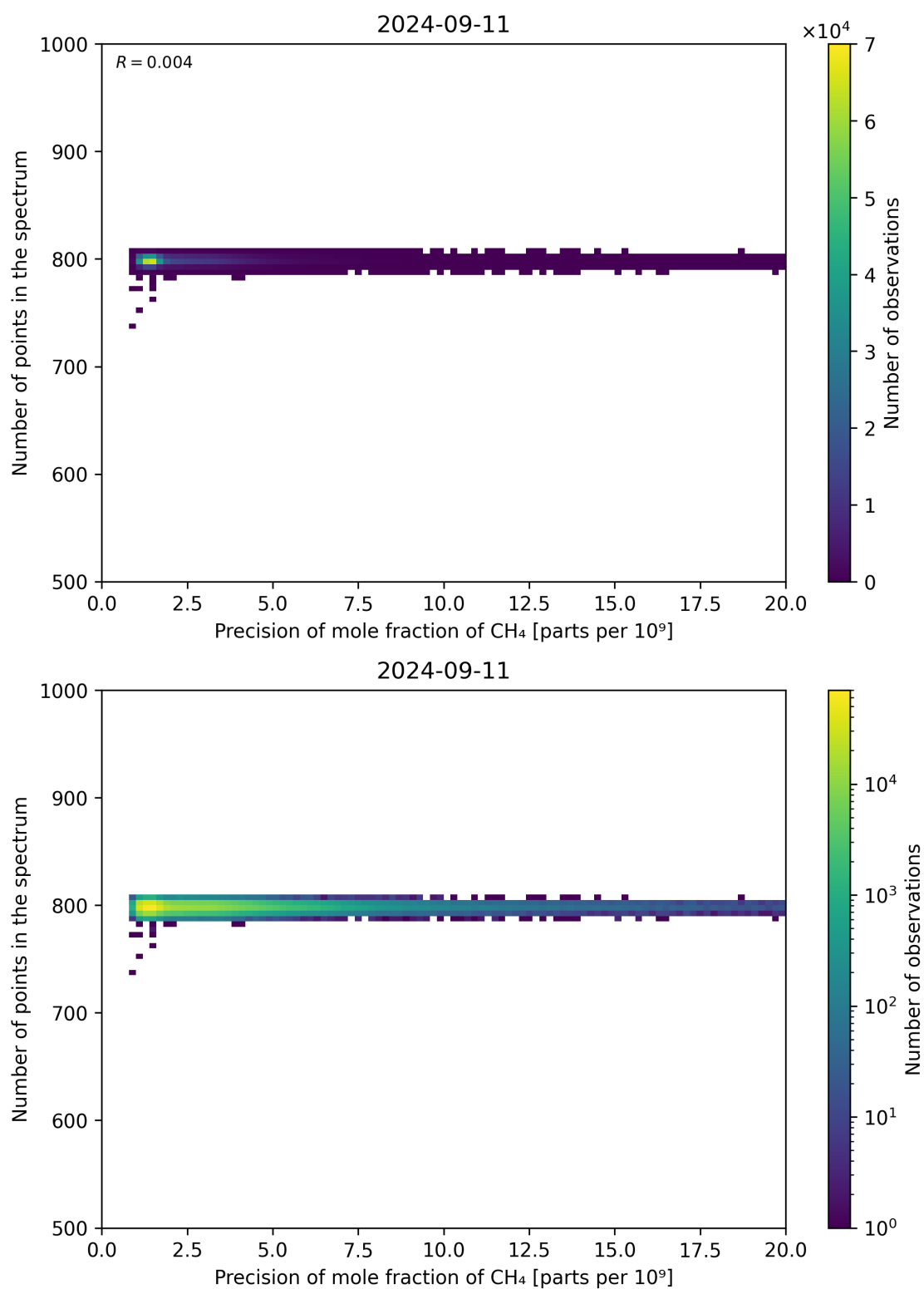
Figure 84: Scatter density plot of “Precision of mole fraction of CH 4 ” against “Number of points in the spectrum” for 2024-09-10 to 2024-09-12.
