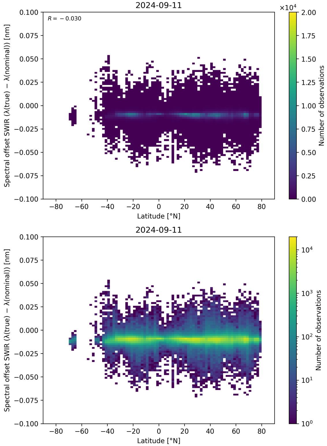
Figure 62: Scatter density plot of “Latitude” against “Spectral offset SWIR ( \lambda_{\text{true}} - \lambda_{\text{nominal}} )” for 2024-09-10 to 2024-09-12.
