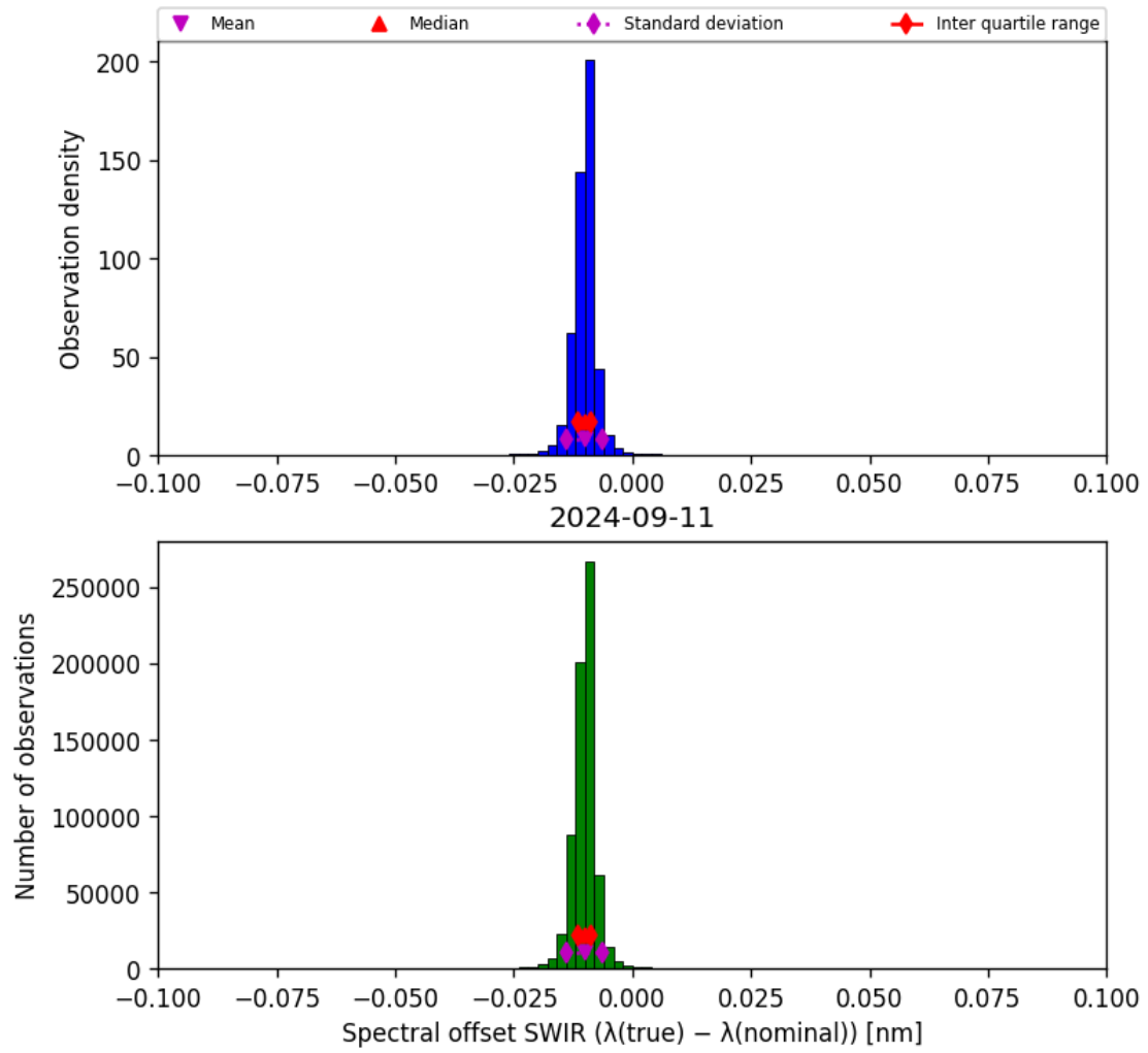
Figure 27: Histogram of “Spectral offset SWIR ( \lambda_{\text{true}} - \lambda_{\text{nominal}} )” for 2024-09-10 to 2024-09-12
