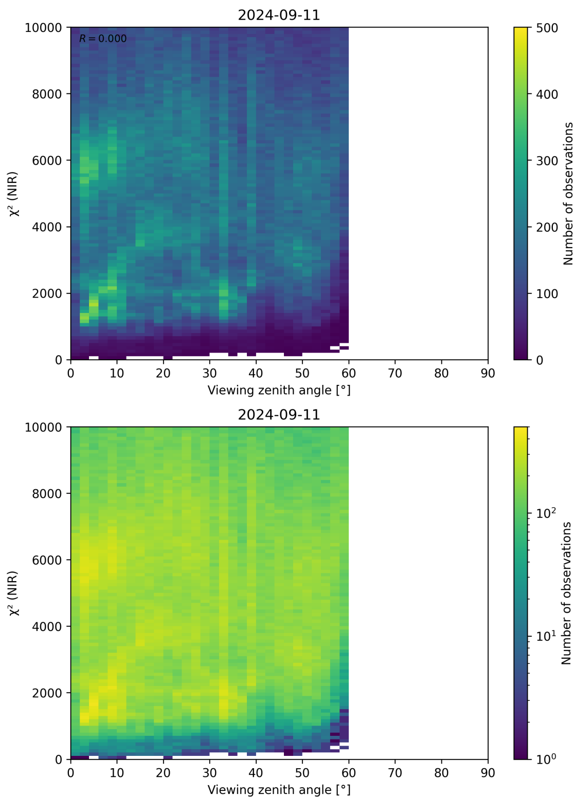
Figure 105: Scatter density plot of “Viewing zenith angle” against “ \chi^2 (NIR)” for 2024-09-10 to 2024-09-12.
