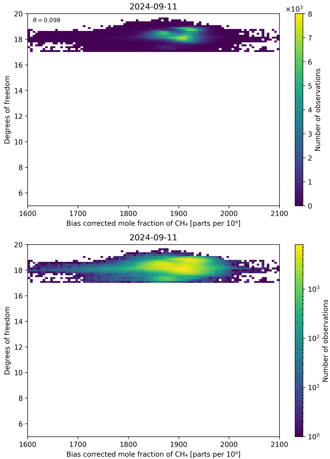
Figure 65: Scatter density plot of “Bias corrected mole fraction of CH 4 ” against “Degrees of freedom” for 2024-09-10 to 2024-09-12.
