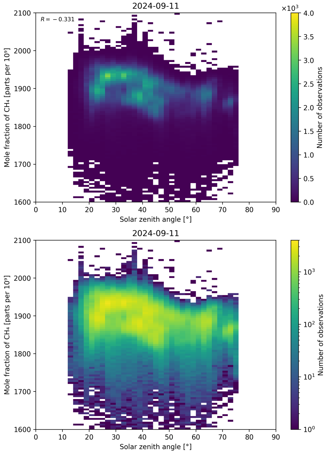
Figure 99: Scatter density plot of “Solar zenith angle” against “Mole fraction of CH 4 ” for 2024-09-10 to 2024-09-12.
