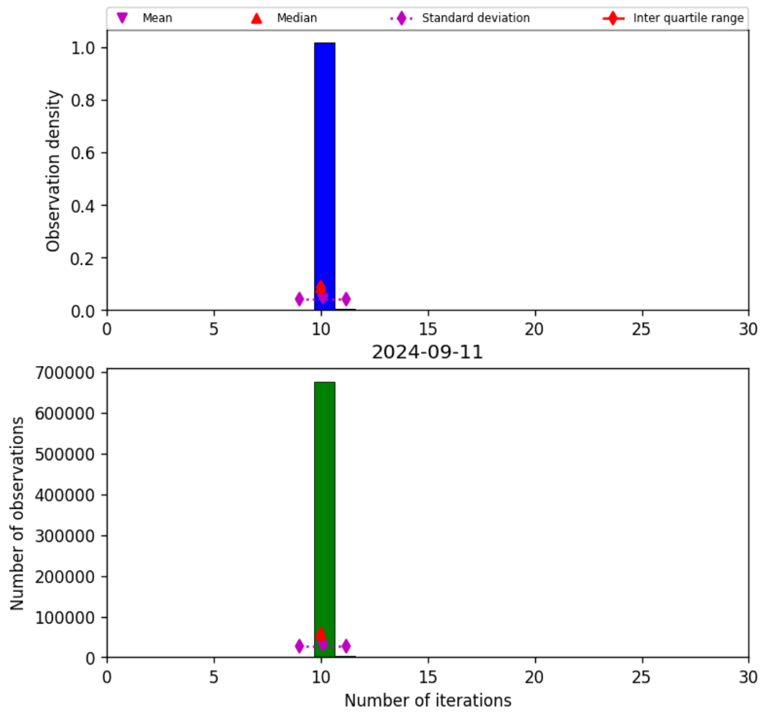
Figure 31: Histogram of “Number of iterations” for 2024-09-10 to 2024-09-12
