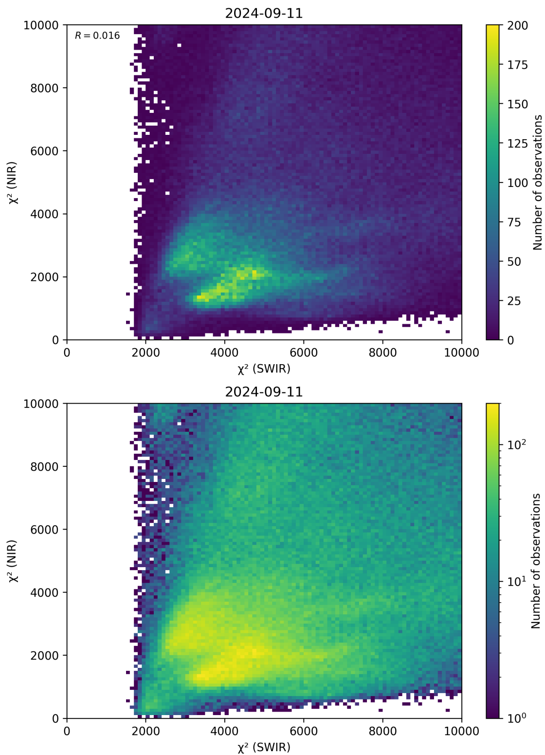
Figure 47: Scatter density plot of “ \chi^2 (SWIR)” against “ \chi^2 (NIR)” for 2024-09-10 to 2024-09-12.
