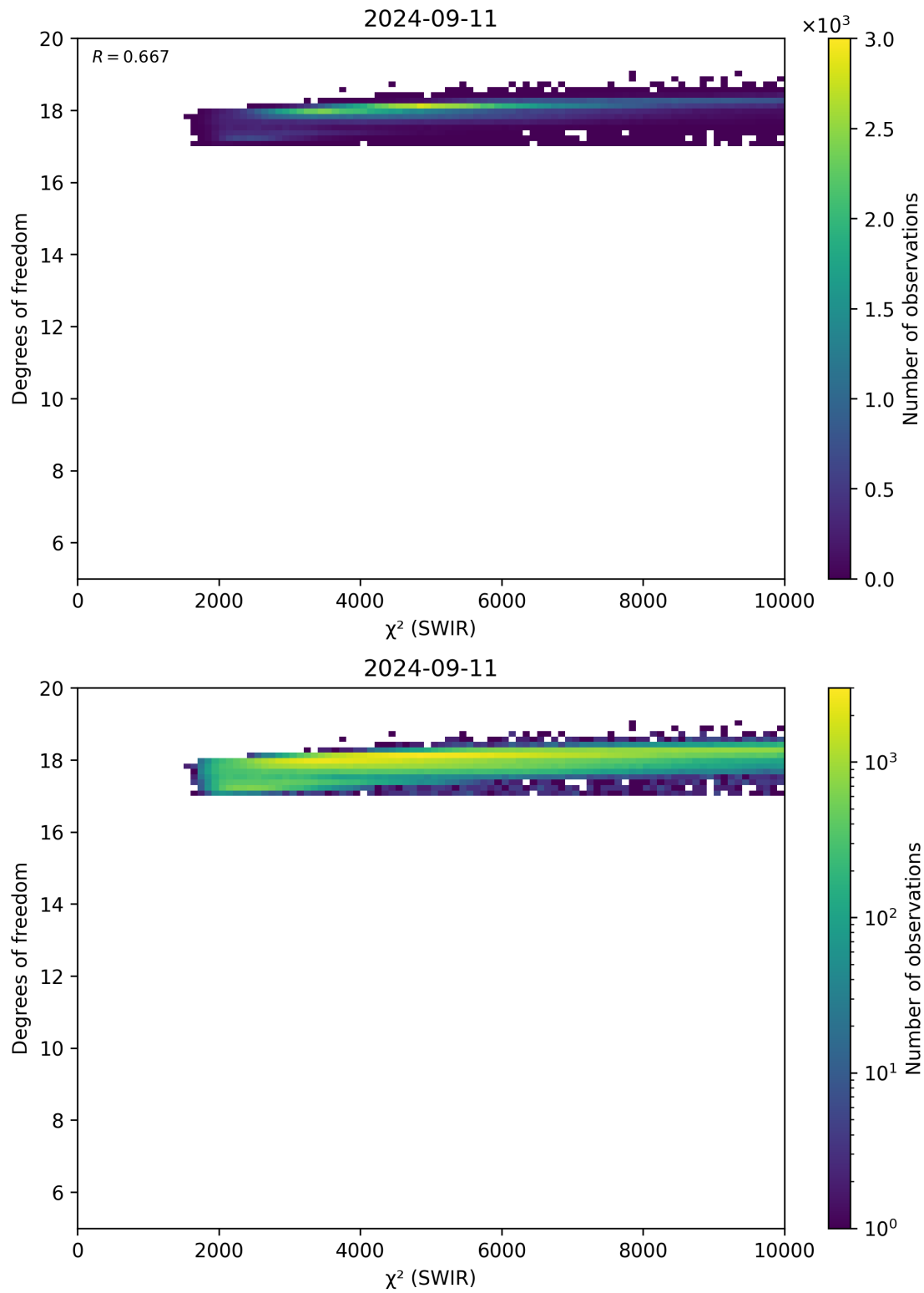
Figure 48: Scatter density plot of “ \chi^2 (SWIR)” against “Degrees of freedom” for 2024-09-10 to 2024-09-12.
