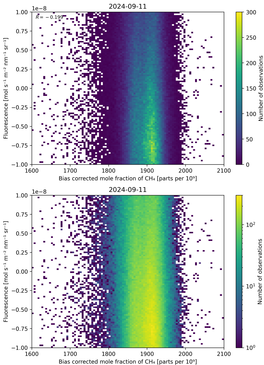
Figure 66: Scatter density plot of “Bias corrected mole fraction of \text{CH}_4 ” against “Fluorescence” for 2024-09-10 to 2024-09-12.
