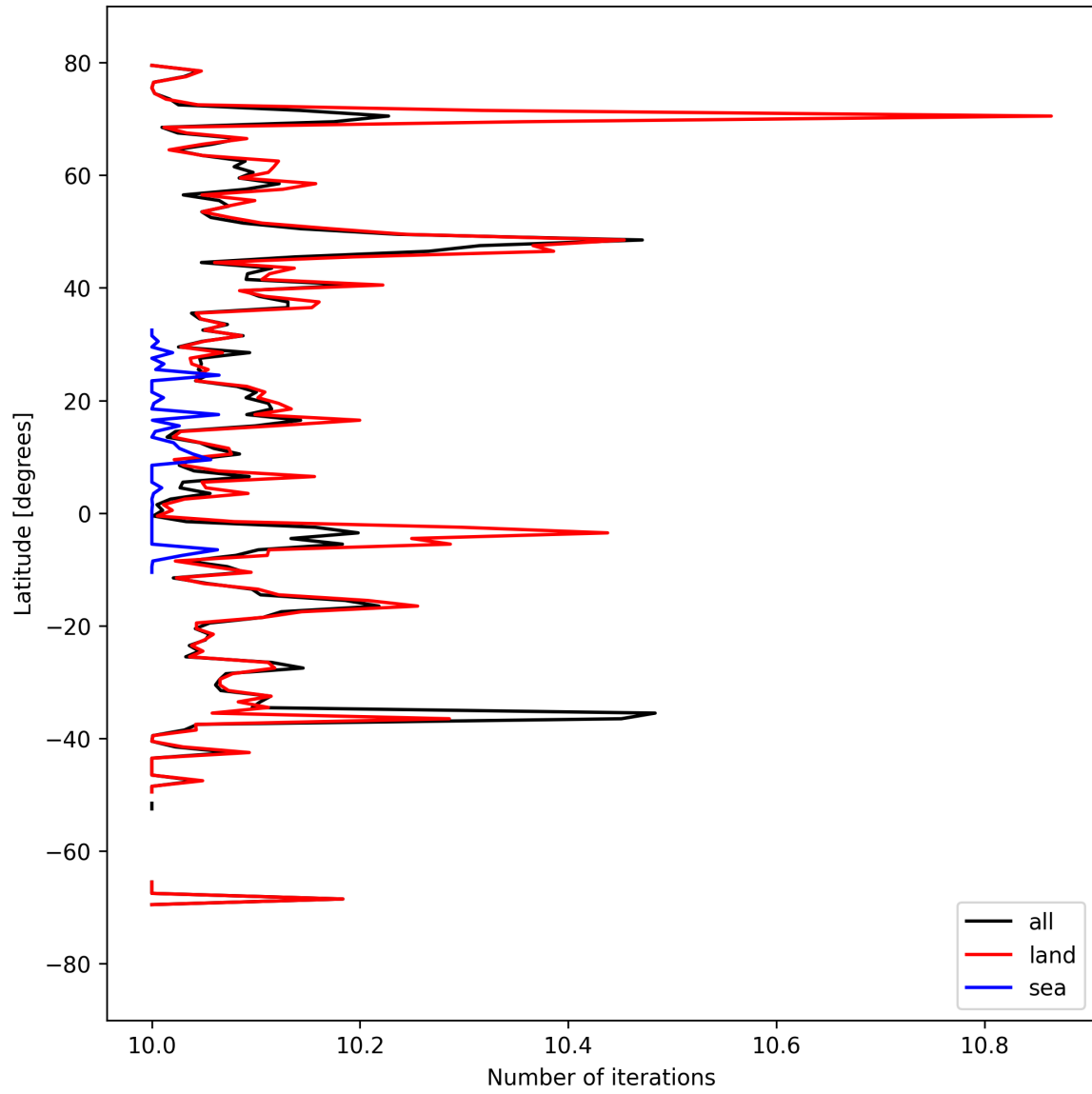
Figure 20: Zonal average of “Number of iterations” for 2024-09-10 to 2024-09-12.
