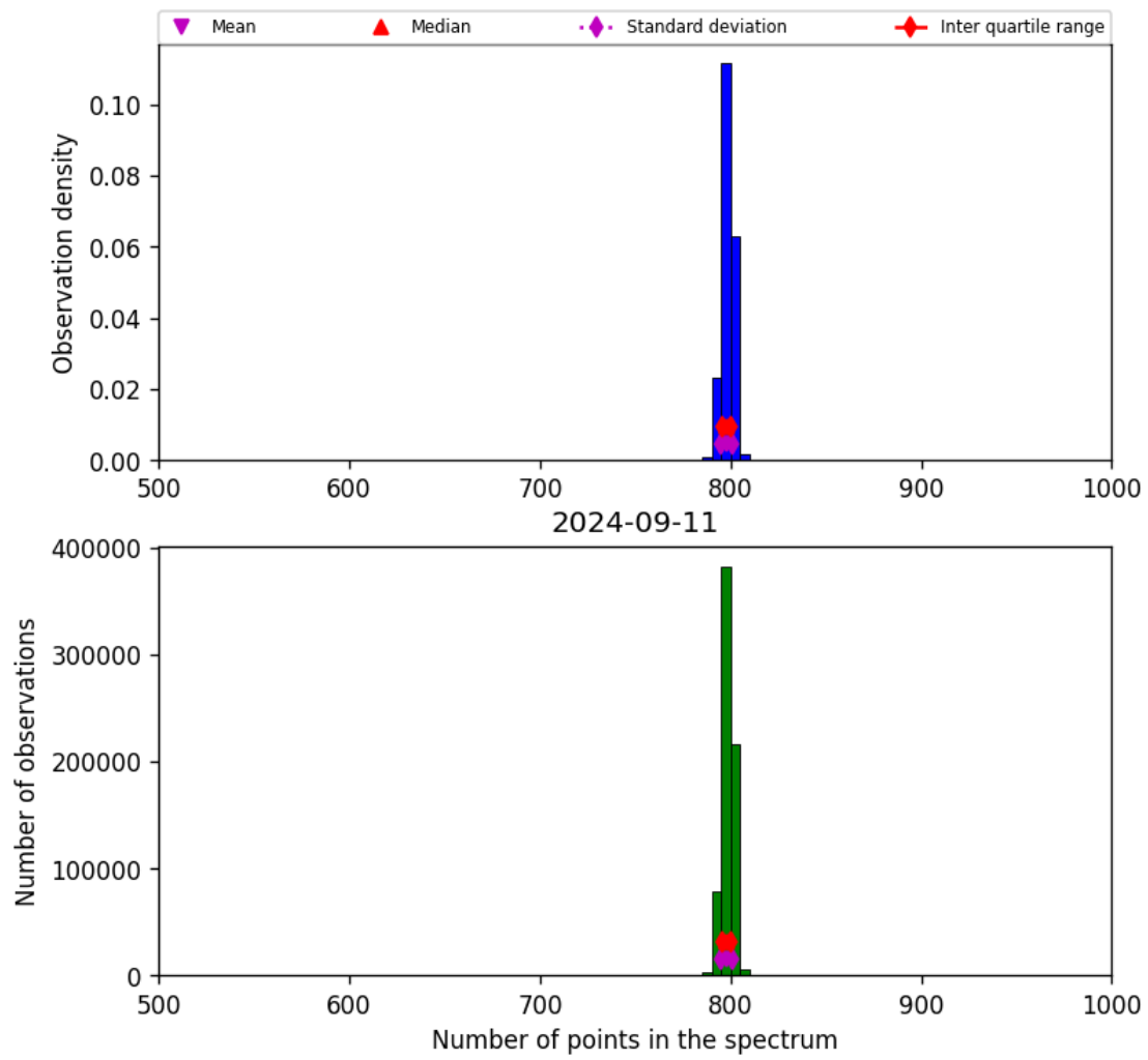
Figure 26: Histogram of “Number of points in the spectrum” for 2024-09-10 to 2024-09-12
