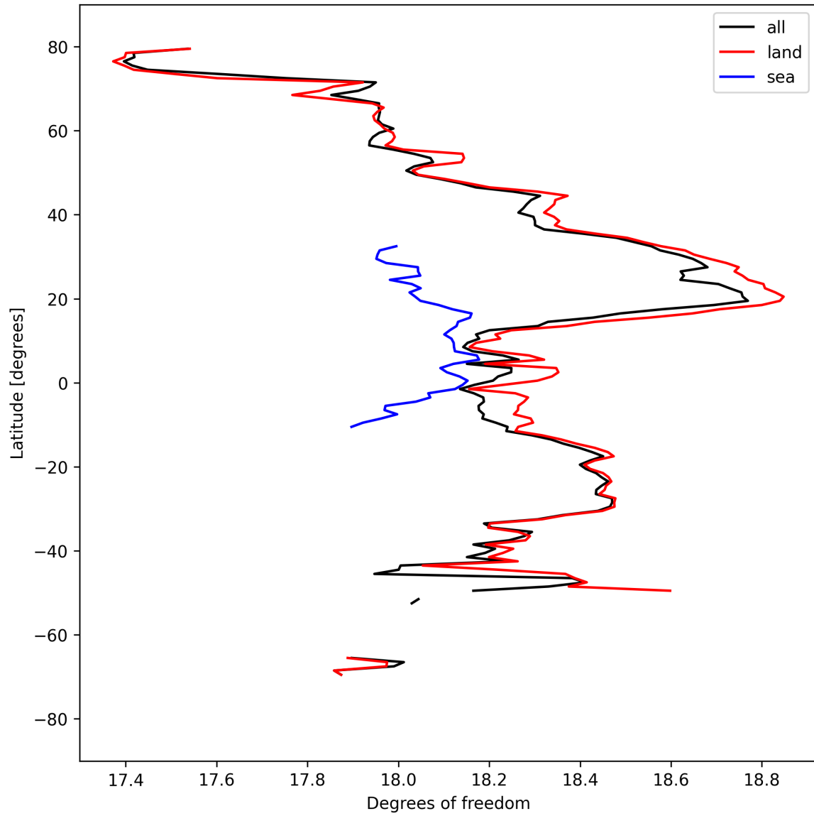
Figure 19: Zonal average of “Degrees of freedom” for 2024-09-10 to 2024-09-12.
