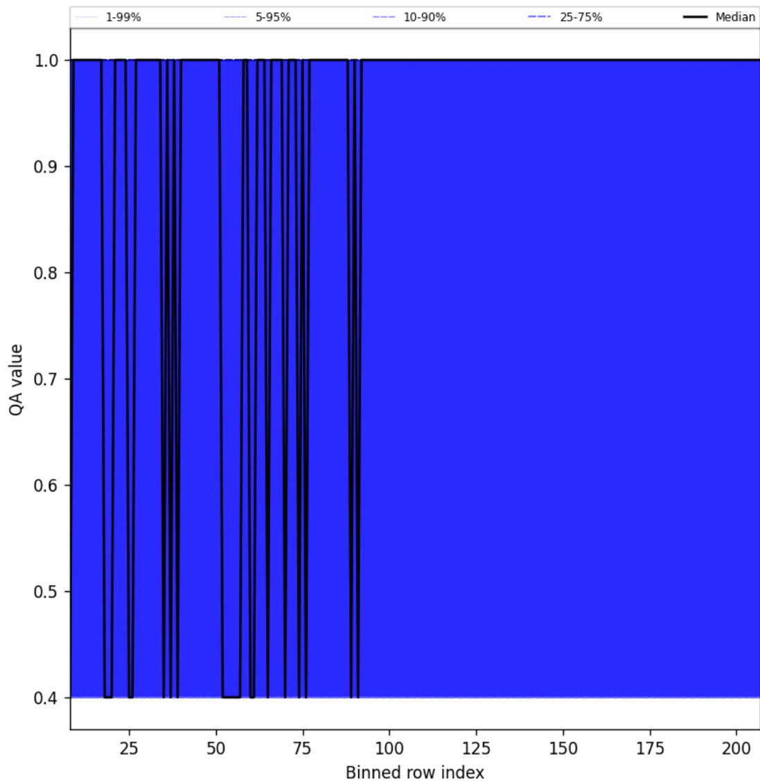
Figure 33: Along track statistics of “QA value” for 2024-09-10 to 2024-09-12
