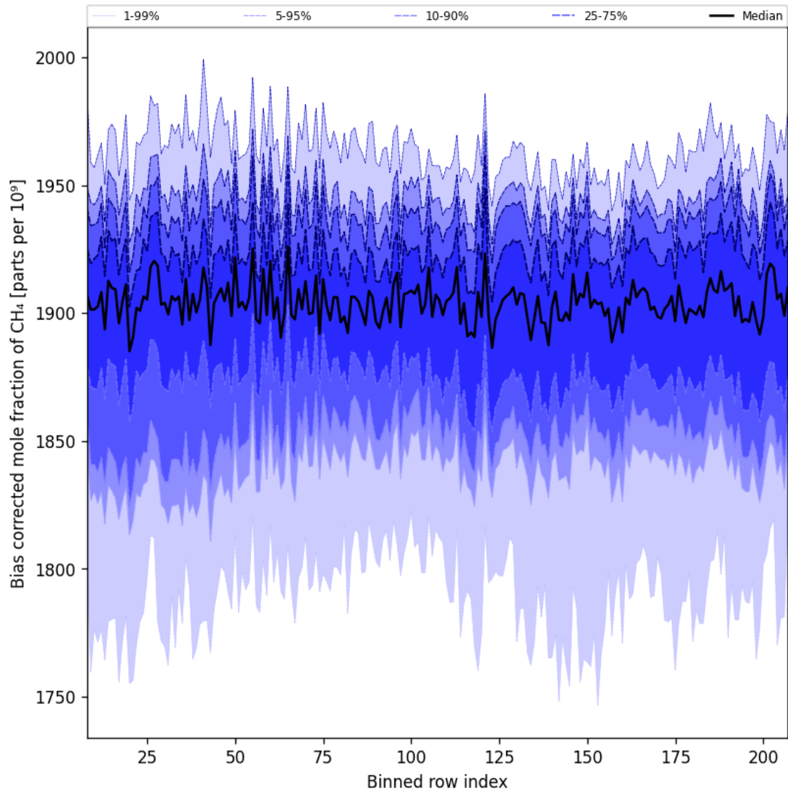
Figure 36: Along track statistics of “Bias corrected mole fraction of CH 4 ” for 2024-09-10 to 2024-09-12
