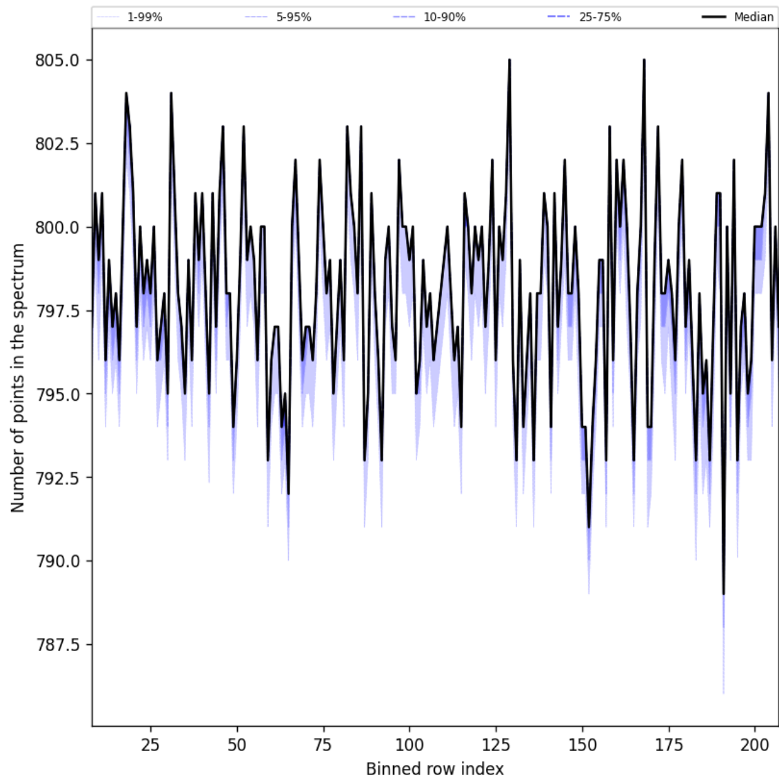
Figure 37: Along track statistics of “Number of points in the spectrum” for 2024-09-10 to 2024-09-12
