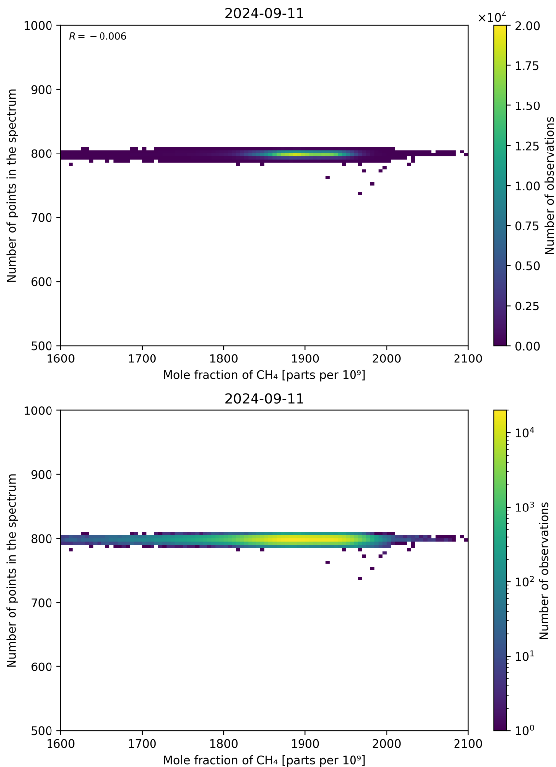
Figure 77: Scatter density plot of “Mole fraction of CH 4 ” against “Number of points in the spectrum” for 2024-09-10 to 2024-09-12.
