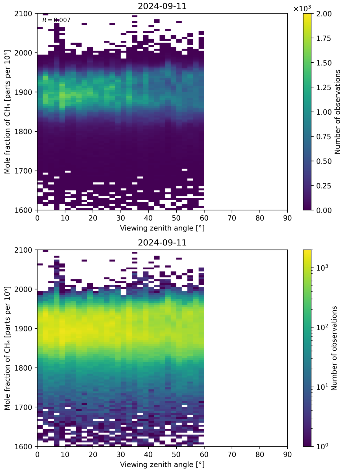
Figure 110: Scatter density plot of “Viewing zenith angle” against “Mole fraction of CH 4 ” for 2024-09-10 to 2024-09-12.
