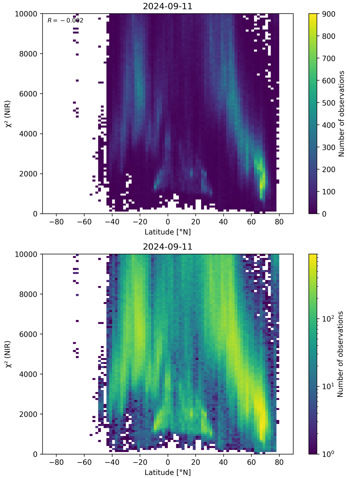
Figure 53: Scatter density plot of “Latitude” against “ \chi^2 (NIR)” for 2024-09-10 to 2024-09-12.
