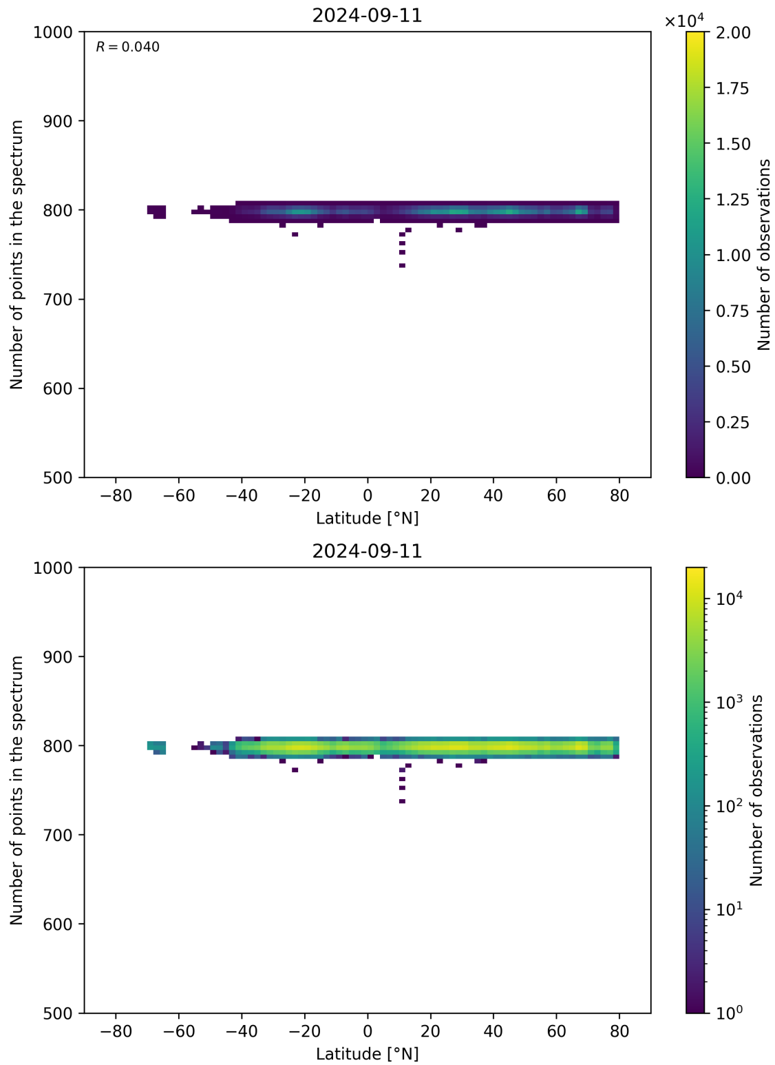
Figure 61: Scatter density plot of “Latitude” against “Number of points in the spectrum” for 2024-09-10 to 2024-09-12.
