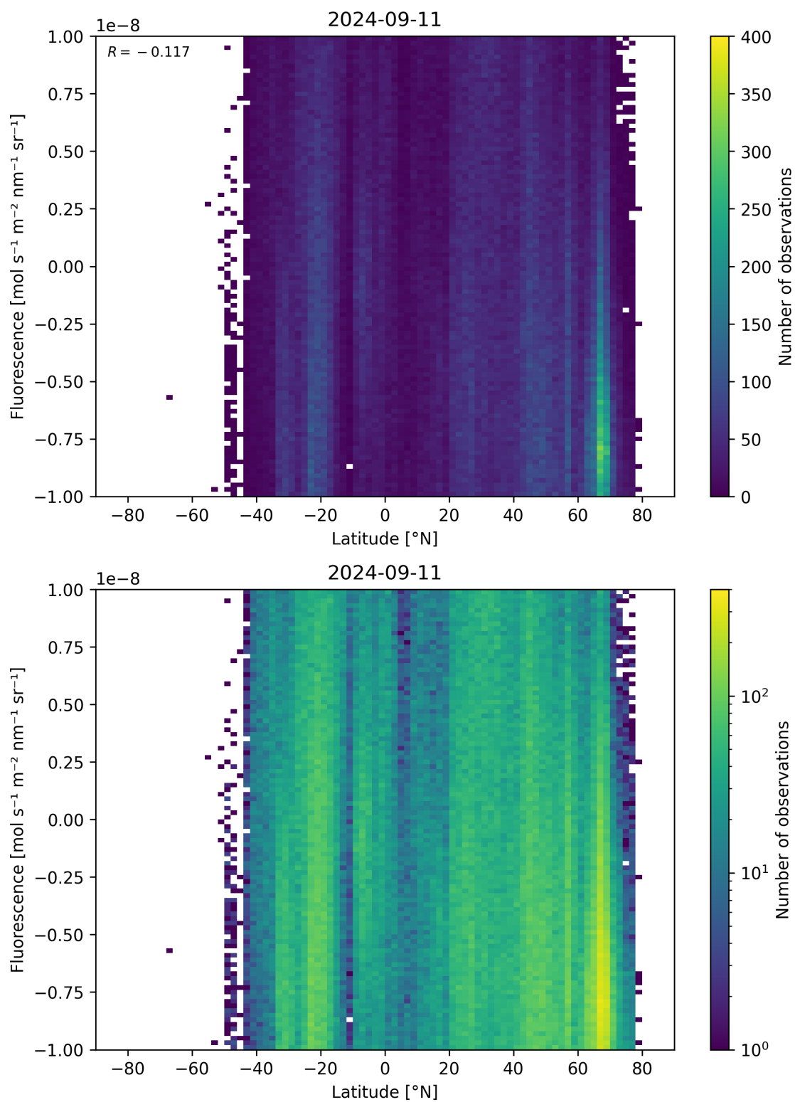
Figure 56: Scatter density plot of “Latitude” against “Fluorescence” for 2024-09-10 to 2024-09-12.
