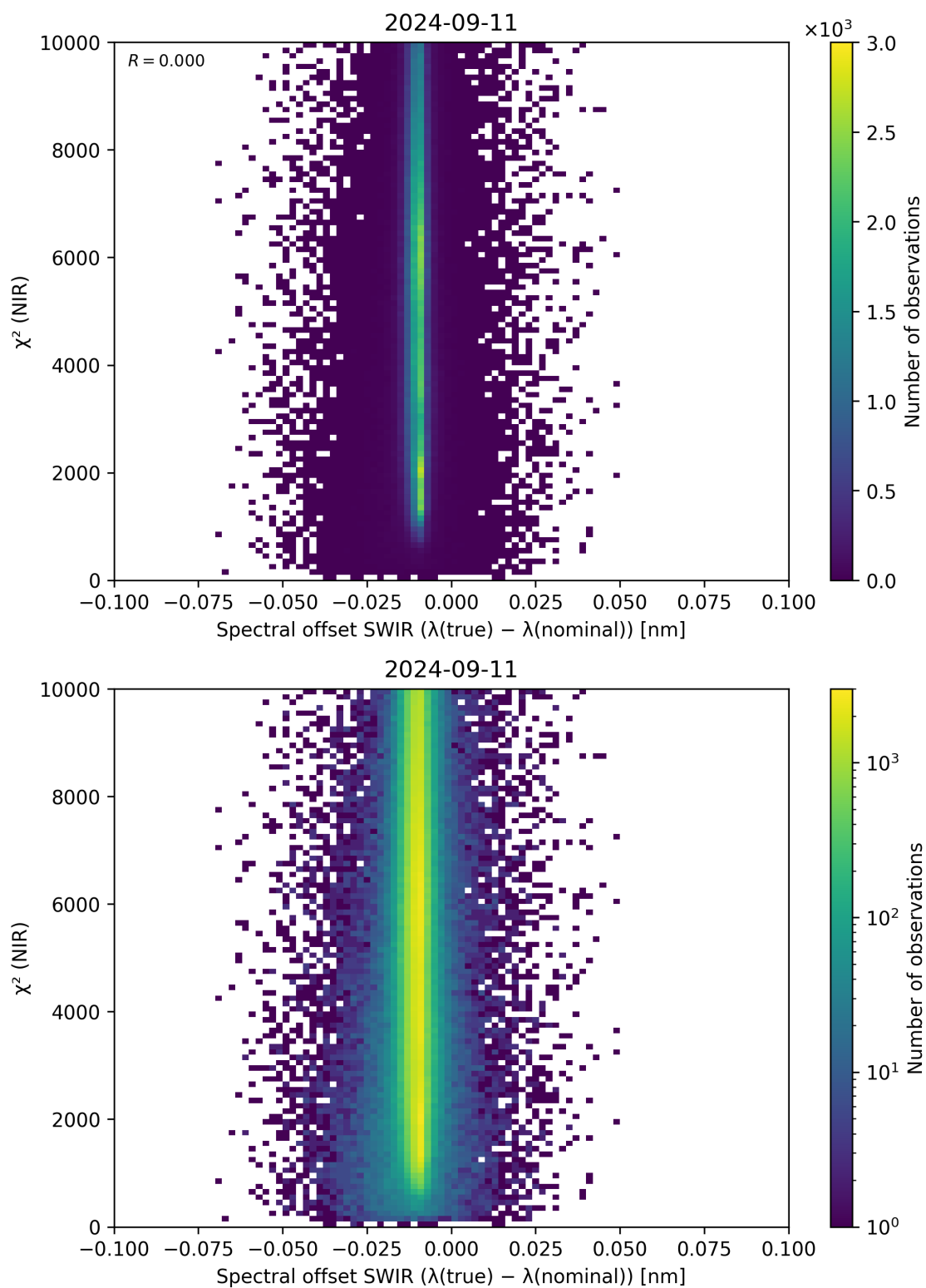
Figure 117: Scatter density plot of “Spectral offset SWIR ( \lambda_{\text{true}} - \lambda_{\text{nominal}} )” against “ \chi^2 (NIR)” for 2024-09-10 to 2024-09-12.
