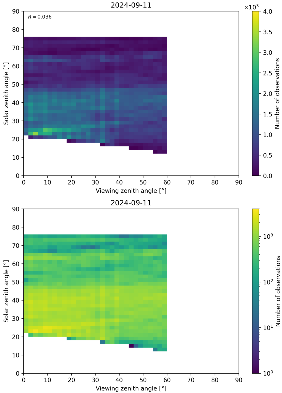
Figure 115: Scatter density plot of “Viewing zenith angle” against “Solar zenith angle” for 2024-09-10 to 2024-09-12.
