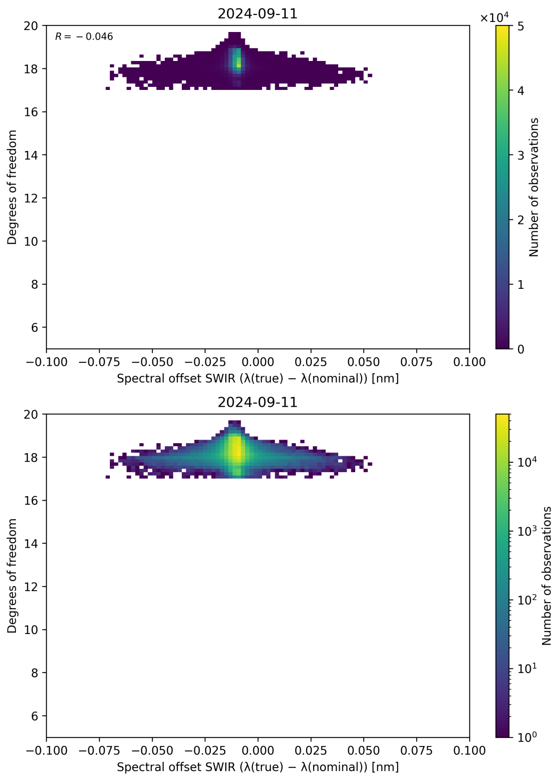
Figure 119: Scatter density plot of “Spectral offset SWIR ( \lambda_{\text{true}} - \lambda_{\text{nominal}} )” against “Degrees of freedom” for 2024-09-10 to 2024-09-12.
