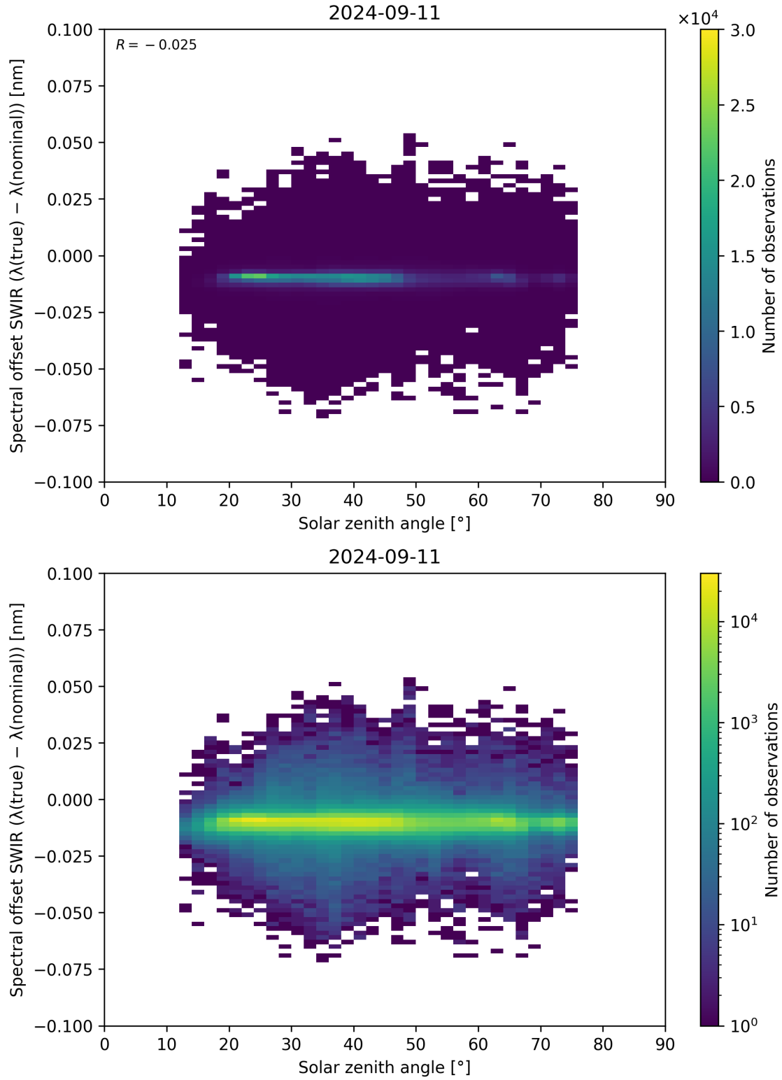
Figure 104: Scatter density plot of “Solar zenith angle” against “Spectral offset SWIR ( \lambda_{\text{true}} - \lambda_{\text{nominal}} )” for 2024-09-10 to 2024-09-12.
