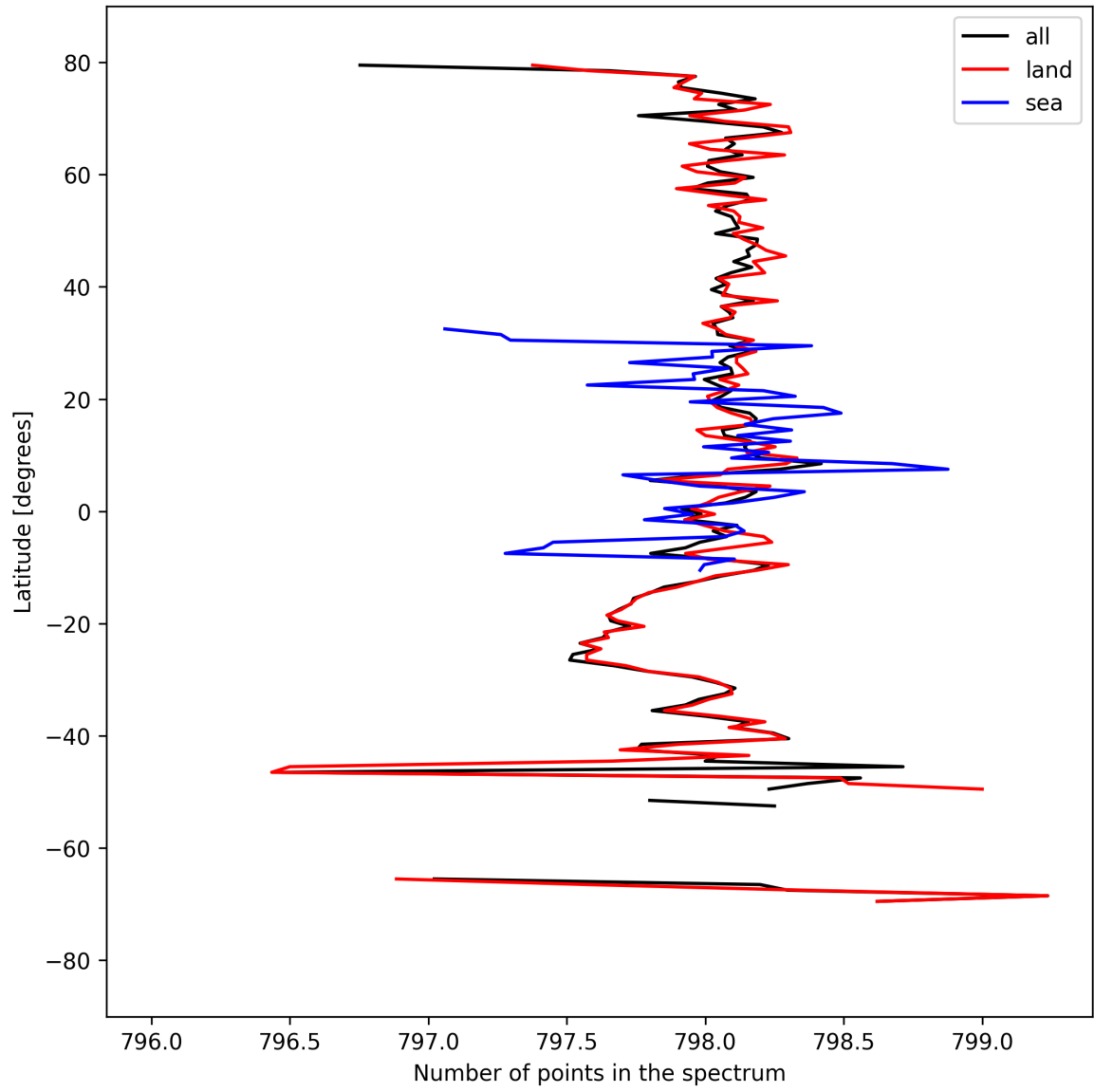
Figure 15: Zonal average of “Number of points in the spectrum” for 2024-09-10 to 2024-09-12.
