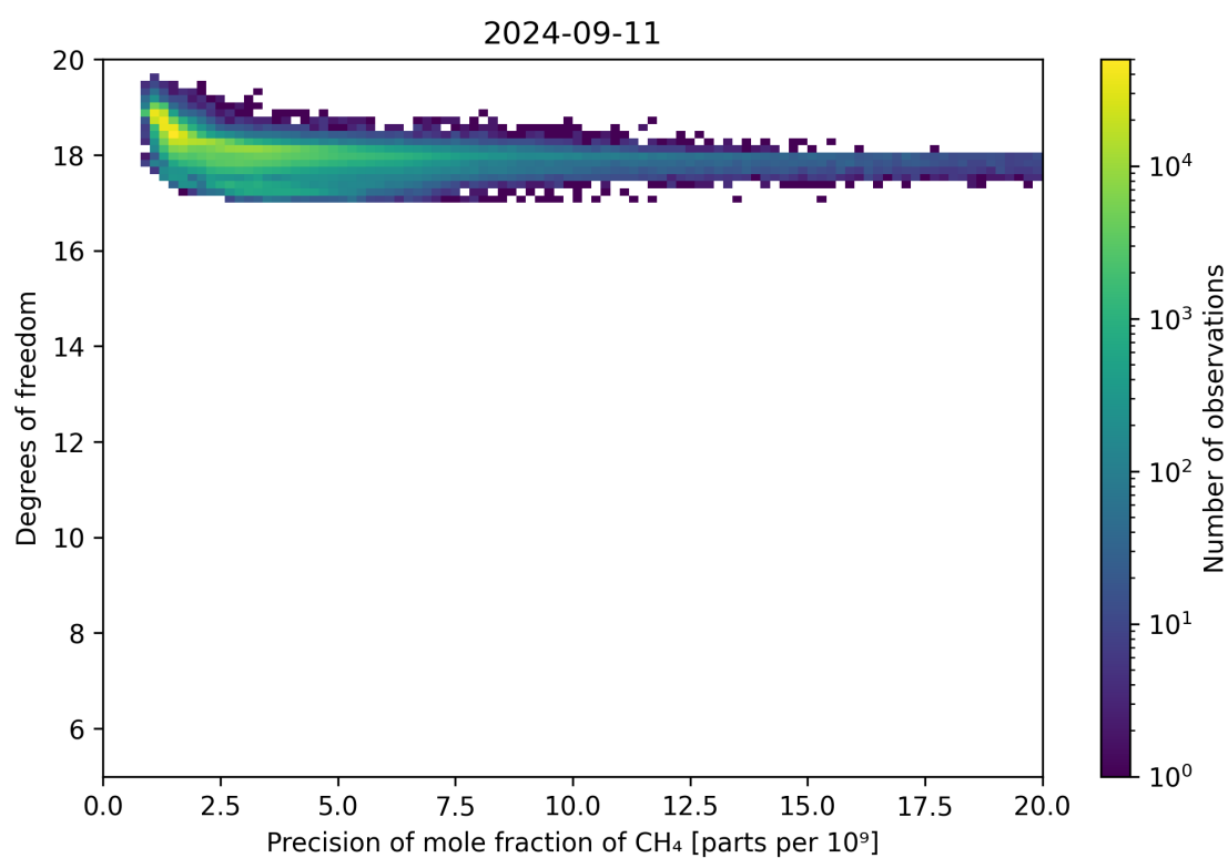
Figure 80: Scatter density plot of “Precision of mole fraction of CH 4 ” against “Degrees of freedom” for 2024-09-10 to 2024-09-12.
