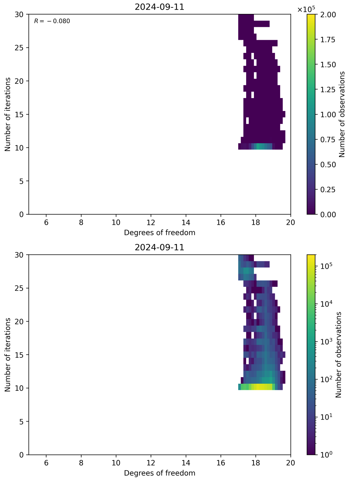
Figure 52: Scatter density plot of “Degrees of freedom” against “Number of iterations” for 2024-09-10 to 2024-09-12.
