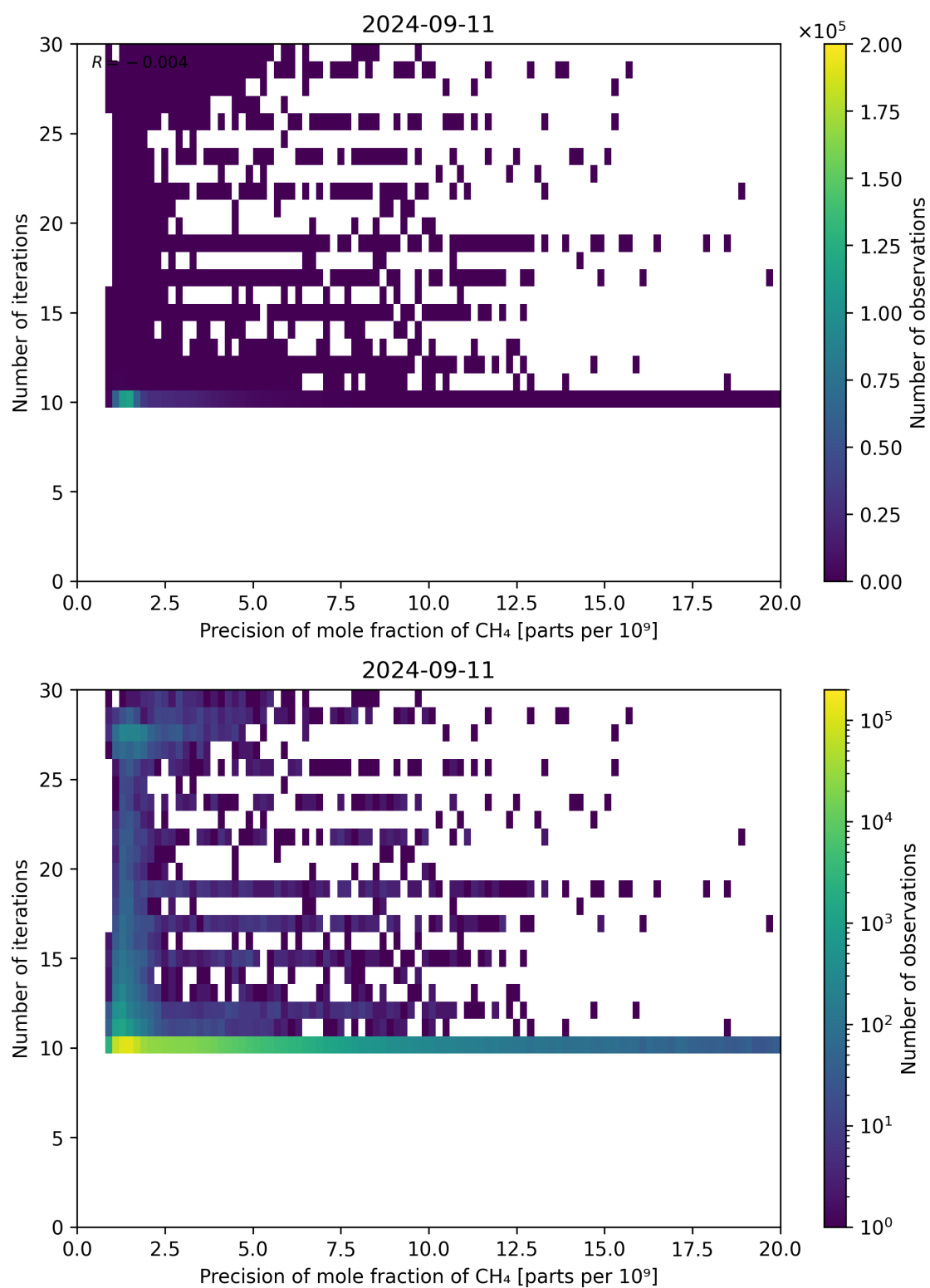
Figure 83: Scatter density plot of “Precision of mole fraction of CH 4 ” against “Number of iterations” for 2024-09-10 to 2024-09-12.
