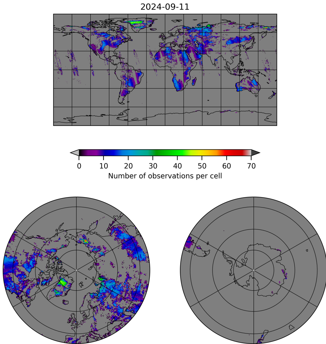
Figure 10: Map of the number of observations for 2024-09-10 to 2024-09-12
