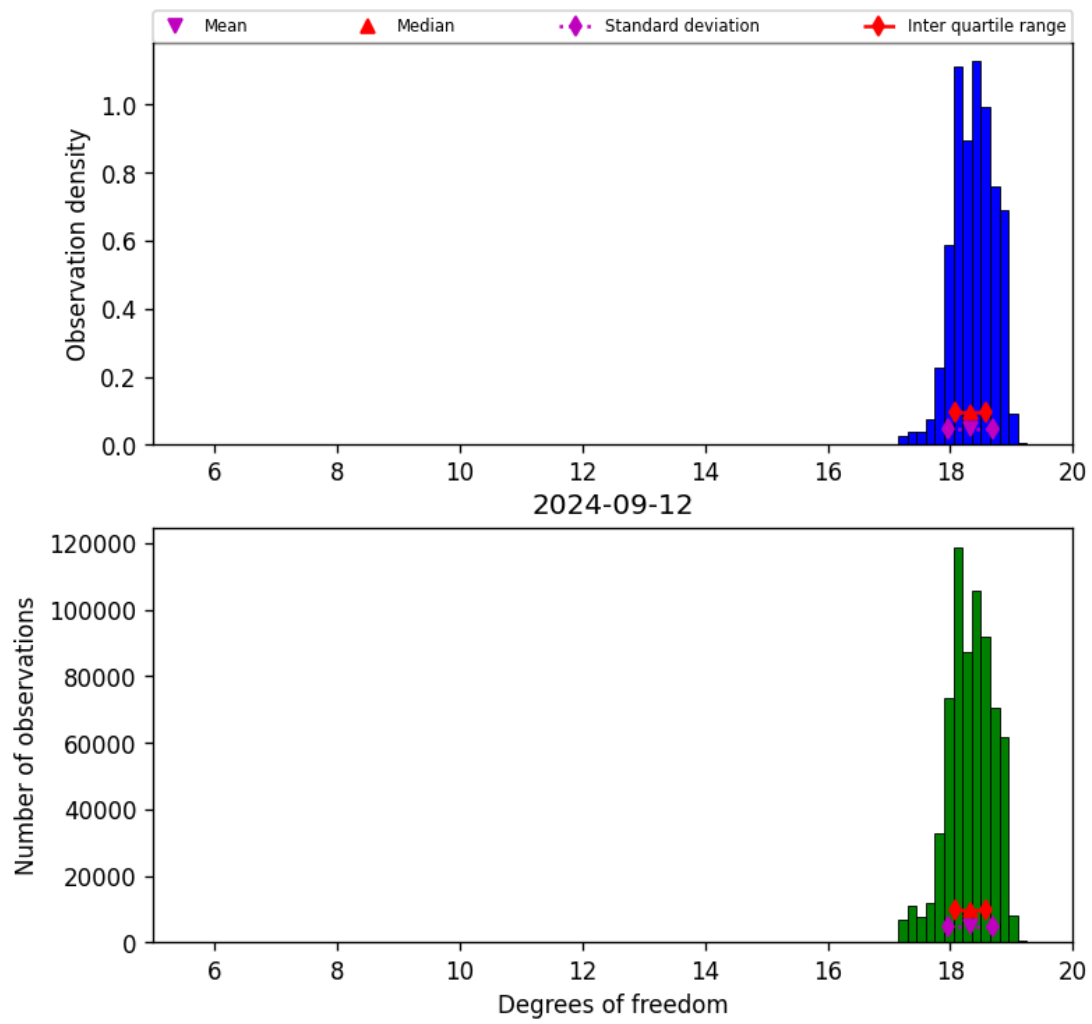
Figure 30: Histogram of “Degrees of freedom” for 2024-09-12 to 2024-09-13
