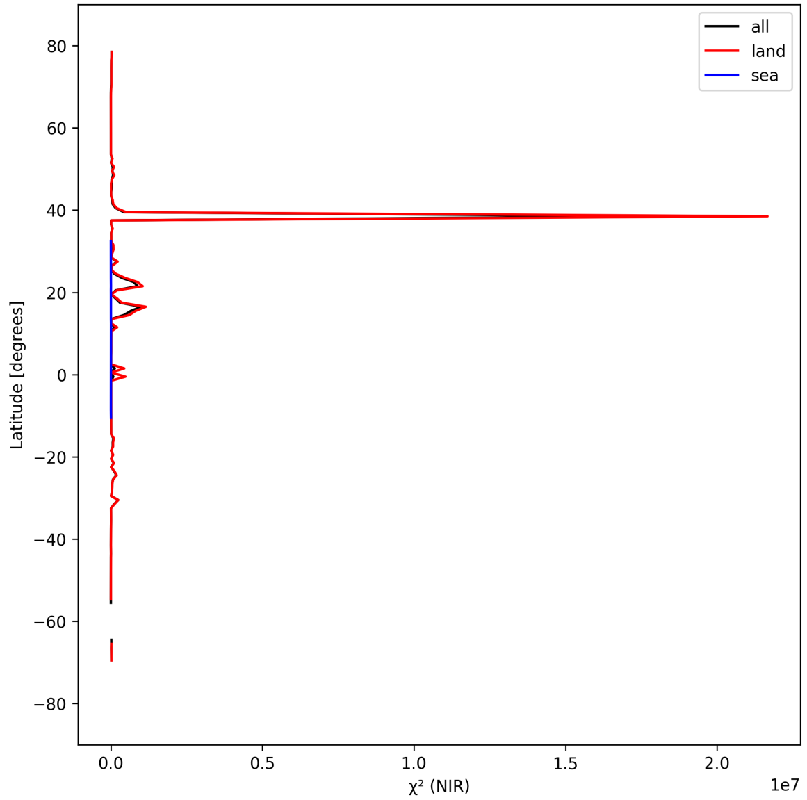
Figure 18: Zonal average of “ \chi^2 (NIR)” for 2024-09-12 to 2024-09-13.
