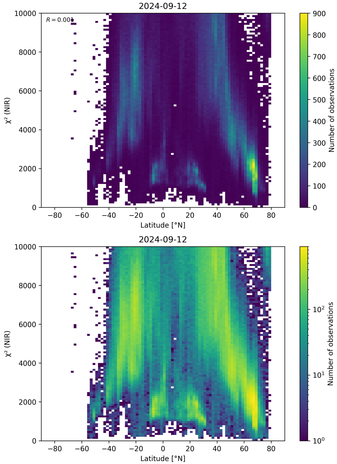
Figure 53: Scatter density plot of “Latitude” against “ \chi^2 (NIR)” for 2024-09-12 to 2024-09-13.
