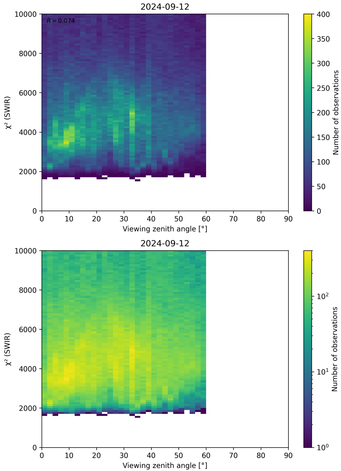
Figure 106: Scatter density plot of “Viewing zenith angle” against “ \chi^2 (SWIR)” for 2024-09-12 to 2024-09-13.
