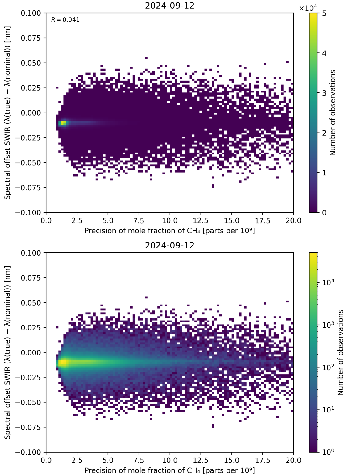
Figure 85: Scatter density plot of “Precision of mole fraction of \text{CH}_4 ” against “Spectral offset SWIR ( \lambda_{\text{true}} - \lambda_{\text{nominal}} )” for 2024-09-12 to 2024-09-13.
