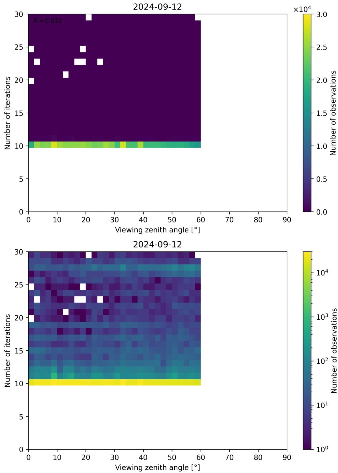
Figure 113: Scatter density plot of “Viewing zenith angle” against “Number of iterations” for 2024-09-12 to 2024-09-13.
