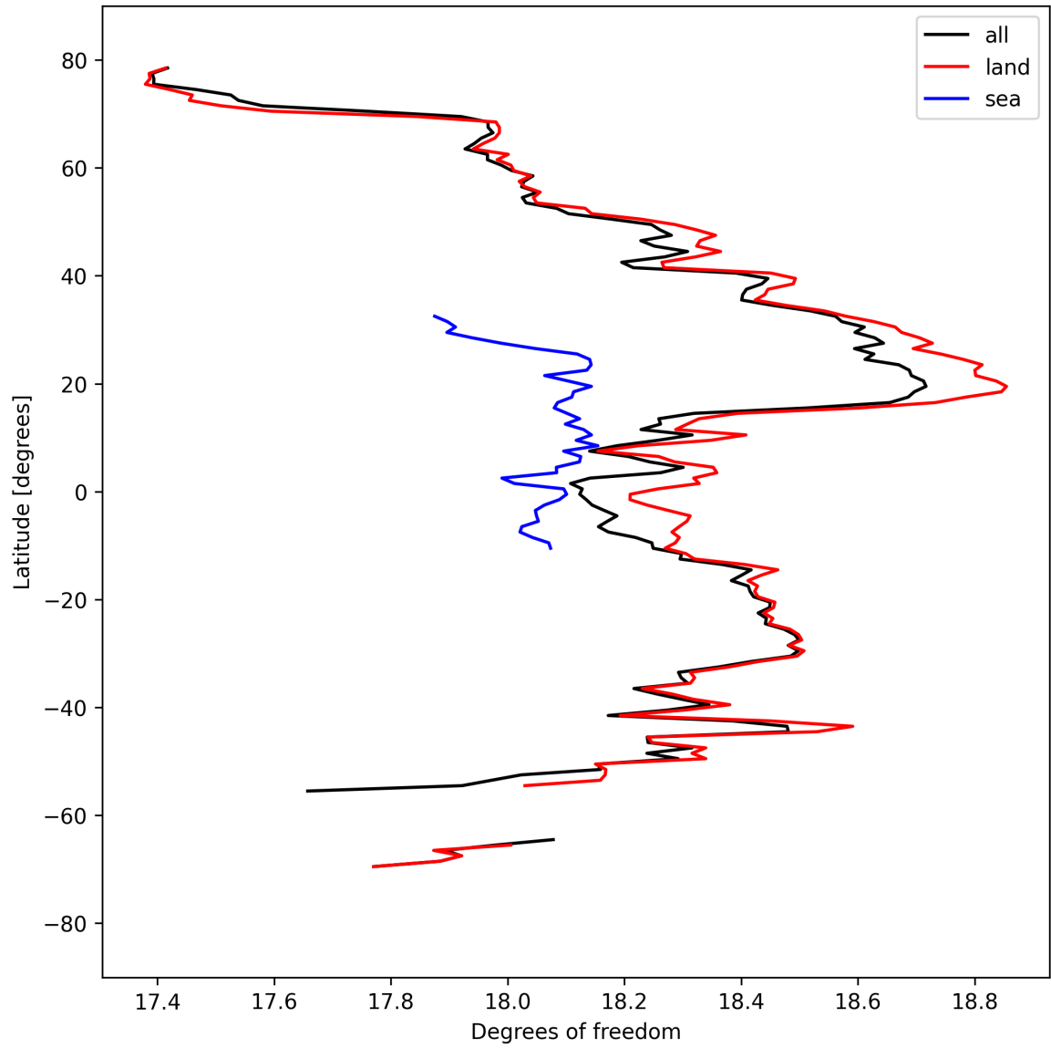
Figure 19: Zonal average of “Degrees of freedom” for 2024-09-12 to 2024-09-13.
