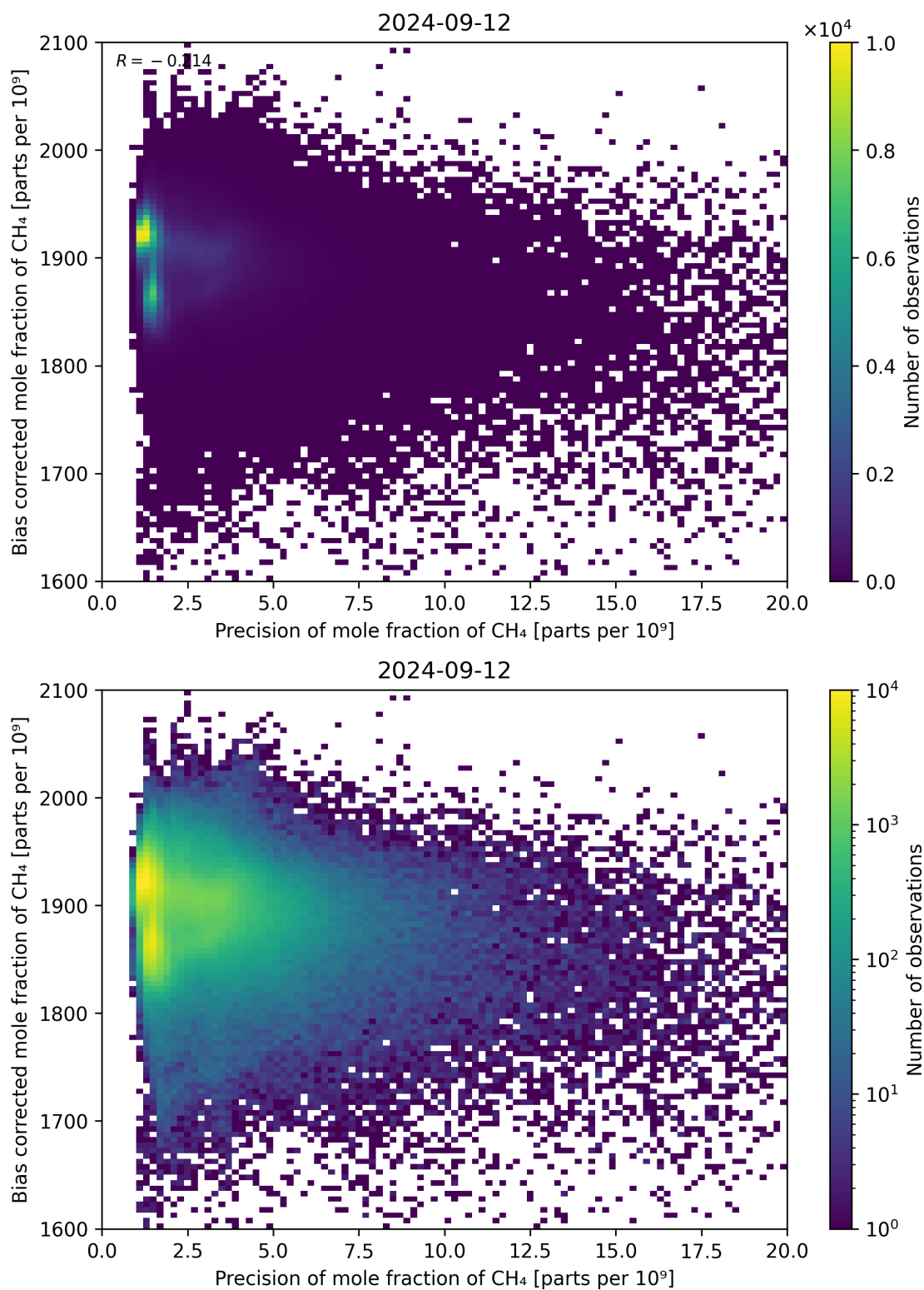
Figure 82: Scatter density plot of “Precision of mole fraction of CH 4 ” against “Bias corrected mole fraction of CH 4 ” for 2024-09-12 to 2024-09-13.
