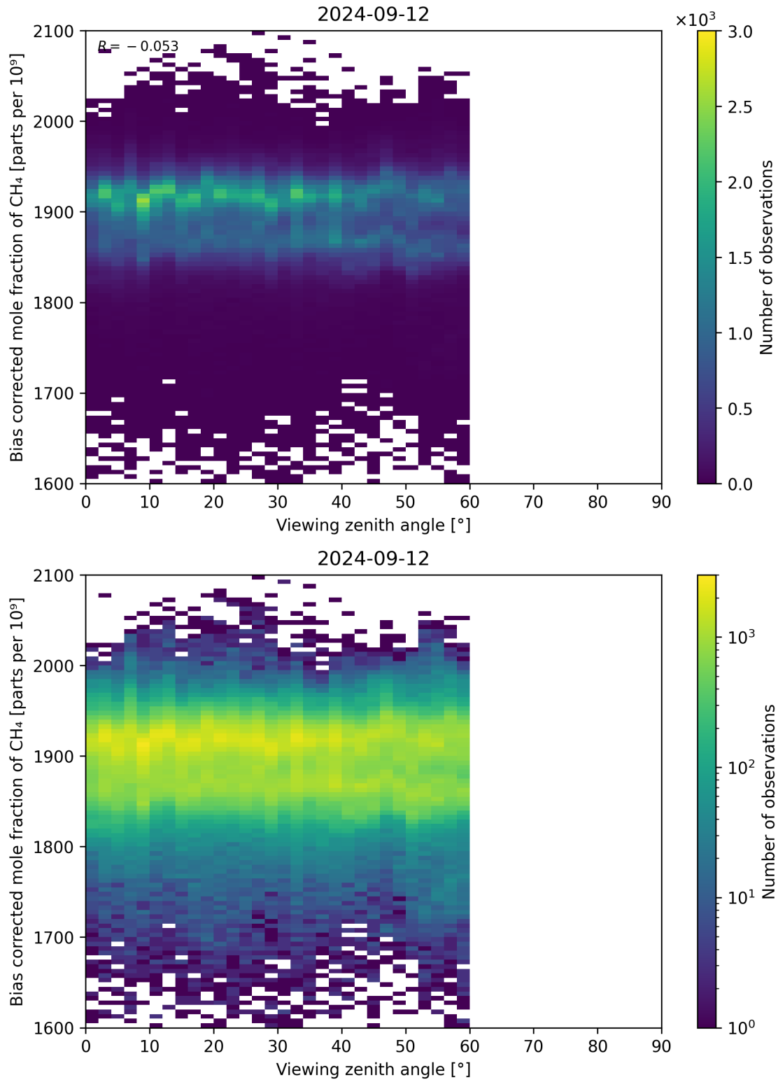
Figure 111: Scatter density plot of “Viewing zenith angle” against “Bias corrected mole fraction of CH 4 ” for 2024-09-12 to 2024-09-13.
