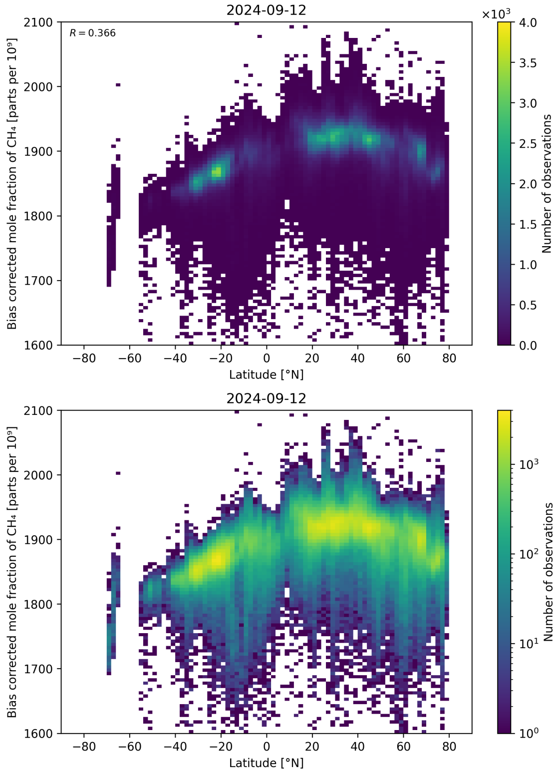
Figure 58: Scatter density plot of “Latitude” against “Bias corrected mole fraction of CH 4 ” for 2024-09-12 to 2024-09-13.
