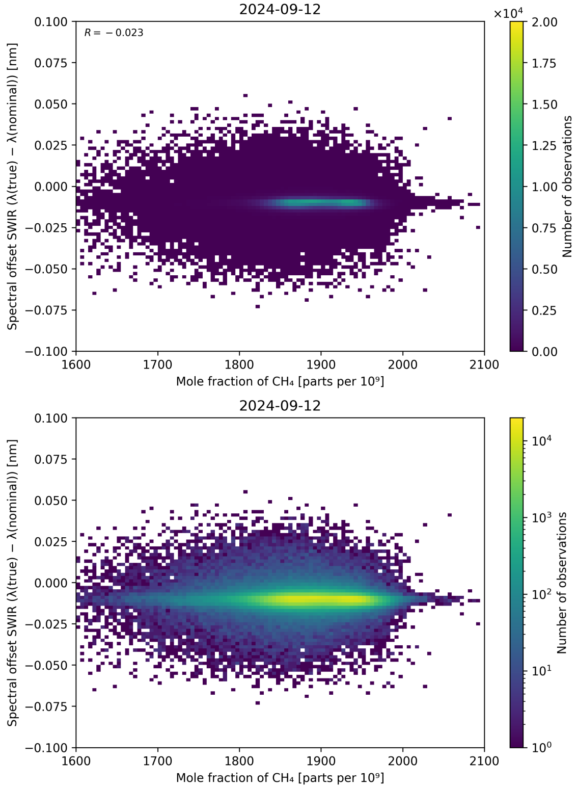
Figure 86: Scatter density plot of “Mole fraction of \text{CH}_4 ” against “Spectral offset SWIR ( \lambda_{\text{true}} - \lambda_{\text{nominal}} )” for 2024-09-12 to 2024-09-13.
