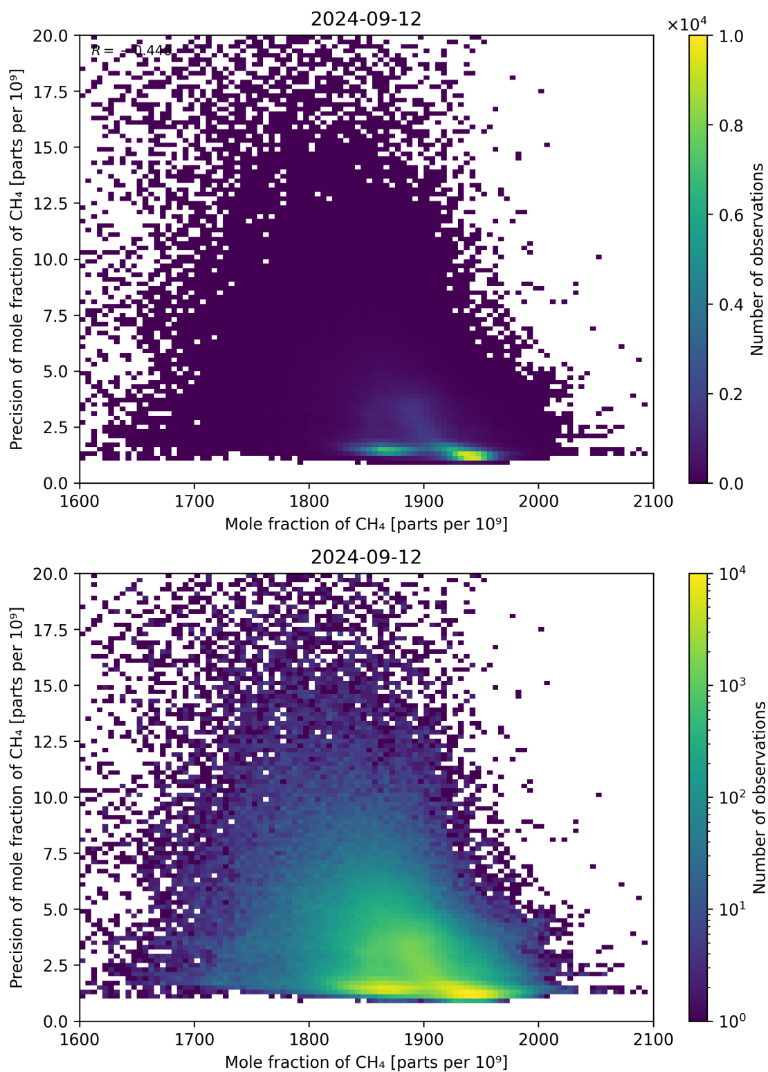
Figure 75: Scatter density plot of “Mole fraction of CH 4 ” against “Precision of mole fraction of CH 4 ” for 2024-09-12 to 2024-09-13.
