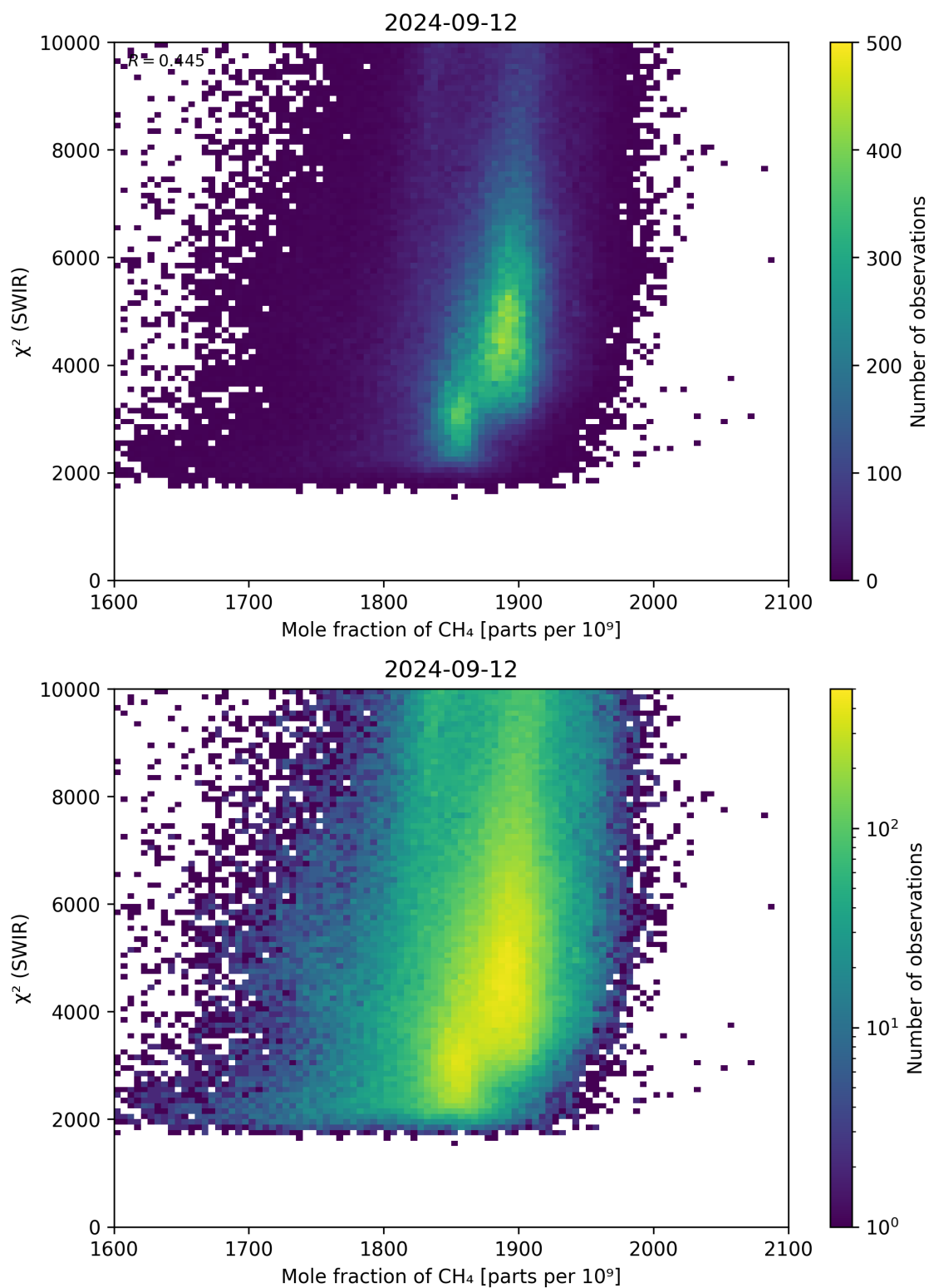
Figure 71: Scatter density plot of “Mole fraction of \text{CH}_4 ” against “ \chi^2 (SWIR)” for 2024-09-12 to 2024-09-13.
