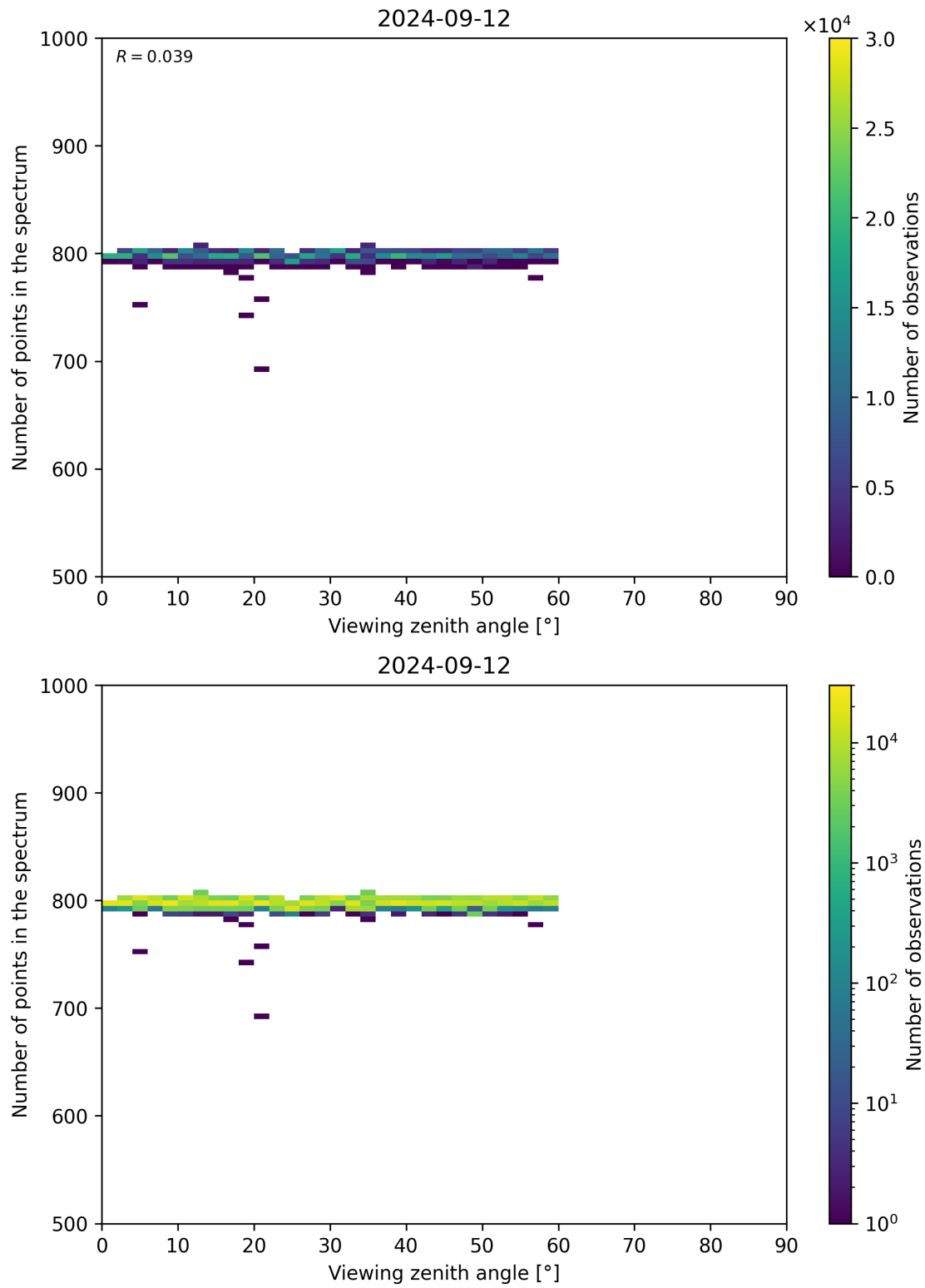
Figure 114: Scatter density plot of “Viewing zenith angle” against “Number of points in the spectrum” for 2024-09-12 to 2024-09-13.
