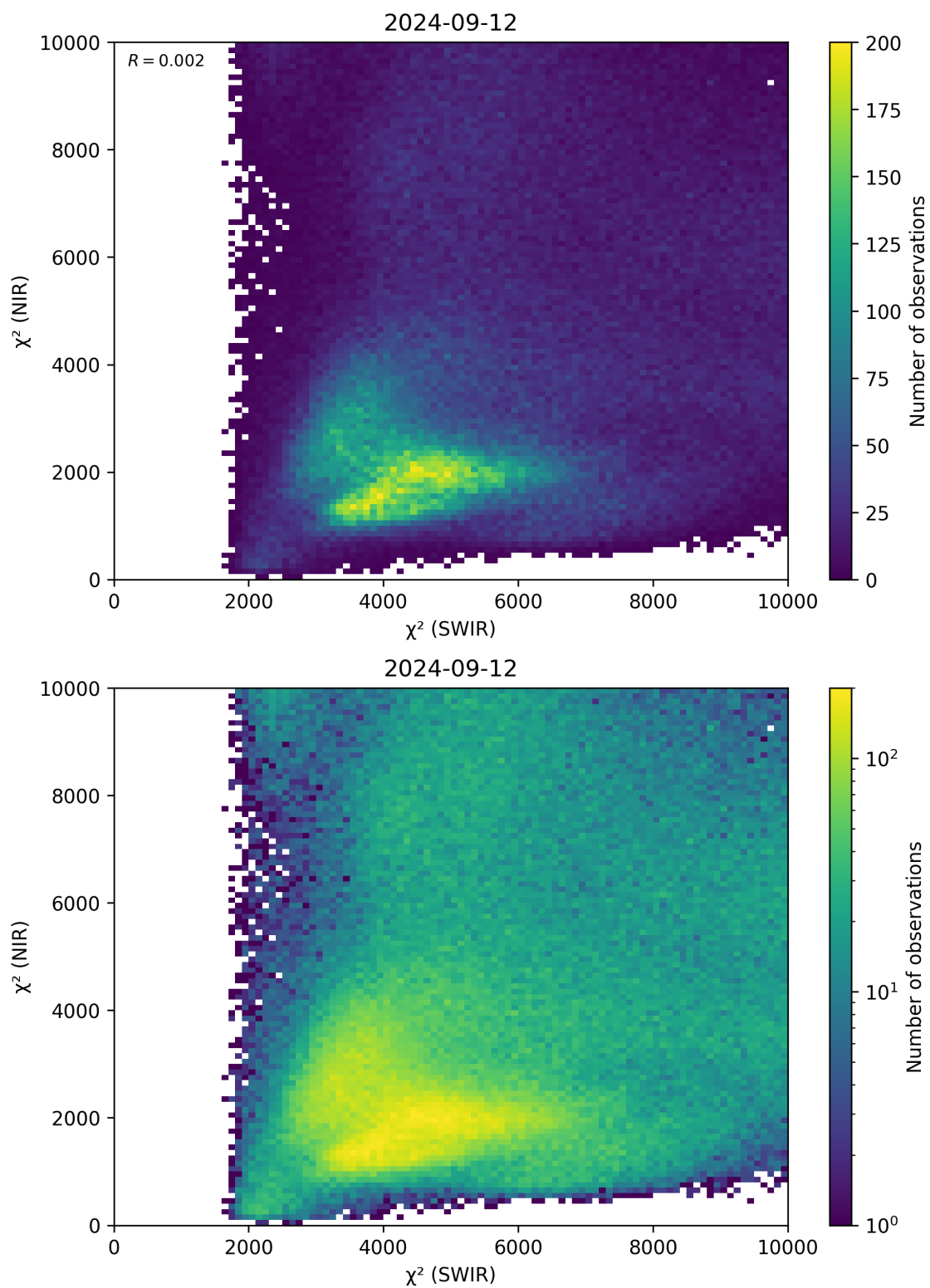
Figure 47: Scatter density plot of “ \chi^2 (SWIR)” against “ \chi^2 (NIR)” for 2024-09-12 to 2024-09-13.
