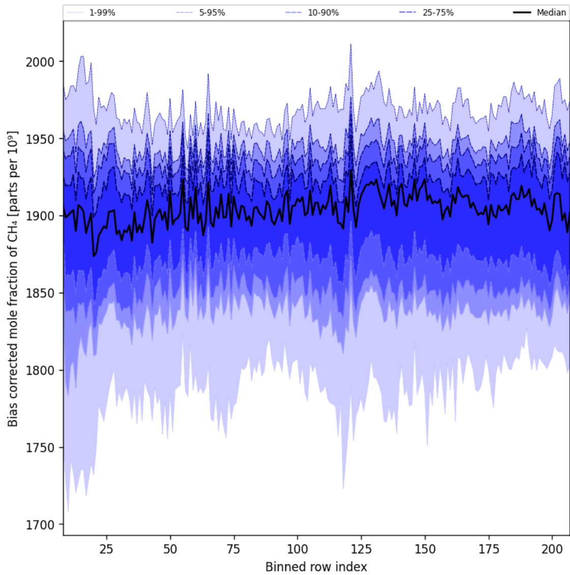
Figure 36: Along track statistics of “Bias corrected mole fraction of CH 4 ” for 2024-09-12 to 2024-09-13
