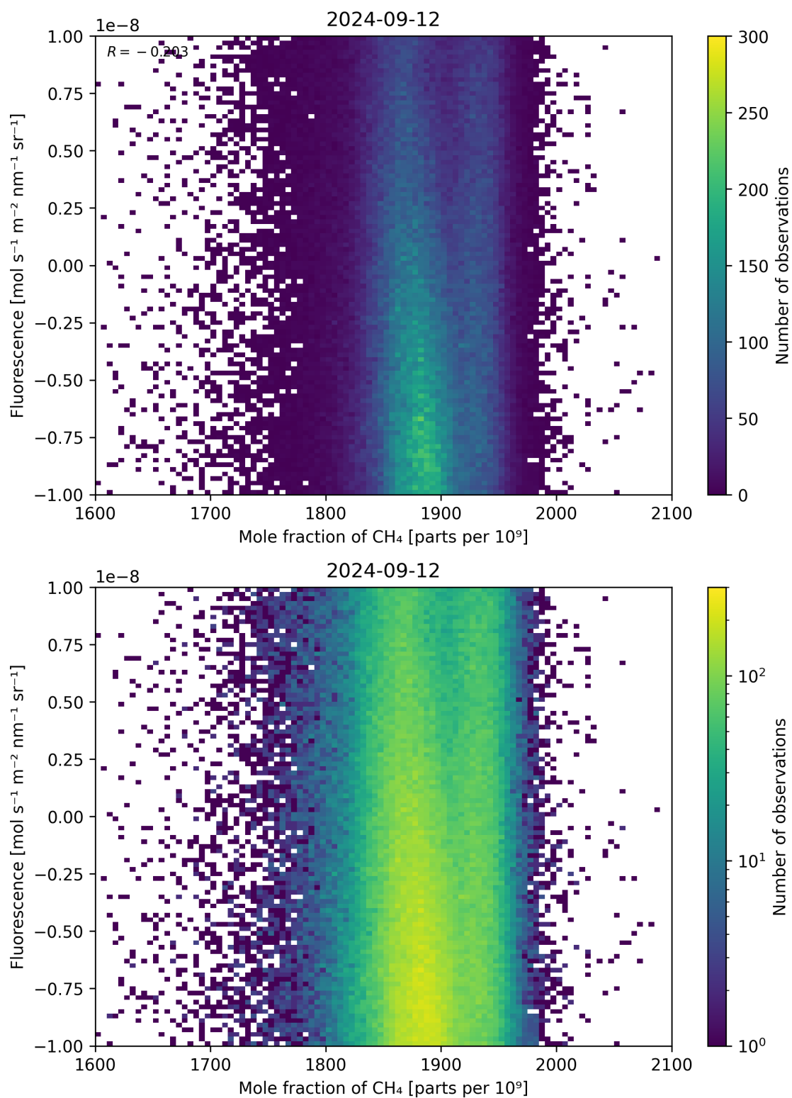
Figure 73: Scatter density plot of “Mole fraction of \text{CH}_4 ” against “Fluorescence” for 2024-09-12 to 2024-09-13.
