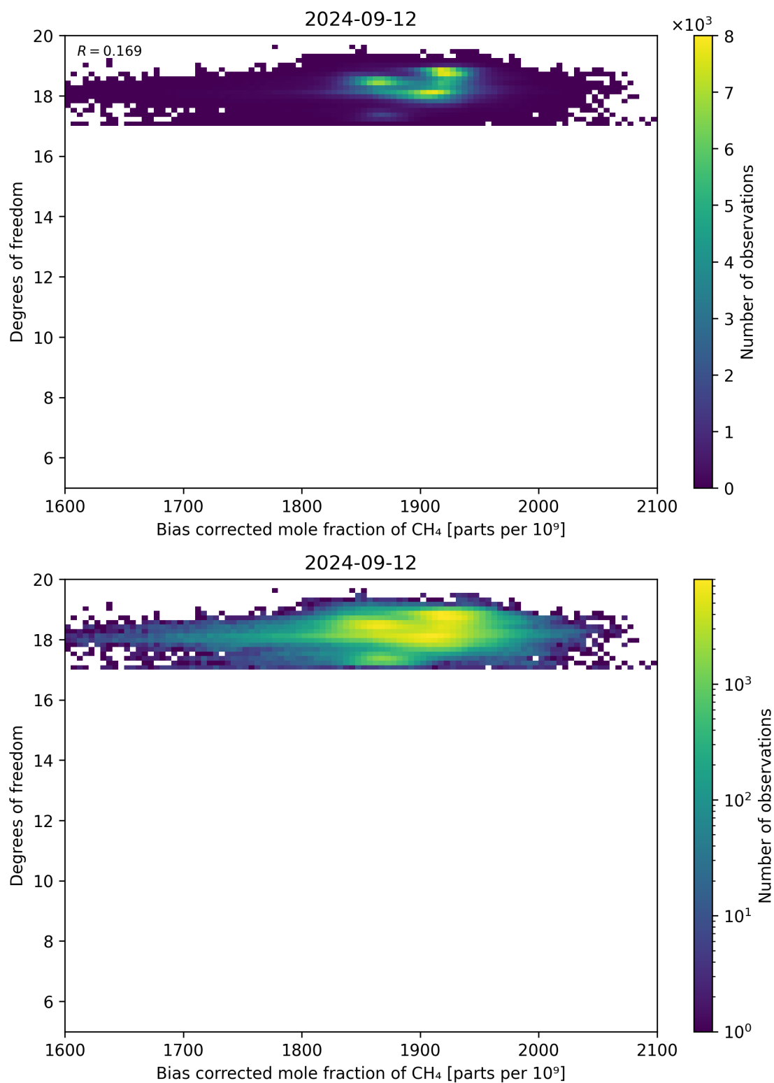
Figure 65: Scatter density plot of “Bias corrected mole fraction of CH 4 ” against “Degrees of freedom” for 2024-09-12 to 2024-09-13.
