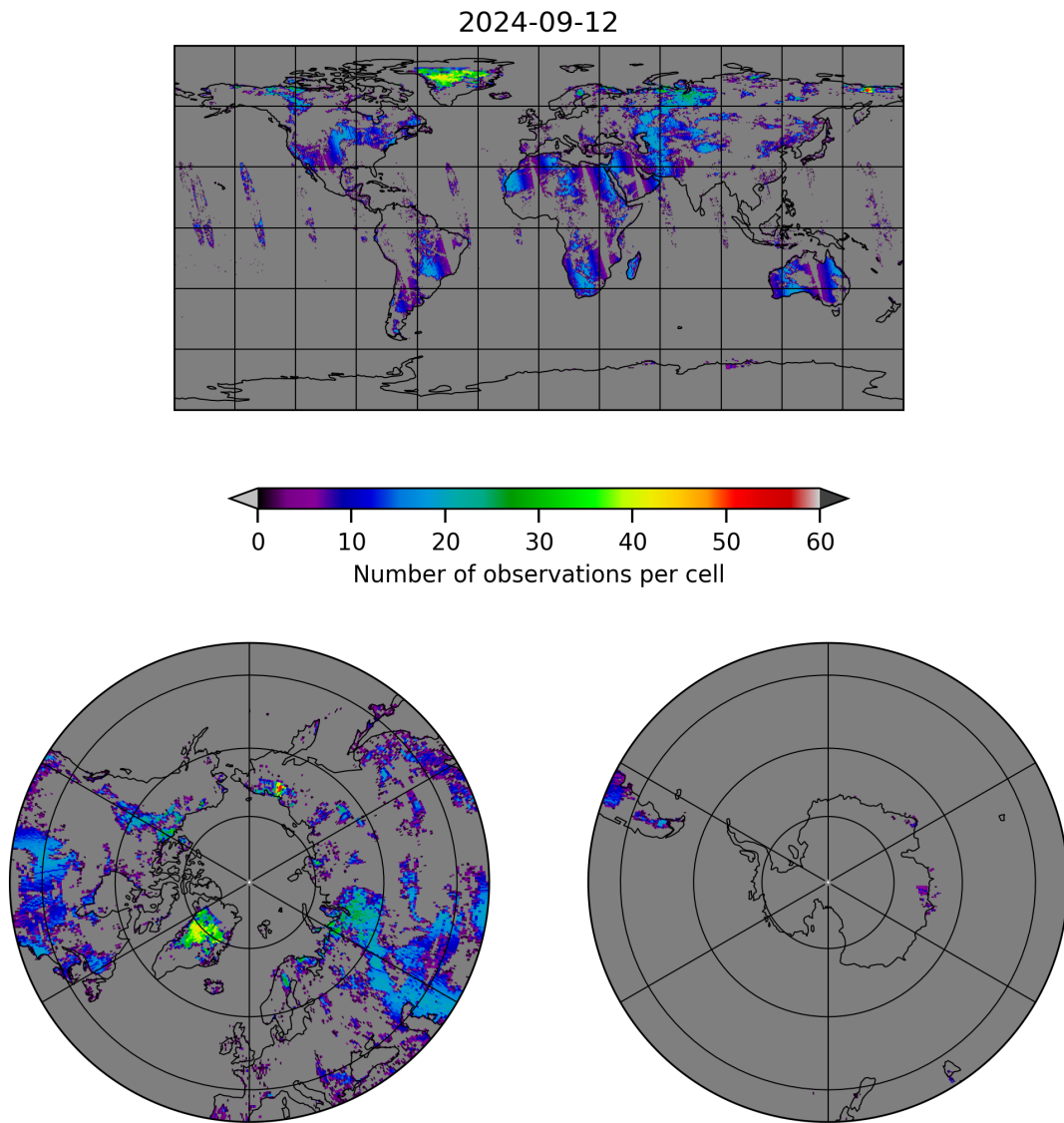
Figure 10: Map of the number of observations for 2024-09-12 to 2024-09-13
