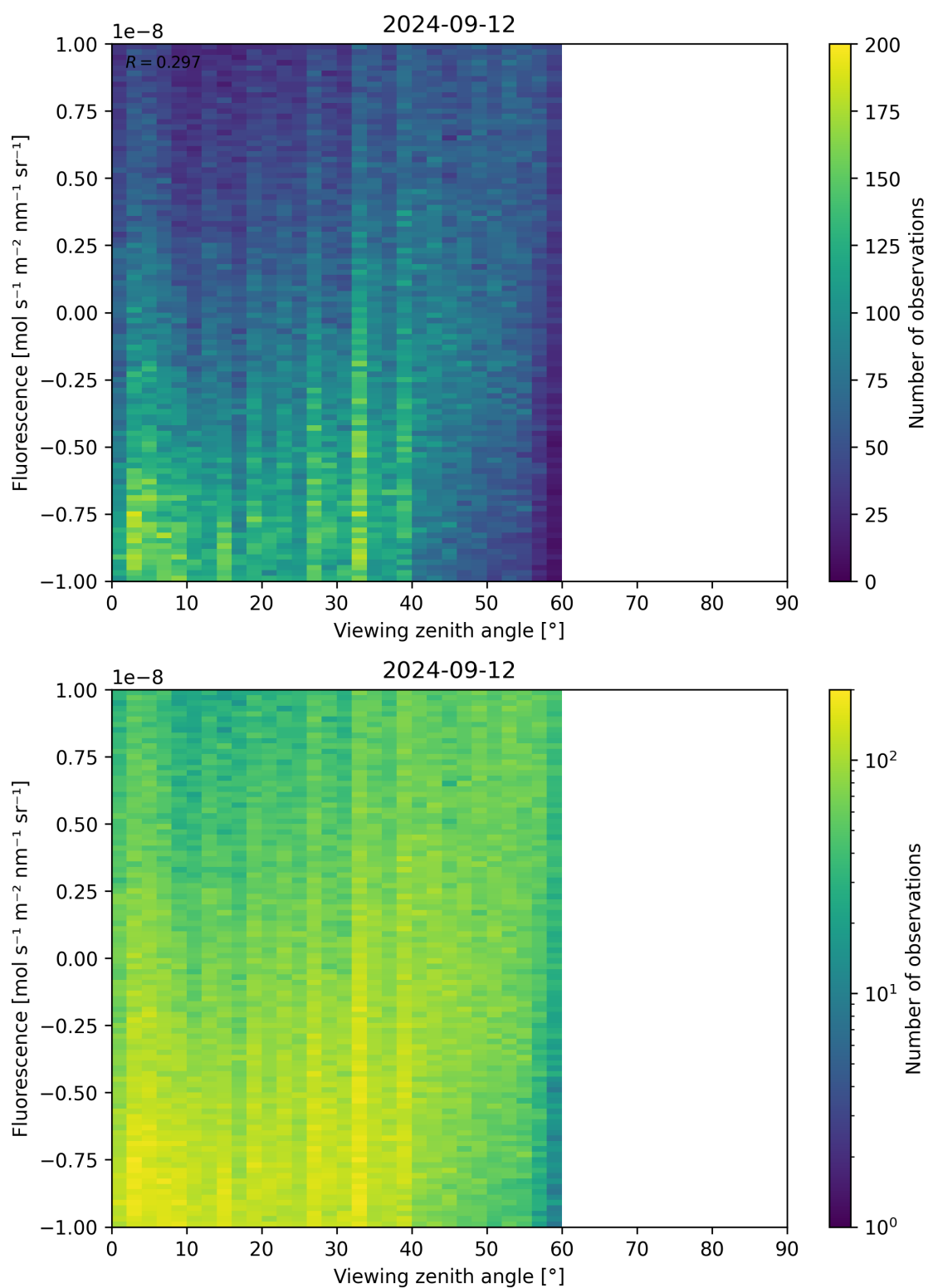
Figure 108: Scatter density plot of “Viewing zenith angle” against “Fluorescence” for 2024-09-12 to 2024-09-13.
