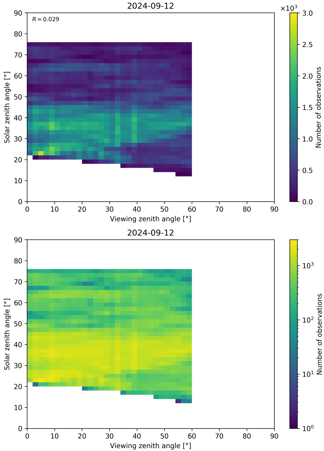
Figure 115: Scatter density plot of “Viewing zenith angle” against “Solar zenith angle” for 2024-09-12 to 2024-09-13.
