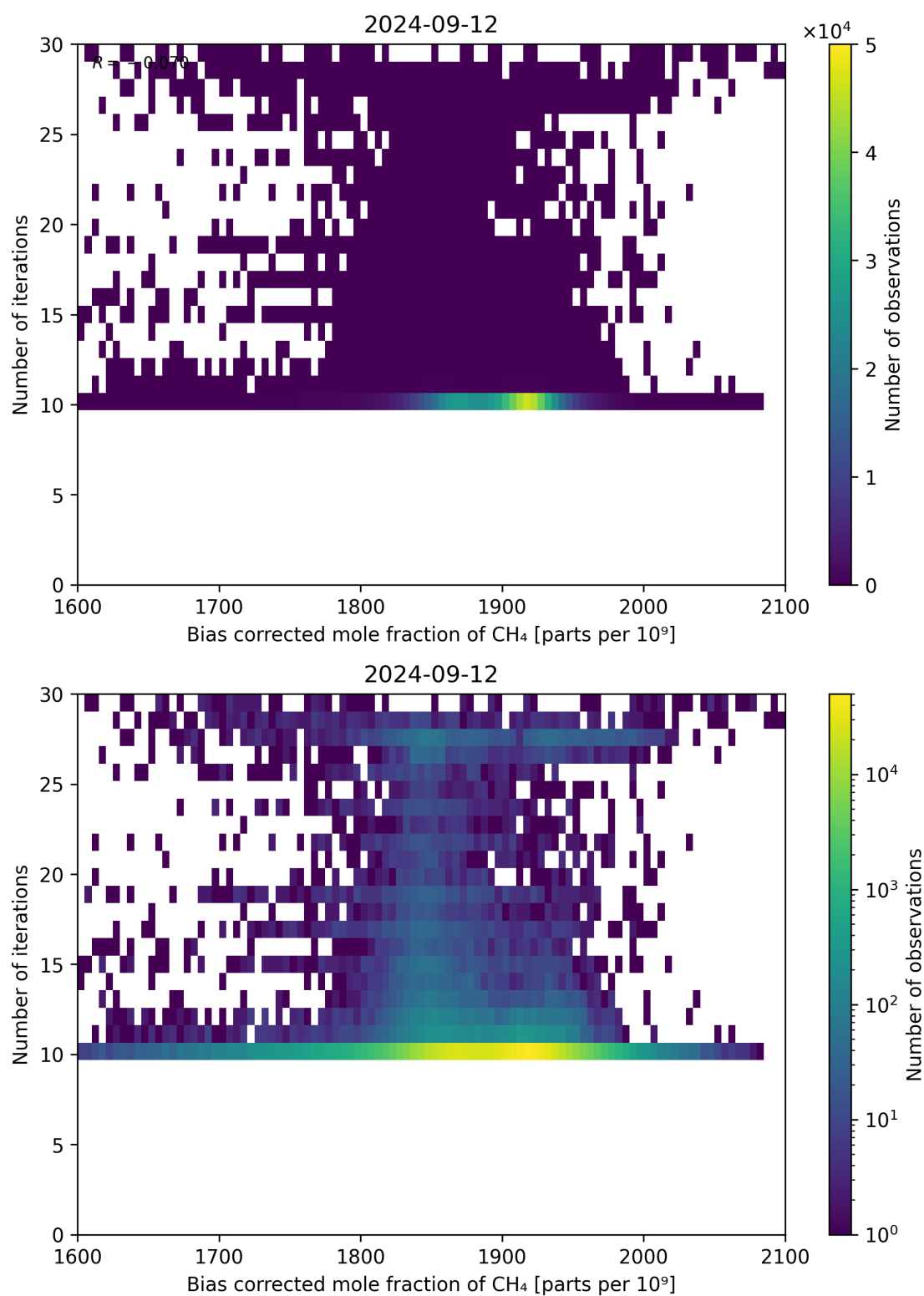
Figure 67: Scatter density plot of “Bias corrected mole fraction of \text{CH}_4 ” against “Number of iterations” for 2024-09-12 to 2024-09-13.
