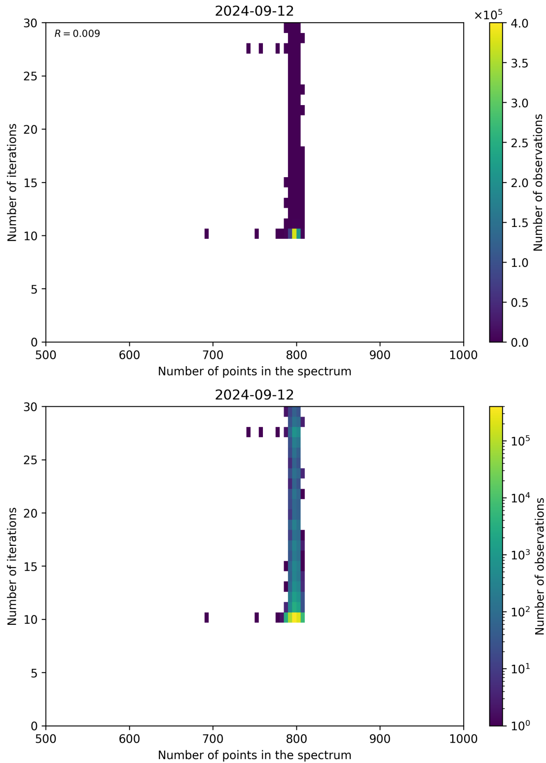
Figure 92: Scatter density plot of “Number of points in the spectrum” against “Number of iterations” for 2024-09-12 to 2024-09-13.
