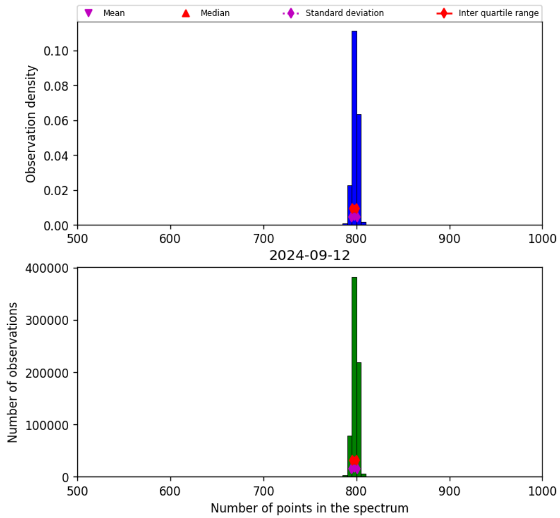
Figure 26: Histogram of “Number of points in the spectrum” for 2024-09-12 to 2024-09-13
