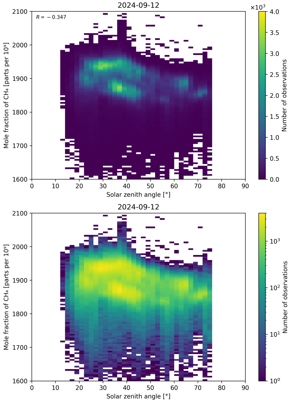
Figure 99: Scatter density plot of “Solar zenith angle” against “Mole fraction of CH 4 ” for 2024-09-12 to 2024-09-13.
