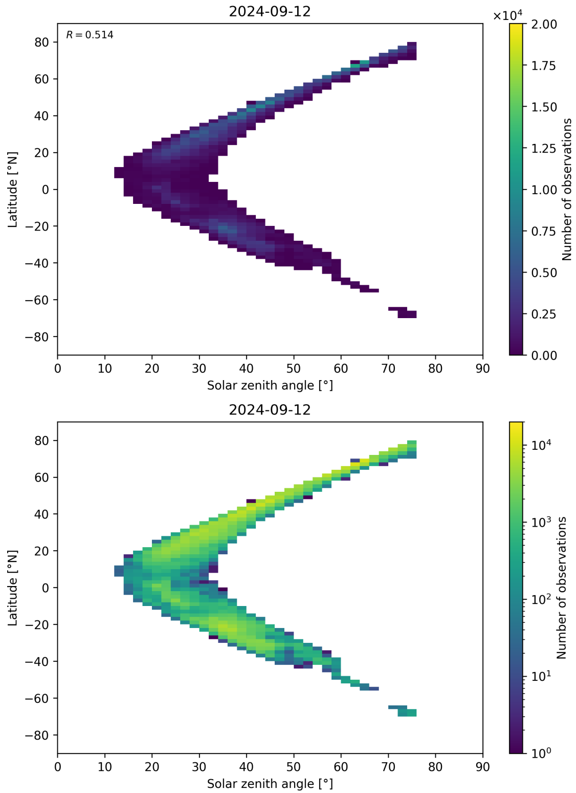
Figure 98: Scatter density plot of “Solar zenith angle” against “Latitude” for 2024-09-12 to 2024-09-13.
