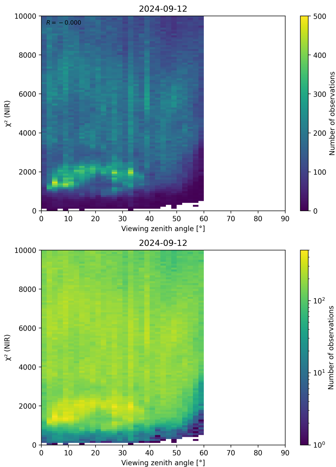
Figure 105: Scatter density plot of “Viewing zenith angle” against “ \chi^2 (NIR)” for 2024-09-12 to 2024-09-13.
