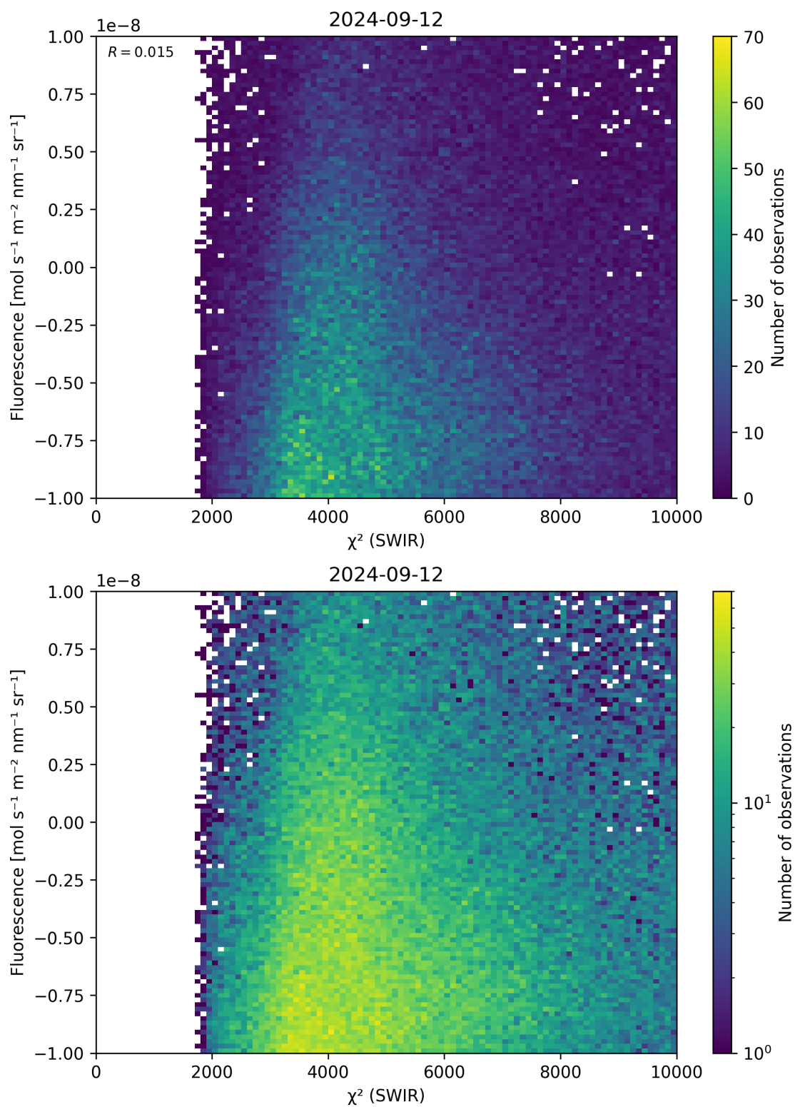
Figure 49: Scatter density plot of “ \chi^2 (SWIR)” against “Fluorescence” for 2024-09-12 to 2024-09-13.
