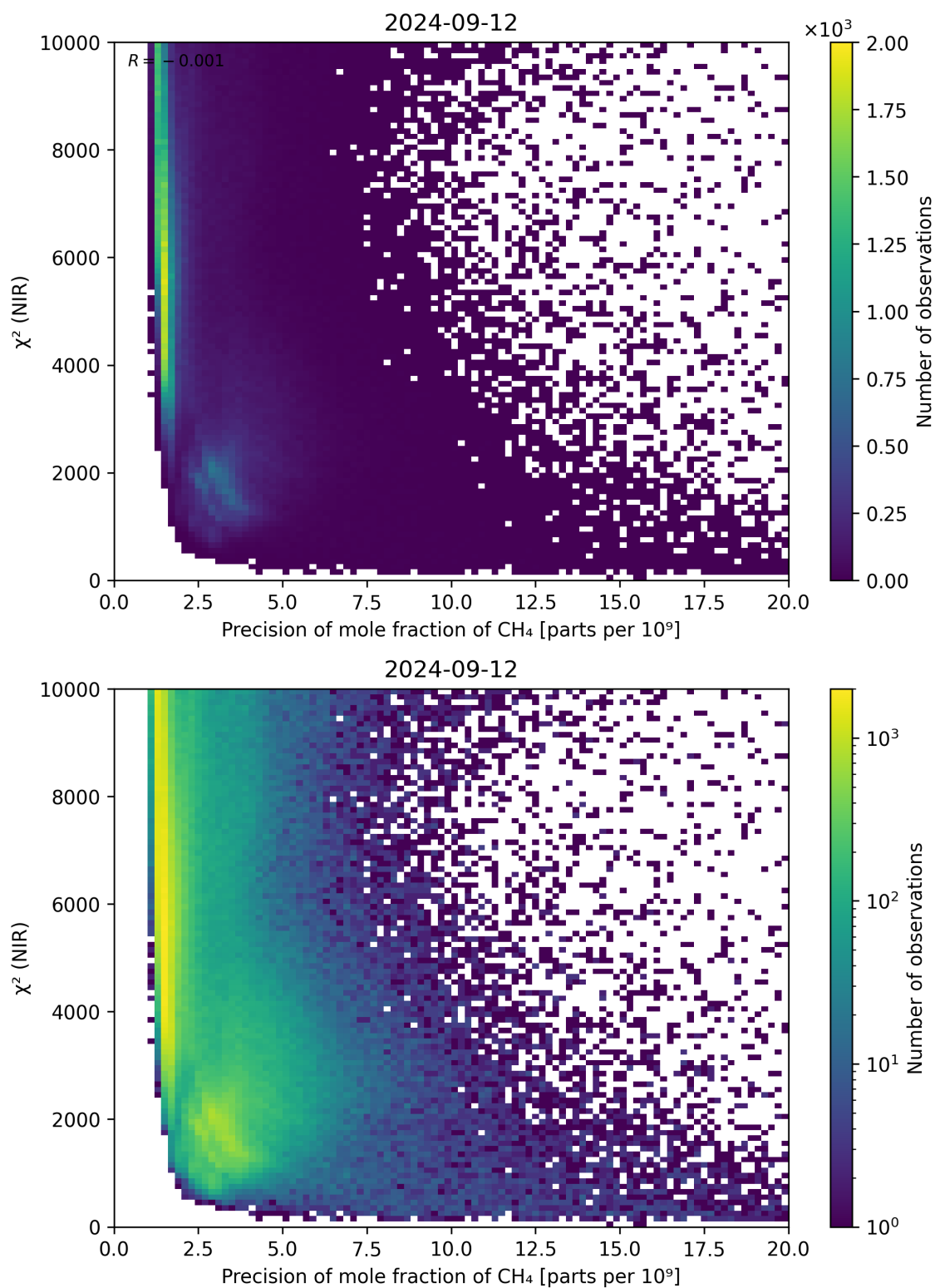
Figure 78: Scatter density plot of “Precision of mole fraction of CH 4 ” against “ \chi^2 (NIR)” for 2024-09-12 to 2024-09-13.
