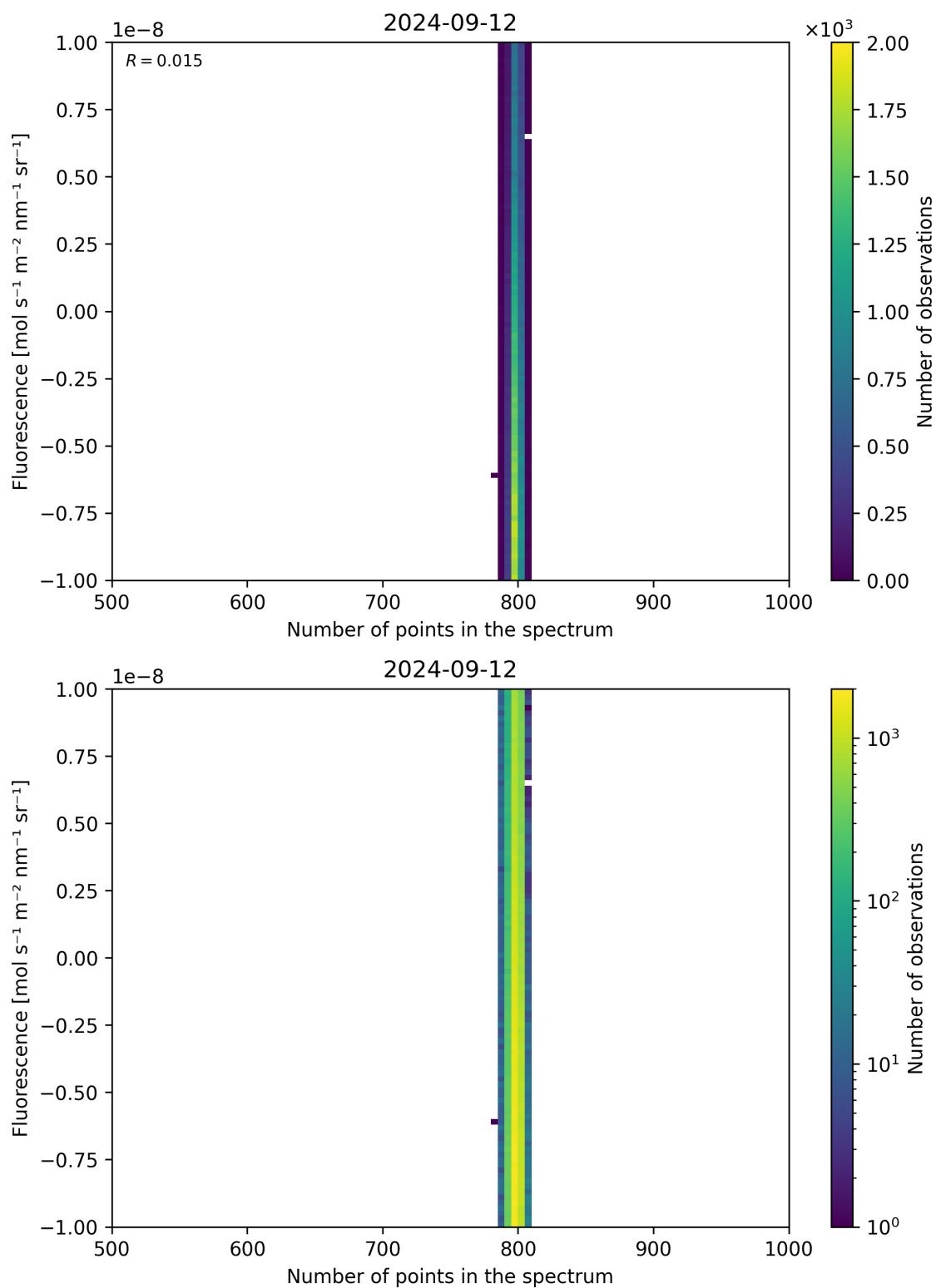
Figure 91: Scatter density plot of “Number of points in the spectrum” against “Fluorescence” for 2024-09-12 to 2024-09-13.
