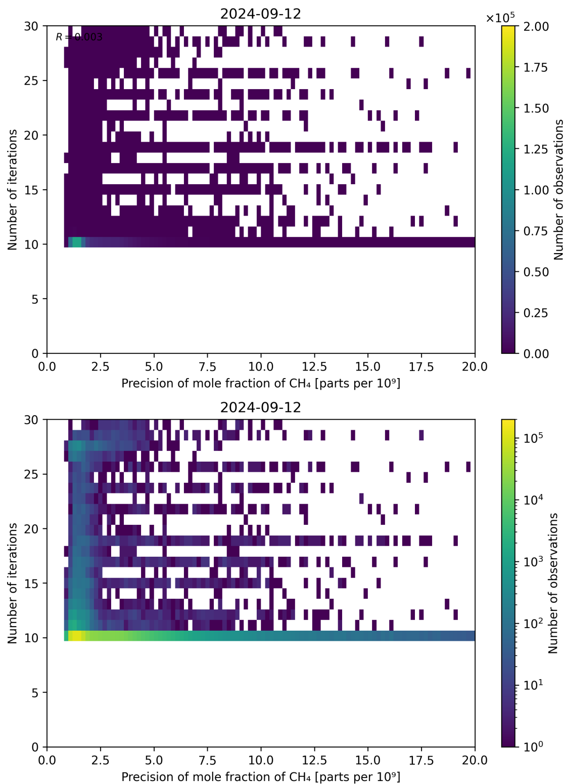
Figure 83: Scatter density plot of “Precision of mole fraction of CH 4 ” against “Number of iterations” for 2024-09-12 to 2024-09-13.
