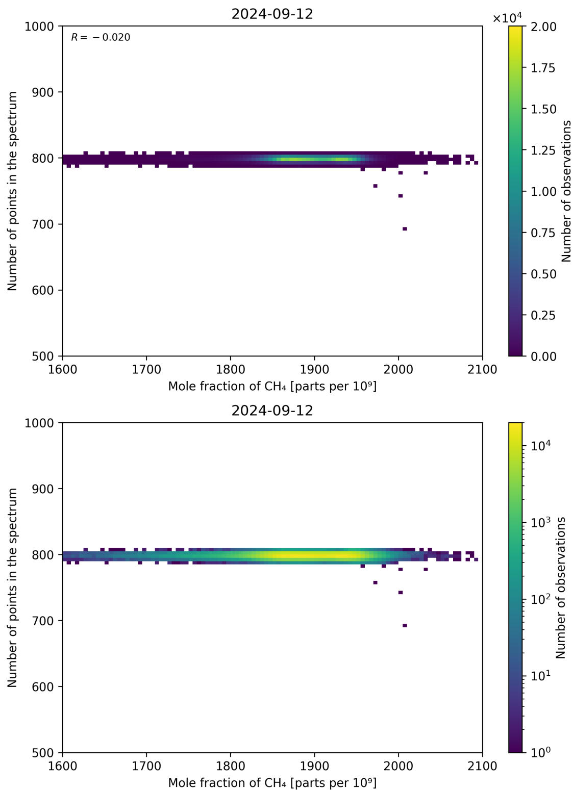
Figure 77: Scatter density plot of “Mole fraction of CH 4 ” against “Number of points in the spectrum” for 2024-09-12 to 2024-09-13.
