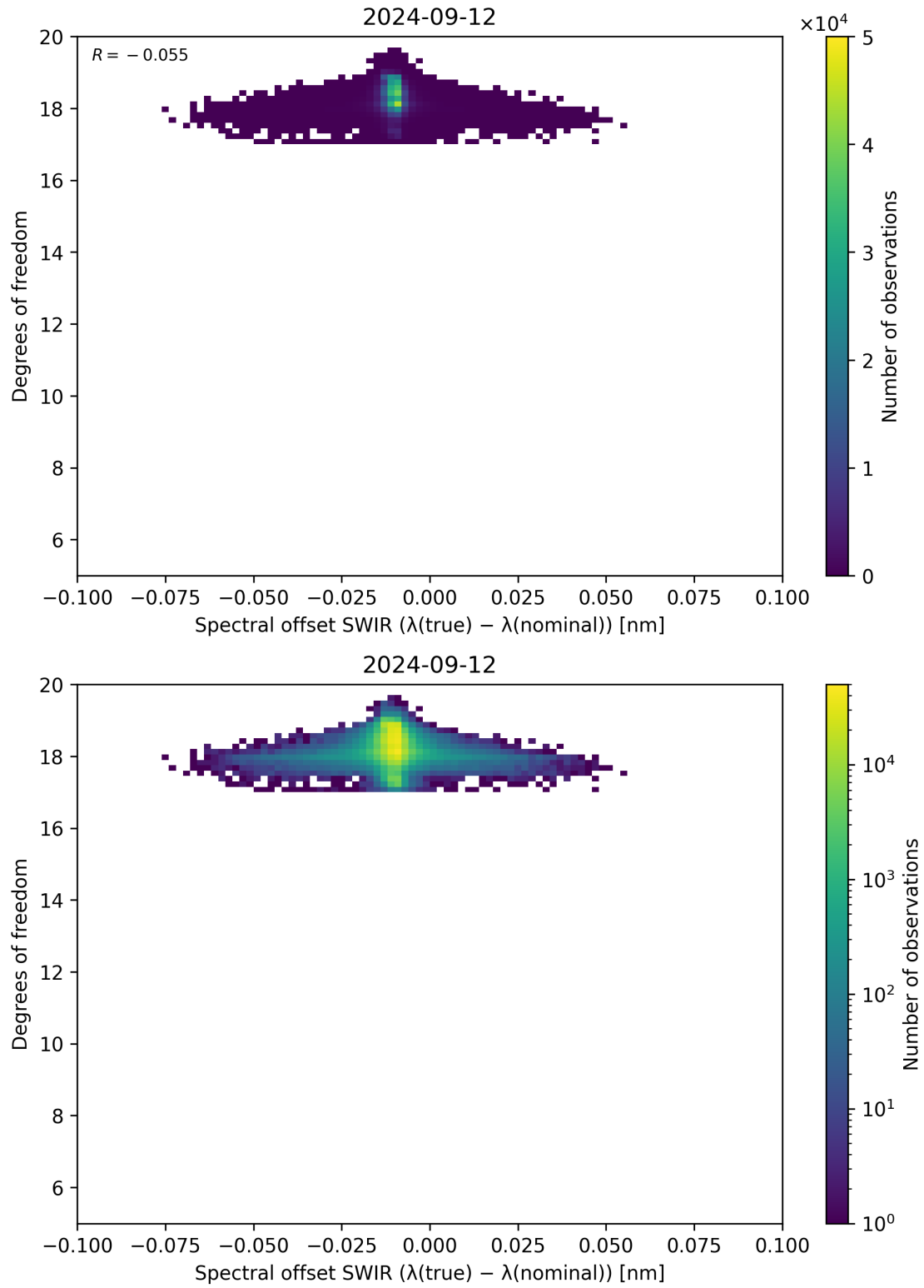
Figure 119: Scatter density plot of “Spectral offset SWIR ( \lambda_{\text{true}} - \lambda_{\text{nominal}} )” against “Degrees of freedom” for 2024-09-12 to 2024-09-13.
