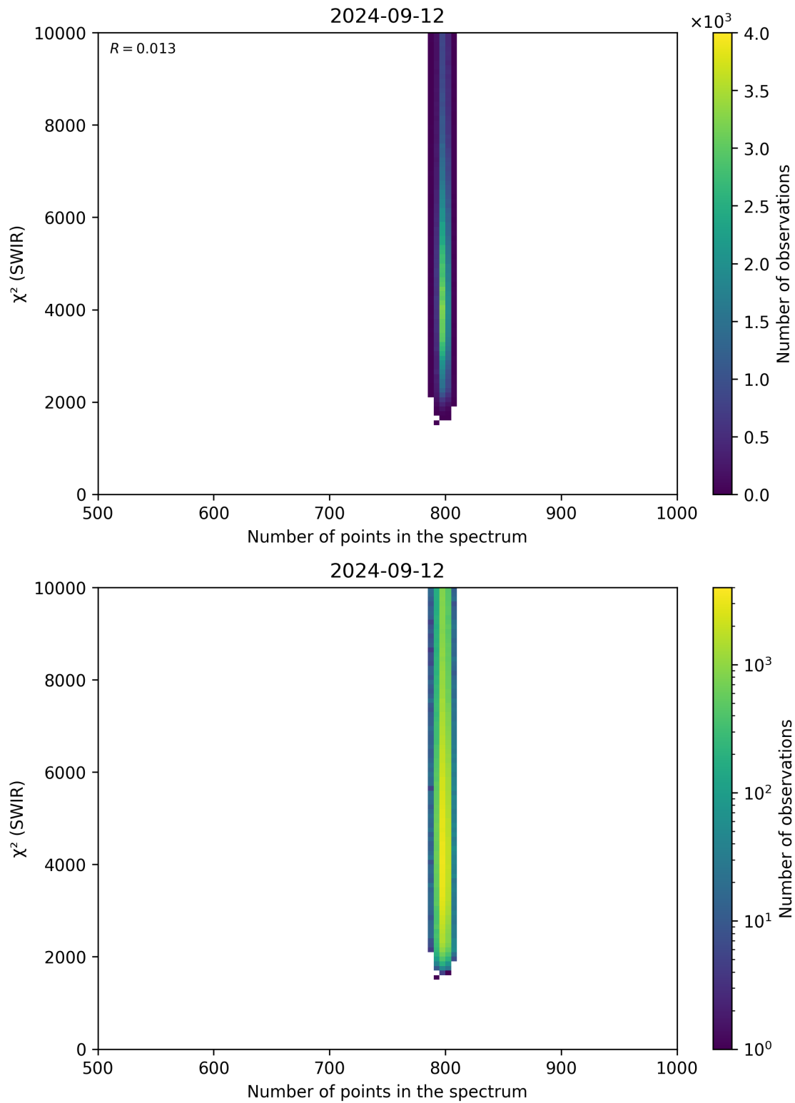
Figure 89: Scatter density plot of “Number of points in the spectrum” against “ \chi^2 (SWIR)” for 2024-09-12 to 2024-09-13.
