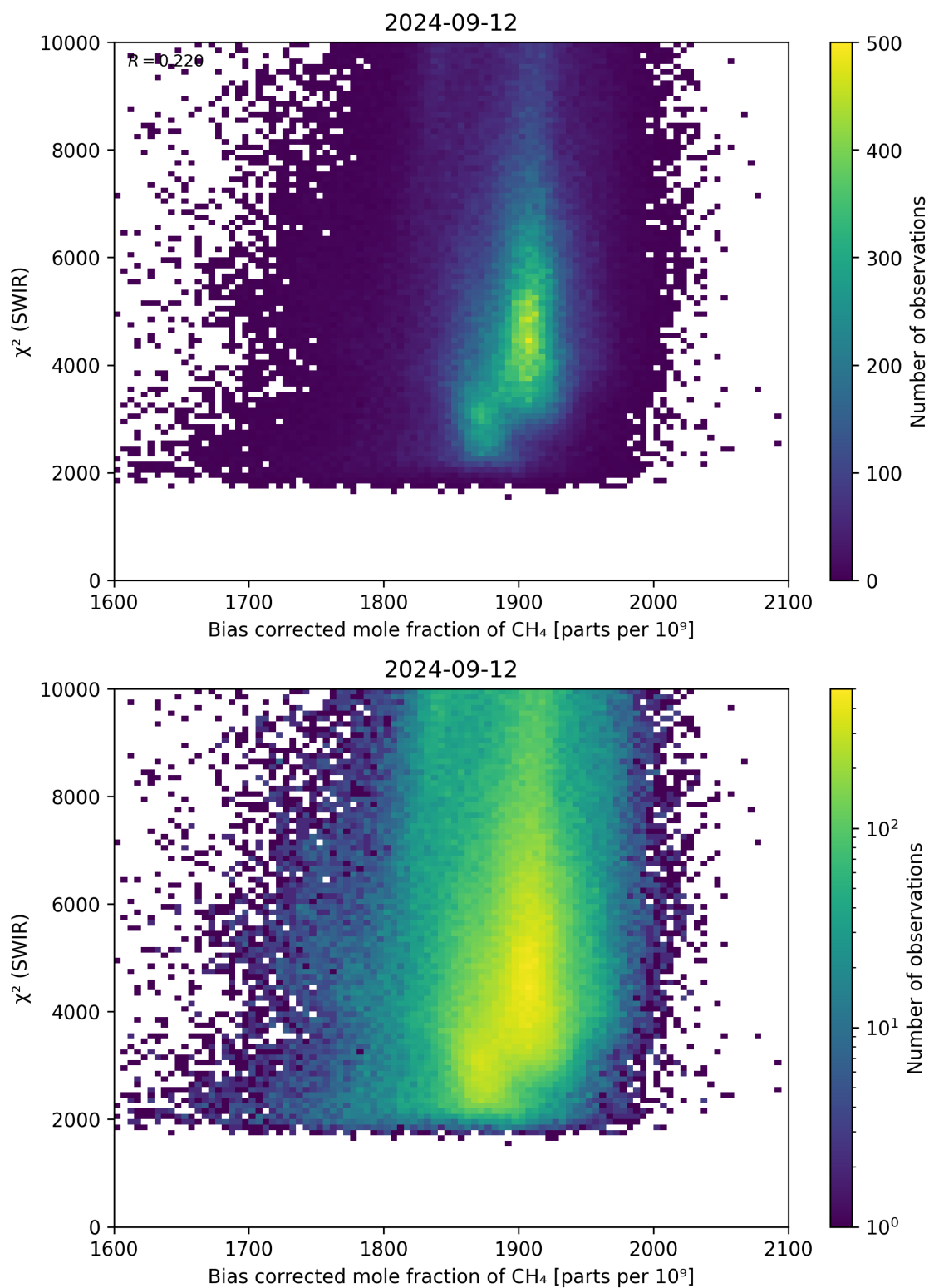
Figure 64: Scatter density plot of “Bias corrected mole fraction of \text{CH}_4 ” against “ \chi^2 (SWIR)” for 2024-09-12 to 2024-09-13.
