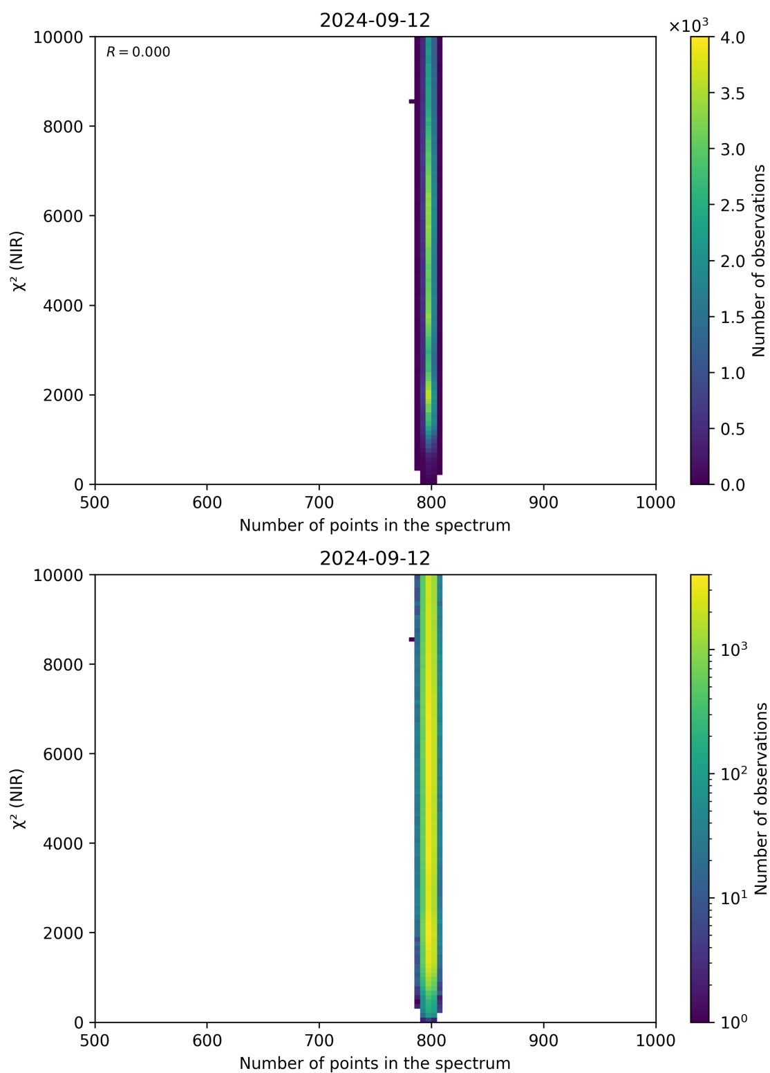
Figure 88: Scatter density plot of “Number of points in the spectrum” against “ \chi^2 (NIR)” for 2024-09-12 to 2024-09-13.
