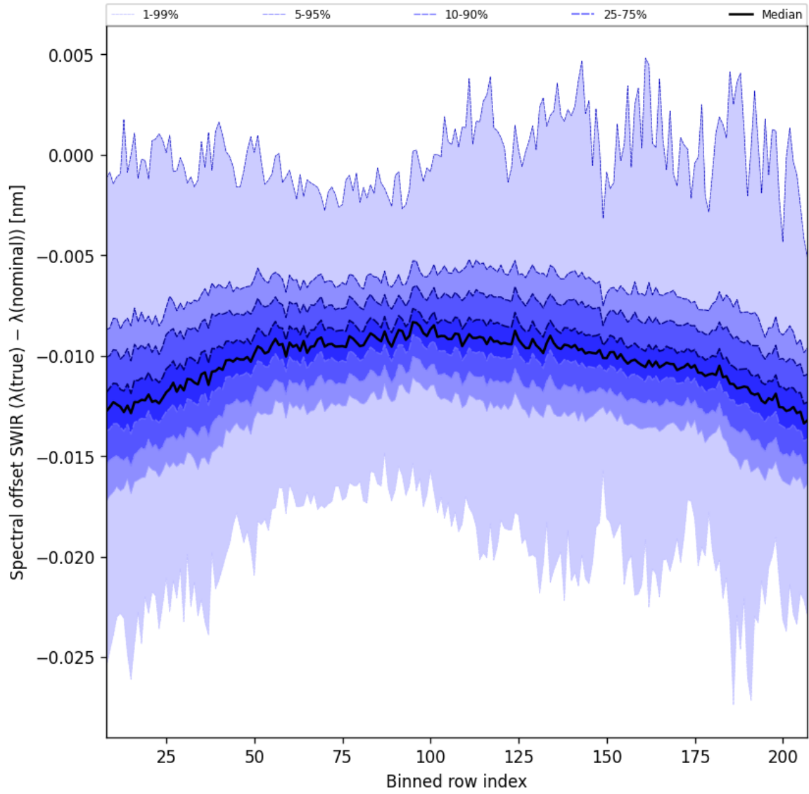
Figure 38: Along track statistics of “Spectral offset SWIR ( \lambda_{\text{true}} - \lambda_{\text{nominal}} )” for 2024-09-12 to 2024-09-13
