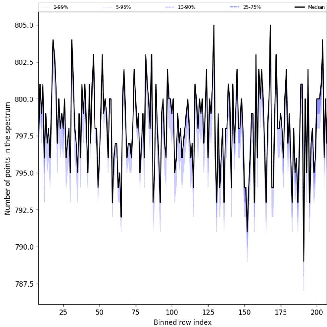
Figure 37: Along track statistics of “Number of points in the spectrum” for 2024-09-12 to 2024-09-13
