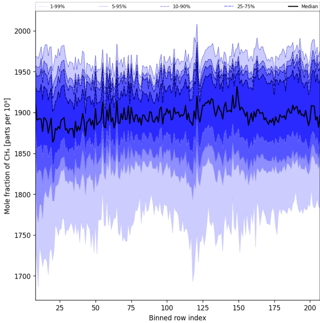
Figure 34: Along track statistics of “Mole fraction of CH 4 ” for 2024-09-12 to 2024-09-13
