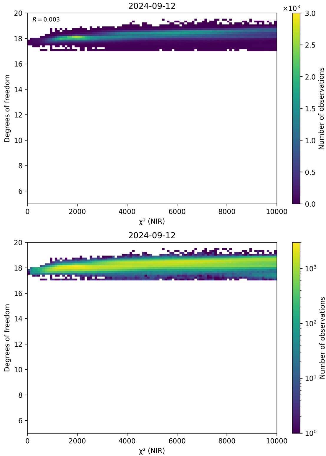
Figure 44: Scatter density plot of “ \chi^2 (NIR)” against “Degrees of freedom” for 2024-09-12 to 2024-09-13.
