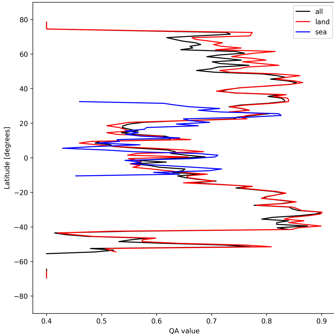
Figure 11: Zonal average of “QA value” for 2024-09-12 to 2024-09-13.
