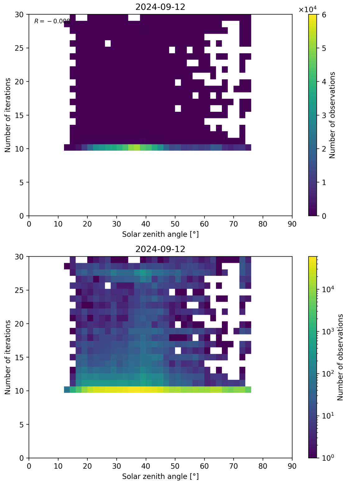
Figure 102: Scatter density plot of “Solar zenith angle” against “Number of iterations” for 2024-09-12 to 2024-09-13.
