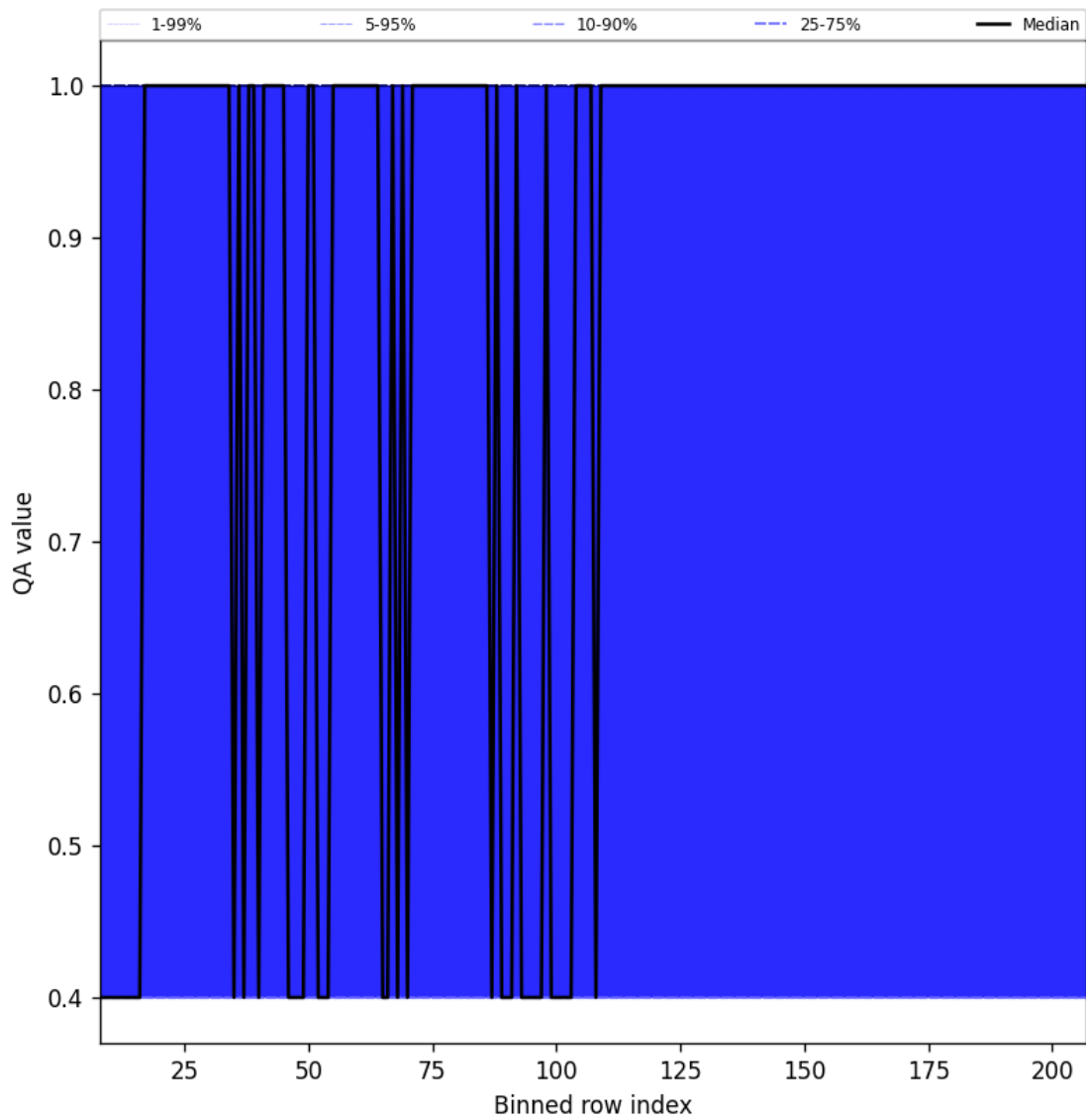
Figure 33: Along track statistics of “QA value” for 2024-09-12 to 2024-09-13
