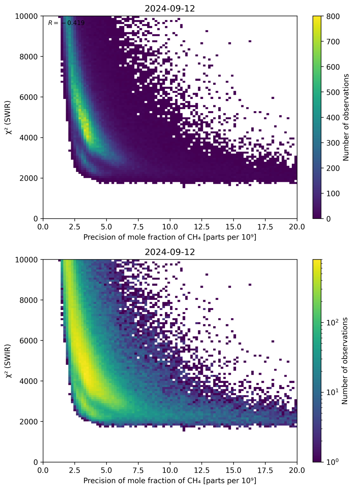
Figure 79: Scatter density plot of “Precision of mole fraction of \text{CH}_4 ” against “ \chi^2 (SWIR)” for 2024-09-12 to 2024-09-13.
