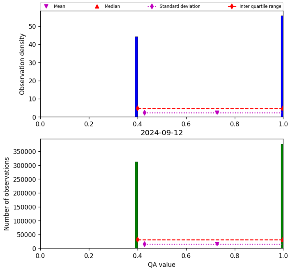
Figure 22: Histogram of “QA value” for 2024-09-12 to 2024-09-13
