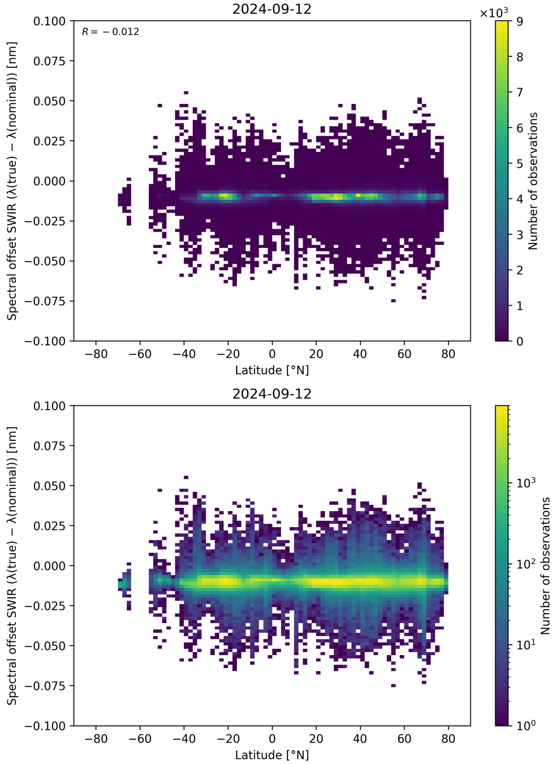
Figure 62: Scatter density plot of “Latitude” against “Spectral offset SWIR ( \lambda_{\text{true}} - \lambda_{\text{nominal}} )” for 2024-09-12 to 2024-09-13.
