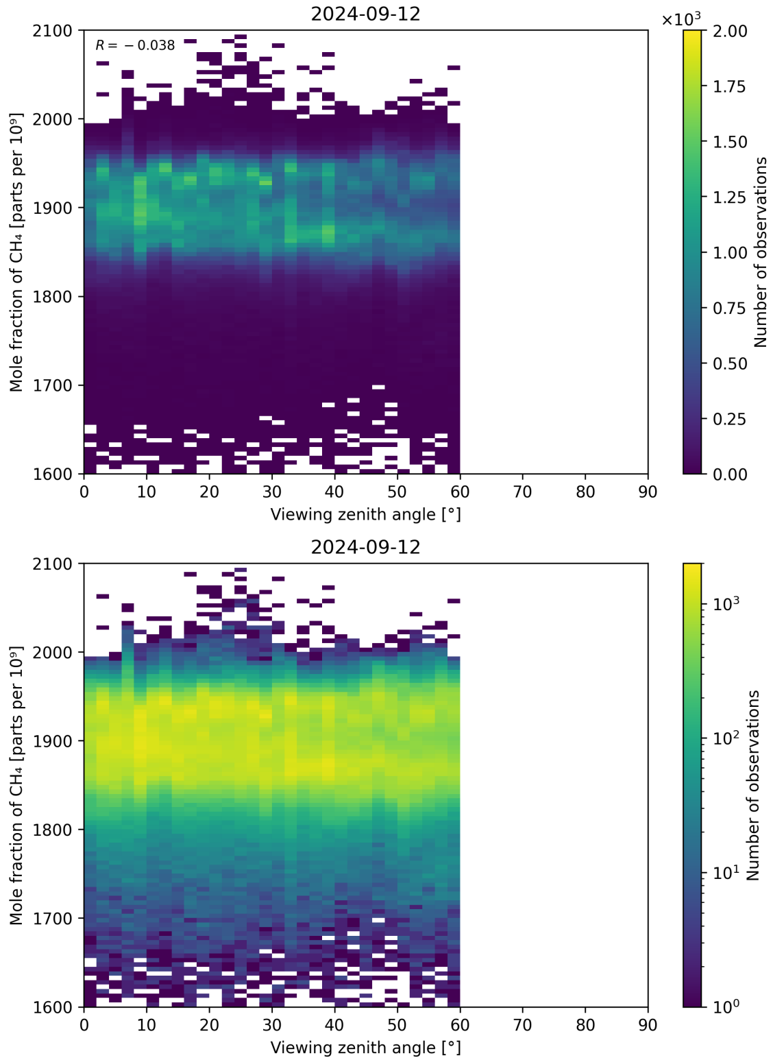
Figure 110: Scatter density plot of “Viewing zenith angle” against “Mole fraction of CH 4 ” for 2024-09-12 to 2024-09-13.
