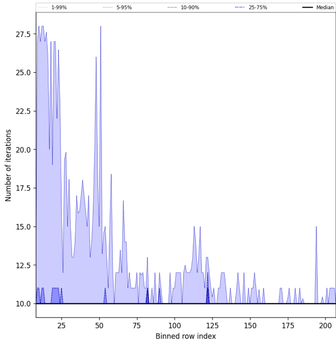
Figure 42: Along track statistics of “Number of iterations” for 2024-09-12 to 2024-09-13
