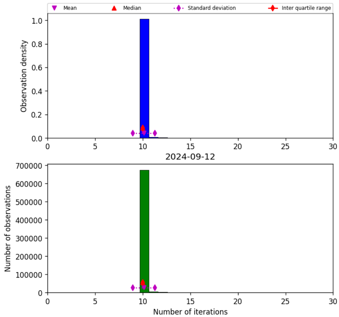
Figure 31: Histogram of “Number of iterations” for 2024-09-12 to 2024-09-13
