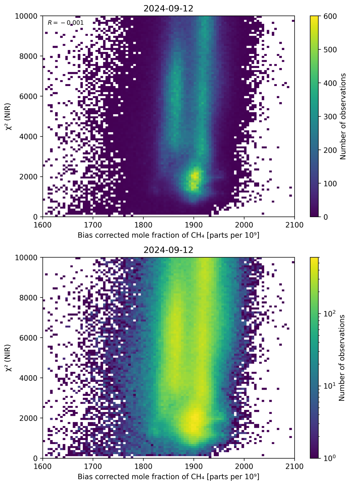
Figure 63: Scatter density plot of “Bias corrected mole fraction of CH 4 ” against “ \chi^2 (NIR)” for 2024-09-12 to 2024-09-13.
