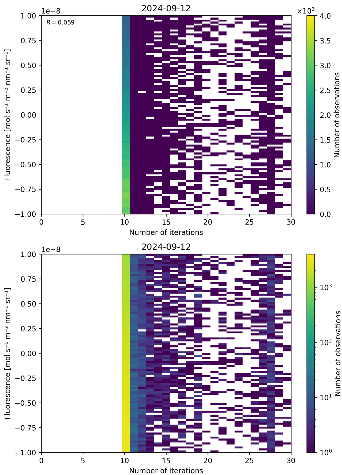
Figure 87: Scatter density plot of “Number of iterations” against “Fluorescence” for 2024-09-12 to 2024-09-13.
