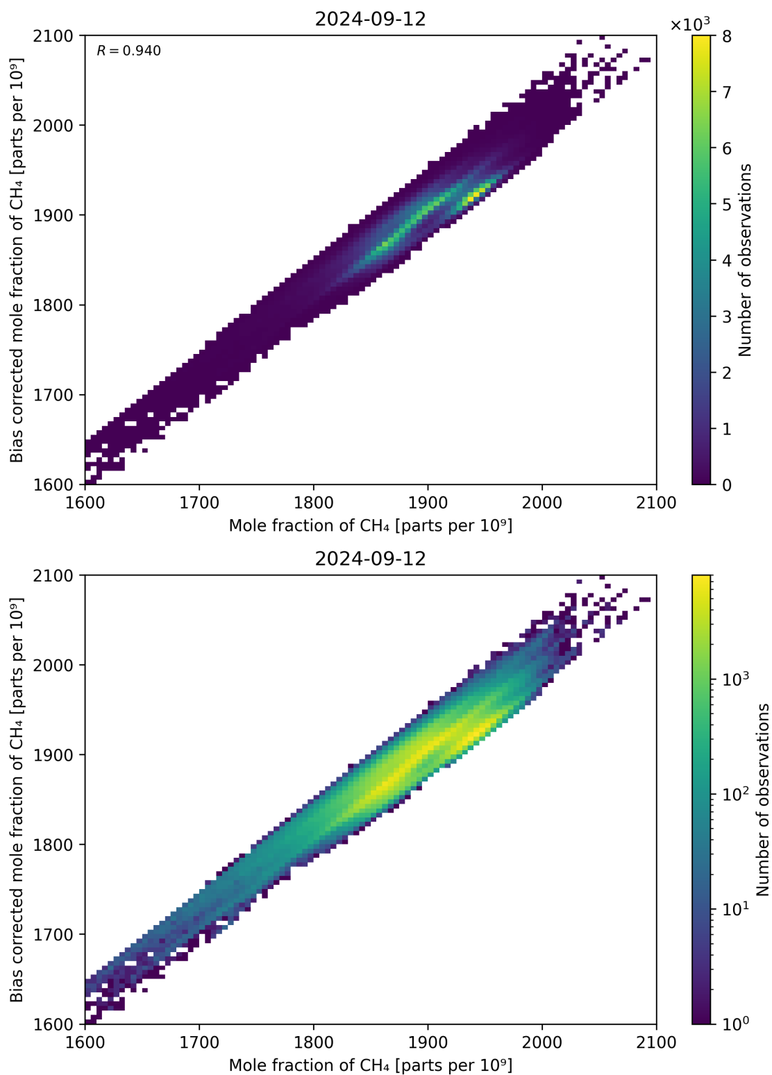
Figure 74: Scatter density plot of “Mole fraction of CH 4 ” against “Bias corrected mole fraction of CH 4 ” for 2024-09-12 to 2024-09-13.
