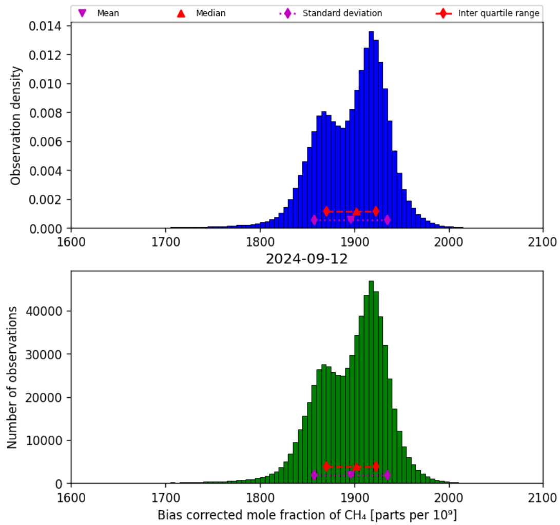
Figure 25: Histogram of “Bias corrected mole fraction of CH 4 ” for 2024-09-12 to 2024-09-13
