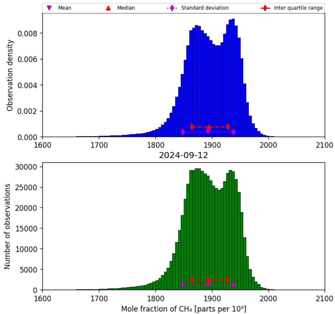
Figure 23: Histogram of “Mole fraction of CH 4 ” for 2024-09-12 to 2024-09-13
