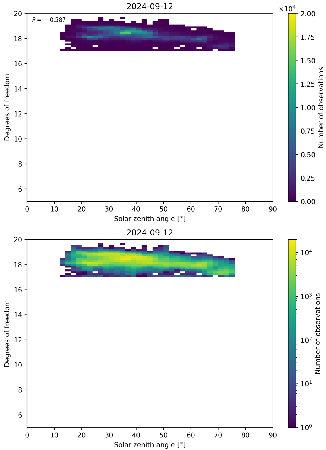
Figure 96: Scatter density plot of “Solar zenith angle” against “Degrees of freedom” for 2024-09-12 to 2024-09-13.
