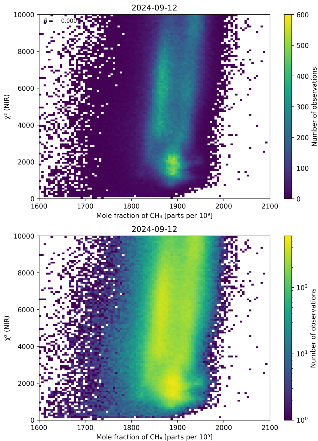
Figure 70: Scatter density plot of “Mole fraction of \text{CH}_4 ” against “ \chi^2 (NIR)” for 2024-09-12 to 2024-09-13.
