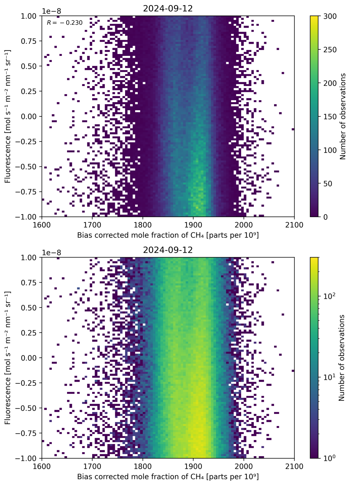
Figure 66: Scatter density plot of “Bias corrected mole fraction of \text{CH}_4 ” against “Fluorescence” for 2024-09-12 to 2024-09-13.
