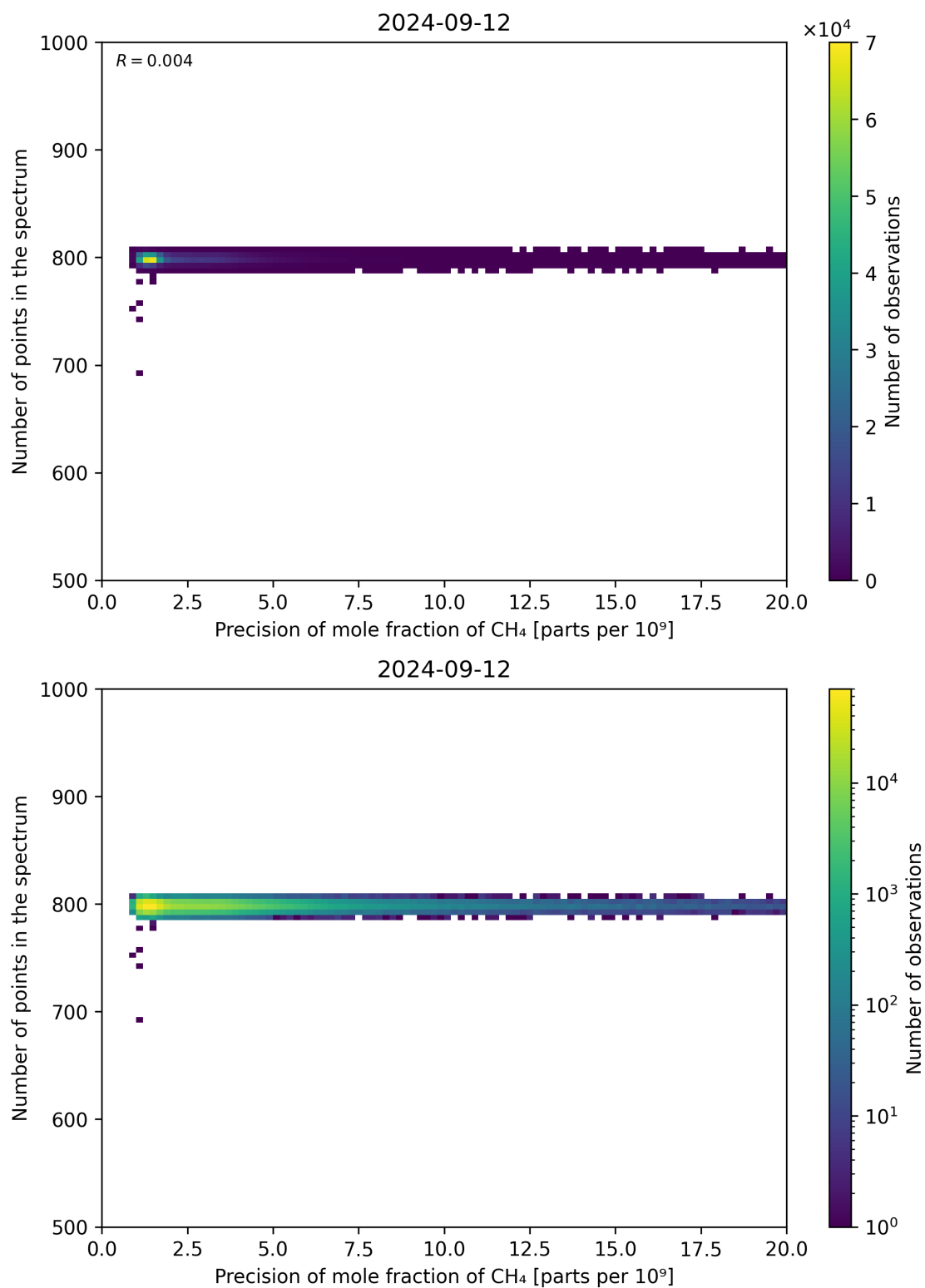
Figure 84: Scatter density plot of “Precision of mole fraction of CH 4 ” against “Number of points in the spectrum” for 2024-09-12 to 2024-09-13.
