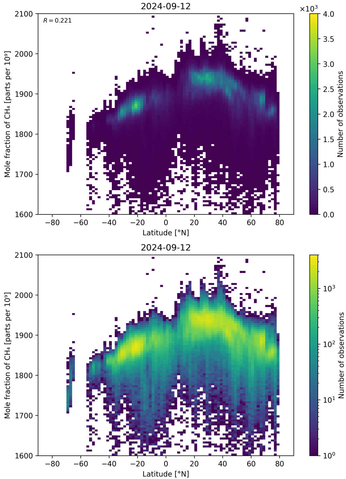
Figure 57: Scatter density plot of “Latitude” against “Mole fraction of \text{CH}_4 ” for 2024-09-12 to 2024-09-13.
