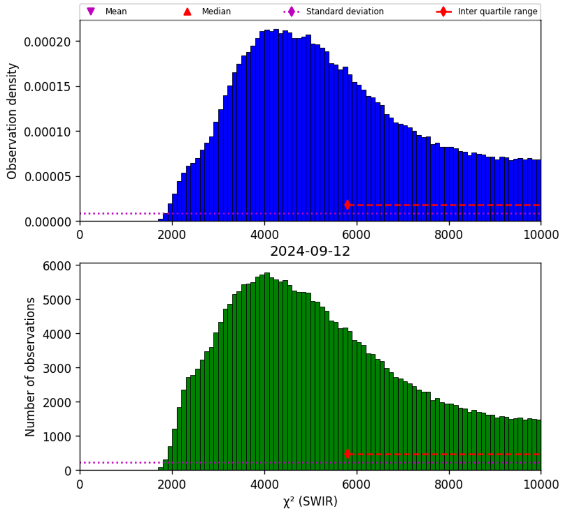
Figure 28: Histogram of “ \chi^2 (SWIR)” for 2024-09-12 to 2024-09-13
