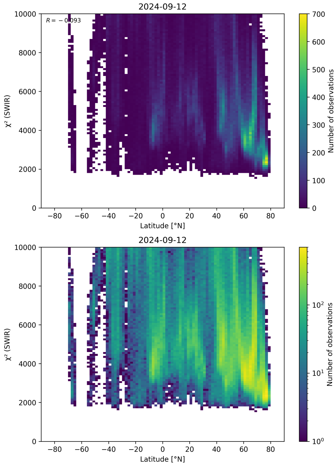
Figure 54: Scatter density plot of “Latitude” against “ \chi^2 (SWIR)” for 2024-09-12 to 2024-09-13.
