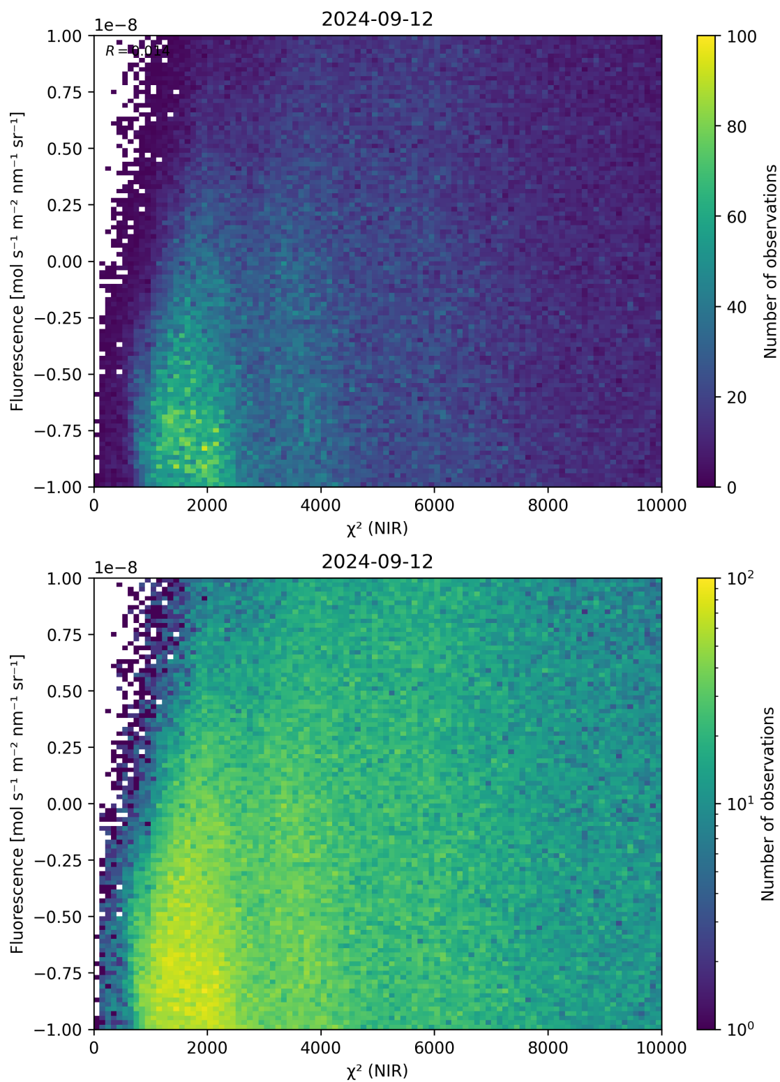
Figure 45: Scatter density plot of “ \chi^2 (NIR)” against “Fluorescence” for 2024-09-12 to 2024-09-13.
