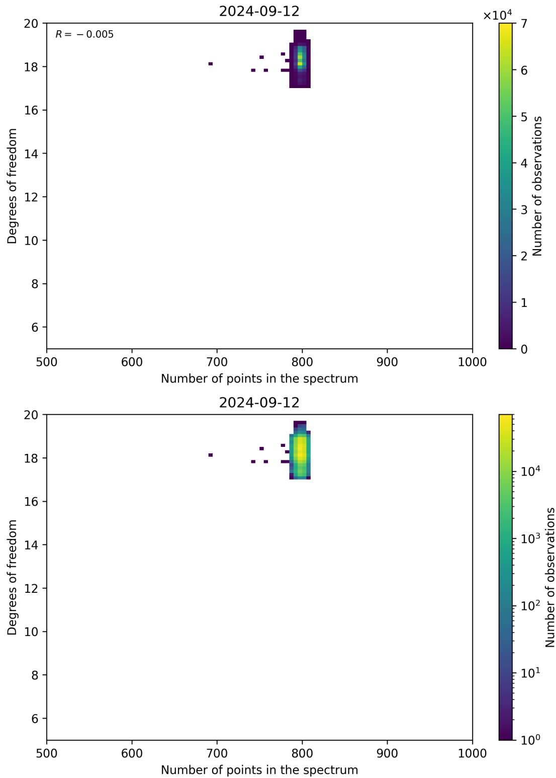
Figure 90: Scatter density plot of “Number of points in the spectrum” against “Degrees of freedom” for 2024-09-12 to 2024-09-13.
