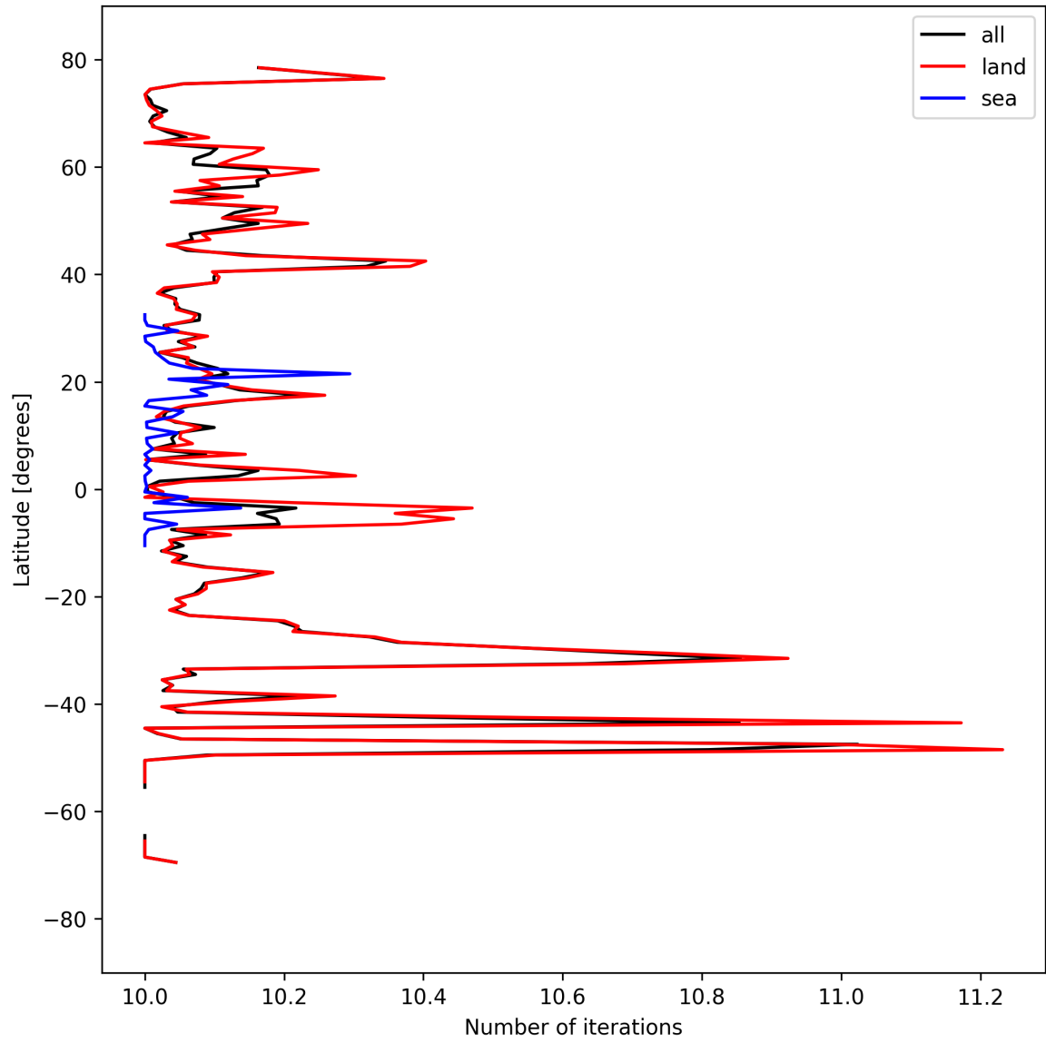
Figure 20: Zonal average of “Number of iterations” for 2024-09-12 to 2024-09-13.
