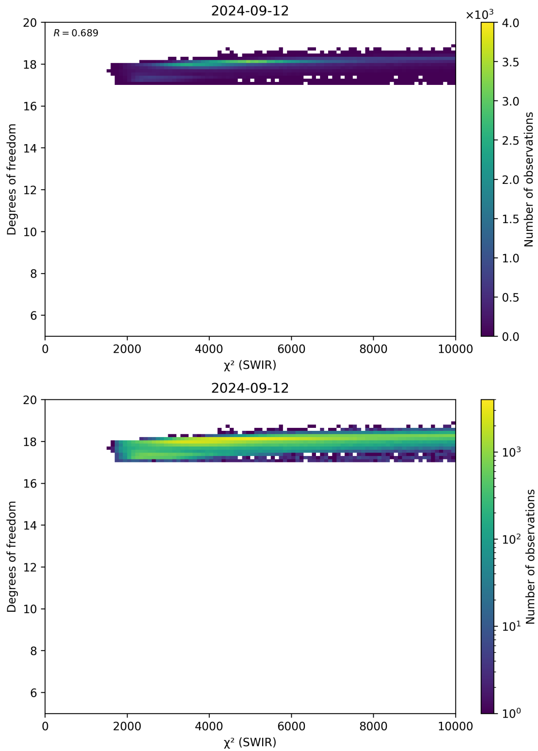
Figure 48: Scatter density plot of “ \chi^2 (SWIR)” against “Degrees of freedom” for 2024-09-12 to 2024-09-13.
