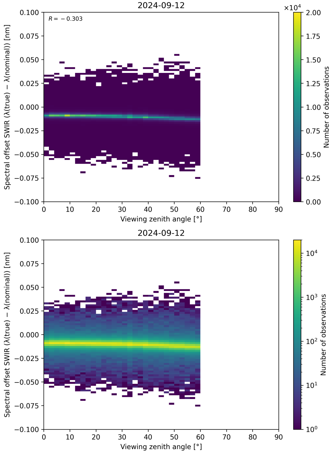
Figure 116: Scatter density plot of “Viewing zenith angle” against “Spectral offset SWIR ( \lambda_{\text{true}} - \lambda_{\text{nominal}} )” for 2024-09-12 to 2024-09-13.
