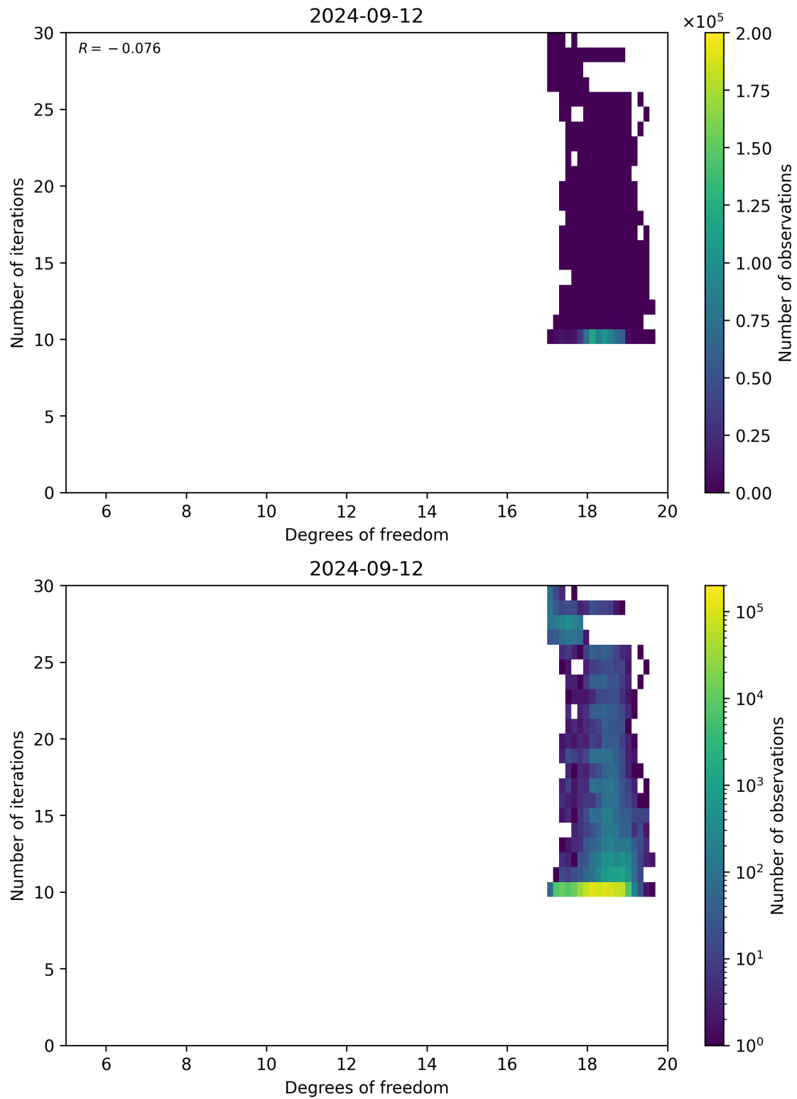
Figure 52: Scatter density plot of “Degrees of freedom” against “Number of iterations” for 2024-09-12 to 2024-09-13.
