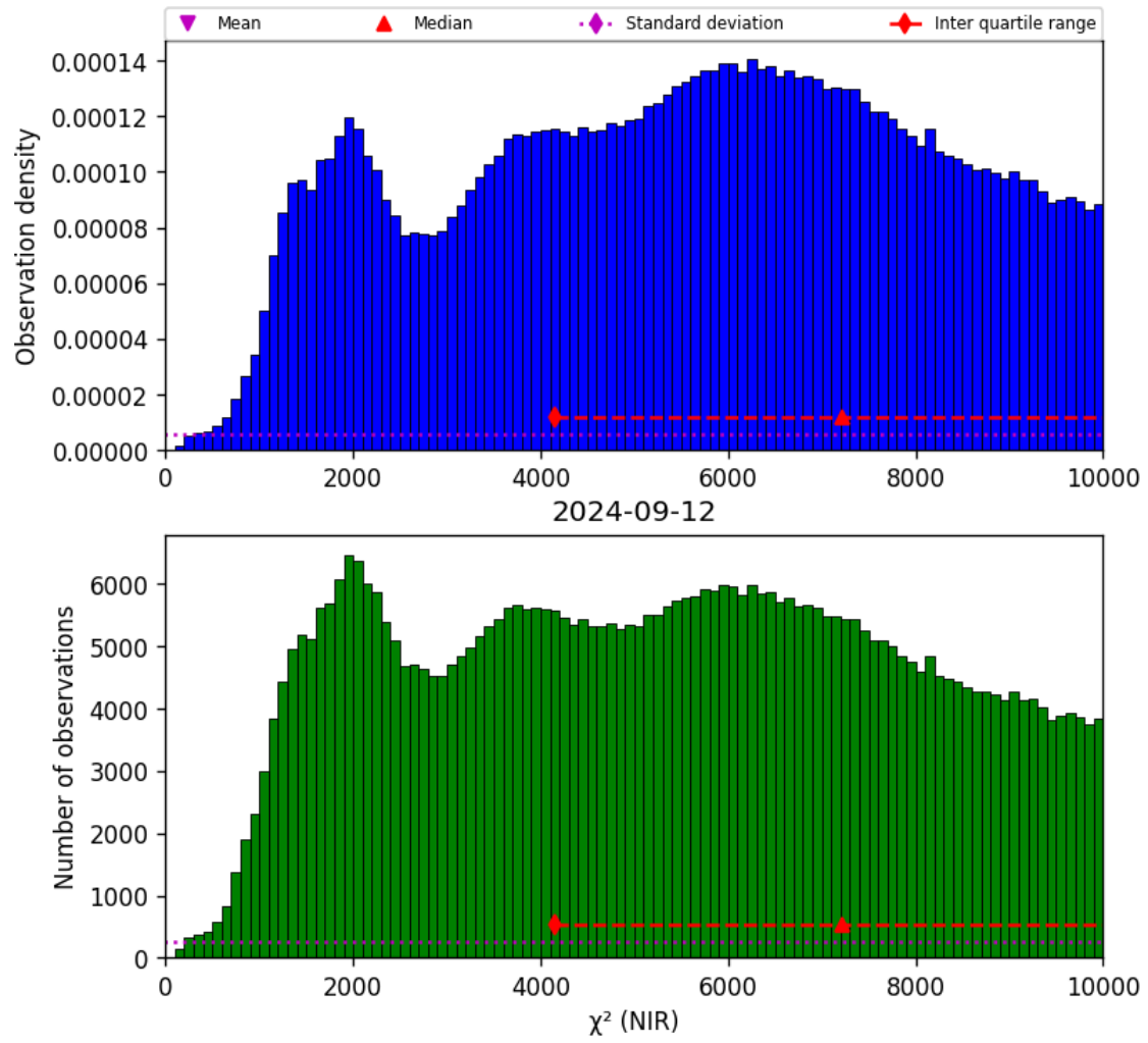
Figure 29: Histogram of “ \chi^2 (NIR)” for 2024-09-12 to 2024-09-13
