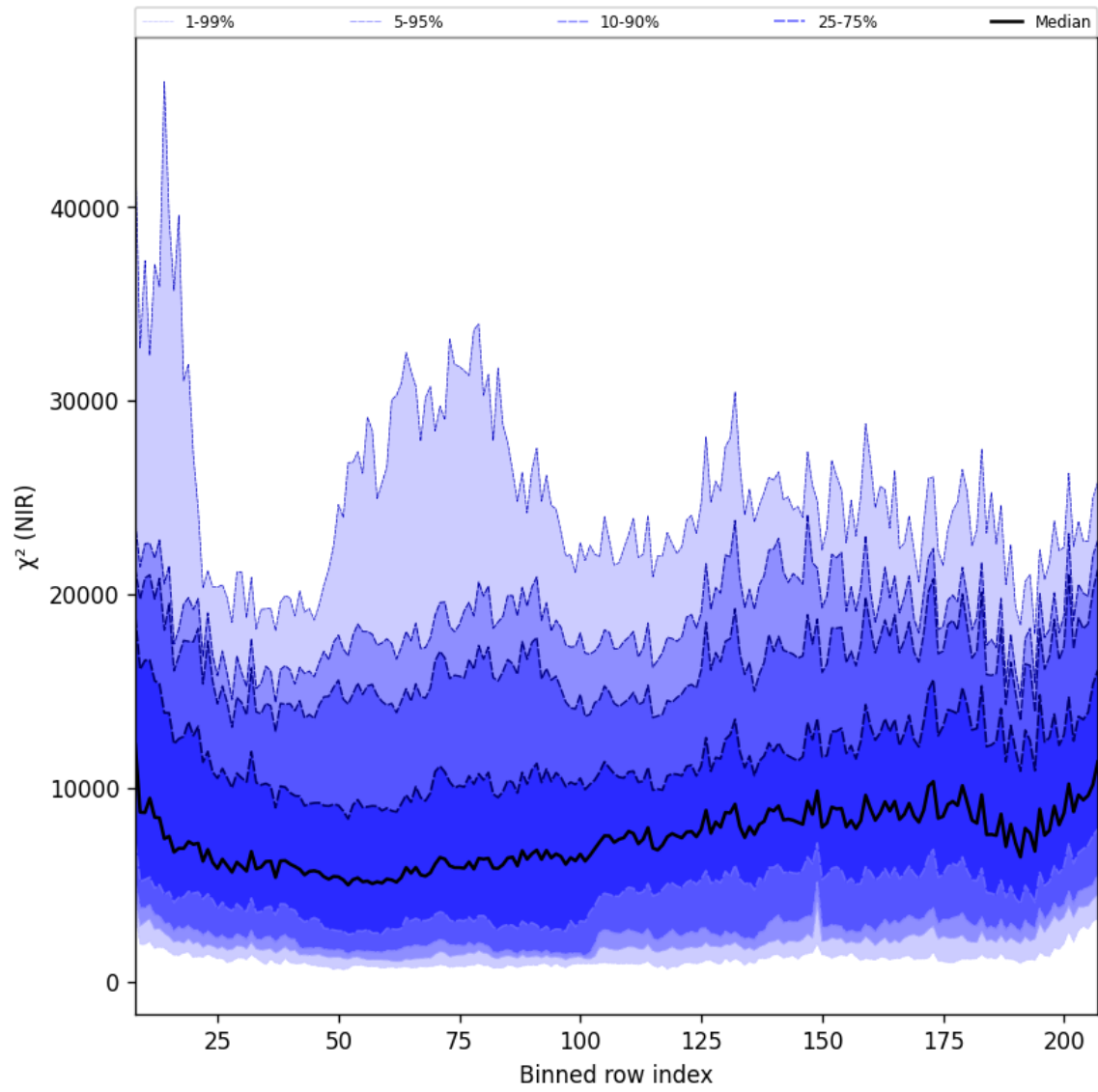
Figure 40: Along track statistics of “ \chi^2 (NIR)” for 2024-09-12 to 2024-09-13
