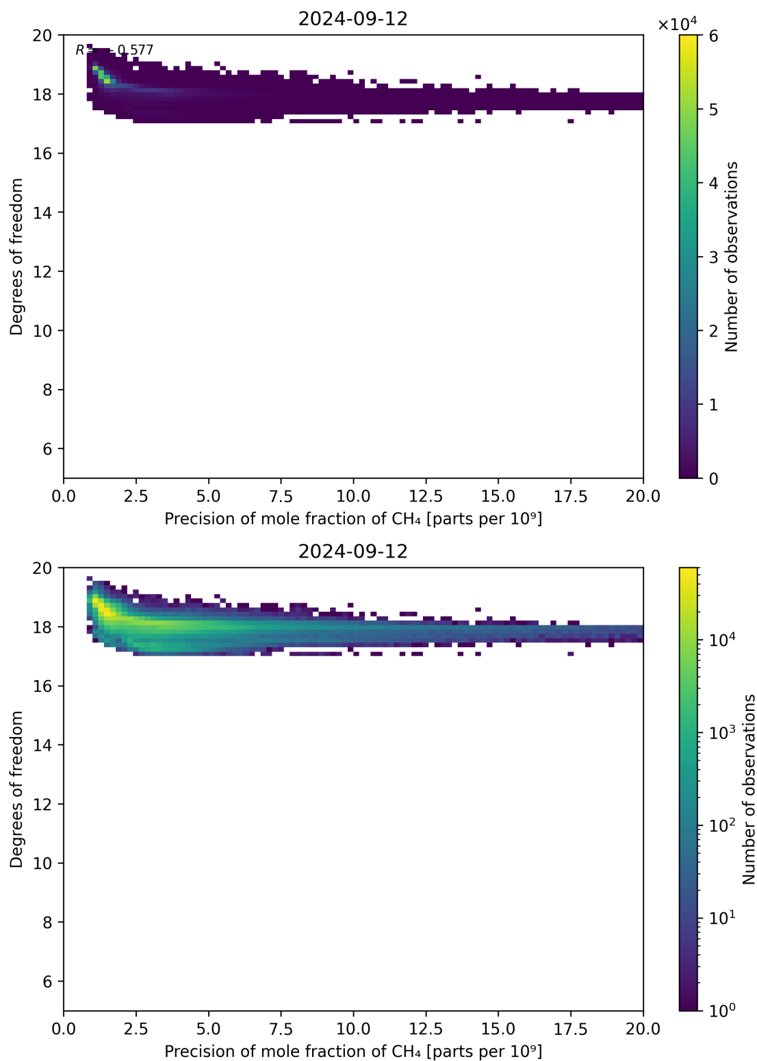
Figure 80: Scatter density plot of “Precision of mole fraction of CH 4 ” against “Degrees of freedom” for 2024-09-12 to 2024-09-13.
