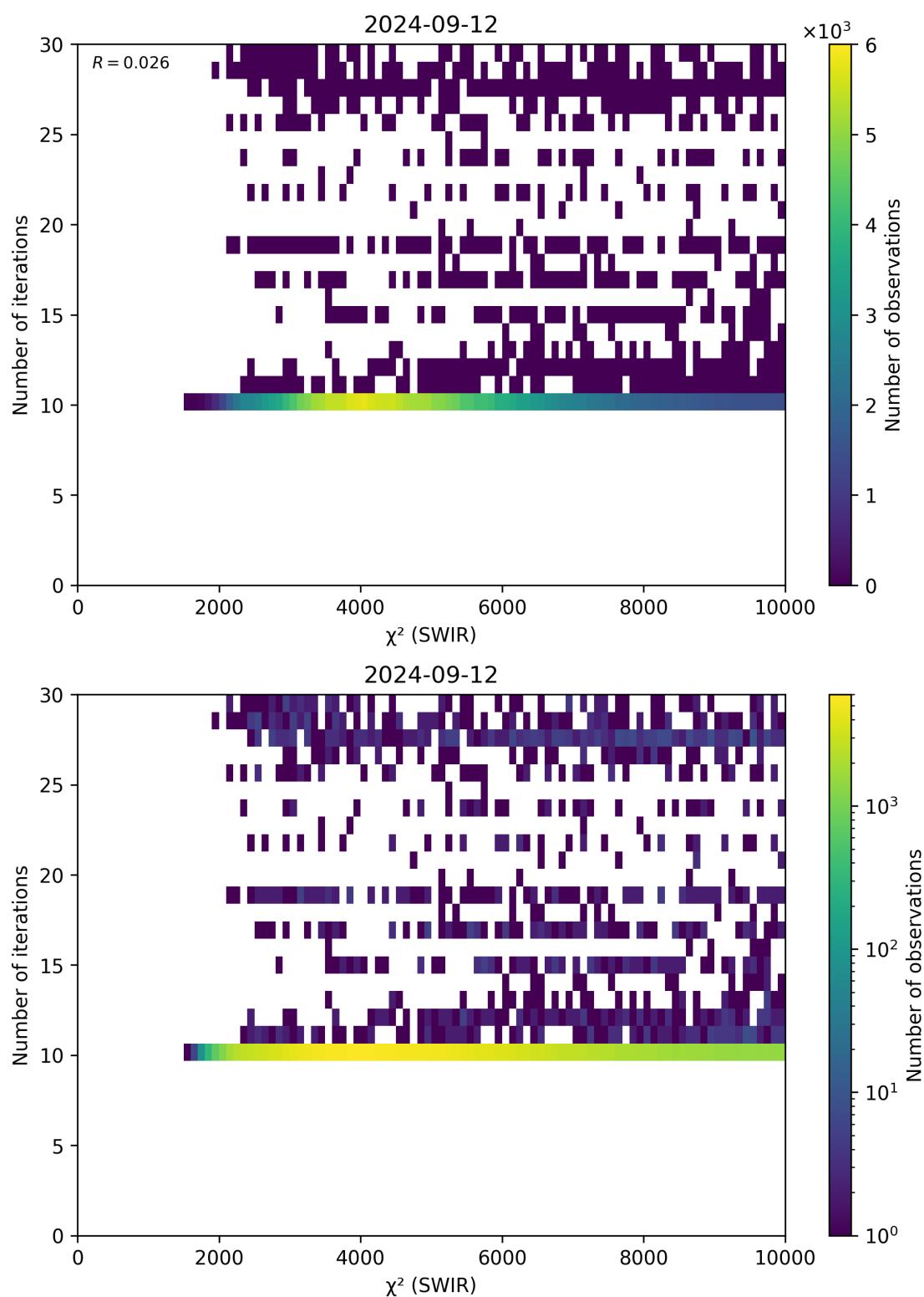
Figure 50: Scatter density plot of “ \chi^2 (SWIR)” against “Number of iterations” for 2024-09-12 to 2024-09-13.
