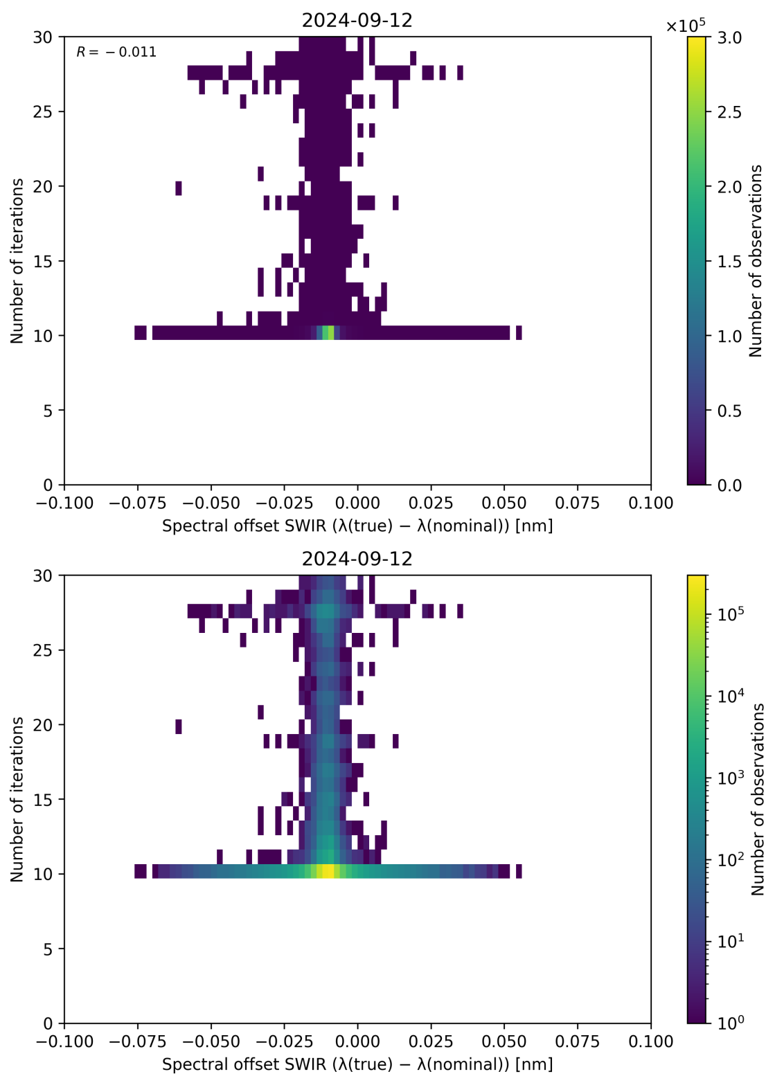
Figure 121: Scatter density plot of “Spectral offset SWIR ( \lambda_{\text{true}} - \lambda_{\text{nominal}} )” against “Number of iterations” for 2024-09-12 to 2024-09-13.
