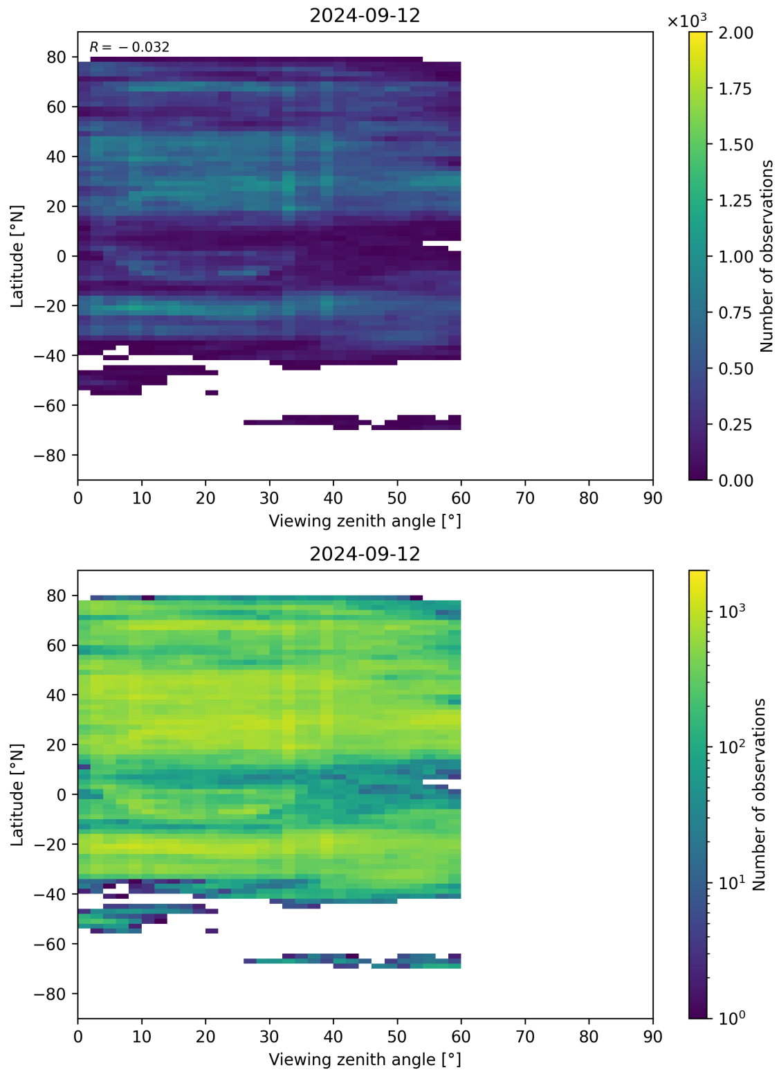
Figure 109: Scatter density plot of “Viewing zenith angle” against “Latitude” for 2024-09-12 to 2024-09-13.
