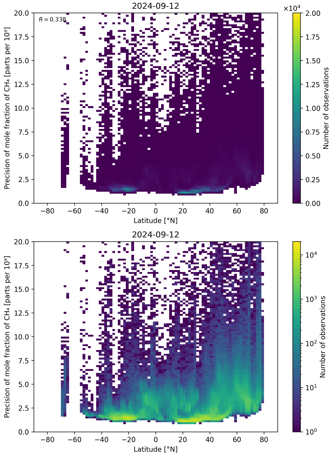
Figure 59: Scatter density plot of “Latitude” against “Precision of mole fraction of \text{CH}_4 ” for 2024-09-12 to 2024-09-13.
