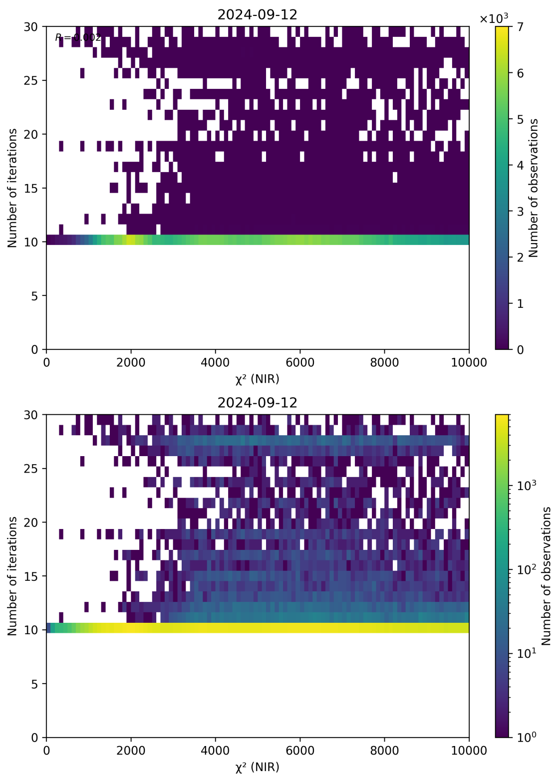
Figure 46: Scatter density plot of “ \chi^2 (NIR)” against “Number of iterations” for 2024-09-12 to 2024-09-13.
