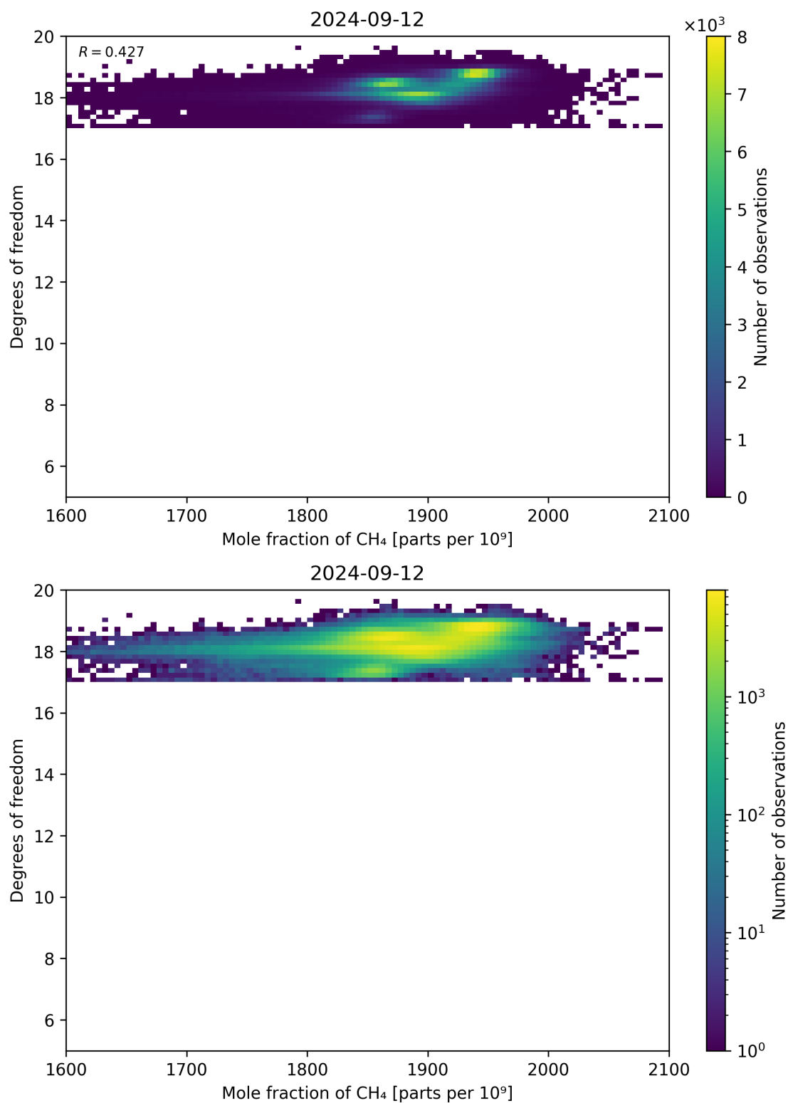
Figure 72: Scatter density plot of “Mole fraction of CH 4 ” against “Degrees of freedom” for 2024-09-12 to 2024-09-13.
