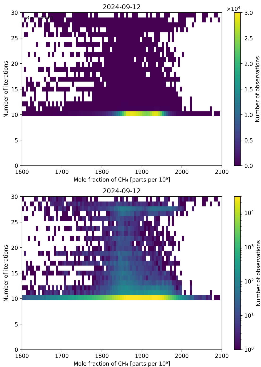
Figure 76: Scatter density plot of “Mole fraction of CH 4 ” against “Number of iterations” for 2024-09-12 to 2024-09-13.
