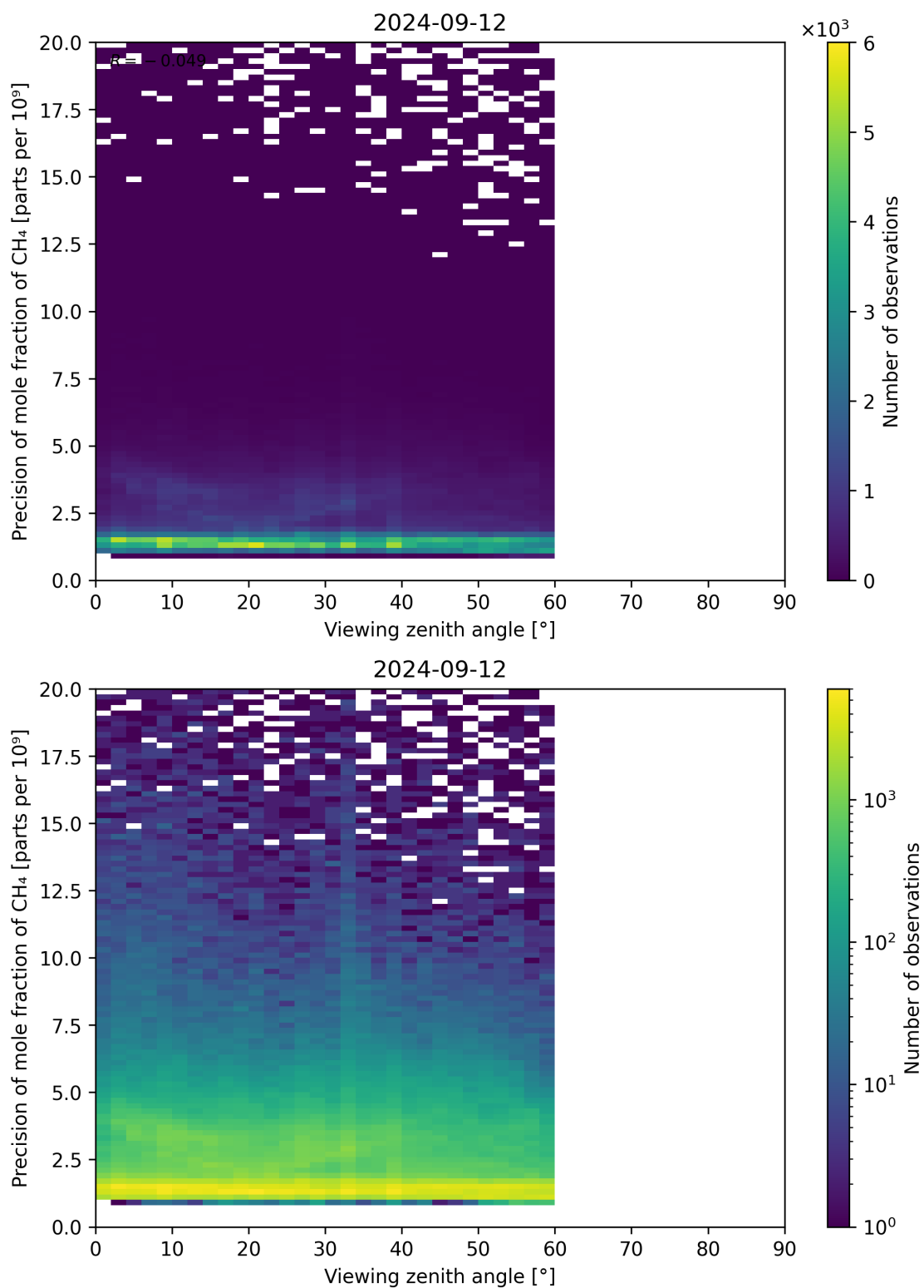
Figure 112: Scatter density plot of “Viewing zenith angle” against “Precision of mole fraction of CH 4 ” for 2024-09-12 to 2024-09-13.
