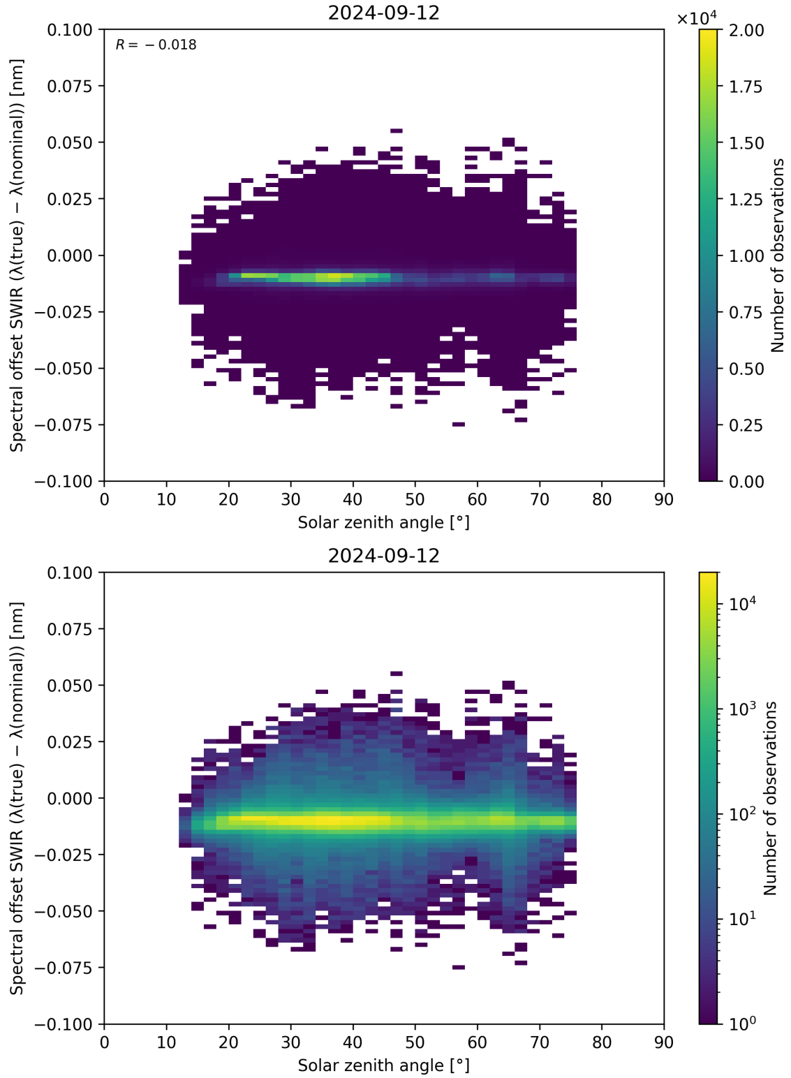
Figure 104: Scatter density plot of “Solar zenith angle” against “Spectral offset SWIR ( \lambda_{\text{true}} - \lambda_{\text{nominal}} )” for 2024-09-12 to 2024-09-13.
