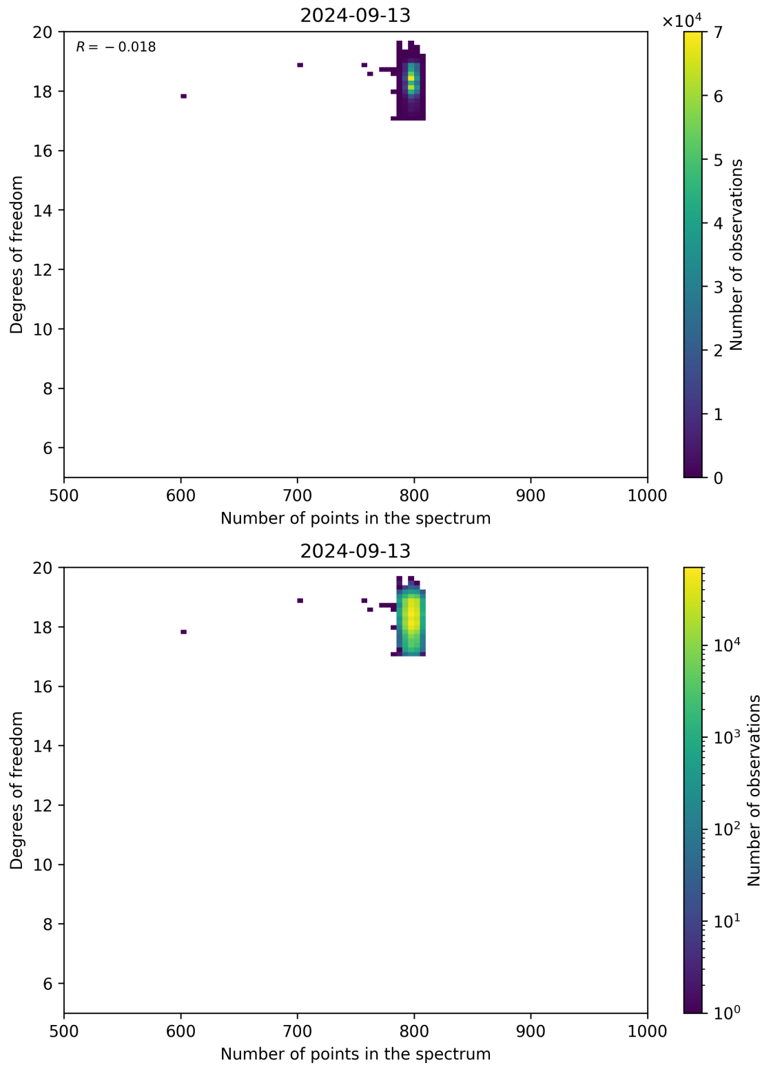
Figure 90: Scatter density plot of “Number of points in the spectrum” against “Degrees of freedom” for 2024-09-12 to 2024-09-14.
