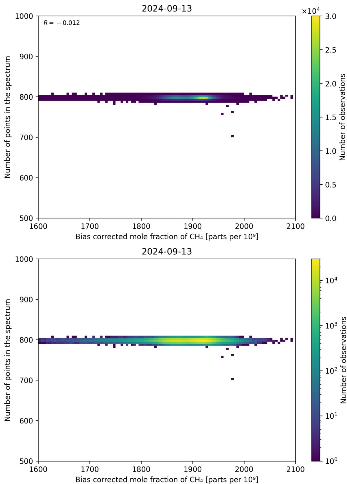
Figure 68: Scatter density plot of “Bias corrected mole fraction of CH 4 ” against “Number of points in the spectrum” for 2024-09-12 to 2024-09-14.
