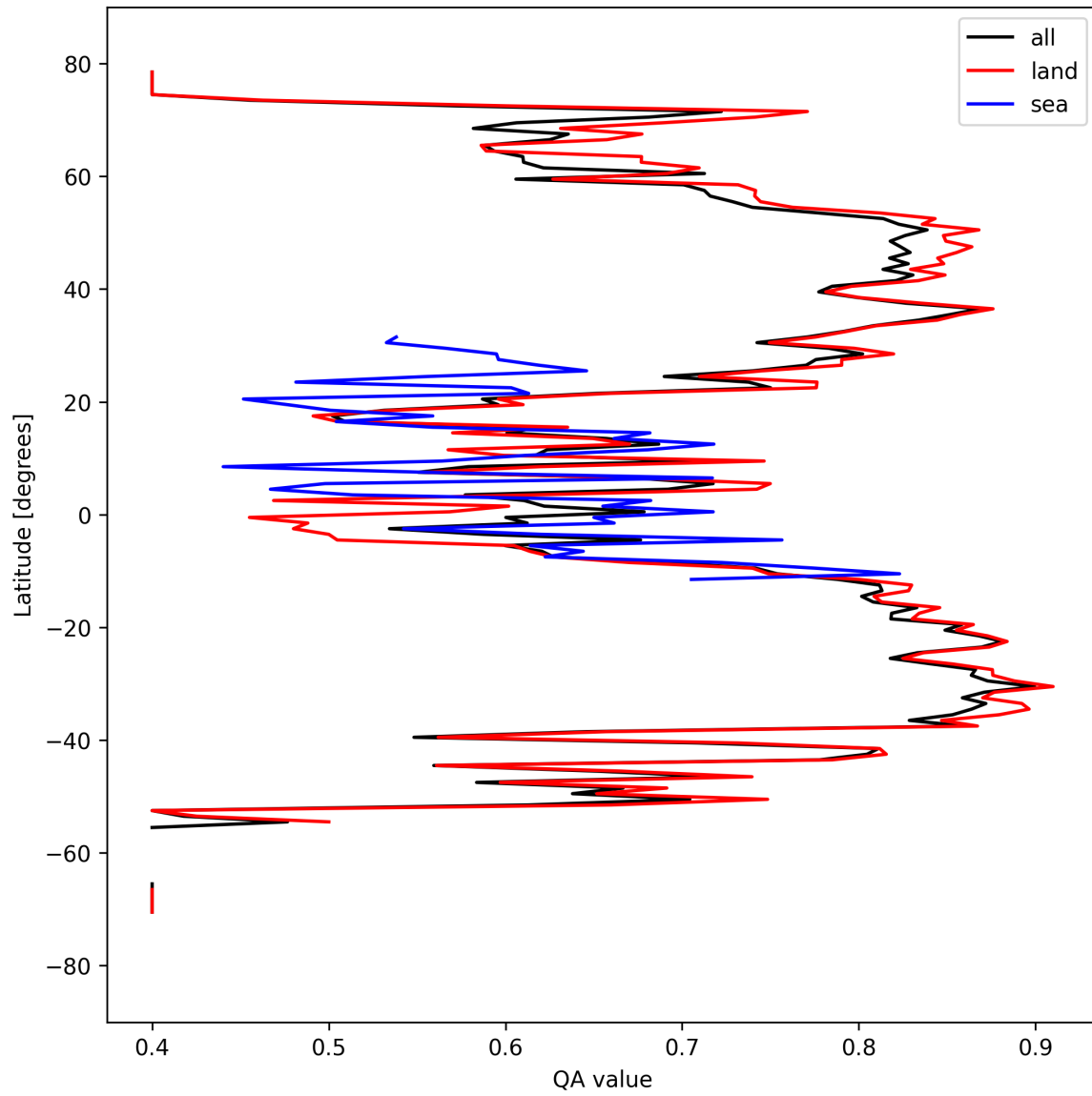
Figure 11: Zonal average of “QA value” for 2024-09-12 to 2024-09-14.
