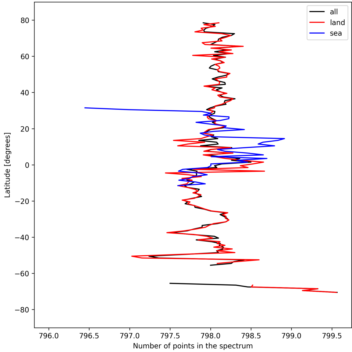
Figure 15: Zonal average of “Number of points in the spectrum” for 2024-09-12 to 2024-09-14.
