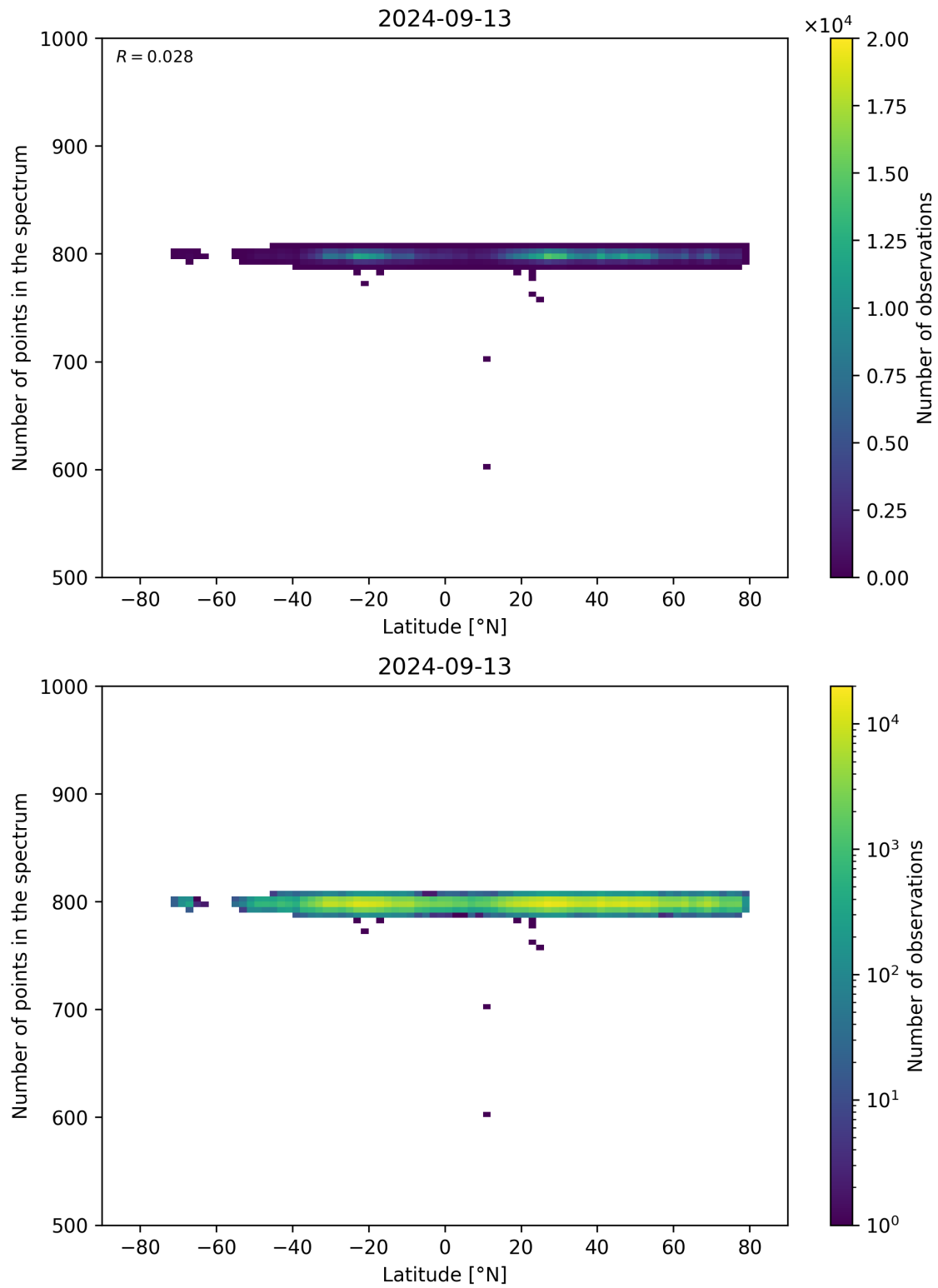
Figure 61: Scatter density plot of “Latitude” against “Number of points in the spectrum” for 2024-09-12 to 2024-09-14.
