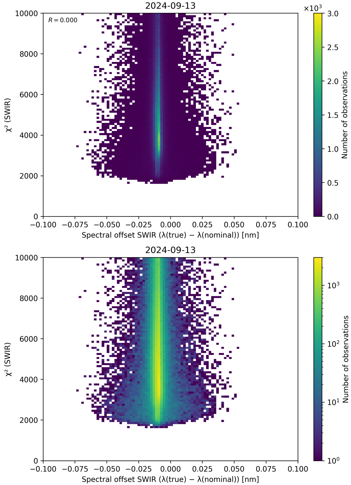
Figure 118: Scatter density plot of “Spectral offset SWIR ( \lambda_{\text{true}} - \lambda_{\text{nominal}} )” against “ \chi^2 (SWIR)” for 2024-09-12 to 2024-09-14.
