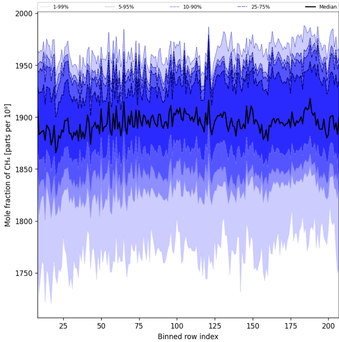
Figure 34: Along track statistics of “Mole fraction of CH 4 ” for 2024-09-12 to 2024-09-14
