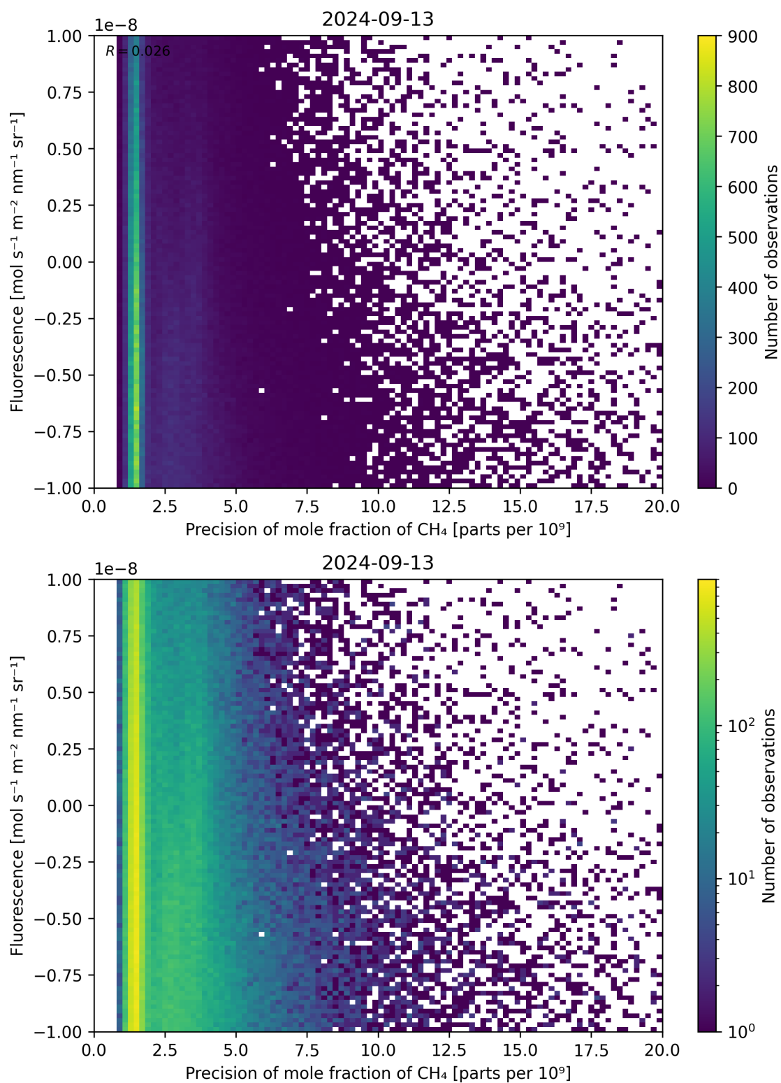
Figure 81: Scatter density plot of “Precision of mole fraction of \text{CH}_4 ” against “Fluorescence” for 2024-09-12 to 2024-09-14.
