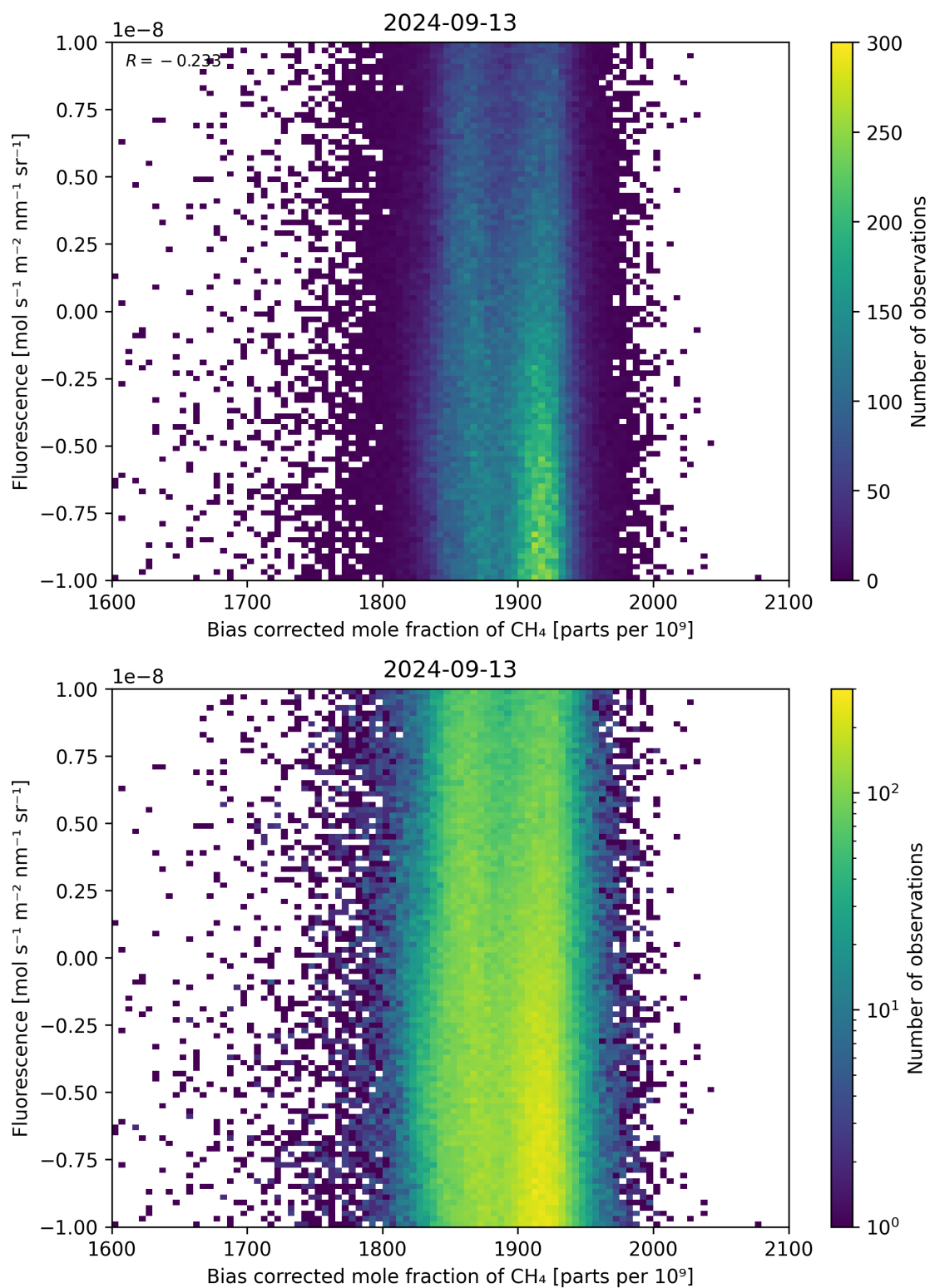
Figure 66: Scatter density plot of “Bias corrected mole fraction of \text{CH}_4 ” against “Fluorescence” for 2024-09-12 to 2024-09-14.
