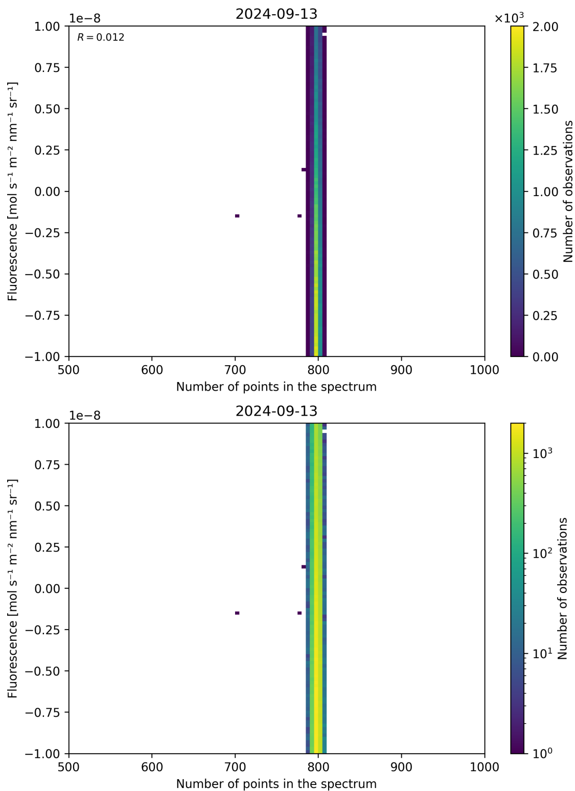
Figure 91: Scatter density plot of “Number of points in the spectrum” against “Fluorescence” for 2024-09-12 to 2024-09-14.
