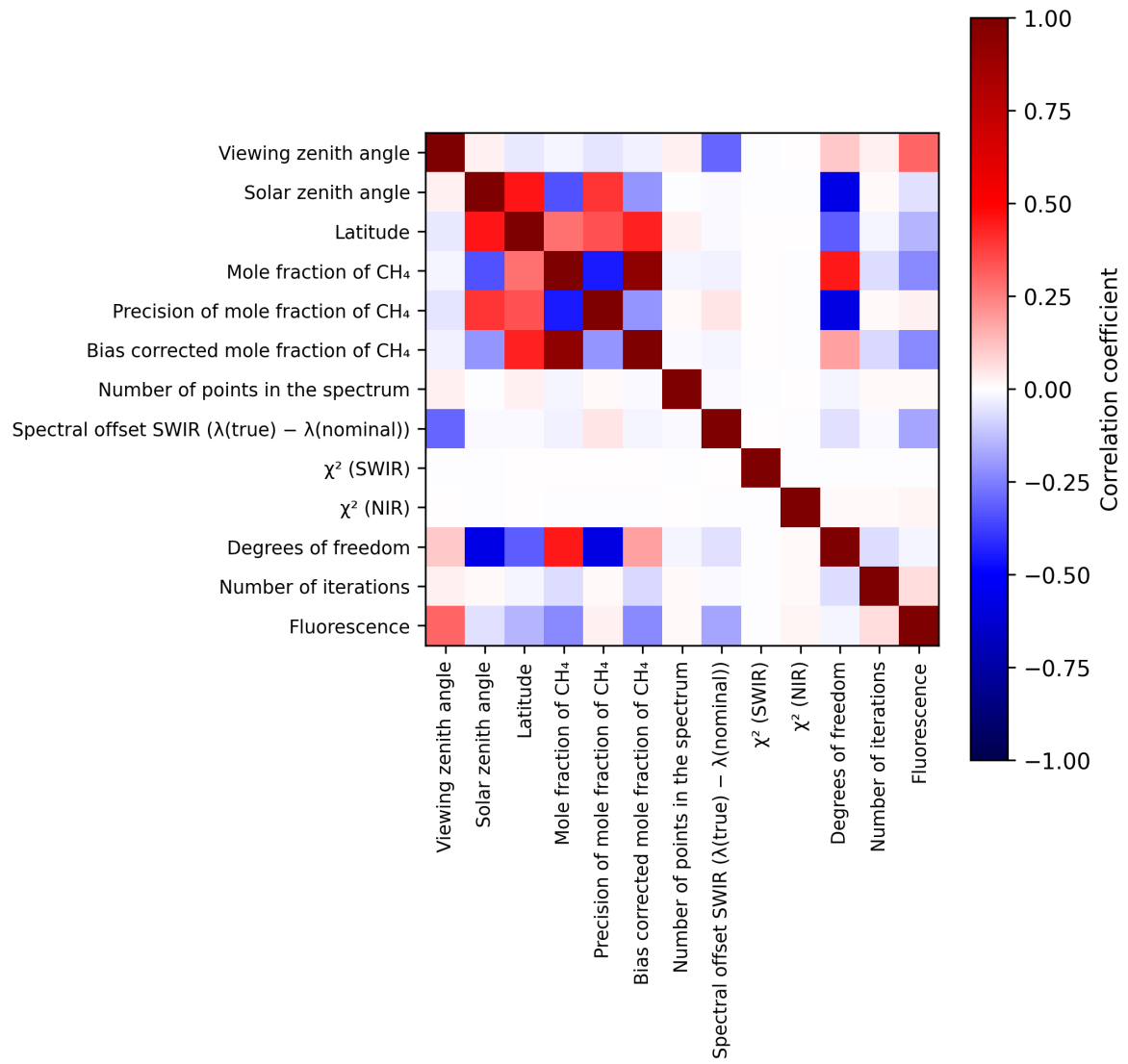
Figure 2: Map of correlation matrix for 2024-09-12 to 2024-09-14.
