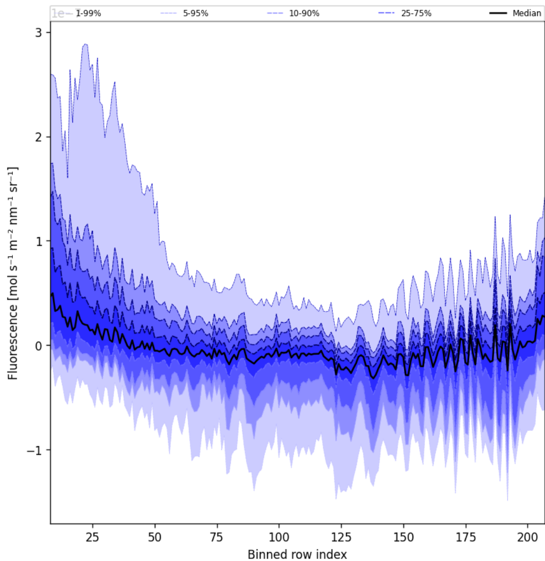
Figure 43: Along track statistics of “Fluorescence” for 2024-09-12 to 2024-09-14
