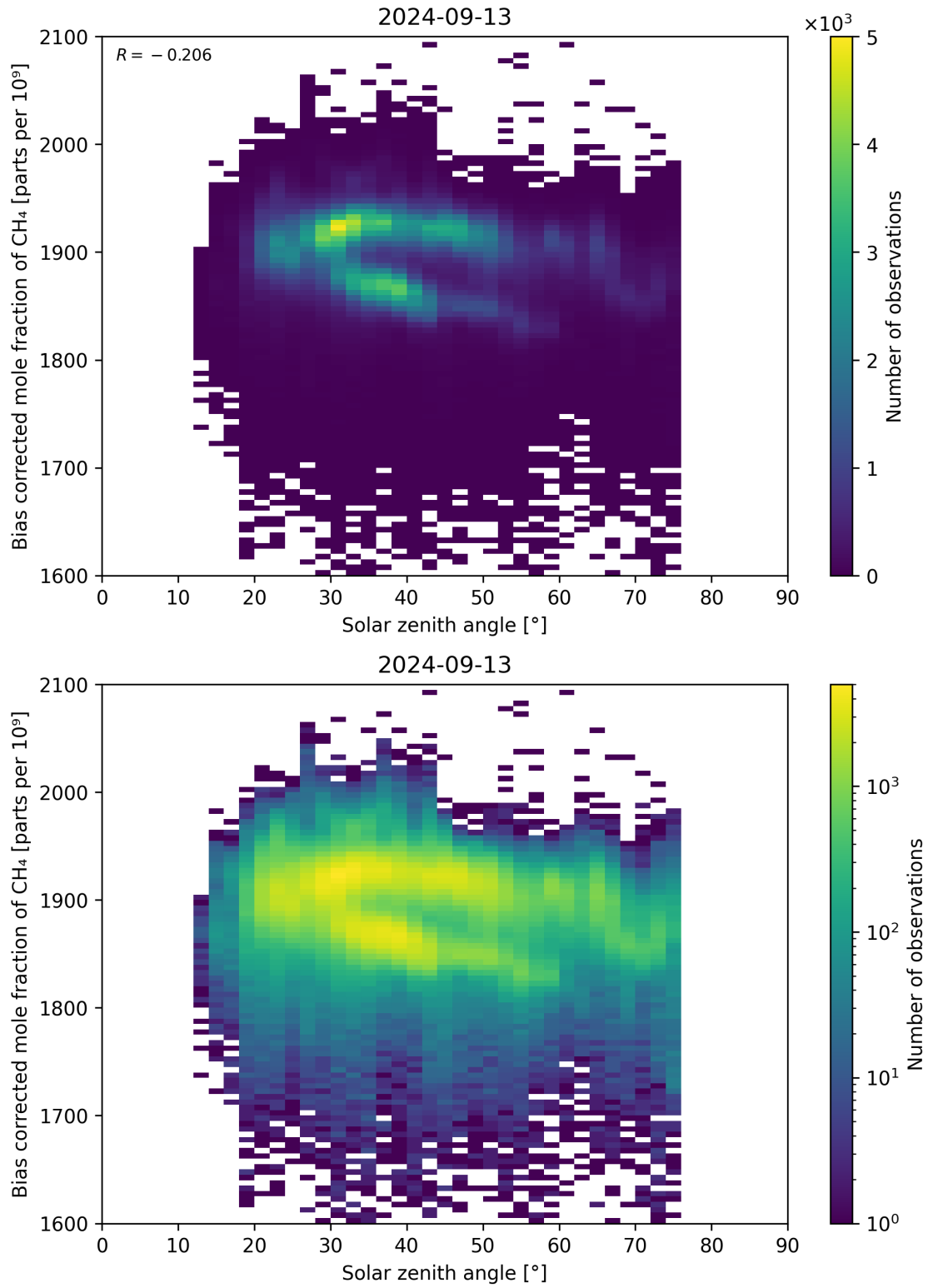
Figure 100: Scatter density plot of “Solar zenith angle” against “Bias corrected mole fraction of \text{CH}_4 ” for 2024-09-12 to 2024-09-14.
