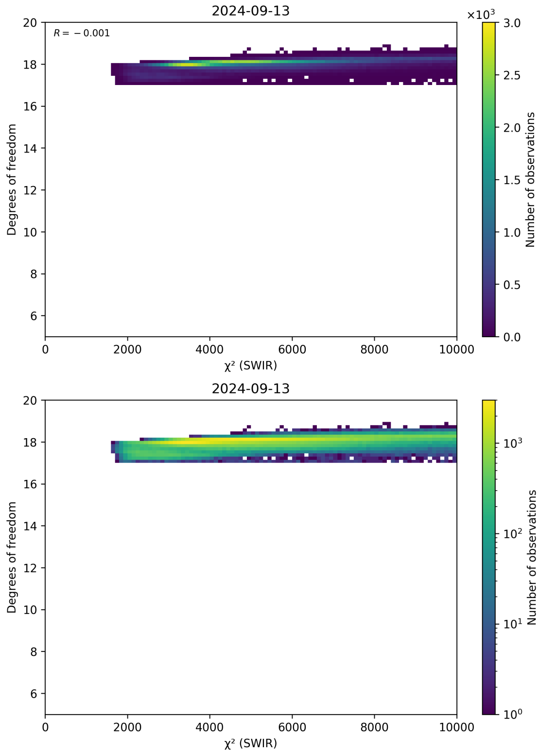
Figure 48: Scatter density plot of “ \chi^2 (SWIR)” against “Degrees of freedom” for 2024-09-12 to 2024-09-14.
