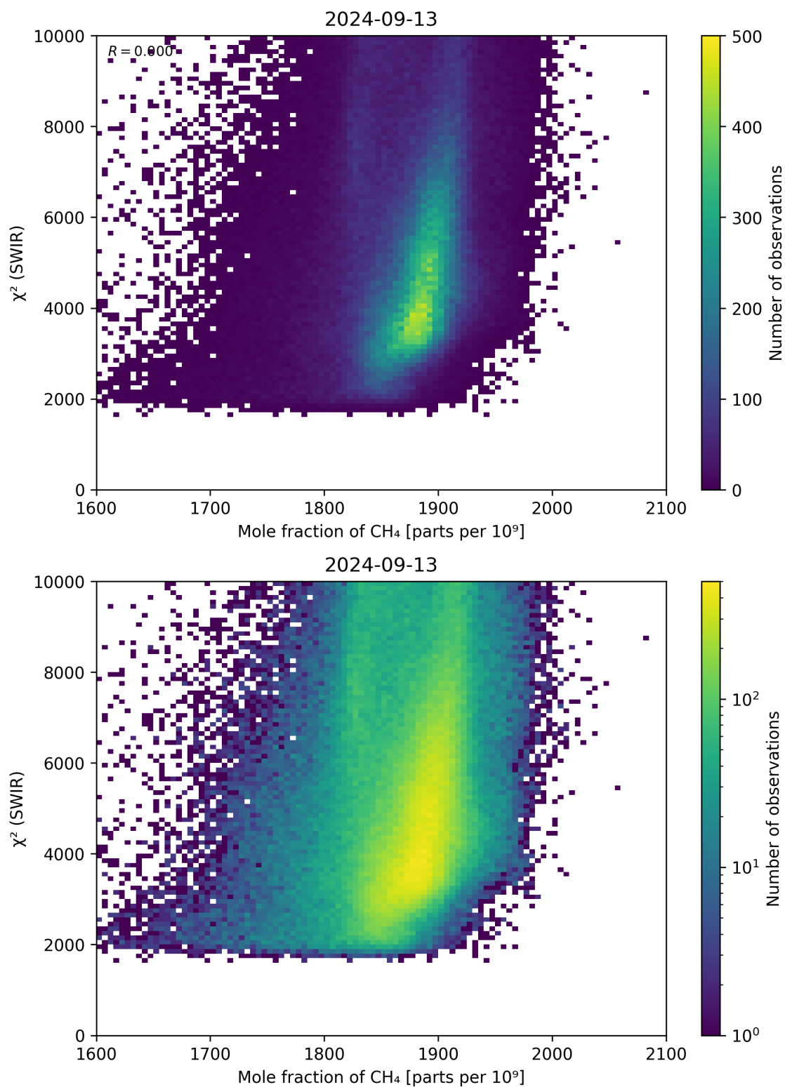
Figure 71: Scatter density plot of “Mole fraction of CH 4 ” against “ \chi^2 (SWIR)” for 2024-09-12 to 2024-09-14.
