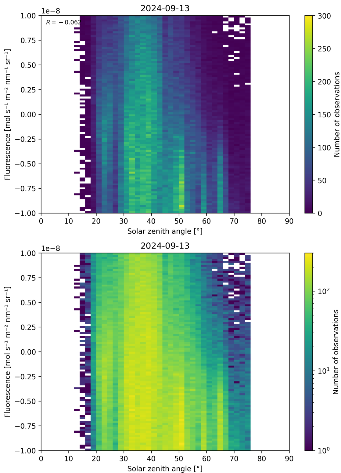
Figure 97: Scatter density plot of “Solar zenith angle” against “Fluorescence” for 2024-09-12 to 2024-09-14.
