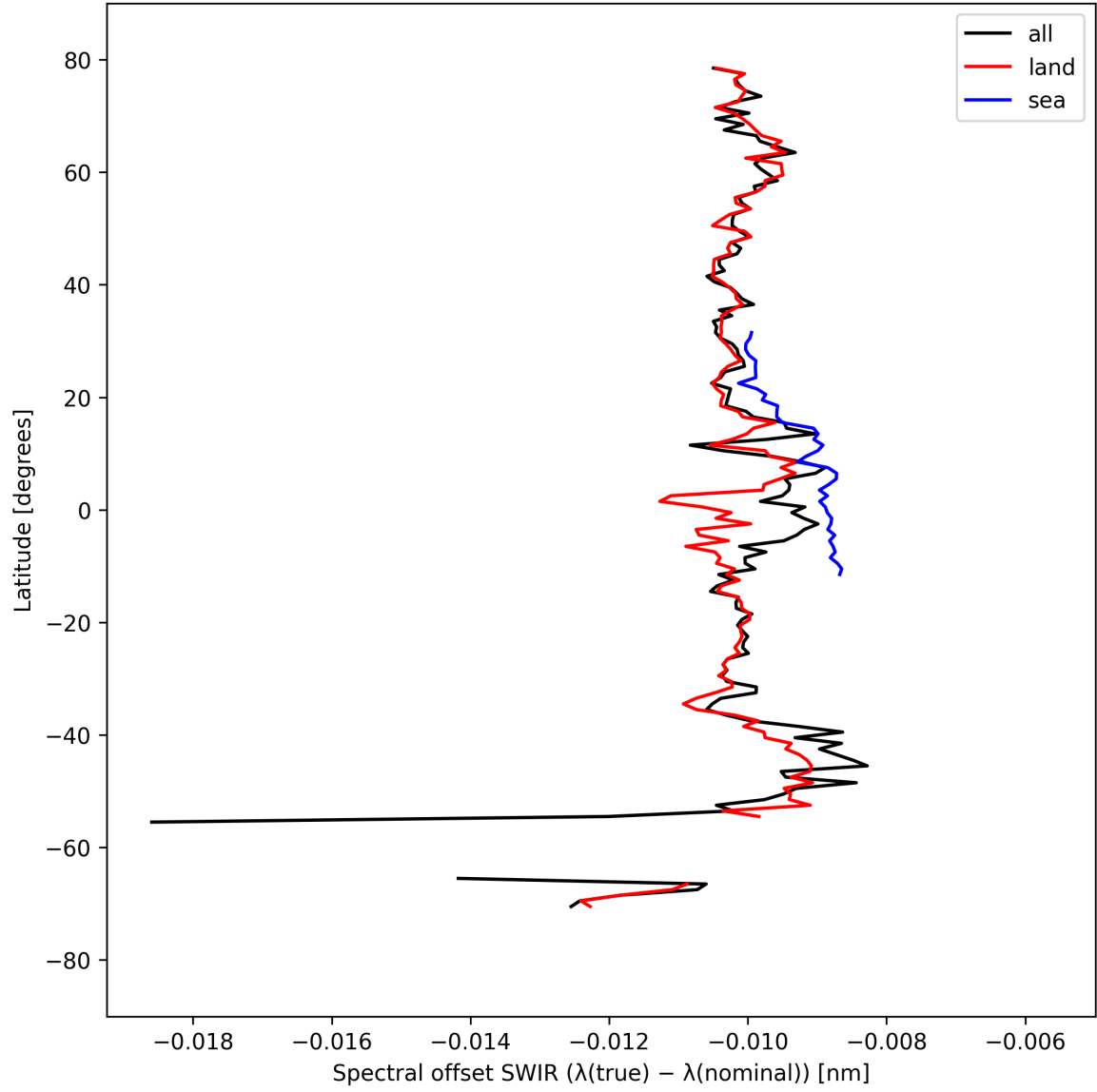
Figure 16: Zonal average of “Spectral offset SWIR ( \lambda_{\text{true}} - \lambda_{\text{nominal}} )” for 2024-09-12 to 2024-09-14.
