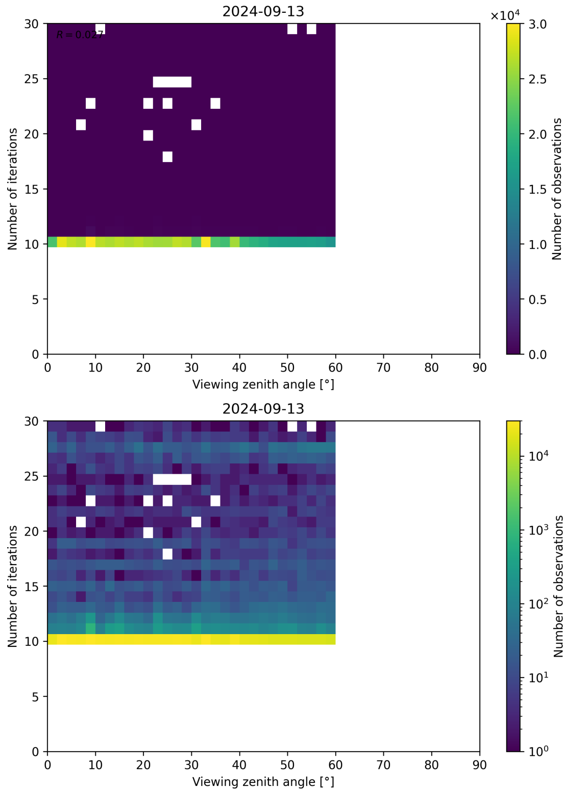
Figure 113: Scatter density plot of “Viewing zenith angle” against “Number of iterations” for 2024-09-12 to 2024-09-14.
