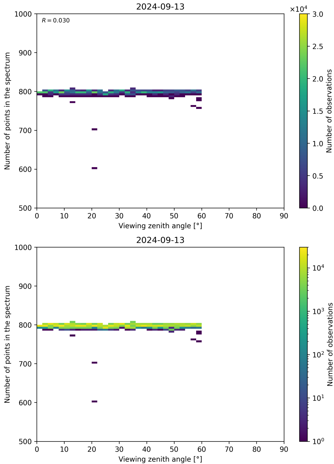
Figure 114: Scatter density plot of “Viewing zenith angle” against “Number of points in the spectrum” for 2024-09-12 to 2024-09-14.
