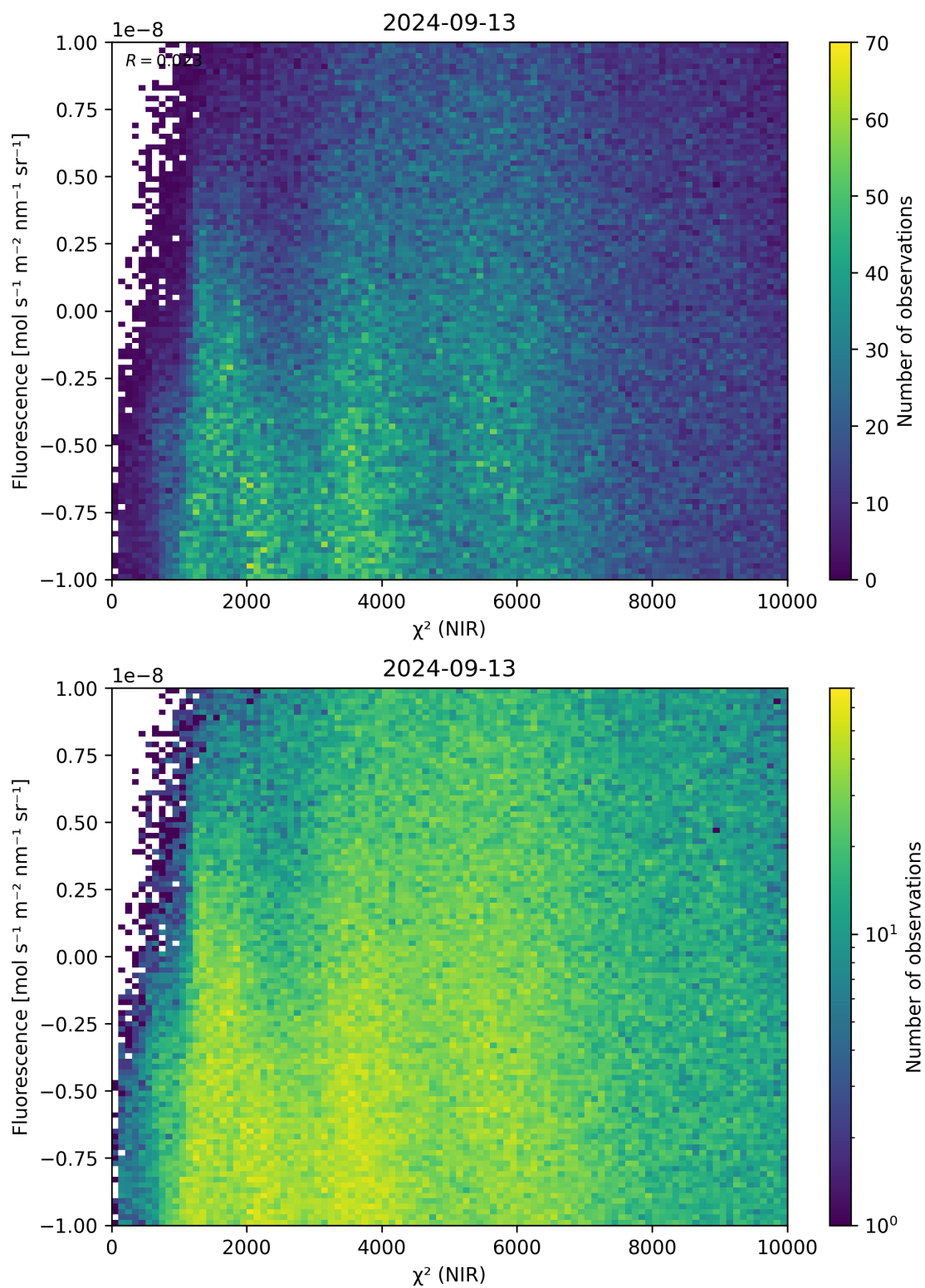
Figure 45: Scatter density plot of “ \chi^2 (NIR)” against “Fluorescence” for 2024-09-12 to 2024-09-14.
