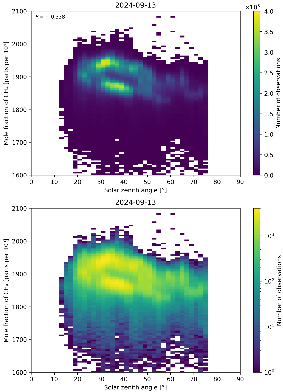
Figure 99: Scatter density plot of “Solar zenith angle” against “Mole fraction of \text{CH}_4 ” for 2024-09-12 to 2024-09-14.
