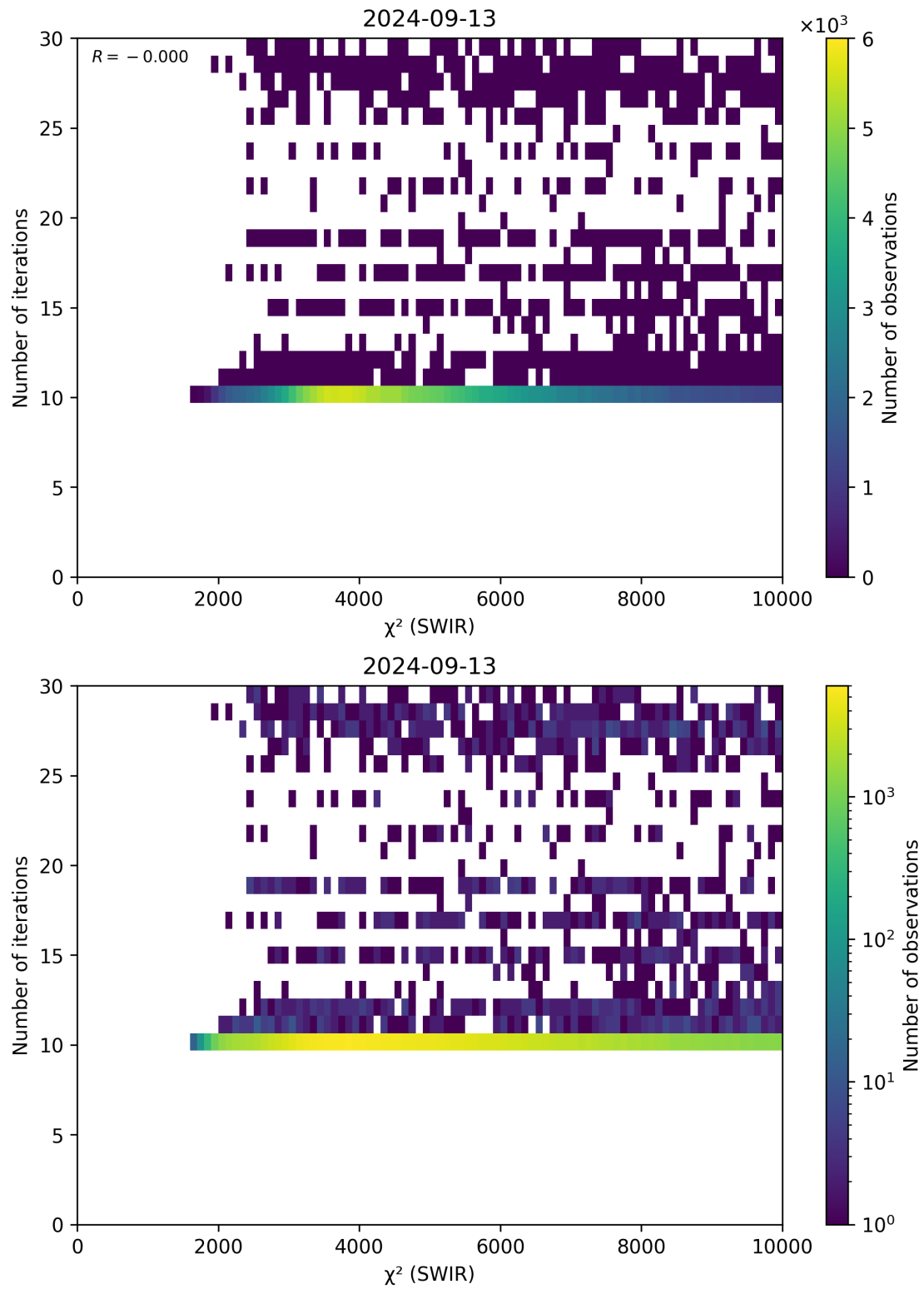
Figure 50: Scatter density plot of “ \chi^2 (SWIR)” against “Number of iterations” for 2024-09-12 to 2024-09-14.
