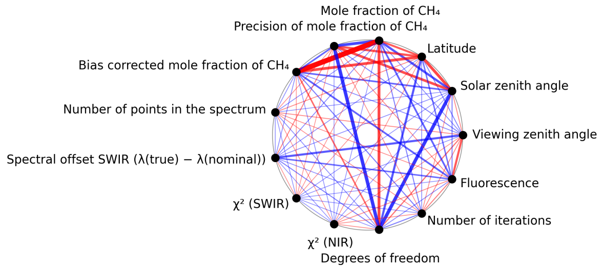
Figure 1: Map of correlation graph for 2024-09-12 to 2024-09-14.
