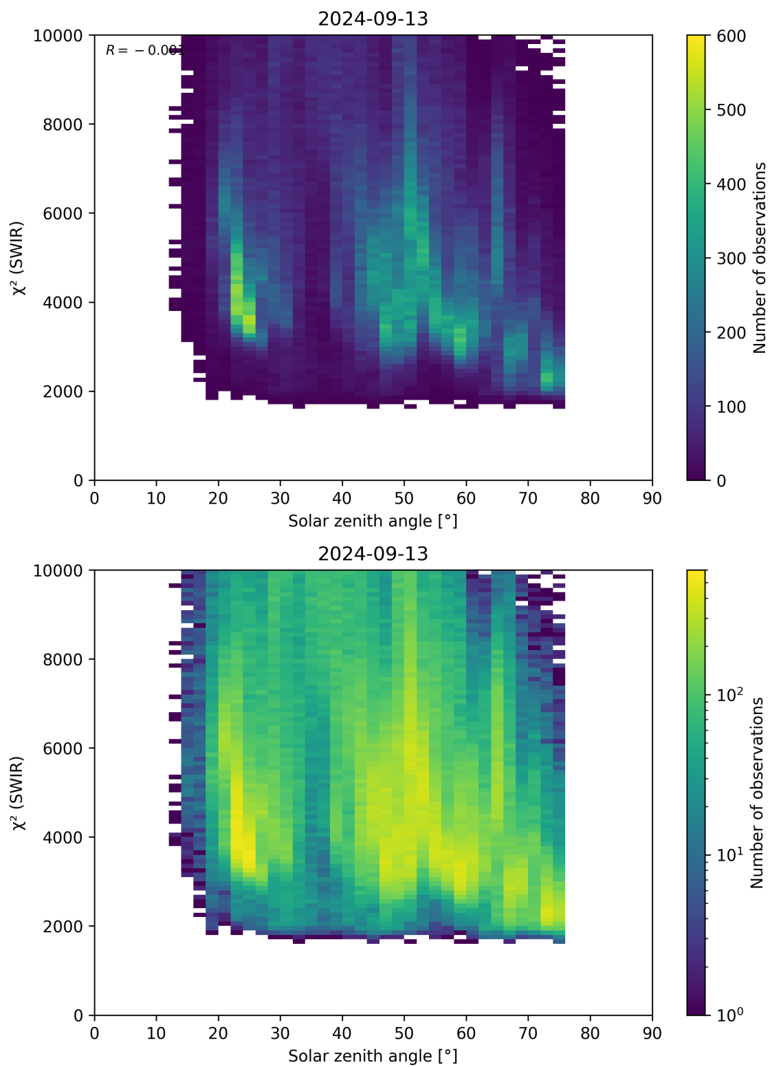
Figure 95: Scatter density plot of “Solar zenith angle” against “ \chi^2 (SWIR)” for 2024-09-12 to 2024-09-14.
