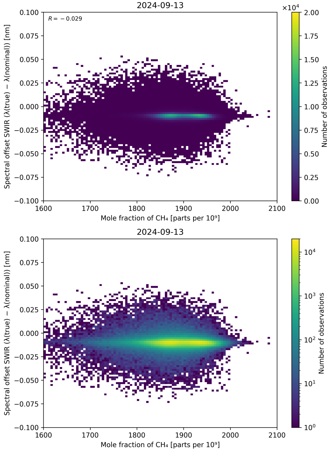
Figure 86: Scatter density plot of “Mole fraction of CH 4 ” against “Spectral offset SWIR ( \lambda_{\text{true}} - \lambda_{\text{nominal}} )” for 2024-09-12 to 2024-09-14.
