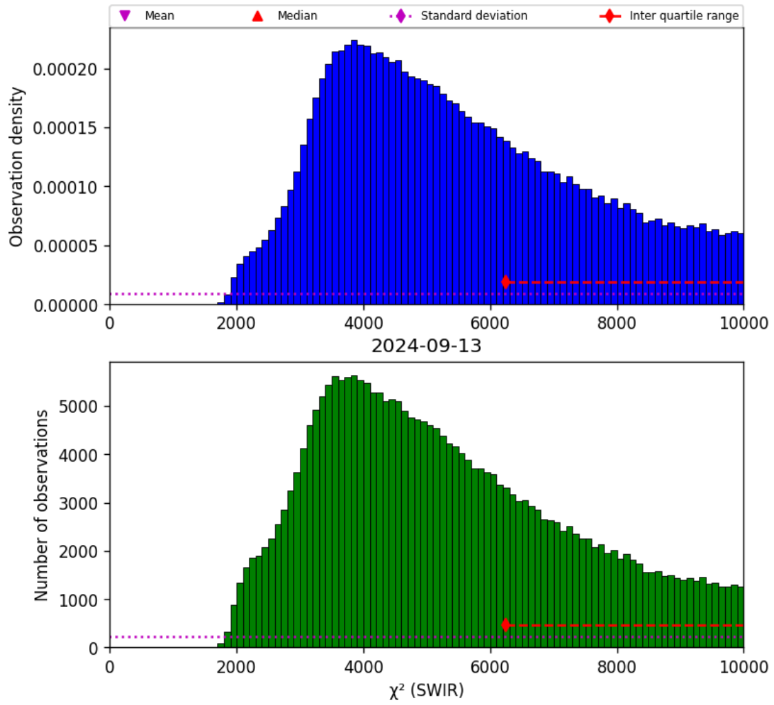
Figure 28: Histogram of " \chi^2 (SWIR)" for 2024-09-12 to 2024-09-14
