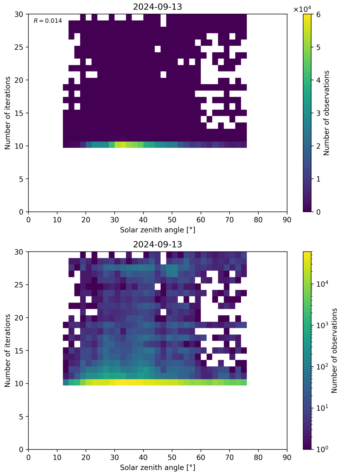
Figure 102: Scatter density plot of “Solar zenith angle” against “Number of iterations” for 2024-09-12 to 2024-09-14.
