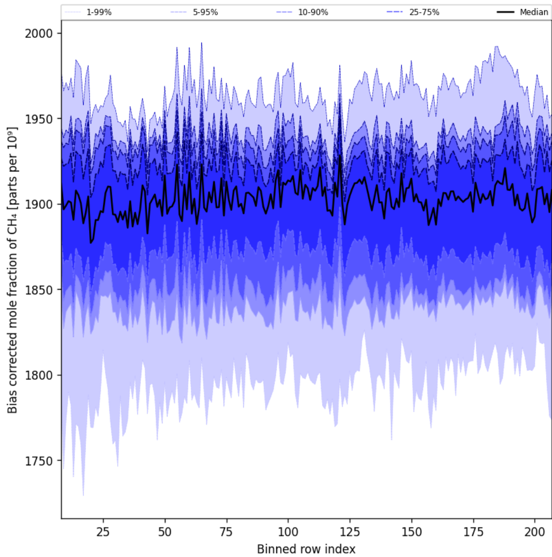
Figure 36: Along track statistics of “Bias corrected mole fraction of CH 4 ” for 2024-09-12 to 2024-09-14
