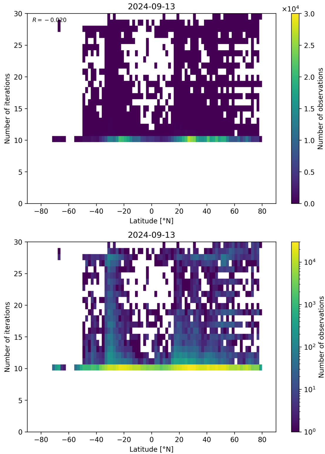
Figure 60: Scatter density plot of “Latitude” against “Number of iterations” for 2024-09-12 to 2024-09-14.
