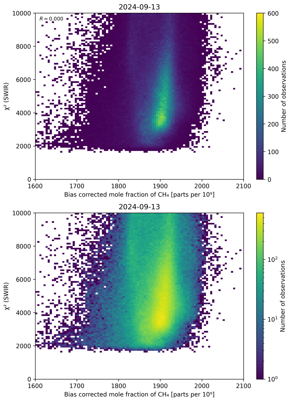
Figure 64: Scatter density plot of “Bias corrected mole fraction of CH 4 ” against “ \chi^2 (SWIR)” for 2024-09-12 to 2024-09-14.
