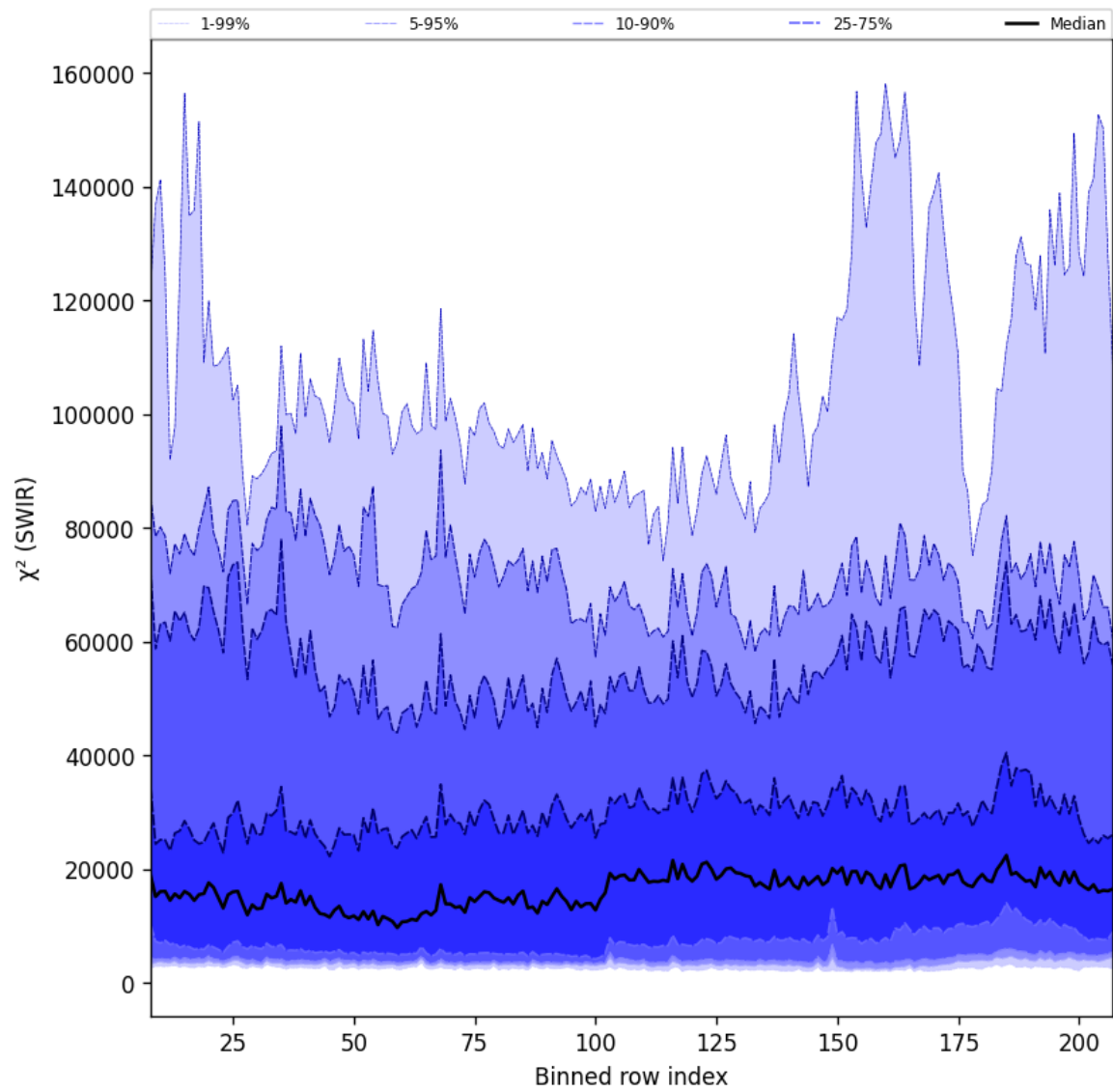
Figure 39: Along track statistics of “ \chi^2 (SWIR)” for 2024-09-12 to 2024-09-14
