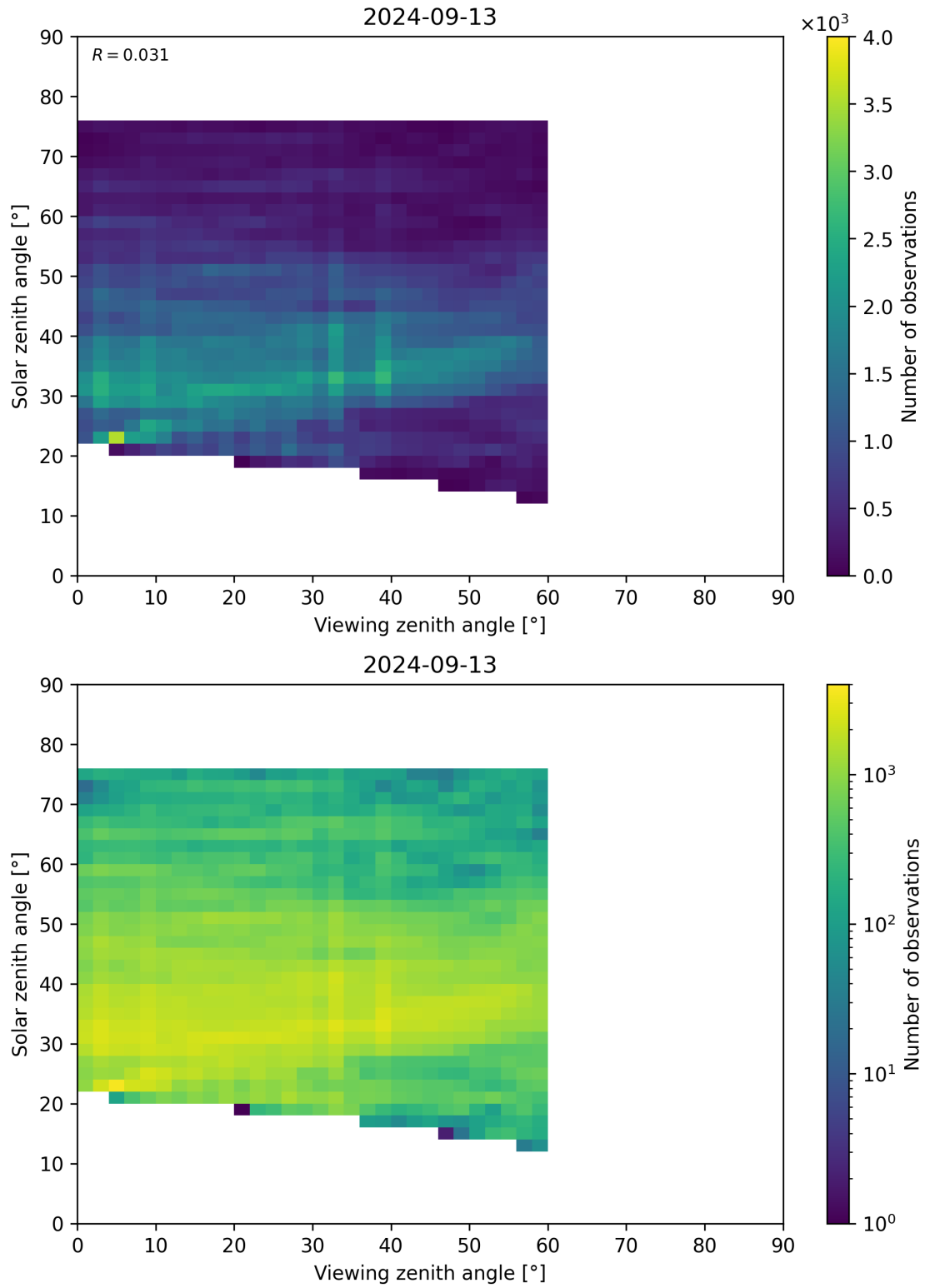
Figure 115: Scatter density plot of “Viewing zenith angle” against “Solar zenith angle” for 2024-09-12 to 2024-09-14.
