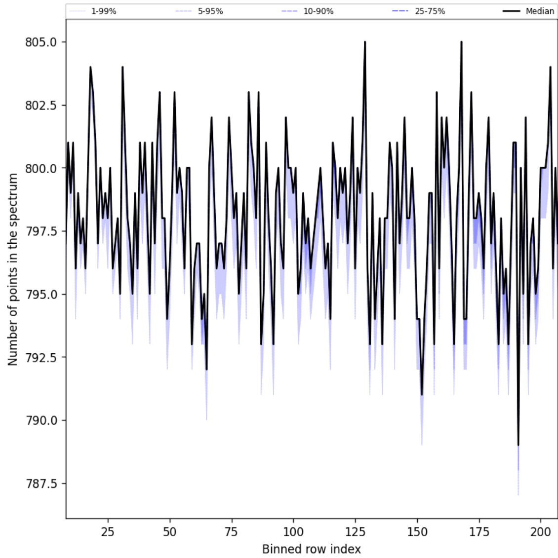
Figure 37: Along track statistics of “Number of points in the spectrum” for 2024-09-12 to 2024-09-14
