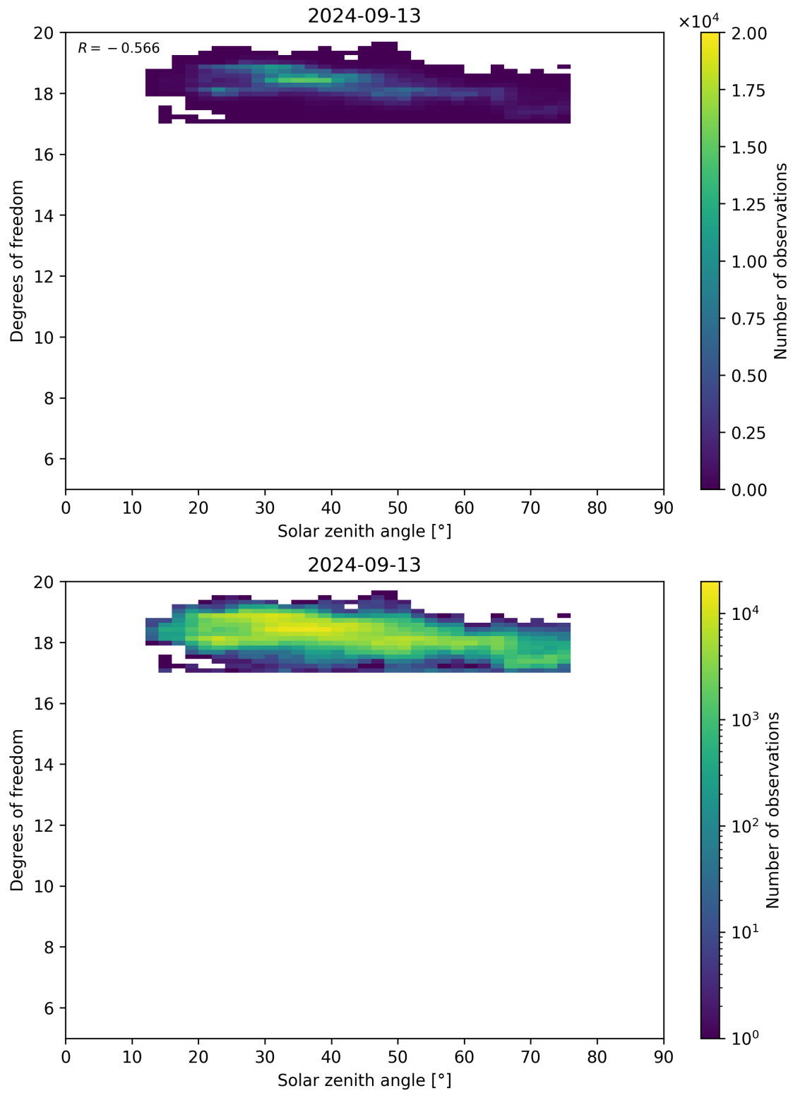
Figure 96: Scatter density plot of “Solar zenith angle” against “Degrees of freedom” for 2024-09-12 to 2024-09-14.
