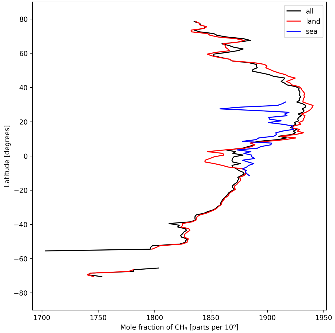
Figure 12: Zonal average of “Mole fraction of \text{CH}_4 ” for 2024-09-12 to 2024-09-14.
