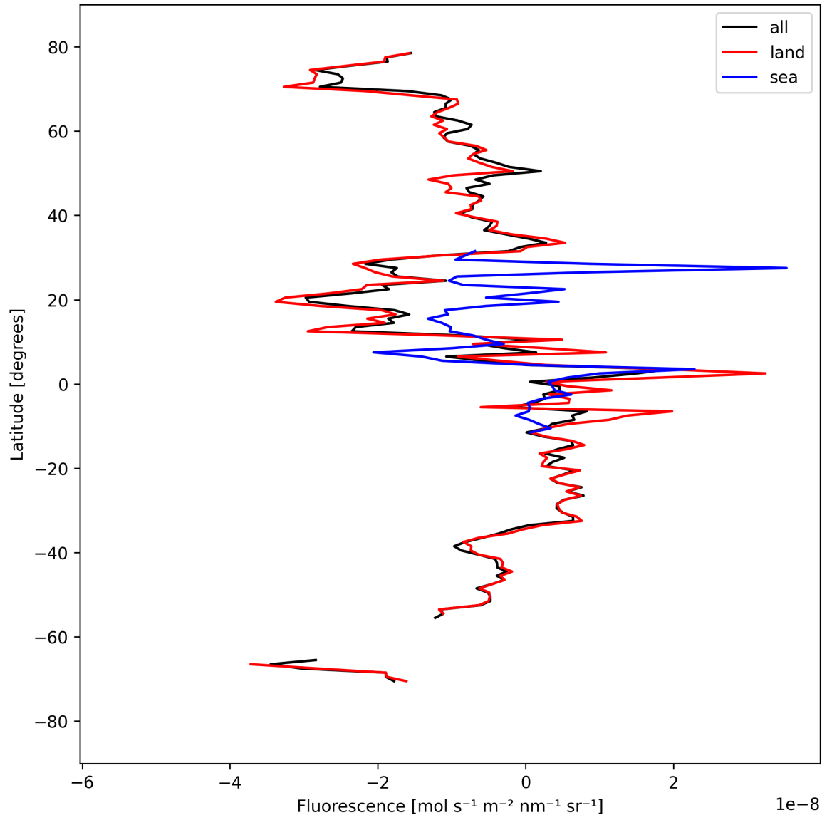
Figure 21: Zonal average of “Fluorescence” for 2024-09-12 to 2024-09-14.
