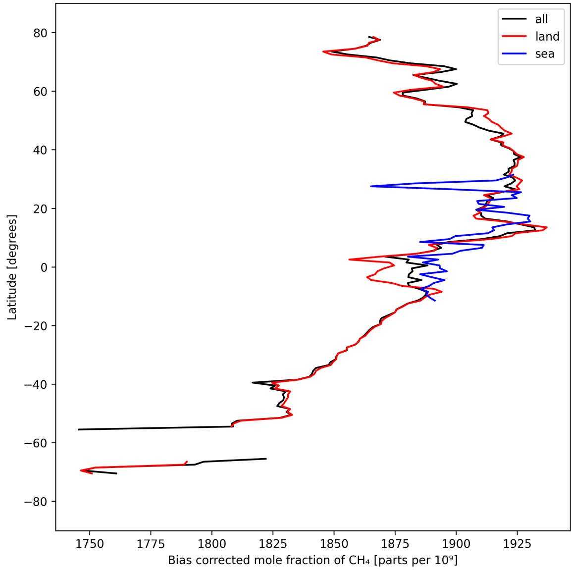
Figure 14: Zonal average of “Bias corrected mole fraction of CH 4 ” for 2024-09-12 to 2024-09-14.
