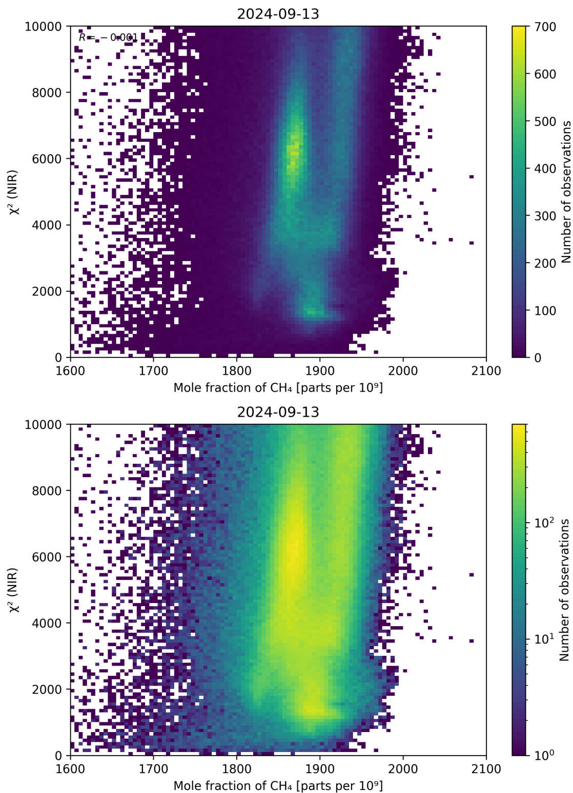
Figure 70: Scatter density plot of “Mole fraction of \text{CH}_4 ” against “ \chi^2 (NIR)” for 2024-09-12 to 2024-09-14.
