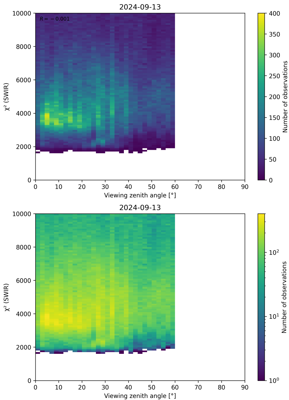
Figure 106: Scatter density plot of “Viewing zenith angle” against “ \chi^2 (SWIR)” for 2024-09-12 to 2024-09-14.
