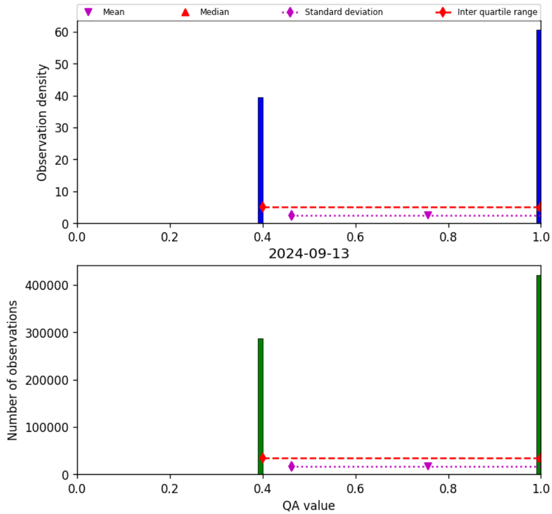
Figure 22: Histogram of “QA value” for 2024-09-12 to 2024-09-14
