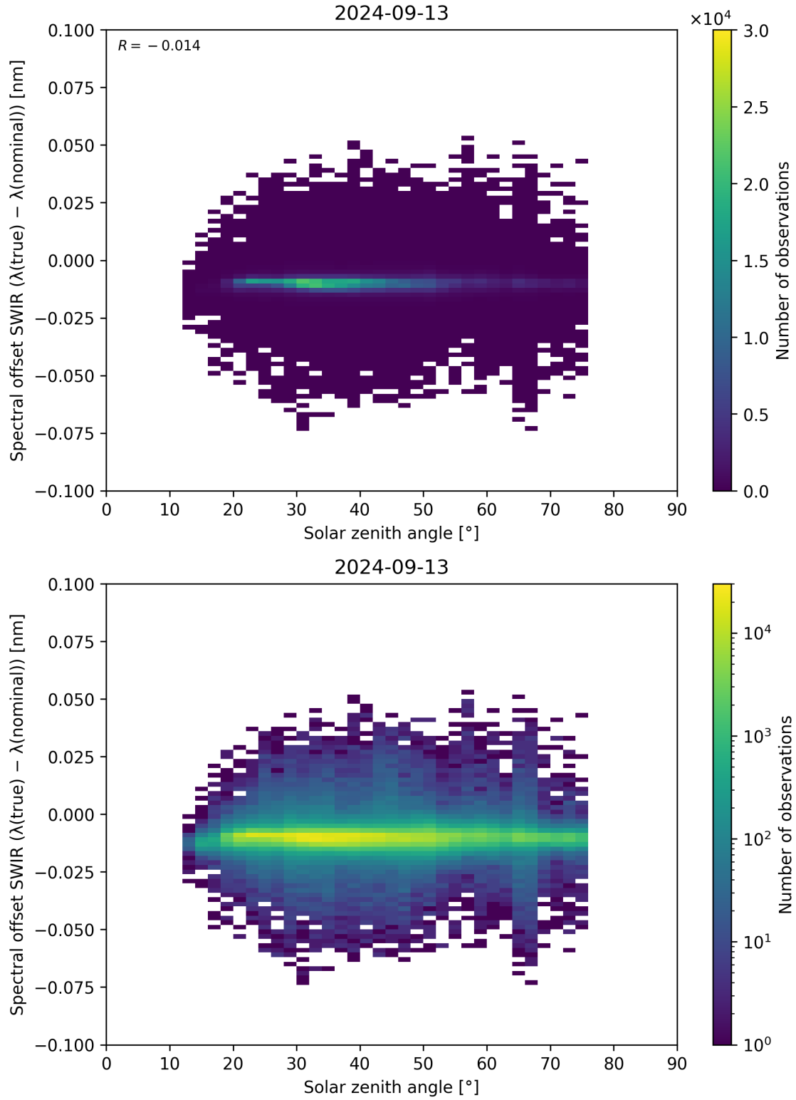
Figure 104: Scatter density plot of “Solar zenith angle” against “Spectral offset SWIR ( \lambda_{\text{true}} - \lambda_{\text{nominal}} )” for 2024-09-12 to 2024-09-14.
