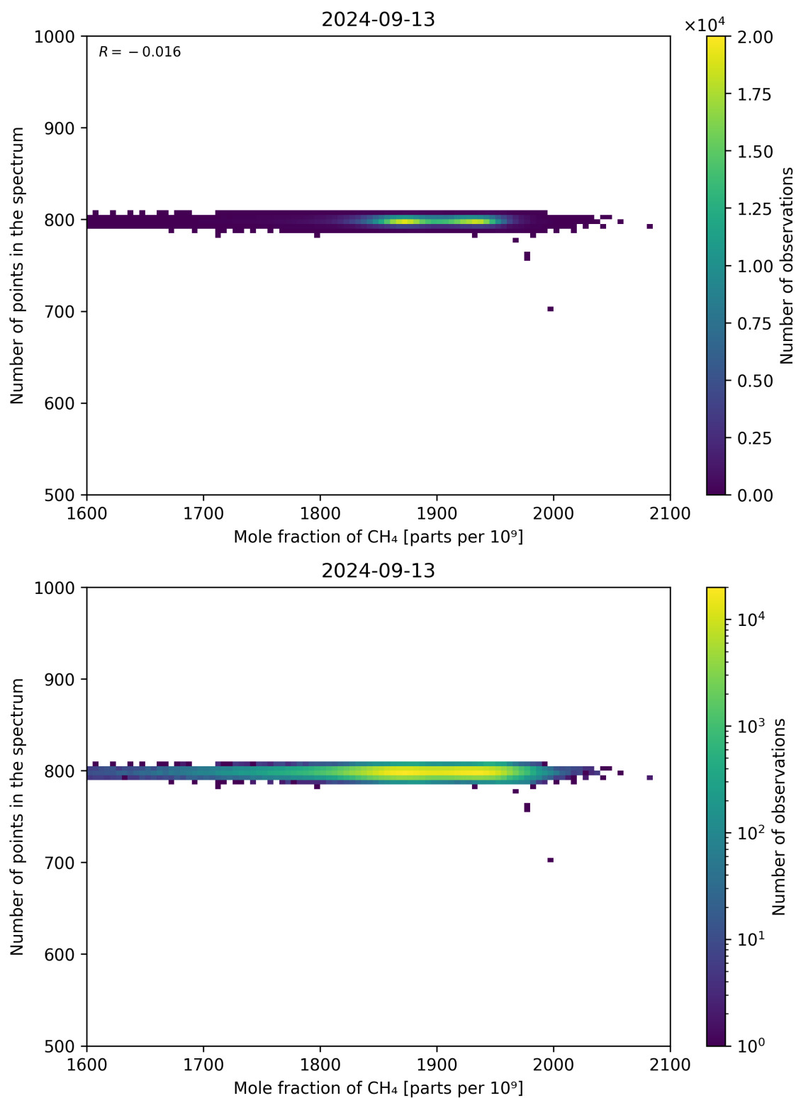
Figure 77: Scatter density plot of “Mole fraction of CH 4 ” against “Number of points in the spectrum” for 2024-09-12 to 2024-09-14.
