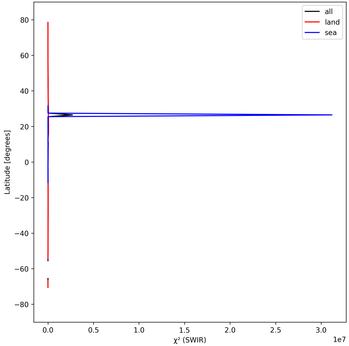
Figure 17: Zonal average of “ \chi^2 (SWIR)” for 2024-09-12 to 2024-09-14.
