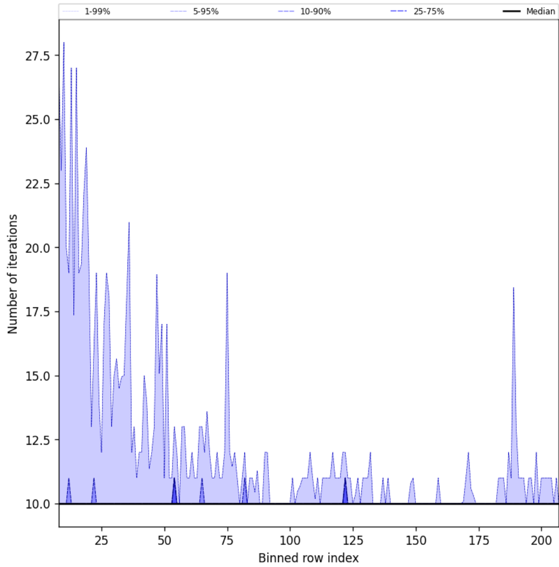
Figure 42: Along track statistics of “Number of iterations” for 2024-09-12 to 2024-09-14
