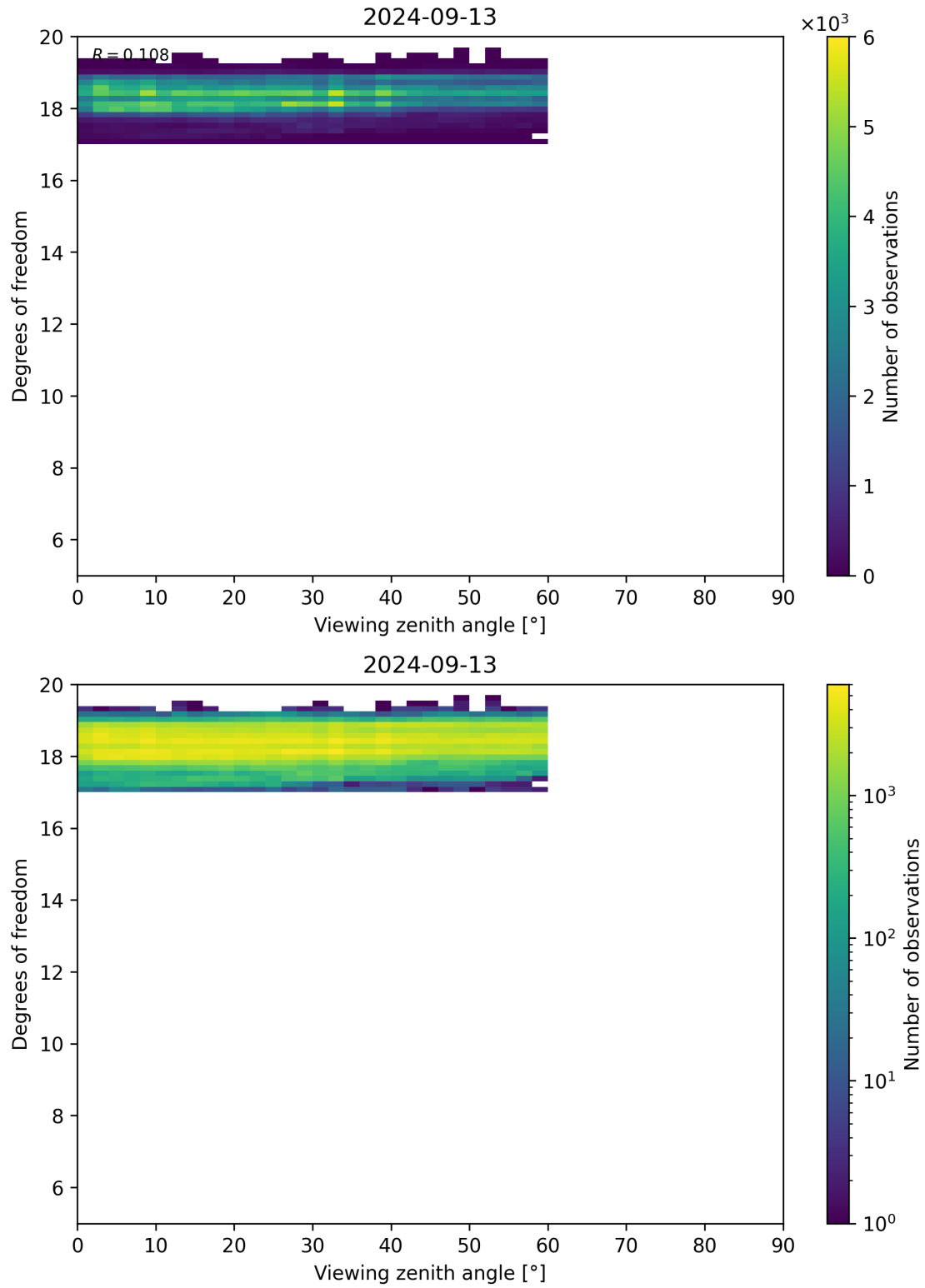
Figure 107: Scatter density plot of “Viewing zenith angle” against “Degrees of freedom” for 2024-09-12 to 2024-09-14.
