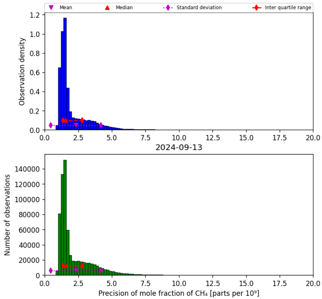
Figure 24: Histogram of “Precision of mole fraction of CH 4 ” for 2024-09-12 to 2024-09-14
