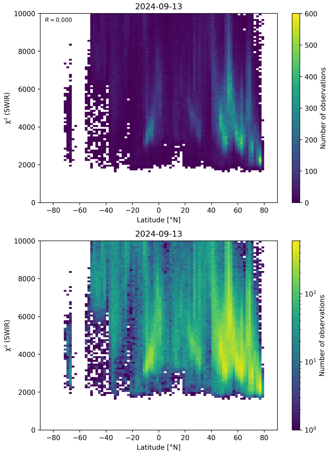
Figure 54: Scatter density plot of “Latitude” against “ \chi^2 (SWIR)” for 2024-09-12 to 2024-09-14.
