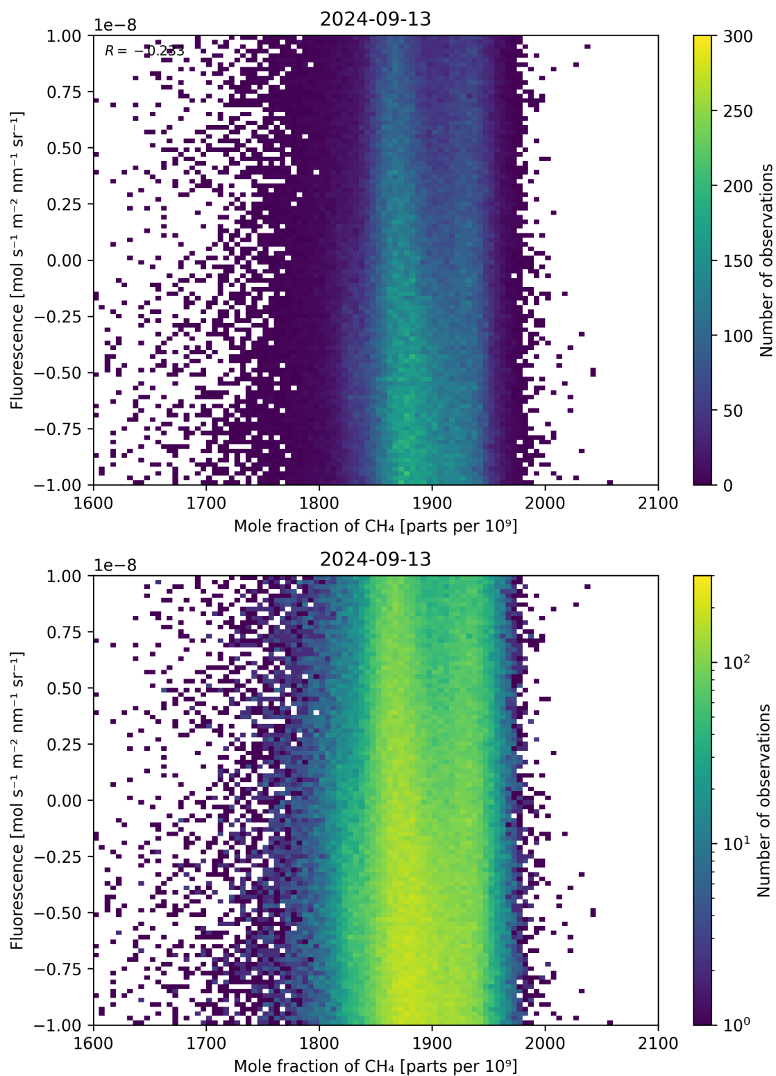
Figure 73: Scatter density plot of “Mole fraction of \text{CH}_4 ” against “Fluorescence” for 2024-09-12 to 2024-09-14.
