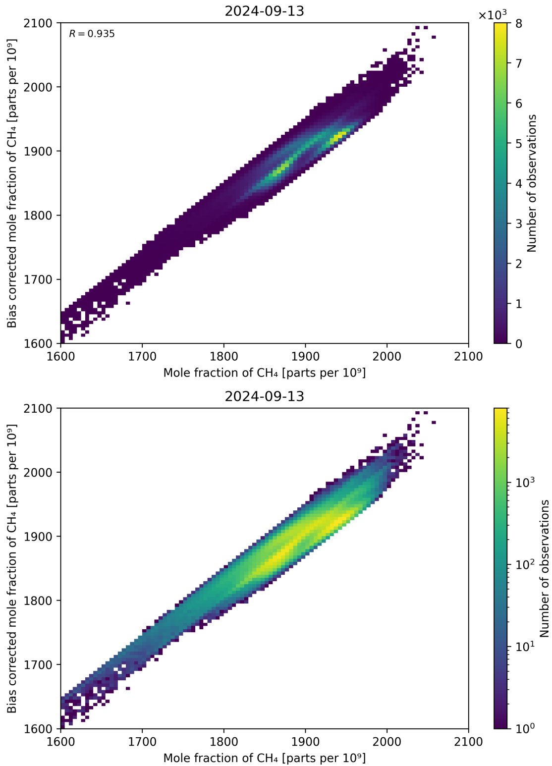
Figure 74: Scatter density plot of “Mole fraction of CH 4 ” against “Bias corrected mole fraction of CH 4 ” for 2024-09-12 to 2024-09-14.
