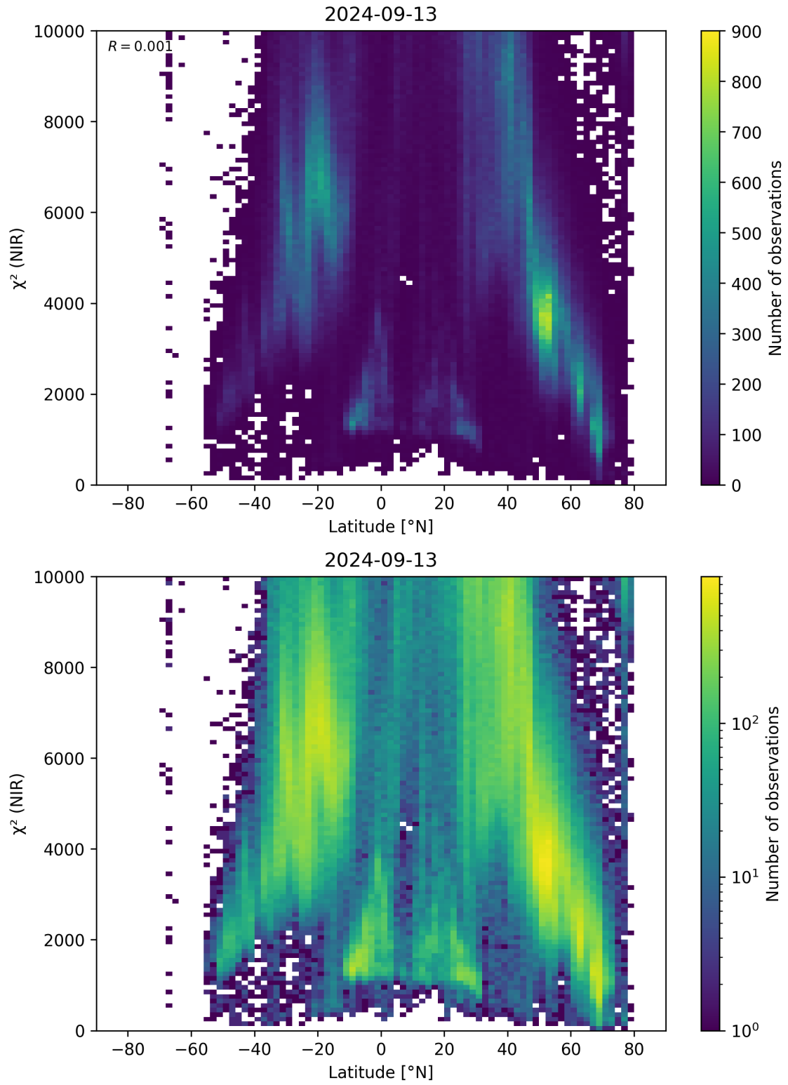
Figure 53: Scatter density plot of “Latitude” against “ \chi^2 (NIR)” for 2024-09-12 to 2024-09-14.
