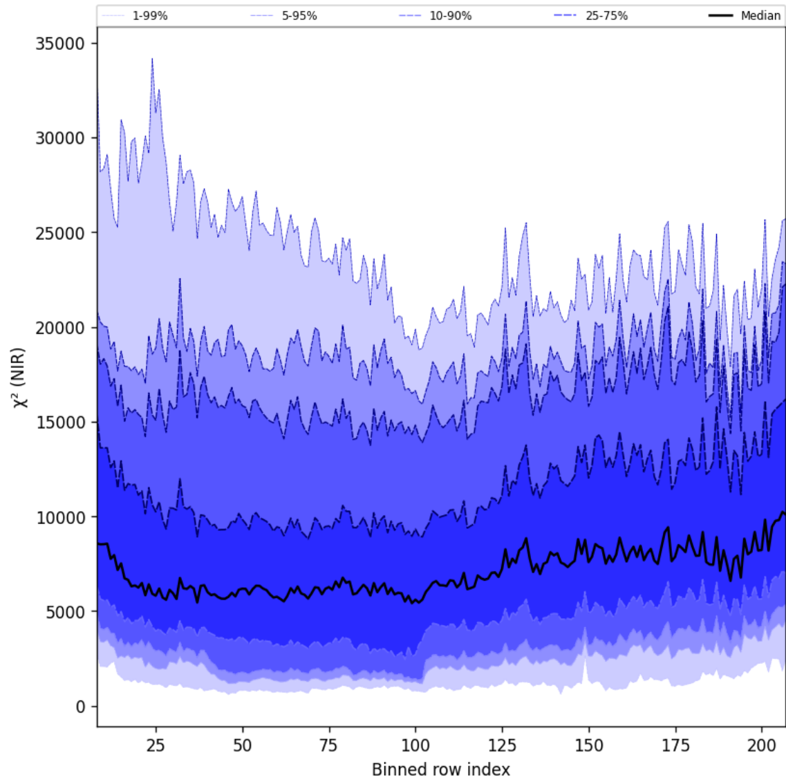
Figure 40: Along track statistics of “ \chi^2 (NIR)” for 2024-09-12 to 2024-09-14
