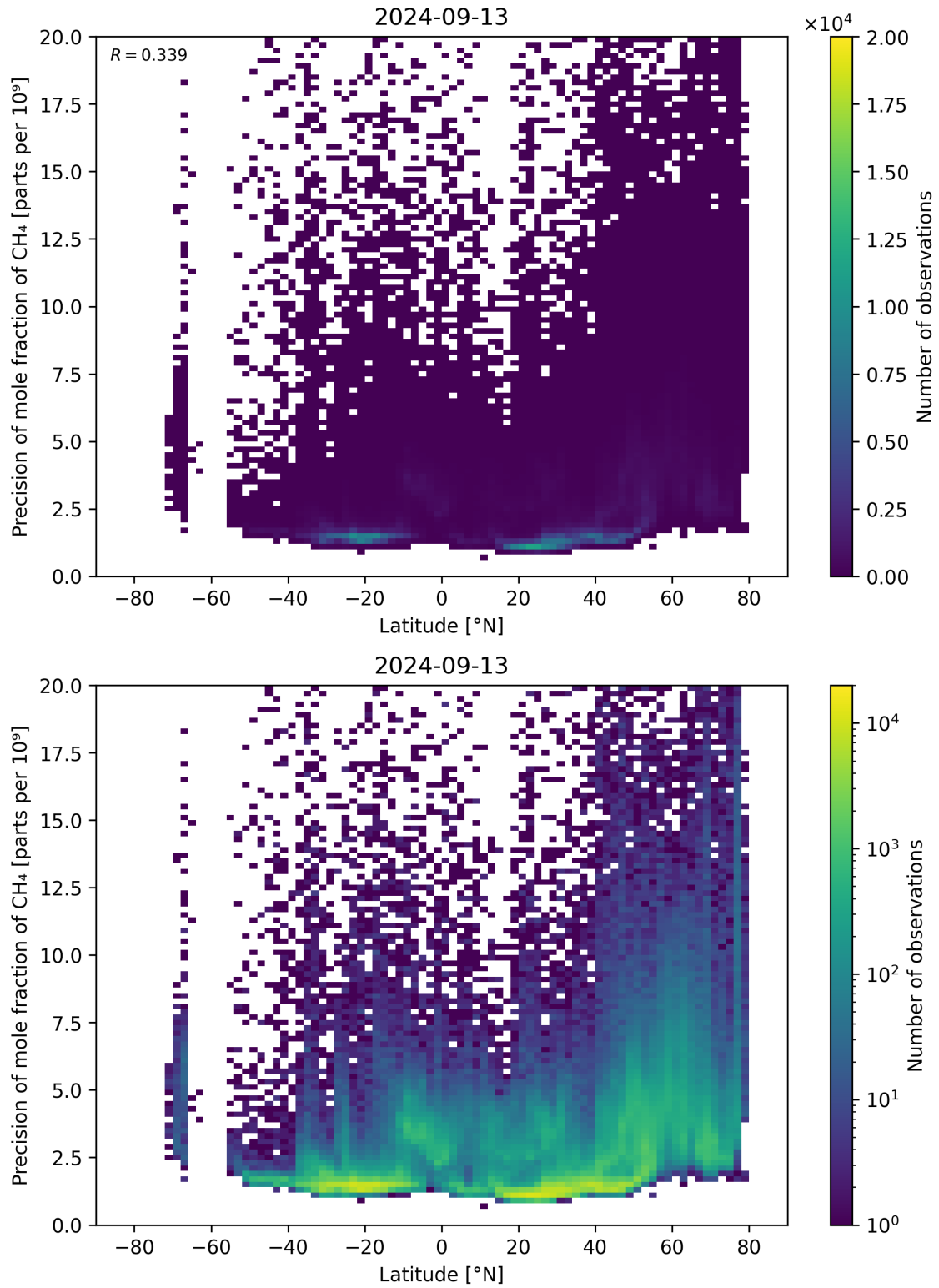
Figure 59: Scatter density plot of “Latitude” against “Precision of mole fraction of \text{CH}_4 ” for 2024-09-12 to 2024-09-14.
