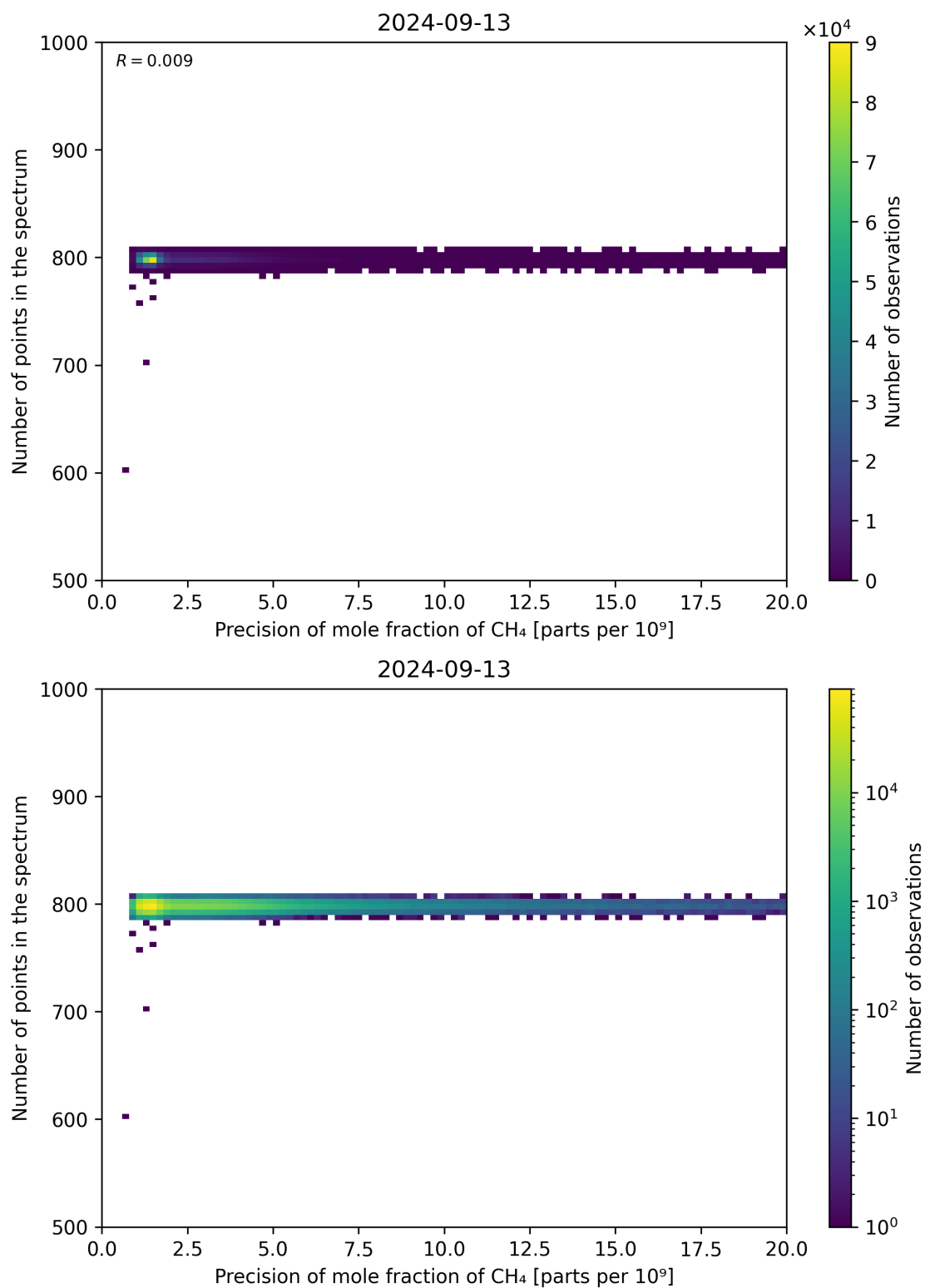
Figure 84: Scatter density plot of “Precision of mole fraction of CH 4 ” against “Number of points in the spectrum” for 2024-09-12 to 2024-09-14.
