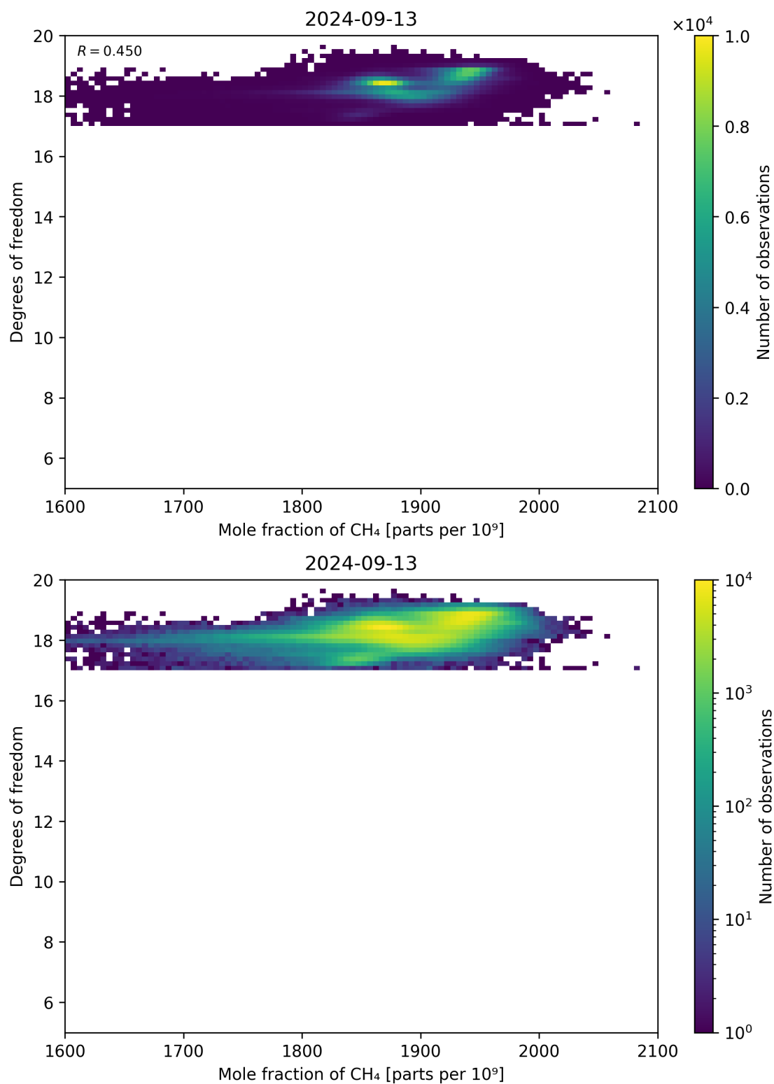
Figure 72: Scatter density plot of “Mole fraction of CH 4 ” against “Degrees of freedom” for 2024-09-12 to 2024-09-14.
