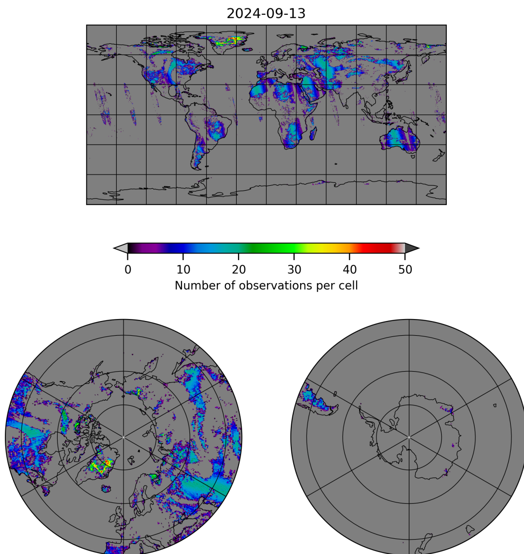
Figure 10: Map of the number of observations for 2024-09-12 to 2024-09-14
