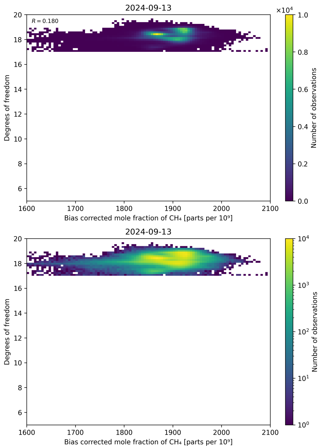
Figure 65: Scatter density plot of “Bias corrected mole fraction of CH 4 ” against “Degrees of freedom” for 2024-09-12 to 2024-09-14.
