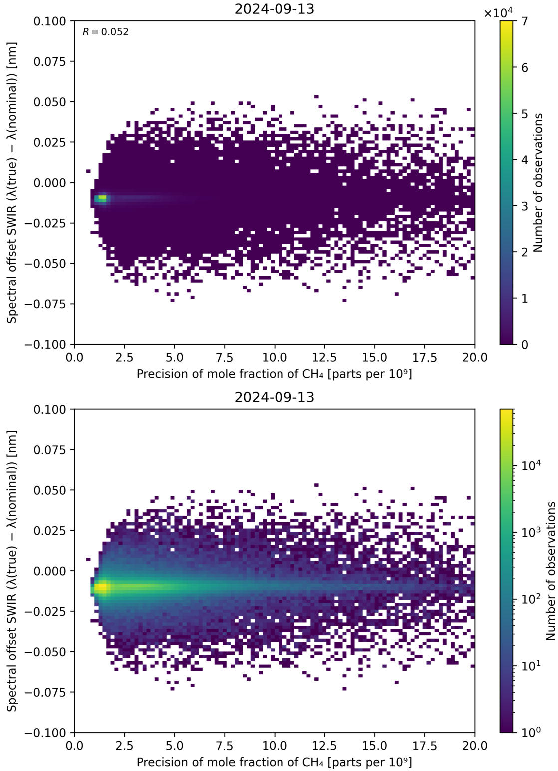
Figure 85: Scatter density plot of “Precision of mole fraction of CH 4 ” against “Spectral offset SWIR ( \lambda_{\text{true}} - \lambda_{\text{nominal}} )” for 2024-09-12 to 2024-09-14.
