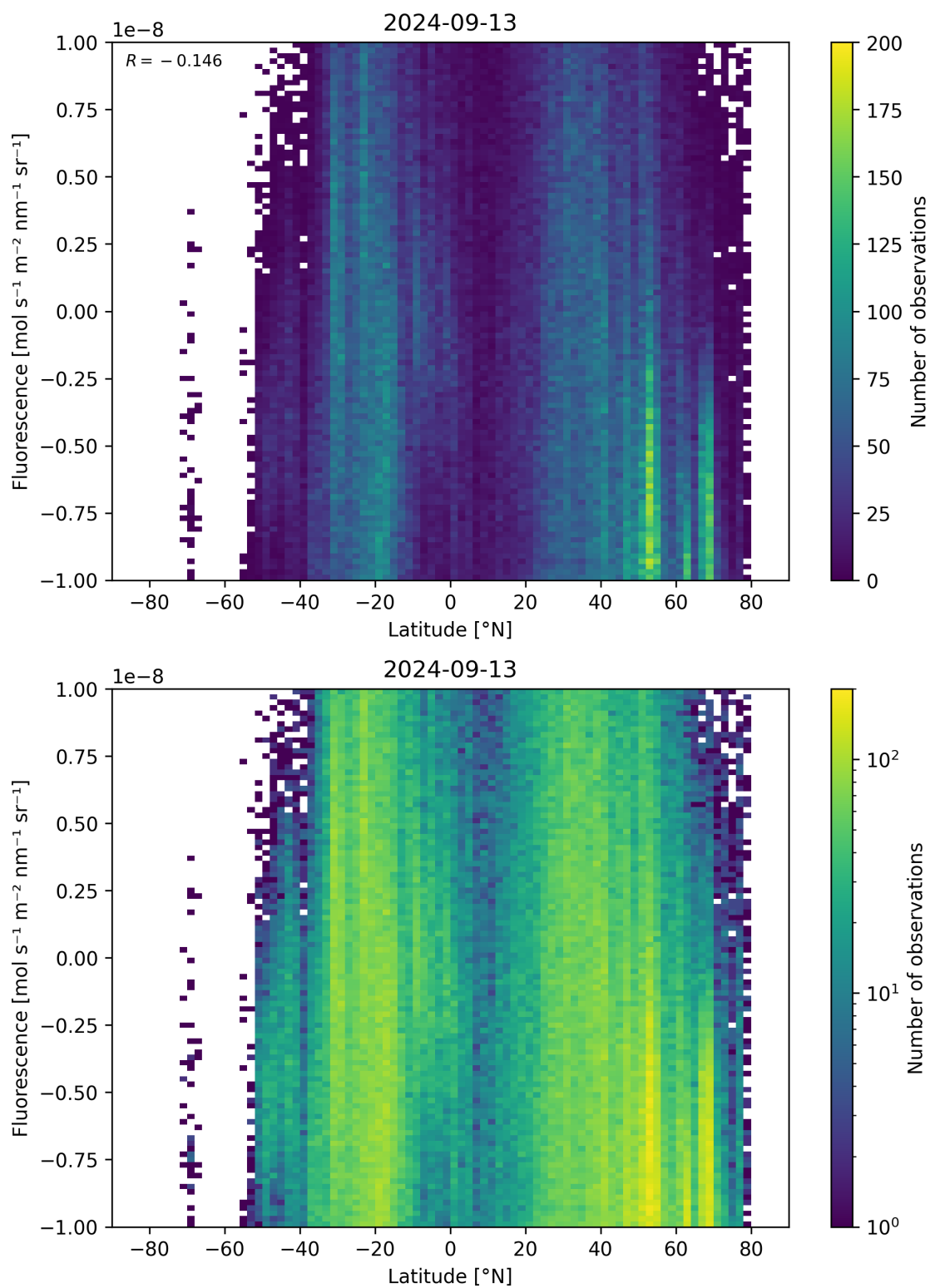
Figure 56: Scatter density plot of “Latitude” against “Fluorescence” for 2024-09-12 to 2024-09-14.
