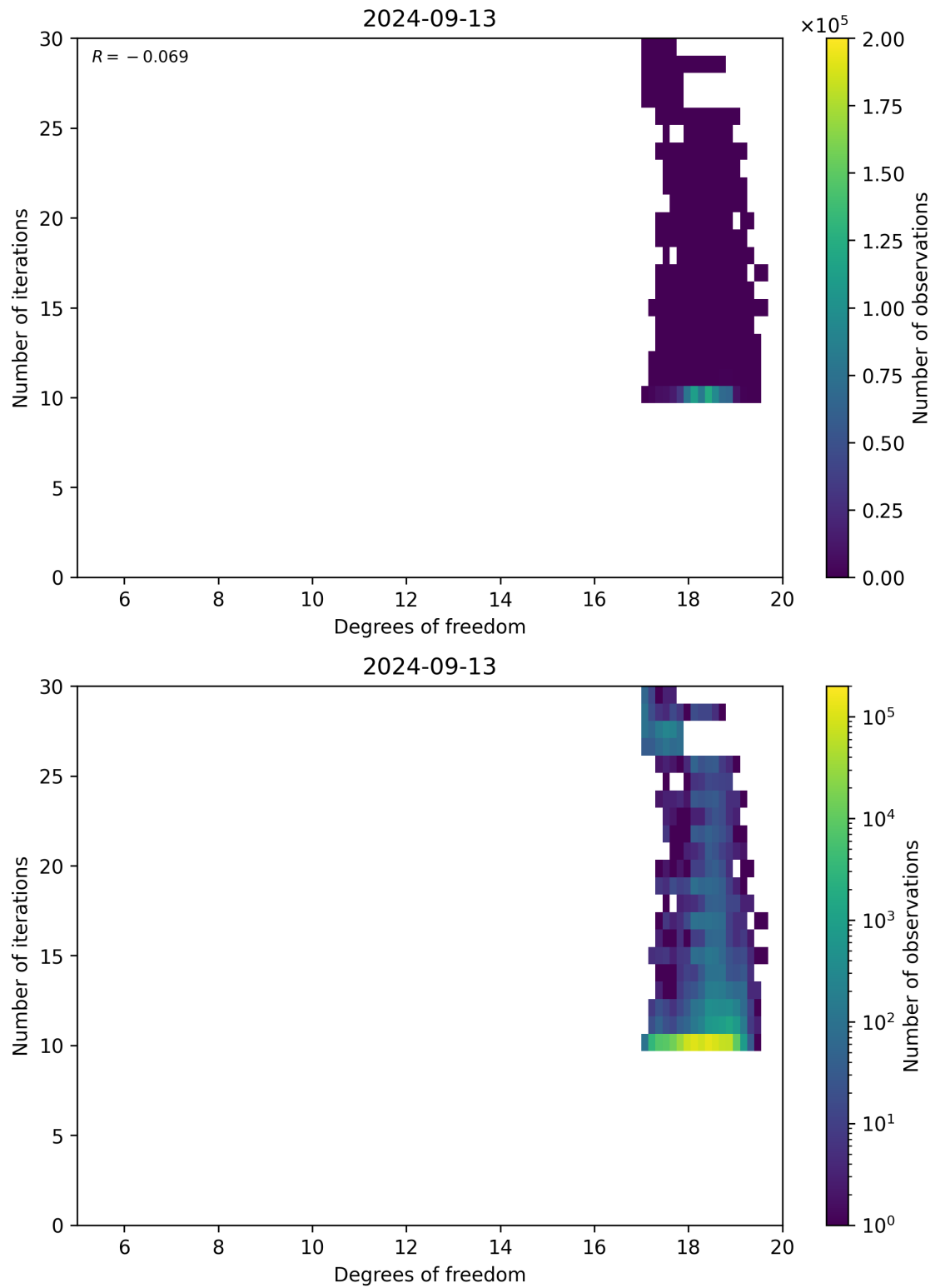
Figure 52: Scatter density plot of “Degrees of freedom” against “Number of iterations” for 2024-09-12 to 2024-09-14.
