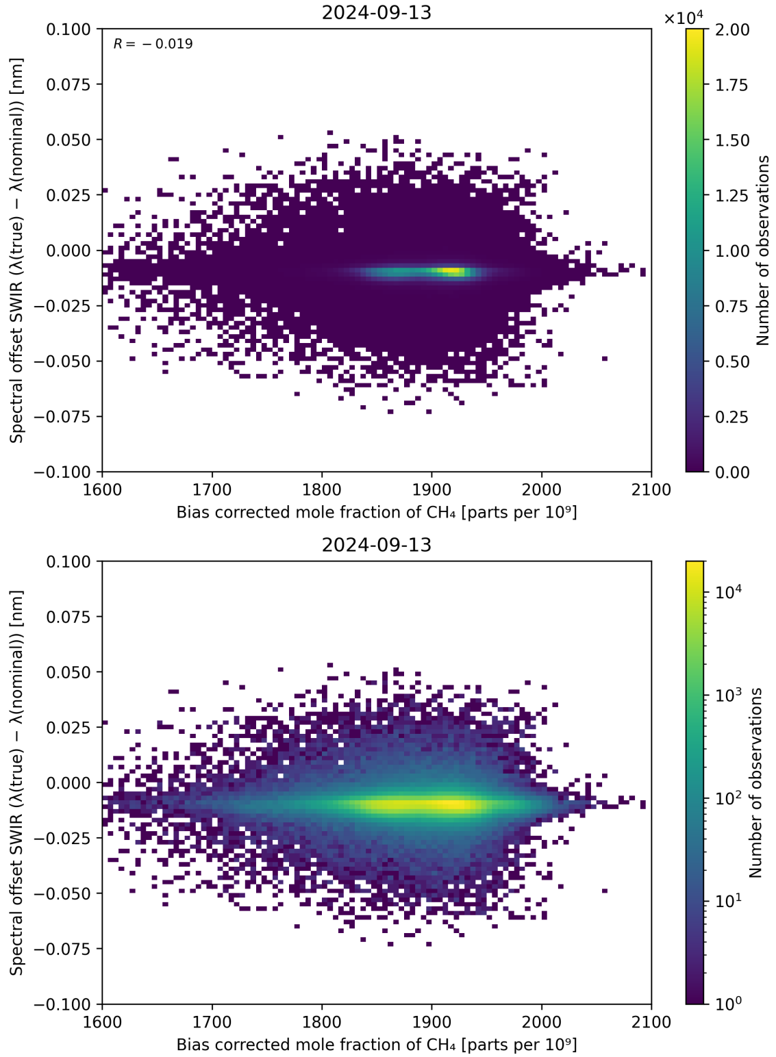
Figure 69: Scatter density plot of “Bias corrected mole fraction of \text{CH}_4 ” against “Spectral offset SWIR ( \lambda_{\text{true}} - \lambda_{\text{nominal}} )” for 2024-09-12 to 2024-09-14.
