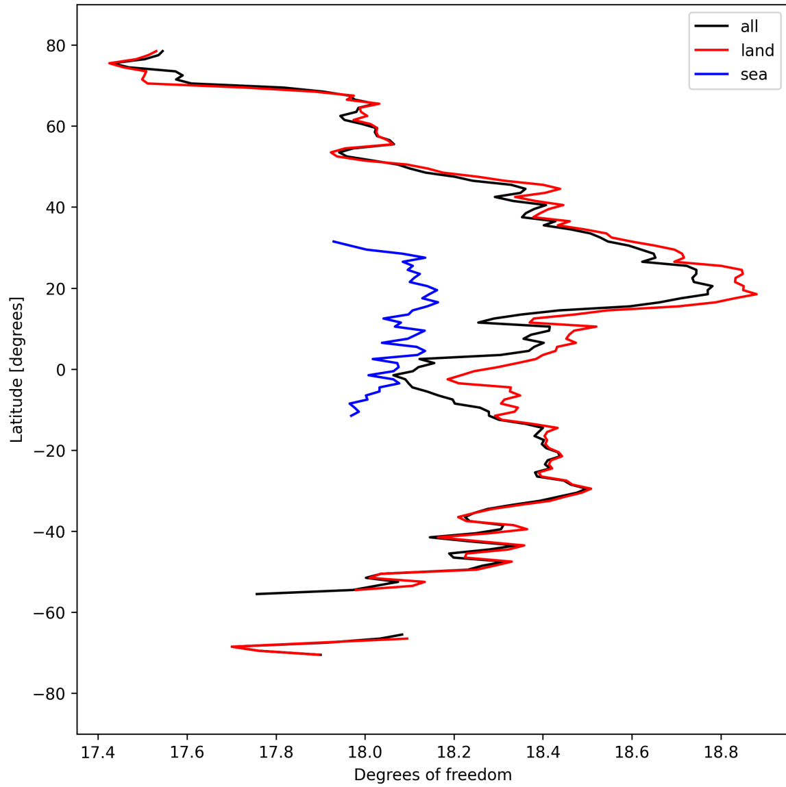
Figure 19: Zonal average of “Degrees of freedom” for 2024-09-12 to 2024-09-14.
