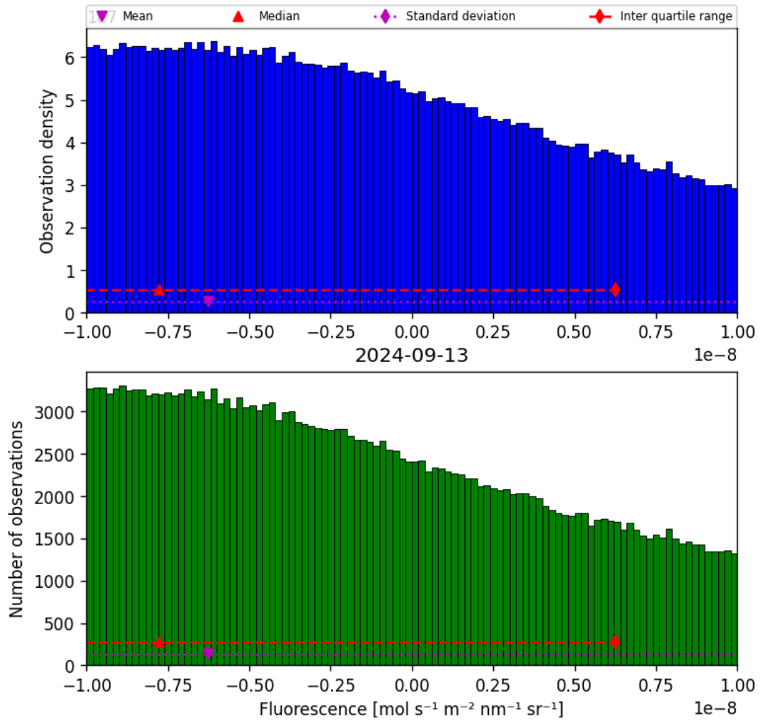
Figure 32: Histogram of “Fluorescence” for 2024-09-12 to 2024-09-14
