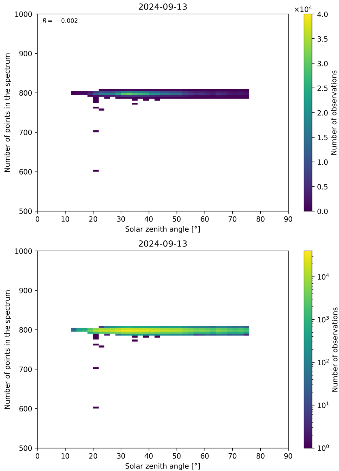
Figure 103: Scatter density plot of “Solar zenith angle” against “Number of points in the spectrum” for 2024-09-12 to 2024-09-14.
