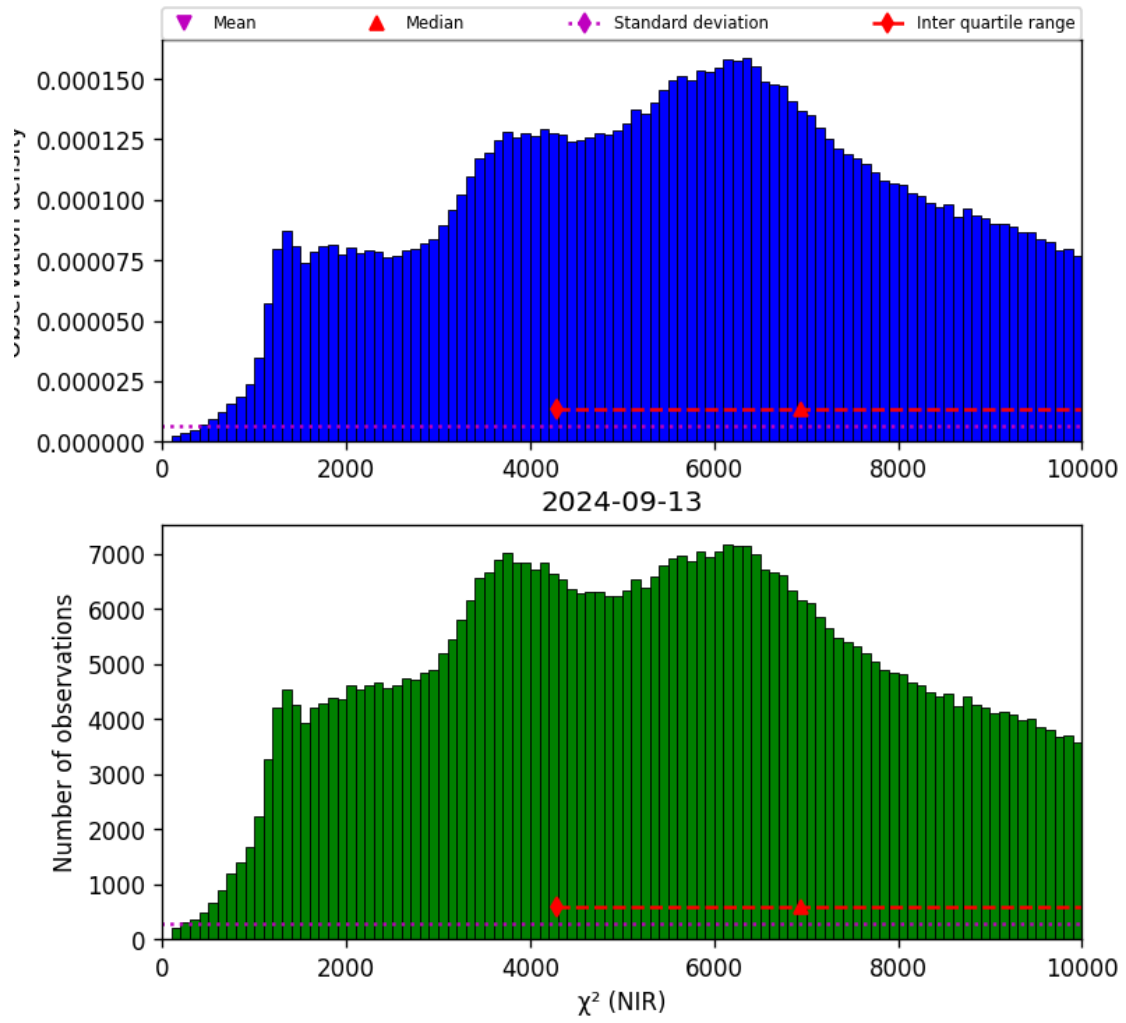
Figure 29: Histogram of “ \chi^2 (NIR)” for 2024-09-12 to 2024-09-14
