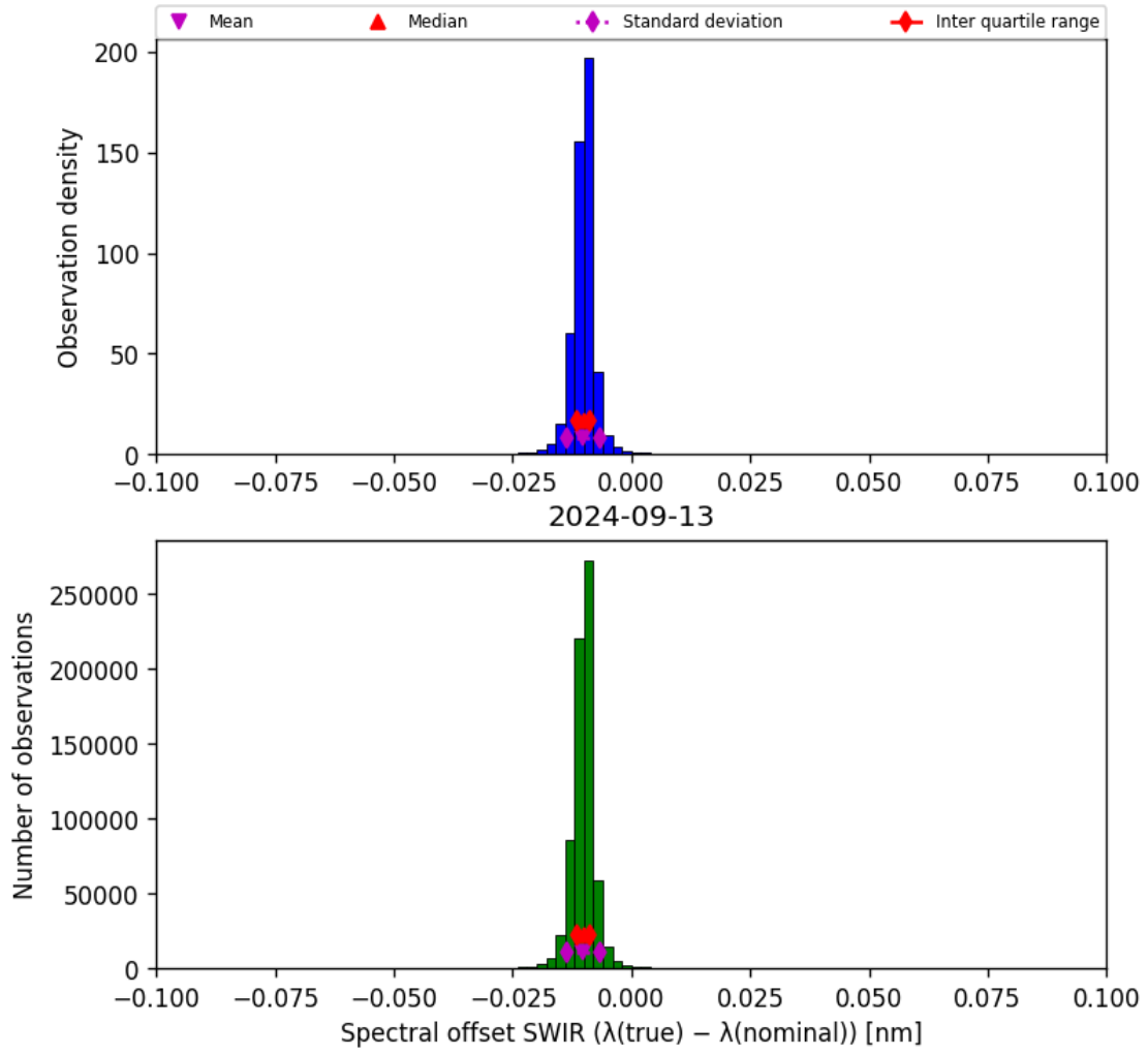
Figure 27: Histogram of “Spectral offset SWIR ( \lambda_{\text{true}} - \lambda_{\text{nominal}} )” for 2024-09-12 to 2024-09-14
