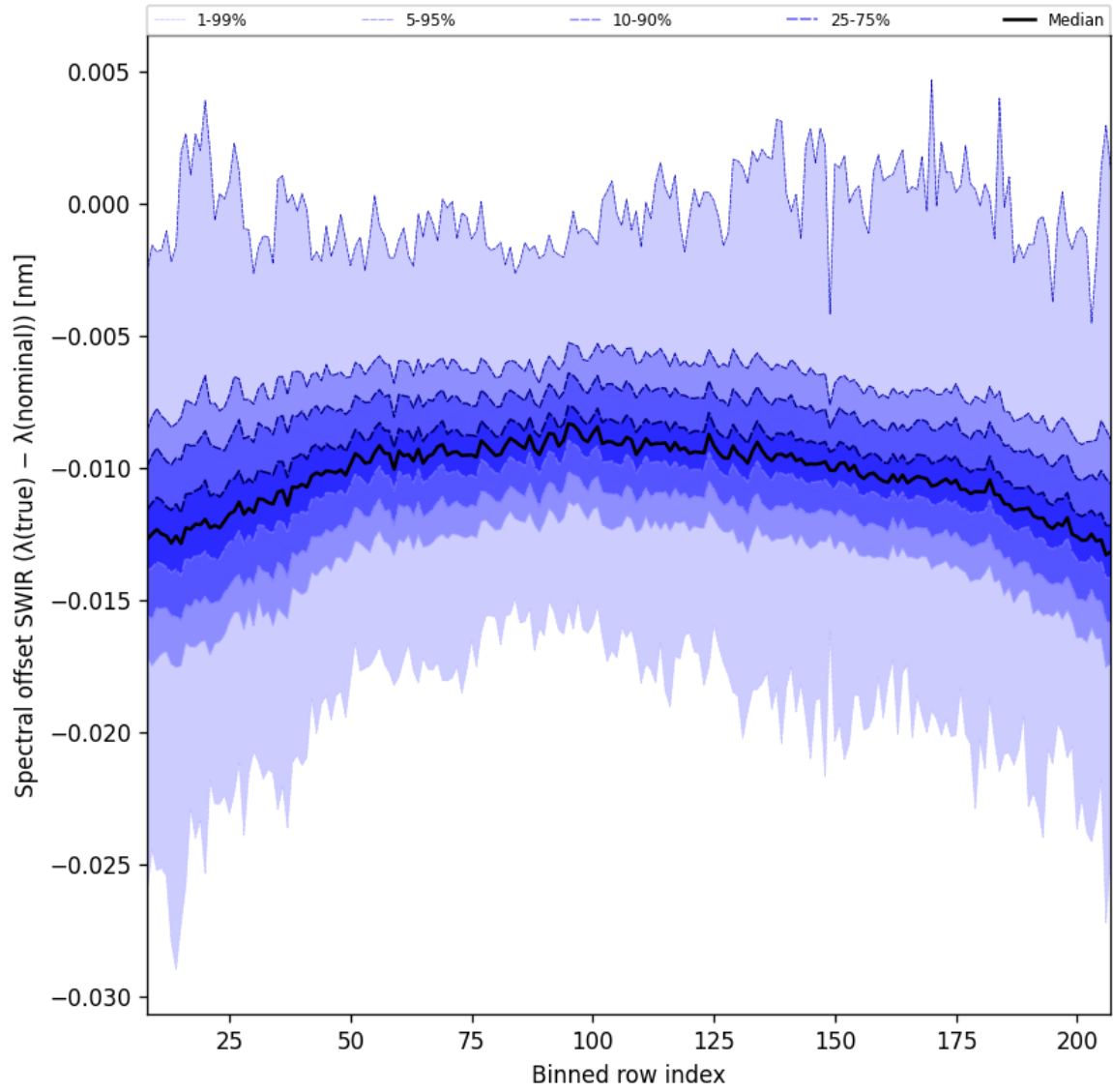
Figure 38: Along track statistics of “Spectral offset SWIR ( \lambda_{\text{true}} - \lambda_{\text{nominal}} )” for 2024-09-12 to 2024-09-14
