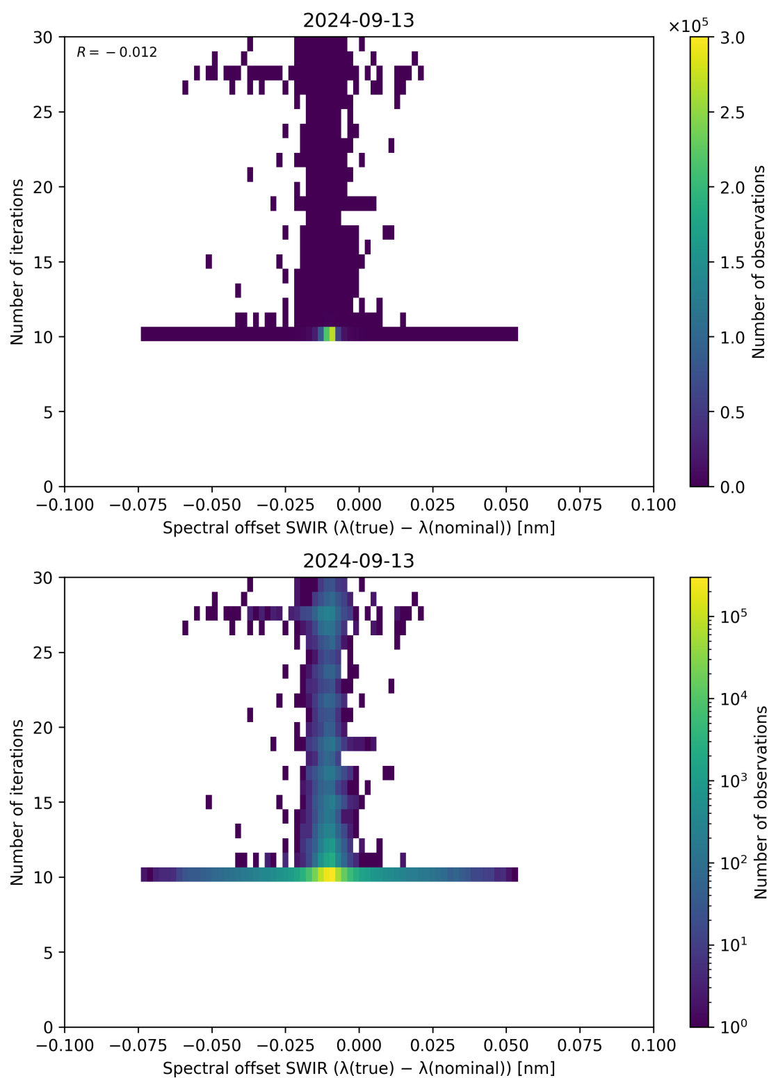
Figure 121: Scatter density plot of “Spectral offset SWIR ( \lambda_{\text{true}} - \lambda_{\text{nominal}} )” against “Number of iterations” for 2024-09-12 to 2024-09-14.
