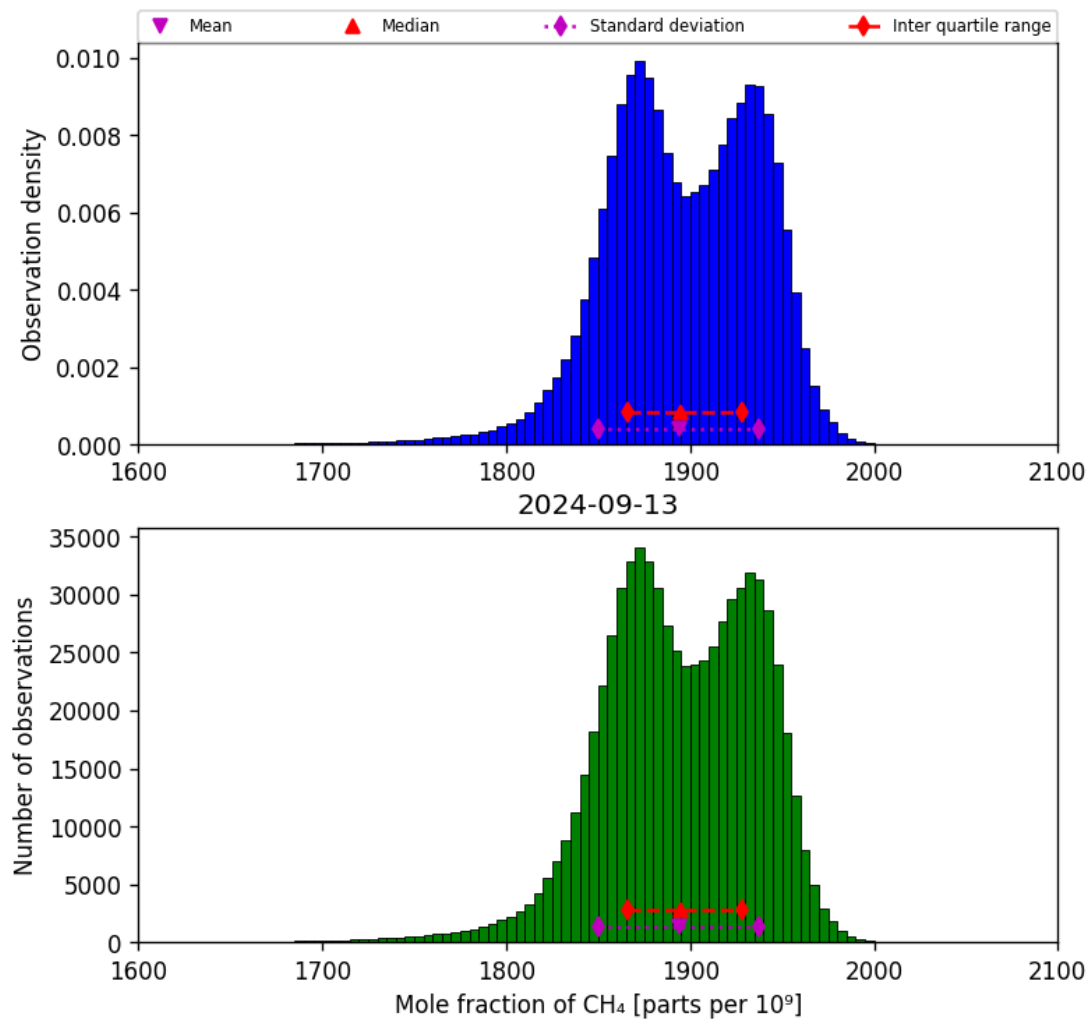
Figure 23: Histogram of “Mole fraction of CH 4 ” for 2024-09-12 to 2024-09-14
