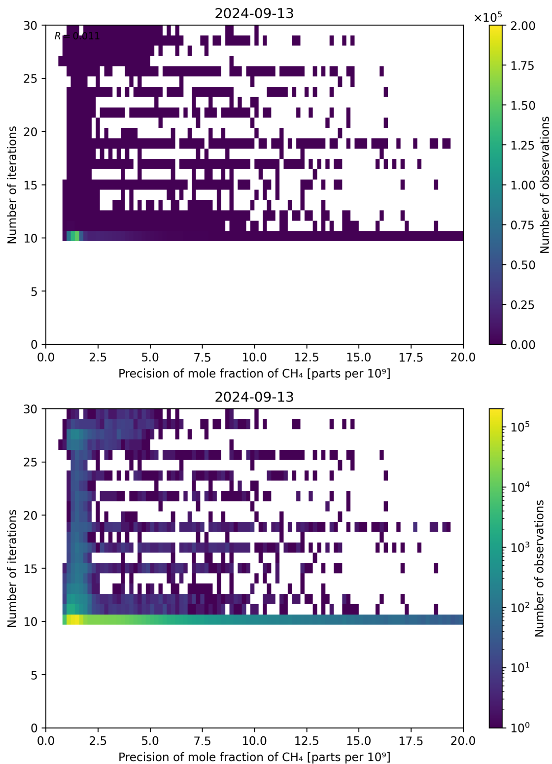
Figure 83: Scatter density plot of “Precision of mole fraction of CH 4 ” against “Number of iterations” for 2024-09-12 to 2024-09-14.
