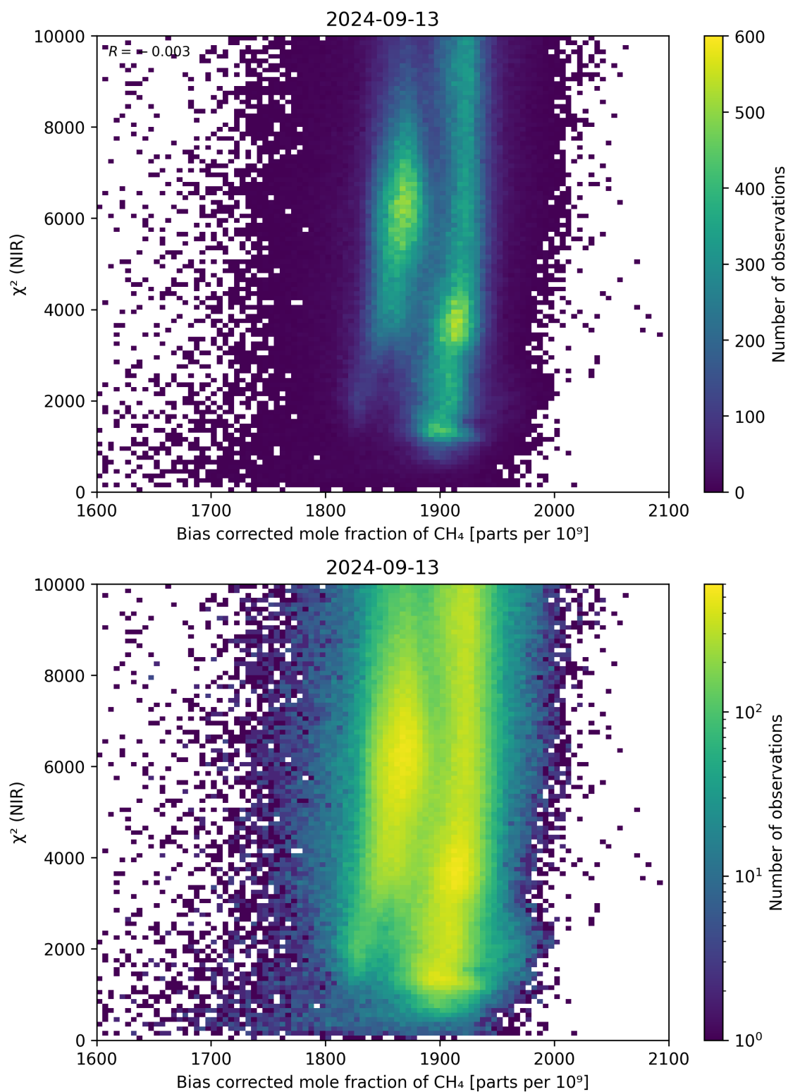
Figure 63: Scatter density plot of “Bias corrected mole fraction of \text{CH}_4 ” against “ \chi^2 (NIR)” for 2024-09-12 to 2024-09-14.
