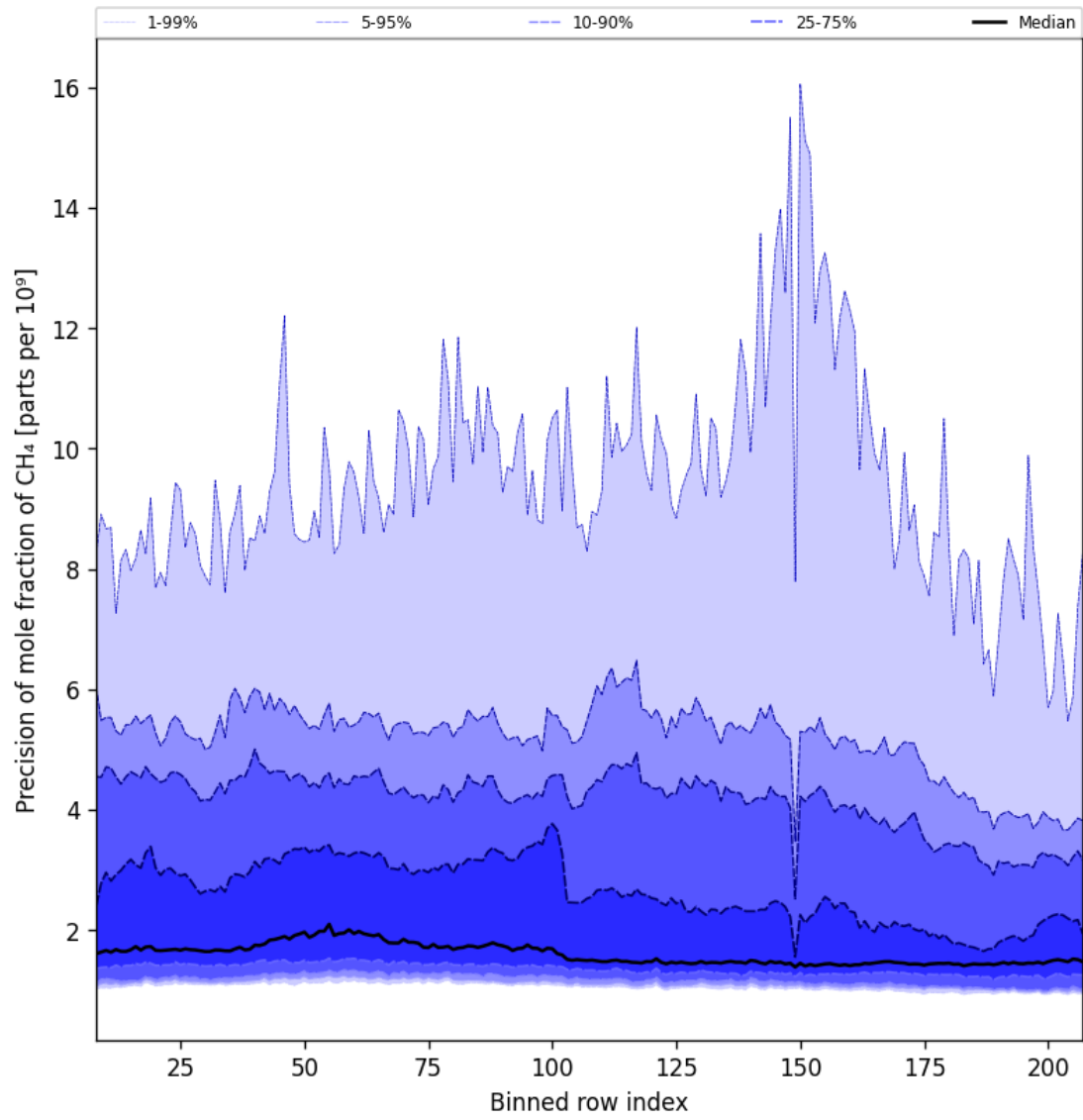
Figure 35: Along track statistics of “Precision of mole fraction of CH 4 ” for 2024-09-12 to 2024-09-14
