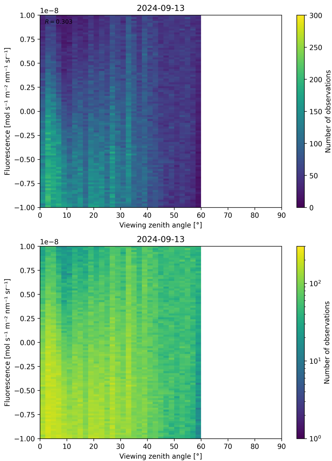
Figure 108: Scatter density plot of “Viewing zenith angle” against “Fluorescence” for 2024-09-12 to 2024-09-14.
