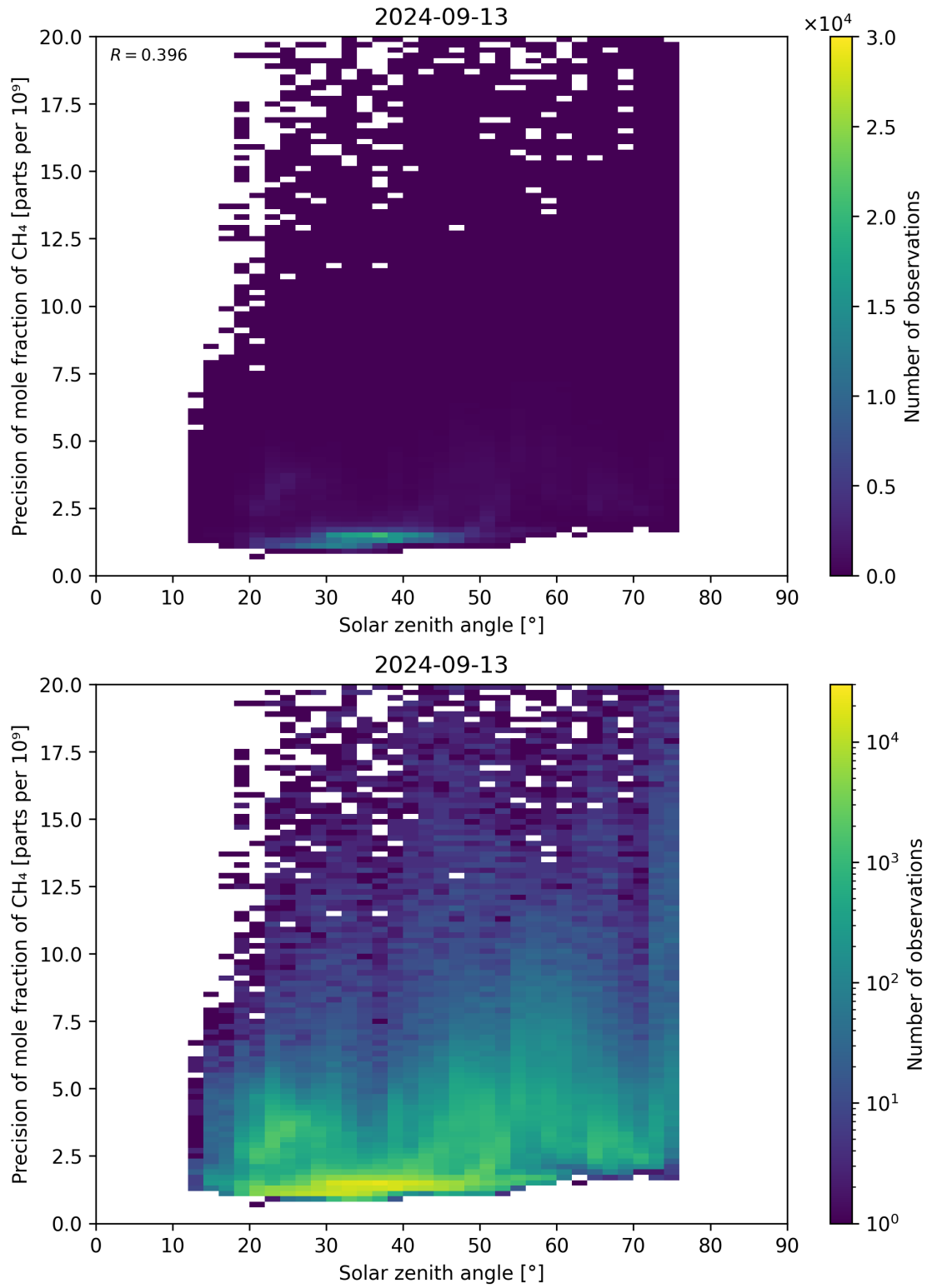
Figure 101: Scatter density plot of “Solar zenith angle” against “Precision of mole fraction of CH 4 ” for 2024-09-12 to 2024-09-14.
