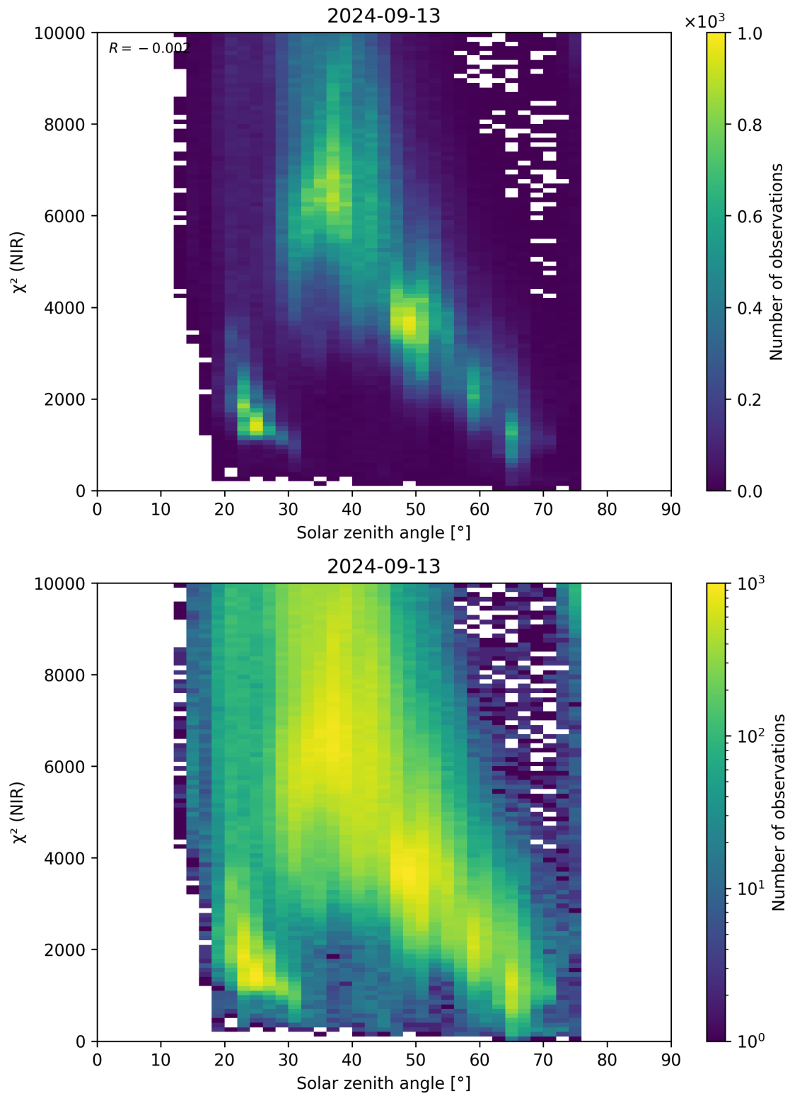
Figure 94: Scatter density plot of “Solar zenith angle” against “ \chi^2 (NIR)” for 2024-09-12 to 2024-09-14.
