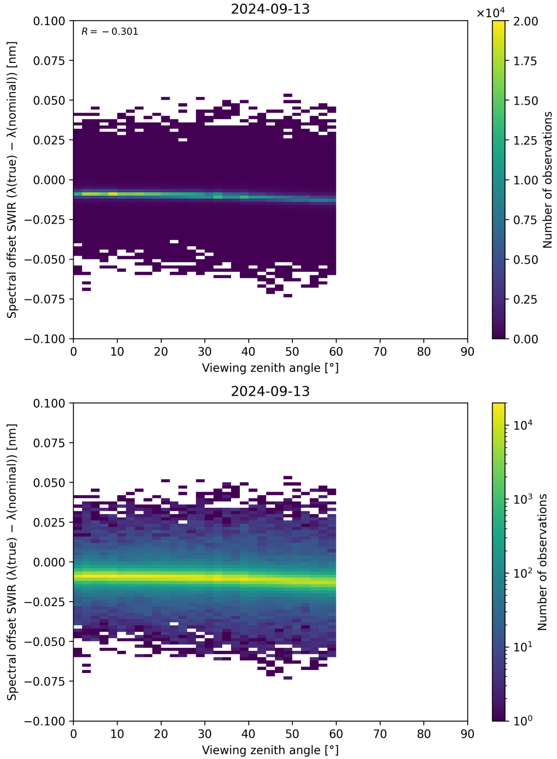
Figure 116: Scatter density plot of “Viewing zenith angle” against “Spectral offset SWIR ( \lambda_{\text{true}} - \lambda_{\text{nominal}} )” for 2024-09-12 to 2024-09-14.
