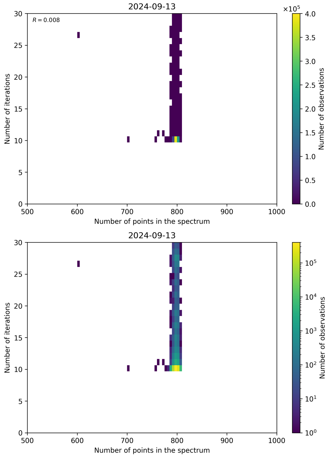
Figure 92: Scatter density plot of “Number of points in the spectrum” against “Number of iterations” for 2024-09-12 to 2024-09-14.
