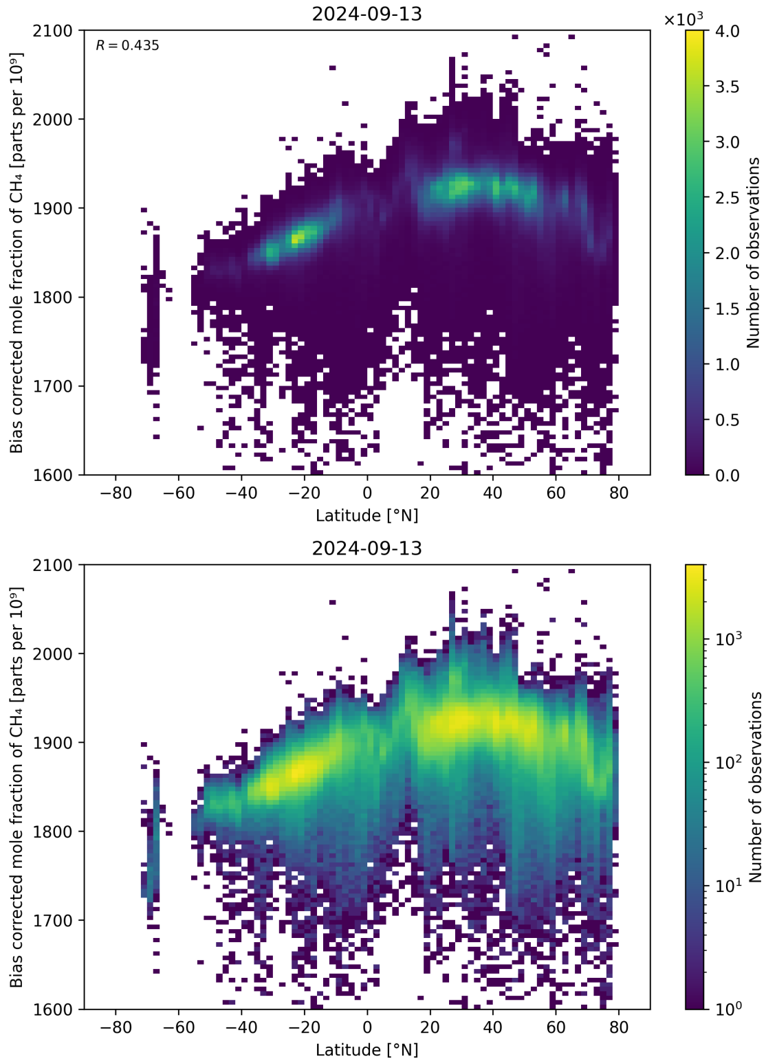
Figure 58: Scatter density plot of “Latitude” against “Bias corrected mole fraction of \text{CH}_4 ” for 2024-09-12 to 2024-09-14.
