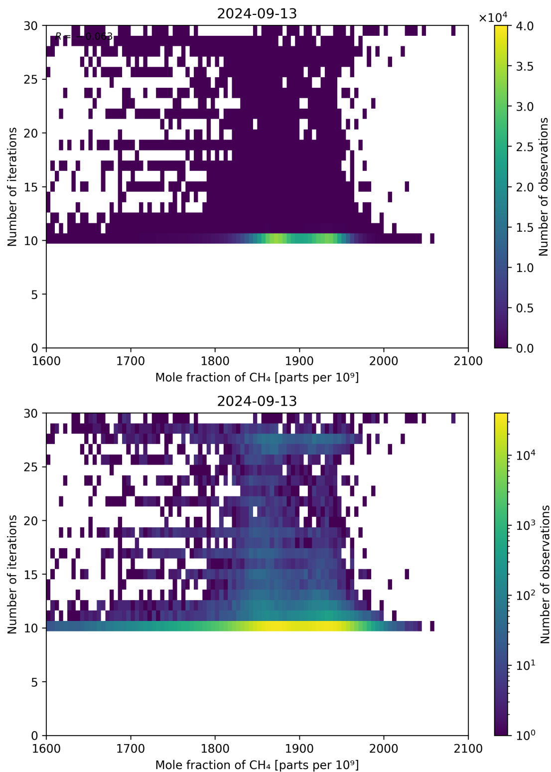
Figure 76: Scatter density plot of “Mole fraction of CH 4 ” against “Number of iterations” for 2024-09-12 to 2024-09-14.
