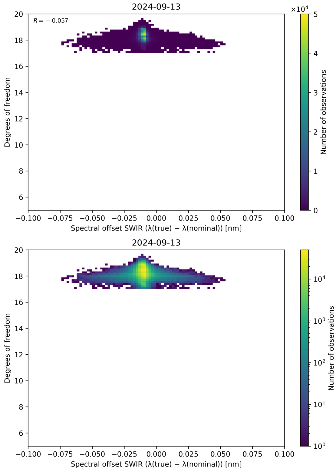
Figure 119: Scatter density plot of “Spectral offset SWIR ( \lambda_{\text{true}} - \lambda_{\text{nominal}} )” against “Degrees of freedom” for 2024-09-12 to 2024-09-14.
