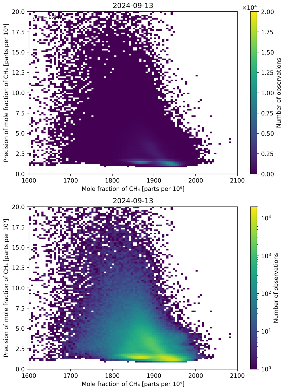
Figure 75: Scatter density plot of “Mole fraction of CH 4 ” against “Precision of mole fraction of CH 4 ” for 2024-09-12 to 2024-09-14.
