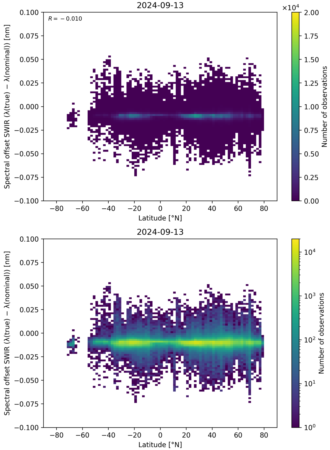
Figure 62: Scatter density plot of “Latitude” against “Spectral offset SWIR ( \lambda_{\text{true}} - \lambda_{\text{nominal}} )” for 2024-09-12 to 2024-09-14.
