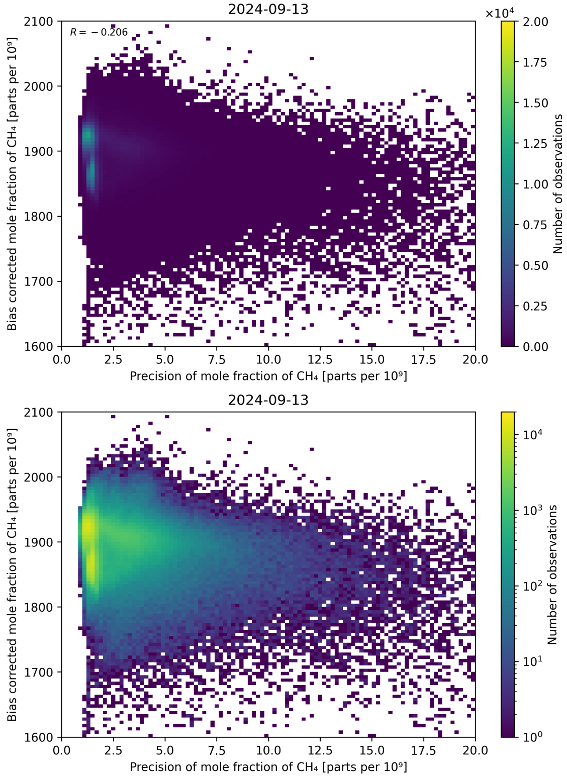
Figure 82: Scatter density plot of “Precision of mole fraction of \text{CH}_4 ” against “Bias corrected mole fraction of \text{CH}_4 ” for 2024-09-12 to 2024-09-14.
