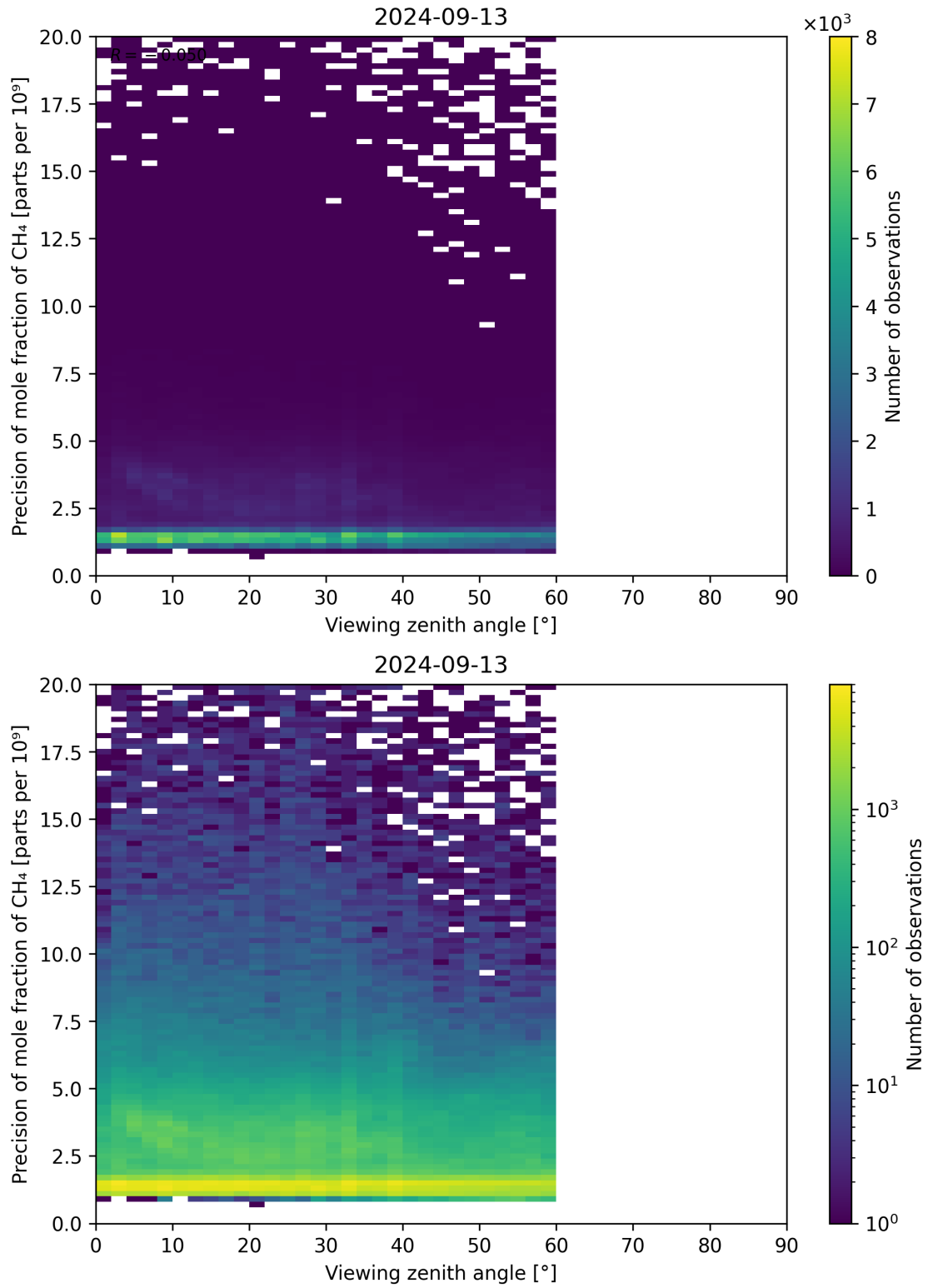
Figure 112: Scatter density plot of “Viewing zenith angle” against “Precision of mole fraction of CH 4 ” for 2024-09-12 to 2024-09-14.
