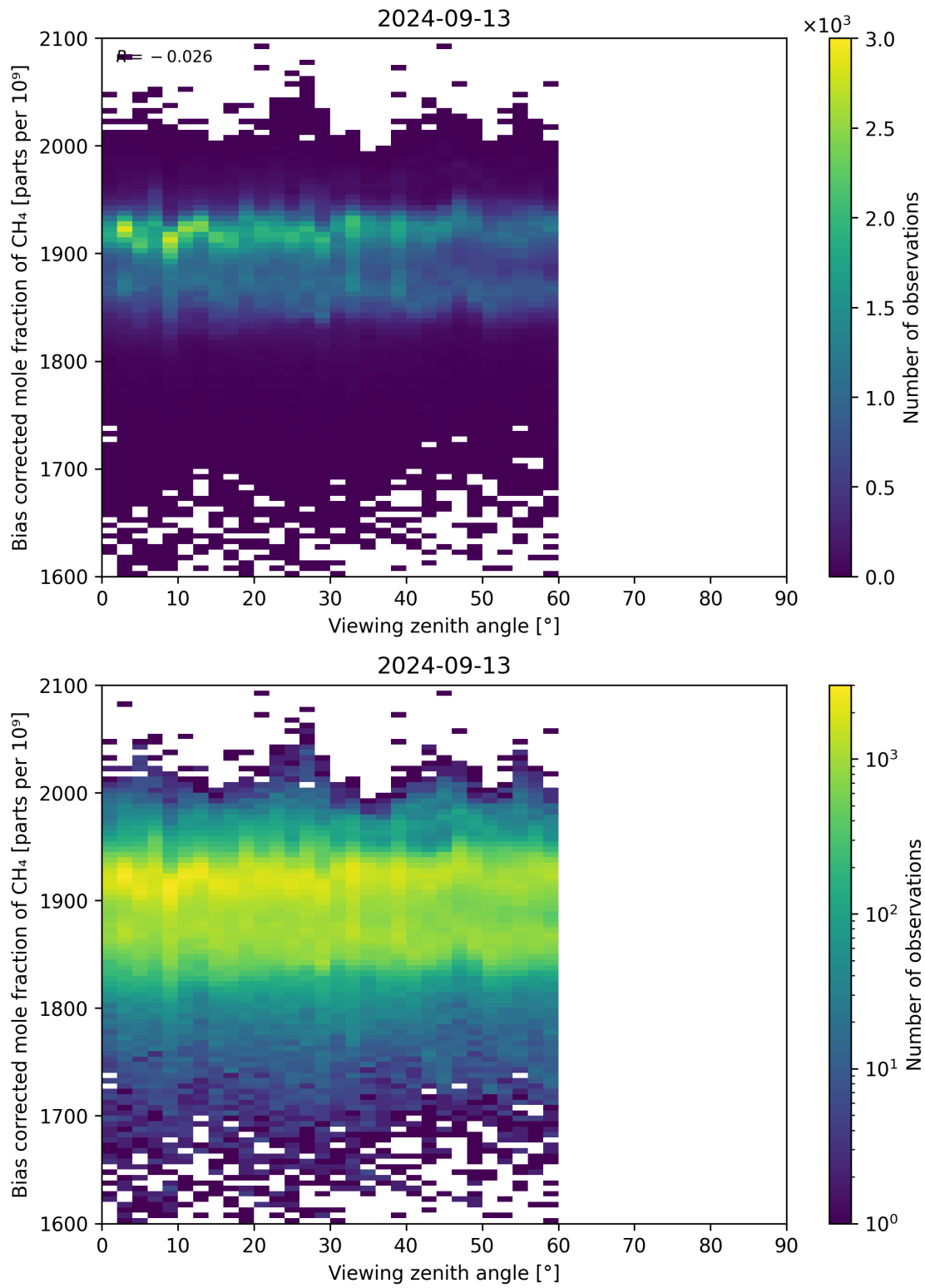
Figure 111: Scatter density plot of “Viewing zenith angle” against “Bias corrected mole fraction of CH 4 ” for 2024-09-12 to 2024-09-14.
