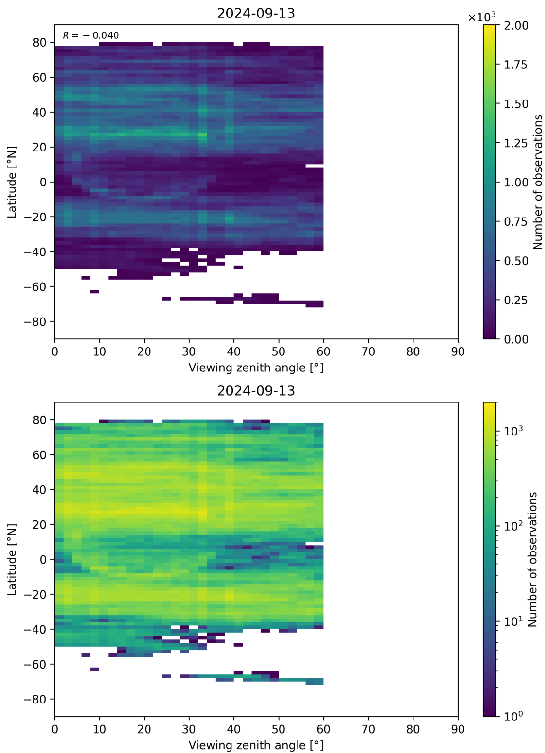
Figure 109: Scatter density plot of “Viewing zenith angle” against “Latitude” for 2024-09-12 to 2024-09-14.
