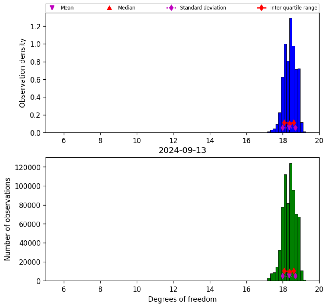
Figure 30: Histogram of “Degrees of freedom” for 2024-09-12 to 2024-09-14
