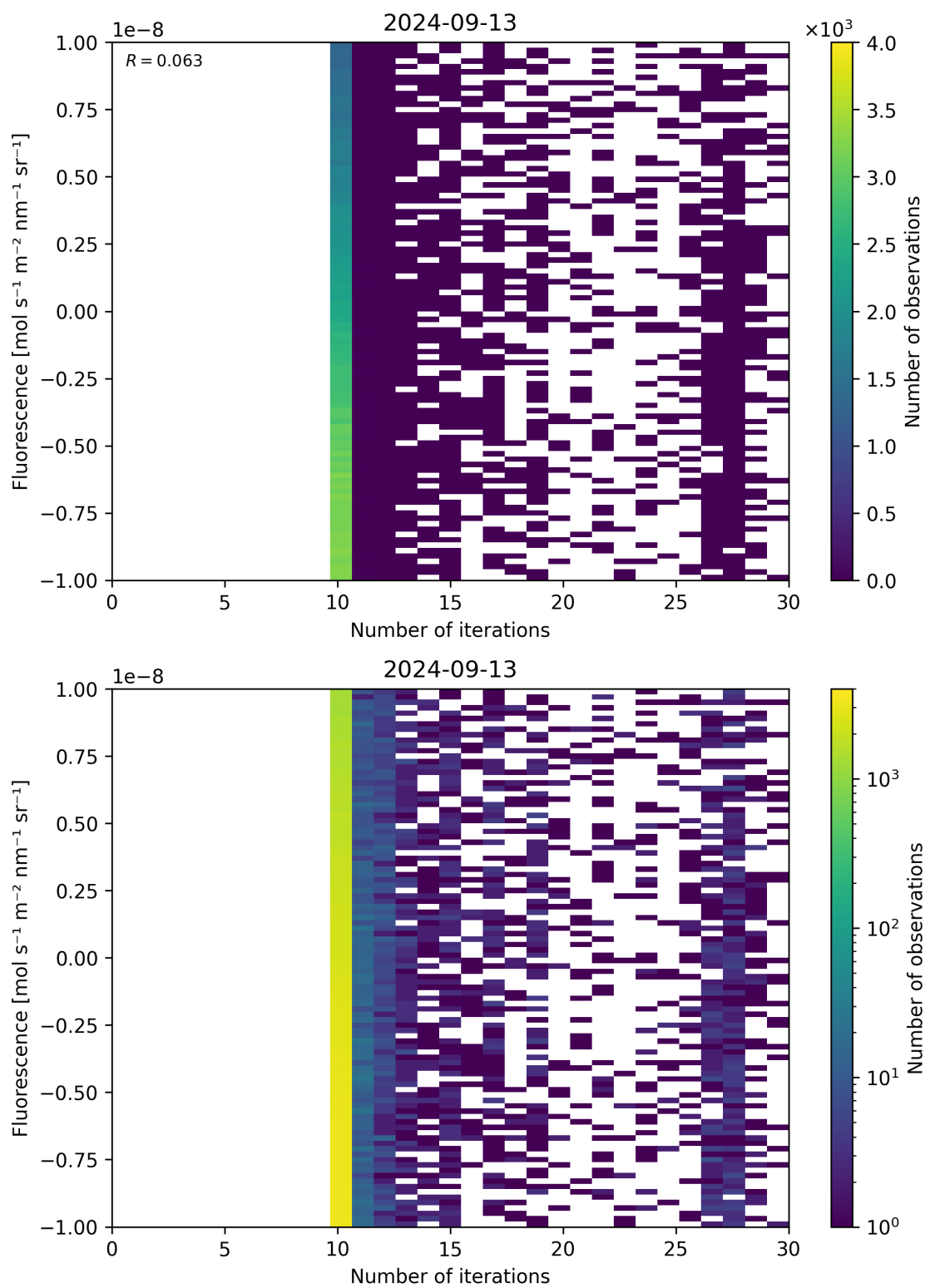
Figure 87: Scatter density plot of “Number of iterations” against “Fluorescence” for 2024-09-12 to 2024-09-14.
