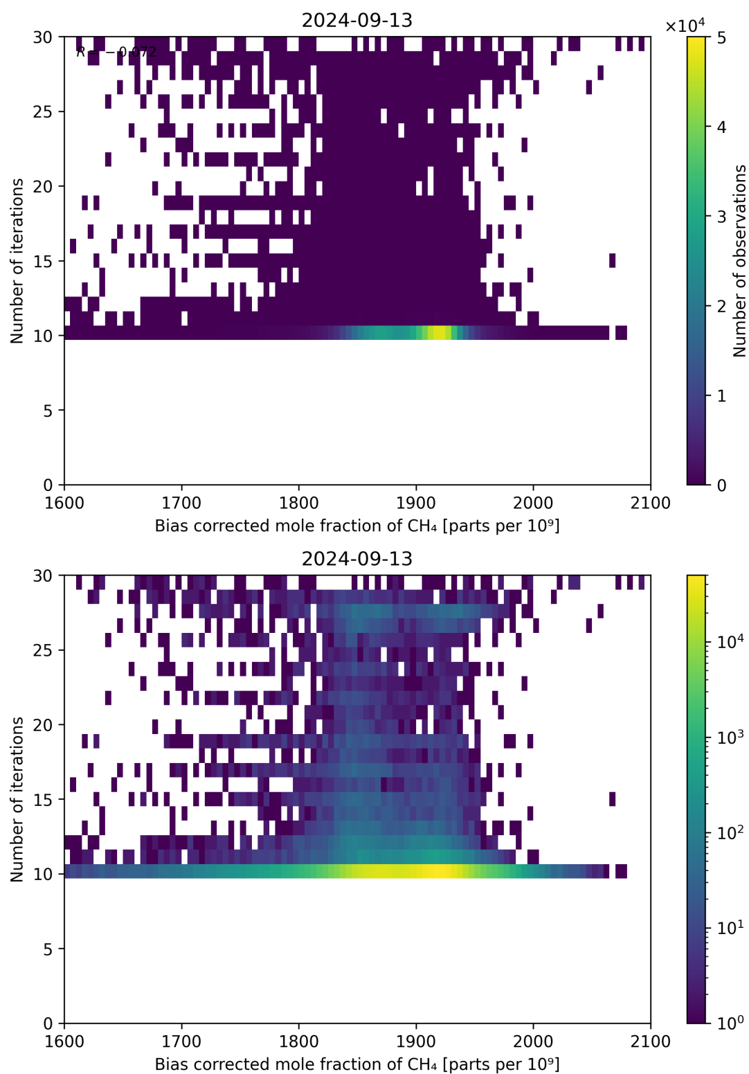
Figure 67: Scatter density plot of “Bias corrected mole fraction of CH 4 ” against “Number of iterations” for 2024-09-12 to 2024-09-14.
