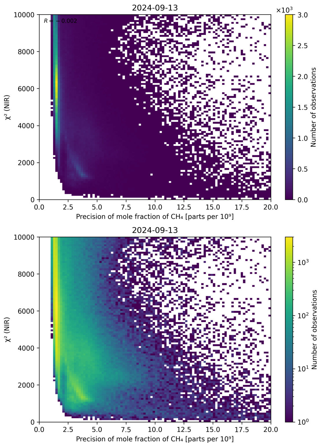
Figure 78: Scatter density plot of “Precision of mole fraction of CH 4 ” against “ \chi^2 (NIR)” for 2024-09-12 to 2024-09-14.
