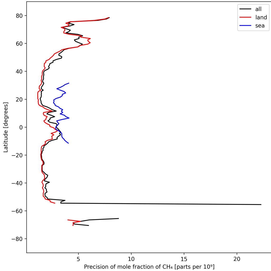
Figure 13: Zonal average of “Precision of mole fraction of CH 4 ” for 2024-09-12 to 2024-09-14.
