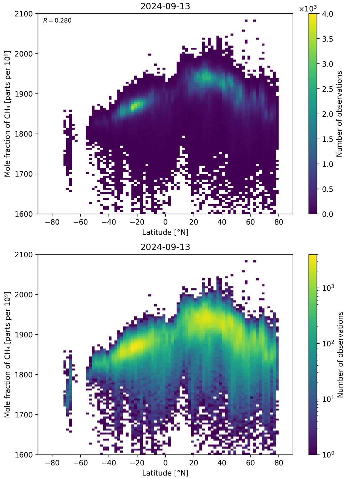
Figure 57: Scatter density plot of “Latitude” against “Mole fraction of CH 4 ” for 2024-09-12 to 2024-09-14.
