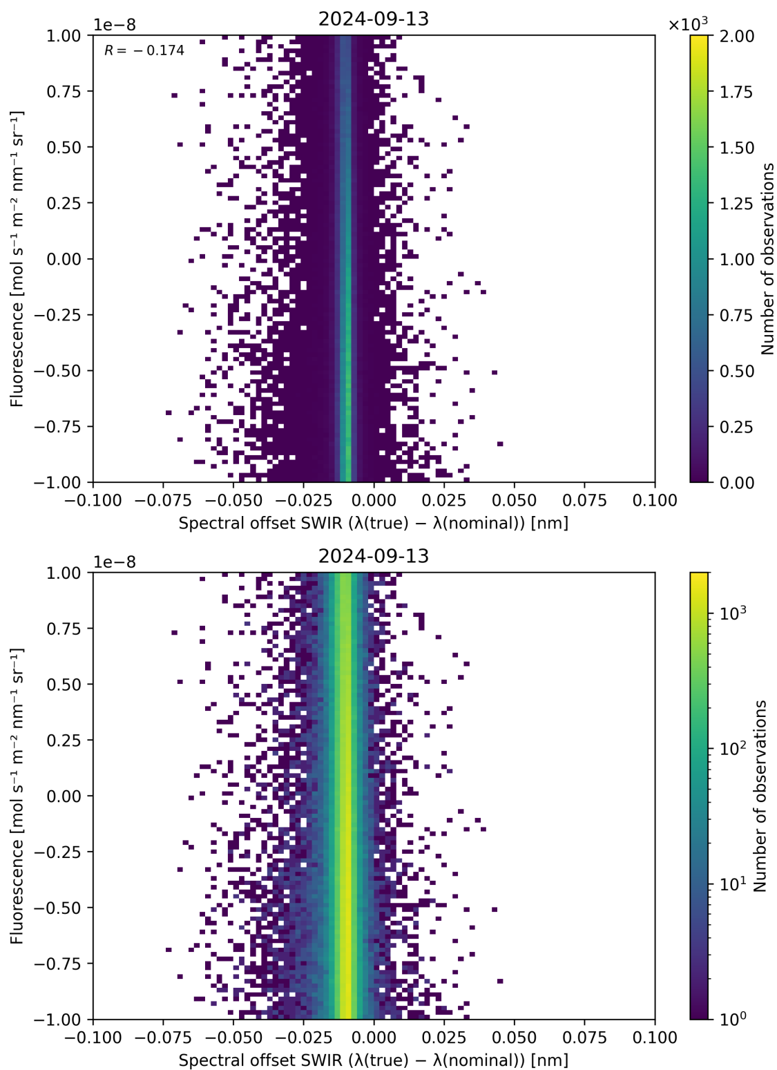
Figure 120: Scatter density plot of “Spectral offset SWIR ( \lambda_{\text{true}} - \lambda_{\text{nominal}} )” against “Fluorescence” for 2024-09-12 to 2024-09-14.
