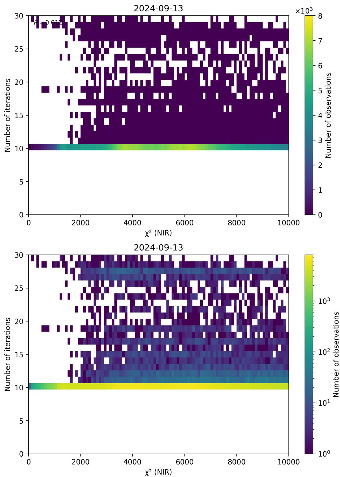
Figure 46: Scatter density plot of “ \chi^2 (NIR)” against “Number of iterations” for 2024-09-12 to 2024-09-14.
