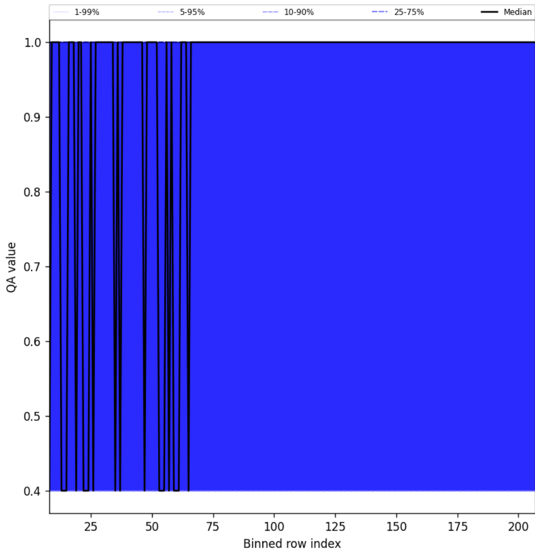
Figure 33: Along track statistics of “QA value” for 2024-09-12 to 2024-09-14
