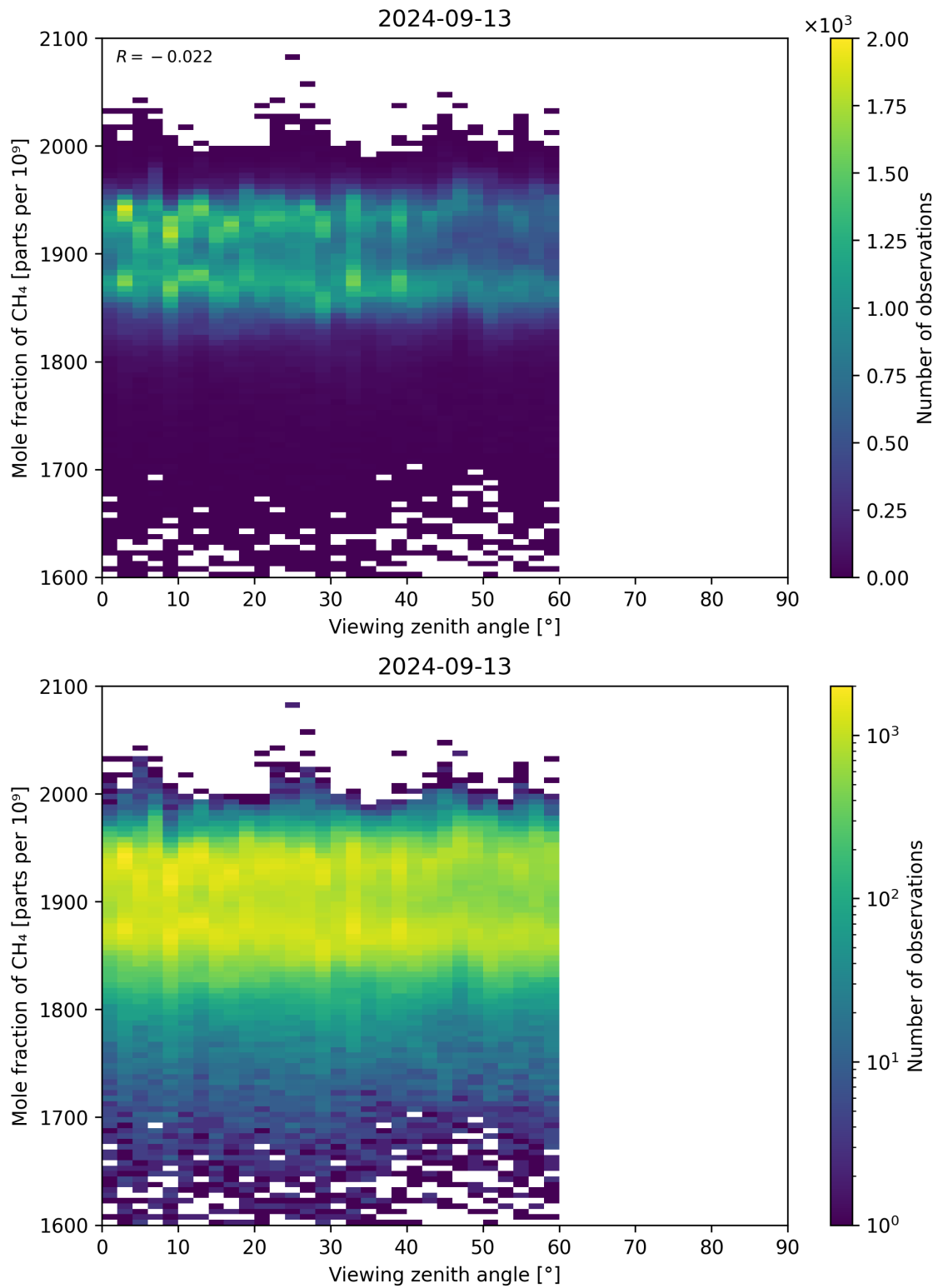
Figure 110: Scatter density plot of “Viewing zenith angle” against “Mole fraction of \text{CH}_4 ” for 2024-09-12 to 2024-09-14.
