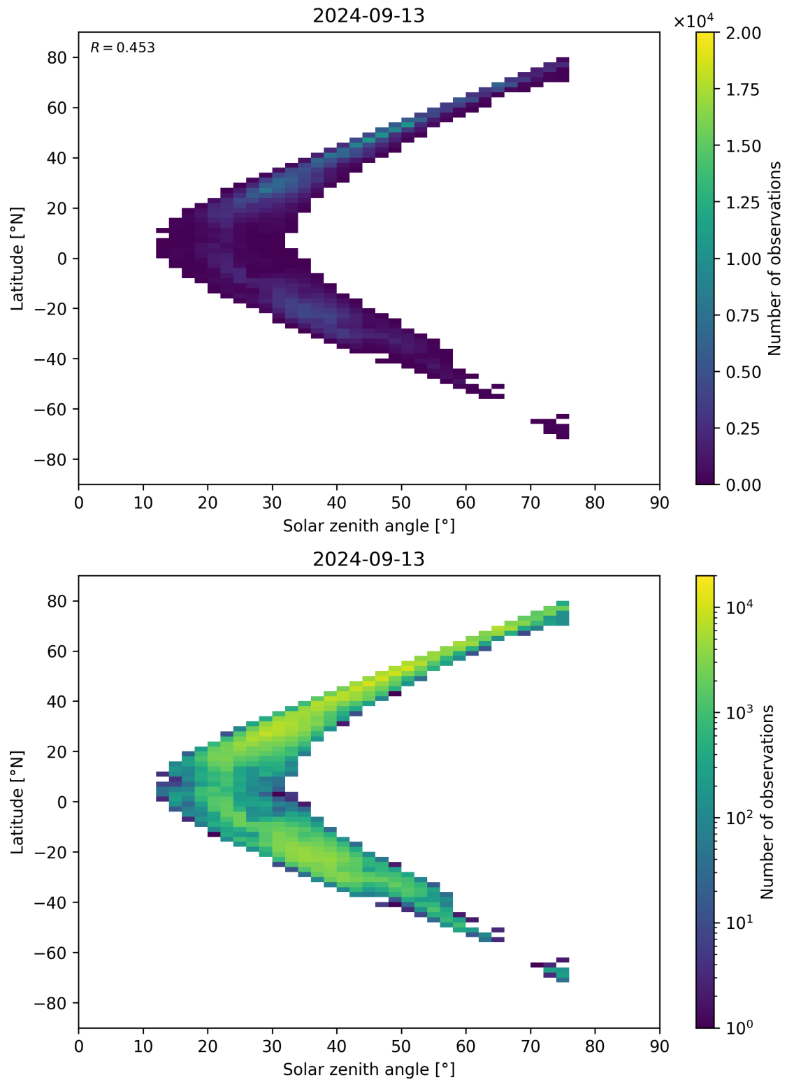
Figure 98: Scatter density plot of “Solar zenith angle” against “Latitude” for 2024-09-12 to 2024-09-14.
