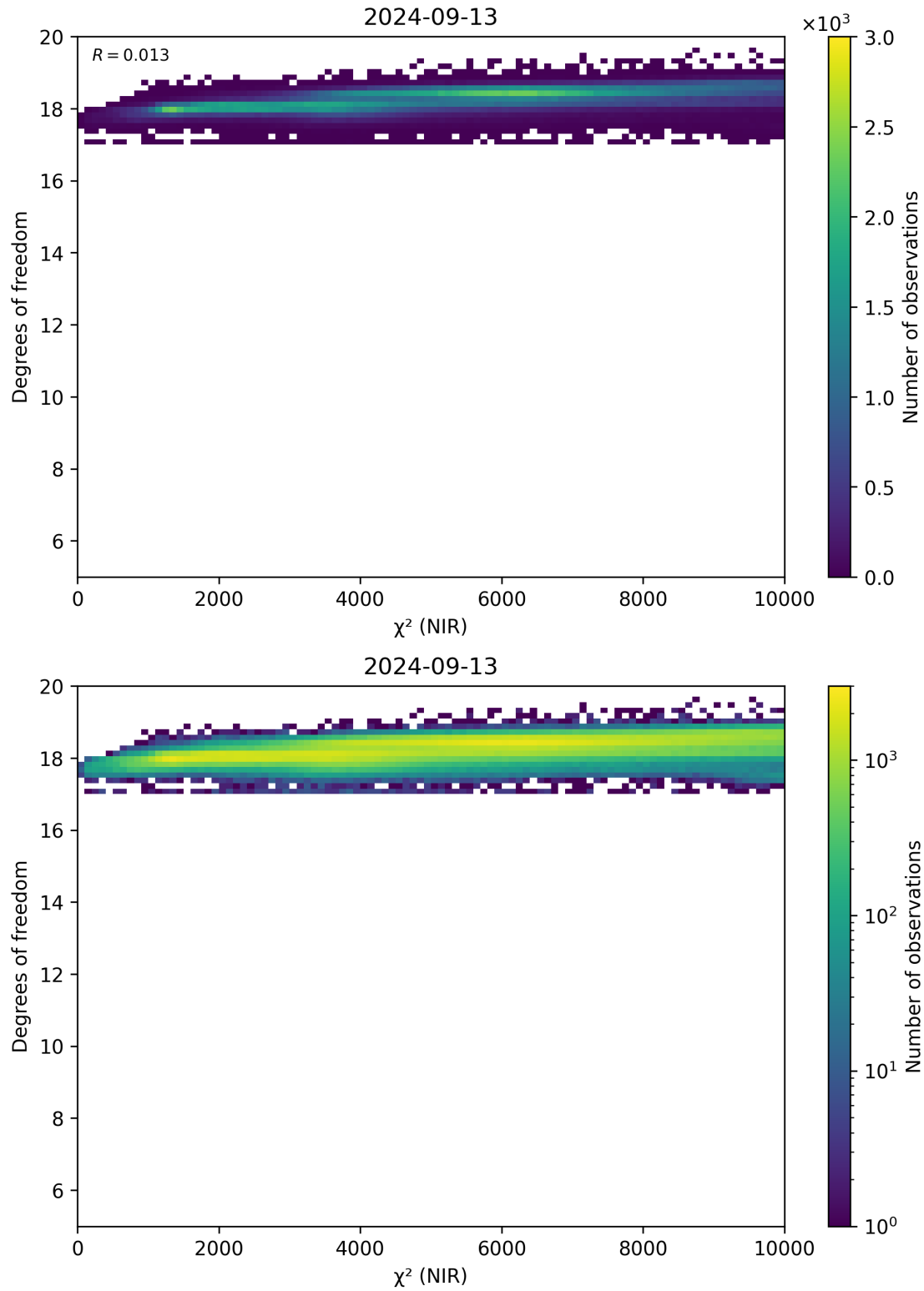
Figure 44: Scatter density plot of “ \chi^2 (NIR)” against “Degrees of freedom” for 2024-09-12 to 2024-09-14.
