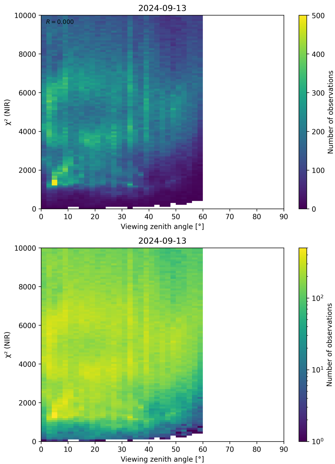
Figure 105: Scatter density plot of “Viewing zenith angle” against “ \chi^2 (NIR)” for 2024-09-12 to 2024-09-14.
