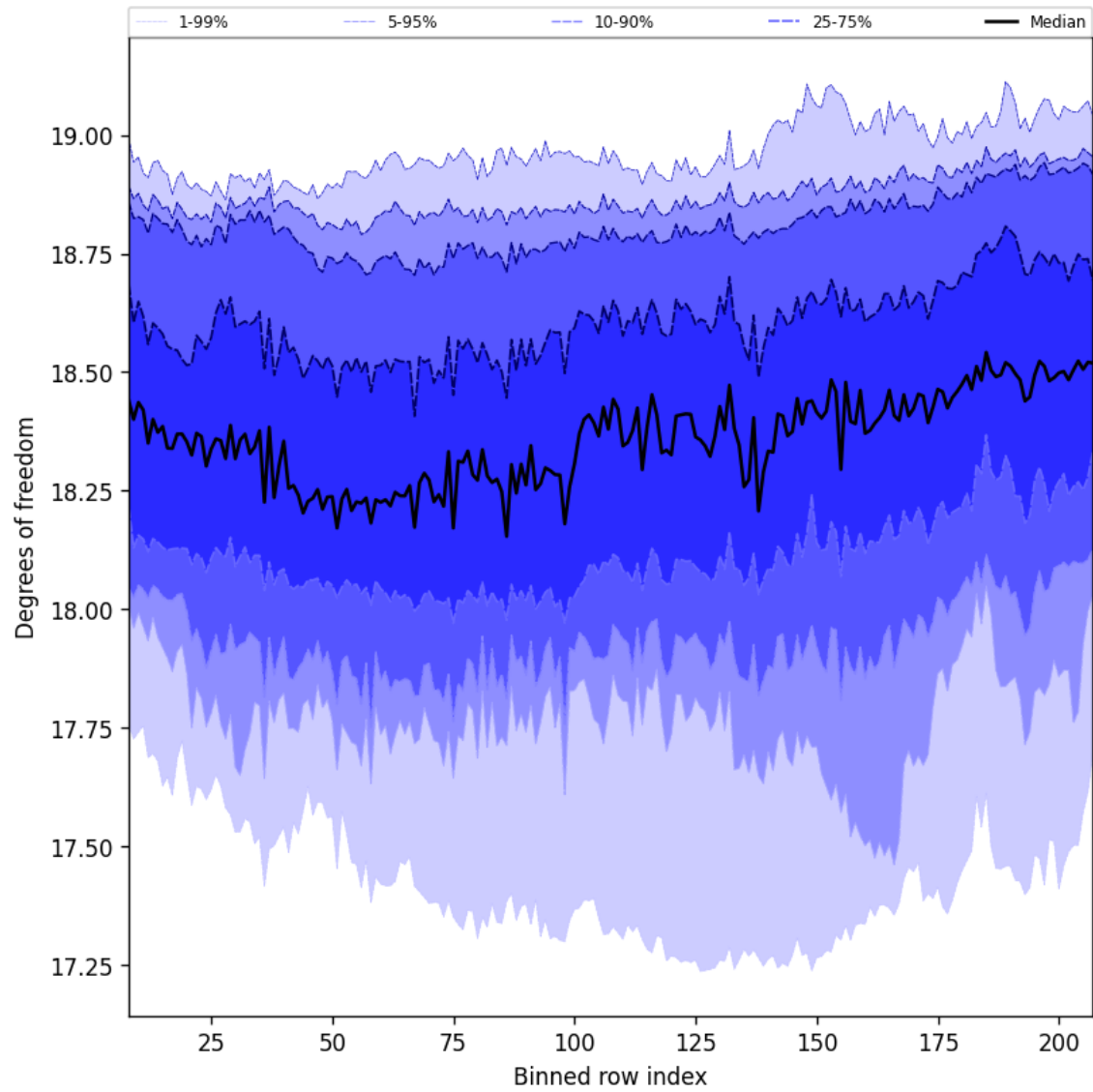
Figure 41: Along track statistics of “Degrees of freedom” for 2024-09-12 to 2024-09-14
