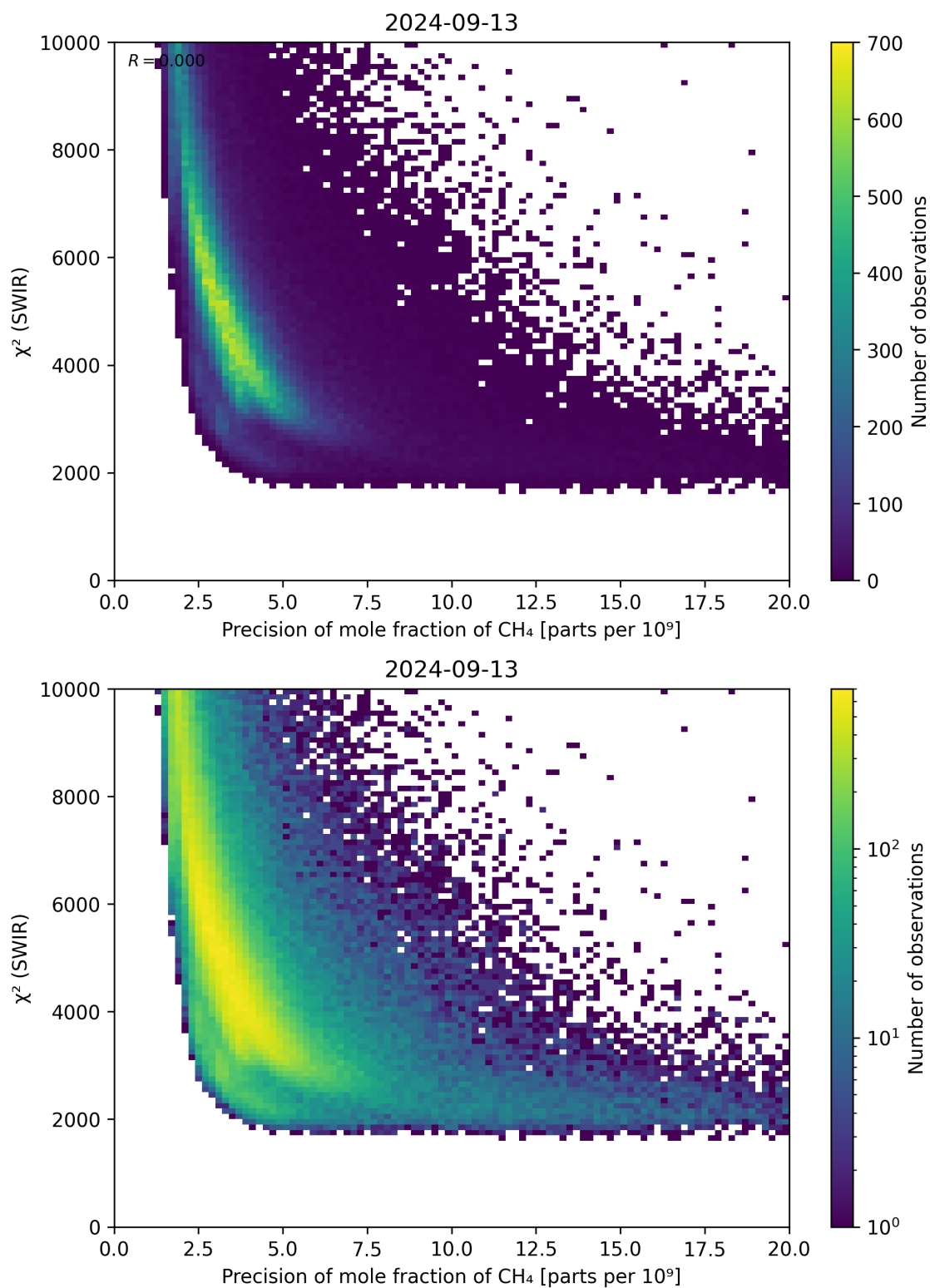
Figure 79: Scatter density plot of “Precision of mole fraction of CH 4 ” against “ \chi^2 (SWIR)” for 2024-09-12 to 2024-09-14.
