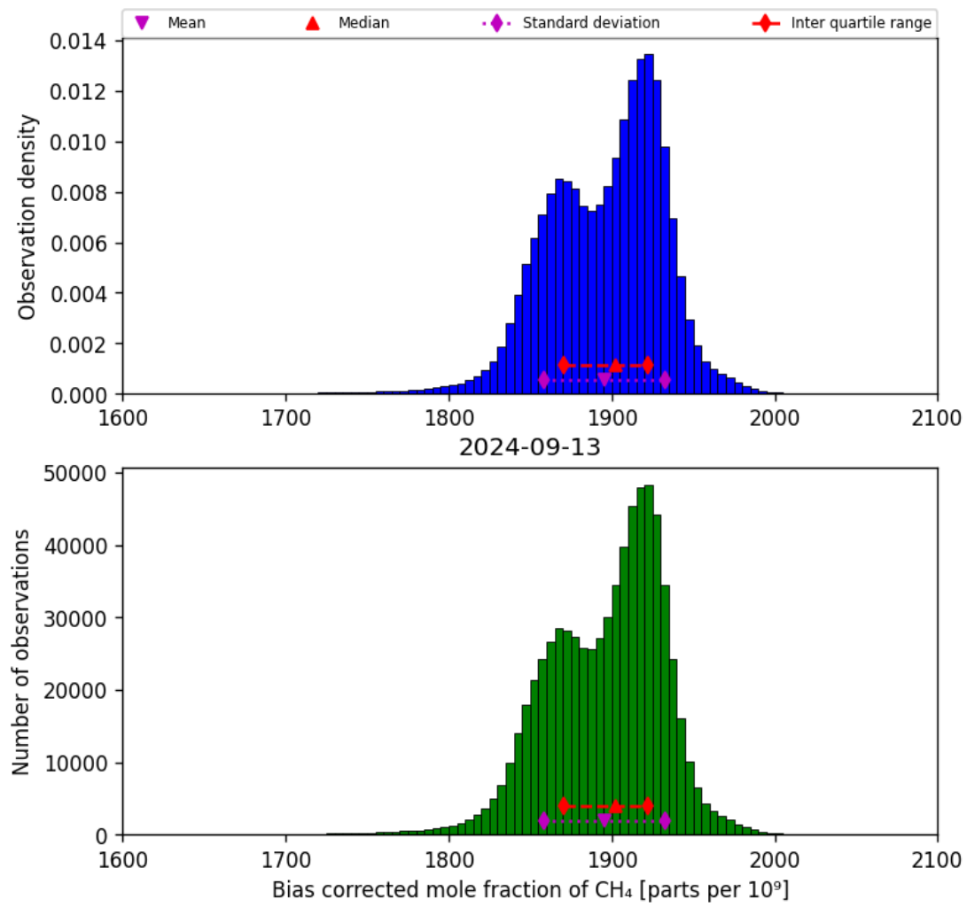
Figure 25: Histogram of “Bias corrected mole fraction of CH 4 ” for 2024-09-12 to 2024-09-14
