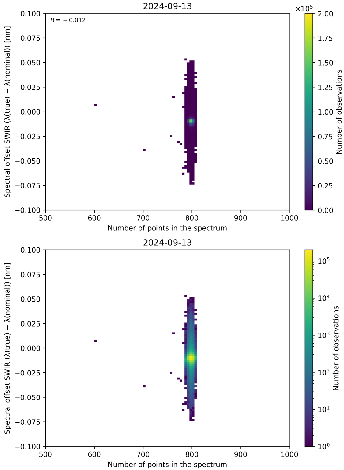
Figure 93: Scatter density plot of “Number of points in the spectrum” against “Spectral offset SWIR ( \lambda_{\text{true}} - \lambda_{\text{nominal}} )” for 2024-09-12 to 2024-09-14.
