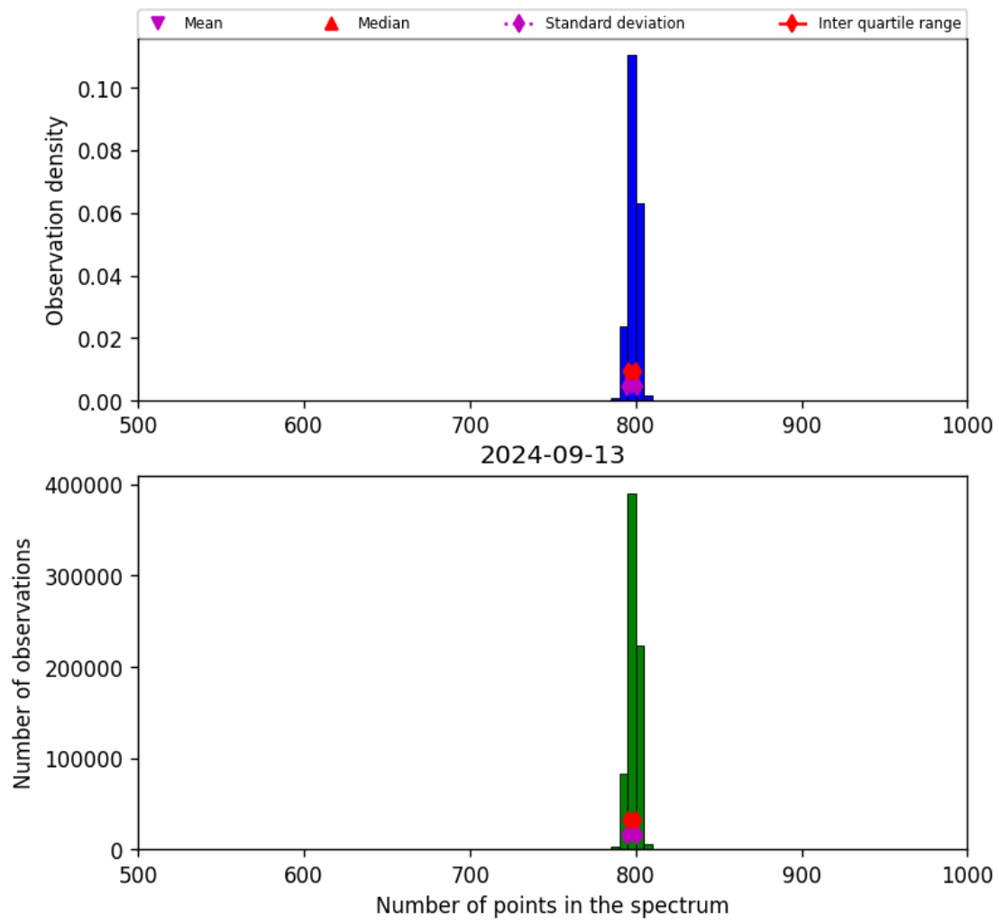
Figure 26: Histogram of “Number of points in the spectrum” for 2024-09-12 to 2024-09-14
