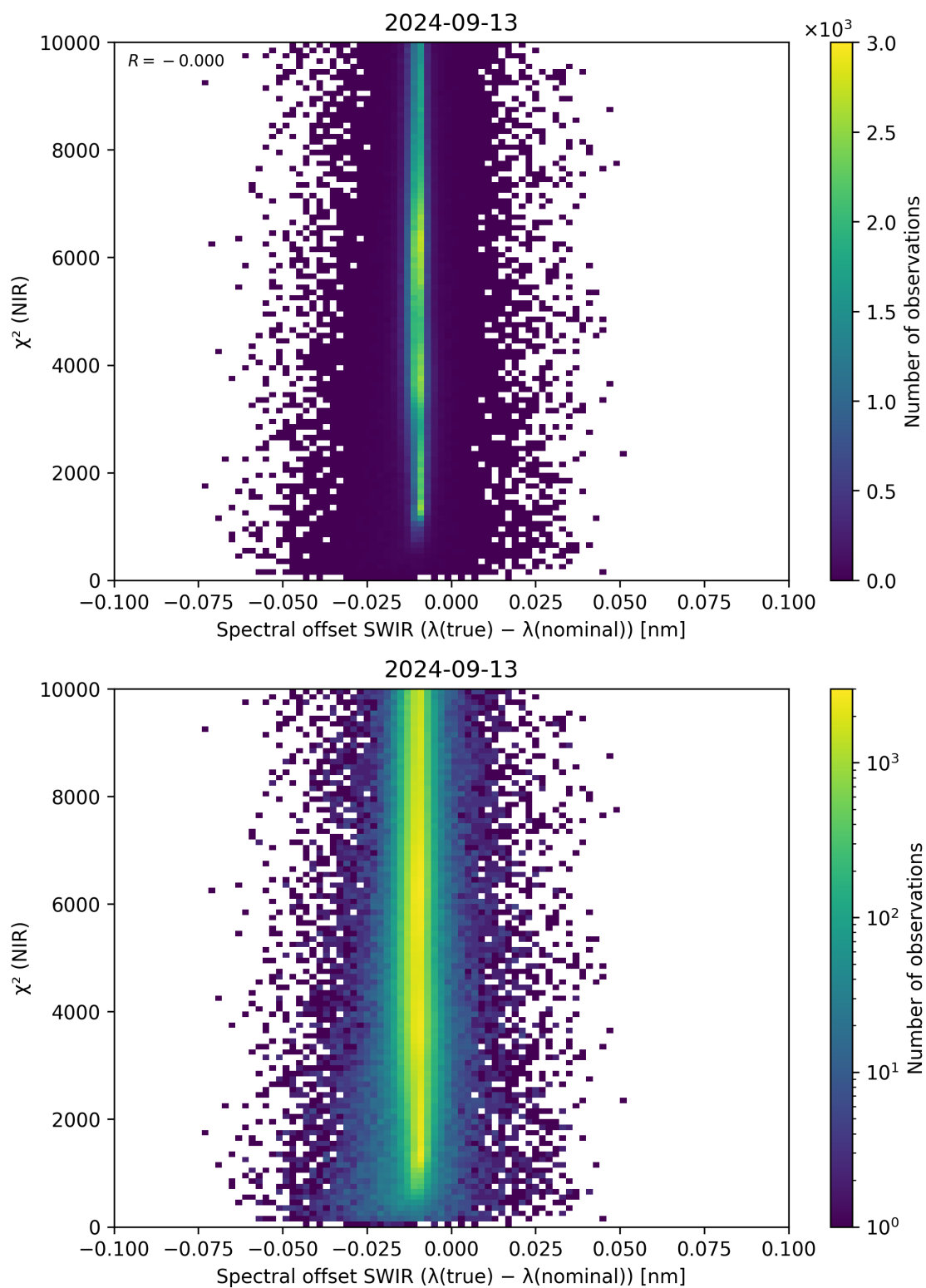
Figure 117: Scatter density plot of “Spectral offset SWIR ( \lambda_{\text{true}} - \lambda_{\text{nominal}} )” against “ \chi^2 (NIR)” for 2024-09-12 to 2024-09-14.
