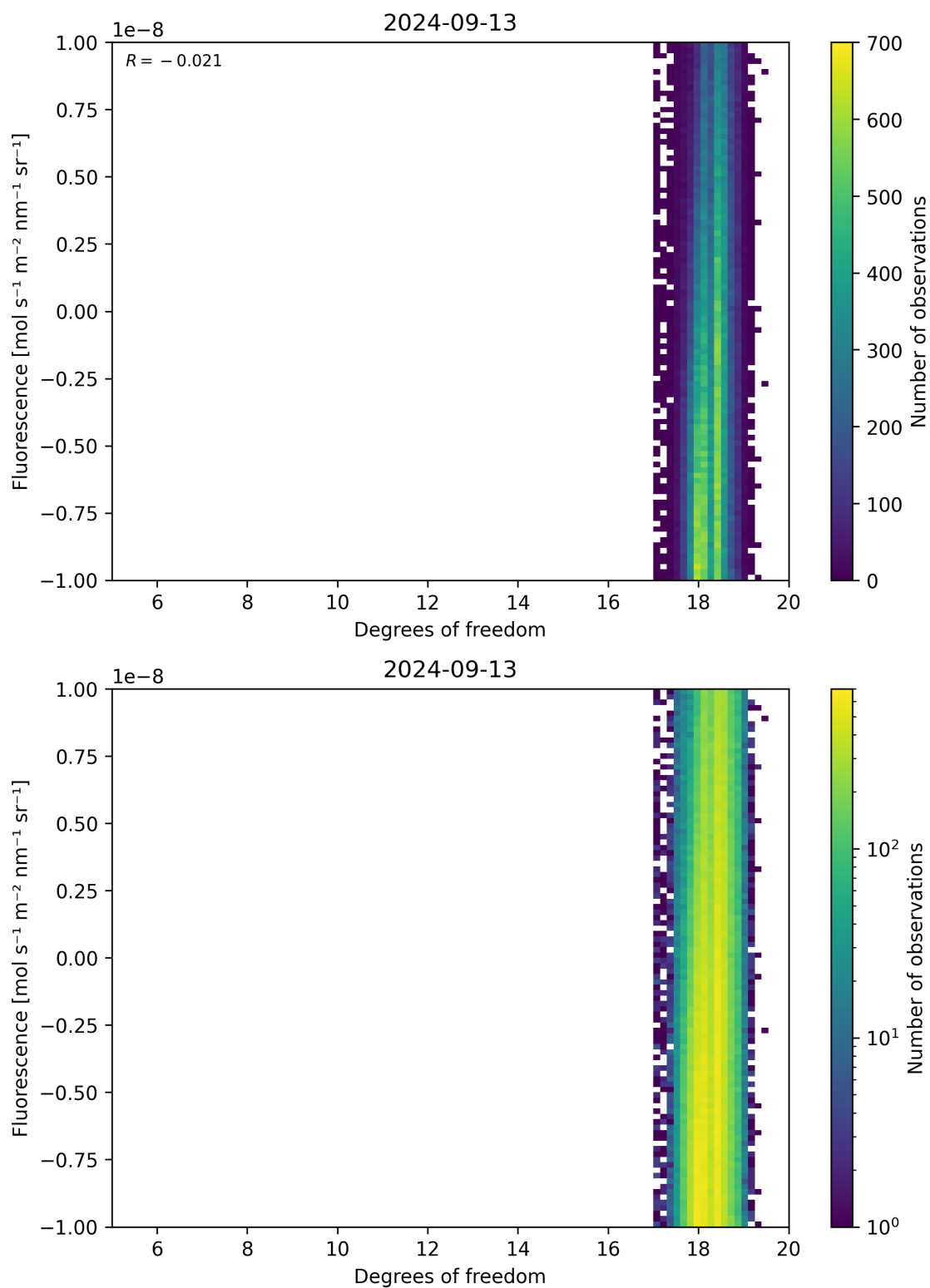
Figure 51: Scatter density plot of “Degrees of freedom” against “Fluorescence” for 2024-09-12 to 2024-09-14.
