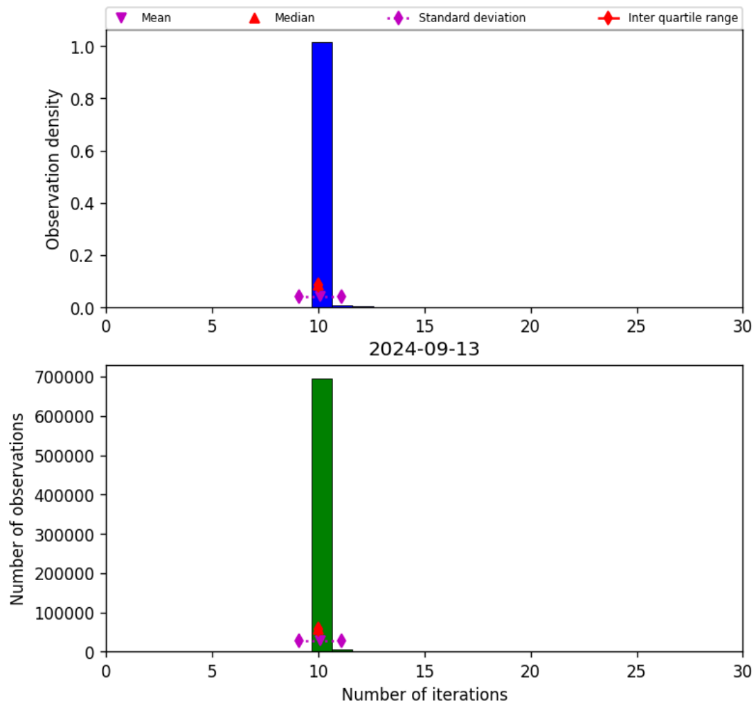
Figure 31: Histogram of “Number of iterations” for 2024-09-12 to 2024-09-14
