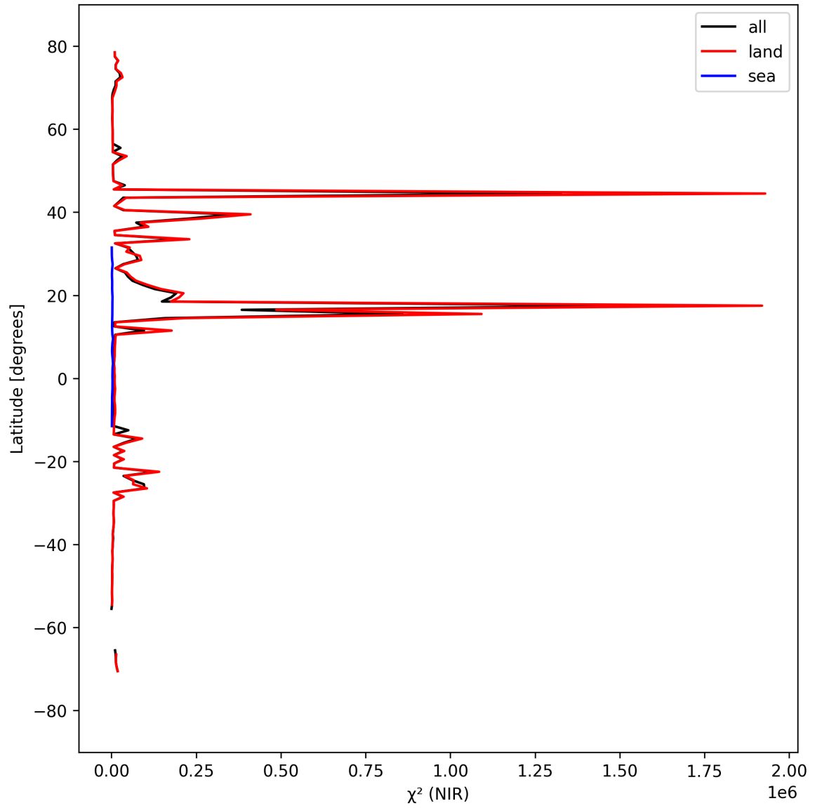
Figure 18: Zonal average of “ \chi^2 (NIR)” for 2024-09-12 to 2024-09-14.
