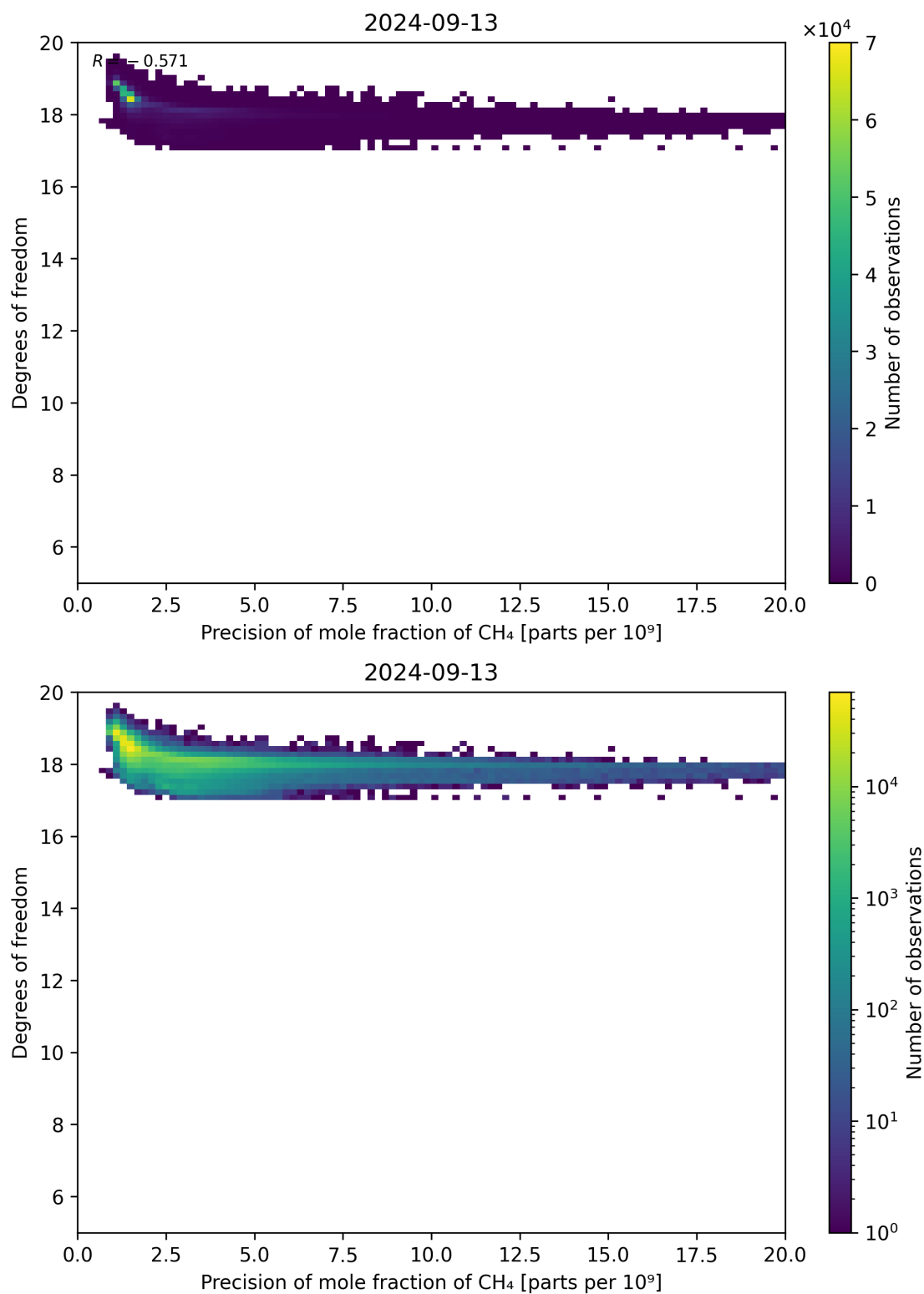
Figure 80: Scatter density plot of “Precision of mole fraction of CH 4 ” against “Degrees of freedom” for 2024-09-12 to 2024-09-14.
