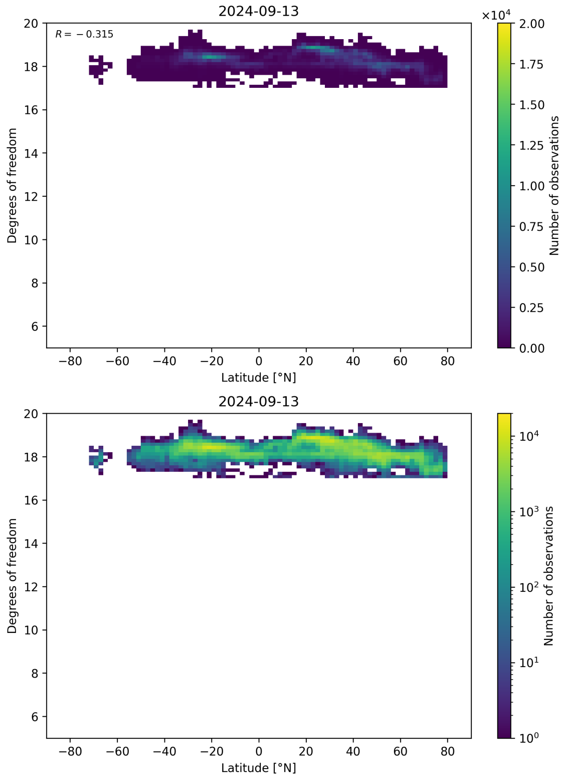
Figure 55: Scatter density plot of “Latitude” against “Degrees of freedom” for 2024-09-12 to 2024-09-14.
