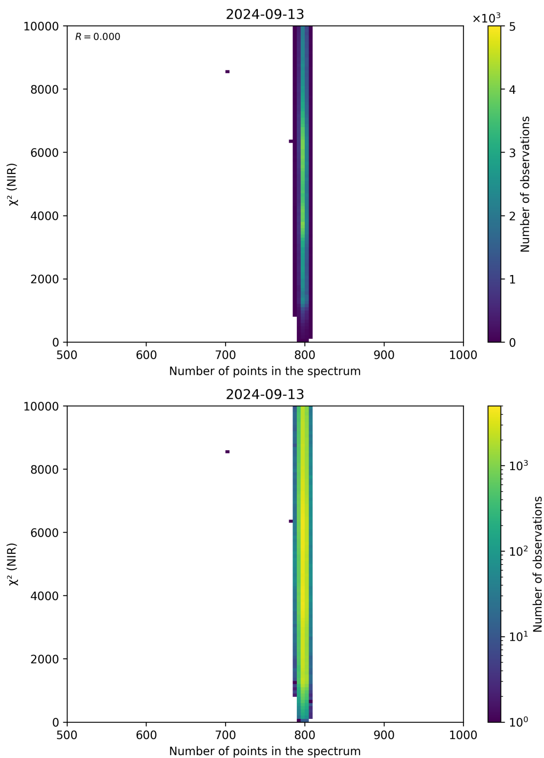
Figure 88: Scatter density plot of “Number of points in the spectrum” against “ \chi^2 (NIR)” for 2024-09-12 to 2024-09-14.
