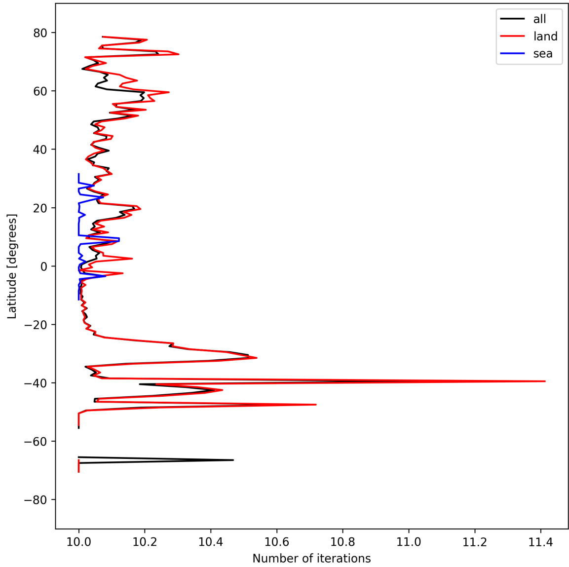
Figure 20: Zonal average of “Number of iterations” for 2024-09-12 to 2024-09-14.
