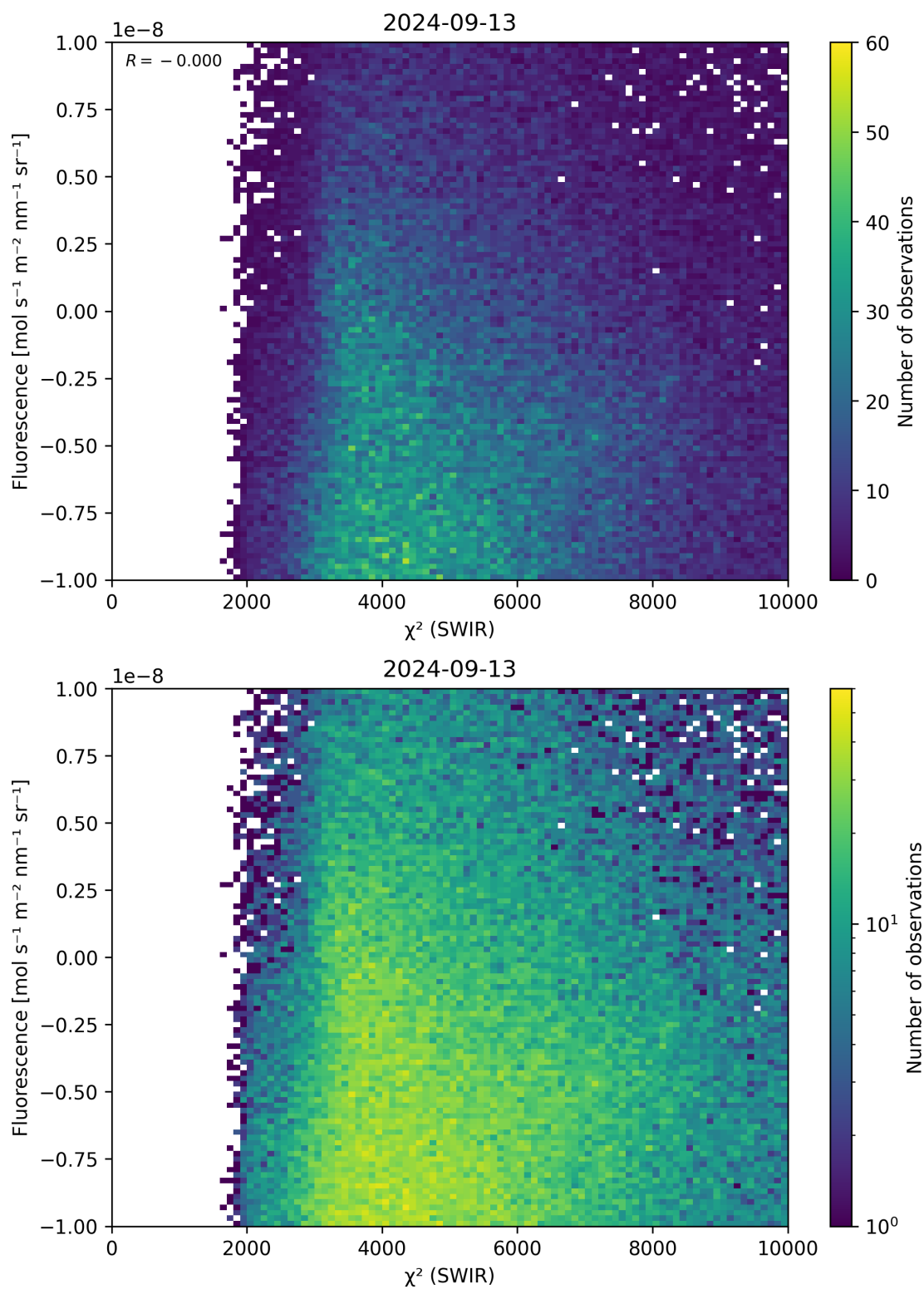
Figure 49: Scatter density plot of “ \chi^2 (SWIR)” against “Fluorescence” for 2024-09-12 to 2024-09-14.
