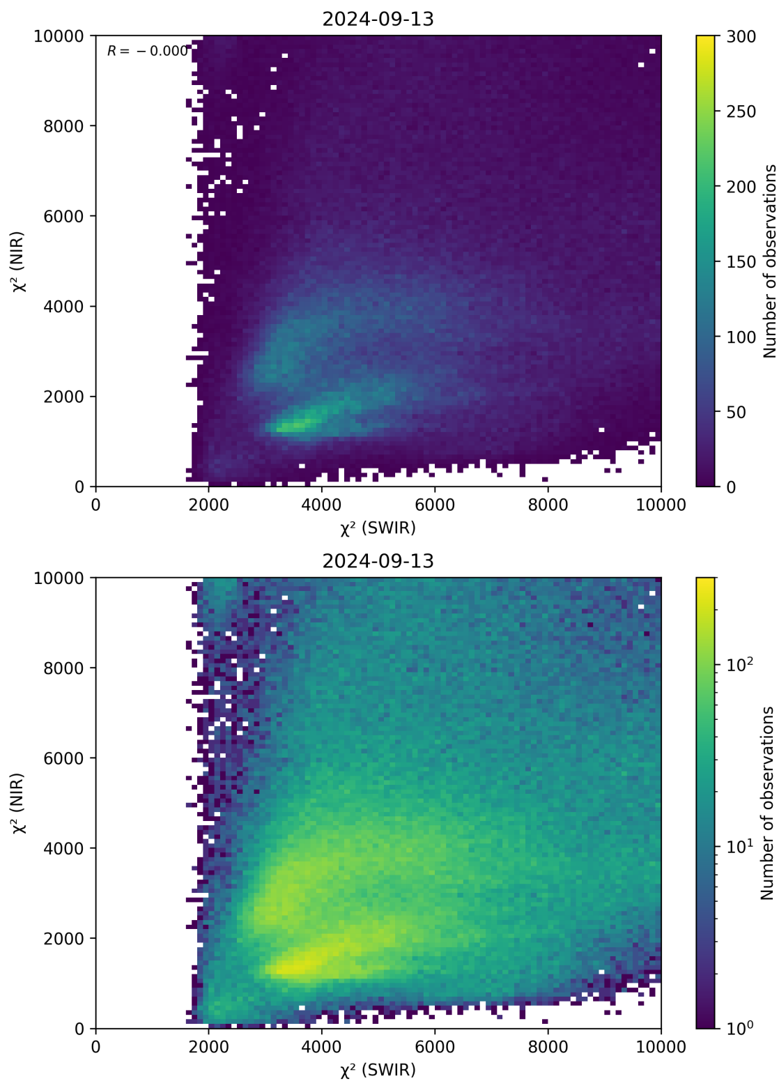
Figure 47: Scatter density plot of “ \chi^2 (SWIR)” against “ \chi^2 (NIR)” for 2024-09-12 to 2024-09-14.
