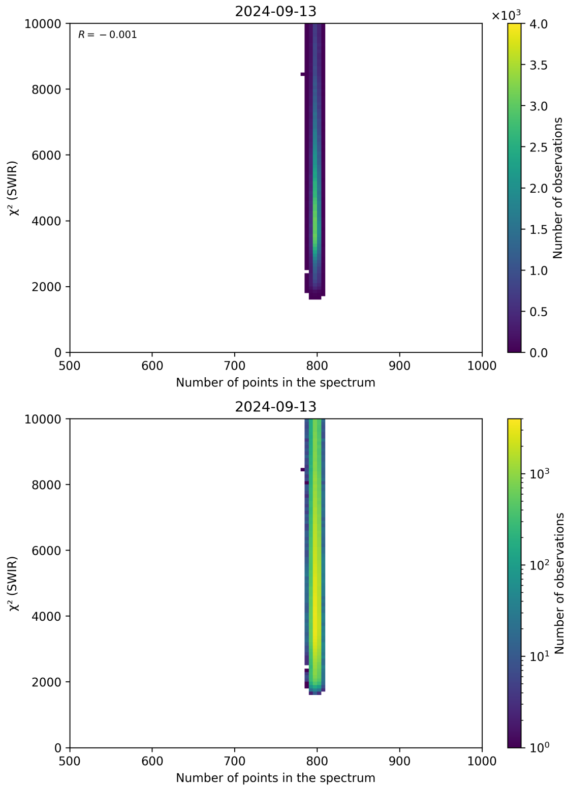
Figure 89: Scatter density plot of “Number of points in the spectrum” against “ \chi^2 (SWIR)” for 2024-09-12 to 2024-09-14.
