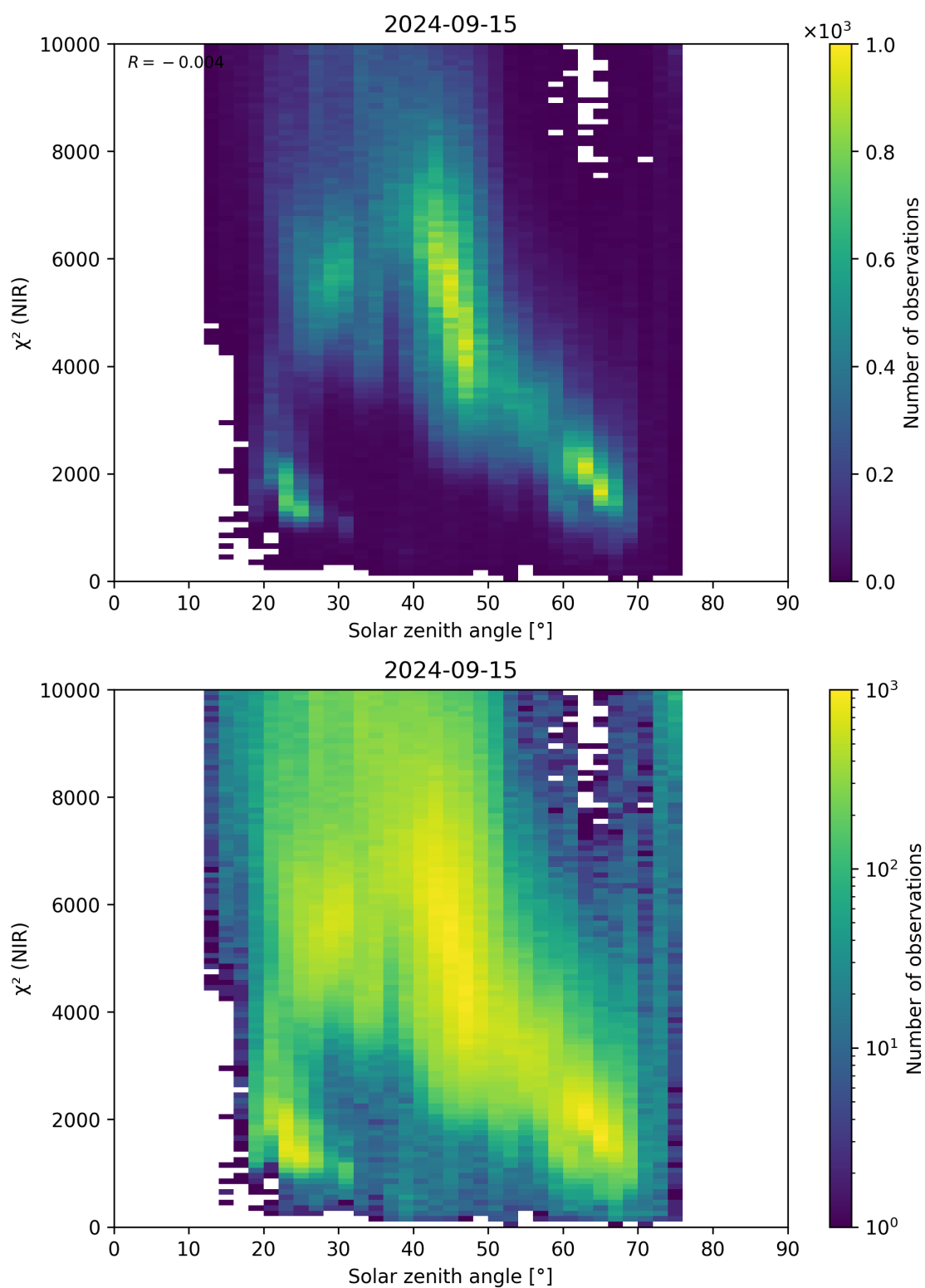
Figure 94: Scatter density plot of “Solar zenith angle” against “ \chi^2 (NIR)” for 2024-09-14 to 2024-09-16.
