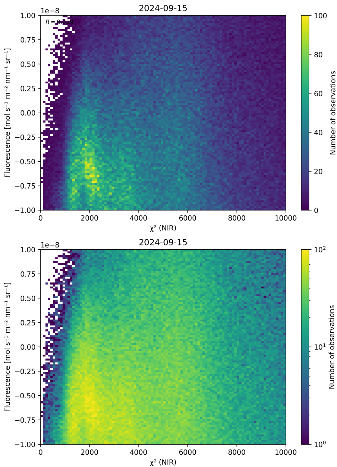
Figure 45: Scatter density plot of “ \chi^2 (NIR)” against “Fluorescence” for 2024-09-14 to 2024-09-16.
