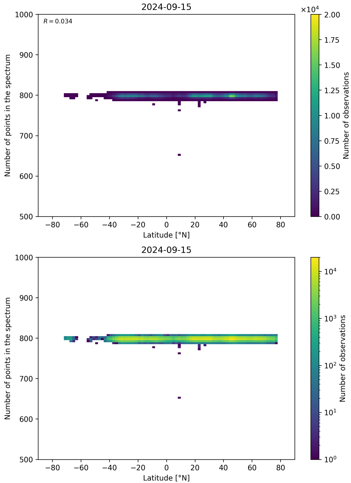
Figure 61: Scatter density plot of “Latitude” against “Number of points in the spectrum” for 2024-09-14 to 2024-09-16.
