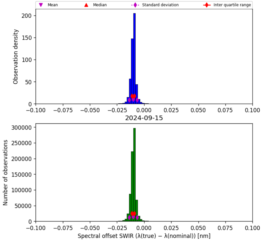
Figure 27: Histogram of “Spectral offset SWIR ( \lambda_{\text{true}} - \lambda_{\text{nominal}} )” for 2024-09-14 to 2024-09-16
