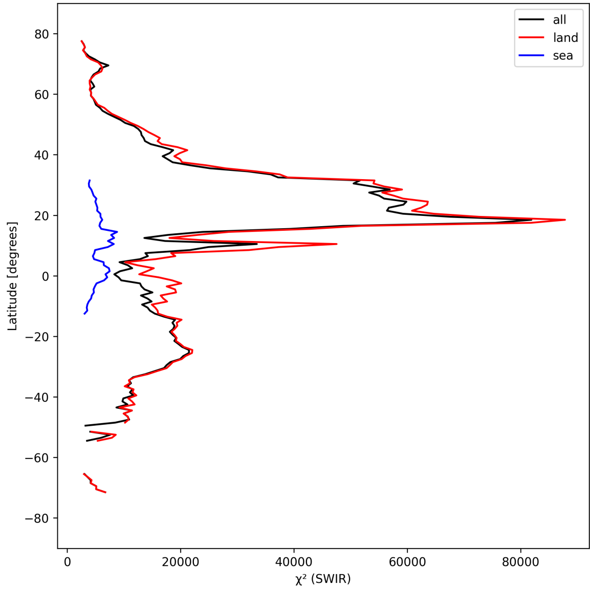
Figure 17: Zonal average of “ \chi^2 (SWIR)” for 2024-09-14 to 2024-09-16.
