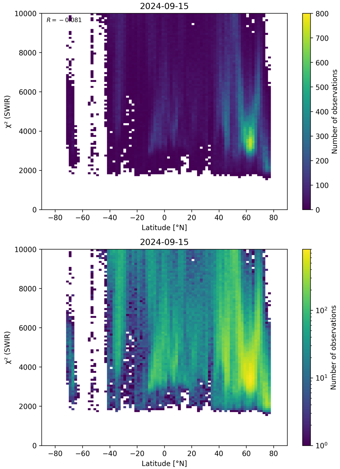
Figure 54: Scatter density plot of “Latitude” against “ \chi^2 (SWIR)” for 2024-09-14 to 2024-09-16.
