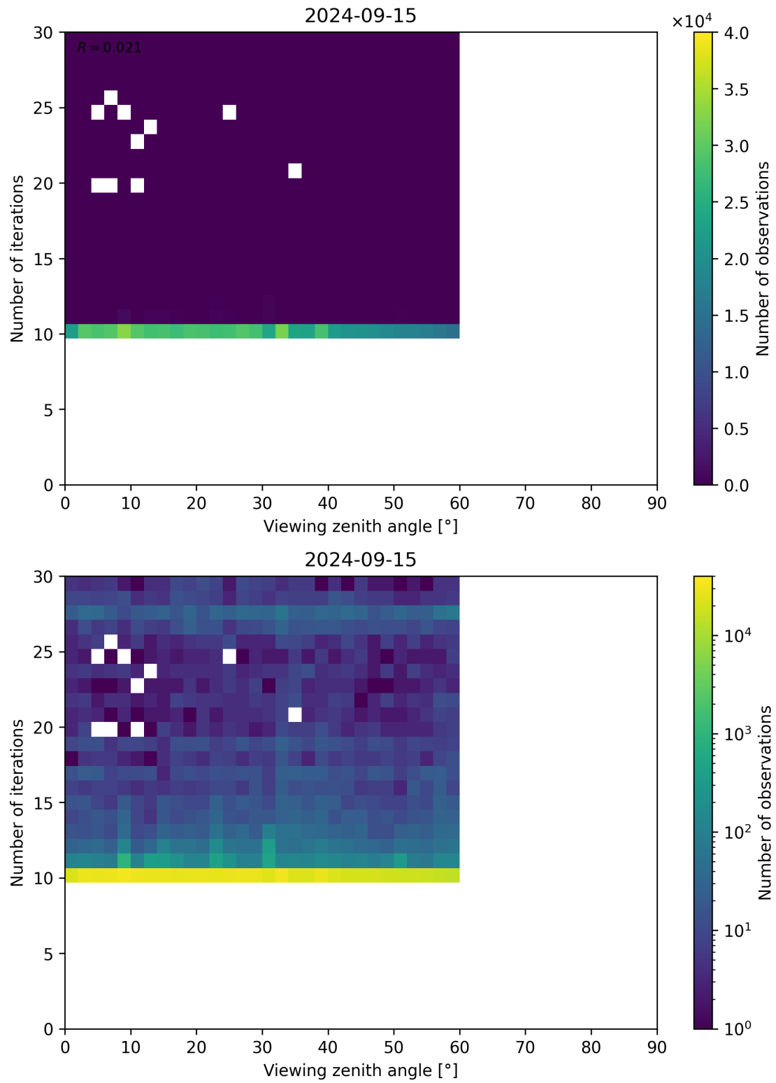
Figure 113: Scatter density plot of “Viewing zenith angle” against “Number of iterations” for 2024-09-14 to 2024-09-16.
