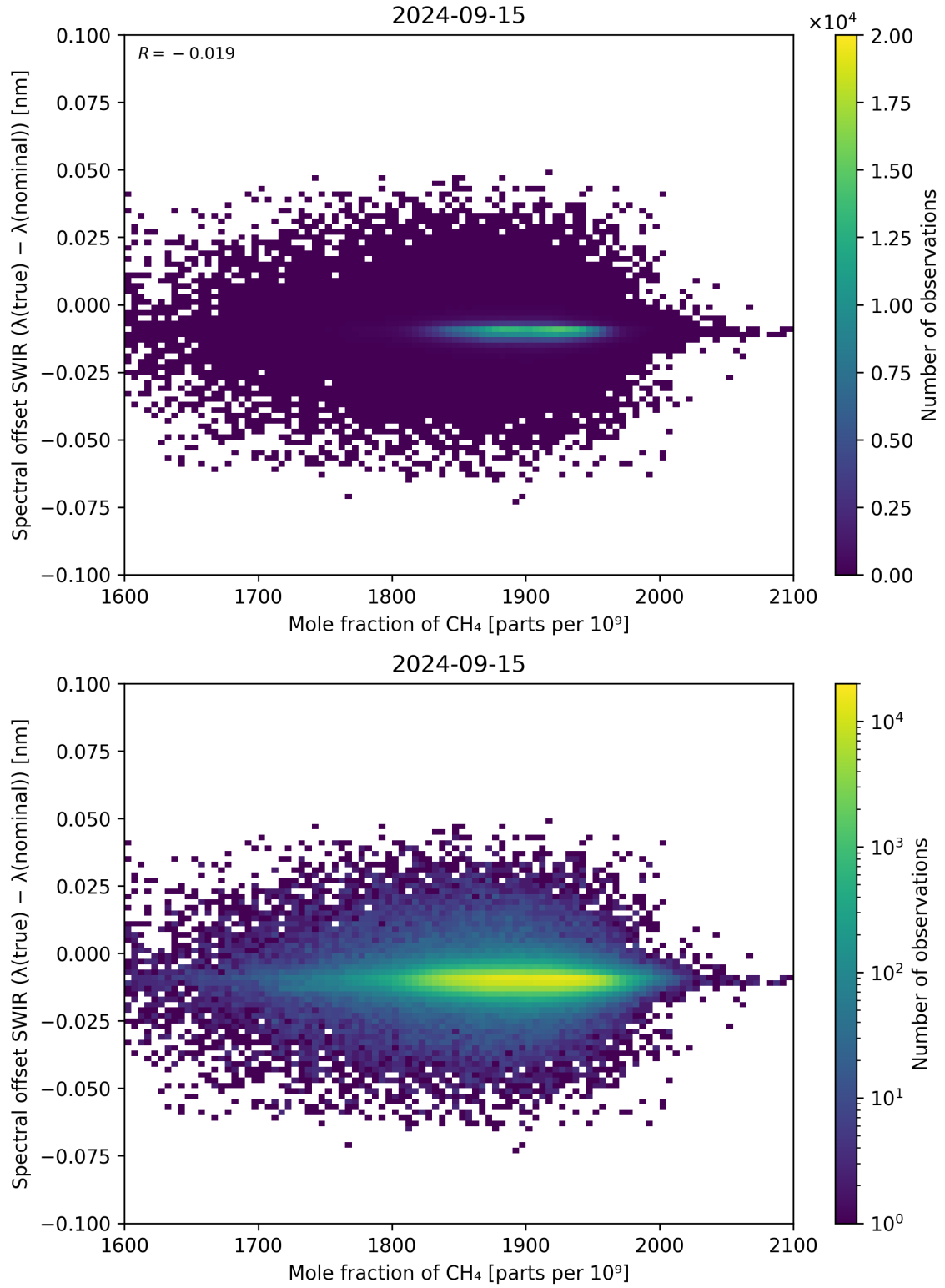
Figure 86: Scatter density plot of “Mole fraction of CH 4 ” against “Spectral offset SWIR ( \lambda_{\text{true}} - \lambda_{\text{nominal}} )” for 2024-09-14 to 2024-09-16.
