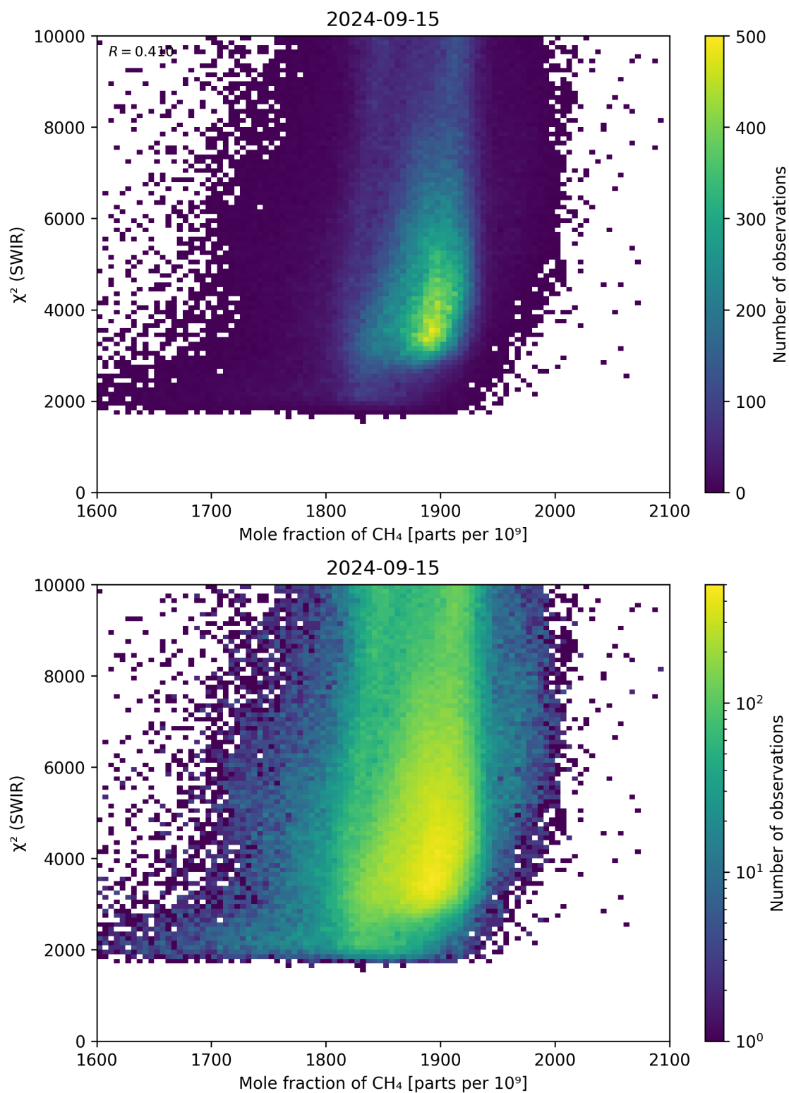
Figure 71: Scatter density plot of “Mole fraction of \text{CH}_4 ” against “ \chi^2 (SWIR)” for 2024-09-14 to 2024-09-16.
