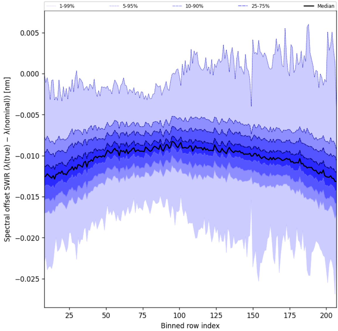
Figure 38: Along track statistics of “Spectral offset SWIR ( \lambda_{\text{true}} - \lambda_{\text{nominal}} )” for 2024-09-14 to 2024-09-16
