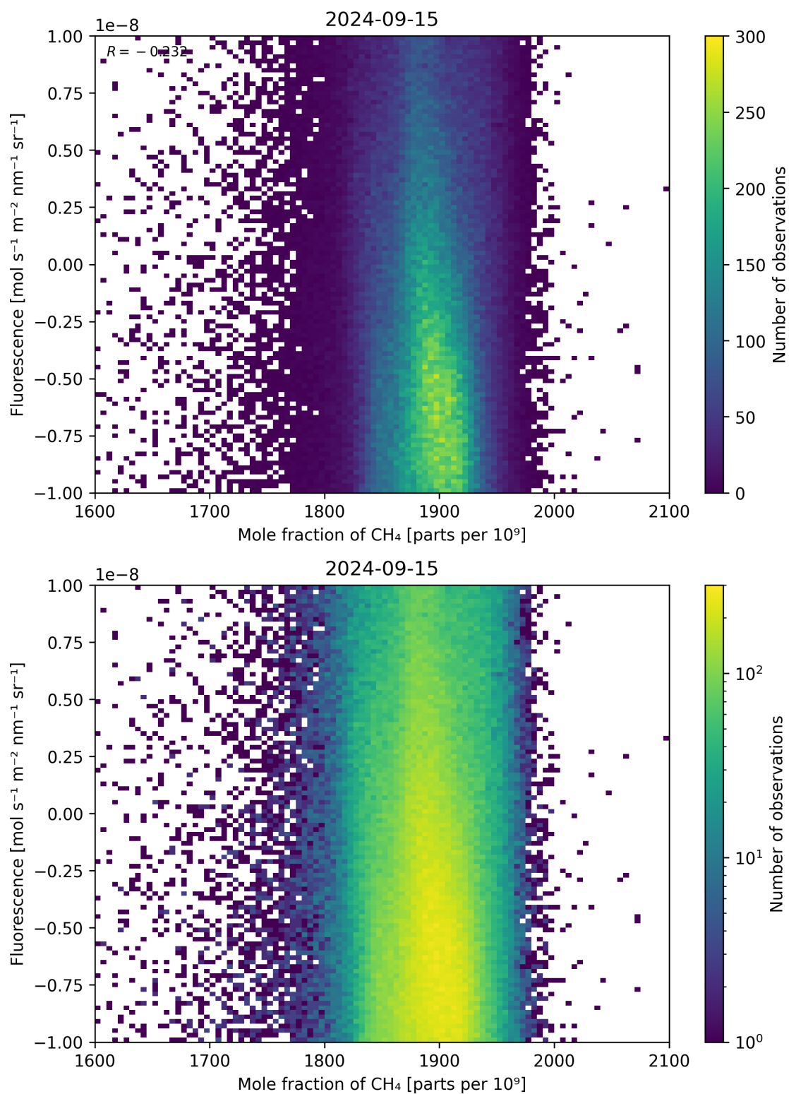
Figure 73: Scatter density plot of “Mole fraction of \text{CH}_4 ” against “Fluorescence” for 2024-09-14 to 2024-09-16.
