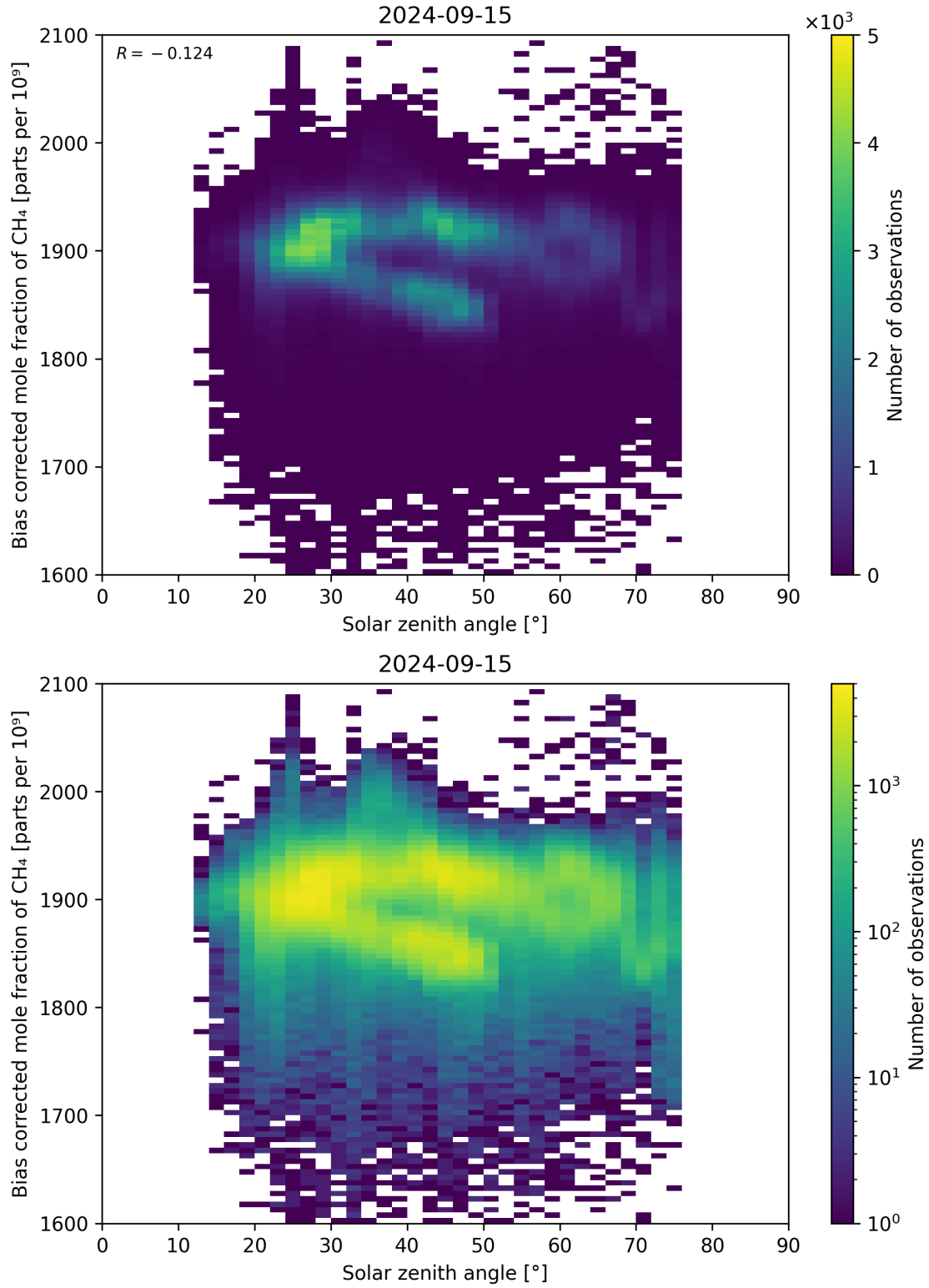
Figure 100: Scatter density plot of “Solar zenith angle” against “Bias corrected mole fraction of CH 4 ” for 2024-09-14 to 2024-09-16.
