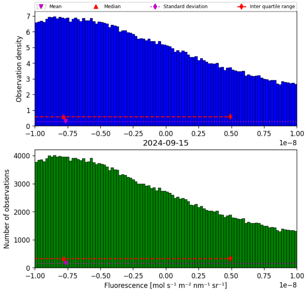
Figure 32: Histogram of “Fluorescence” for 2024-09-14 to 2024-09-16
