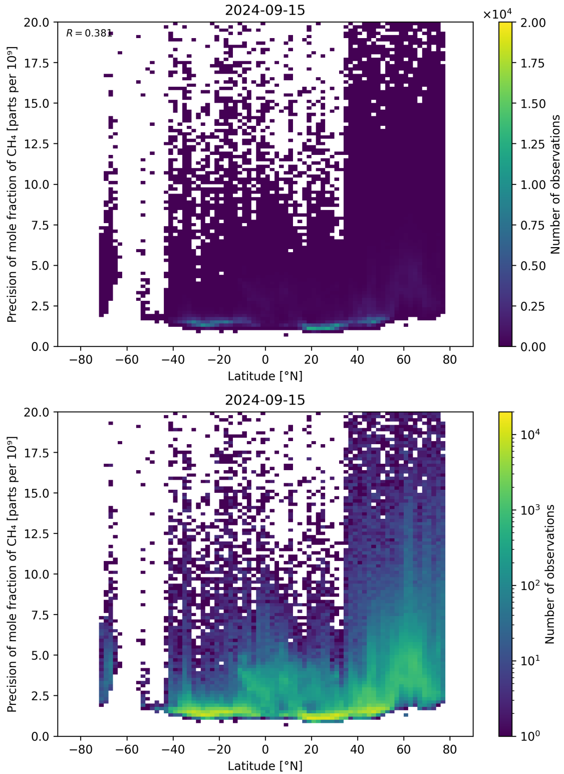
Figure 59: Scatter density plot of “Latitude” against “Precision of mole fraction of CH 4 ” for 2024-09-14 to 2024-09-16.
