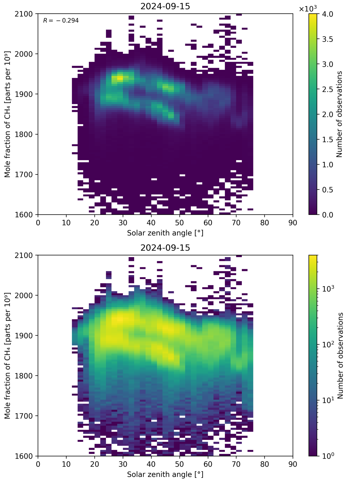
Figure 99: Scatter density plot of “Solar zenith angle” against “Mole fraction of CH 4 ” for 2024-09-14 to 2024-09-16.
