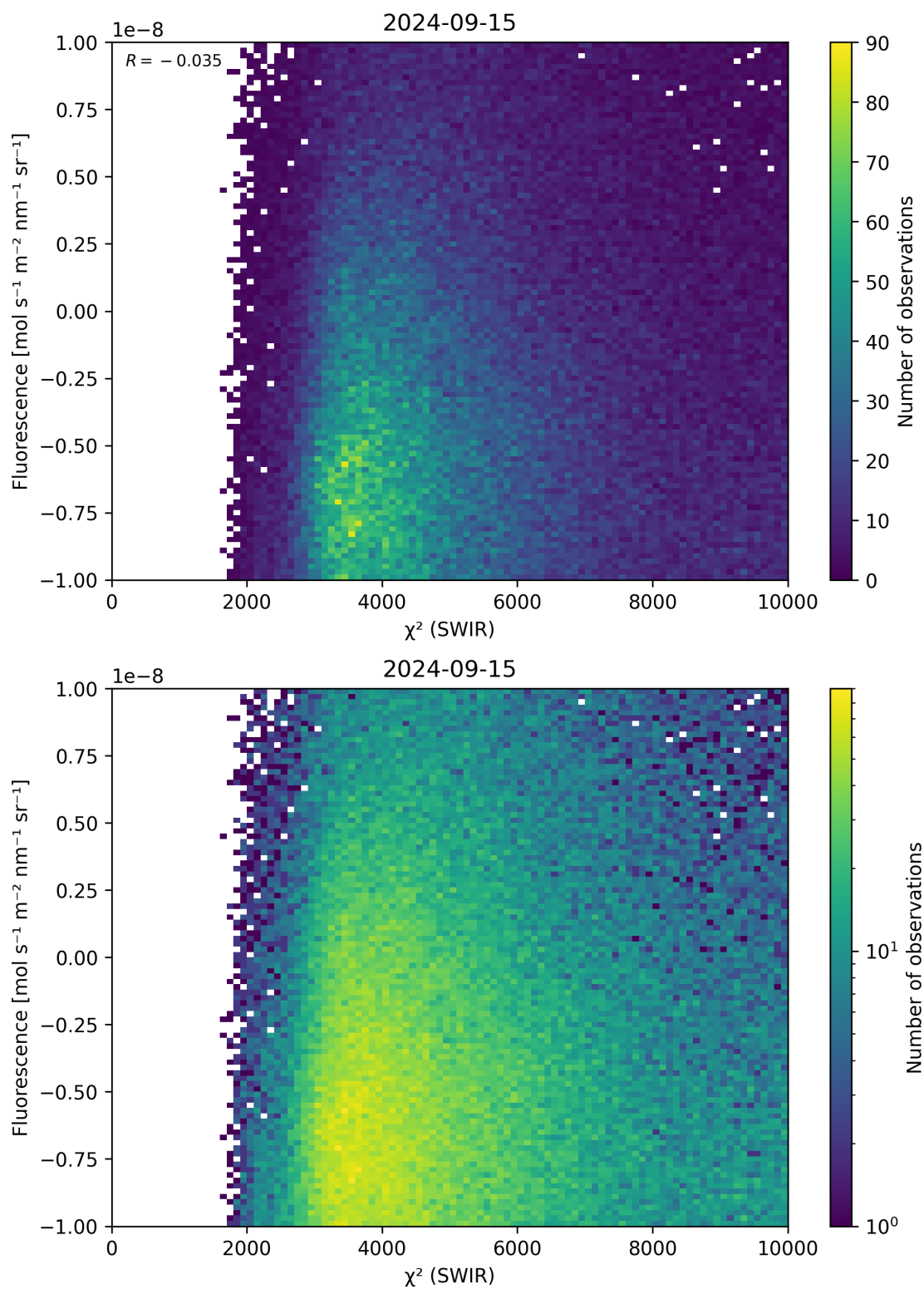
Figure 49: Scatter density plot of “ \chi^2 (SWIR)” against “Fluorescence” for 2024-09-14 to 2024-09-16.
