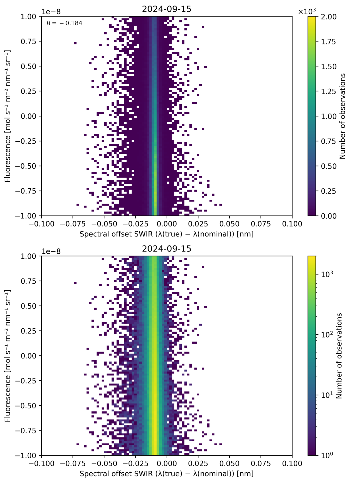
Figure 120: Scatter density plot of “Spectral offset SWIR ( \lambda_{\text{true}} - \lambda_{\text{nominal}} )” against “Fluorescence” for 2024-09-14 to 2024-09-16.
