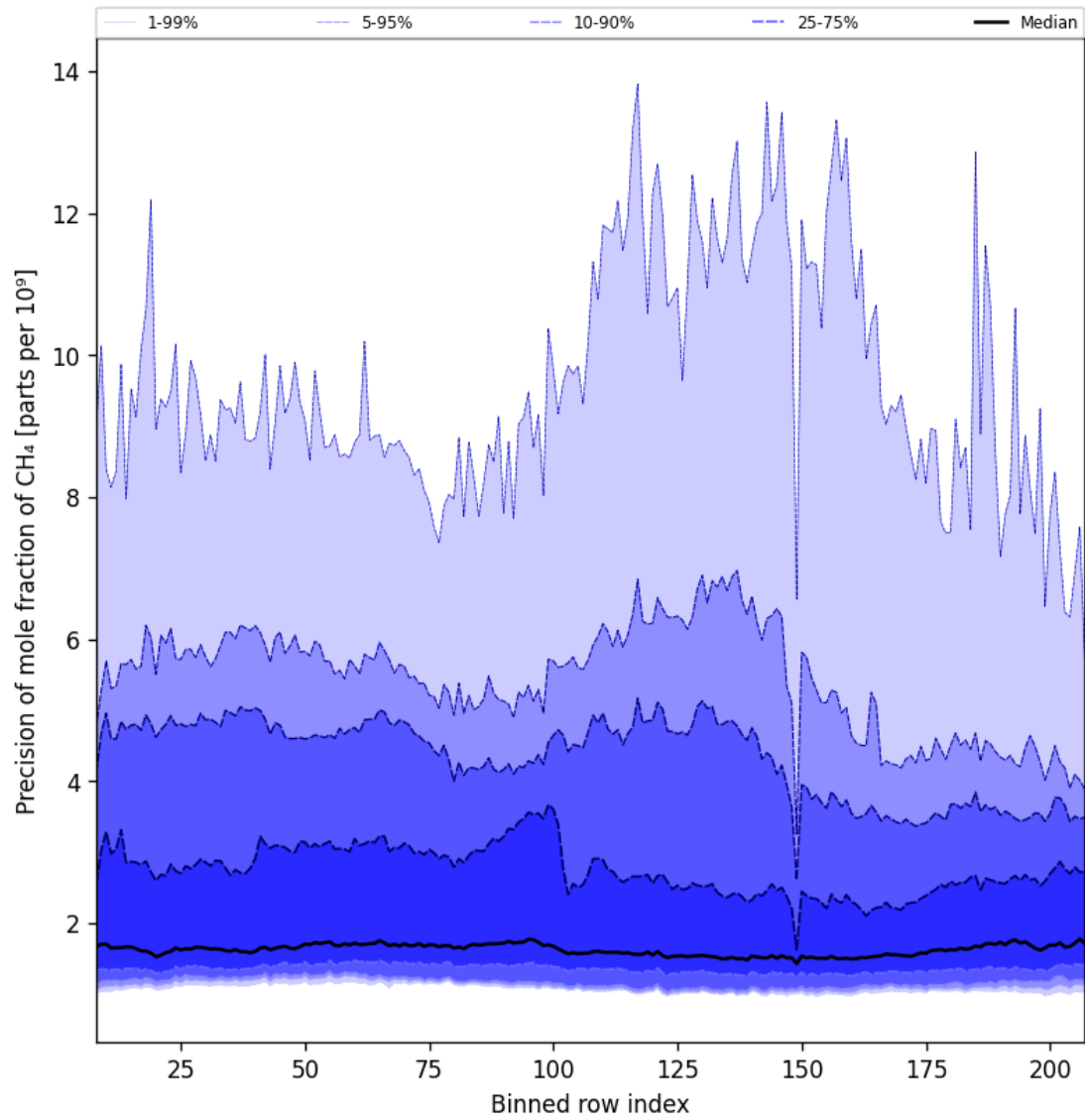
Figure 35: Along track statistics of “Precision of mole fraction of CH 4 ” for 2024-09-14 to 2024-09-16
