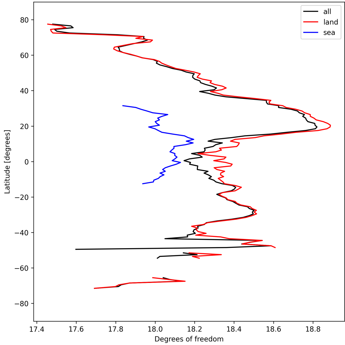
Figure 19: Zonal average of “Degrees of freedom” for 2024-09-14 to 2024-09-16.
