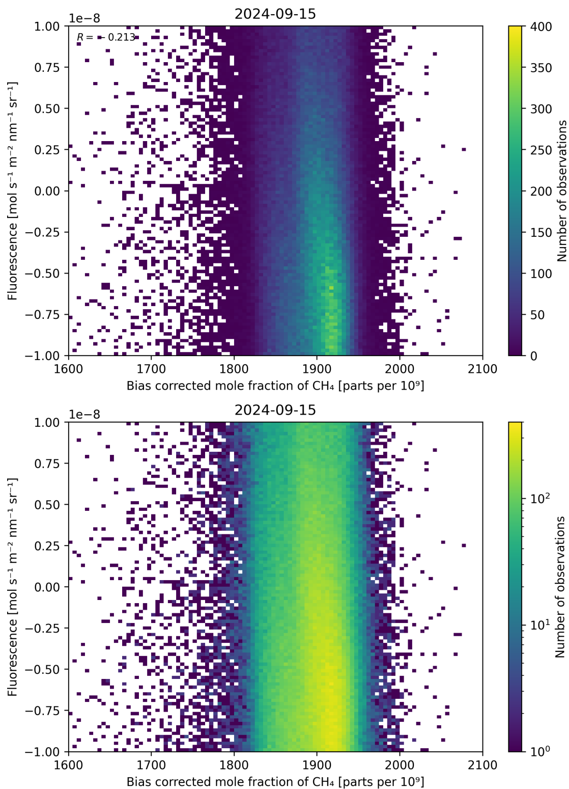
Figure 66: Scatter density plot of “Bias corrected mole fraction of \text{CH}_4 ” against “Fluorescence” for 2024-09-14 to 2024-09-16.
