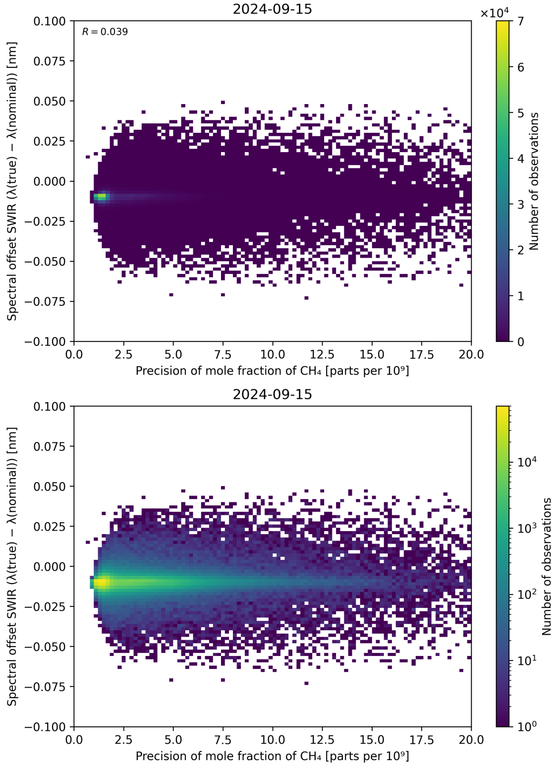
Figure 85: Scatter density plot of “Precision of mole fraction of \text{CH}_4 ” against “Spectral offset SWIR ( \lambda_{\text{true}} - \lambda_{\text{nominal}} )” for 2024-09-14 to 2024-09-16.
