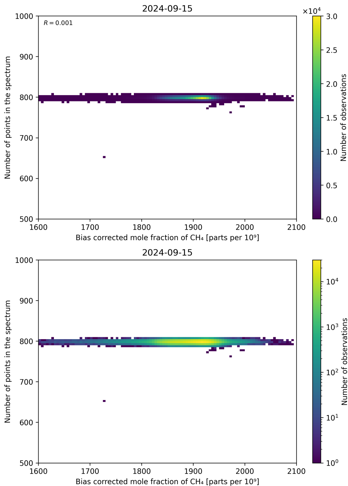
Figure 68: Scatter density plot of “Bias corrected mole fraction of CH 4 ” against “Number of points in the spectrum” for 2024-09-14 to 2024-09-16.
