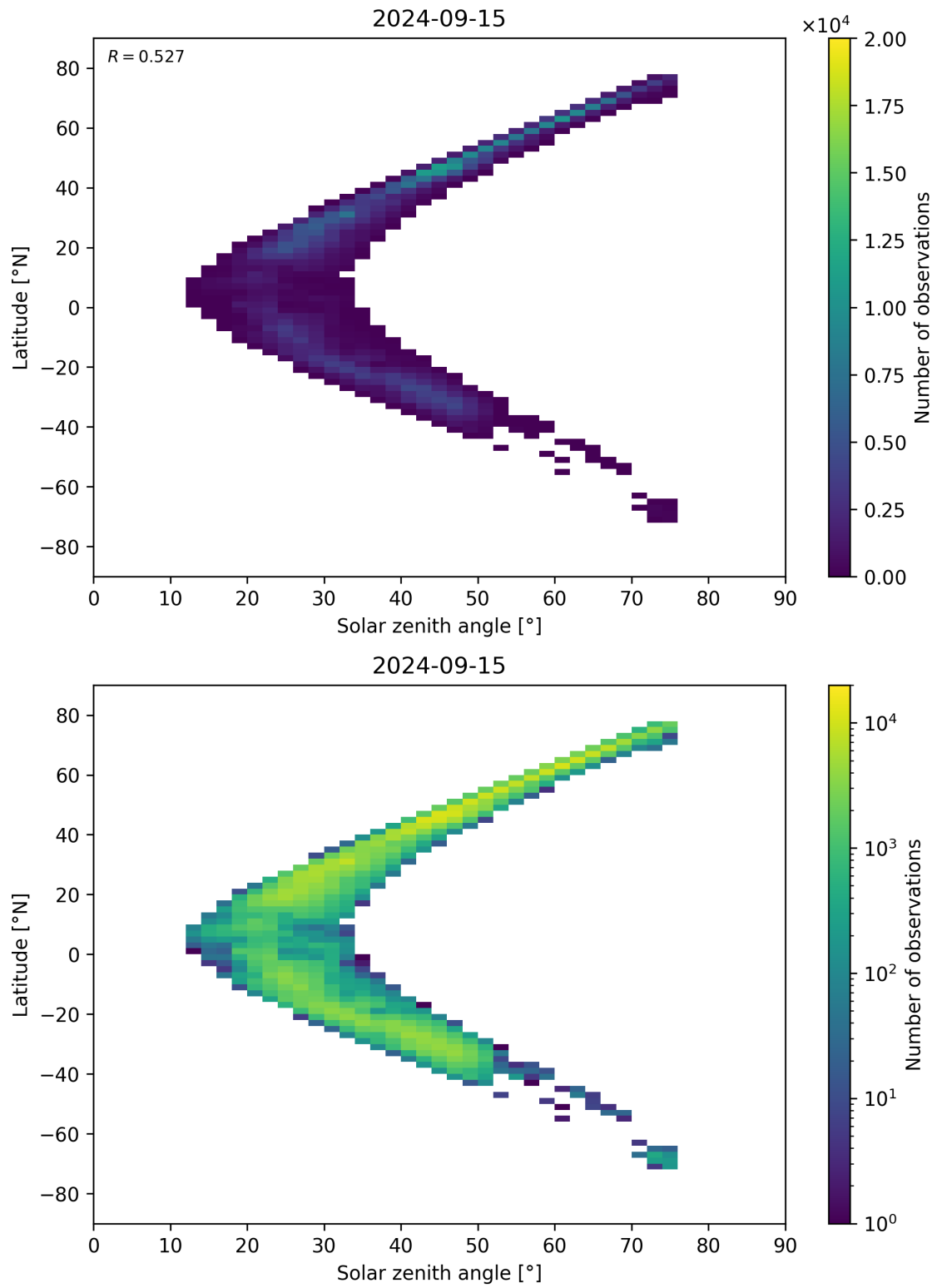
Figure 98: Scatter density plot of “Solar zenith angle” against “Latitude” for 2024-09-14 to 2024-09-16.
