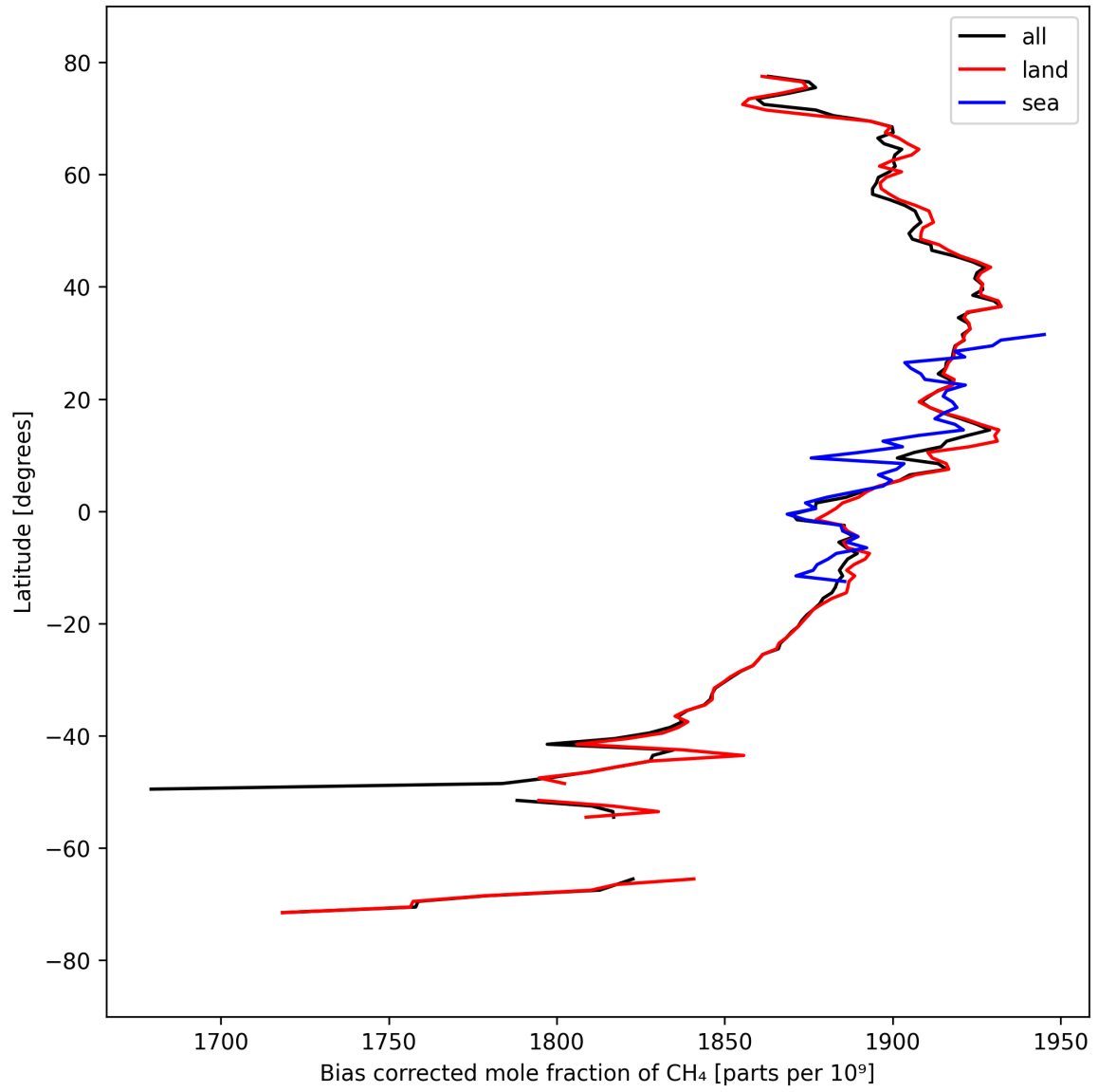
Figure 14: Zonal average of “Bias corrected mole fraction of CH 4 ” for 2024-09-14 to 2024-09-16.
