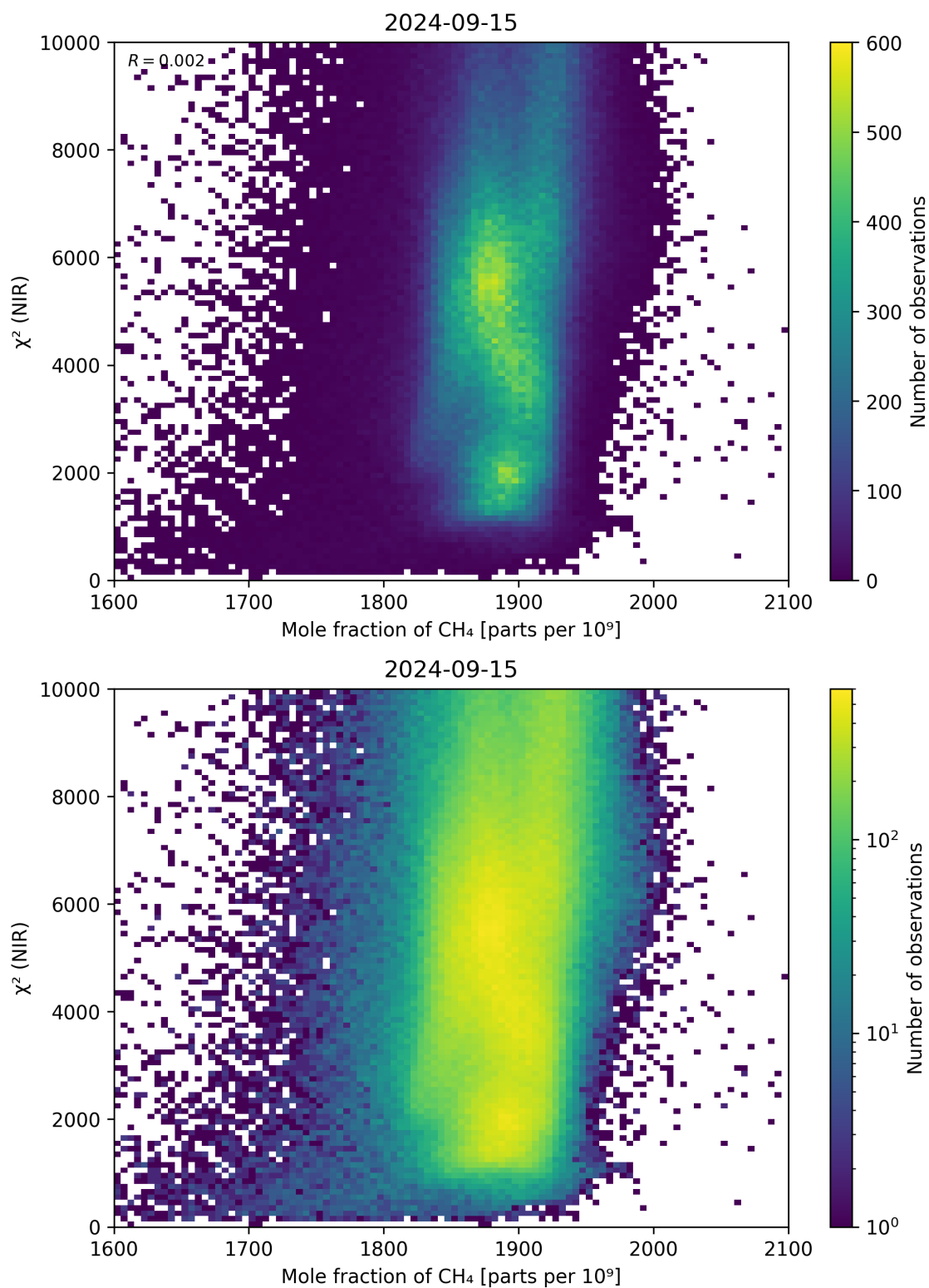
Figure 70: Scatter density plot of “Mole fraction of \text{CH}_4 ” against “ \chi^2 (NIR)” for 2024-09-14 to 2024-09-16.
