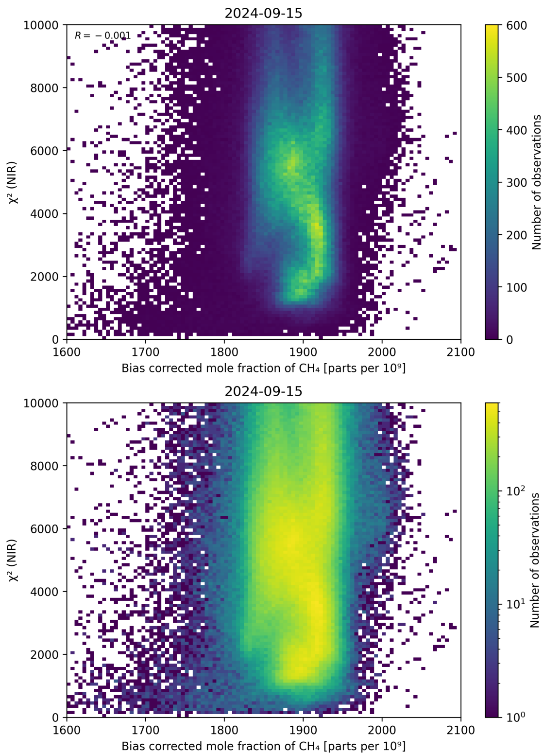
Figure 63: Scatter density plot of “Bias corrected mole fraction of \text{CH}_4 ” against “ \chi^2 (NIR)” for 2024-09-14 to 2024-09-16.
