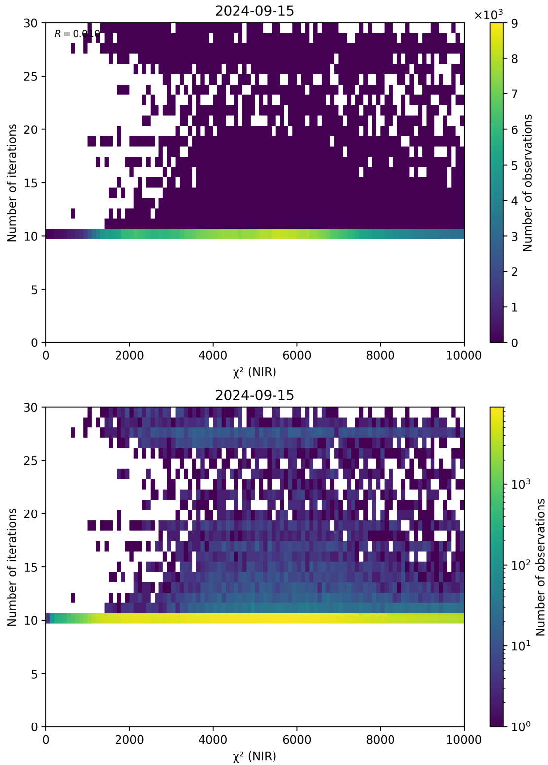
Figure 46: Scatter density plot of “ \chi^2 (NIR)” against “Number of iterations” for 2024-09-14 to 2024-09-16.
