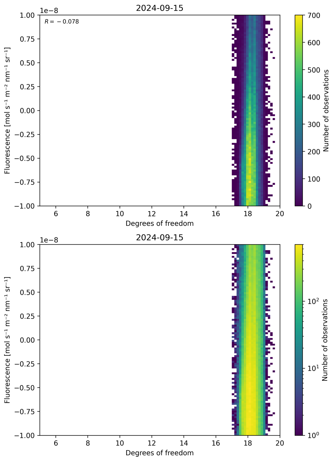
Figure 51: Scatter density plot of “Degrees of freedom” against “Fluorescence” for 2024-09-14 to 2024-09-16.
