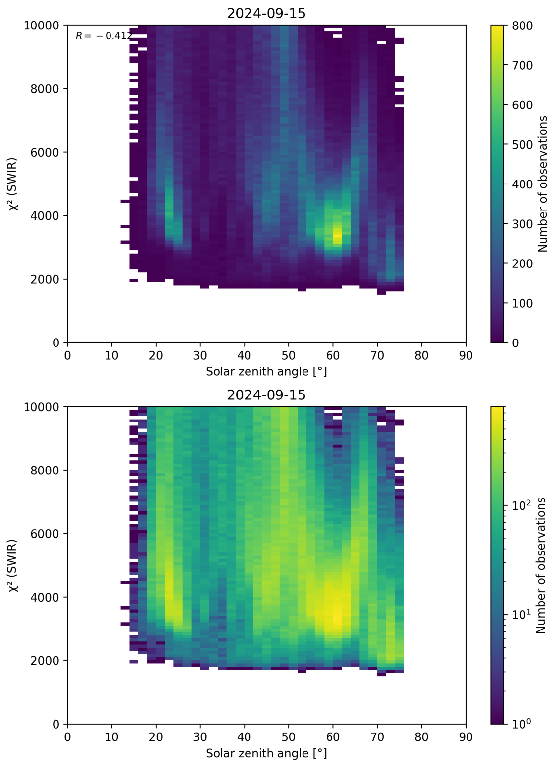
Figure 95: Scatter density plot of “Solar zenith angle” against “ \chi^2 (SWIR)” for 2024-09-14 to 2024-09-16.
