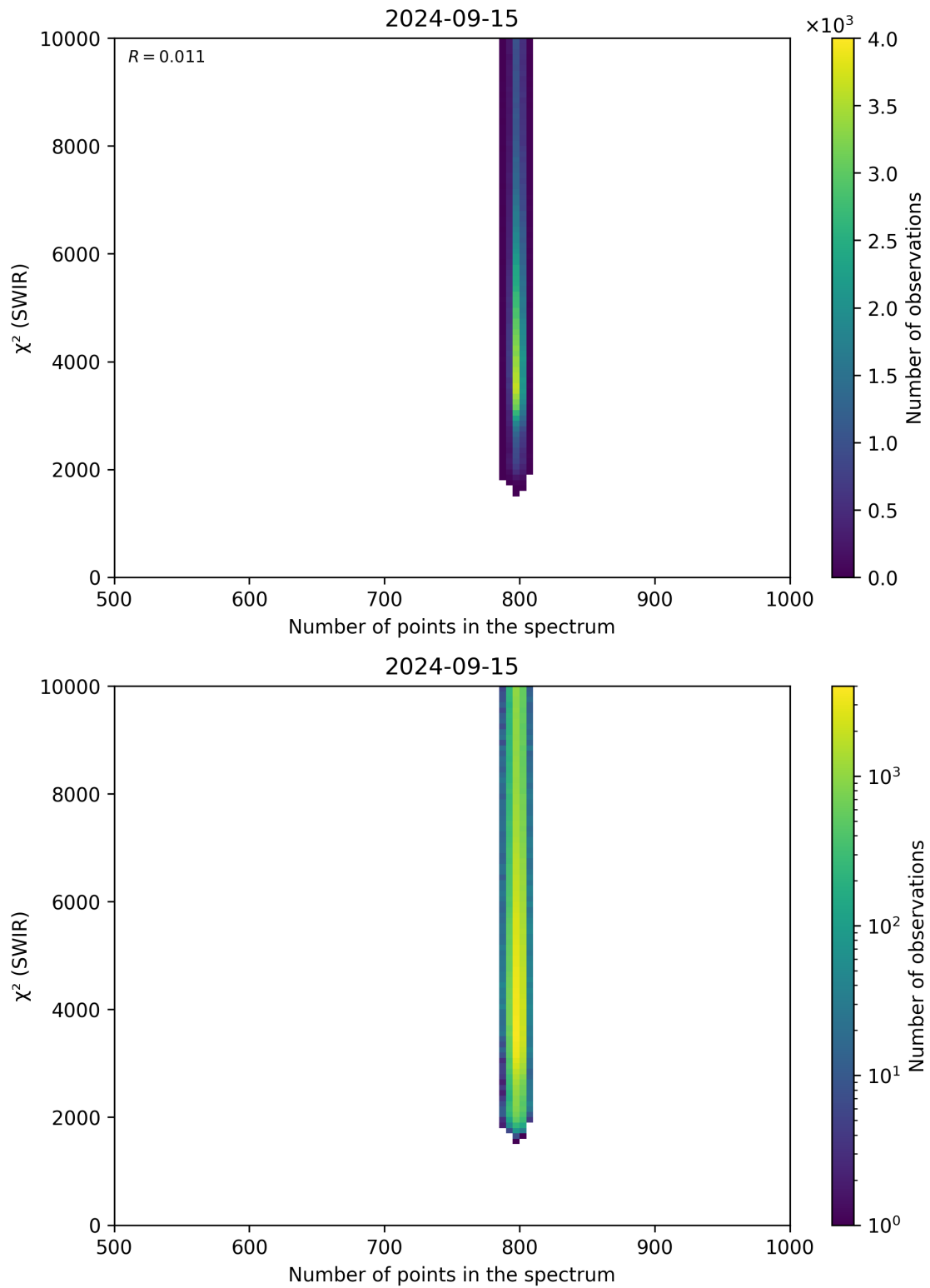
Figure 89: Scatter density plot of “Number of points in the spectrum” against “ \chi^2 (SWIR)” for 2024-09-14 to 2024-09-16.
