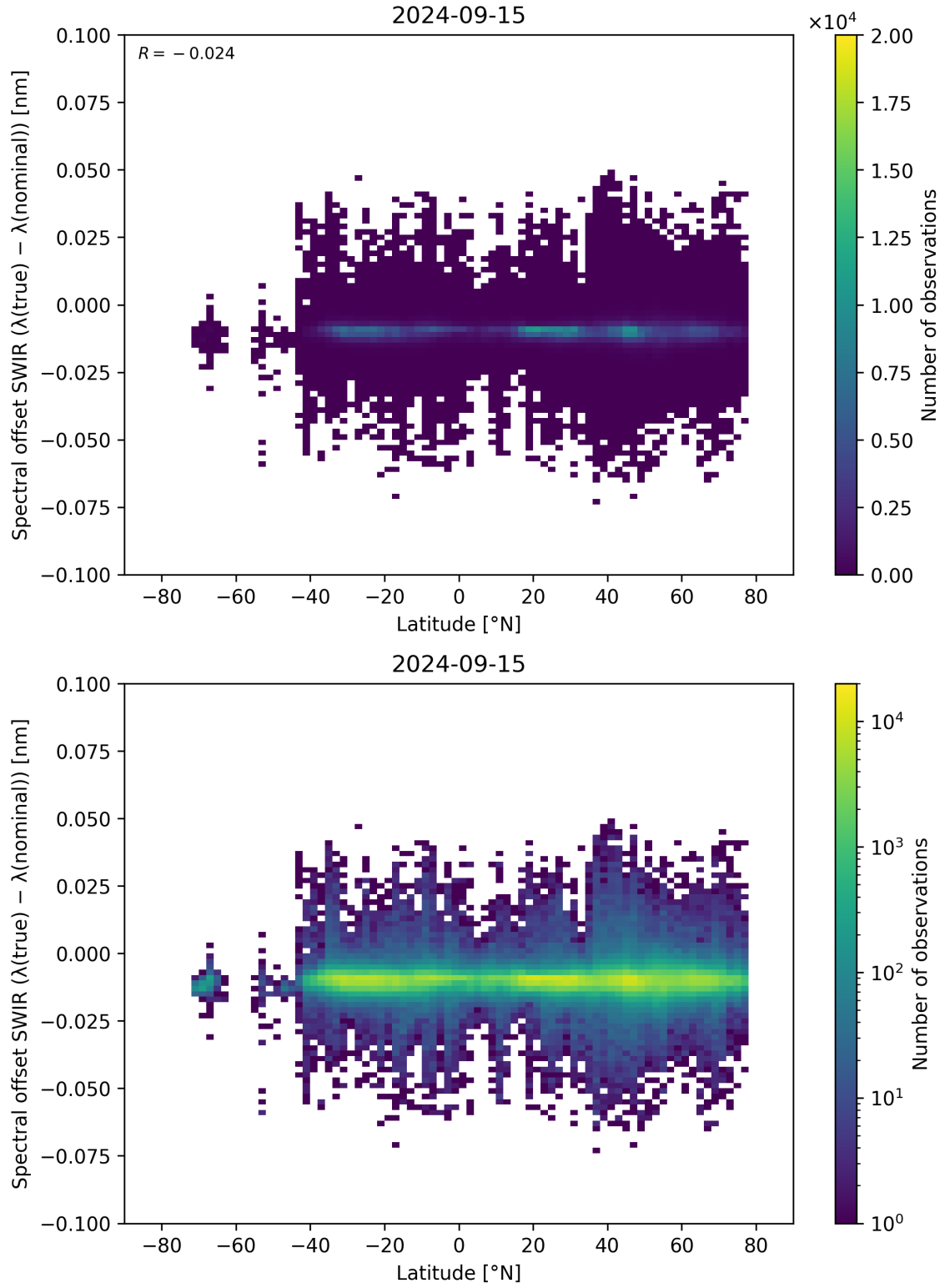
Figure 62: Scatter density plot of “Latitude” against “Spectral offset SWIR ( \lambda_{\text{true}} - \lambda_{\text{nominal}} )” for 2024-09-14 to 2024-09-16.
