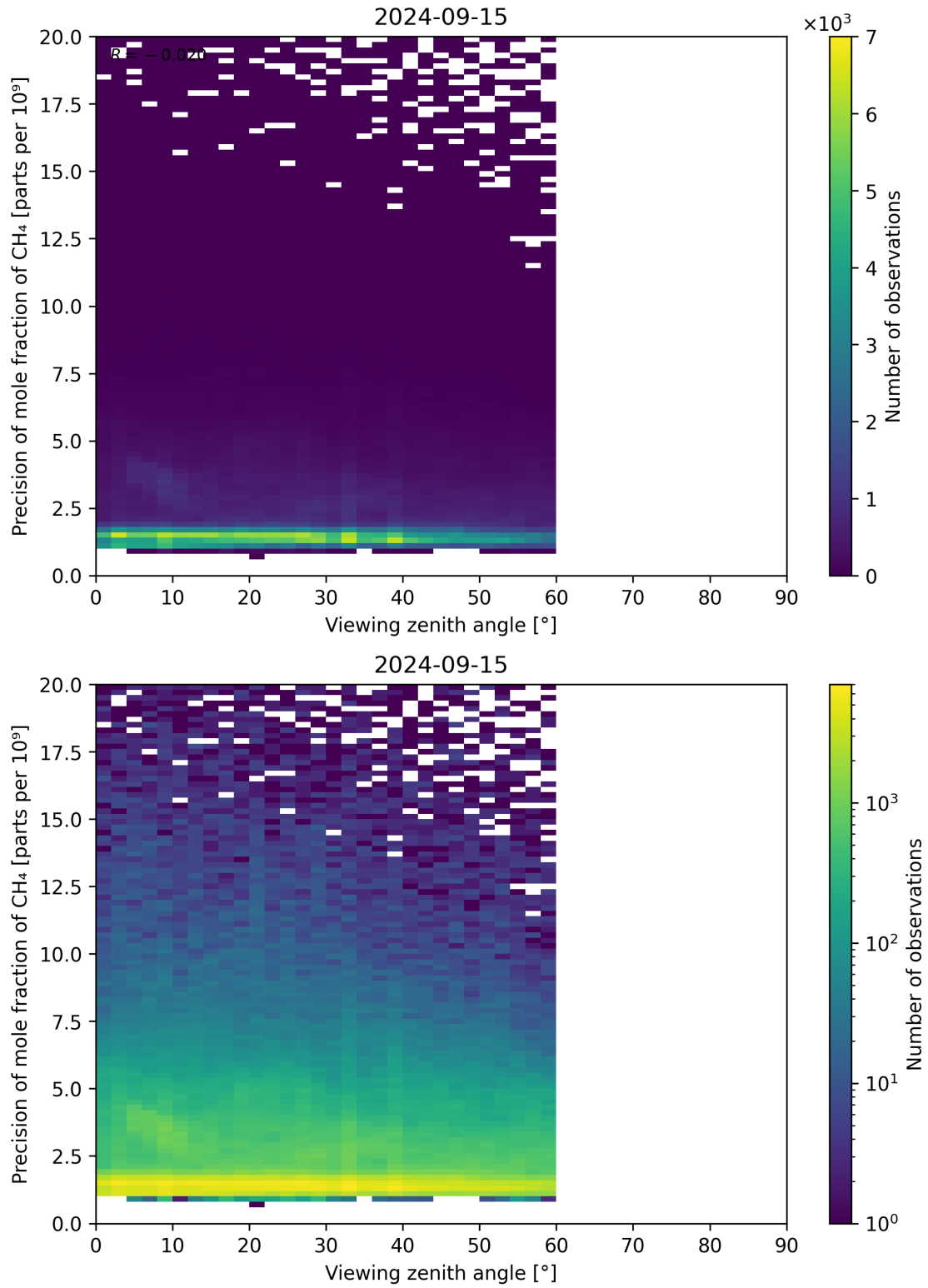
Figure 112: Scatter density plot of “Viewing zenith angle” against “Precision of mole fraction of CH 4 ” for 2024-09-14 to 2024-09-16.
