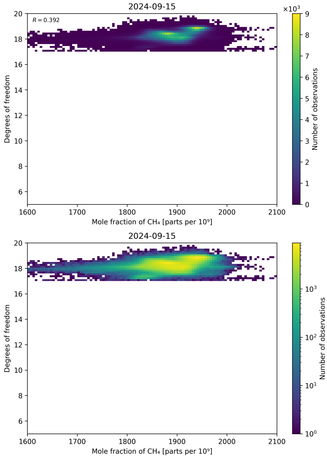
Figure 72: Scatter density plot of “Mole fraction of CH 4 ” against “Degrees of freedom” for 2024-09-14 to 2024-09-16.
