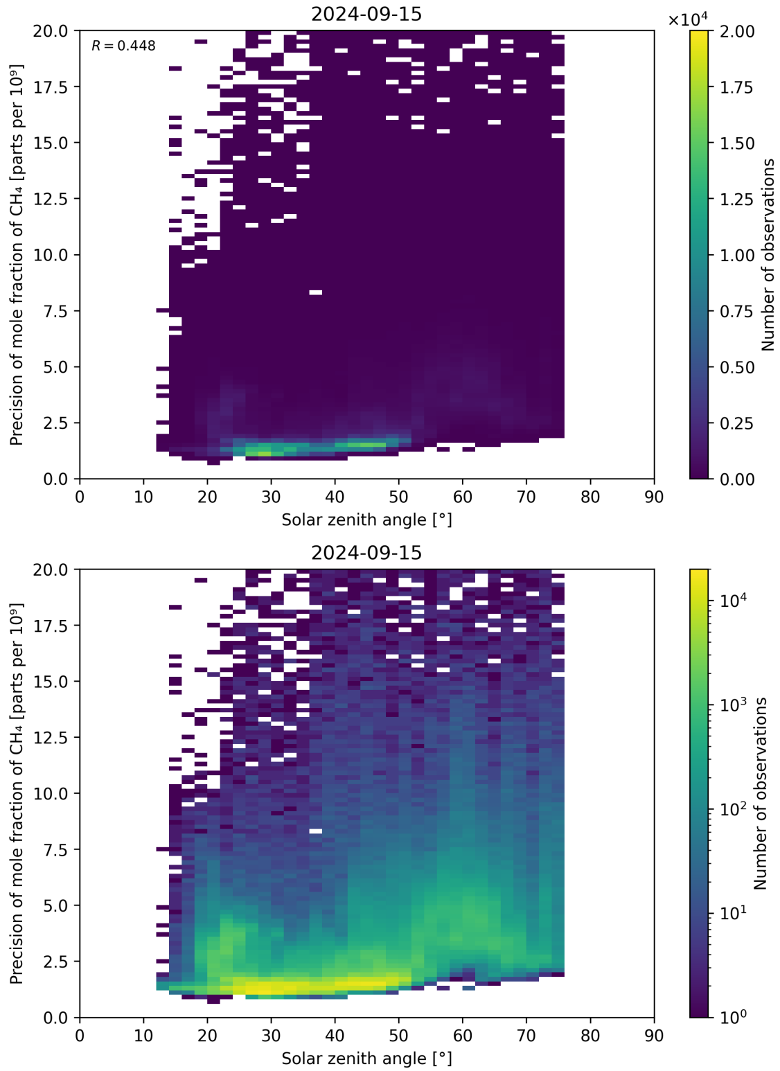
Figure 101: Scatter density plot of “Solar zenith angle” against “Precision of mole fraction of CH 4 ” for 2024-09-14 to 2024-09-16.
