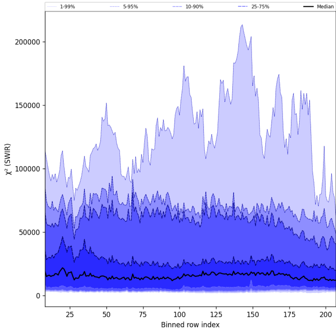
Figure 39: Along track statistics of “ \chi^2 (SWIR)” for 2024-09-14 to 2024-09-16
