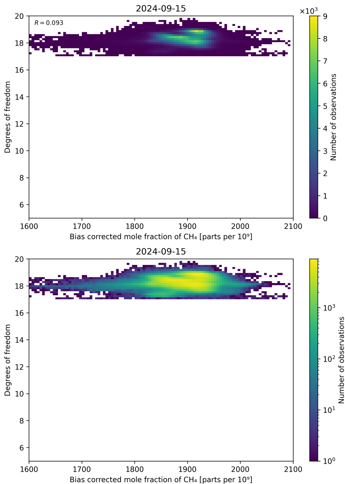
Figure 65: Scatter density plot of “Bias corrected mole fraction of CH 4 ” against “Degrees of freedom” for 2024-09-14 to 2024-09-16.
