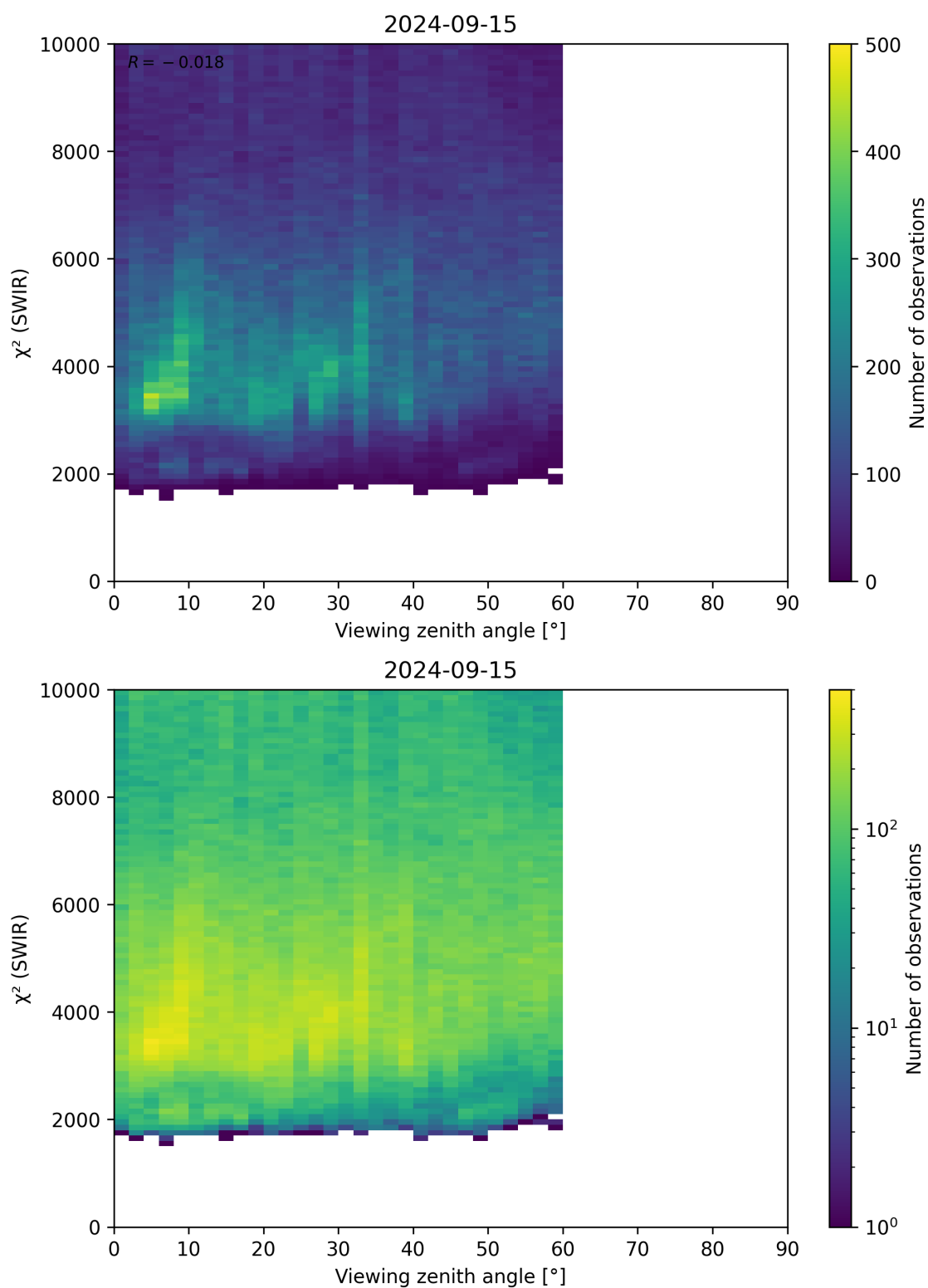
Figure 106: Scatter density plot of “Viewing zenith angle” against “ \chi^2 (SWIR)” for 2024-09-14 to 2024-09-16.
