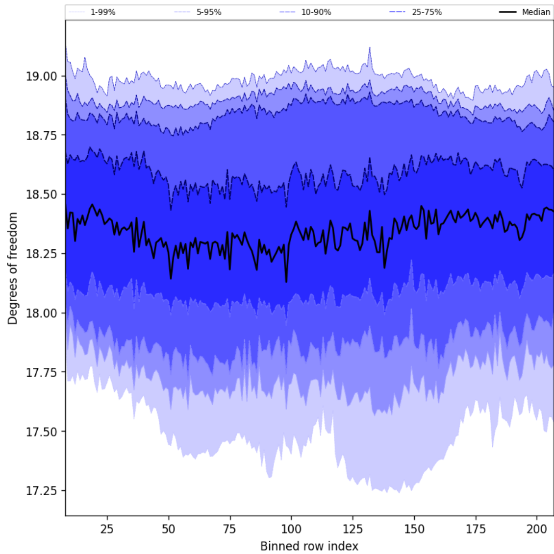
Figure 41: Along track statistics of “Degrees of freedom” for 2024-09-14 to 2024-09-16
