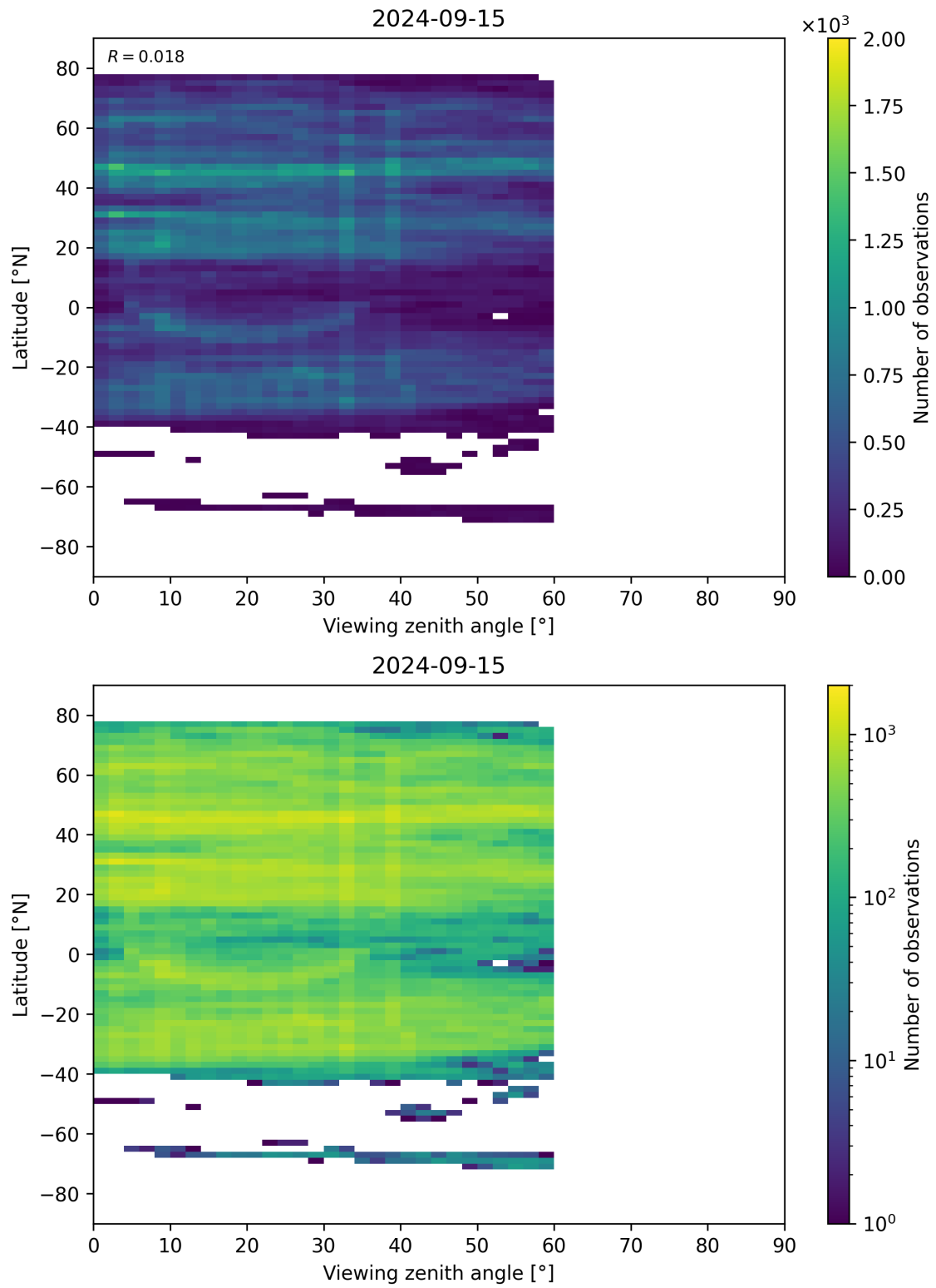
Figure 109: Scatter density plot of “Viewing zenith angle” against “Latitude” for 2024-09-14 to 2024-09-16.
