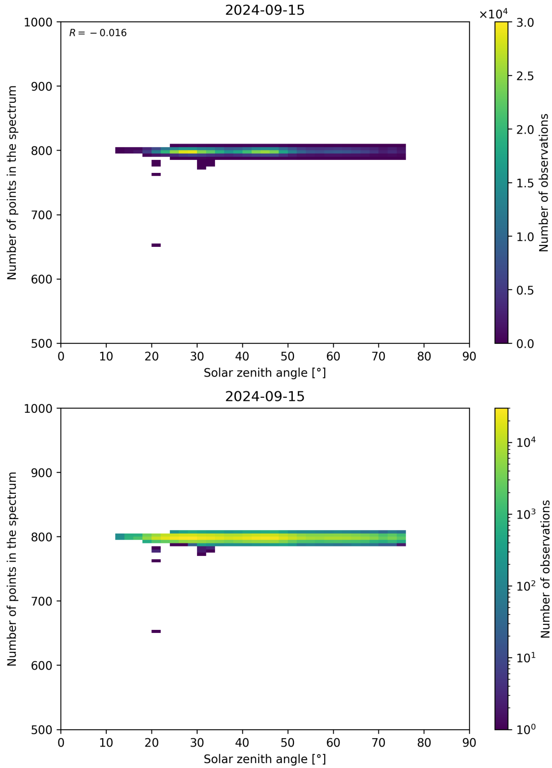
Figure 103: Scatter density plot of “Solar zenith angle” against “Number of points in the spectrum” for 2024-09-14 to 2024-09-16.
