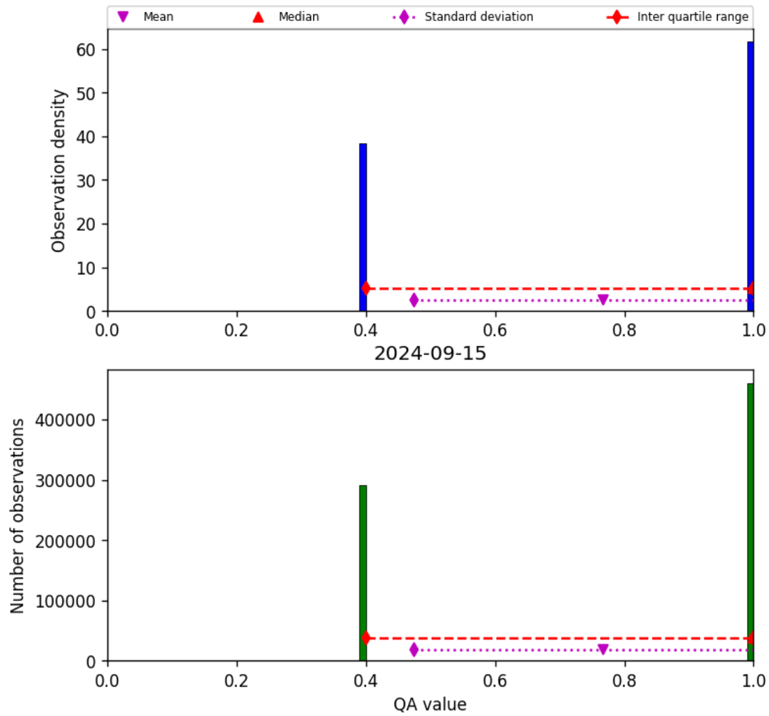
Figure 22: Histogram of “QA value” for 2024-09-14 to 2024-09-16
