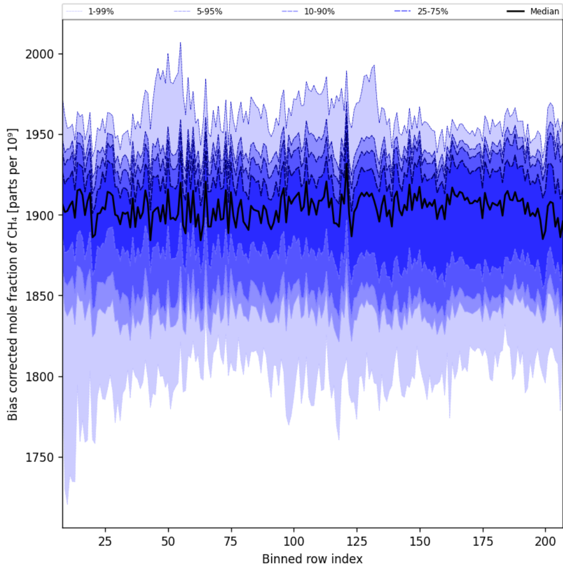
Figure 36: Along track statistics of “Bias corrected mole fraction of CH 4 ” for 2024-09-14 to 2024-09-16
