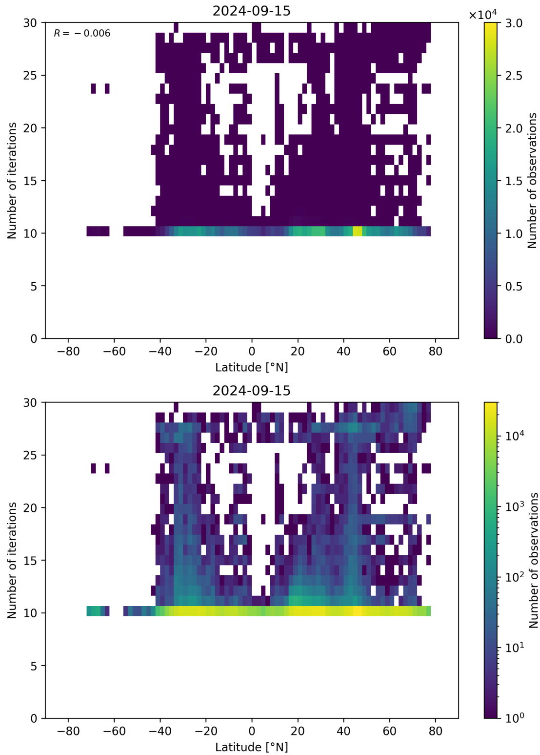
Figure 60: Scatter density plot of “Latitude” against “Number of iterations” for 2024-09-14 to 2024-09-16.
