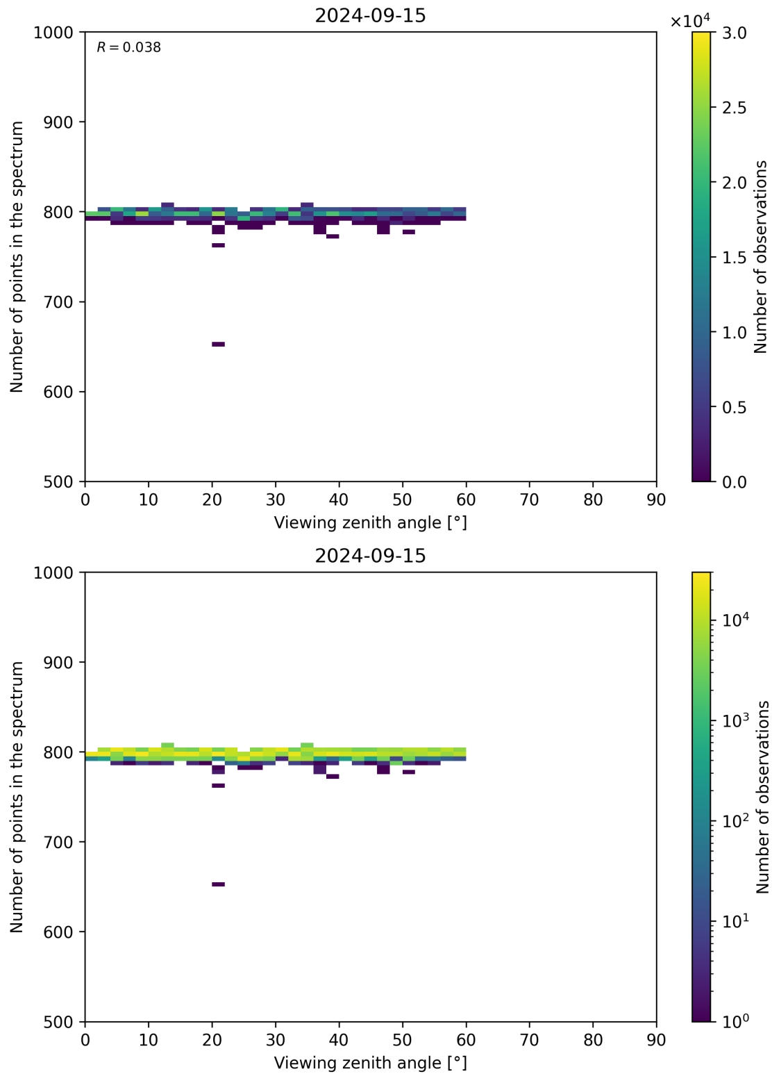
Figure 114: Scatter density plot of “Viewing zenith angle” against “Number of points in the spectrum” for 2024-09-14 to 2024-09-16.
