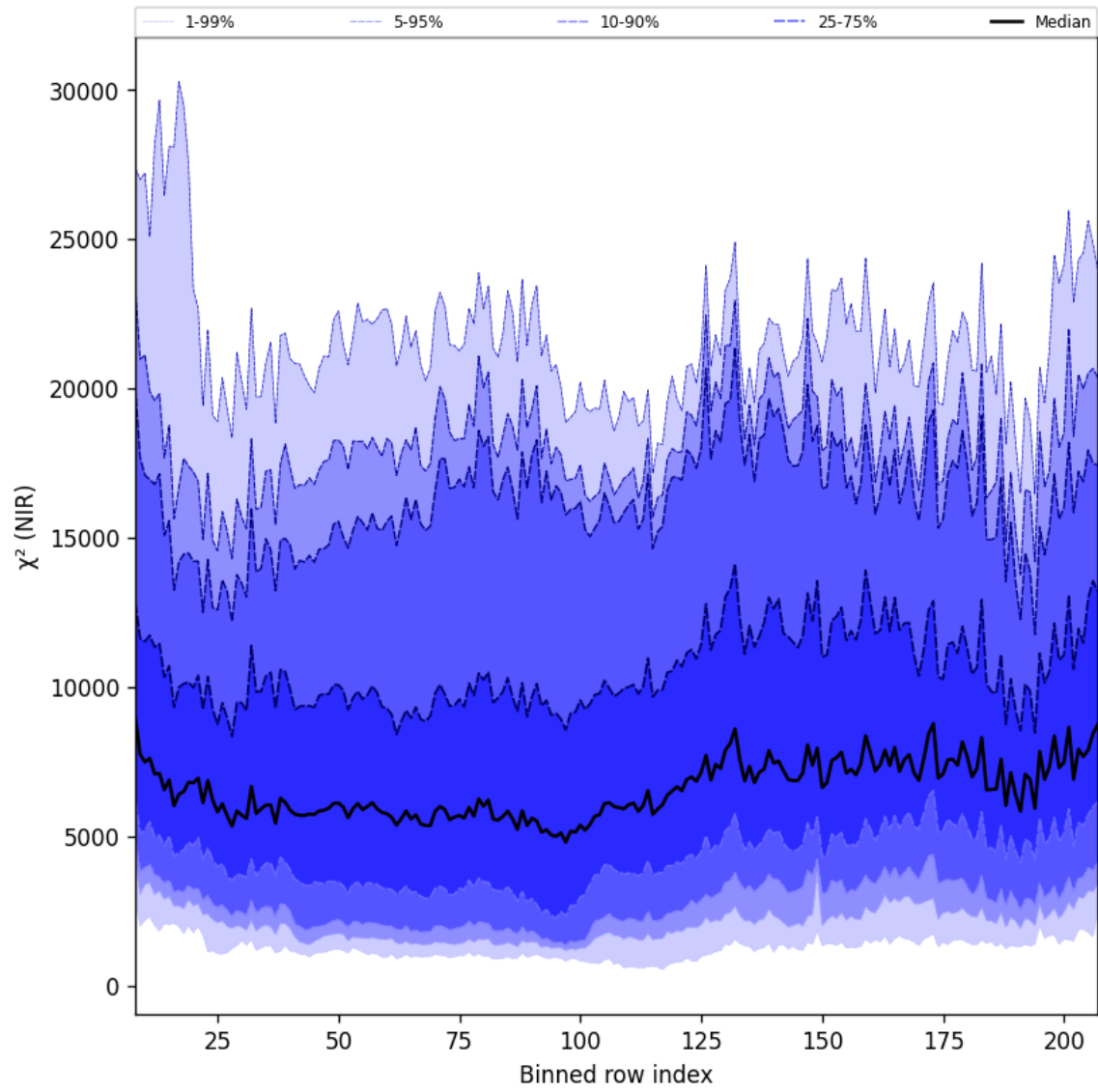
Figure 40: Along track statistics of “ \chi^2 (NIR)” for 2024-09-14 to 2024-09-16
