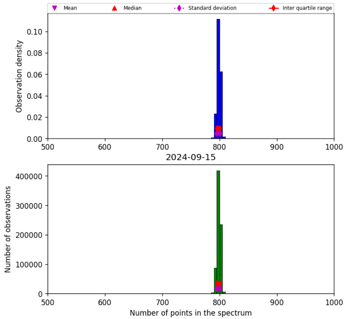
Figure 26: Histogram of “Number of points in the spectrum” for 2024-09-14 to 2024-09-16
