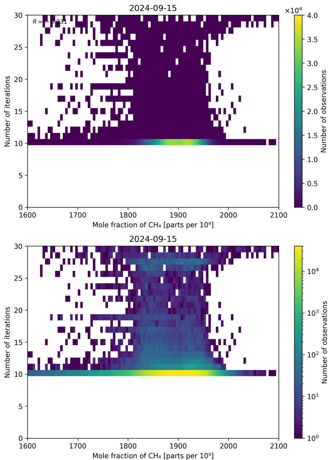
Figure 76: Scatter density plot of “Mole fraction of CH 4 ” against “Number of iterations” for 2024-09-14 to 2024-09-16.
