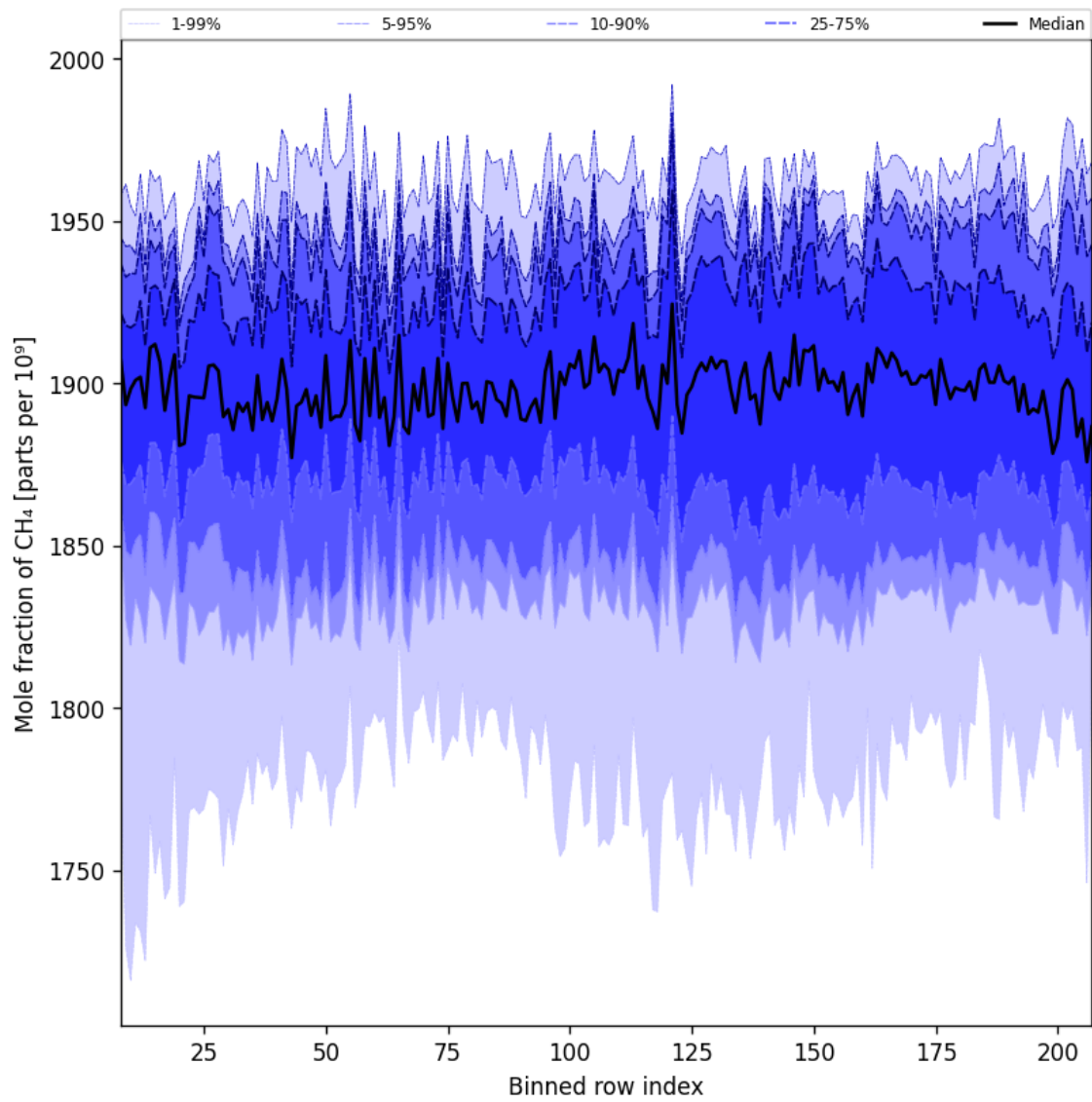
Figure 34: Along track statistics of “Mole fraction of CH 4 ” for 2024-09-14 to 2024-09-16
