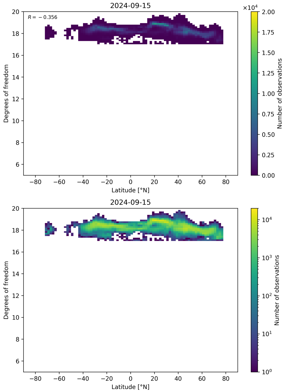
Figure 55: Scatter density plot of “Latitude” against “Degrees of freedom” for 2024-09-14 to 2024-09-16.
