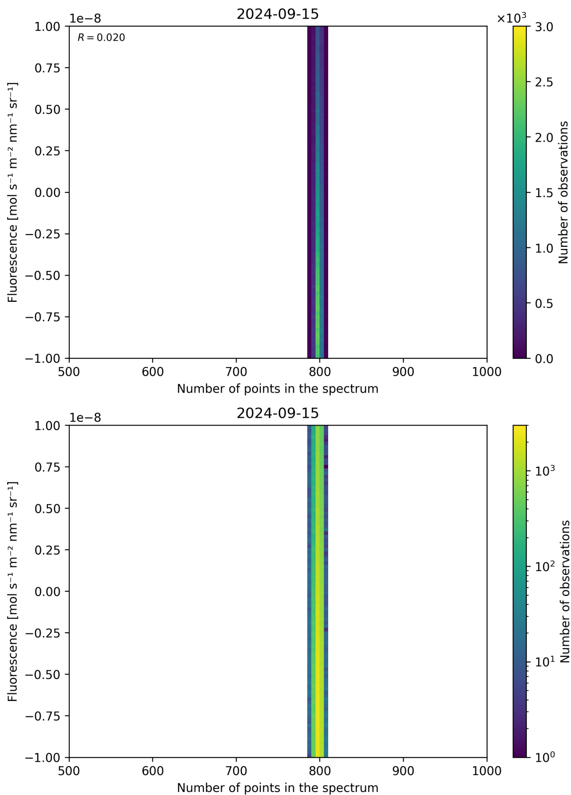
Figure 91: Scatter density plot of “Number of points in the spectrum” against “Fluorescence” for 2024-09-14 to 2024-09-16.
