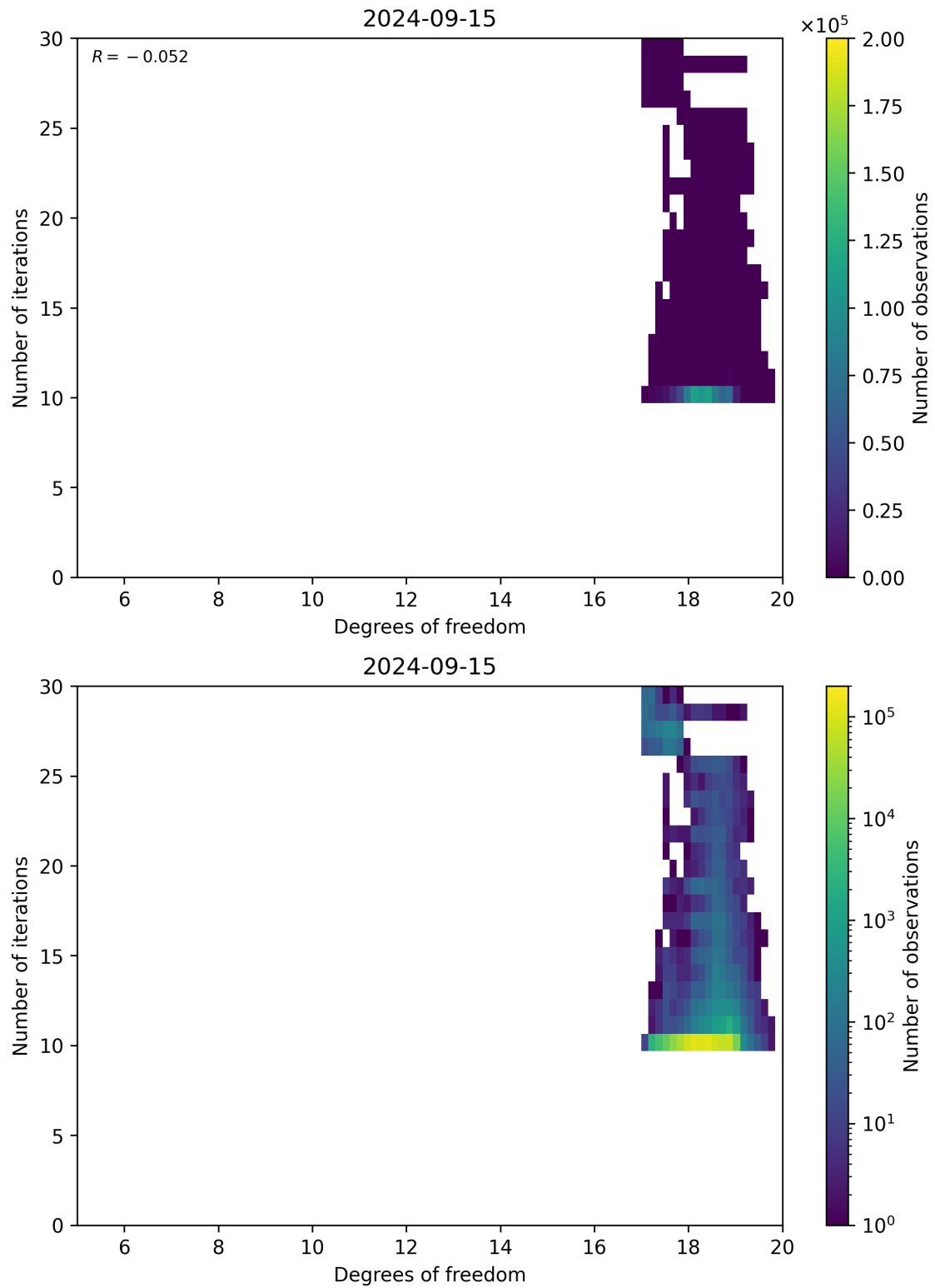
Figure 52: Scatter density plot of “Degrees of freedom” against “Number of iterations” for 2024-09-14 to 2024-09-16.
