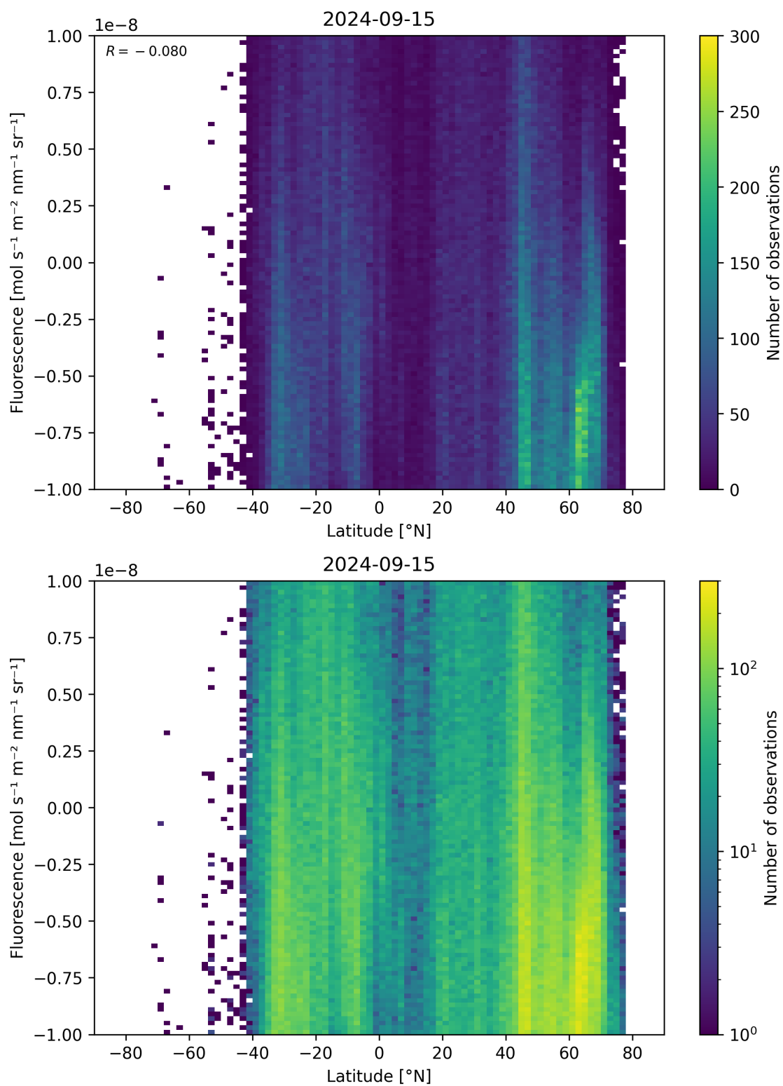
Figure 56: Scatter density plot of “Latitude” against “Fluorescence” for 2024-09-14 to 2024-09-16.
