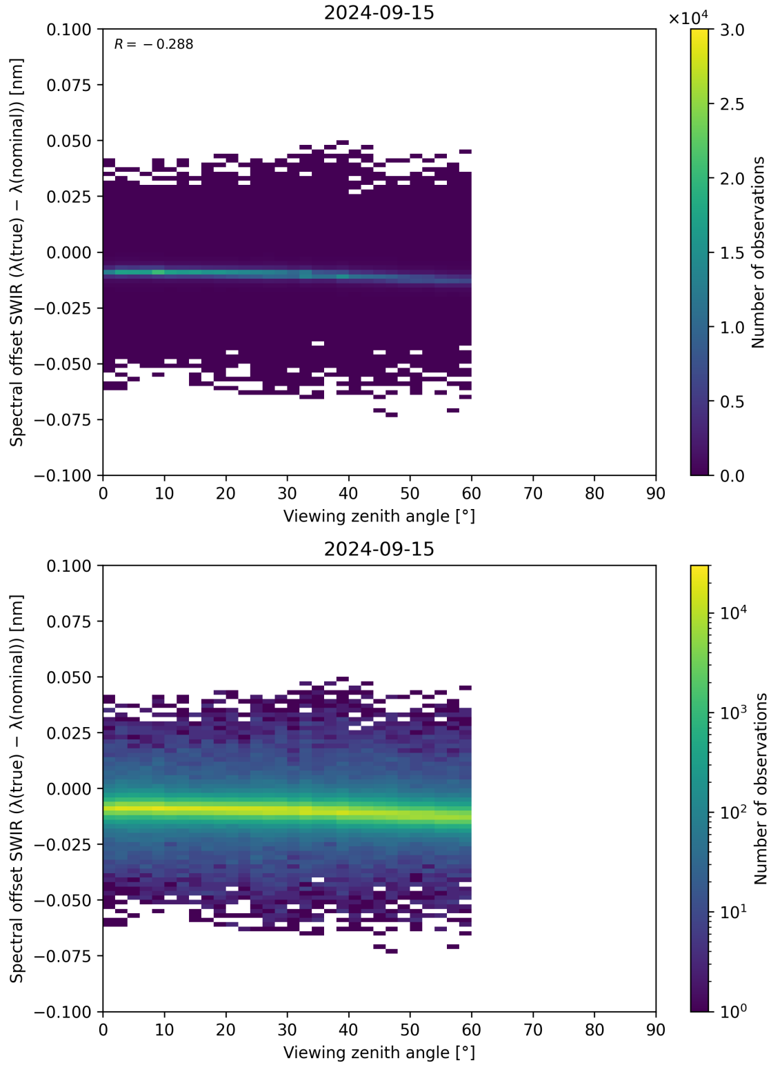
Figure 116: Scatter density plot of “Viewing zenith angle” against “Spectral offset SWIR ( \lambda_{\text{true}} - \lambda_{\text{nominal}} )” for 2024-09-14 to 2024-09-16.
