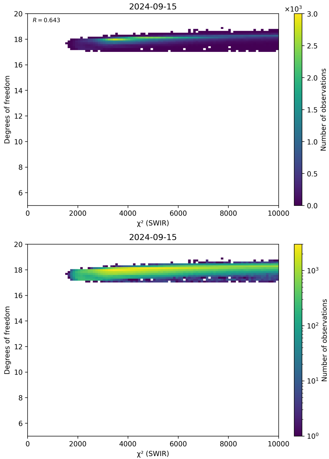
Figure 48: Scatter density plot of " \chi^2 (SWIR)" against "Degrees of freedom" for 2024-09-14 to 2024-09-16.
