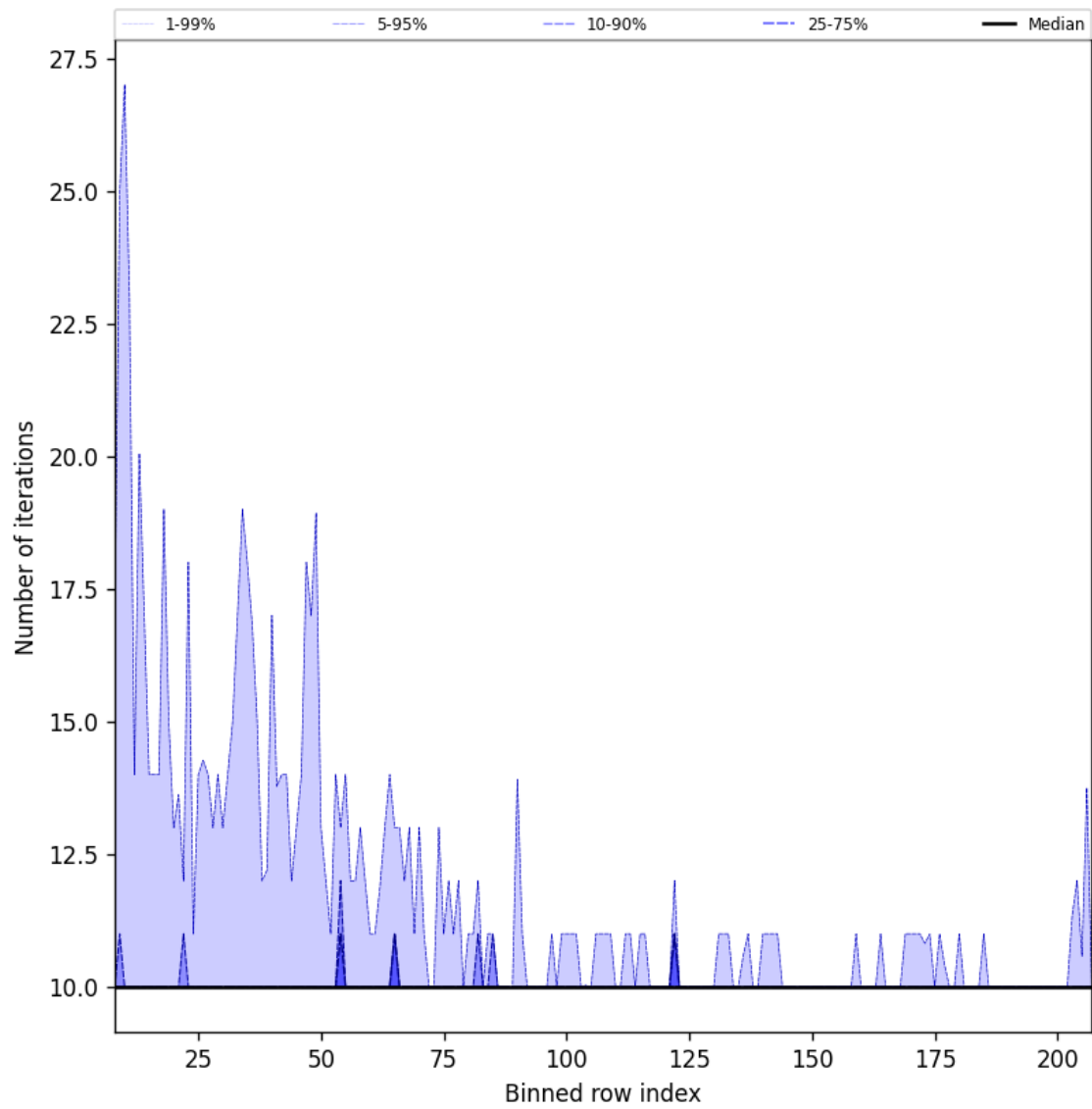
Figure 42: Along track statistics of “Number of iterations” for 2024-09-14 to 2024-09-16
