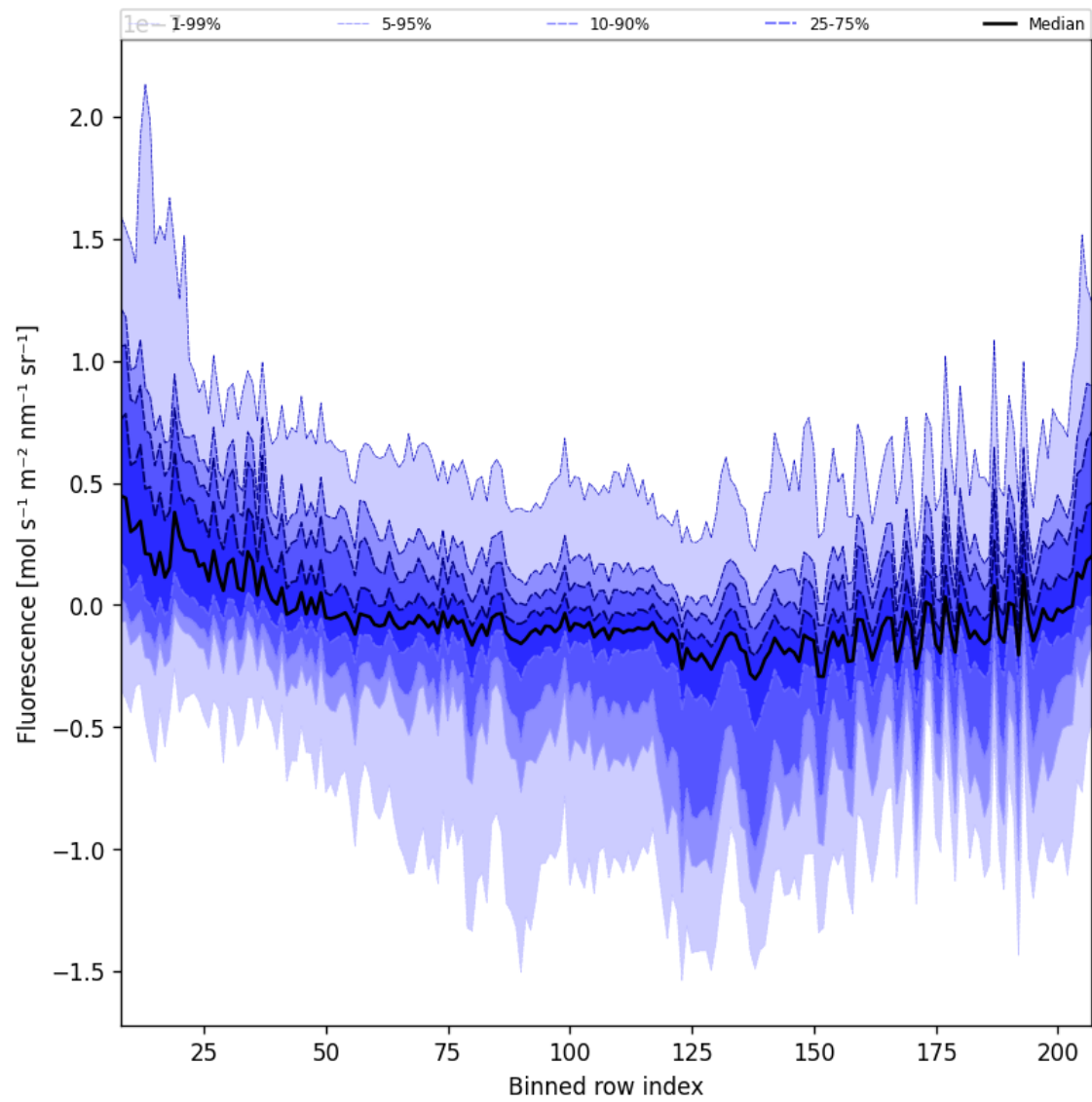
Figure 43: Along track statistics of “Fluorescence” for 2024-09-14 to 2024-09-16
