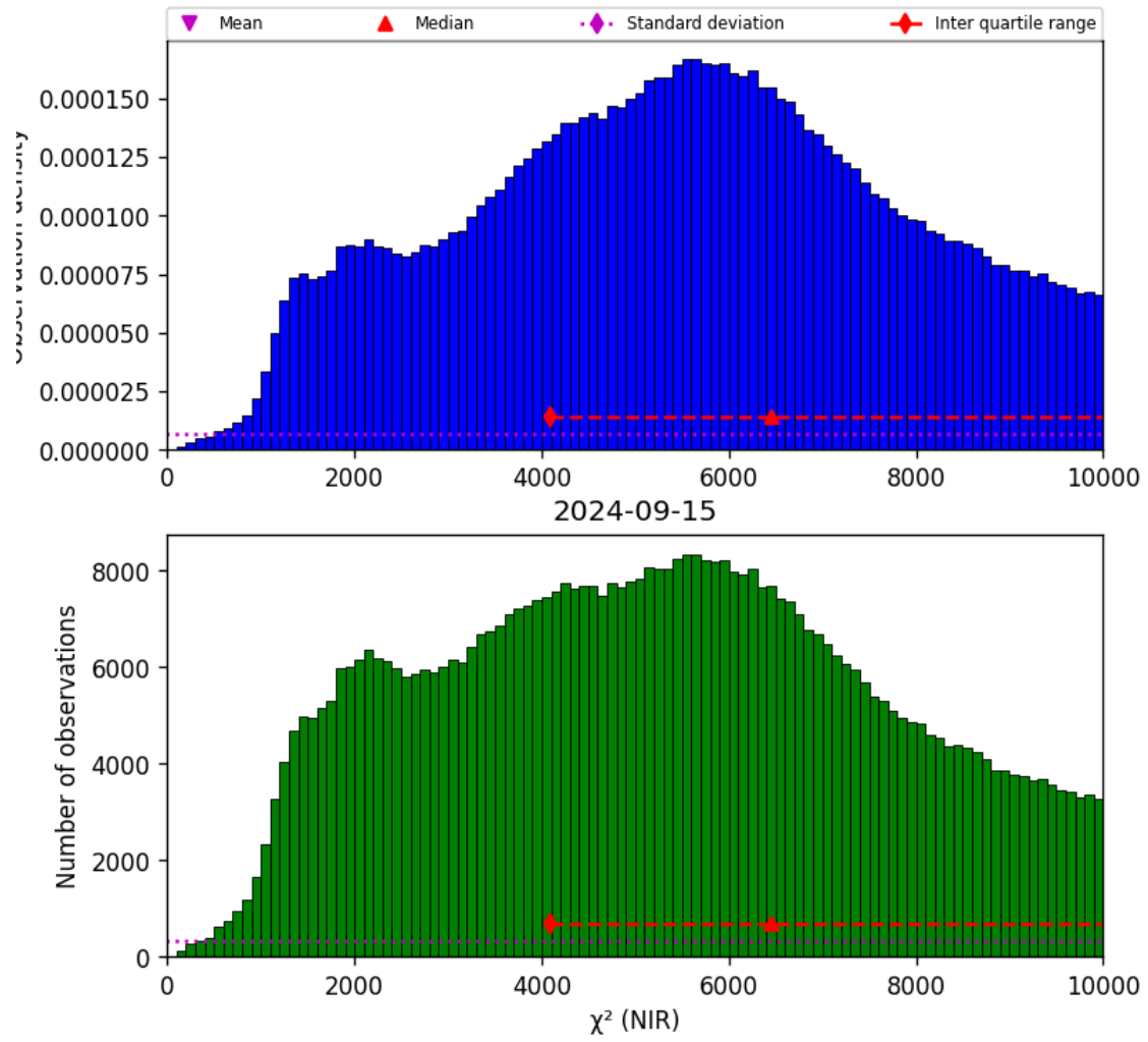
Figure 29: Histogram of “ \chi^2 (NIR)” for 2024-09-14 to 2024-09-16
