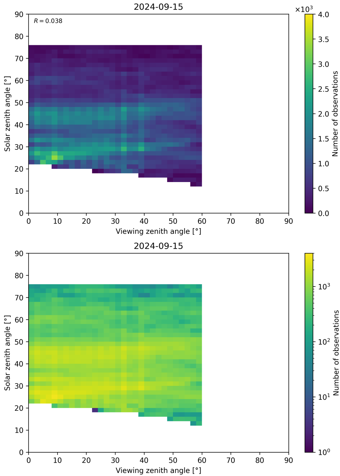
Figure 115: Scatter density plot of “Viewing zenith angle” against “Solar zenith angle” for 2024-09-14 to 2024-09-16.
