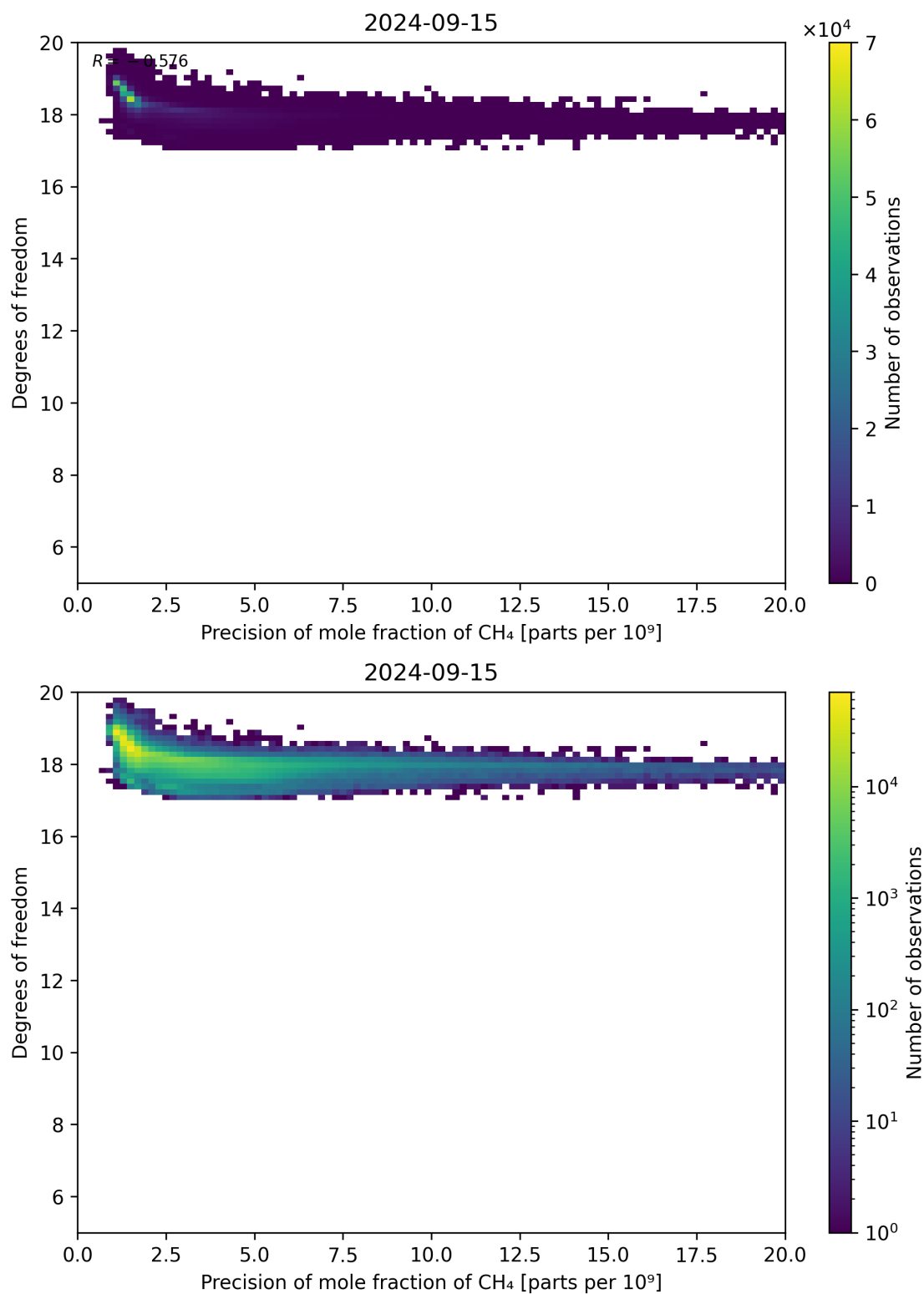
Figure 80: Scatter density plot of “Precision of mole fraction of CH 4 ” against “Degrees of freedom” for 2024-09-14 to 2024-09-16.
