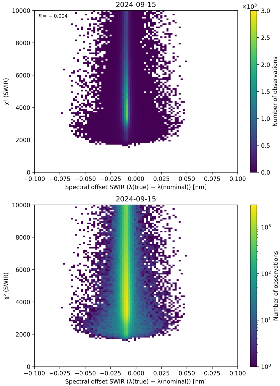
Figure 118: Scatter density plot of “Spectral offset SWIR ( \lambda_{\text{true}} - \lambda_{\text{nominal}} )” against “ \chi^2 (SWIR)” for 2024-09-14 to 2024-09-16.
