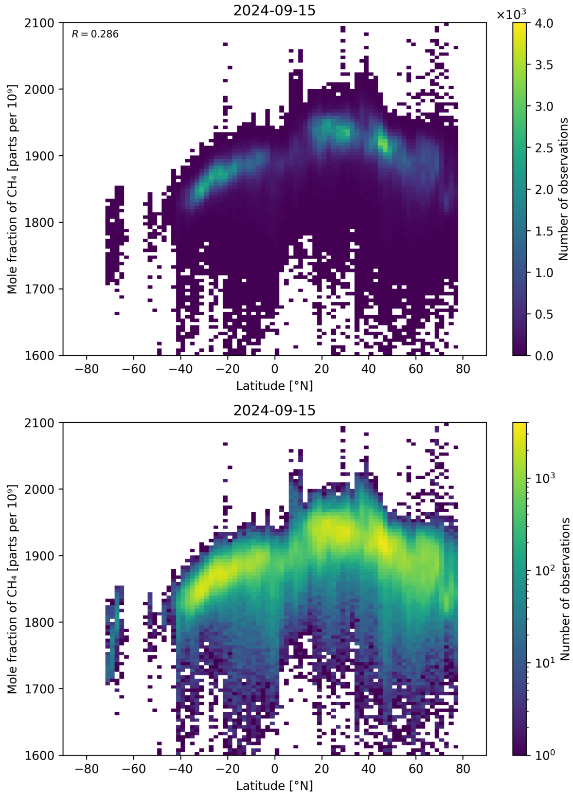
Figure 57: Scatter density plot of “Latitude” against “Mole fraction of \text{CH}_4 ” for 2024-09-14 to 2024-09-16.
