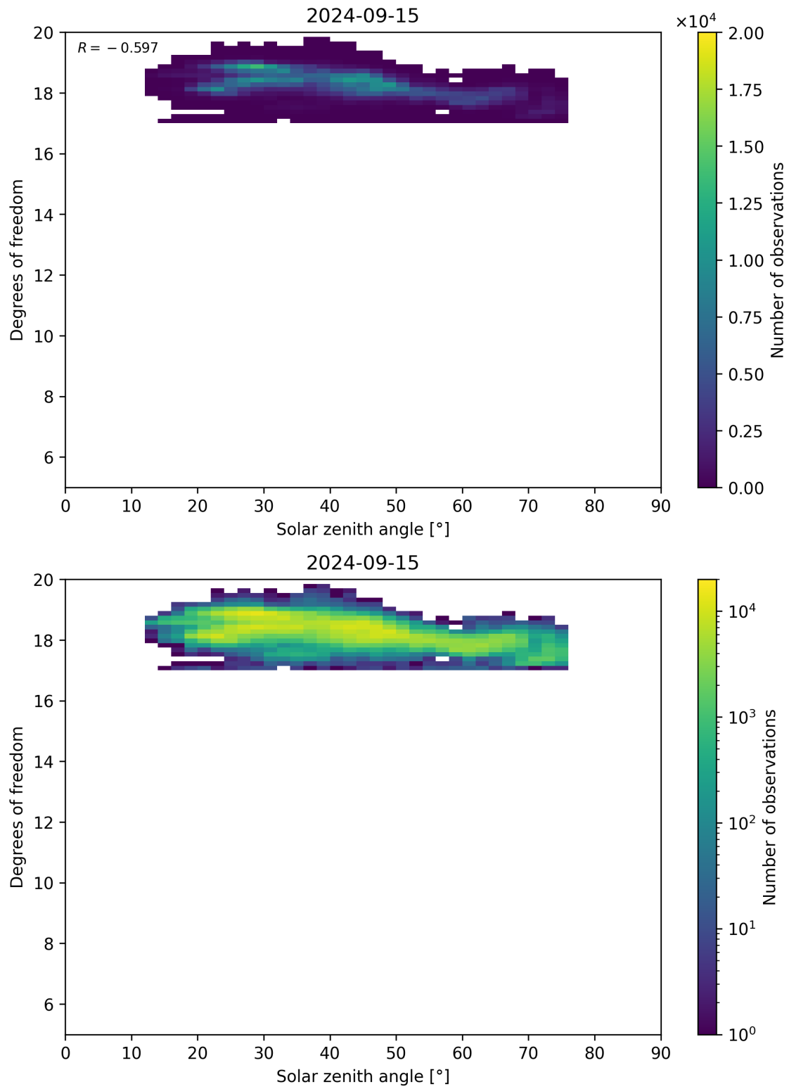
Figure 96: Scatter density plot of “Solar zenith angle” against “Degrees of freedom” for 2024-09-14 to 2024-09-16.
