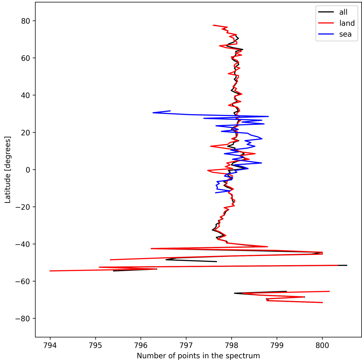
Figure 15: Zonal average of “Number of points in the spectrum” for 2024-09-14 to 2024-09-16.
