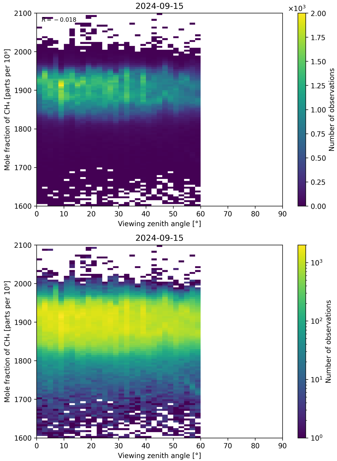
Figure 110: Scatter density plot of “Viewing zenith angle” against “Mole fraction of CH 4 ” for 2024-09-14 to 2024-09-16.
