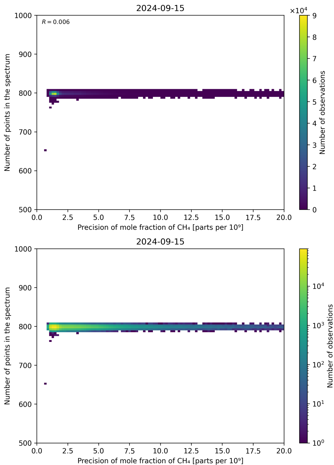
Figure 84: Scatter density plot of “Precision of mole fraction of CH 4 ” against “Number of points in the spectrum” for 2024-09-14 to 2024-09-16.
