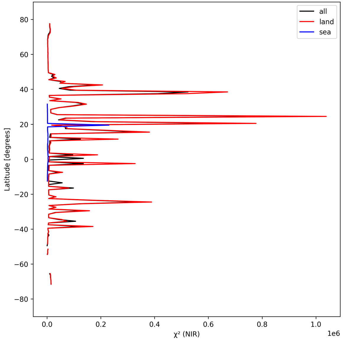
Figure 18: Zonal average of “ \chi^2 (NIR)” for 2024-09-14 to 2024-09-16.
