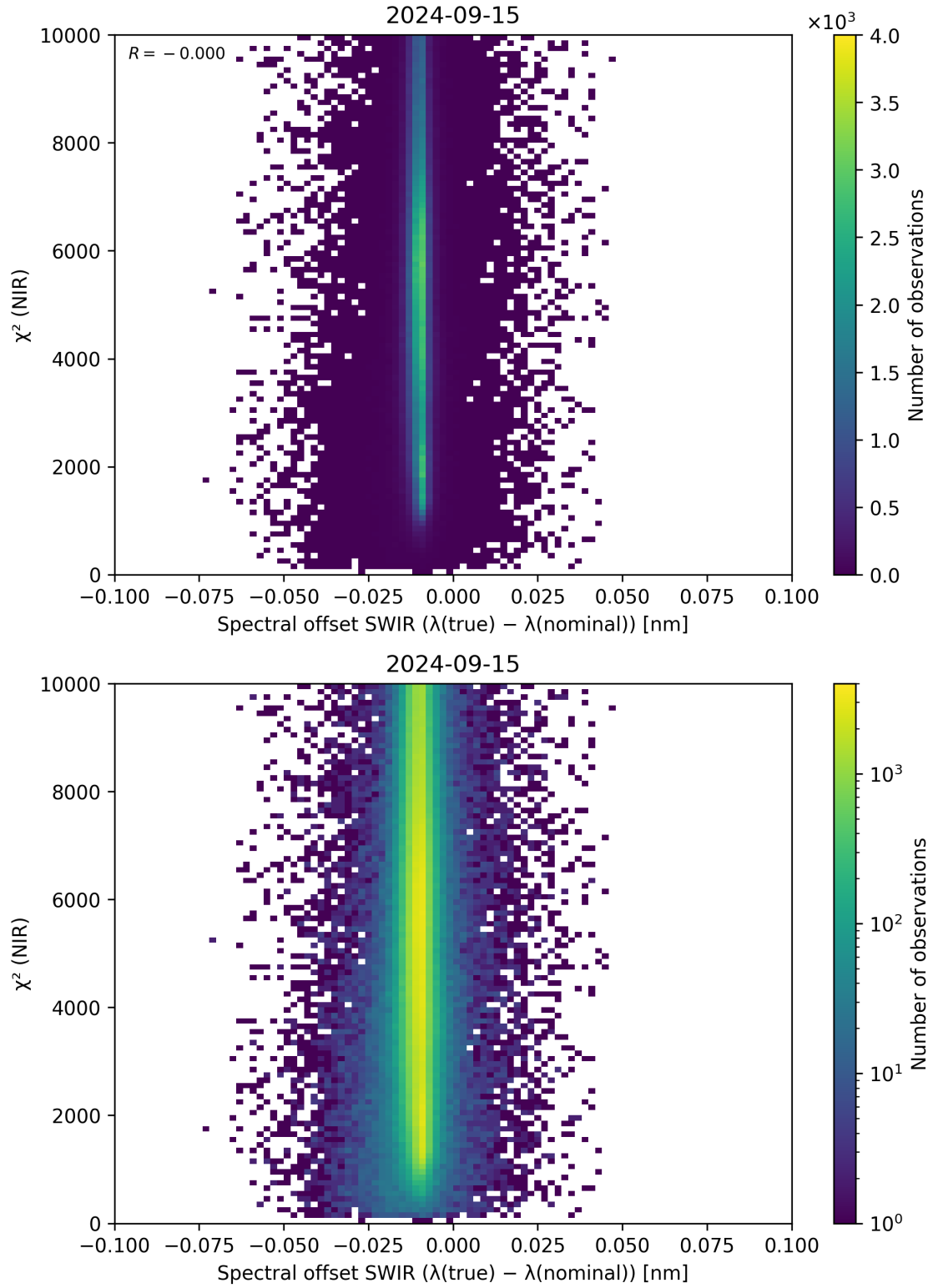
Figure 117: Scatter density plot of “Spectral offset SWIR ( \lambda_{\text{true}} - \lambda_{\text{nominal}} )” against “ \chi^2 (NIR)” for 2024-09-14 to 2024-09-16.
