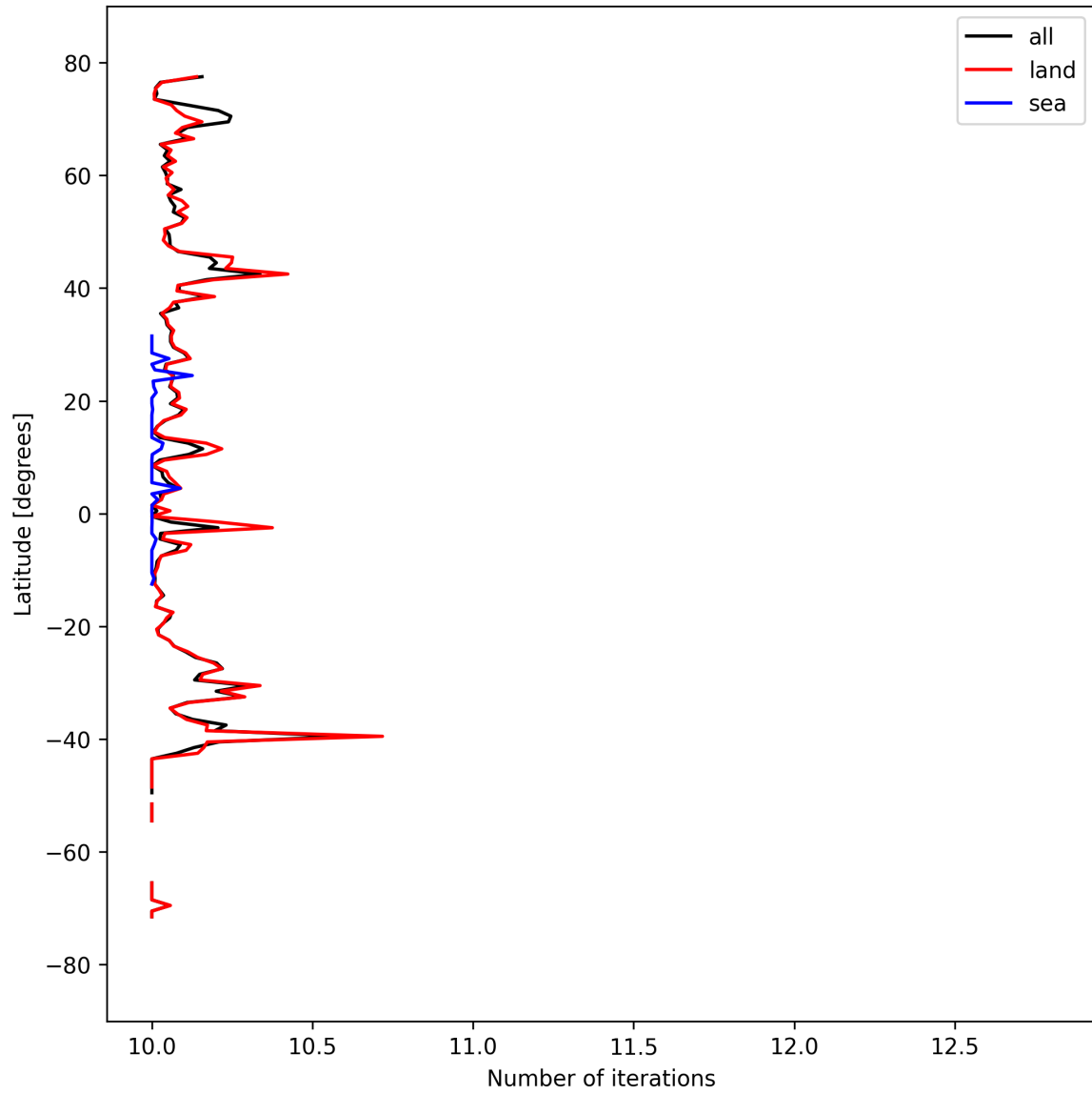
Figure 20: Zonal average of “Number of iterations” for 2024-09-14 to 2024-09-16.
