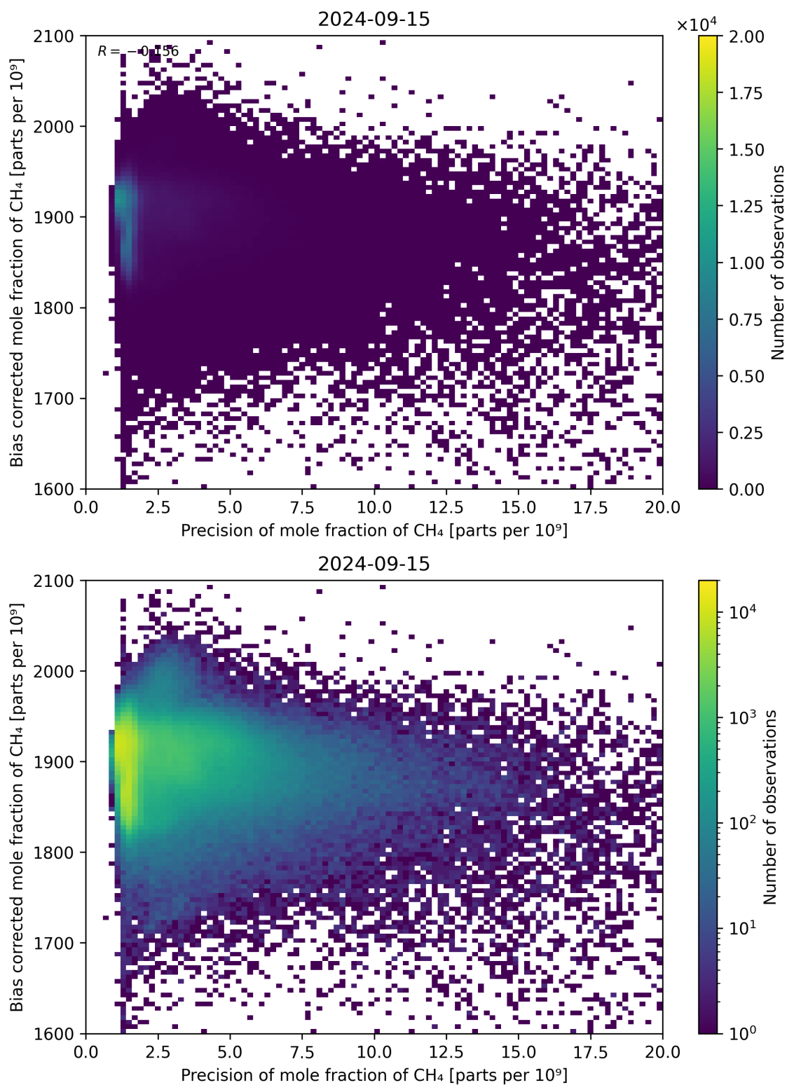
Figure 82: Scatter density plot of “Precision of mole fraction of CH 4 ” against “Bias corrected mole fraction of CH 4 ” for 2024-09-14 to 2024-09-16.
