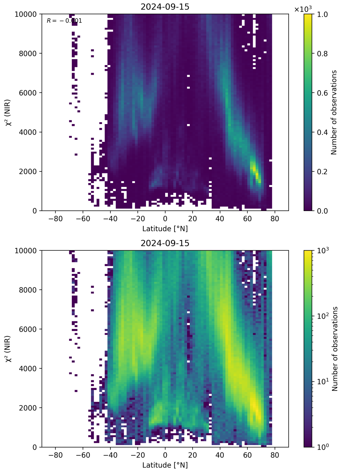
Figure 53: Scatter density plot of “Latitude” against “ \chi^2 (NIR)” for 2024-09-14 to 2024-09-16.
