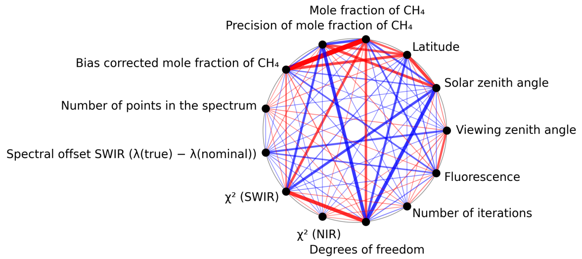
Figure 1: Map of correlation graph for 2024-09-14 to 2024-09-16.
