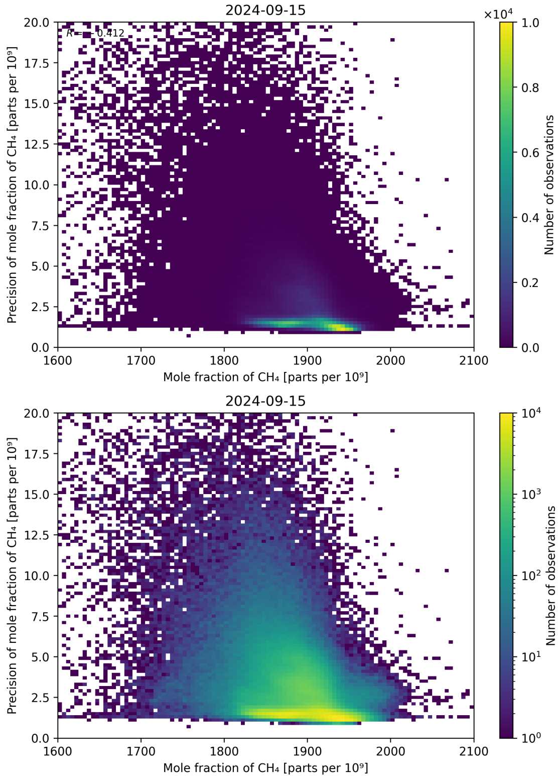
Figure 75: Scatter density plot of “Mole fraction of CH 4 ” against “Precision of mole fraction of CH 4 ” for 2024-09-14 to 2024-09-16.
