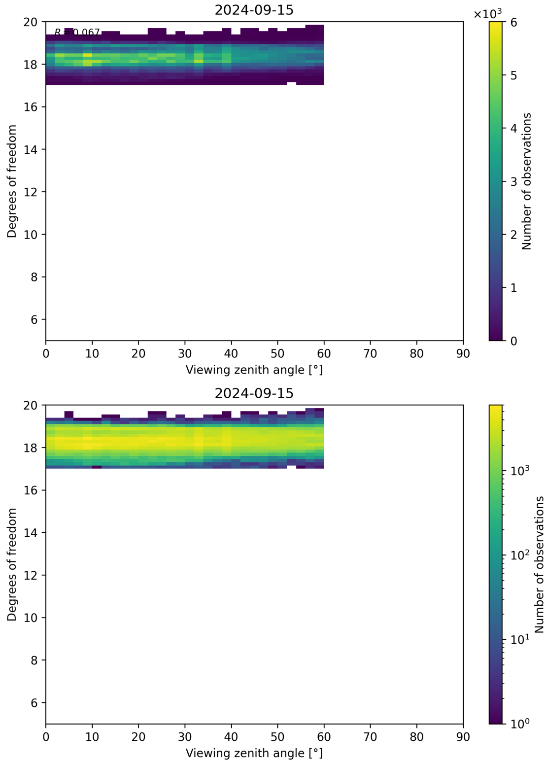
Figure 107: Scatter density plot of “Viewing zenith angle” against “Degrees of freedom” for 2024-09-14 to 2024-09-16.
