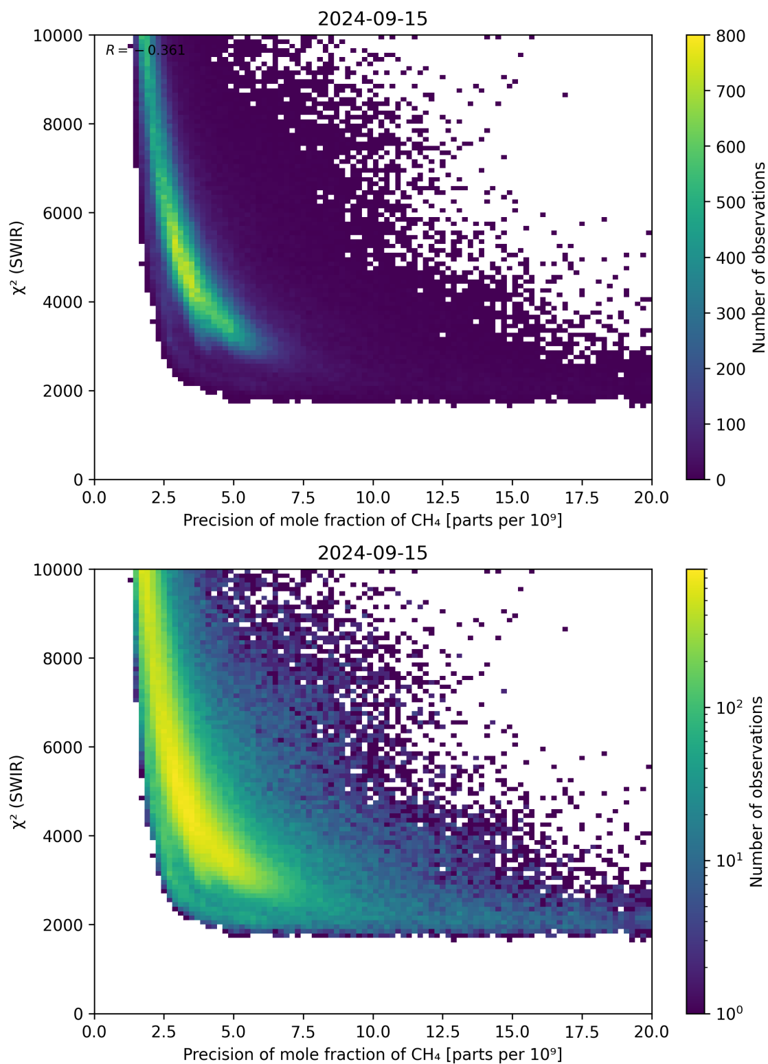
Figure 79: Scatter density plot of “Precision of mole fraction of \text{CH}_4 ” against “ \chi^2 (SWIR)” for 2024-09-14 to 2024-09-16.
