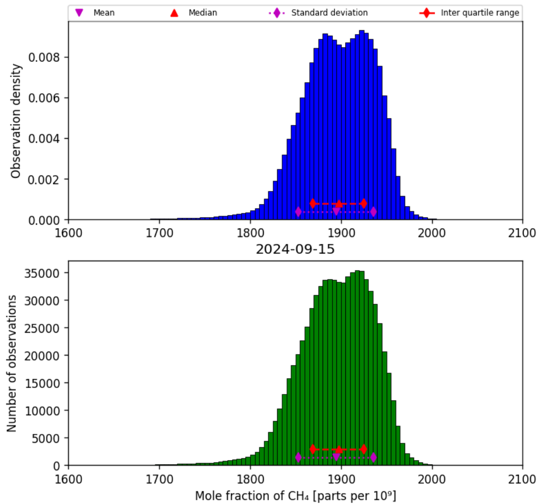
Figure 23: Histogram of “Mole fraction of CH 4 ” for 2024-09-14 to 2024-09-16
