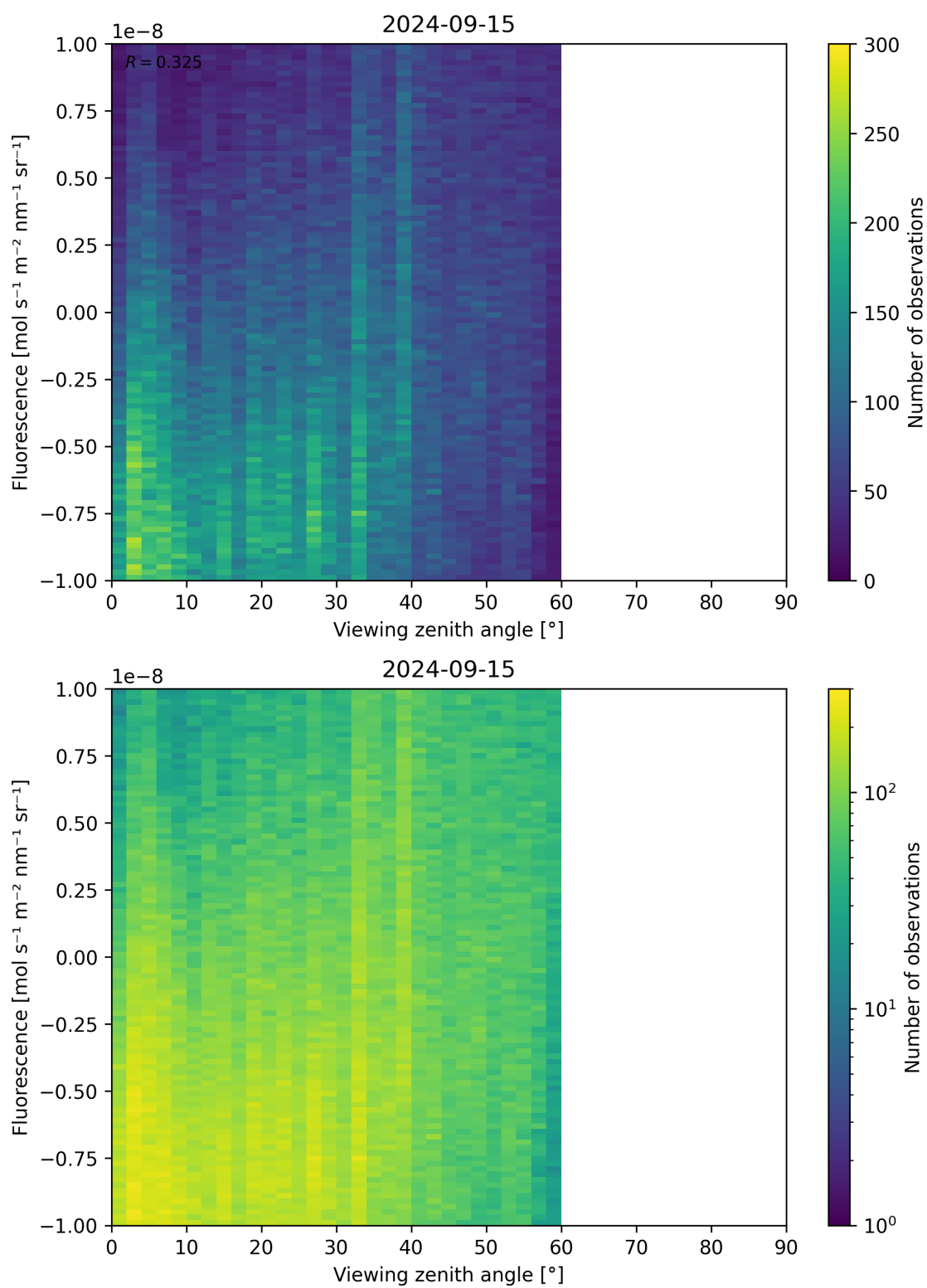
Figure 108: Scatter density plot of “Viewing zenith angle” against “Fluorescence” for 2024-09-14 to 2024-09-16.
