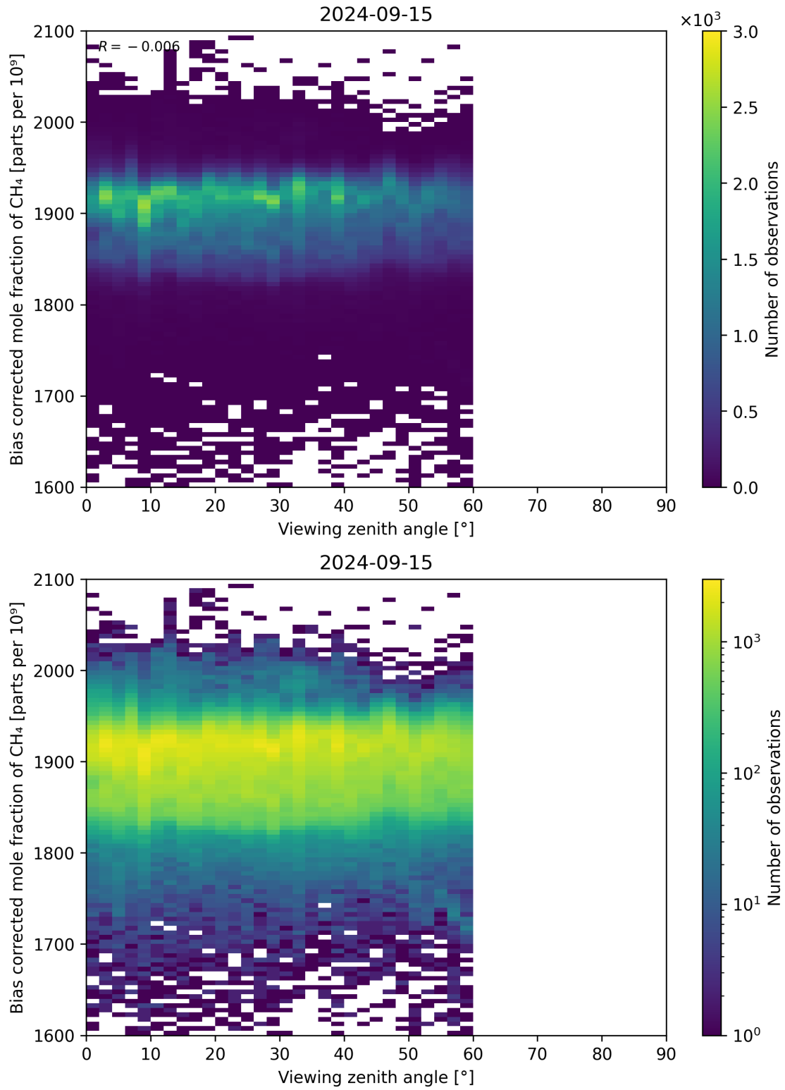
Figure 111: Scatter density plot of “Viewing zenith angle” against “Bias corrected mole fraction of CH 4 ” for 2024-09-14 to 2024-09-16.
