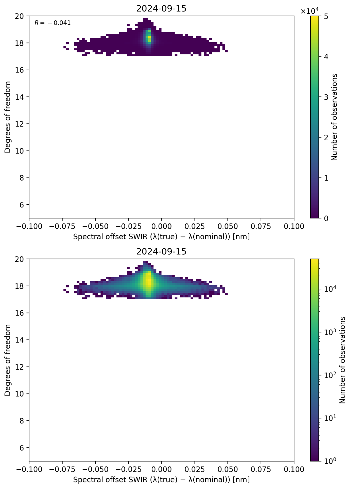
Figure 119: Scatter density plot of “Spectral offset SWIR ( \lambda_{\text{true}} - \lambda_{\text{nominal}} )” against “Degrees of freedom” for 2024-09-14 to 2024-09-16.
