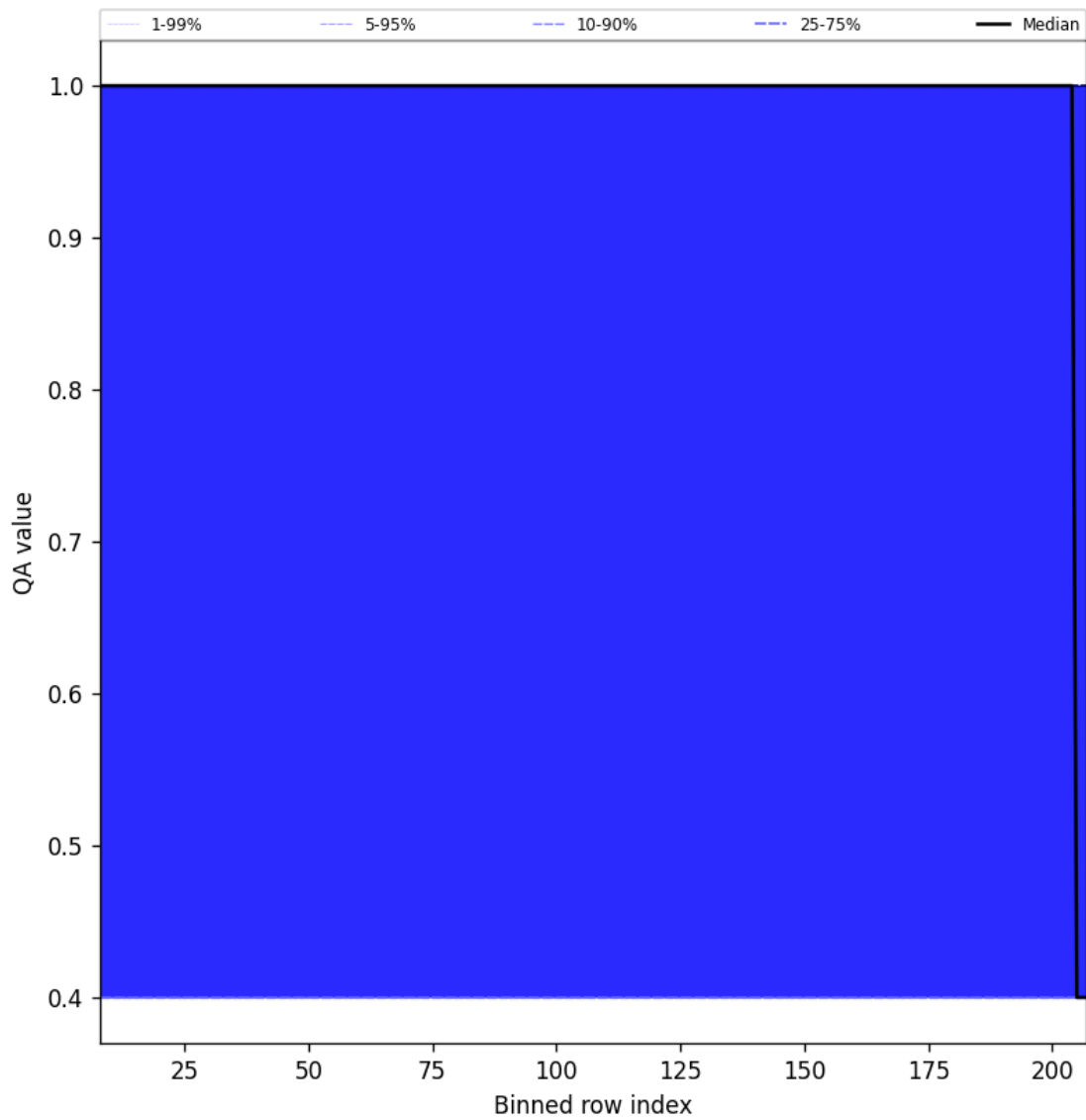
Figure 33: Along track statistics of “QA value” for 2024-09-14 to 2024-09-16
