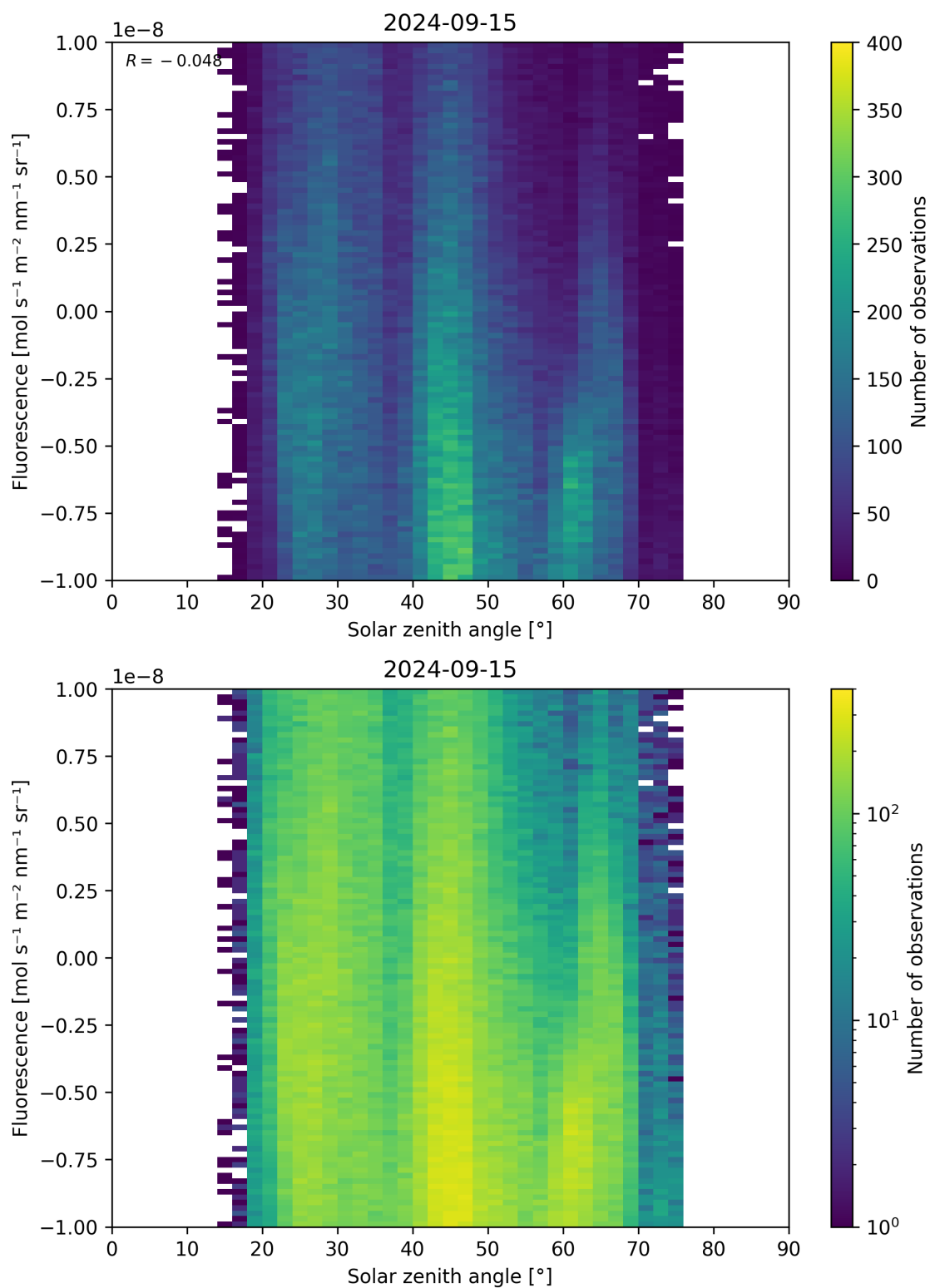
Figure 97: Scatter density plot of “Solar zenith angle” against “Fluorescence” for 2024-09-14 to 2024-09-16.
