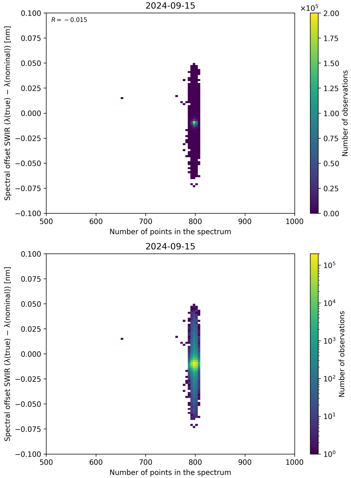
Figure 93: Scatter density plot of “Number of points in the spectrum” against “Spectral offset SWIR ( \lambda_{\text{true}} - \lambda_{\text{nominal}} )” for 2024-09-14 to 2024-09-16.
