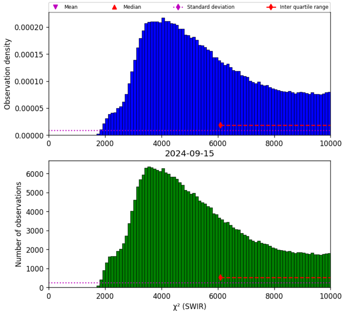
Figure 28: Histogram of “ \chi^2 (SWIR)” for 2024-09-14 to 2024-09-16
