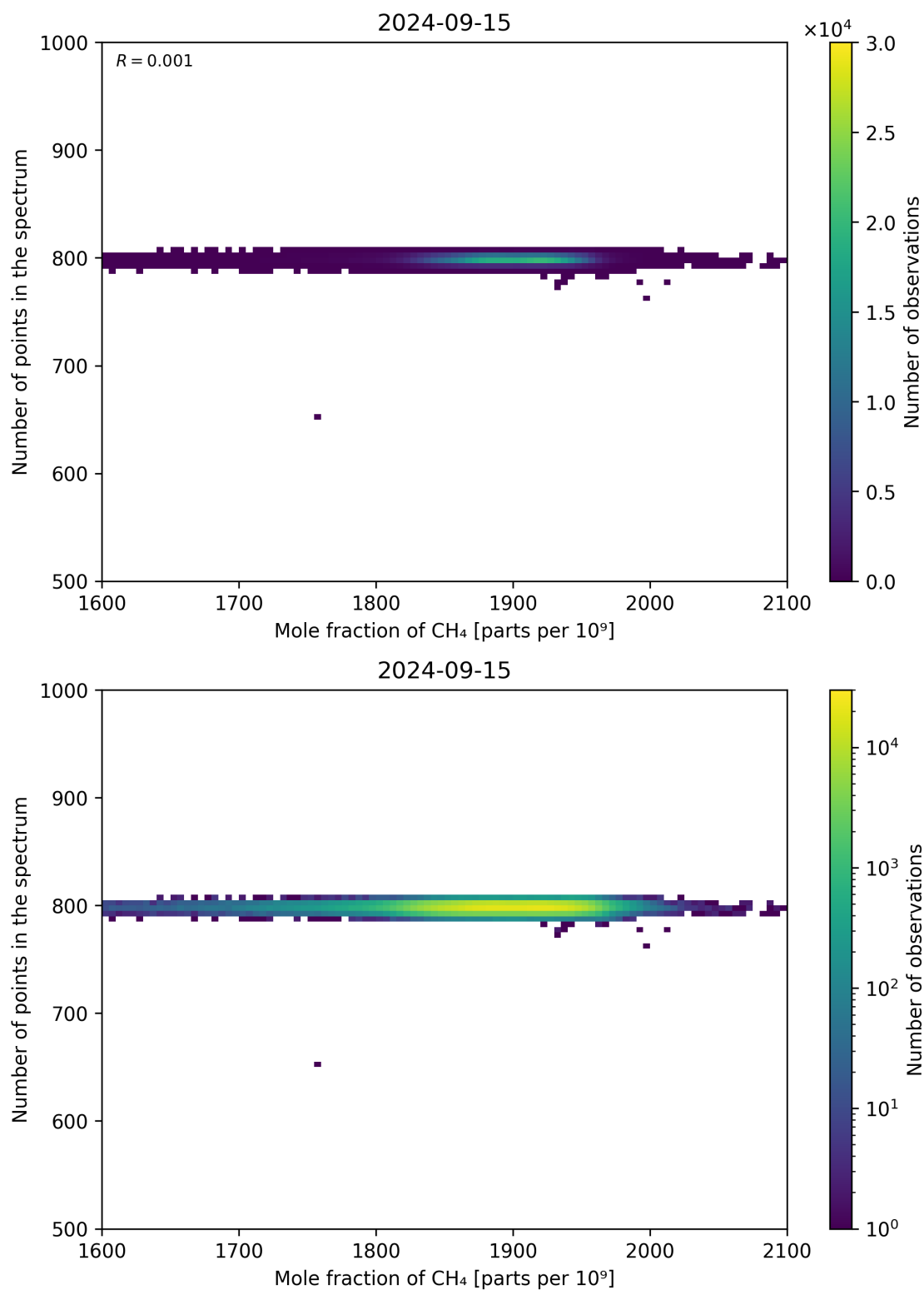
Figure 77: Scatter density plot of “Mole fraction of CH 4 ” against “Number of points in the spectrum” for 2024-09-14 to 2024-09-16.
