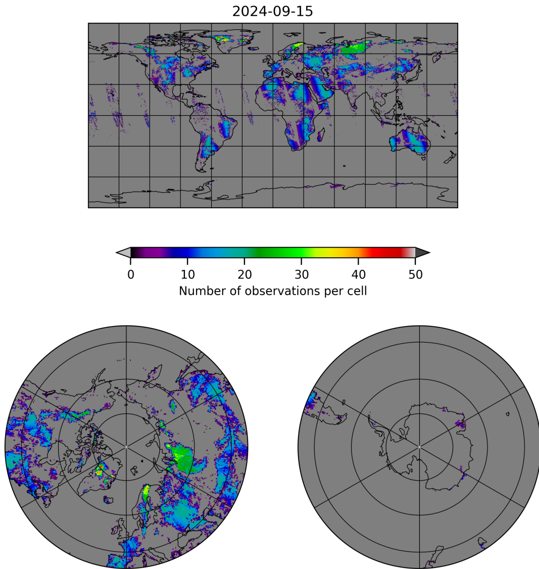
Figure 10: Map of the number of observations for 2024-09-14 to 2024-09-16
