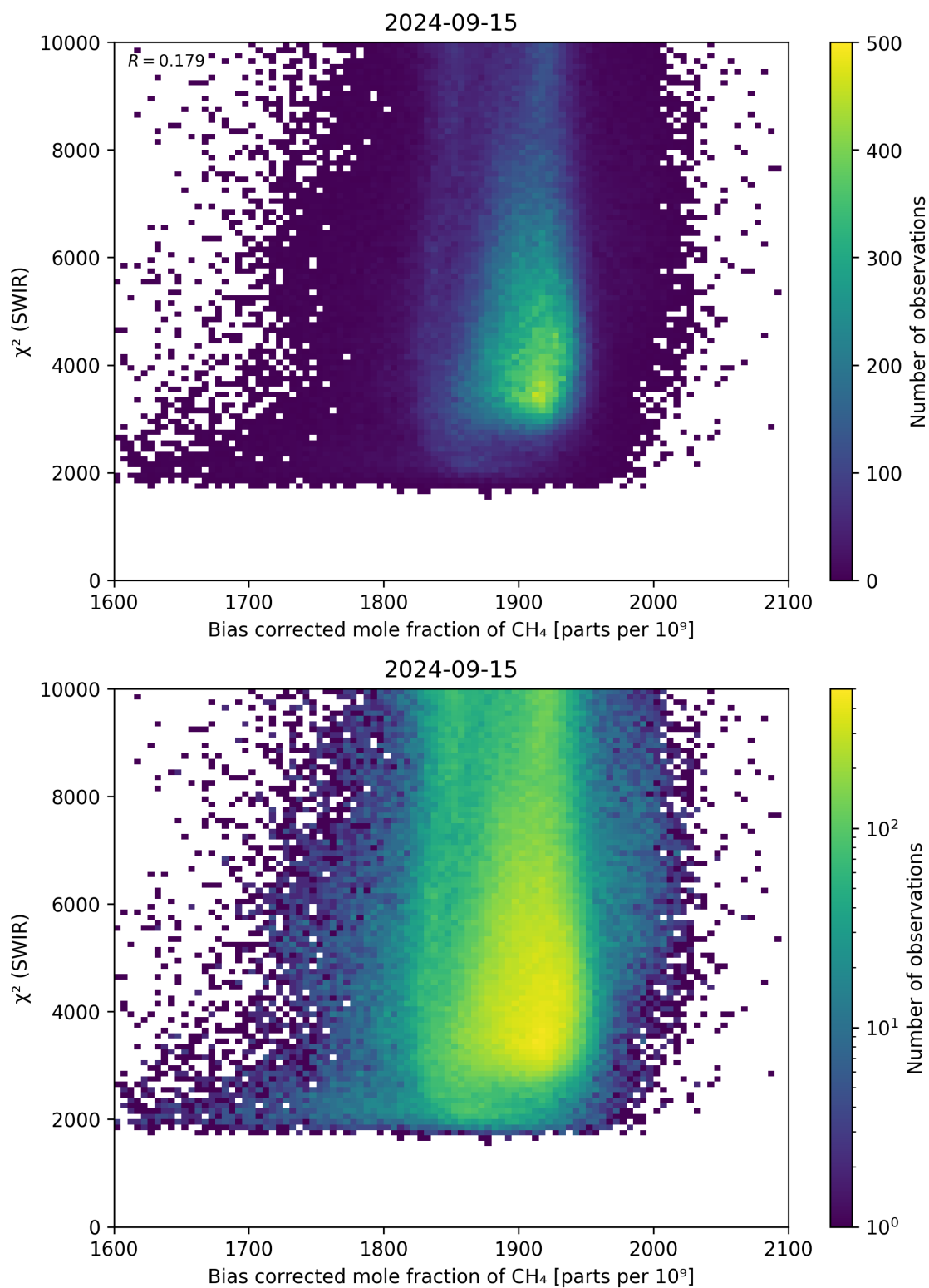
Figure 64: Scatter density plot of “Bias corrected mole fraction of \text{CH}_4 ” against “ \chi^2 (SWIR)” for 2024-09-14 to 2024-09-16.
