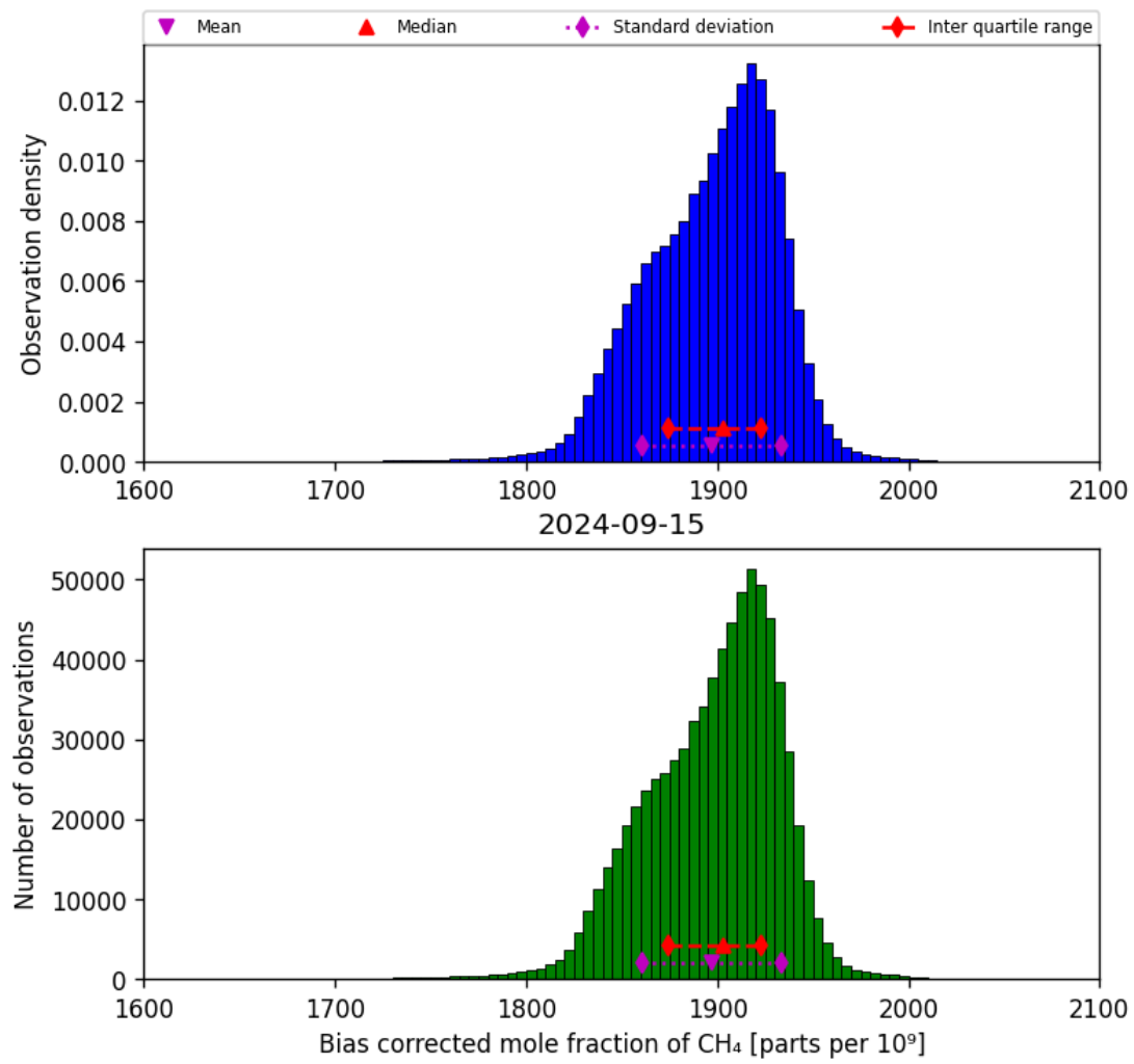
Figure 25: Histogram of “Bias corrected mole fraction of CH 4 ” for 2024-09-14 to 2024-09-16
