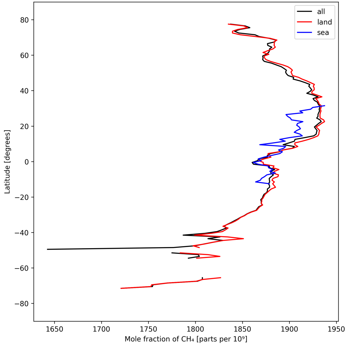
Figure 12: Zonal average of “Mole fraction of \text{CH}_4 ” for 2024-09-14 to 2024-09-16.
