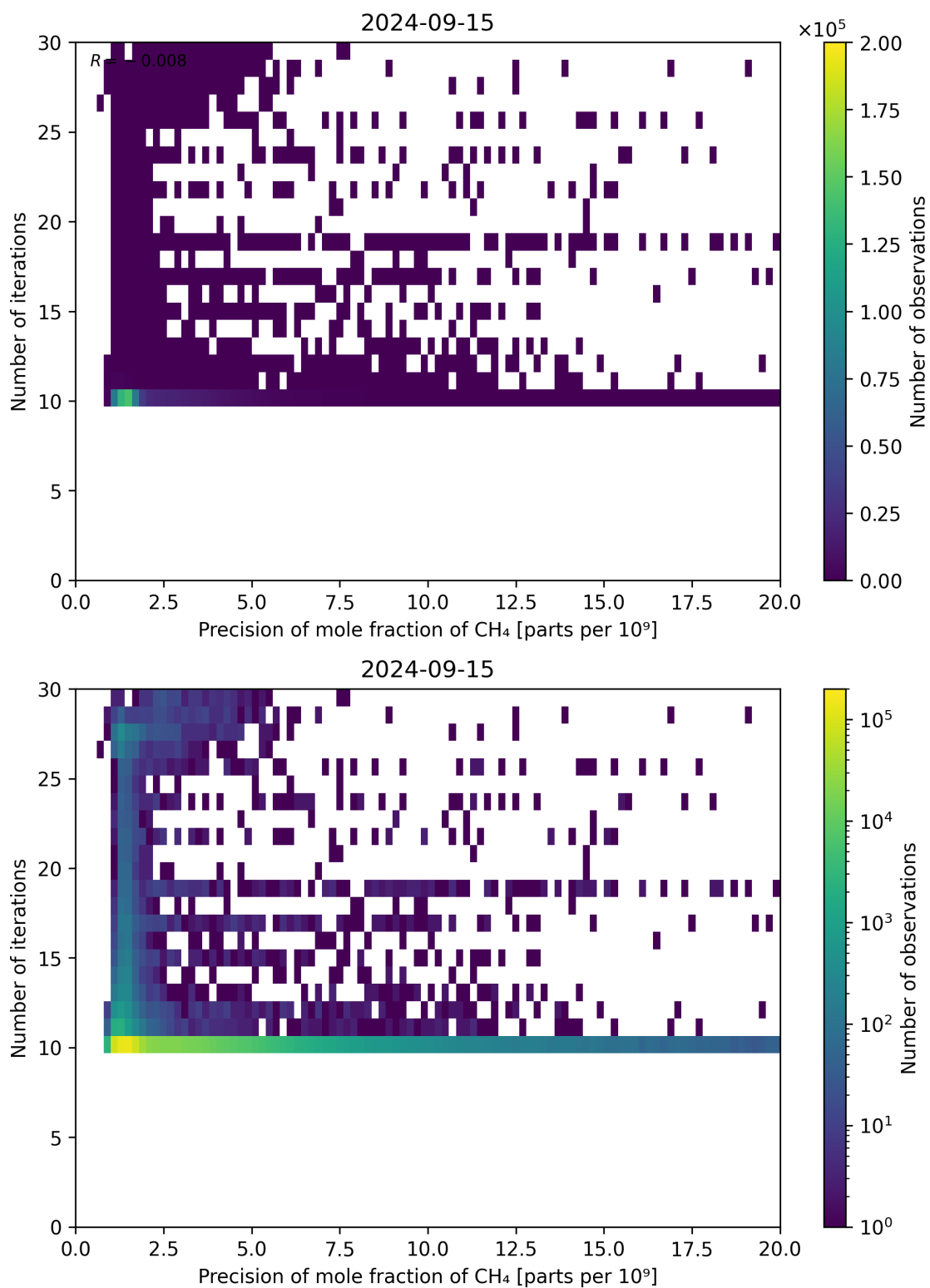
Figure 83: Scatter density plot of “Precision of mole fraction of CH 4 ” against “Number of iterations” for 2024-09-14 to 2024-09-16.
