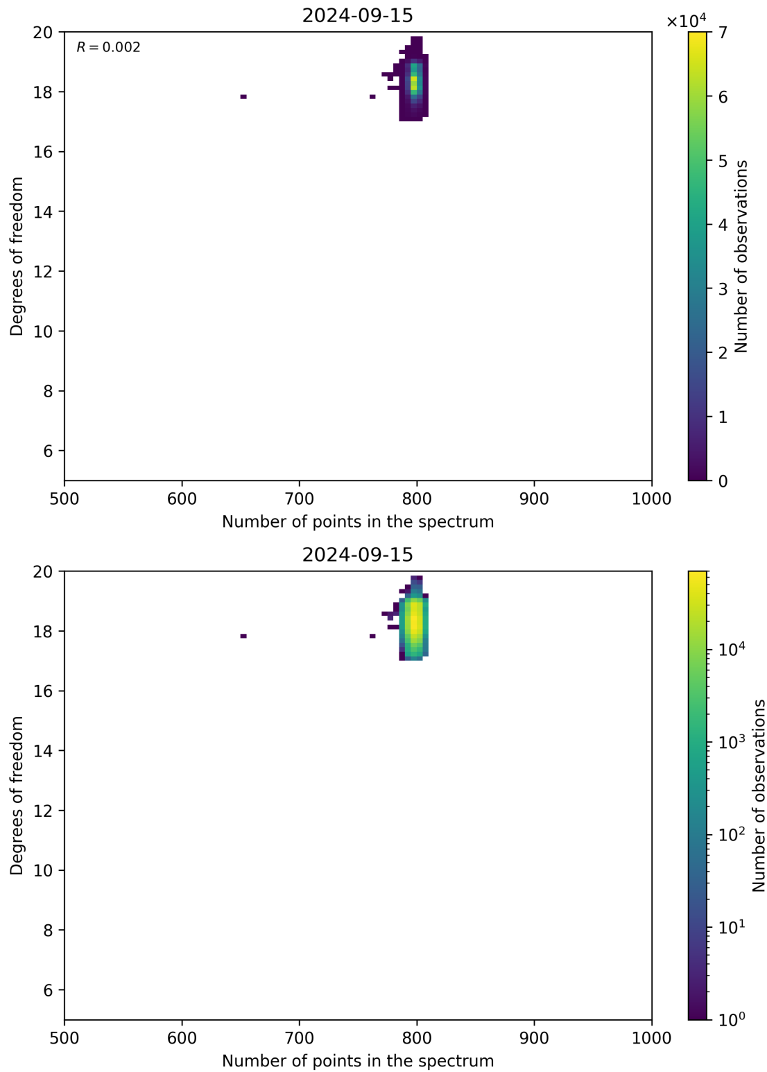
Figure 90: Scatter density plot of “Number of points in the spectrum” against “Degrees of freedom” for 2024-09-14 to 2024-09-16.
