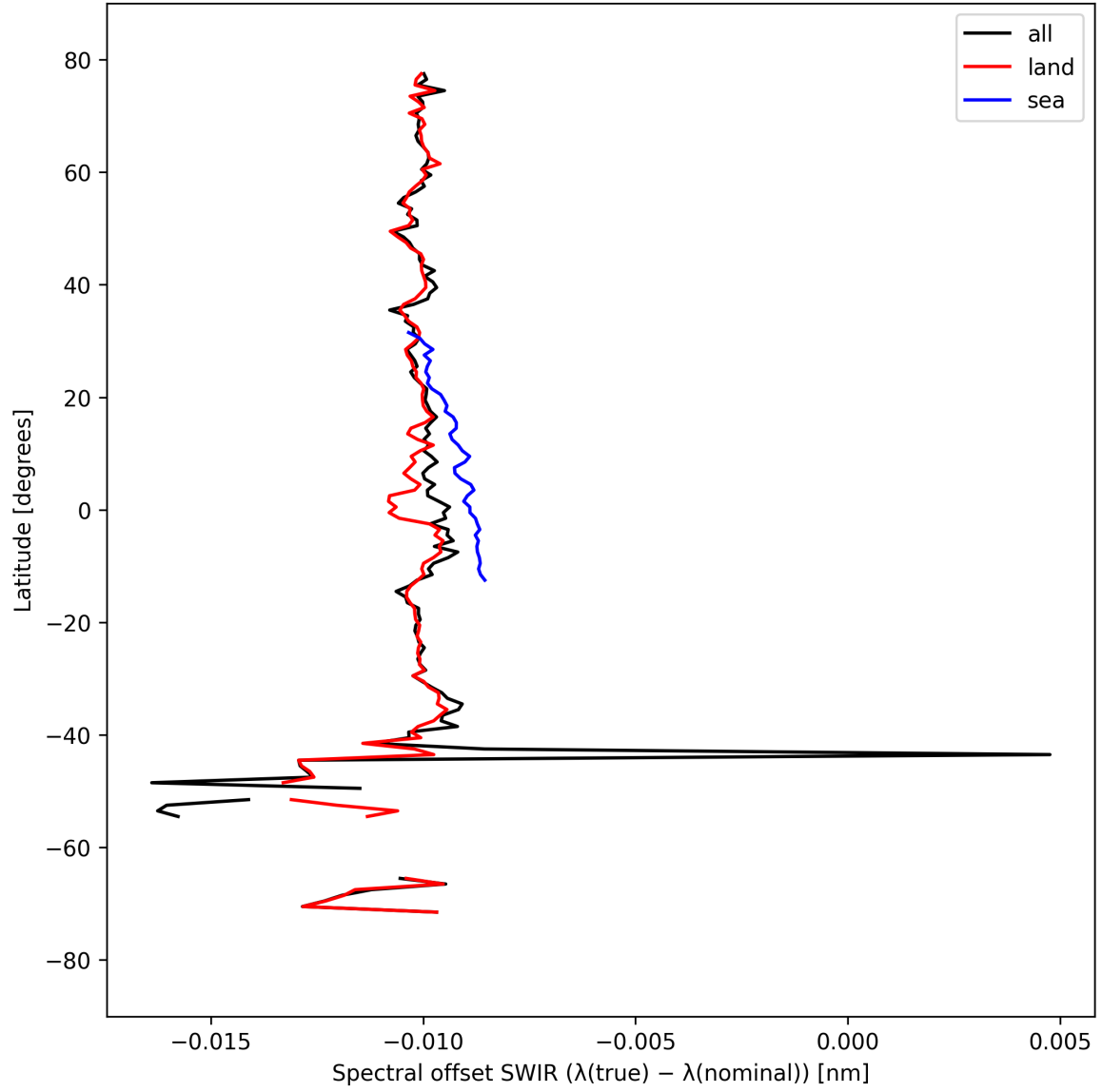
Figure 16: Zonal average of “Spectral offset SWIR ( \lambda_{\text{true}} - \lambda_{\text{nominal}} )” for 2024-09-14 to 2024-09-16.
