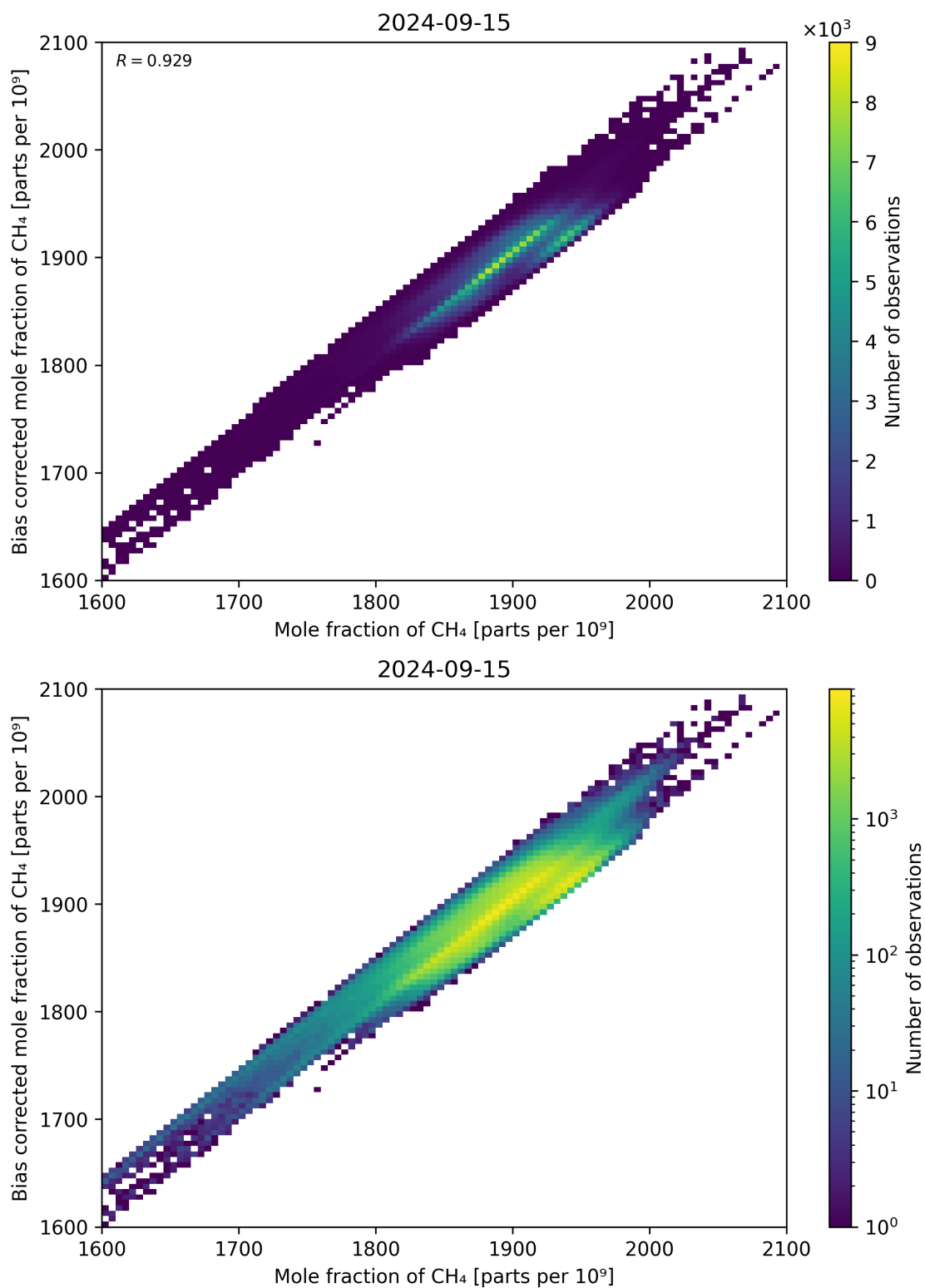
Figure 74: Scatter density plot of “Mole fraction of CH 4 ” against “Bias corrected mole fraction of CH 4 ” for 2024-09-14 to 2024-09-16.
