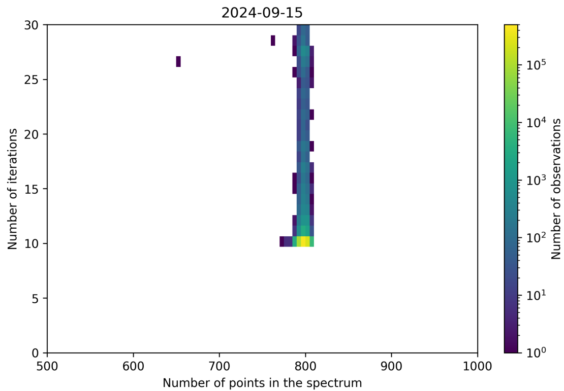
Figure 92: Scatter density plot of “Number of points in the spectrum” against “Number of iterations” for 2024-09-14 to 2024-09-16.
