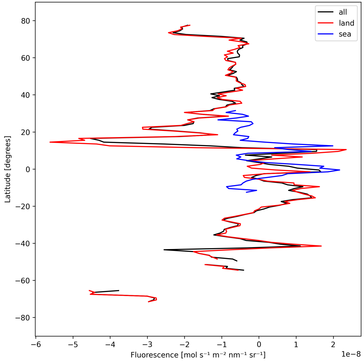
Figure 21: Zonal average of “Fluorescence” for 2024-09-14 to 2024-09-16.
