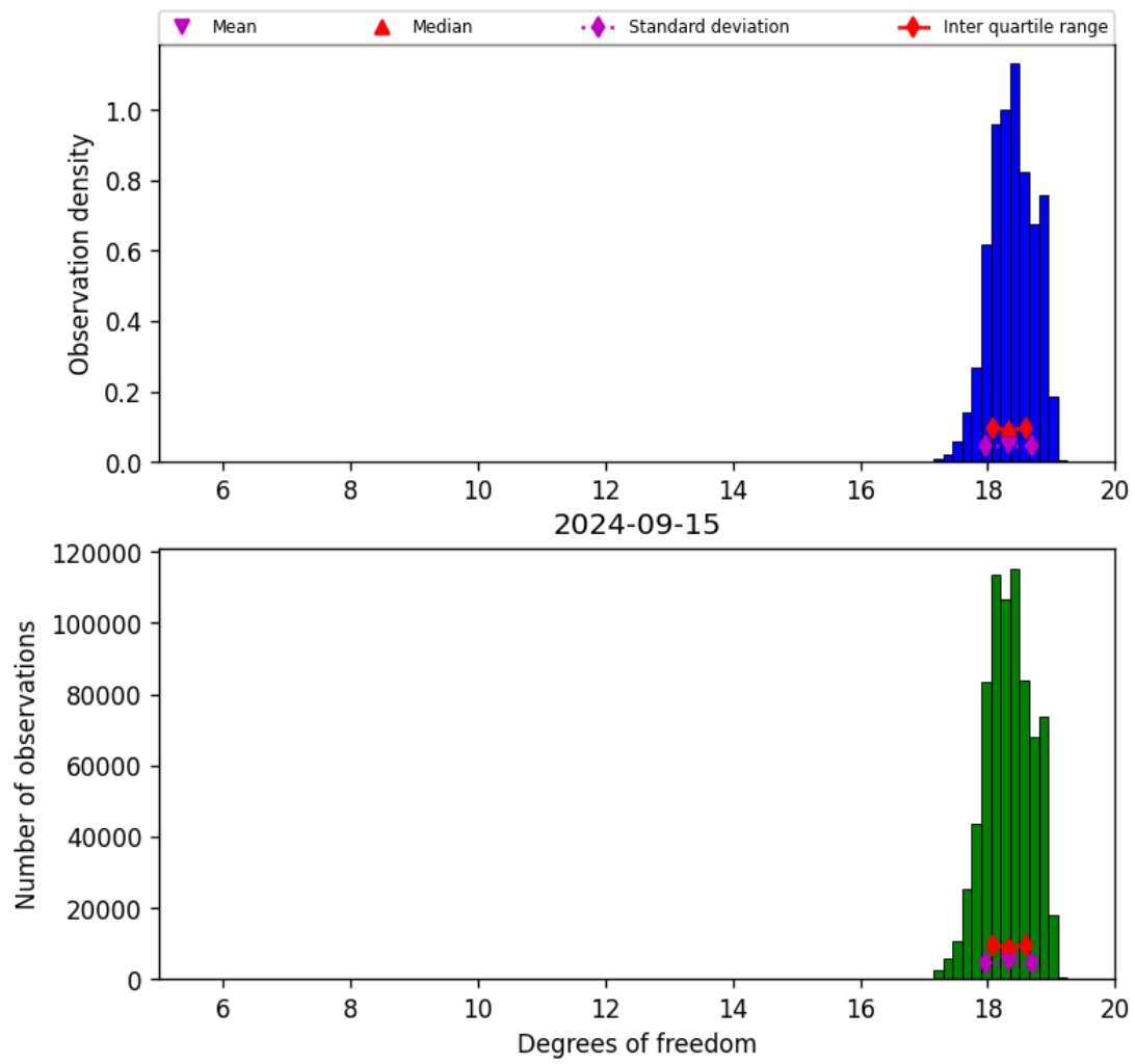
Figure 30: Histogram of “Degrees of freedom” for 2024-09-14 to 2024-09-16
