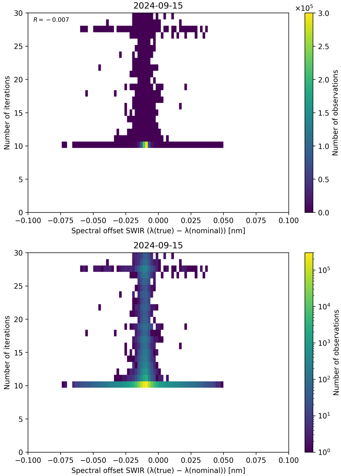
Figure 121: Scatter density plot of “Spectral offset SWIR ( \lambda_{\text{true}} - \lambda_{\text{nominal}} )” against “Number of iterations” for 2024-09-14 to 2024-09-16.
