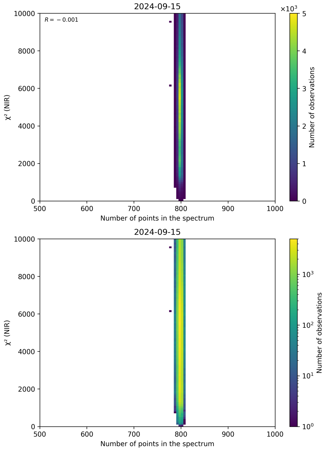
Figure 88: Scatter density plot of “Number of points in the spectrum” against “ \chi^2 (NIR)” for 2024-09-14 to 2024-09-16.
