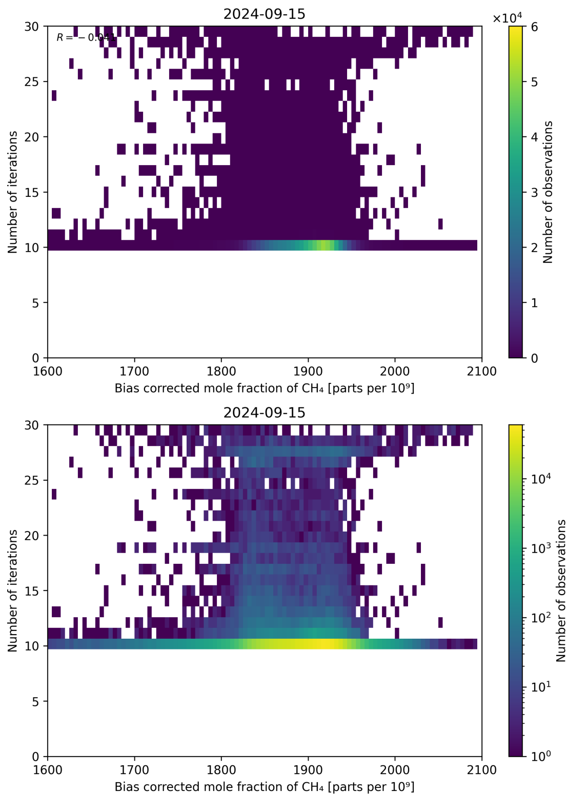
Figure 67: Scatter density plot of “Bias corrected mole fraction of CH 4 ” against “Number of iterations” for 2024-09-14 to 2024-09-16.
