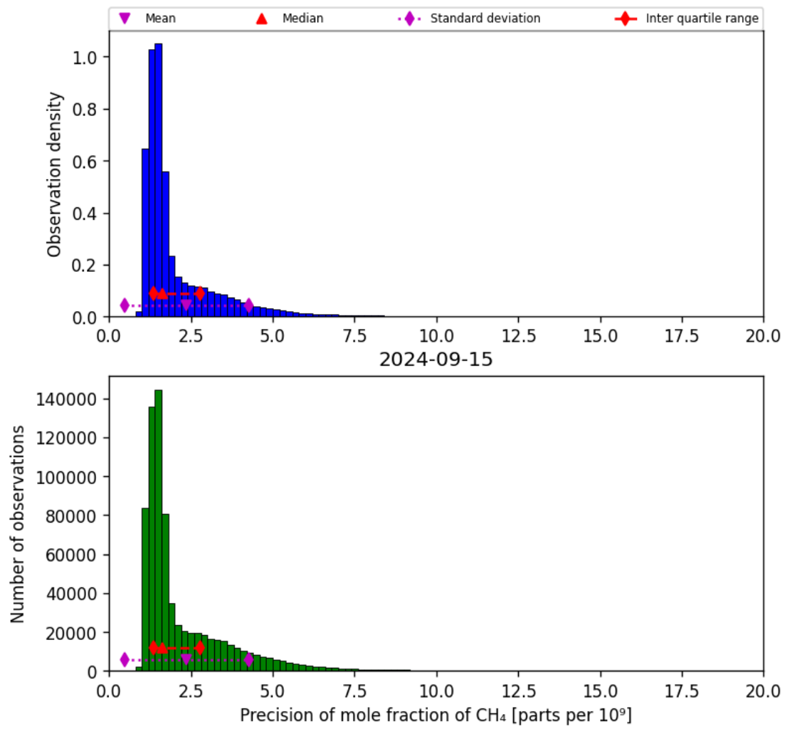
Figure 24: Histogram of “Precision of mole fraction of CH 4 ” for 2024-09-14 to 2024-09-16
