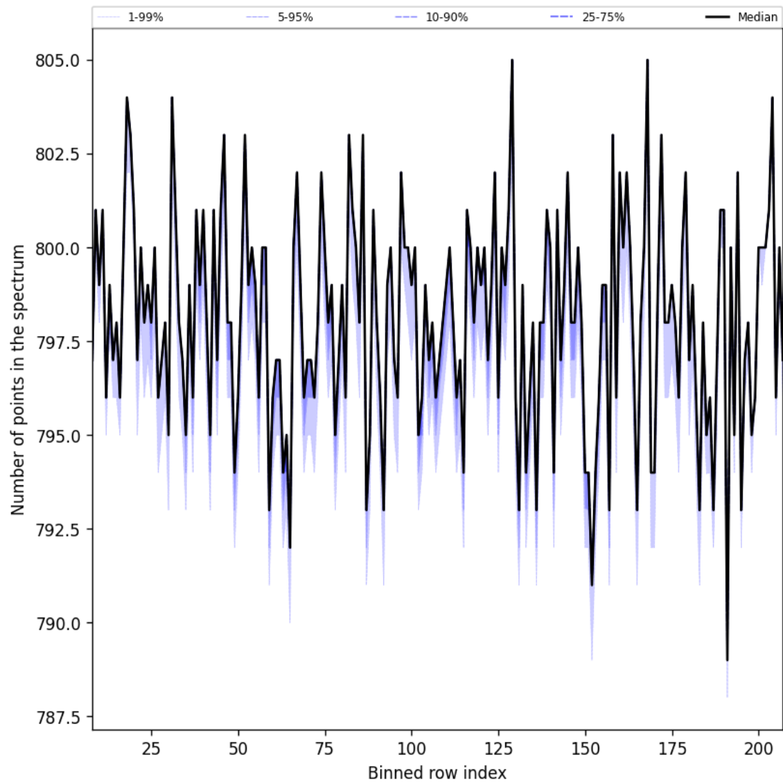
Figure 37: Along track statistics of “Number of points in the spectrum” for 2024-09-14 to 2024-09-16
