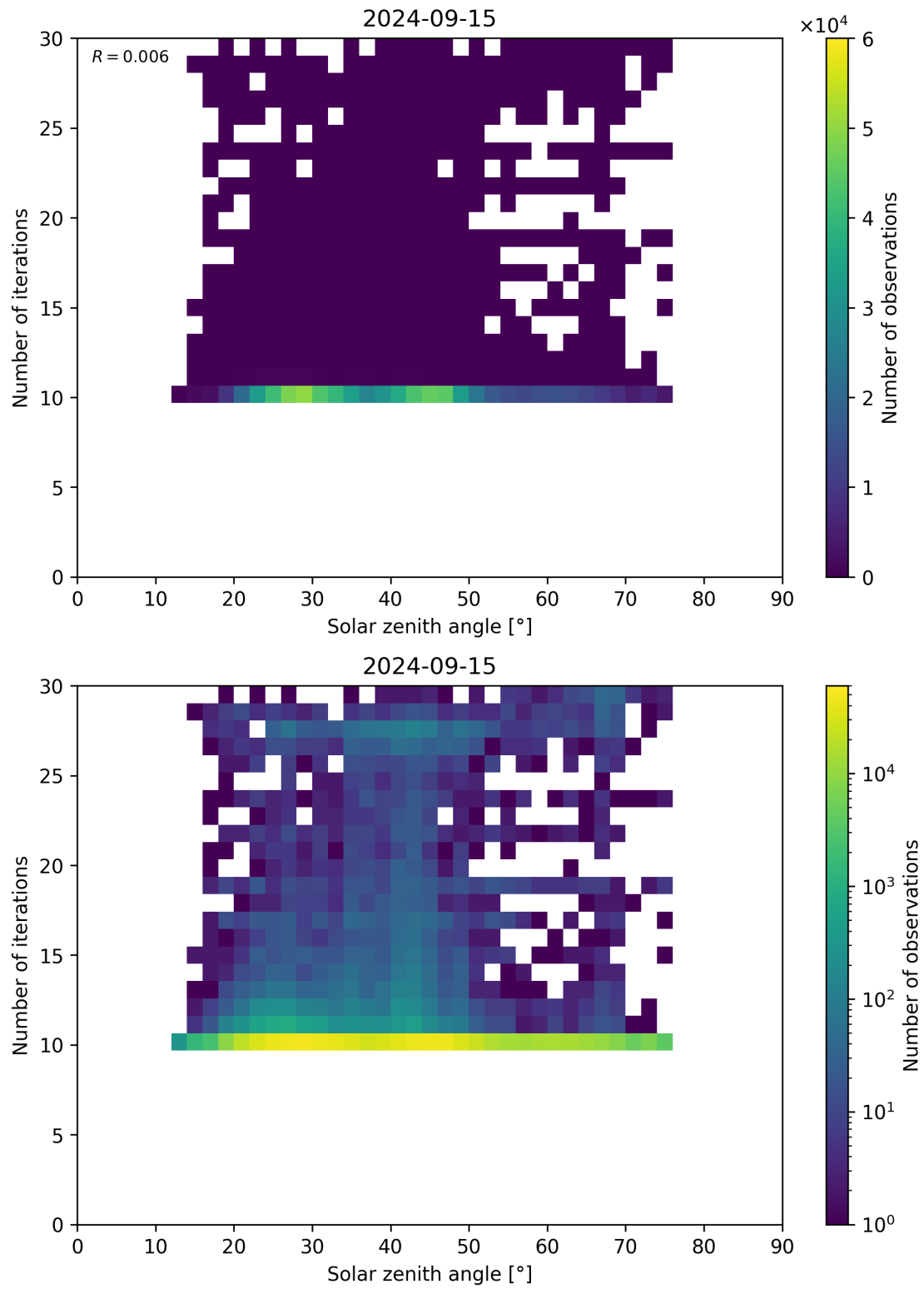
Figure 102: Scatter density plot of “Solar zenith angle” against “Number of iterations” for 2024-09-14 to 2024-09-16.
