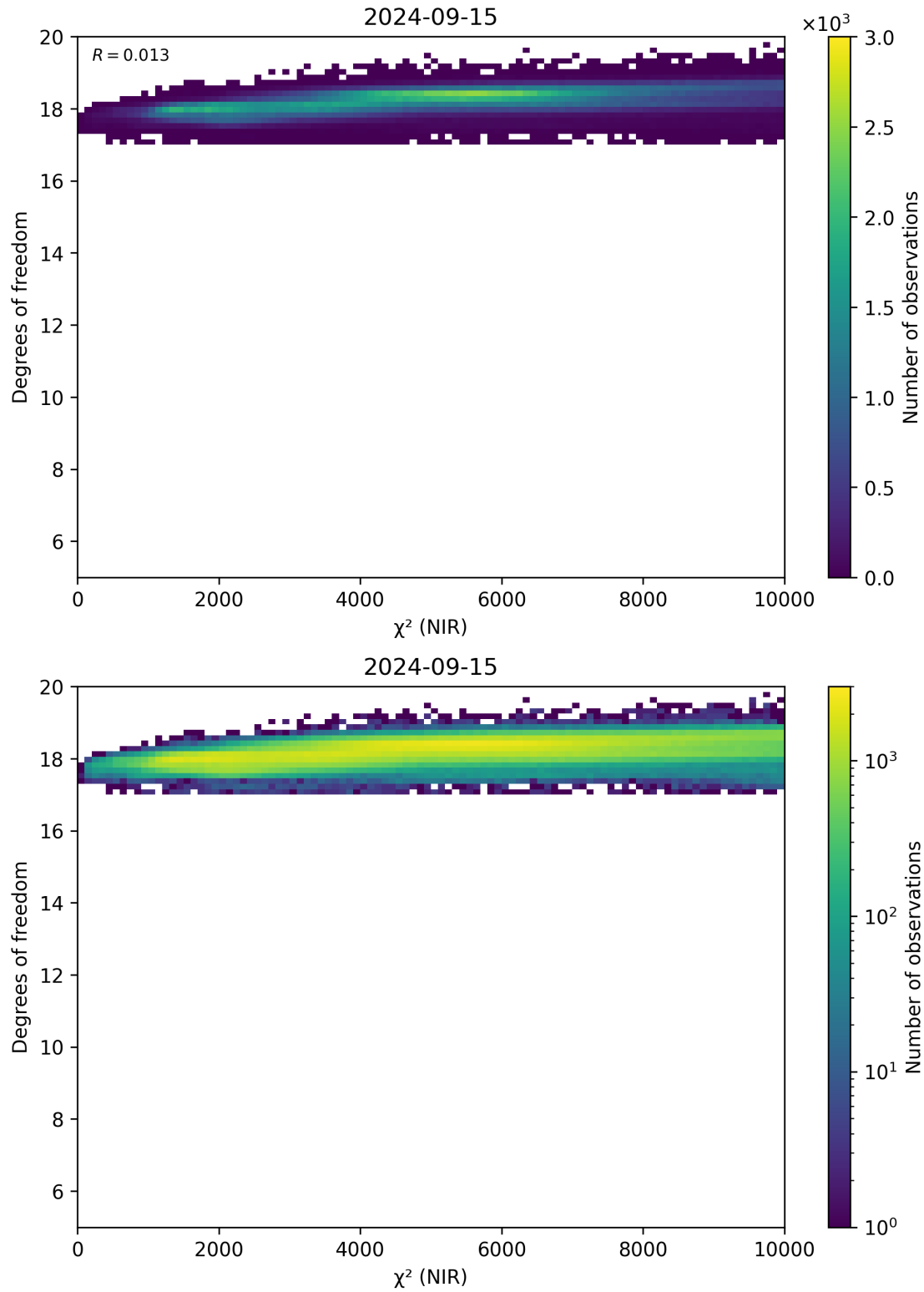
Figure 44: Scatter density plot of “ \chi^2 (NIR)” against “Degrees of freedom” for 2024-09-14 to 2024-09-16.
