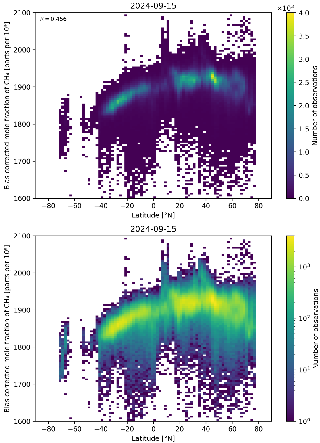
Figure 58: Scatter density plot of “Latitude” against “Bias corrected mole fraction of \text{CH}_4 ” for 2024-09-14 to 2024-09-16.
