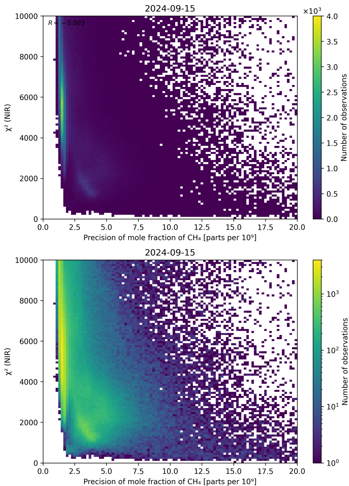
Figure 78: Scatter density plot of “Precision of mole fraction of CH 4 ” against “ \chi^2 (NIR)” for 2024-09-14 to 2024-09-16.
