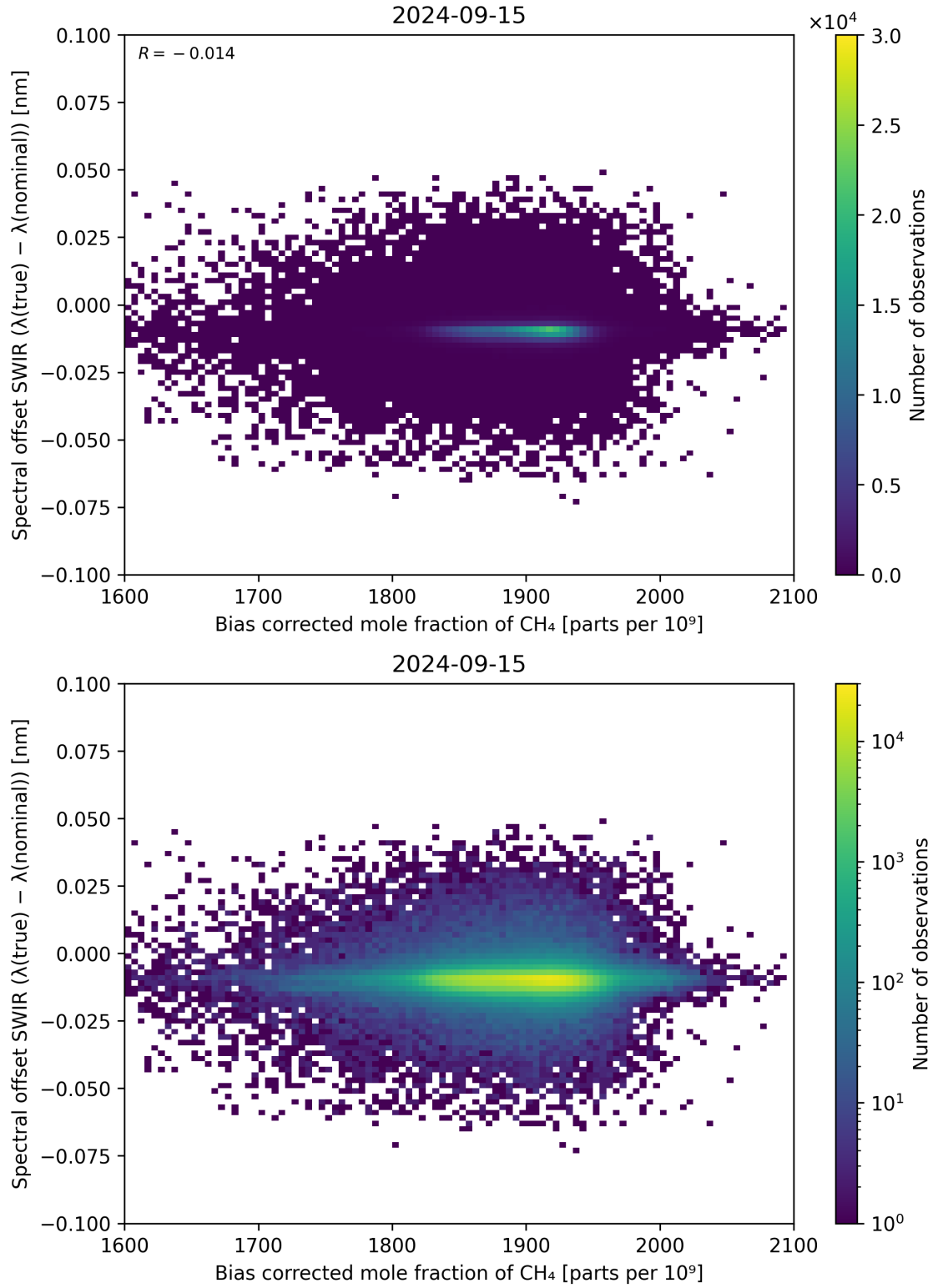
Figure 69: Scatter density plot of “Bias corrected mole fraction of CH 4 ” against “Spectral offset SWIR ( \lambda_{\text{true}} - \lambda_{\text{nominal}} )” for 2024-09-14 to 2024-09-16.
