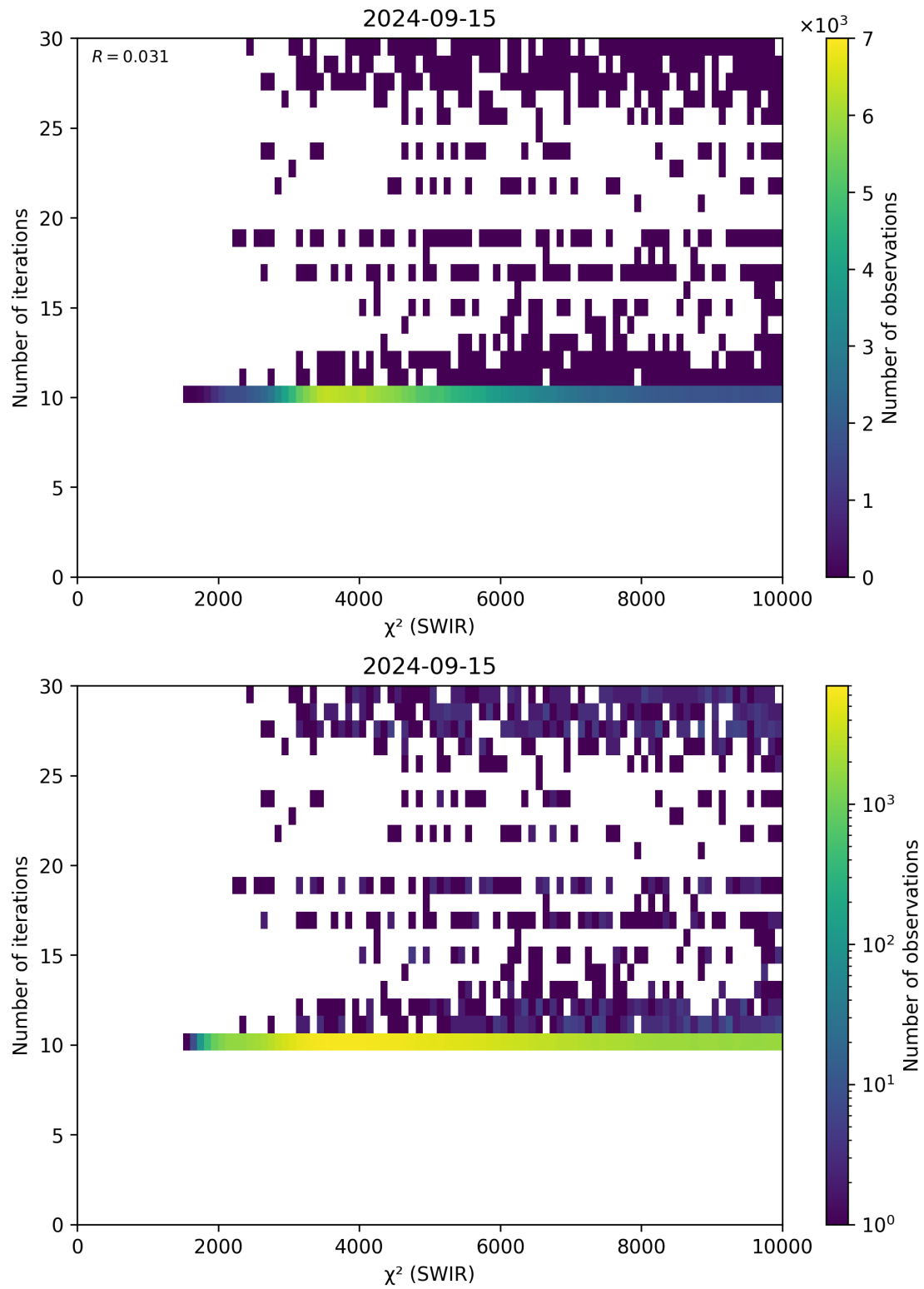
Figure 50: Scatter density plot of “ \chi^2 (SWIR)” against “Number of iterations” for 2024-09-14 to 2024-09-16.
