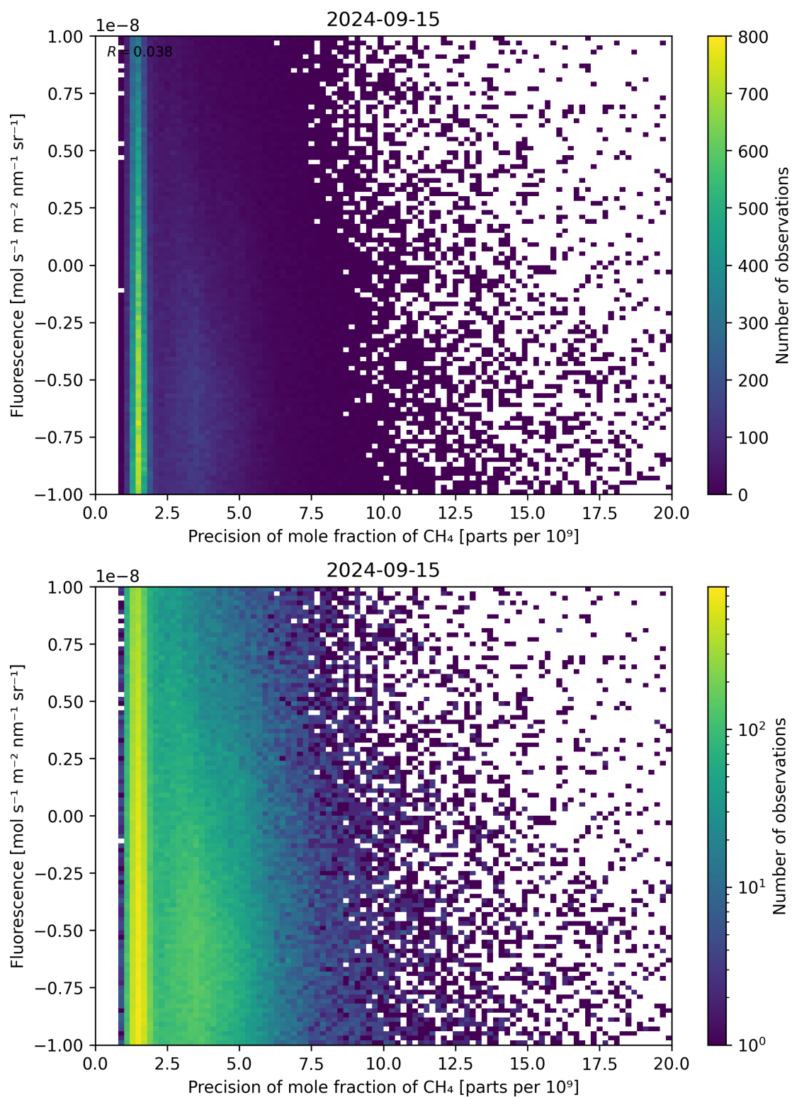
Figure 81: Scatter density plot of “Precision of mole fraction of \text{CH}_4 ” against “Fluorescence” for 2024-09-14 to 2024-09-16.
