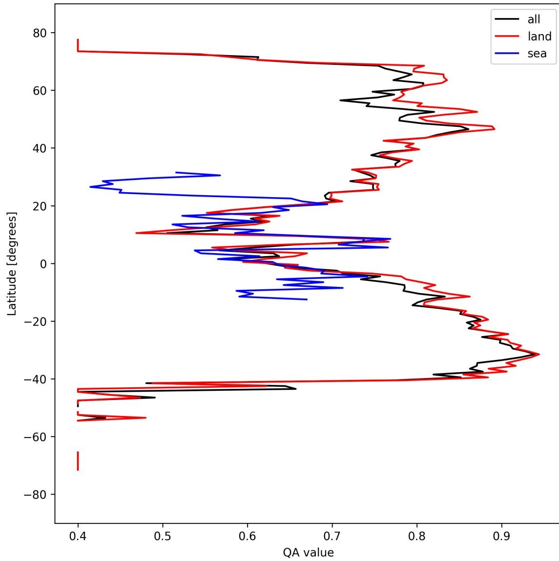
Figure 11: Zonal average of “QA value” for 2024-09-14 to 2024-09-16.
