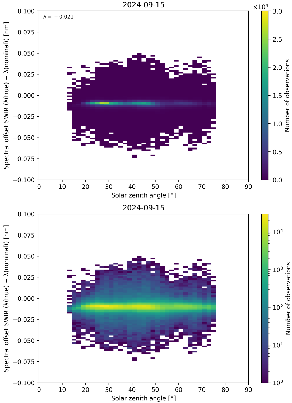
Figure 104: Scatter density plot of “Solar zenith angle” against “Spectral offset SWIR ( \lambda_{\text{true}} - \lambda_{\text{nominal}} )” for 2024-09-14 to 2024-09-16.
