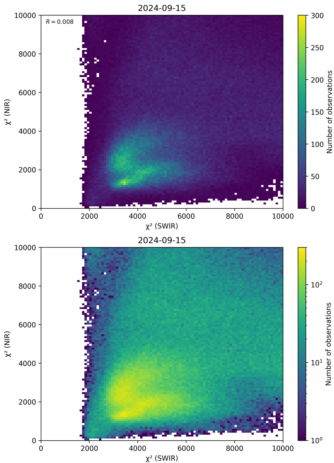
Figure 47: Scatter density plot of “ \chi^2 (SWIR)” against “ \chi^2 (NIR)” for 2024-09-14 to 2024-09-16.
