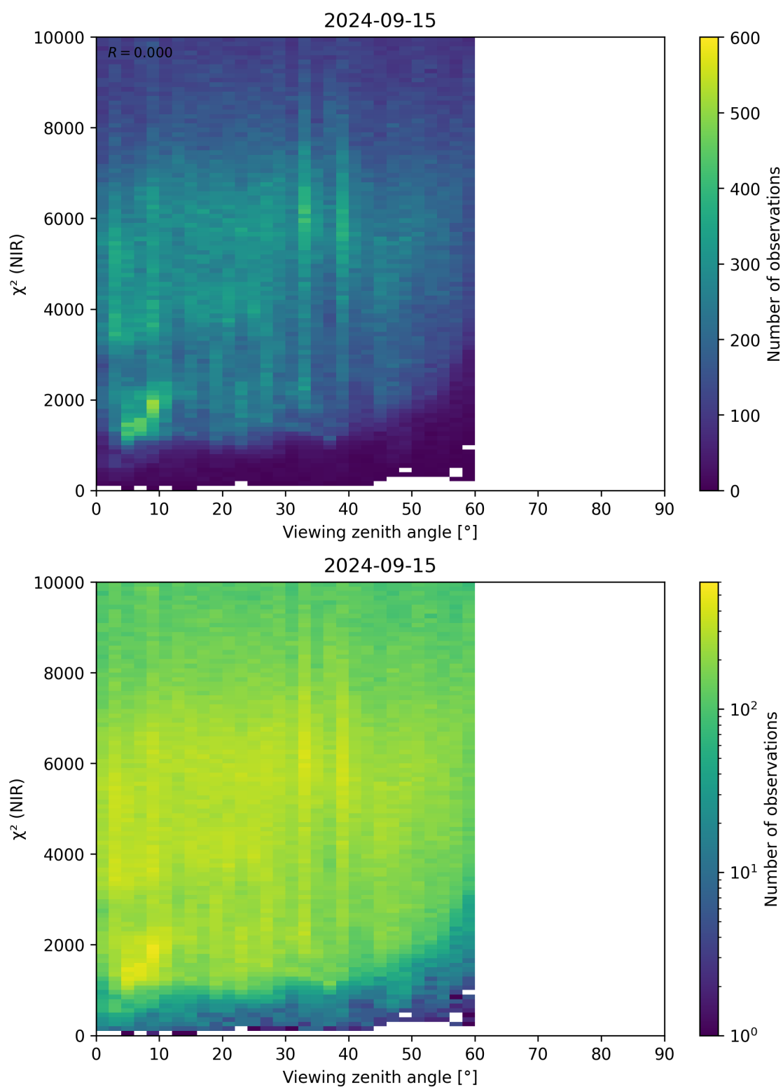
Figure 105: Scatter density plot of “Viewing zenith angle” against “ \chi^2 (NIR)” for 2024-09-14 to 2024-09-16.
