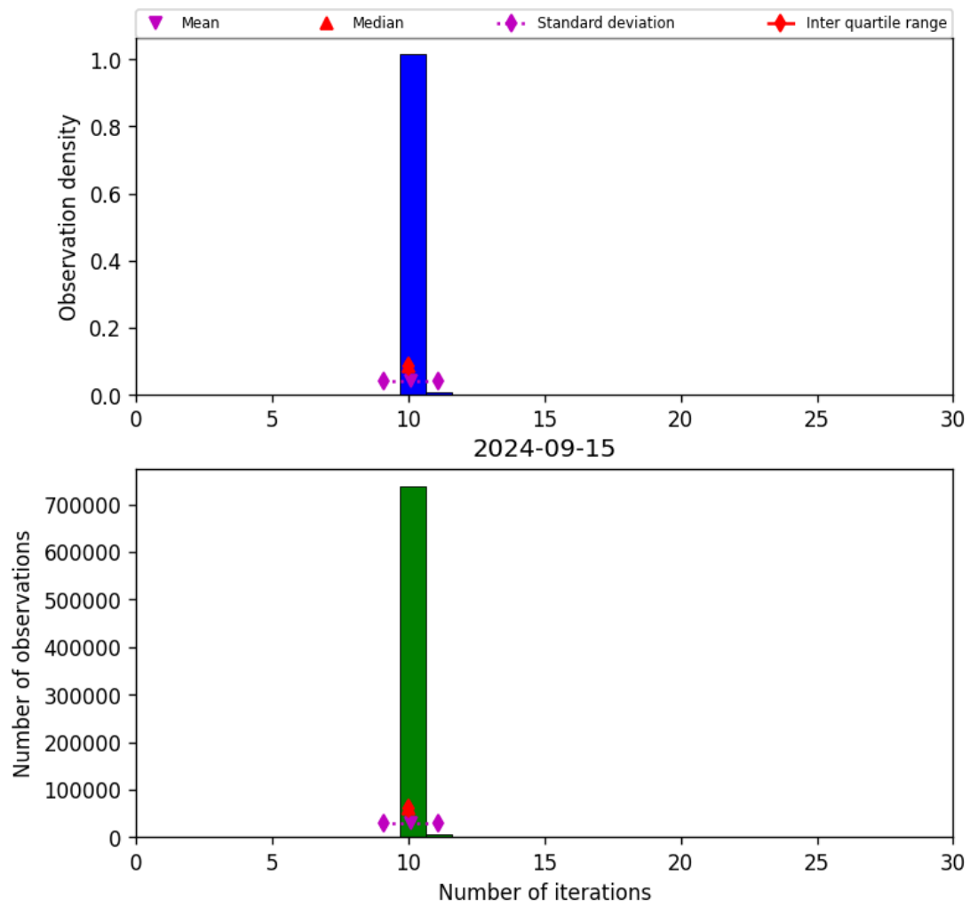
Figure 31: Histogram of “Number of iterations” for 2024-09-14 to 2024-09-16
