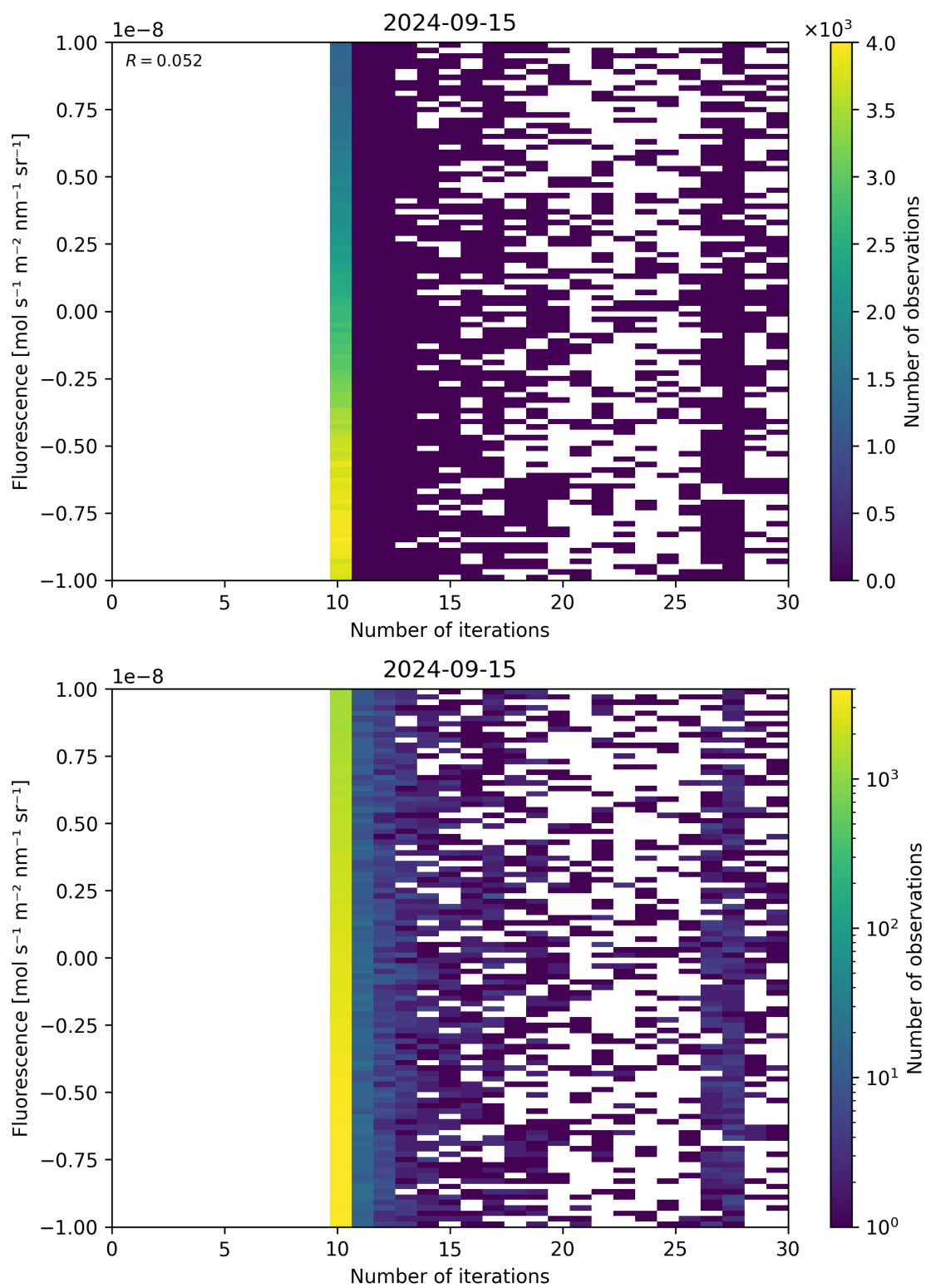
Figure 87: Scatter density plot of “Number of iterations” against “Fluorescence” for 2024-09-14 to 2024-09-16.
