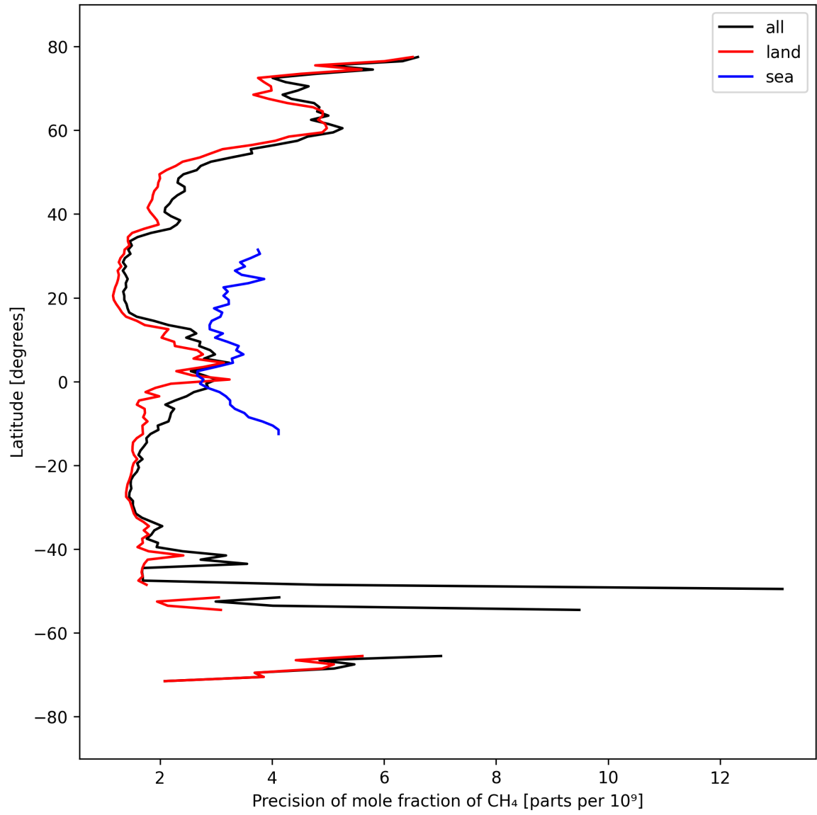
Figure 13: Zonal average of “Precision of mole fraction of CH 4 ” for 2024-09-14 to 2024-09-16.
