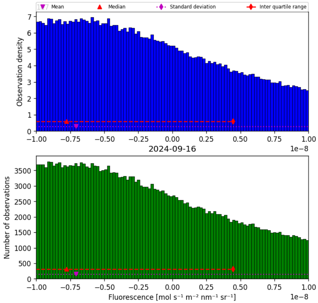
Figure 32: Histogram of “Fluorescence” for 2024-09-15 to 2024-09-17
