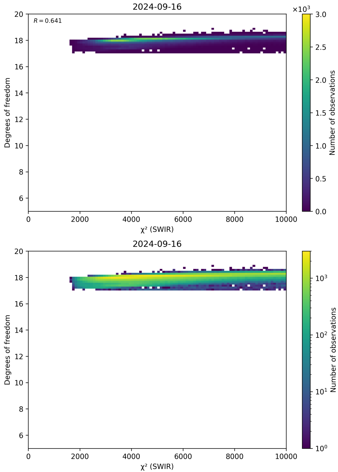
Figure 48: Scatter density plot of “ \chi^2 (SWIR)” against “Degrees of freedom” for 2024-09-15 to 2024-09-17.
