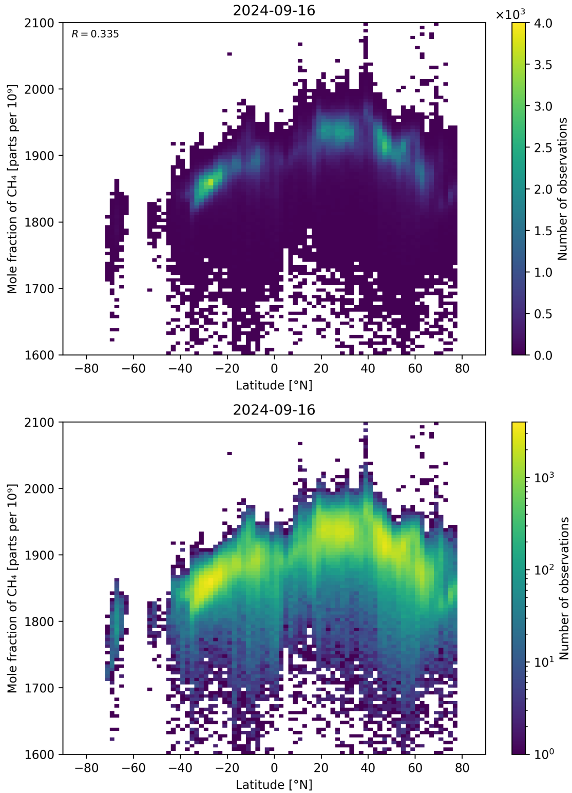
Figure 57: Scatter density plot of “Latitude” against “Mole fraction of \text{CH}_4 ” for 2024-09-15 to 2024-09-17.
