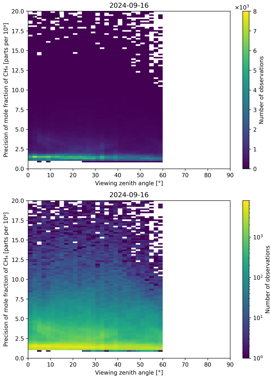
Figure 112: Scatter density plot of “Viewing zenith angle” against “Precision of mole fraction of CH 4 ” for 2024-09-15 to 2024-09-17.
