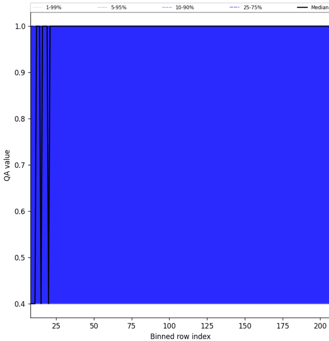
Figure 33: Along track statistics of “QA value” for 2024-09-15 to 2024-09-17
