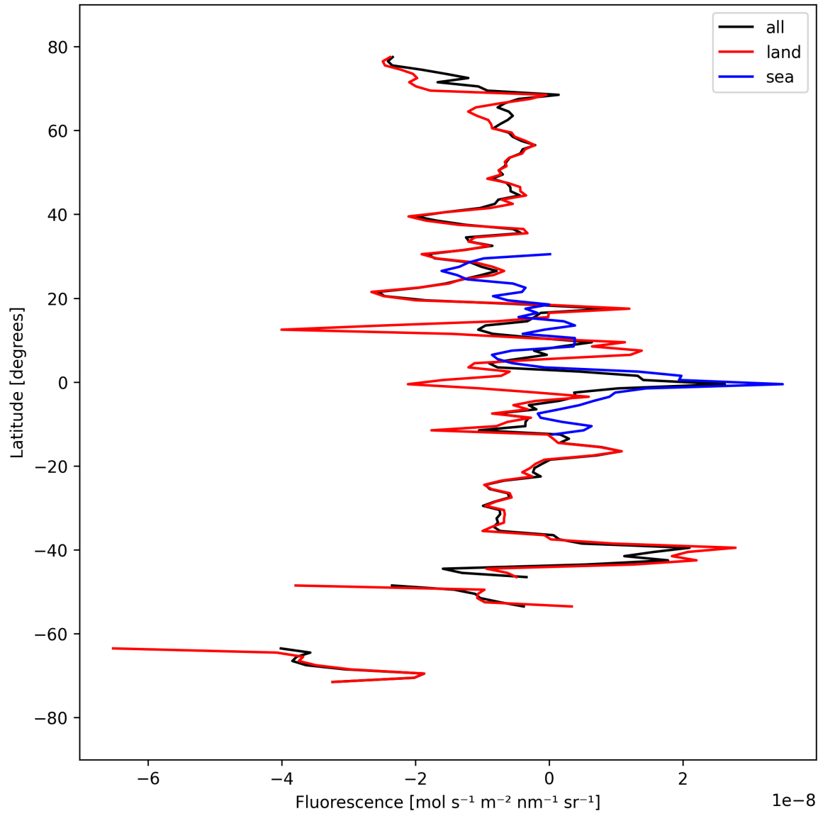
Figure 21: Zonal average of “Fluorescence” for 2024-09-15 to 2024-09-17.
