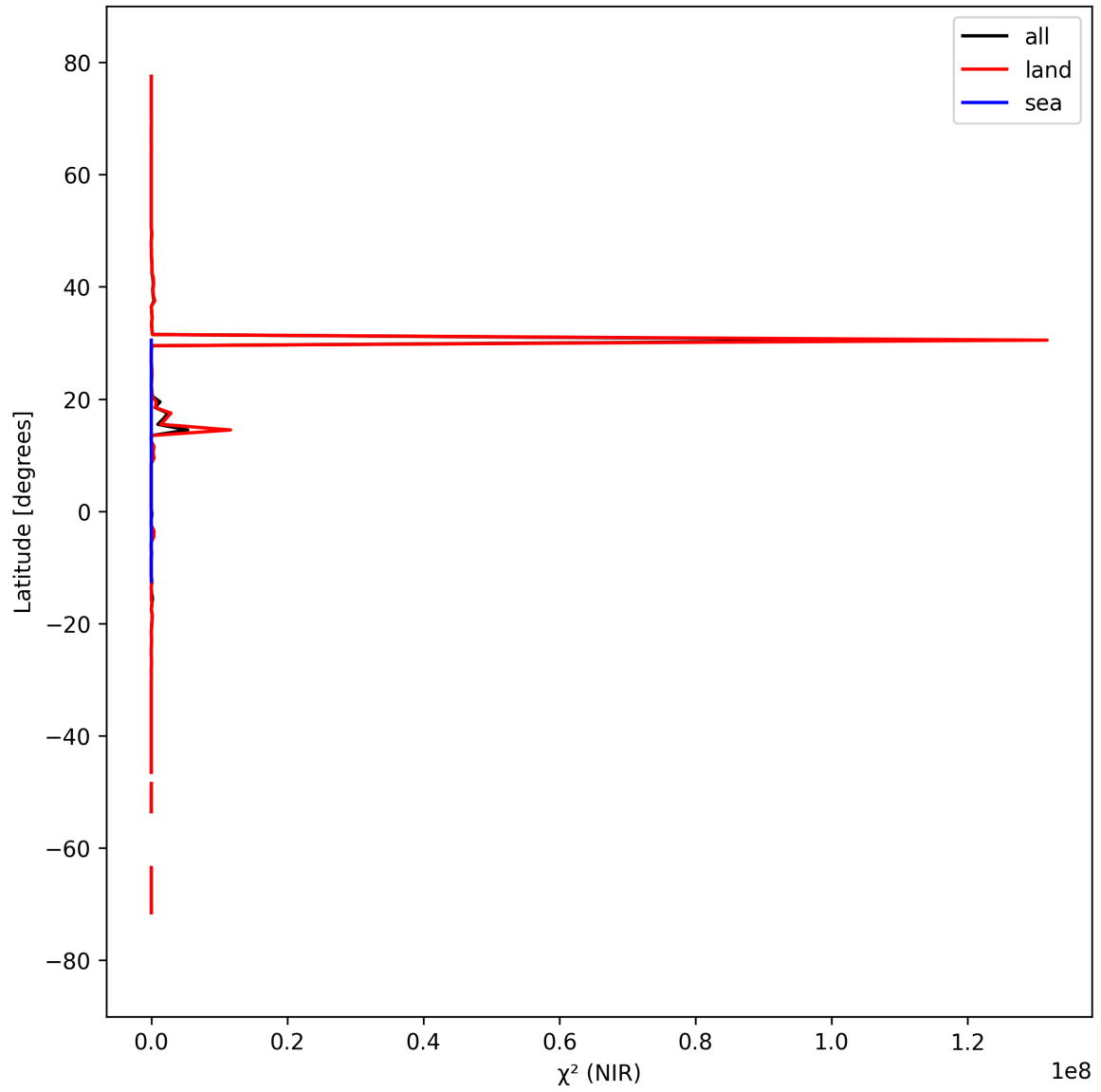
Figure 18: Zonal average of “ \chi^2 (NIR)” for 2024-09-15 to 2024-09-17.
