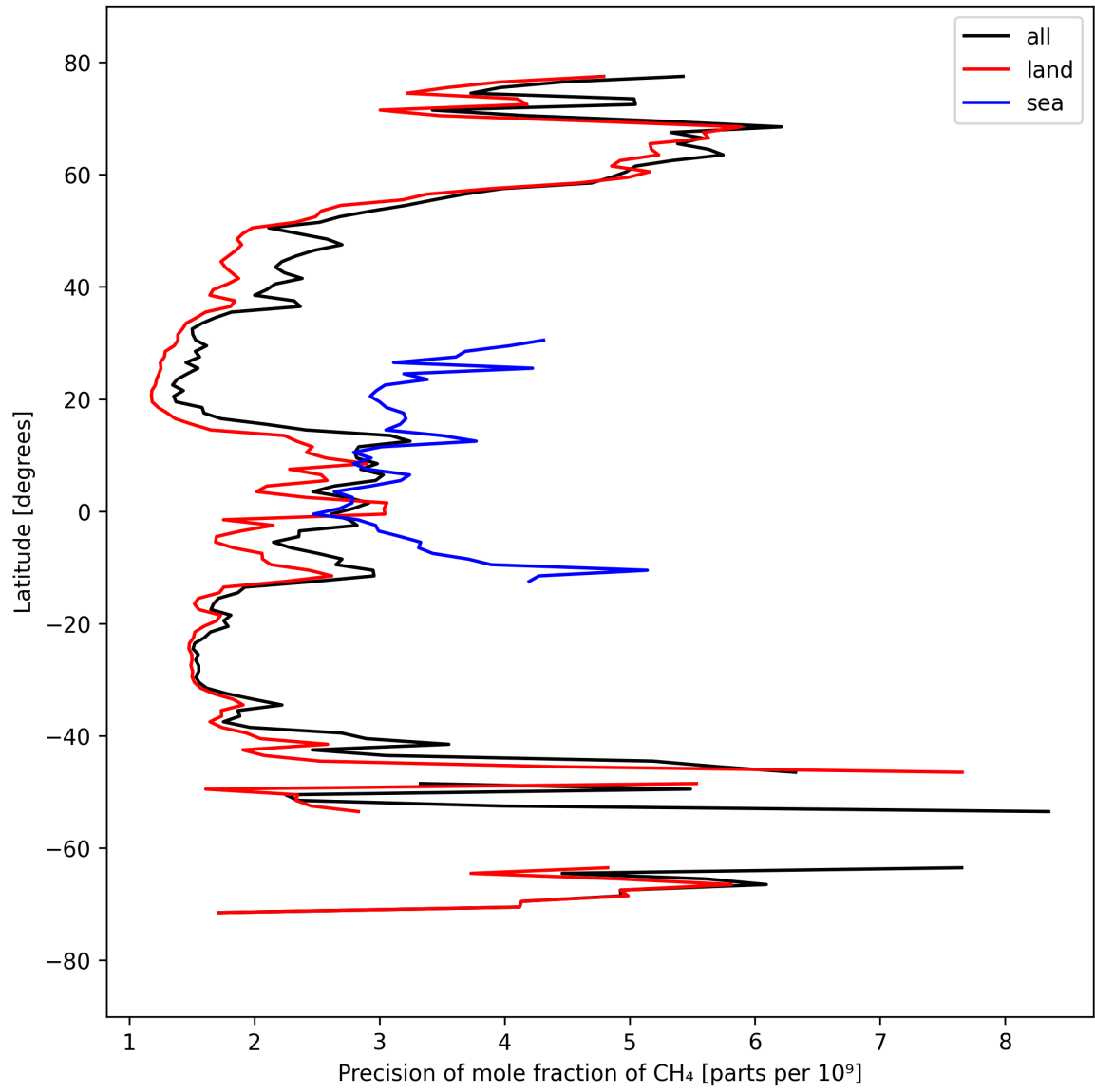
Figure 13: Zonal average of “Precision of mole fraction of CH 4 ” for 2024-09-15 to 2024-09-17.
