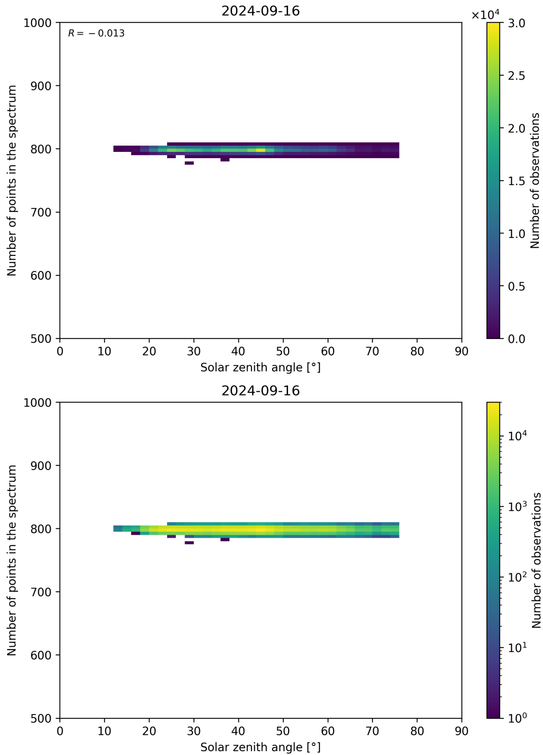
Figure 103: Scatter density plot of “Solar zenith angle” against “Number of points in the spectrum” for 2024-09-15 to 2024-09-17.
