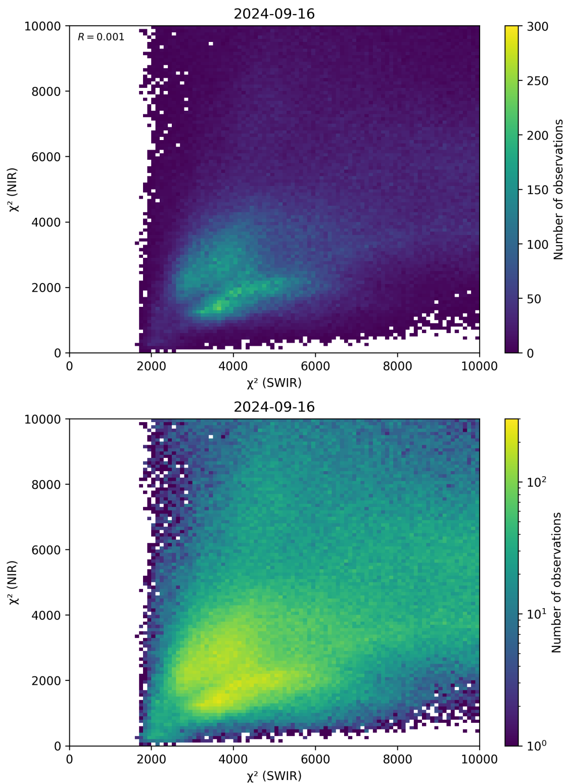
Figure 47: Scatter density plot of “ \chi^2 (SWIR)” against “ \chi^2 (NIR)” for 2024-09-15 to 2024-09-17.
