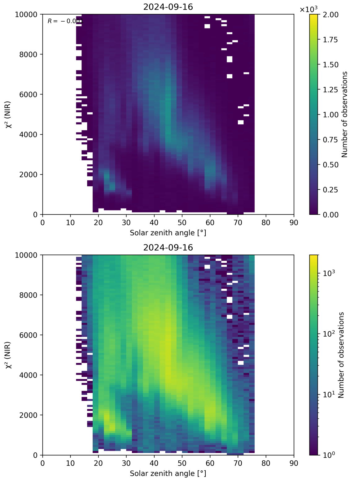
Figure 94: Scatter density plot of “Solar zenith angle” against “ \chi^2 (NIR)” for 2024-09-15 to 2024-09-17.
