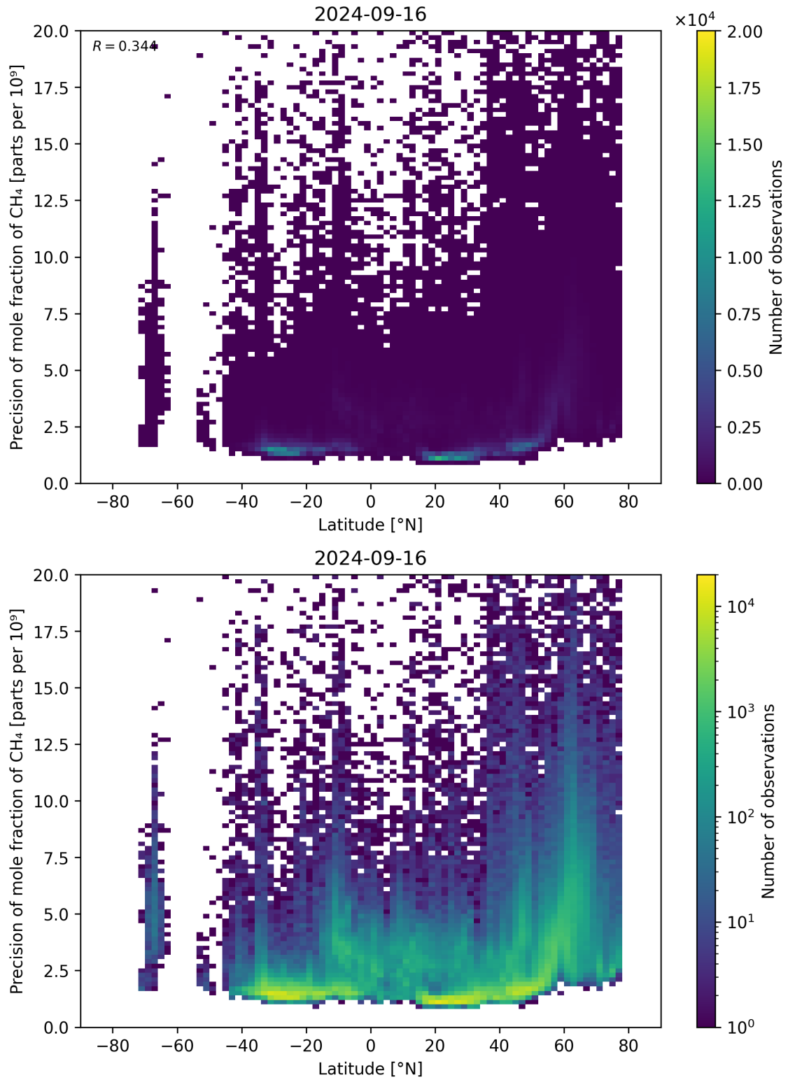
Figure 59: Scatter density plot of “Latitude” against “Precision of mole fraction of \text{CH}_4 ” for 2024-09-15 to 2024-09-17.
