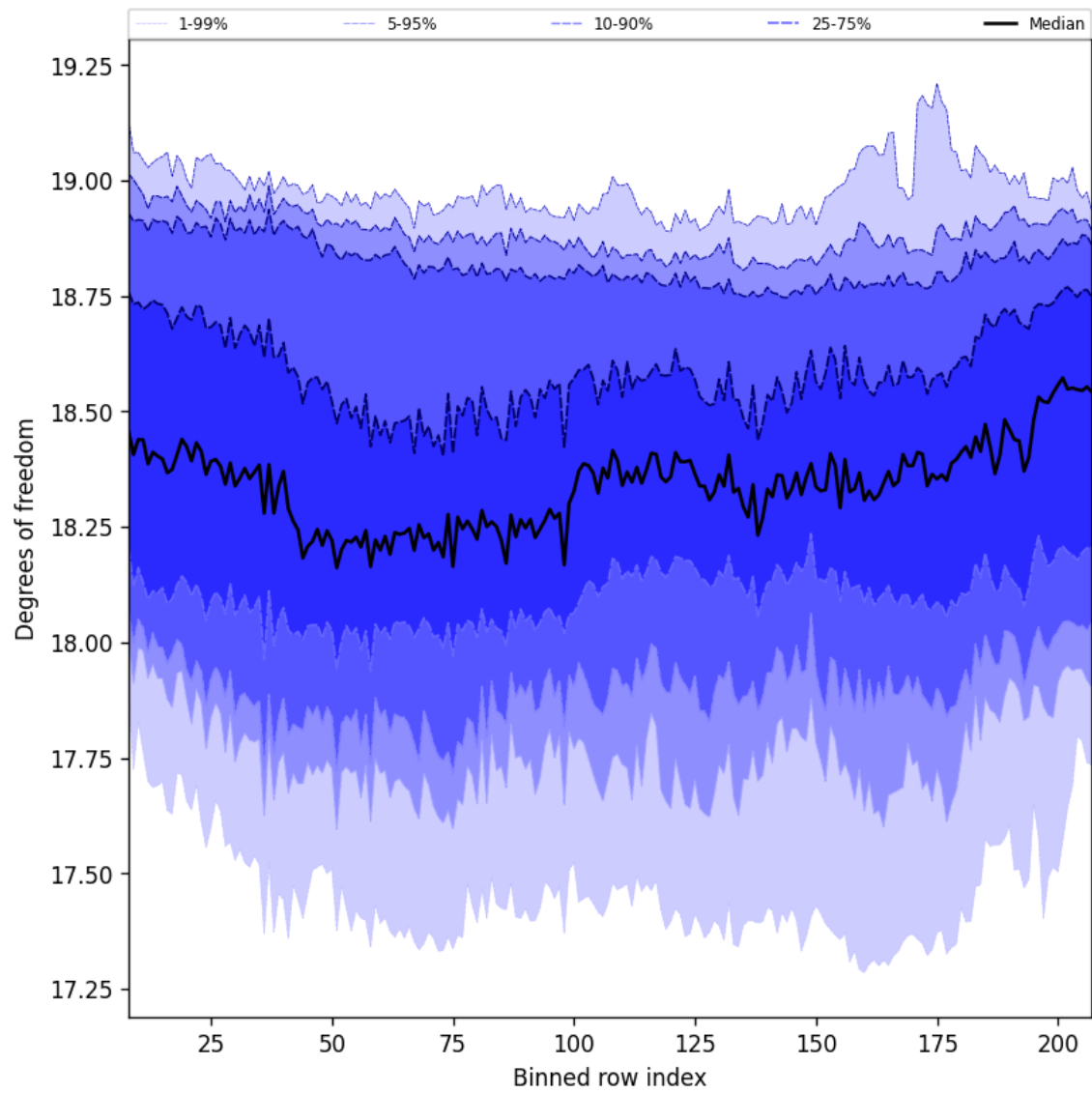
Figure 41: Along track statistics of “Degrees of freedom” for 2024-09-15 to 2024-09-17
