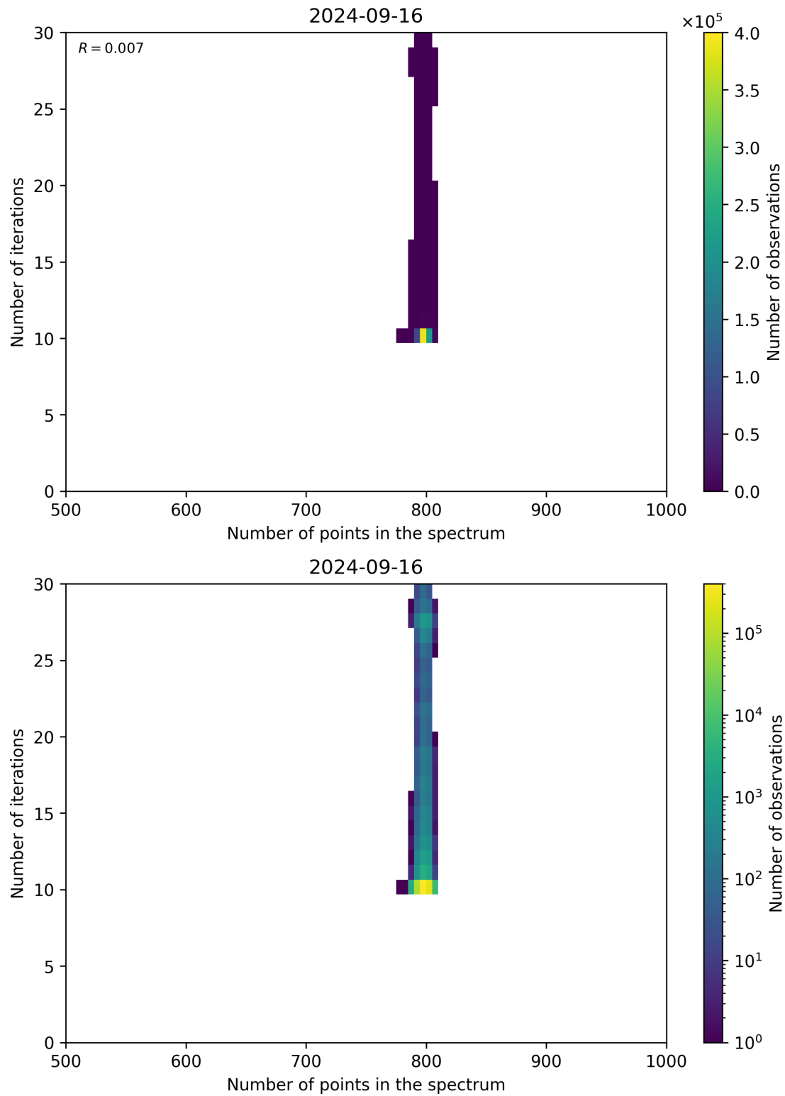
Figure 92: Scatter density plot of “Number of points in the spectrum” against “Number of iterations” for 2024-09-15 to 2024-09-17.
