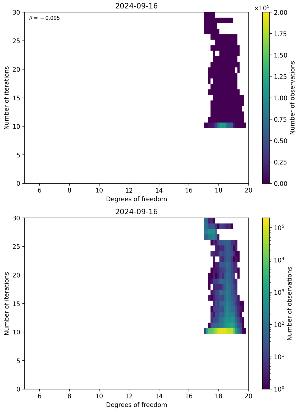
Figure 52: Scatter density plot of “Degrees of freedom” against “Number of iterations” for 2024-09-15 to 2024-09-17.
