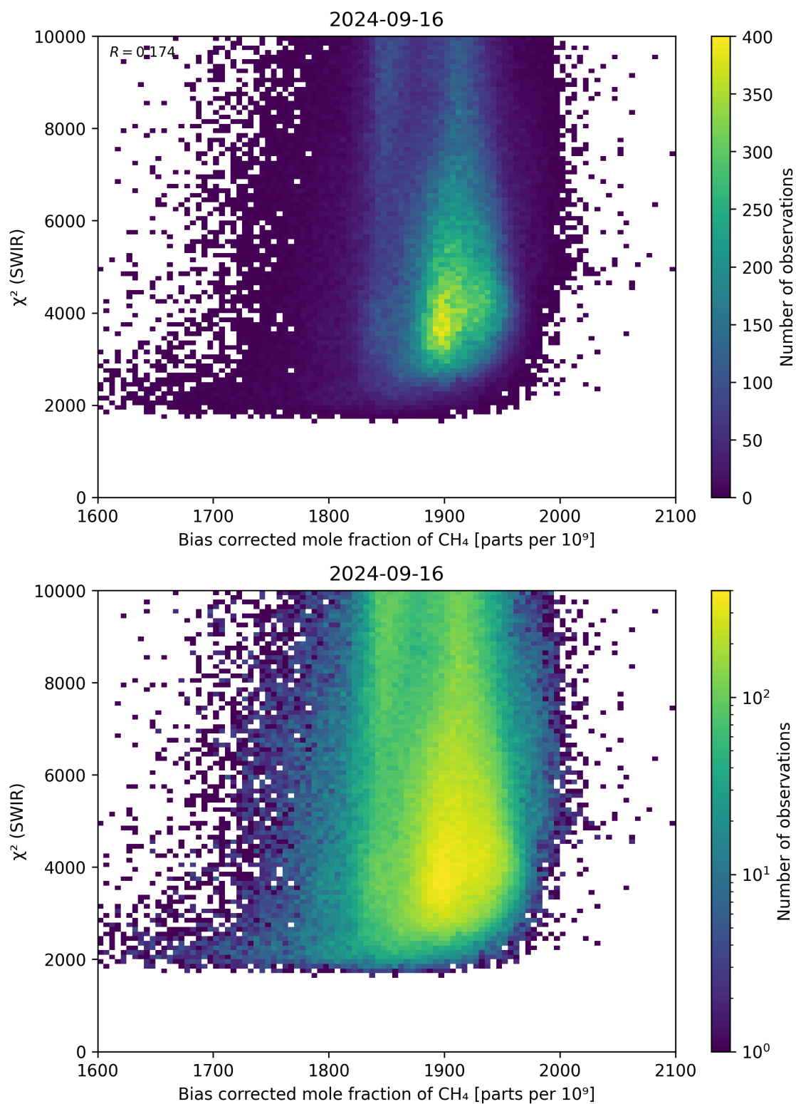
Figure 64: Scatter density plot of “Bias corrected mole fraction of CH 4 ” against “ \chi^2 (SWIR)” for 2024-09-15 to 2024-09-17.
