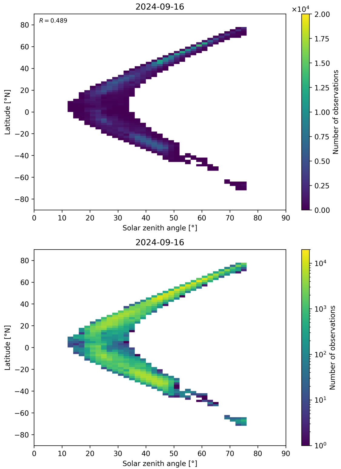
Figure 98: Scatter density plot of “Solar zenith angle” against “Latitude” for 2024-09-15 to 2024-09-17.
