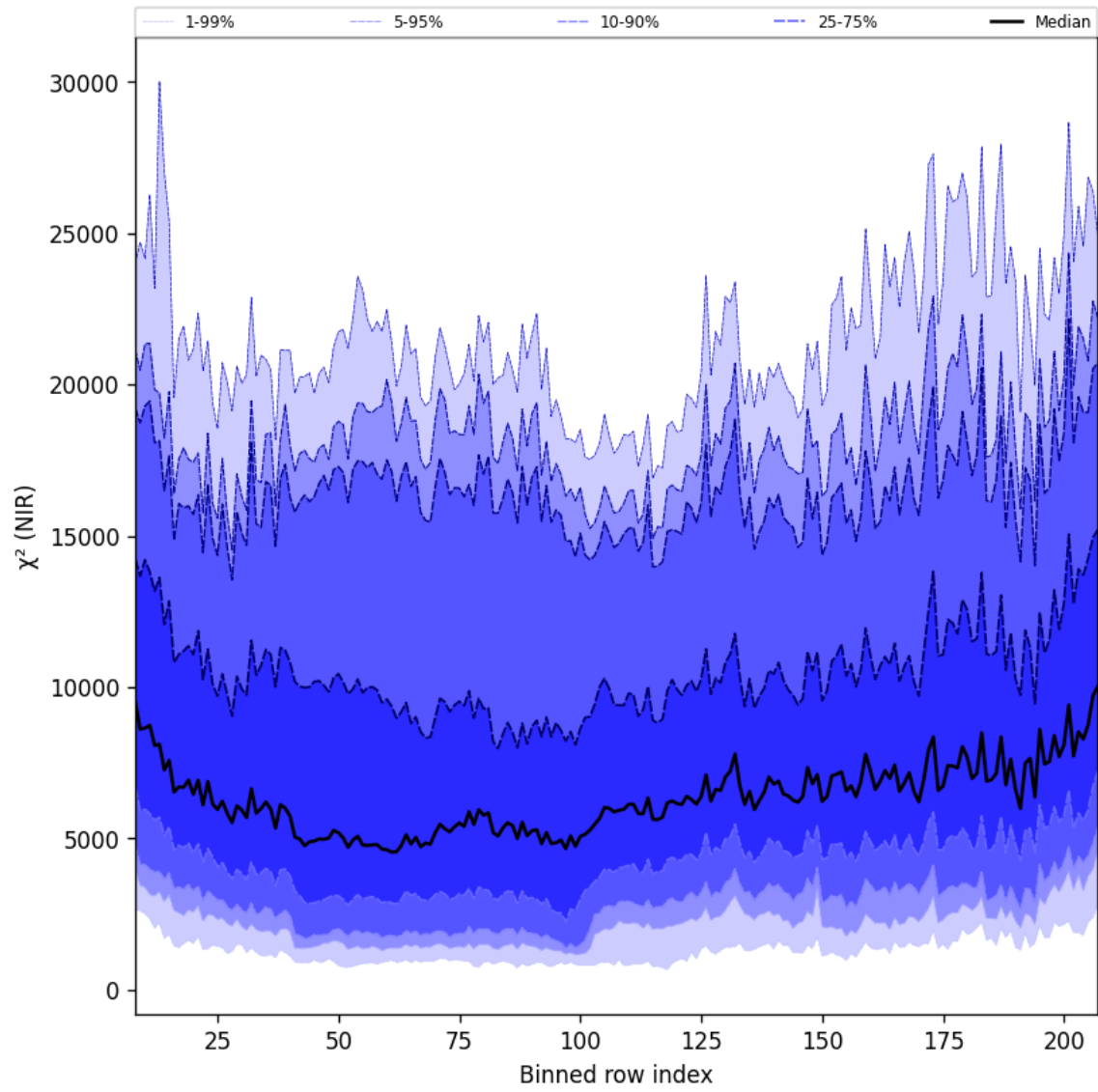
Figure 40: Along track statistics of “ \chi^2 (NIR)” for 2024-09-15 to 2024-09-17
