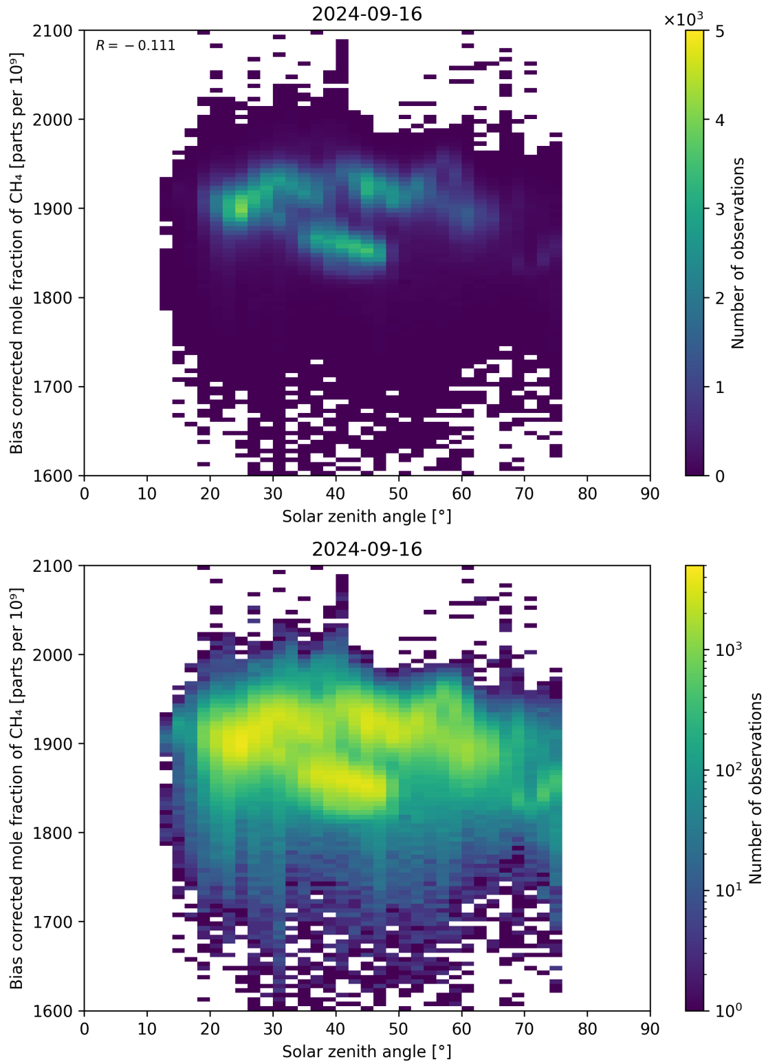
Figure 100: Scatter density plot of “Solar zenith angle” against “Bias corrected mole fraction of \text{CH}_4 ” for 2024-09-15 to 2024-09-17.
