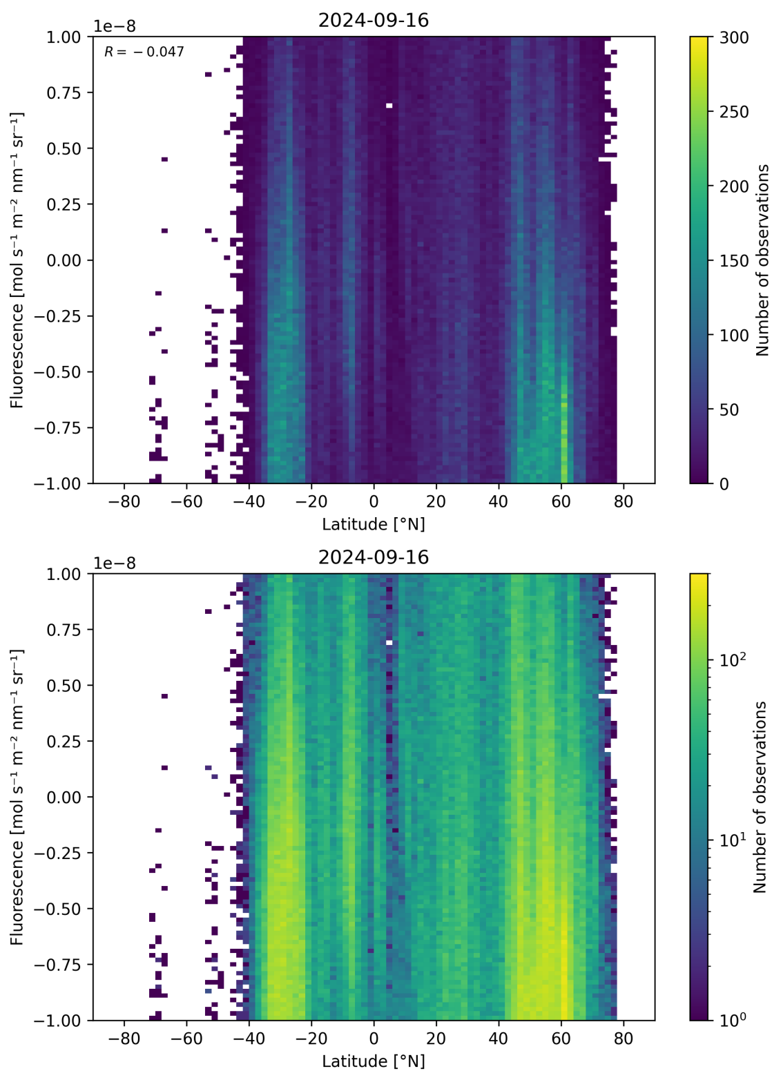
Figure 56: Scatter density plot of “Latitude” against “Fluorescence” for 2024-09-15 to 2024-09-17.
