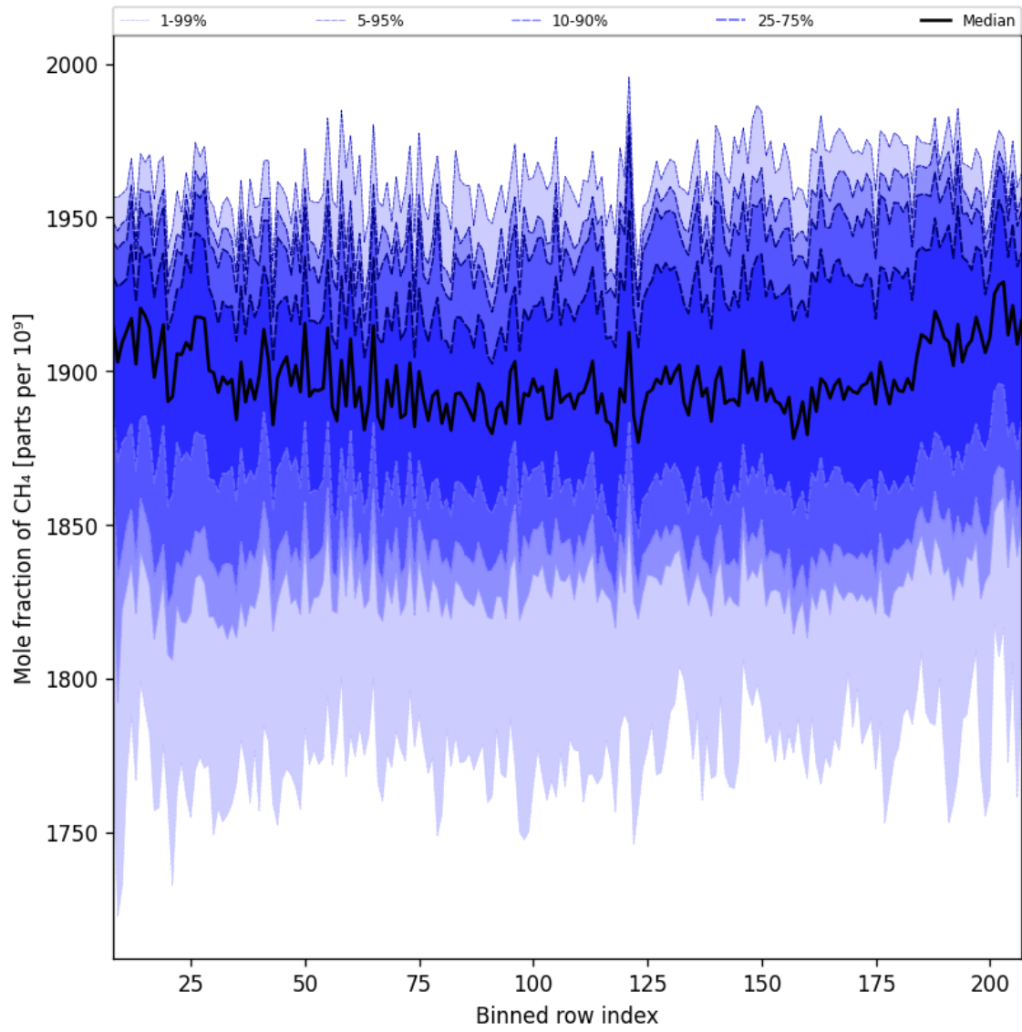
Figure 34: Along track statistics of “Mole fraction of CH 4 ” for 2024-09-15 to 2024-09-17
