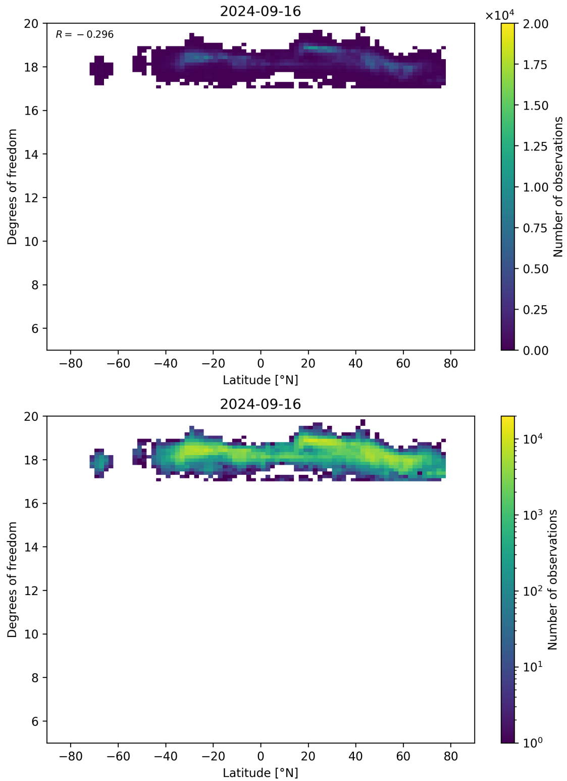
Figure 55: Scatter density plot of “Latitude” against “Degrees of freedom” for 2024-09-15 to 2024-09-17.
