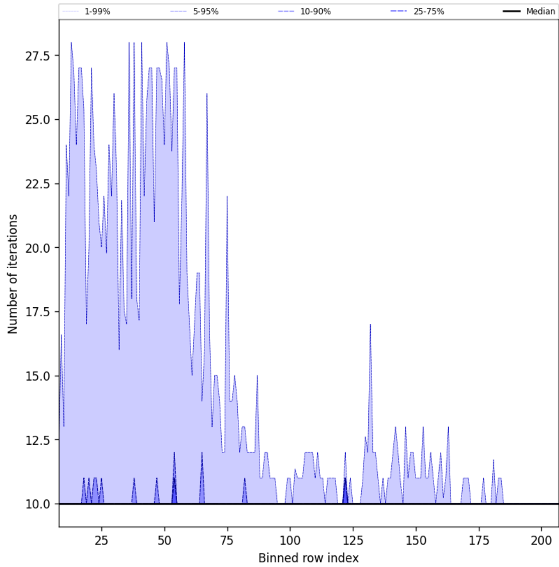
Figure 42: Along track statistics of “Number of iterations” for 2024-09-15 to 2024-09-17
