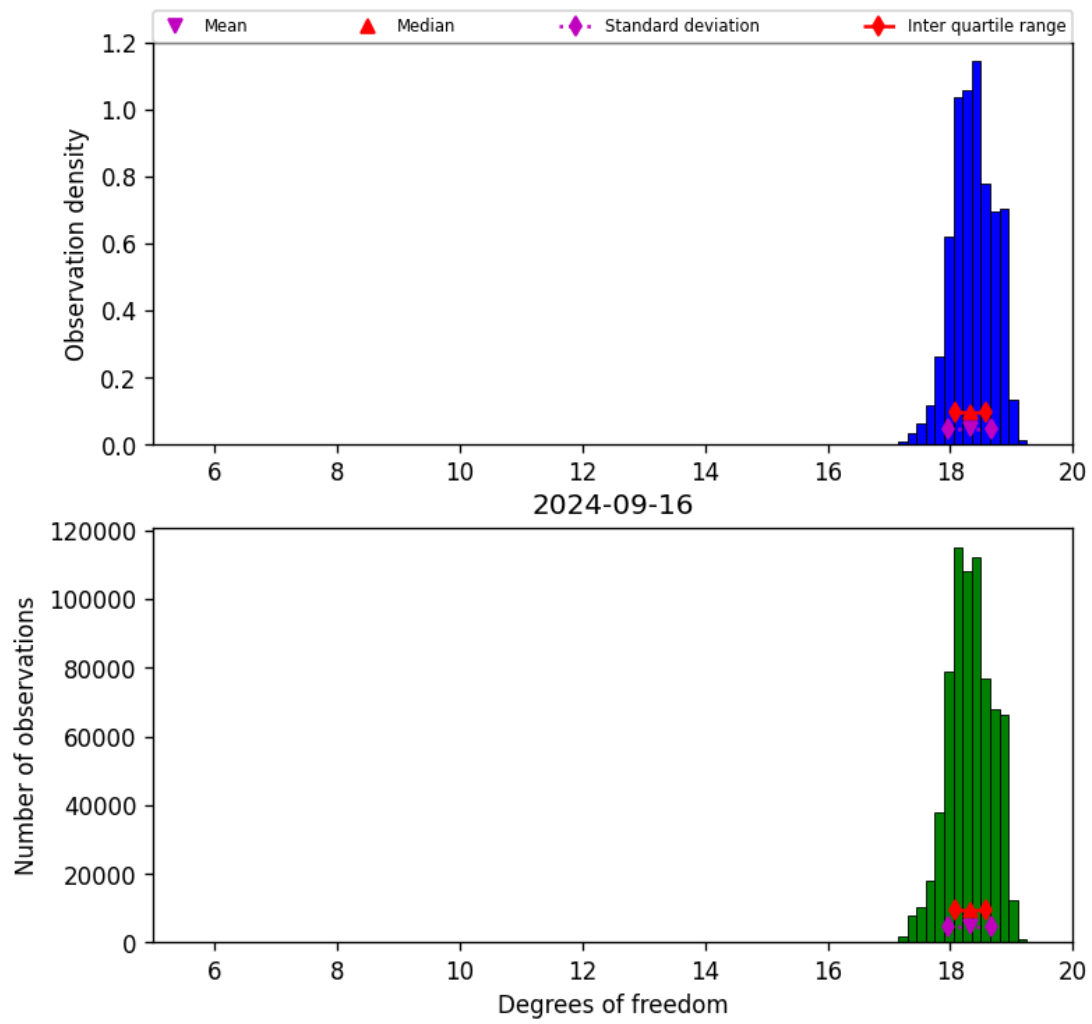
Figure 30: Histogram of “Degrees of freedom” for 2024-09-15 to 2024-09-17
