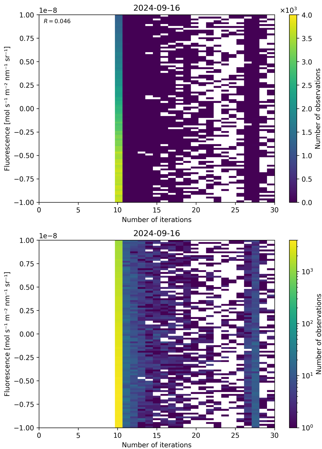
Figure 87: Scatter density plot of “Number of iterations” against “Fluorescence” for 2024-09-15 to 2024-09-17.
