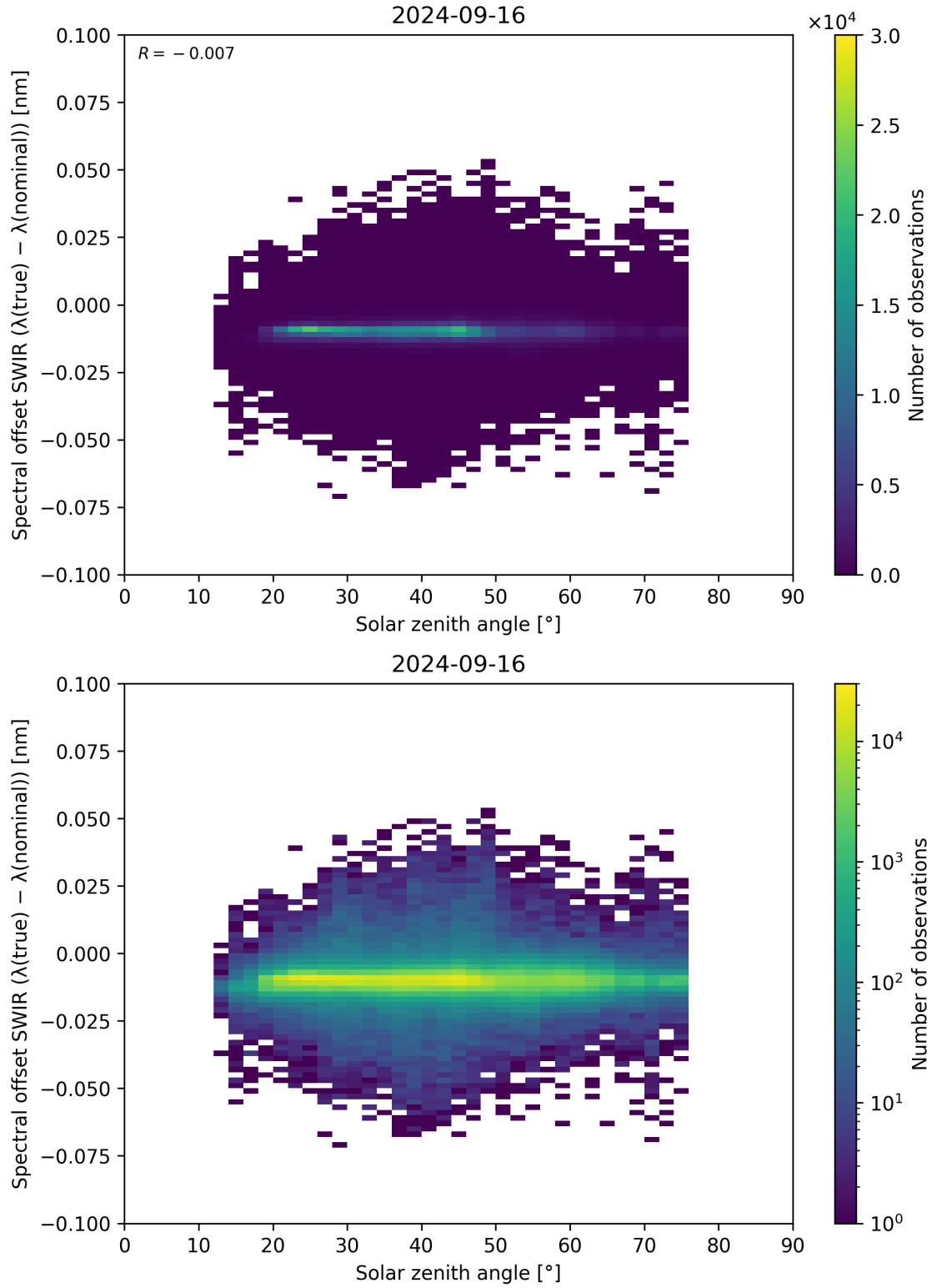
Figure 104: Scatter density plot of “Solar zenith angle” against “Spectral offset SWIR ( \lambda_{\text{true}} - \lambda_{\text{nominal}} )” for 2024-09-15 to 2024-09-17.
