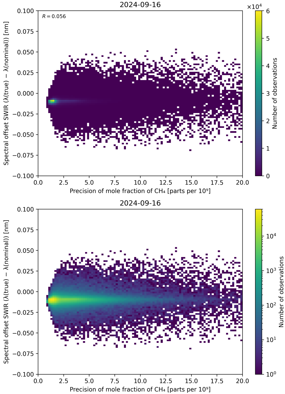
Figure 85: Scatter density plot of “Precision of mole fraction of CH 4 ” against “Spectral offset SWIR ( \lambda_{\text{true}} - \lambda_{\text{nominal}} )” for 2024-09-15 to 2024-09-17.
