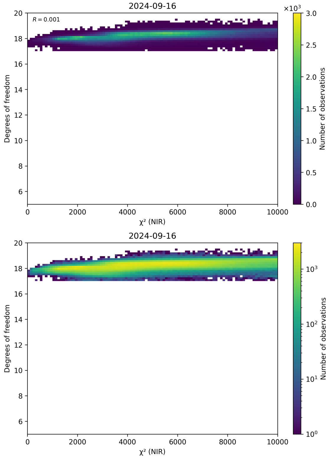
Figure 44: Scatter density plot of “ \chi^2 (NIR)” against “Degrees of freedom” for 2024-09-15 to 2024-09-17.
