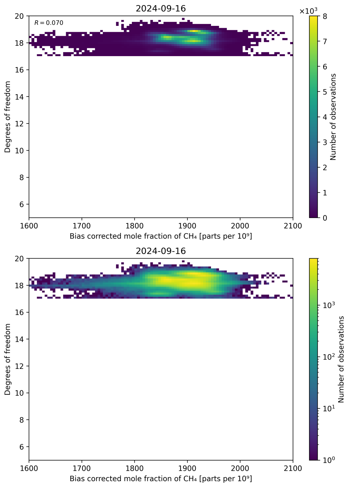
Figure 65: Scatter density plot of “Bias corrected mole fraction of CH 4 ” against “Degrees of freedom” for 2024-09-15 to 2024-09-17.
