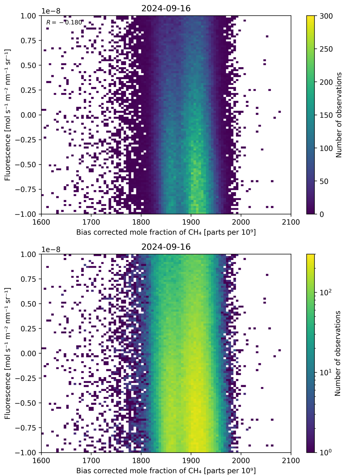
Figure 66: Scatter density plot of “Bias corrected mole fraction of CH 4 ” against “Fluorescence” for 2024-09-15 to 2024-09-17.
