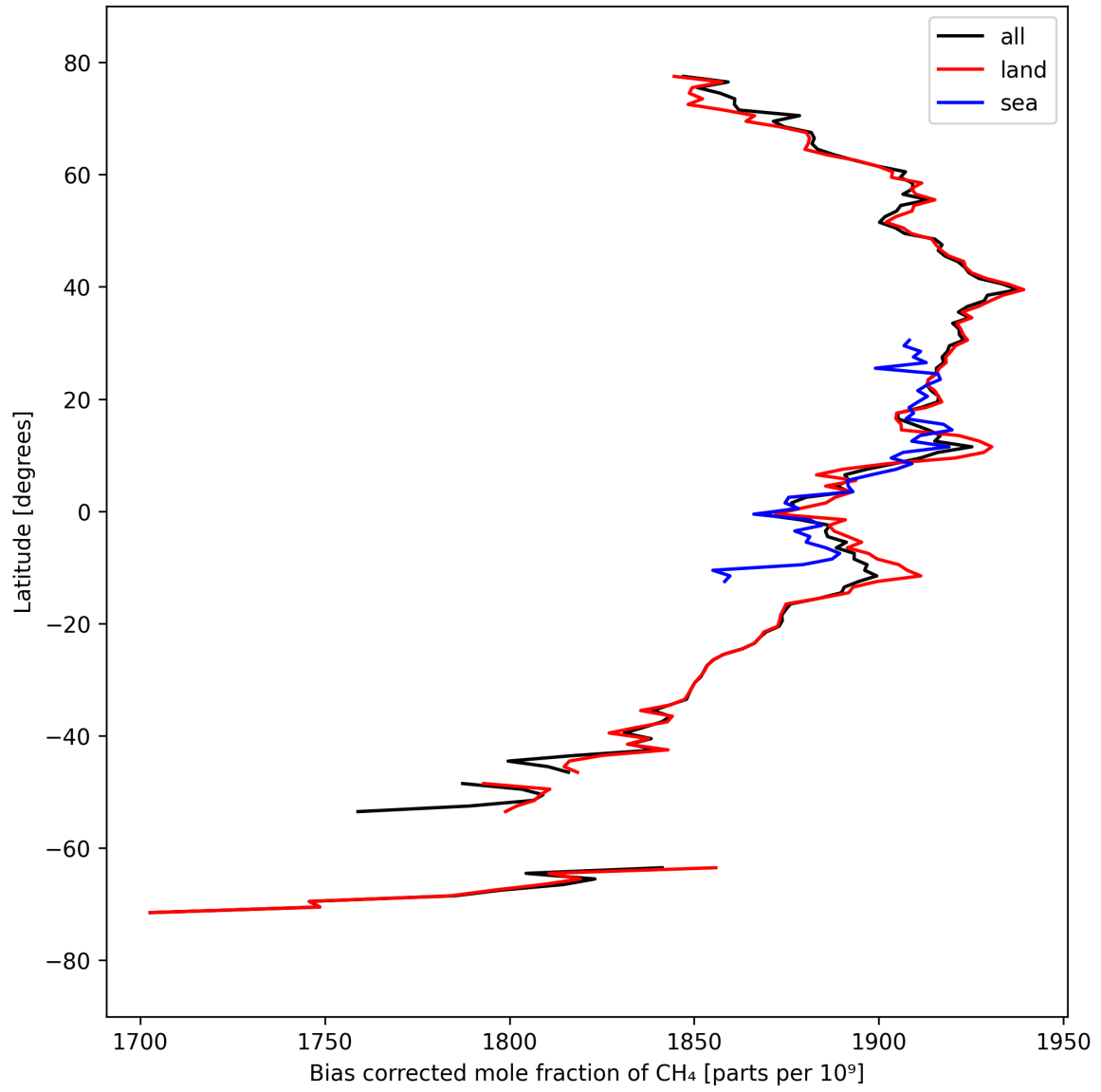
Figure 14: Zonal average of “Bias corrected mole fraction of CH 4 ” for 2024-09-15 to 2024-09-17.
