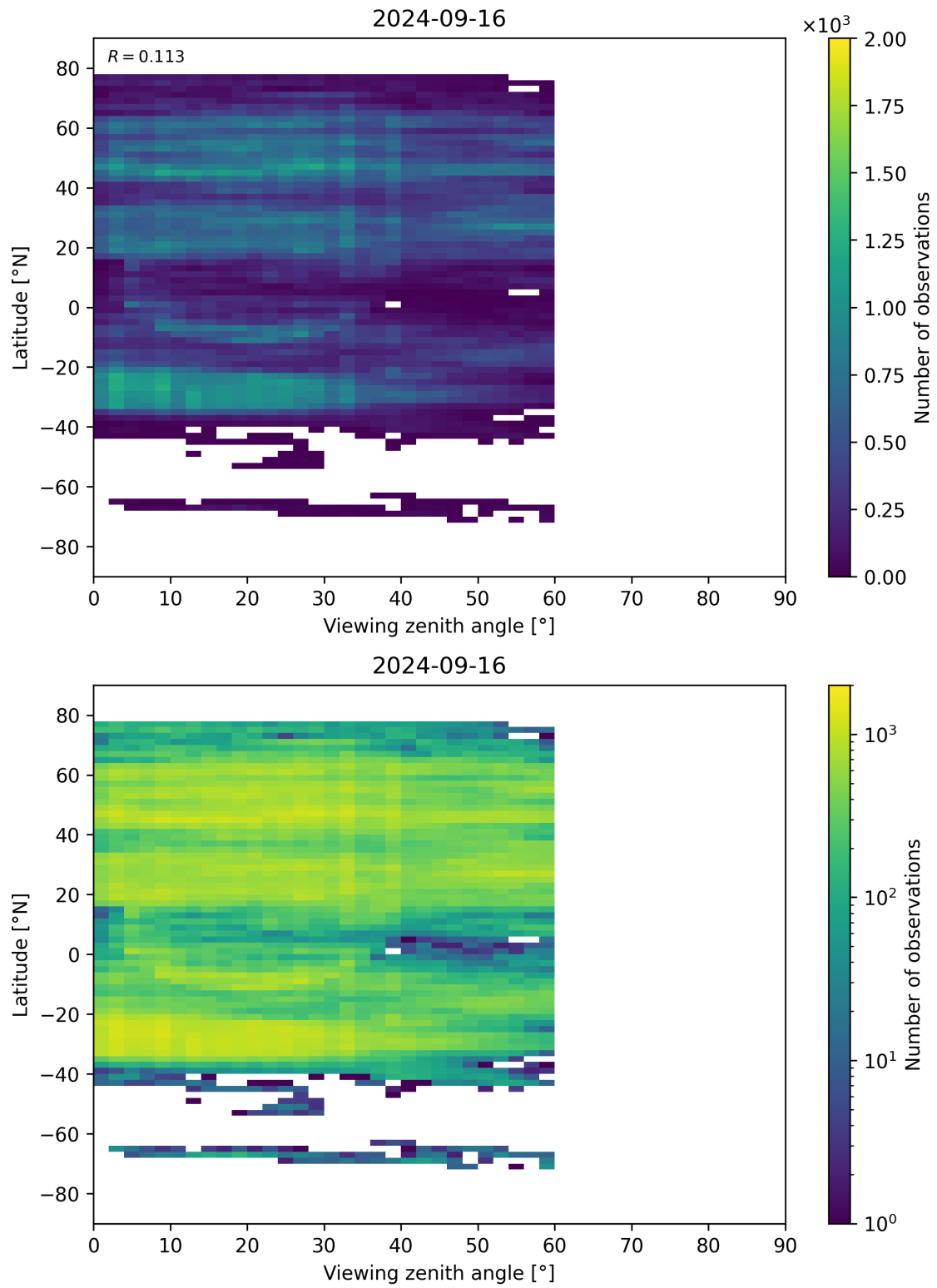
Figure 109: Scatter density plot of “Viewing zenith angle” against “Latitude” for 2024-09-15 to 2024-09-17.
