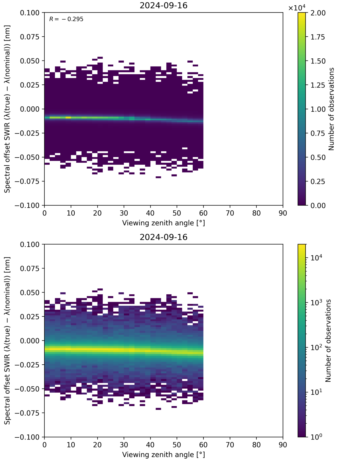
Figure 116: Scatter density plot of “Viewing zenith angle” against “Spectral offset SWIR ( \lambda_{\text{true}} - \lambda_{\text{nominal}} )” for 2024-09-15 to 2024-09-17.
