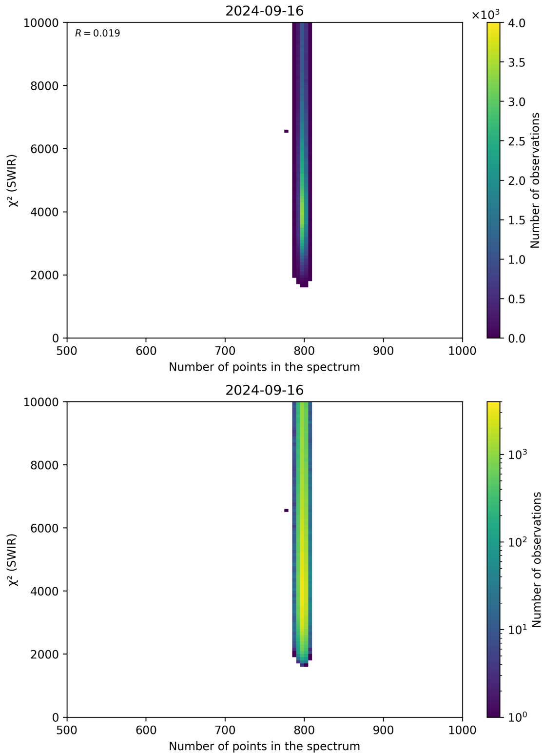
Figure 89: Scatter density plot of “Number of points in the spectrum” against “ \chi^2 (SWIR)” for 2024-09-15 to 2024-09-17.
