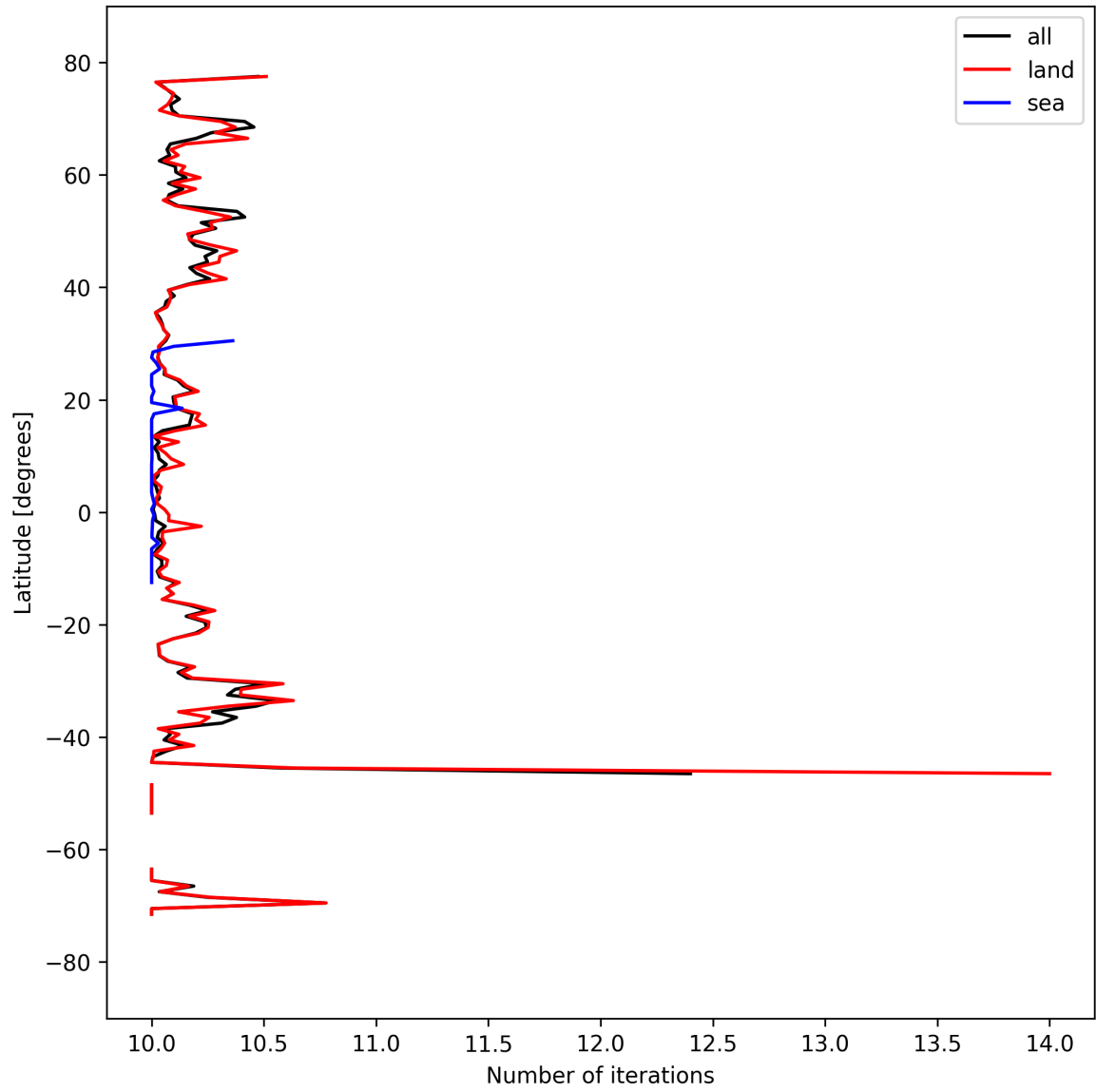
Figure 20: Zonal average of “Number of iterations” for 2024-09-15 to 2024-09-17.
