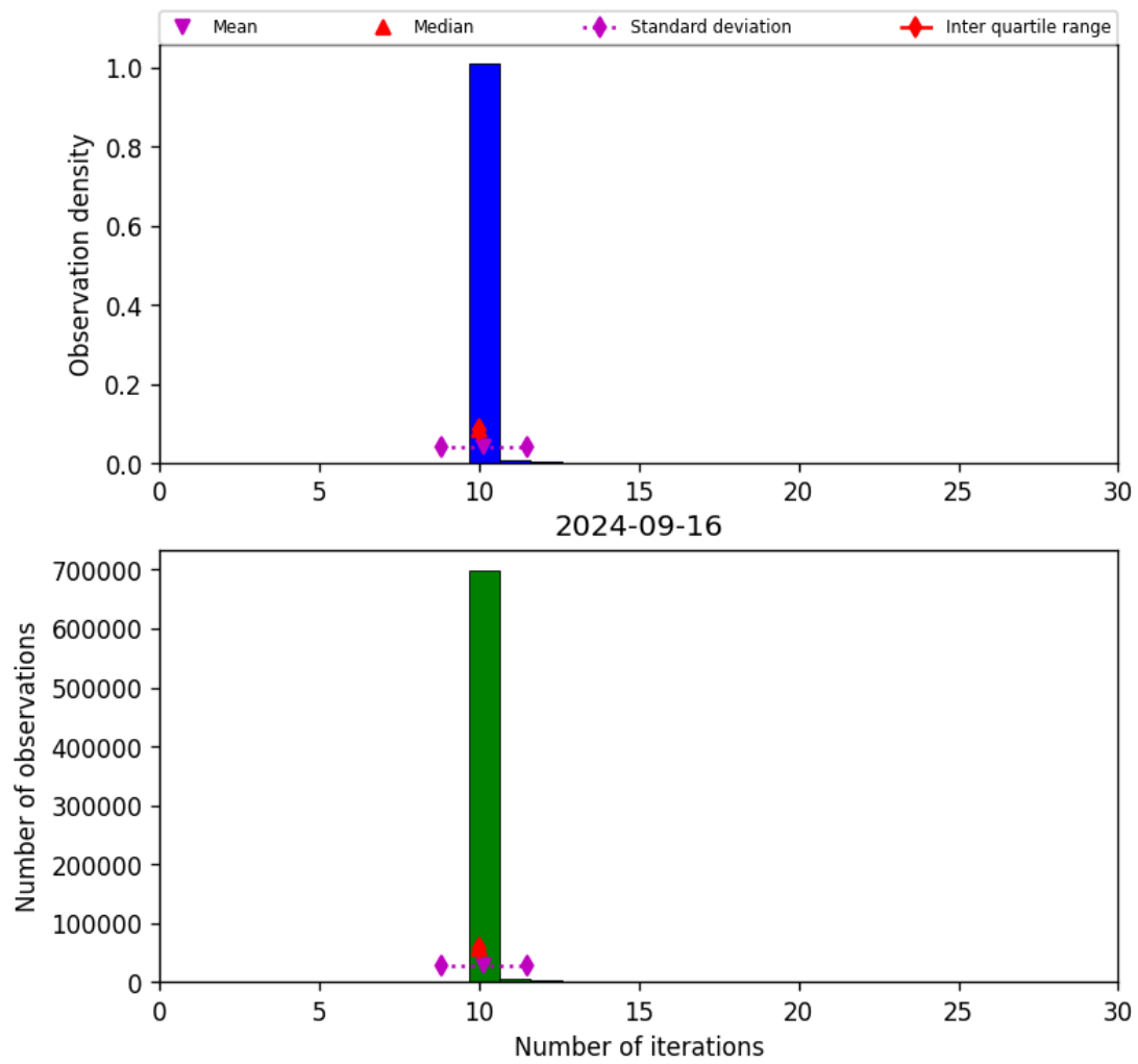
Figure 31: Histogram of “Number of iterations” for 2024-09-15 to 2024-09-17
