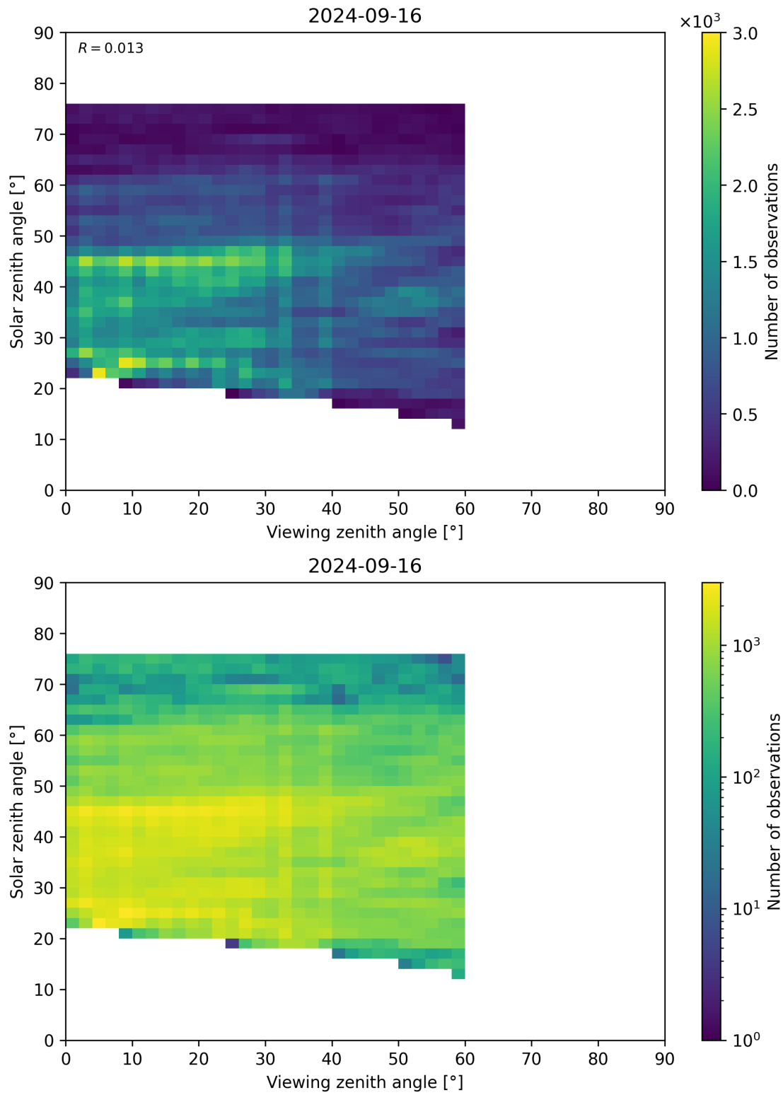
Figure 115: Scatter density plot of “Viewing zenith angle” against “Solar zenith angle” for 2024-09-15 to 2024-09-17.
