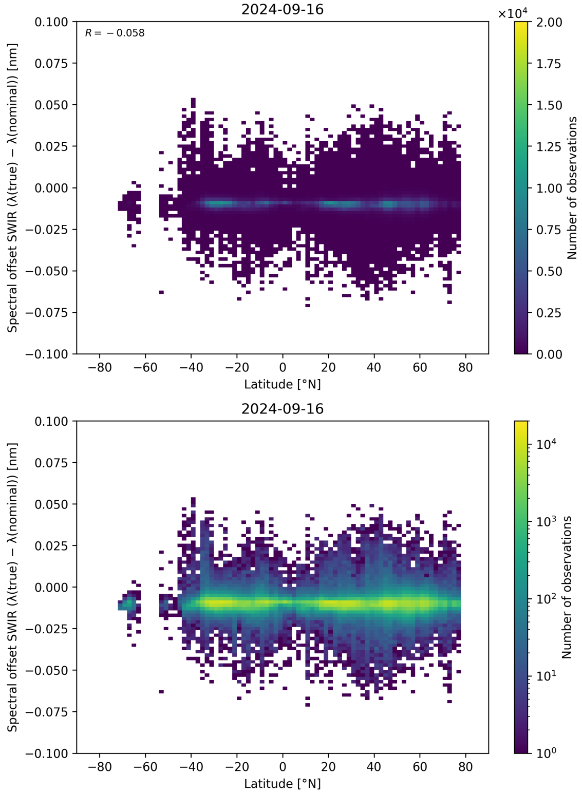
Figure 62: Scatter density plot of “Latitude” against “Spectral offset SWIR ( \lambda_{\text{true}} - \lambda_{\text{nominal}} )” for 2024-09-15 to 2024-09-17.
