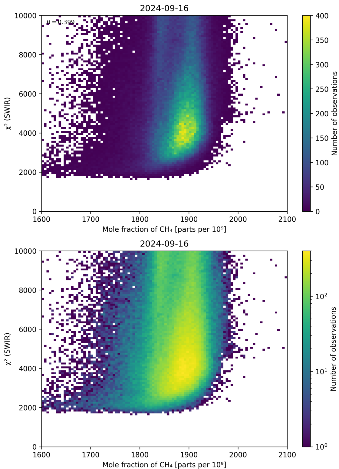
Figure 71: Scatter density plot of “Mole fraction of \text{CH}_4 ” against “ \chi^2 (SWIR)” for 2024-09-15 to 2024-09-17.
