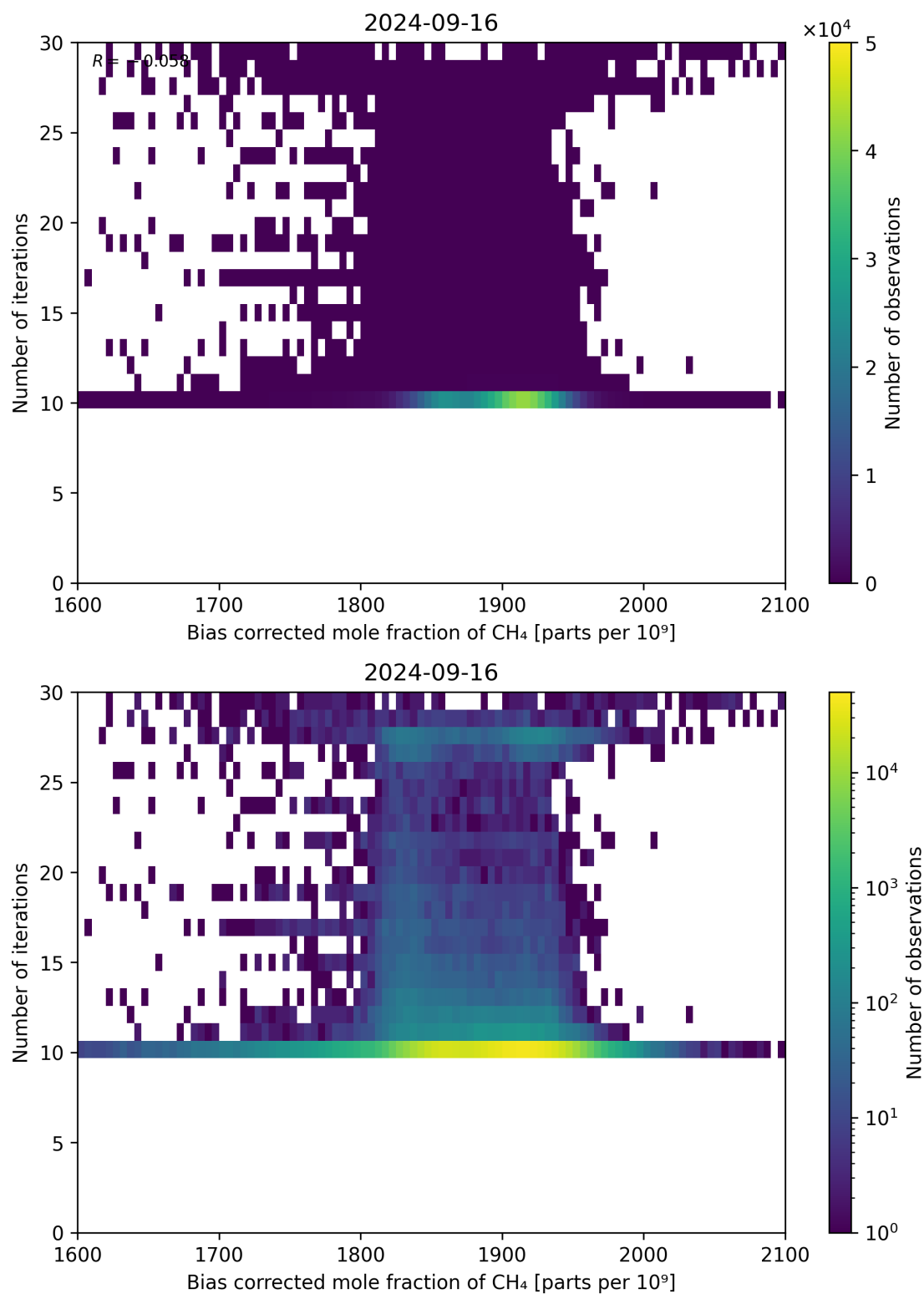
Figure 67: Scatter density plot of “Bias corrected mole fraction of CH 4 ” against “Number of iterations” for 2024-09-15 to 2024-09-17.
