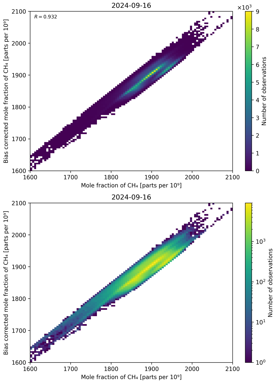
Figure 74: Scatter density plot of “Mole fraction of CH 4 ” against “Bias corrected mole fraction of CH 4 ” for 2024-09-15 to 2024-09-17.
