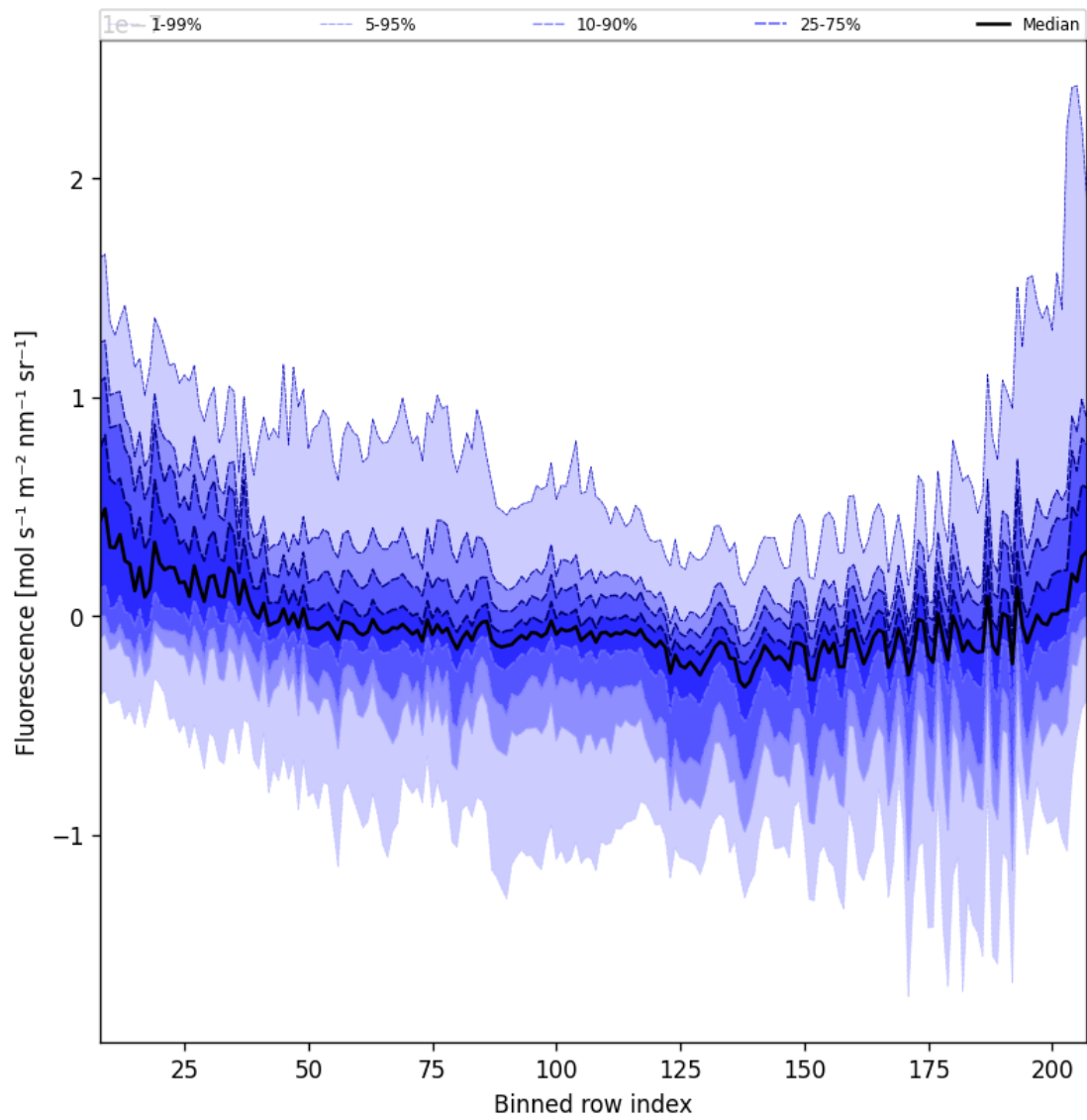
Figure 43: Along track statistics of “Fluorescence” for 2024-09-15 to 2024-09-17
