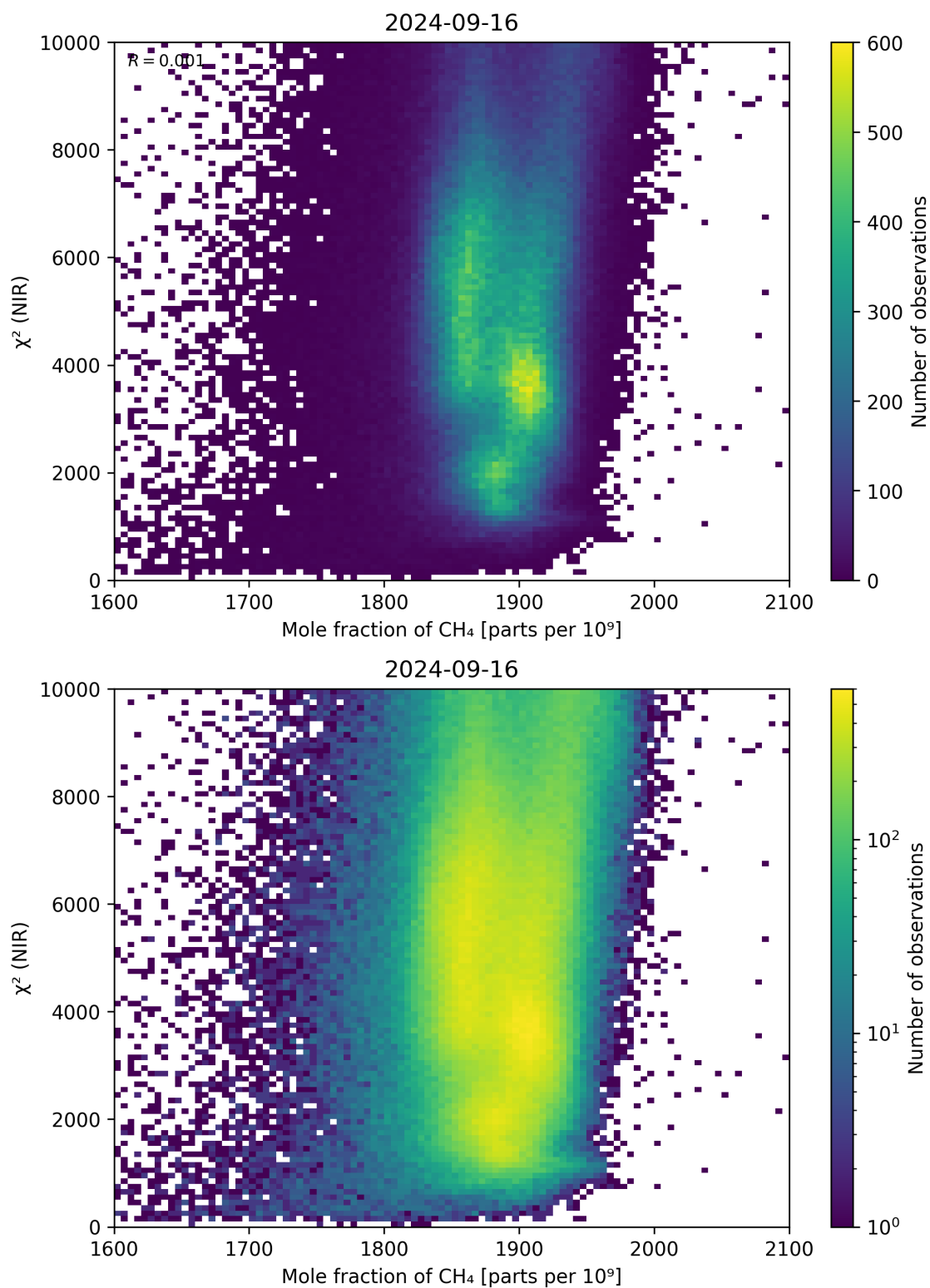
Figure 70: Scatter density plot of “Mole fraction of \text{CH}_4 ” against “ \chi^2 (NIR)” for 2024-09-15 to 2024-09-17.
