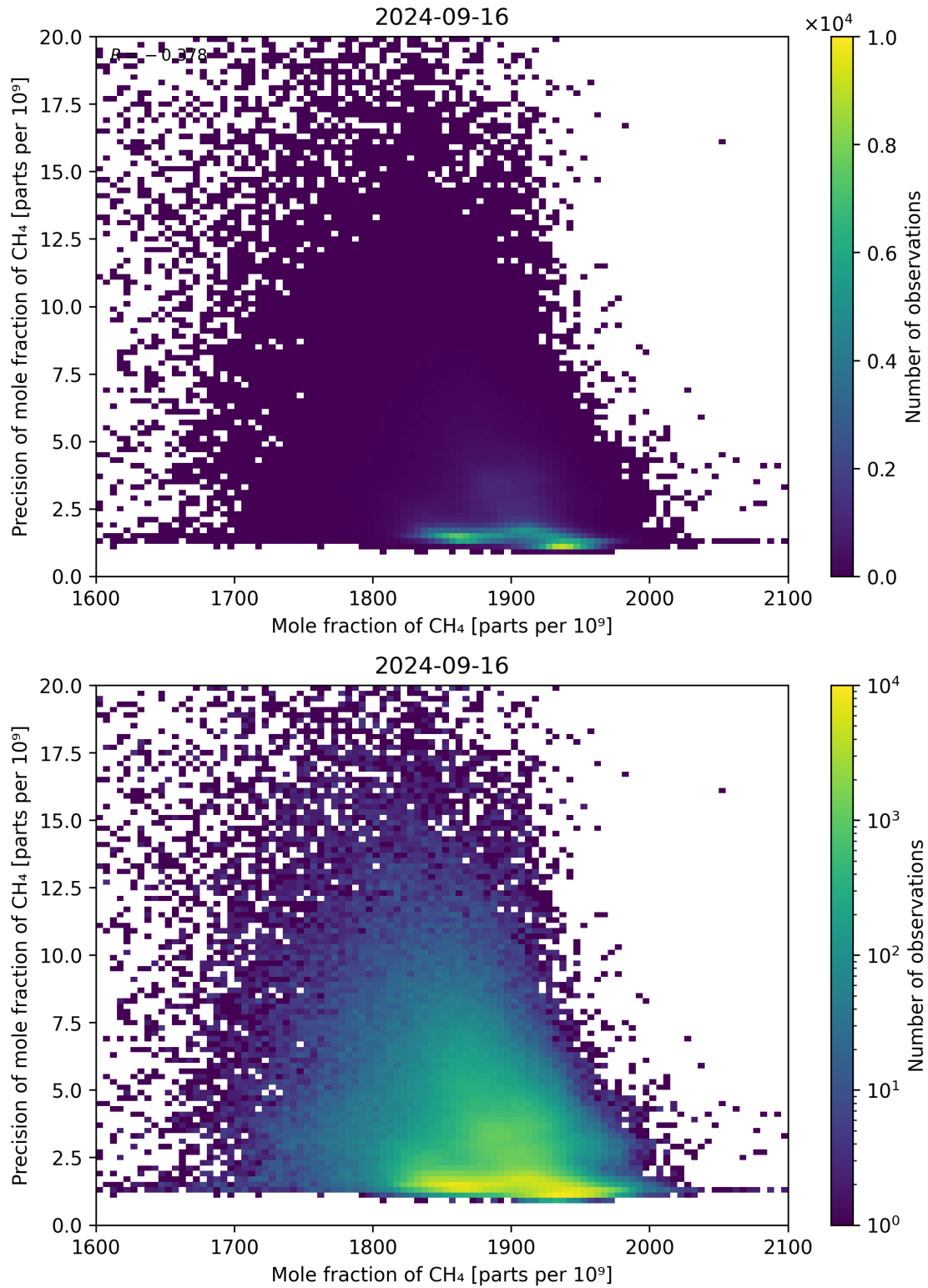
Figure 75: Scatter density plot of “Mole fraction of CH 4 ” against “Precision of mole fraction of CH 4 ” for 2024-09-15 to 2024-09-17.
