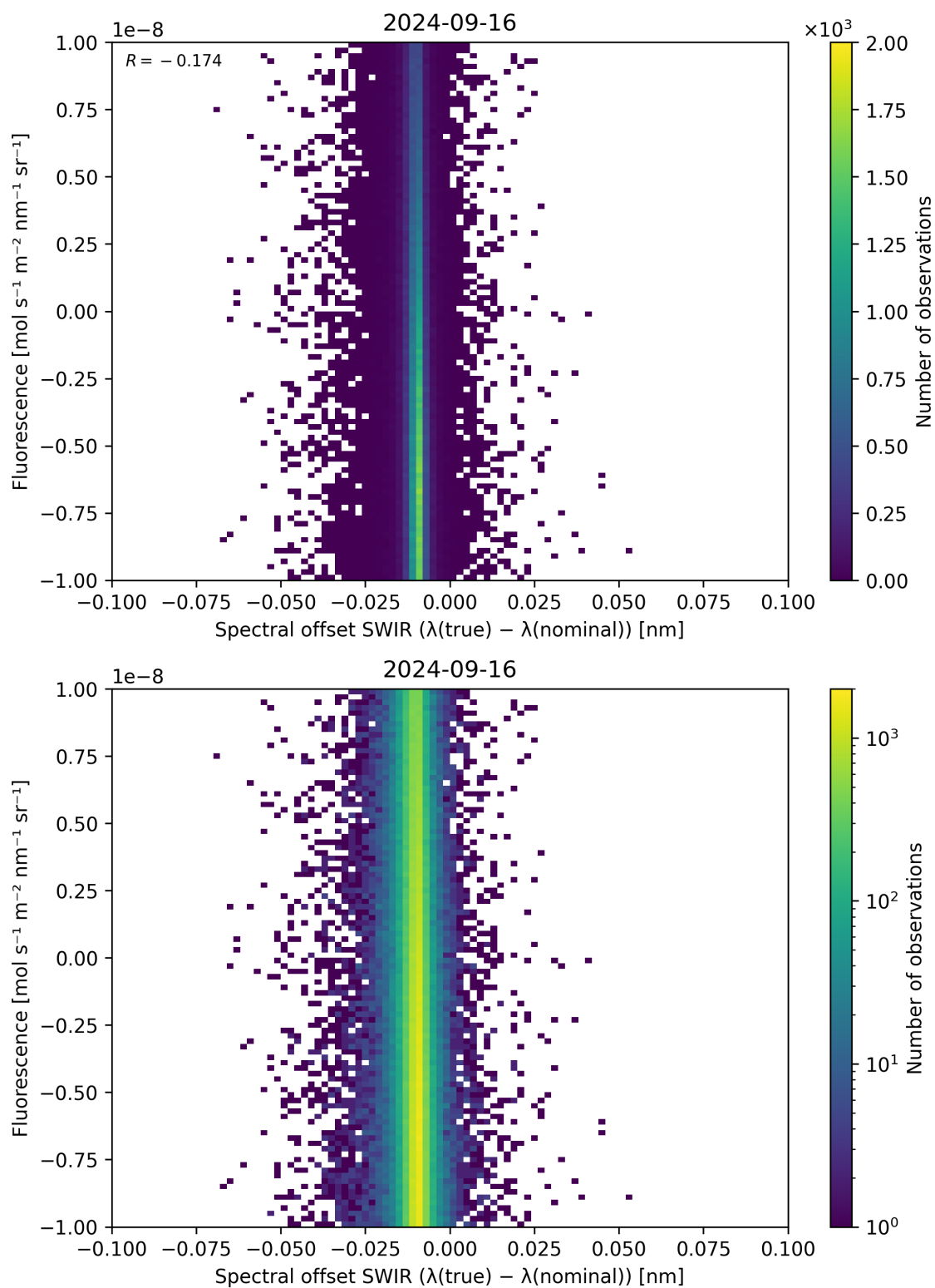
Figure 120: Scatter density plot of “Spectral offset SWIR ( \lambda_{\text{true}} - \lambda_{\text{nominal}} )” against “Fluorescence” for 2024-09-15 to 2024-09-17.
