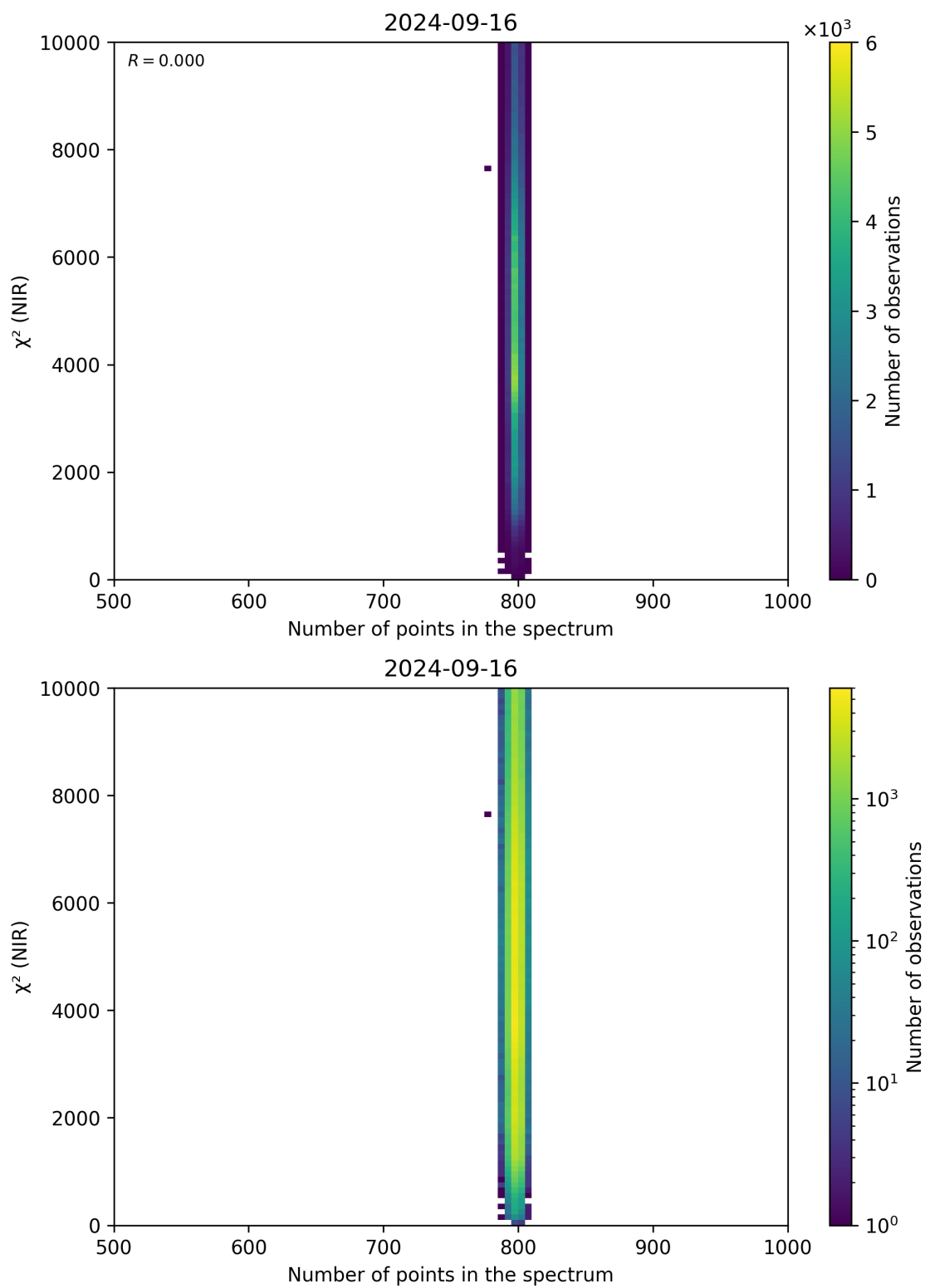
Figure 88: Scatter density plot of “Number of points in the spectrum” against “ \chi^2 (NIR)” for 2024-09-15 to 2024-09-17.
