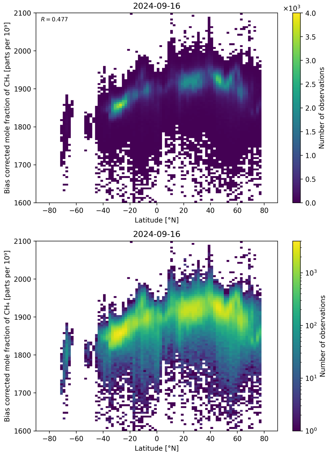
Figure 58: Scatter density plot of “Latitude” against “Bias corrected mole fraction of \text{CH}_4 ” for 2024-09-15 to 2024-09-17.
