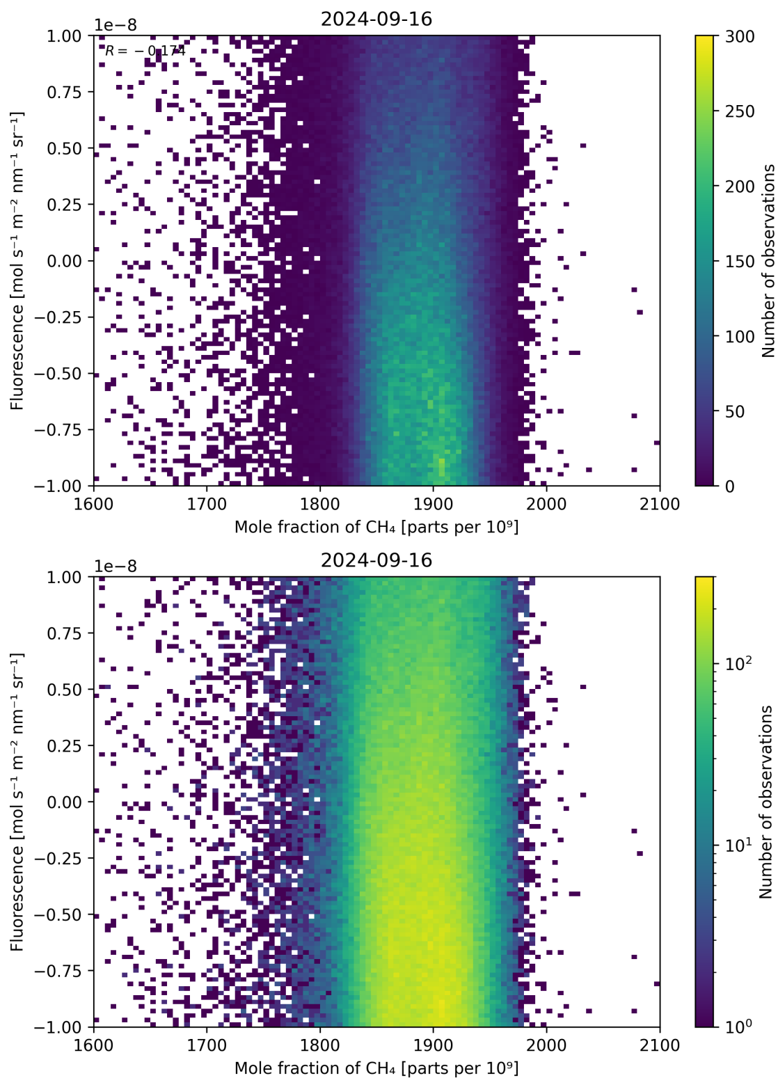
Figure 73: Scatter density plot of “Mole fraction of \text{CH}_4 ” against “Fluorescence” for 2024-09-15 to 2024-09-17.
