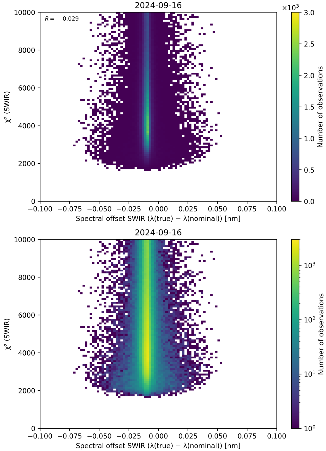
Figure 118: Scatter density plot of “Spectral offset SWIR ( \lambda_{\text{true}} - \lambda_{\text{nominal}} )” against “ \chi^2 (SWIR)” for 2024-09-15 to 2024-09-17.
