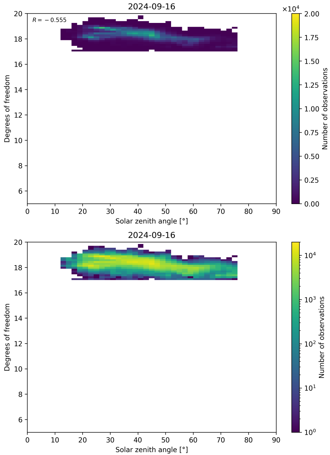
Figure 96: Scatter density plot of “Solar zenith angle” against “Degrees of freedom” for 2024-09-15 to 2024-09-17.
