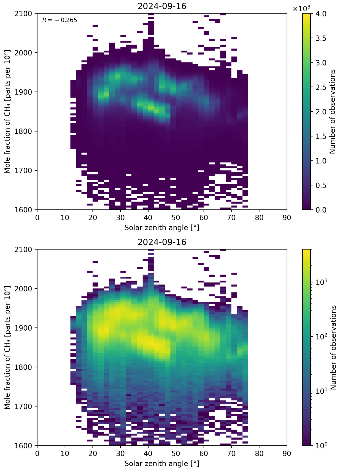
Figure 99: Scatter density plot of “Solar zenith angle” against “Mole fraction of \text{CH}_4 ” for 2024-09-15 to 2024-09-17.
