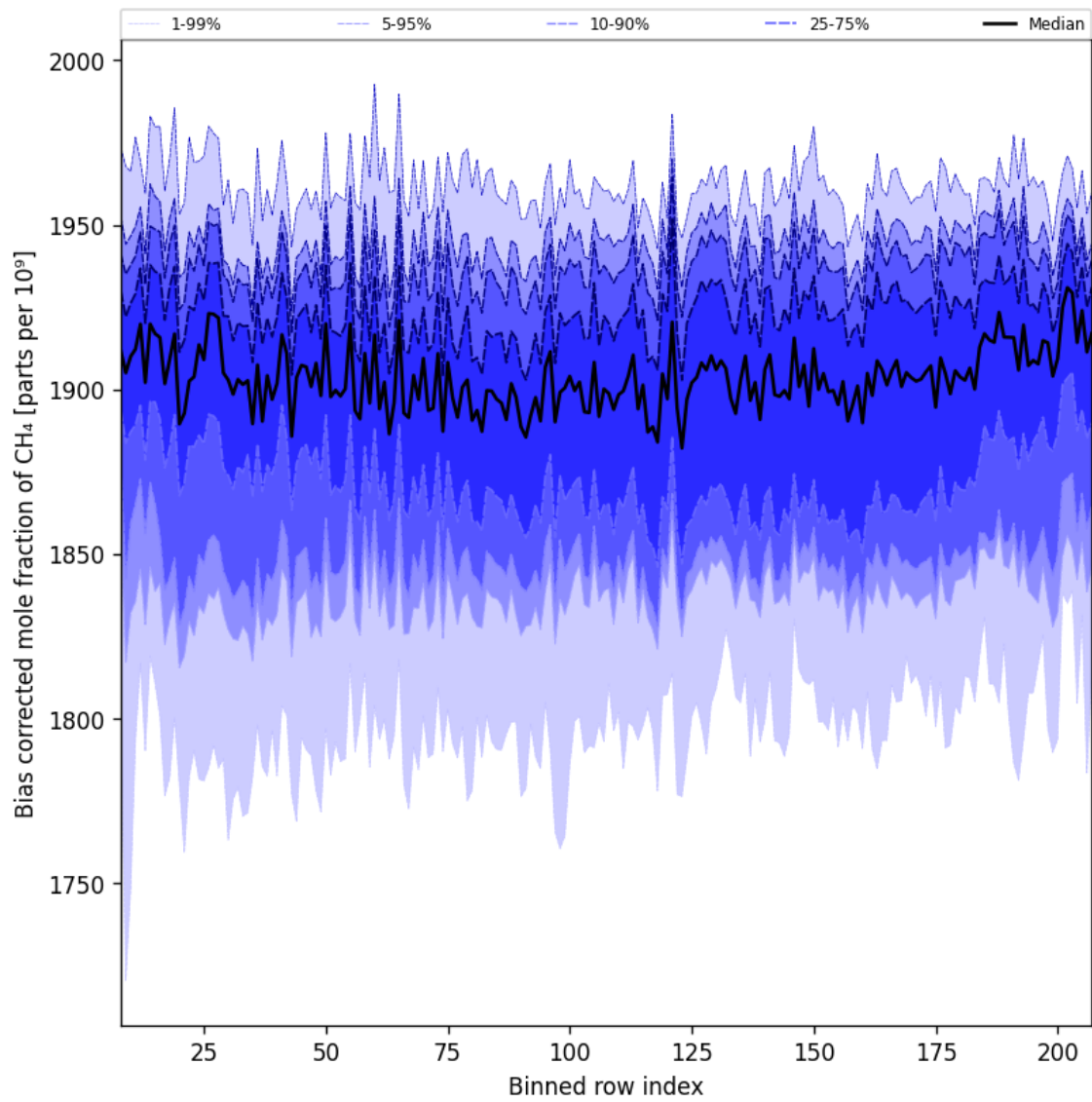
Figure 36: Along track statistics of “Bias corrected mole fraction of CH 4 ” for 2024-09-15 to 2024-09-17
