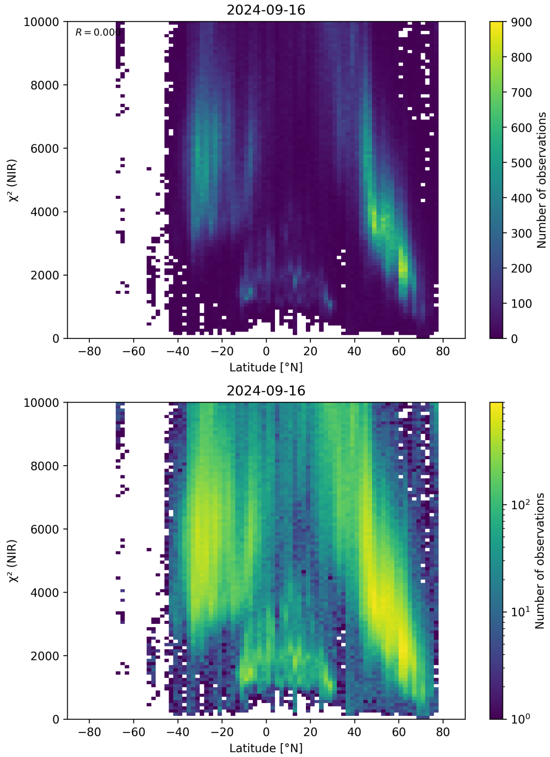
Figure 53: Scatter density plot of “Latitude” against “ \chi^2 (NIR)” for 2024-09-15 to 2024-09-17.
