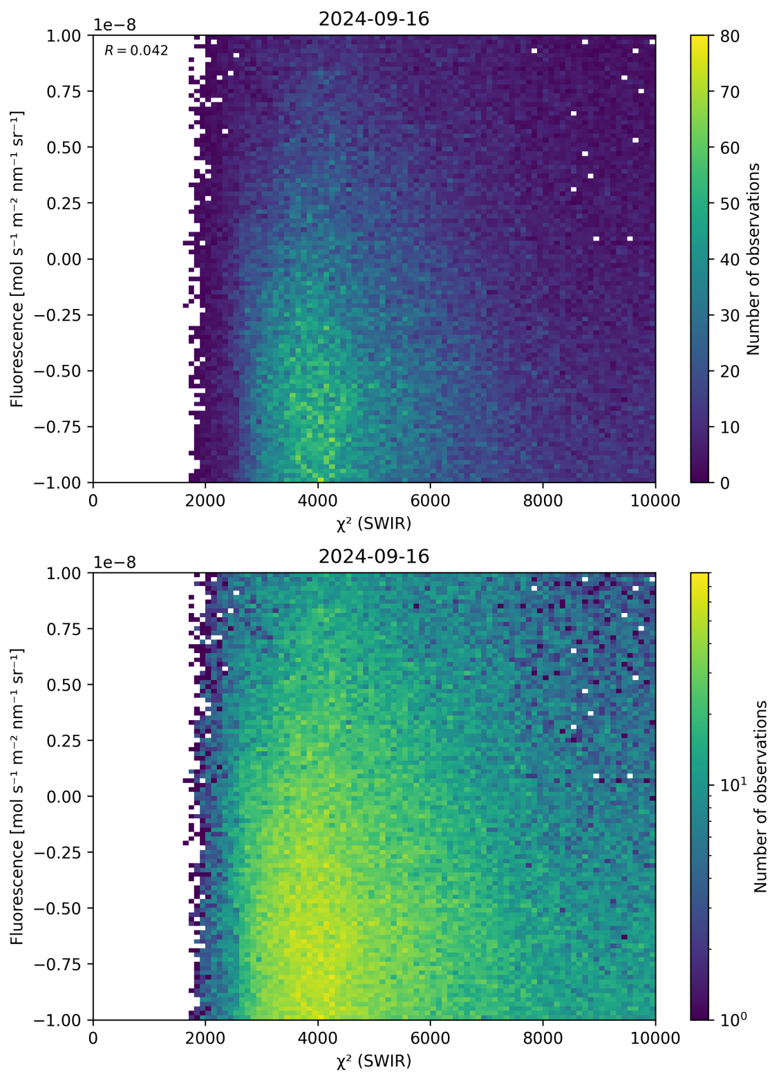
Figure 49: Scatter density plot of “ \chi^2 (SWIR)” against “Fluorescence” for 2024-09-15 to 2024-09-17.
