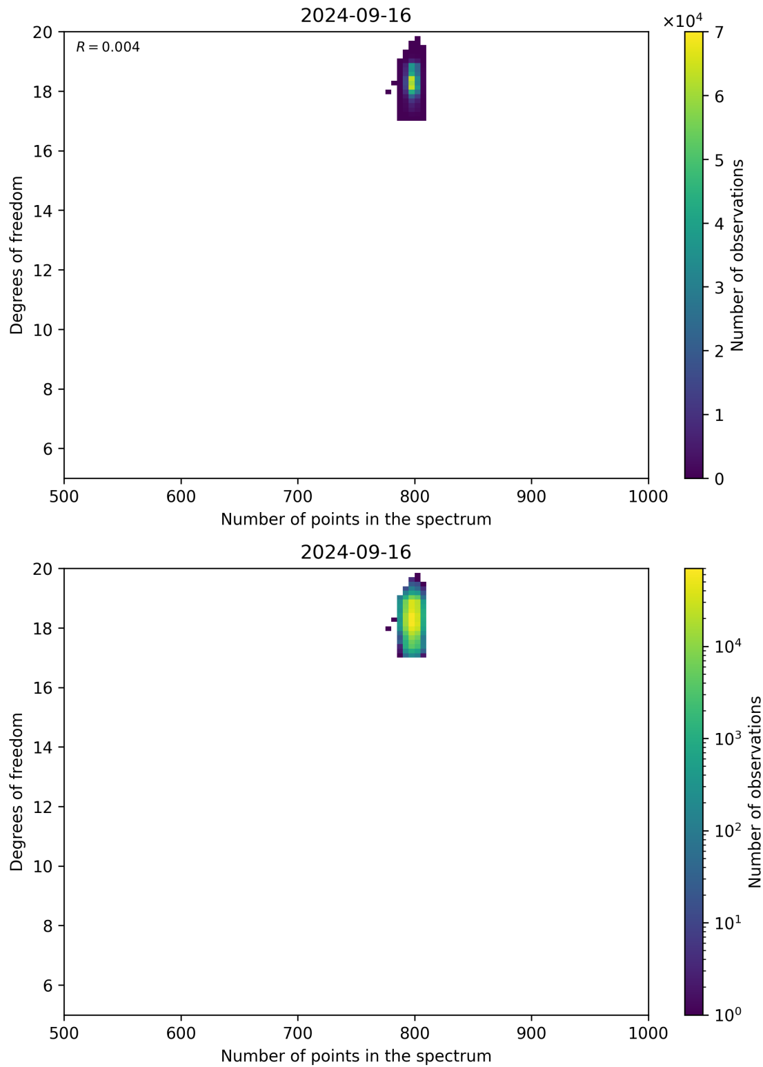
Figure 90: Scatter density plot of “Number of points in the spectrum” against “Degrees of freedom” for 2024-09-15 to 2024-09-17.
