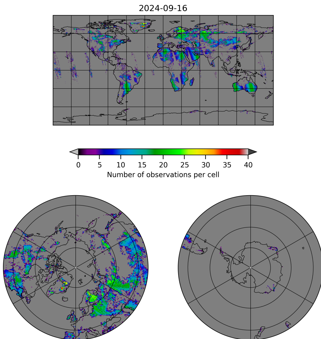
Figure 10: Map of the number of observations for 2024-09-15 to 2024-09-17
