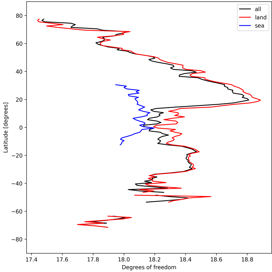
Figure 19: Zonal average of “Degrees of freedom” for 2024-09-15 to 2024-09-17.
