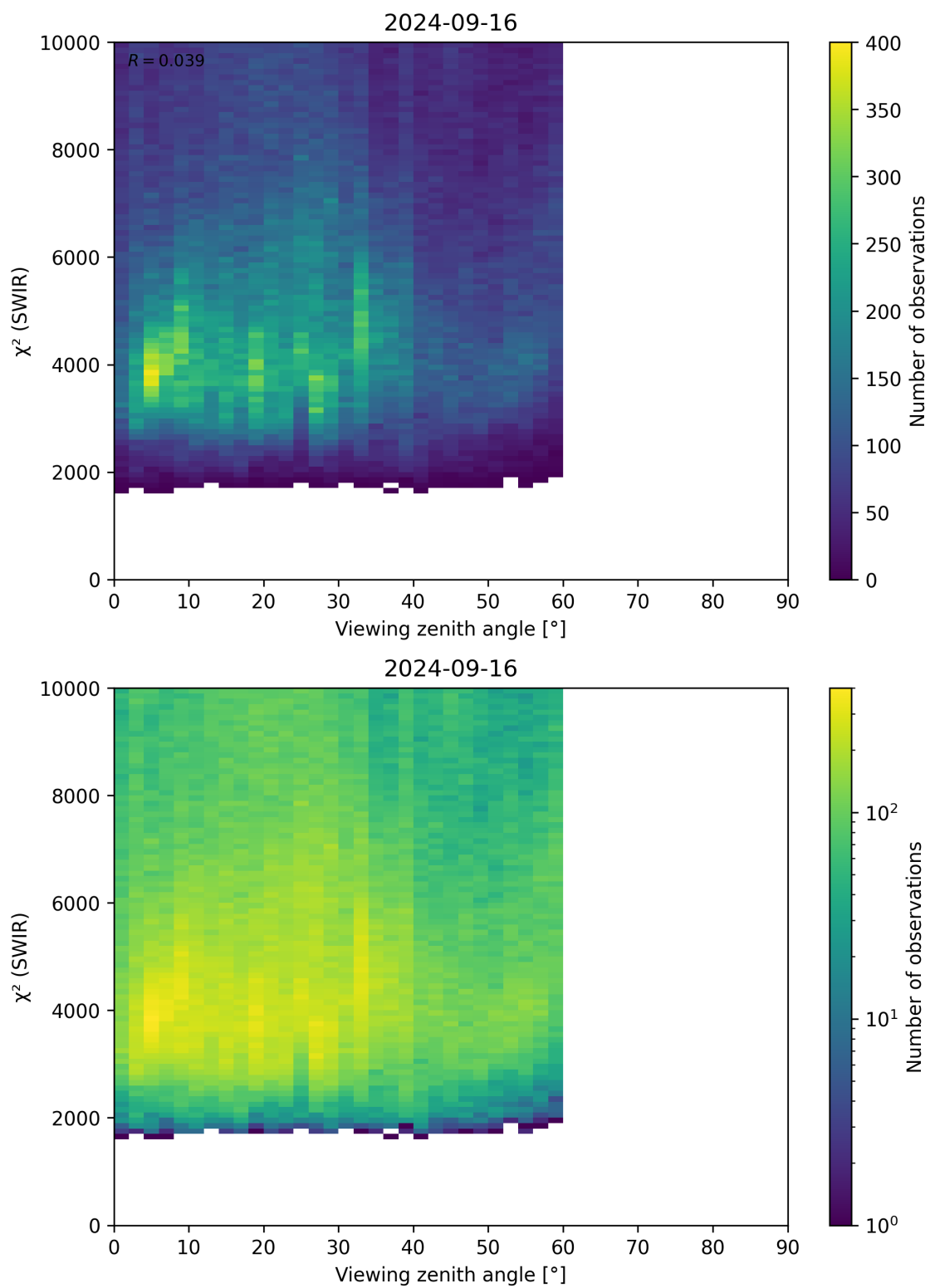
Figure 106: Scatter density plot of “Viewing zenith angle” against “ \chi^2 (SWIR)” for 2024-09-15 to 2024-09-17.
