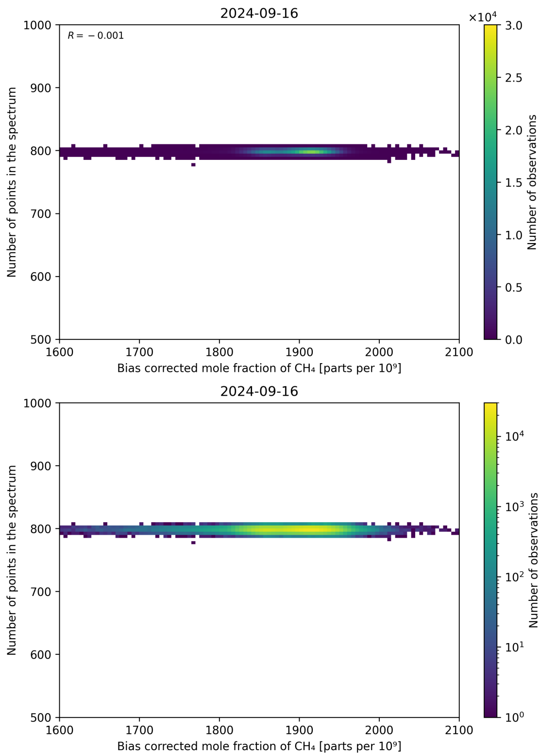
Figure 68: Scatter density plot of “Bias corrected mole fraction of CH 4 ” against “Number of points in the spectrum” for 2024-09-15 to 2024-09-17.
