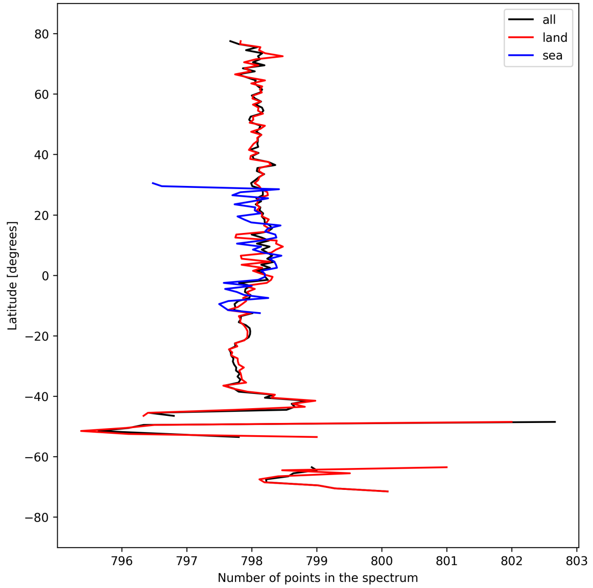
Figure 15: Zonal average of “Number of points in the spectrum” for 2024-09-15 to 2024-09-17.
