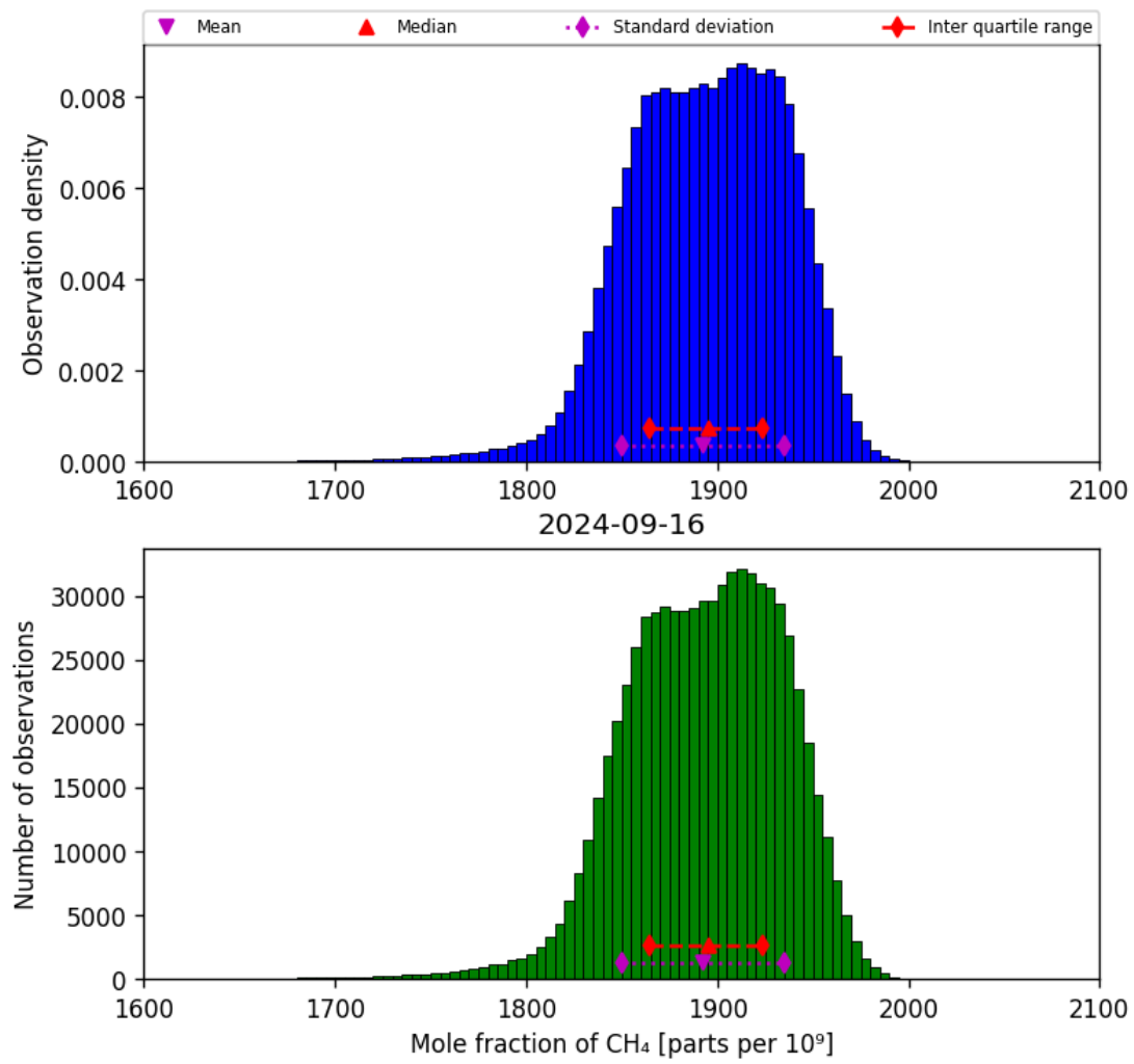
Figure 23: Histogram of “Mole fraction of CH 4 ” for 2024-09-15 to 2024-09-17
