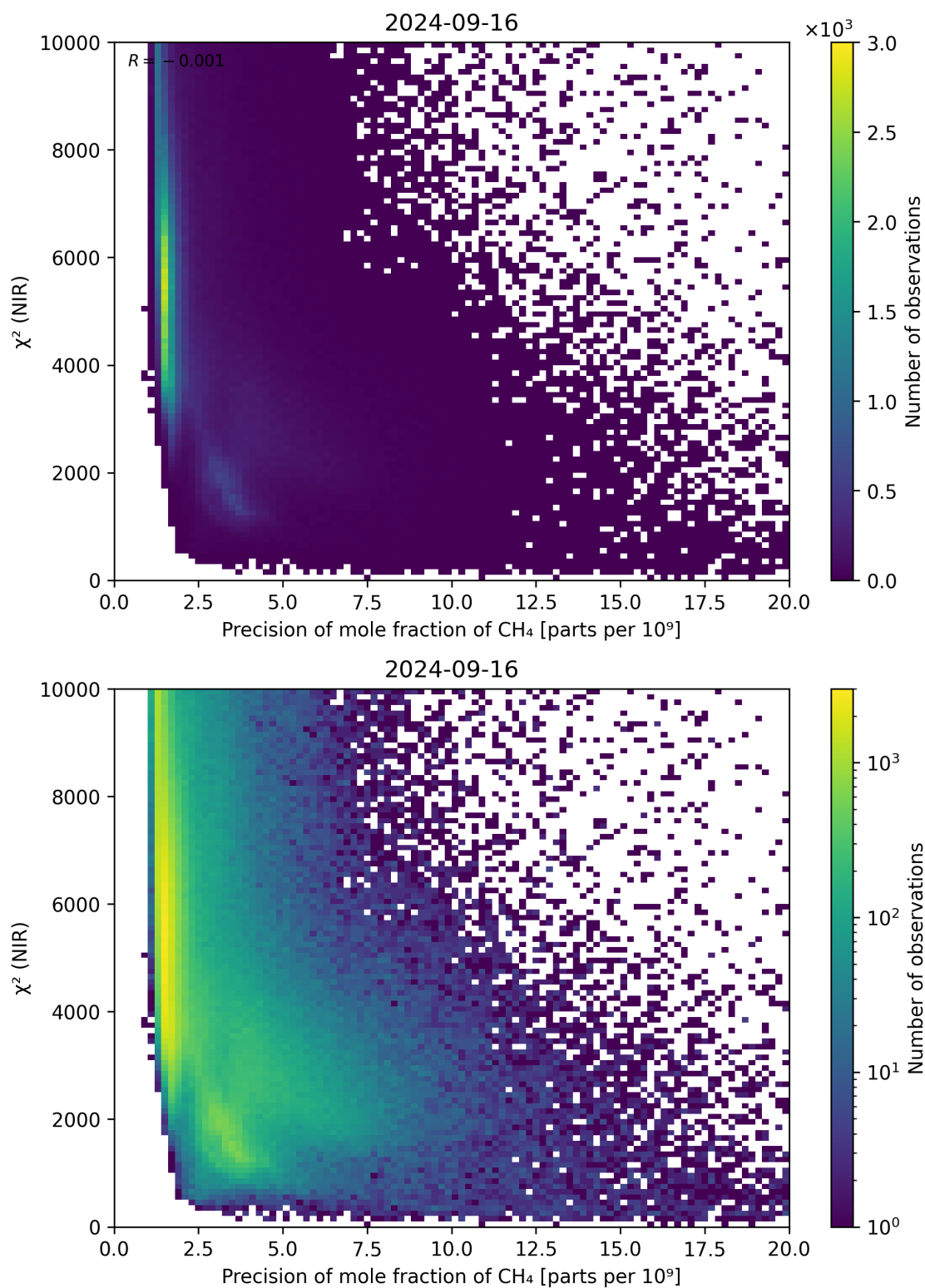
Figure 78: Scatter density plot of “Precision of mole fraction of CH 4 ” against “ \chi^2 (NIR)” for 2024-09-15 to 2024-09-17.
