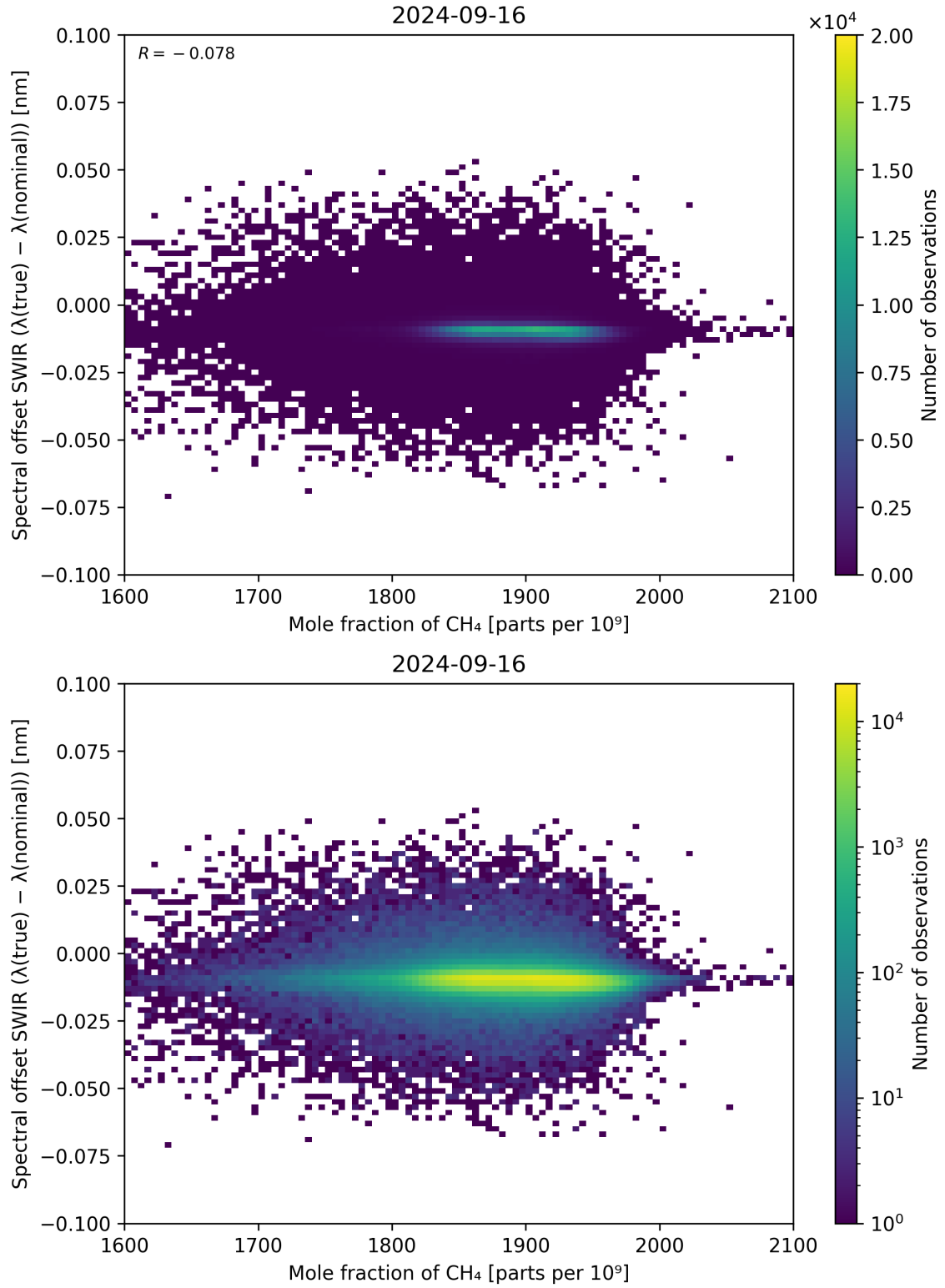
Figure 86: Scatter density plot of “Mole fraction of CH 4 ” against “Spectral offset SWIR ( \lambda_{\text{true}} - \lambda_{\text{nominal}} )” for 2024-09-15 to 2024-09-17.
