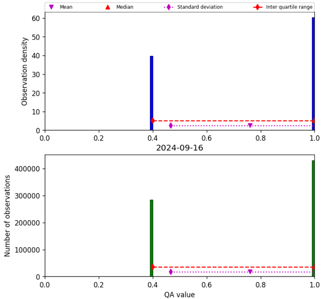
Figure 22: Histogram of “QA value” for 2024-09-15 to 2024-09-17
