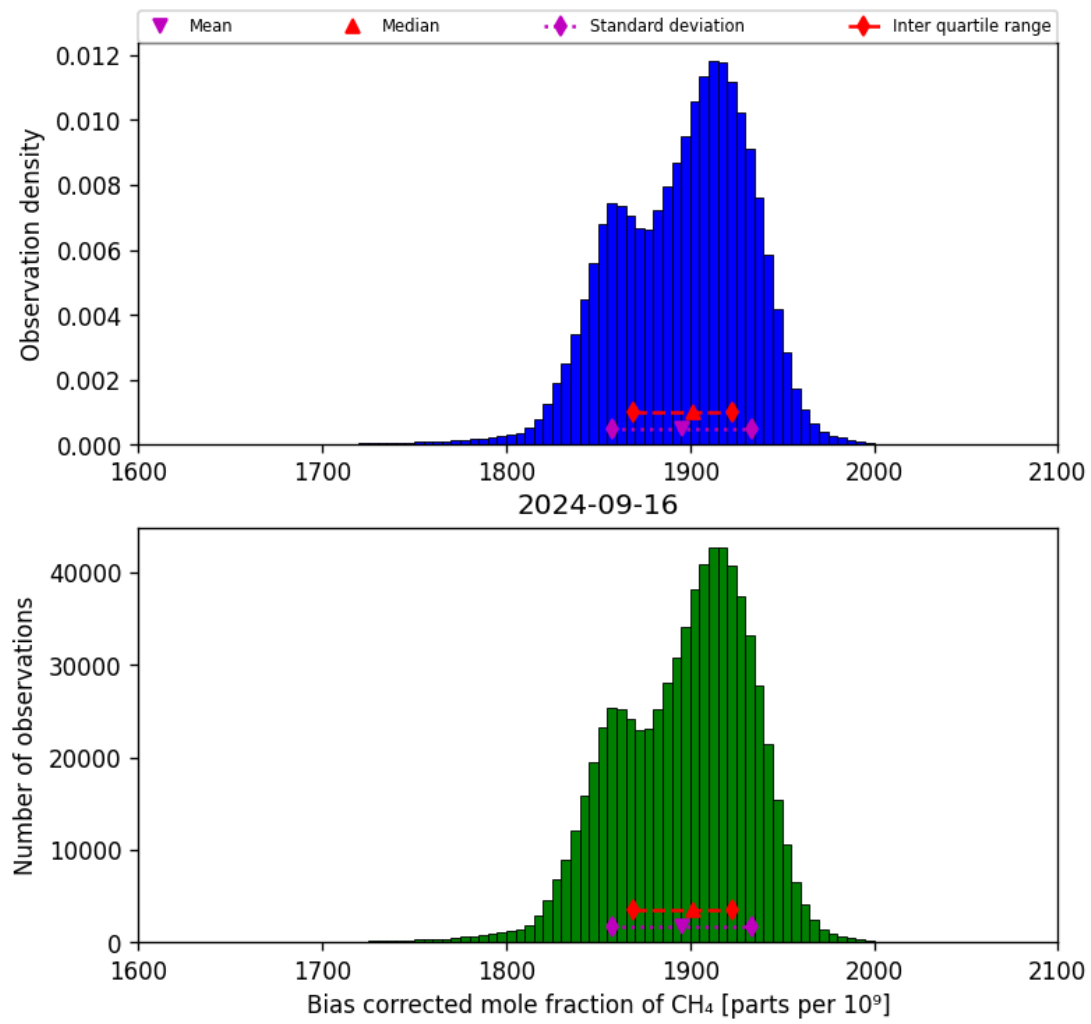
Figure 25: Histogram of “Bias corrected mole fraction of CH 4 ” for 2024-09-15 to 2024-09-17
