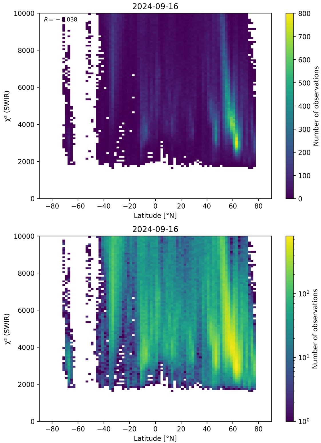
Figure 54: Scatter density plot of “Latitude” against “ \chi^2 (SWIR)” for 2024-09-15 to 2024-09-17.
