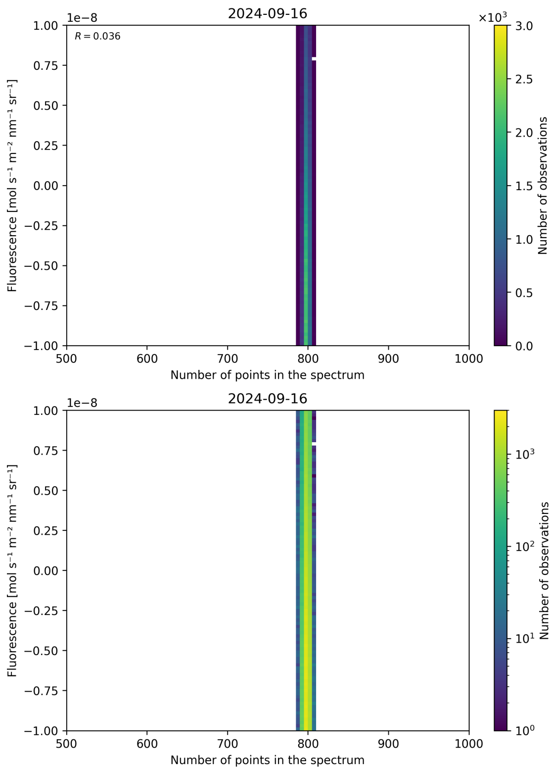
Figure 91: Scatter density plot of “Number of points in the spectrum” against “Fluorescence” for 2024-09-15 to 2024-09-17.
