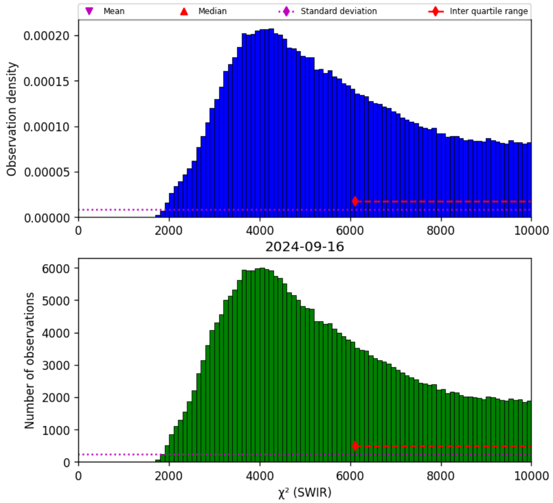
Figure 28: Histogram of " \chi^2 (SWIR)" for 2024-09-15 to 2024-09-17
