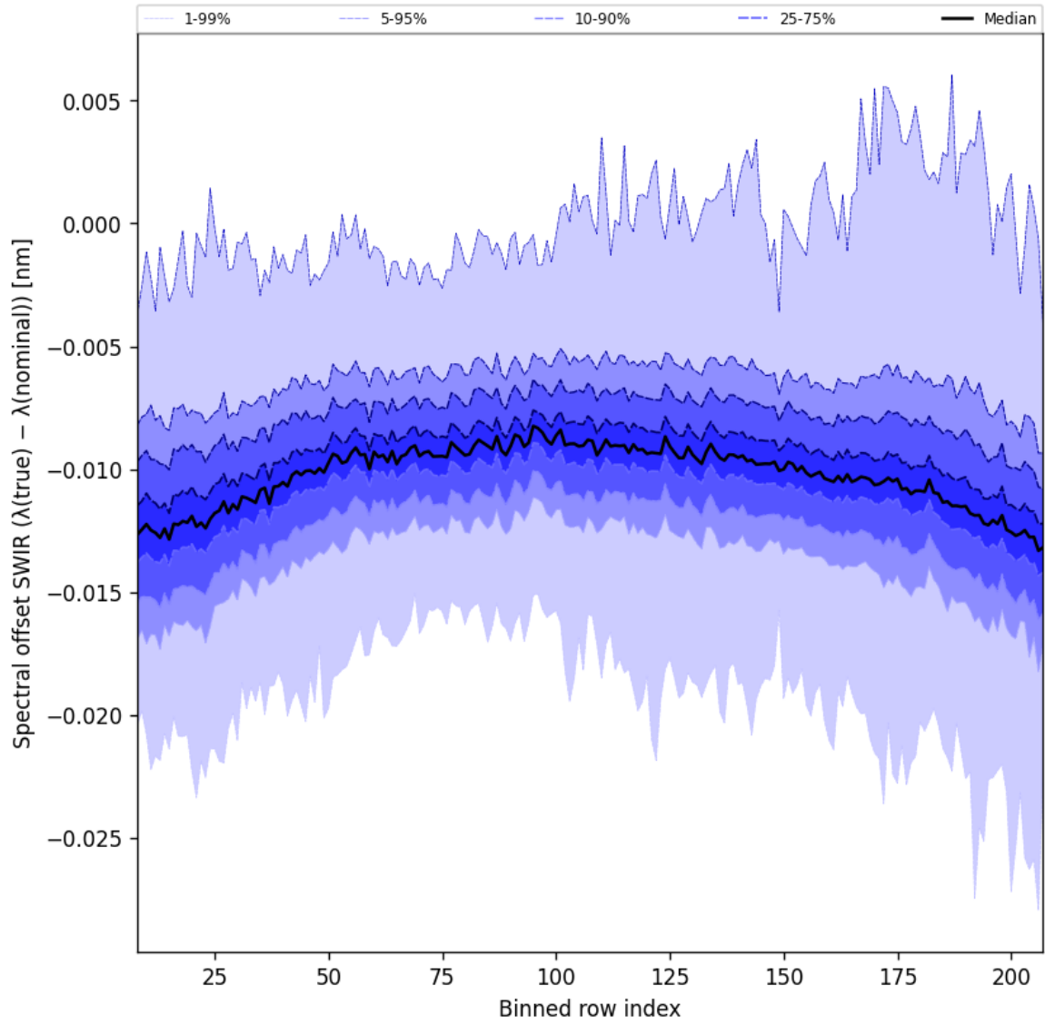
Figure 38: Along track statistics of “Spectral offset SWIR ( \lambda_{\text{true}} - \lambda_{\text{nominal}} )” for 2024-09-15 to 2024-09-17
