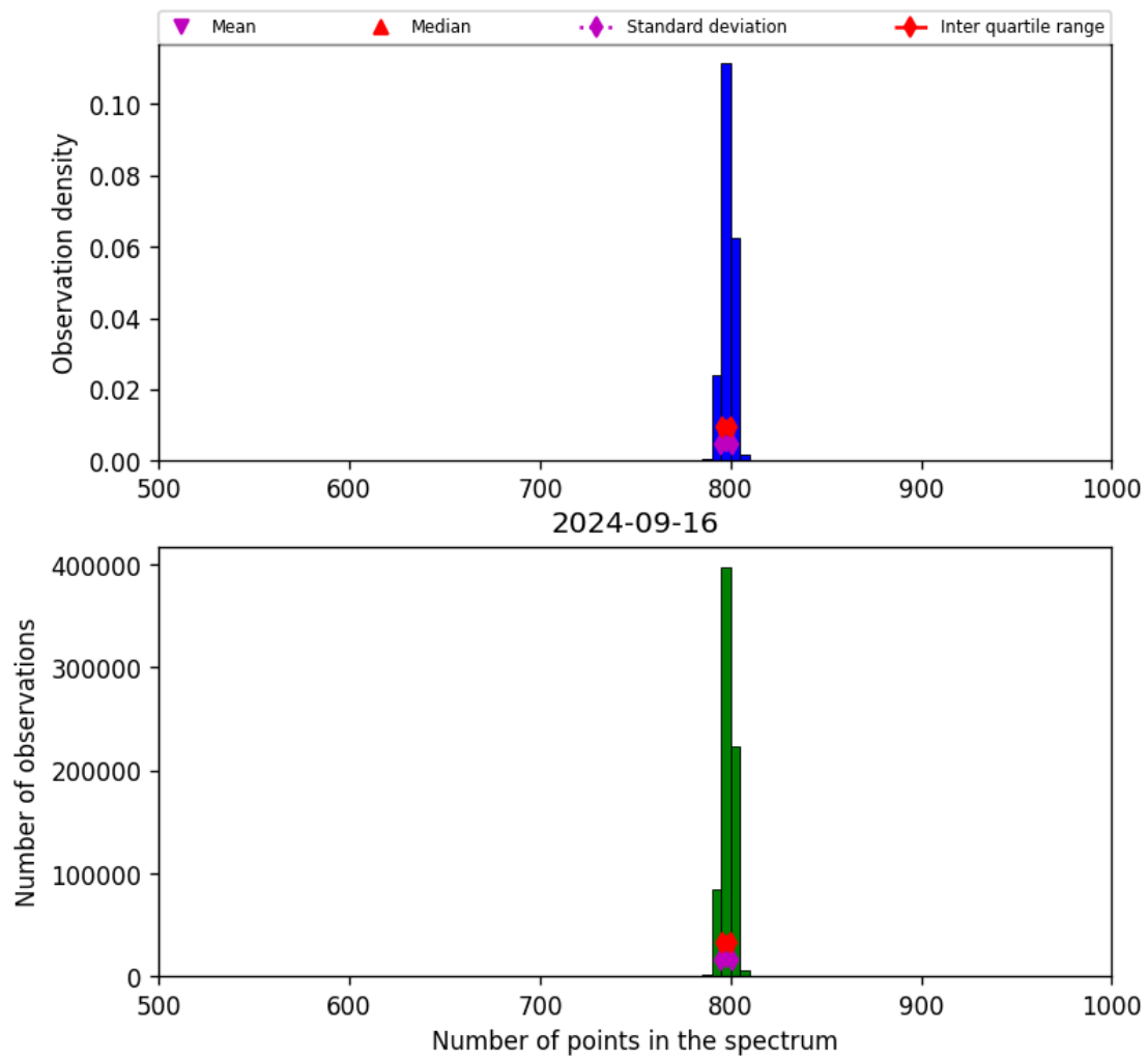
Figure 26: Histogram of “Number of points in the spectrum” for 2024-09-15 to 2024-09-17
