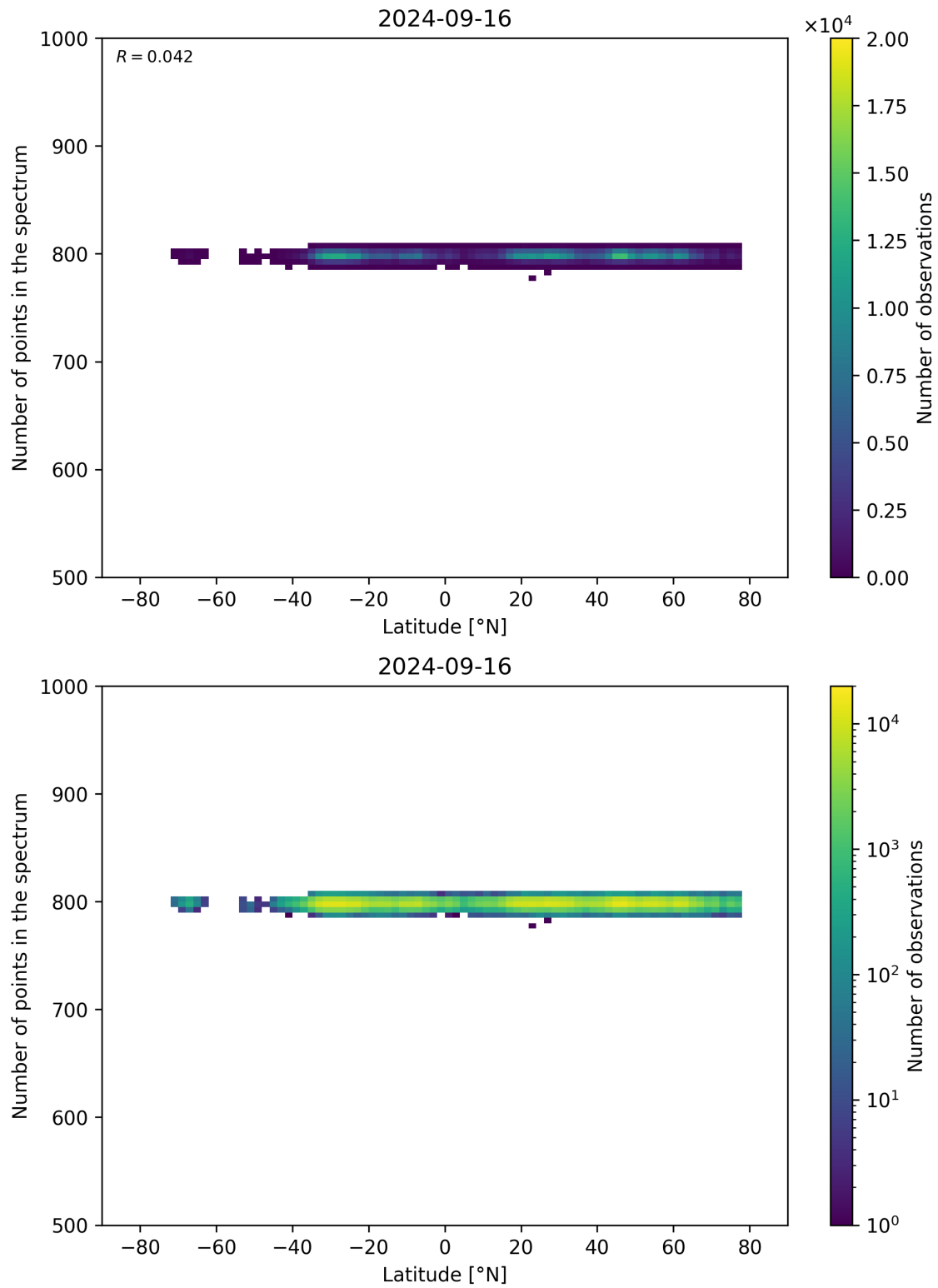
Figure 61: Scatter density plot of “Latitude” against “Number of points in the spectrum” for 2024-09-15 to 2024-09-17.
