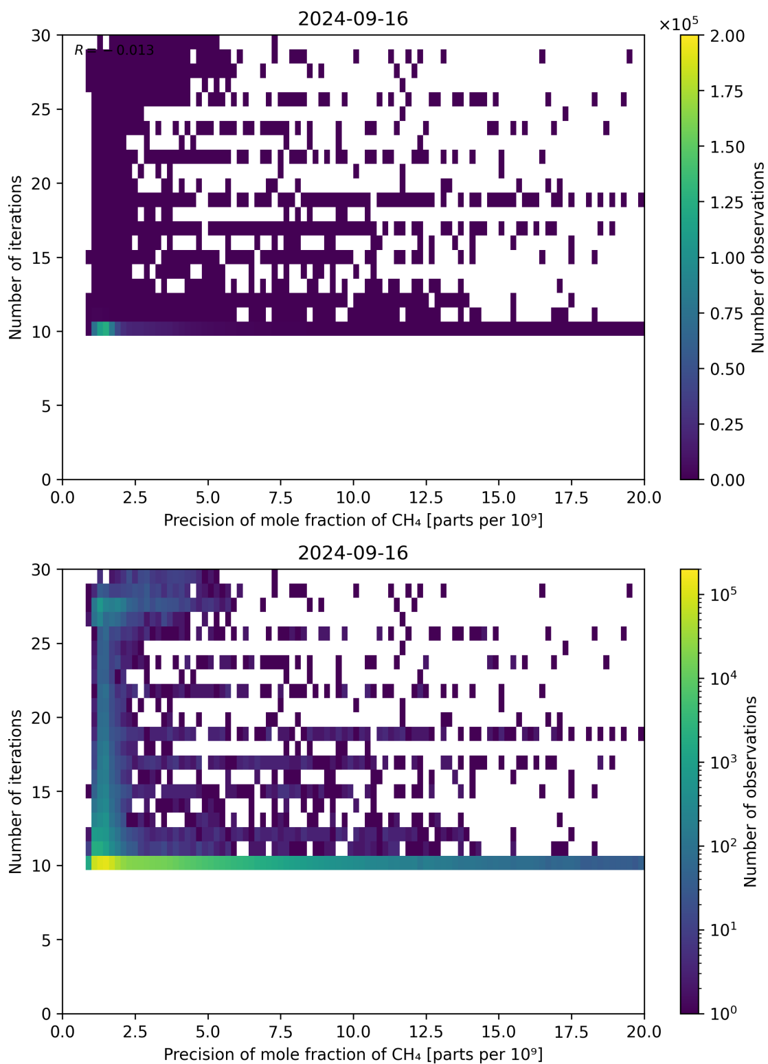
Figure 83: Scatter density plot of “Precision of mole fraction of CH 4 ” against “Number of iterations” for 2024-09-15 to 2024-09-17.
