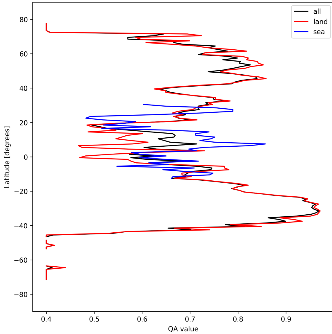
Figure 11: Zonal average of “QA value” for 2024-09-15 to 2024-09-17.
