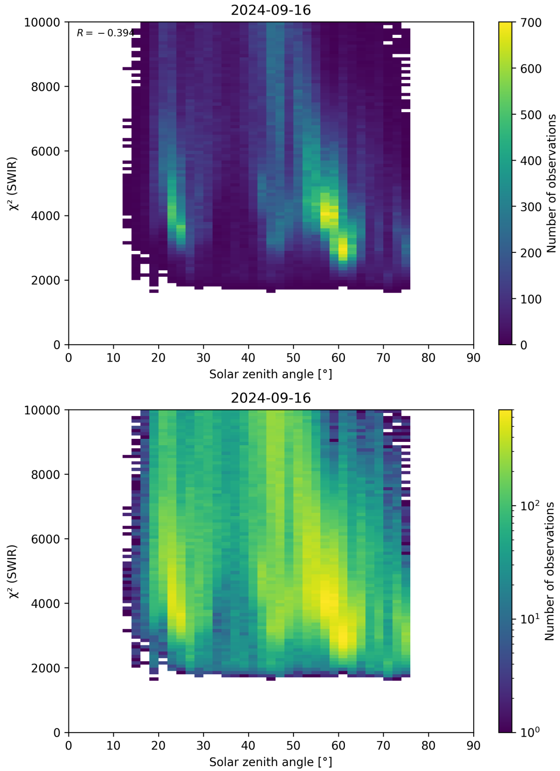
Figure 95: Scatter density plot of “Solar zenith angle” against “ \chi^2 (SWIR)” for 2024-09-15 to 2024-09-17.
