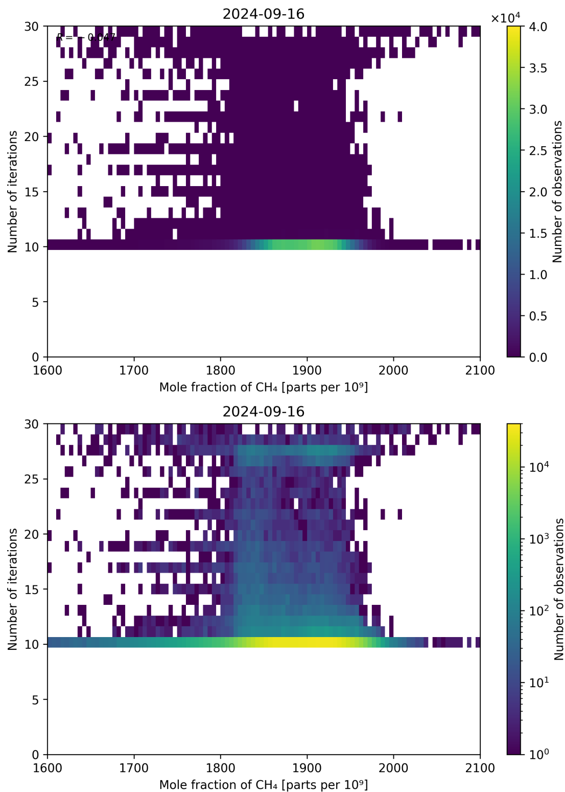
Figure 76: Scatter density plot of “Mole fraction of CH 4 ” against “Number of iterations” for 2024-09-15 to 2024-09-17.
