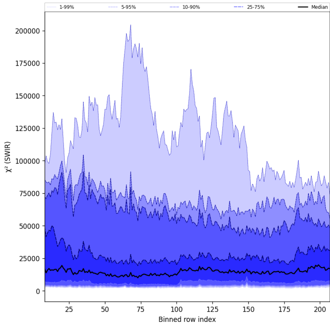
Figure 39: Along track statistics of “ \chi^2 (SWIR)” for 2024-09-15 to 2024-09-17
