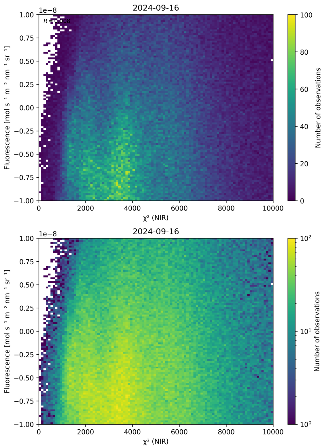
Figure 45: Scatter density plot of “ \chi^2 (NIR)” against “Fluorescence” for 2024-09-15 to 2024-09-17.
