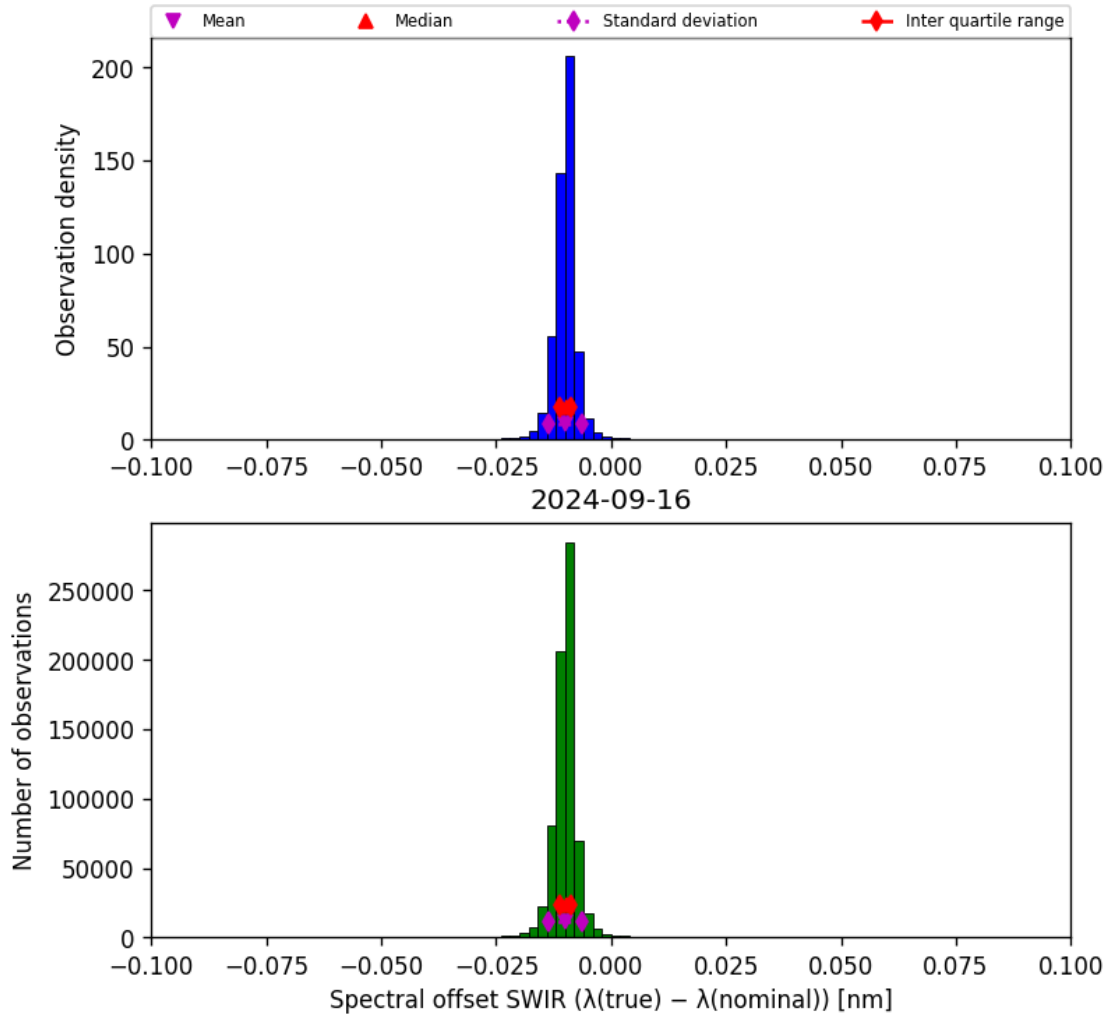
Figure 27: Histogram of “Spectral offset SWIR ( \lambda_{\text{true}} - \lambda_{\text{nominal}} )” for 2024-09-15 to 2024-09-17
