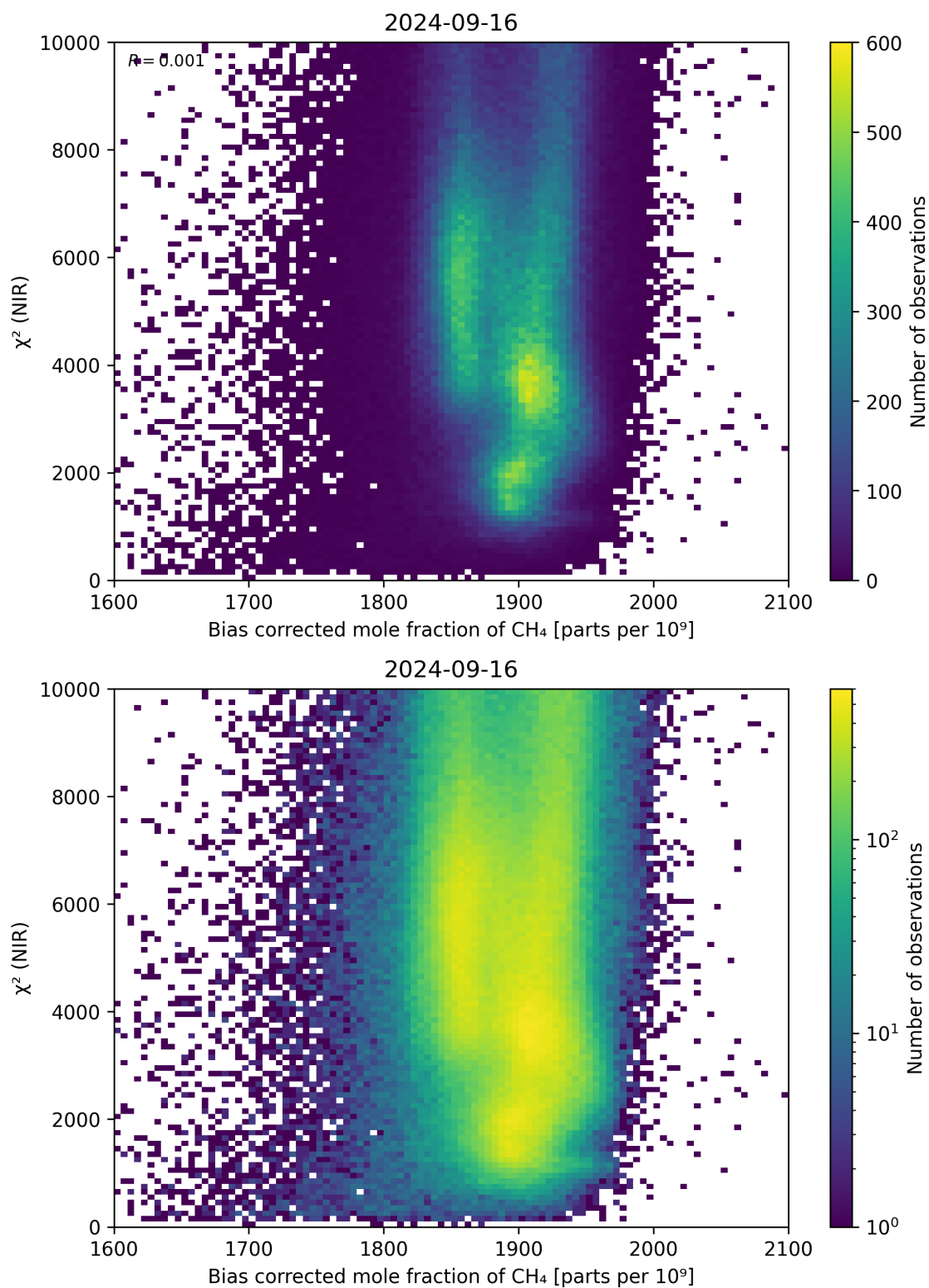
Figure 63: Scatter density plot of “Bias corrected mole fraction of \text{CH}_4 ” against “ \chi^2 (NIR)” for 2024-09-15 to 2024-09-17.
