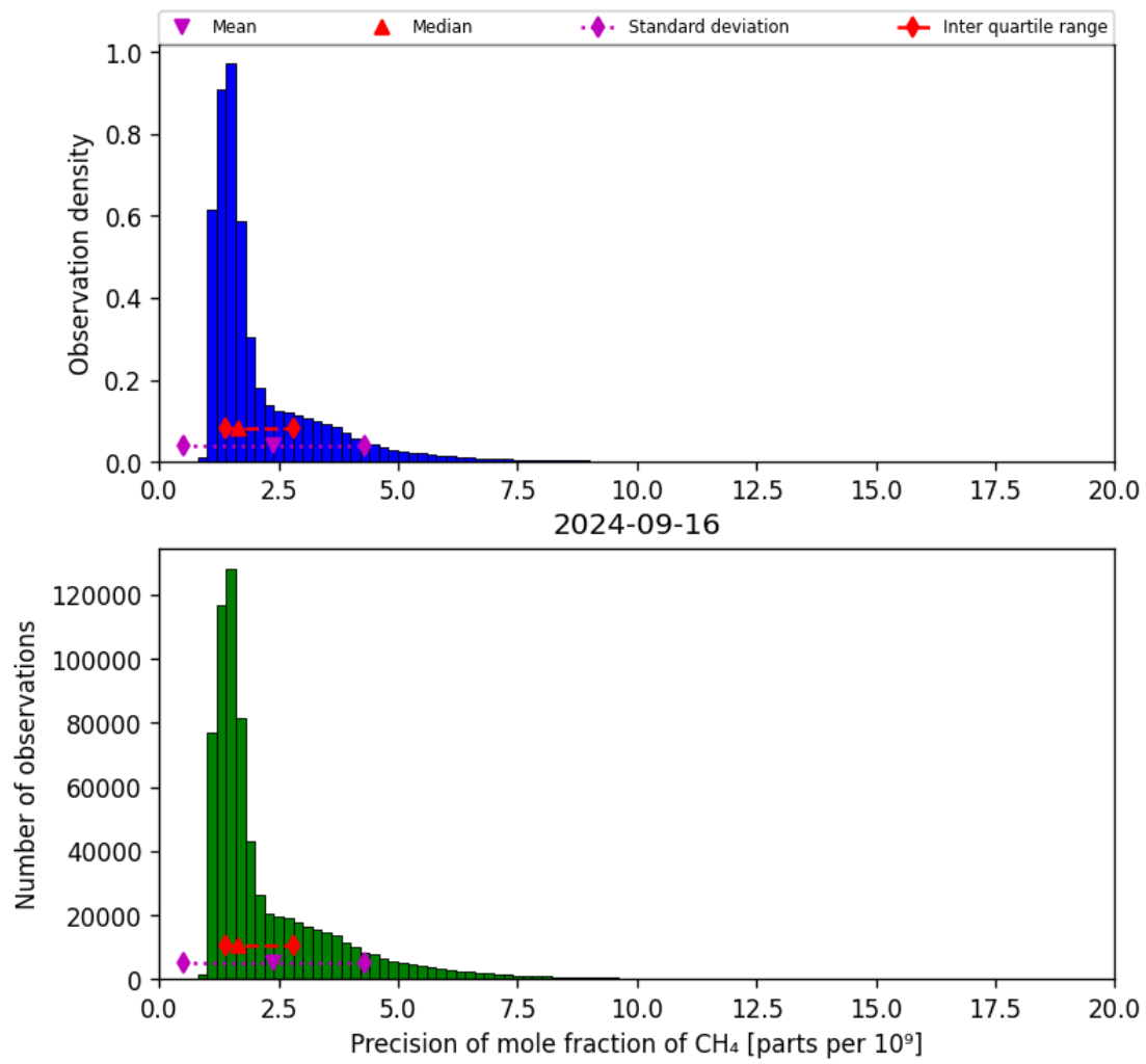
Figure 24: Histogram of “Precision of mole fraction of CH 4 ” for 2024-09-15 to 2024-09-17
