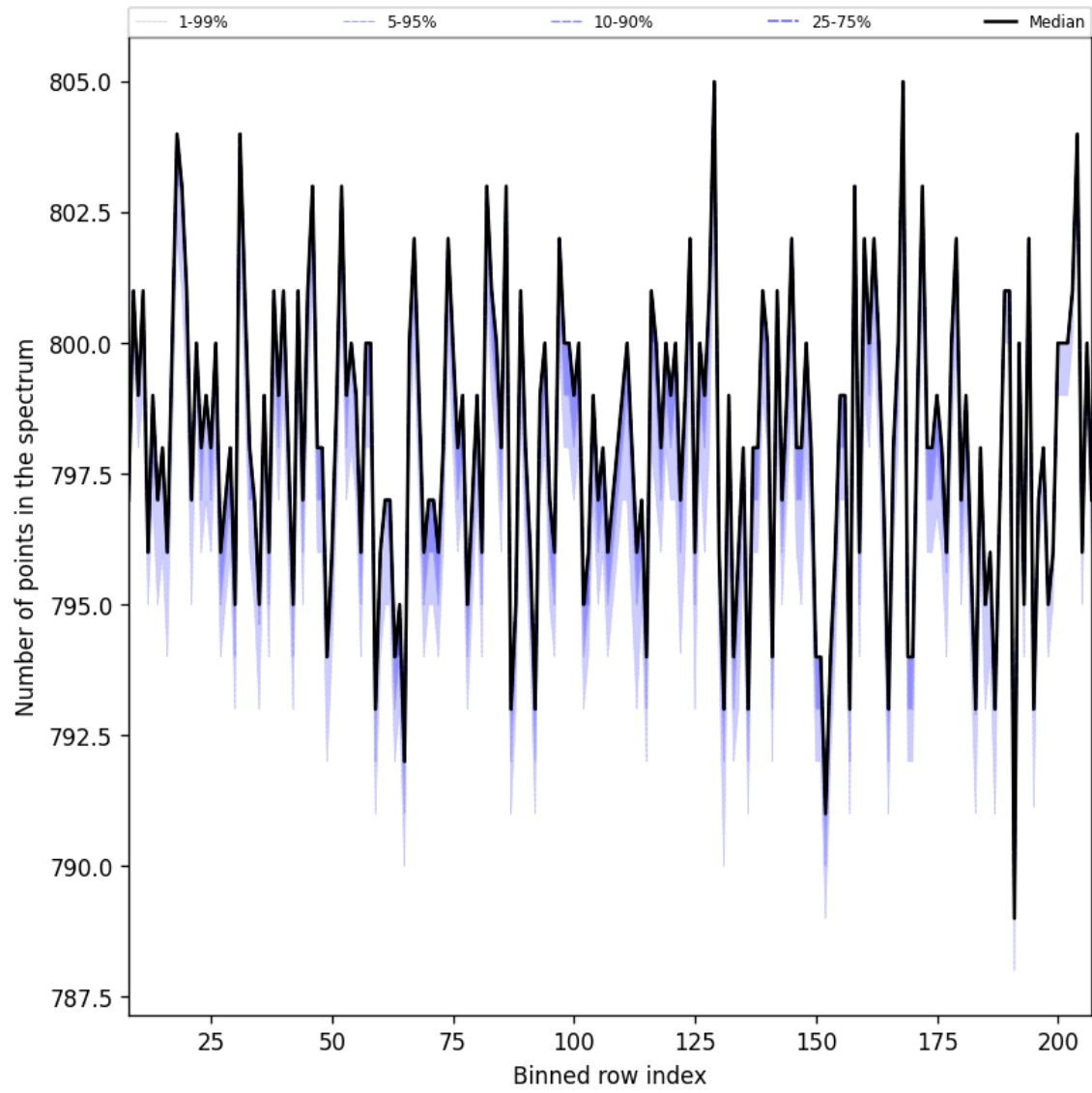
Figure 37: Along track statistics of “Number of points in the spectrum” for 2024-09-15 to 2024-09-17
