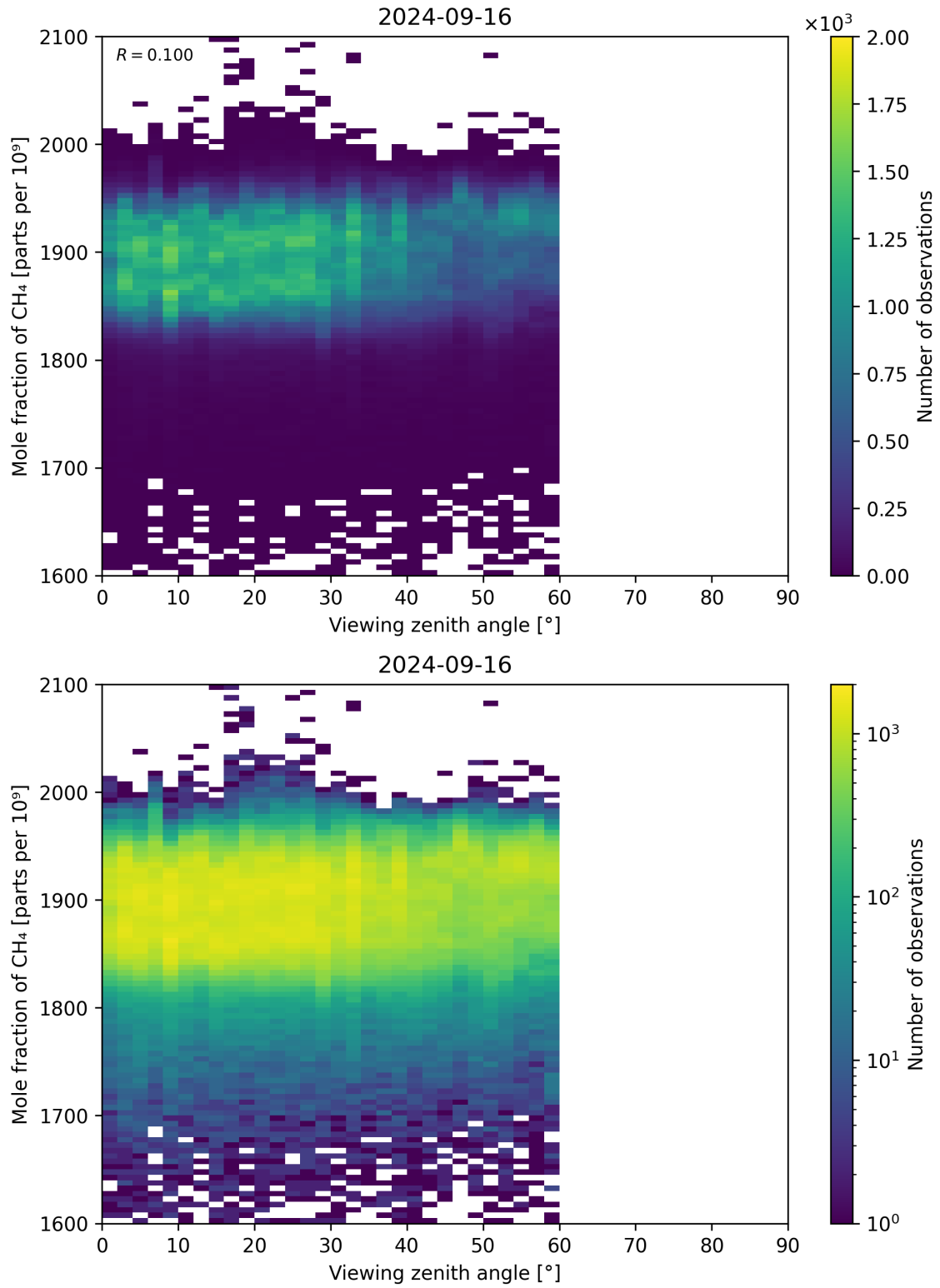
Figure 110: Scatter density plot of “Viewing zenith angle” against “Mole fraction of \text{CH}_4 ” for 2024-09-15 to 2024-09-17.
