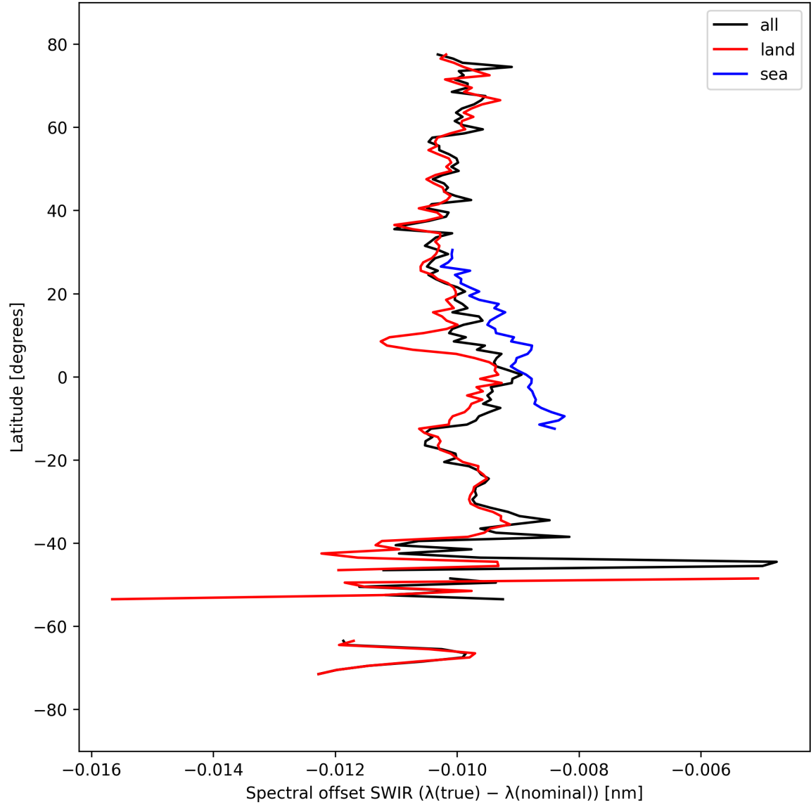
Figure 16: Zonal average of “Spectral offset SWIR ( \lambda_{\text{true}} - \lambda_{\text{nominal}} )” for 2024-09-15 to 2024-09-17.
