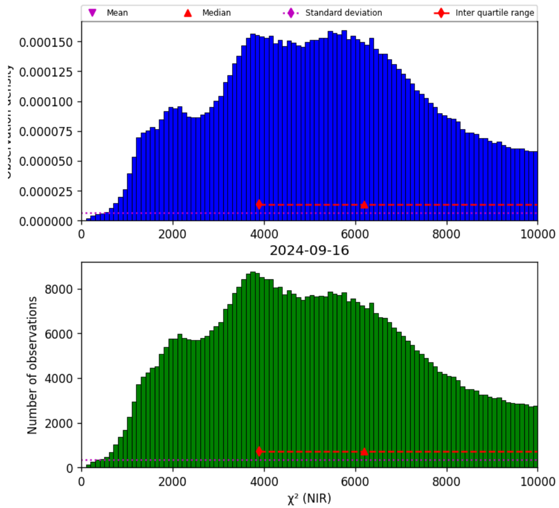
Figure 29: Histogram of “ \chi^2 (NIR)” for 2024-09-15 to 2024-09-17
