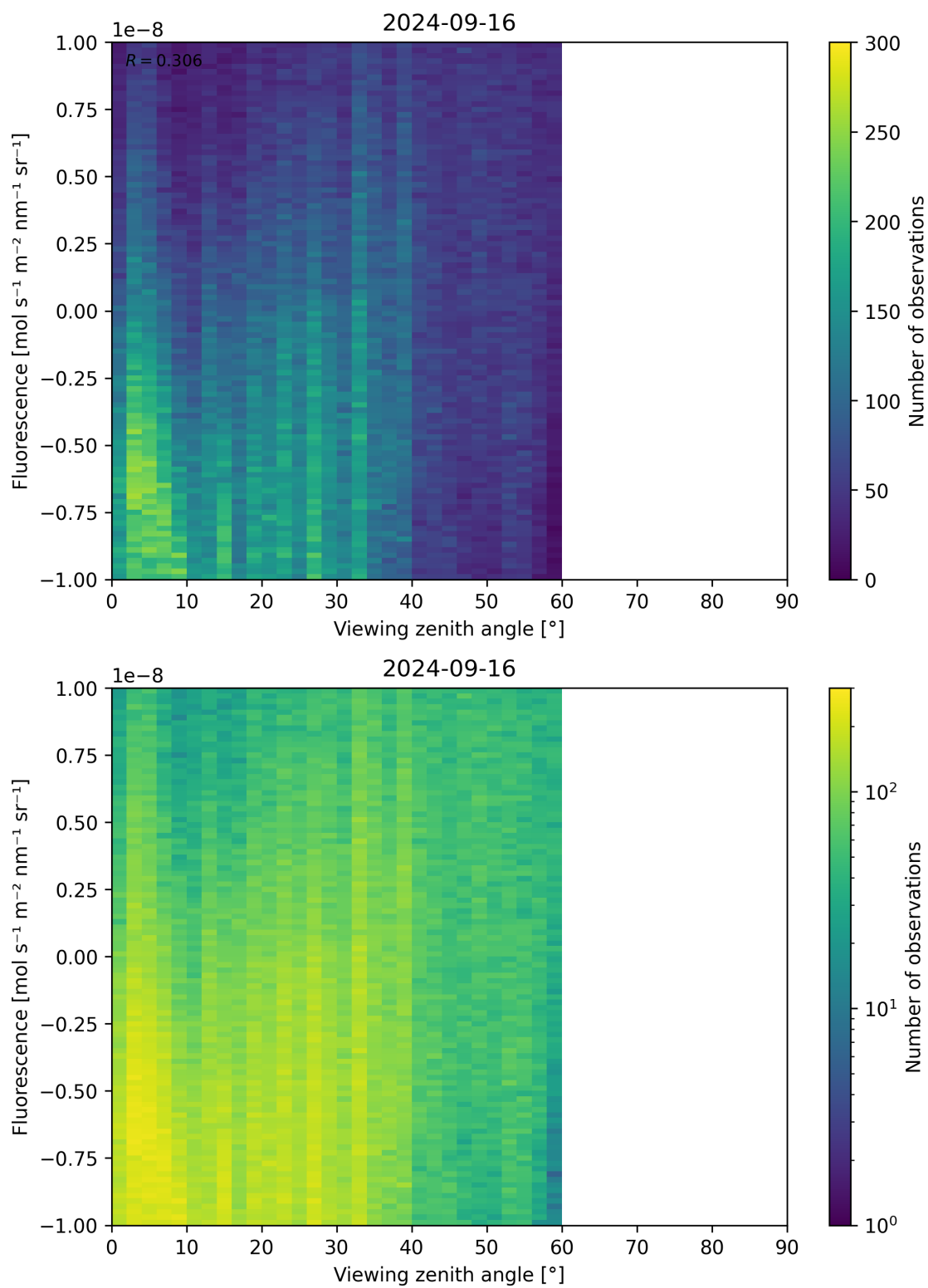
Figure 108: Scatter density plot of “Viewing zenith angle” against “Fluorescence” for 2024-09-15 to 2024-09-17.
