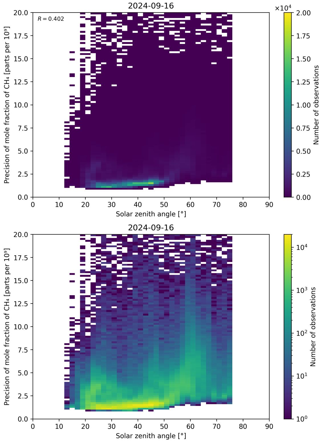
Figure 101: Scatter density plot of “Solar zenith angle” against “Precision of mole fraction of \text{CH}_4 ” for 2024-09-15 to 2024-09-17.
