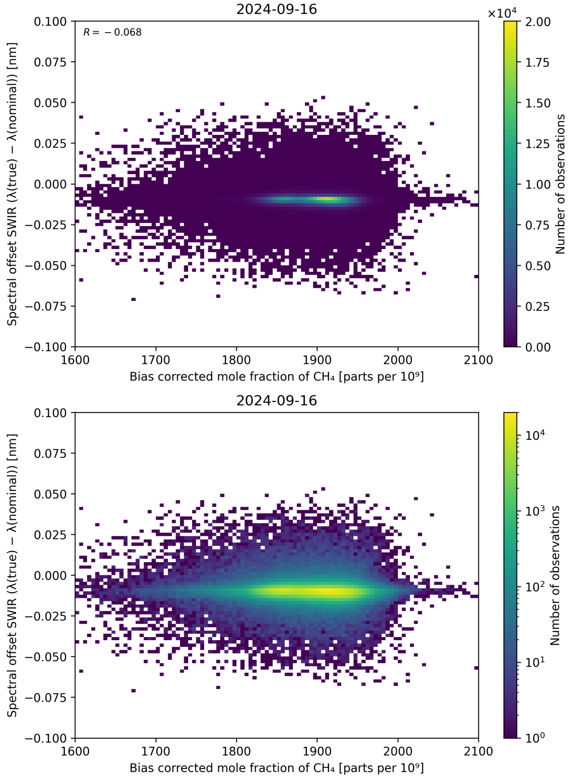
Figure 69: Scatter density plot of “Bias corrected mole fraction of \text{CH}_4 ” against “Spectral offset SWIR ( \lambda_{\text{true}} - \lambda_{\text{nominal}} )” for 2024-09-15 to 2024-09-17.
