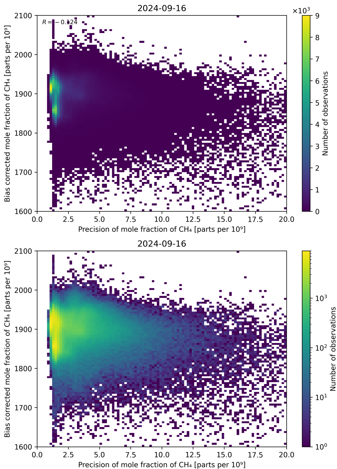
Figure 82: Scatter density plot of “Precision of mole fraction of CH 4 ” against “Bias corrected mole fraction of CH 4 ” for 2024-09-15 to 2024-09-17.
