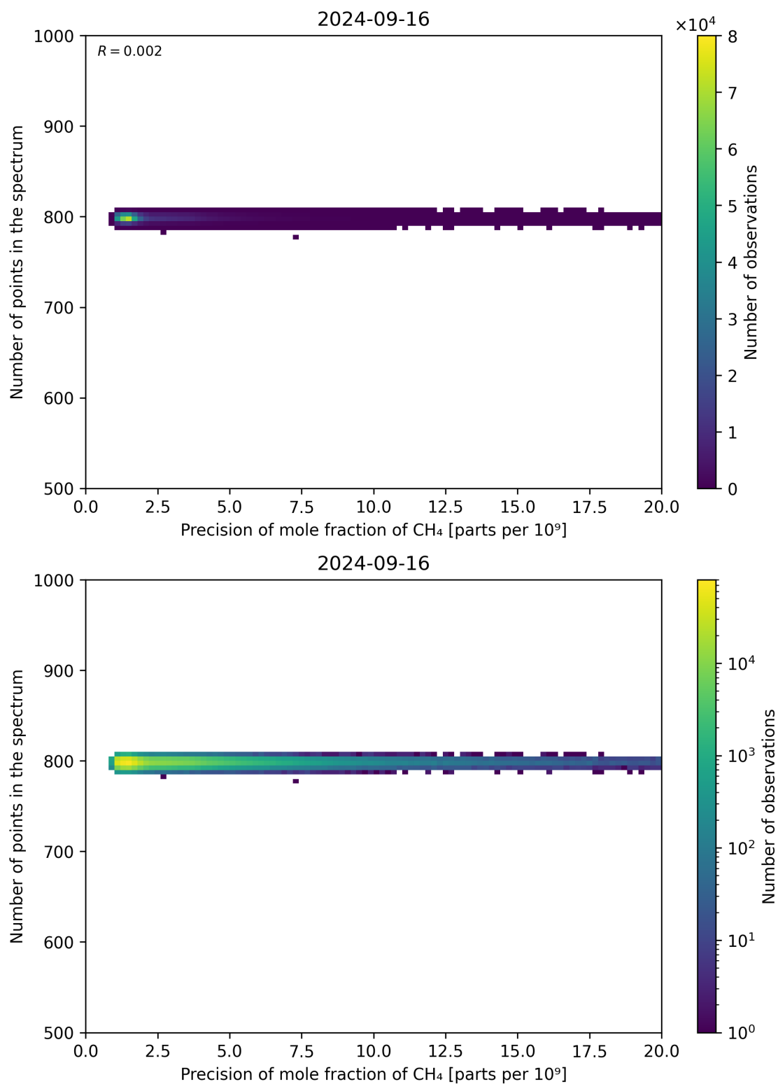
Figure 84: Scatter density plot of “Precision of mole fraction of CH 4 ” against “Number of points in the spectrum” for 2024-09-15 to 2024-09-17.
