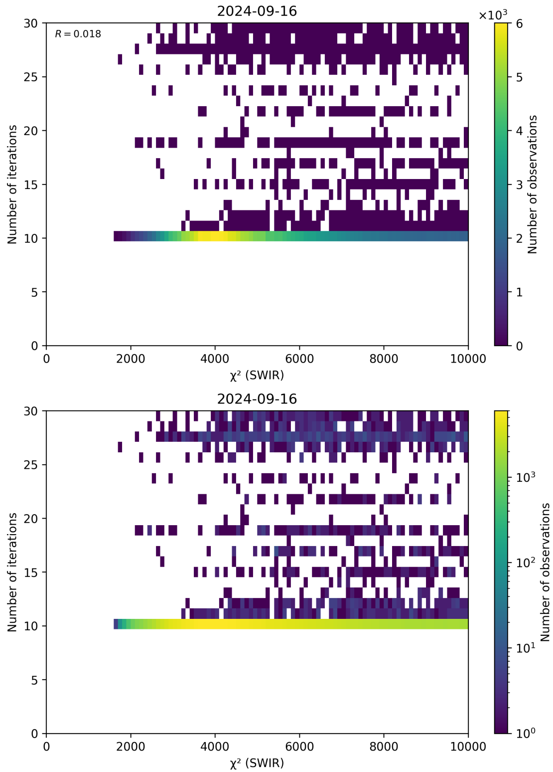
Figure 50: Scatter density plot of “ \chi^2 (SWIR)” against “Number of iterations” for 2024-09-15 to 2024-09-17.
