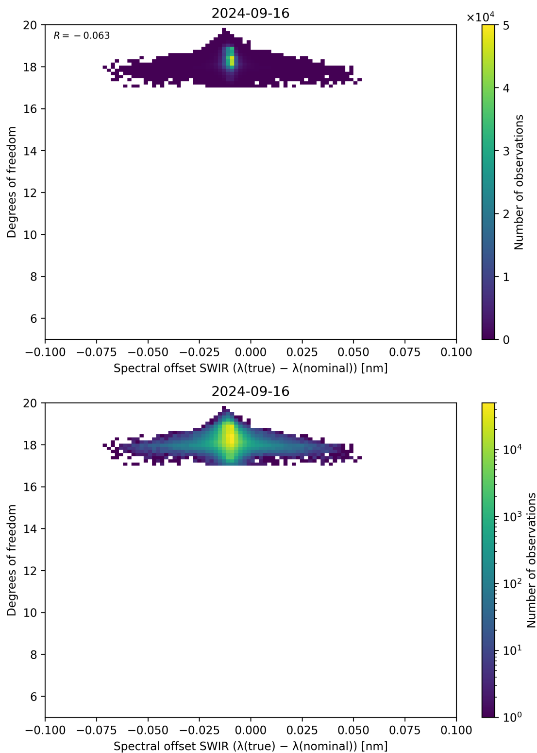
Figure 119: Scatter density plot of “Spectral offset SWIR ( \lambda_{\text{true}} - \lambda_{\text{nominal}} )” against “Degrees of freedom” for 2024-09-15 to 2024-09-17.
