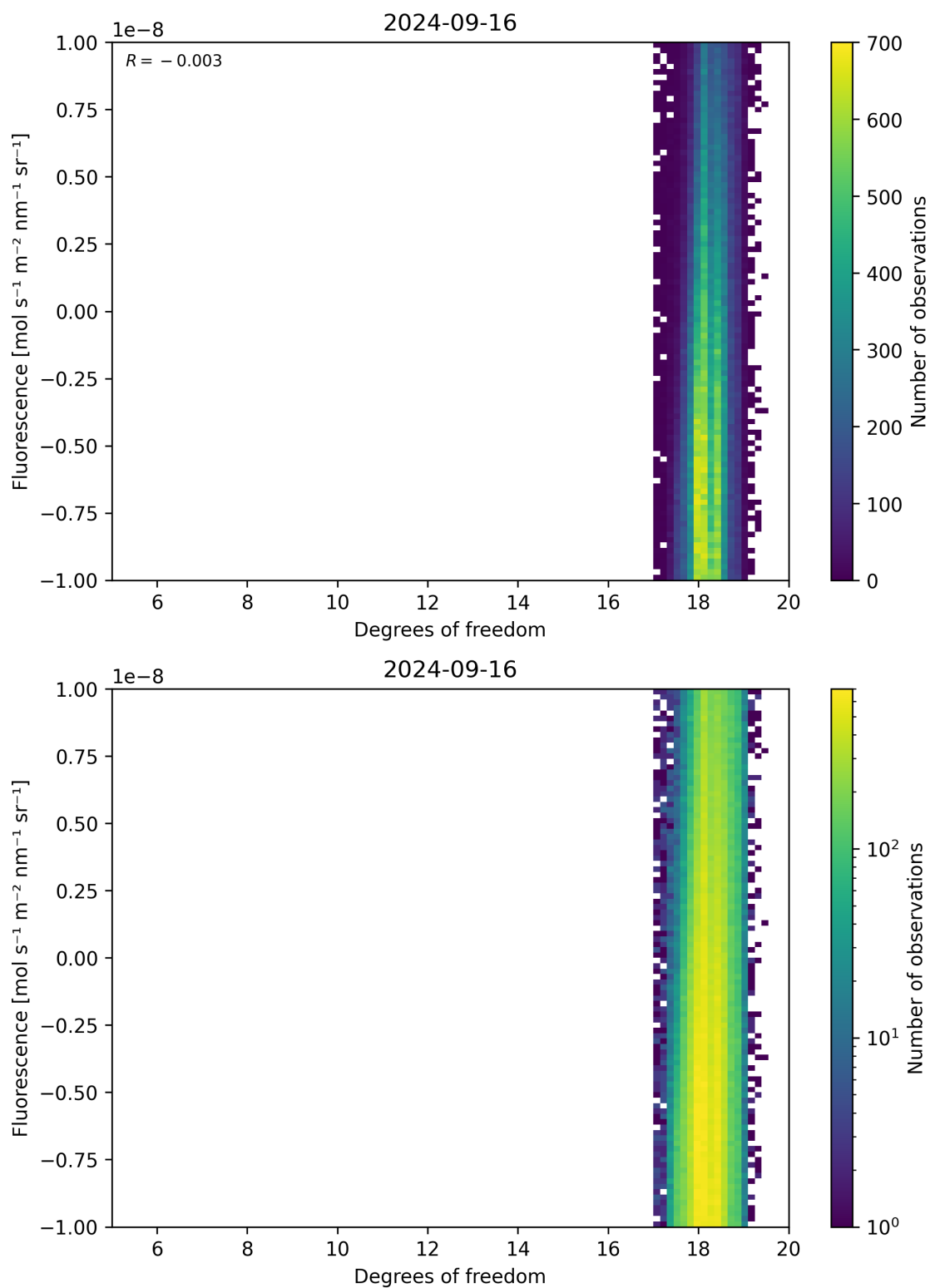
Figure 51: Scatter density plot of “Degrees of freedom” against “Fluorescence” for 2024-09-15 to 2024-09-17.
