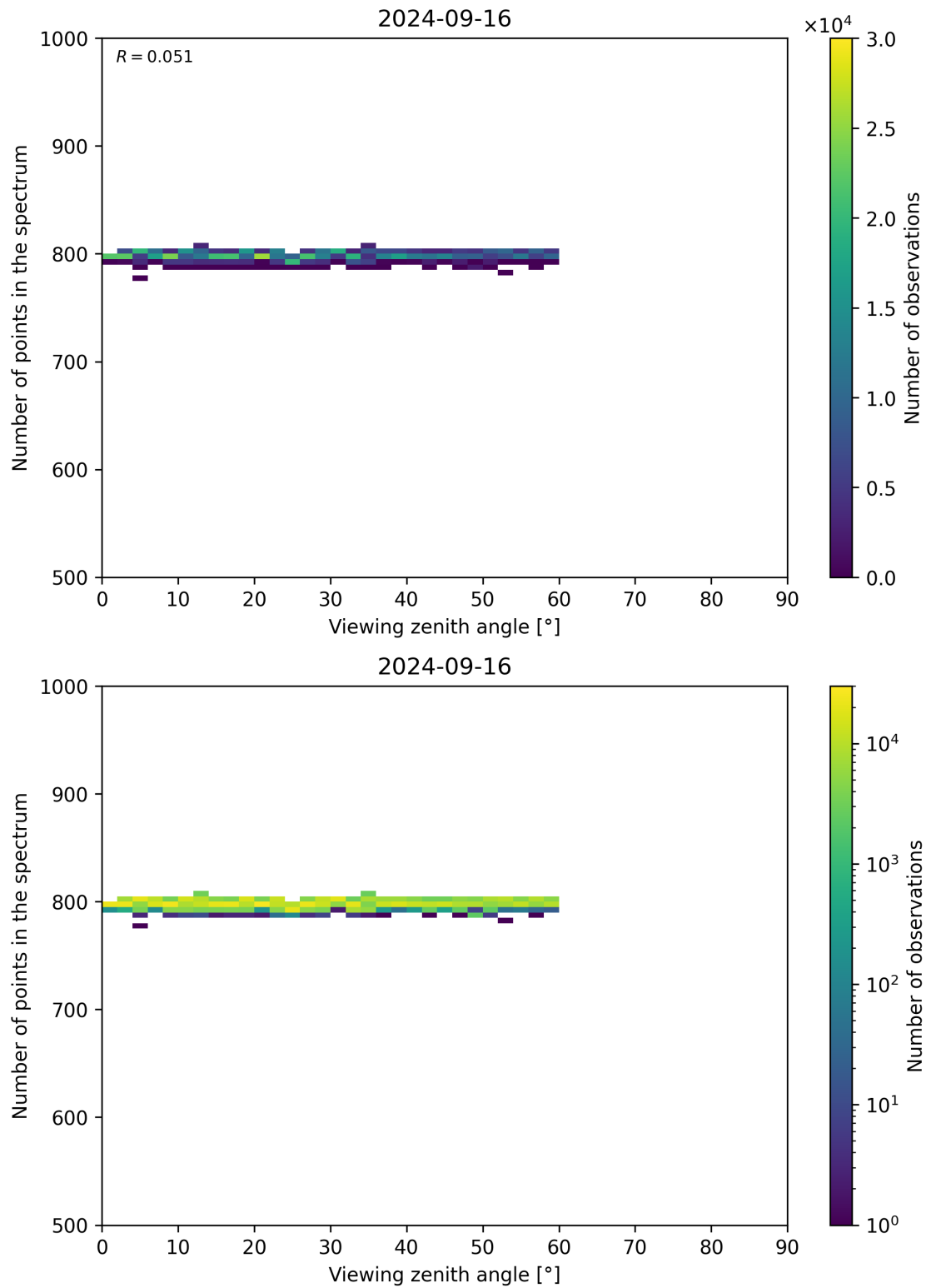
Figure 114: Scatter density plot of “Viewing zenith angle” against “Number of points in the spectrum” for 2024-09-15 to 2024-09-17.
