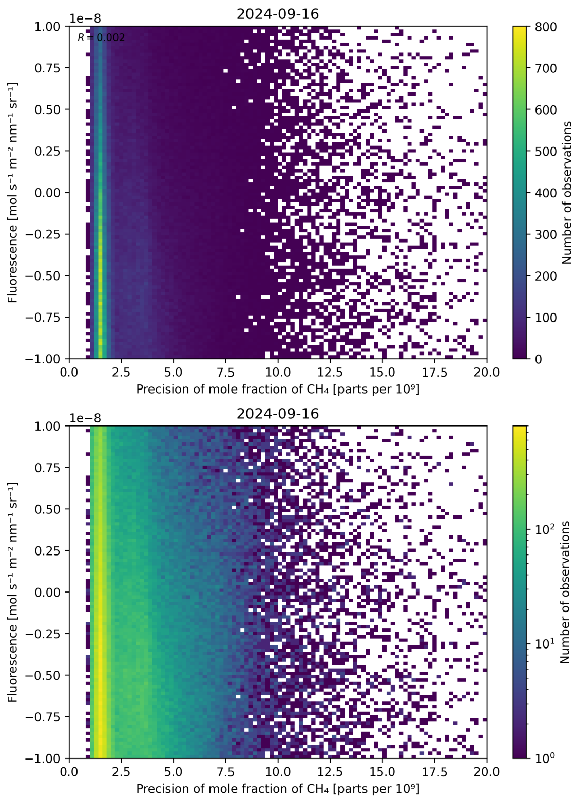
Figure 81: Scatter density plot of “Precision of mole fraction of \text{CH}_4 ” against “Fluorescence” for 2024-09-15 to 2024-09-17.
