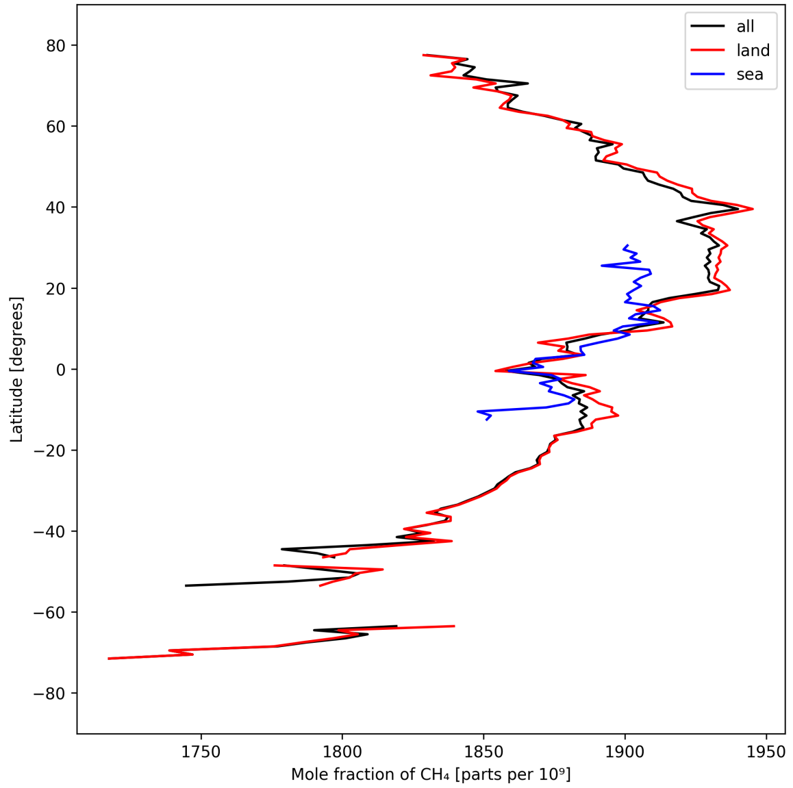
Figure 12: Zonal average of “Mole fraction of \text{CH}_4 ” for 2024-09-15 to 2024-09-17.
