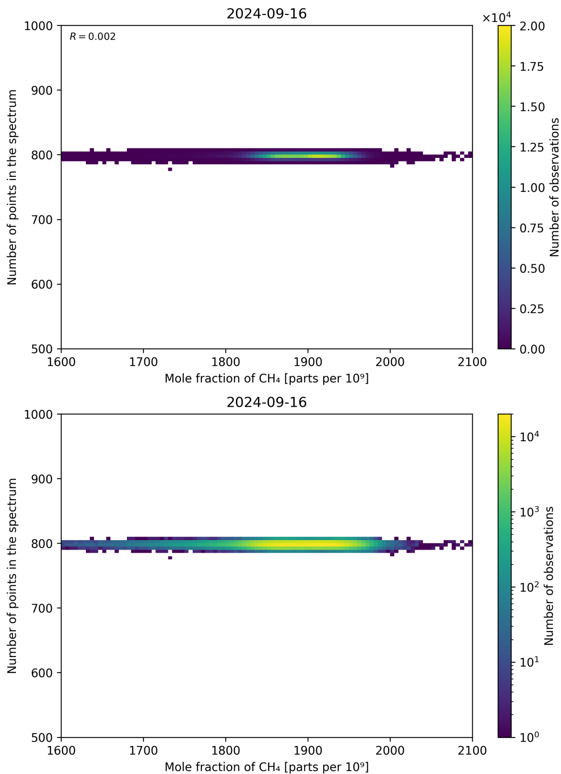
Figure 77: Scatter density plot of “Mole fraction of CH 4 ” against “Number of points in the spectrum” for 2024-09-15 to 2024-09-17.
