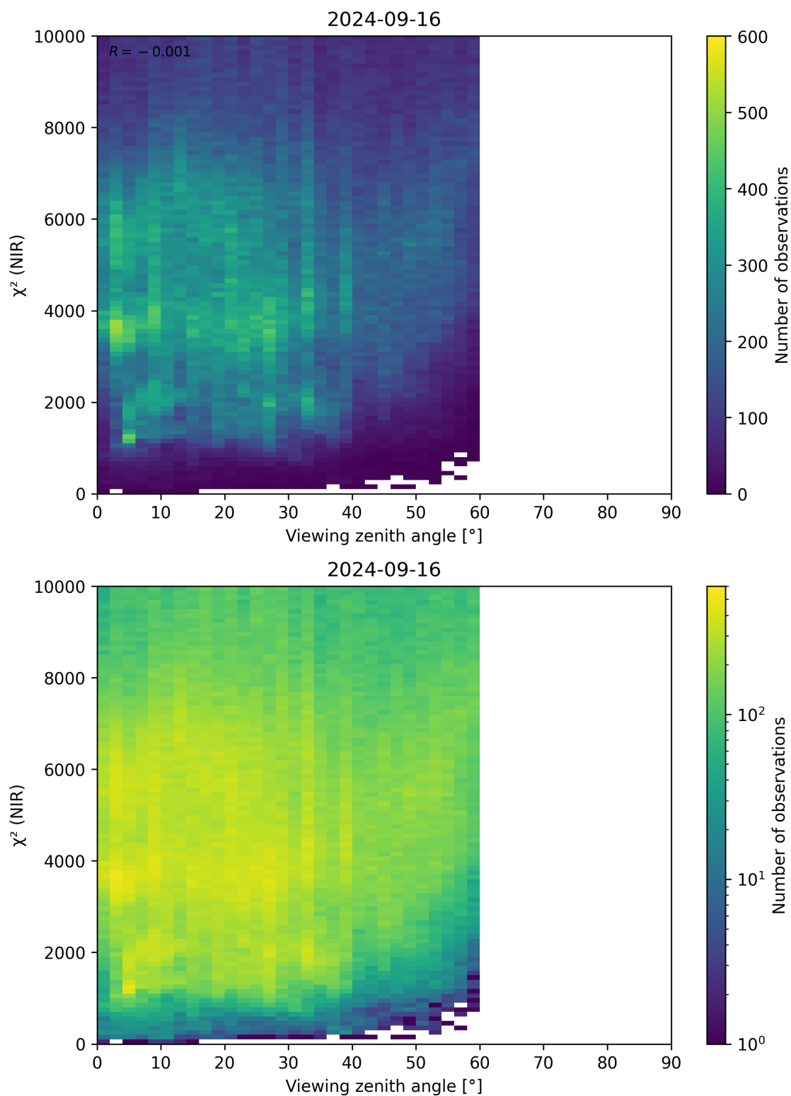
Figure 105: Scatter density plot of “Viewing zenith angle” against “ \chi^2 (NIR)” for 2024-09-15 to 2024-09-17.
