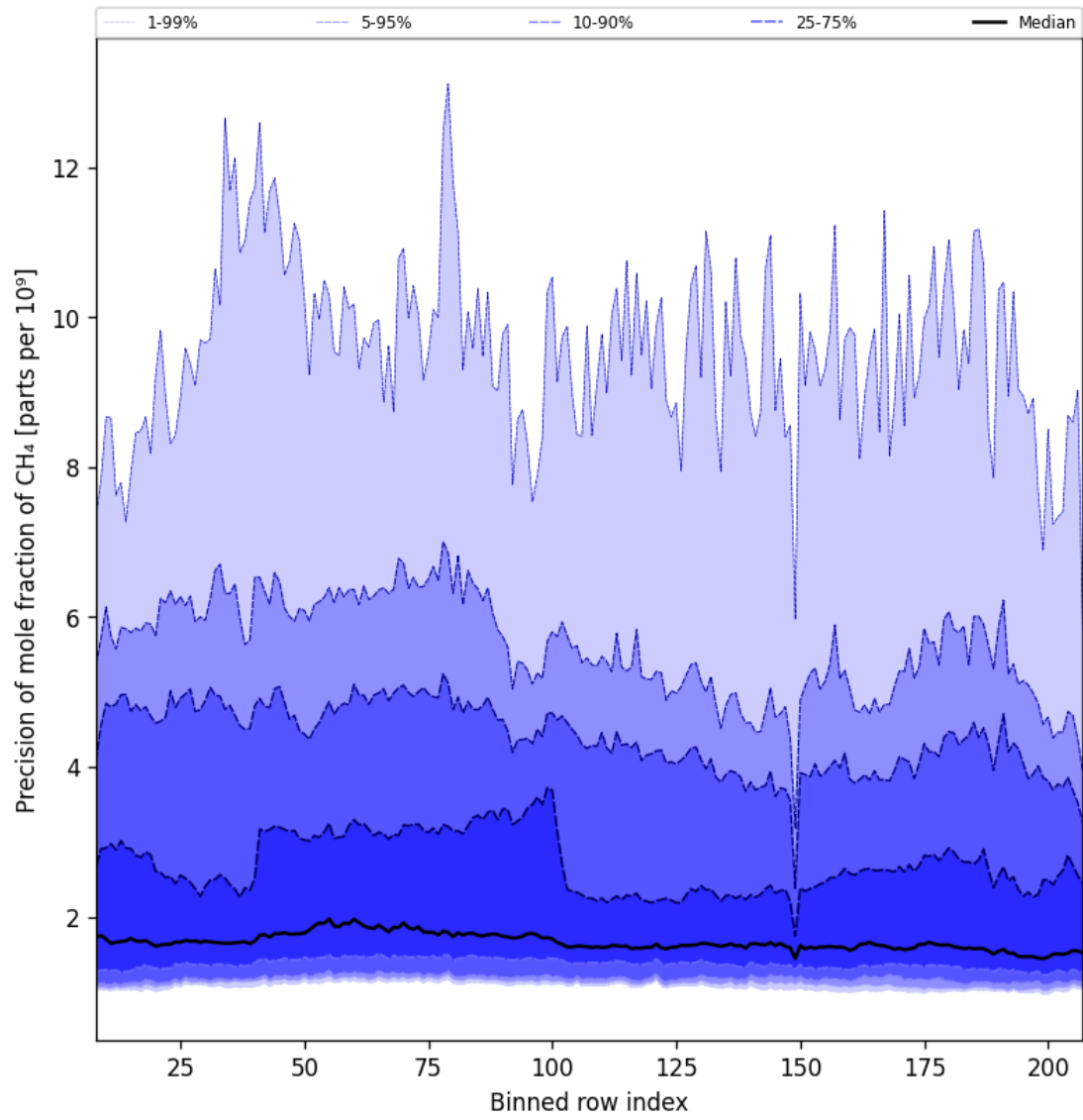
Figure 35: Along track statistics of “Precision of mole fraction of CH 4 ” for 2024-09-15 to 2024-09-17
