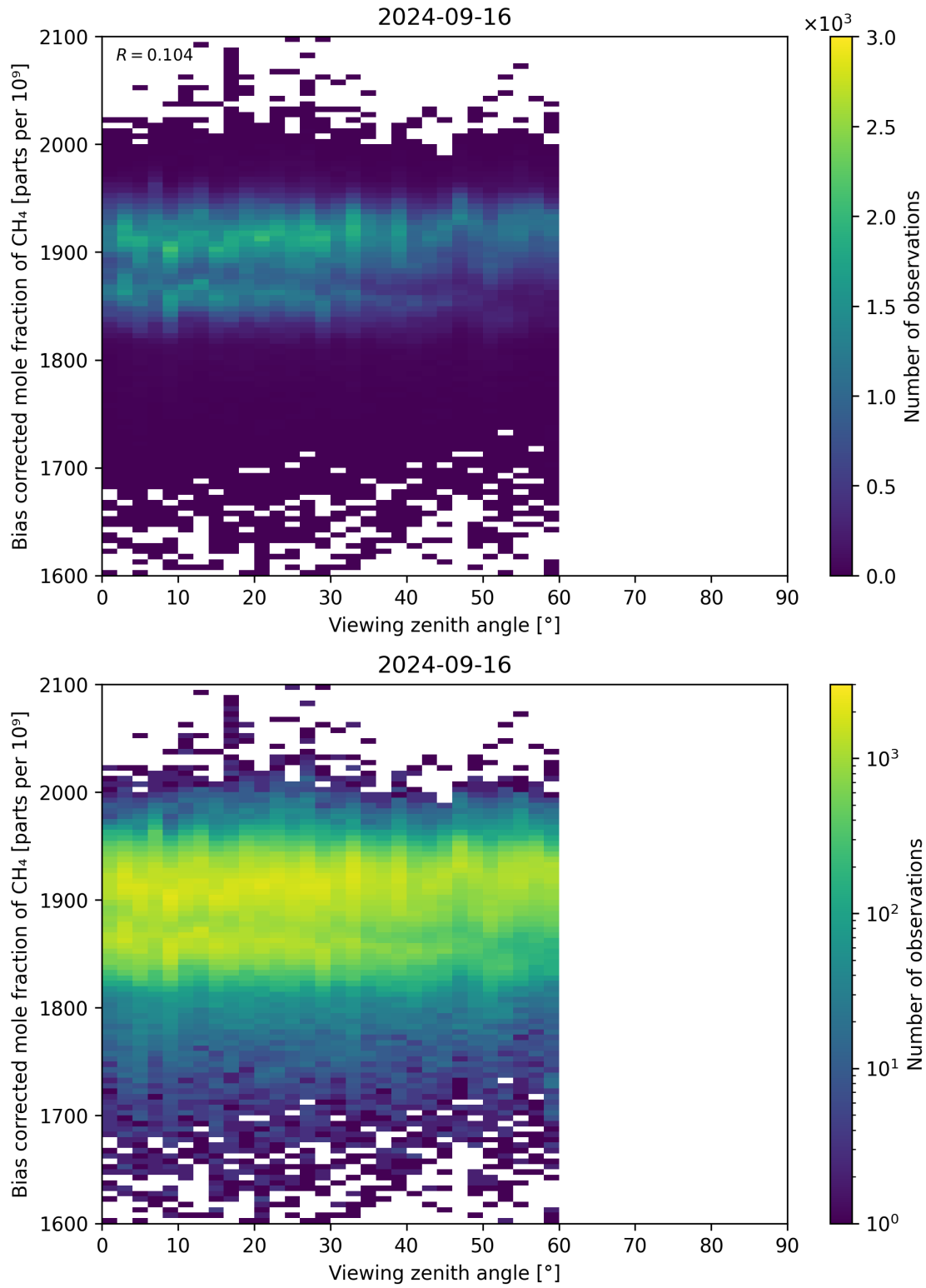
Figure 111: Scatter density plot of “Viewing zenith angle” against “Bias corrected mole fraction of CH 4 ” for 2024-09-15 to 2024-09-17.
