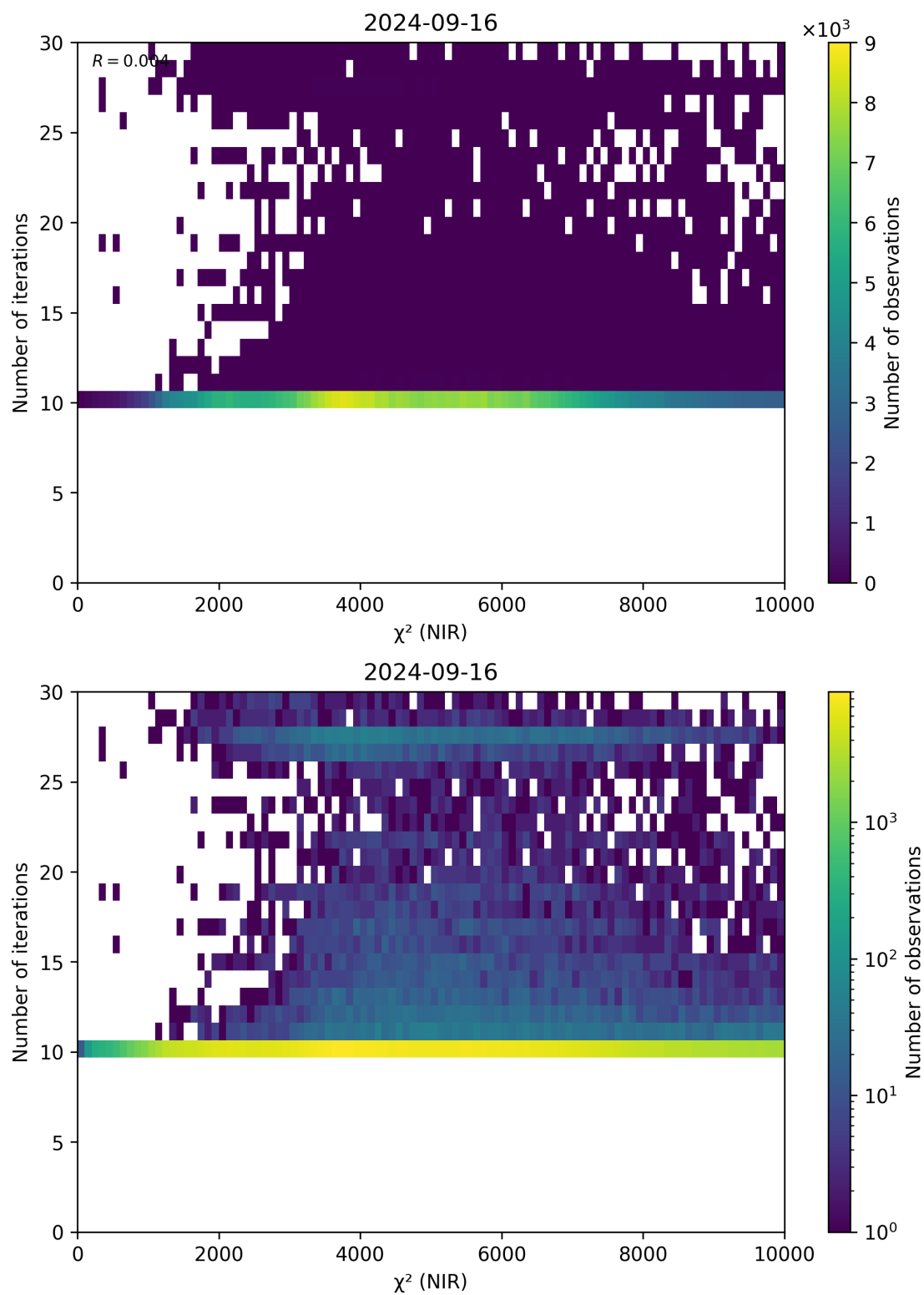
Figure 46: Scatter density plot of “ \chi^2 (NIR)” against “Number of iterations” for 2024-09-15 to 2024-09-17.
