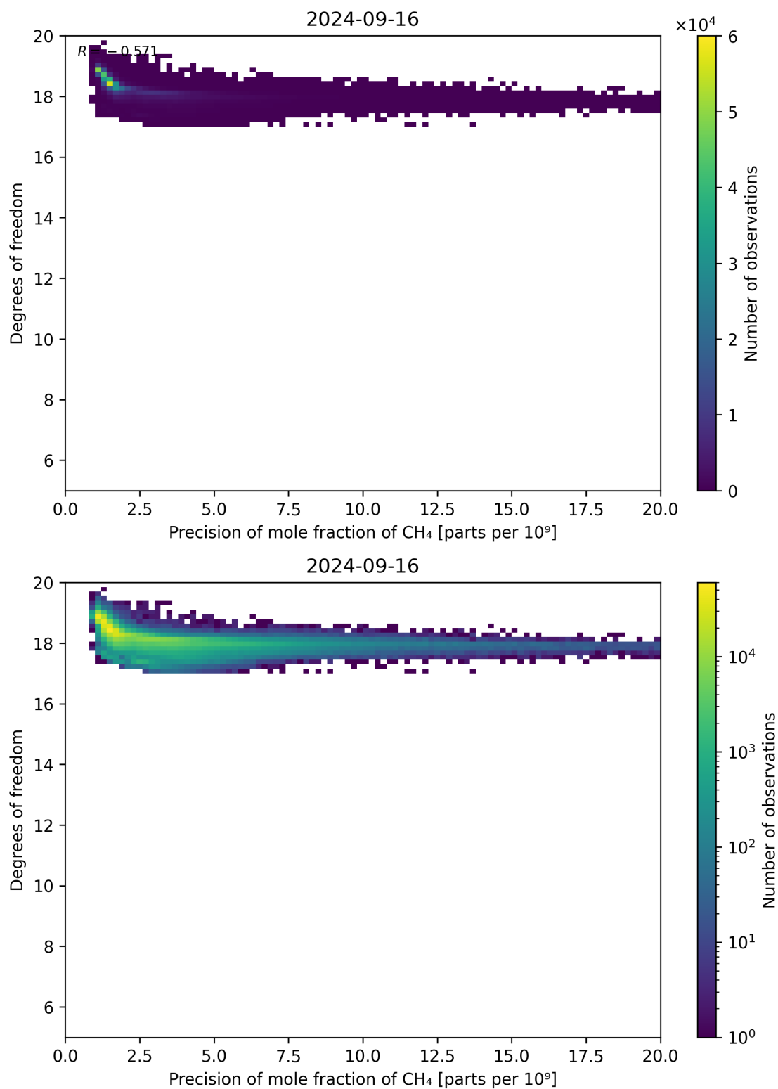
Figure 80: Scatter density plot of “Precision of mole fraction of CH 4 ” against “Degrees of freedom” for 2024-09-15 to 2024-09-17.
