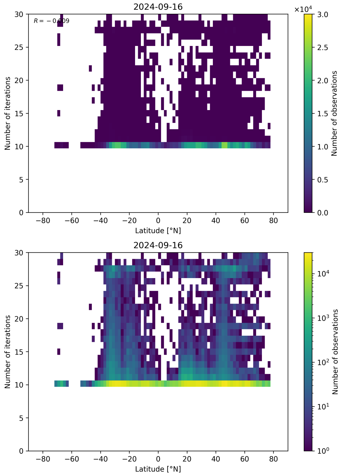
Figure 60: Scatter density plot of “Latitude” against “Number of iterations” for 2024-09-15 to 2024-09-17.
