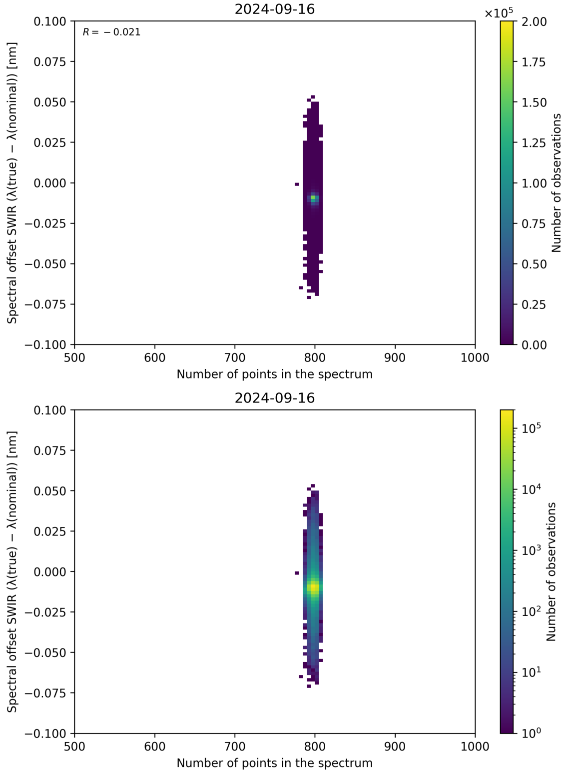
Figure 93: Scatter density plot of “Number of points in the spectrum” against “Spectral offset SWIR ( \lambda_{\text{true}} - \lambda_{\text{nominal}} )” for 2024-09-15 to 2024-09-17.
