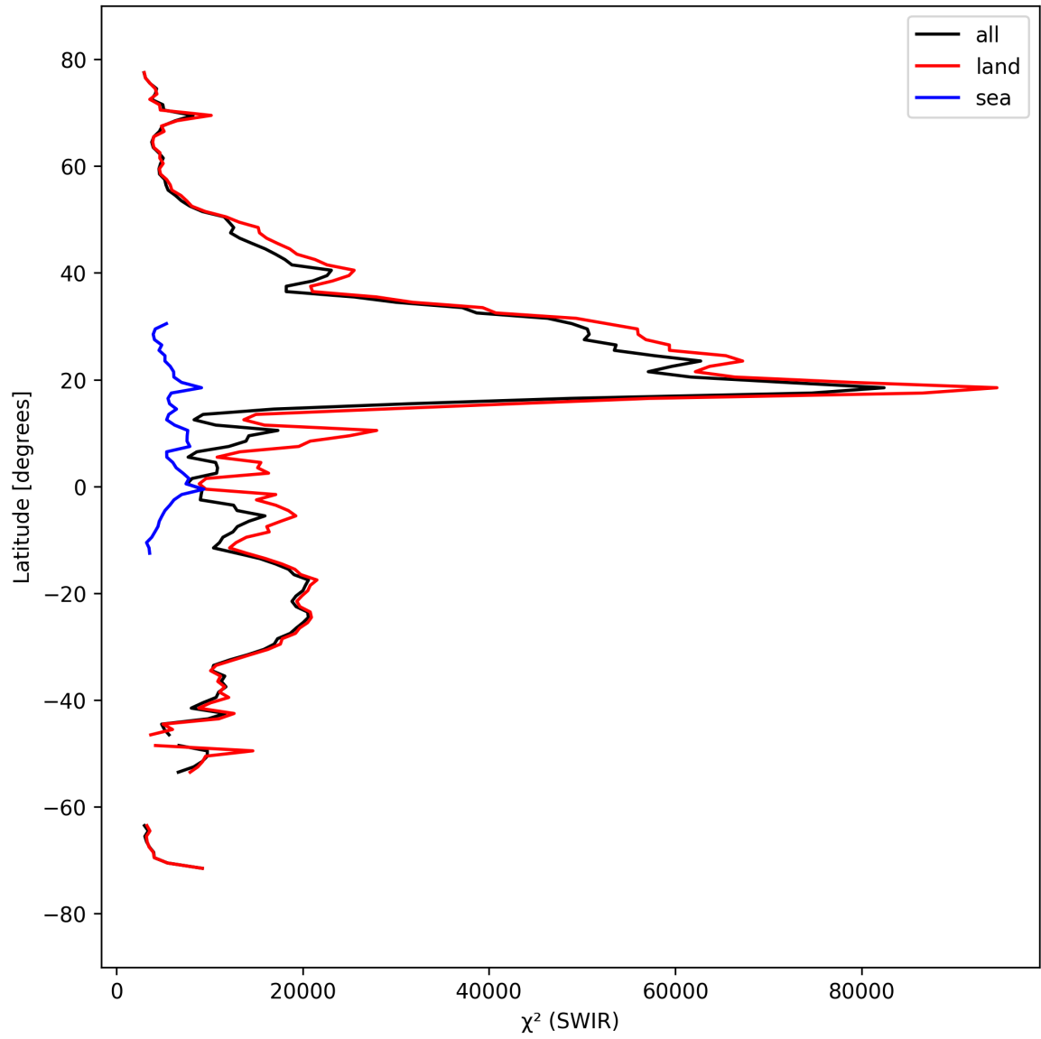
Figure 17: Zonal average of “ \chi^2 (SWIR)” for 2024-09-15 to 2024-09-17.
