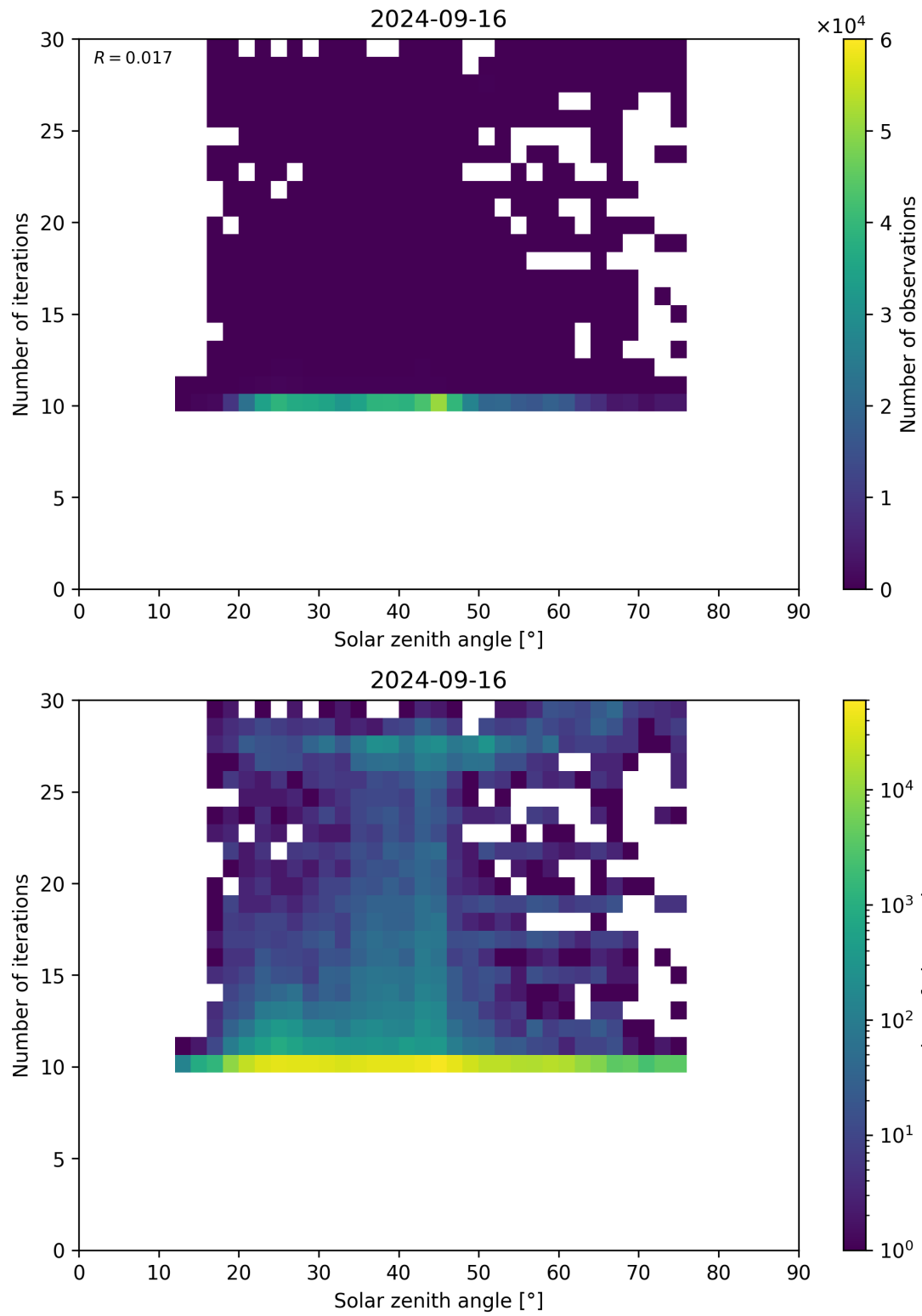
Figure 102: Scatter density plot of “Solar zenith angle” against “Number of iterations” for 2024-09-15 to 2024-09-17.
