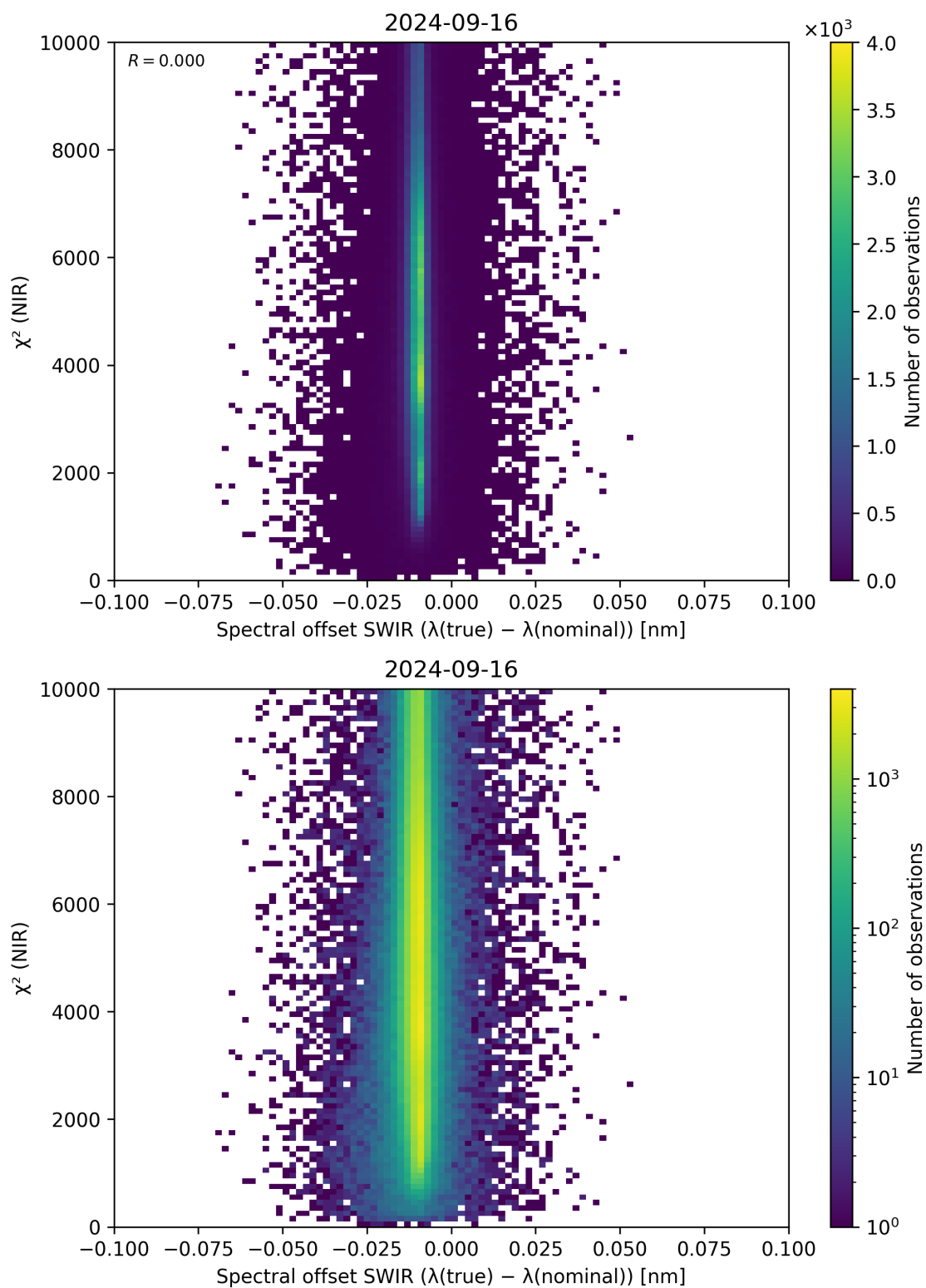
Figure 117: Scatter density plot of “Spectral offset SWIR ( \lambda_{\text{true}} - \lambda_{\text{nominal}} )” against “ \chi^2 (NIR)” for 2024-09-15 to 2024-09-17.
