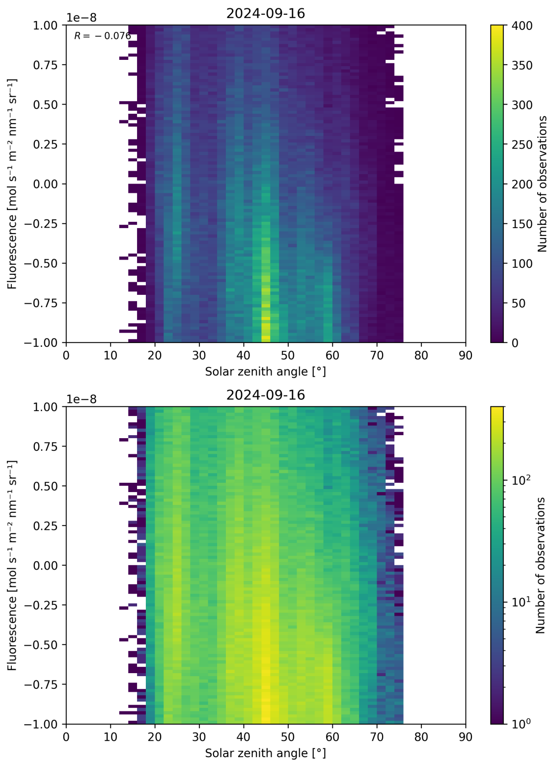
Figure 97: Scatter density plot of “Solar zenith angle” against “Fluorescence” for 2024-09-15 to 2024-09-17.
