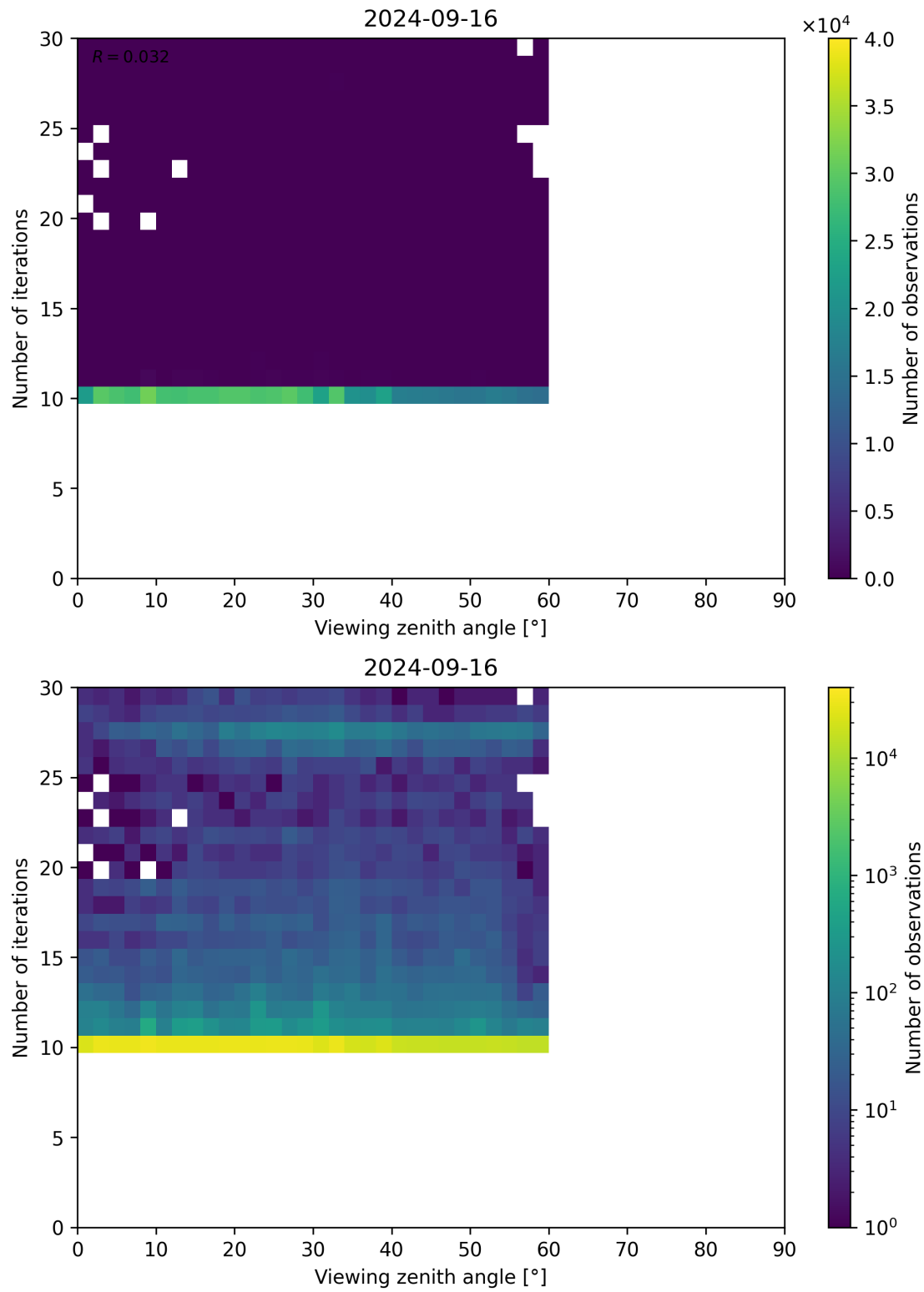
Figure 113: Scatter density plot of “Viewing zenith angle” against “Number of iterations” for 2024-09-15 to 2024-09-17.
