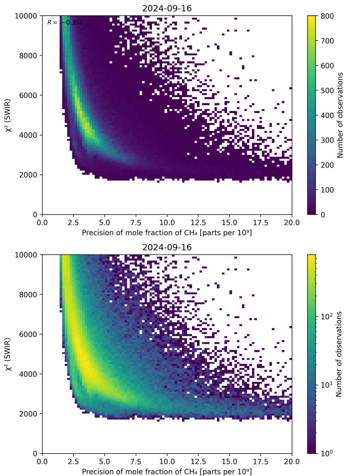
Figure 79: Scatter density plot of “Precision of mole fraction of CH 4 ” against “ \chi^2 (SWIR)” for 2024-09-15 to 2024-09-17.
