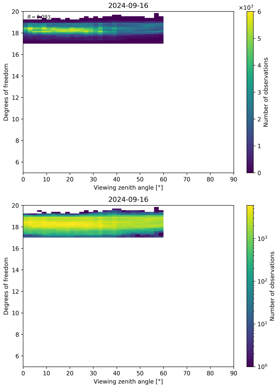
Figure 107: Scatter density plot of “Viewing zenith angle” against “Degrees of freedom” for 2024-09-15 to 2024-09-17.
