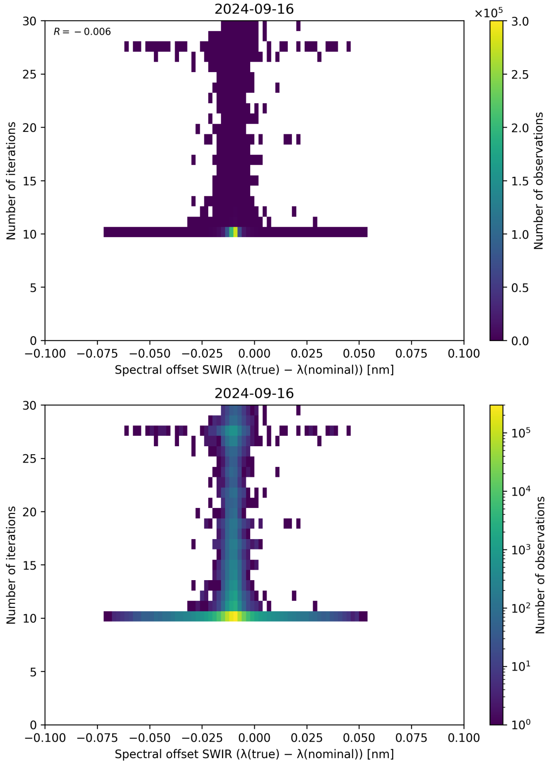
Figure 121: Scatter density plot of “Spectral offset SWIR ( \lambda_{\text{true}} - \lambda_{\text{nominal}} )” against “Number of iterations” for 2024-09-15 to 2024-09-17.
