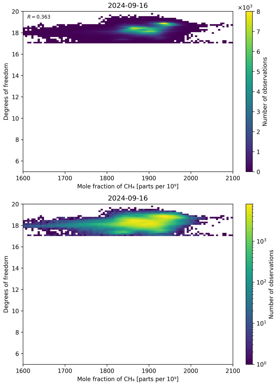
Figure 72: Scatter density plot of “Mole fraction of CH 4 ” against “Degrees of freedom” for 2024-09-15 to 2024-09-17.
