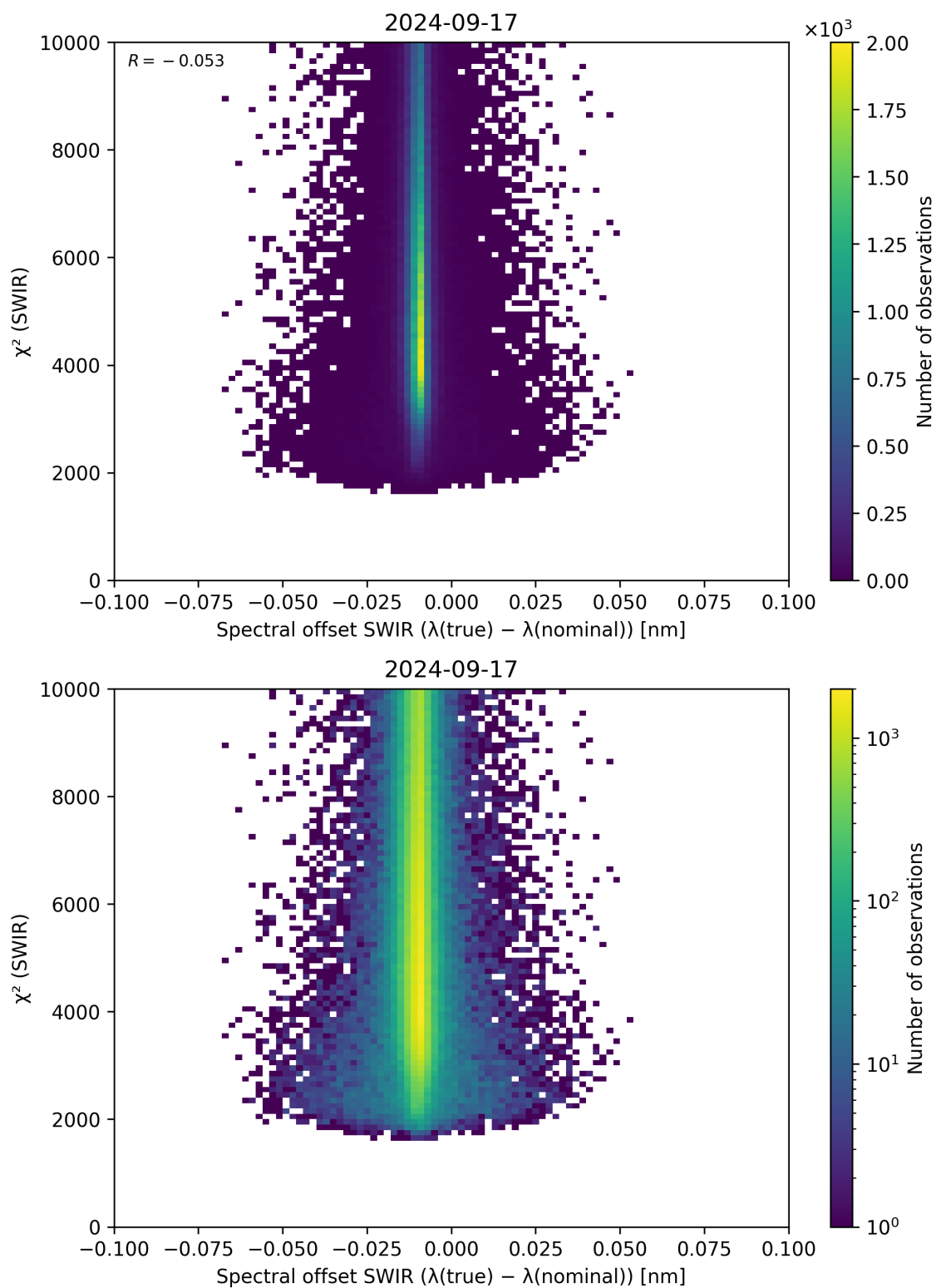
Figure 118: Scatter density plot of “Spectral offset SWIR ( \lambda_{\text{true}} - \lambda_{\text{nominal}} )” against “ \chi^2 (SWIR)” for 2024-09-17 to 2024-09-18.
