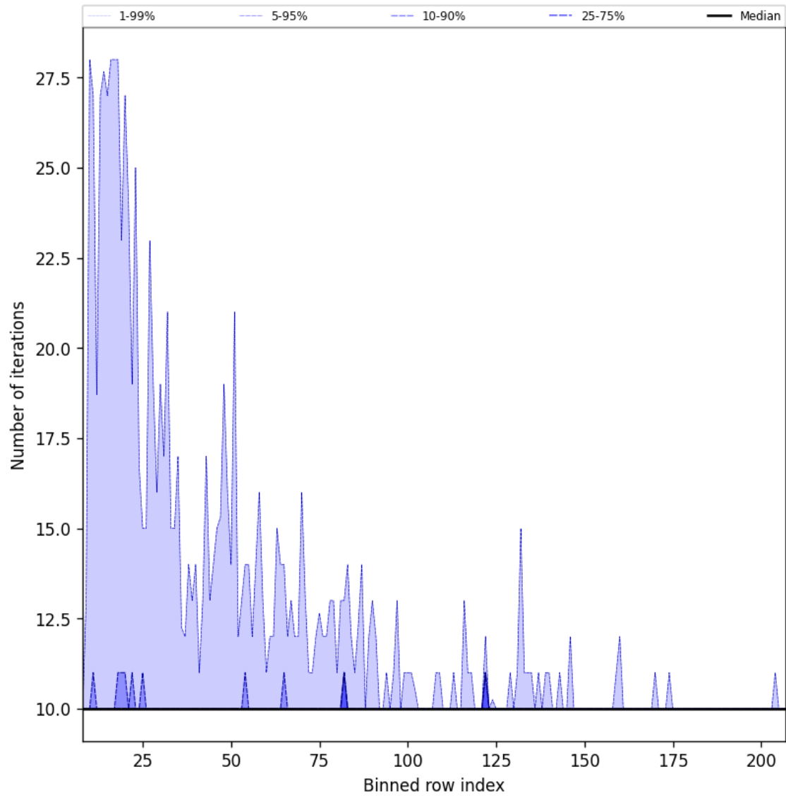
Figure 42: Along track statistics of “Number of iterations” for 2024-09-17 to 2024-09-18
