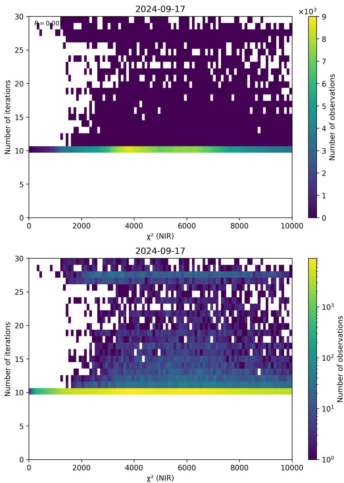
Figure 46: Scatter density plot of “ \chi^2 (NIR)” against “Number of iterations” for 2024-09-17 to 2024-09-18.
