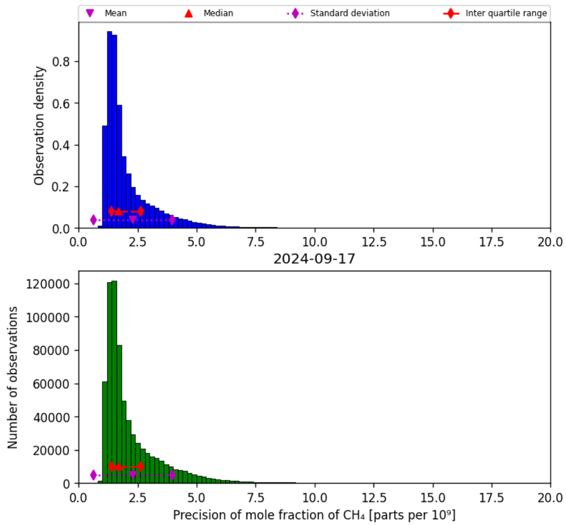
Figure 24: Histogram of “Precision of mole fraction of CH 4 ” for 2024-09-17 to 2024-09-18
