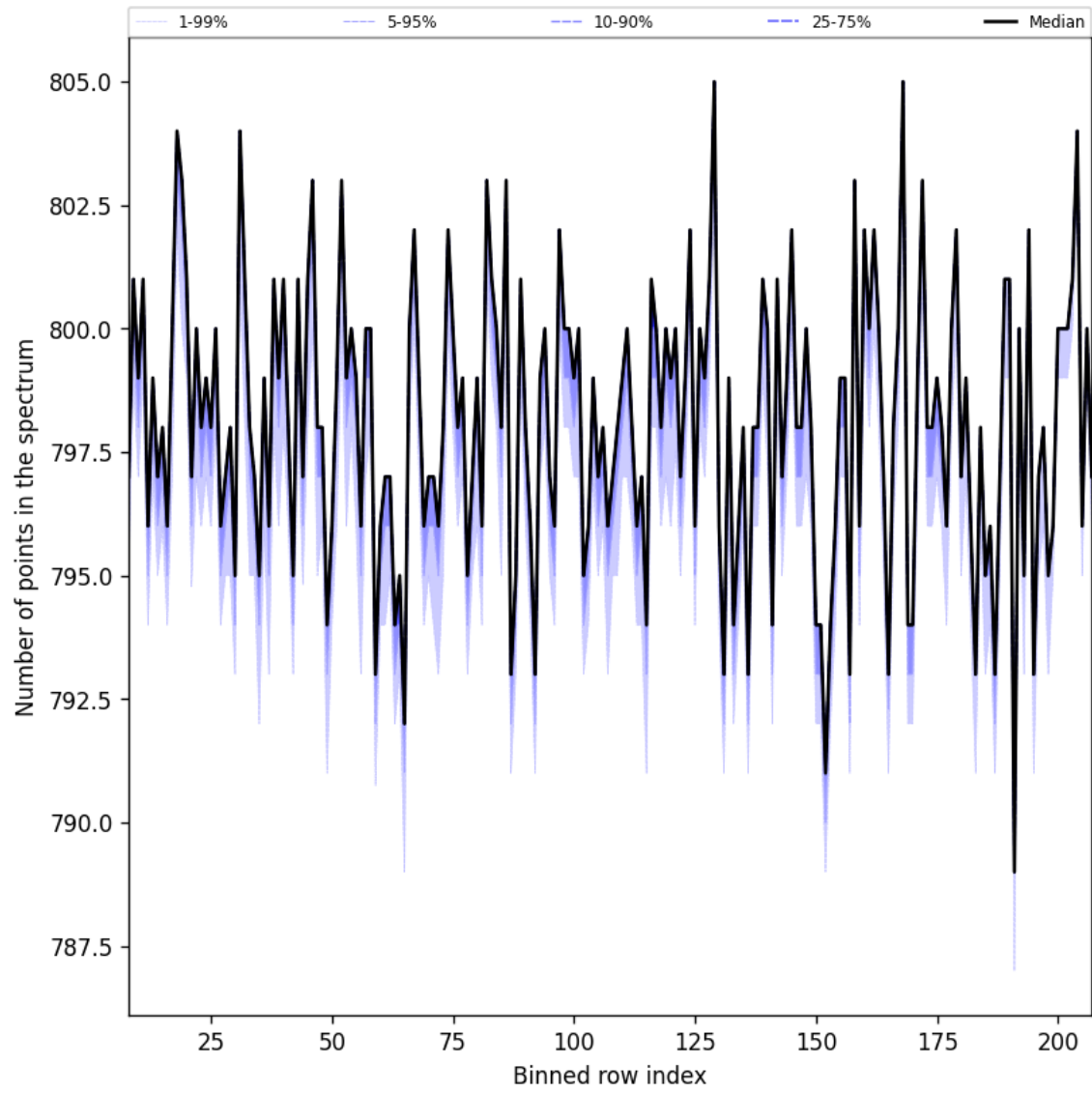
Figure 37: Along track statistics of “Number of points in the spectrum” for 2024-09-17 to 2024-09-18
