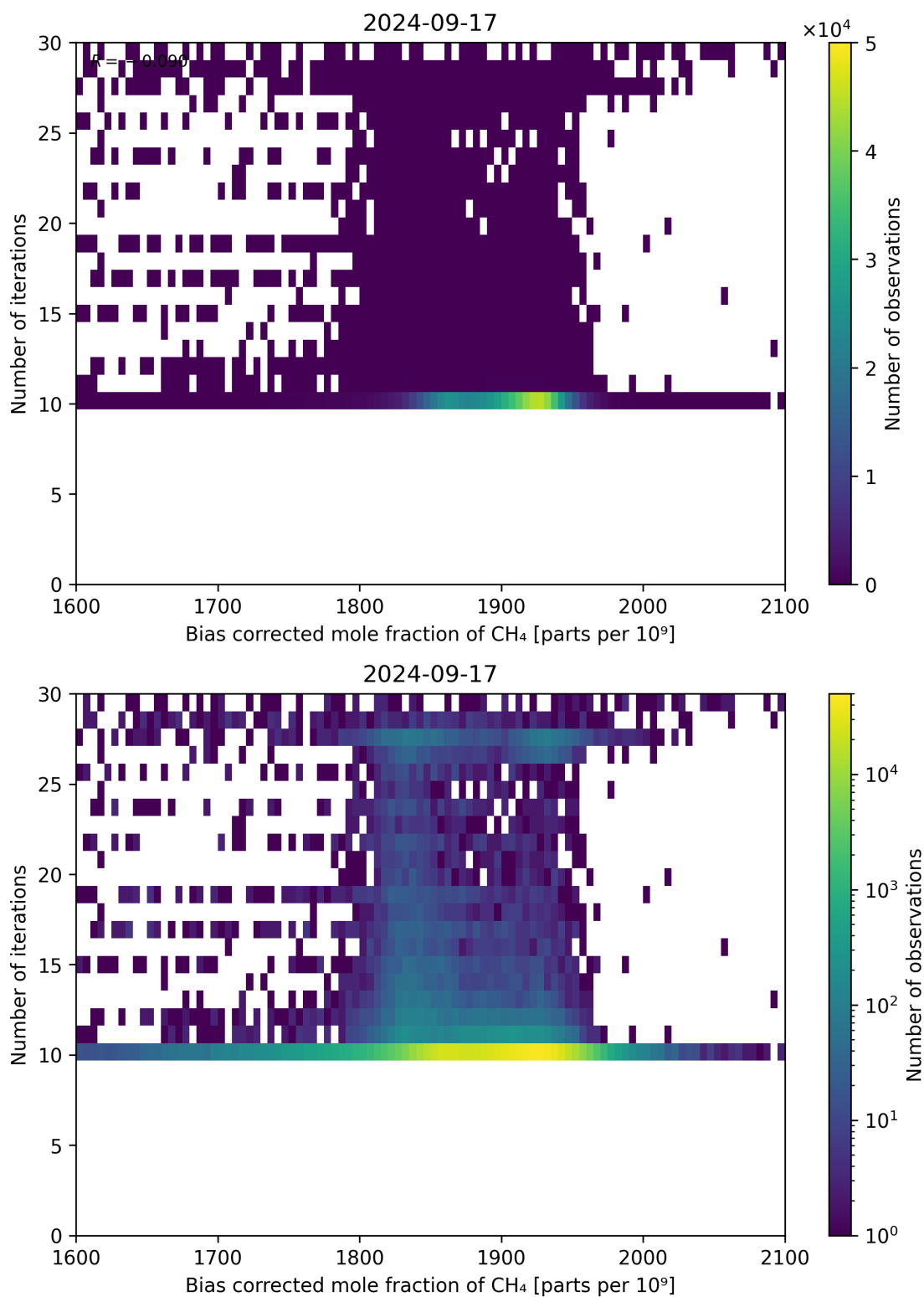
Figure 67: Scatter density plot of “Bias corrected mole fraction of \text{CH}_4 ” against “Number of iterations” for 2024-09-17 to 2024-09-18.
