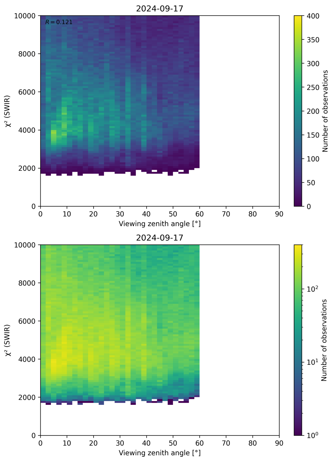
Figure 106: Scatter density plot of “Viewing zenith angle” against “ \chi^2 (SWIR)” for 2024-09-17 to 2024-09-18.
