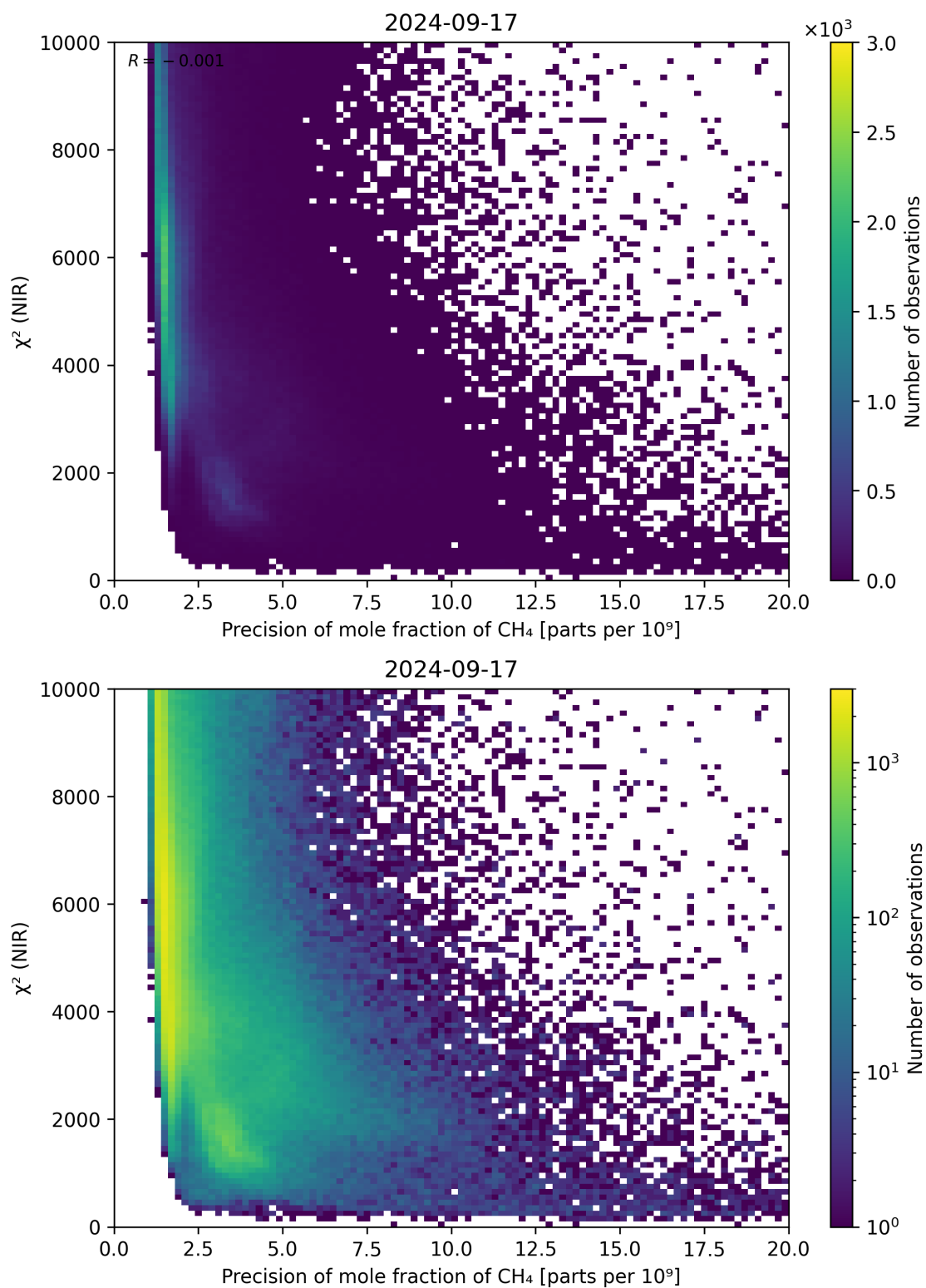
Figure 78: Scatter density plot of “Precision of mole fraction of \text{CH}_4 ” against “ \chi^2 (NIR)” for 2024-09-17 to 2024-09-18.
