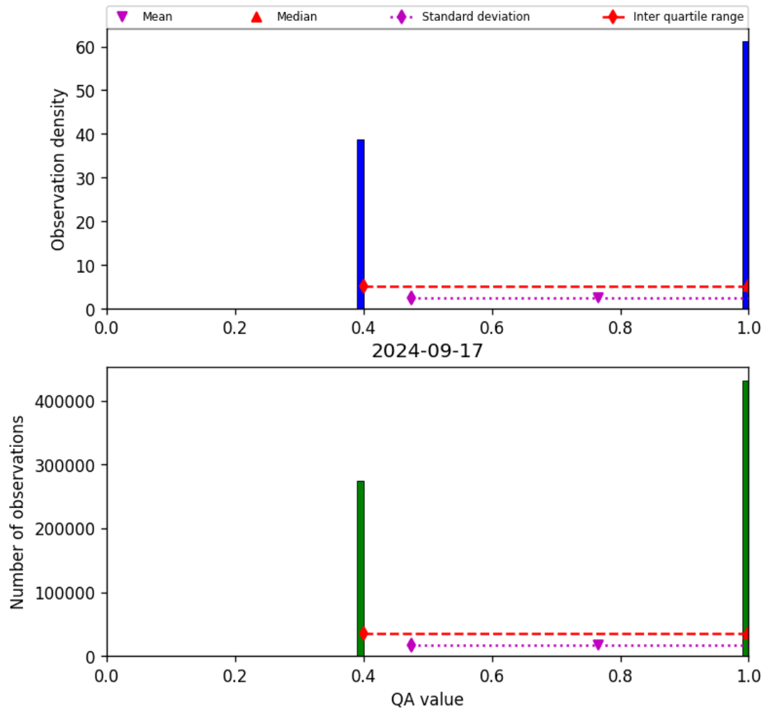
Figure 22: Histogram of “QA value” for 2024-09-17 to 2024-09-18
