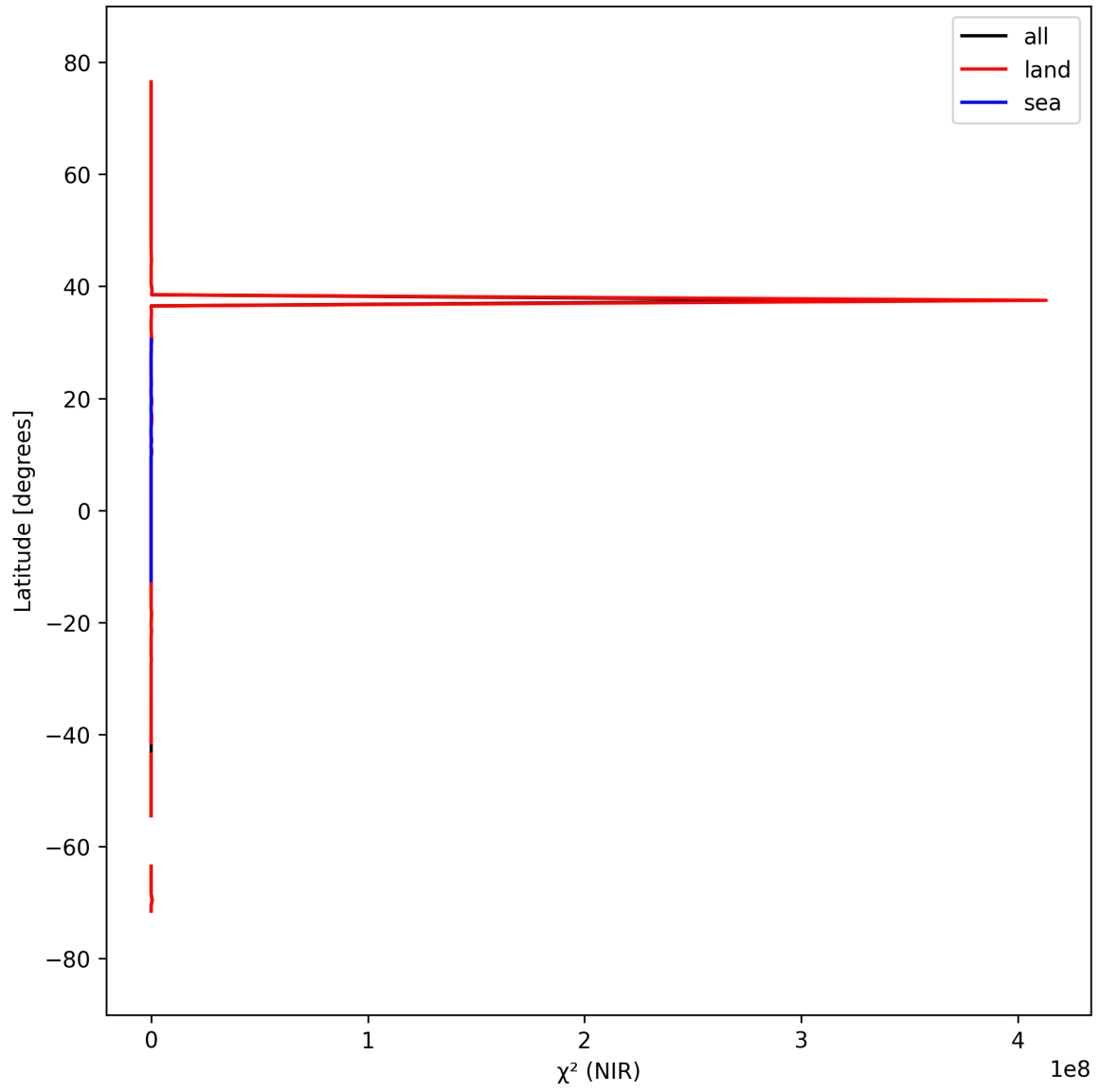
Figure 18: Zonal average of “ \chi^2 (NIR)” for 2024-09-17 to 2024-09-18.
