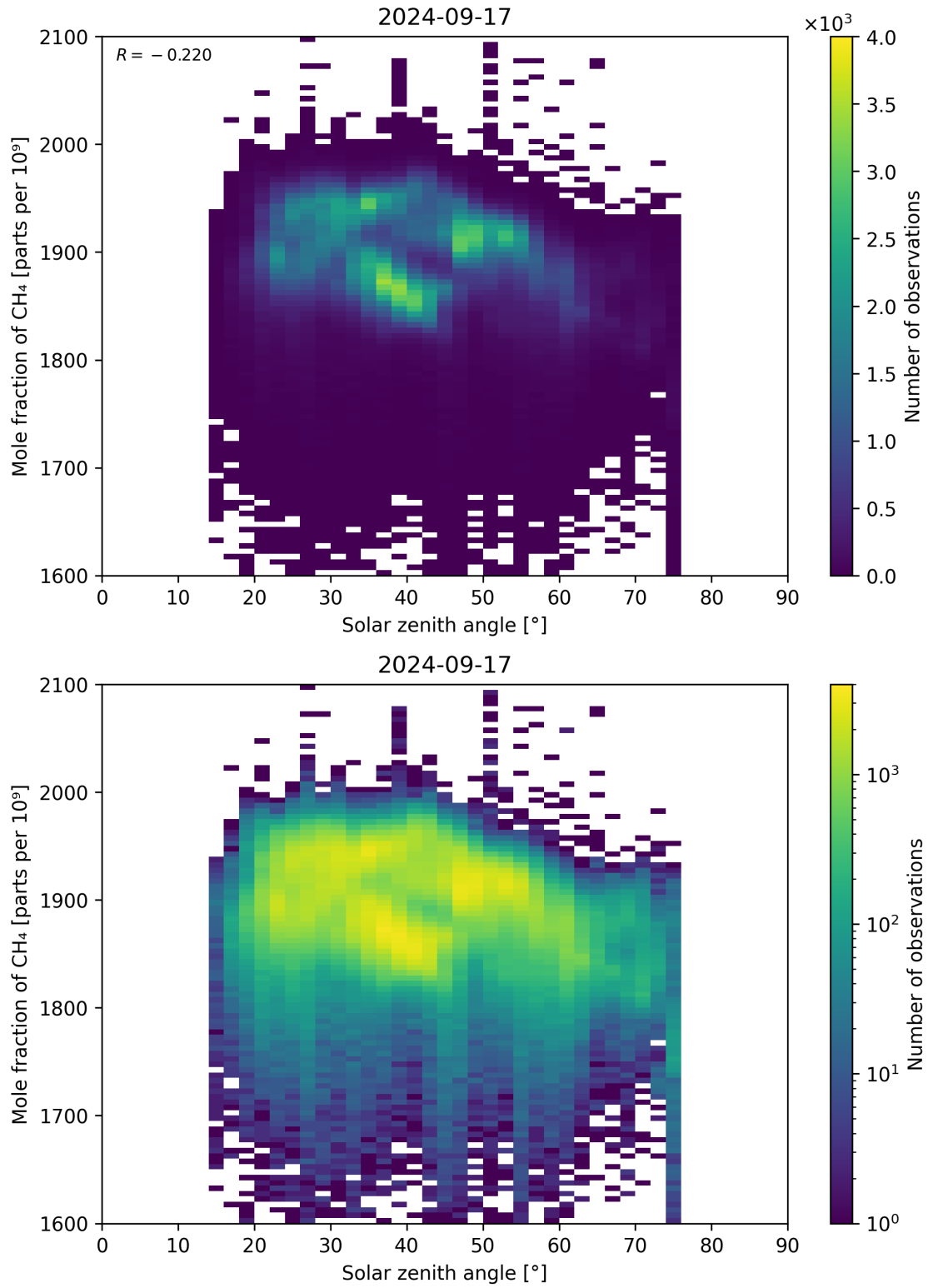
Figure 99: Scatter density plot of “Solar zenith angle” against “Mole fraction of \text{CH}_4 ” for 2024-09-17 to 2024-09-18.
