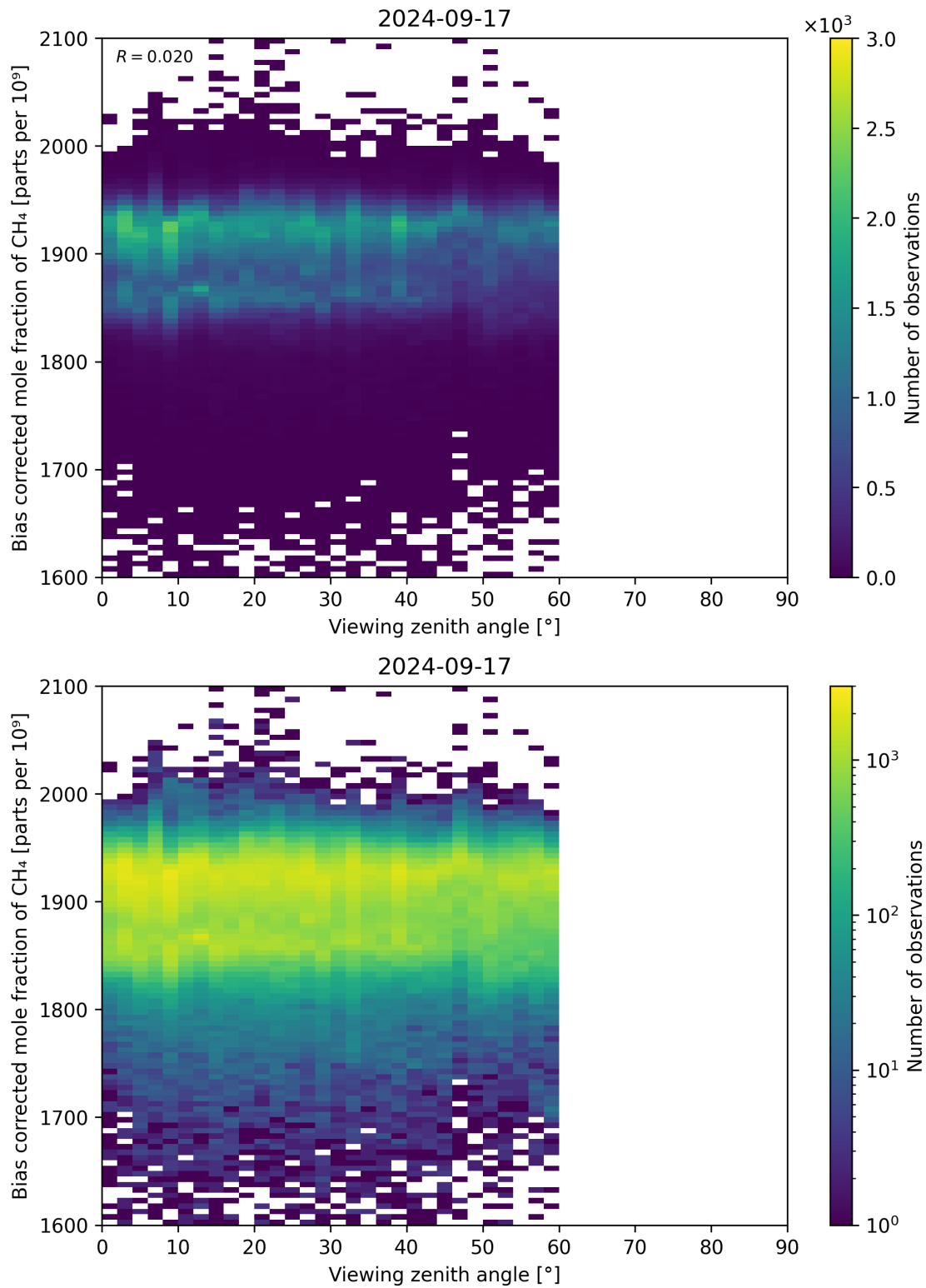
Figure 111: Scatter density plot of “Viewing zenith angle” against “Bias corrected mole fraction of CH 4 ” for 2024-09-17 to 2024-09-18.
