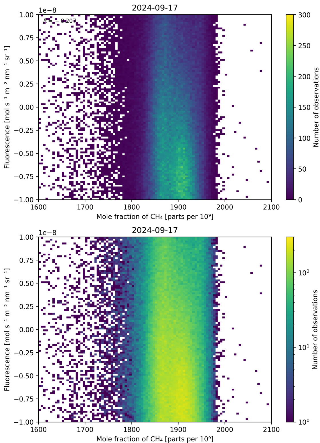
Figure 73: Scatter density plot of “Mole fraction of CH 4 ” against “Fluorescence” for 2024-09-17 to 2024-09-18.
