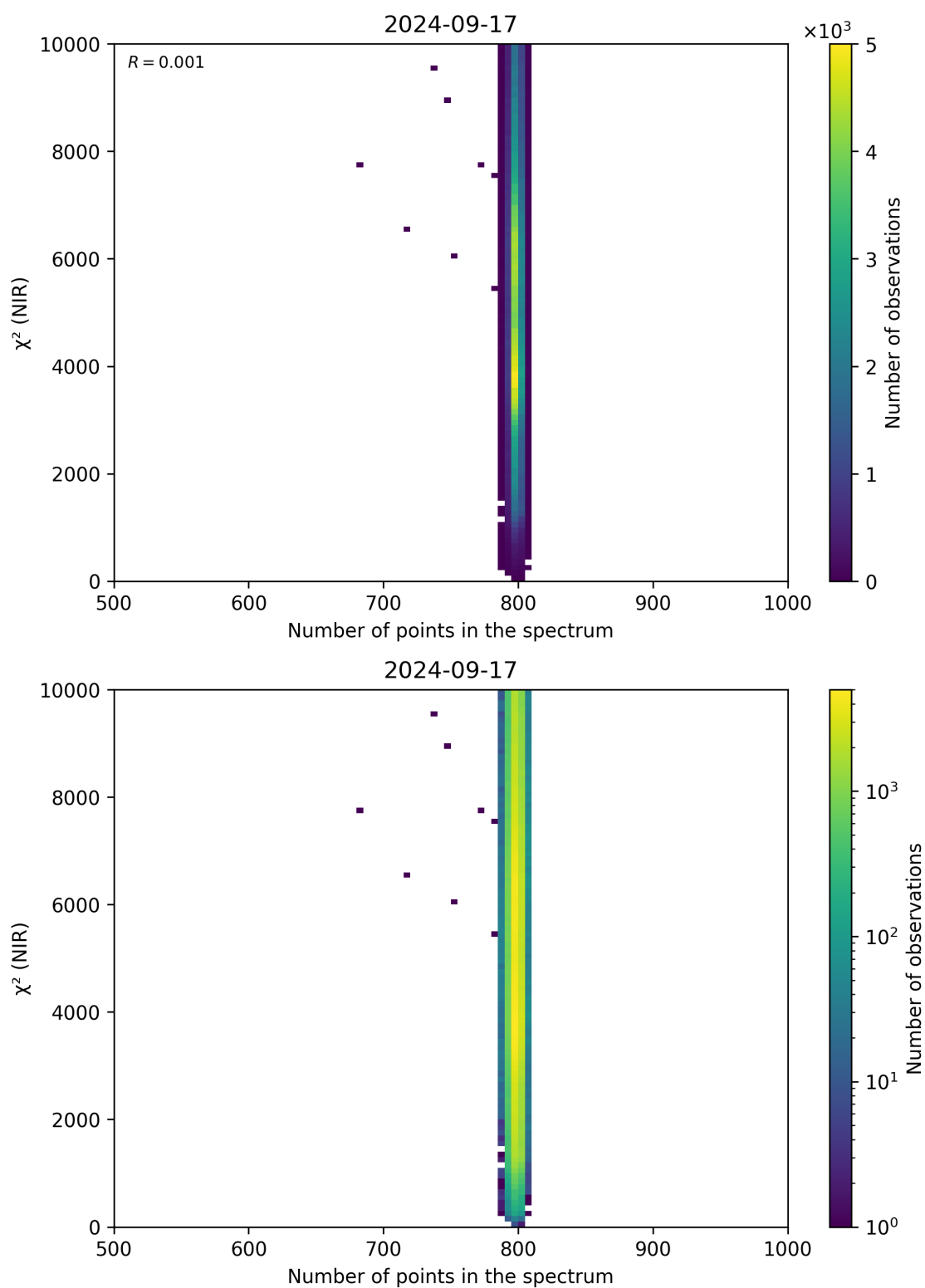
Figure 88: Scatter density plot of “Number of points in the spectrum” against “ \chi^2 (NIR)” for 2024-09-17 to 2024-09-18.
