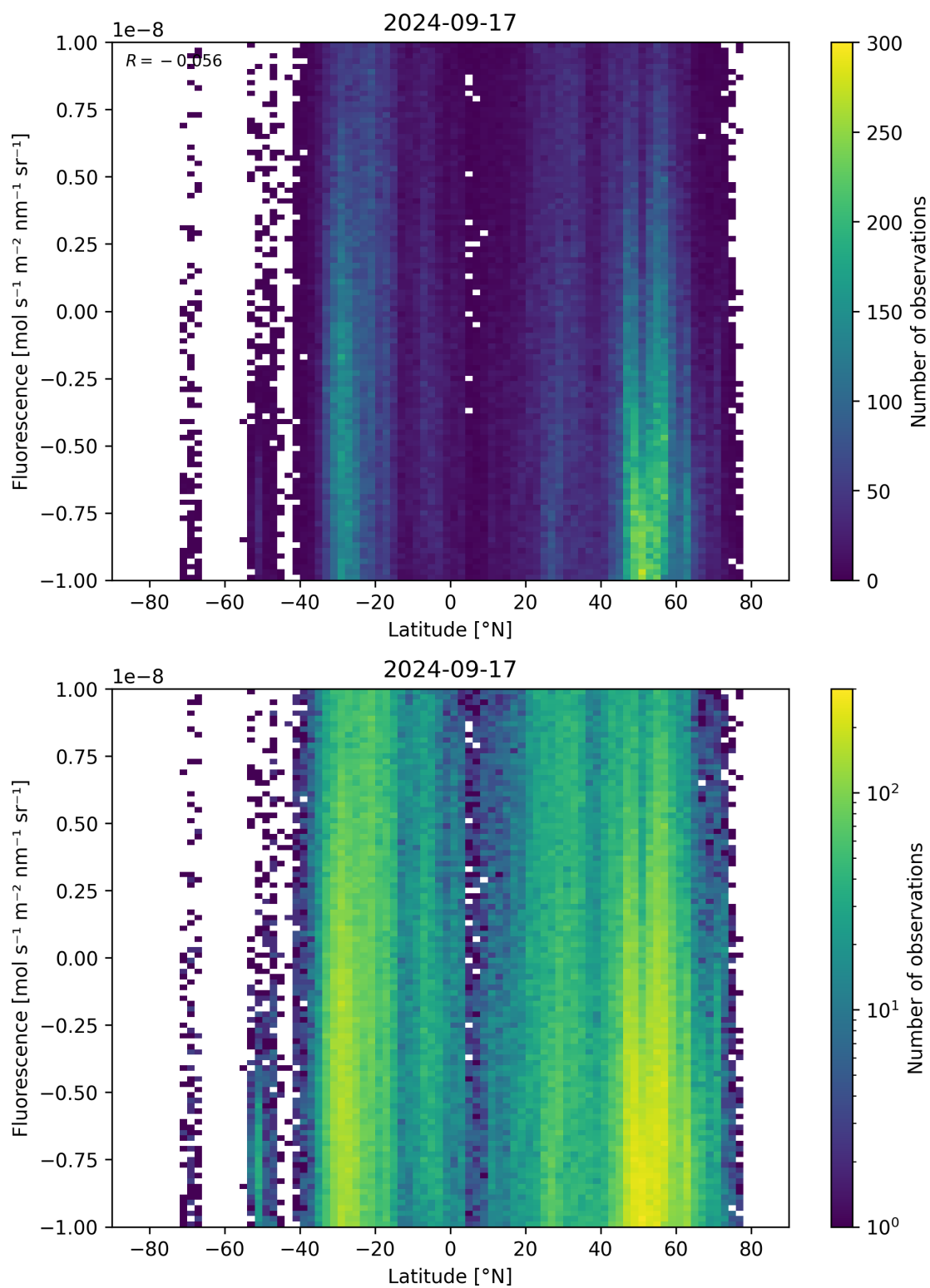
Figure 56: Scatter density plot of “Latitude” against “Fluorescence” for 2024-09-17 to 2024-09-18.
