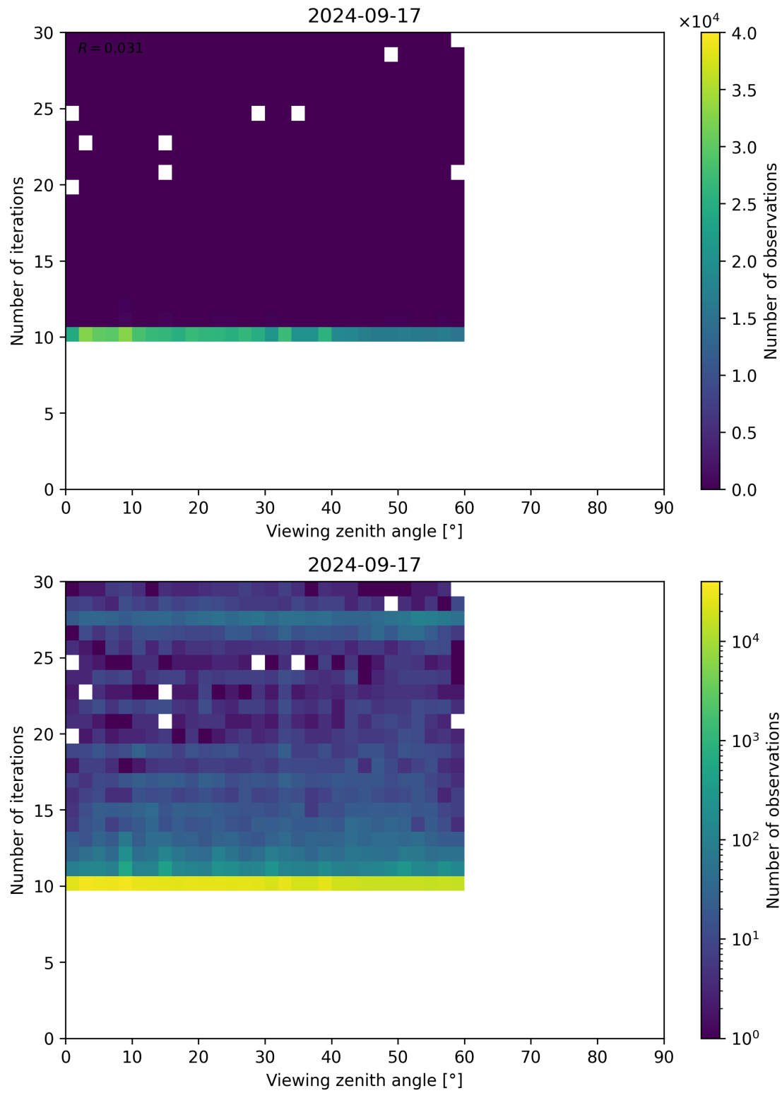
Figure 113: Scatter density plot of “Viewing zenith angle” against “Number of iterations” for 2024-09-17 to 2024-09-18.
