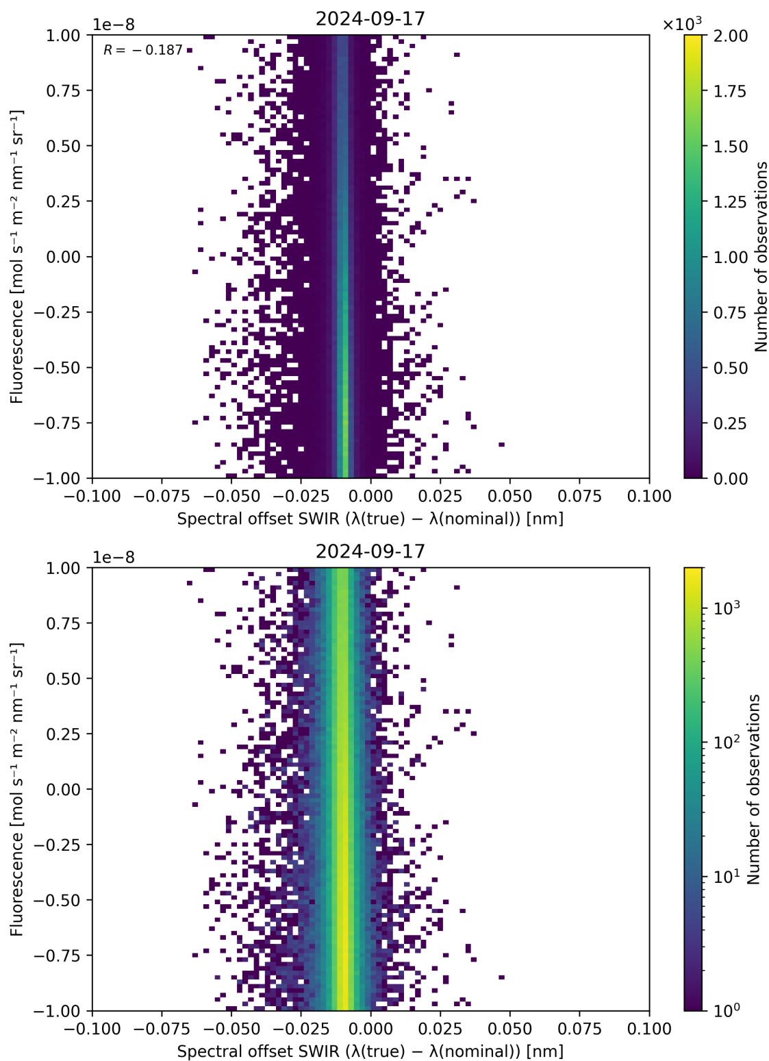
Figure 120: Scatter density plot of “Spectral offset SWIR ( \lambda_{\text{true}} - \lambda_{\text{nominal}} )” against “Fluorescence” for 2024-09-17 to 2024-09-18.
