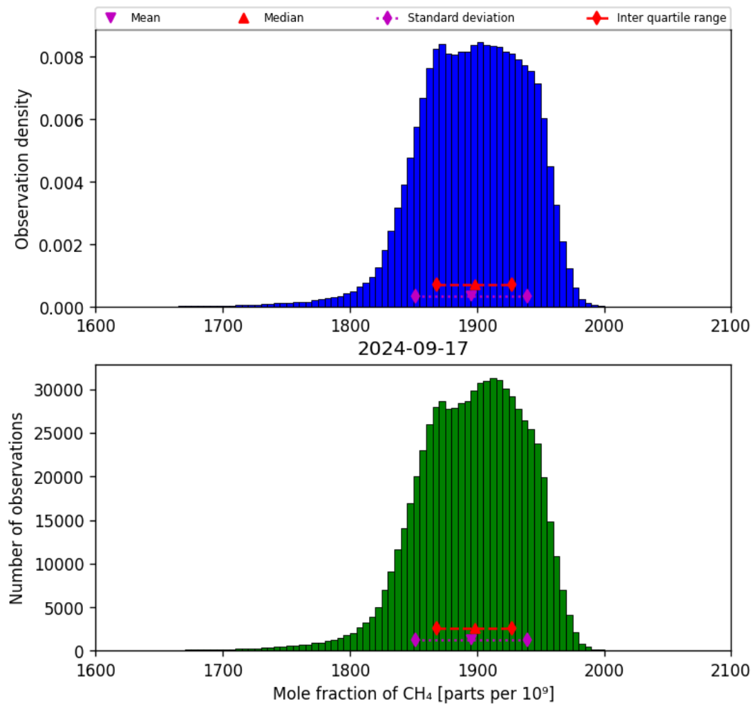
Figure 23: Histogram of “Mole fraction of CH 4 ” for 2024-09-17 to 2024-09-18
