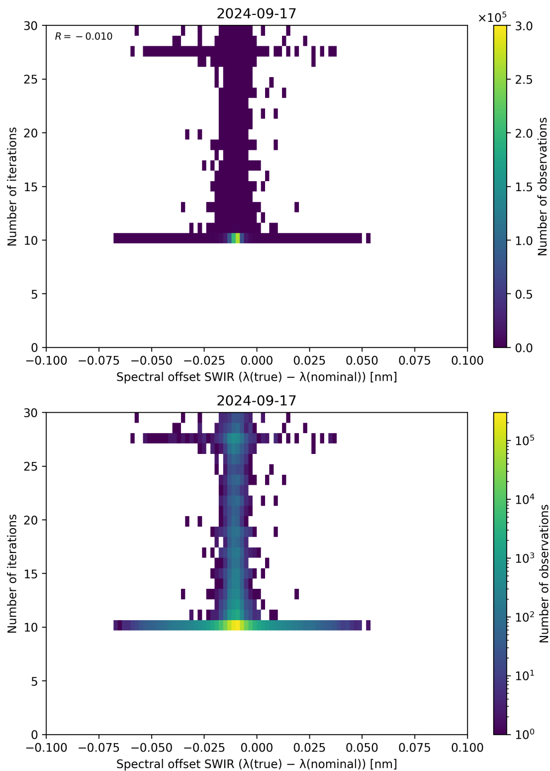
Figure 121: Scatter density plot of “Spectral offset SWIR ( \lambda_{\text{true}} - \lambda_{\text{nominal}} )” against “Number of iterations” for 2024-09-17 to 2024-09-18.
