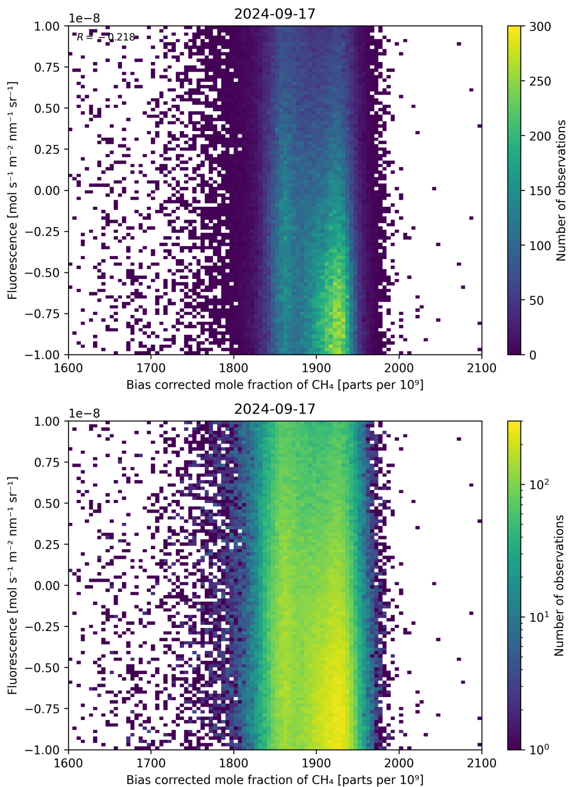
Figure 66: Scatter density plot of “Bias corrected mole fraction of \text{CH}_4 ” against “Fluorescence” for 2024-09-17 to 2024-09-18.
