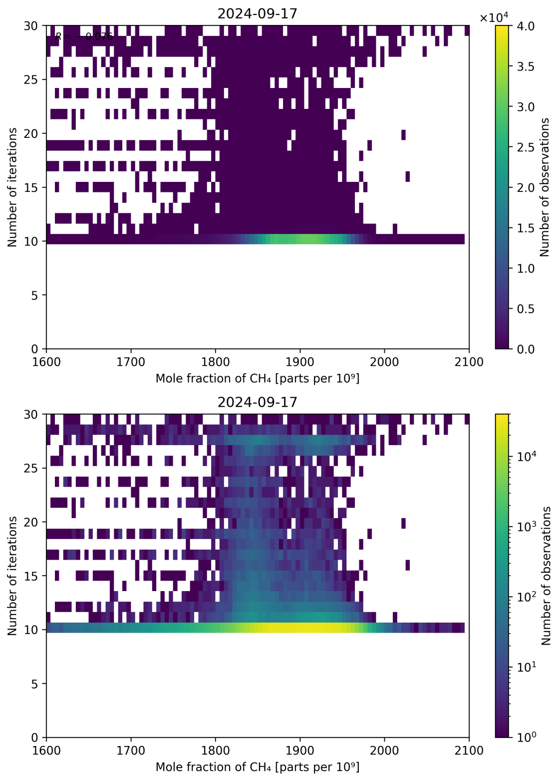
Figure 76: Scatter density plot of “Mole fraction of CH 4 ” against “Number of iterations” for 2024-09-17 to 2024-09-18.
