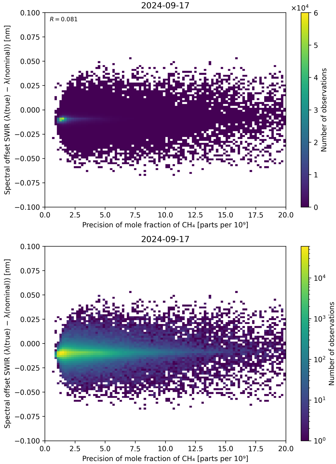
Figure 85: Scatter density plot of “Precision of mole fraction of CH 4 ” against “Spectral offset SWIR ( \lambda_{\text{true}} - \lambda_{\text{nominal}} )” for 2024-09-17 to 2024-09-18.
