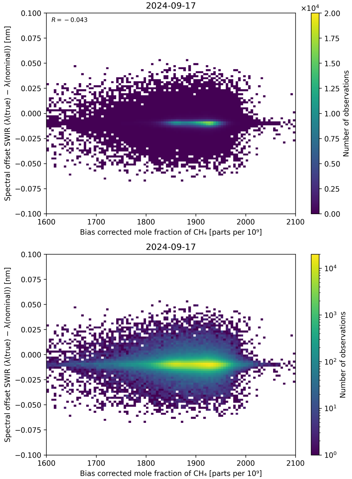
Figure 69: Scatter density plot of “Bias corrected mole fraction of \text{CH}_4 ” against “Spectral offset SWIR ( \lambda_{\text{true}} - \lambda_{\text{nominal}} )” for 2024-09-17 to 2024-09-18.
