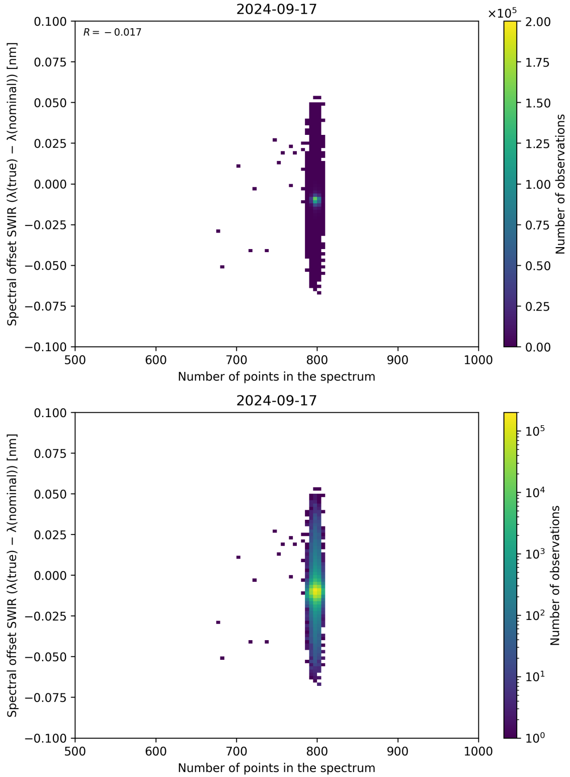
Figure 93: Scatter density plot of “Number of points in the spectrum” against “Spectral offset SWIR ( \lambda_{\text{true}} - \lambda_{\text{nominal}} )” for 2024-09-17 to 2024-09-18.
