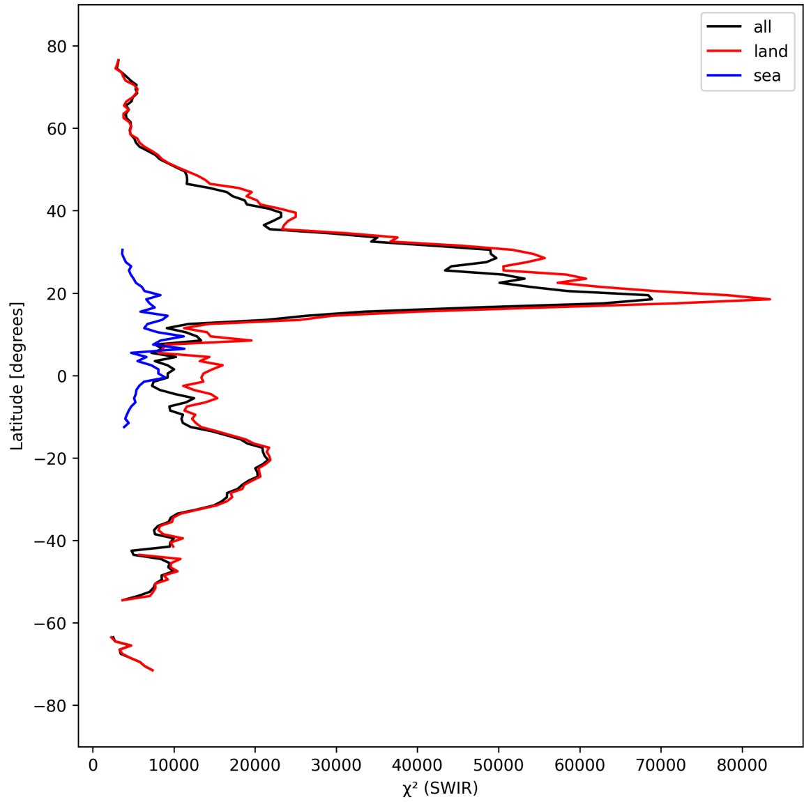
Figure 17: Zonal average of “ \chi^2 (SWIR)” for 2024-09-17 to 2024-09-18.
