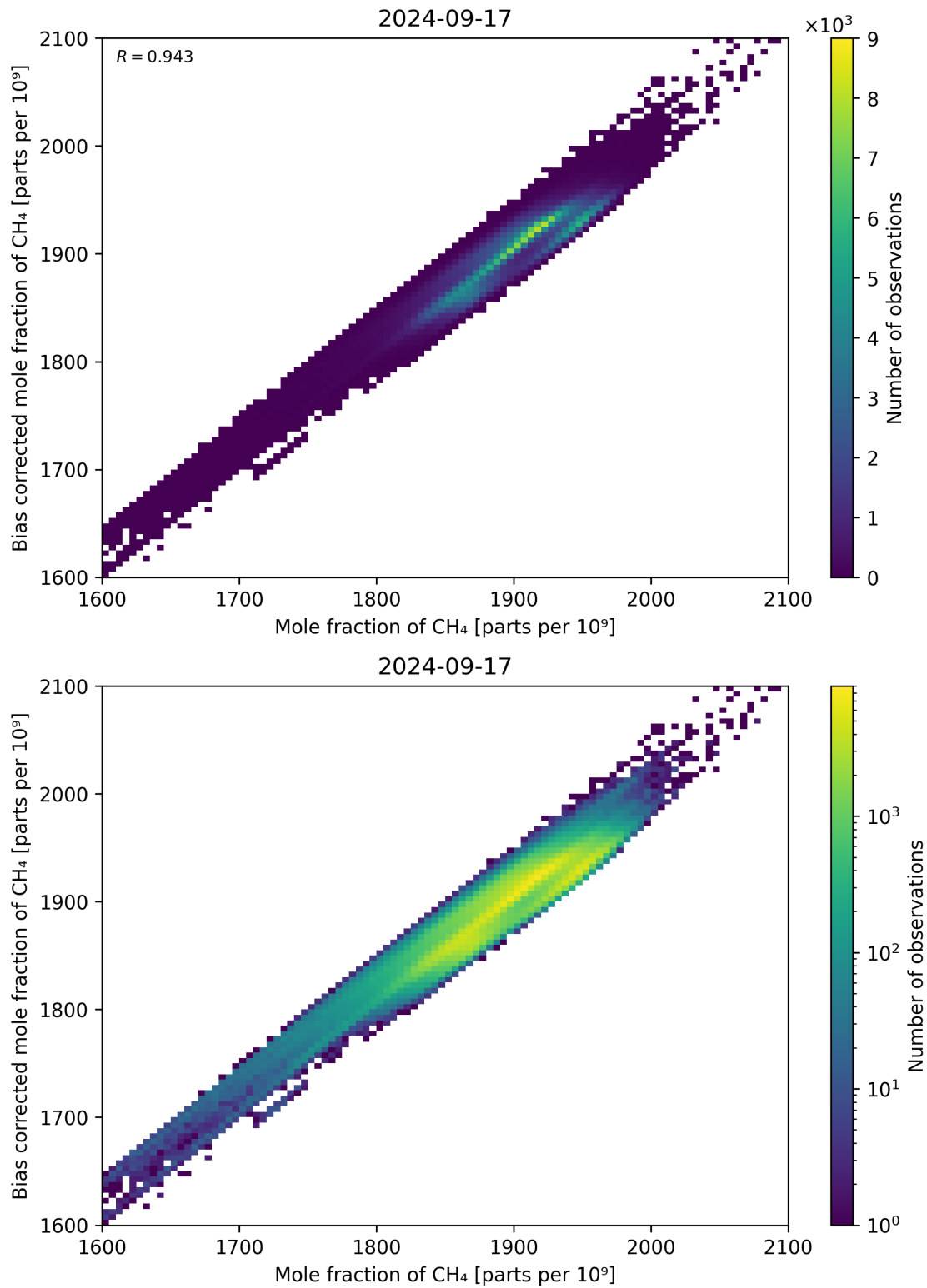
Figure 74: Scatter density plot of “Mole fraction of CH 4 ” against “Bias corrected mole fraction of CH 4 ” for 2024-09-17 to 2024-09-18.
