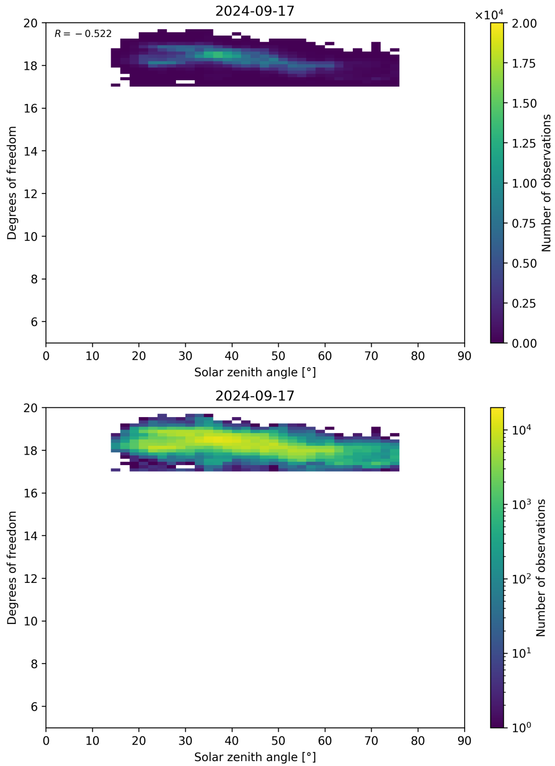
Figure 96: Scatter density plot of “Solar zenith angle” against “Degrees of freedom” for 2024-09-17 to 2024-09-18.
