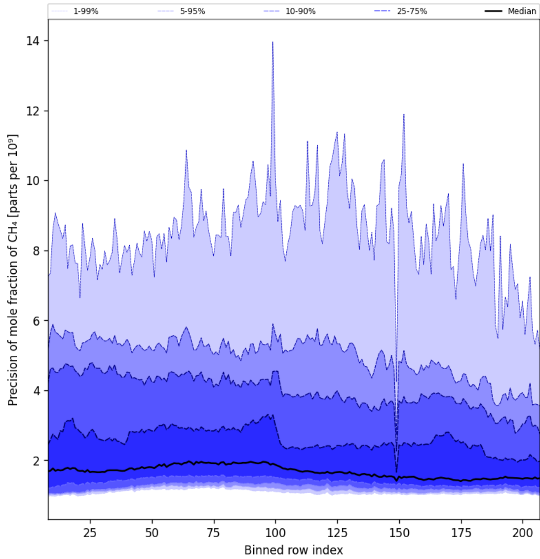
Figure 35: Along track statistics of “Precision of mole fraction of CH 4 ” for 2024-09-17 to 2024-09-18
