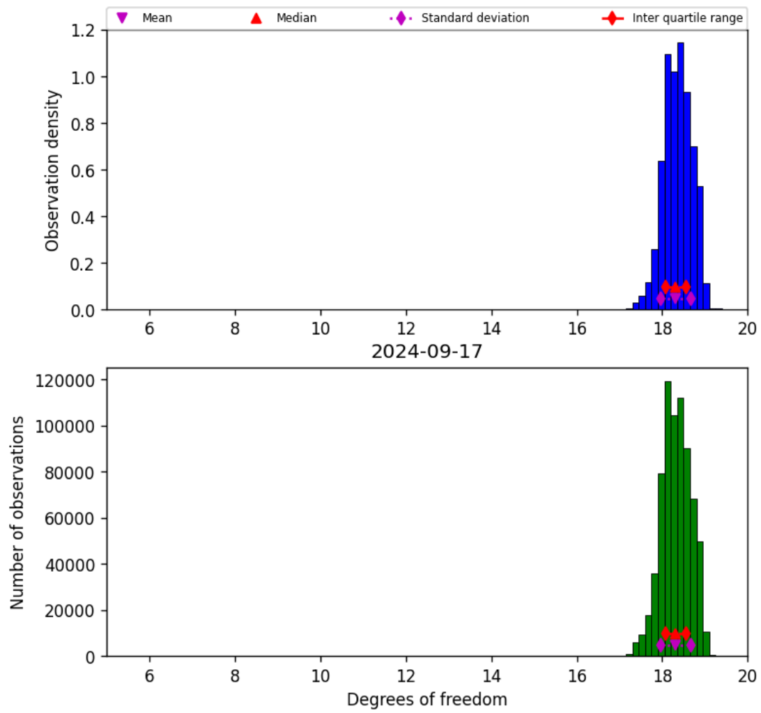
Figure 30: Histogram of “Degrees of freedom” for 2024-09-17 to 2024-09-18
