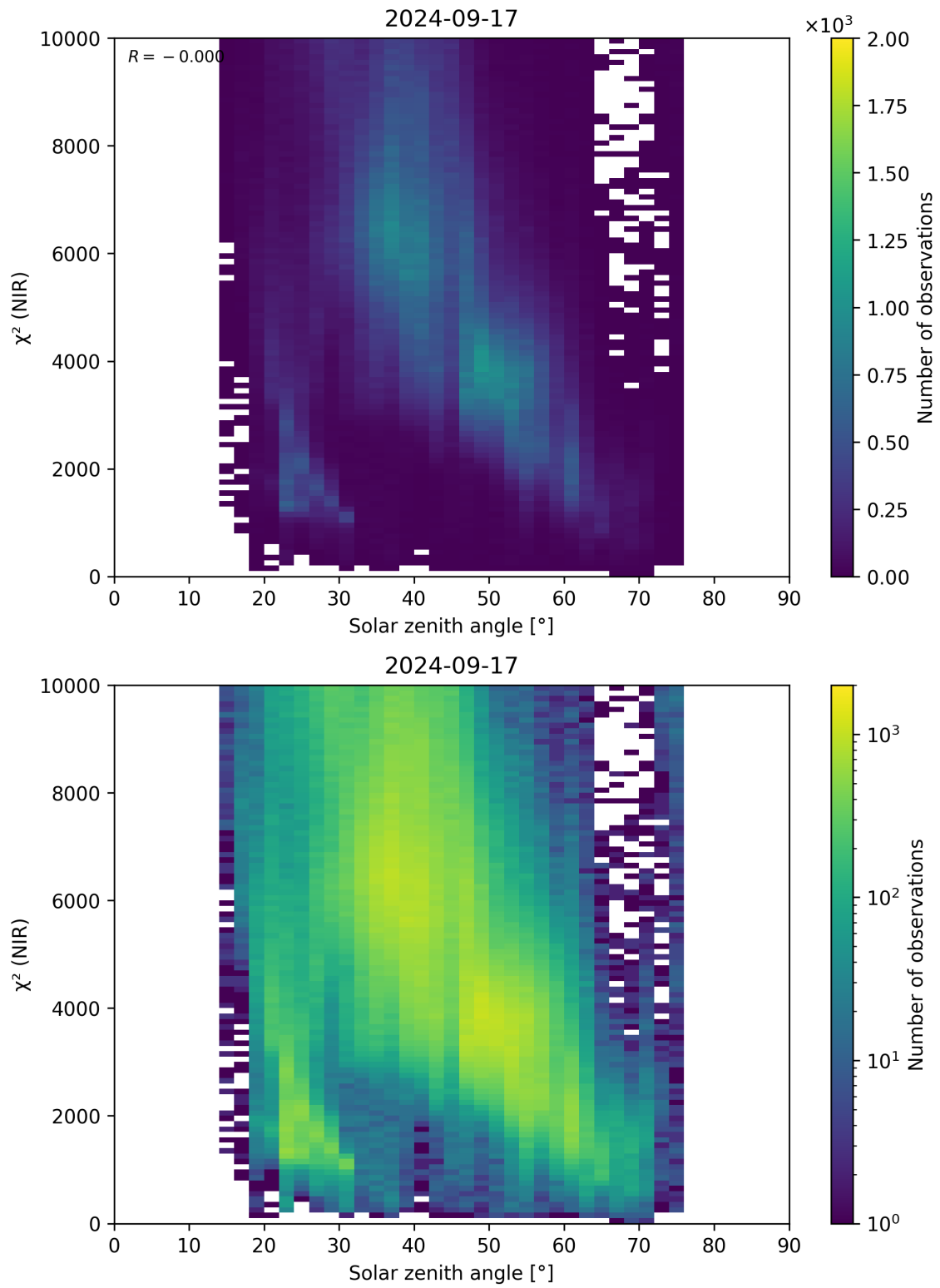
Figure 94: Scatter density plot of “Solar zenith angle” against “ \chi^2 (NIR)” for 2024-09-17 to 2024-09-18.
