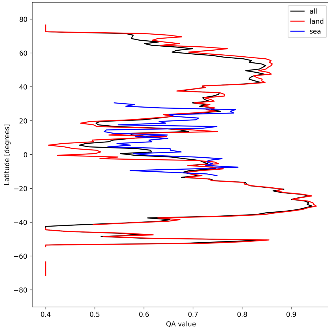
Figure 11: Zonal average of “QA value” for 2024-09-17 to 2024-09-18.
