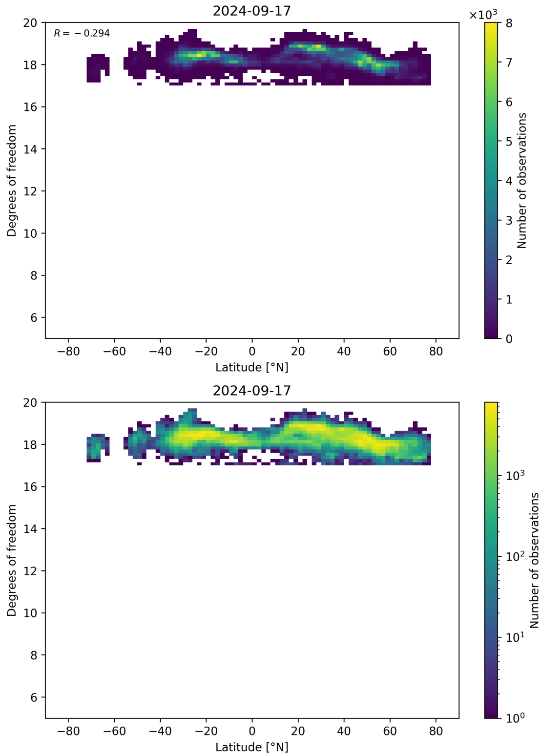
Figure 55: Scatter density plot of “Latitude” against “Degrees of freedom” for 2024-09-17 to 2024-09-18.
