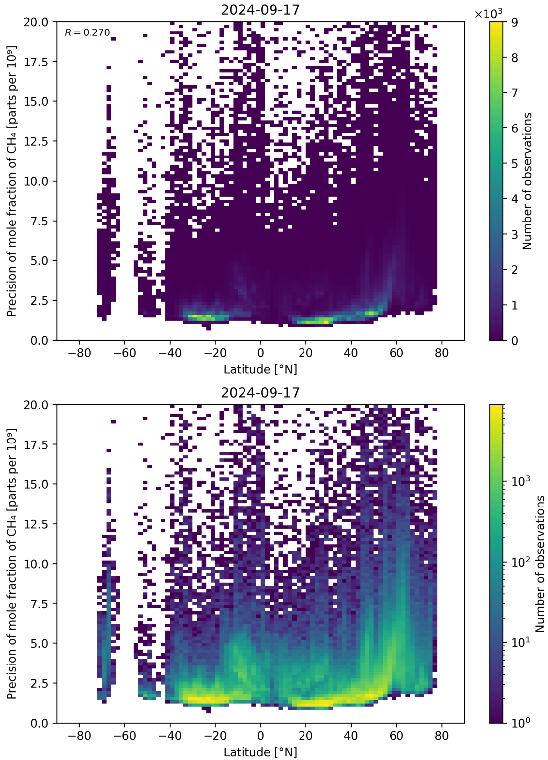
Figure 59: Scatter density plot of “Latitude” against “Precision of mole fraction of CH 4 ” for 2024-09-17 to 2024-09-18.
