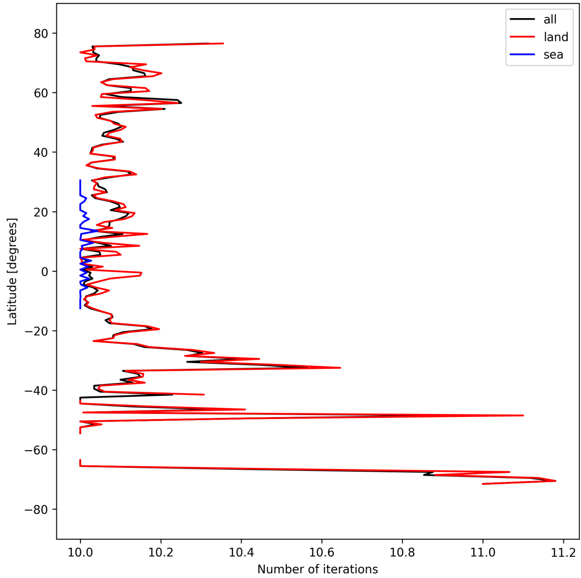
Figure 20: Zonal average of “Number of iterations” for 2024-09-17 to 2024-09-18.
