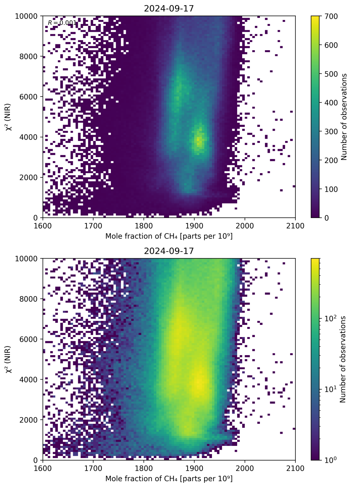
Figure 70: Scatter density plot of “Mole fraction of CH 4 ” against “ \chi^2 (NIR)” for 2024-09-17 to 2024-09-18.
