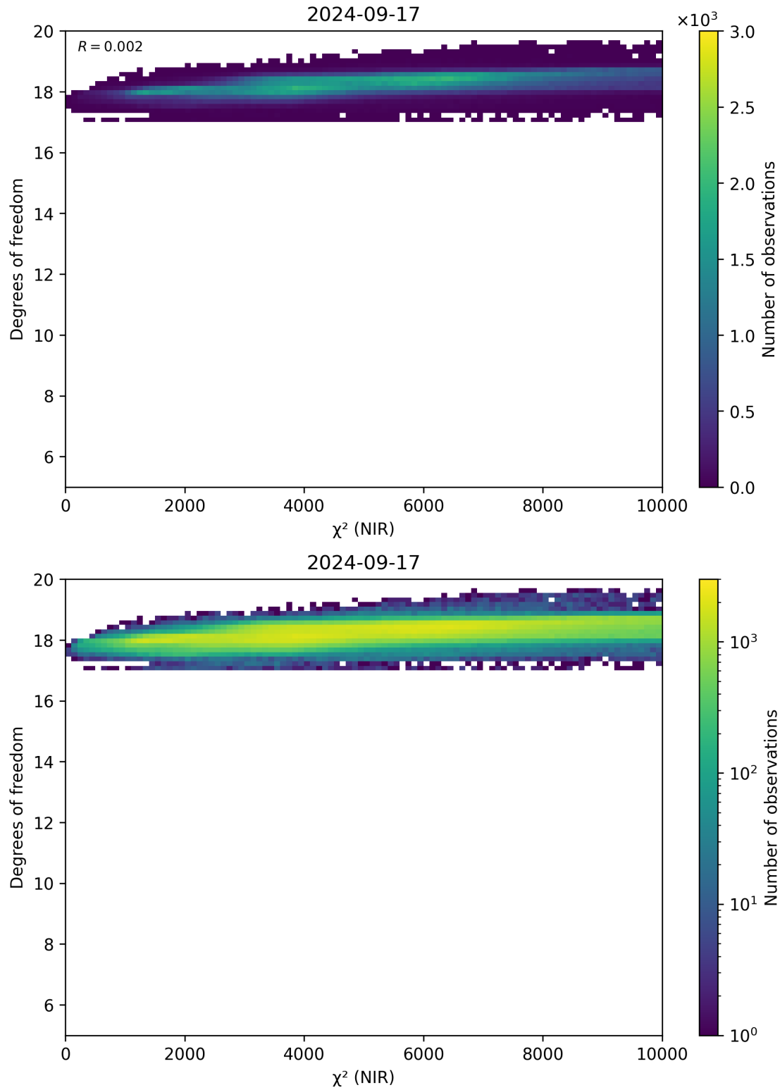
Figure 44: Scatter density plot of “ \chi^2 (NIR)” against “Degrees of freedom” for 2024-09-17 to 2024-09-18.
