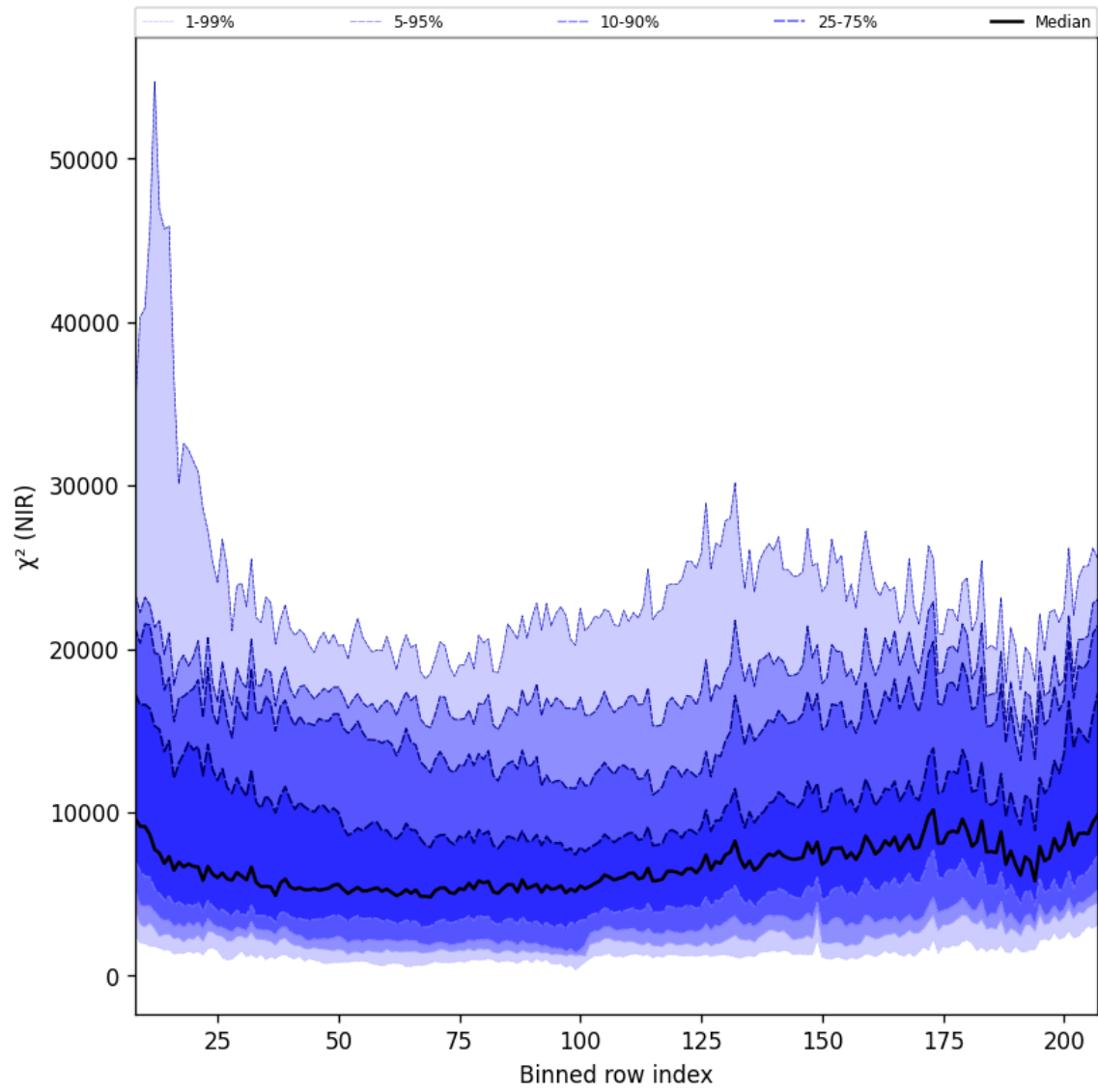
Figure 40: Along track statistics of “ \chi^2 (NIR)” for 2024-09-17 to 2024-09-18
