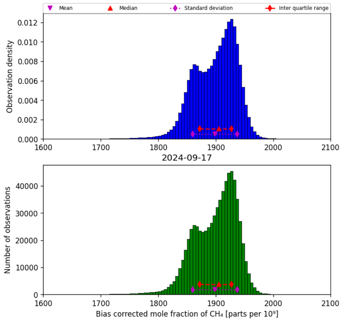
Figure 25: Histogram of “Bias corrected mole fraction of CH 4 ” for 2024-09-17 to 2024-09-18
