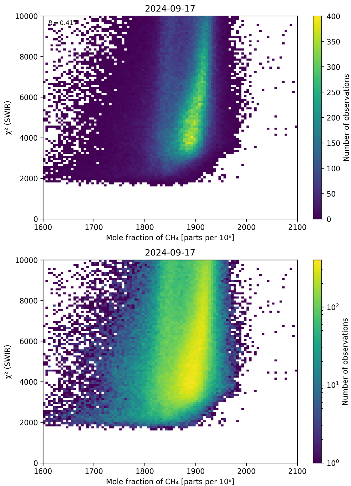
Figure 71: Scatter density plot of “Mole fraction of CH 4 ” against “ \chi^2 (SWIR)” for 2024-09-17 to 2024-09-18.
