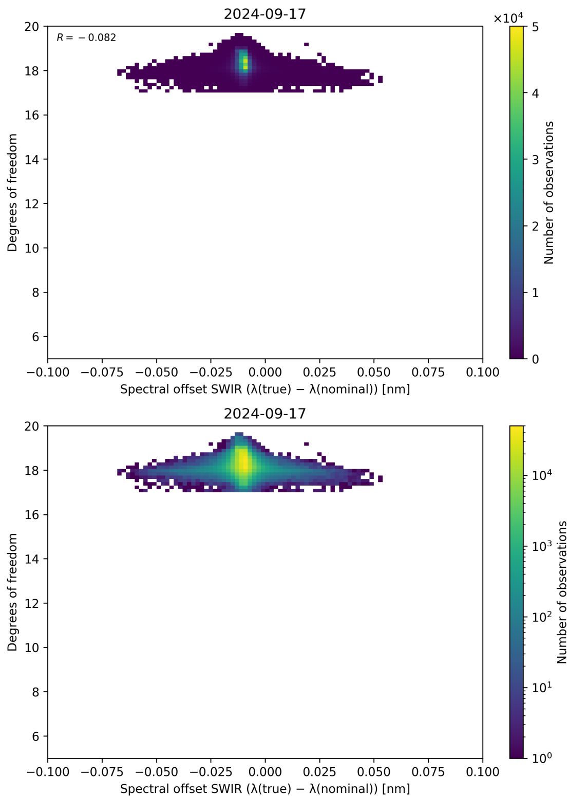
Figure 119: Scatter density plot of “Spectral offset SWIR ( \lambda_{\text{true}} - \lambda_{\text{nominal}} )” against “Degrees of freedom” for 2024-09-17 to 2024-09-18.
