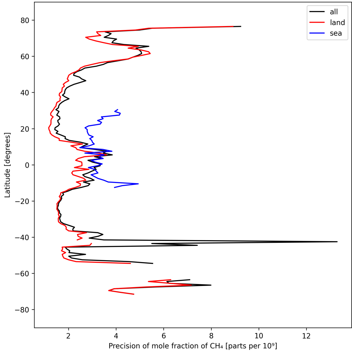
Figure 13: Zonal average of “Precision of mole fraction of \text{CH}_4 ” for 2024-09-17 to 2024-09-18.
