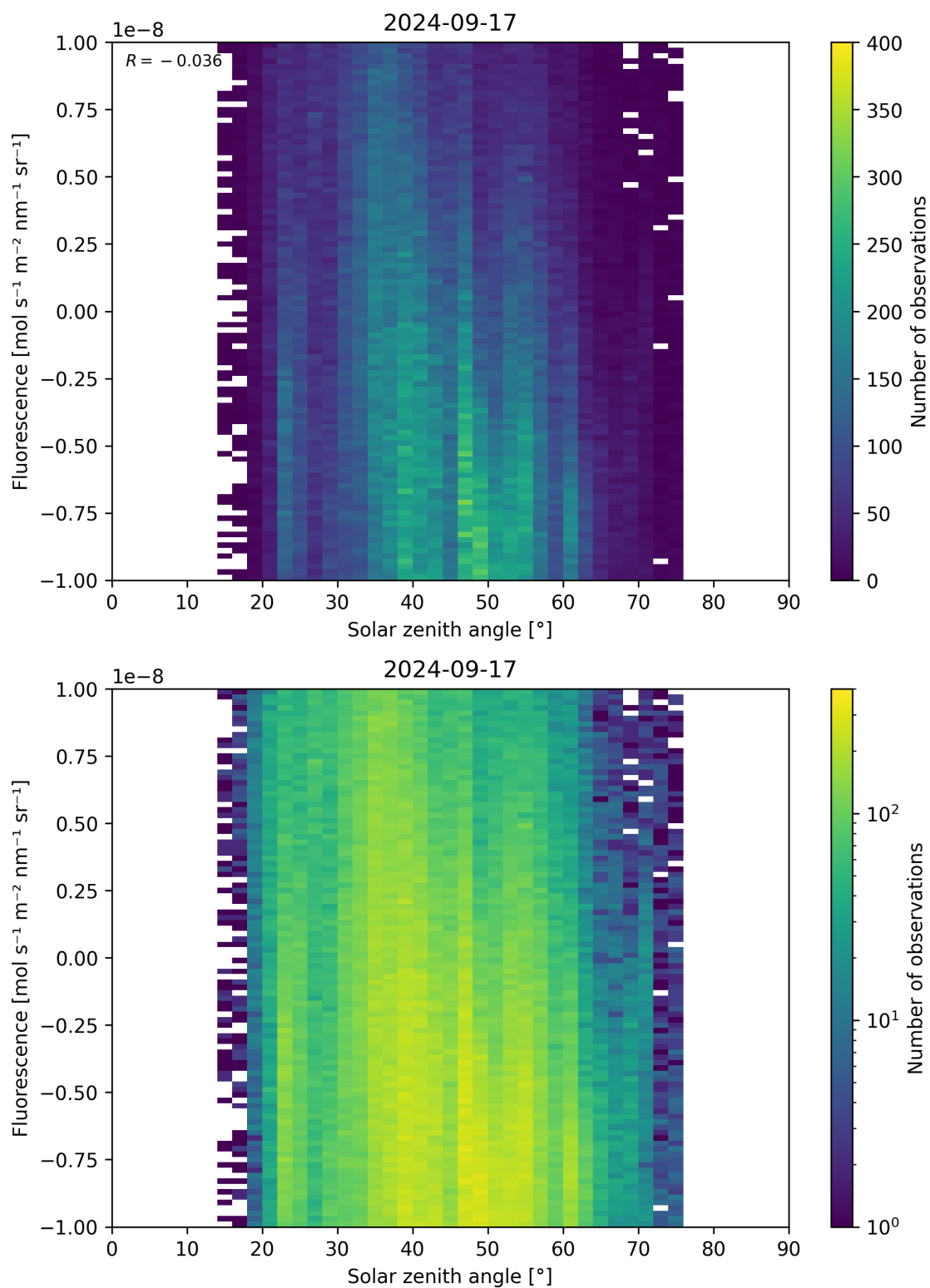
Figure 97: Scatter density plot of “Solar zenith angle” against “Fluorescence” for 2024-09-17 to 2024-09-18.
