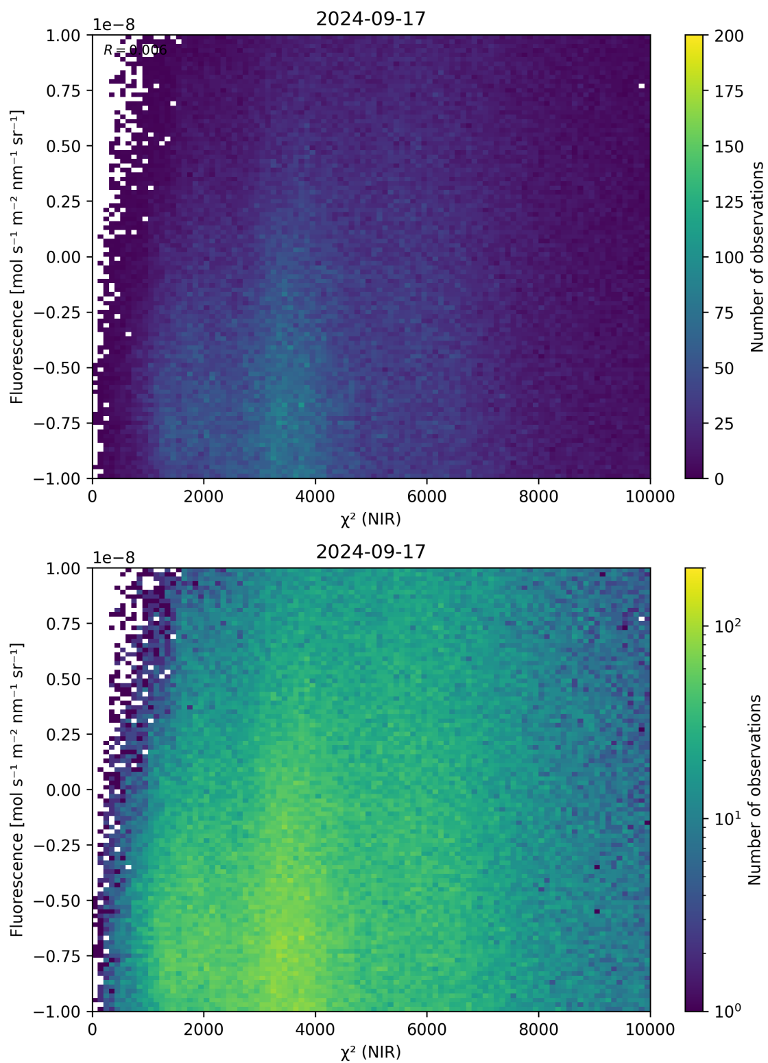
Figure 45: Scatter density plot of “ \chi^2 (NIR)” against “Fluorescence” for 2024-09-17 to 2024-09-18.
