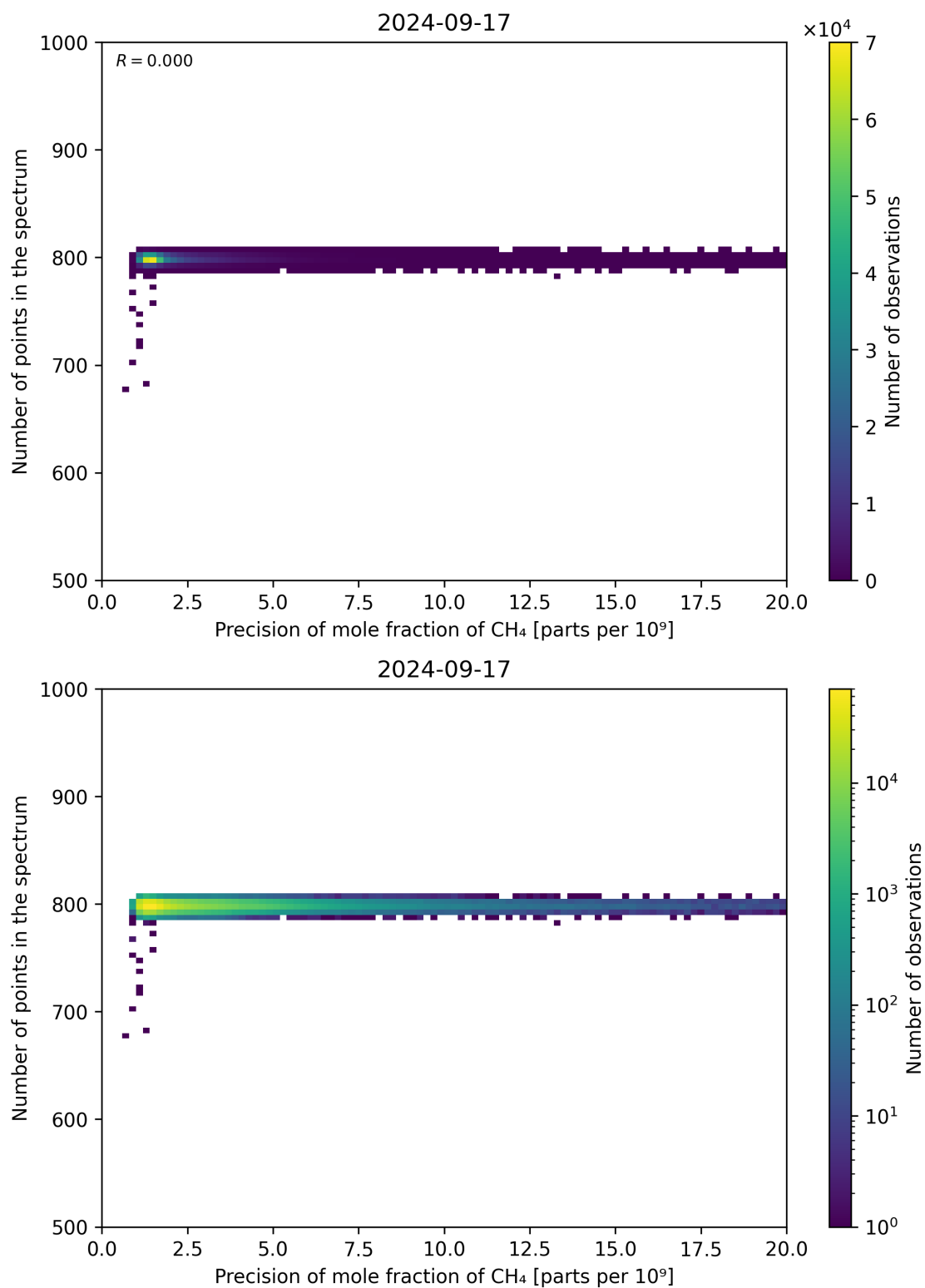
Figure 84: Scatter density plot of “Precision of mole fraction of CH 4 ” against “Number of points in the spectrum” for 2024-09-17 to 2024-09-18.
