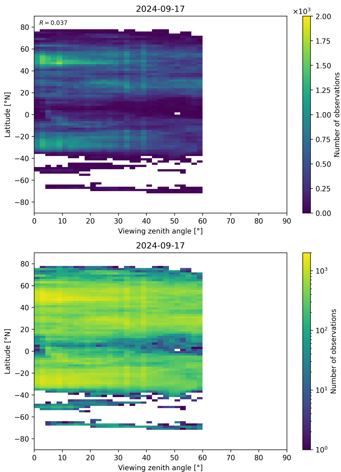
Figure 109: Scatter density plot of “Viewing zenith angle” against “Latitude” for 2024-09-17 to 2024-09-18.
