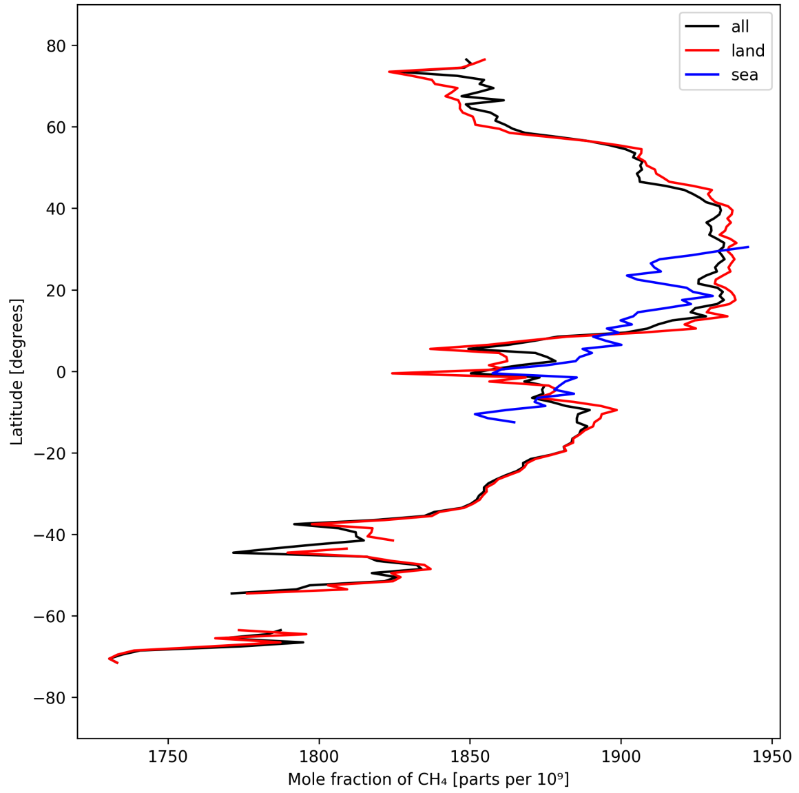
Figure 12: Zonal average of “Mole fraction of \text{CH}_4 ” for 2024-09-17 to 2024-09-18.
