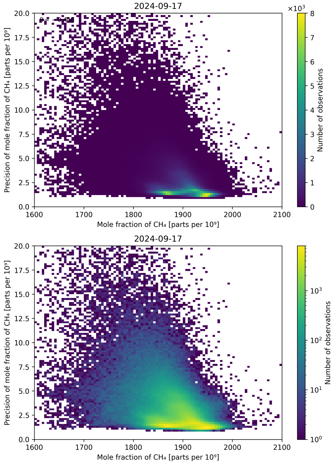
Figure 75: Scatter density plot of “Mole fraction of CH 4 ” against “Precision of mole fraction of CH 4 ” for 2024-09-17 to 2024-09-18.
