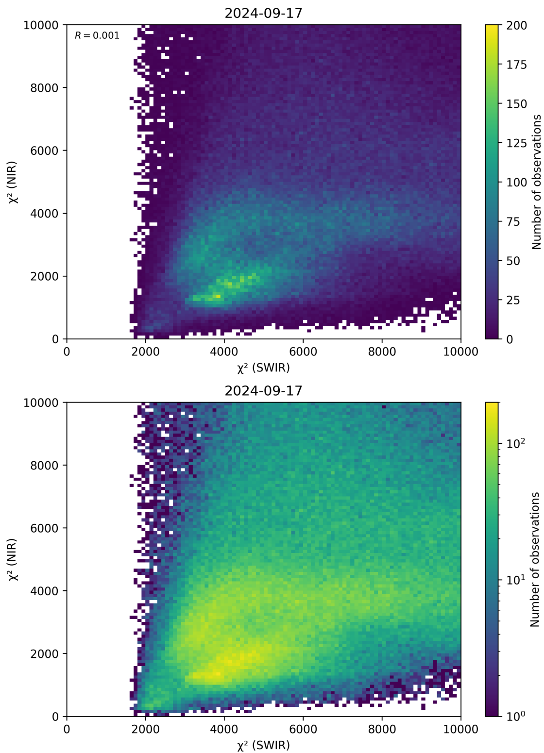
Figure 47: Scatter density plot of “ \chi^2 (SWIR)” against “ \chi^2 (NIR)” for 2024-09-17 to 2024-09-18.
