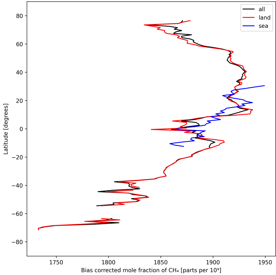
Figure 14: Zonal average of “Bias corrected mole fraction of \text{CH}_4 ” for 2024-09-17 to 2024-09-18.
