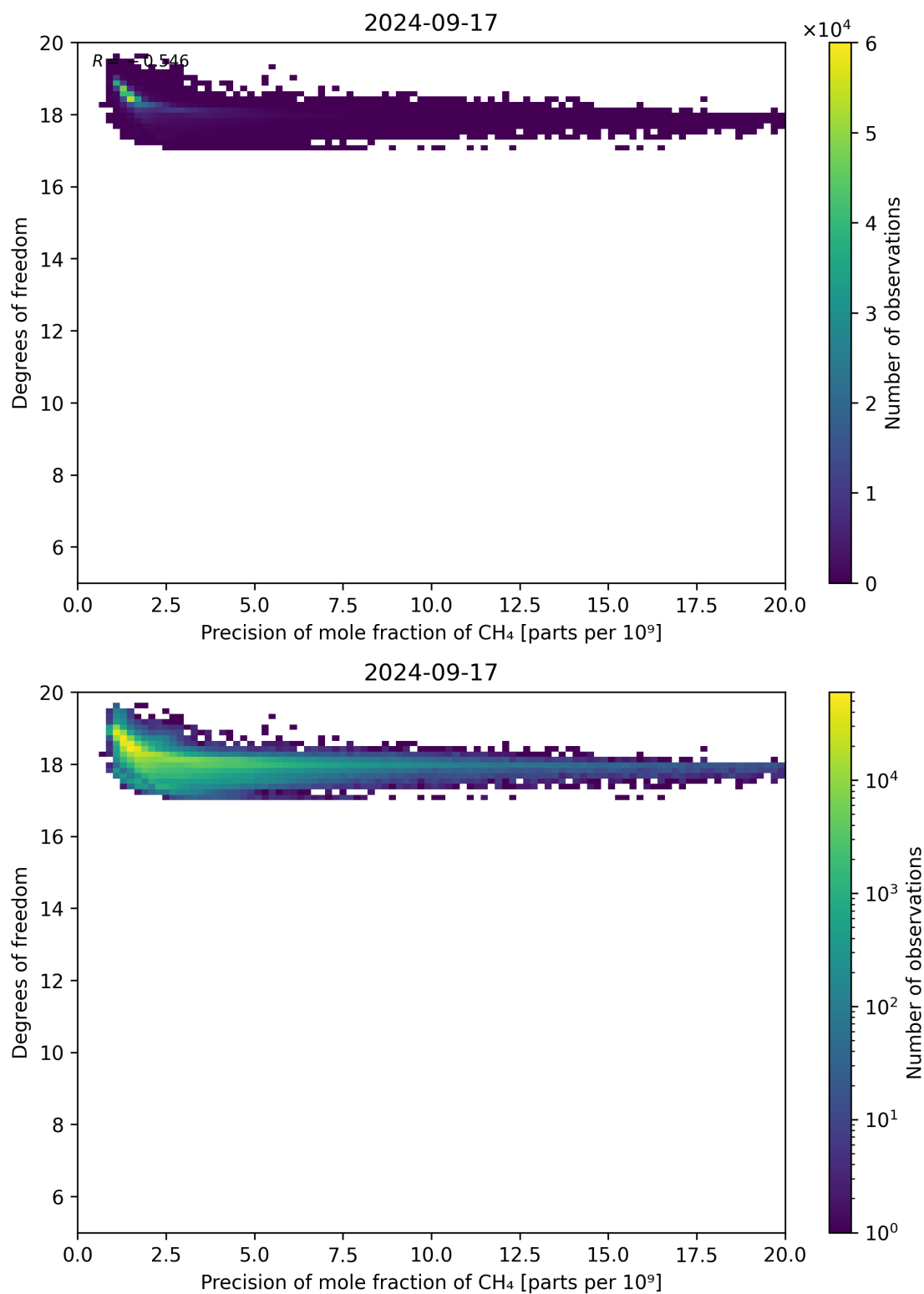
Figure 80: Scatter density plot of “Precision of mole fraction of CH 4 ” against “Degrees of freedom” for 2024-09-17 to 2024-09-18.
