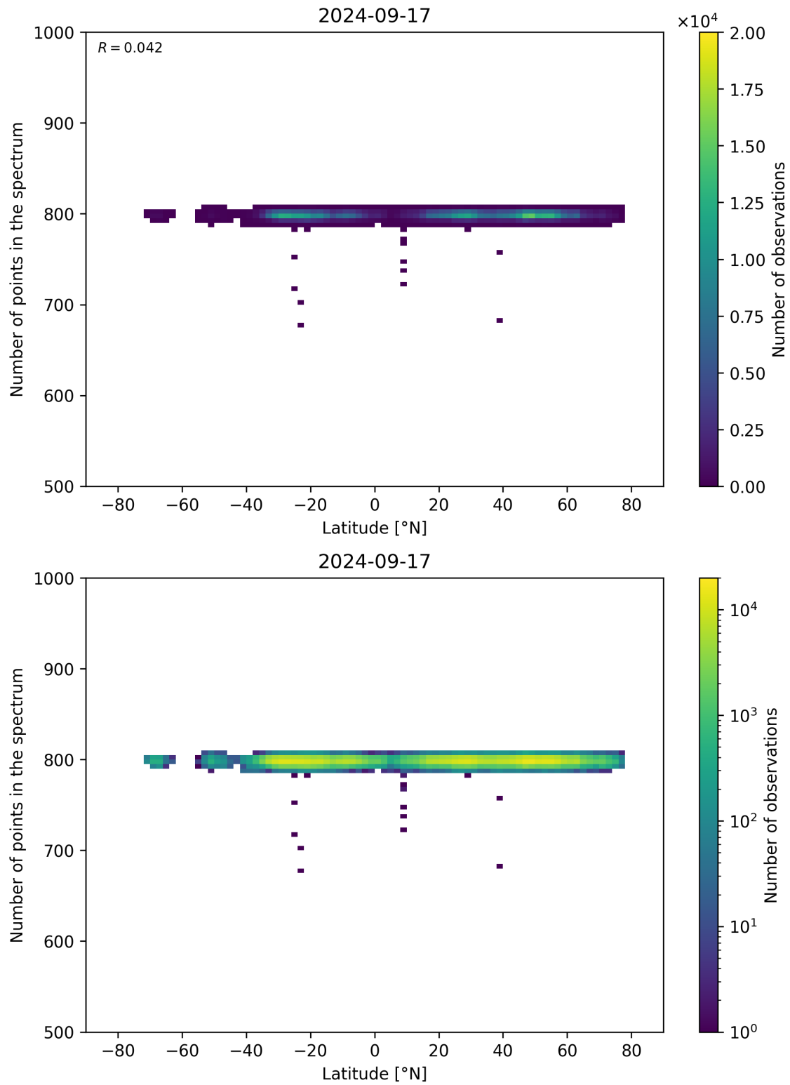
Figure 61: Scatter density plot of “Latitude” against “Number of points in the spectrum” for 2024-09-17 to 2024-09-18.
