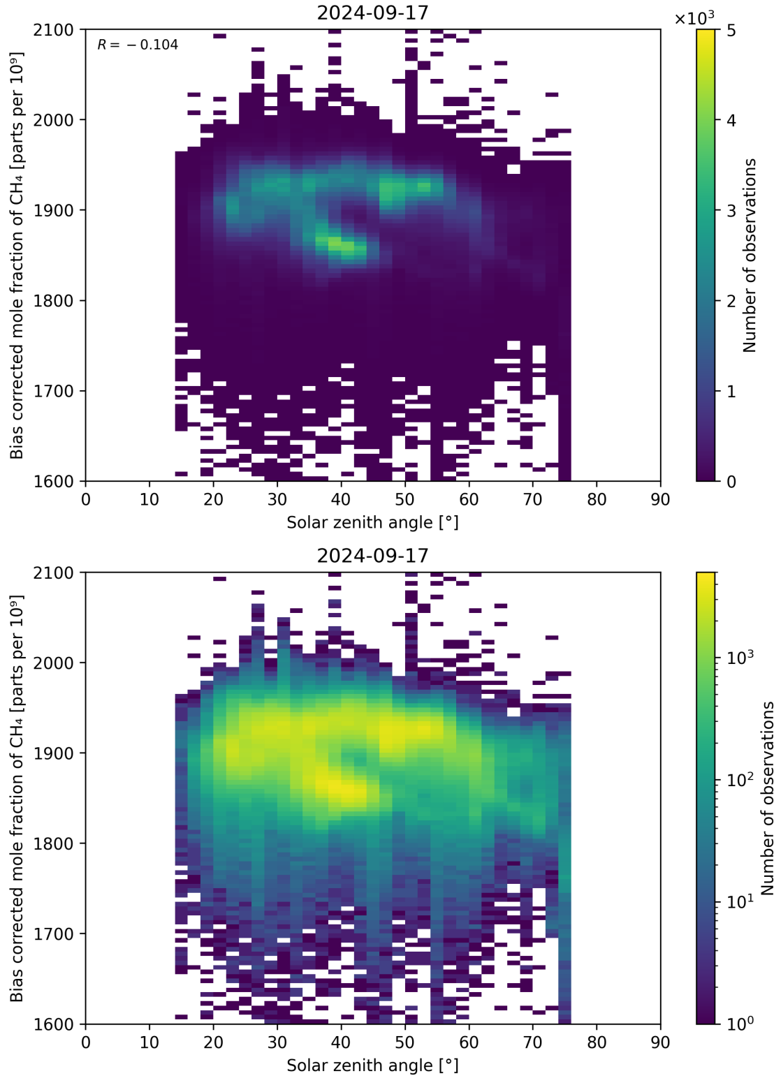
Figure 100: Scatter density plot of “Solar zenith angle” against “Bias corrected mole fraction of \text{CH}_4 ” for 2024-09-17 to 2024-09-18.
