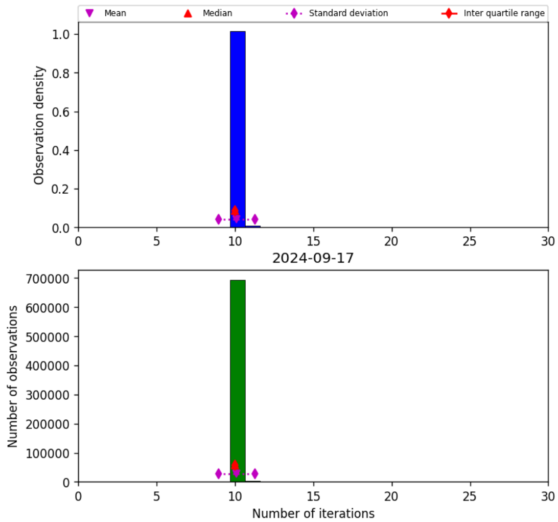
Figure 31: Histogram of “Number of iterations” for 2024-09-17 to 2024-09-18
