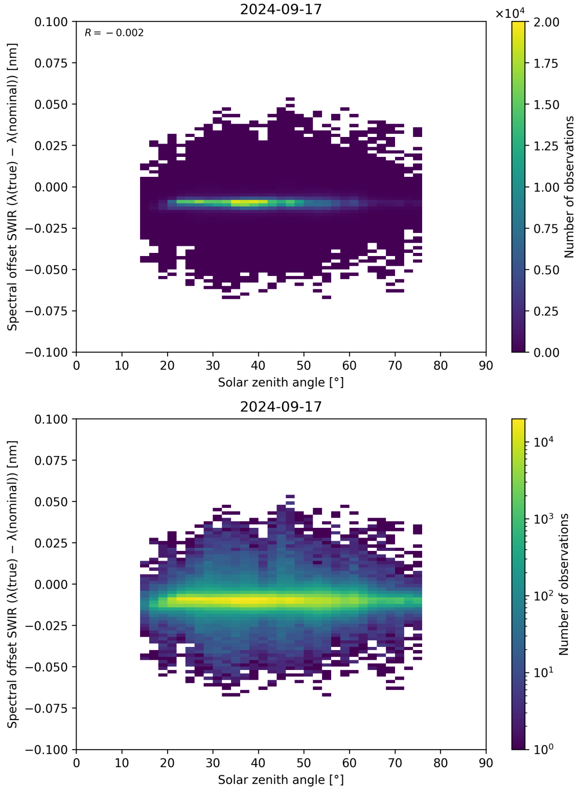
Figure 104: Scatter density plot of “Solar zenith angle” against “Spectral offset SWIR ( \lambda_{\text{true}} - \lambda_{\text{nominal}} )” for 2024-09-17 to 2024-09-18.
