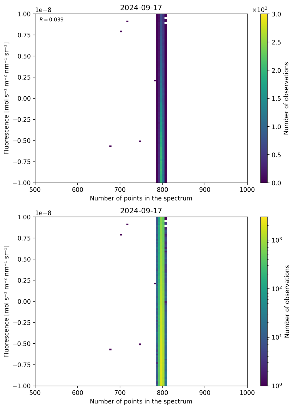
Figure 91: Scatter density plot of “Number of points in the spectrum” against “Fluorescence” for 2024-09-17 to 2024-09-18.
