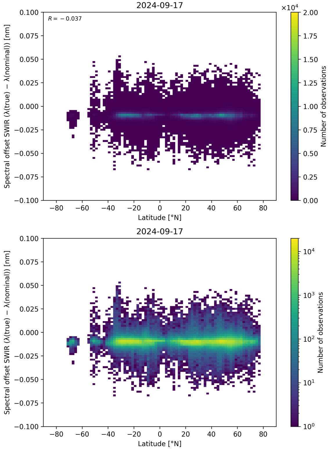
Figure 62: Scatter density plot of “Latitude” against “Spectral offset SWIR ( \lambda_{\text{true}} - \lambda_{\text{nominal}} )” for 2024-09-17 to 2024-09-18.
