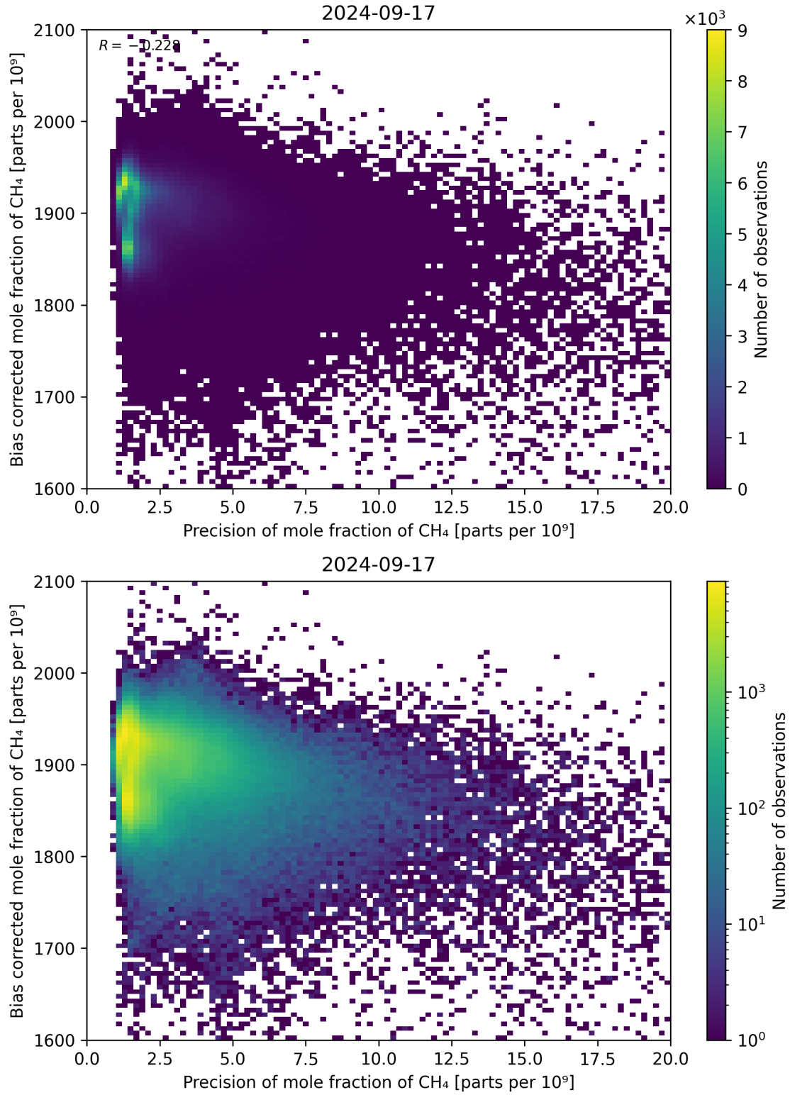
Figure 82: Scatter density plot of “Precision of mole fraction of CH 4 ” against “Bias corrected mole fraction of CH 4 ” for 2024-09-17 to 2024-09-18.
