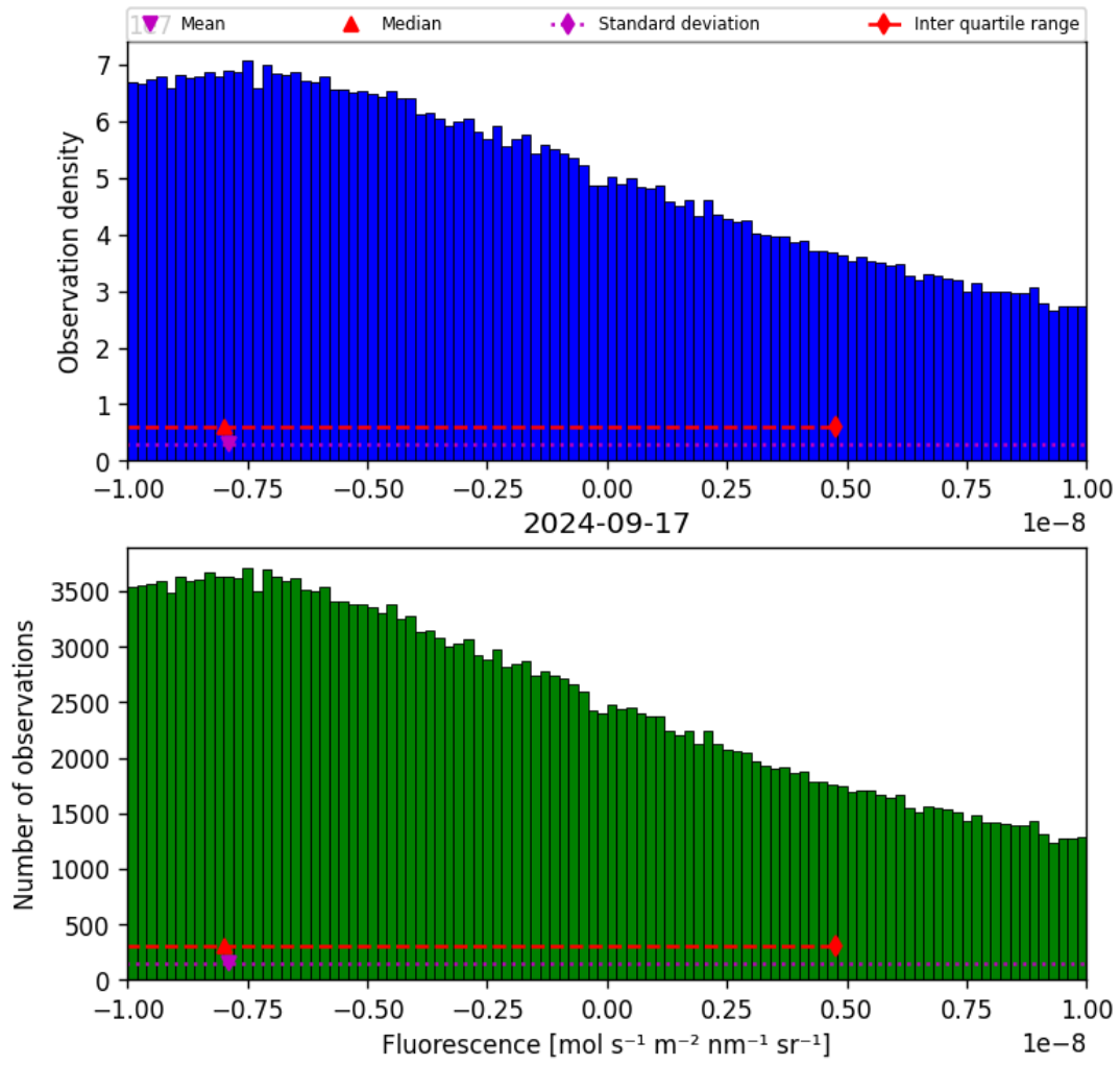
Figure 32: Histogram of “Fluorescence” for 2024-09-17 to 2024-09-18
