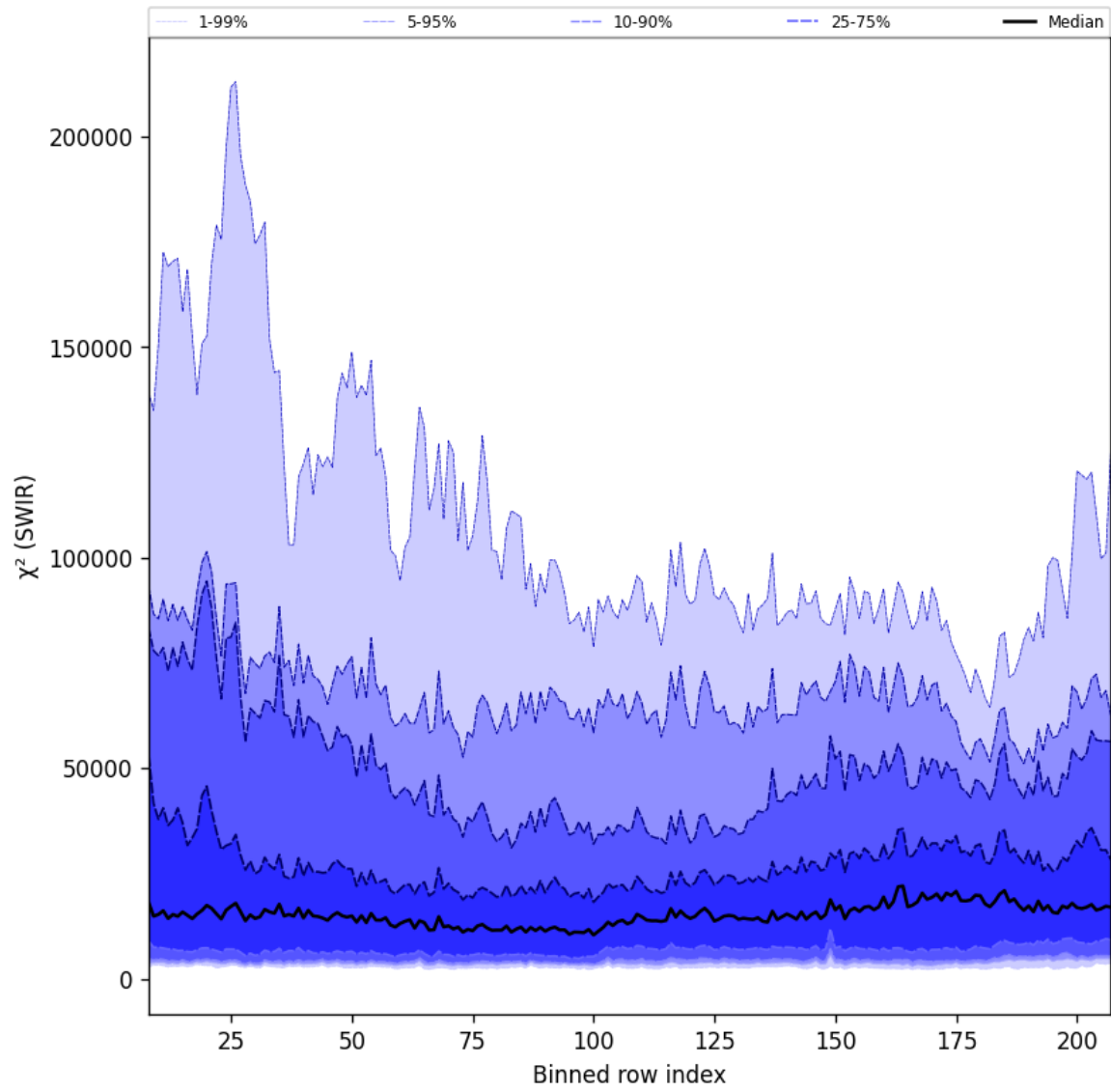
Figure 39: Along track statistics of “ \chi^2 (SWIR)” for 2024-09-17 to 2024-09-18
