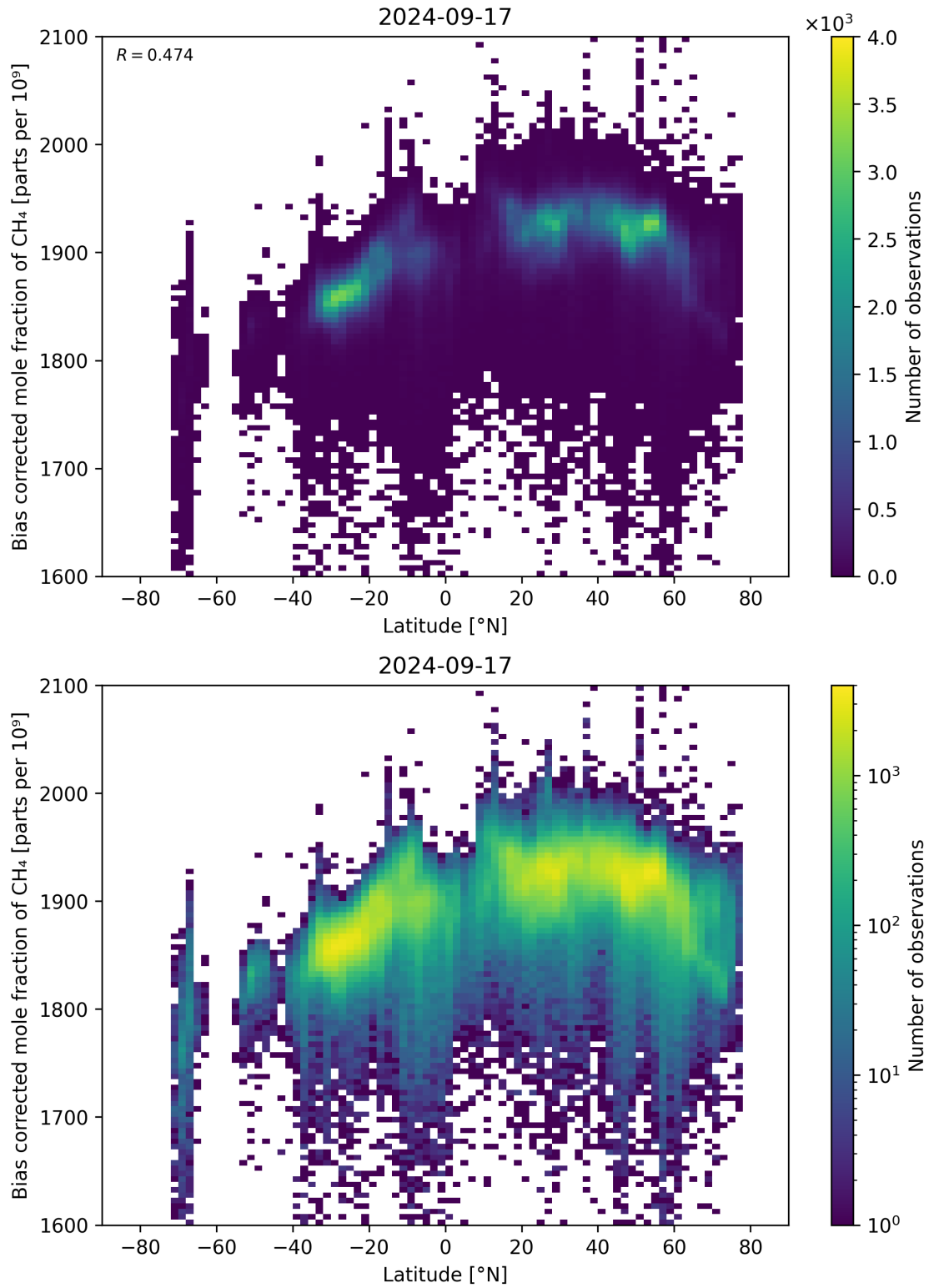
Figure 58: Scatter density plot of “Latitude” against “Bias corrected mole fraction of CH 4 ” for 2024-09-17 to 2024-09-18.
