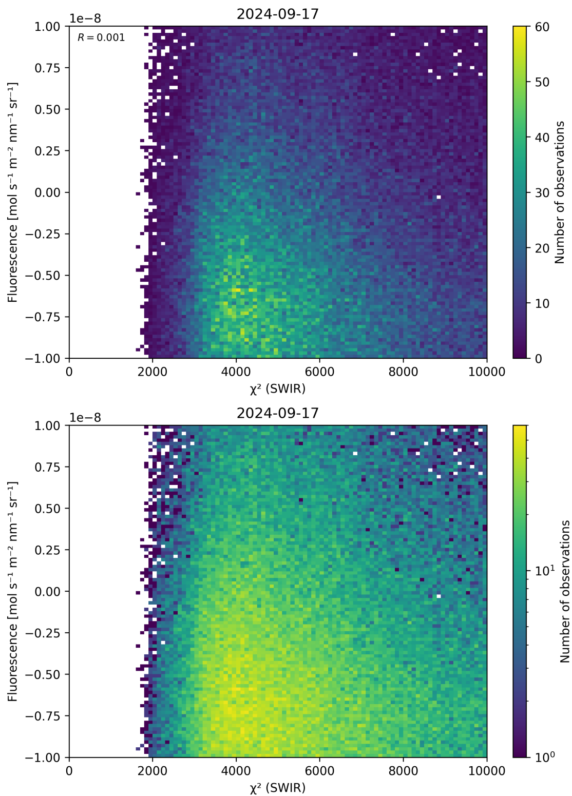
Figure 49: Scatter density plot of “ \chi^2 (SWIR)” against “Fluorescence” for 2024-09-17 to 2024-09-18.
