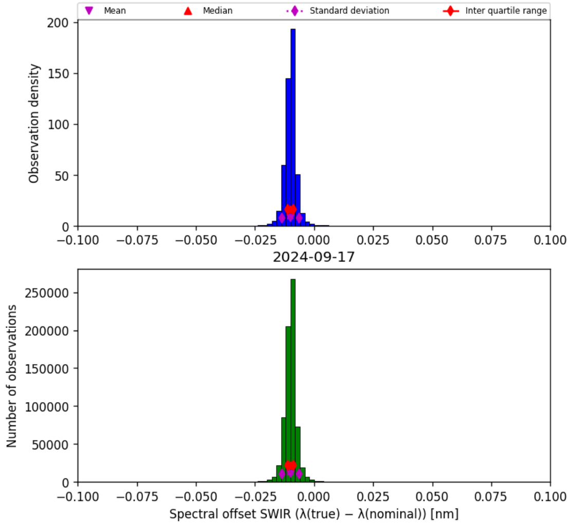
Figure 27: Histogram of “Spectral offset SWIR ( \lambda_{\text{true}} - \lambda_{\text{nominal}} )” for 2024-09-17 to 2024-09-18
