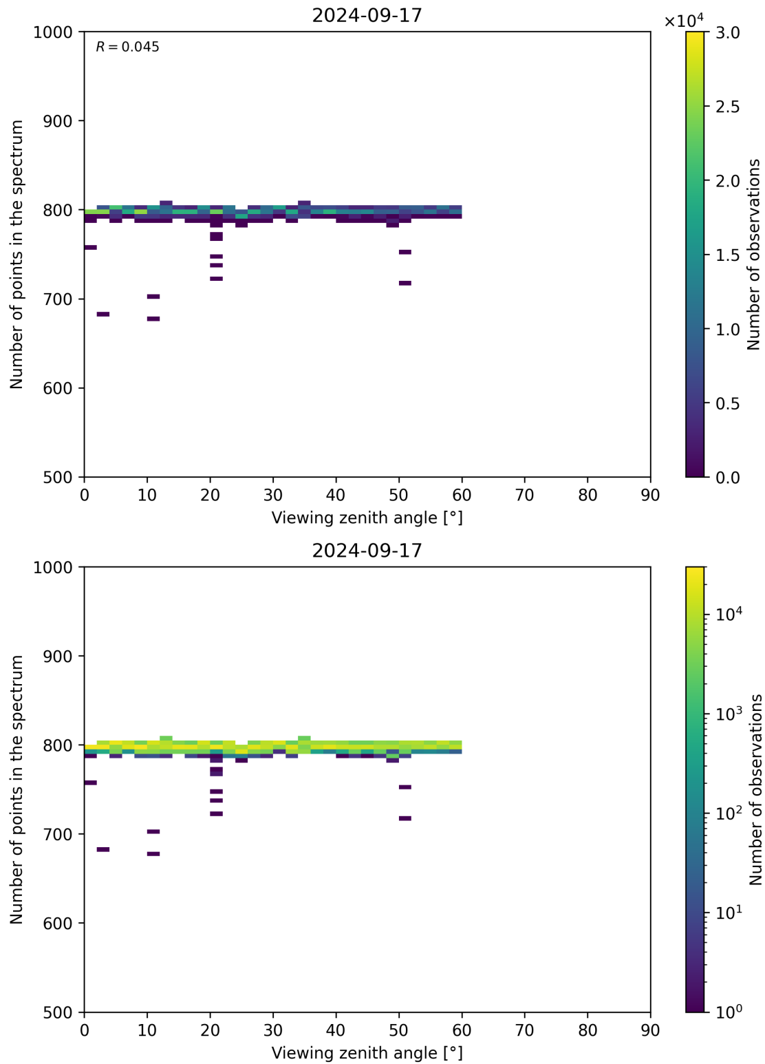
Figure 114: Scatter density plot of “Viewing zenith angle” against “Number of points in the spectrum” for 2024-09-17 to 2024-09-18.
