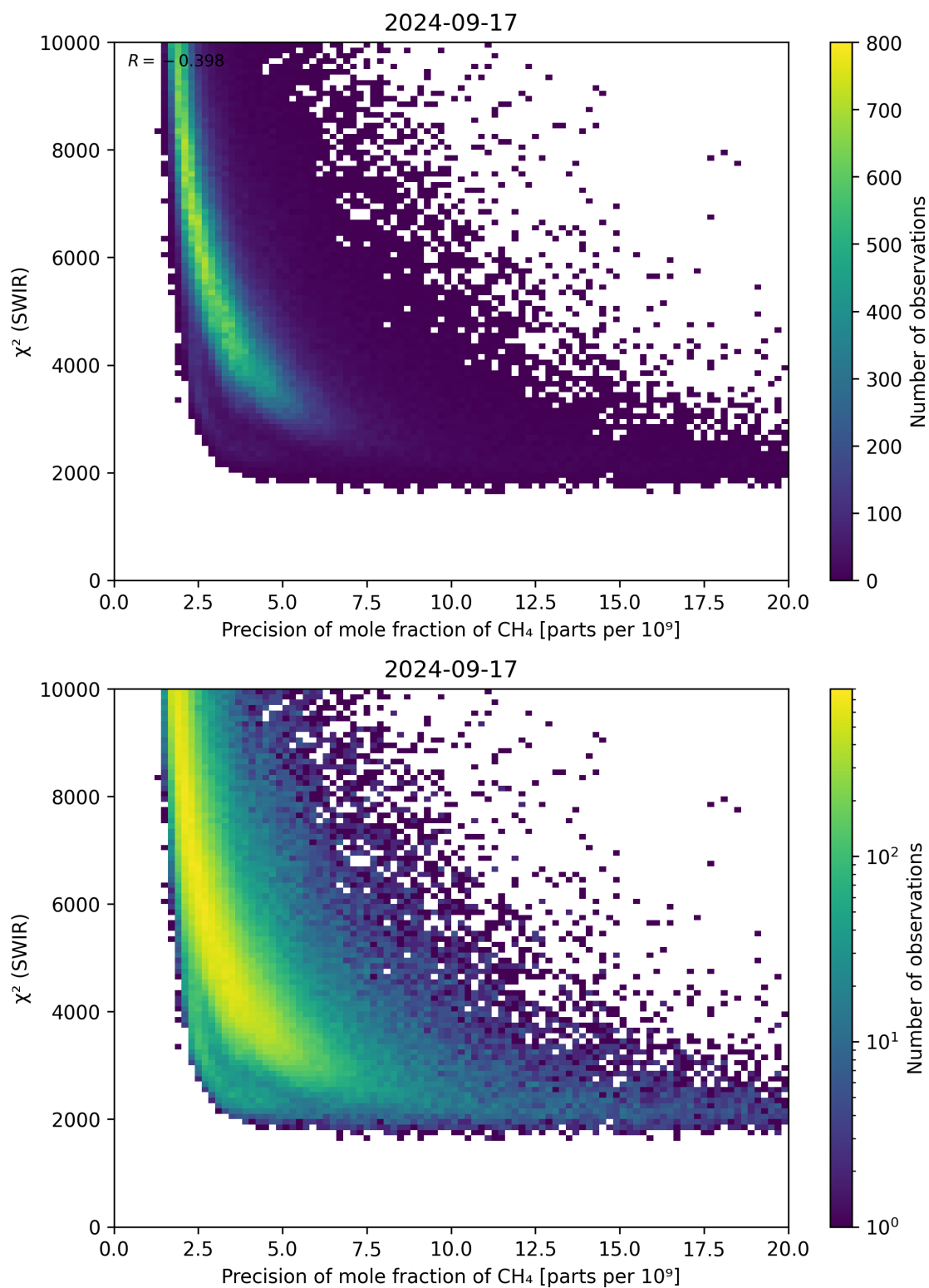
Figure 79: Scatter density plot of “Precision of mole fraction of \text{CH}_4 ” against “ \chi^2 (SWIR)” for 2024-09-17 to 2024-09-18.
