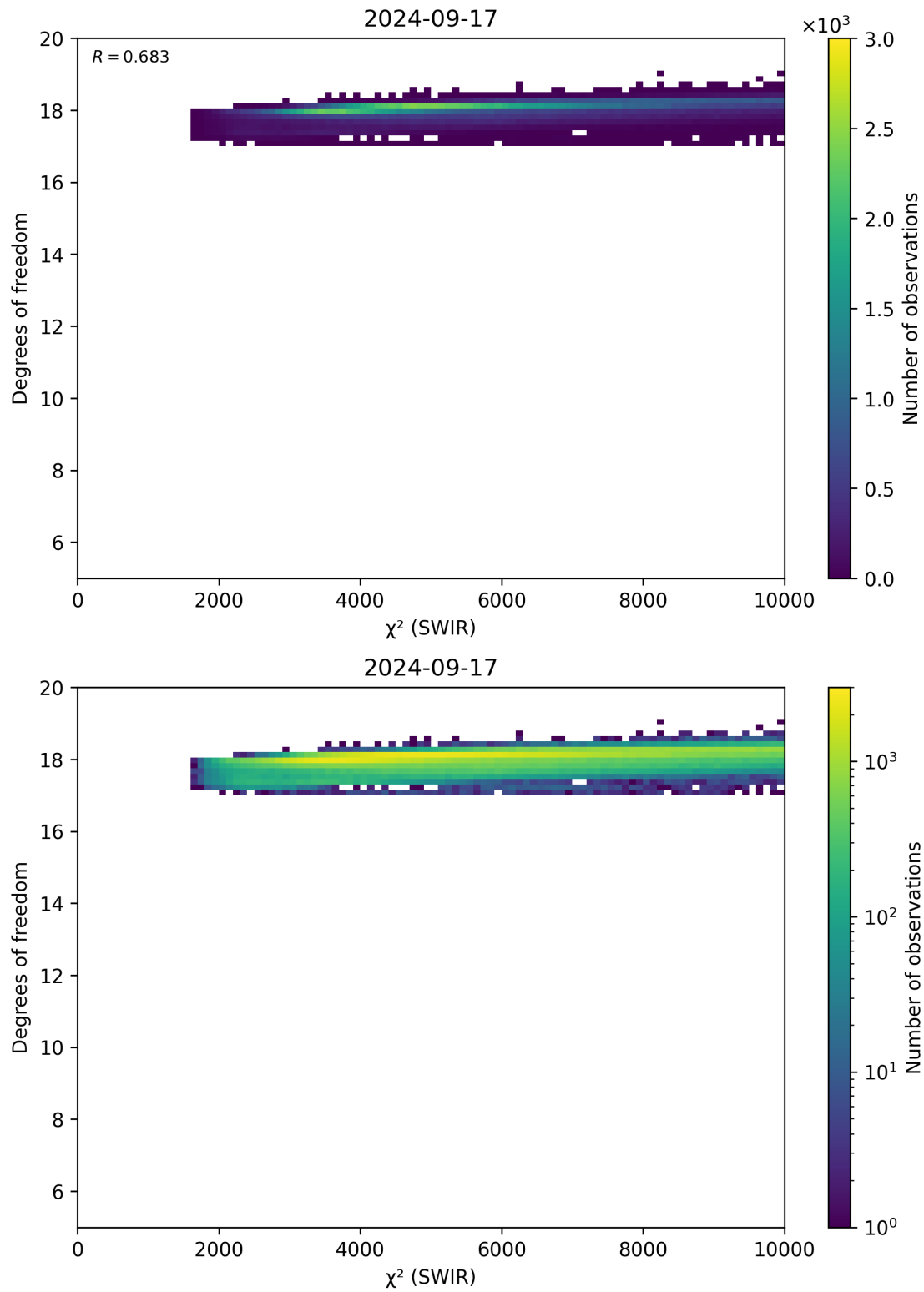
Figure 48: Scatter density plot of " \chi^2 (SWIR)" against "Degrees of freedom" for 2024-09-17 to 2024-09-18.
