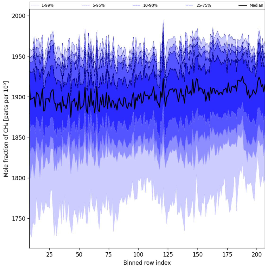
Figure 34: Along track statistics of “Mole fraction of CH 4 ” for 2024-09-17 to 2024-09-18
