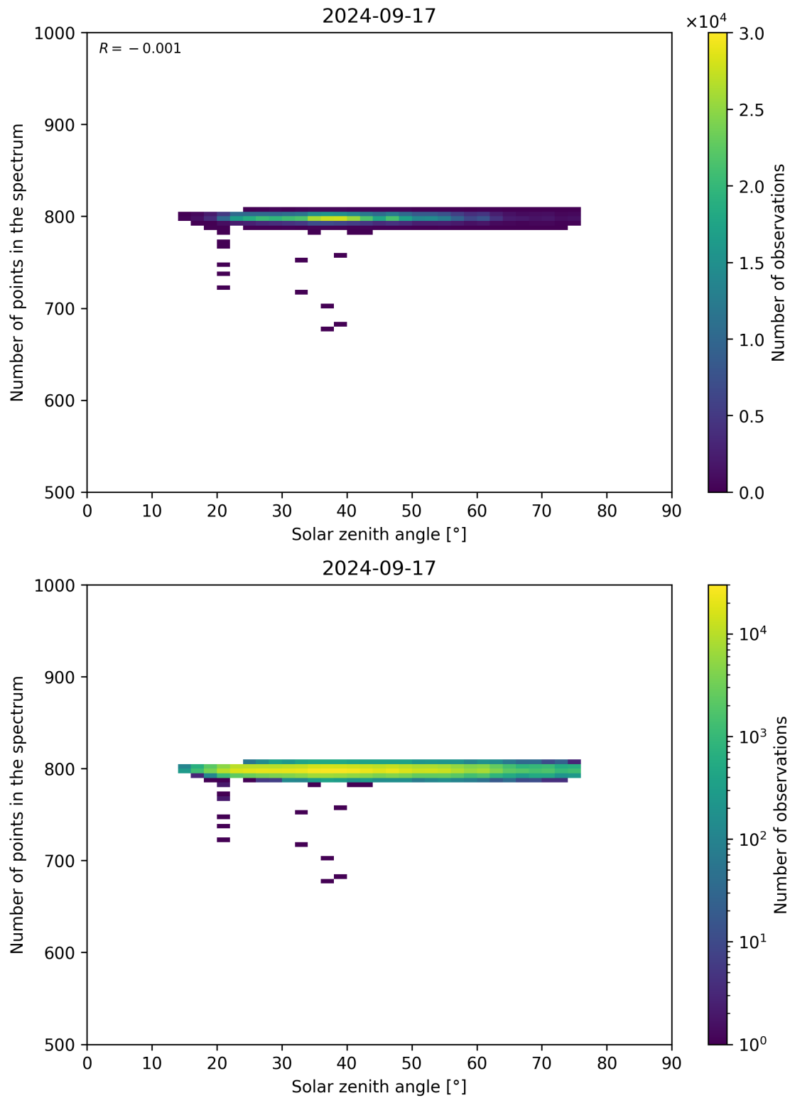
Figure 103: Scatter density plot of “Solar zenith angle” against “Number of points in the spectrum” for 2024-09-17 to 2024-09-18.
