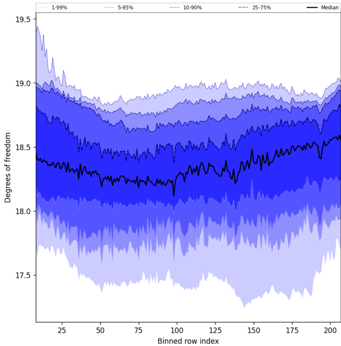
Figure 41: Along track statistics of “Degrees of freedom” for 2024-09-17 to 2024-09-18
