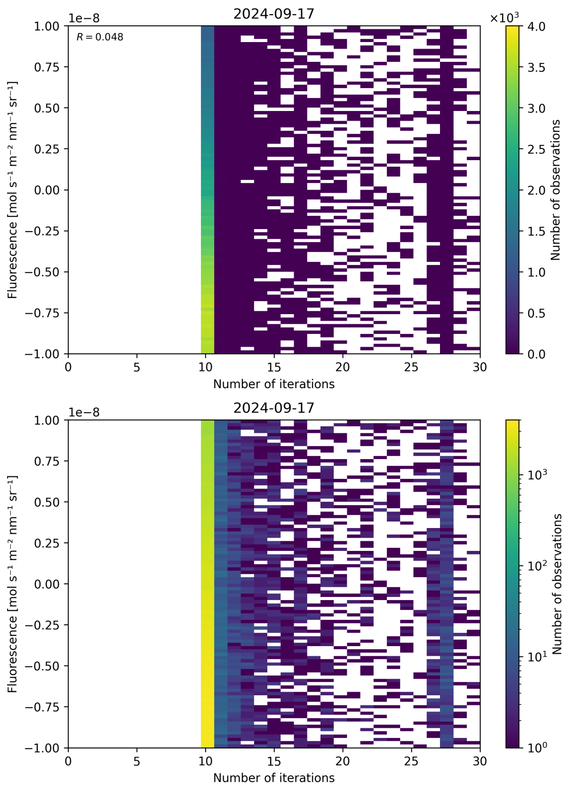
Figure 87: Scatter density plot of “Number of iterations” against “Fluorescence” for 2024-09-17 to 2024-09-18.
