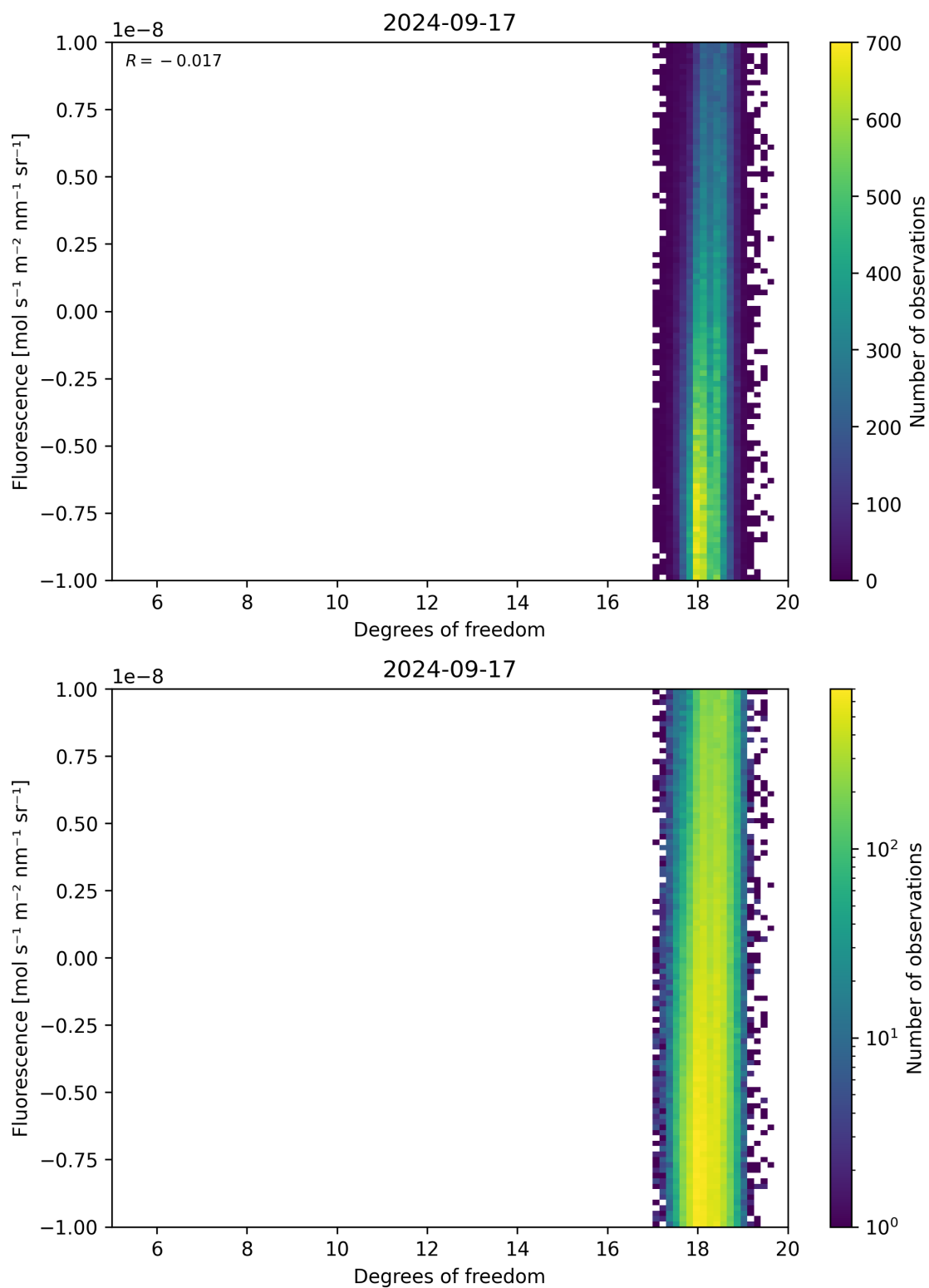
Figure 51: Scatter density plot of “Degrees of freedom” against “Fluorescence” for 2024-09-17 to 2024-09-18.
