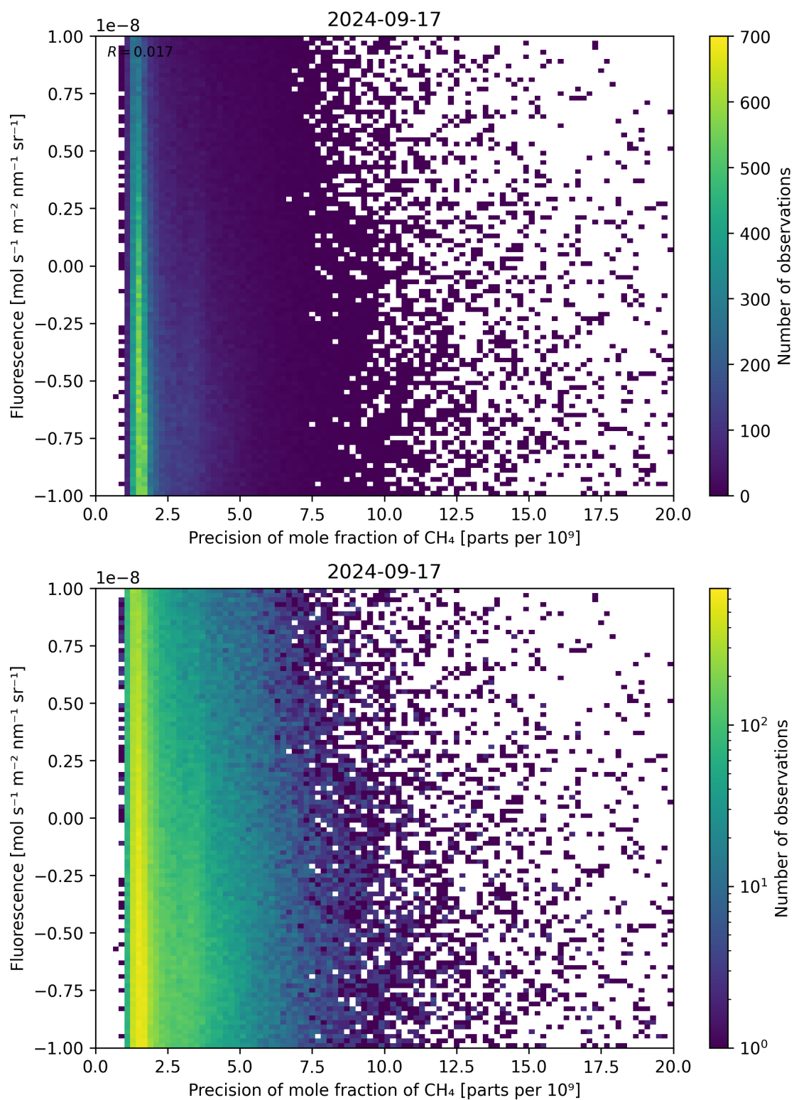
Figure 81: Scatter density plot of “Precision of mole fraction of \text{CH}_4 ” against “Fluorescence” for 2024-09-17 to 2024-09-18.
