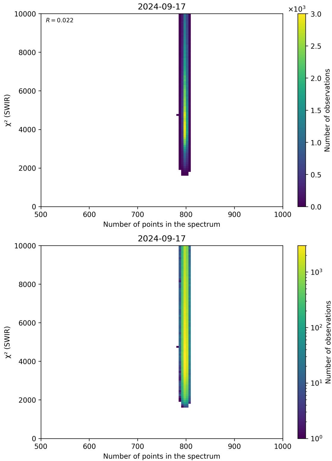
Figure 89: Scatter density plot of “Number of points in the spectrum” against “ \chi^2 (SWIR)” for 2024-09-17 to 2024-09-18.
