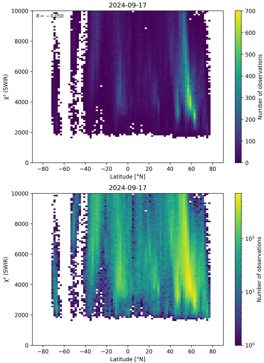
Figure 54: Scatter density plot of “Latitude” against “ \chi^2 (SWIR)” for 2024-09-17 to 2024-09-18.
