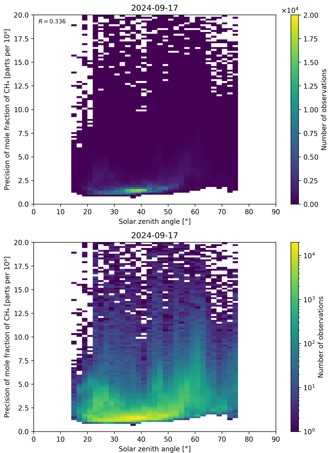
Figure 101: Scatter density plot of “Solar zenith angle” against “Precision of mole fraction of CH 4 ” for 2024-09-17 to 2024-09-18.
