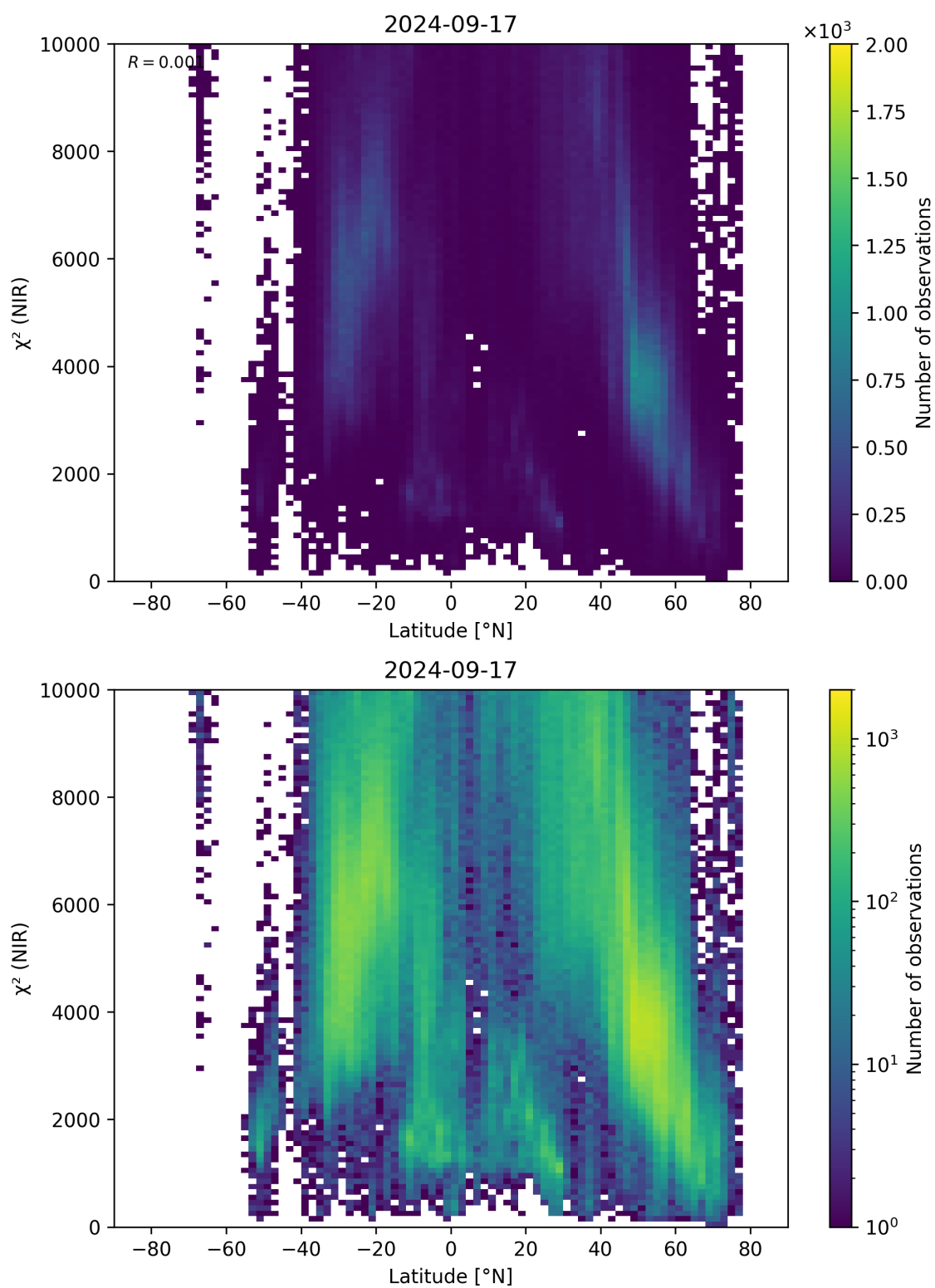
Figure 53: Scatter density plot of “Latitude” against “ \chi^2 (NIR)” for 2024-09-17 to 2024-09-18.
