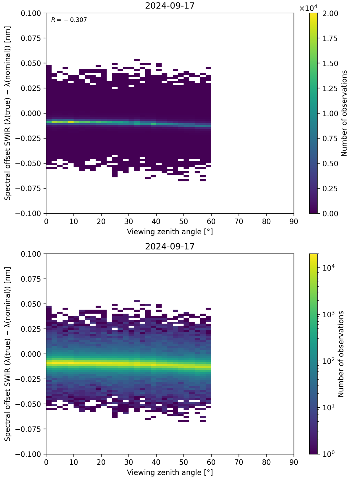
Figure 116: Scatter density plot of “Viewing zenith angle” against “Spectral offset SWIR ( \lambda_{\text{true}} - \lambda_{\text{nominal}} )” for 2024-09-17 to 2024-09-18.
