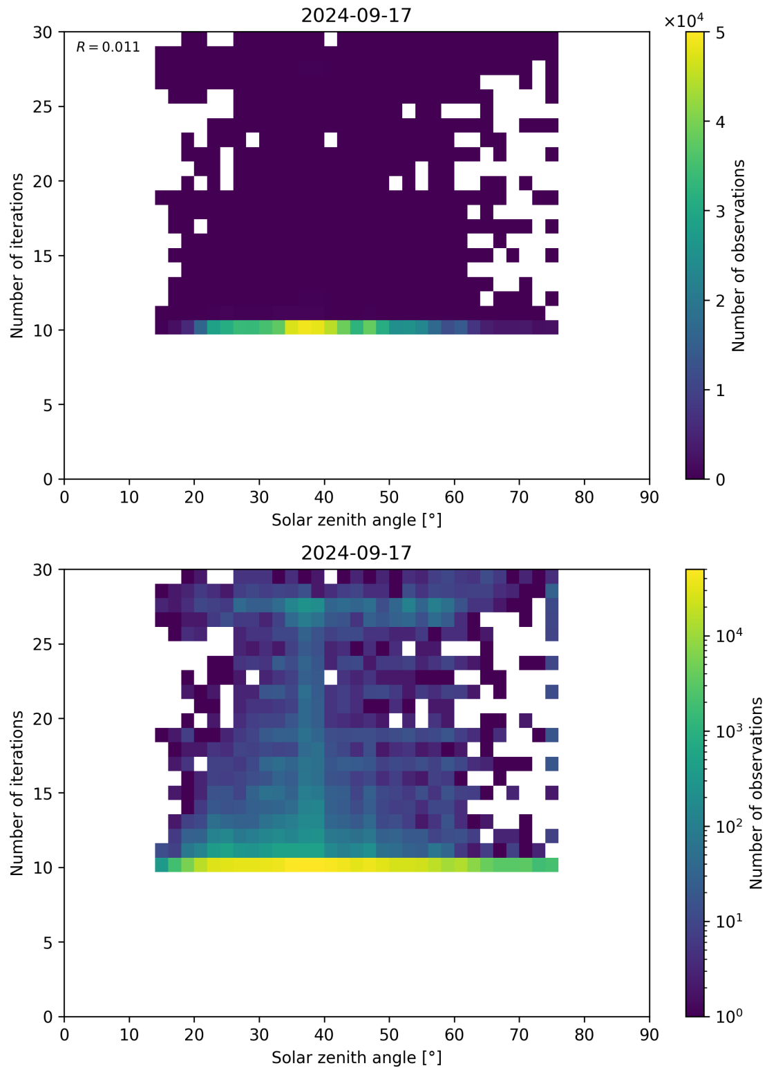
Figure 102: Scatter density plot of “Solar zenith angle” against “Number of iterations” for 2024-09-17 to 2024-09-18.
