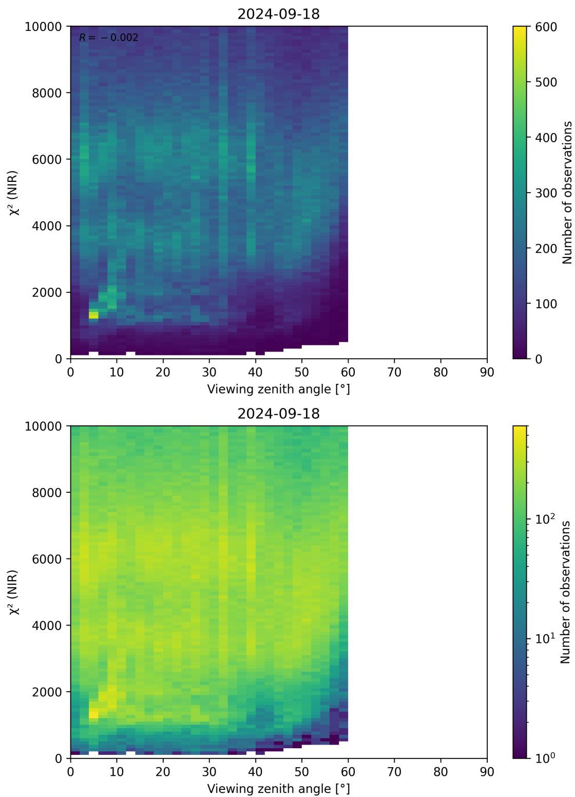
Figure 105: Scatter density plot of “Viewing zenith angle” against “ \chi^2 (NIR)” for 2024-09-17 to 2024-09-19.
