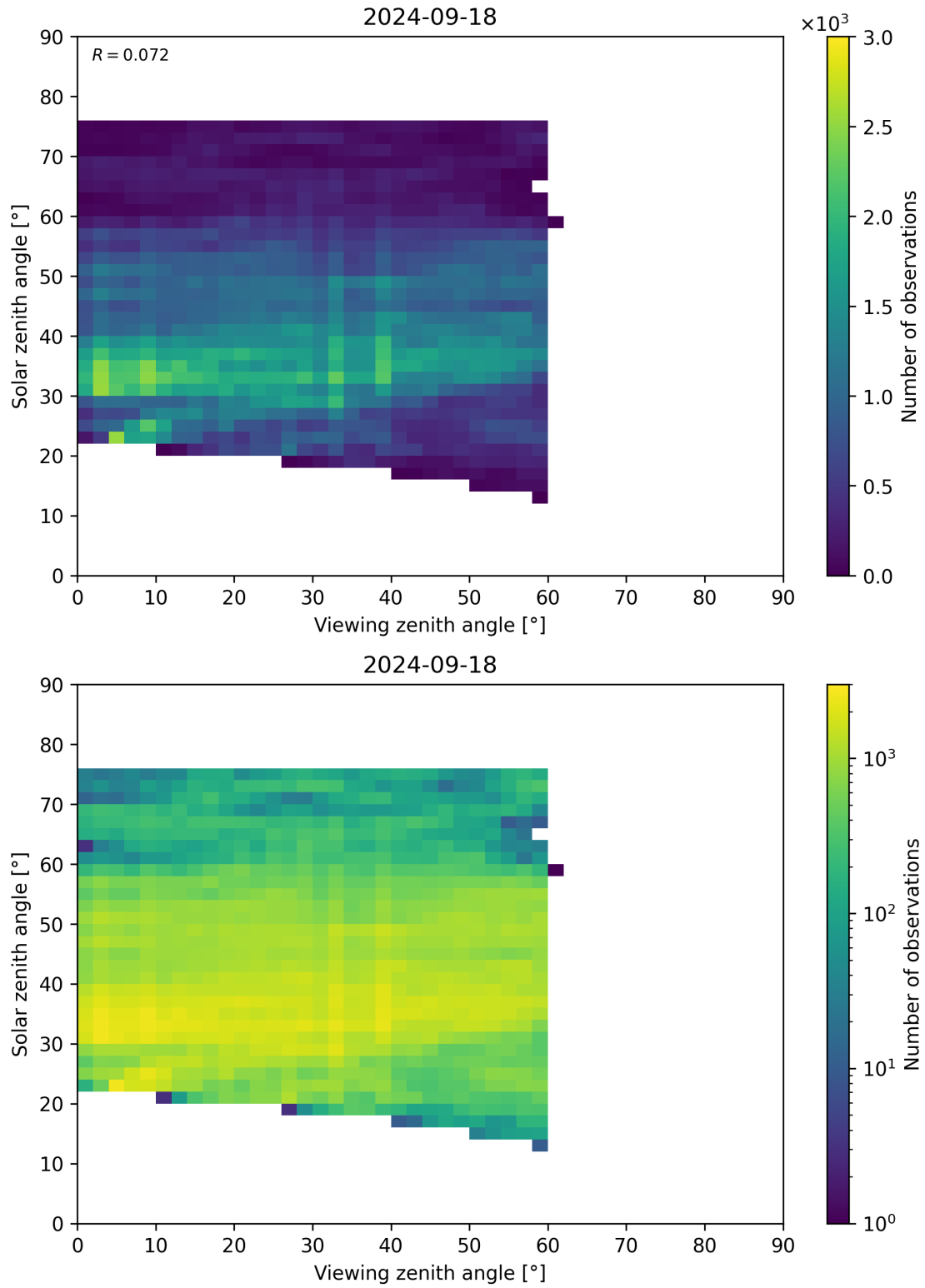
Figure 115: Scatter density plot of “Viewing zenith angle” against “Solar zenith angle” for 2024-09-17 to 2024-09-19.
