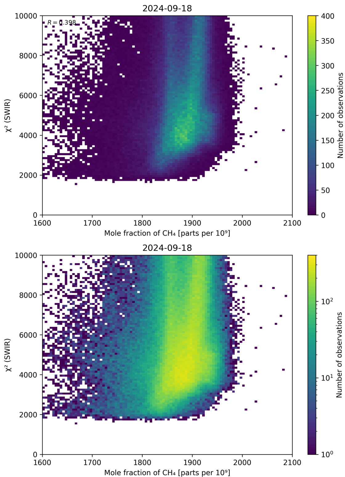
Figure 71: Scatter density plot of “Mole fraction of \text{CH}_4 ” against “ \chi^2 (SWIR)” for 2024-09-17 to 2024-09-19.
