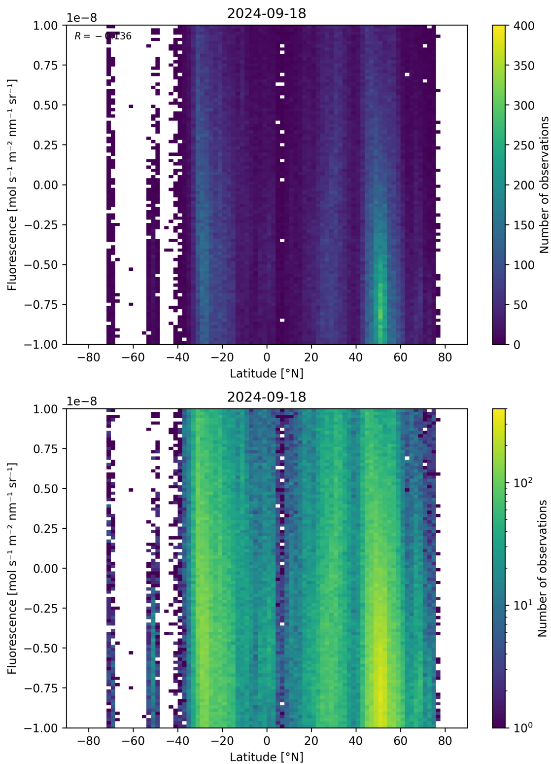
Figure 56: Scatter density plot of “Latitude” against “Fluorescence” for 2024-09-17 to 2024-09-19.
