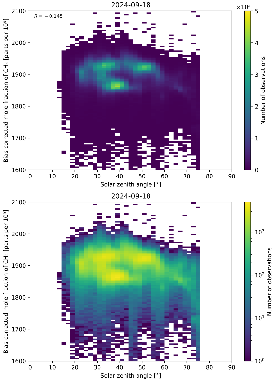
Figure 100: Scatter density plot of “Solar zenith angle” against “Bias corrected mole fraction of CH 4 ” for 2024-09-17 to 2024-09-19.
