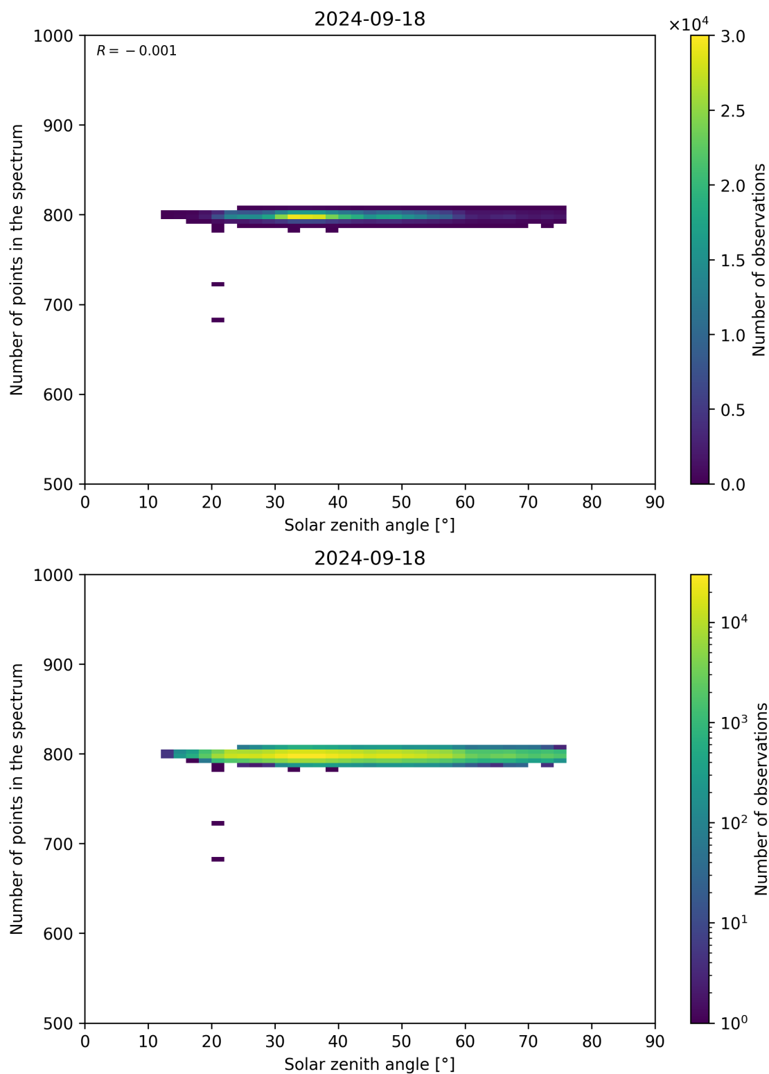
Figure 103: Scatter density plot of “Solar zenith angle” against “Number of points in the spectrum” for 2024-09-17 to 2024-09-19.
