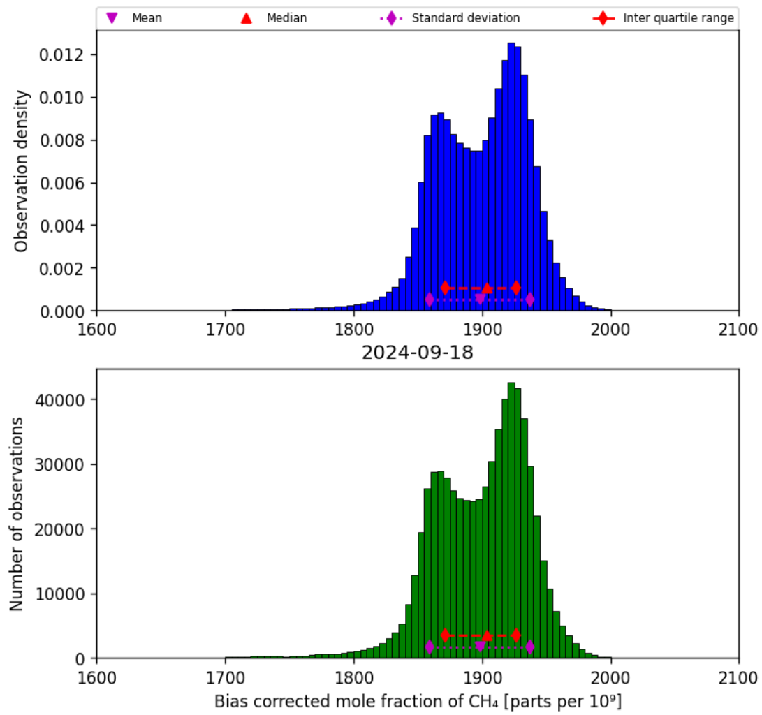
Figure 25: Histogram of “Bias corrected mole fraction of CH 4 ” for 2024-09-17 to 2024-09-19
