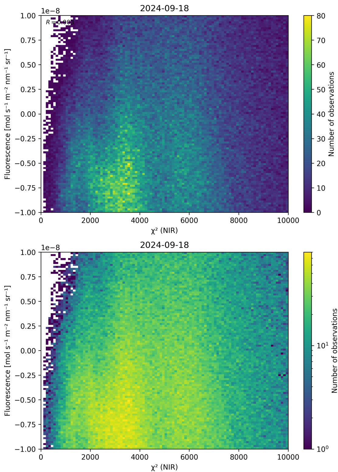
Figure 45: Scatter density plot of “ \chi^2 (NIR)” against “Fluorescence” for 2024-09-17 to 2024-09-19.
