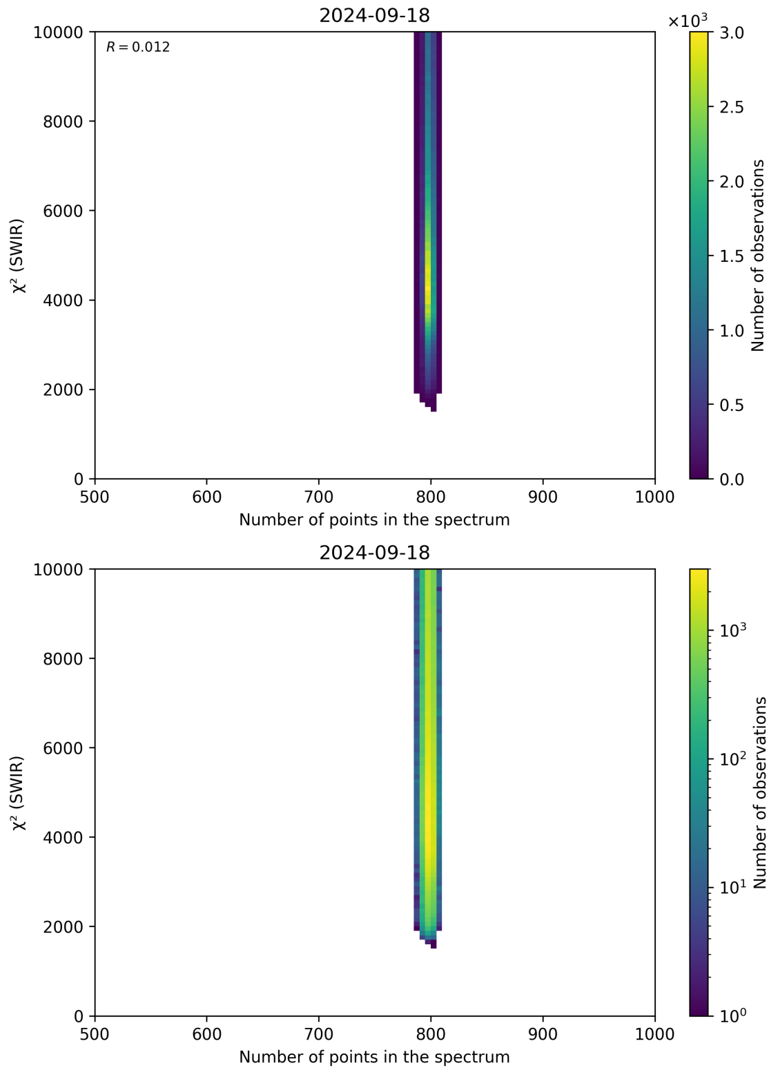
Figure 89: Scatter density plot of “Number of points in the spectrum” against “ \chi^2 (SWIR)” for 2024-09-17 to 2024-09-19.
