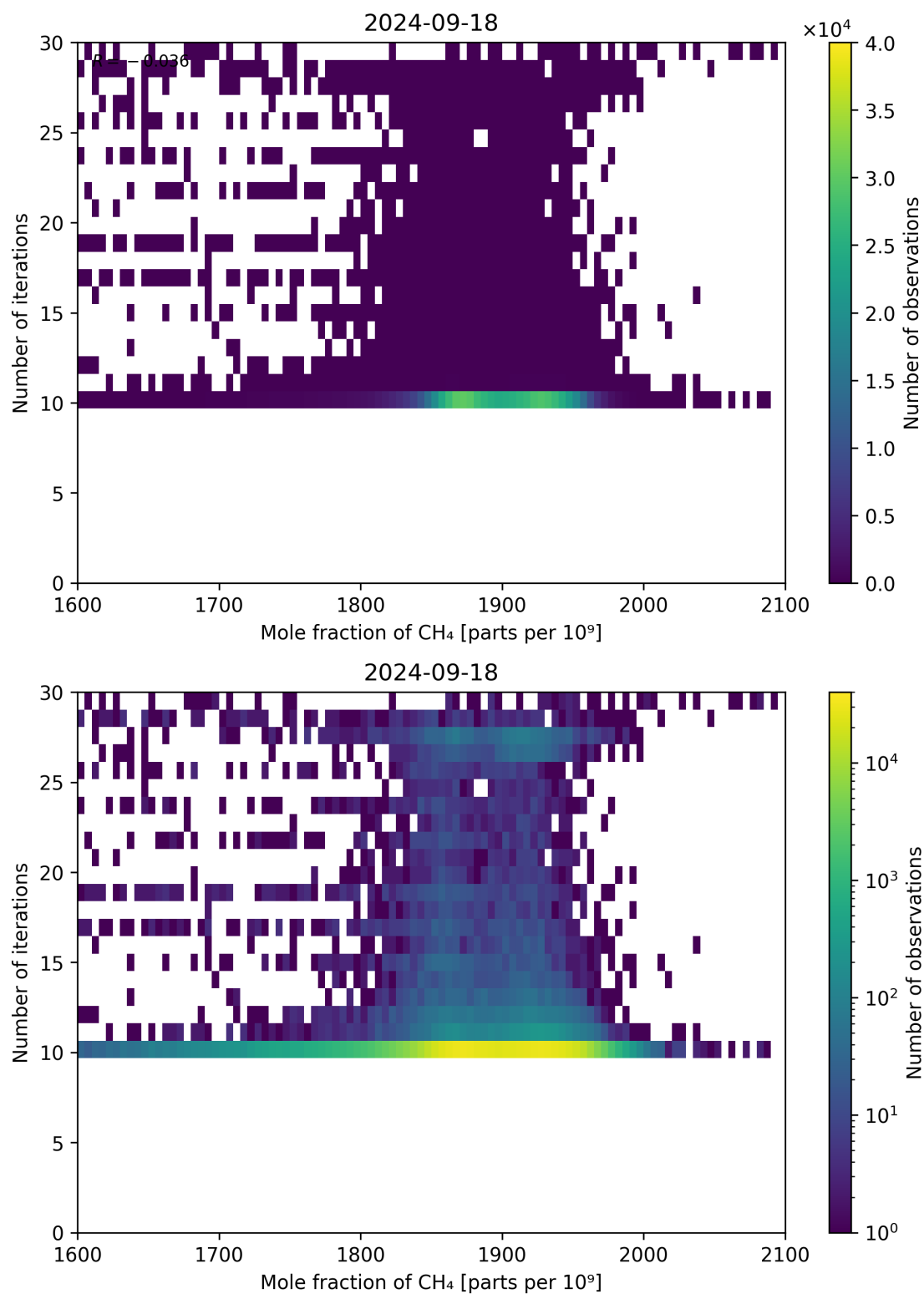
Figure 76: Scatter density plot of “Mole fraction of CH 4 ” against “Number of iterations” for 2024-09-17 to 2024-09-19.
