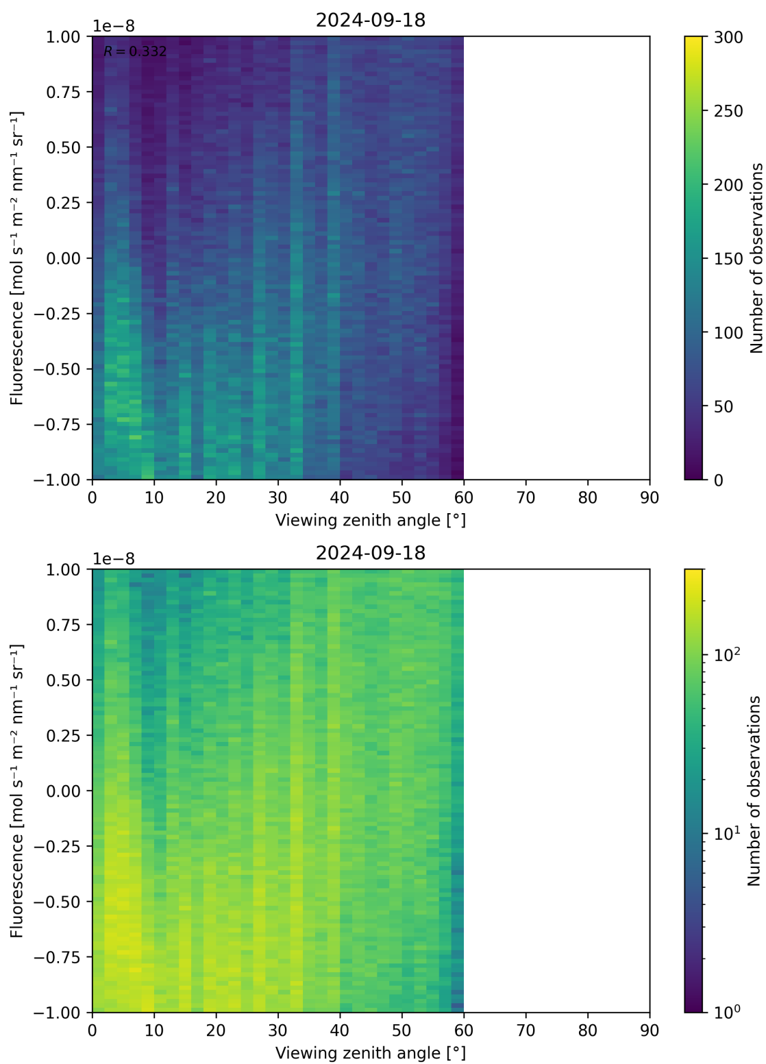
Figure 108: Scatter density plot of “Viewing zenith angle” against “Fluorescence” for 2024-09-17 to 2024-09-19.
