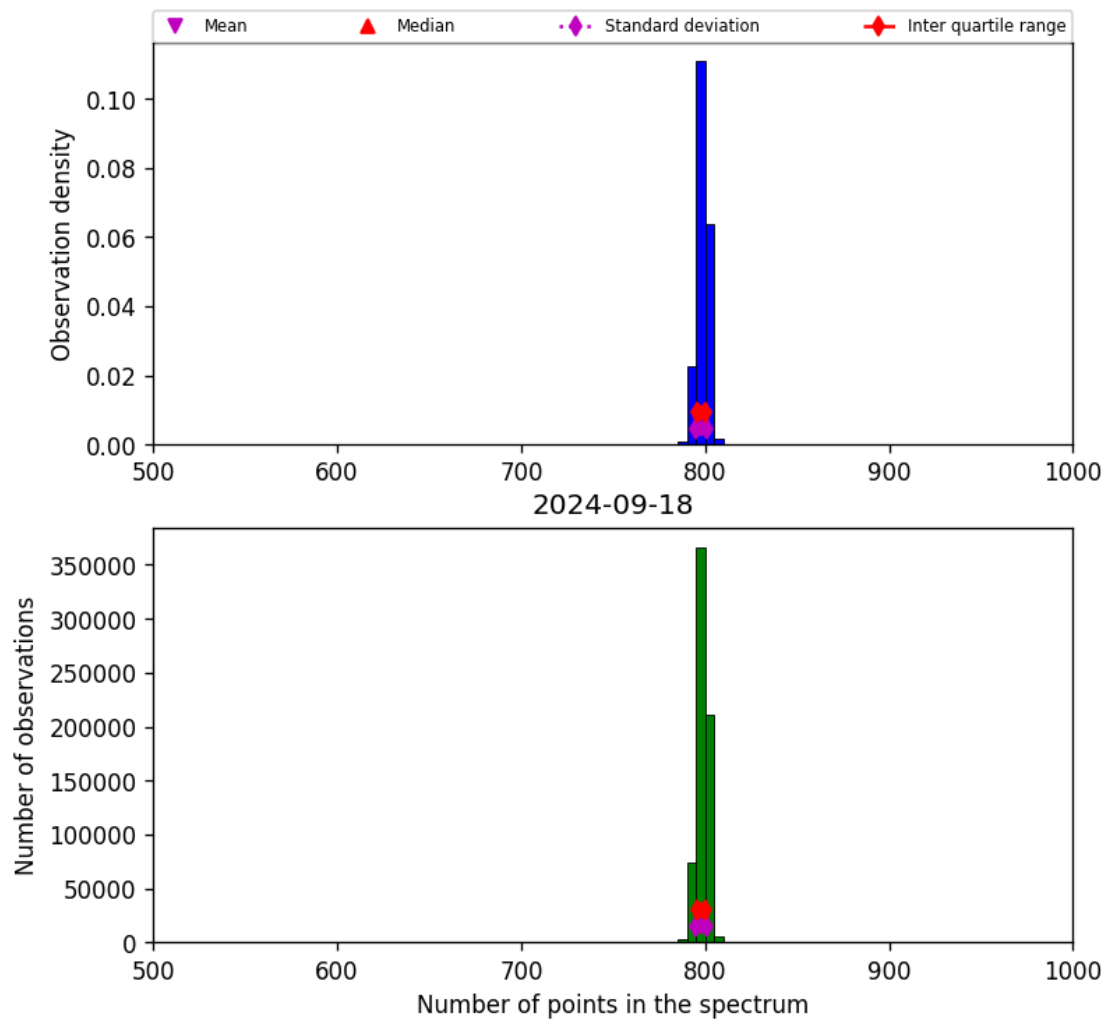
Figure 26: Histogram of “Number of points in the spectrum” for 2024-09-17 to 2024-09-19
