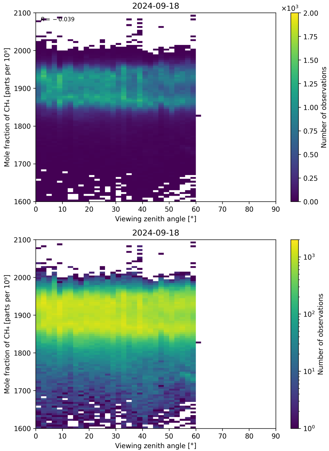
Figure 110: Scatter density plot of “Viewing zenith angle” against “Mole fraction of CH 4 ” for 2024-09-17 to 2024-09-19.
