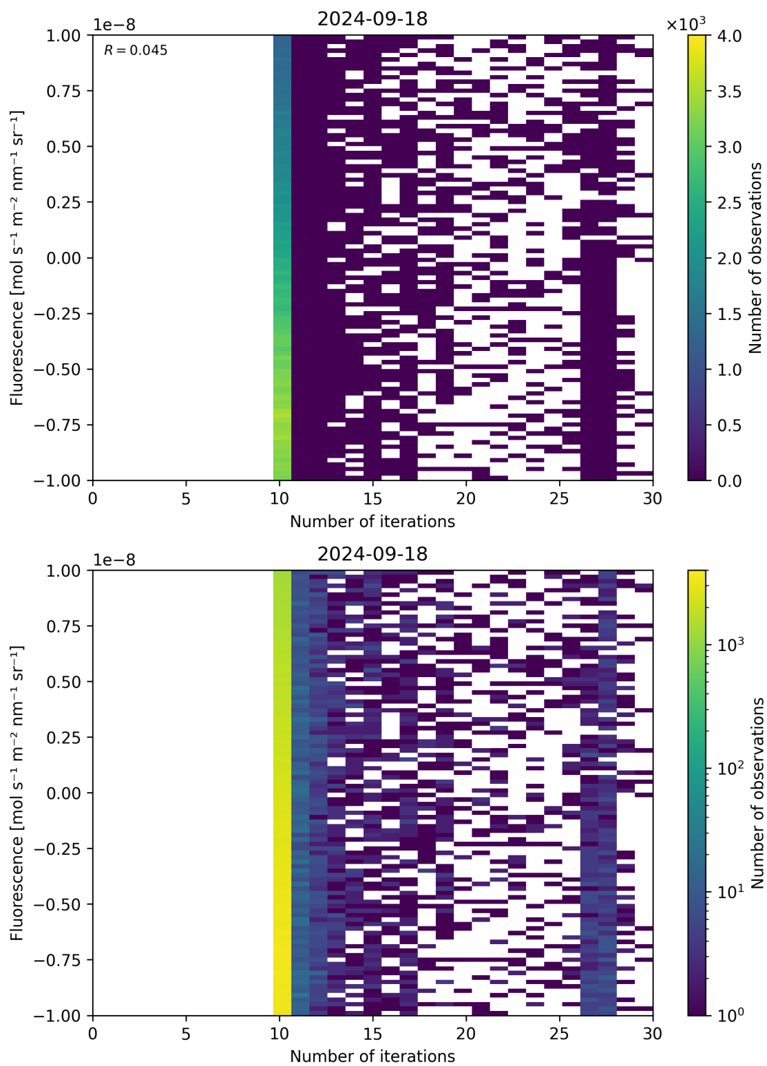
Figure 87: Scatter density plot of “Number of iterations” against “Fluorescence” for 2024-09-17 to 2024-09-19.
