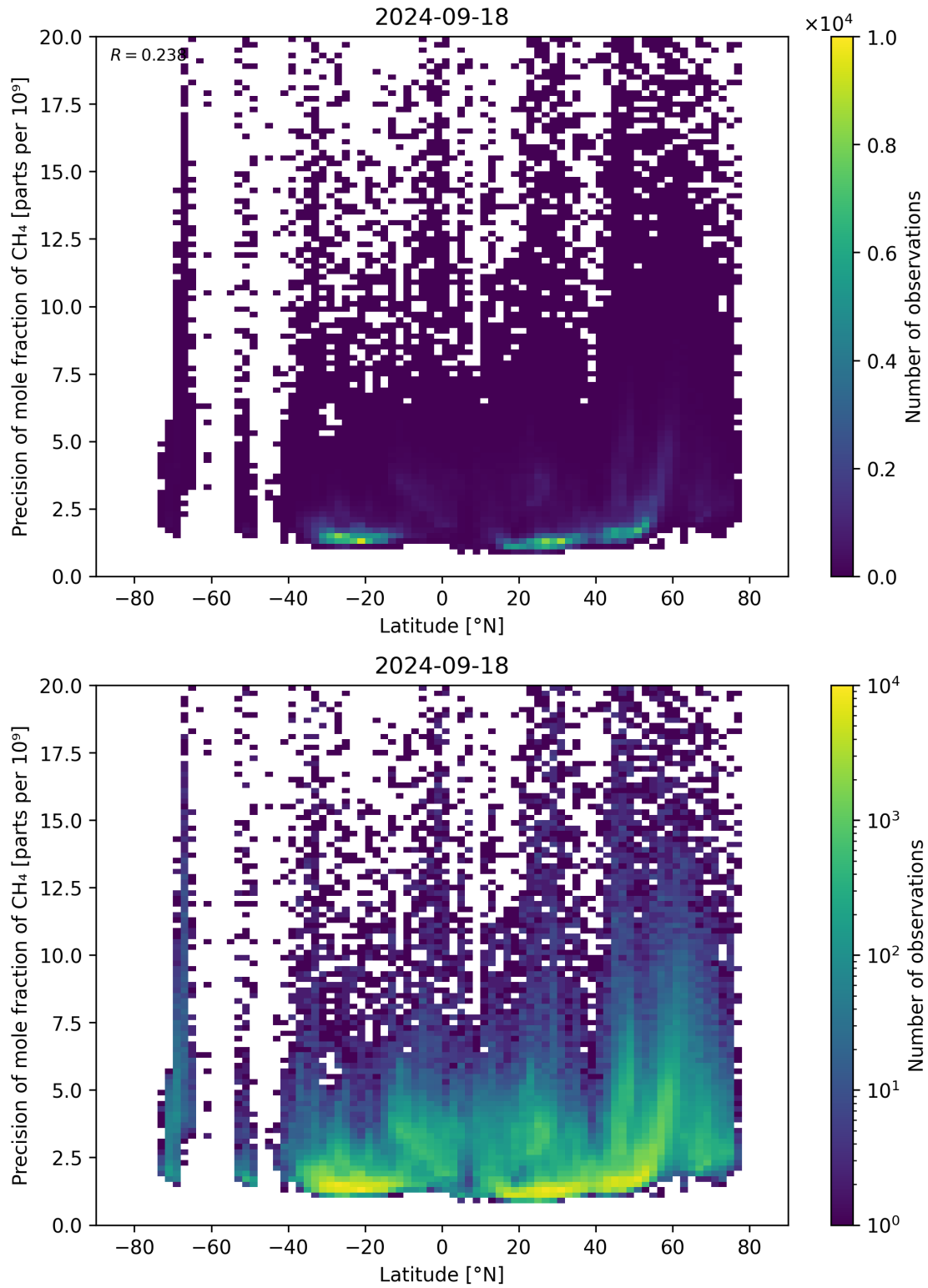
Figure 59: Scatter density plot of “Latitude” against “Precision of mole fraction of \text{CH}_4 ” for 2024-09-17 to 2024-09-19.
