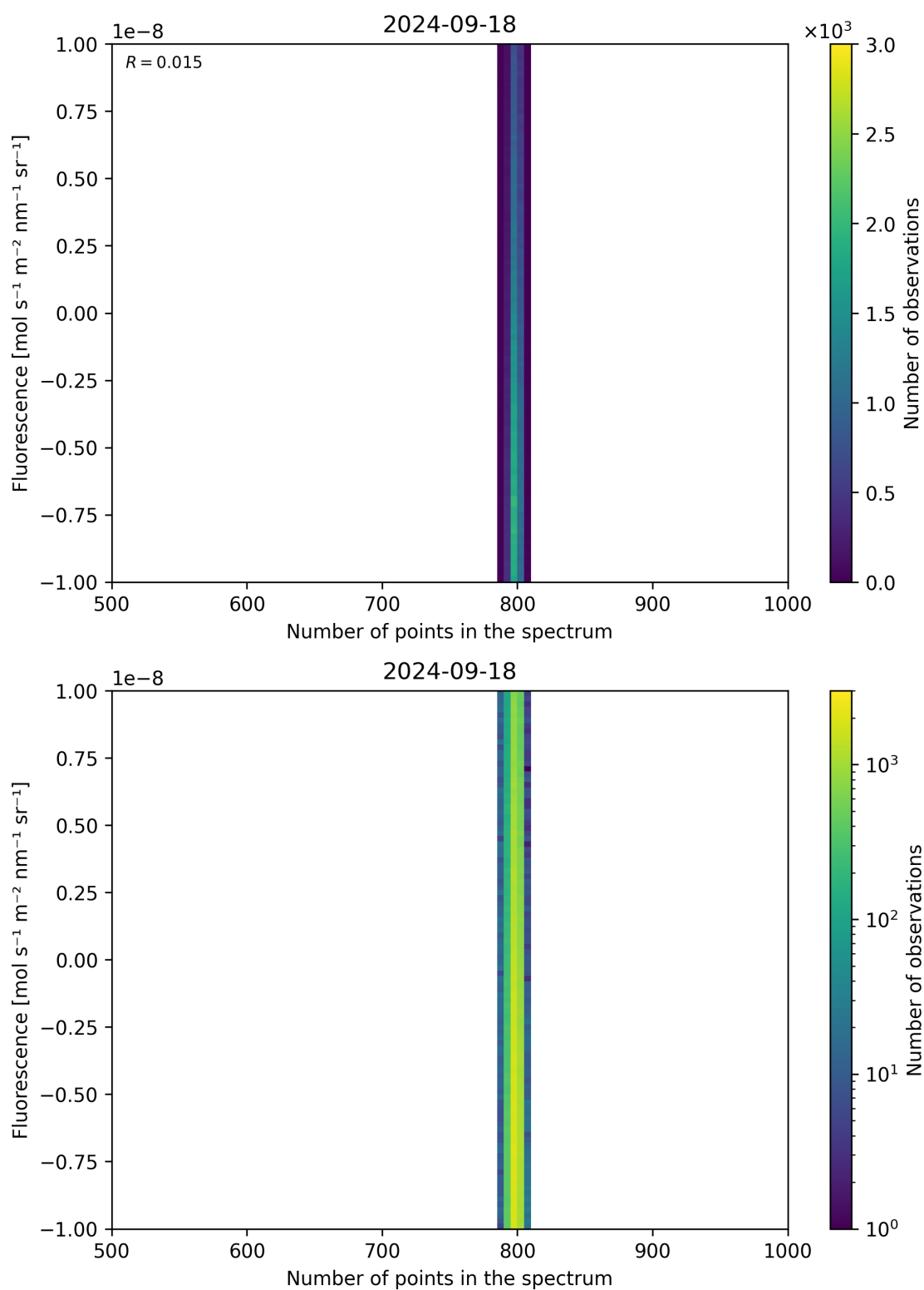
Figure 91: Scatter density plot of “Number of points in the spectrum” against “Fluorescence” for 2024-09-17 to 2024-09-19.
