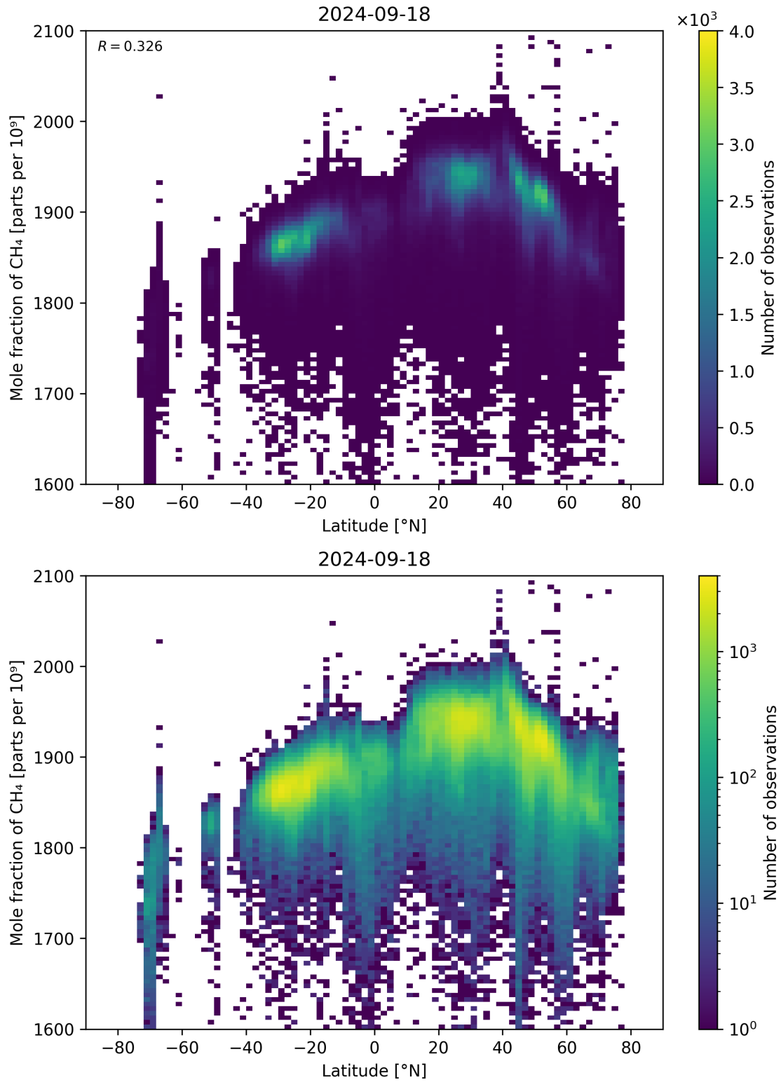
Figure 57: Scatter density plot of “Latitude” against “Mole fraction of \text{CH}_4 ” for 2024-09-17 to 2024-09-19.
