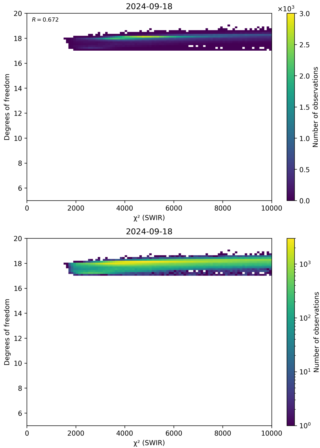
Figure 48: Scatter density plot of “ \chi^2 (SWIR)” against “Degrees of freedom” for 2024-09-17 to 2024-09-19.
