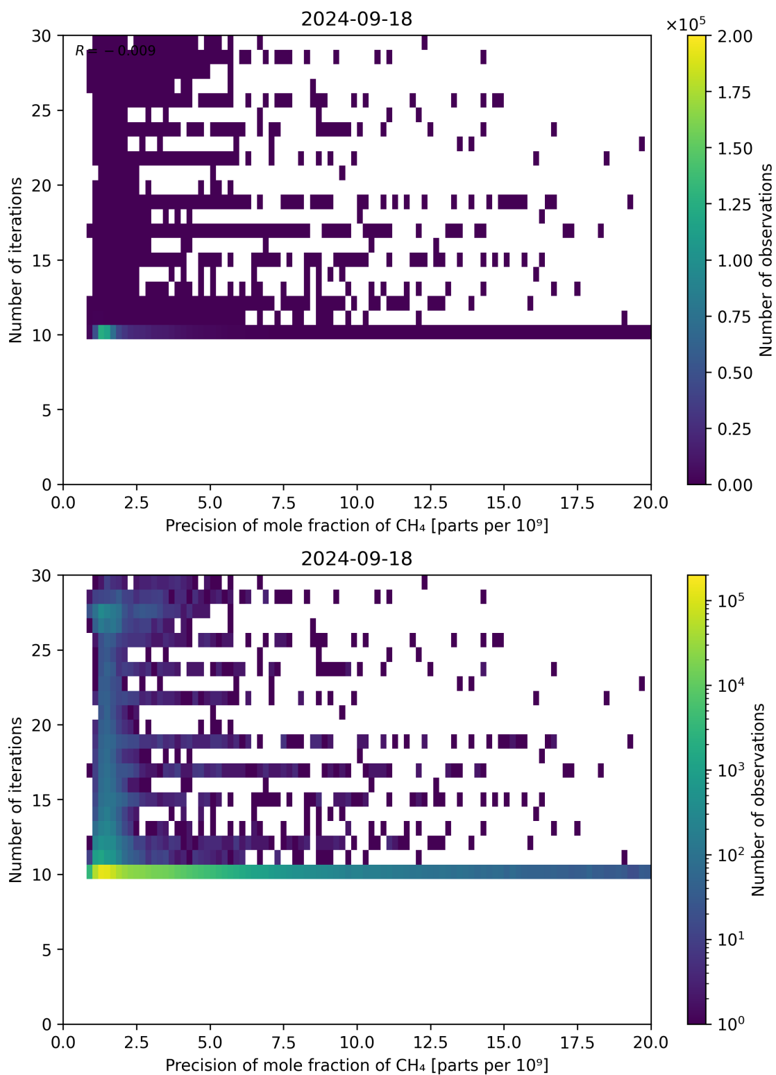
Figure 83: Scatter density plot of “Precision of mole fraction of CH 4 ” against “Number of iterations” for 2024-09-17 to 2024-09-19.
