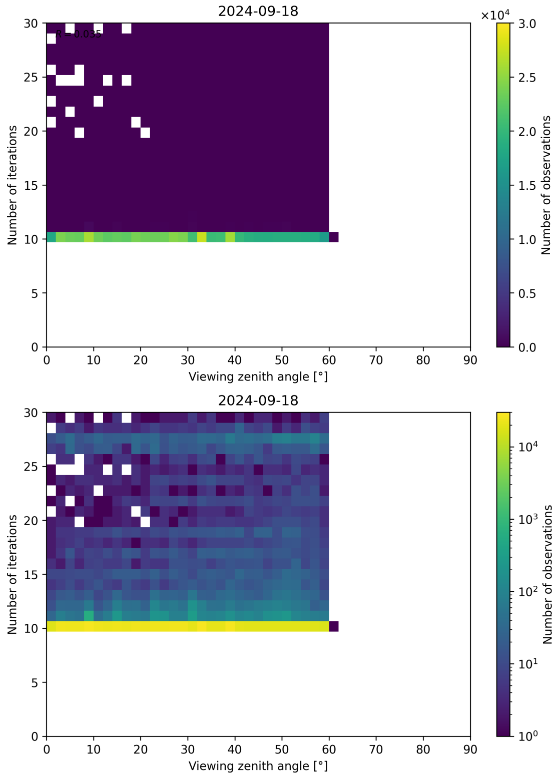
Figure 113: Scatter density plot of “Viewing zenith angle” against “Number of iterations” for 2024-09-17 to 2024-09-19.
