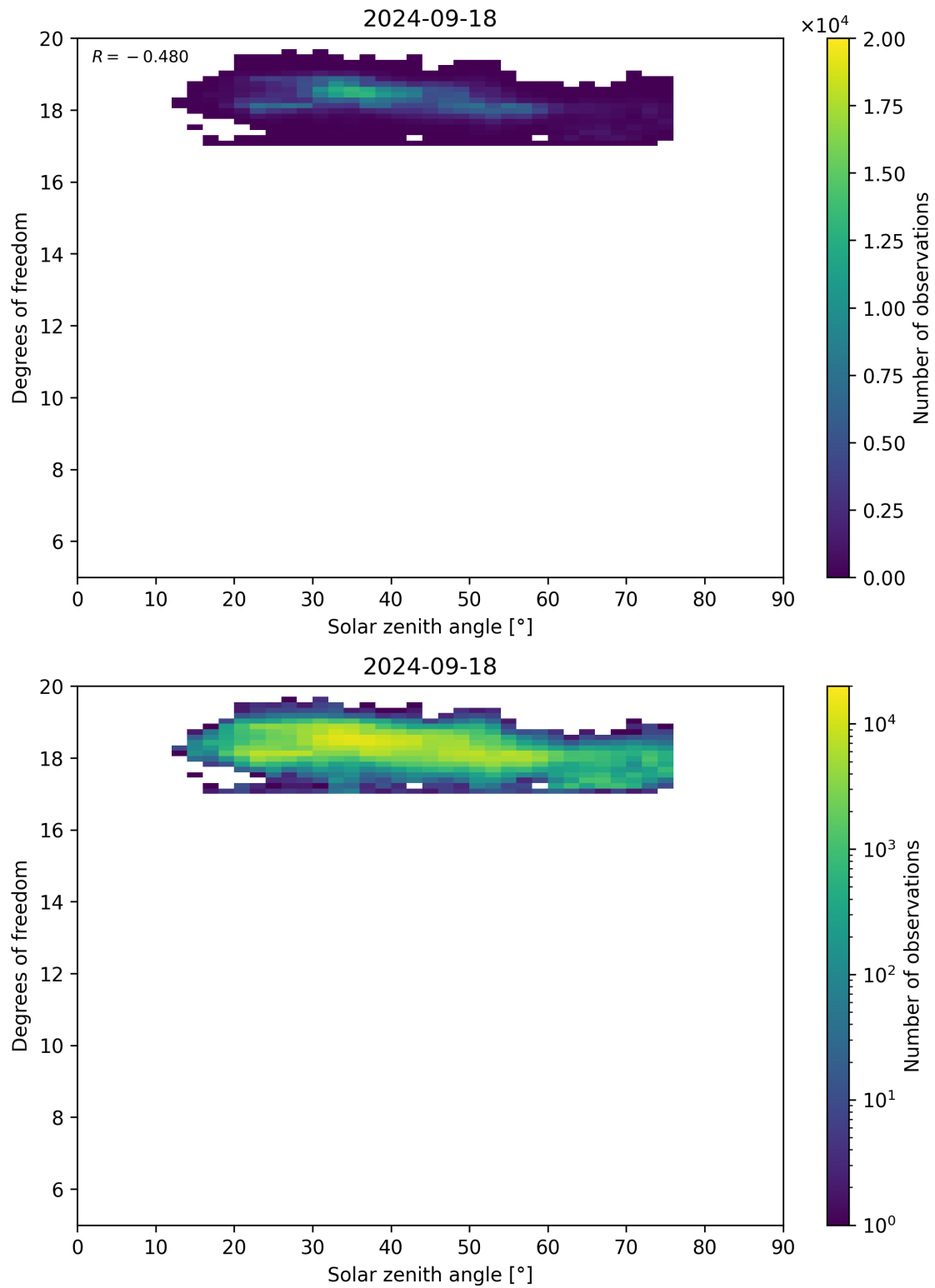
Figure 96: Scatter density plot of “Solar zenith angle” against “Degrees of freedom” for 2024-09-17 to 2024-09-19.
