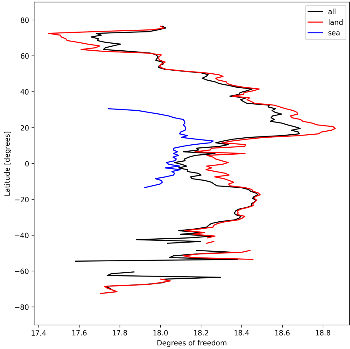
Figure 19: Zonal average of “Degrees of freedom” for 2024-09-17 to 2024-09-19.
