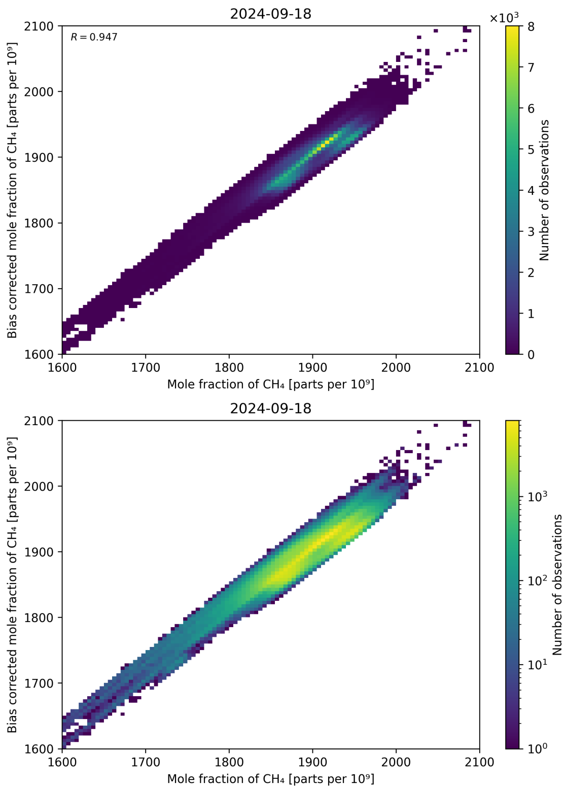
Figure 74: Scatter density plot of “Mole fraction of CH 4 ” against “Bias corrected mole fraction of CH 4 ” for 2024-09-17 to 2024-09-19.
