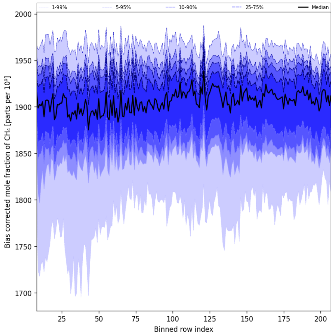
Figure 36: Along track statistics of “Bias corrected mole fraction of CH 4 ” for 2024-09-17 to 2024-09-19
