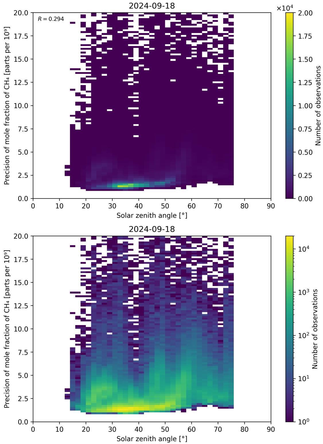
Figure 101: Scatter density plot of “Solar zenith angle” against “Precision of mole fraction of \text{CH}_4 ” for 2024-09-17 to 2024-09-19.
