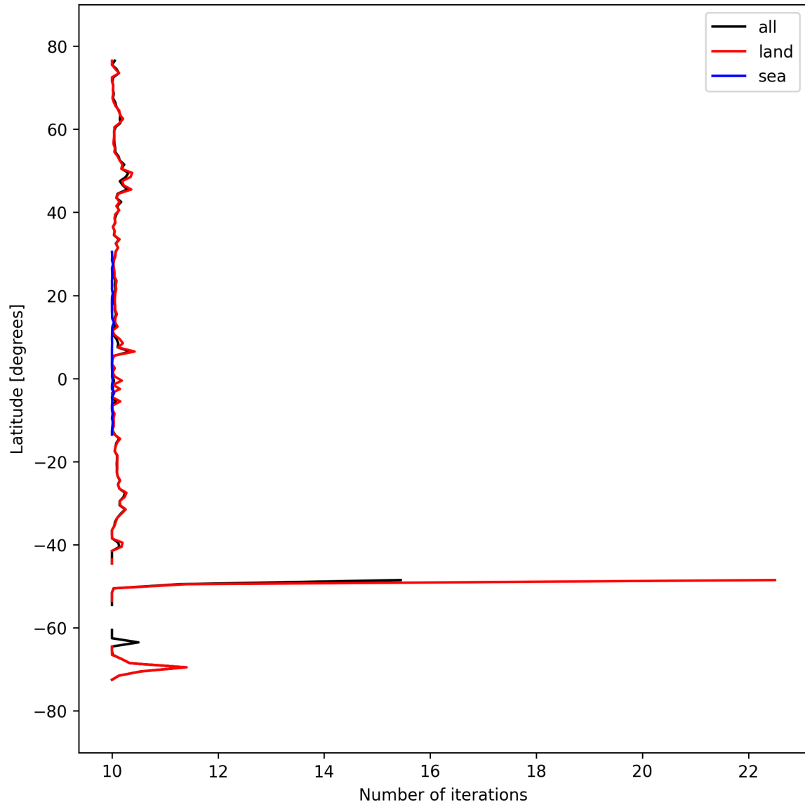
Figure 20: Zonal average of “Number of iterations” for 2024-09-17 to 2024-09-19.
