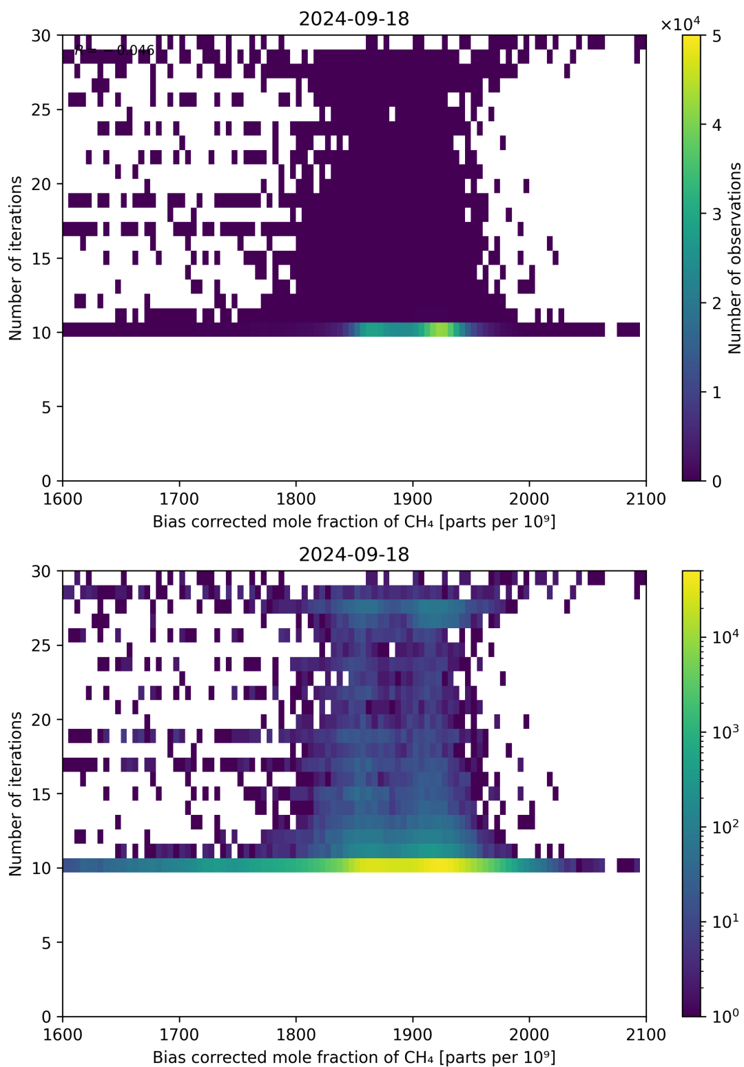
Figure 67: Scatter density plot of “Bias corrected mole fraction of CH 4 ” against “Number of iterations” for 2024-09-17 to 2024-09-19.
