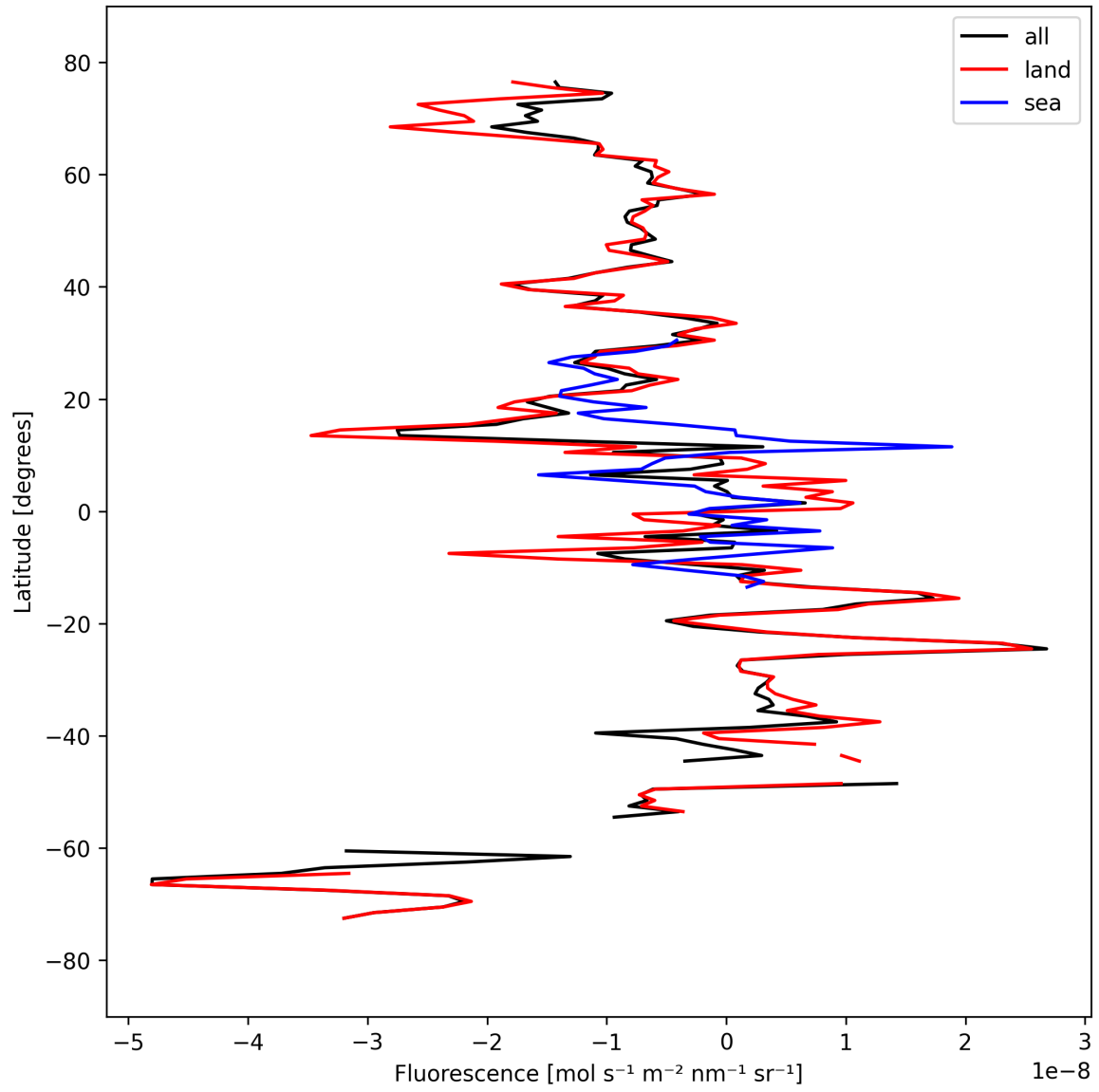
Figure 21: Zonal average of “Fluorescence” for 2024-09-17 to 2024-09-19.
