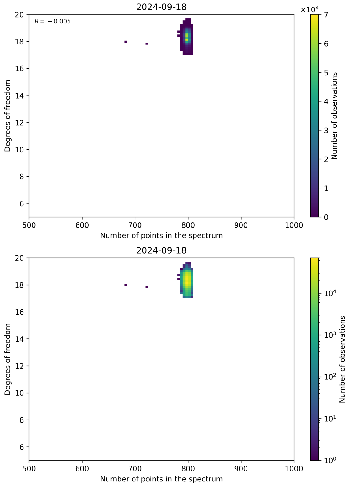
Figure 90: Scatter density plot of “Number of points in the spectrum” against “Degrees of freedom” for 2024-09-17 to 2024-09-19.
