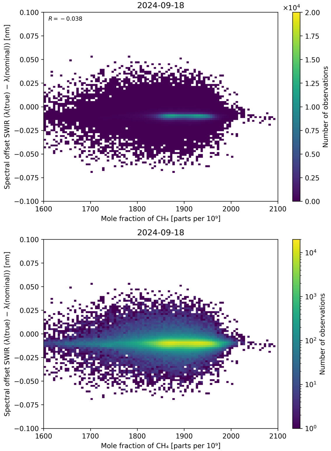
Figure 86: Scatter density plot of “Mole fraction of CH 4 ” against “Spectral offset SWIR ( \lambda_{\text{true}} - \lambda_{\text{nominal}} )” for 2024-09-17 to 2024-09-19.
