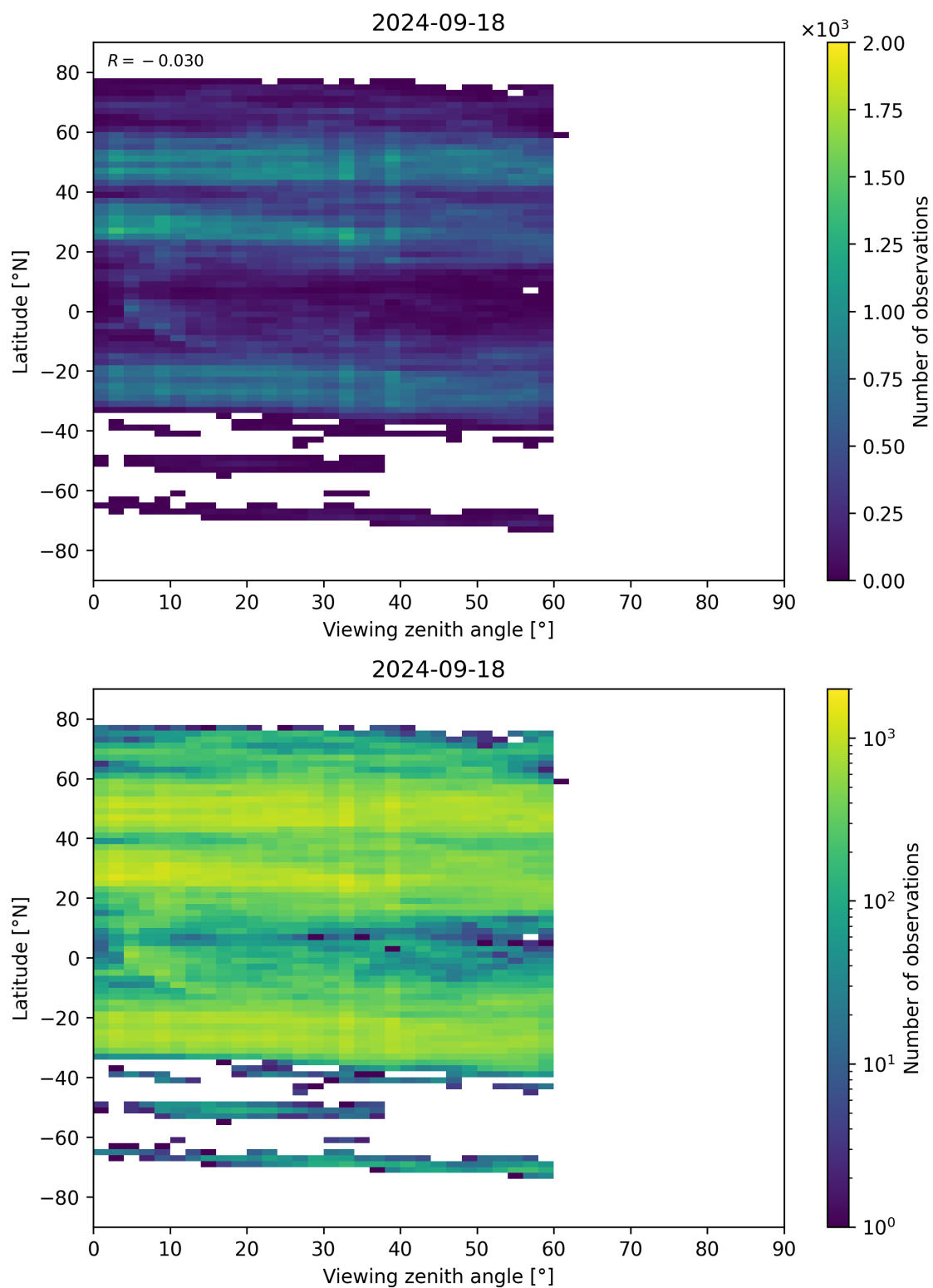
Figure 109: Scatter density plot of “Viewing zenith angle” against “Latitude” for 2024-09-17 to 2024-09-19.
