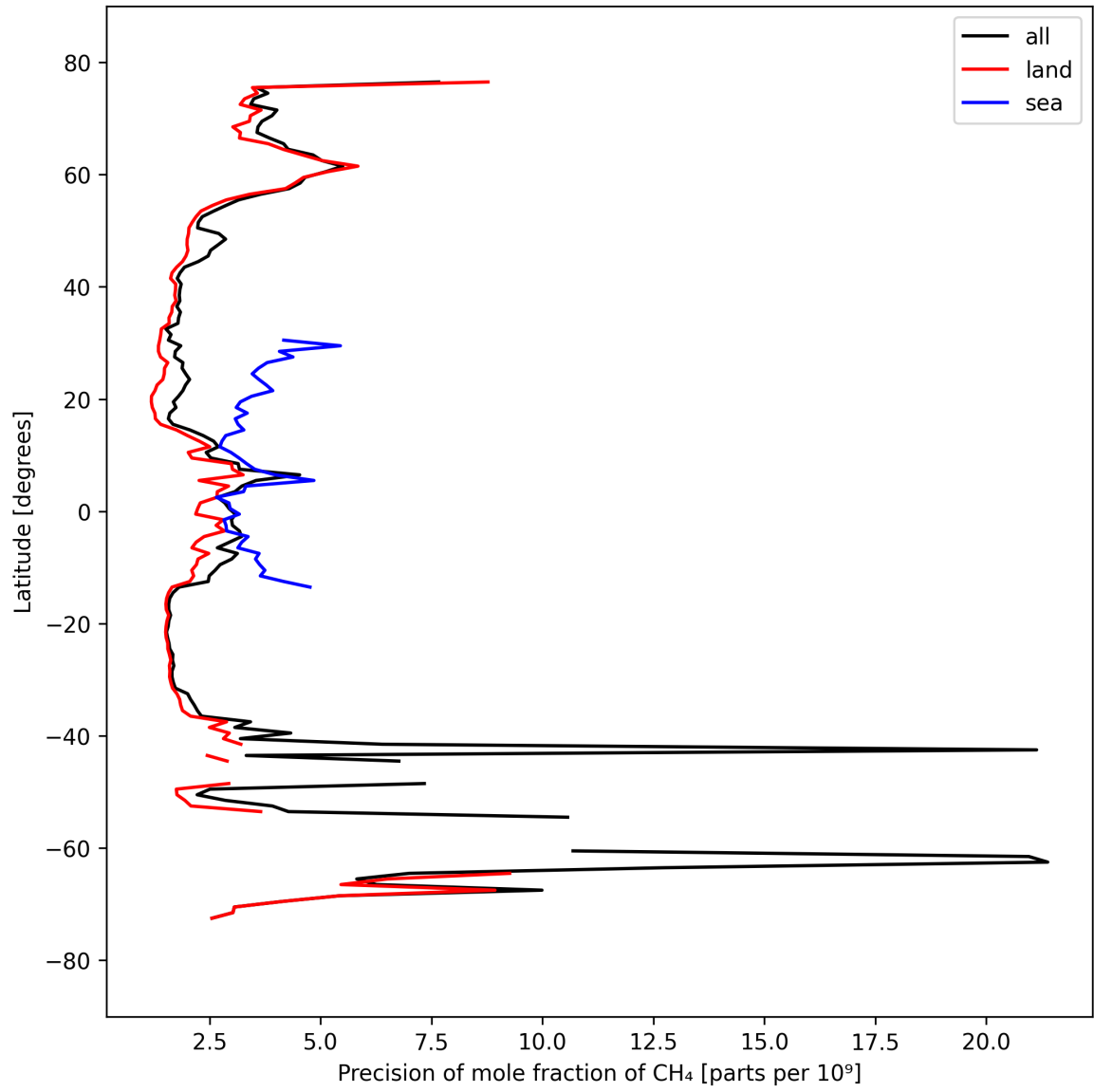
Figure 13: Zonal average of “Precision of mole fraction of \text{CH}_4 ” for 2024-09-17 to 2024-09-19.
