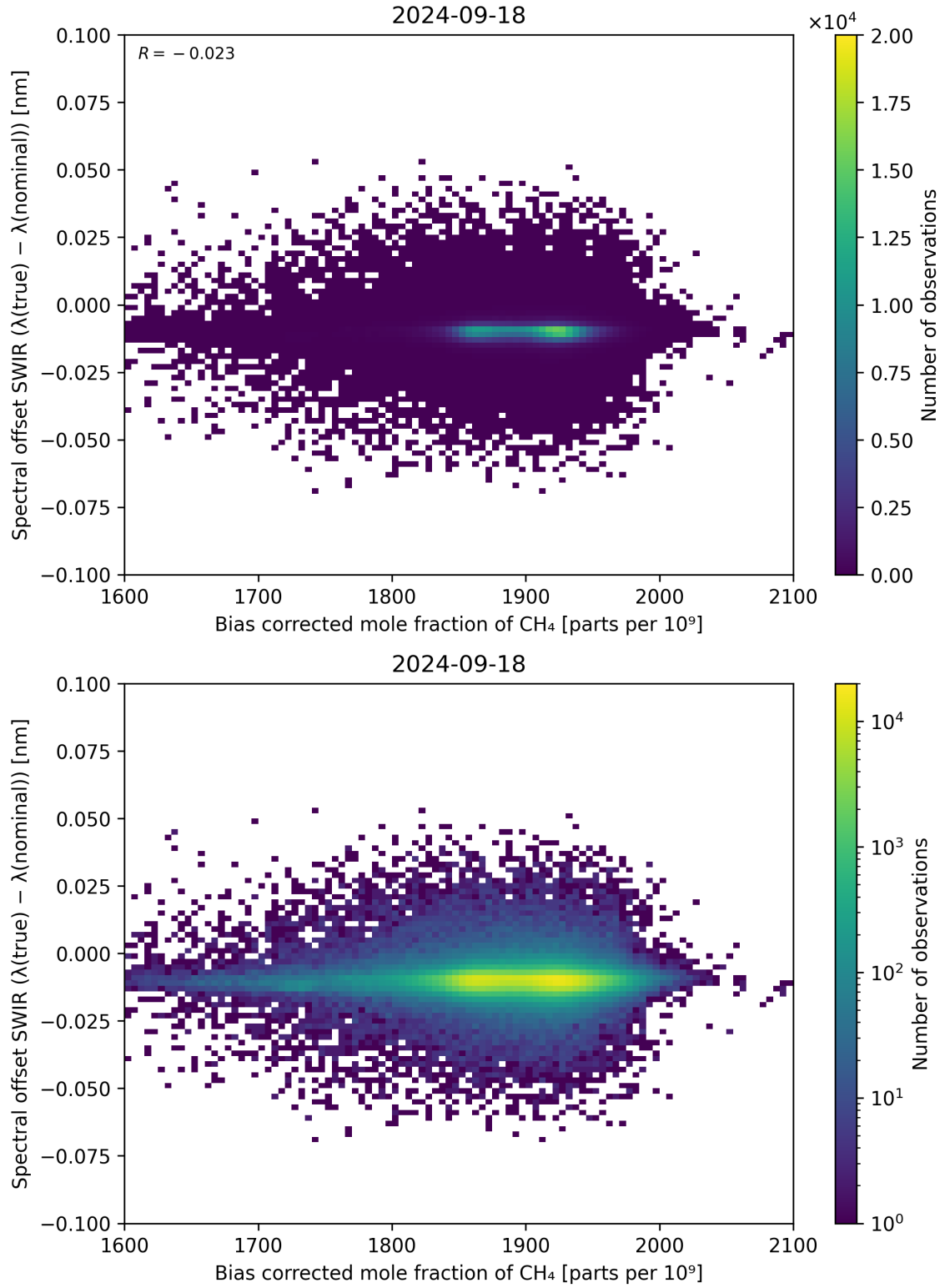
Figure 69: Scatter density plot of “Bias corrected mole fraction of CH 4 ” against “Spectral offset SWIR ( \lambda_{\text{true}} - \lambda_{\text{nominal}} )” for 2024-09-17 to 2024-09-19.
