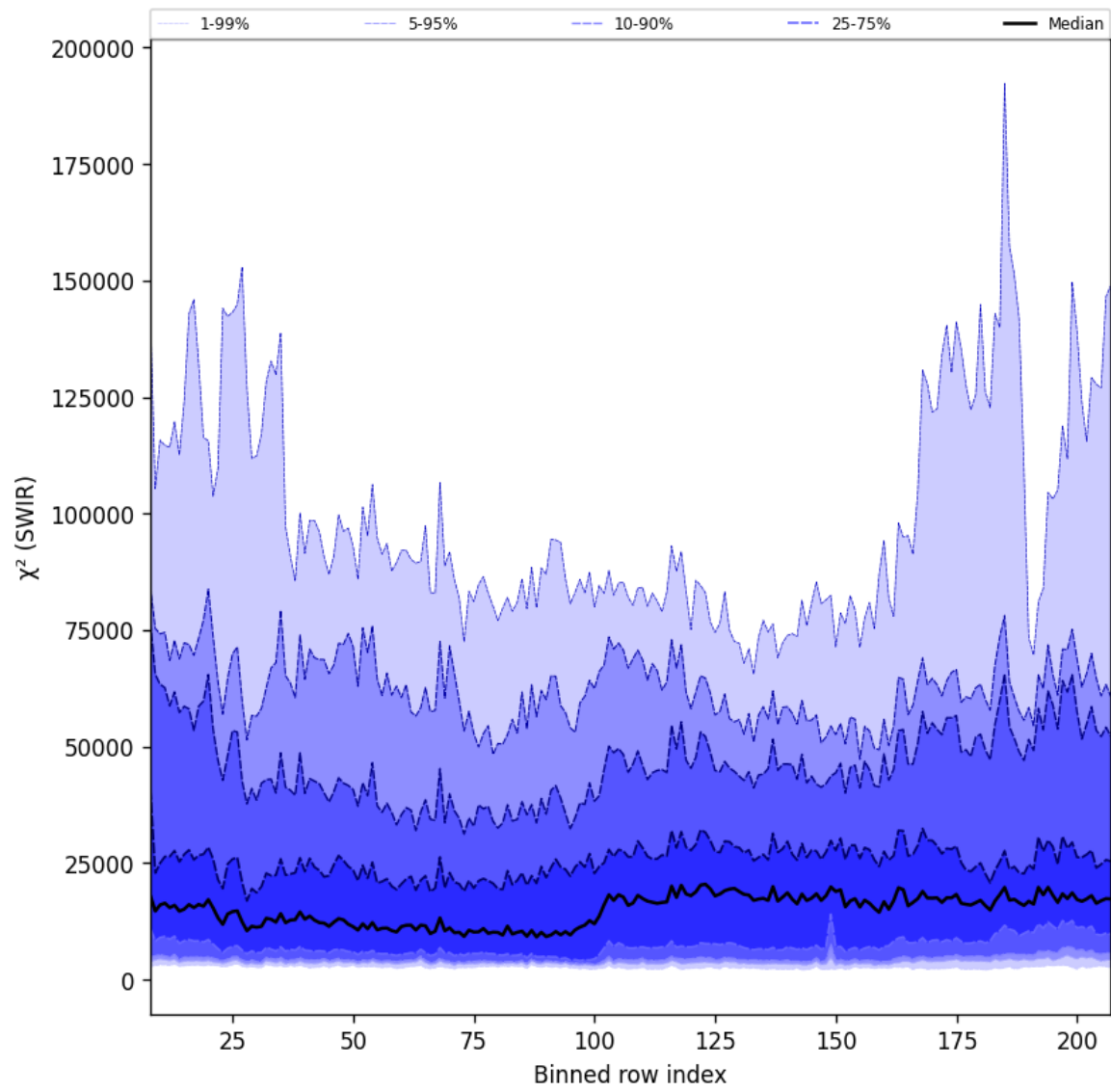
Figure 39: Along track statistics of " \chi^2 (SWIR)" for 2024-09-17 to 2024-09-19
