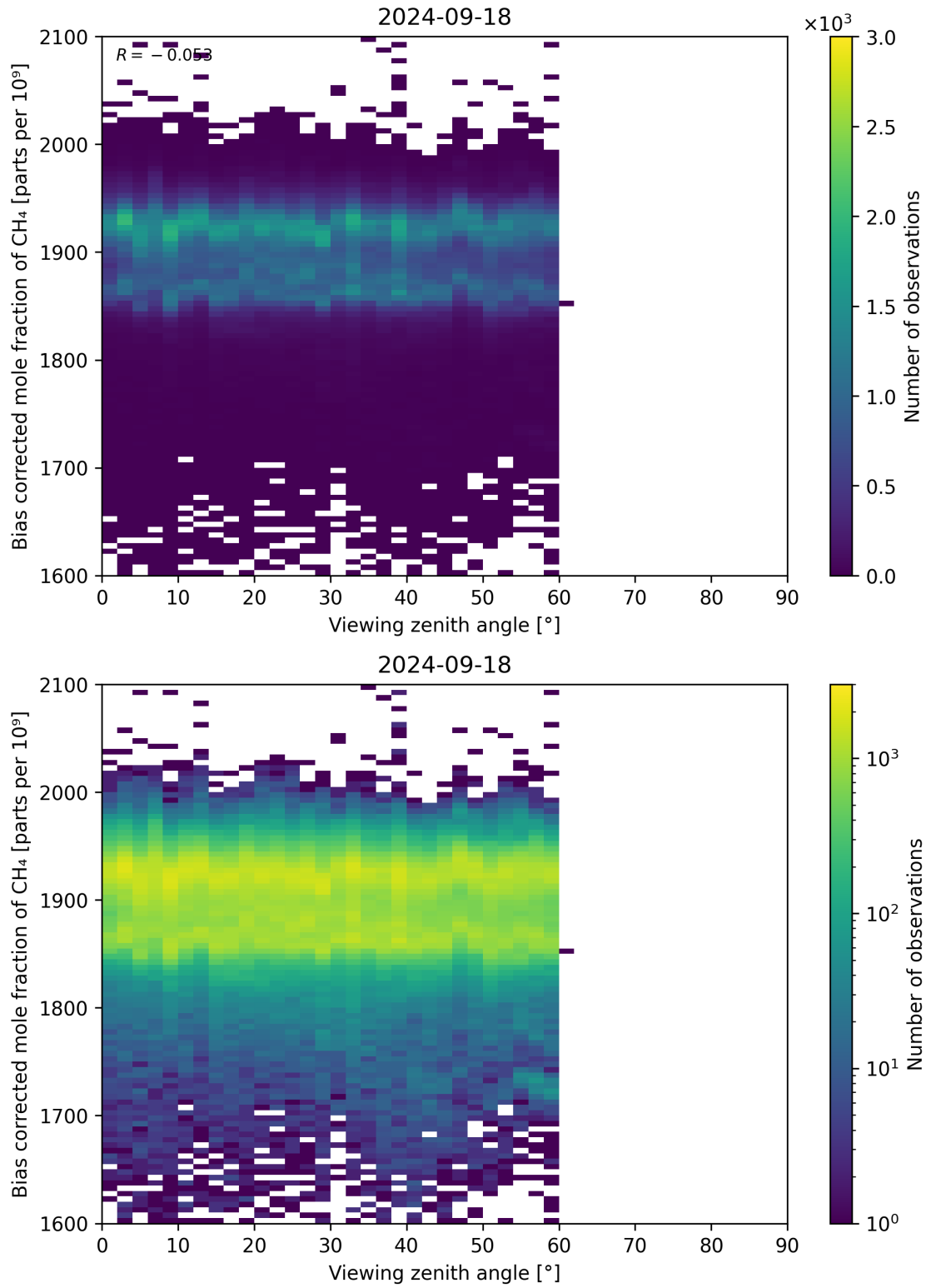
Figure 111: Scatter density plot of “Viewing zenith angle” against “Bias corrected mole fraction of CH 4 ” for 2024-09-17 to 2024-09-19.
