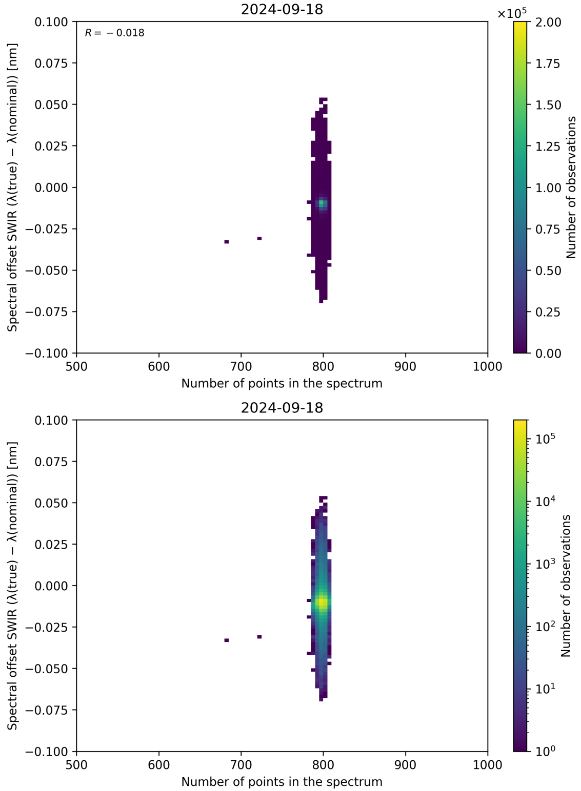
Figure 93: Scatter density plot of “Number of points in the spectrum” against “Spectral offset SWIR ( \lambda_{\text{true}} - \lambda_{\text{nominal}} )” for 2024-09-17 to 2024-09-19.
