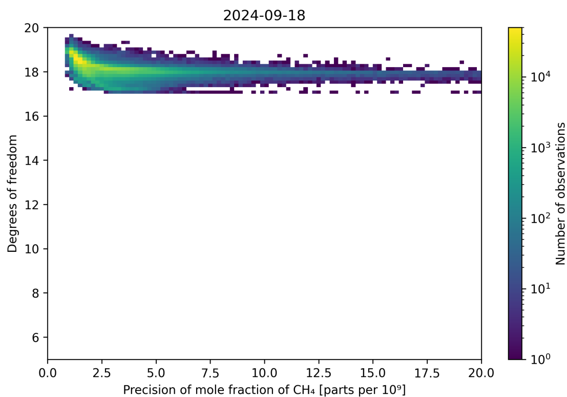
Figure 80: Scatter density plot of “Precision of mole fraction of CH 4 ” against “Degrees of freedom” for 2024-09-17 to 2024-09-19.
