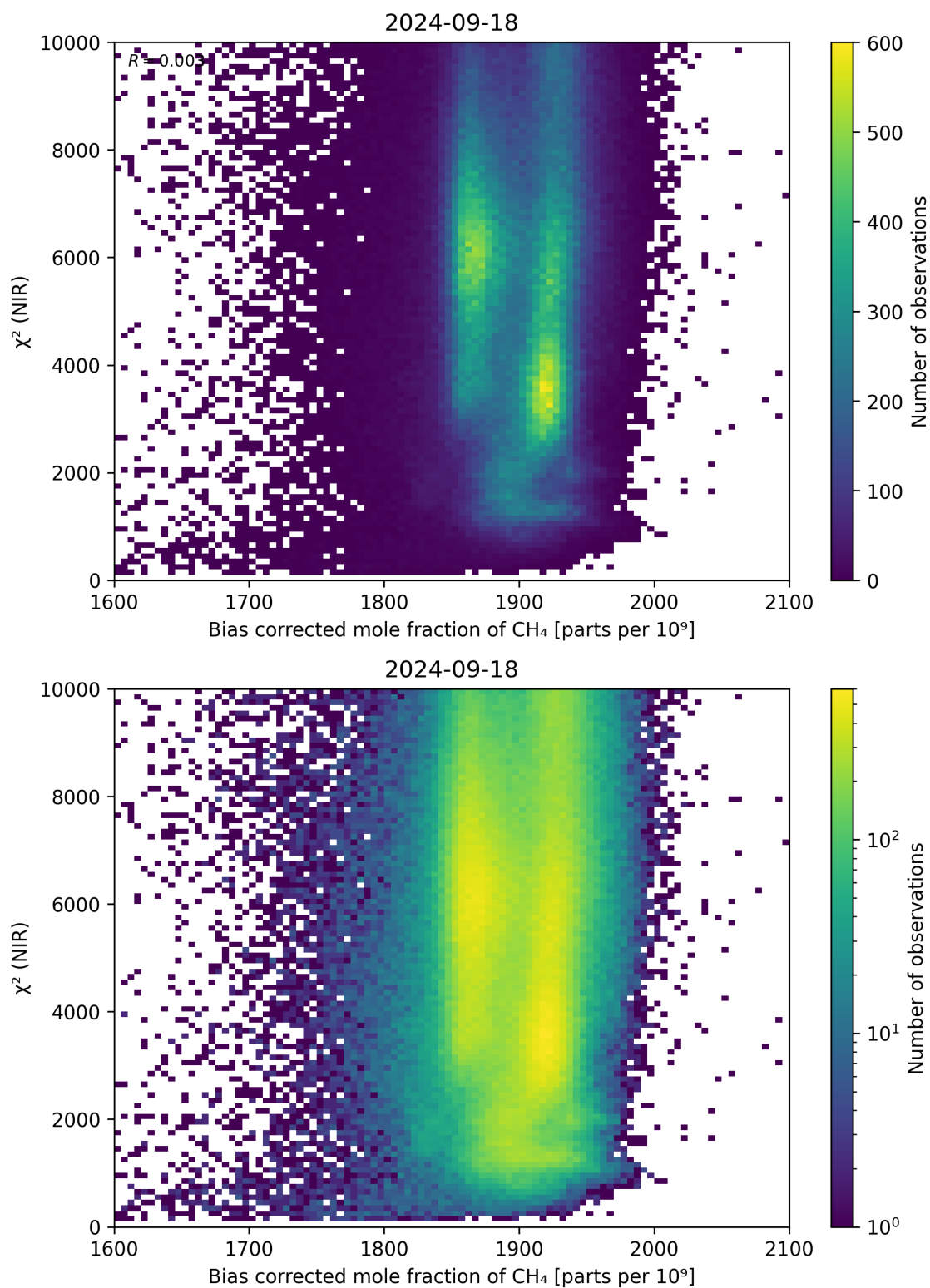
Figure 63: Scatter density plot of “Bias corrected mole fraction of \text{CH}_4 ” against “ \chi^2 (NIR)” for 2024-09-17 to 2024-09-19.
