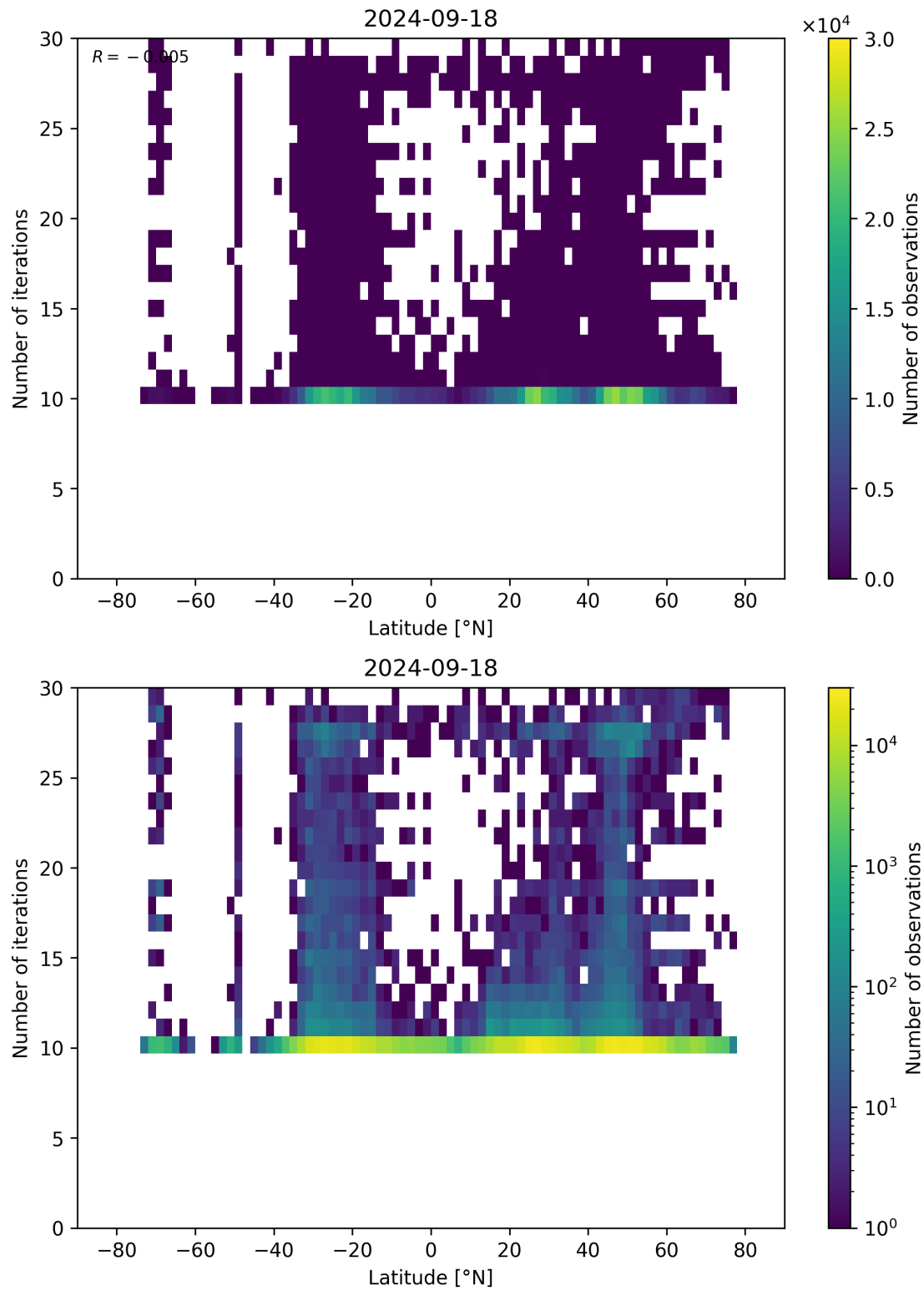
Figure 60: Scatter density plot of “Latitude” against “Number of iterations” for 2024-09-17 to 2024-09-19.
