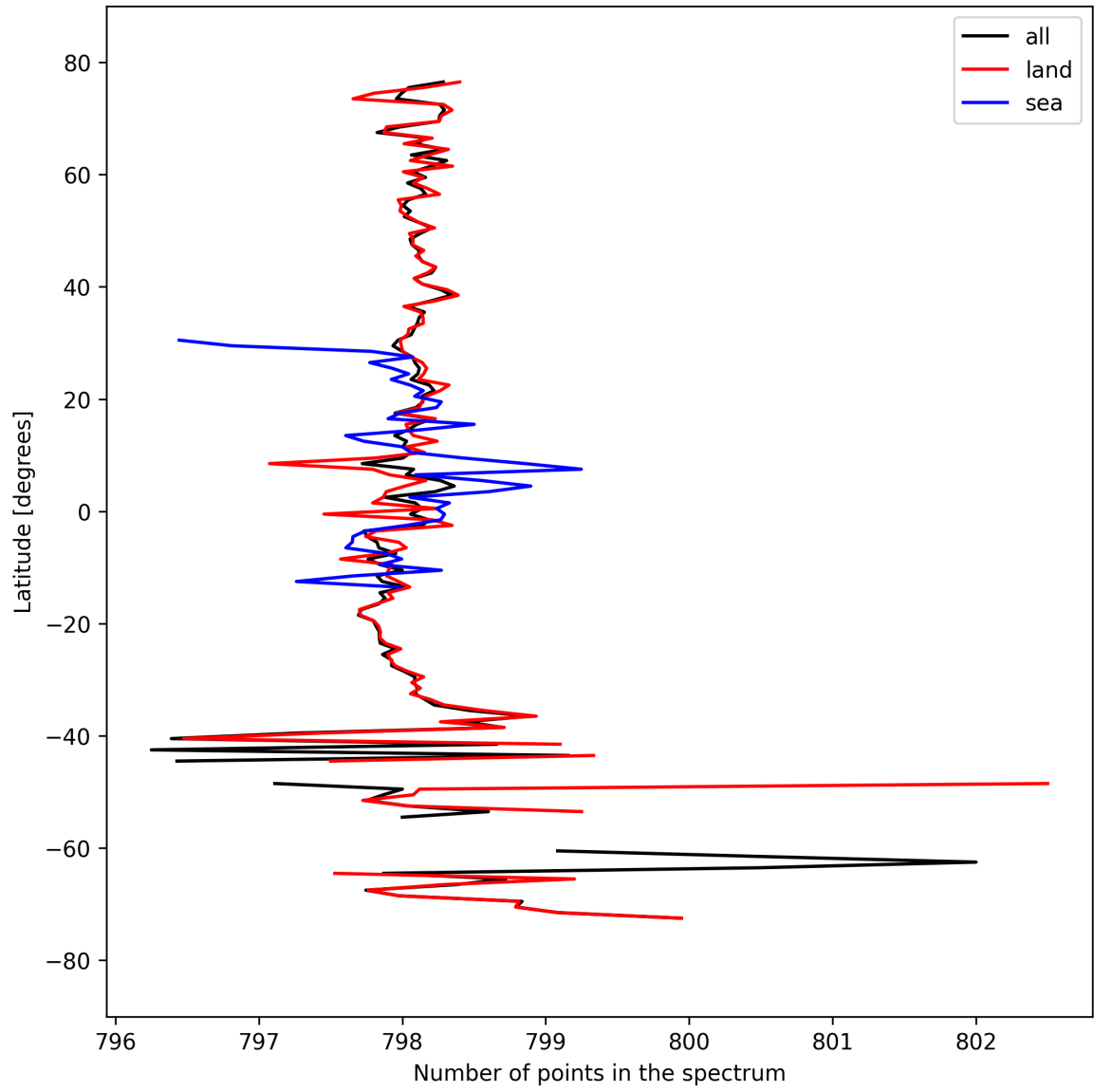
Figure 15: Zonal average of “Number of points in the spectrum” for 2024-09-17 to 2024-09-19.
