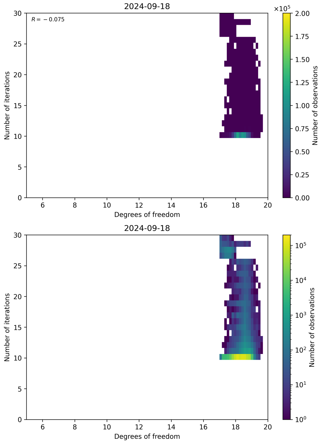
Figure 52: Scatter density plot of “Degrees of freedom” against “Number of iterations” for 2024-09-17 to 2024-09-19.
