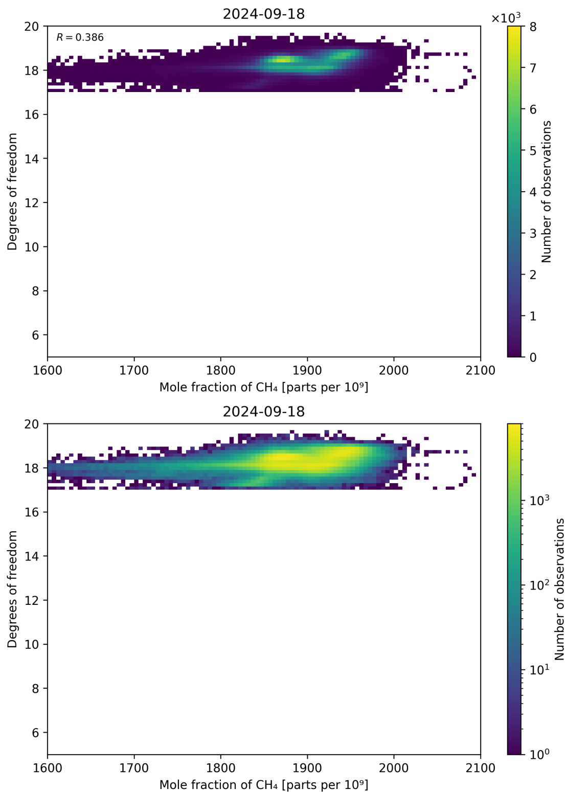
Figure 72: Scatter density plot of “Mole fraction of CH 4 ” against “Degrees of freedom” for 2024-09-17 to 2024-09-19.
