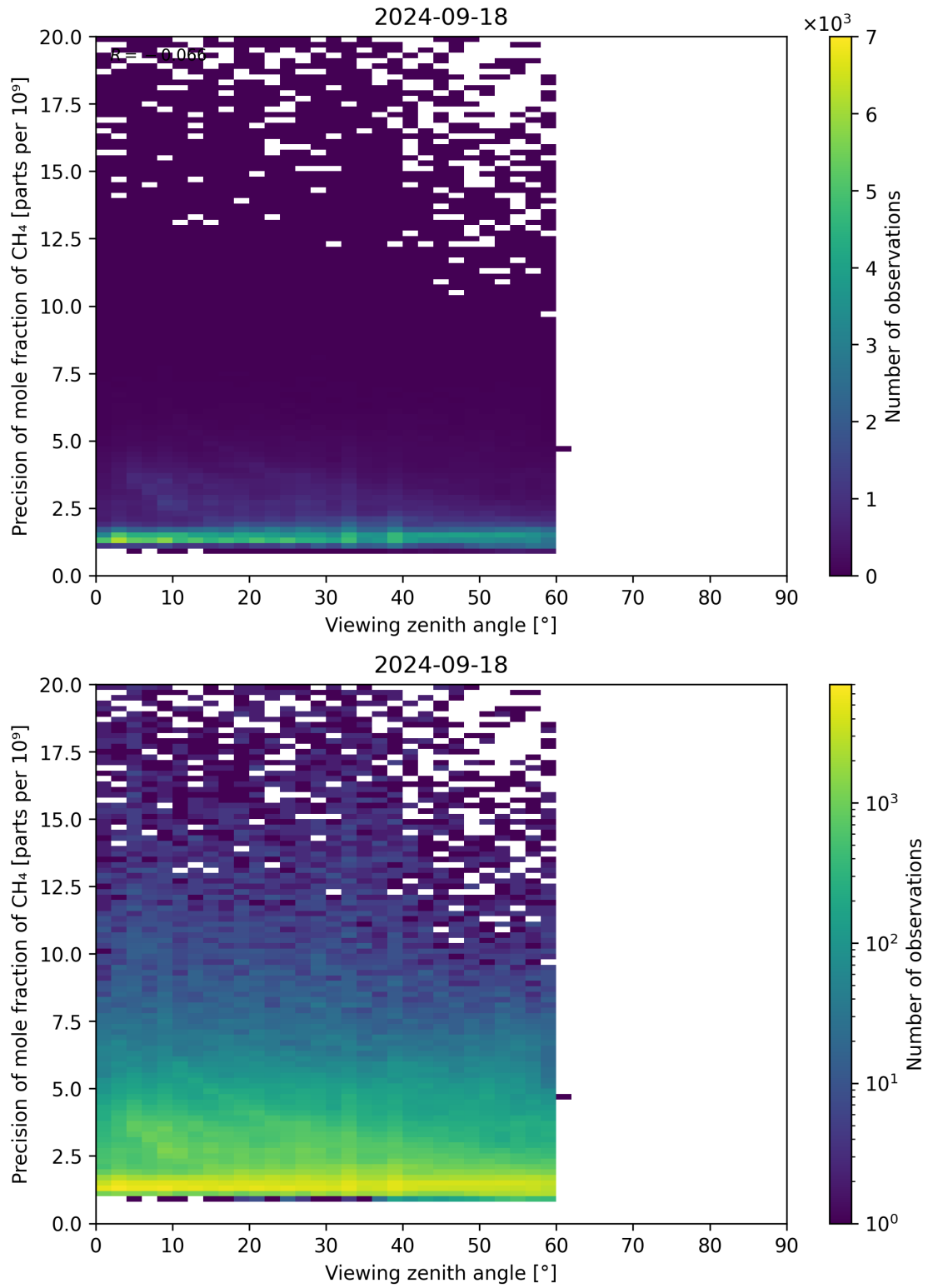
Figure 112: Scatter density plot of “Viewing zenith angle” against “Precision of mole fraction of CH 4 ” for 2024-09-17 to 2024-09-19.
