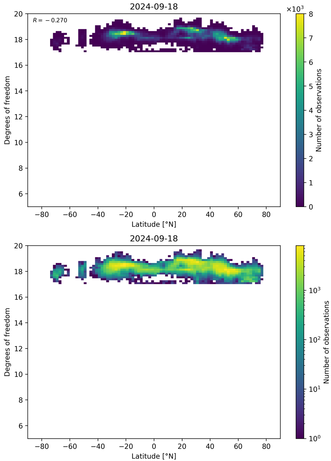
Figure 55: Scatter density plot of “Latitude” against “Degrees of freedom” for 2024-09-17 to 2024-09-19.
