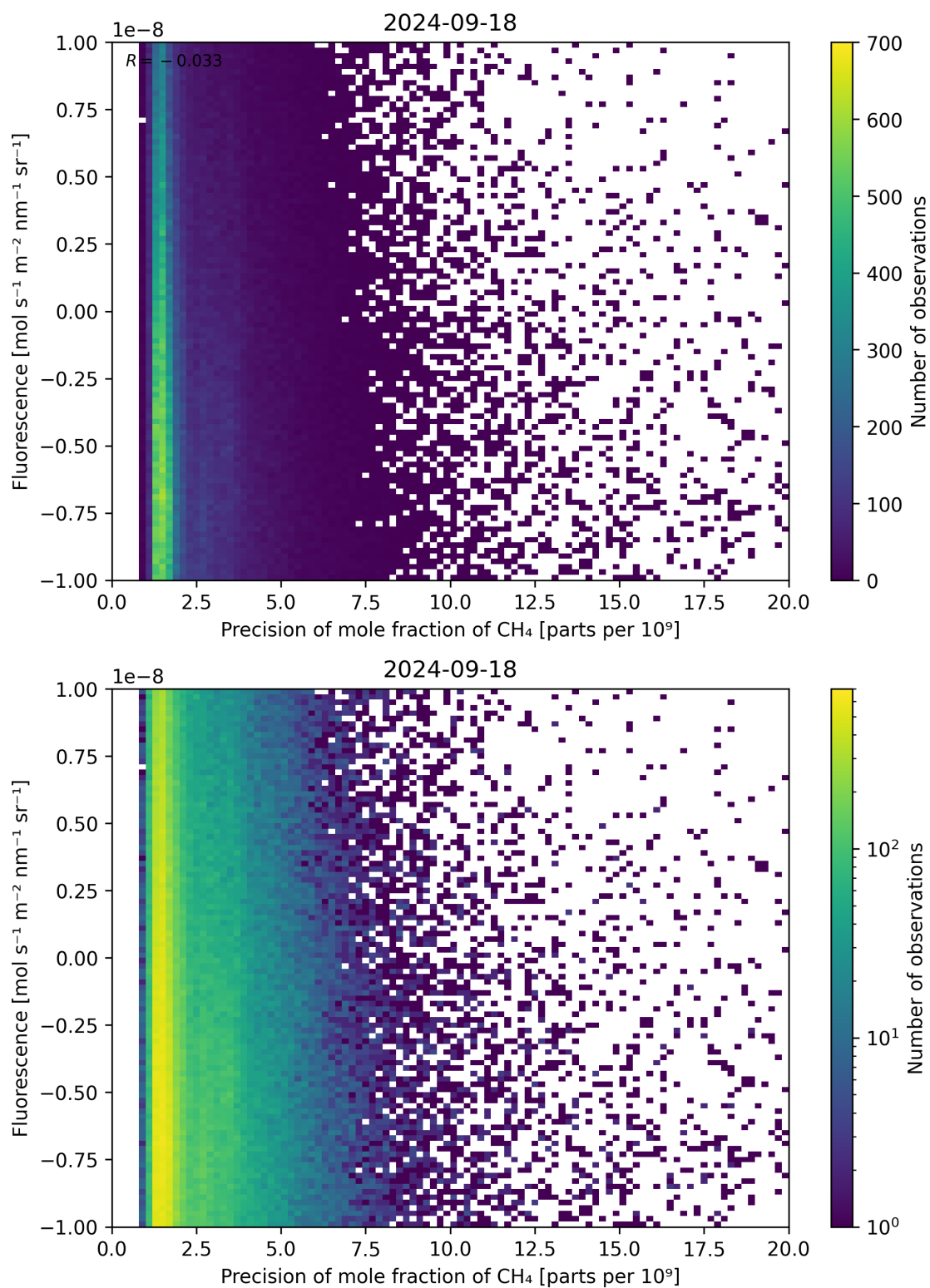
Figure 81: Scatter density plot of “Precision of mole fraction of \text{CH}_4 ” against “Fluorescence” for 2024-09-17 to 2024-09-19.
