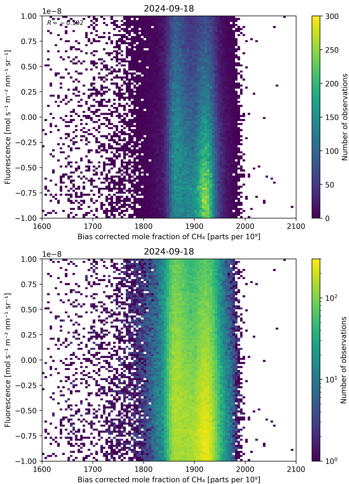
Figure 66: Scatter density plot of “Bias corrected mole fraction of \text{CH}_4 ” against “Fluorescence” for 2024-09-17 to 2024-09-19.
