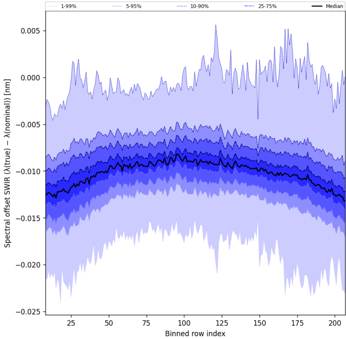
Figure 38: Along track statistics of “Spectral offset SWIR ( \lambda_{\text{true}} - \lambda_{\text{nominal}} )” for 2024-09-17 to 2024-09-19
