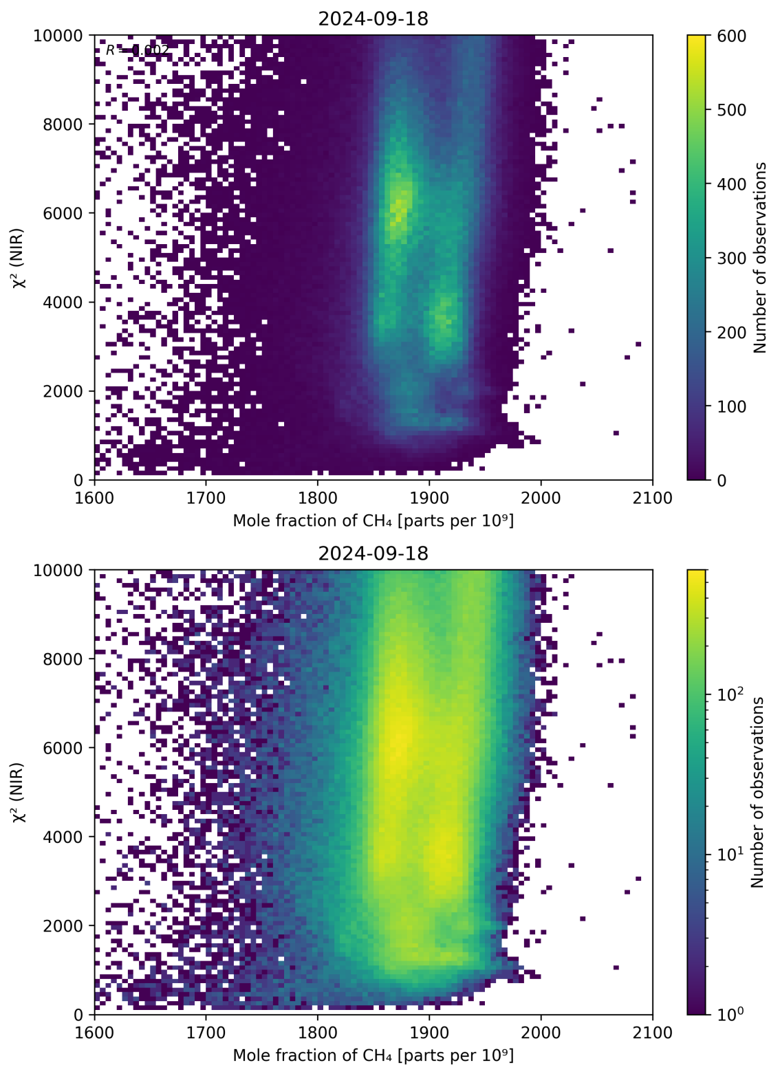
Figure 70: Scatter density plot of “Mole fraction of \text{CH}_4 ” against “ \chi^2 (NIR)” for 2024-09-17 to 2024-09-19.
