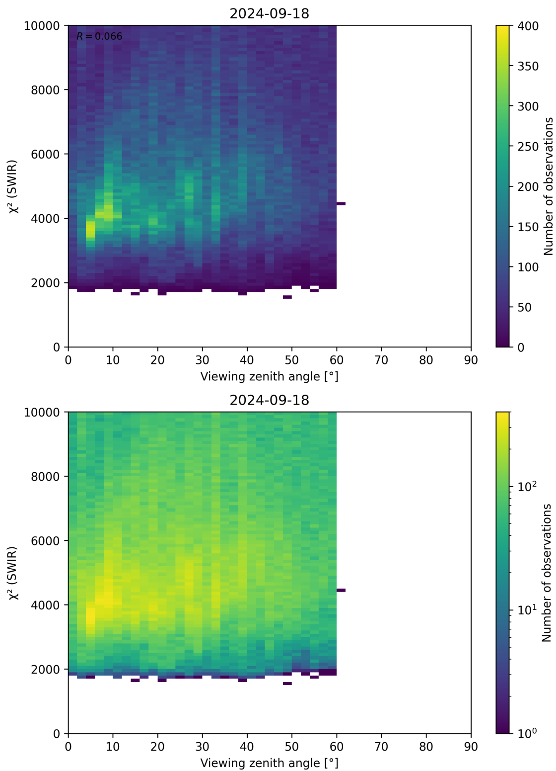
Figure 106: Scatter density plot of “Viewing zenith angle” against “ \chi^2 (SWIR)” for 2024-09-17 to 2024-09-19.
