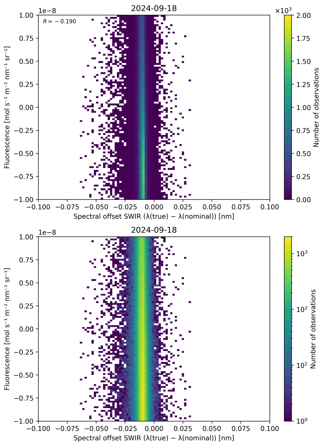
Figure 120: Scatter density plot of “Spectral offset SWIR ( \lambda_{\text{true}} - \lambda_{\text{nominal}} )” against “Fluorescence” for 2024-09-17 to 2024-09-19.
