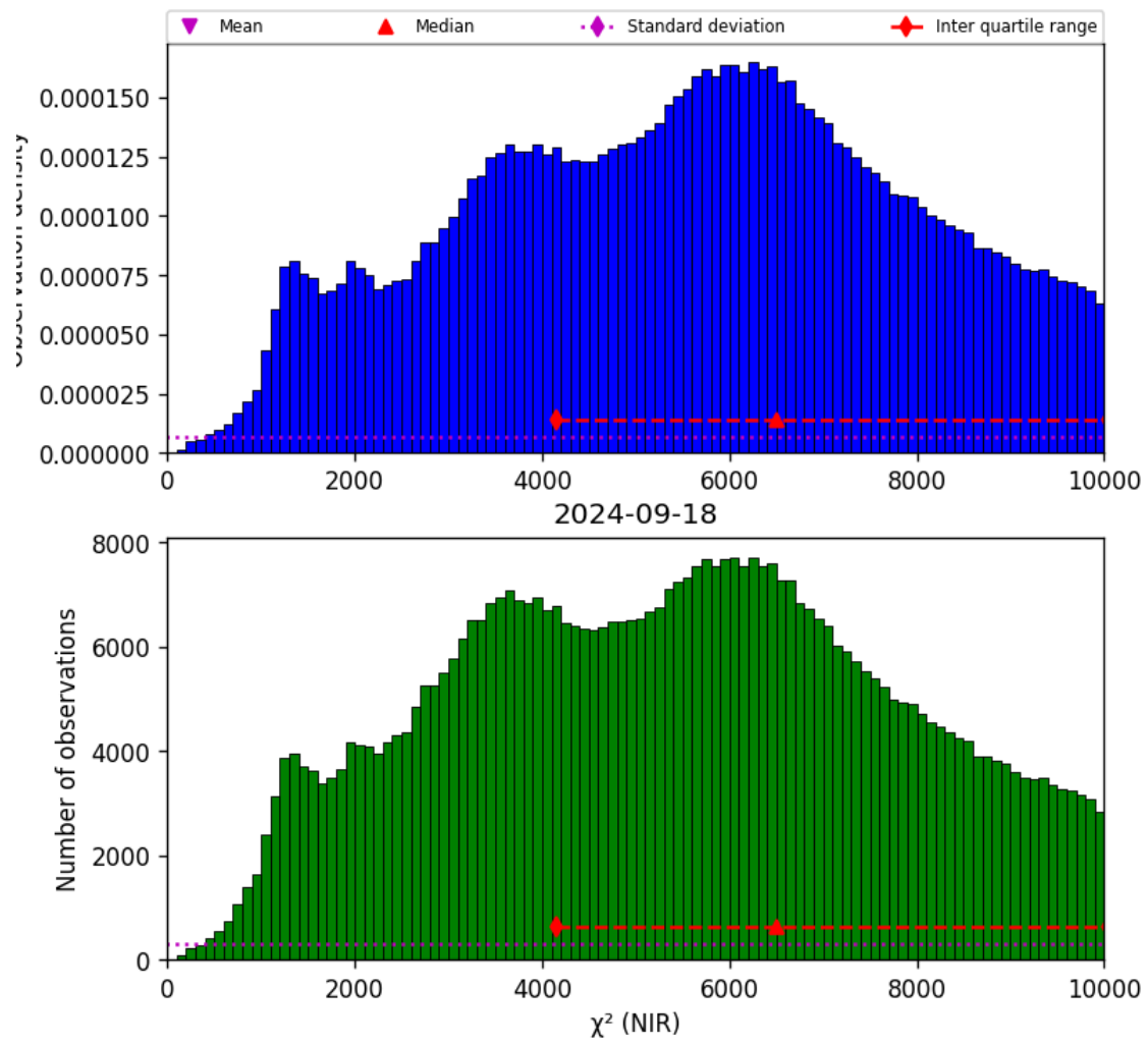
Figure 29: Histogram of “ \chi^2 (NIR)” for 2024-09-17 to 2024-09-19
