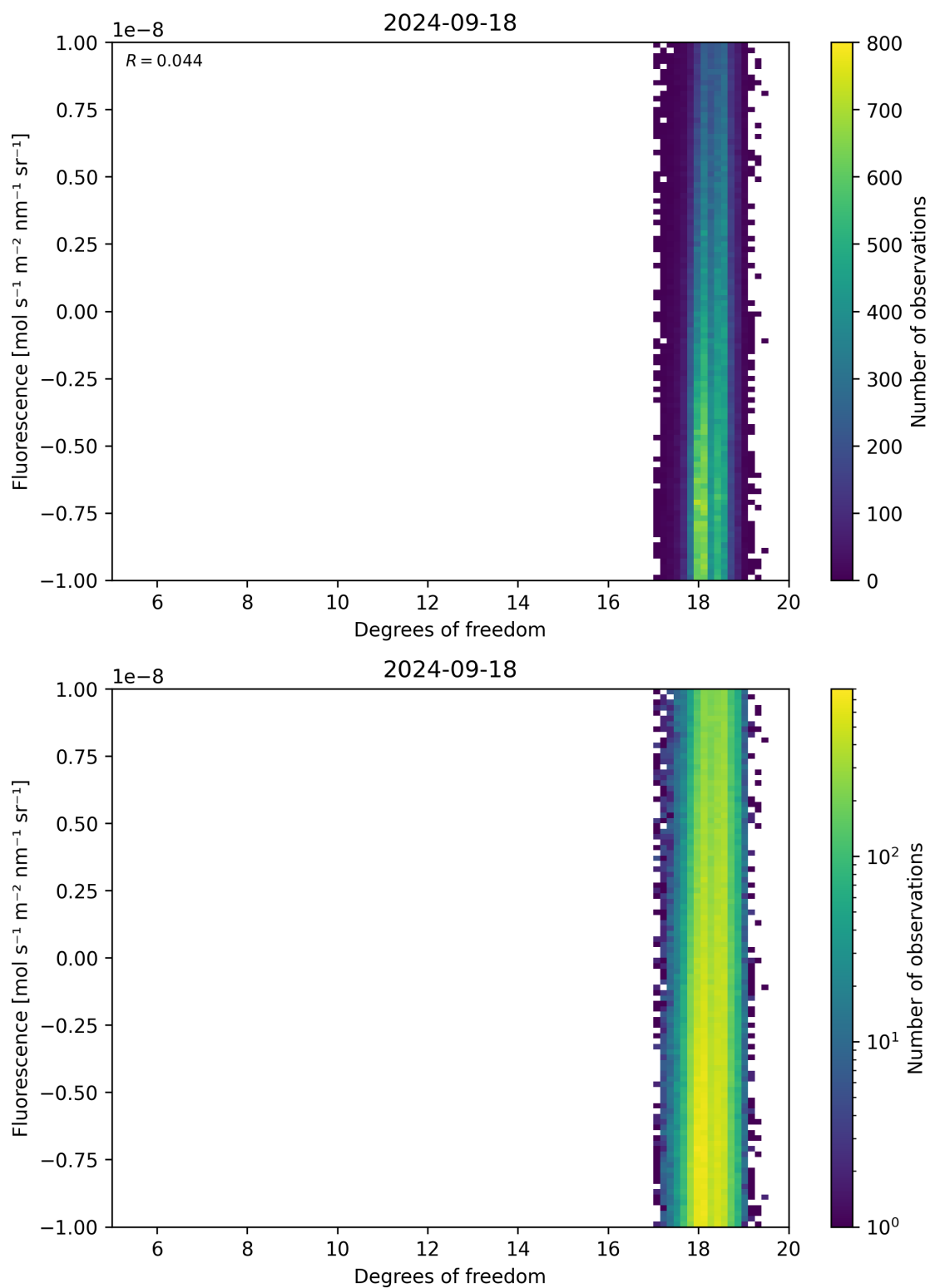
Figure 51: Scatter density plot of “Degrees of freedom” against “Fluorescence” for 2024-09-17 to 2024-09-19.
