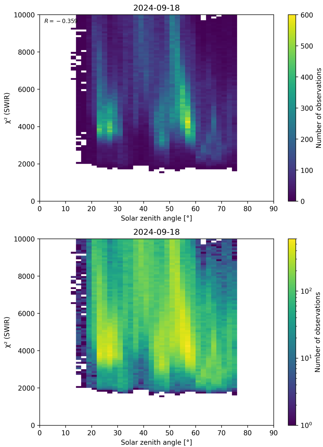
Figure 95: Scatter density plot of “Solar zenith angle” against “ \chi^2 (SWIR)” for 2024-09-17 to 2024-09-19.
