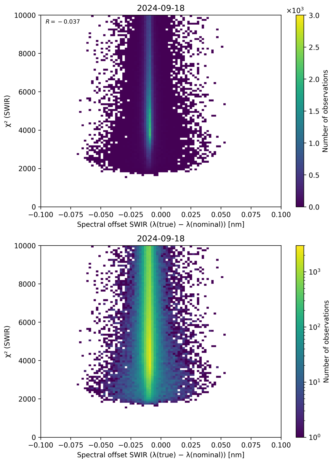
Figure 118: Scatter density plot of “Spectral offset SWIR ( \lambda_{\text{true}} - \lambda_{\text{nominal}} )” against “ \chi^2 (SWIR)” for 2024-09-17 to 2024-09-19.
