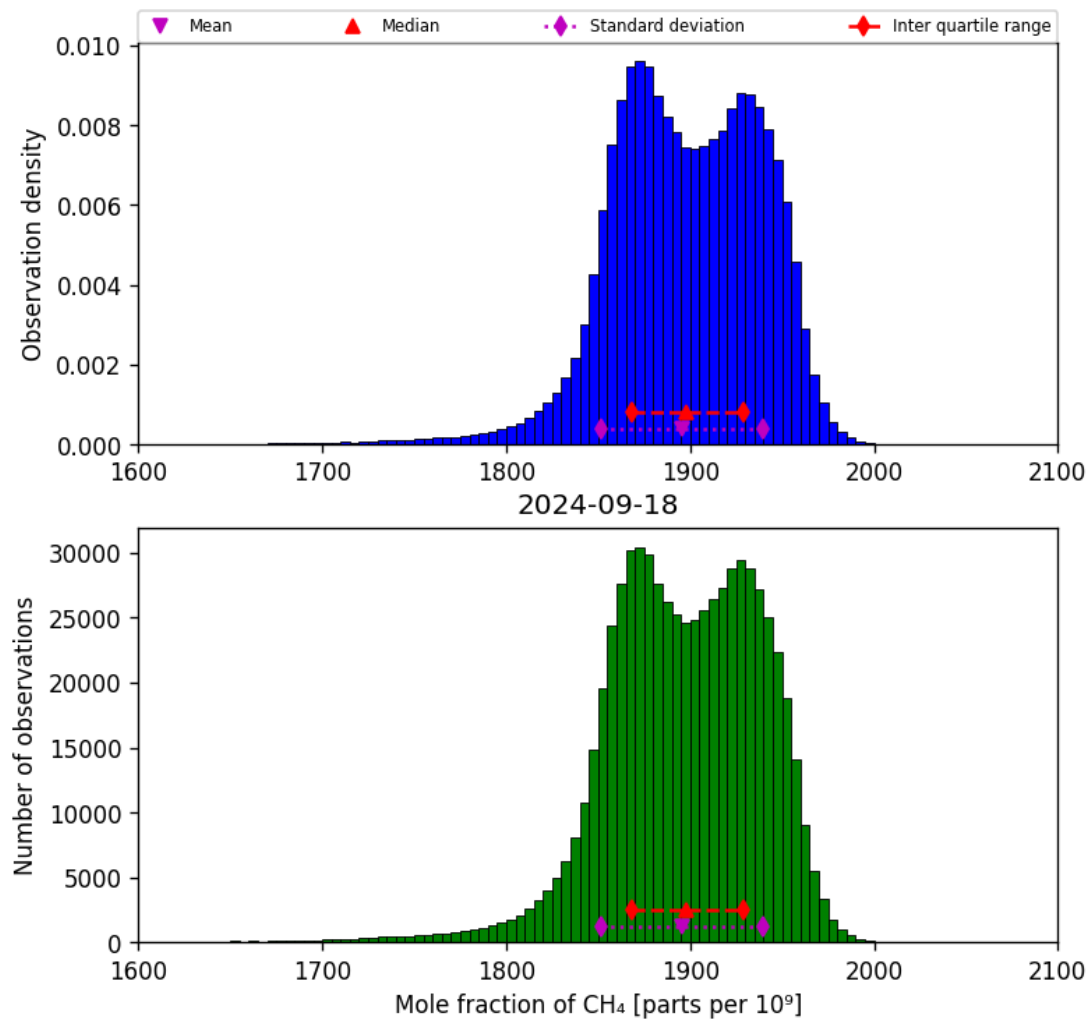
Figure 23: Histogram of “Mole fraction of CH 4 ” for 2024-09-17 to 2024-09-19
