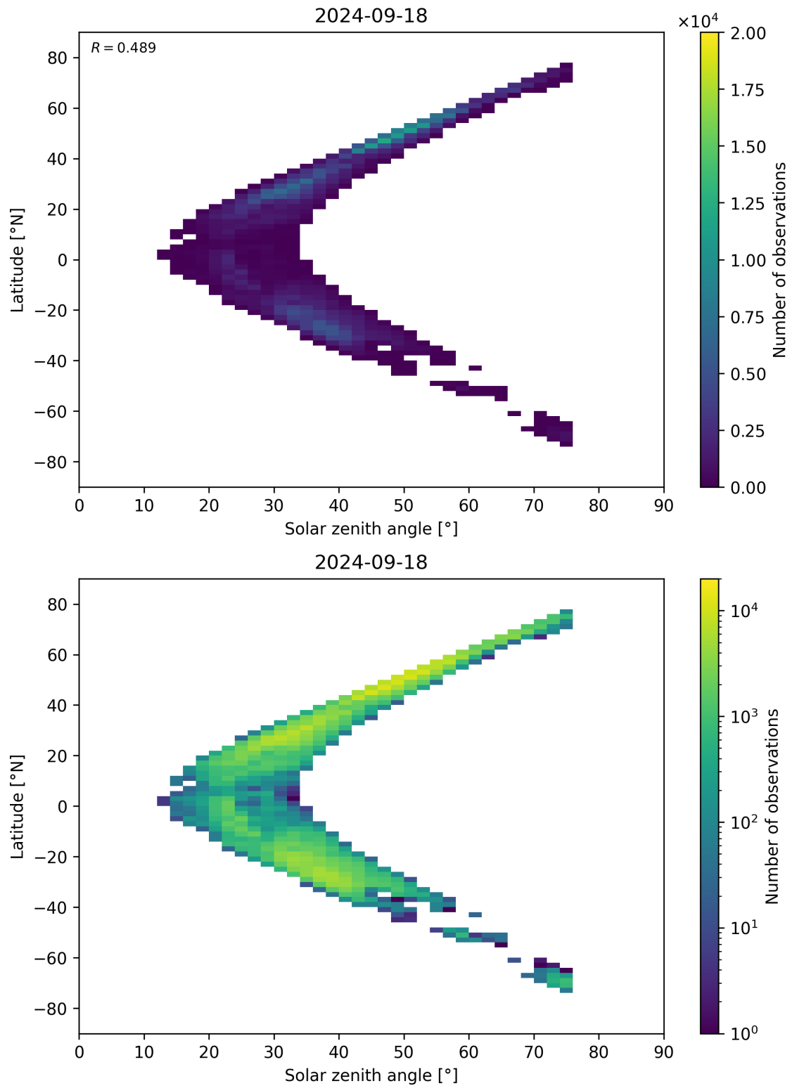
Figure 98: Scatter density plot of “Solar zenith angle” against “Latitude” for 2024-09-17 to 2024-09-19.
