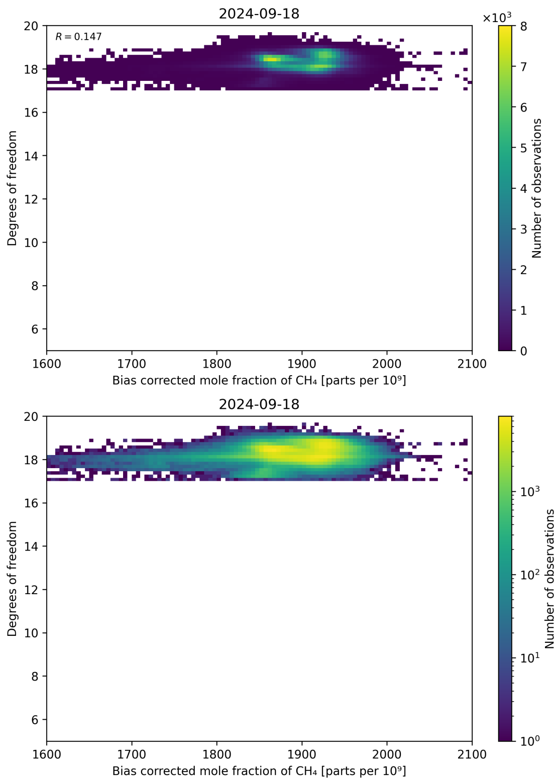
Figure 65: Scatter density plot of “Bias corrected mole fraction of CH 4 ” against “Degrees of freedom” for 2024-09-17 to 2024-09-19.
