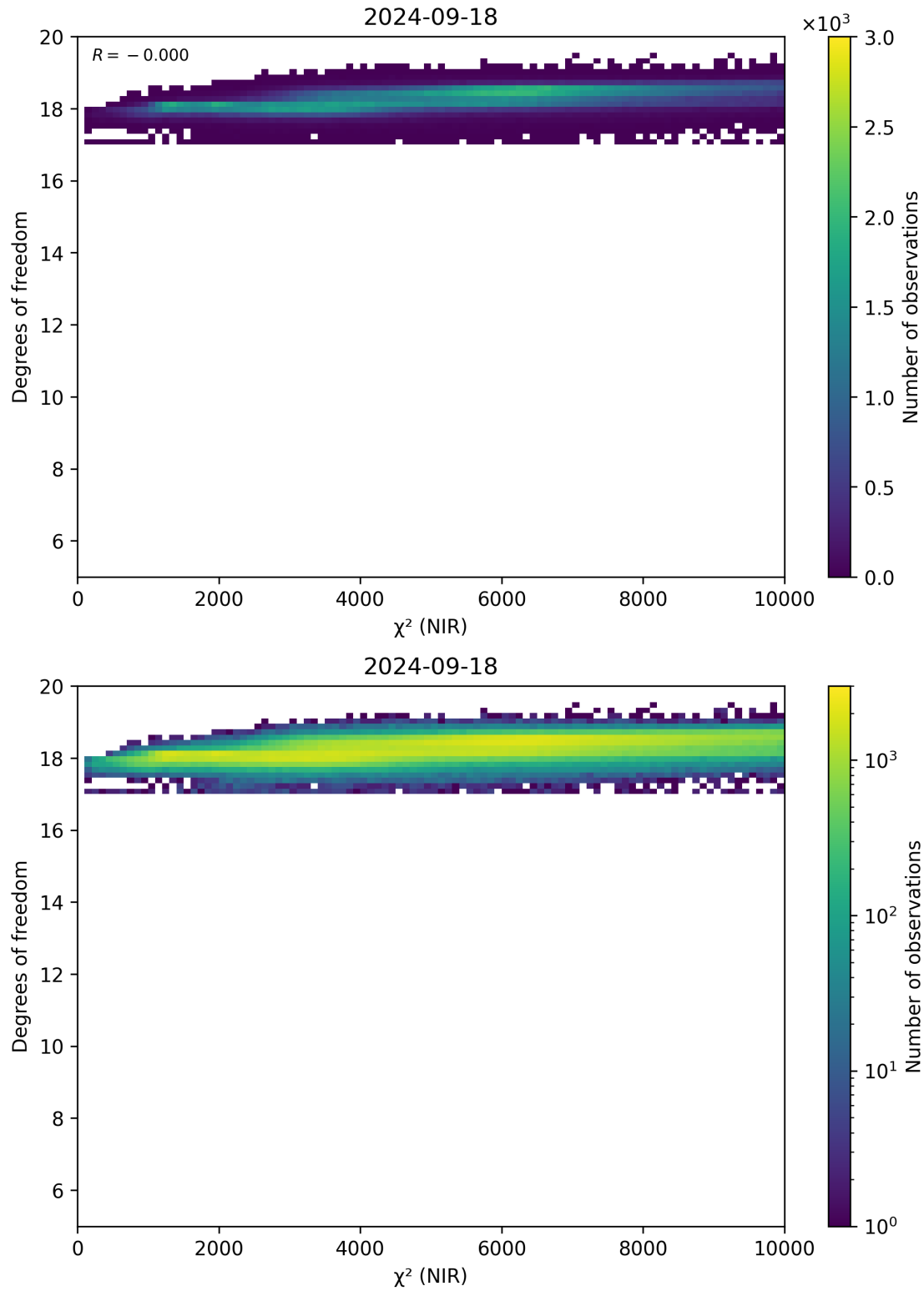
Figure 44: Scatter density plot of “ \chi^2 (NIR)” against “Degrees of freedom” for 2024-09-17 to 2024-09-19.
