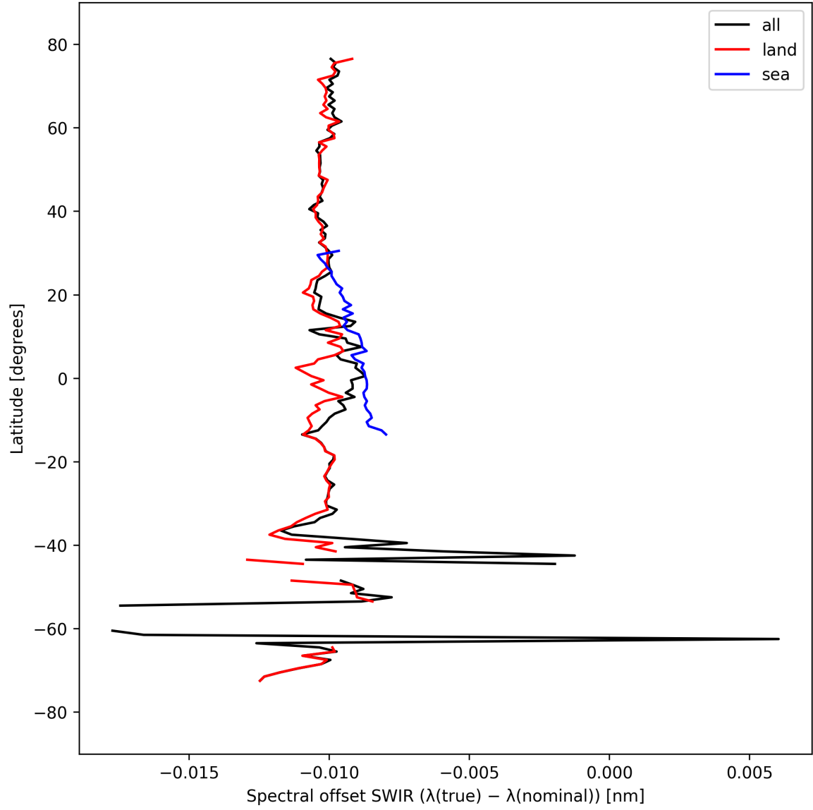
Figure 16: Zonal average of “Spectral offset SWIR ( \lambda_{\text{true}} - \lambda_{\text{nominal}} )” for 2024-09-17 to 2024-09-19.
