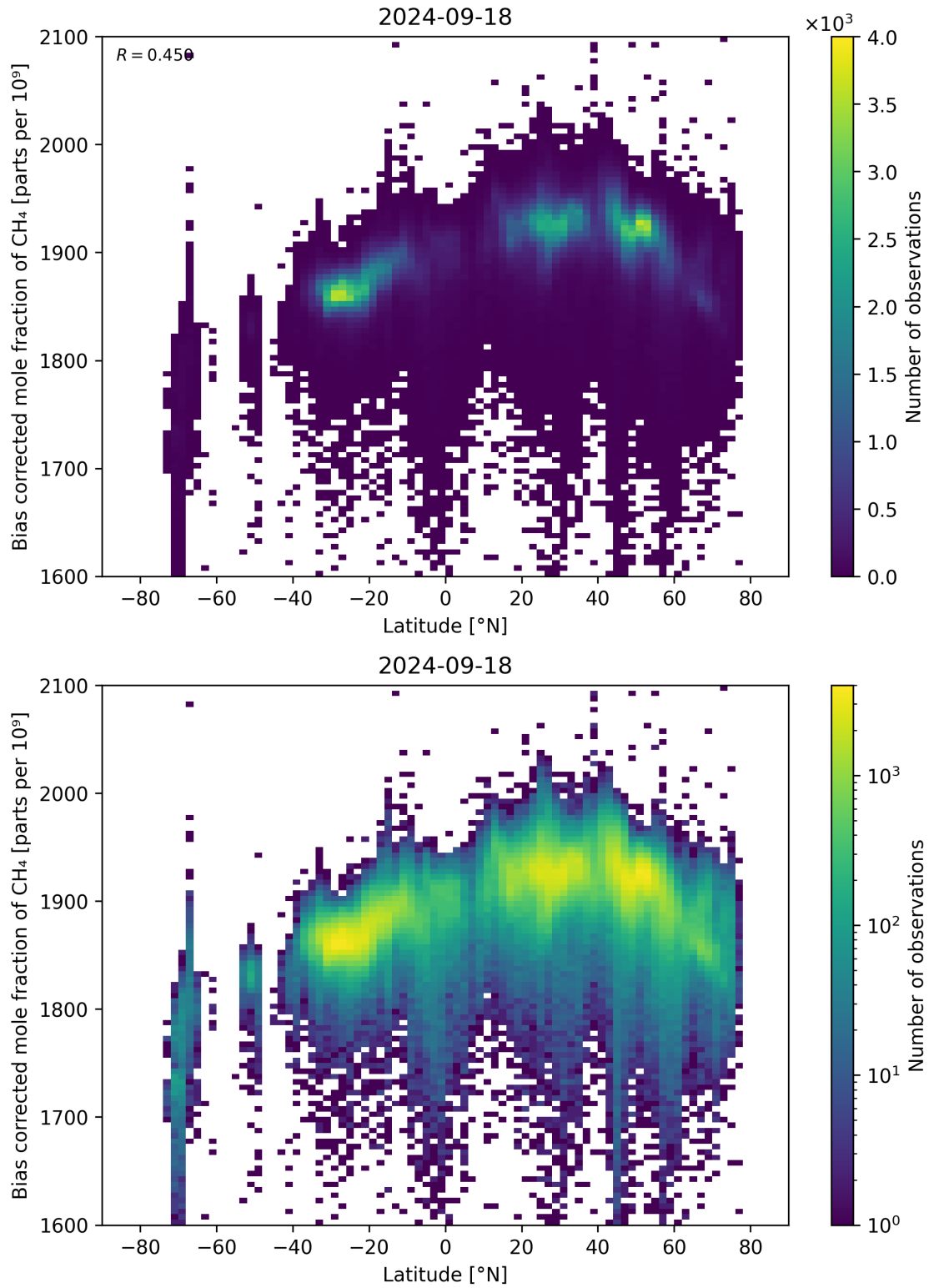
Figure 58: Scatter density plot of “Latitude” against “Bias corrected mole fraction of \text{CH}_4 ” for 2024-09-17 to 2024-09-19.
