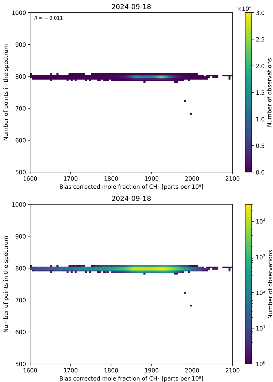
Figure 68: Scatter density plot of “Bias corrected mole fraction of CH 4 ” against “Number of points in the spectrum” for 2024-09-17 to 2024-09-19.
