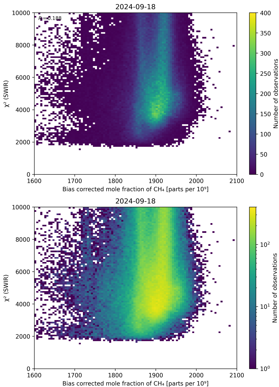
Figure 64: Scatter density plot of “Bias corrected mole fraction of \text{CH}_4 ” against “ \chi^2 (SWIR)” for 2024-09-17 to 2024-09-19.
