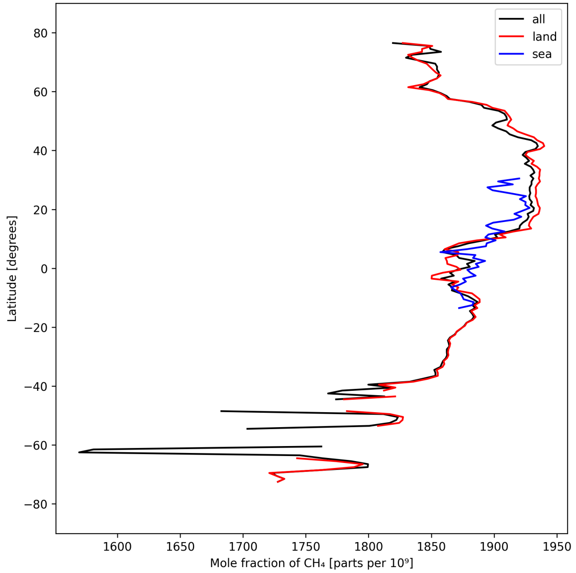
Figure 12: Zonal average of “Mole fraction of CH 4 ” for 2024-09-17 to 2024-09-19.
