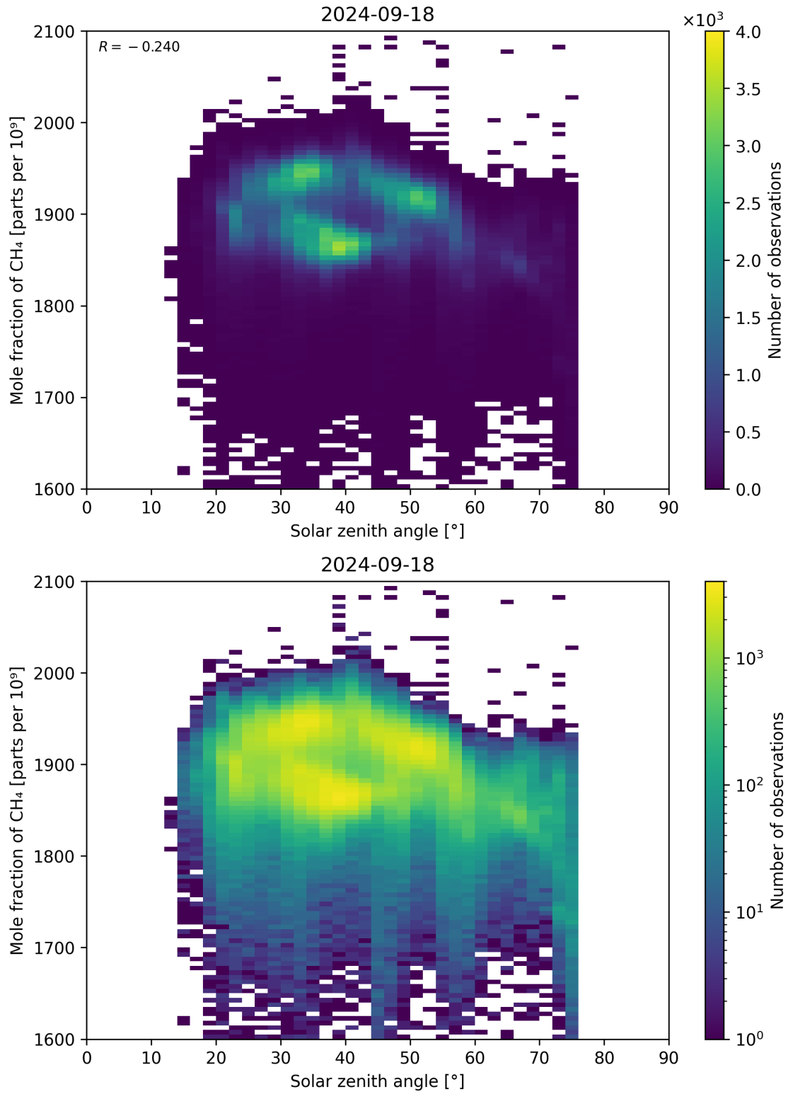
Figure 99: Scatter density plot of “Solar zenith angle” against “Mole fraction of CH 4 ” for 2024-09-17 to 2024-09-19.
