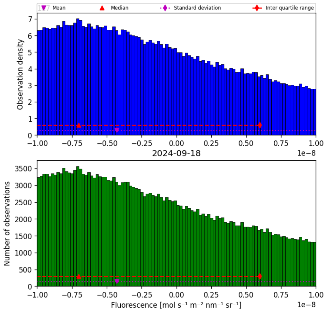
Figure 32: Histogram of “Fluorescence” for 2024-09-17 to 2024-09-19
