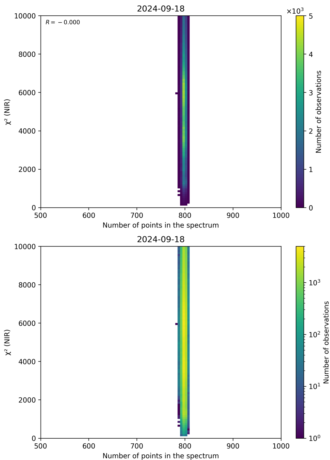
Figure 88: Scatter density plot of “Number of points in the spectrum” against “ \chi^2 (NIR)” for 2024-09-17 to 2024-09-19.
