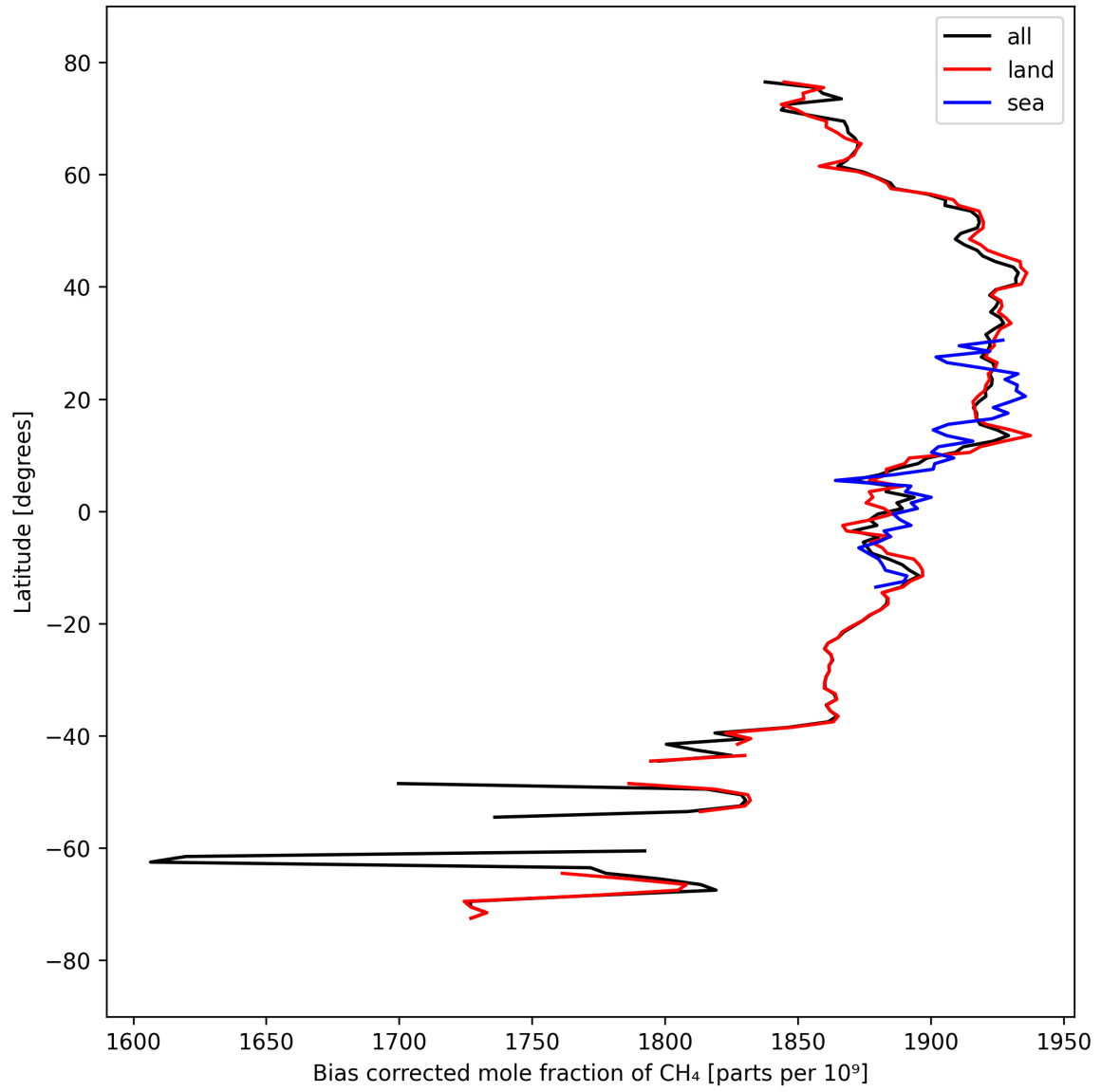
Figure 14: Zonal average of “Bias corrected mole fraction of CH 4 ” for 2024-09-17 to 2024-09-19.
