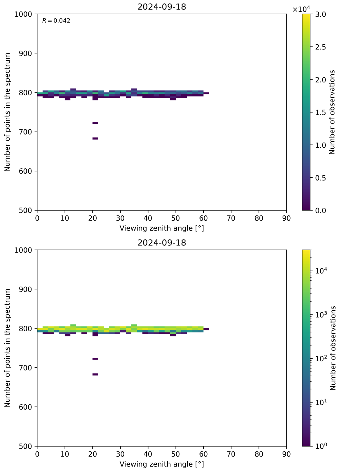
Figure 114: Scatter density plot of “Viewing zenith angle” against “Number of points in the spectrum” for 2024-09-17 to 2024-09-19.
