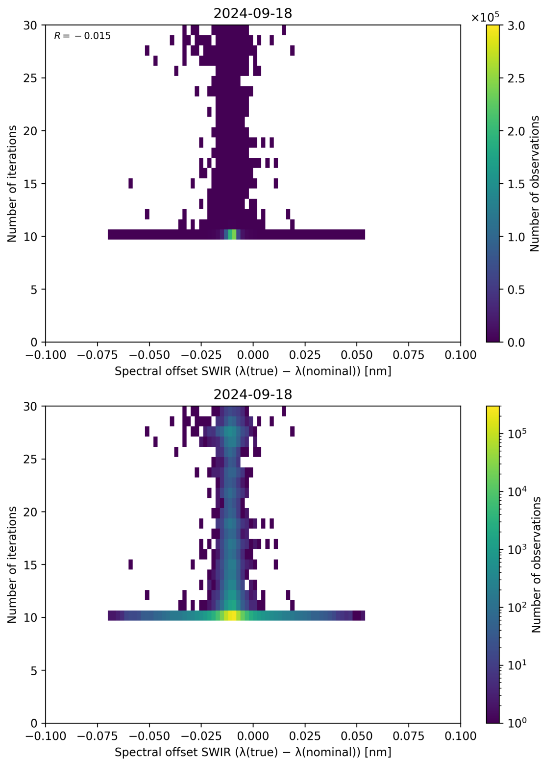
Figure 121: Scatter density plot of “Spectral offset SWIR ( \lambda_{\text{true}} - \lambda_{\text{nominal}} )” against “Number of iterations” for 2024-09-17 to 2024-09-19.
