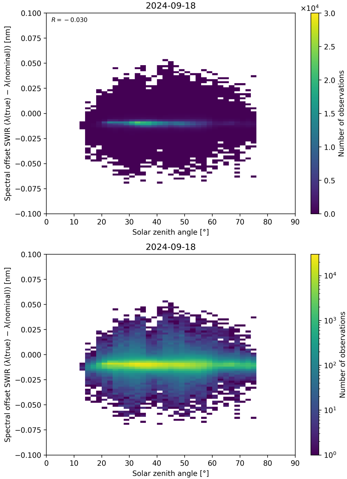
Figure 104: Scatter density plot of “Solar zenith angle” against “Spectral offset SWIR ( \lambda_{\text{true}} - \lambda_{\text{nominal}} )” for 2024-09-17 to 2024-09-19.
