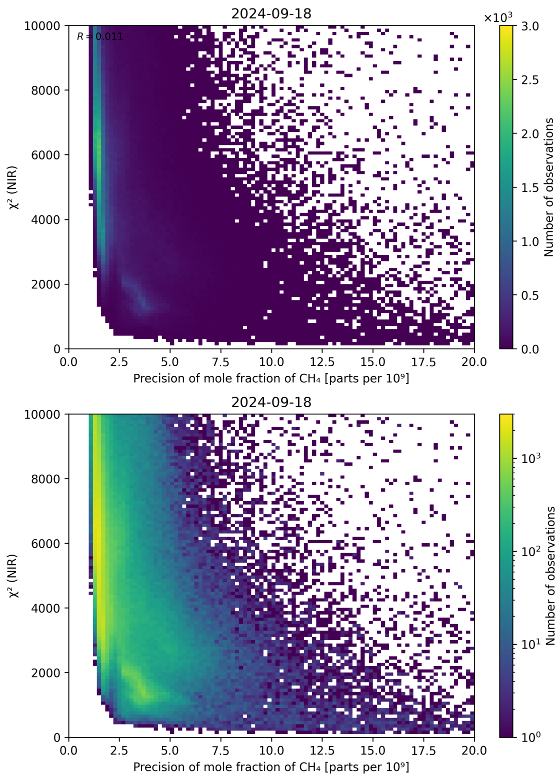
Figure 78: Scatter density plot of “Precision of mole fraction of \text{CH}_4 ” against “ \chi^2 (NIR)” for 2024-09-17 to 2024-09-19.
