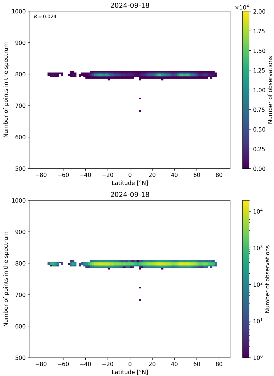
Figure 61: Scatter density plot of “Latitude” against “Number of points in the spectrum” for 2024-09-17 to 2024-09-19.
