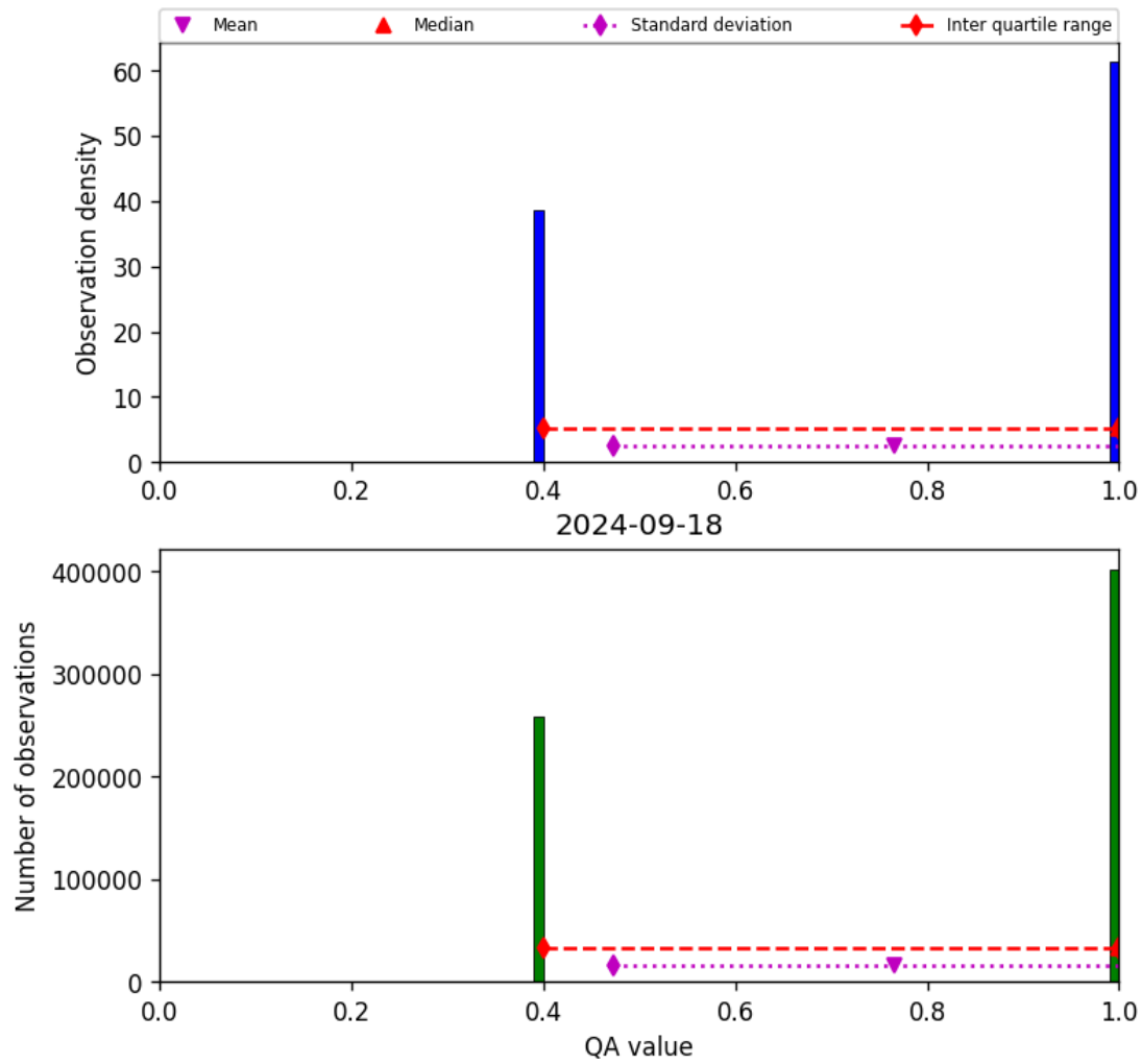
Figure 22: Histogram of “QA value” for 2024-09-17 to 2024-09-19
