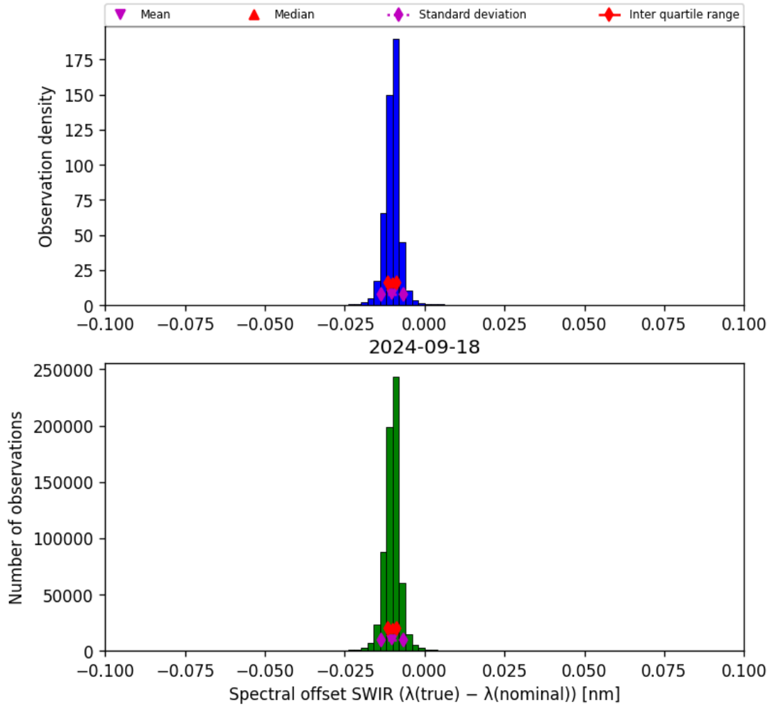
Figure 27: Histogram of “Spectral offset SWIR ( \lambda_{\text{true}} - \lambda_{\text{nominal}} )” for 2024-09-17 to 2024-09-19
