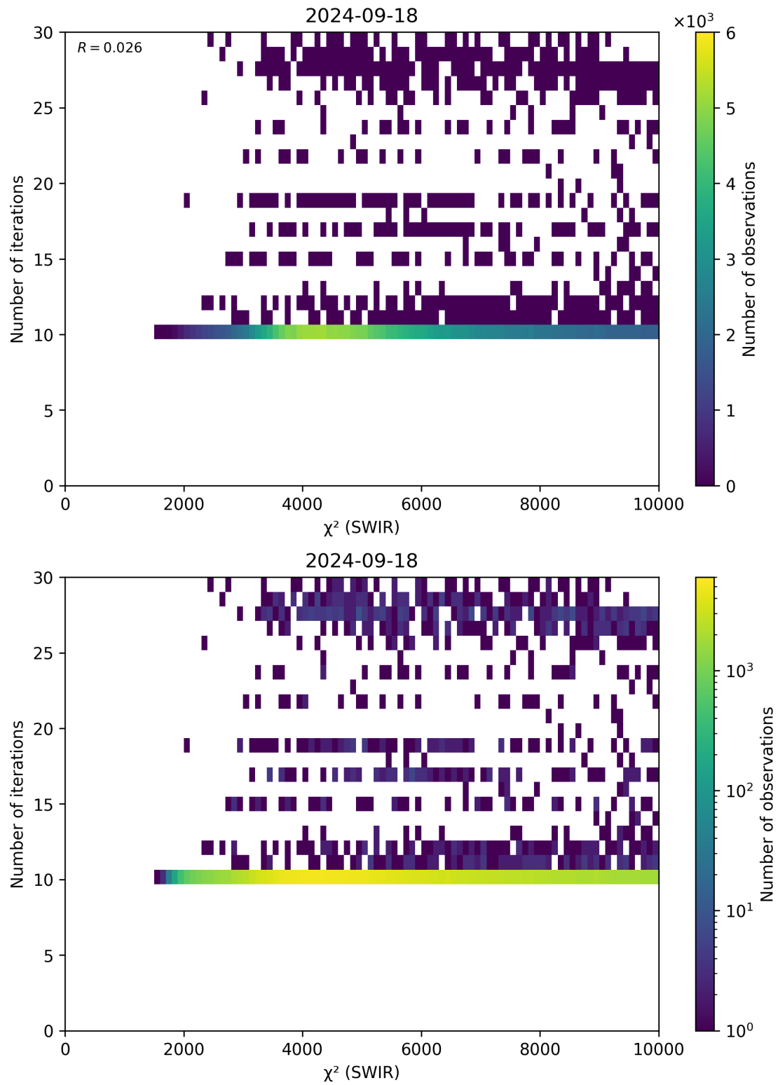
Figure 50: Scatter density plot of “ \chi^2 (SWIR)” against “Number of iterations” for 2024-09-17 to 2024-09-19.
