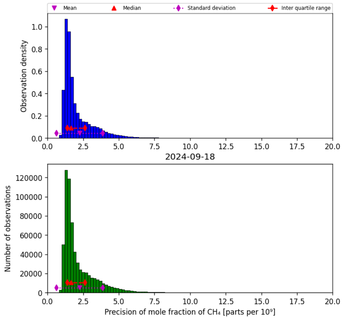
Figure 24: Histogram of “Precision of mole fraction of CH 4 ” for 2024-09-17 to 2024-09-19
