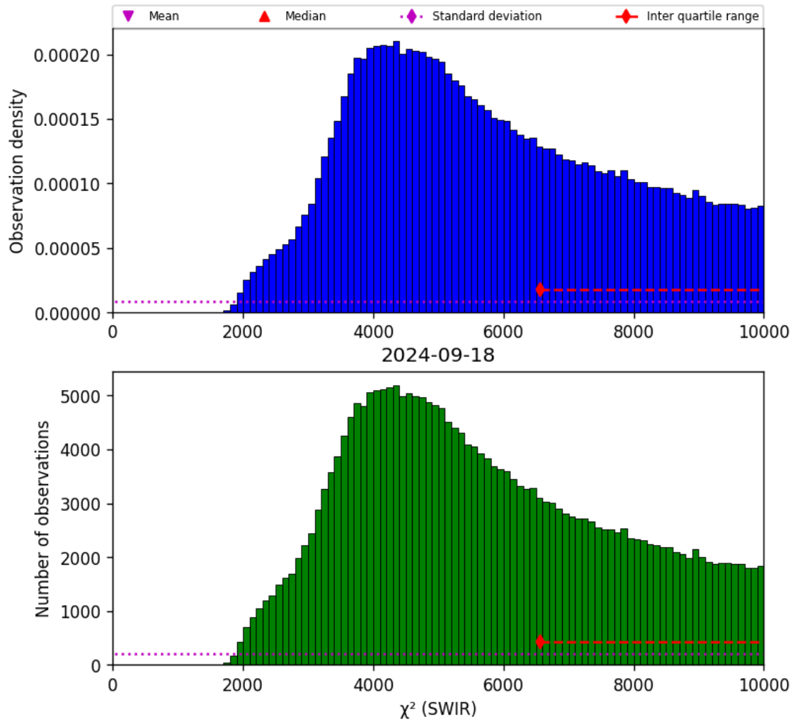
Figure 28: Histogram of “ \chi^2 (SWIR)” for 2024-09-17 to 2024-09-19
