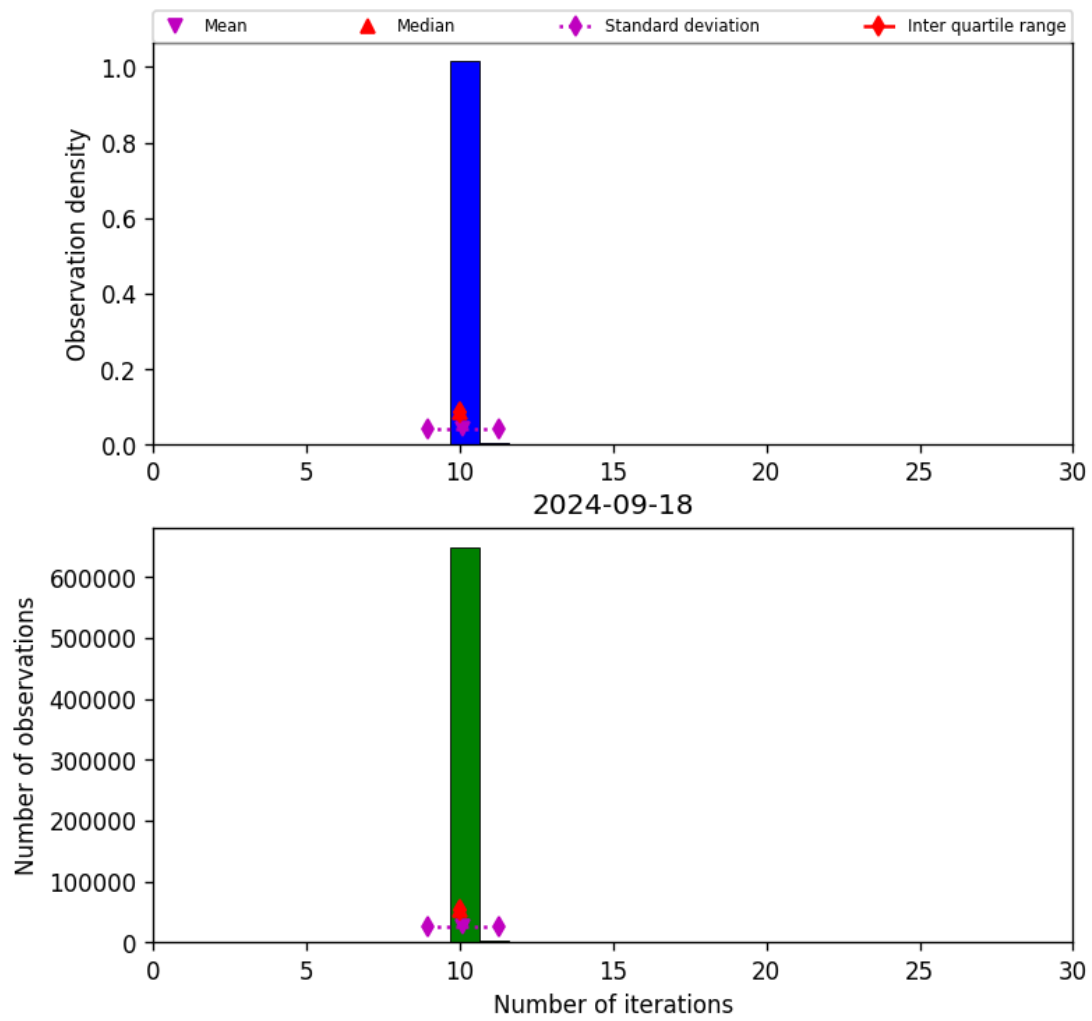
Figure 31: Histogram of “Number of iterations” for 2024-09-17 to 2024-09-19
