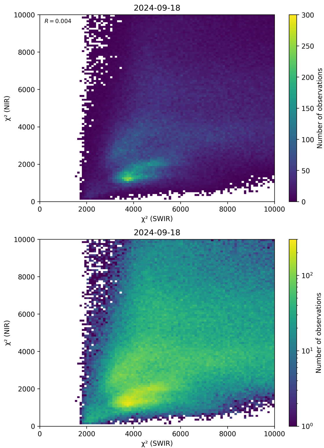
Figure 47: Scatter density plot of “ \chi^2 (SWIR)” against “ \chi^2 (NIR)” for 2024-09-17 to 2024-09-19.
