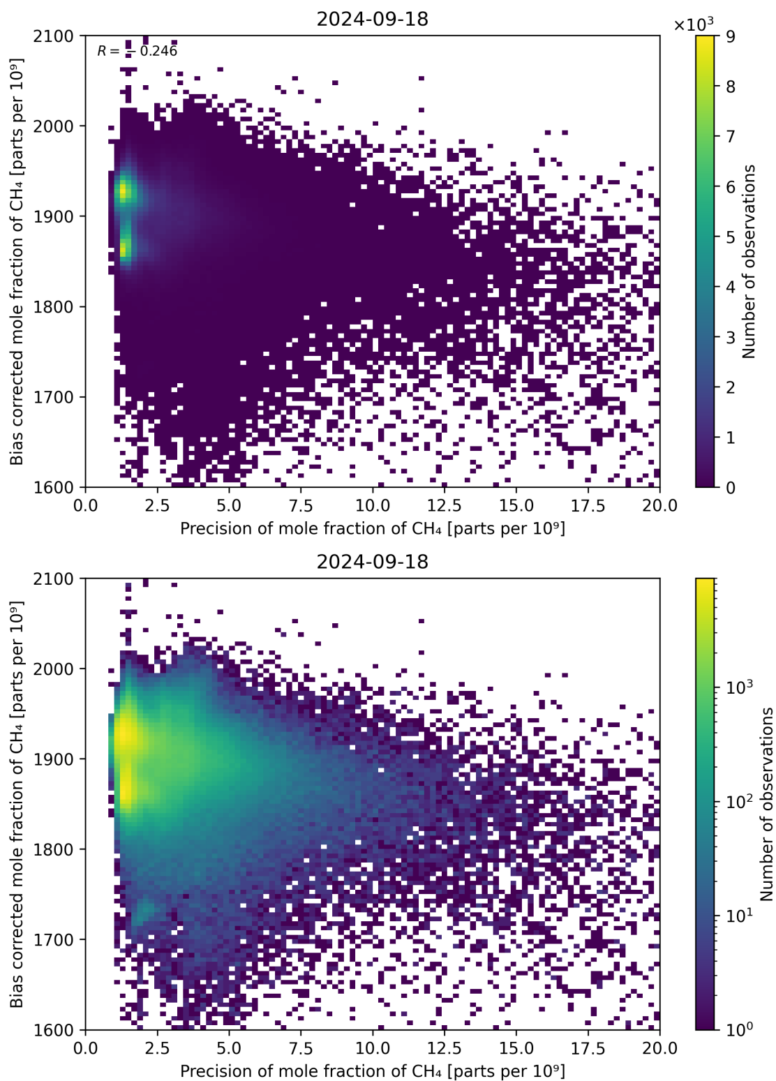
Figure 82: Scatter density plot of “Precision of mole fraction of CH 4 ” against “Bias corrected mole fraction of CH 4 ” for 2024-09-17 to 2024-09-19.
