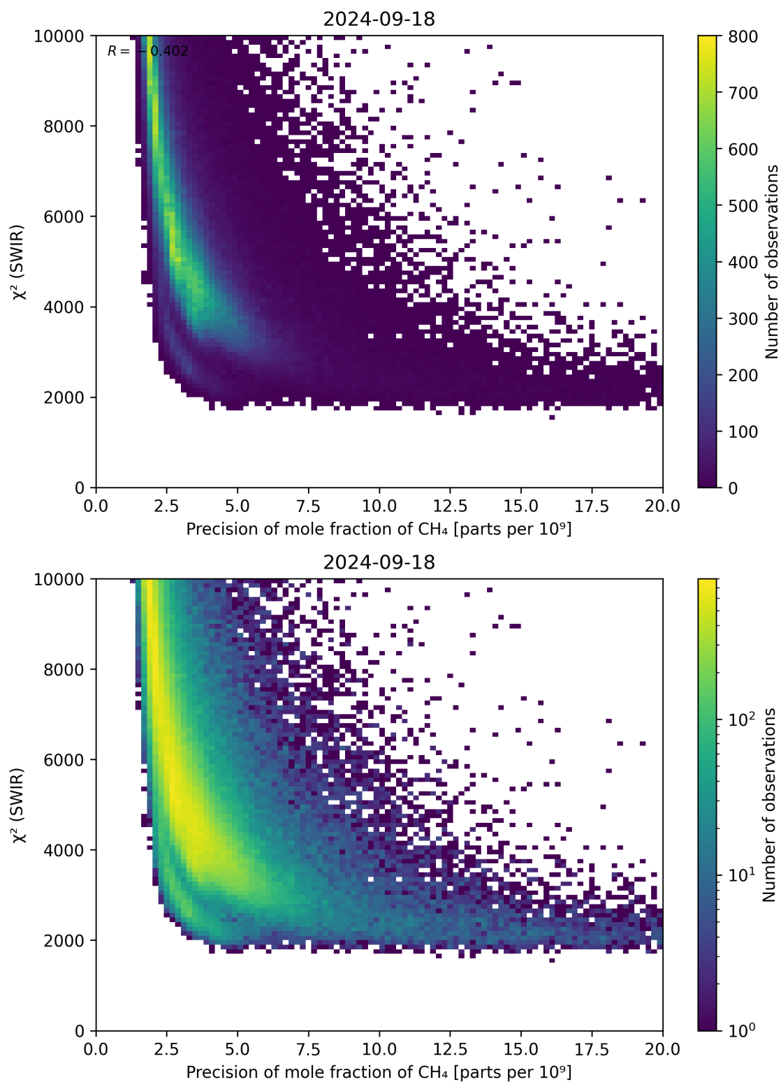
Figure 79: Scatter density plot of “Precision of mole fraction of \text{CH}_4 ” against “ \chi^2 (SWIR)” for 2024-09-17 to 2024-09-19.
