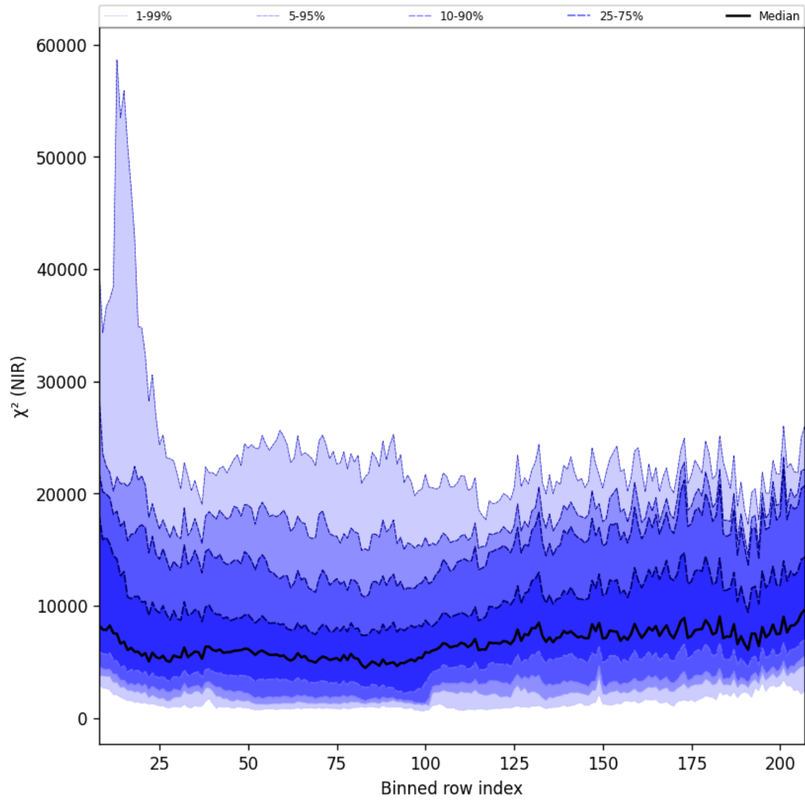
Figure 40: Along track statistics of “ \chi^2 (NIR)” for 2024-09-17 to 2024-09-19
