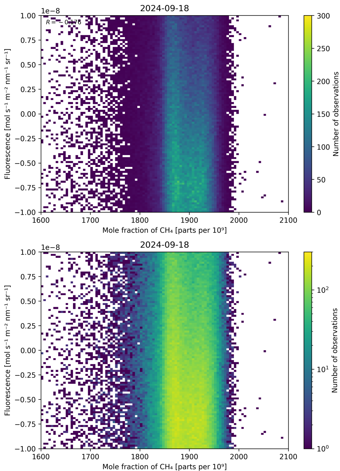
Figure 73: Scatter density plot of “Mole fraction of \text{CH}_4 ” against “Fluorescence” for 2024-09-17 to 2024-09-19.
