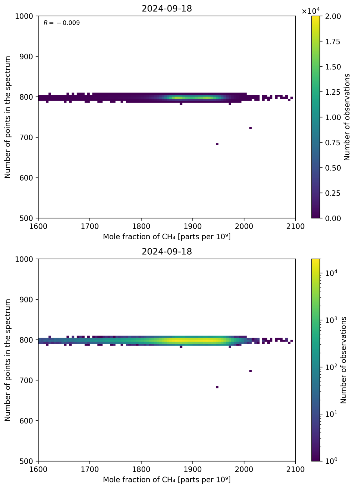
Figure 77: Scatter density plot of “Mole fraction of CH 4 ” against “Number of points in the spectrum” for 2024-09-17 to 2024-09-19.
