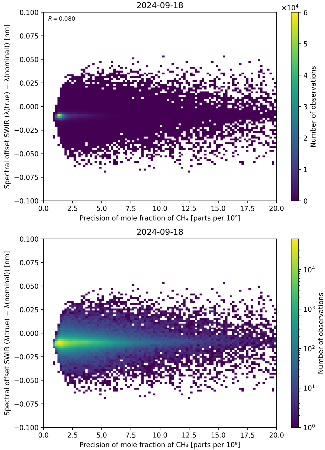
Figure 85: Scatter density plot of “Precision of mole fraction of \text{CH}_4 ” against “Spectral offset SWIR ( \lambda_{\text{true}} - \lambda_{\text{nominal}} )” for 2024-09-17 to 2024-09-19.
