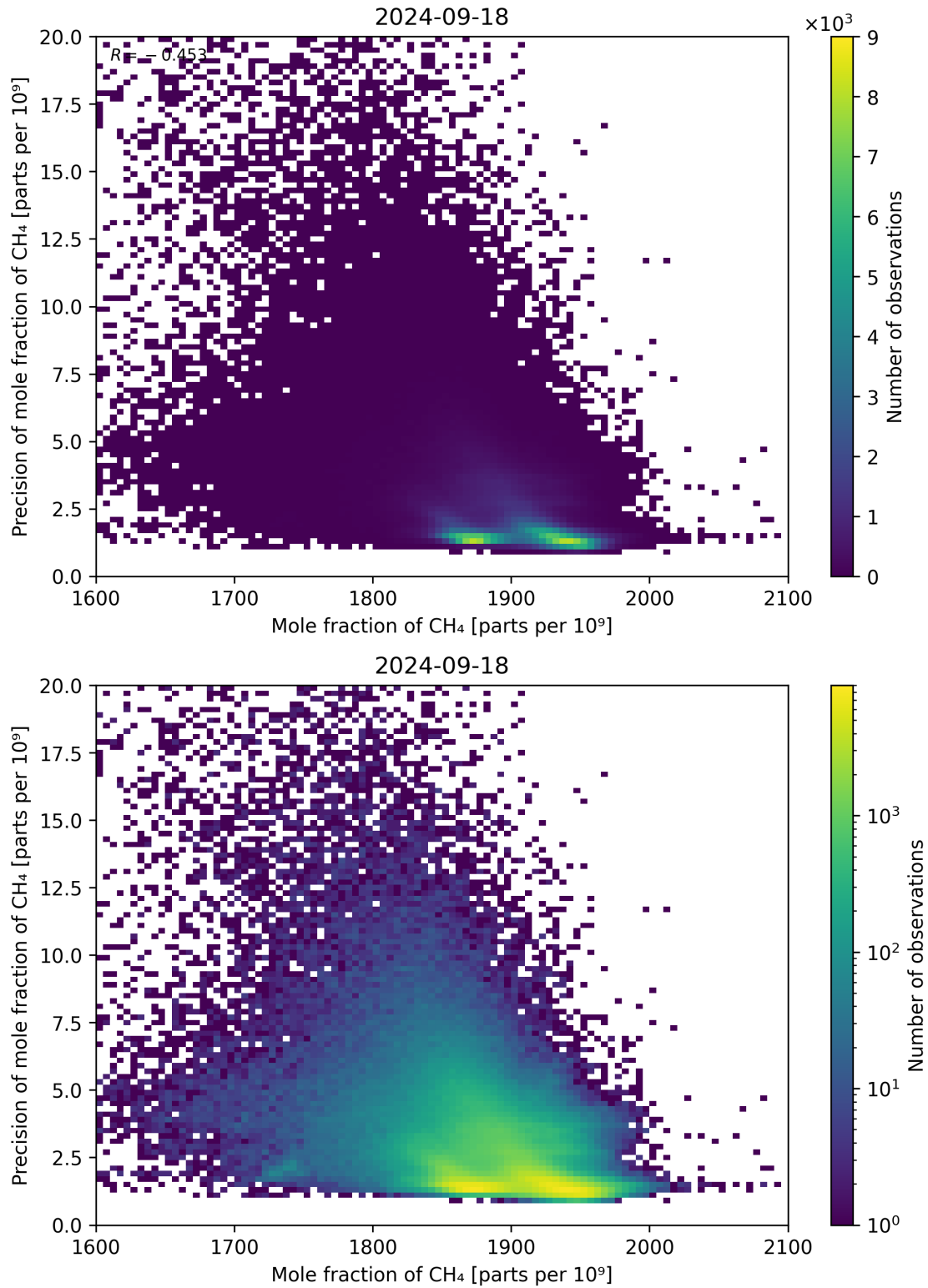
Figure 75: Scatter density plot of “Mole fraction of CH 4 ” against “Precision of mole fraction of CH 4 ” for 2024-09-17 to 2024-09-19.
