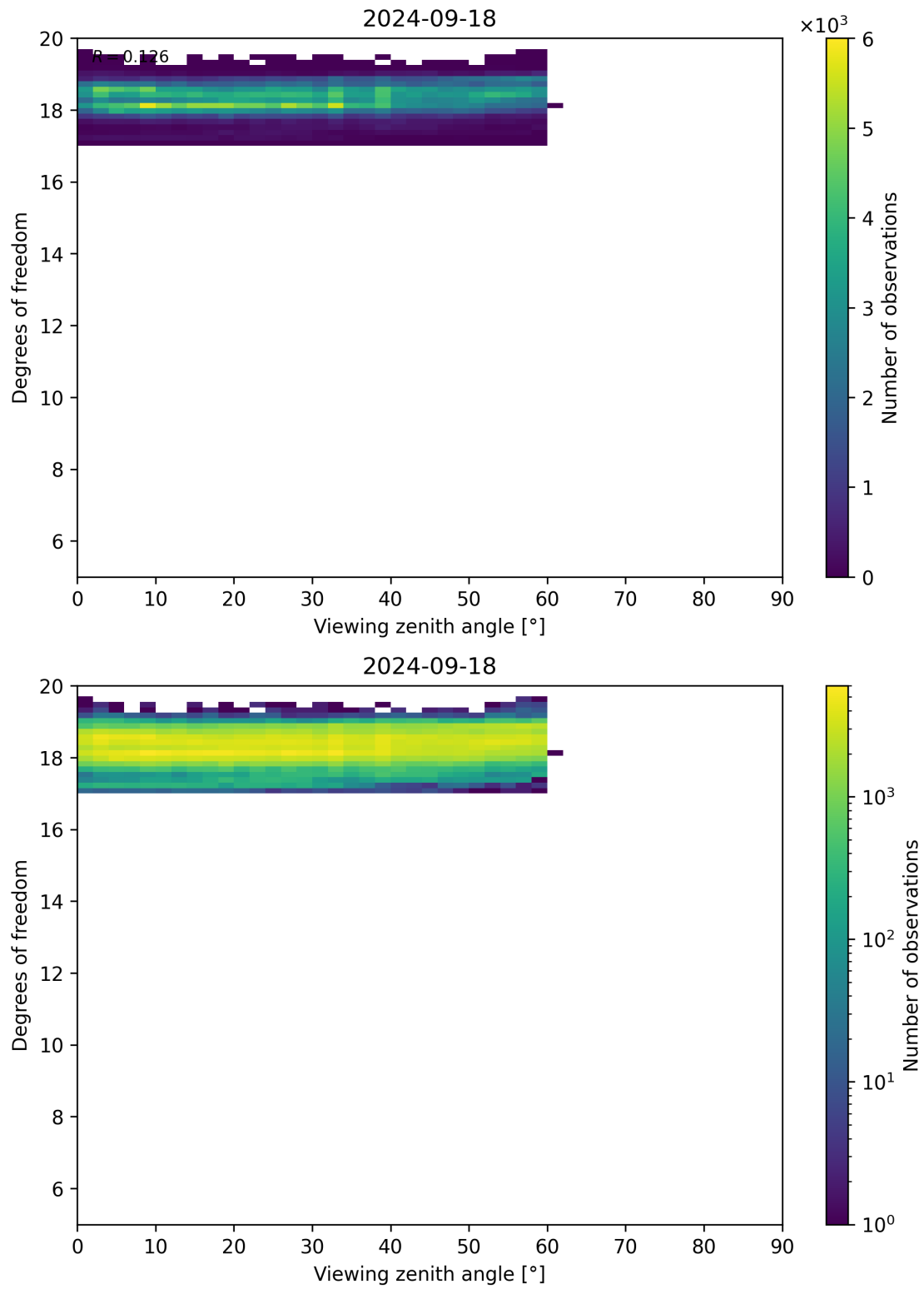
Figure 107: Scatter density plot of “Viewing zenith angle” against “Degrees of freedom” for 2024-09-17 to 2024-09-19.
