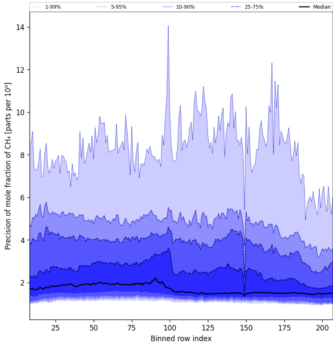
Figure 35: Along track statistics of “Precision of mole fraction of CH 4 ” for 2024-09-17 to 2024-09-19
