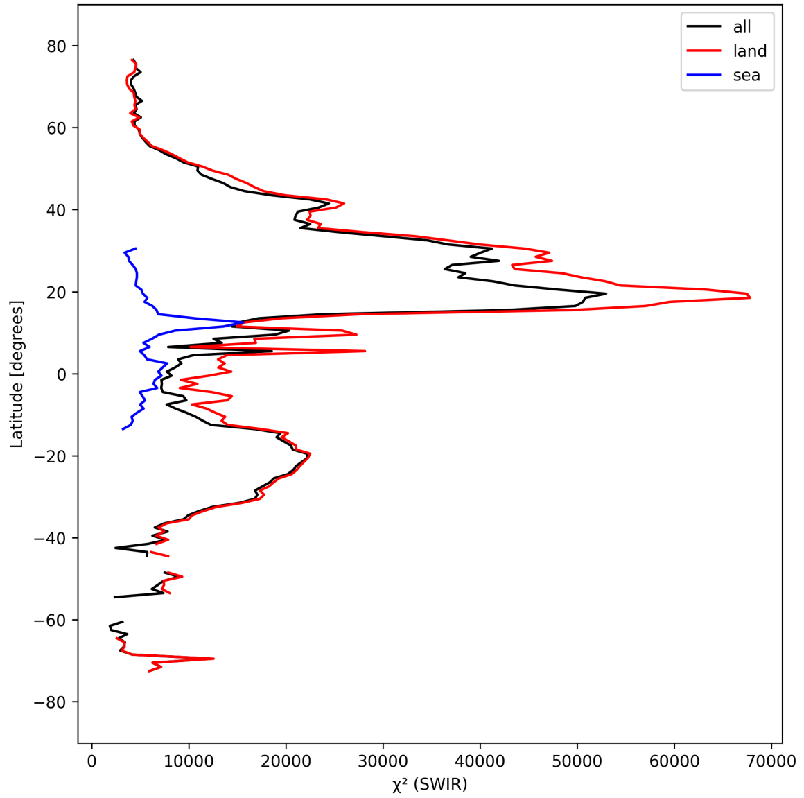
Figure 17: Zonal average of " \chi^2 (SWIR)" for 2024-09-17 to 2024-09-19.
