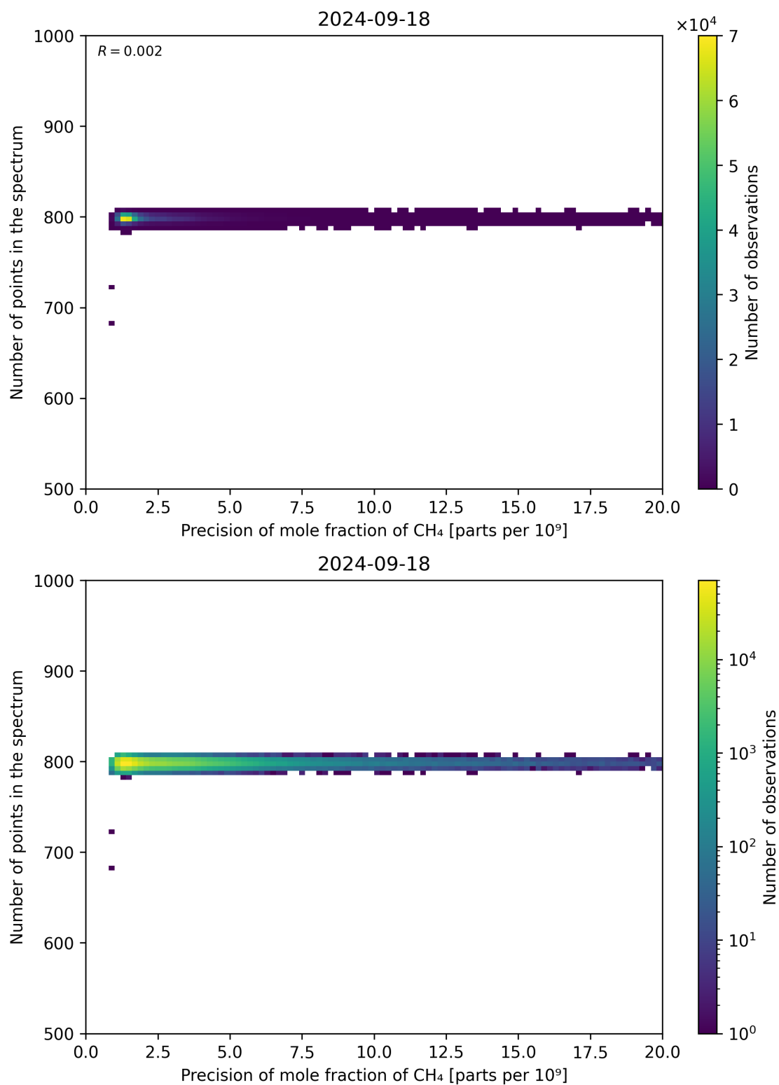
Figure 84: Scatter density plot of “Precision of mole fraction of CH 4 ” against “Number of points in the spectrum” for 2024-09-17 to 2024-09-19.
