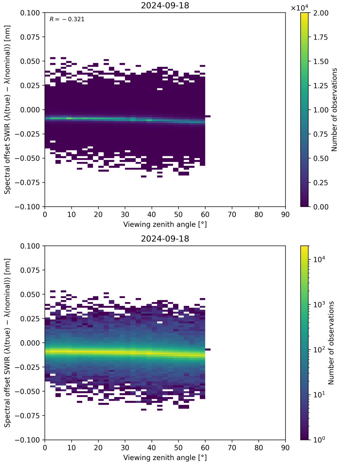
Figure 116: Scatter density plot of “Viewing zenith angle” against “Spectral offset SWIR ( \lambda_{\text{true}} - \lambda_{\text{nominal}} )” for 2024-09-17 to 2024-09-19.
