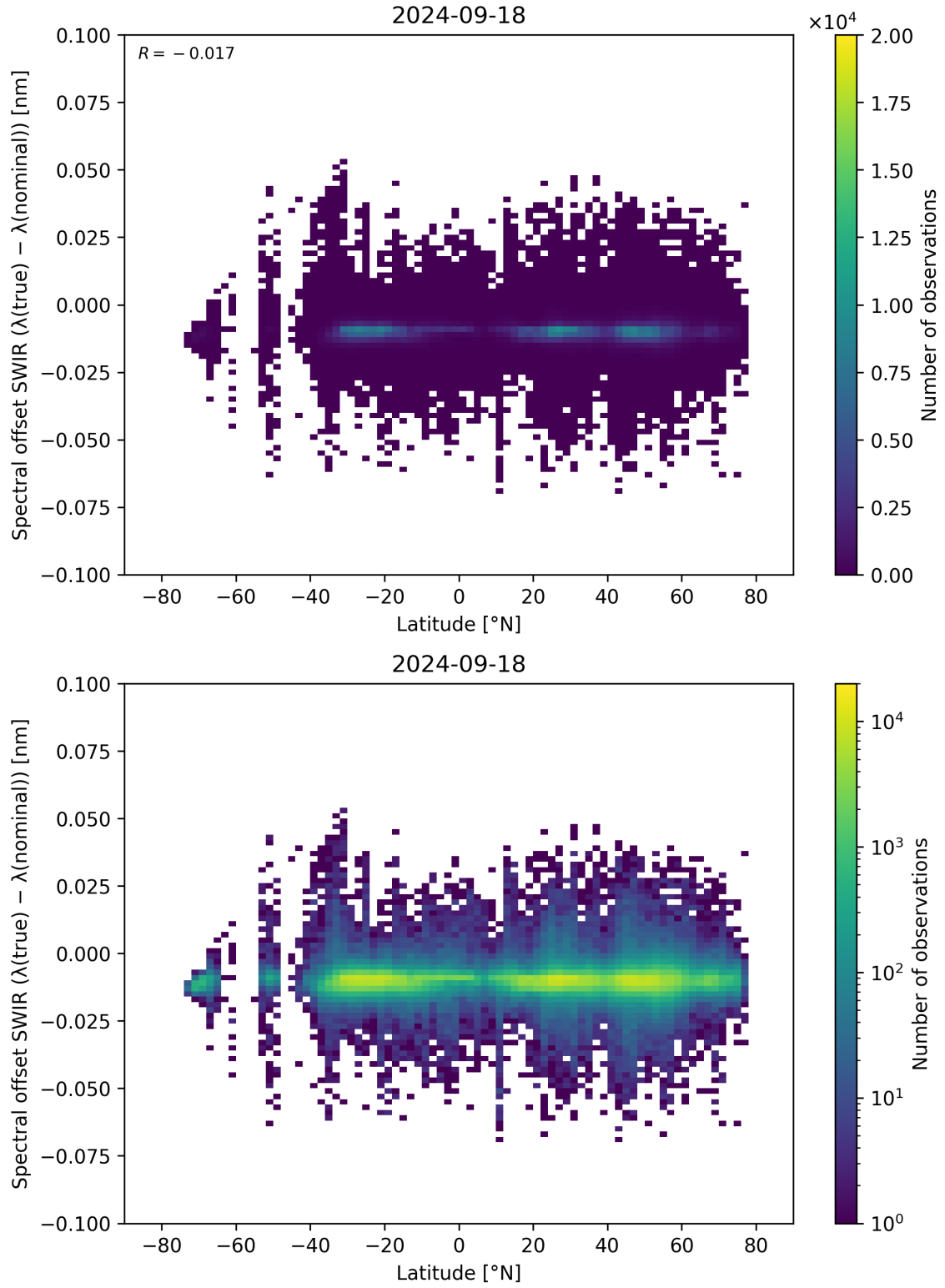
Figure 62: Scatter density plot of “Latitude” against “Spectral offset SWIR ( \lambda_{\text{true}} - \lambda_{\text{nominal}} )” for 2024-09-17 to 2024-09-19.
