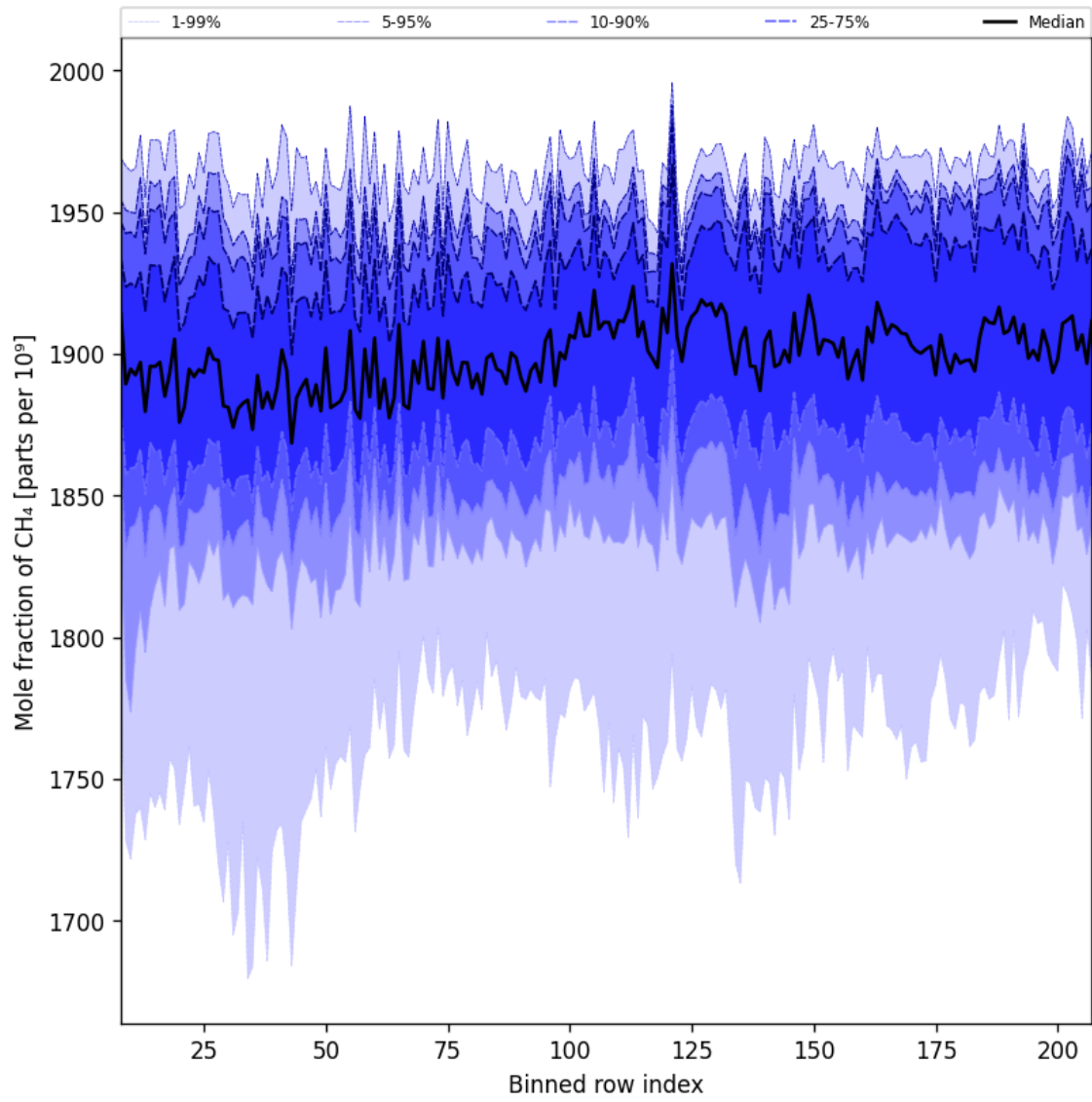
Figure 34: Along track statistics of “Mole fraction of CH 4 ” for 2024-09-17 to 2024-09-19
