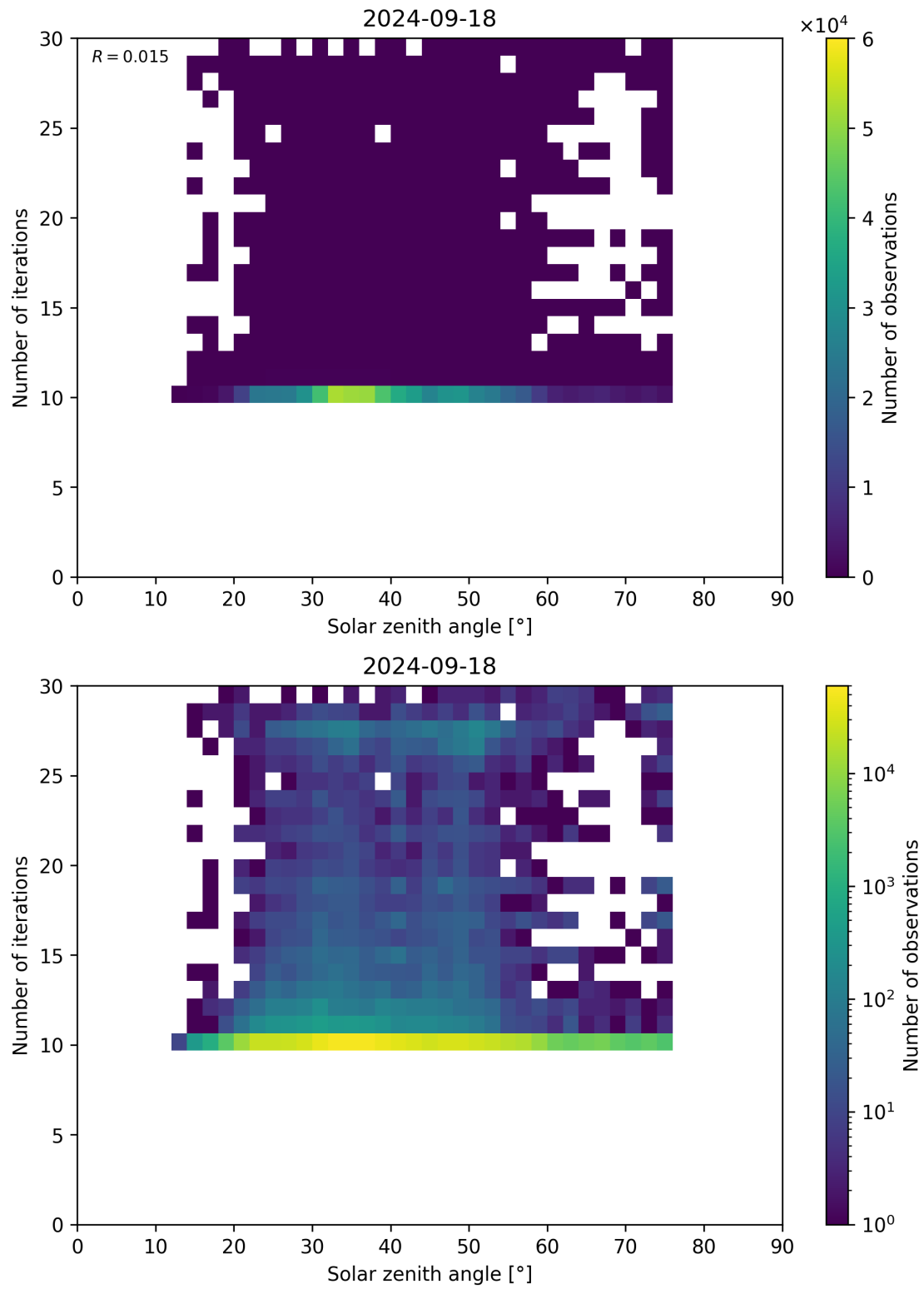
Figure 102: Scatter density plot of “Solar zenith angle” against “Number of iterations” for 2024-09-17 to 2024-09-19.
