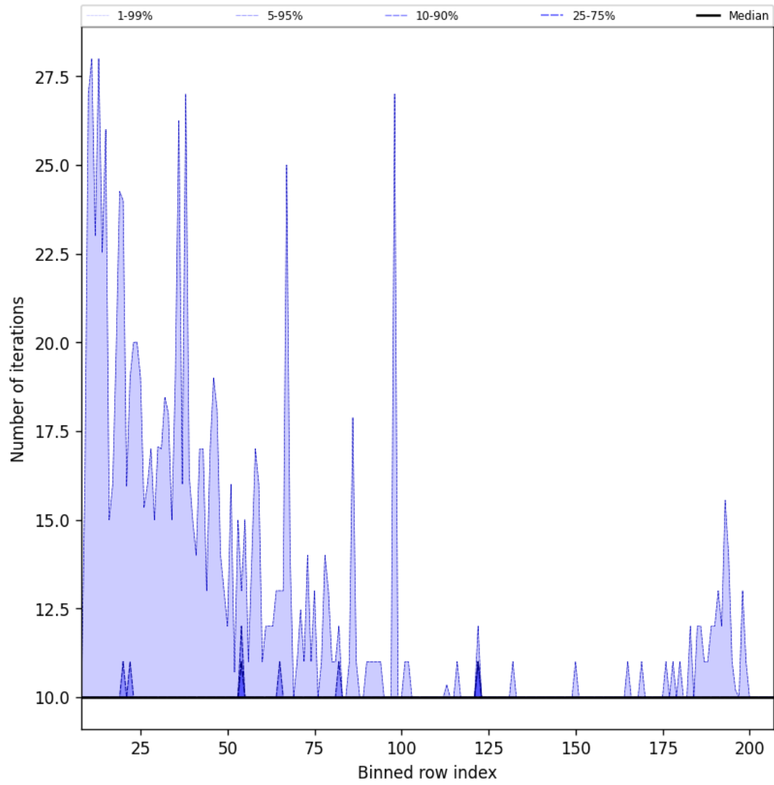
Figure 42: Along track statistics of “Number of iterations” for 2024-09-17 to 2024-09-19
