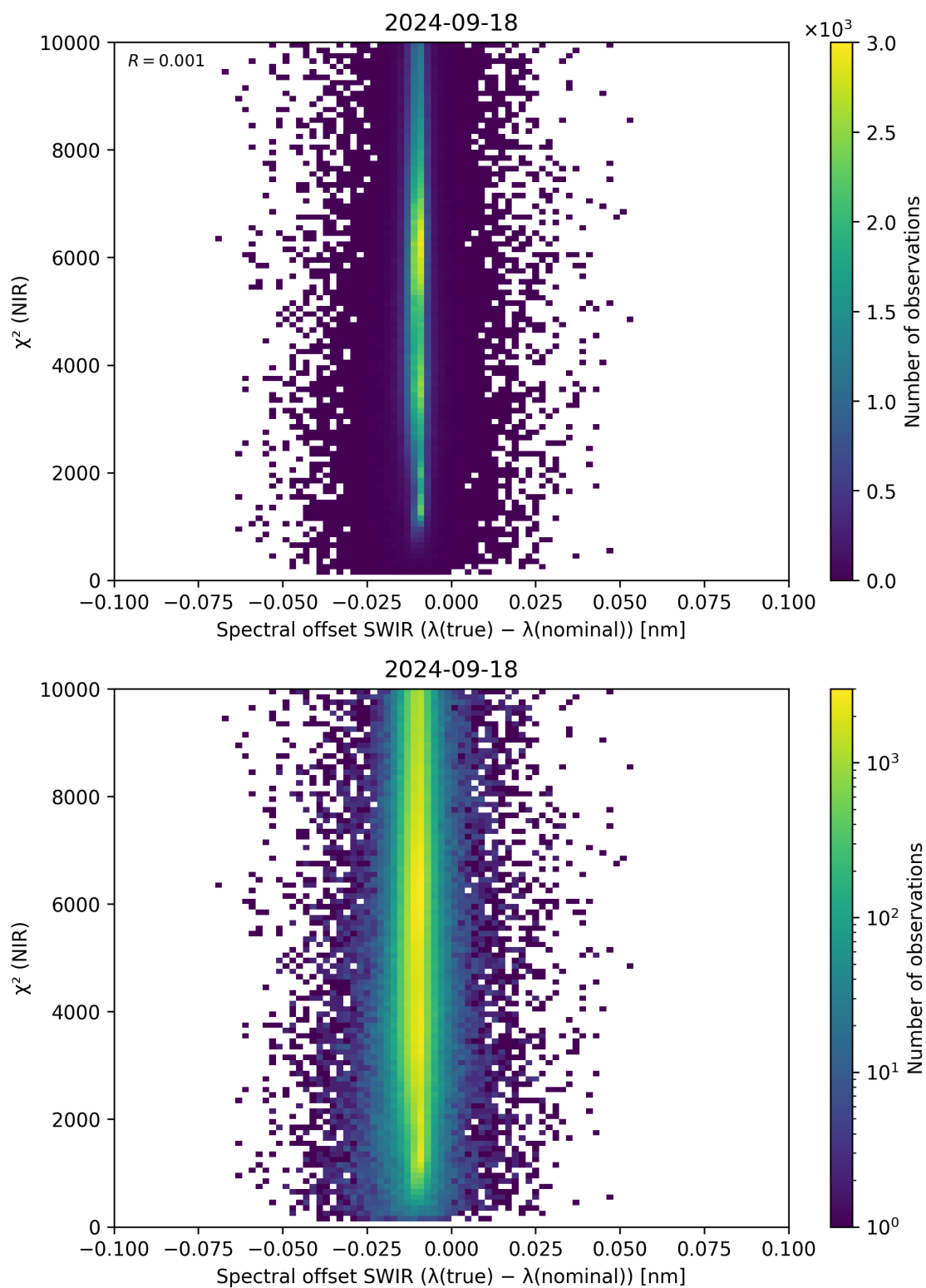
Figure 117: Scatter density plot of “Spectral offset SWIR ( \lambda_{\text{true}} - \lambda_{\text{nominal}} )” against “ \chi^2 (NIR)” for 2024-09-17 to 2024-09-19.
