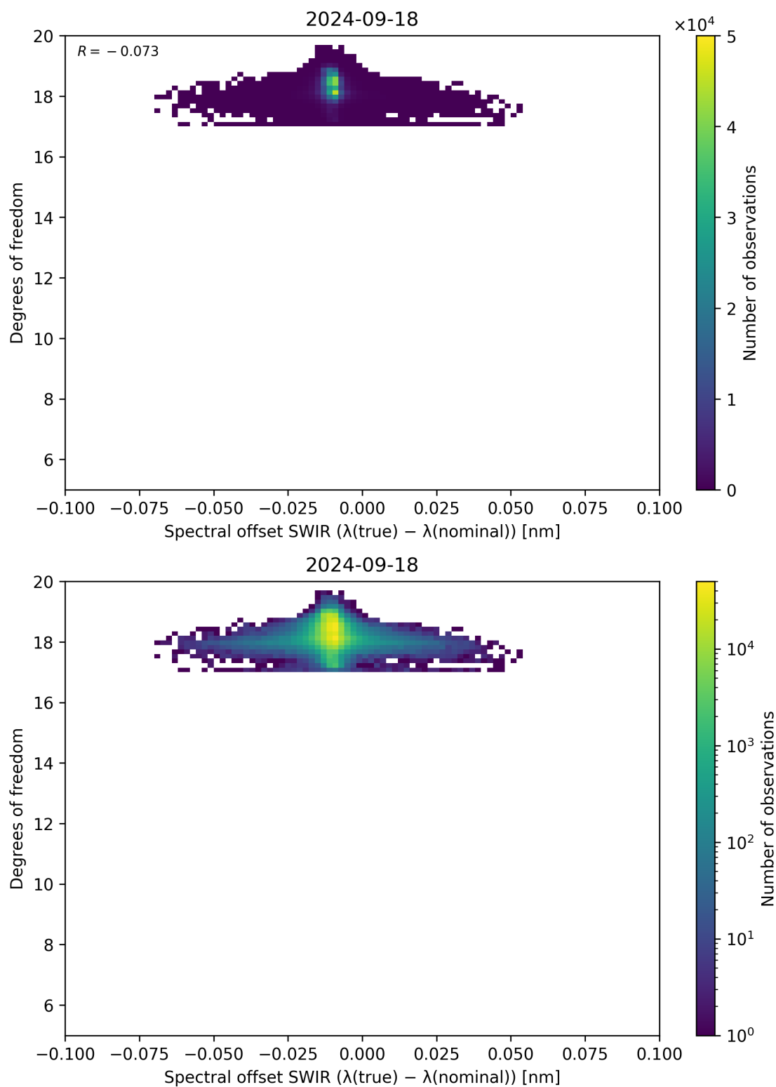
Figure 119: Scatter density plot of “Spectral offset SWIR ( \lambda_{\text{true}} - \lambda_{\text{nominal}} )” against “Degrees of freedom” for 2024-09-17 to 2024-09-19.
