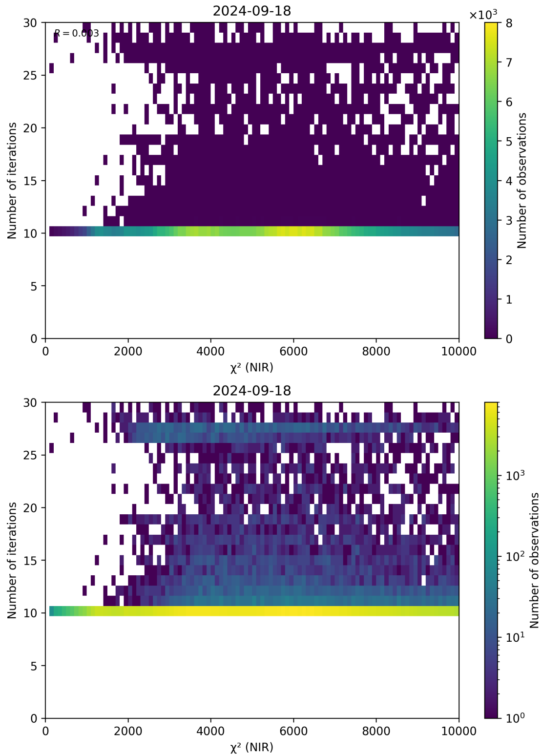
Figure 46: Scatter density plot of “ \chi^2 (NIR)” against “Number of iterations” for 2024-09-17 to 2024-09-19.
