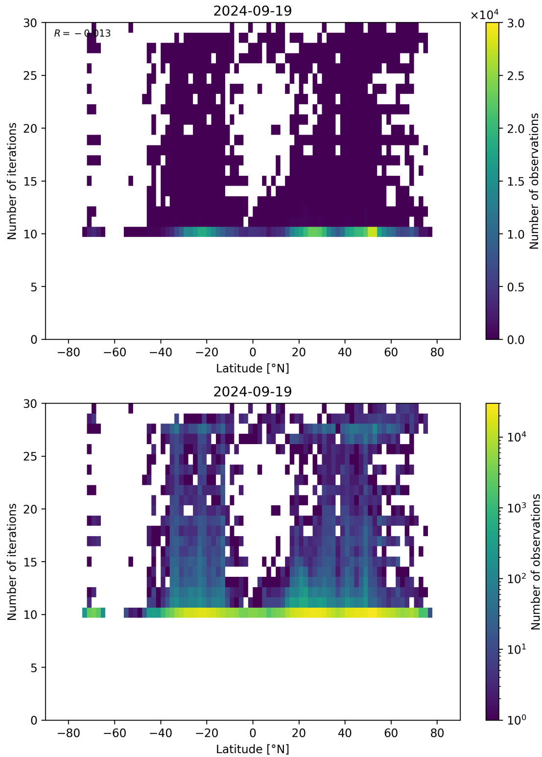
Figure 60: Scatter density plot of “Latitude” against “Number of iterations” for 2024-09-18 to 2024-09-20.
