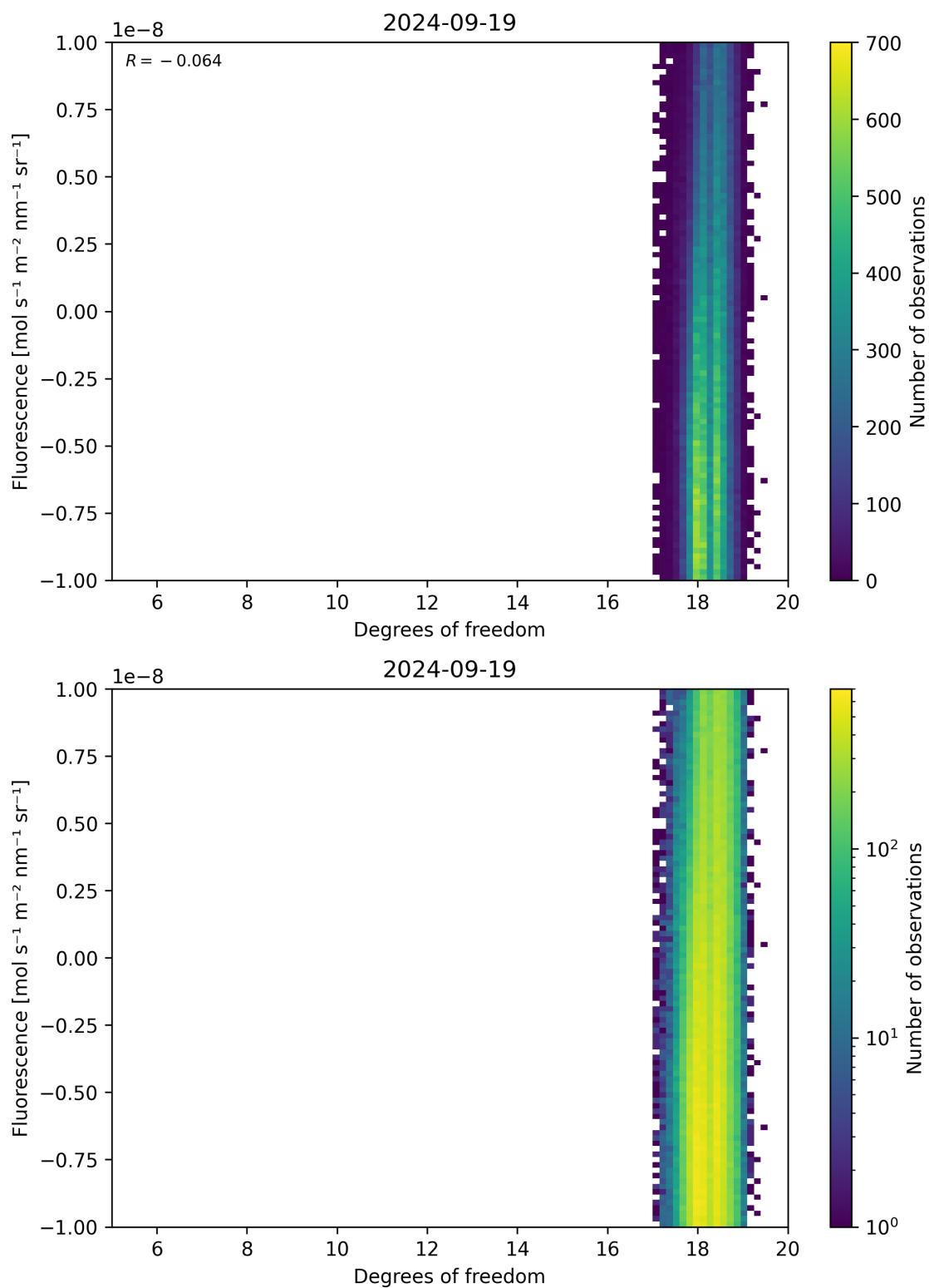
Figure 51: Scatter density plot of “Degrees of freedom” against “Fluorescence” for 2024-09-18 to 2024-09-20.
