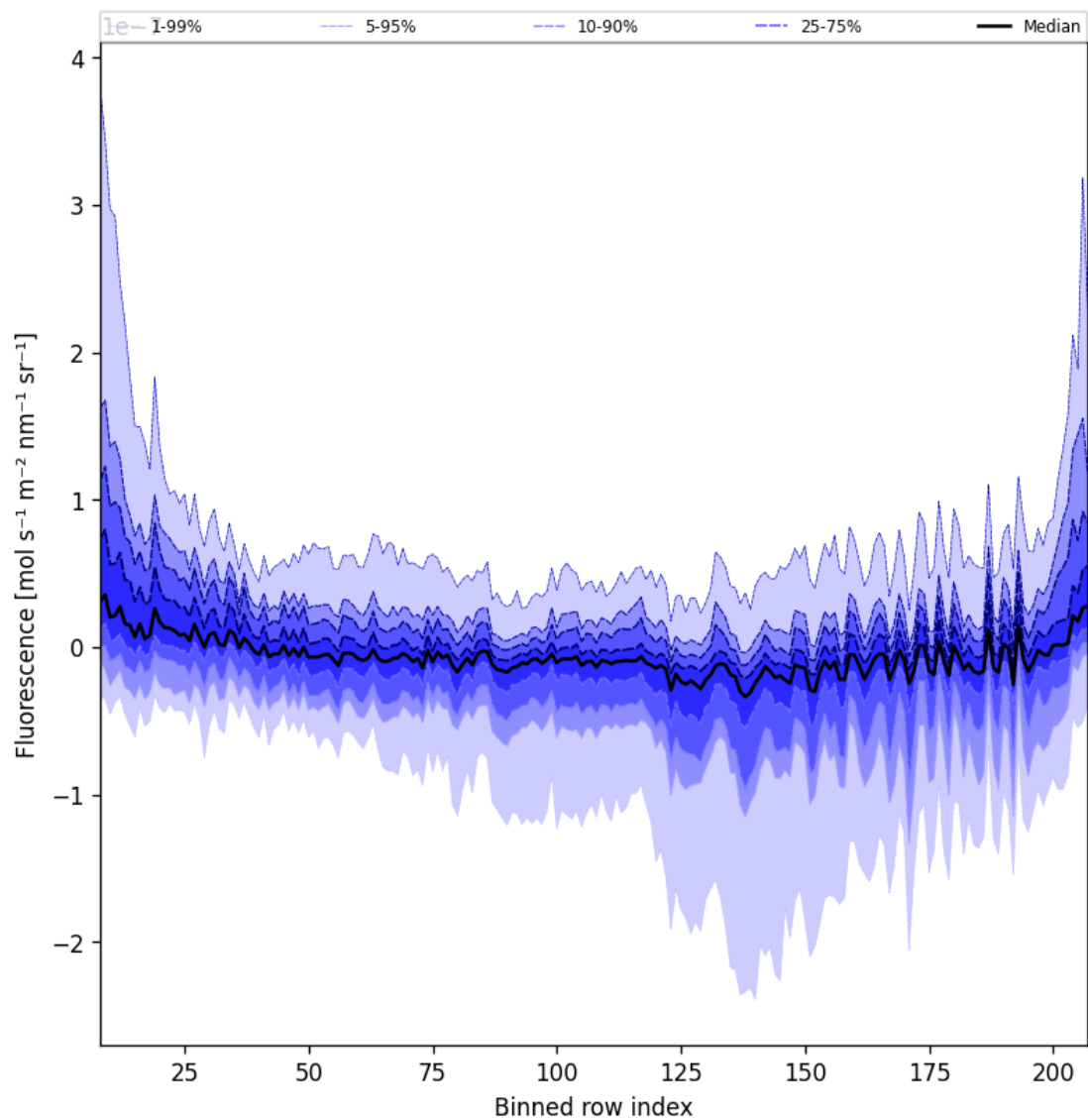
Figure 43: Along track statistics of “Fluorescence” for 2024-09-18 to 2024-09-20
