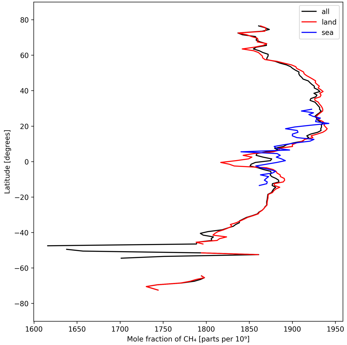
Figure 12: Zonal average of “Mole fraction of \text{CH}_4 ” for 2024-09-18 to 2024-09-20.
