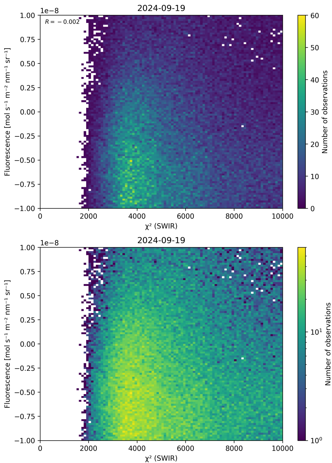
Figure 49: Scatter density plot of “ \chi^2 (SWIR)” against “Fluorescence” for 2024-09-18 to 2024-09-20.
