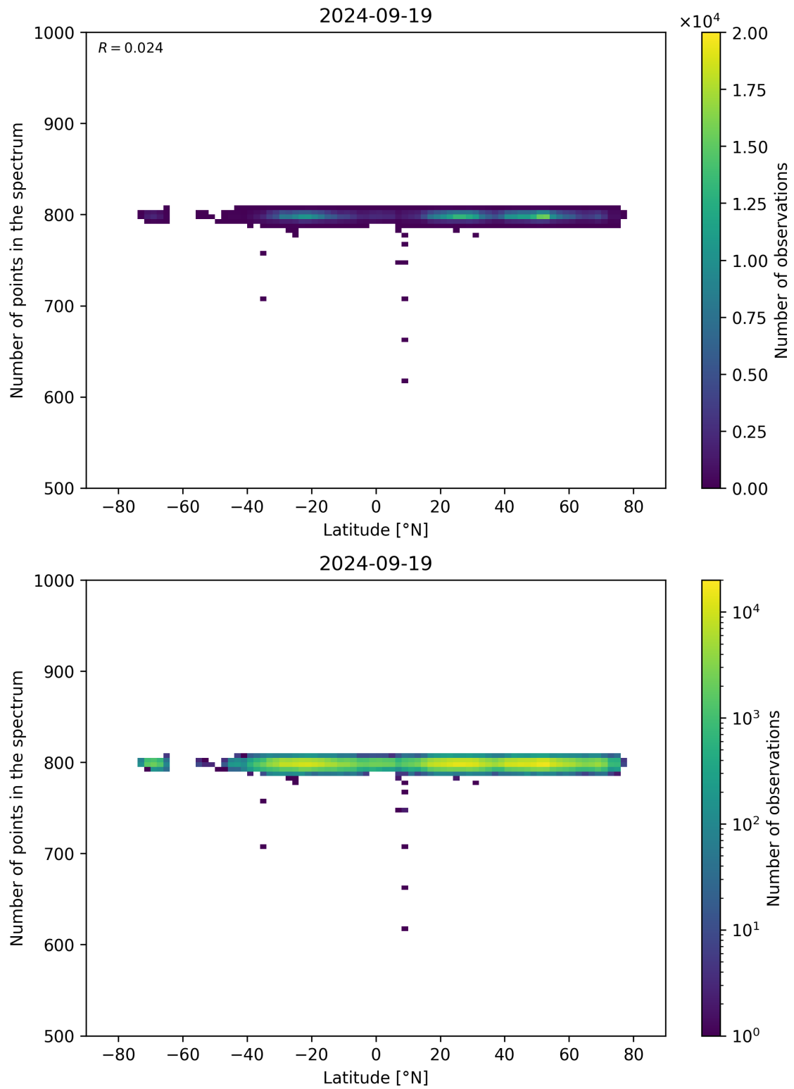
Figure 61: Scatter density plot of “Latitude” against “Number of points in the spectrum” for 2024-09-18 to 2024-09-20.
