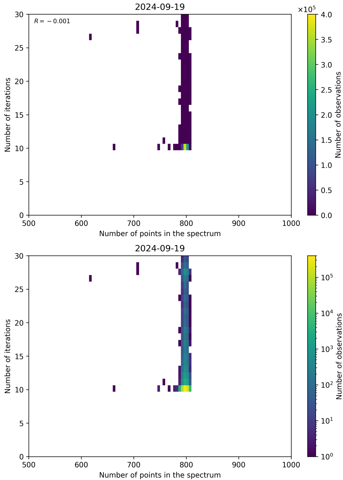
Figure 92: Scatter density plot of “Number of points in the spectrum” against “Number of iterations” for 2024-09-18 to 2024-09-20.
