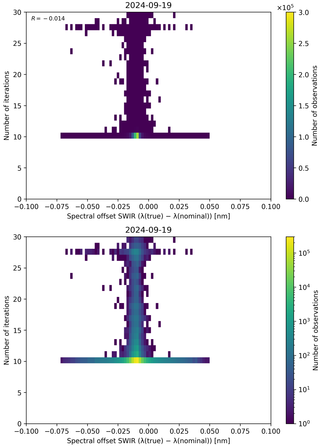
Figure 121: Scatter density plot of “Spectral offset SWIR ( \lambda_{\text{true}} - \lambda_{\text{nominal}} )” against “Number of iterations” for 2024-09-18 to 2024-09-20.
