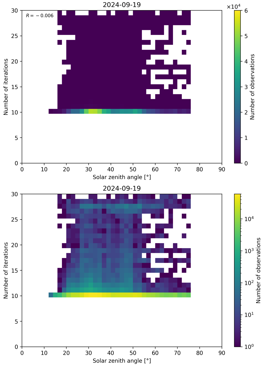
Figure 102: Scatter density plot of “Solar zenith angle” against “Number of iterations” for 2024-09-18 to 2024-09-20.
