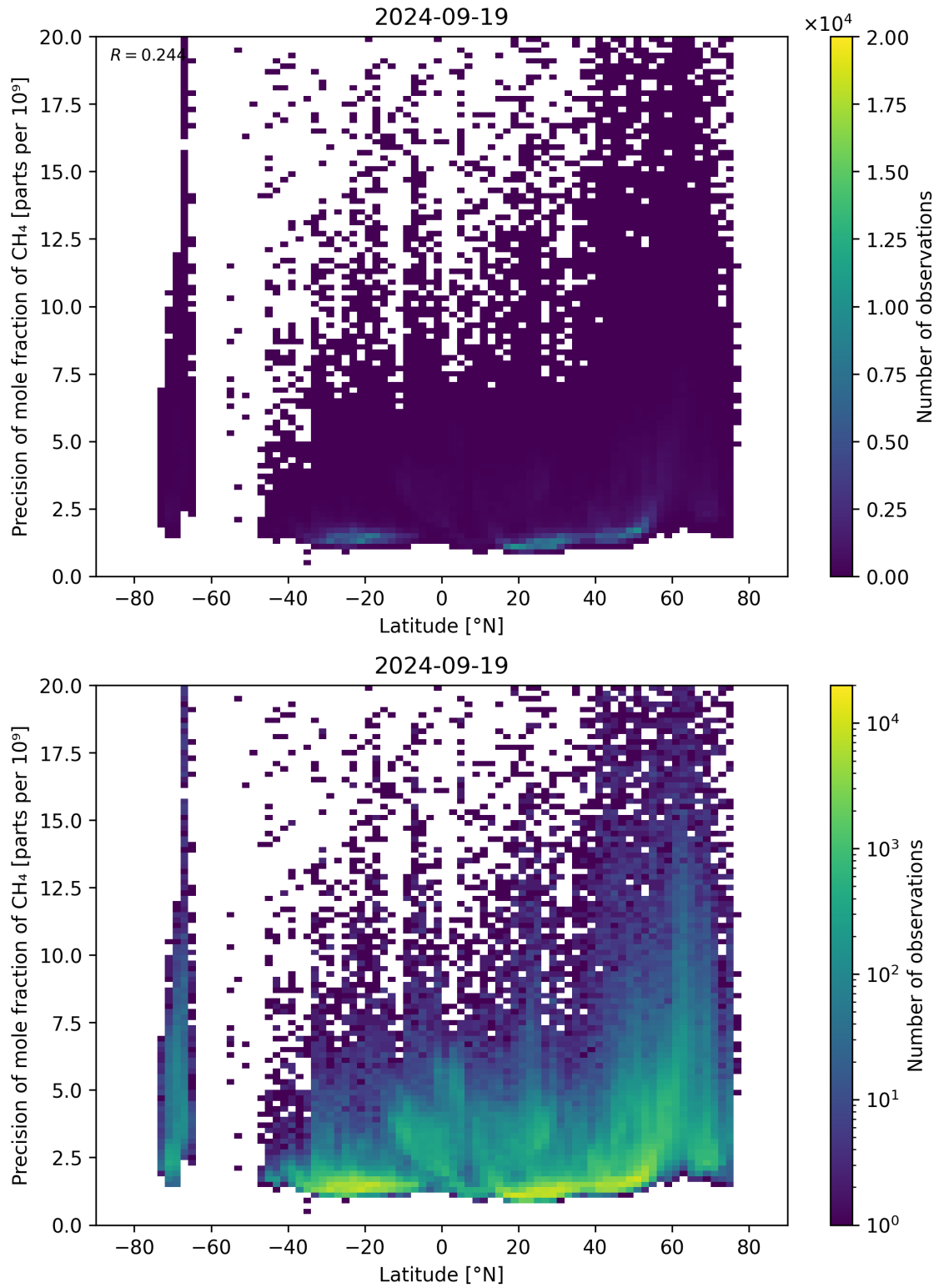
Figure 59: Scatter density plot of “Latitude” against “Precision of mole fraction of \text{CH}_4 ” for 2024-09-18 to 2024-09-20.
