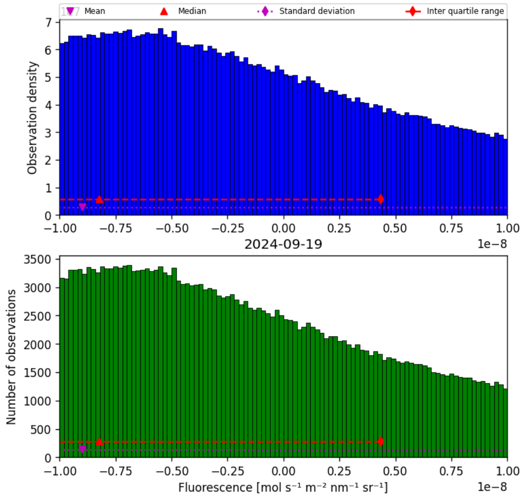
Figure 32: Histogram of “Fluorescence” for 2024-09-18 to 2024-09-20
