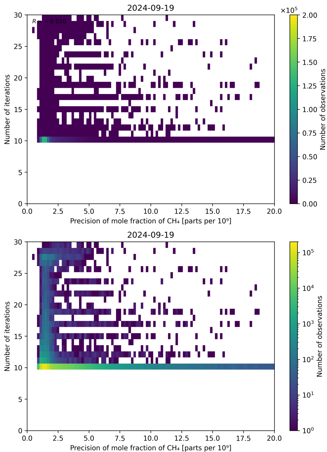
Figure 83: Scatter density plot of “Precision of mole fraction of CH 4 ” against “Number of iterations” for 2024-09-18 to 2024-09-20.
