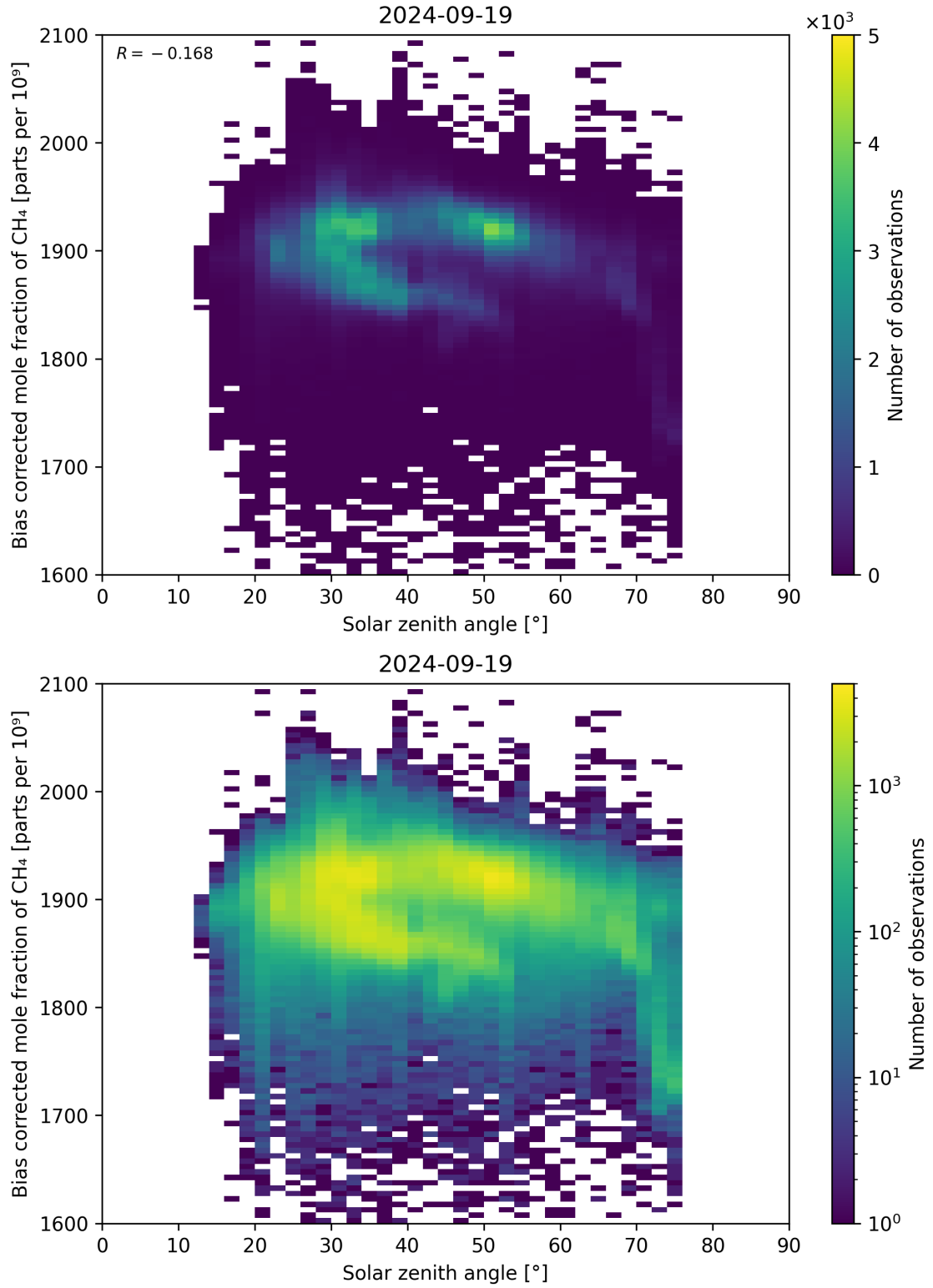
Figure 100: Scatter density plot of “Solar zenith angle” against “Bias corrected mole fraction of CH 4 ” for 2024-09-18 to 2024-09-20.
