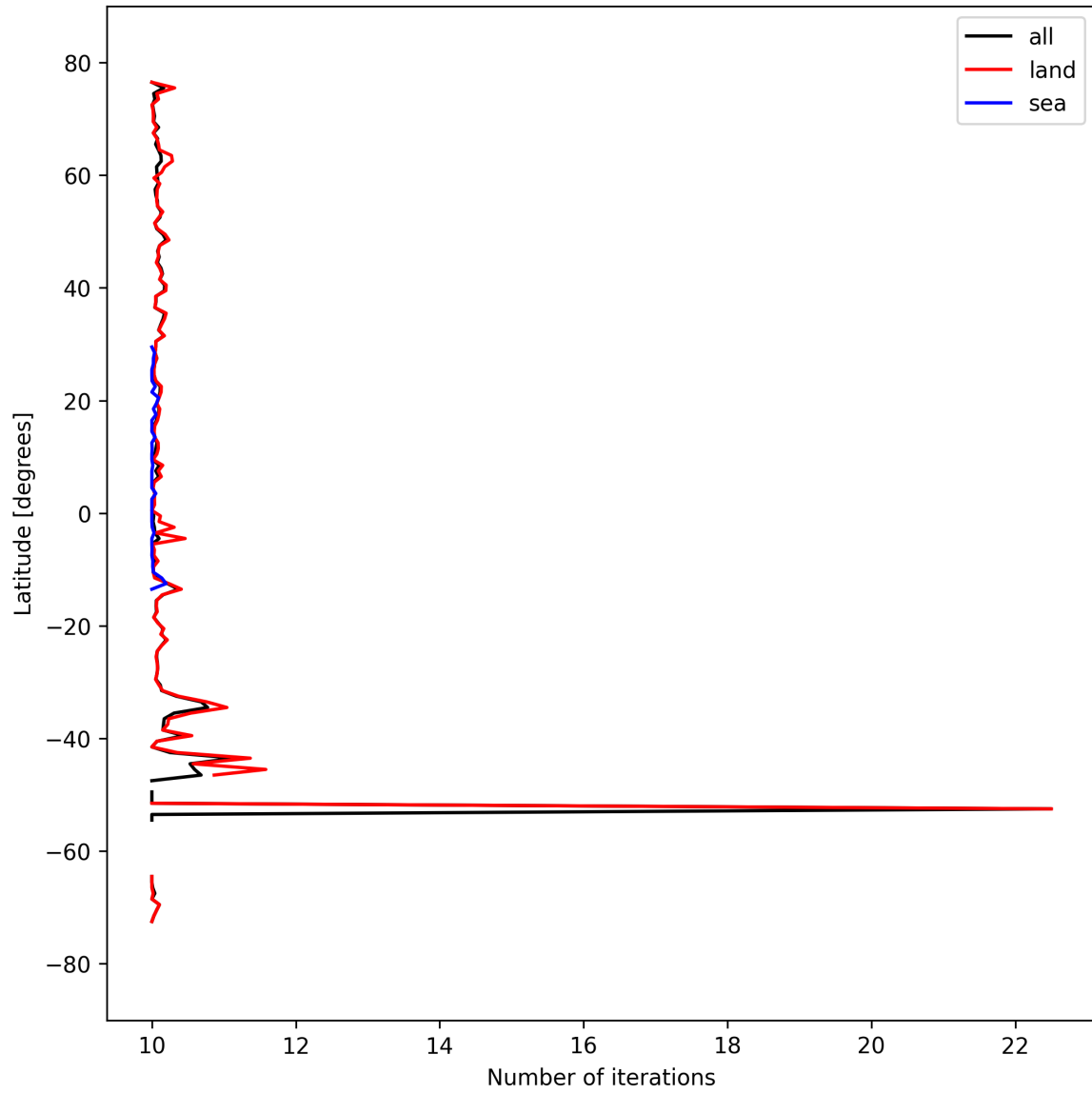
Figure 20: Zonal average of “Number of iterations” for 2024-09-18 to 2024-09-20.
