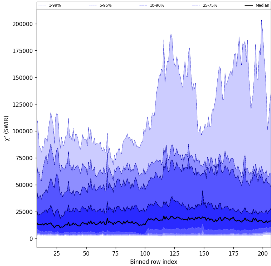
Figure 39: Along track statistics of “ \chi^2 (SWIR)” for 2024-09-18 to 2024-09-20
