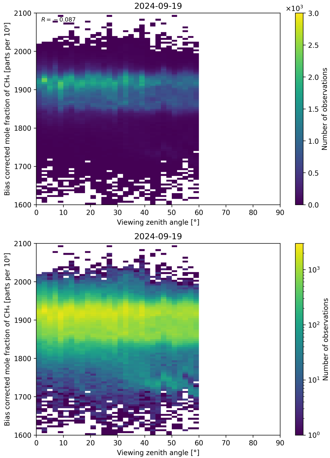
Figure 111: Scatter density plot of “Viewing zenith angle” against “Bias corrected mole fraction of CH 4 ” for 2024-09-18 to 2024-09-20.
