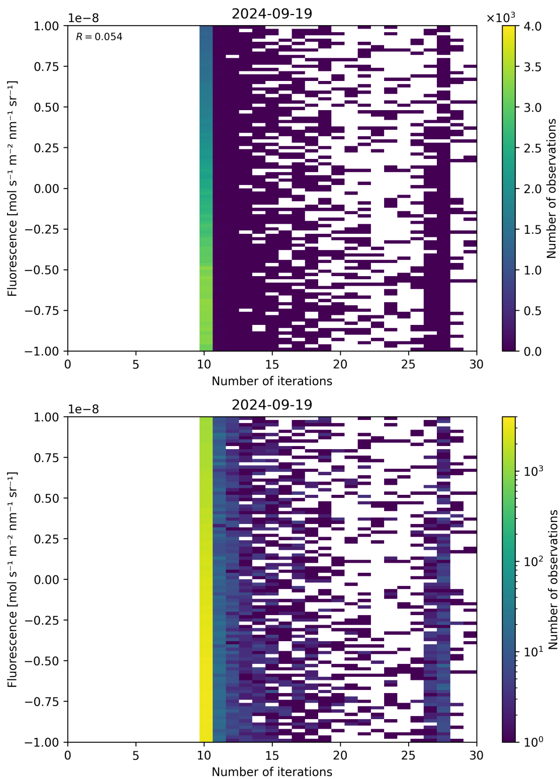
Figure 87: Scatter density plot of “Number of iterations” against “Fluorescence” for 2024-09-18 to 2024-09-20.
