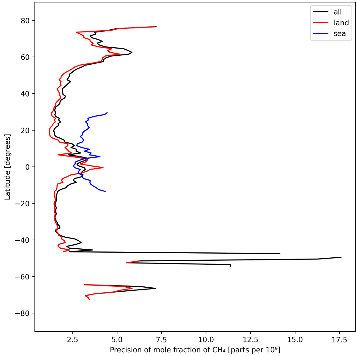
Figure 13: Zonal average of “Precision of mole fraction of CH 4 ” for 2024-09-18 to 2024-09-20.
