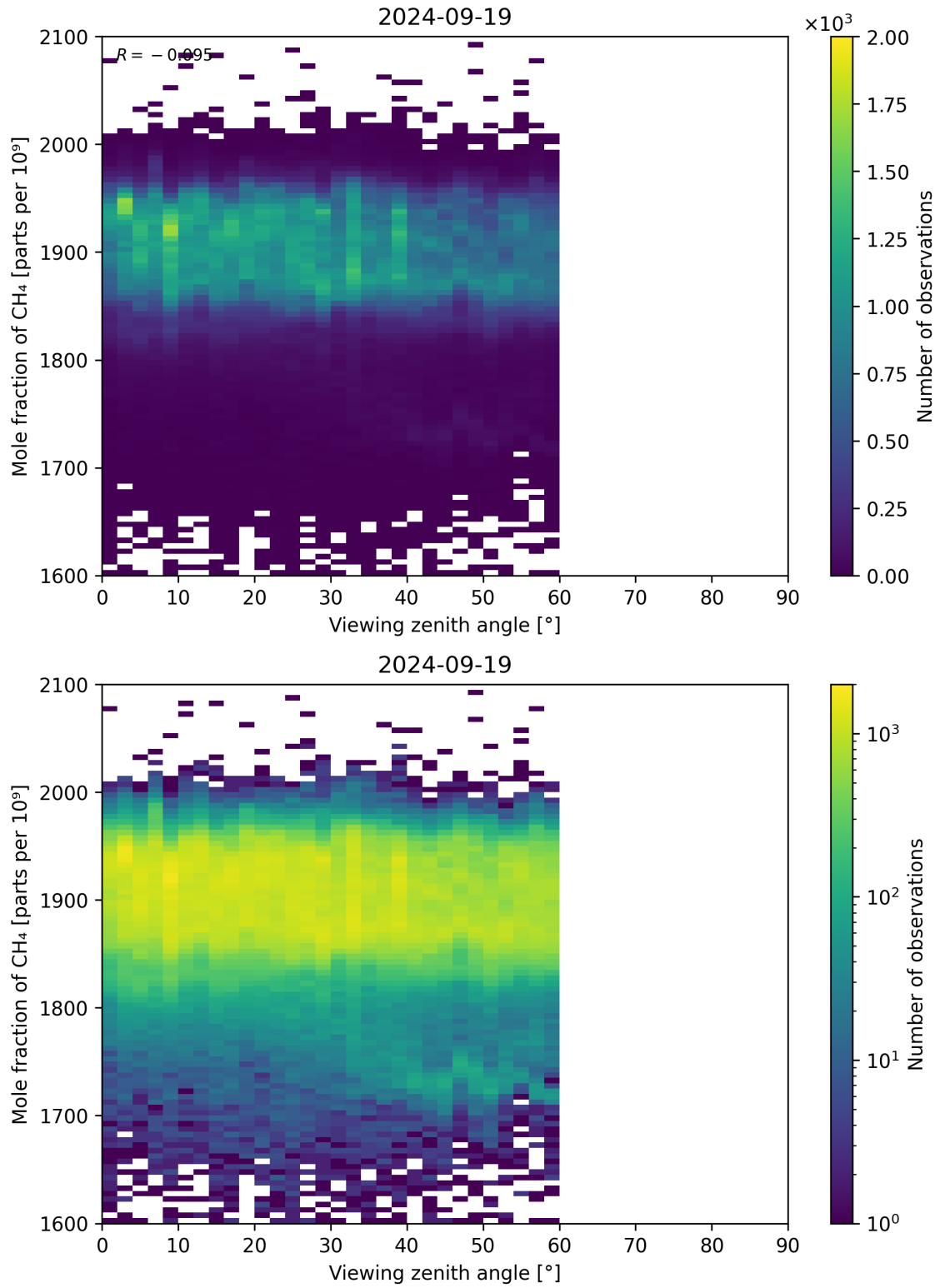
Figure 110: Scatter density plot of “Viewing zenith angle” against “Mole fraction of CH 4 ” for 2024-09-18 to 2024-09-20.
