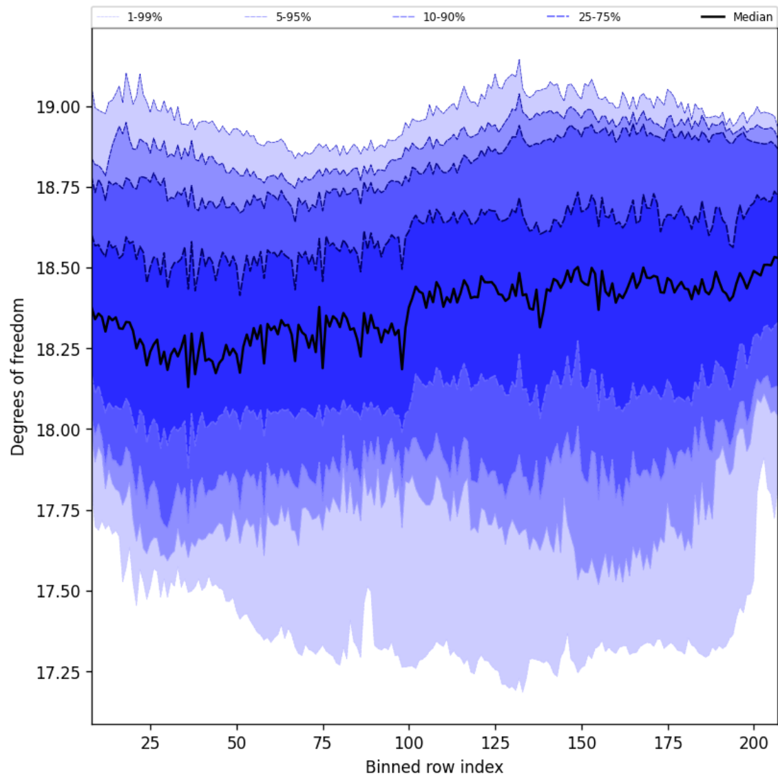
Figure 41: Along track statistics of “Degrees of freedom” for 2024-09-18 to 2024-09-20
