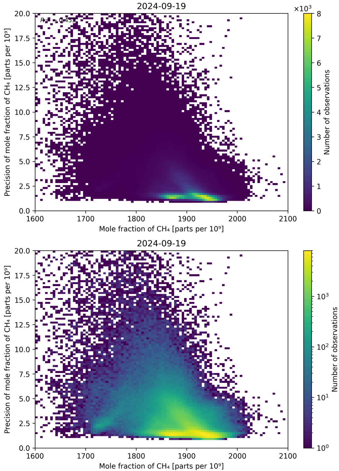
Figure 75: Scatter density plot of “Mole fraction of CH 4 ” against “Precision of mole fraction of CH 4 ” for 2024-09-18 to 2024-09-20.
