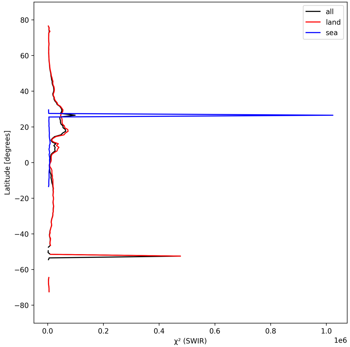
Figure 17: Zonal average of “ \chi^2 (SWIR)” for 2024-09-18 to 2024-09-20.
