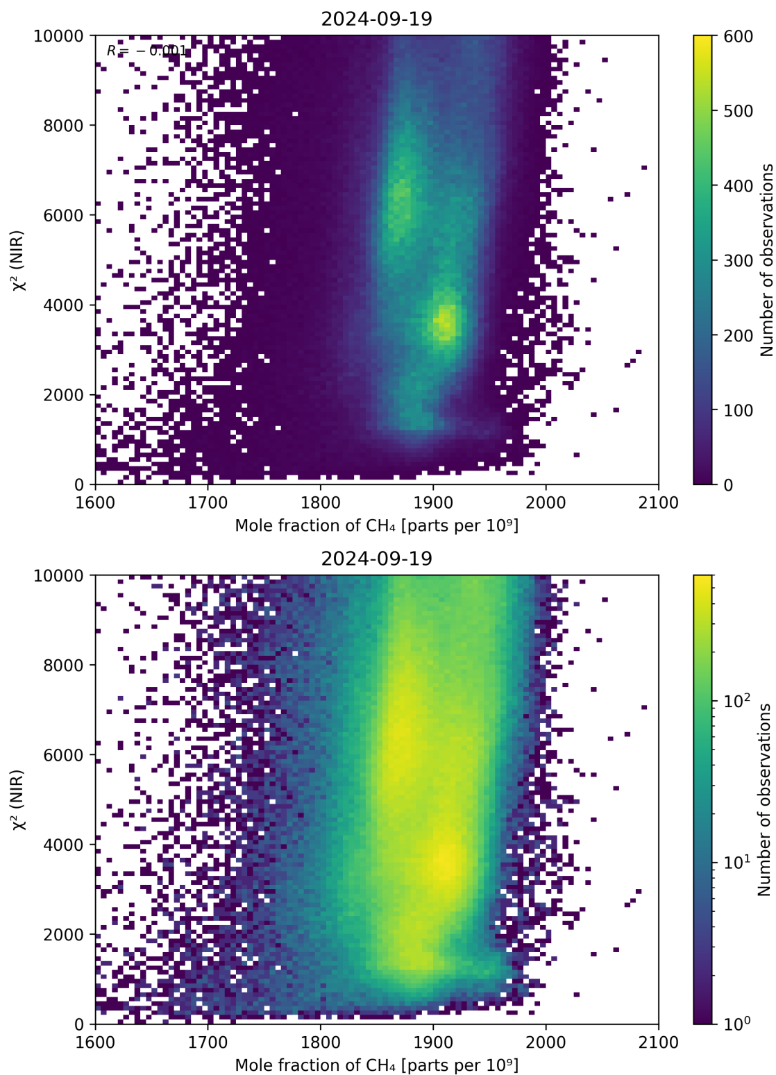
Figure 70: Scatter density plot of “Mole fraction of CH 4 ” against “ \chi^2 (NIR)” for 2024-09-18 to 2024-09-20.
