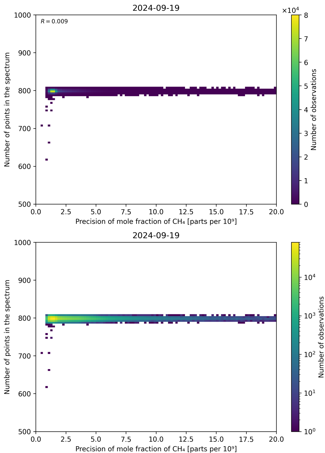
Figure 84: Scatter density plot of “Precision of mole fraction of CH 4 ” against “Number of points in the spectrum” for 2024-09-18 to 2024-09-20.
