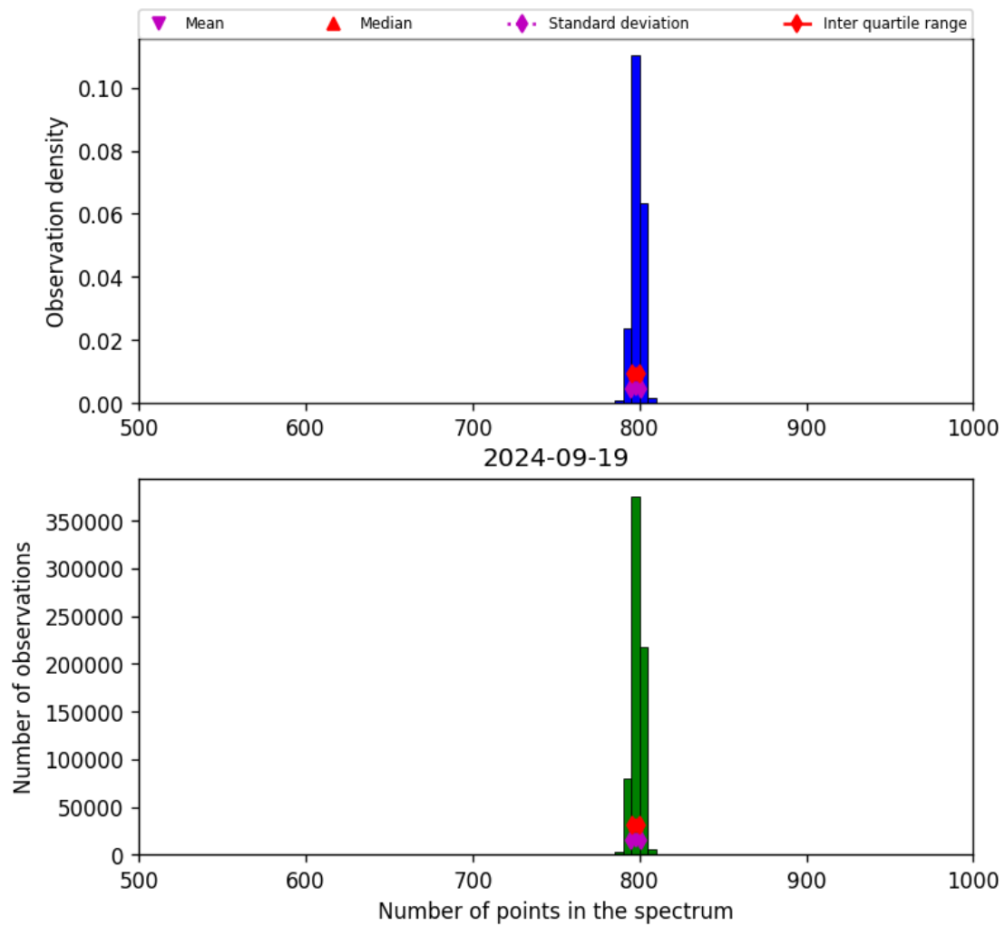
Figure 26: Histogram of “Number of points in the spectrum” for 2024-09-18 to 2024-09-20
