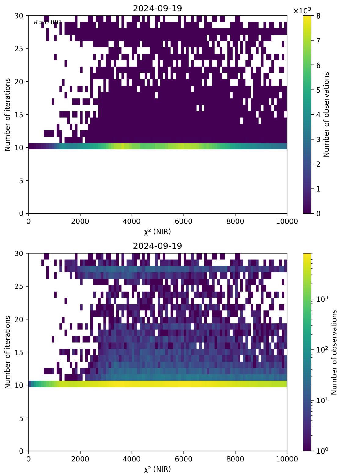
Figure 46: Scatter density plot of “ \chi^2 (NIR)” against “Number of iterations” for 2024-09-18 to 2024-09-20.
