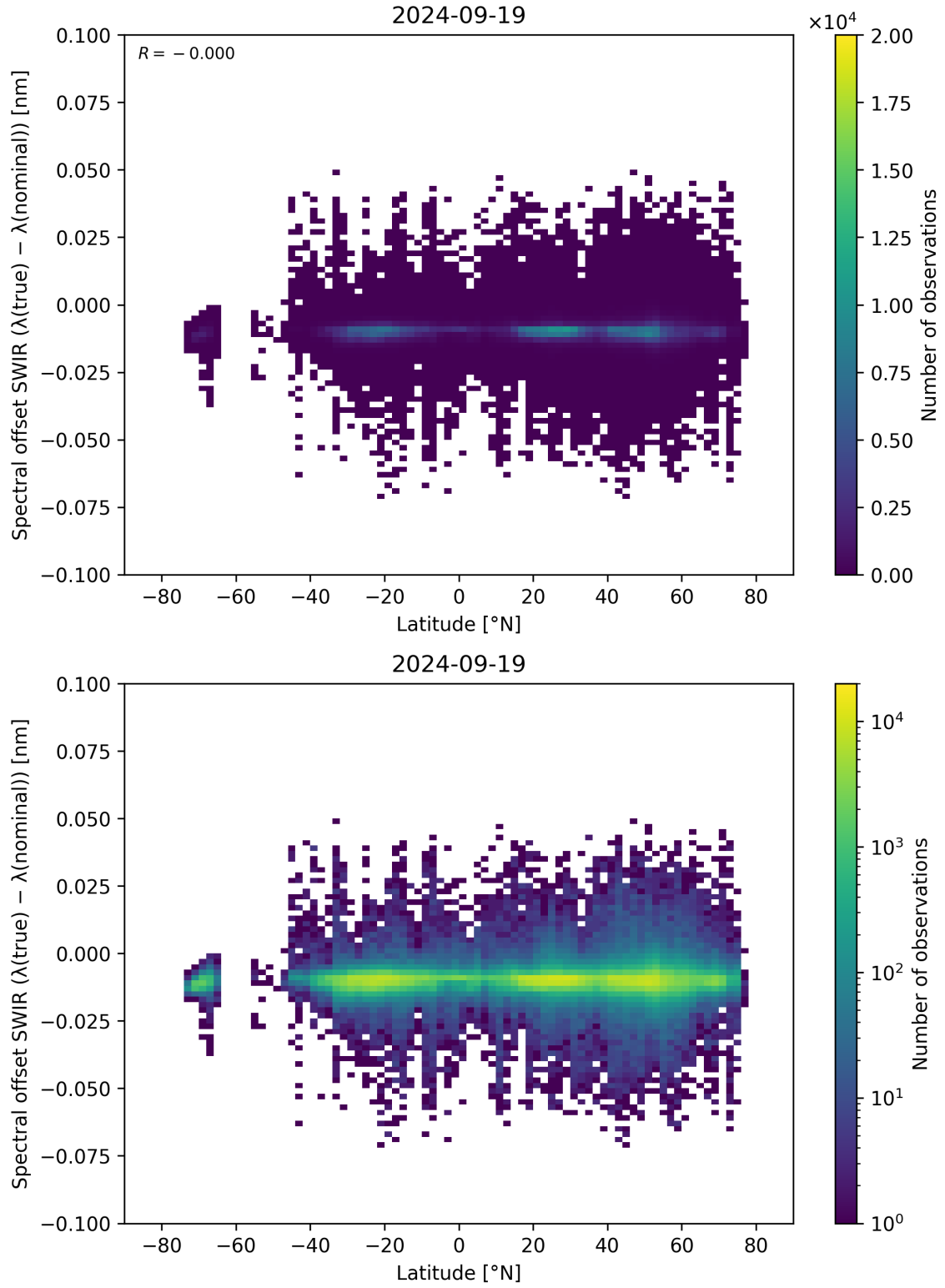
Figure 62: Scatter density plot of “Latitude” against “Spectral offset SWIR ( \lambda_{\text{true}} - \lambda_{\text{nominal}} )” for 2024-09-18 to 2024-09-20.
