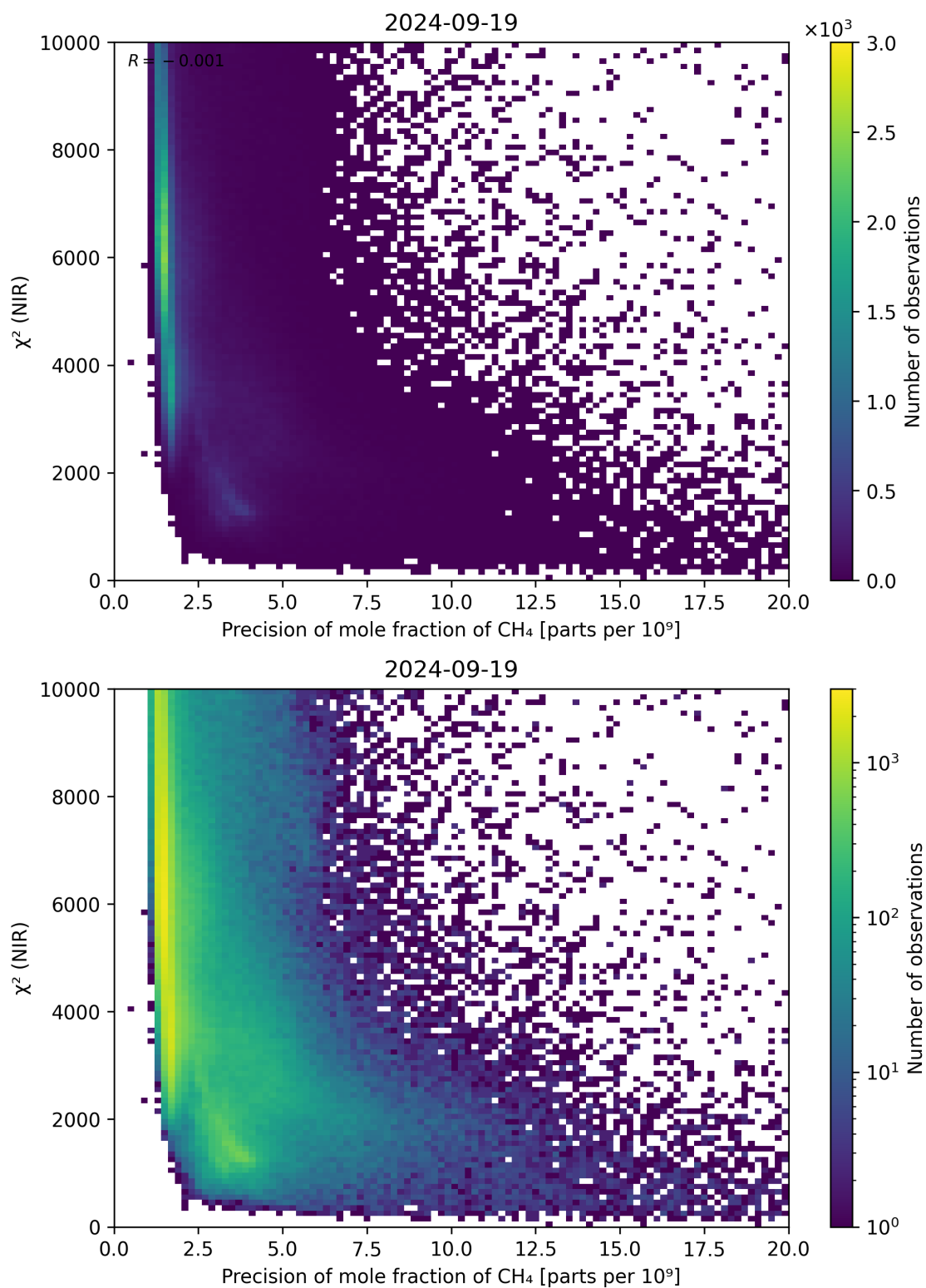
Figure 78: Scatter density plot of “Precision of mole fraction of \text{CH}_4 ” against “ \chi^2 (NIR)” for 2024-09-18 to 2024-09-20.
