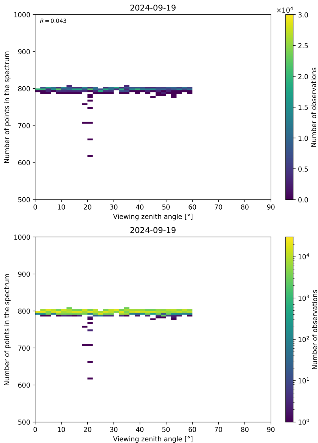
Figure 114: Scatter density plot of “Viewing zenith angle” against “Number of points in the spectrum” for 2024-09-18 to 2024-09-20.
