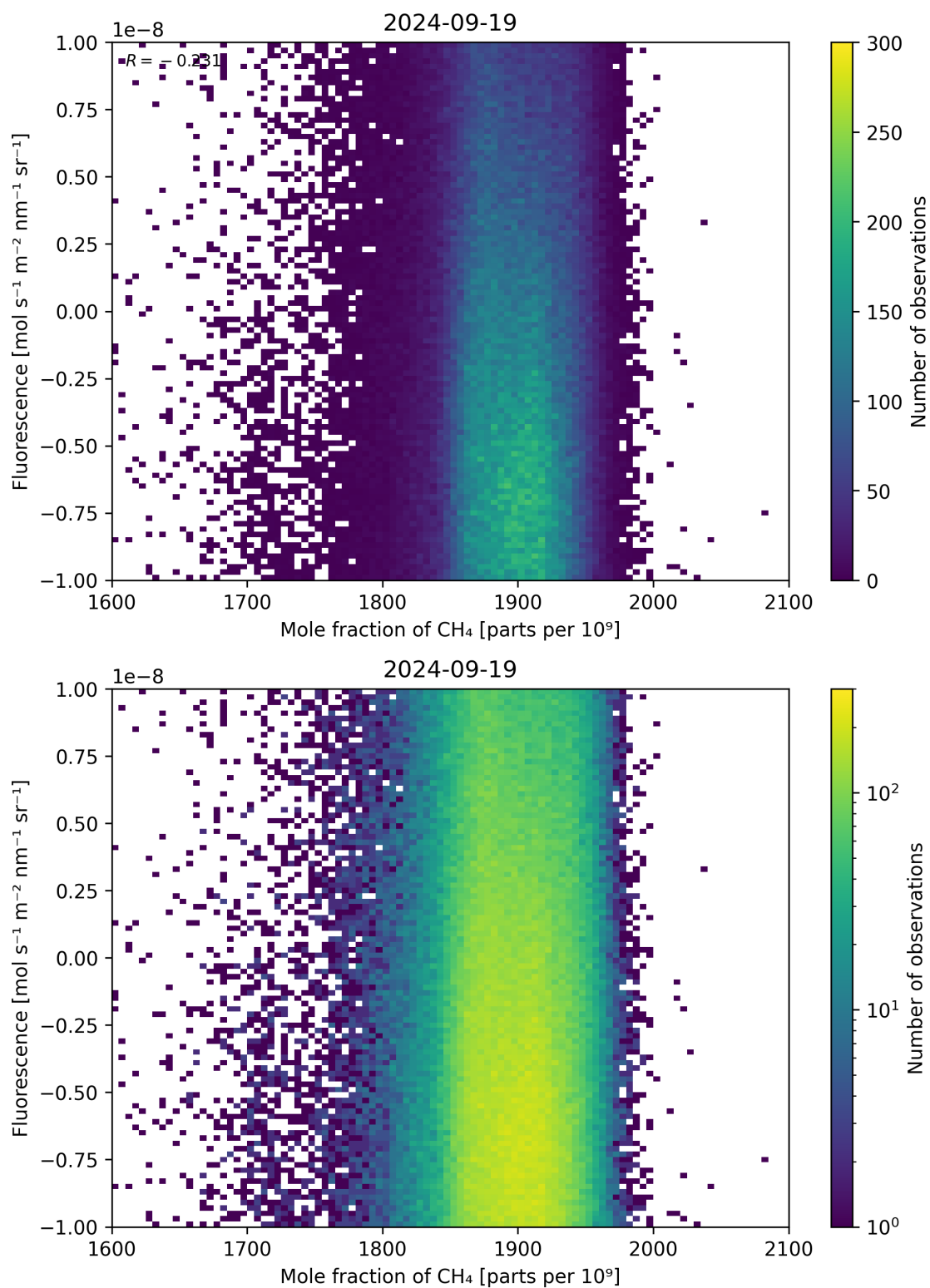
Figure 73: Scatter density plot of “Mole fraction of \text{CH}_4 ” against “Fluorescence” for 2024-09-18 to 2024-09-20.
