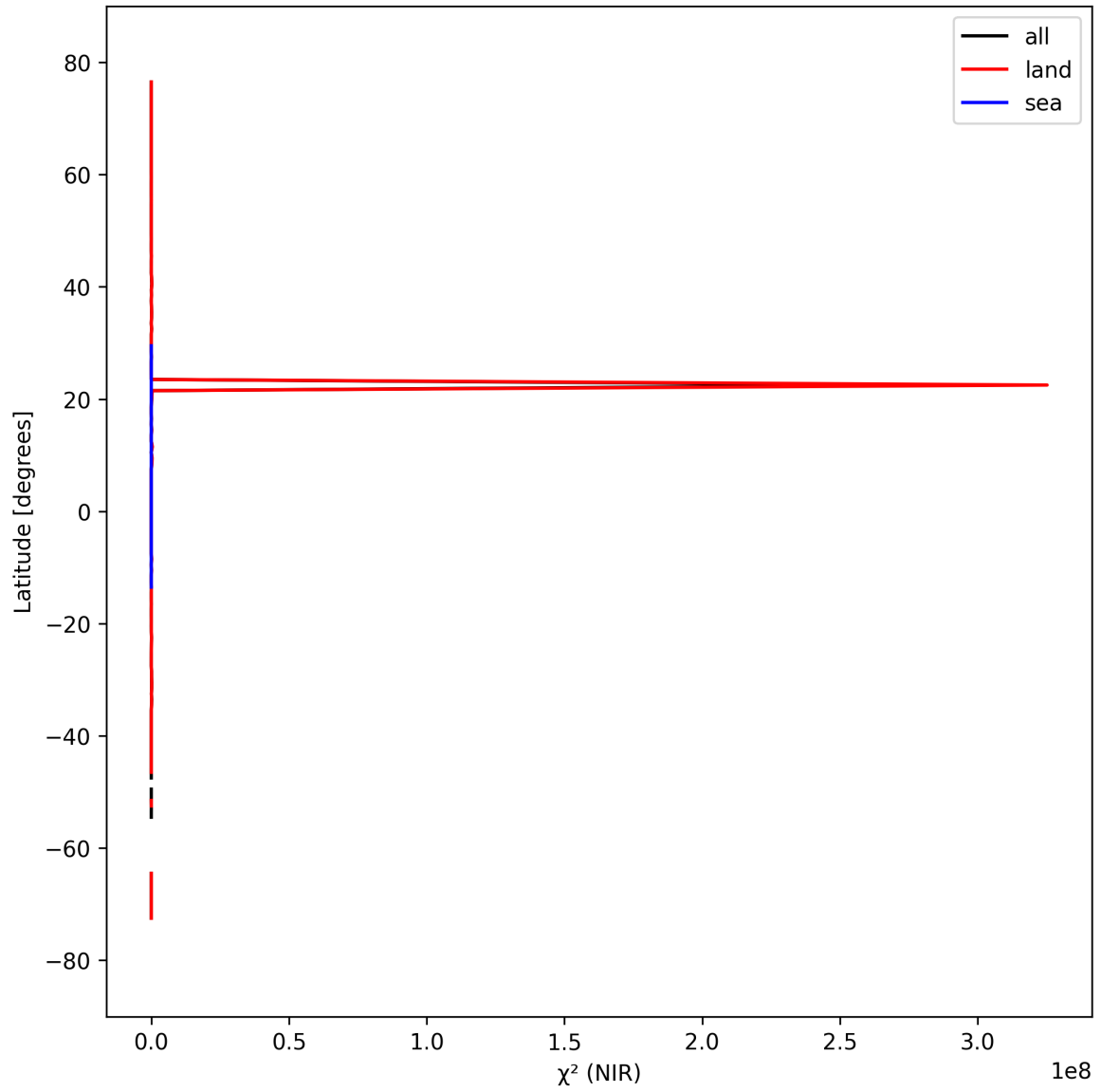
Figure 18: Zonal average of “ \chi^2 (NIR)” for 2024-09-18 to 2024-09-20.
