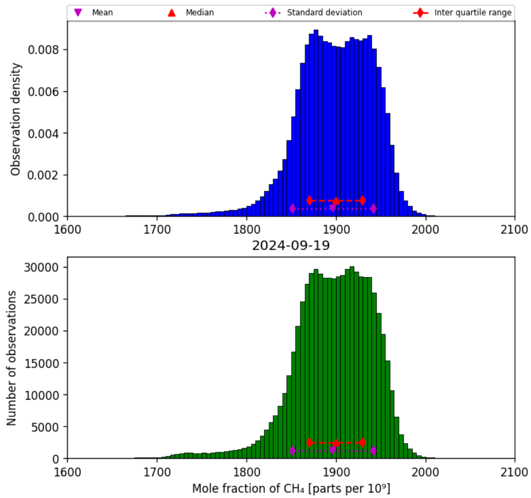
Figure 23: Histogram of “Mole fraction of CH 4 ” for 2024-09-18 to 2024-09-20
