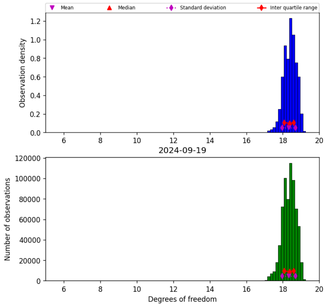
Figure 30: Histogram of “Degrees of freedom” for 2024-09-18 to 2024-09-20
