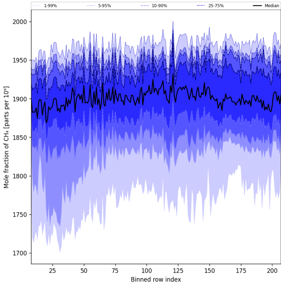
Figure 34: Along track statistics of “Mole fraction of CH 4 ” for 2024-09-18 to 2024-09-20
