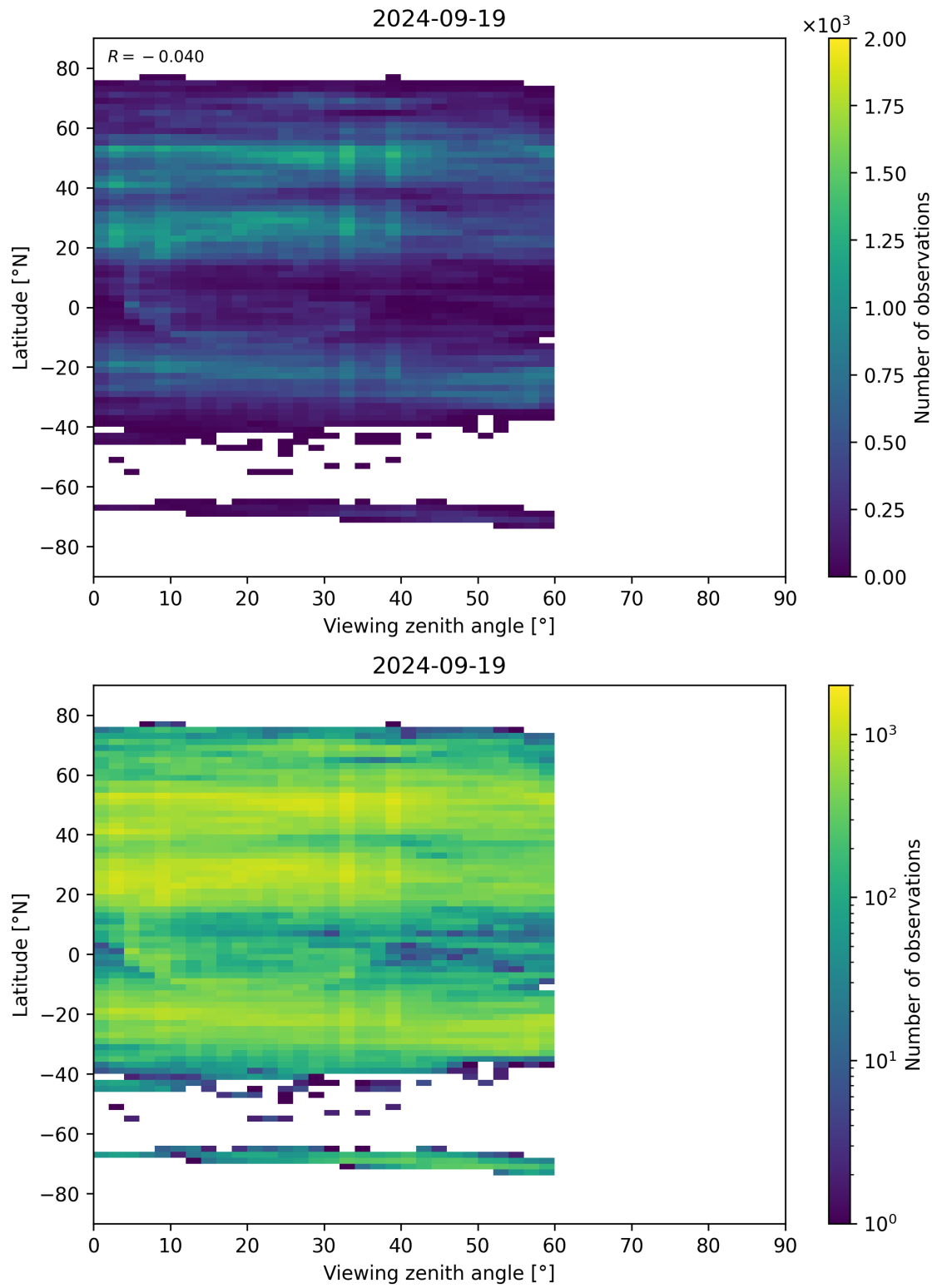
Figure 109: Scatter density plot of “Viewing zenith angle” against “Latitude” for 2024-09-18 to 2024-09-20.
