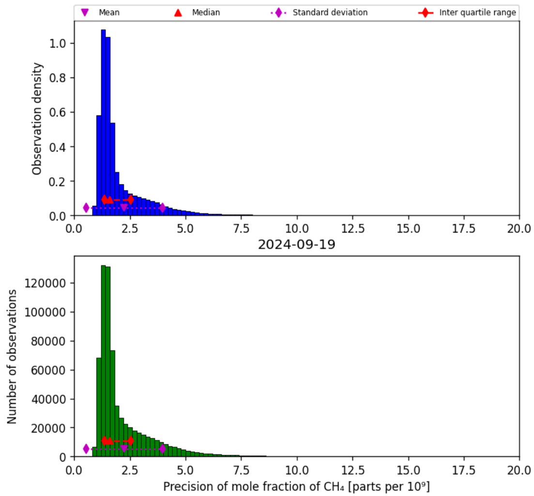
Figure 24: Histogram of “Precision of mole fraction of CH 4 ” for 2024-09-18 to 2024-09-20
