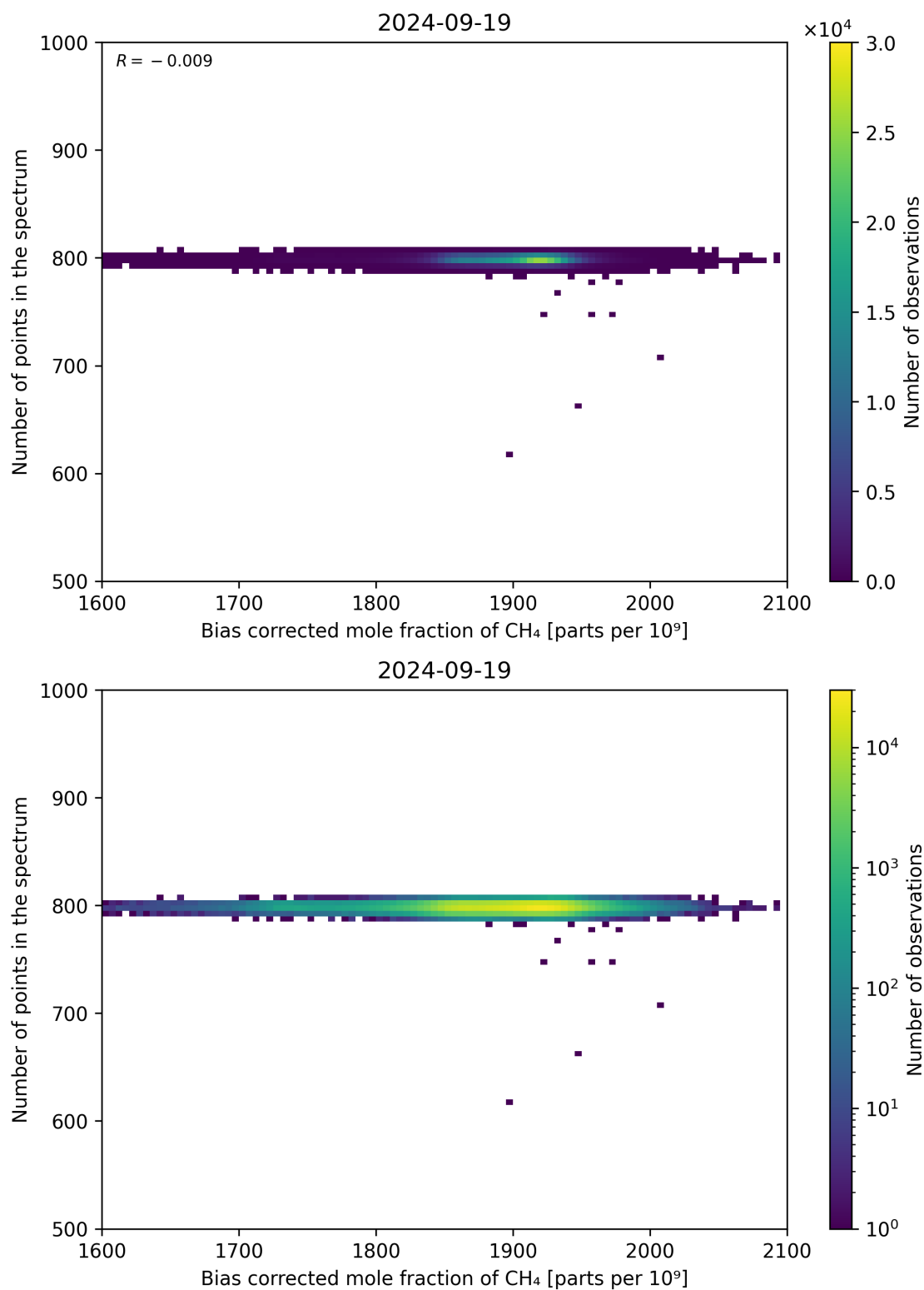
Figure 68: Scatter density plot of “Bias corrected mole fraction of CH 4 ” against “Number of points in the spectrum” for 2024-09-18 to 2024-09-20.
