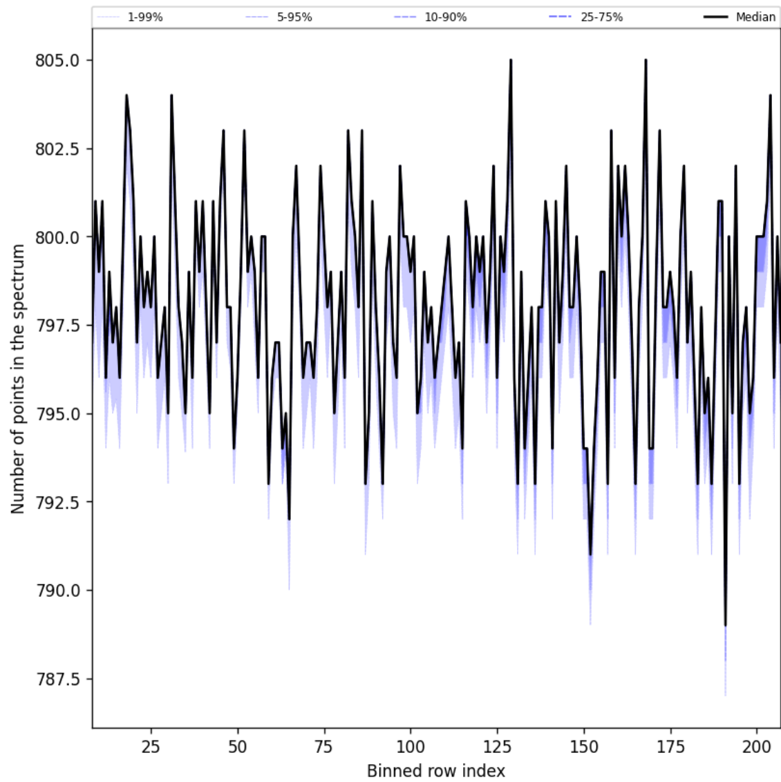
Figure 37: Along track statistics of “Number of points in the spectrum” for 2024-09-18 to 2024-09-20
