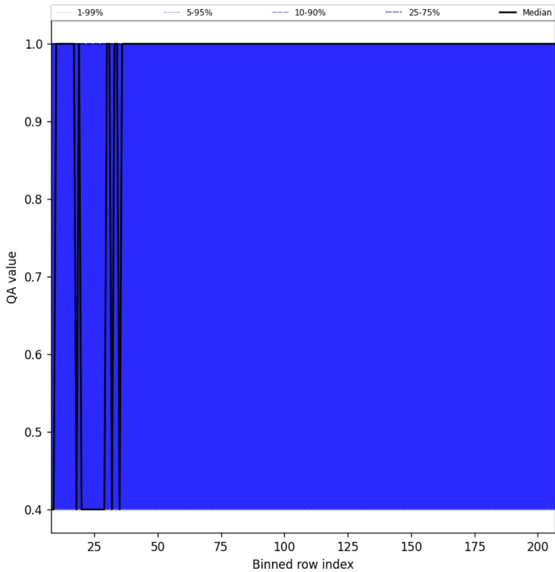
Figure 33: Along track statistics of “QA value” for 2024-09-18 to 2024-09-20
