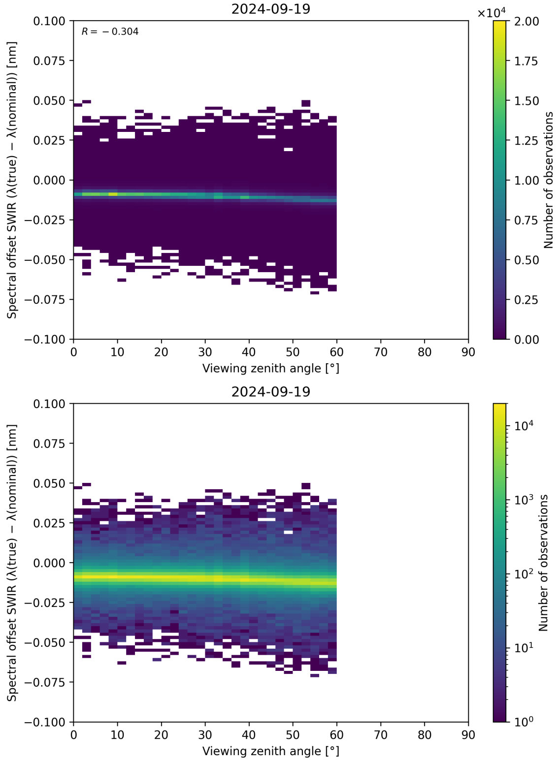
Figure 116: Scatter density plot of “Viewing zenith angle” against “Spectral offset SWIR ( \lambda_{\text{true}} - \lambda_{\text{nominal}} )” for 2024-09-18 to 2024-09-20.
