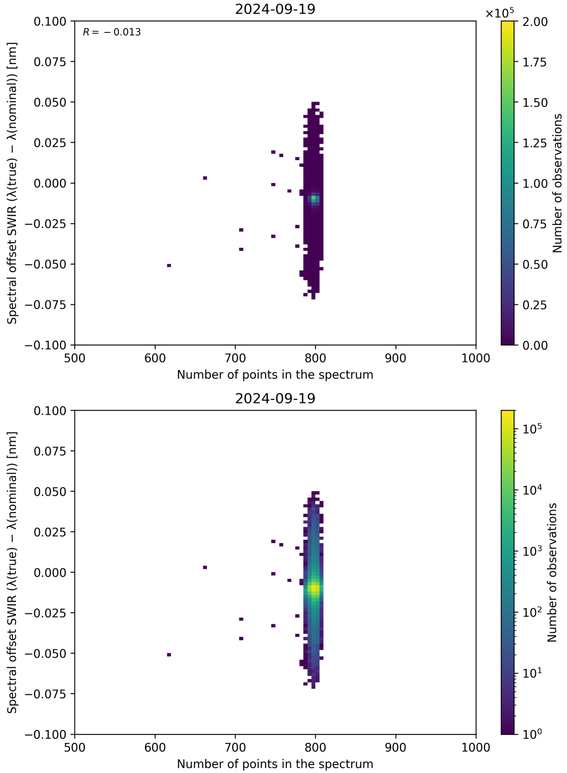
Figure 93: Scatter density plot of “Number of points in the spectrum” against “Spectral offset SWIR ( \lambda_{\text{true}} - \lambda_{\text{nominal}} )” for 2024-09-18 to 2024-09-20.
