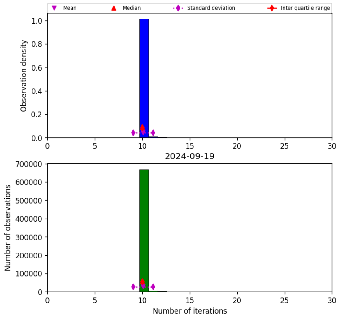
Figure 31: Histogram of “Number of iterations” for 2024-09-18 to 2024-09-20
