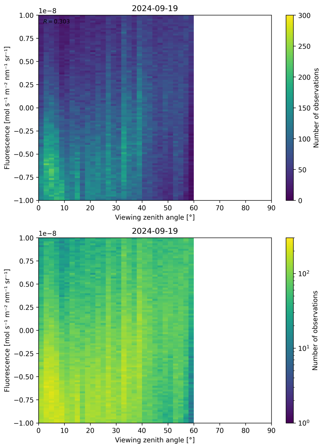
Figure 108: Scatter density plot of “Viewing zenith angle” against “Fluorescence” for 2024-09-18 to 2024-09-20.
