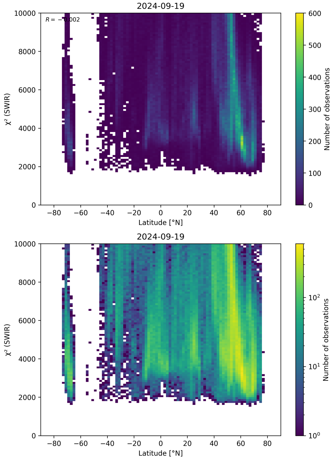
Figure 54: Scatter density plot of “Latitude” against “ \chi^2 (SWIR)” for 2024-09-18 to 2024-09-20.
