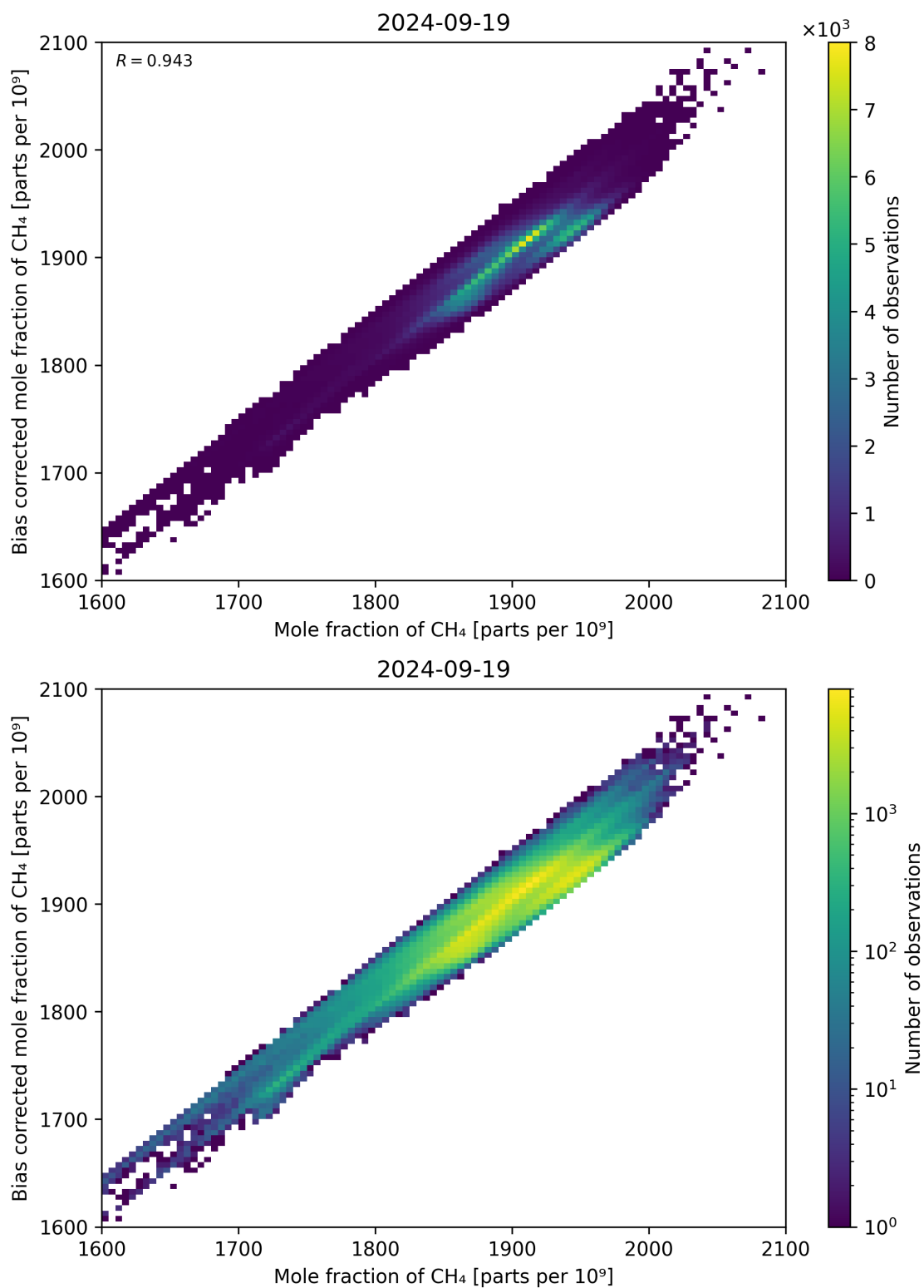
Figure 74: Scatter density plot of “Mole fraction of CH 4 ” against “Bias corrected mole fraction of CH 4 ” for 2024-09-18 to 2024-09-20.
