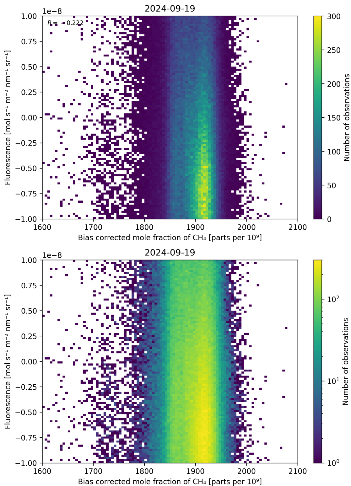
Figure 66: Scatter density plot of “Bias corrected mole fraction of \text{CH}_4 ” against “Fluorescence” for 2024-09-18 to 2024-09-20.
