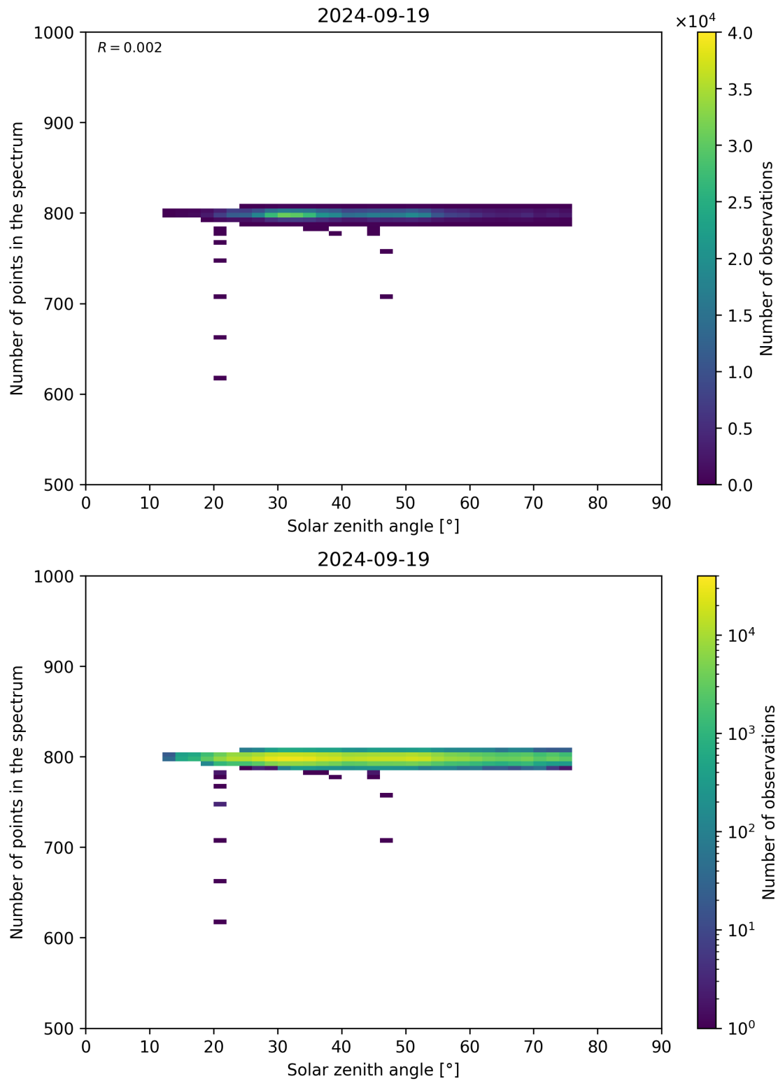
Figure 103: Scatter density plot of “Solar zenith angle” against “Number of points in the spectrum” for 2024-09-18 to 2024-09-20.
