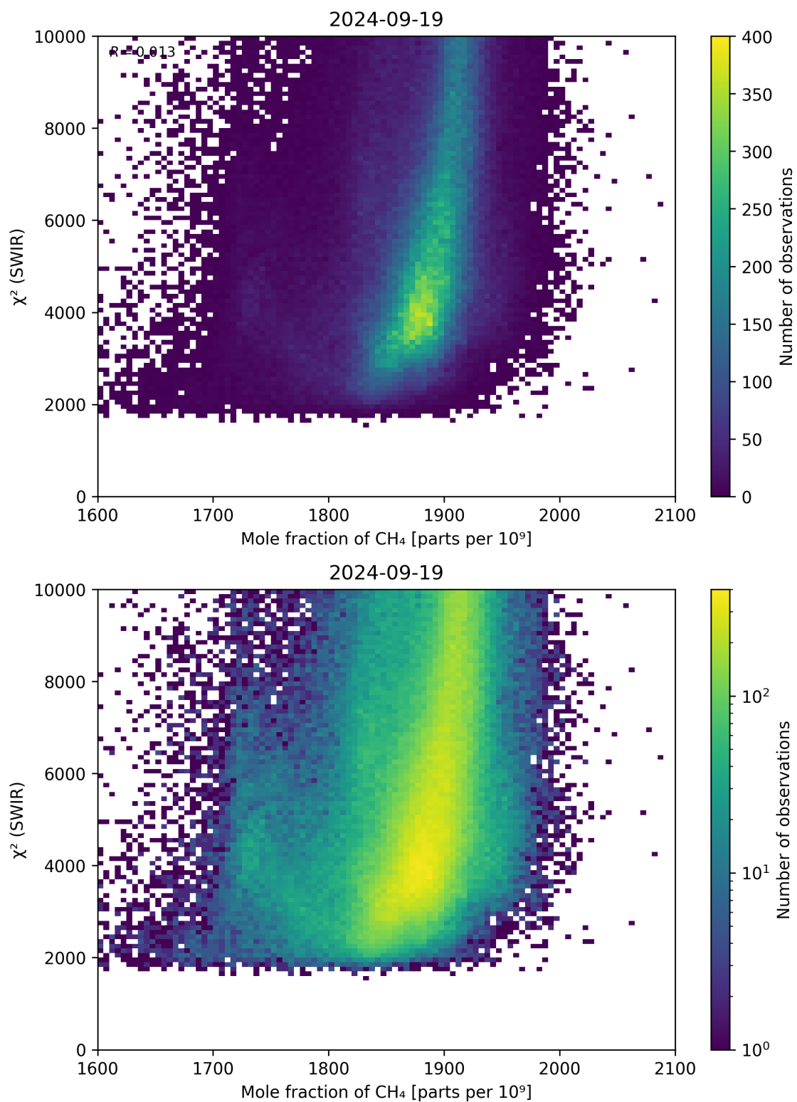
Figure 71: Scatter density plot of “Mole fraction of \text{CH}_4 ” against “ \chi^2 (SWIR)” for 2024-09-18 to 2024-09-20.
