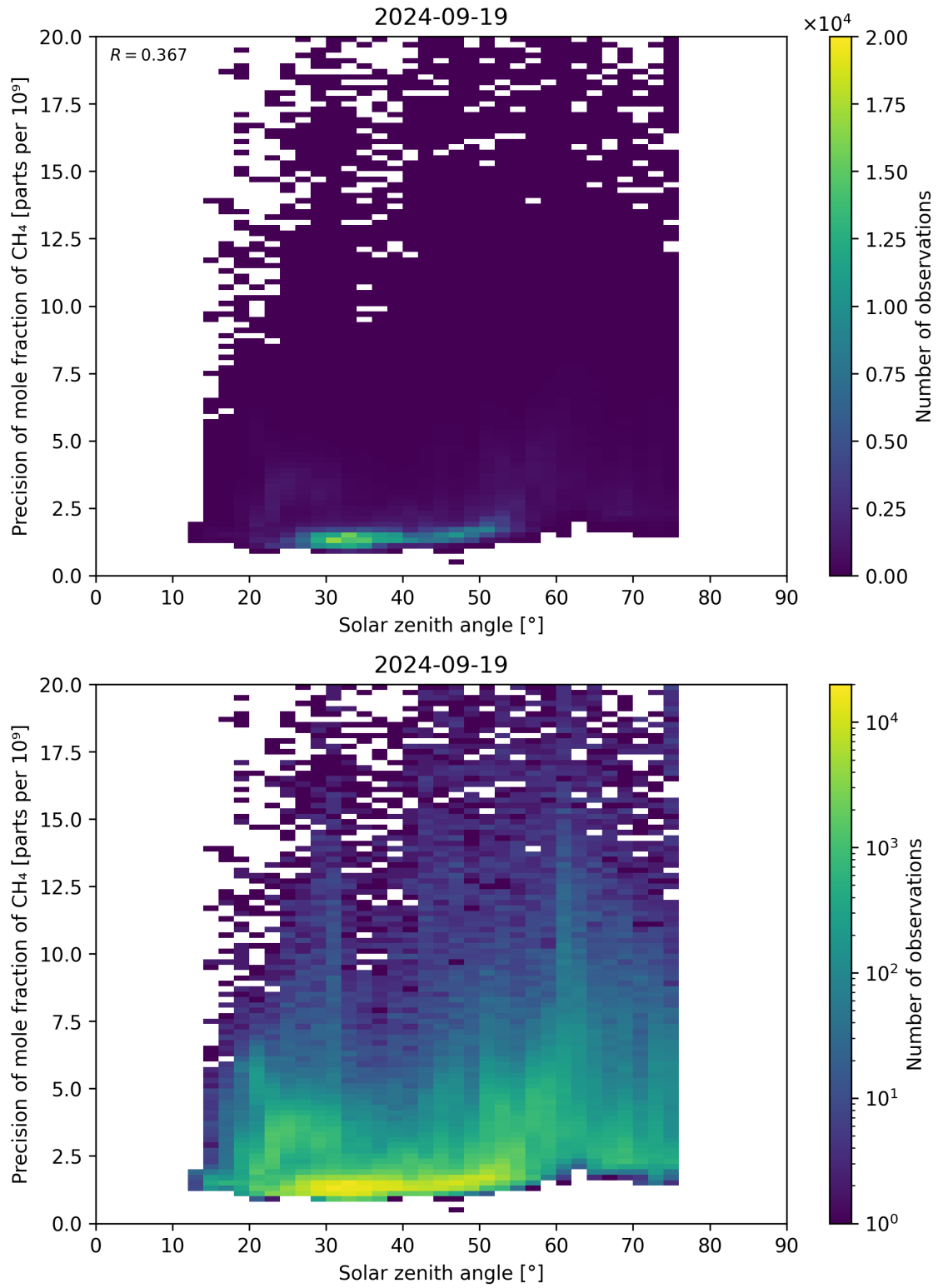
Figure 101: Scatter density plot of “Solar zenith angle” against “Precision of mole fraction of CH 4 ” for 2024-09-18 to 2024-09-20.
