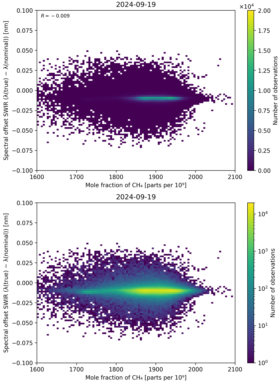
Figure 86: Scatter density plot of “Mole fraction of CH 4 ” against “Spectral offset SWIR ( \lambda_{\text{true}} - \lambda_{\text{nominal}} )” for 2024-09-18 to 2024-09-20.
