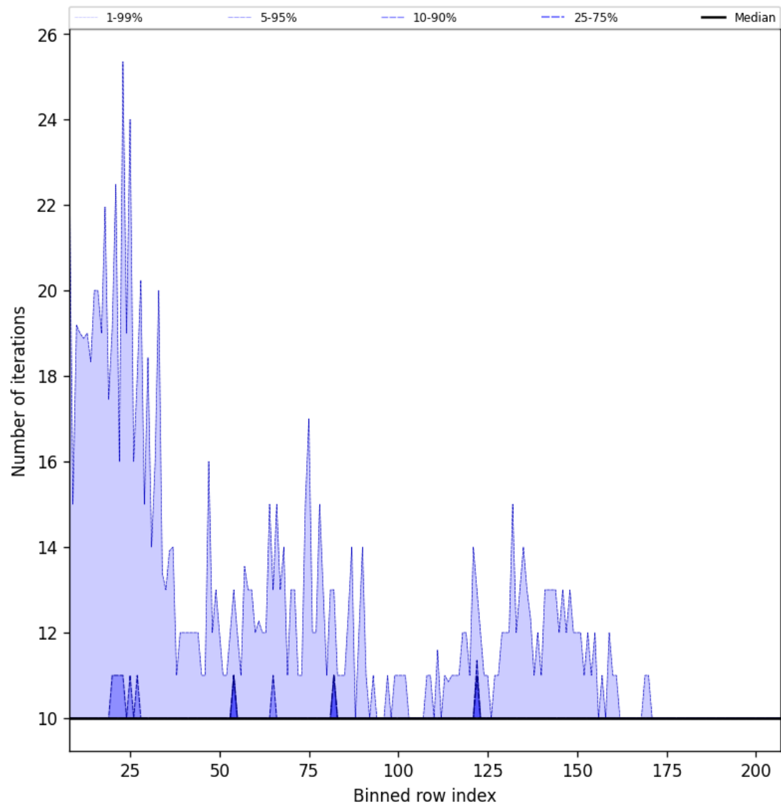
Figure 42: Along track statistics of “Number of iterations” for 2024-09-18 to 2024-09-20
