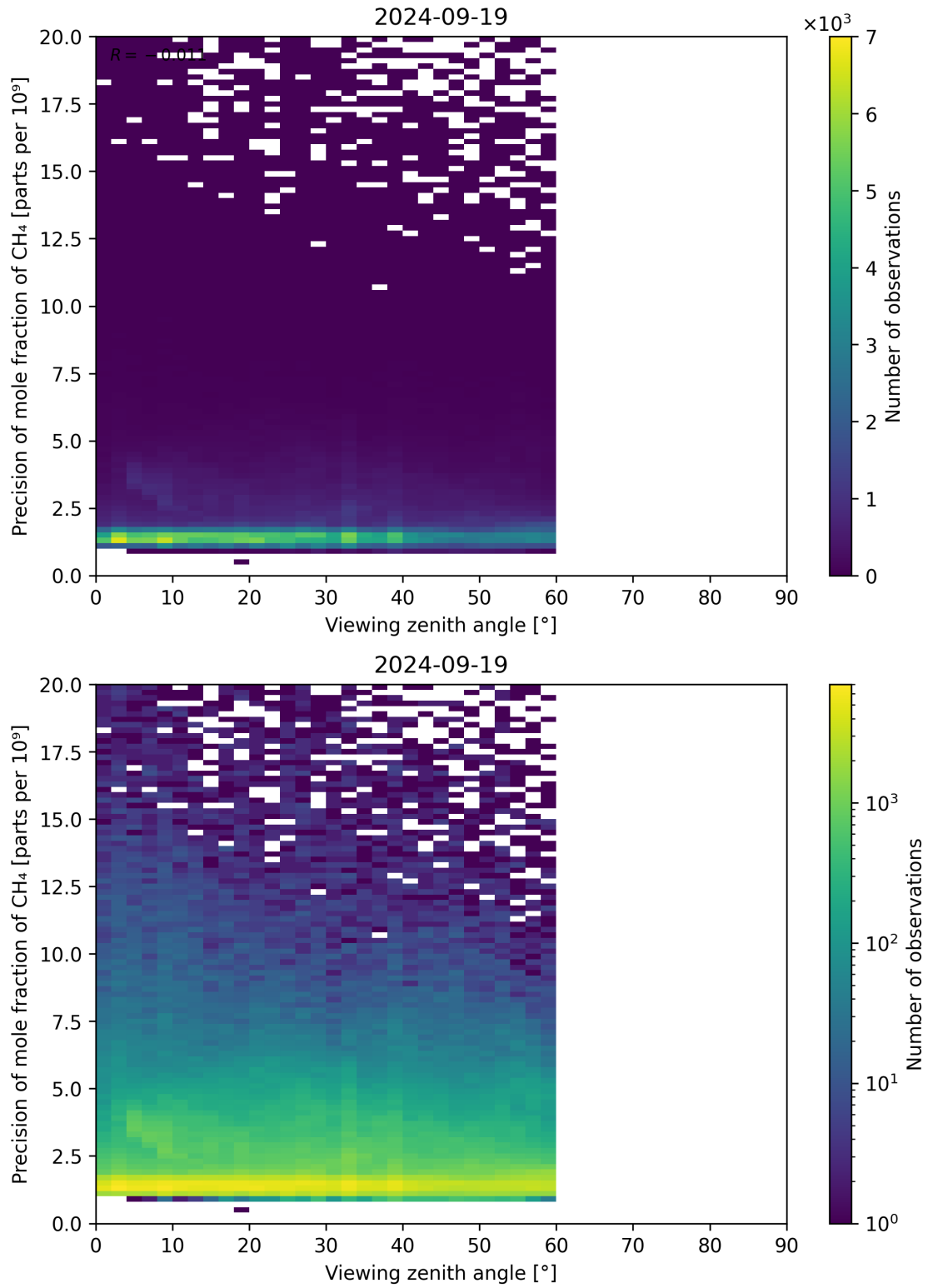
Figure 112: Scatter density plot of “Viewing zenith angle” against “Precision of mole fraction of CH 4 ” for 2024-09-18 to 2024-09-20.
