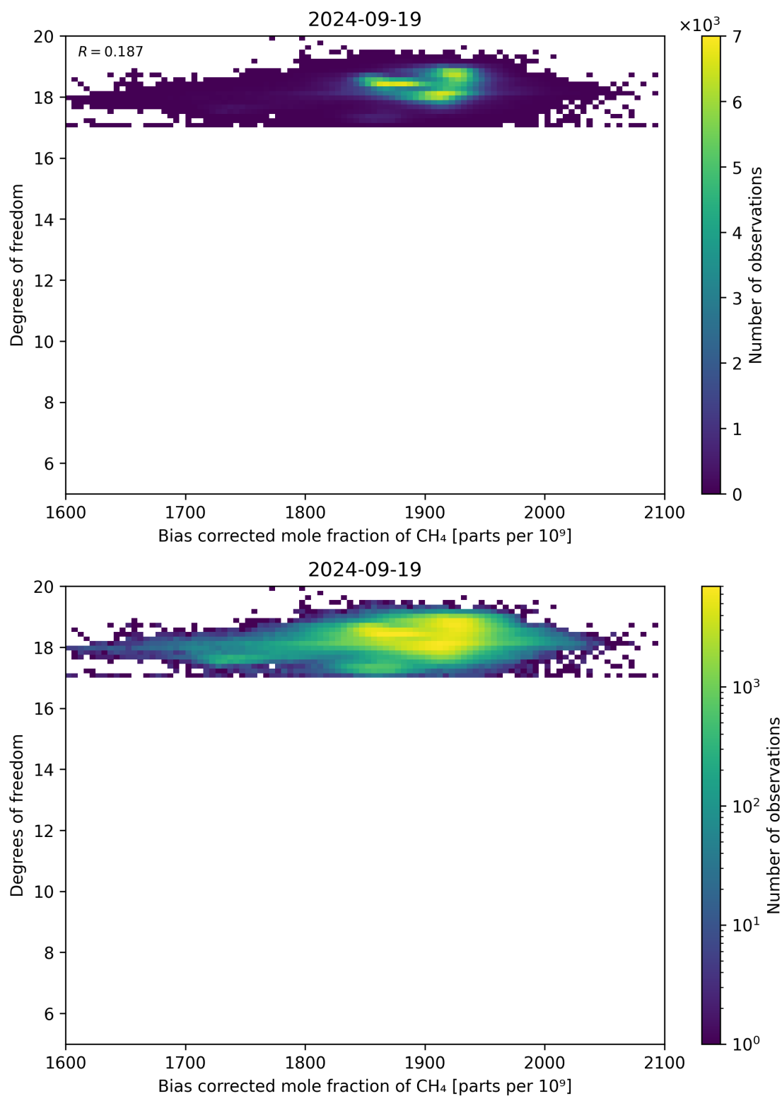
Figure 65: Scatter density plot of “Bias corrected mole fraction of CH 4 ” against “Degrees of freedom” for 2024-09-18 to 2024-09-20.
