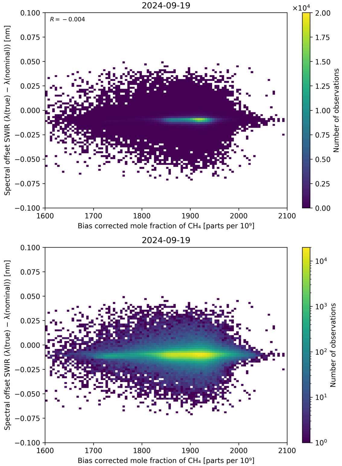
Figure 69: Scatter density plot of “Bias corrected mole fraction of \text{CH}_4 ” against “Spectral offset SWIR ( \lambda_{\text{true}} - \lambda_{\text{nominal}} )” for 2024-09-18 to 2024-09-20.
