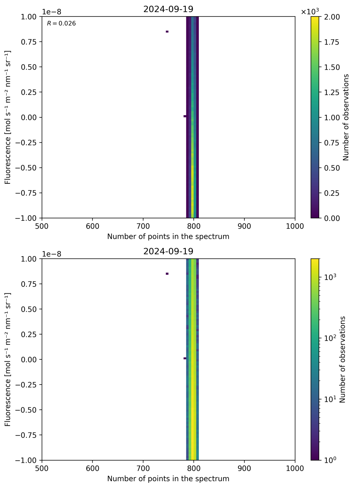
Figure 91: Scatter density plot of “Number of points in the spectrum” against “Fluorescence” for 2024-09-18 to 2024-09-20.
