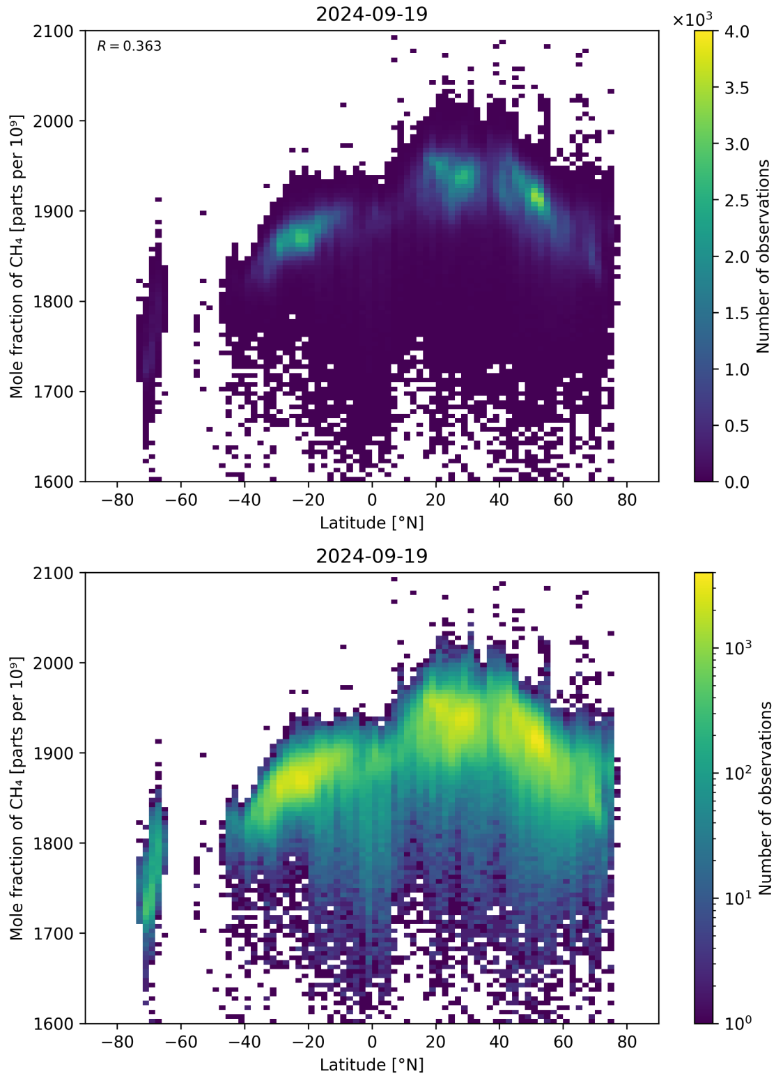
Figure 57: Scatter density plot of “Latitude” against “Mole fraction of CH 4 ” for 2024-09-18 to 2024-09-20.
