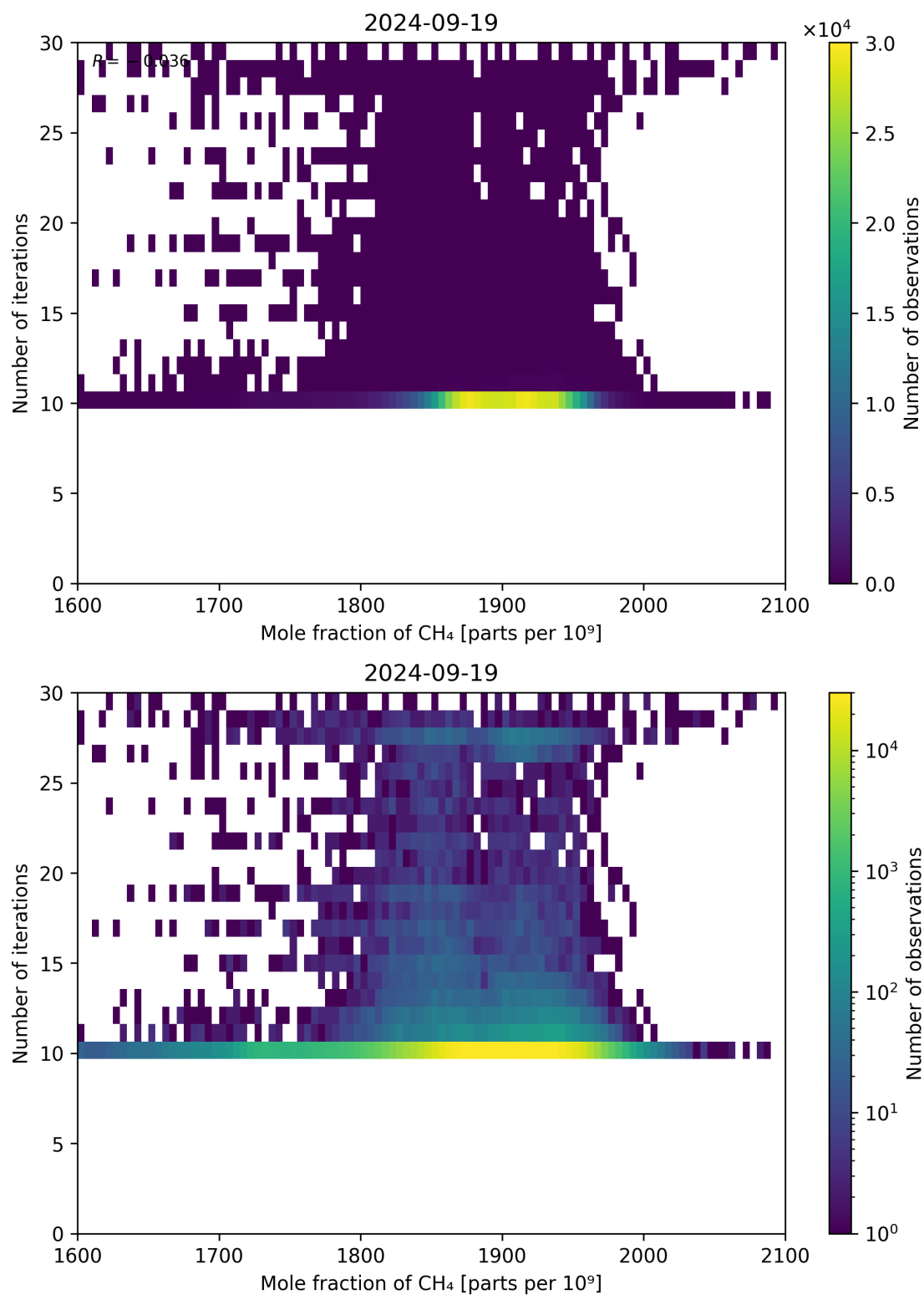
Figure 76: Scatter density plot of “Mole fraction of CH 4 ” against “Number of iterations” for 2024-09-18 to 2024-09-20.
