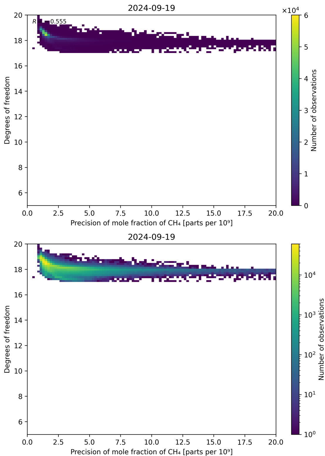
Figure 80: Scatter density plot of “Precision of mole fraction of CH 4 ” against “Degrees of freedom” for 2024-09-18 to 2024-09-20.
