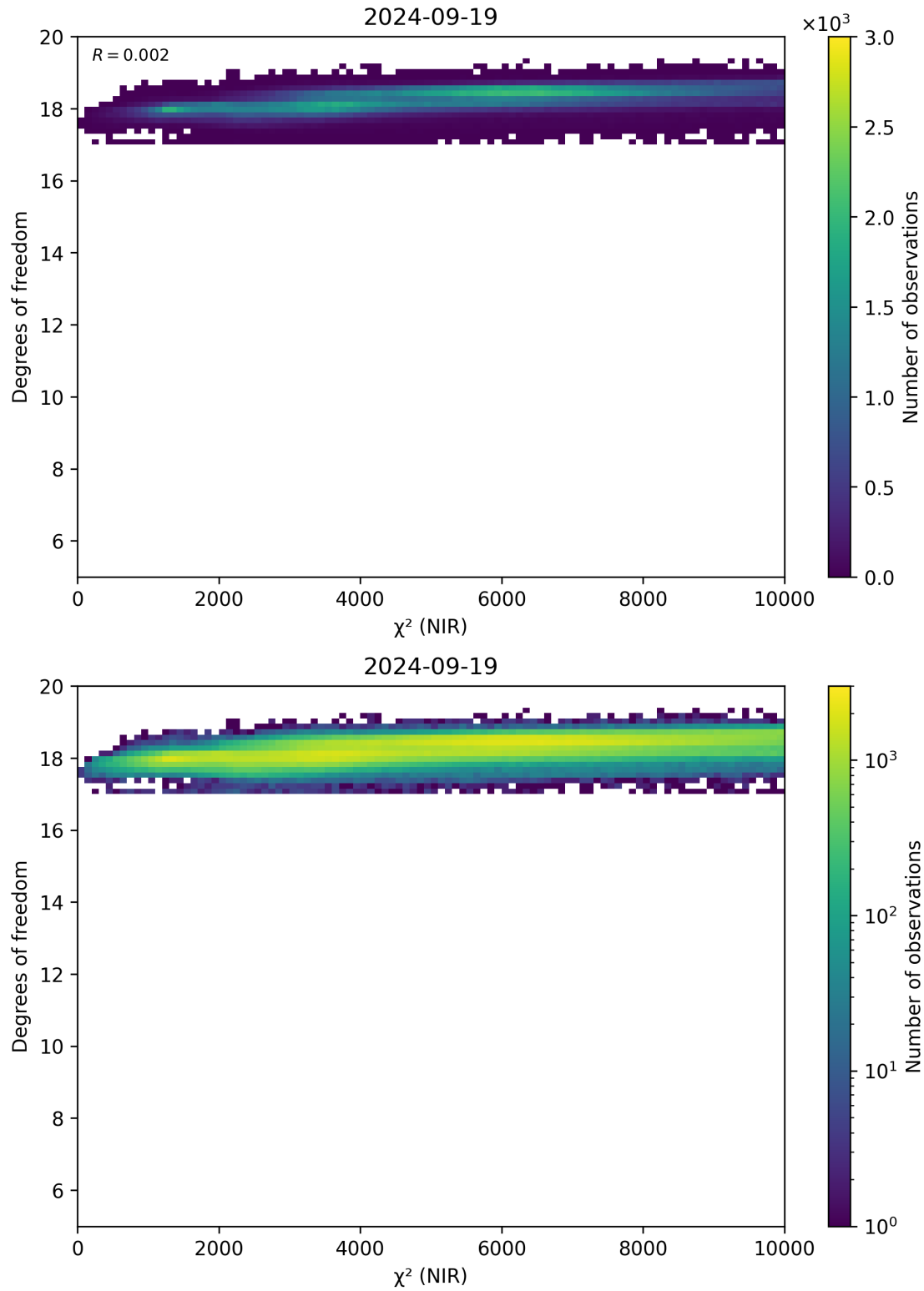
Figure 44: Scatter density plot of “ \chi^2 (NIR)” against “Degrees of freedom” for 2024-09-18 to 2024-09-20.
