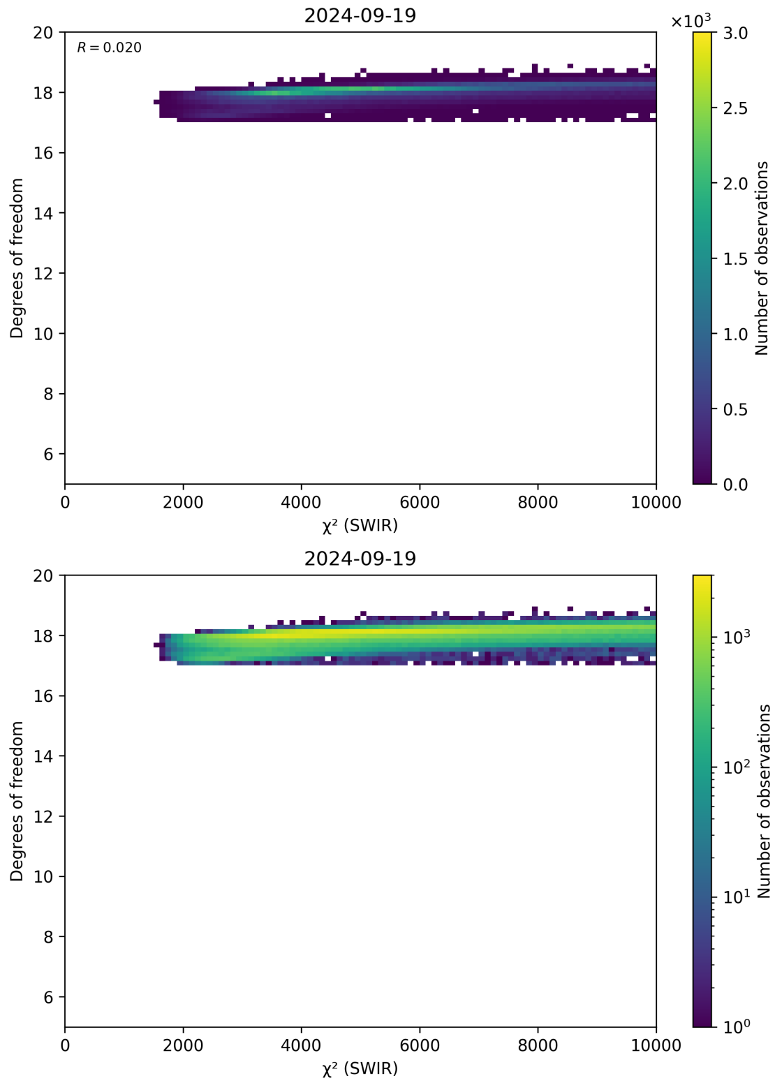
Figure 48: Scatter density plot of “ \chi^2 (SWIR)” against “Degrees of freedom” for 2024-09-18 to 2024-09-20.
