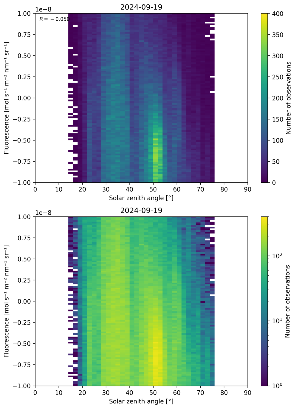
Figure 97: Scatter density plot of “Solar zenith angle” against “Fluorescence” for 2024-09-18 to 2024-09-20.
