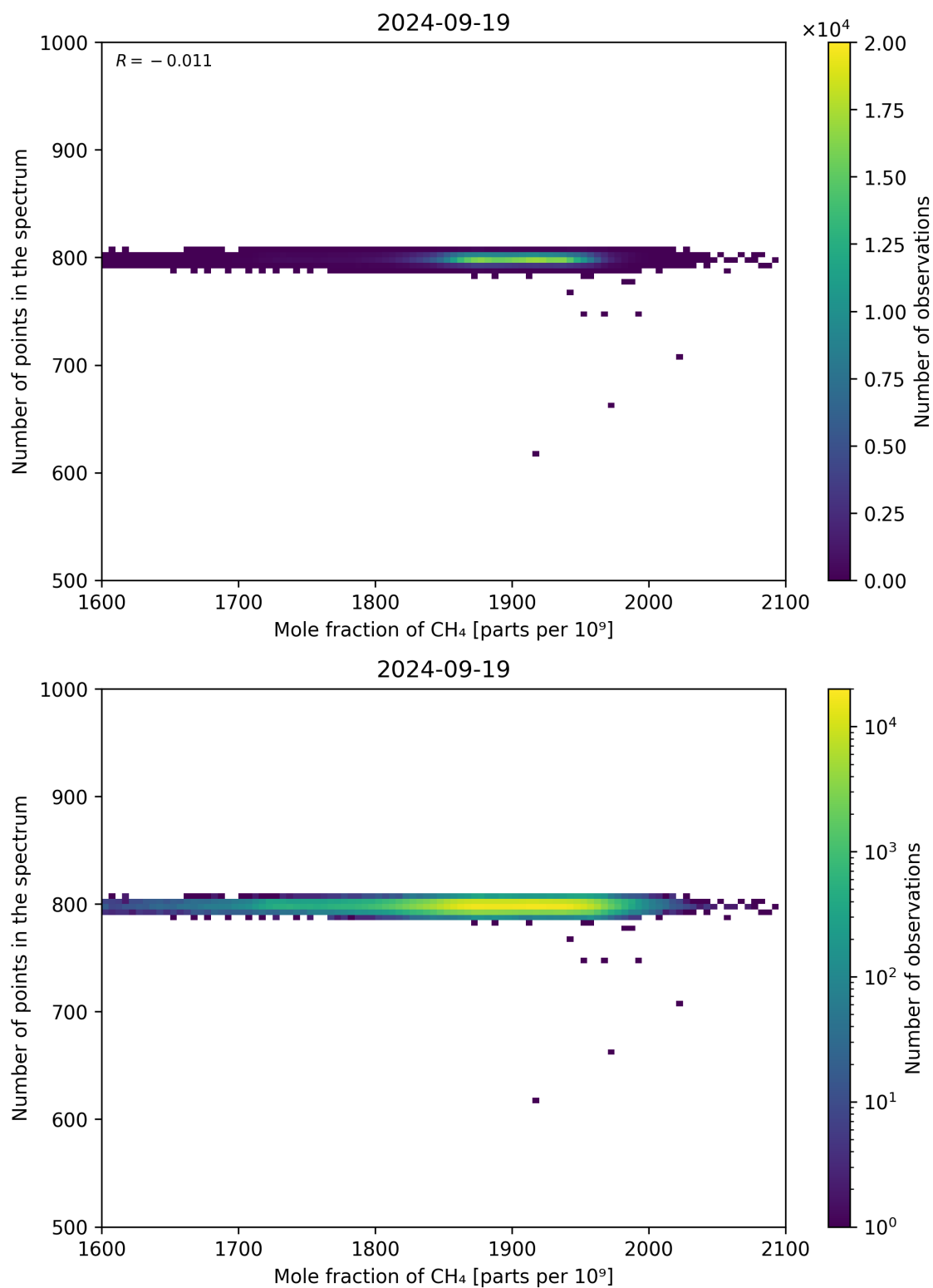
Figure 77: Scatter density plot of “Mole fraction of CH 4 ” against “Number of points in the spectrum” for 2024-09-18 to 2024-09-20.
