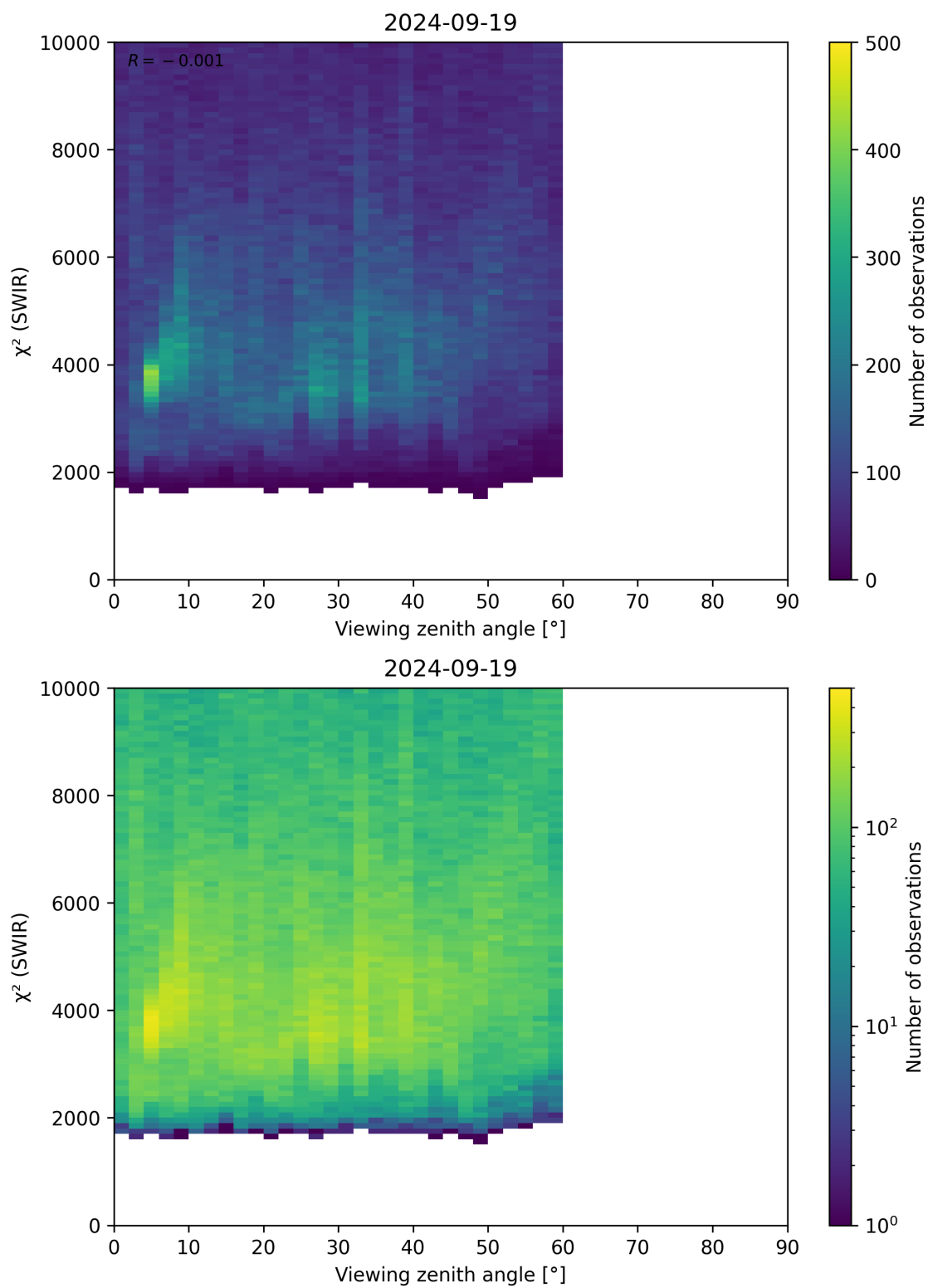
Figure 106: Scatter density plot of “Viewing zenith angle” against “ \chi^2 (SWIR)” for 2024-09-18 to 2024-09-20.
