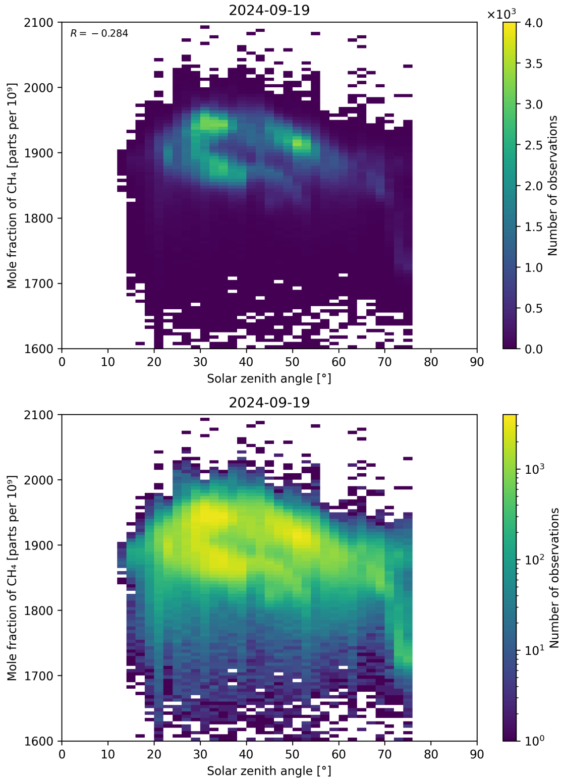
Figure 99: Scatter density plot of “Solar zenith angle” against “Mole fraction of CH 4 ” for 2024-09-18 to 2024-09-20.
