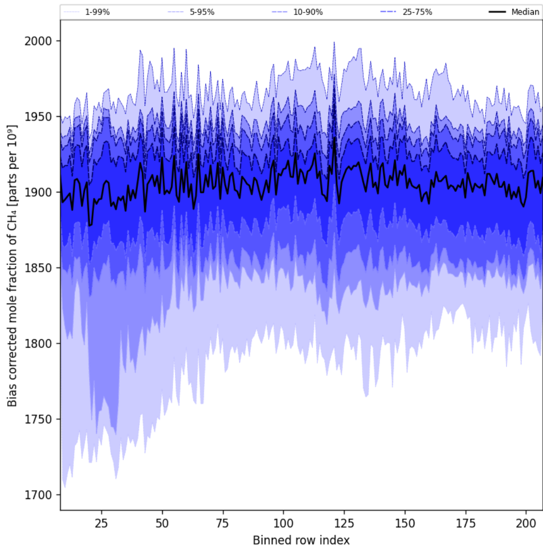
Figure 36: Along track statistics of “Bias corrected mole fraction of CH 4 ” for 2024-09-18 to 2024-09-20
