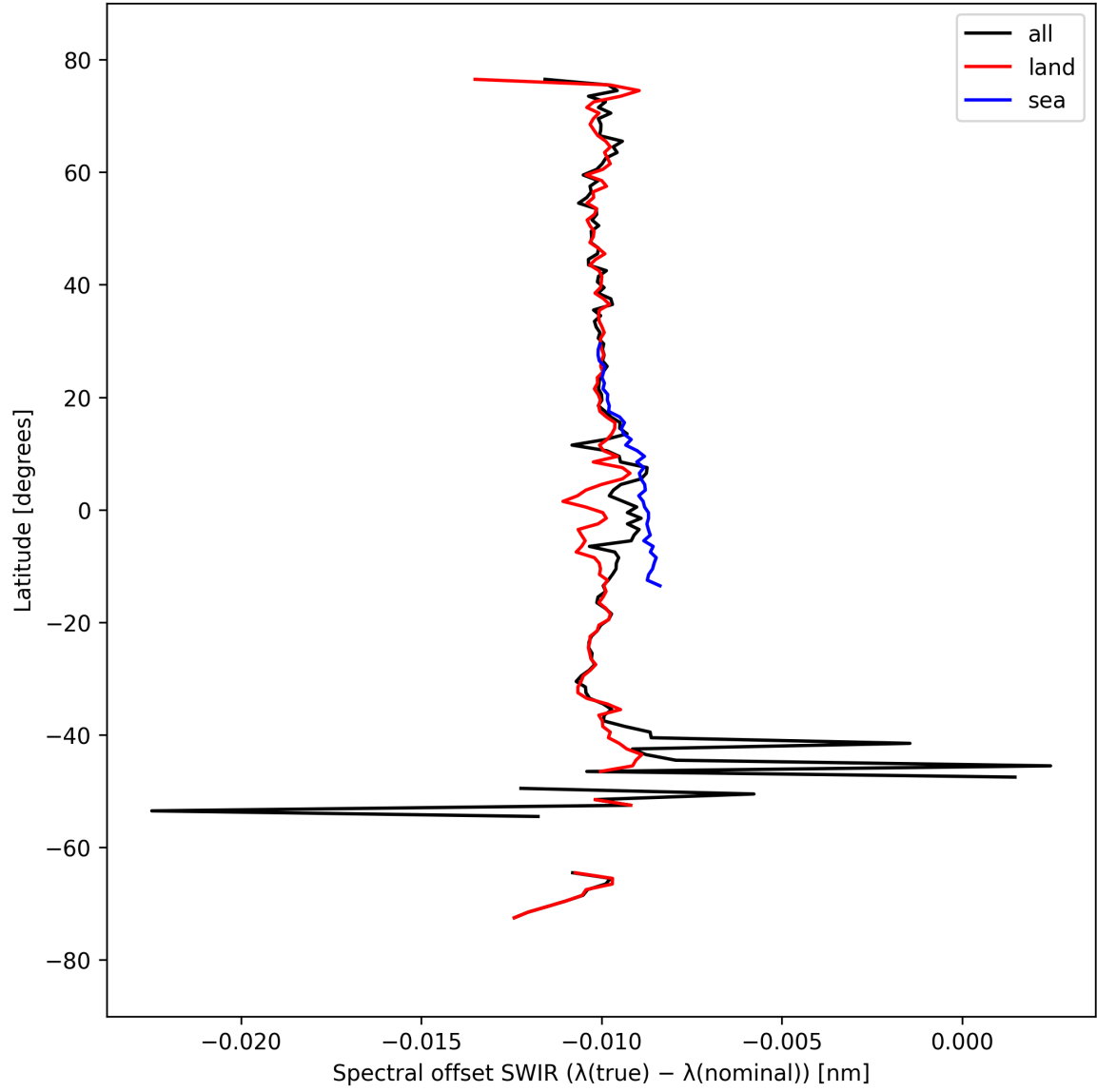
Figure 16: Zonal average of “Spectral offset SWIR ( \lambda_{\text{true}} - \lambda_{\text{nominal}} )” for 2024-09-18 to 2024-09-20.
