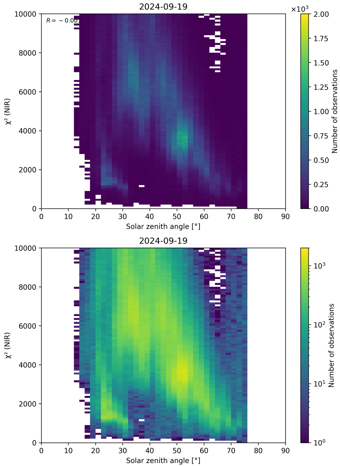
Figure 94: Scatter density plot of “Solar zenith angle” against “ \chi^2 (NIR)” for 2024-09-18 to 2024-09-20.
