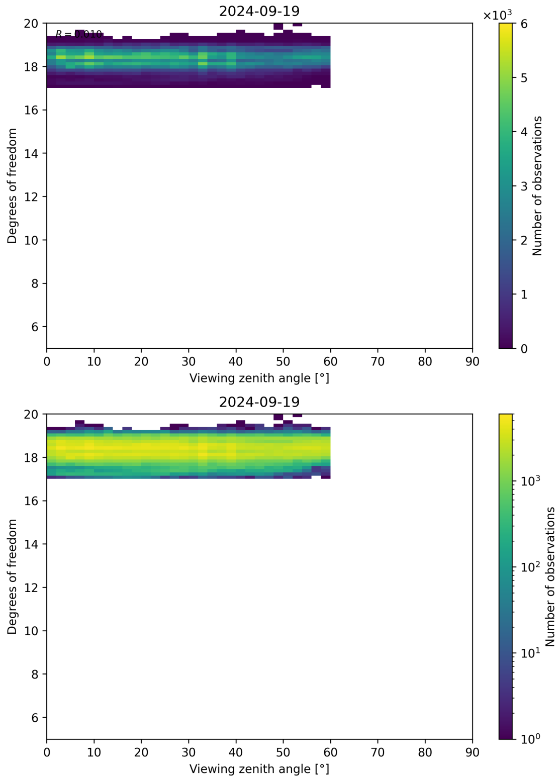
Figure 107: Scatter density plot of “Viewing zenith angle” against “Degrees of freedom” for 2024-09-18 to 2024-09-20.
