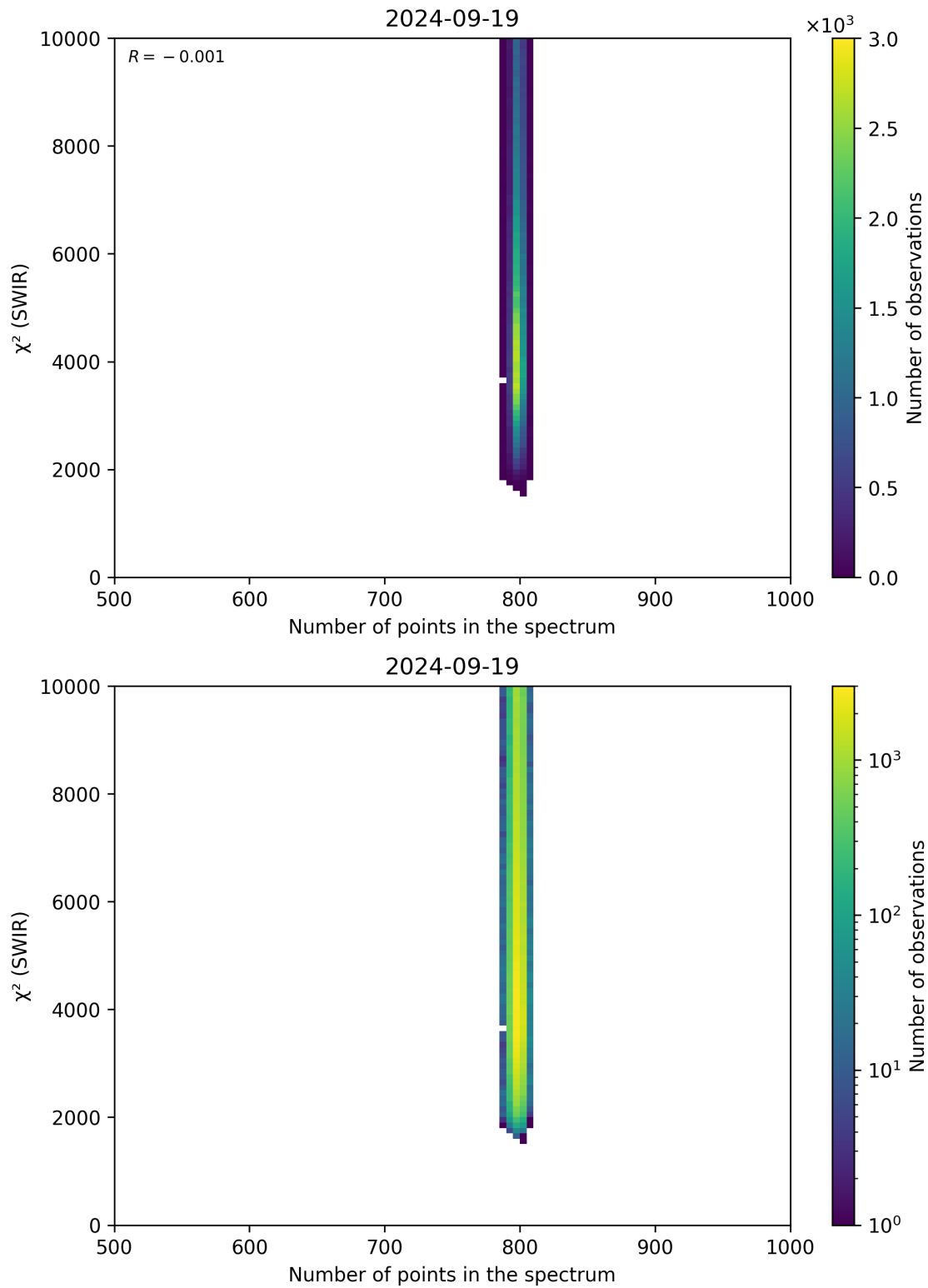
Figure 89: Scatter density plot of “Number of points in the spectrum” against “ \chi^2 (SWIR)” for 2024-09-18 to 2024-09-20.
