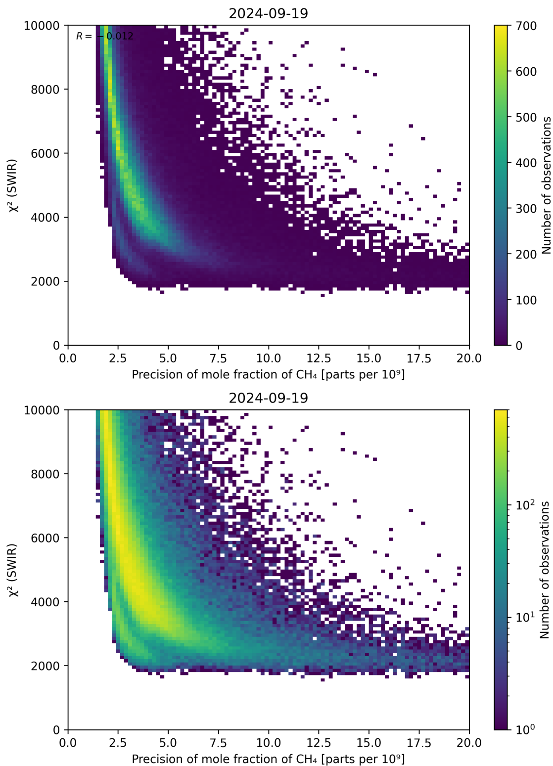
Figure 79: Scatter density plot of “Precision of mole fraction of \text{CH}_4 ” against “ \chi^2 (SWIR)” for 2024-09-18 to 2024-09-20.
