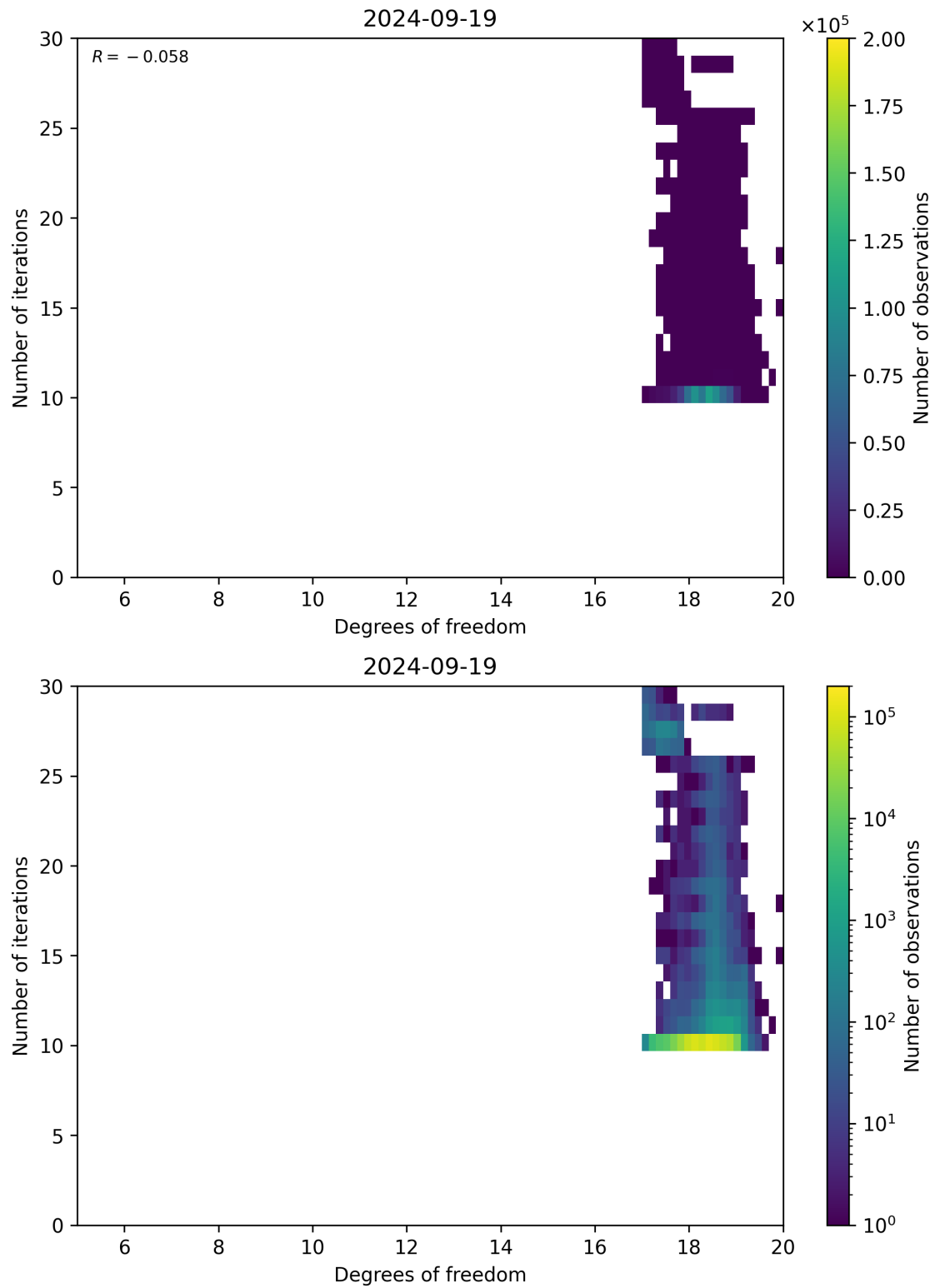
Figure 52: Scatter density plot of “Degrees of freedom” against “Number of iterations” for 2024-09-18 to 2024-09-20.
