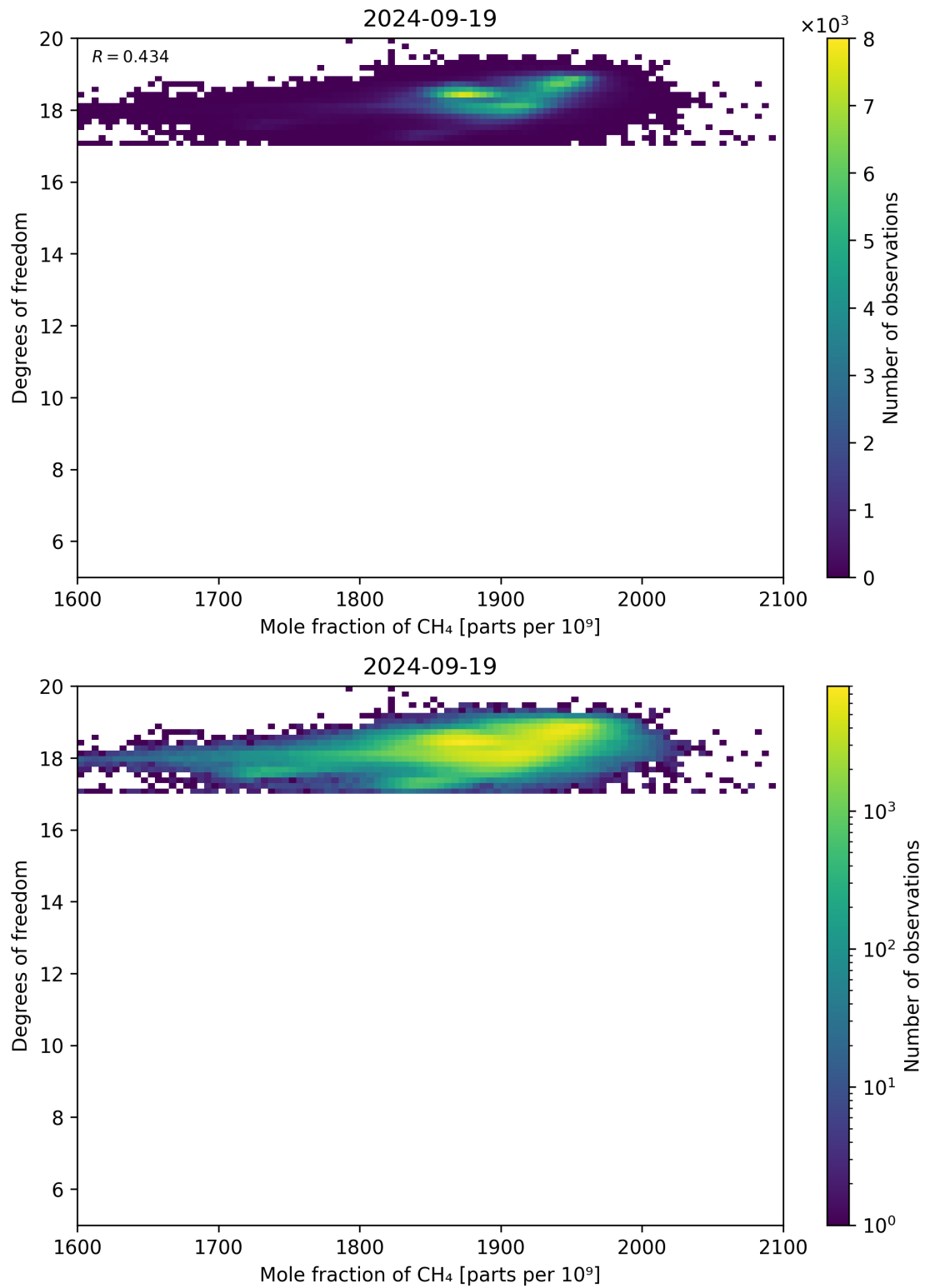
Figure 72: Scatter density plot of “Mole fraction of CH 4 ” against “Degrees of freedom” for 2024-09-18 to 2024-09-20.
