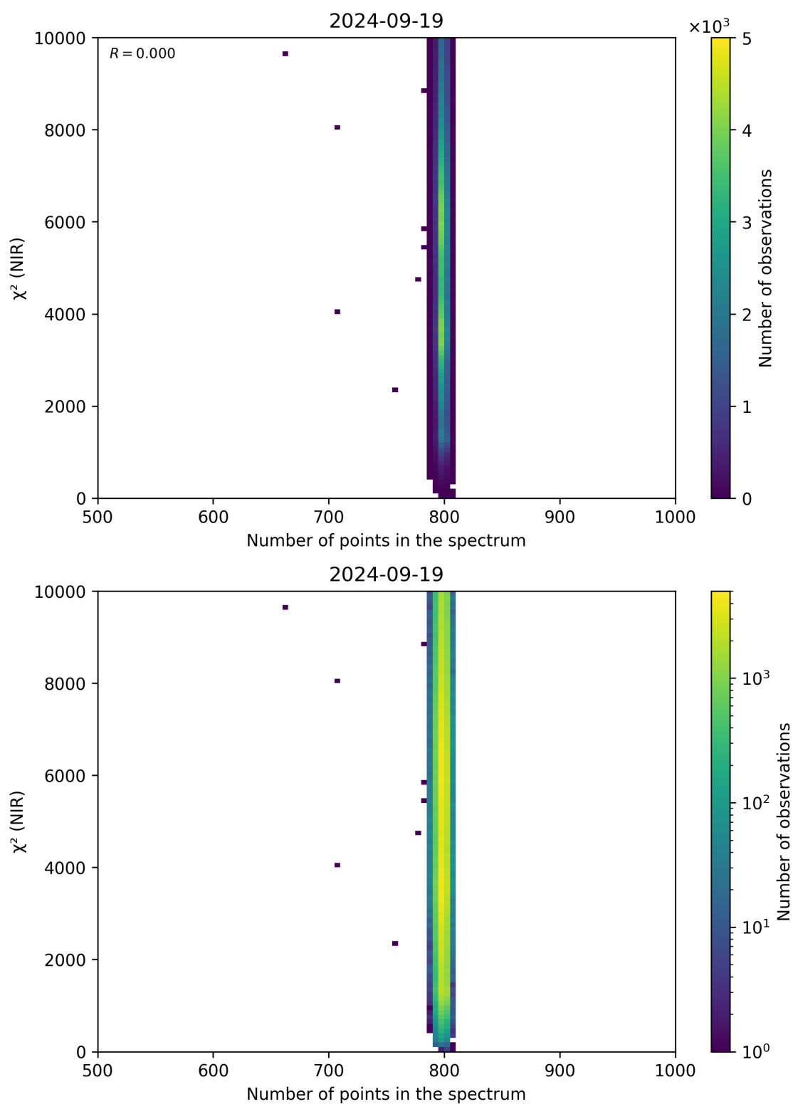
Figure 88: Scatter density plot of “Number of points in the spectrum” against “ \chi^2 (NIR)” for 2024-09-18 to 2024-09-20.
