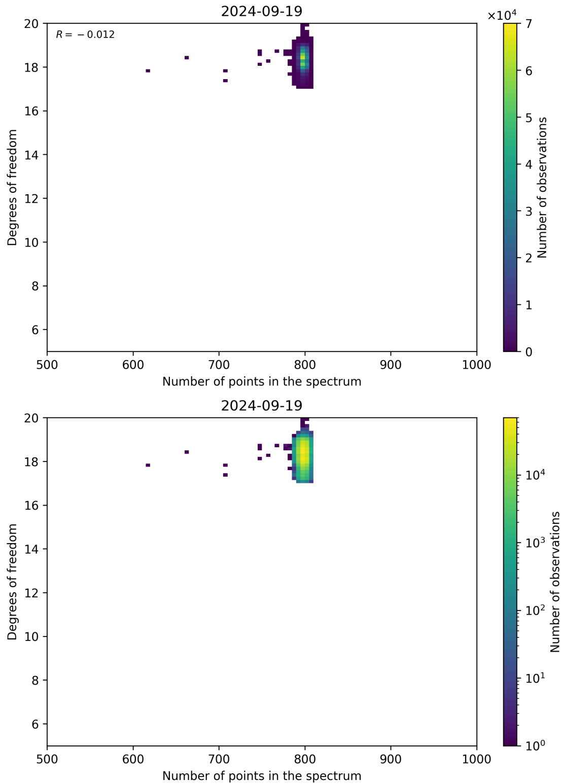
Figure 90: Scatter density plot of “Number of points in the spectrum” against “Degrees of freedom” for 2024-09-18 to 2024-09-20.
