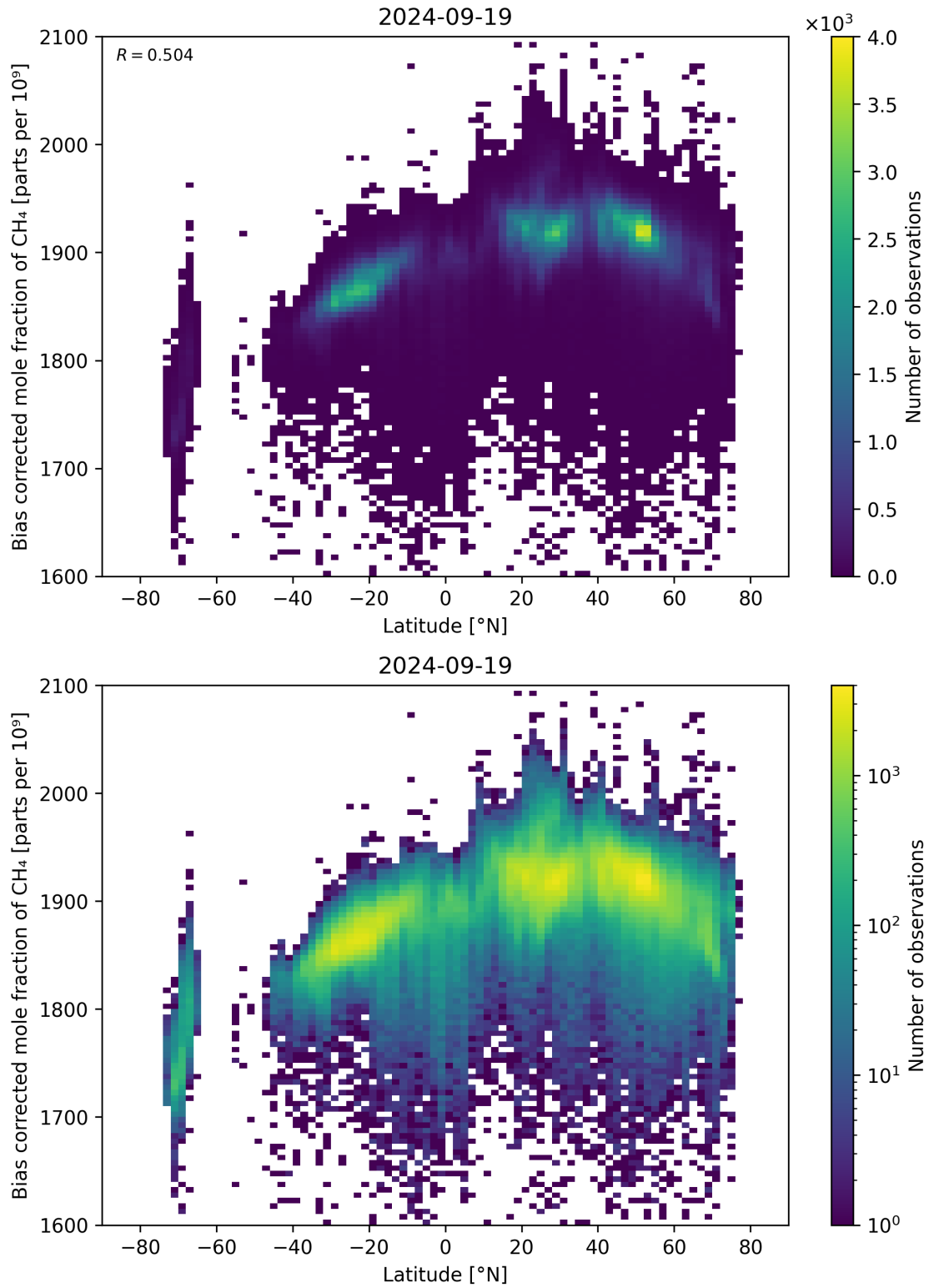
Figure 58: Scatter density plot of “Latitude” against “Bias corrected mole fraction of \text{CH}_4 ” for 2024-09-18 to 2024-09-20.
