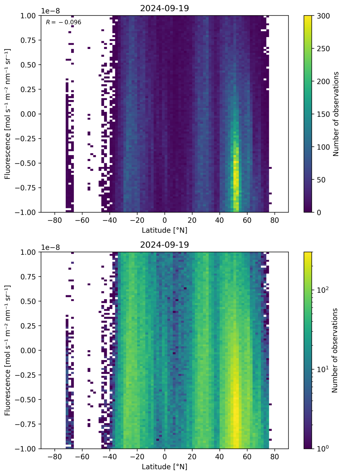
Figure 56: Scatter density plot of “Latitude” against “Fluorescence” for 2024-09-18 to 2024-09-20.
