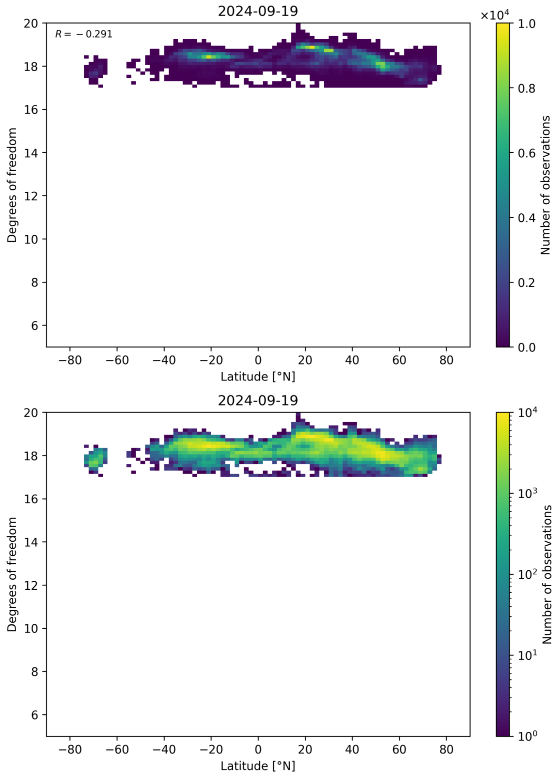
Figure 55: Scatter density plot of “Latitude” against “Degrees of freedom” for 2024-09-18 to 2024-09-20.
