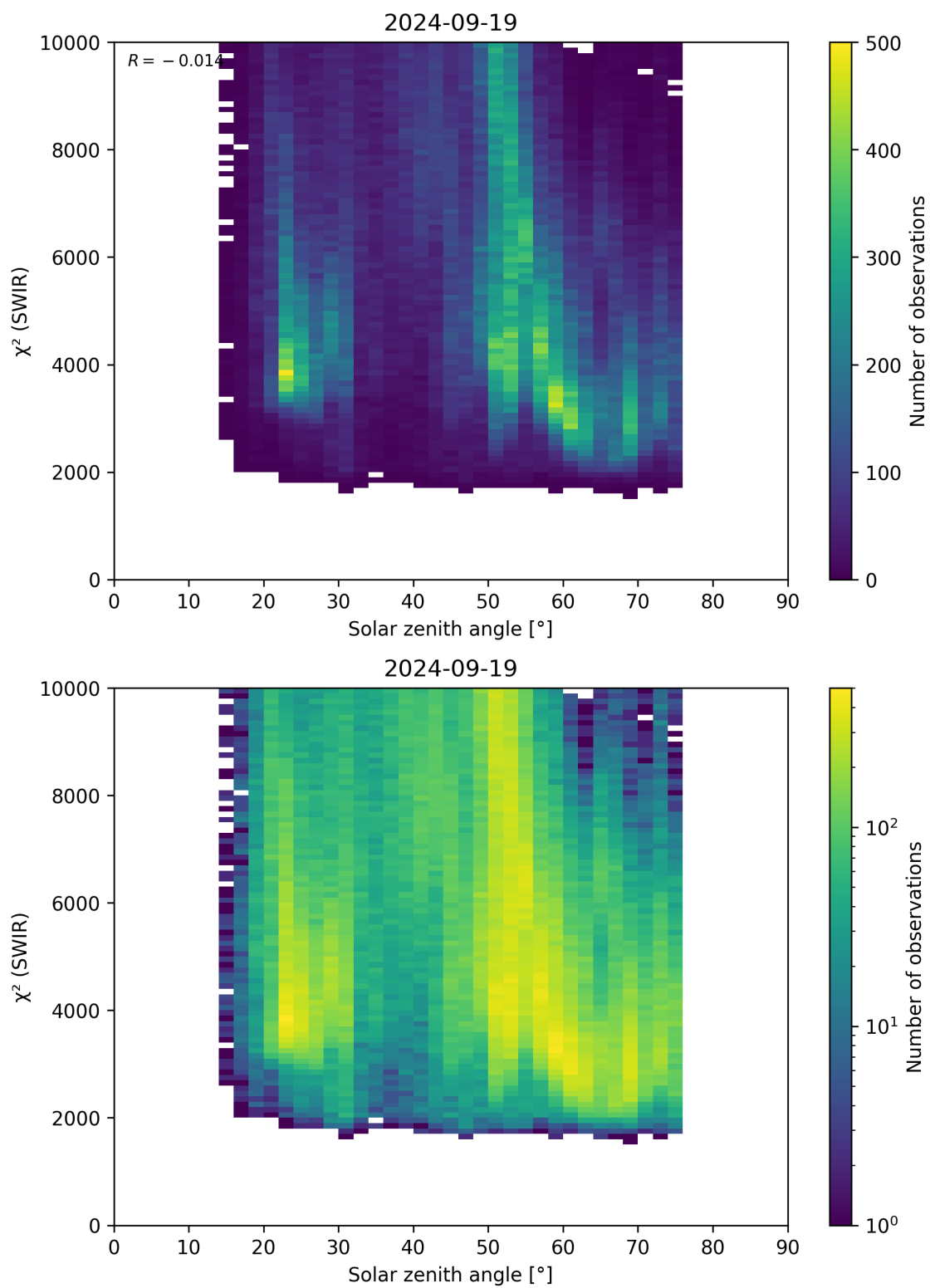
Figure 95: Scatter density plot of “Solar zenith angle” against “ \chi^2 (SWIR)” for 2024-09-18 to 2024-09-20.
