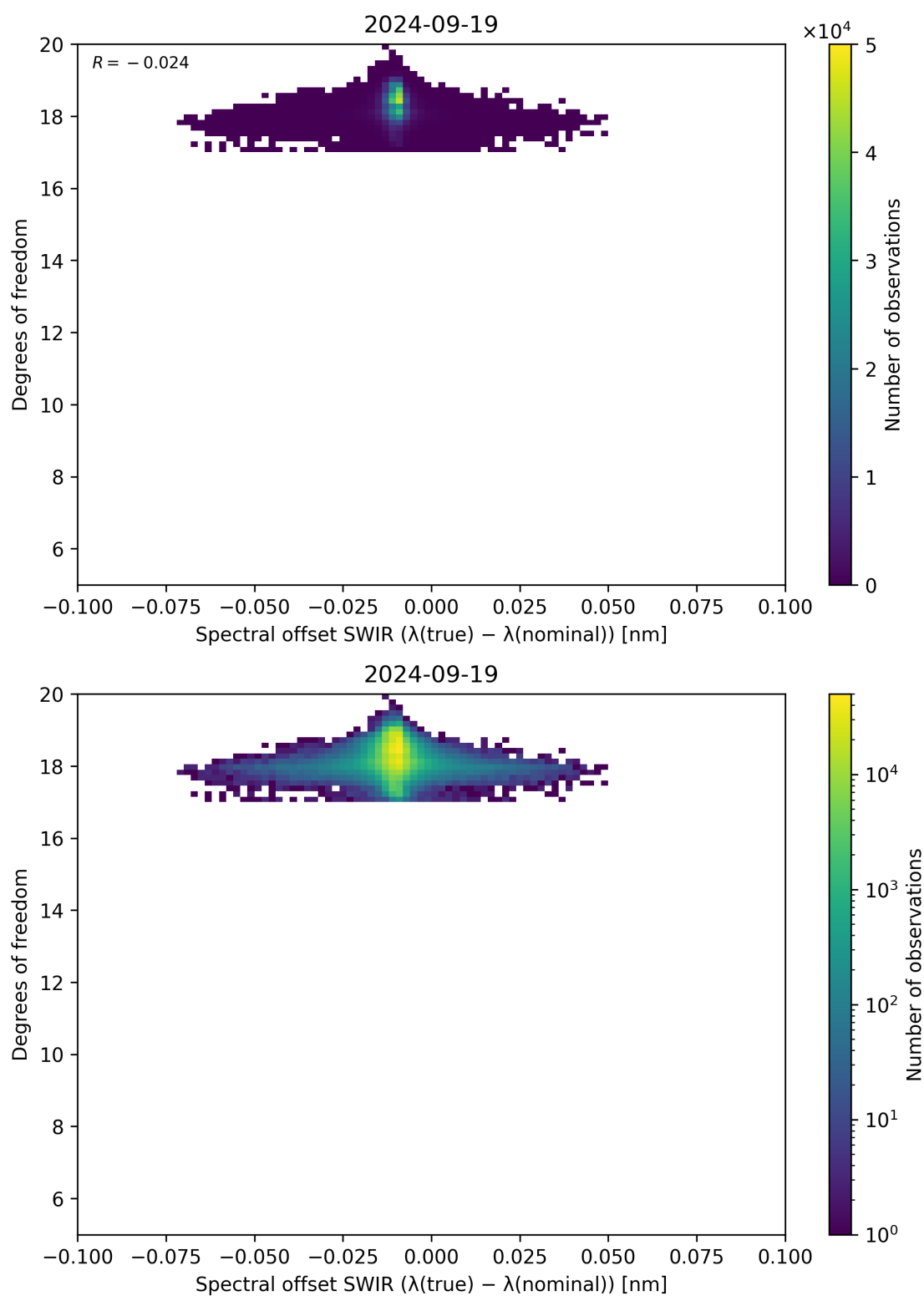
Figure 119: Scatter density plot of “Spectral offset SWIR ( \lambda_{\text{true}} - \lambda_{\text{nominal}} )” against “Degrees of freedom” for 2024-09-18 to 2024-09-20.
