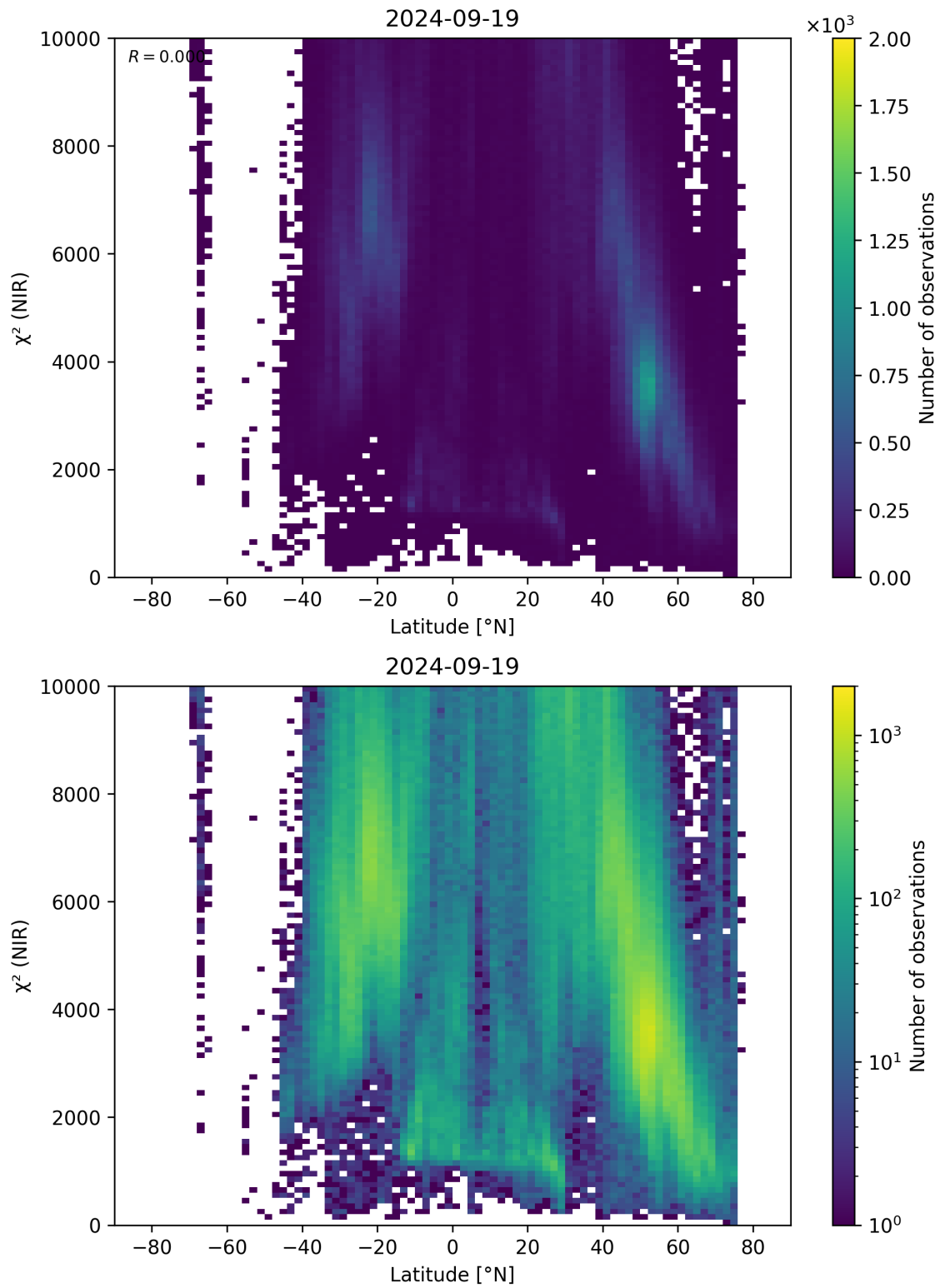
Figure 53: Scatter density plot of “Latitude” against “ \chi^2 (NIR)” for 2024-09-18 to 2024-09-20.
