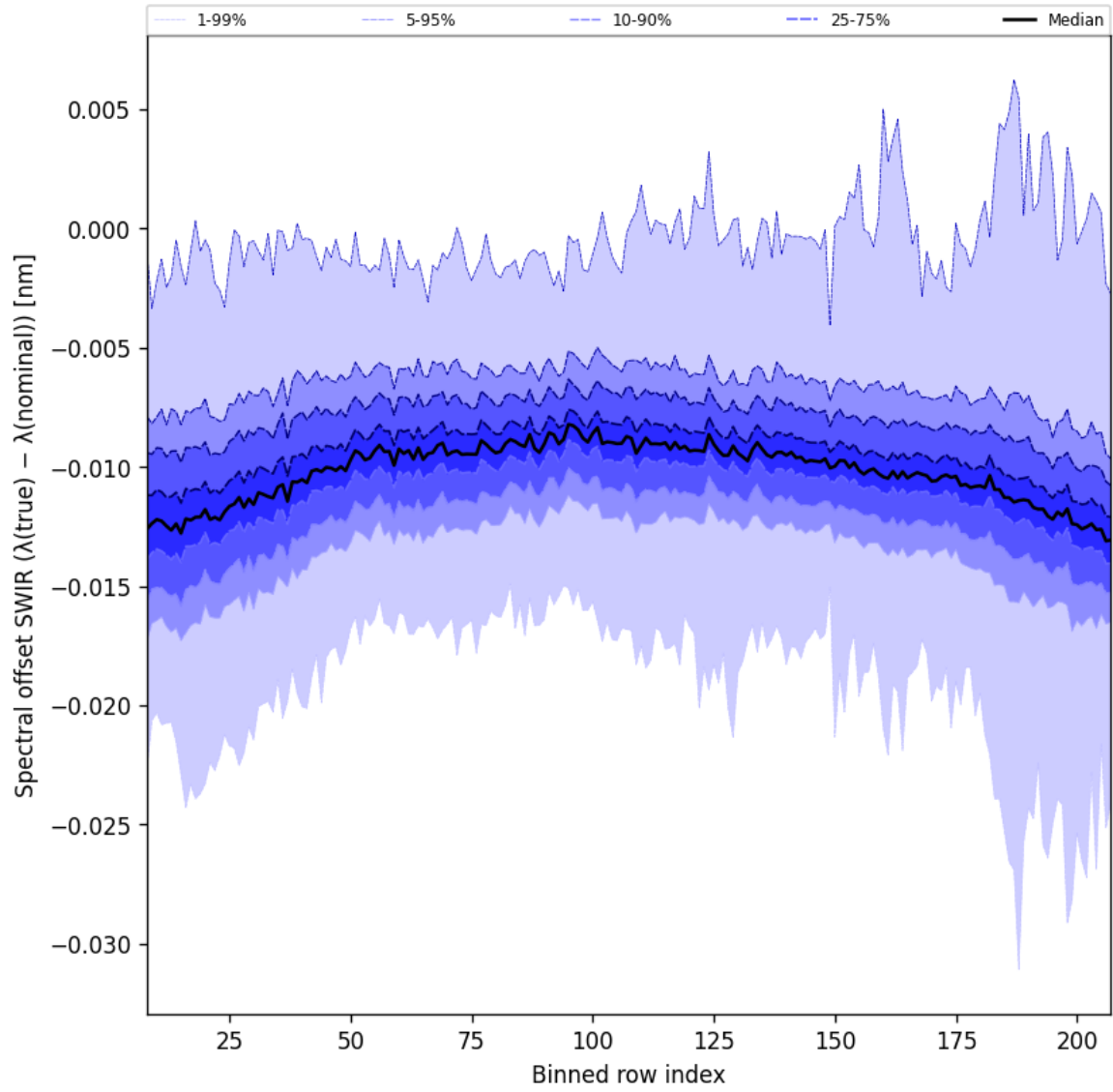
Figure 38: Along track statistics of “Spectral offset SWIR ( \lambda_{\text{true}} - \lambda_{\text{nominal}} )” for 2024-09-18 to 2024-09-20
