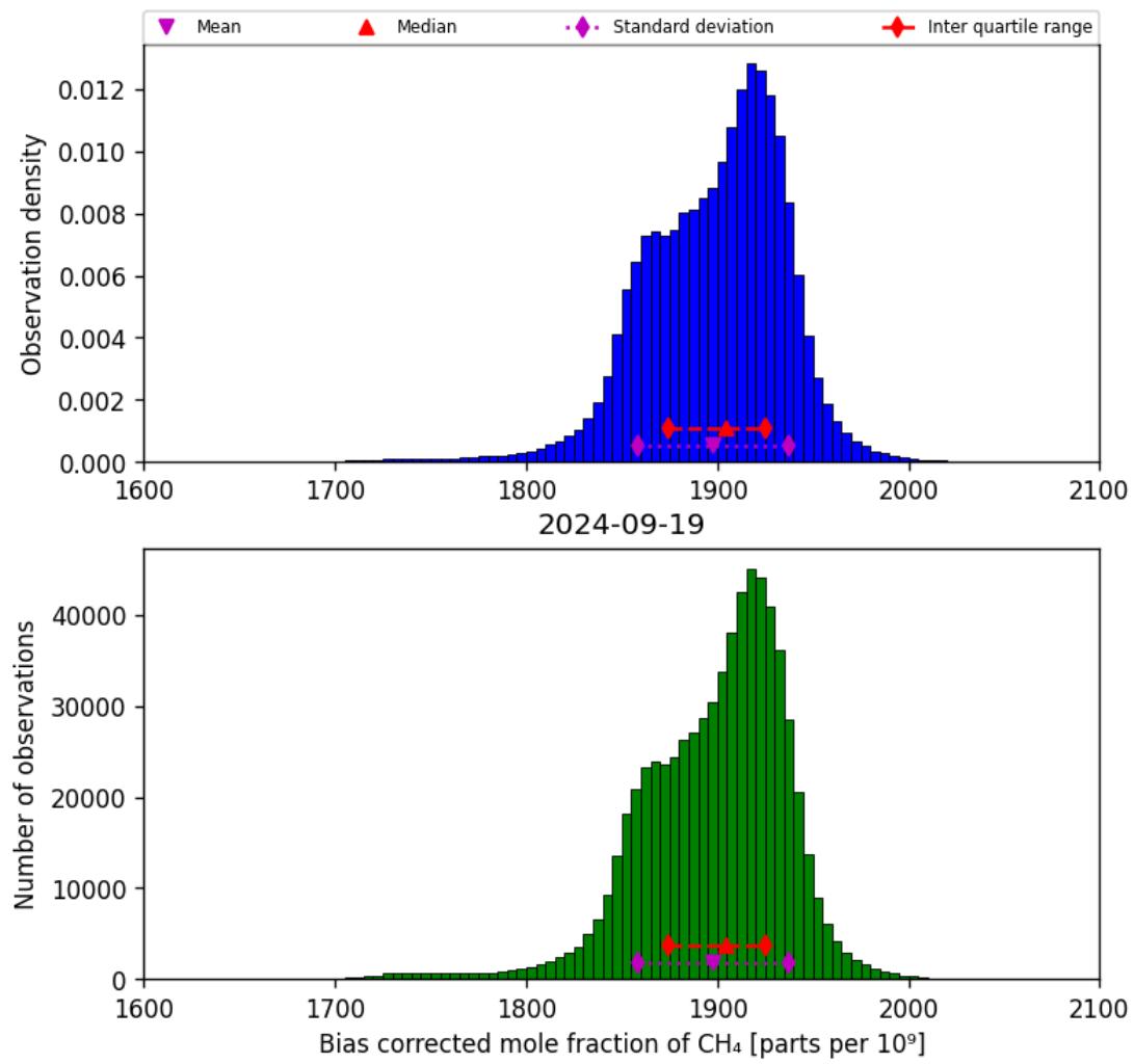
Figure 25: Histogram of “Bias corrected mole fraction of CH 4 ” for 2024-09-18 to 2024-09-20
