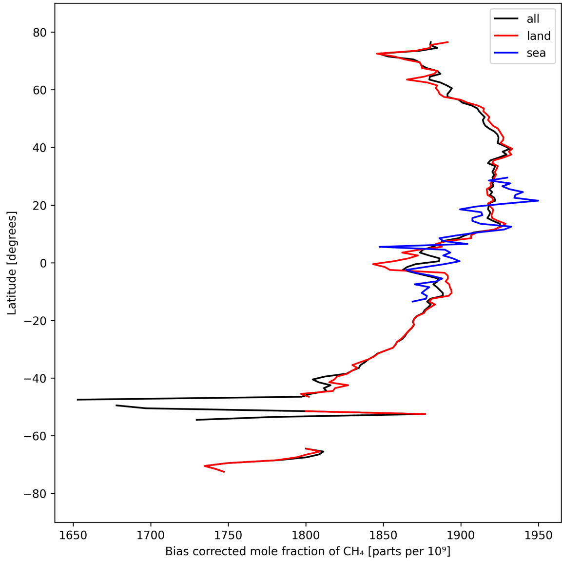
Figure 14: Zonal average of “Bias corrected mole fraction of \text{CH}_4 ” for 2024-09-18 to 2024-09-20.
