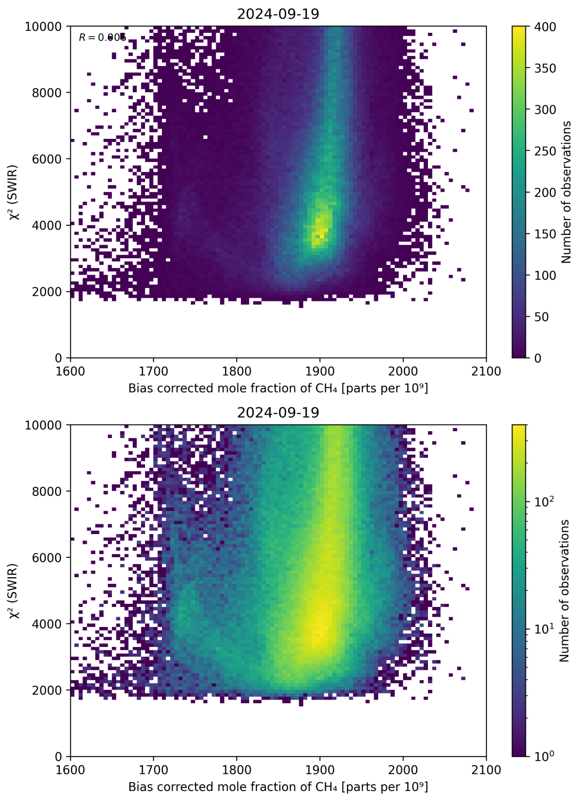
Figure 64: Scatter density plot of “Bias corrected mole fraction of \text{CH}_4 ” against “ \chi^2 (SWIR)” for 2024-09-18 to 2024-09-20.
