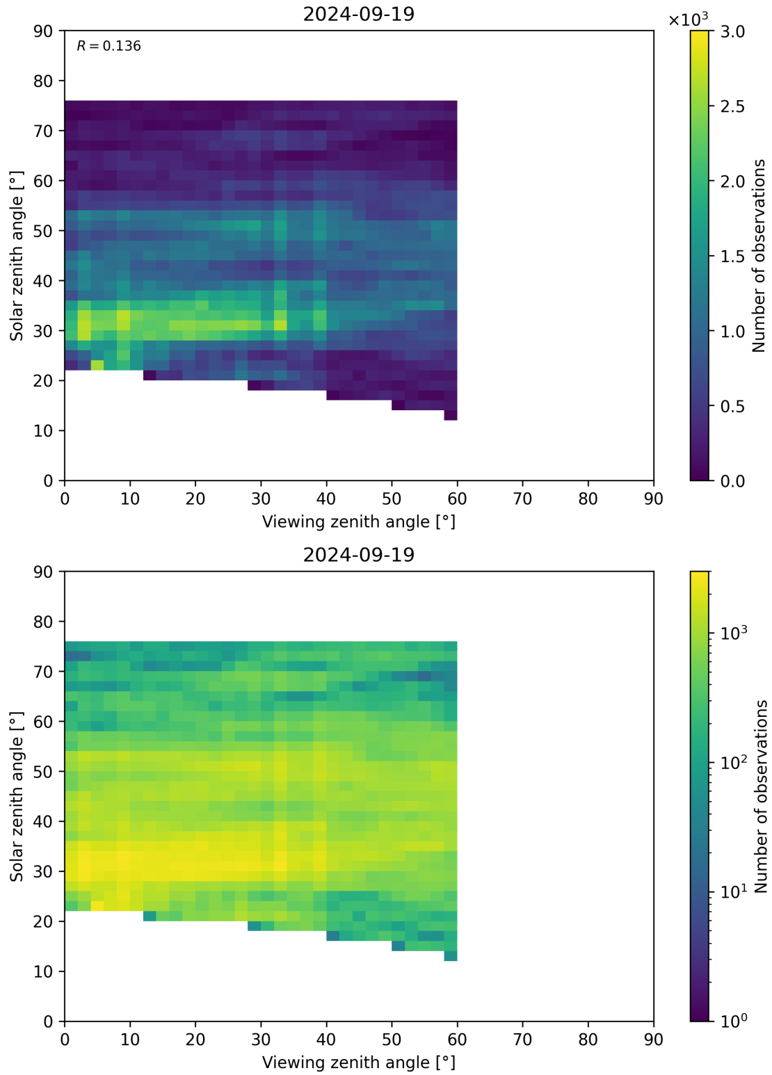
Figure 115: Scatter density plot of “Viewing zenith angle” against “Solar zenith angle” for 2024-09-18 to 2024-09-20.
