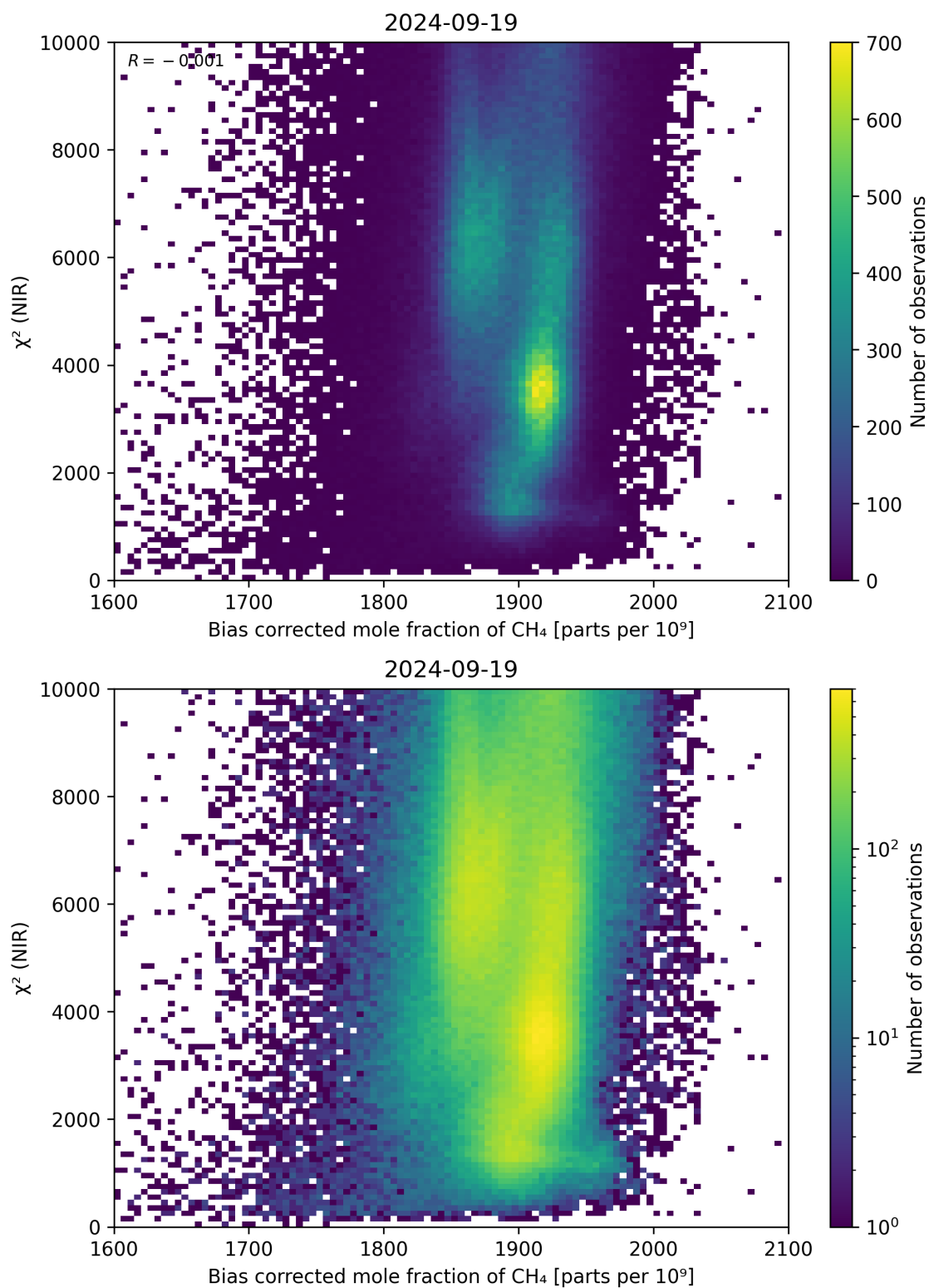
Figure 63: Scatter density plot of “Bias corrected mole fraction of CH 4 ” against “ \chi^2 (NIR)” for 2024-09-18 to 2024-09-20.
