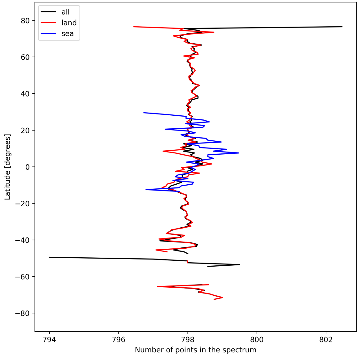
Figure 15: Zonal average of “Number of points in the spectrum” for 2024-09-18 to 2024-09-20.
