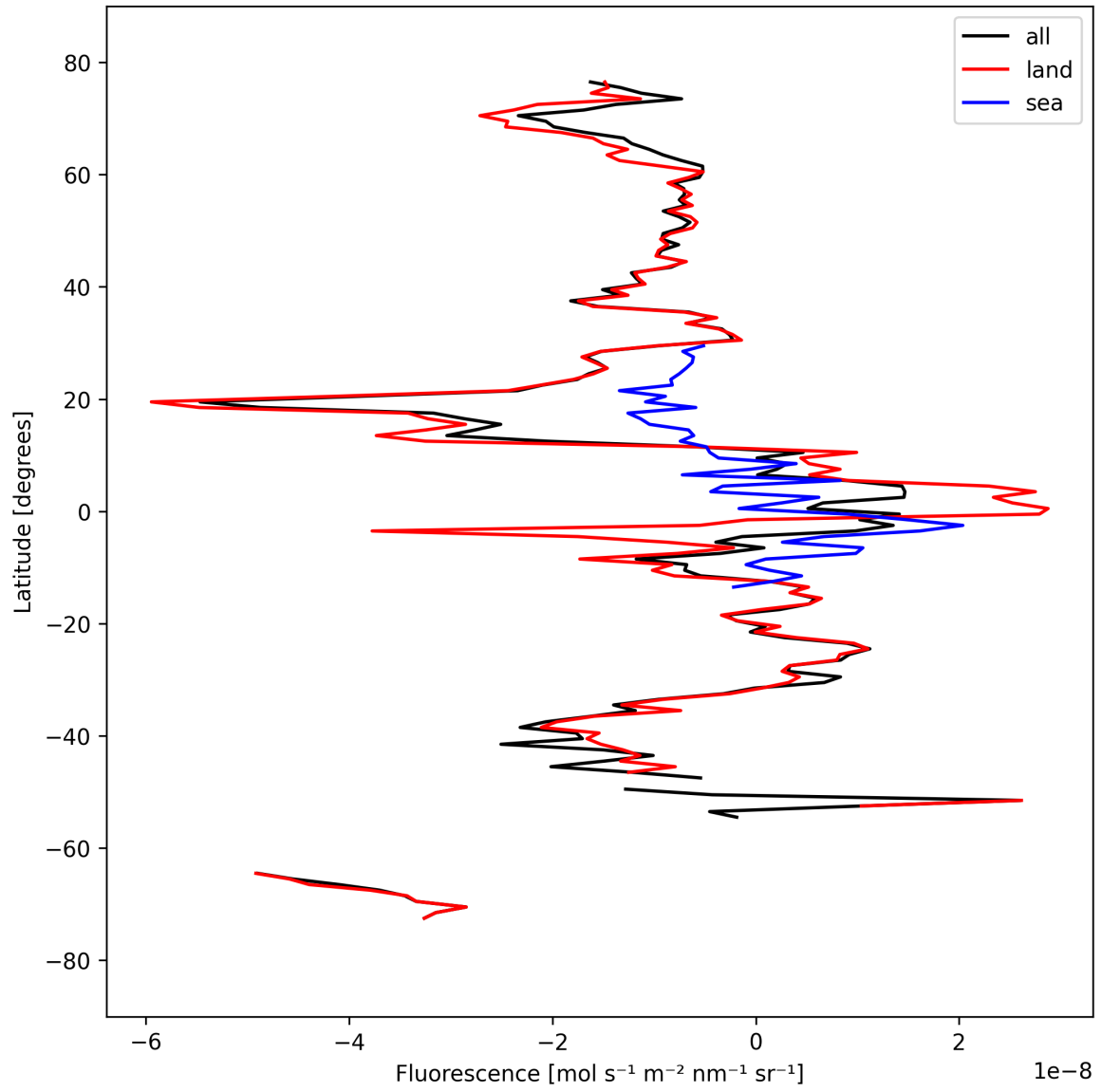
Figure 21: Zonal average of “Fluorescence” for 2024-09-18 to 2024-09-20.
