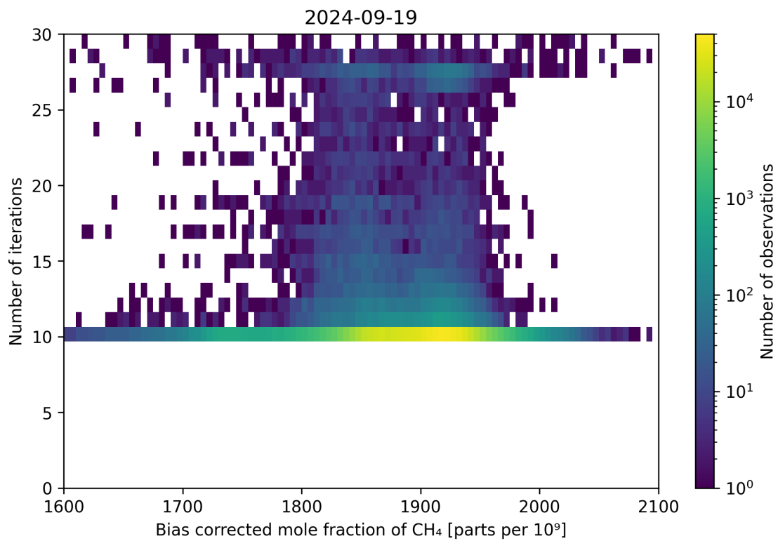
Figure 67: Scatter density plot of “Bias corrected mole fraction of CH 4 ” against “Number of iterations” for 2024-09-18 to 2024-09-20.
