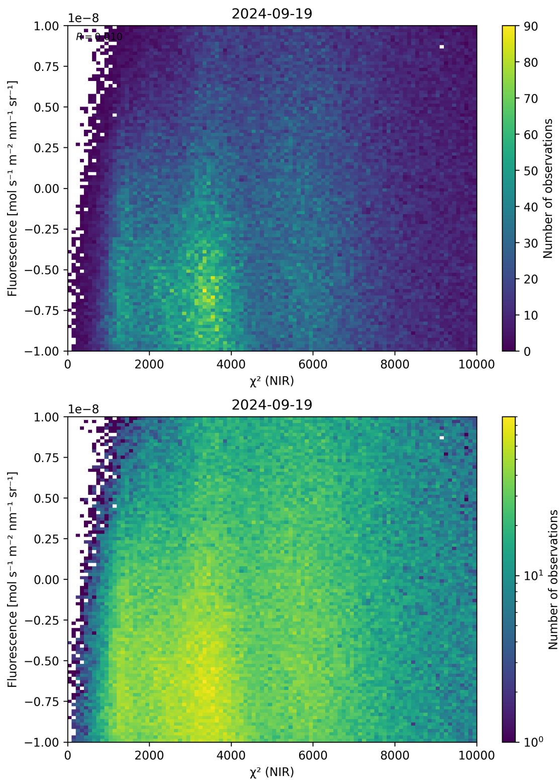
Figure 45: Scatter density plot of “ \chi^2 (NIR)” against “Fluorescence” for 2024-09-18 to 2024-09-20.
