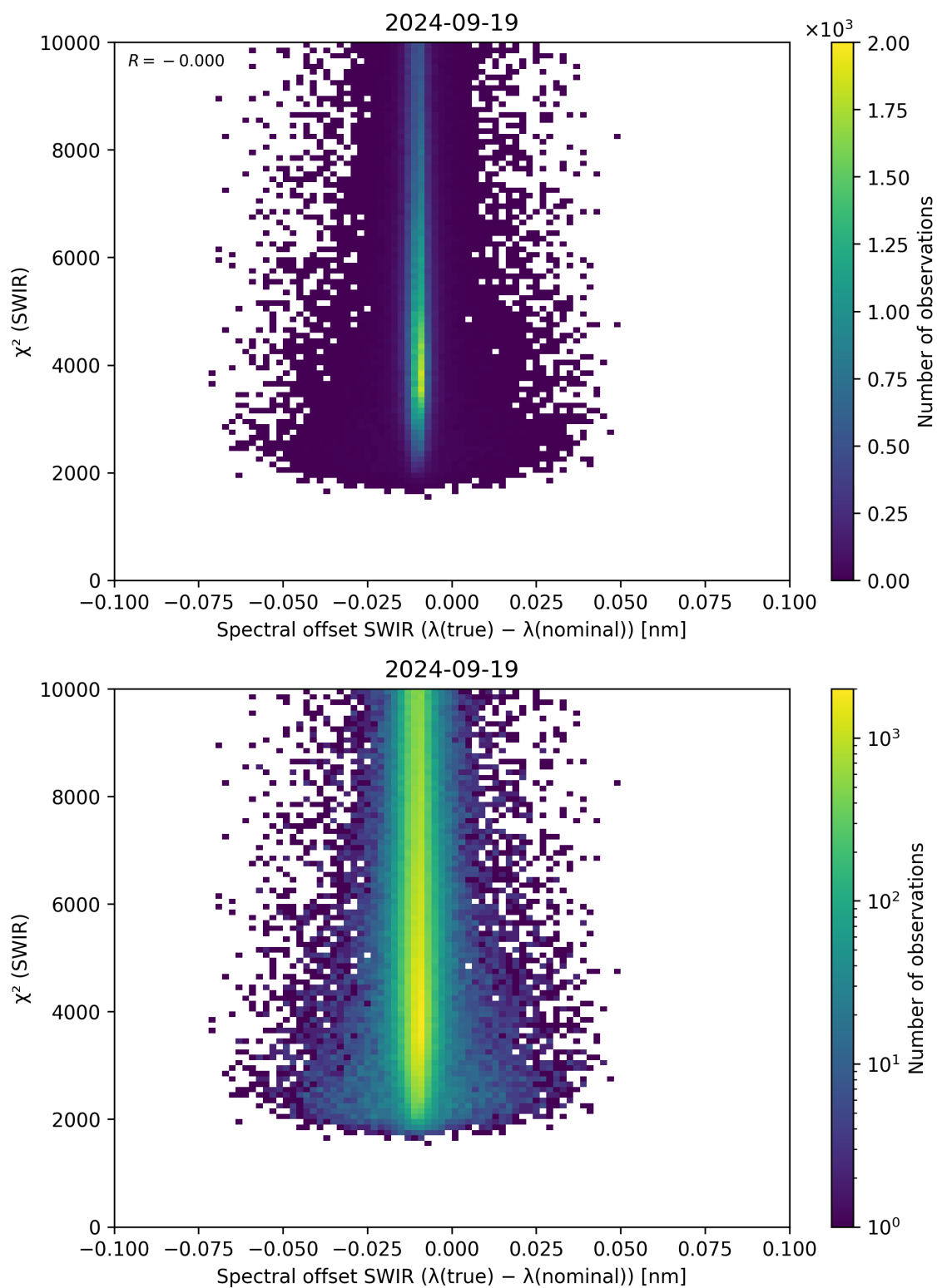
Figure 118: Scatter density plot of “Spectral offset SWIR ( \lambda_{\text{true}} - \lambda_{\text{nominal}} )” against “ \chi^2 (SWIR)” for 2024-09-18 to 2024-09-20.
