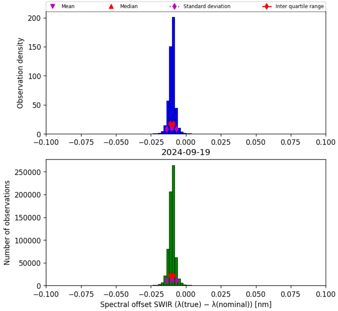
Figure 27: Histogram of “Spectral offset SWIR ( \lambda_{\text{true}} - \lambda_{\text{nominal}} )” for 2024-09-18 to 2024-09-20
