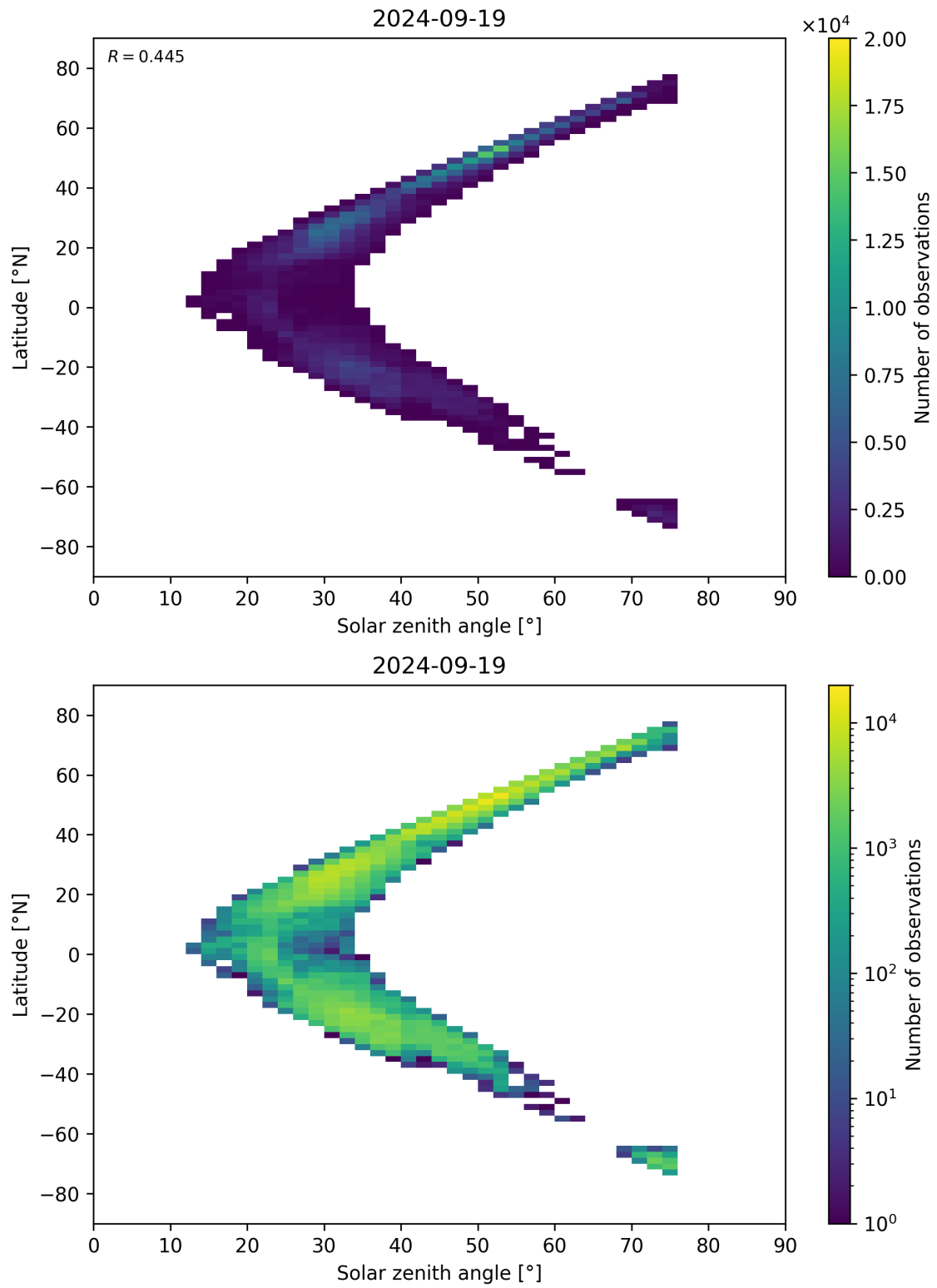
Figure 98: Scatter density plot of “Solar zenith angle” against “Latitude” for 2024-09-18 to 2024-09-20.
