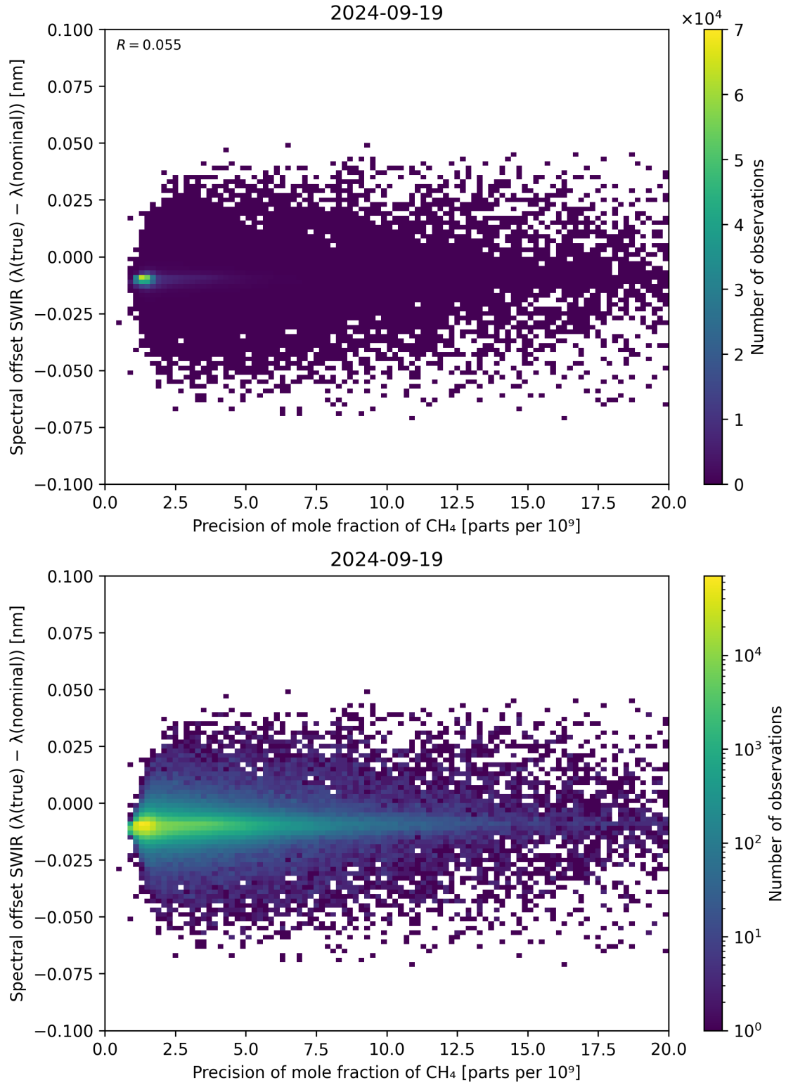
Figure 85: Scatter density plot of “Precision of mole fraction of CH 4 ” against “Spectral offset SWIR ( \lambda_{\text{true}} - \lambda_{\text{nominal}} )” for 2024-09-18 to 2024-09-20.
