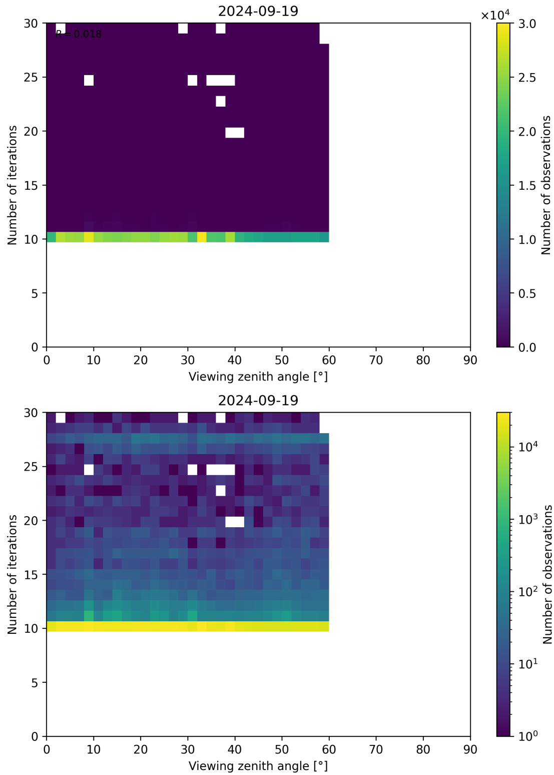
Figure 113: Scatter density plot of “Viewing zenith angle” against “Number of iterations” for 2024-09-18 to 2024-09-20.
