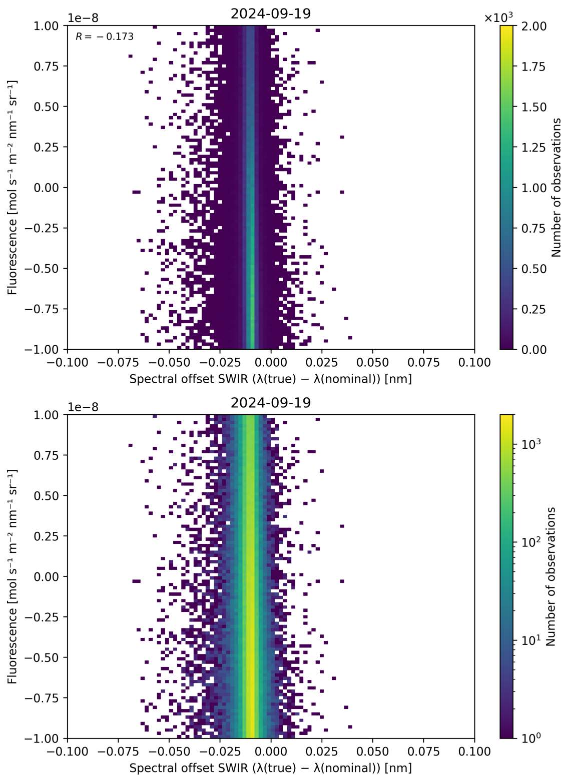
Figure 120: Scatter density plot of “Spectral offset SWIR ( \lambda_{\text{true}} - \lambda_{\text{nominal}} )” against “Fluorescence” for 2024-09-18 to 2024-09-20.
