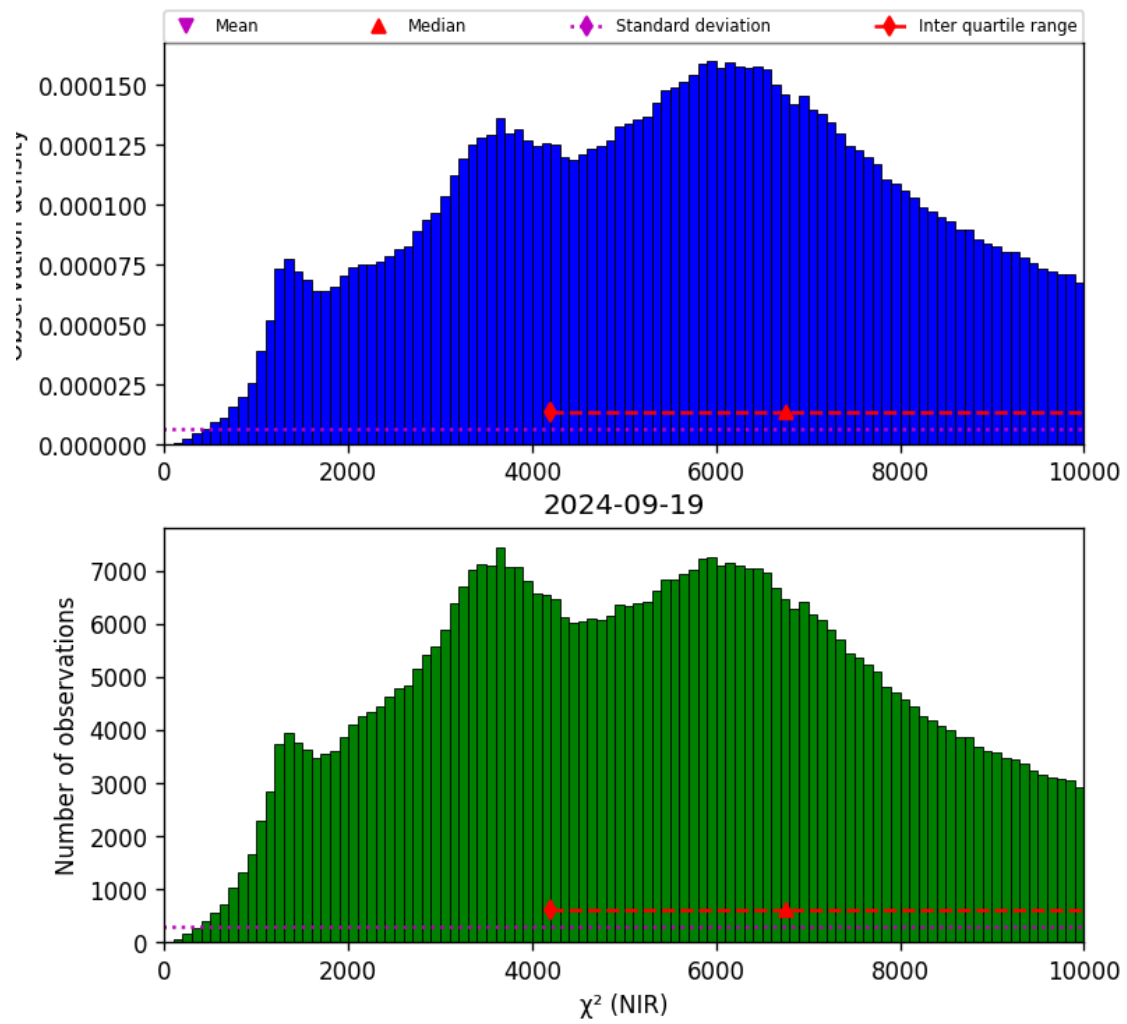
Figure 29: Histogram of “ \chi^2 (NIR)” for 2024-09-18 to 2024-09-20
