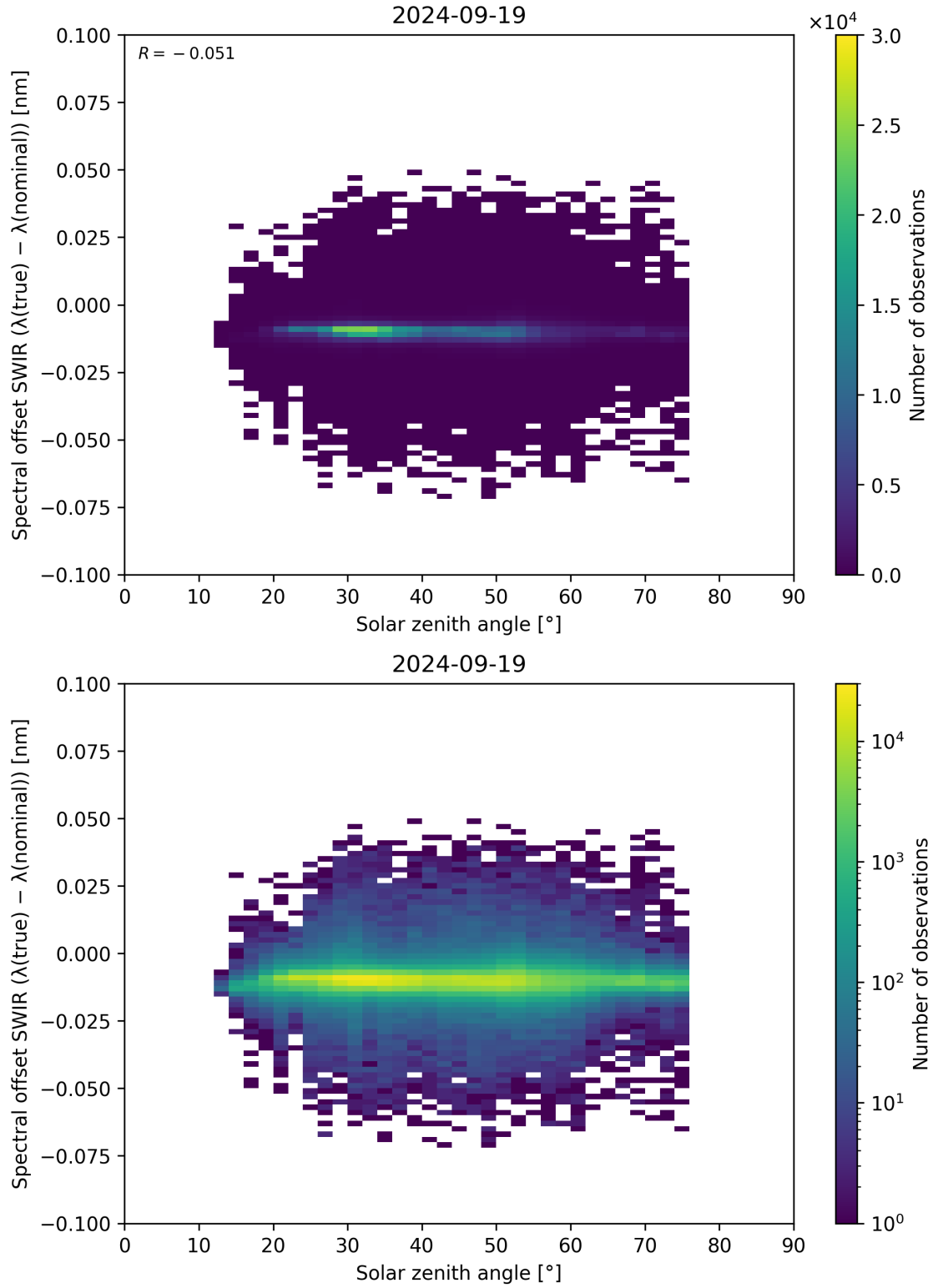
Figure 104: Scatter density plot of “Solar zenith angle” against “Spectral offset SWIR ( \lambda_{\text{true}} - \lambda_{\text{nominal}} )” for 2024-09-18 to 2024-09-20.
