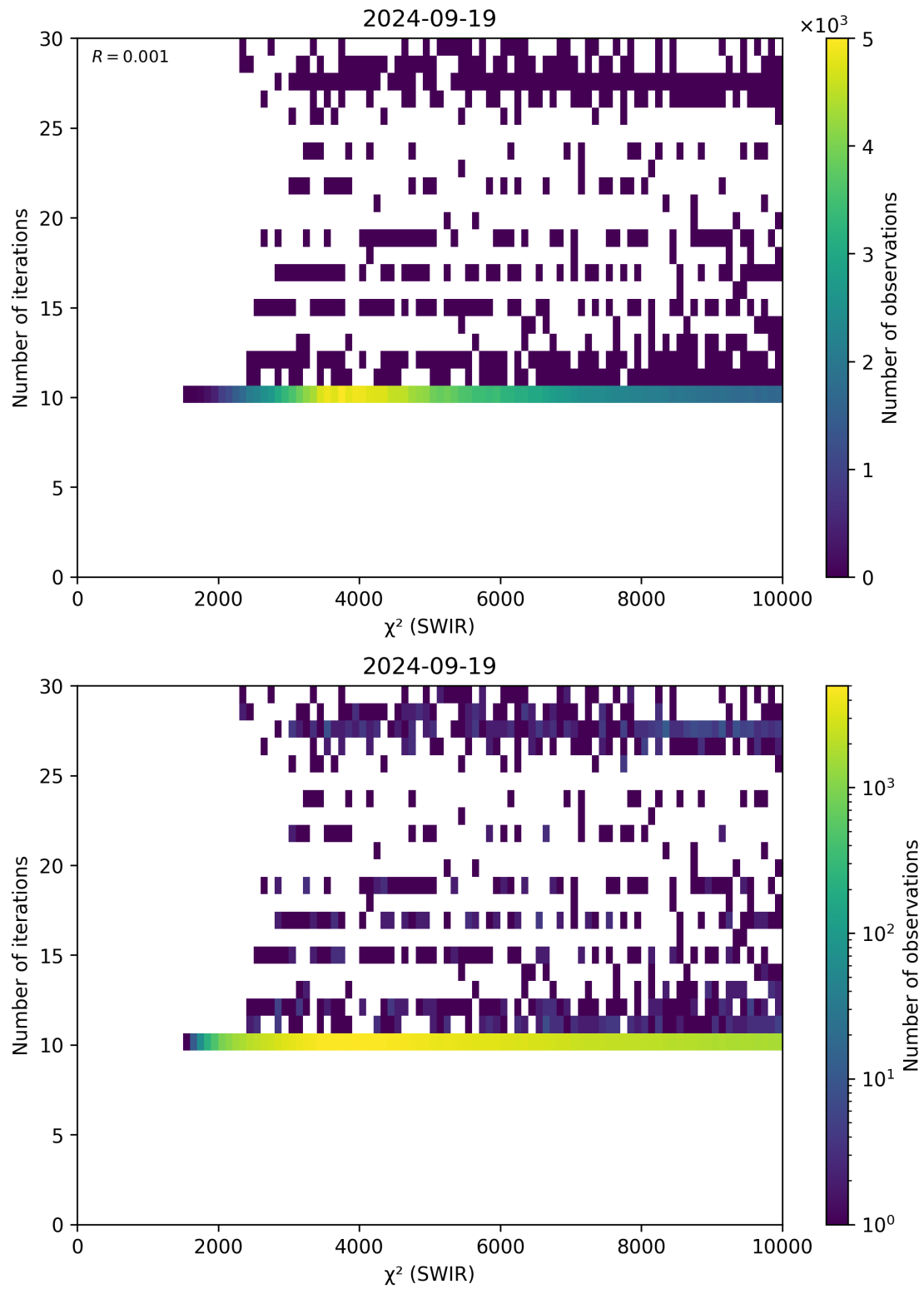
Figure 50: Scatter density plot of “ \chi^2 (SWIR)” against “Number of iterations” for 2024-09-18 to 2024-09-20.
