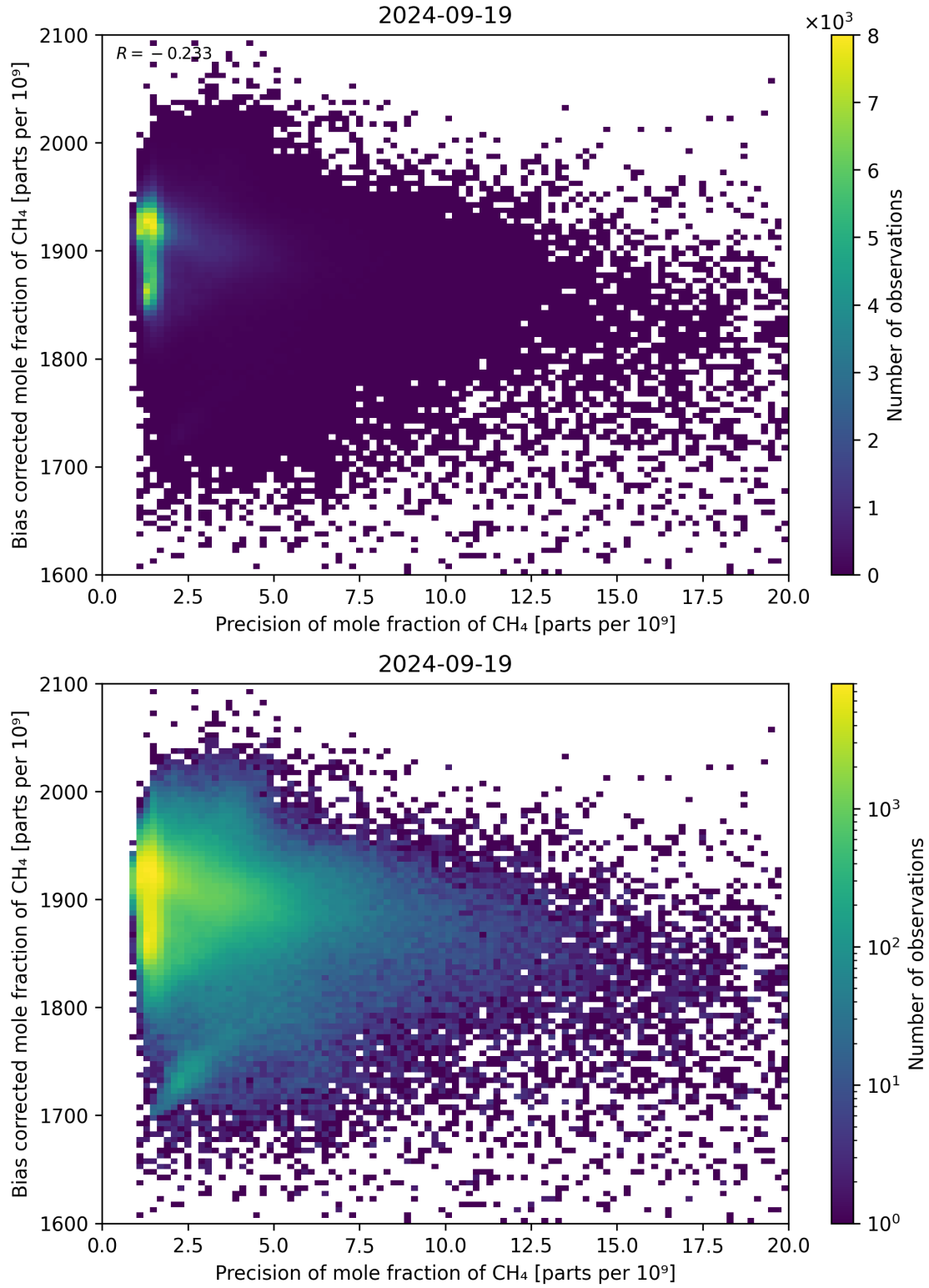
Figure 82: Scatter density plot of “Precision of mole fraction of CH 4 ” against “Bias corrected mole fraction of CH 4 ” for 2024-09-18 to 2024-09-20.
