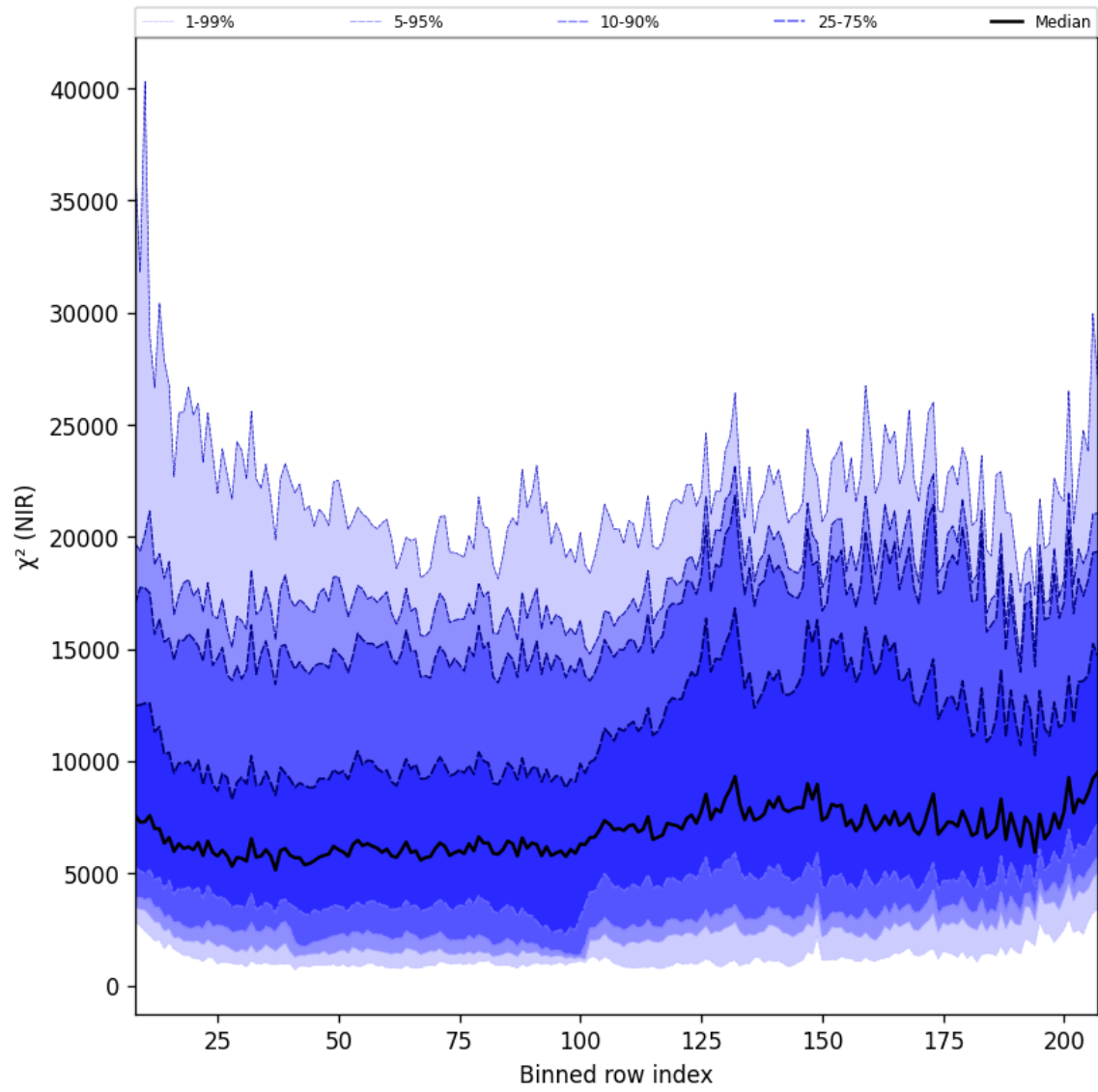
Figure 40: Along track statistics of “ \chi^2 (NIR)” for 2024-09-18 to 2024-09-20
