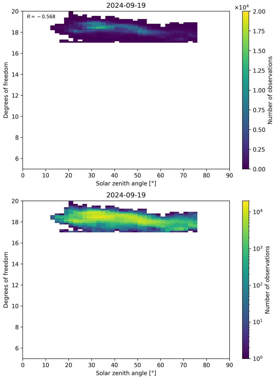
Figure 96: Scatter density plot of “Solar zenith angle” against “Degrees of freedom” for 2024-09-18 to 2024-09-20.
