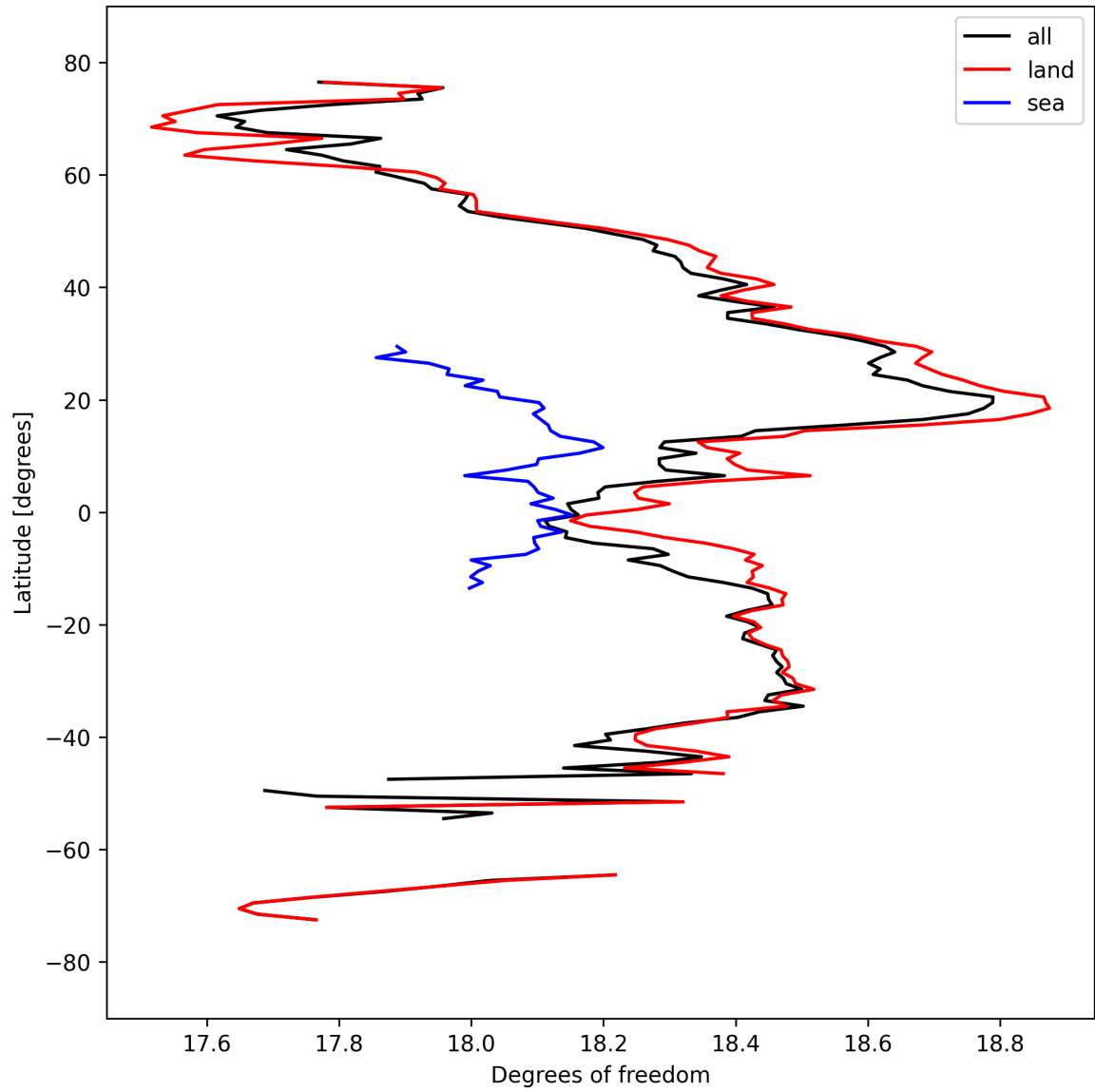
Figure 19: Zonal average of “Degrees of freedom” for 2024-09-18 to 2024-09-20.
