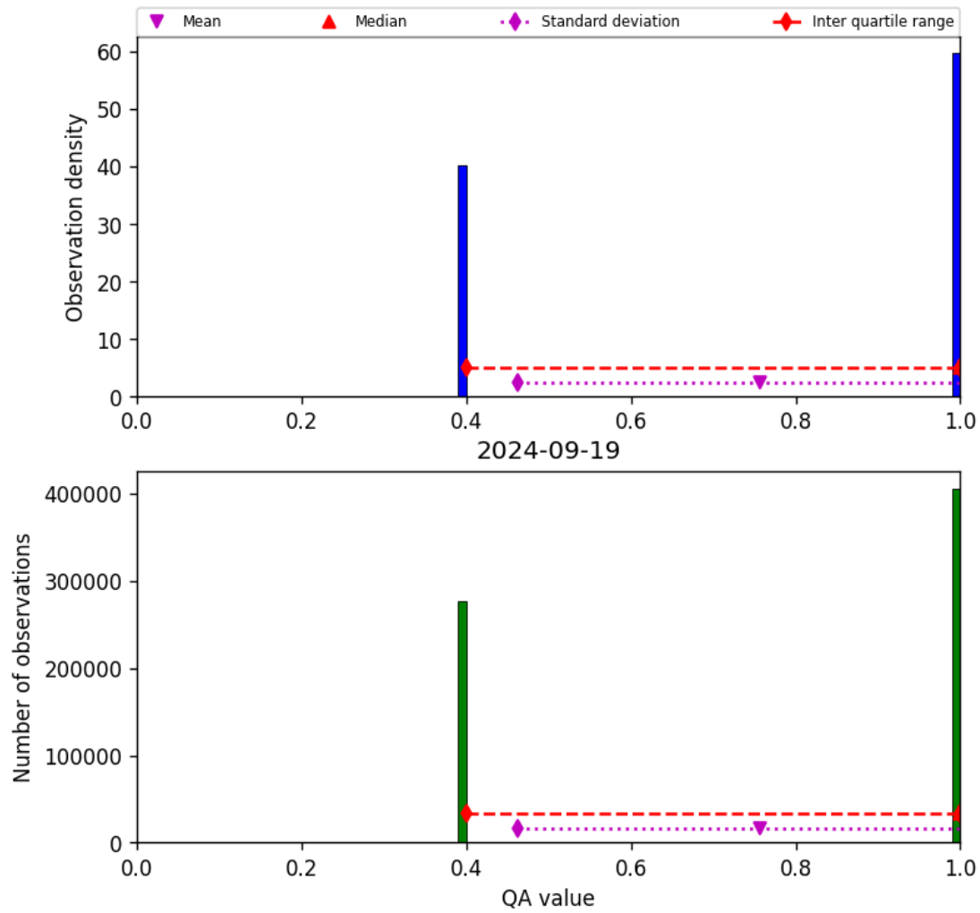
Figure 22: Histogram of “QA value” for 2024-09-18 to 2024-09-20
