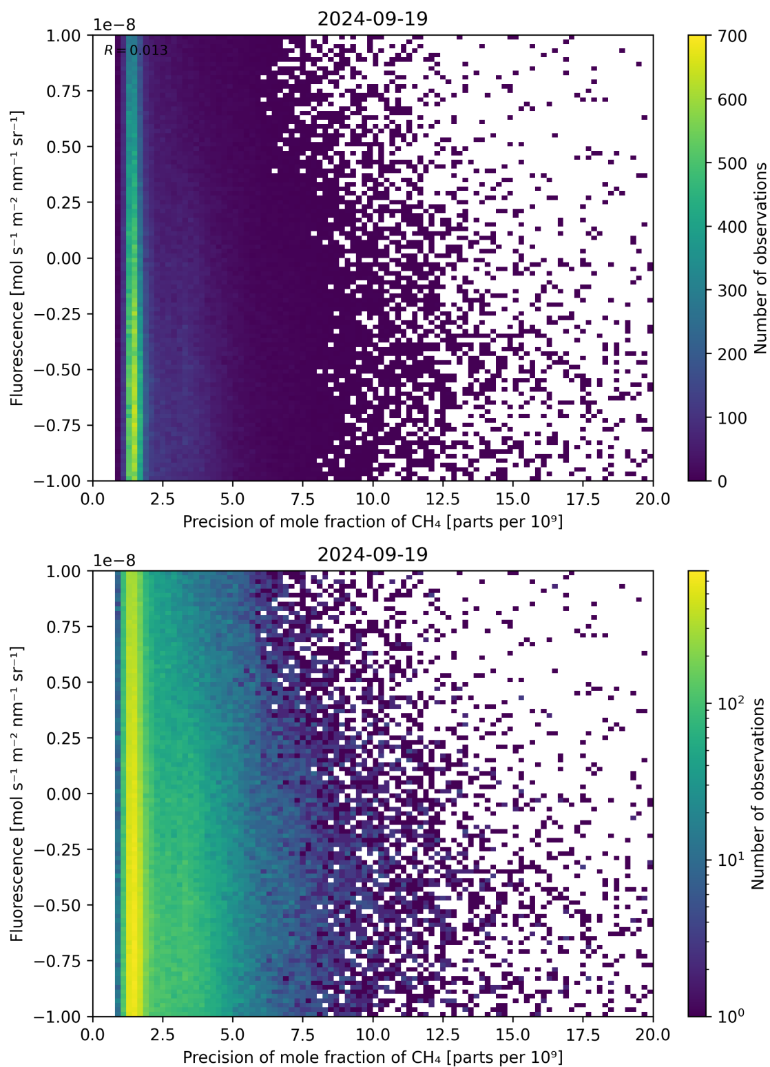
Figure 81: Scatter density plot of “Precision of mole fraction of \text{CH}_4 ” against “Fluorescence” for 2024-09-18 to 2024-09-20.
