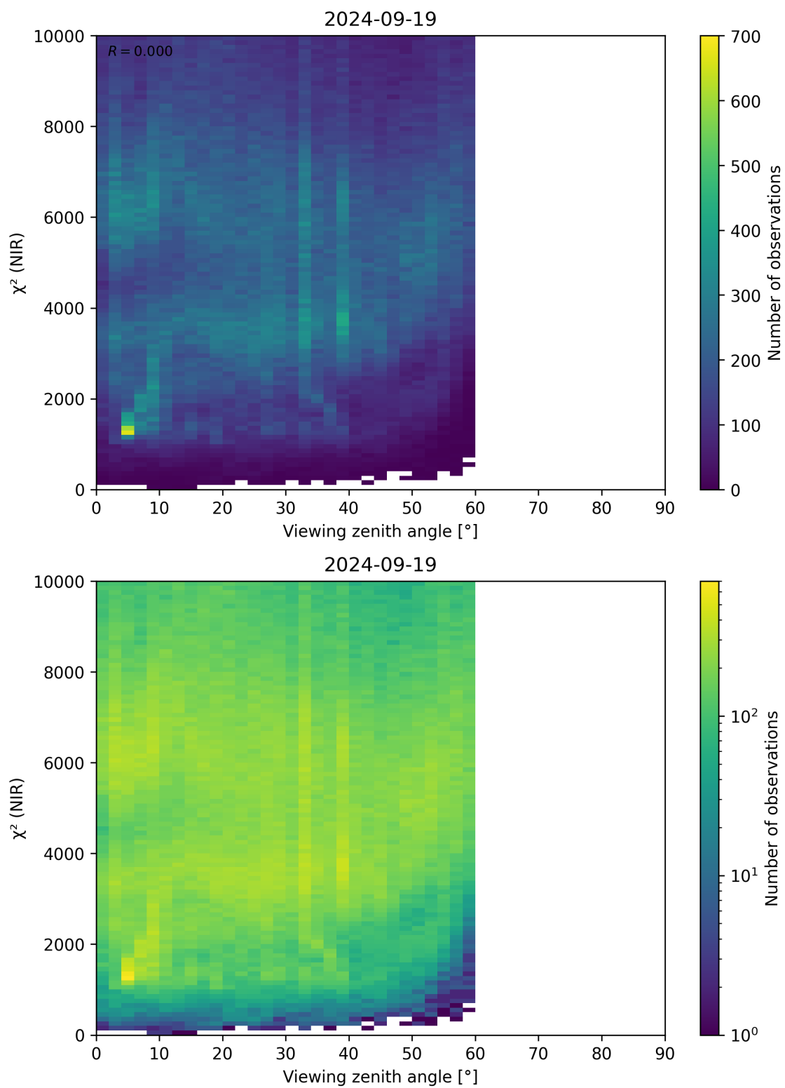
Figure 105: Scatter density plot of “Viewing zenith angle” against “ \chi^2 (NIR)” for 2024-09-18 to 2024-09-20.
