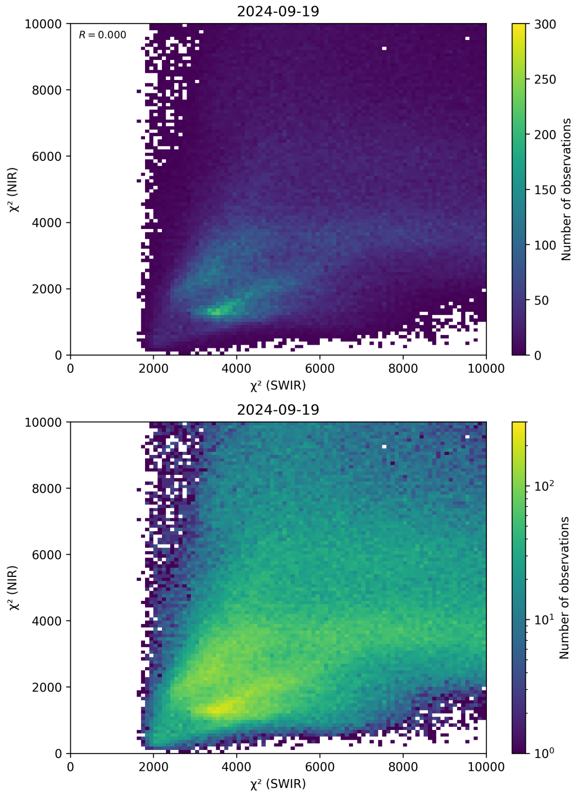
Figure 47: Scatter density plot of “ \chi^2 (SWIR)” against “ \chi^2 (NIR)” for 2024-09-18 to 2024-09-20.
