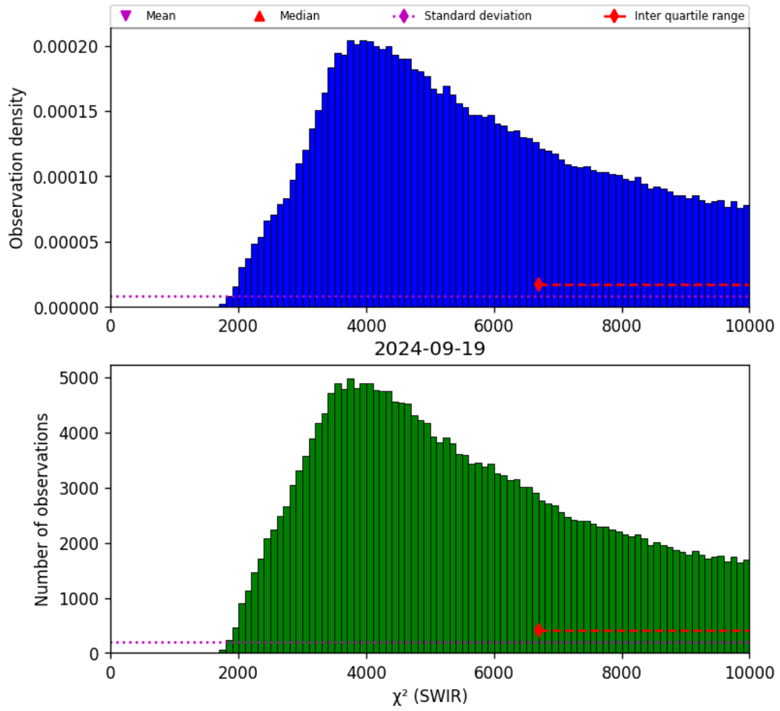
Figure 28: Histogram of “ \chi^2 (SWIR)” for 2024-09-18 to 2024-09-20
