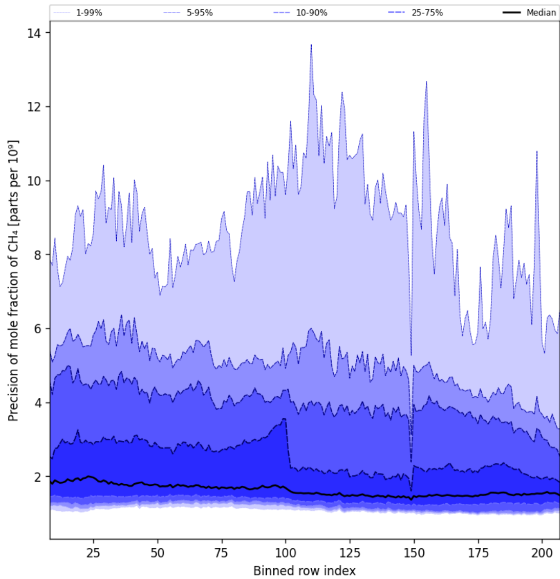
Figure 35: Along track statistics of “Precision of mole fraction of CH 4 ” for 2024-09-18 to 2024-09-20
