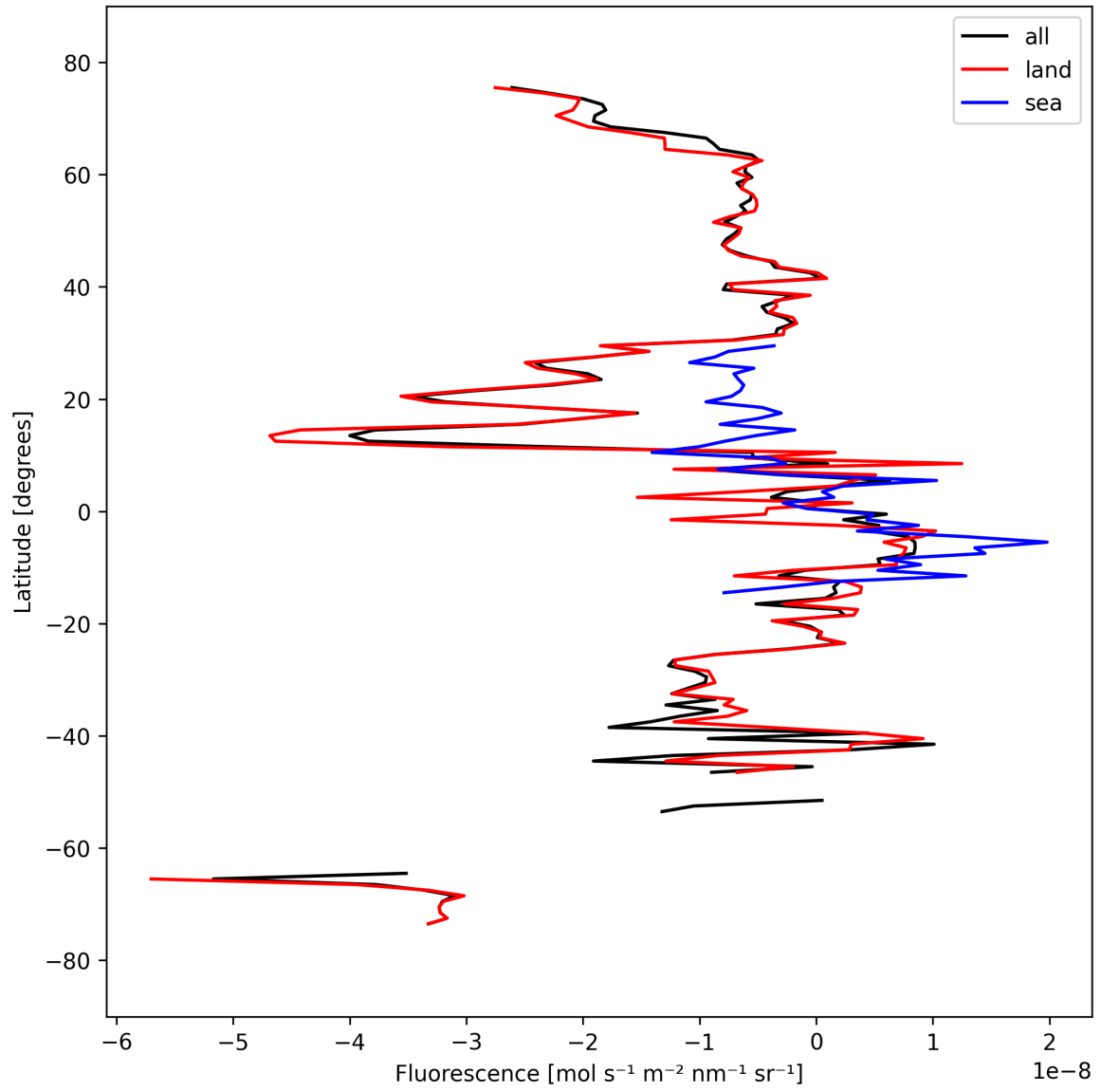
Figure 21: Zonal average of “Fluorescence” for 2024-09-19 to 2024-09-21.
