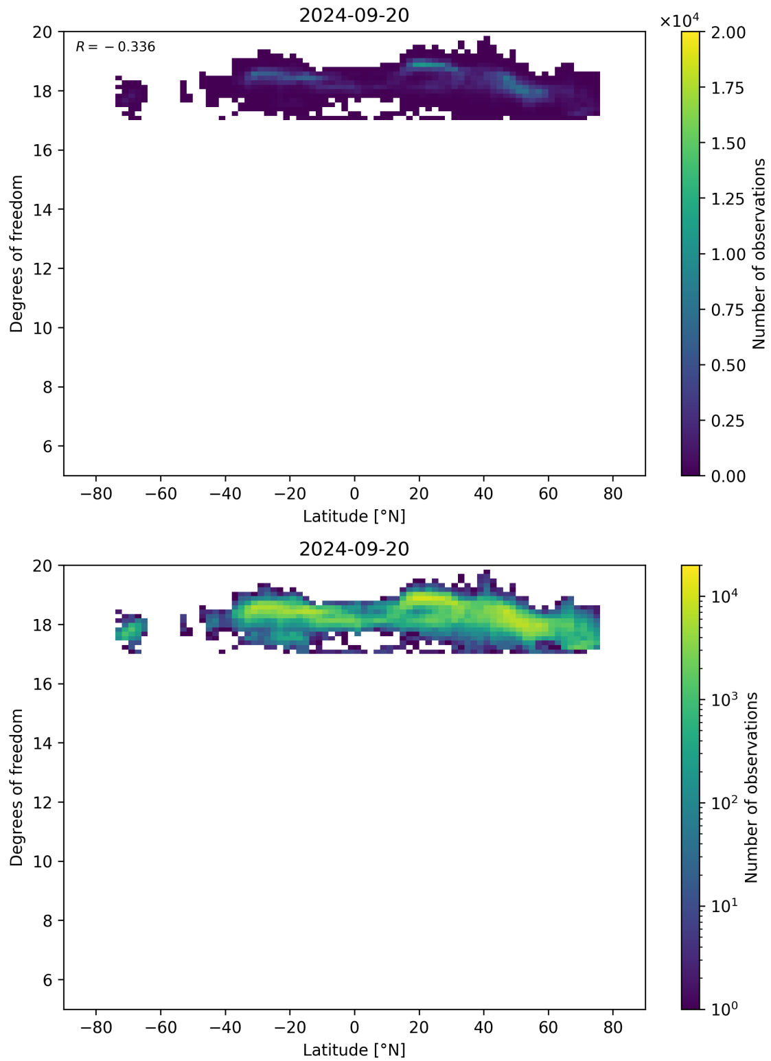
Figure 55: Scatter density plot of “Latitude” against “Degrees of freedom” for 2024-09-19 to 2024-09-21.
