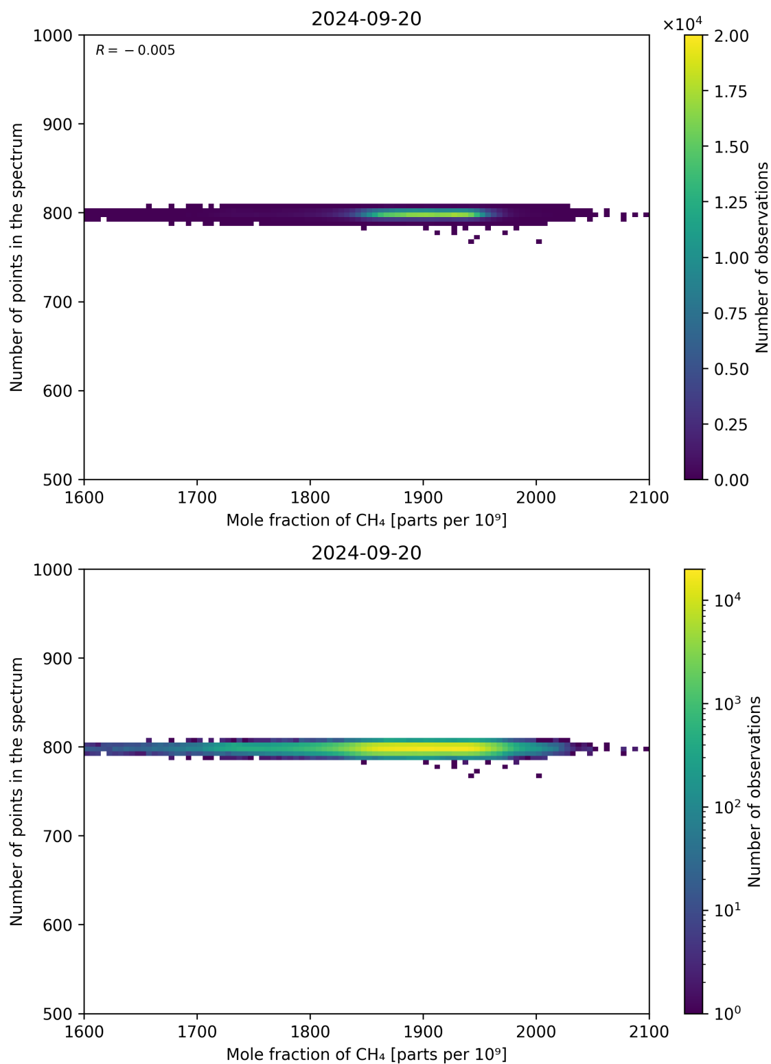
Figure 77: Scatter density plot of “Mole fraction of CH 4 ” against “Number of points in the spectrum” for 2024-09-19 to 2024-09-21.
