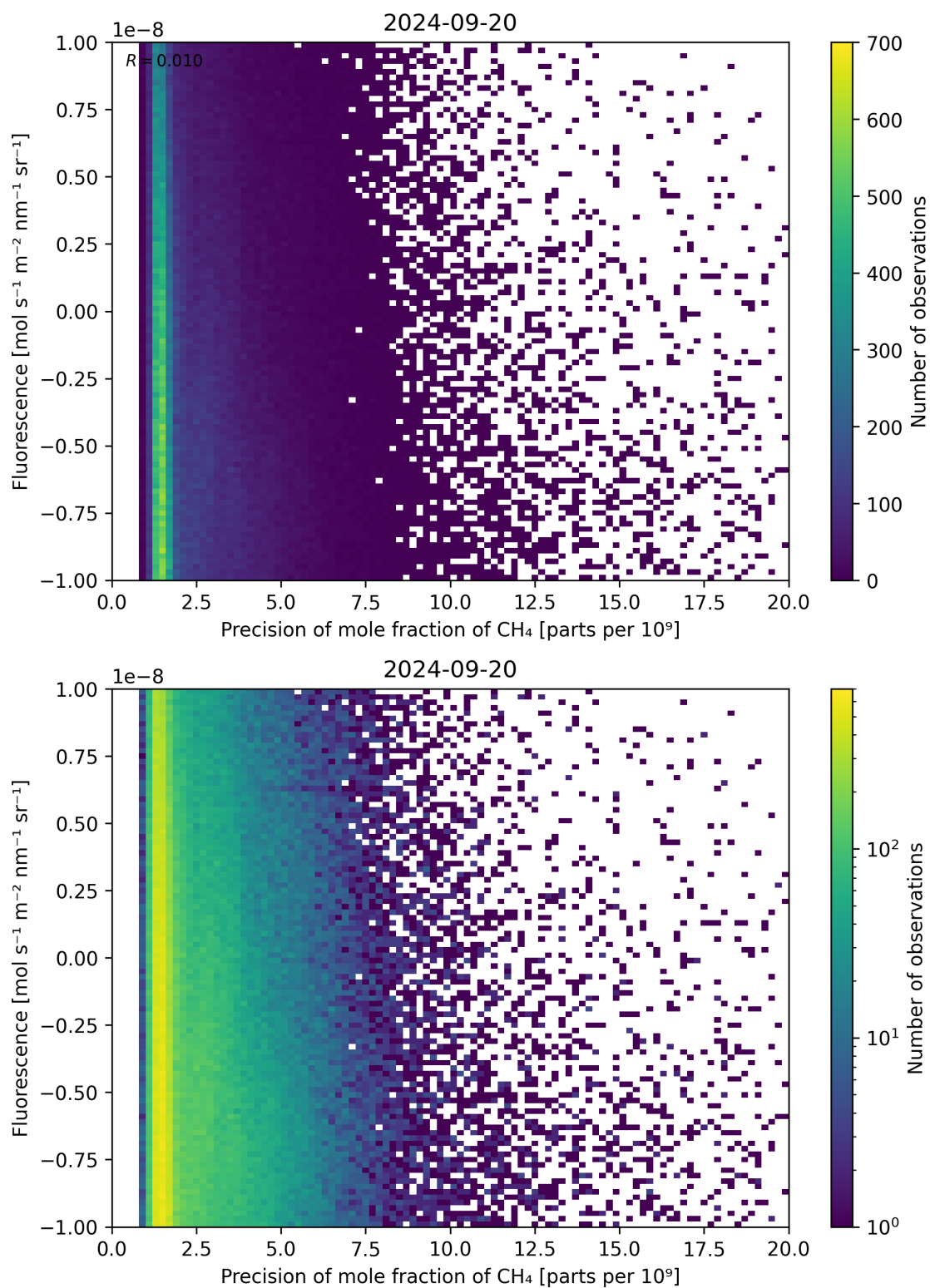
Figure 81: Scatter density plot of “Precision of mole fraction of \text{CH}_4 ” against “Fluorescence” for 2024-09-19 to 2024-09-21.
