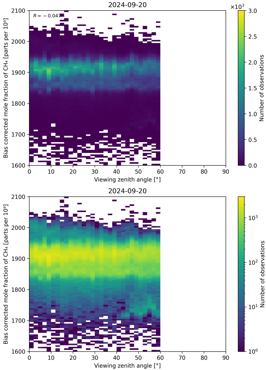
Figure 111: Scatter density plot of “Viewing zenith angle” against “Bias corrected mole fraction of CH 4 ” for 2024-09-19 to 2024-09-21.
