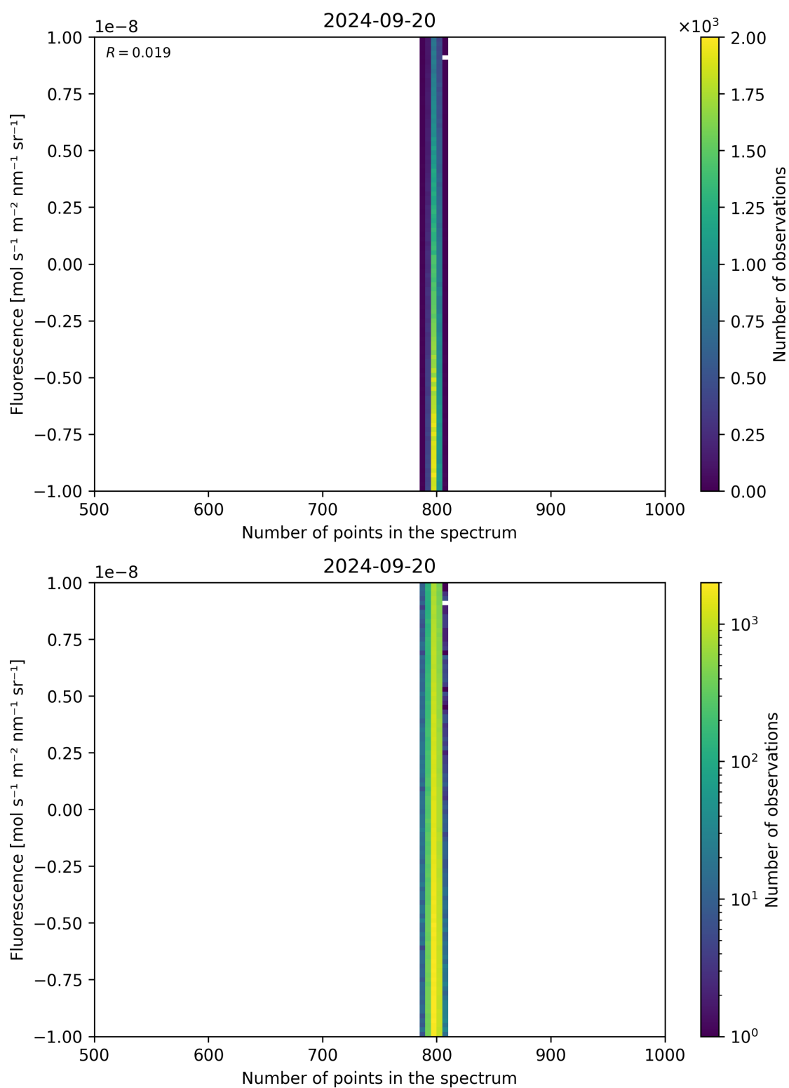
Figure 91: Scatter density plot of “Number of points in the spectrum” against “Fluorescence” for 2024-09-19 to 2024-09-21.
