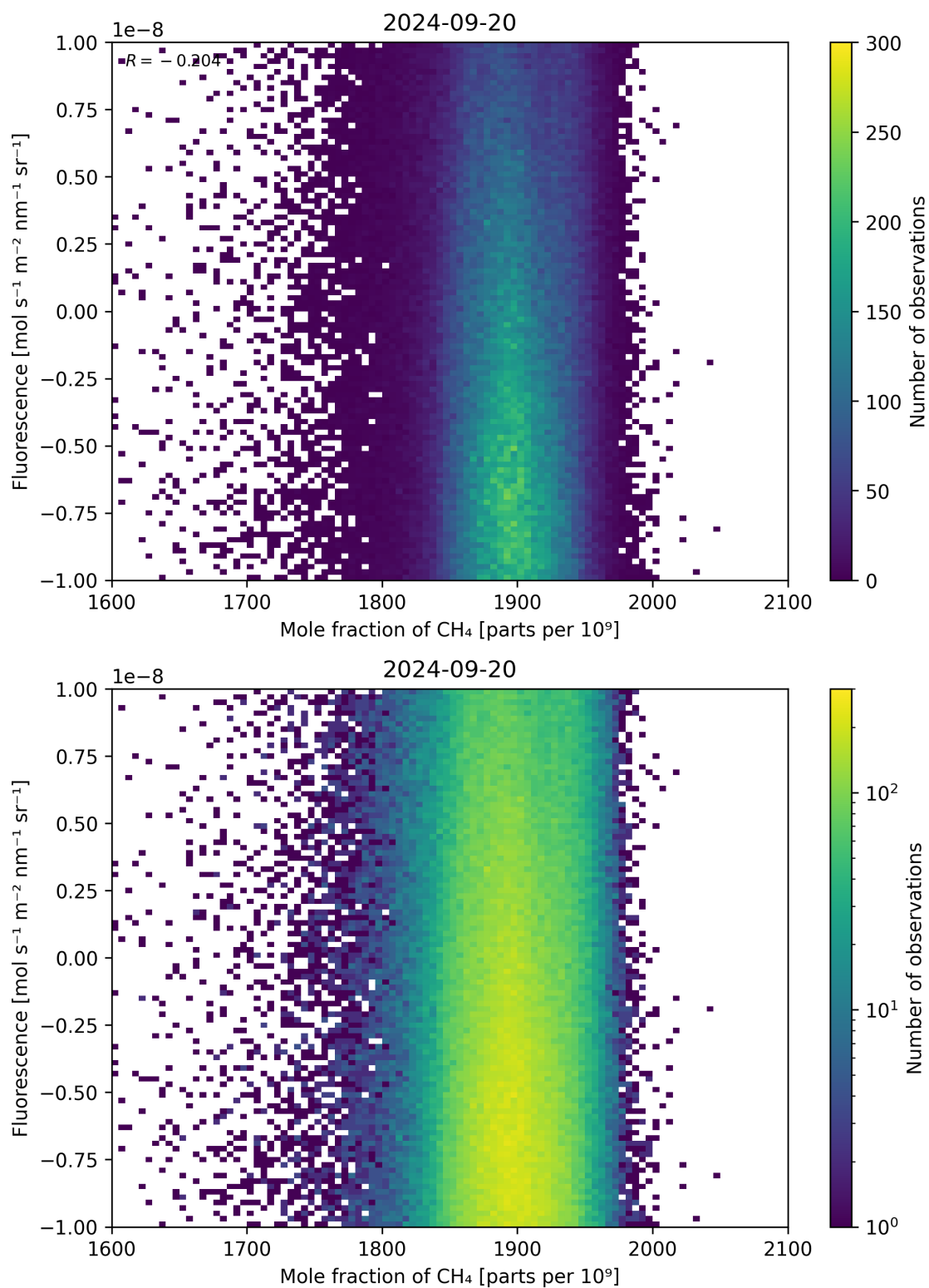
Figure 73: Scatter density plot of “Mole fraction of \text{CH}_4 ” against “Fluorescence” for 2024-09-19 to 2024-09-21.
