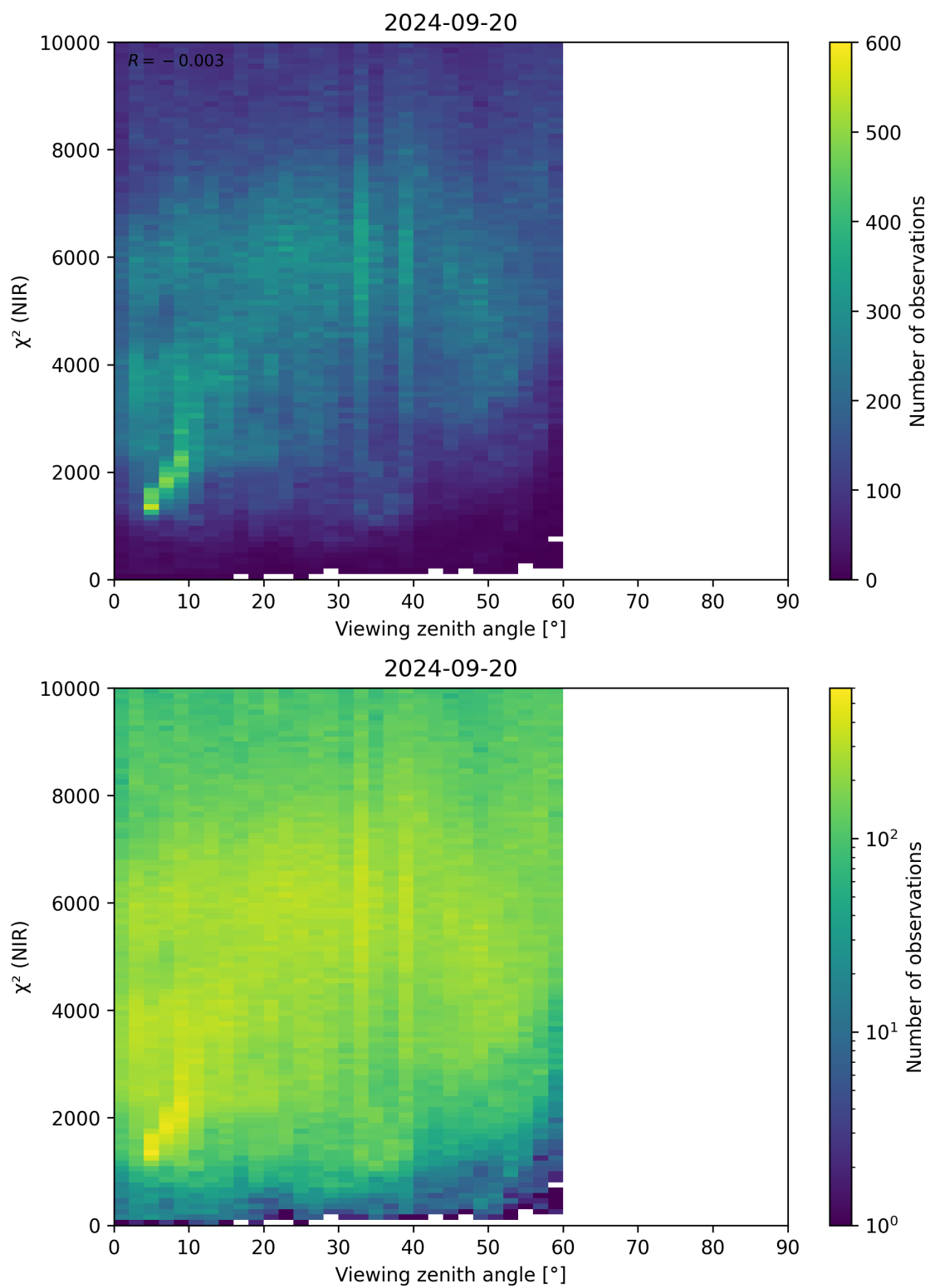
Figure 105: Scatter density plot of “Viewing zenith angle” against “ \chi^2 (NIR)” for 2024-09-19 to 2024-09-21.
