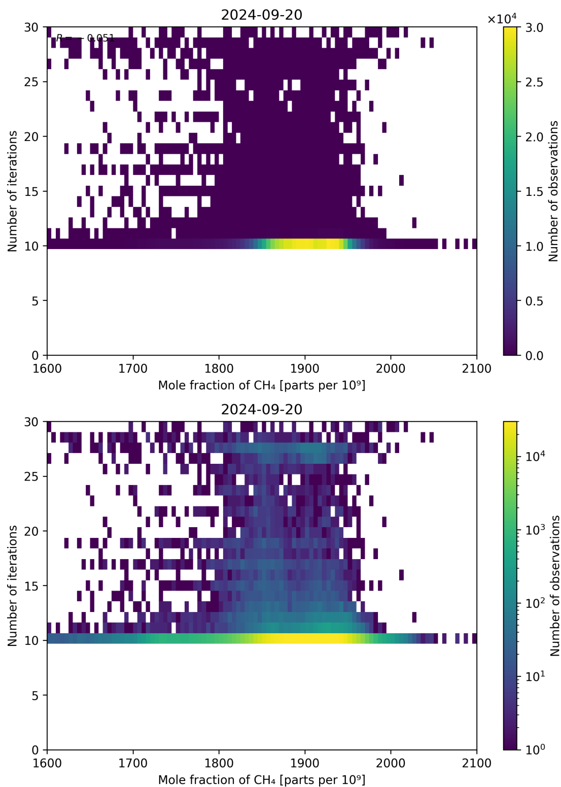
Figure 76: Scatter density plot of “Mole fraction of CH 4 ” against “Number of iterations” for 2024-09-19 to 2024-09-21.
