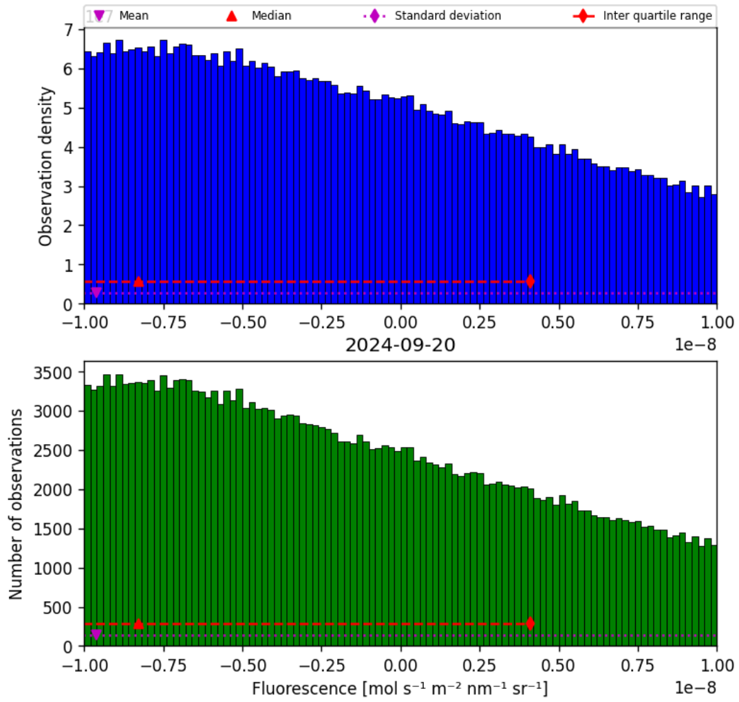
Figure 32: Histogram of “Fluorescence” for 2024-09-19 to 2024-09-21
