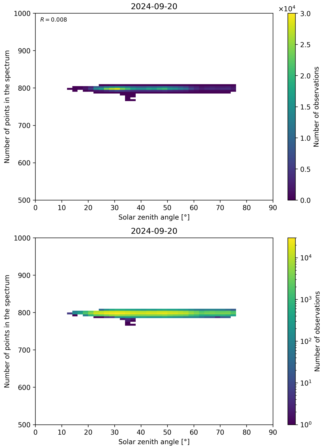
Figure 103: Scatter density plot of “Solar zenith angle” against “Number of points in the spectrum” for 2024-09-19 to 2024-09-21.
