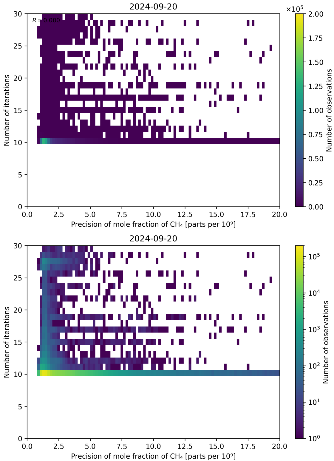
Figure 83: Scatter density plot of “Precision of mole fraction of CH 4 ” against “Number of iterations” for 2024-09-19 to 2024-09-21.
