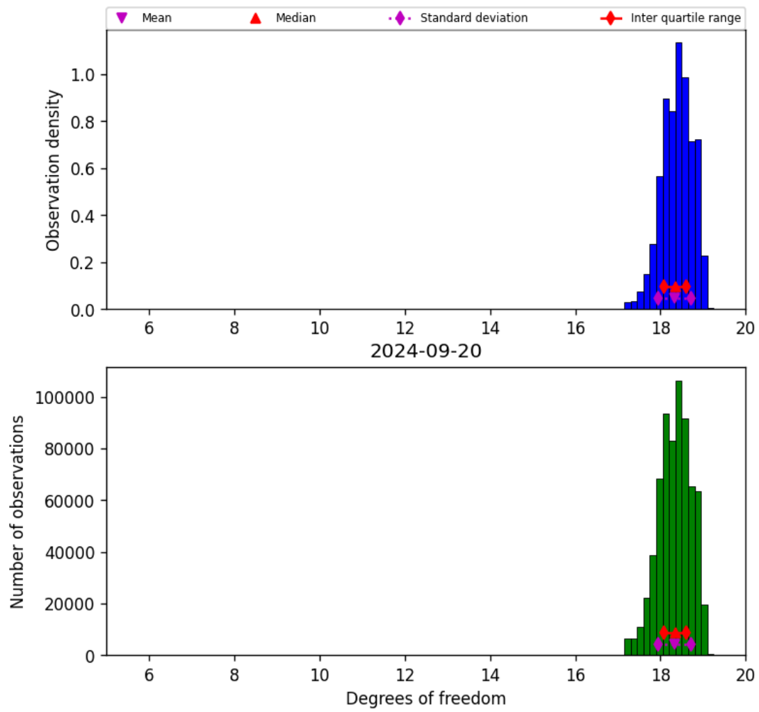
Figure 30: Histogram of “Degrees of freedom” for 2024-09-19 to 2024-09-21
