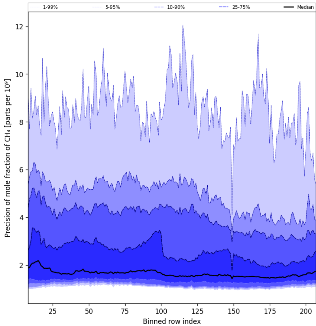
Figure 35: Along track statistics of “Precision of mole fraction of CH 4 ” for 2024-09-19 to 2024-09-21
