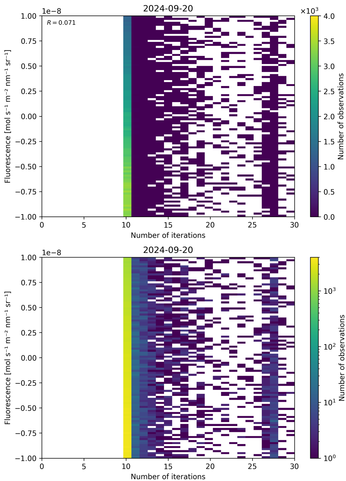
Figure 87: Scatter density plot of “Number of iterations” against “Fluorescence” for 2024-09-19 to 2024-09-21.
