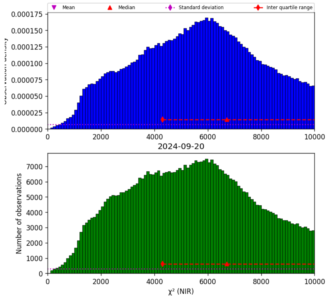
Figure 29: Histogram of “ \chi^2 (NIR)” for 2024-09-19 to 2024-09-21
