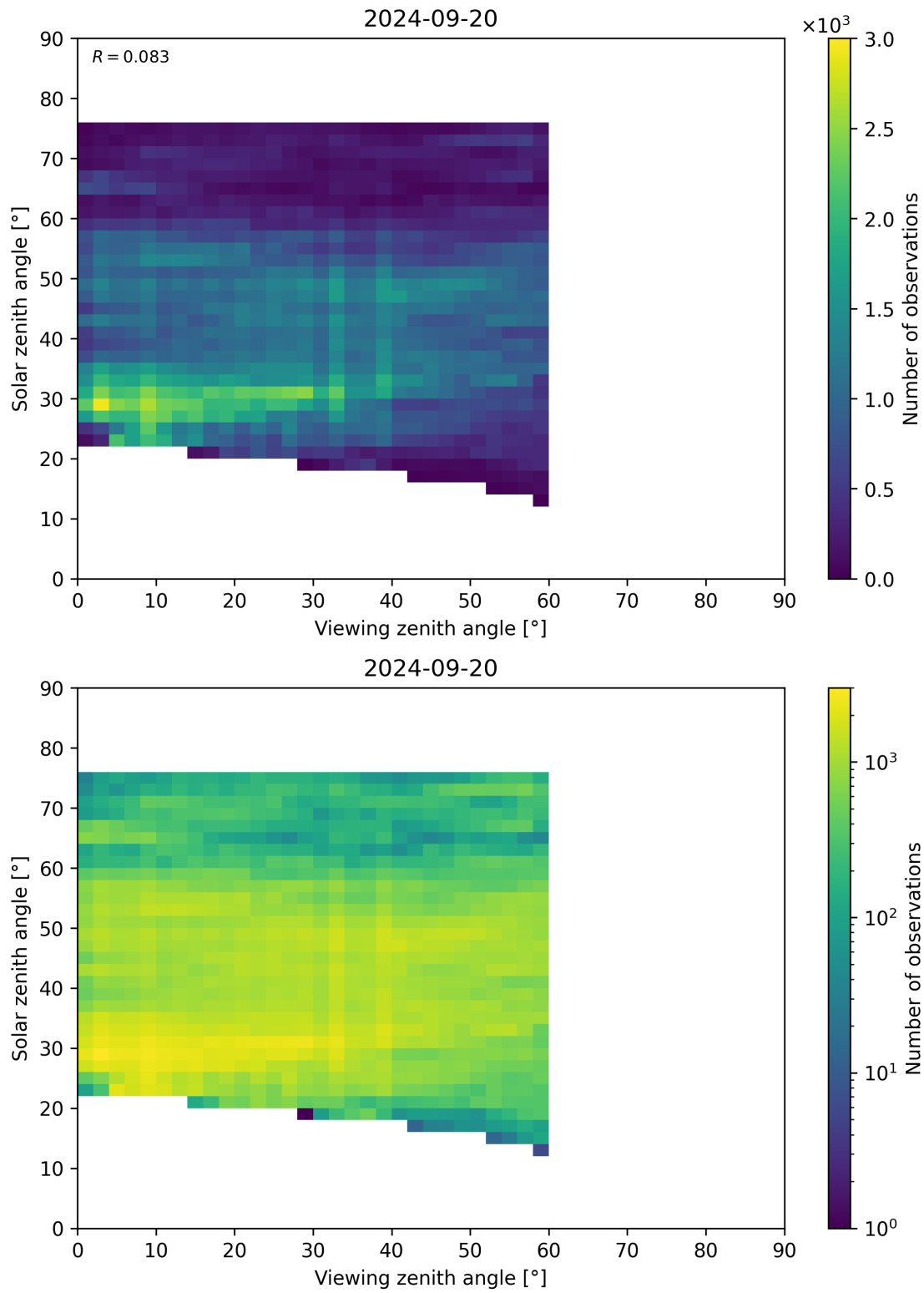
Figure 115: Scatter density plot of “Viewing zenith angle” against “Solar zenith angle” for 2024-09-19 to 2024-09-21.
