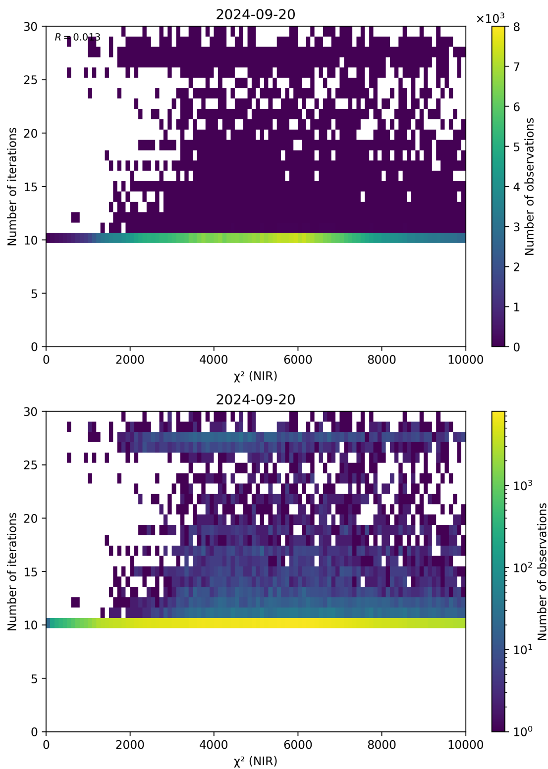
Figure 46: Scatter density plot of “ \chi^2 (NIR)” against “Number of iterations” for 2024-09-19 to 2024-09-21.
