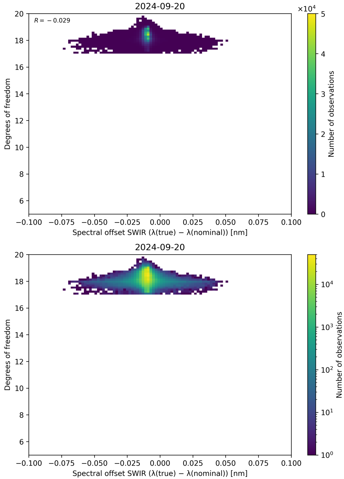
Figure 119: Scatter density plot of “Spectral offset SWIR ( \lambda_{\text{true}} - \lambda_{\text{nominal}} )” against “Degrees of freedom” for 2024-09-19 to 2024-09-21.
