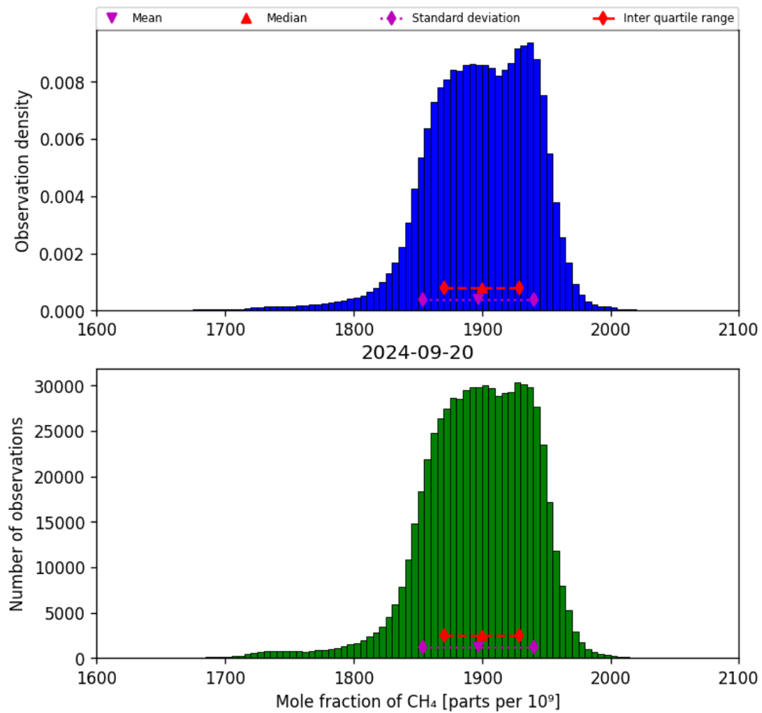
Figure 23: Histogram of “Mole fraction of CH 4 ” for 2024-09-19 to 2024-09-21
