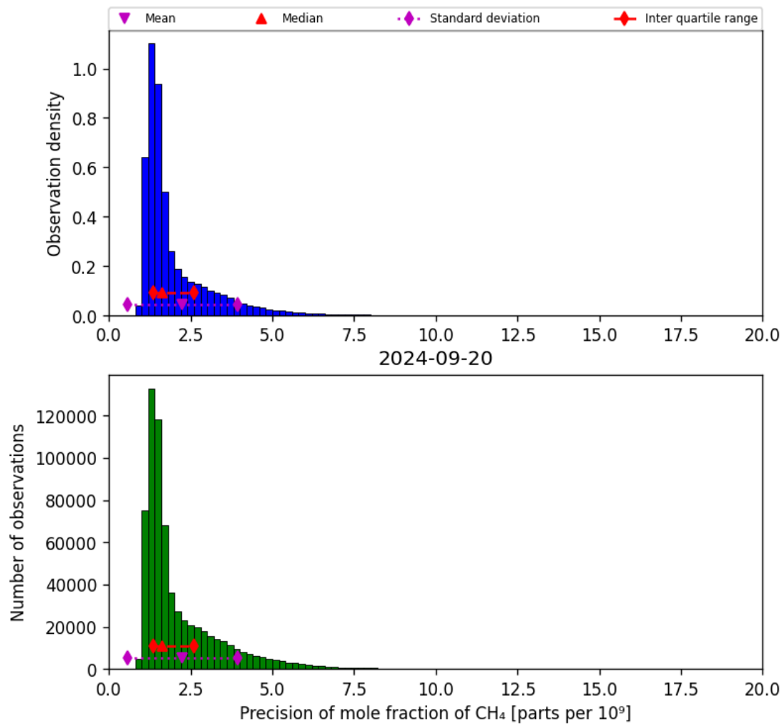
Figure 24: Histogram of “Precision of mole fraction of CH 4 ” for 2024-09-19 to 2024-09-21
