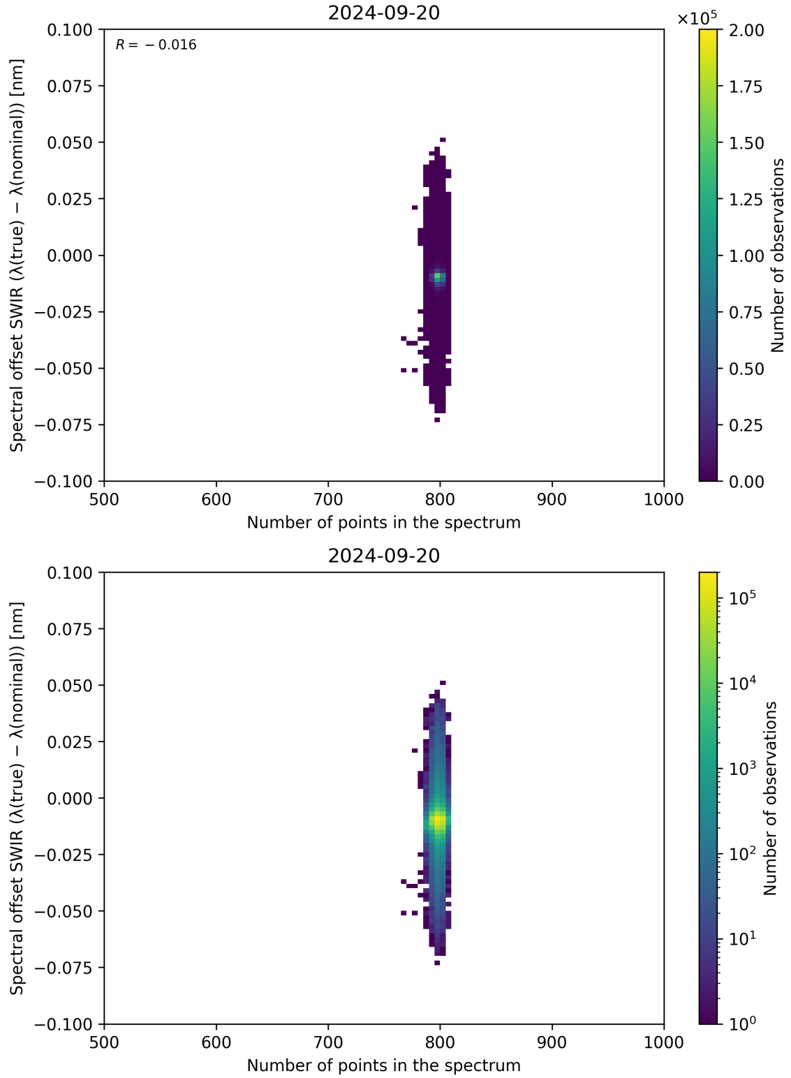
Figure 93: Scatter density plot of “Number of points in the spectrum” against “Spectral offset SWIR ( \lambda_{\text{true}} - \lambda_{\text{nominal}} )” for 2024-09-19 to 2024-09-21.
