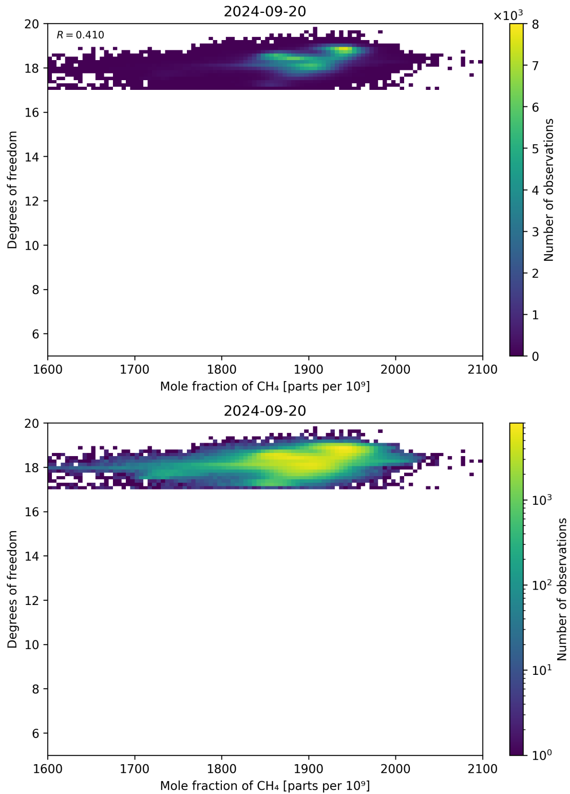
Figure 72: Scatter density plot of “Mole fraction of CH 4 ” against “Degrees of freedom” for 2024-09-19 to 2024-09-21.
