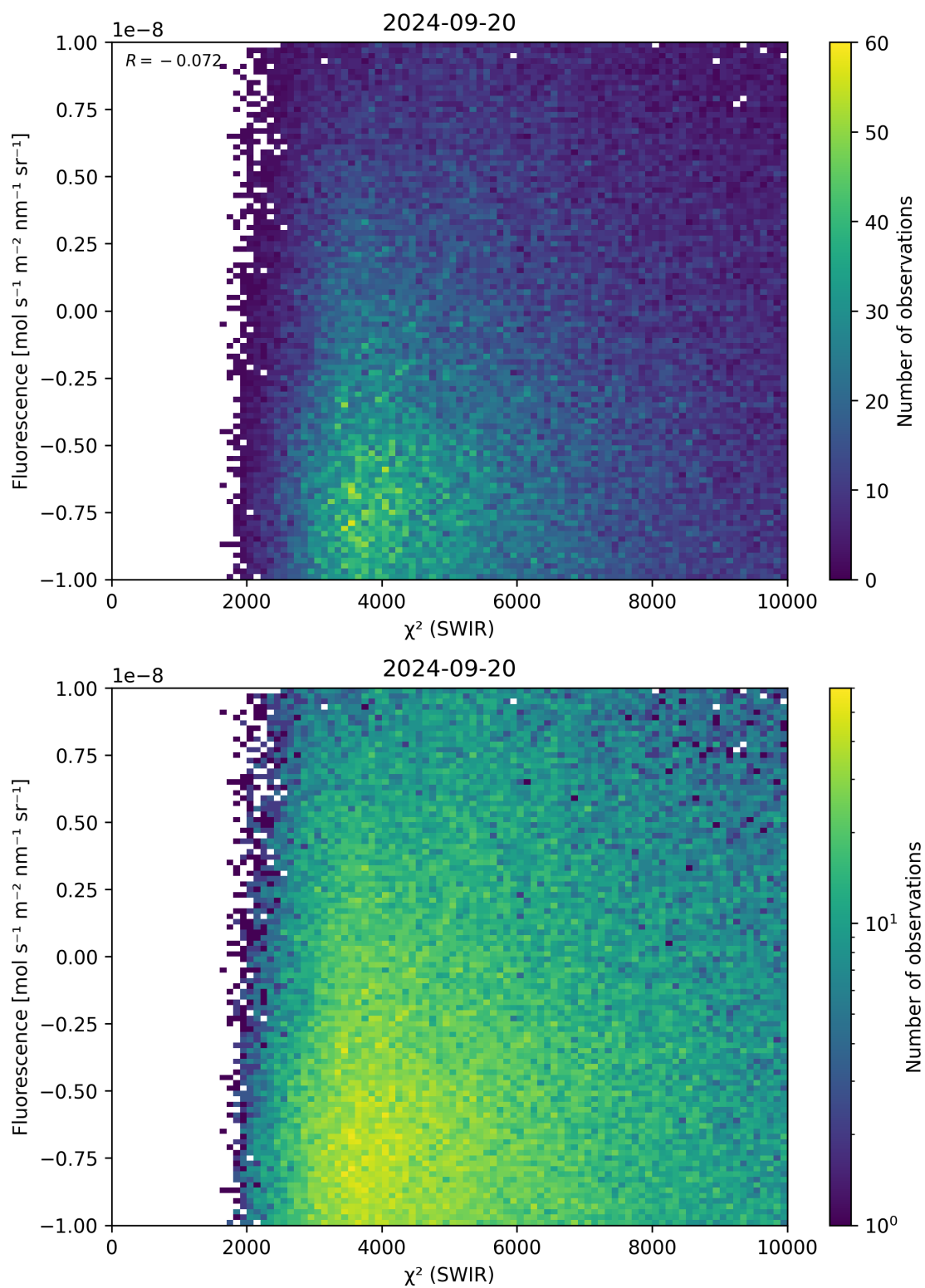
Figure 49: Scatter density plot of “ \chi^2 (SWIR)” against “Fluorescence” for 2024-09-19 to 2024-09-21.
