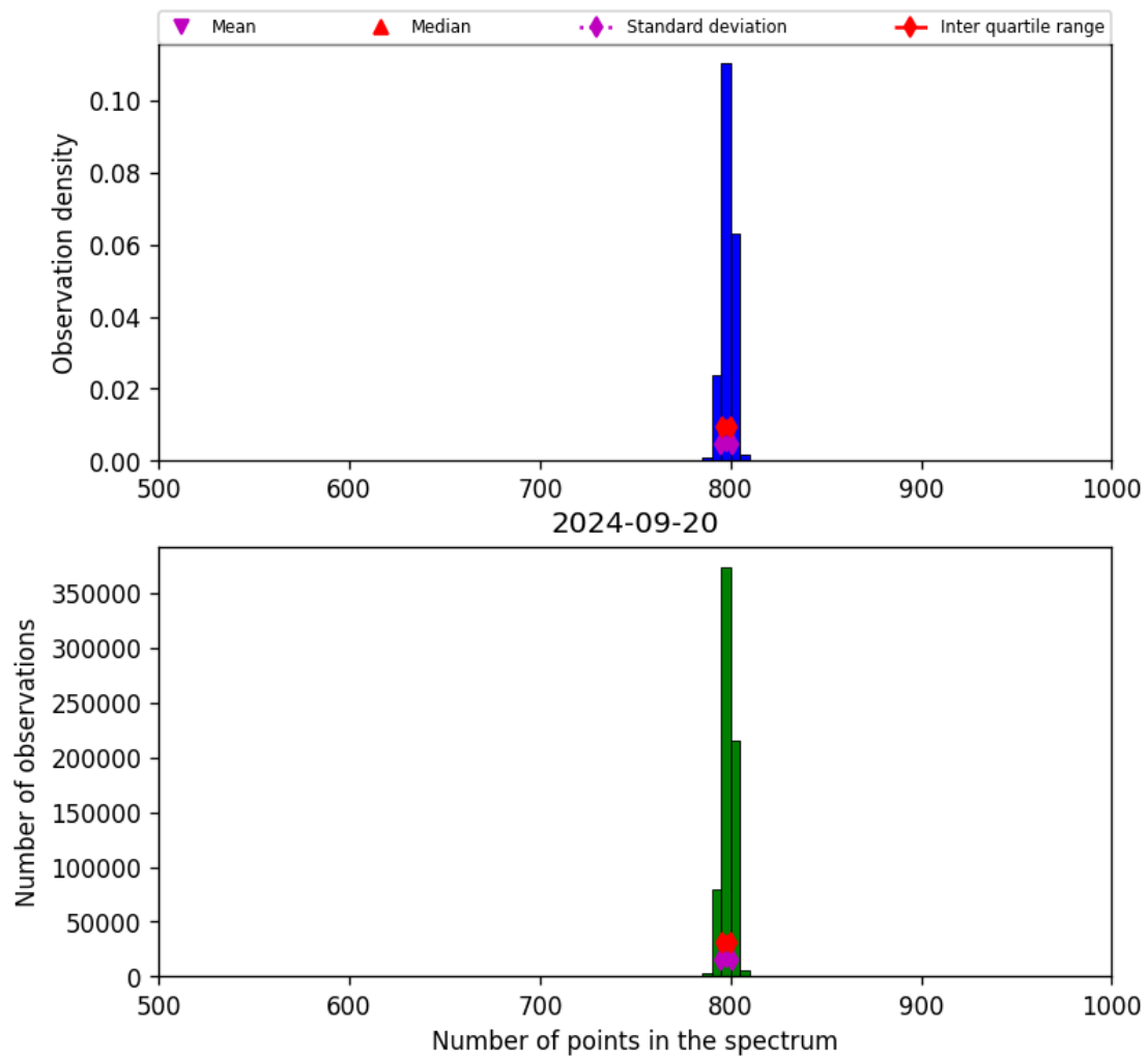
Figure 26: Histogram of “Number of points in the spectrum” for 2024-09-19 to 2024-09-21
