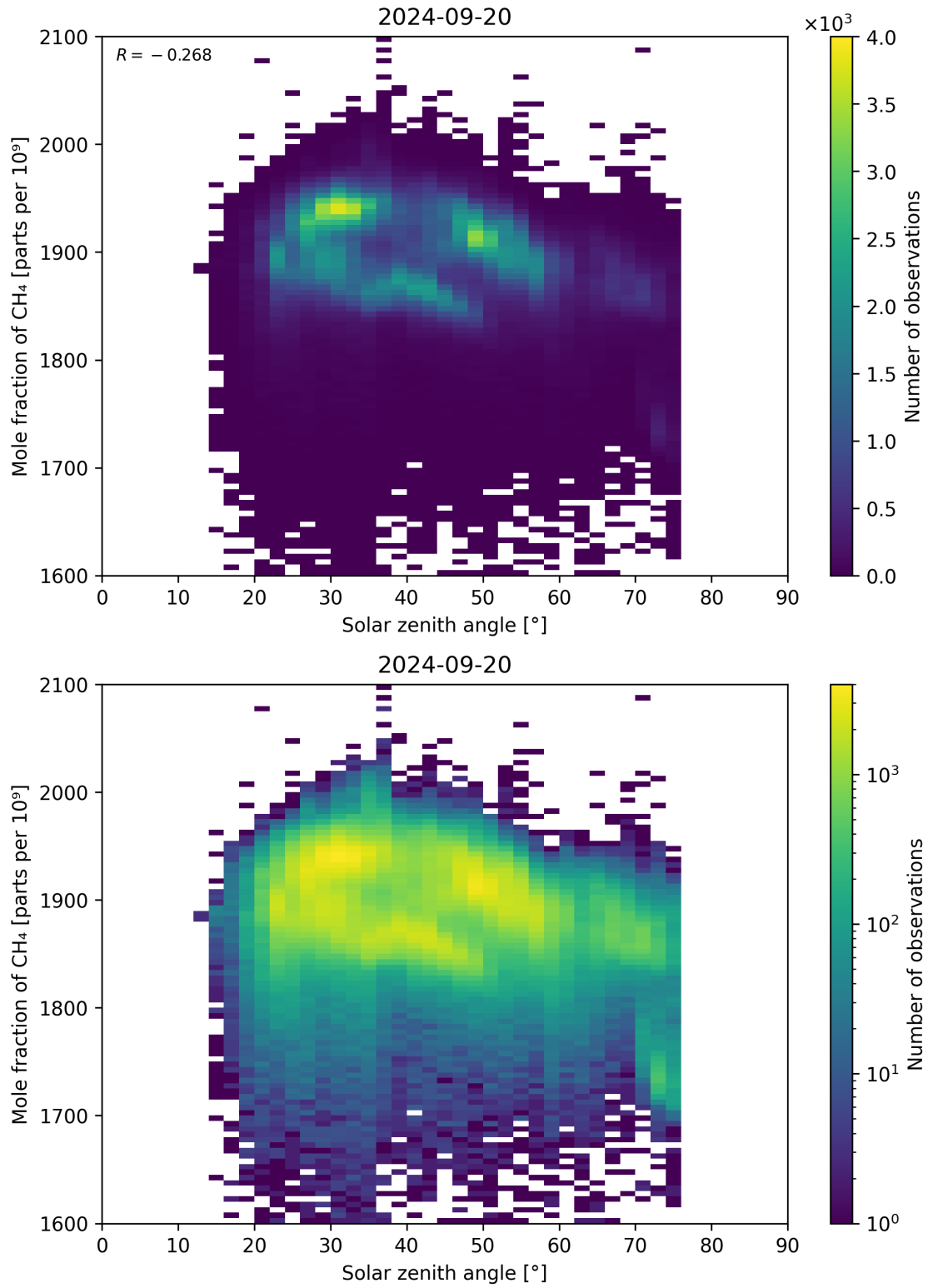
Figure 99: Scatter density plot of “Solar zenith angle” against “Mole fraction of CH 4 ” for 2024-09-19 to 2024-09-21.
