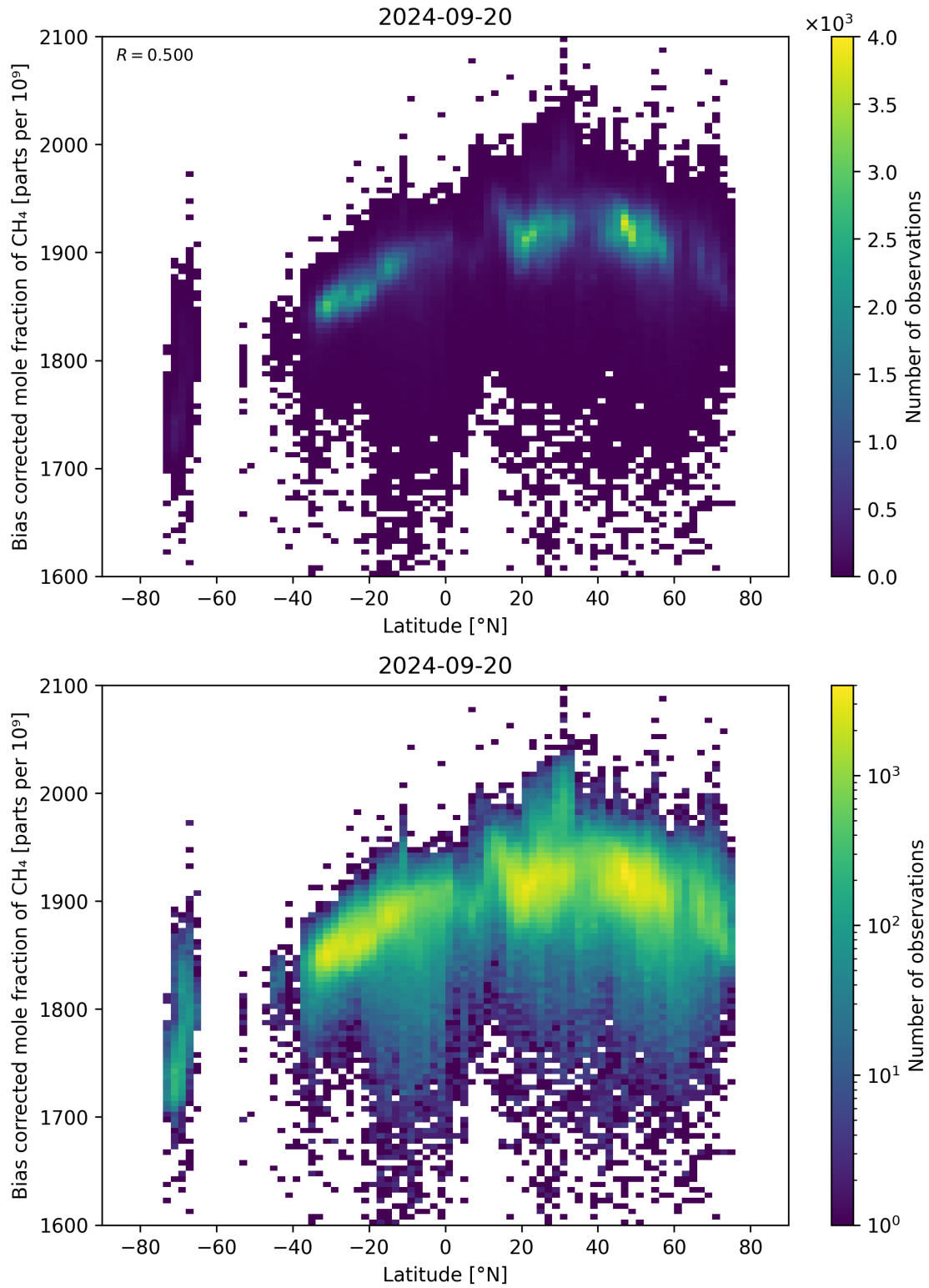
Figure 58: Scatter density plot of “Latitude” against “Bias corrected mole fraction of CH 4 ” for 2024-09-19 to 2024-09-21.
