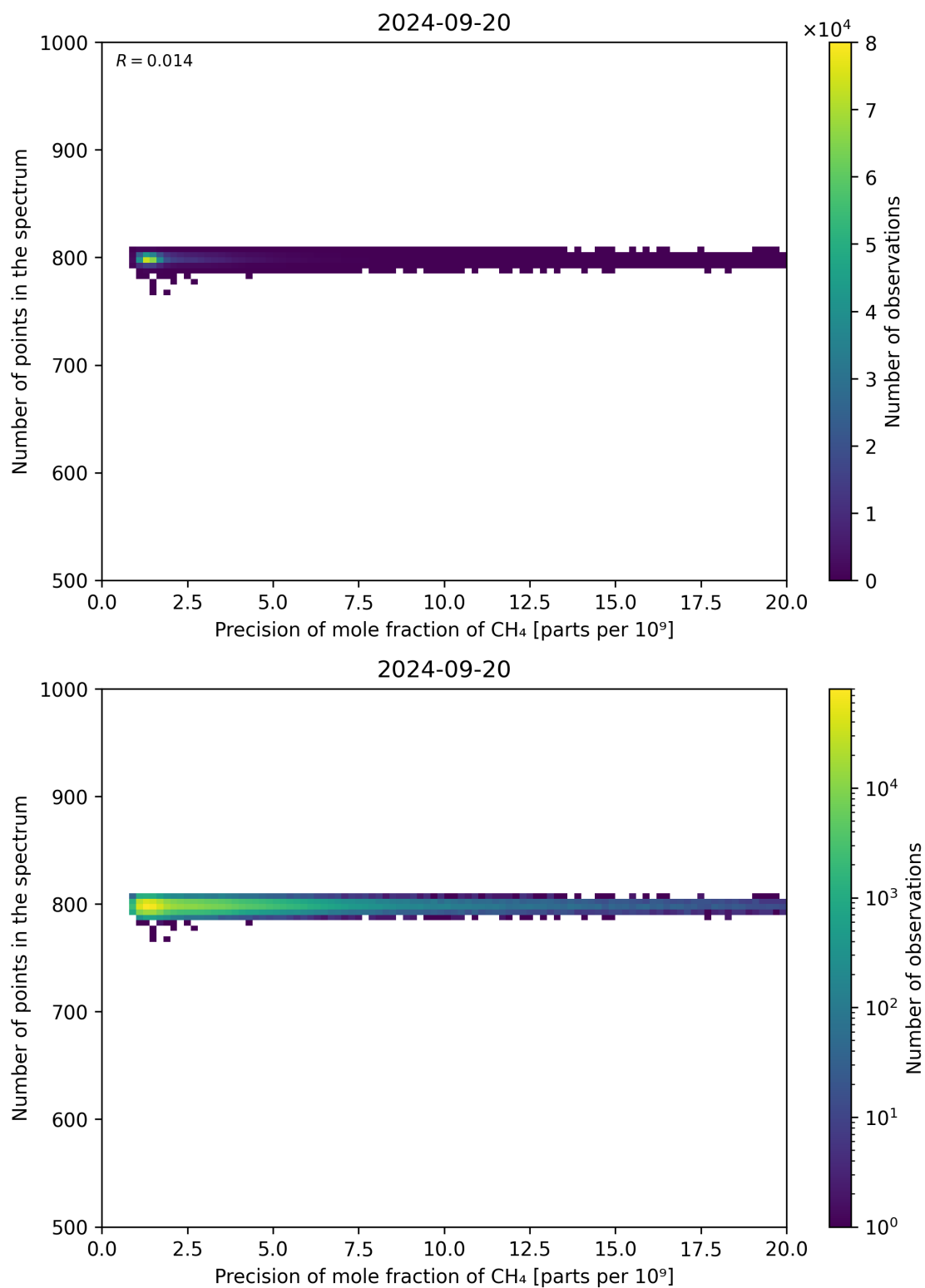
Figure 84: Scatter density plot of “Precision of mole fraction of CH 4 ” against “Number of points in the spectrum” for 2024-09-19 to 2024-09-21.
