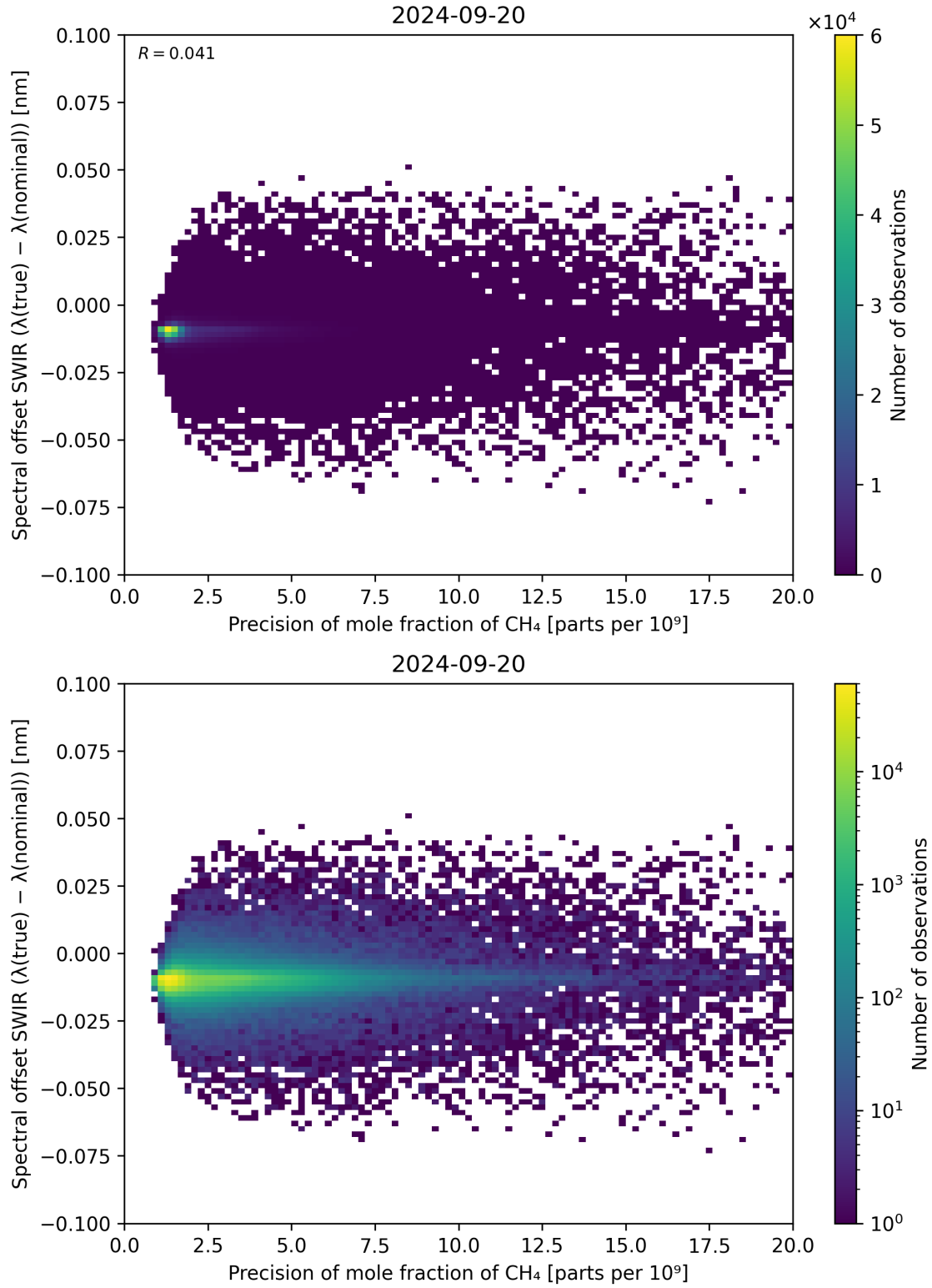
Figure 85: Scatter density plot of “Precision of mole fraction of CH 4 ” against “Spectral offset SWIR ( \lambda_{\text{true}} - \lambda_{\text{nominal}} )” for 2024-09-19 to 2024-09-21.
