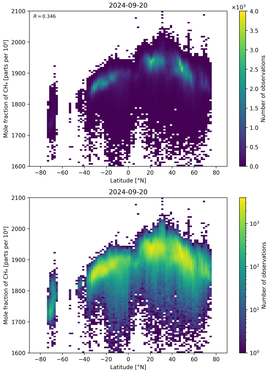
Figure 57: Scatter density plot of “Latitude” against “Mole fraction of \text{CH}_4 ” for 2024-09-19 to 2024-09-21.
