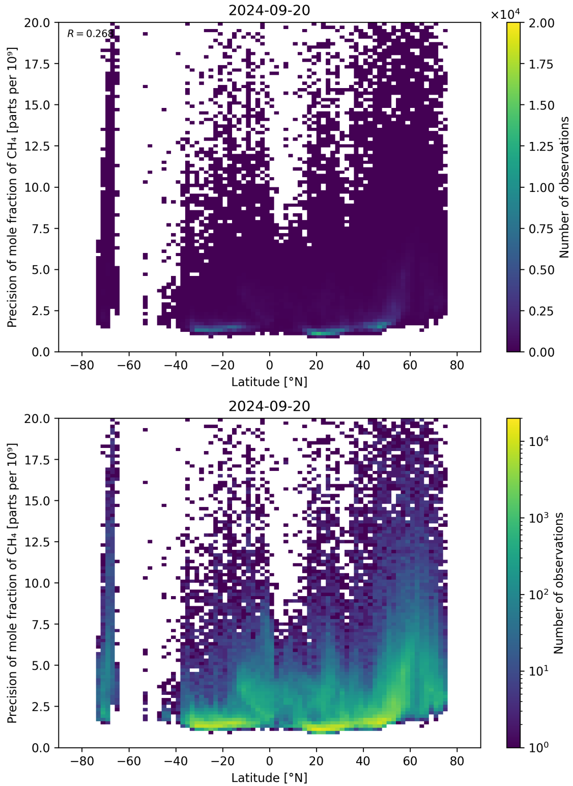
Figure 59: Scatter density plot of “Latitude” against “Precision of mole fraction of CH 4 ” for 2024-09-19 to 2024-09-21.
