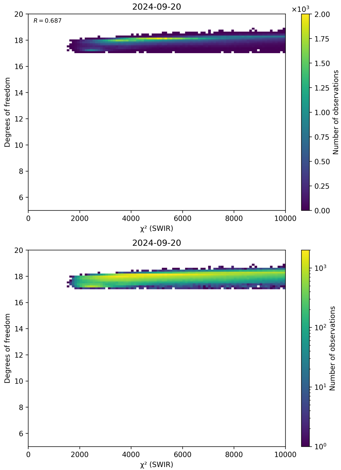
Figure 48: Scatter density plot of “ \chi^2 (SWIR)” against “Degrees of freedom” for 2024-09-19 to 2024-09-21.
