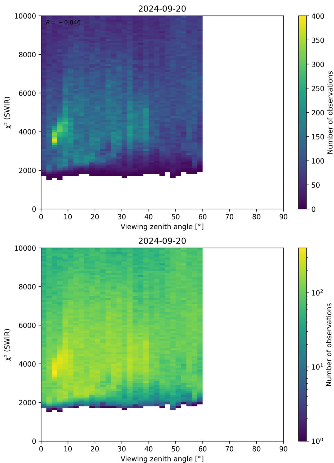
Figure 106: Scatter density plot of “Viewing zenith angle” against “ \chi^2 (SWIR)” for 2024-09-19 to 2024-09-21.
