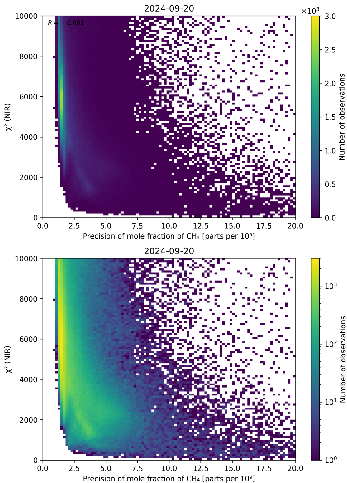
Figure 78: Scatter density plot of “Precision of mole fraction of CH 4 ” against “ \chi^2 (NIR)” for 2024-09-19 to 2024-09-21.
