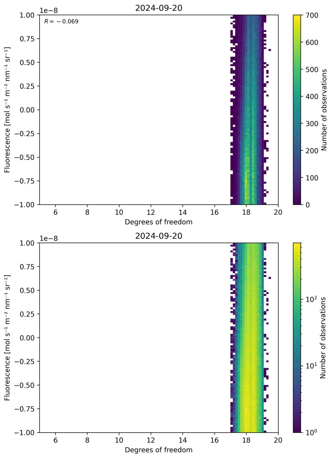
Figure 51: Scatter density plot of “Degrees of freedom” against “Fluorescence” for 2024-09-19 to 2024-09-21.
