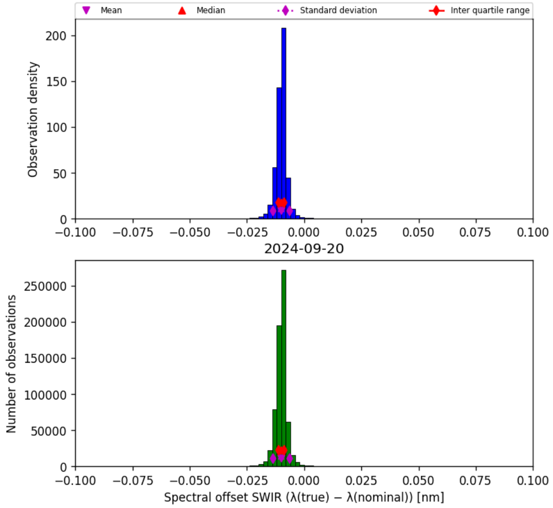
Figure 27: Histogram of “Spectral offset SWIR ( \lambda_{\text{true}} - \lambda_{\text{nominal}} )” for 2024-09-19 to 2024-09-21
