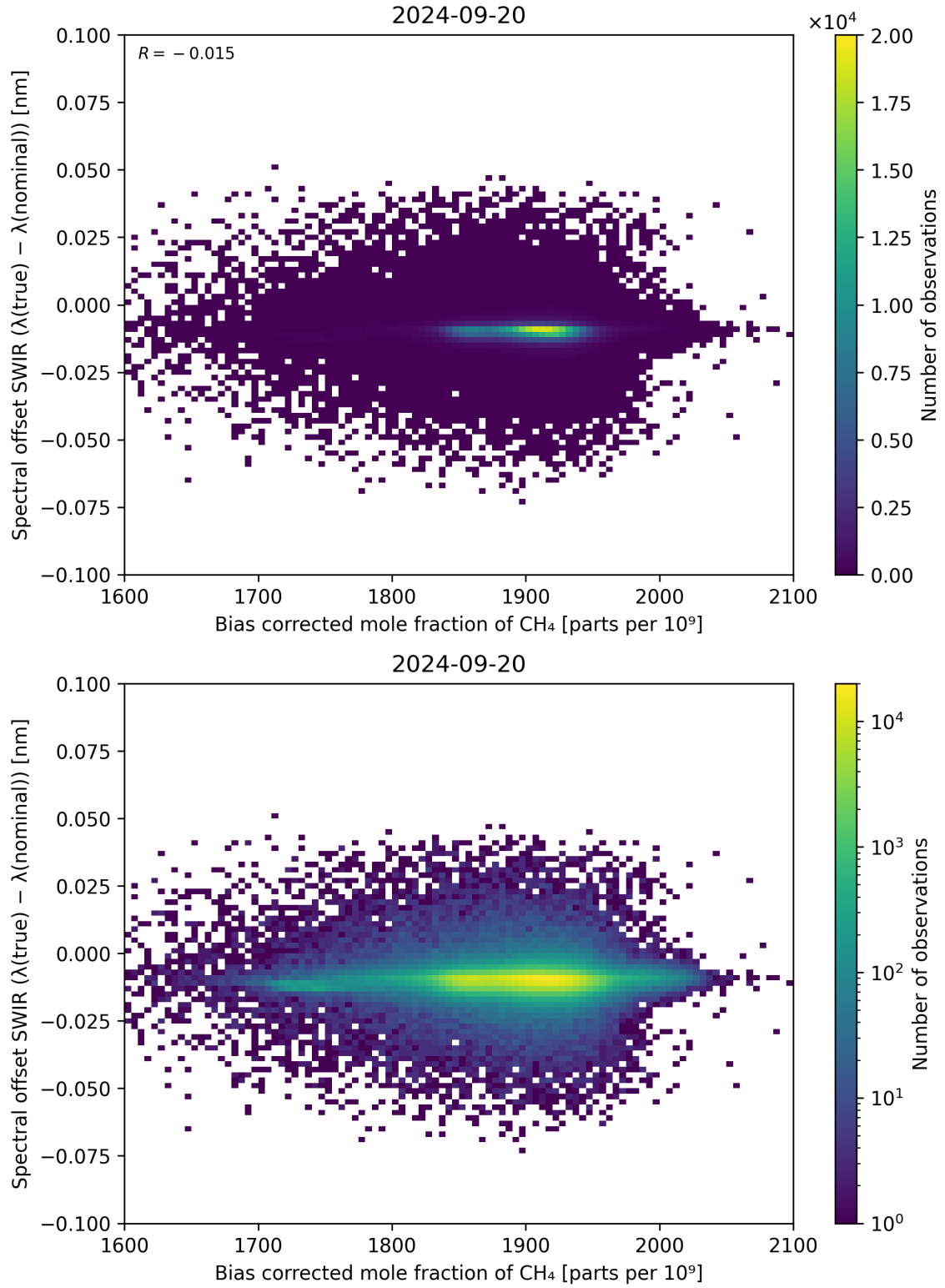
Figure 69: Scatter density plot of “Bias corrected mole fraction of \text{CH}_4 ” against “Spectral offset SWIR ( \lambda_{\text{true}} - \lambda_{\text{nominal}} )” for 2024-09-19 to 2024-09-21.
