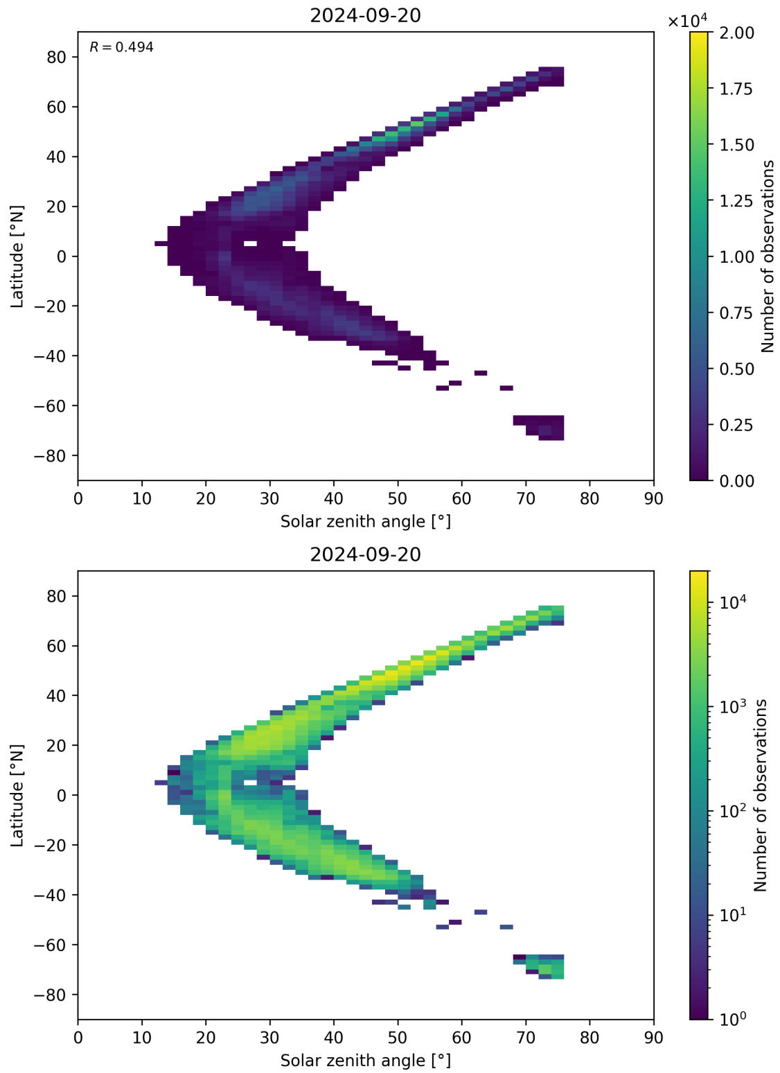
Figure 98: Scatter density plot of “Solar zenith angle” against “Latitude” for 2024-09-19 to 2024-09-21.
