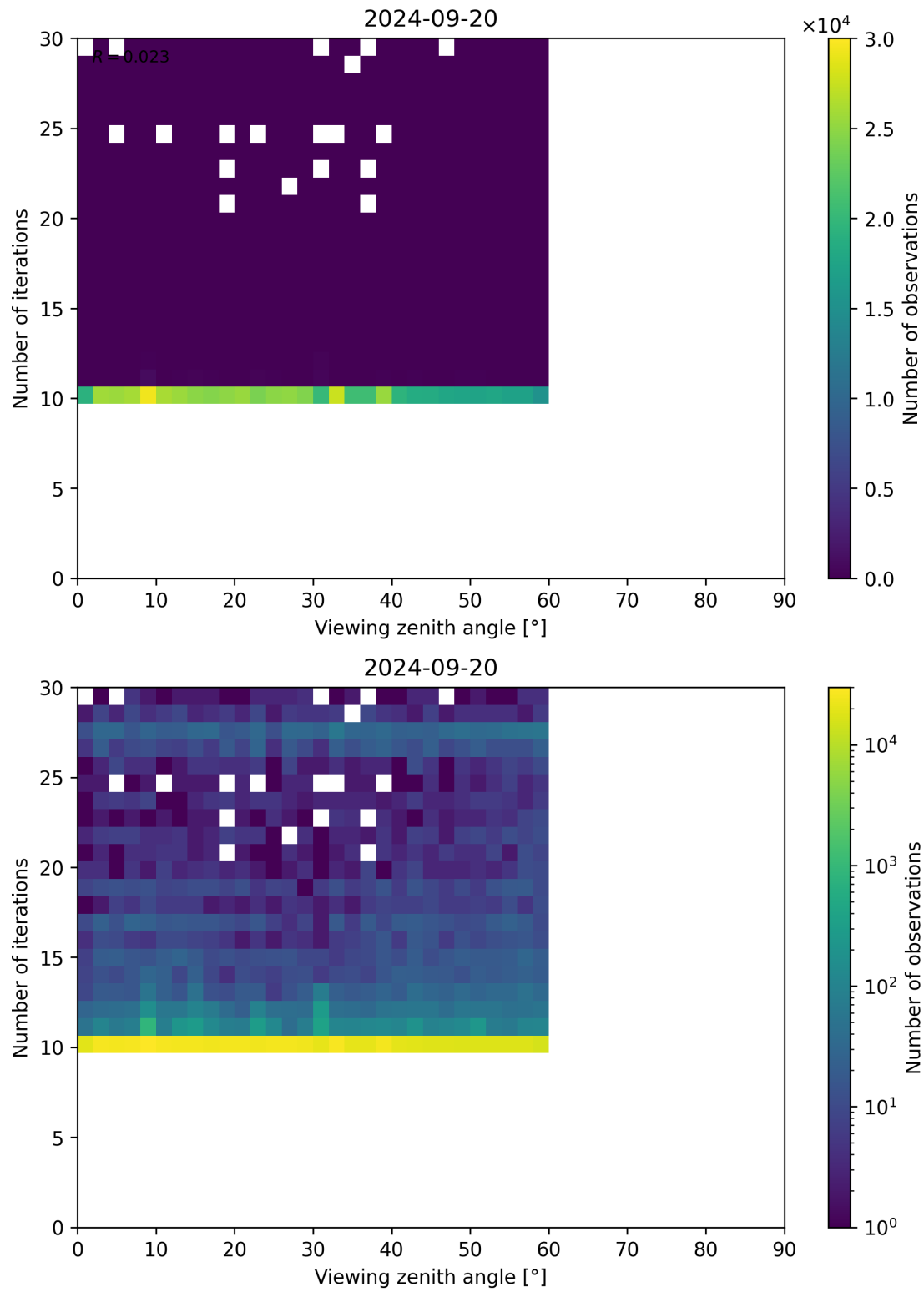
Figure 113: Scatter density plot of “Viewing zenith angle” against “Number of iterations” for 2024-09-19 to 2024-09-21.
