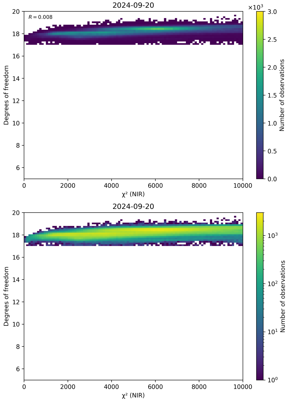
Figure 44: Scatter density plot of “ \chi^2 (NIR)” against “Degrees of freedom” for 2024-09-19 to 2024-09-21.
