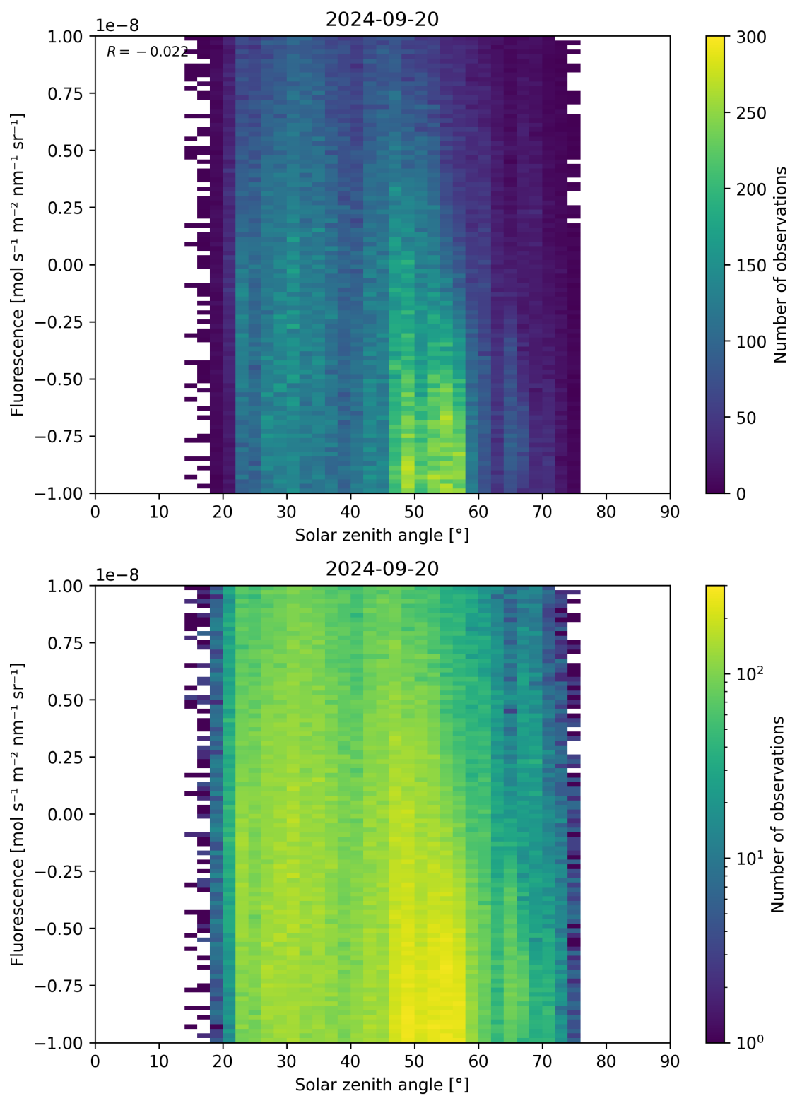
Figure 97: Scatter density plot of “Solar zenith angle” against “Fluorescence” for 2024-09-19 to 2024-09-21.
