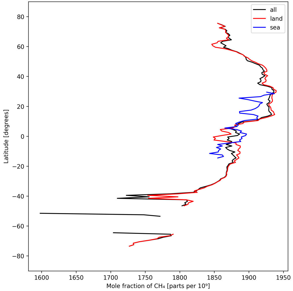
Figure 12: Zonal average of “Mole fraction of \text{CH}_4 ” for 2024-09-19 to 2024-09-21.
