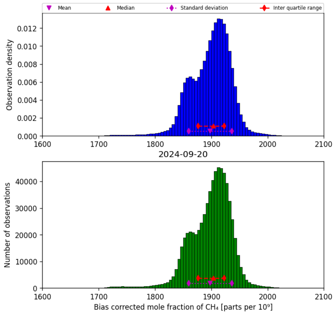
Figure 25: Histogram of “Bias corrected mole fraction of CH 4 ” for 2024-09-19 to 2024-09-21
