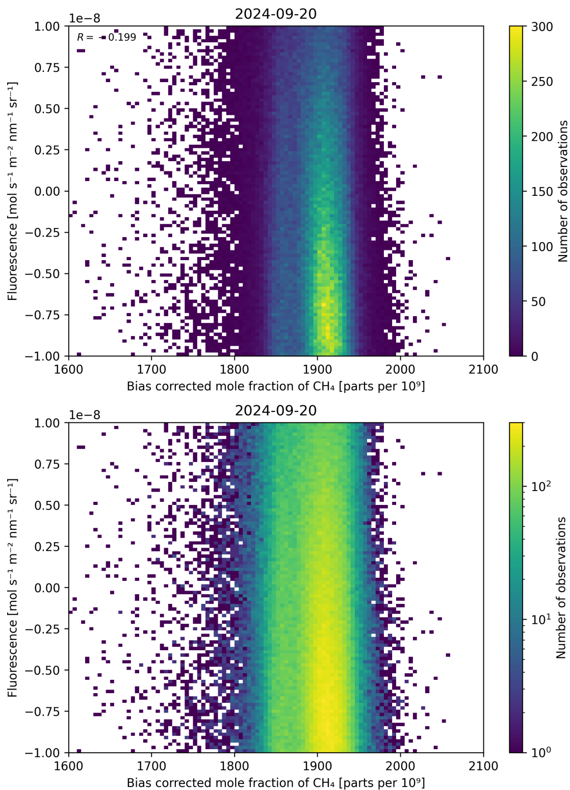
Figure 66: Scatter density plot of “Bias corrected mole fraction of CH 4 ” against “Fluorescence” for 2024-09-19 to 2024-09-21.
