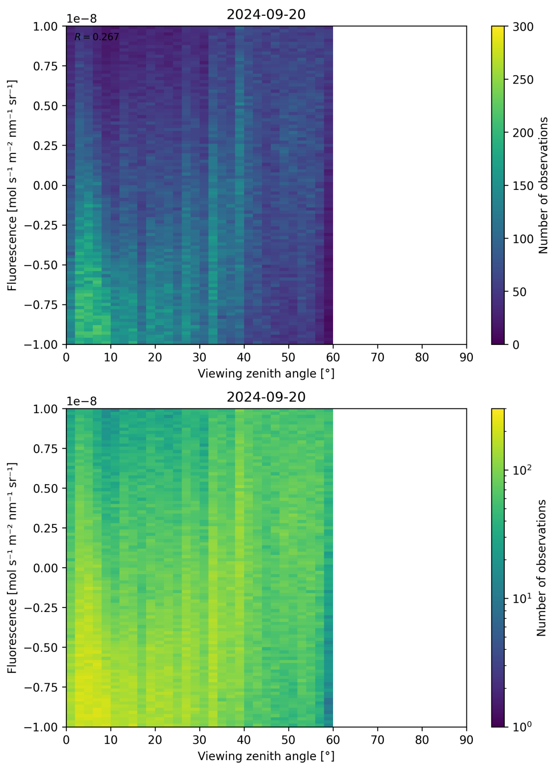
Figure 108: Scatter density plot of “Viewing zenith angle” against “Fluorescence” for 2024-09-19 to 2024-09-21.
