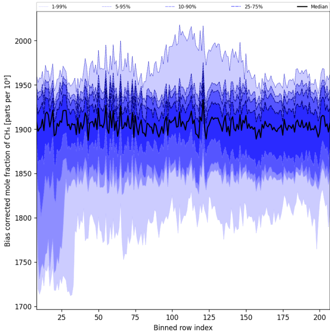
Figure 36: Along track statistics of “Bias corrected mole fraction of CH 4 ” for 2024-09-19 to 2024-09-21
