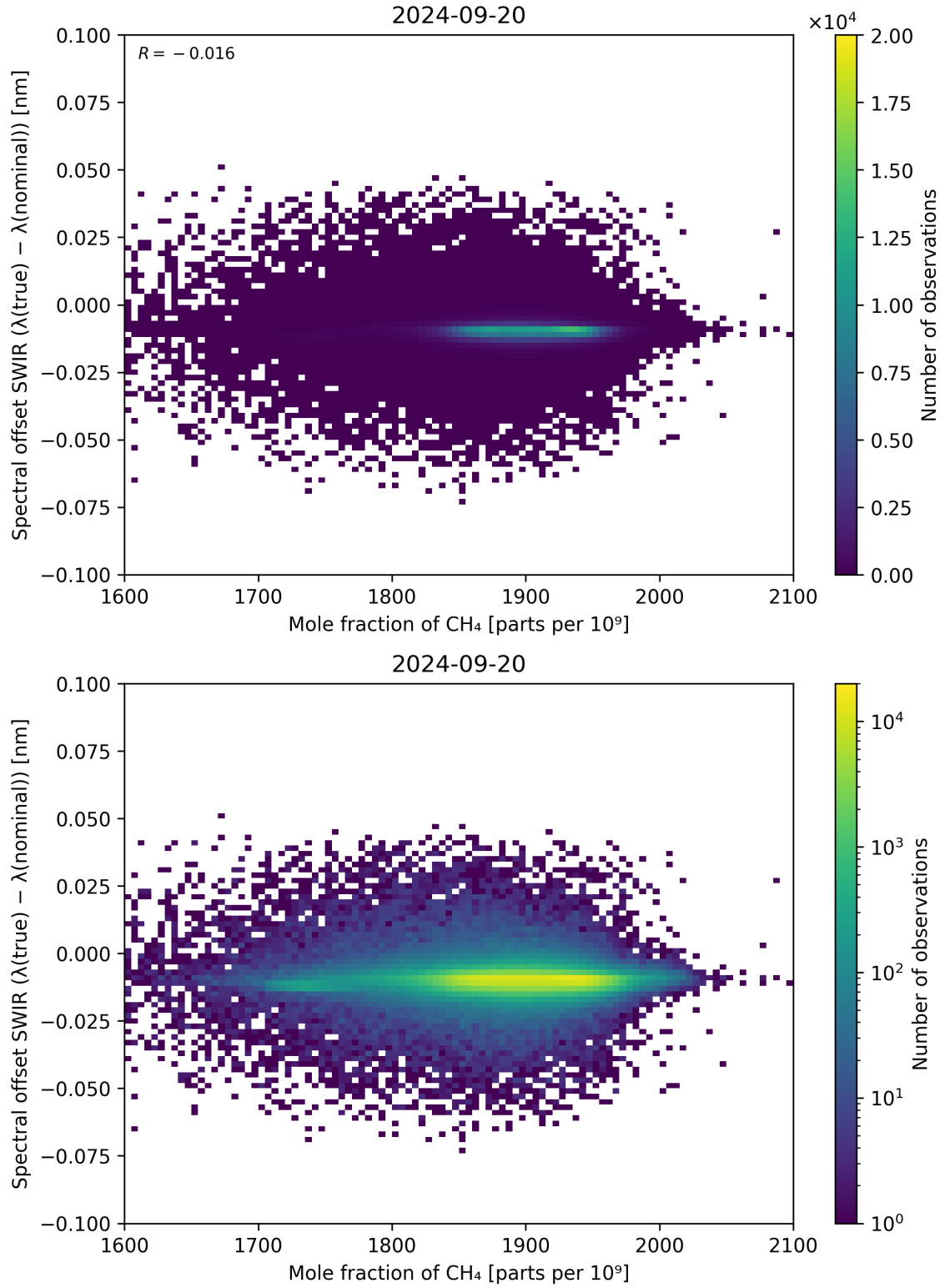
Figure 86: Scatter density plot of “Mole fraction of CH 4 ” against “Spectral offset SWIR ( \lambda_{\text{true}} - \lambda_{\text{nominal}} )” for 2024-09-19 to 2024-09-21.
