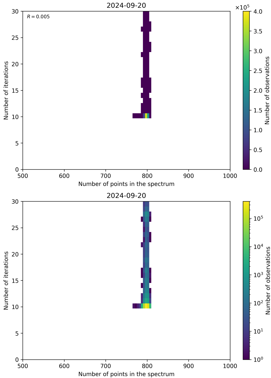
Figure 92: Scatter density plot of “Number of points in the spectrum” against “Number of iterations” for 2024-09-19 to 2024-09-21.
