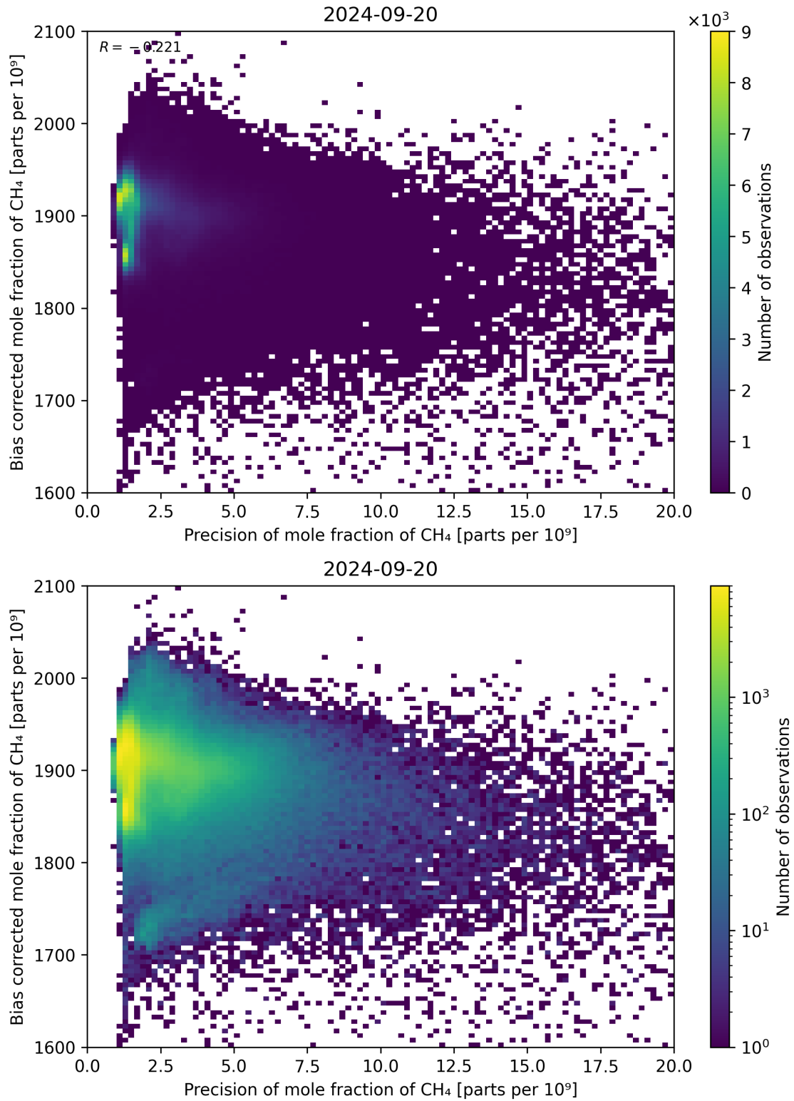
Figure 82: Scatter density plot of “Precision of mole fraction of CH 4 ” against “Bias corrected mole fraction of CH 4 ” for 2024-09-19 to 2024-09-21.
