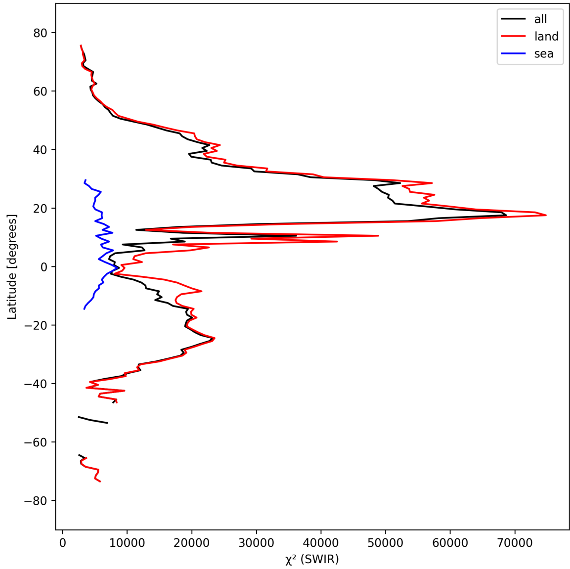
Figure 17: Zonal average of “ \chi^2 (SWIR)” for 2024-09-19 to 2024-09-21.
