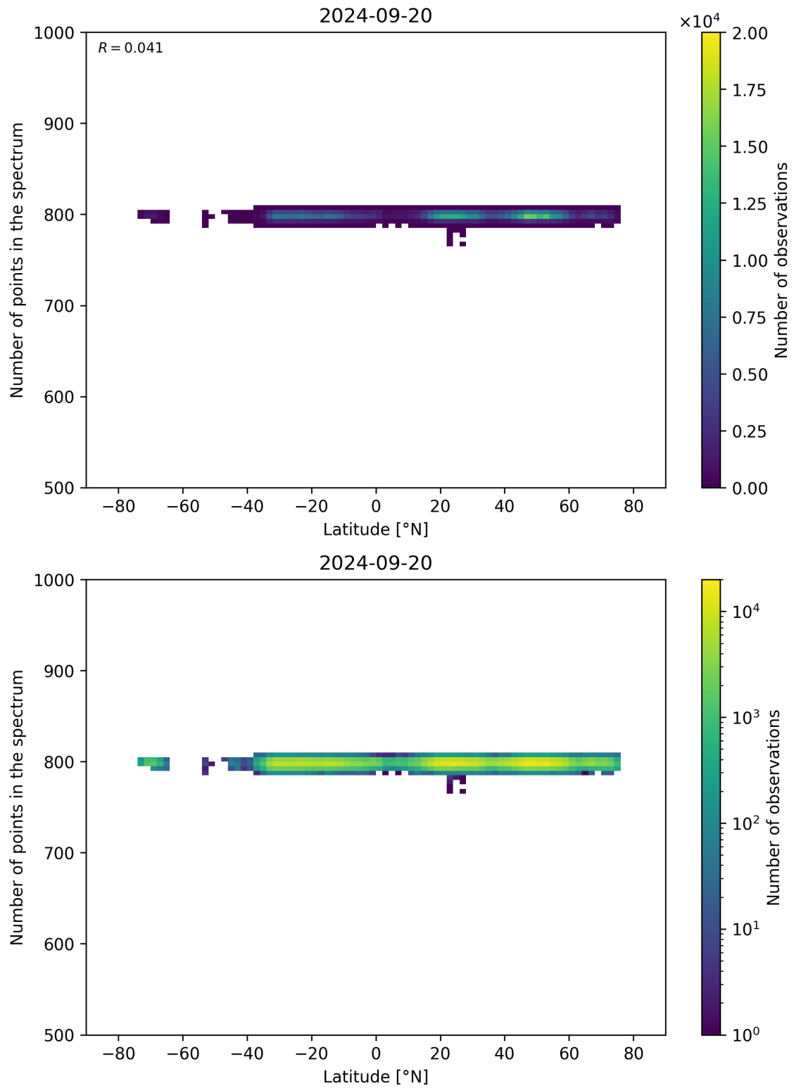
Figure 61: Scatter density plot of “Latitude” against “Number of points in the spectrum” for 2024-09-19 to 2024-09-21.
