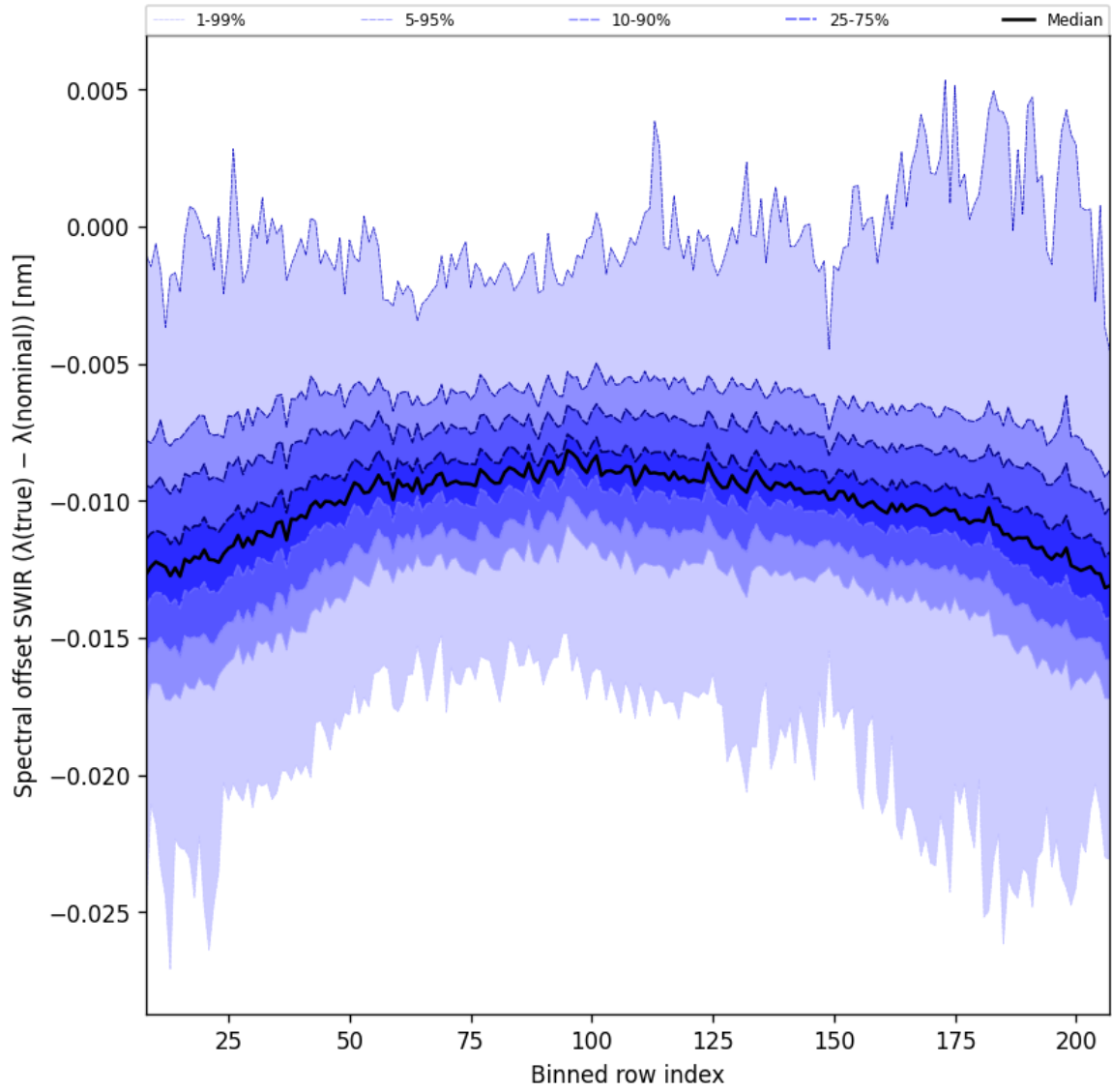
Figure 38: Along track statistics of “Spectral offset SWIR ( \lambda_{\text{true}} - \lambda_{\text{nominal}} )” for 2024-09-19 to 2024-09-21
