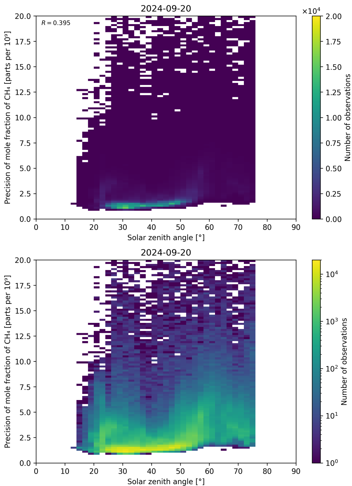
Figure 101: Scatter density plot of “Solar zenith angle” against “Precision of mole fraction of \text{CH}_4 ” for 2024-09-19 to 2024-09-21.
