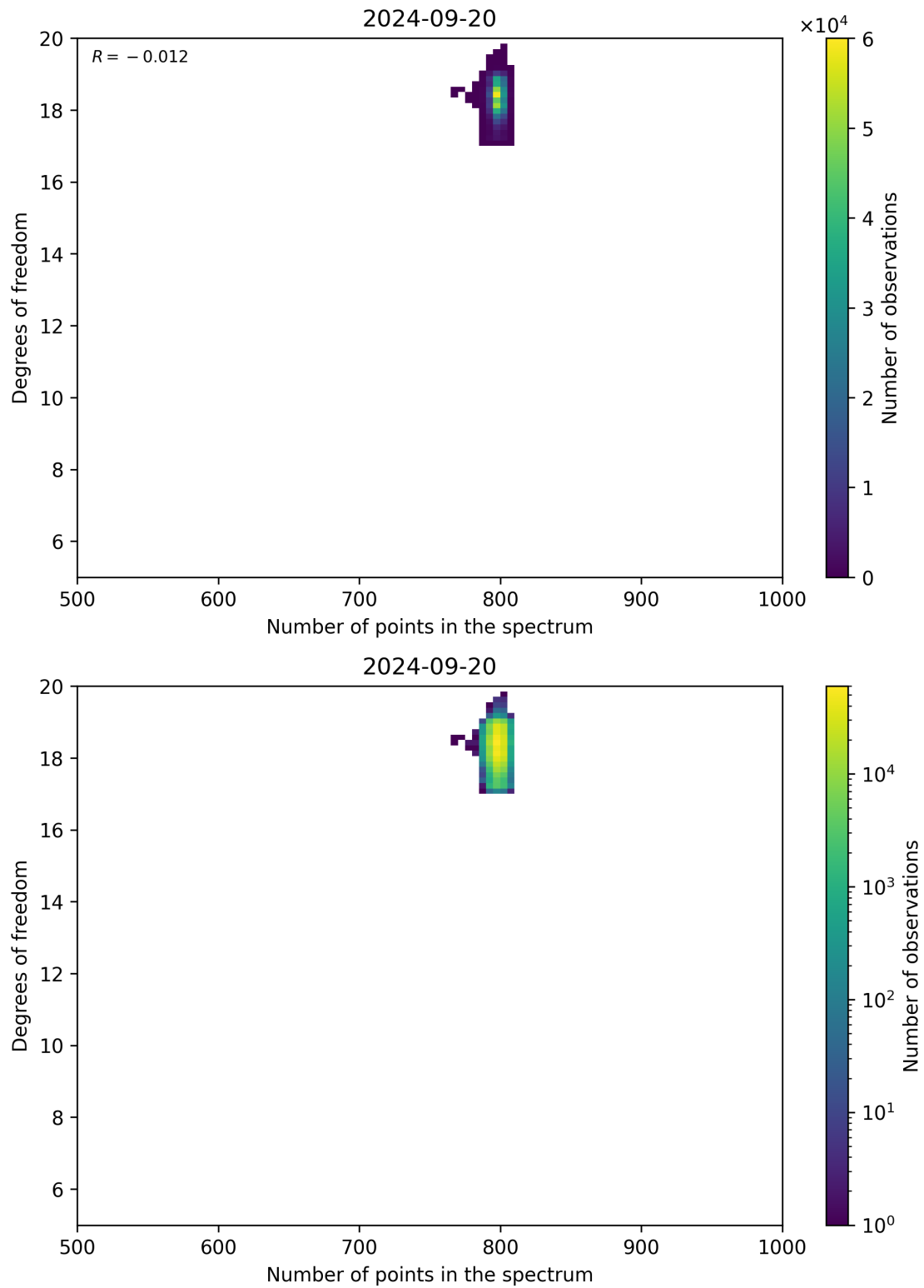
Figure 90: Scatter density plot of “Number of points in the spectrum” against “Degrees of freedom” for 2024-09-19 to 2024-09-21.
