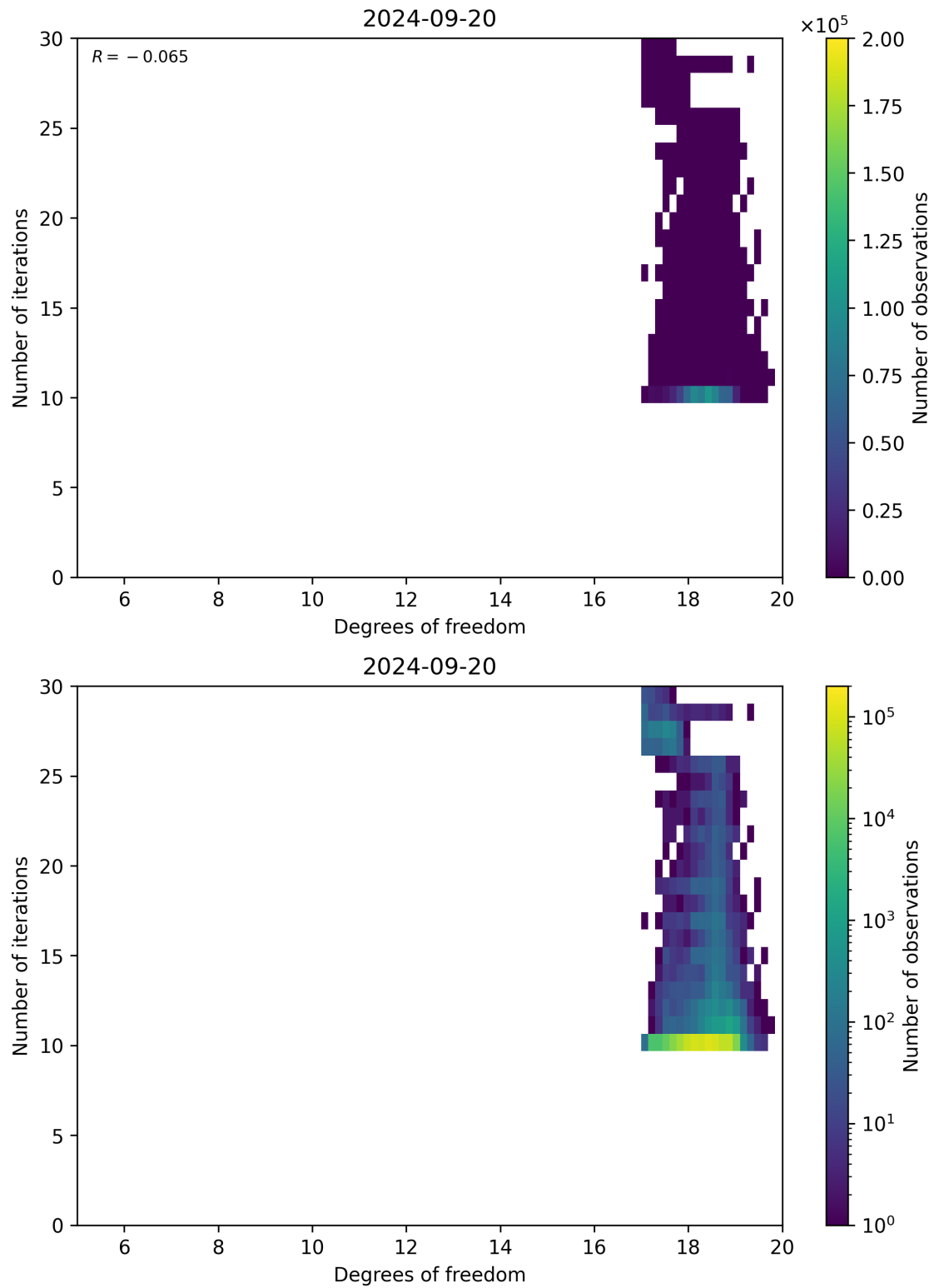
Figure 52: Scatter density plot of “Degrees of freedom” against “Number of iterations” for 2024-09-19 to 2024-09-21.
