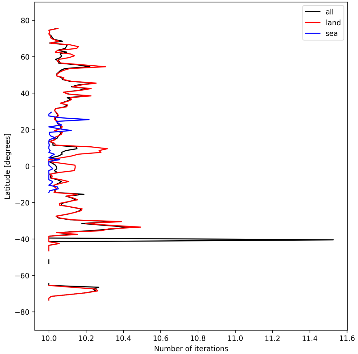
Figure 20: Zonal average of “Number of iterations” for 2024-09-19 to 2024-09-21.
