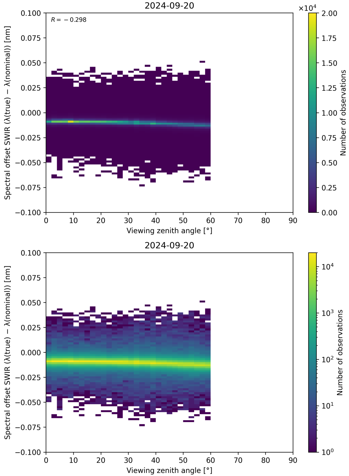
Figure 116: Scatter density plot of “Viewing zenith angle” against “Spectral offset SWIR ( \lambda_{\text{true}} - \lambda_{\text{nominal}} )” for 2024-09-19 to 2024-09-21.
