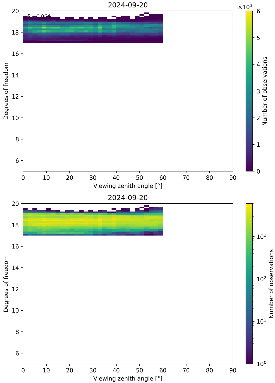
Figure 107: Scatter density plot of “Viewing zenith angle” against “Degrees of freedom” for 2024-09-19 to 2024-09-21.
