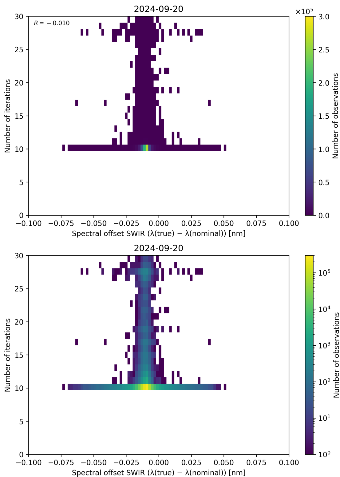
Figure 121: Scatter density plot of “Spectral offset SWIR ( \lambda_{\text{true}} - \lambda_{\text{nominal}} )” against “Number of iterations” for 2024-09-19 to 2024-09-21.
