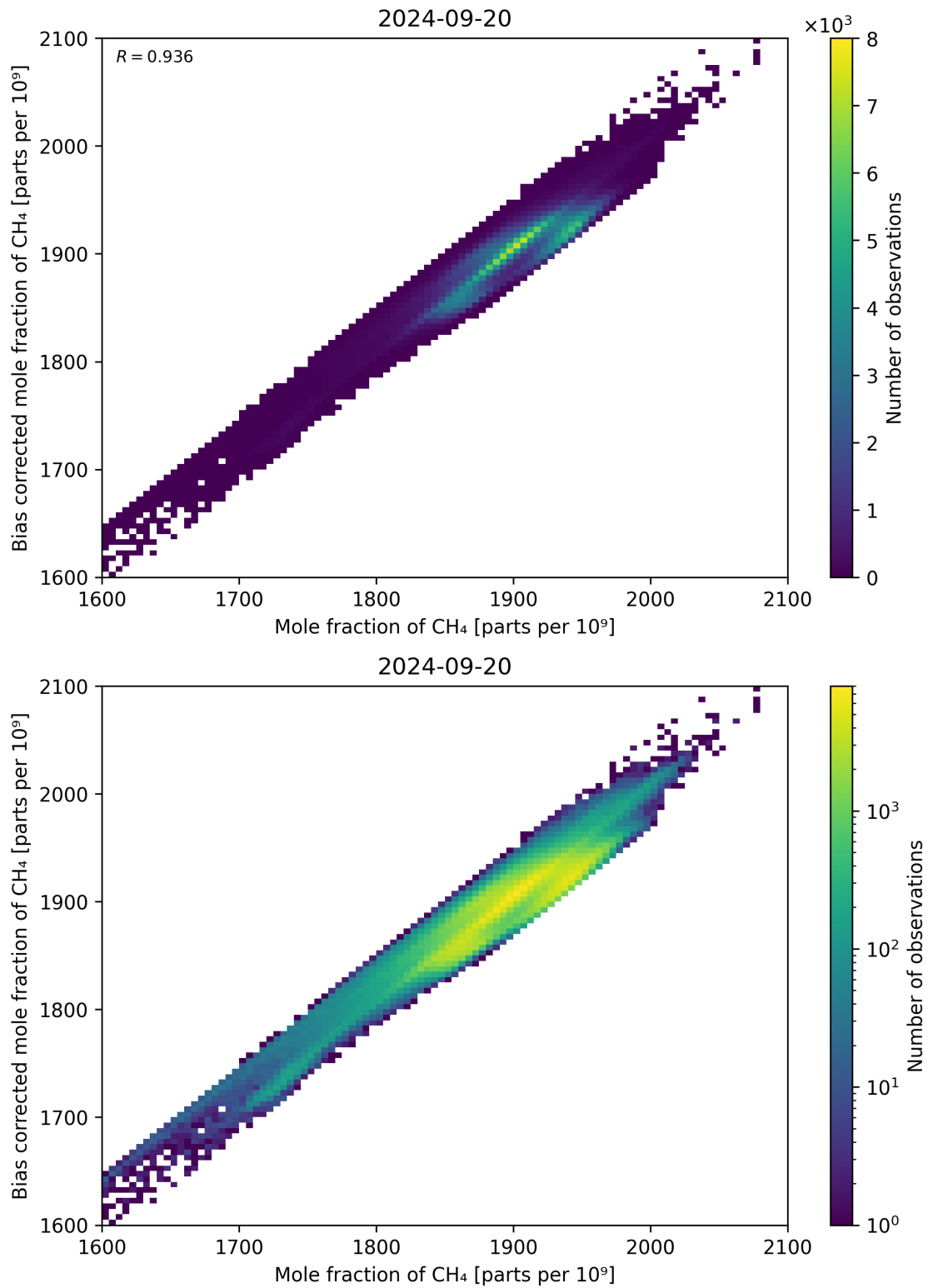
Figure 74: Scatter density plot of “Mole fraction of CH 4 ” against “Bias corrected mole fraction of CH 4 ” for 2024-09-19 to 2024-09-21.
