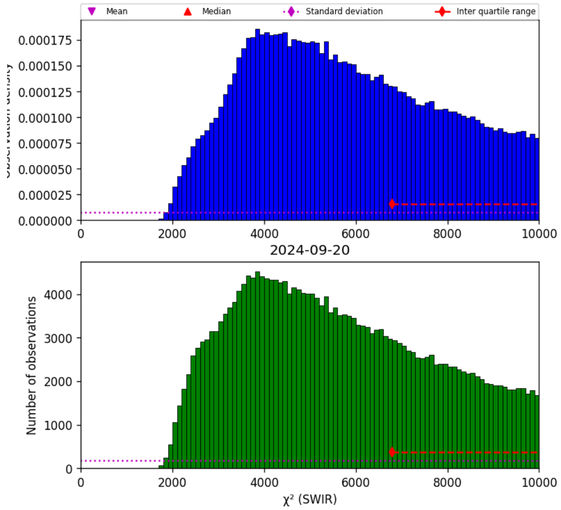
Figure 28: Histogram of " \chi^2 (SWIR)" for 2024-09-19 to 2024-09-21
