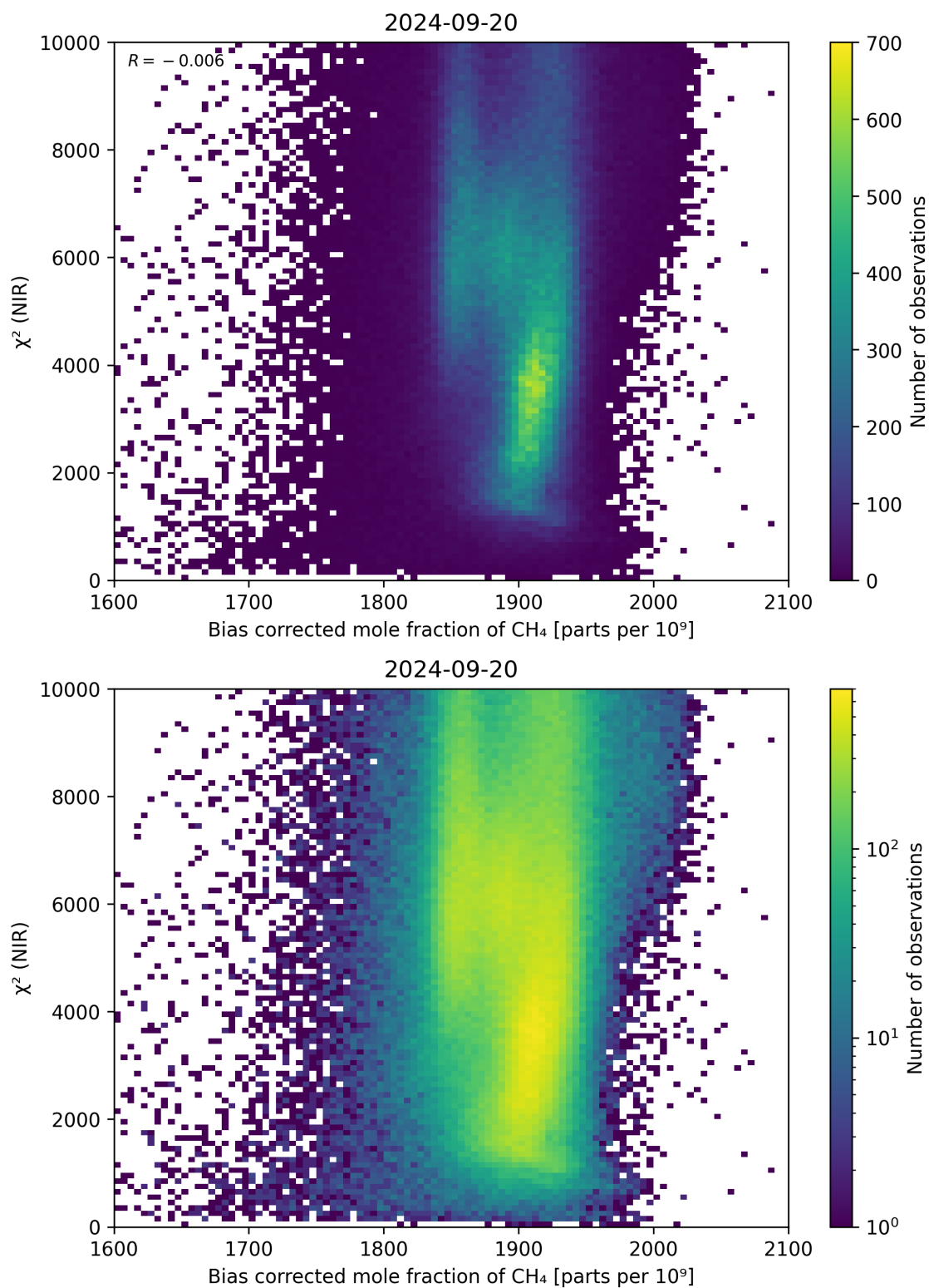
Figure 63: Scatter density plot of “Bias corrected mole fraction of CH 4 ” against “ \chi^2 (NIR)” for 2024-09-19 to 2024-09-21.
