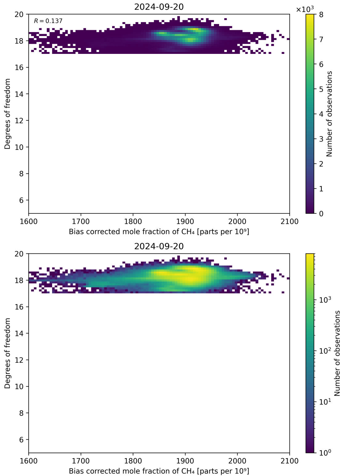
Figure 65: Scatter density plot of “Bias corrected mole fraction of CH 4 ” against “Degrees of freedom” for 2024-09-19 to 2024-09-21.
