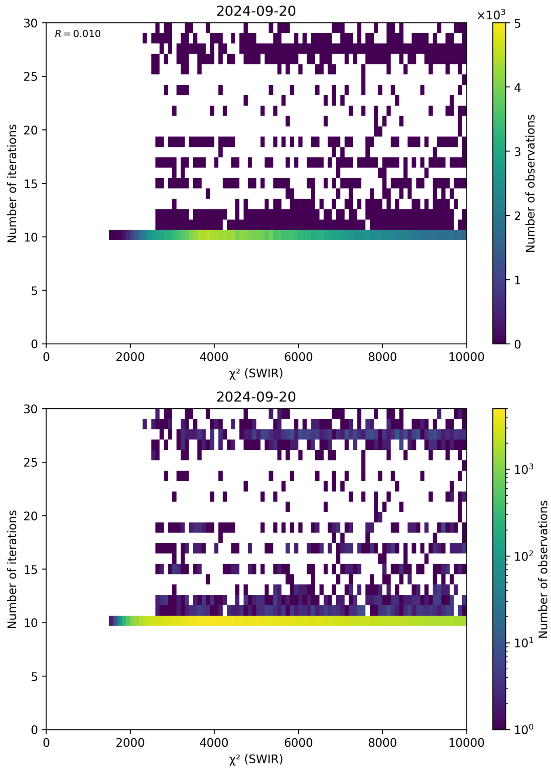
Figure 50: Scatter density plot of “ \chi^2 (SWIR)” against “Number of iterations” for 2024-09-19 to 2024-09-21.
