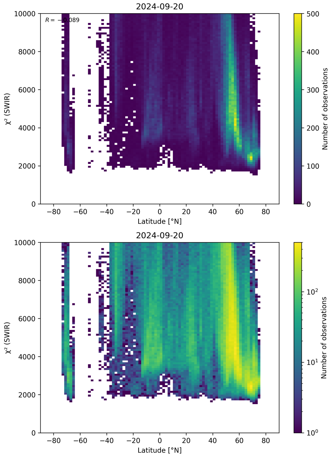
Figure 54: Scatter density plot of “Latitude” against “ \chi^2 (SWIR)” for 2024-09-19 to 2024-09-21.
