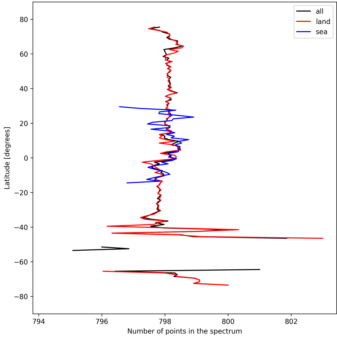
Figure 15: Zonal average of “Number of points in the spectrum” for 2024-09-19 to 2024-09-21.
