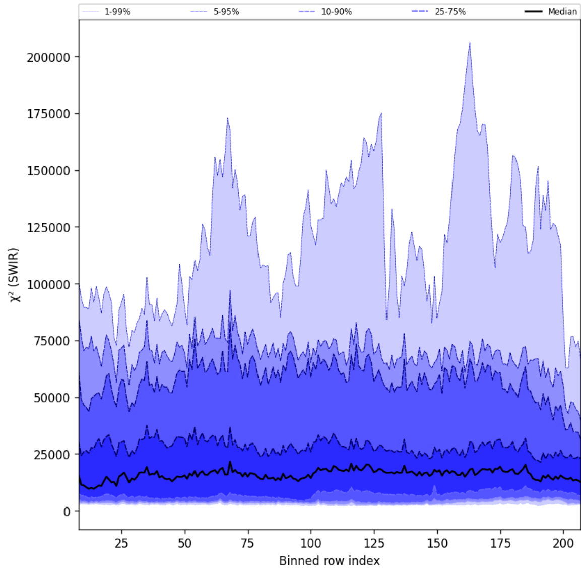
Figure 39: Along track statistics of “ \chi^2 (SWIR)” for 2024-09-19 to 2024-09-21
