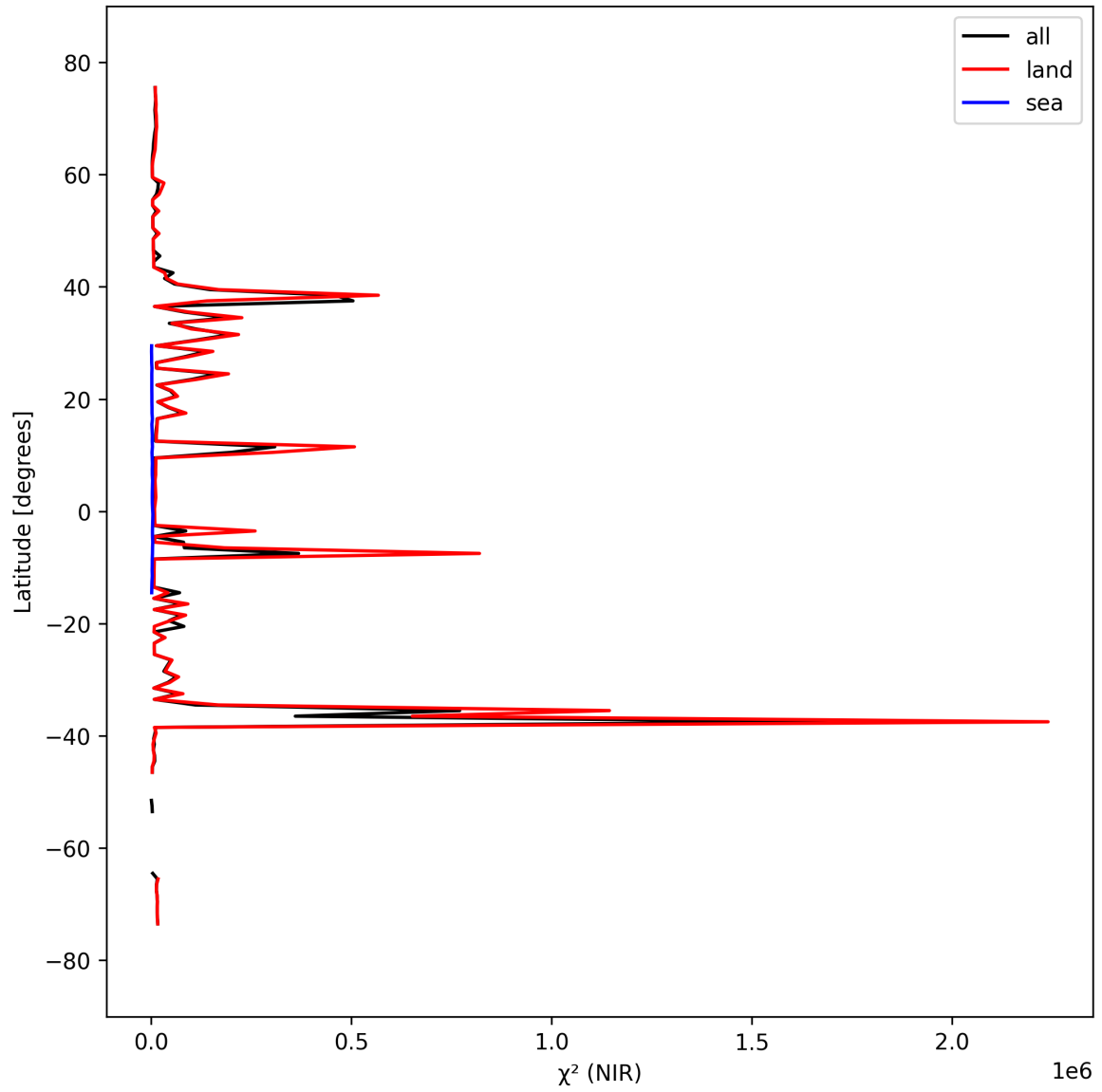
Figure 18: Zonal average of “ \chi^2 (NIR)” for 2024-09-19 to 2024-09-21.
