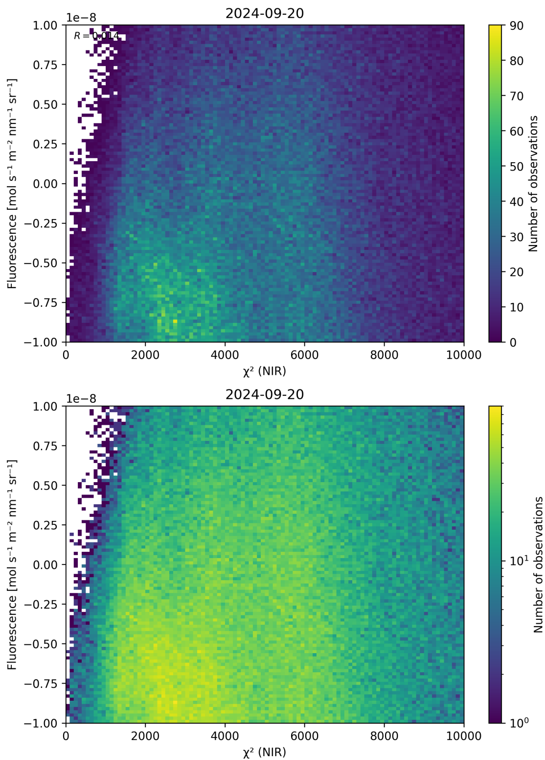
Figure 45: Scatter density plot of “ \chi^2 (NIR)” against “Fluorescence” for 2024-09-19 to 2024-09-21.
