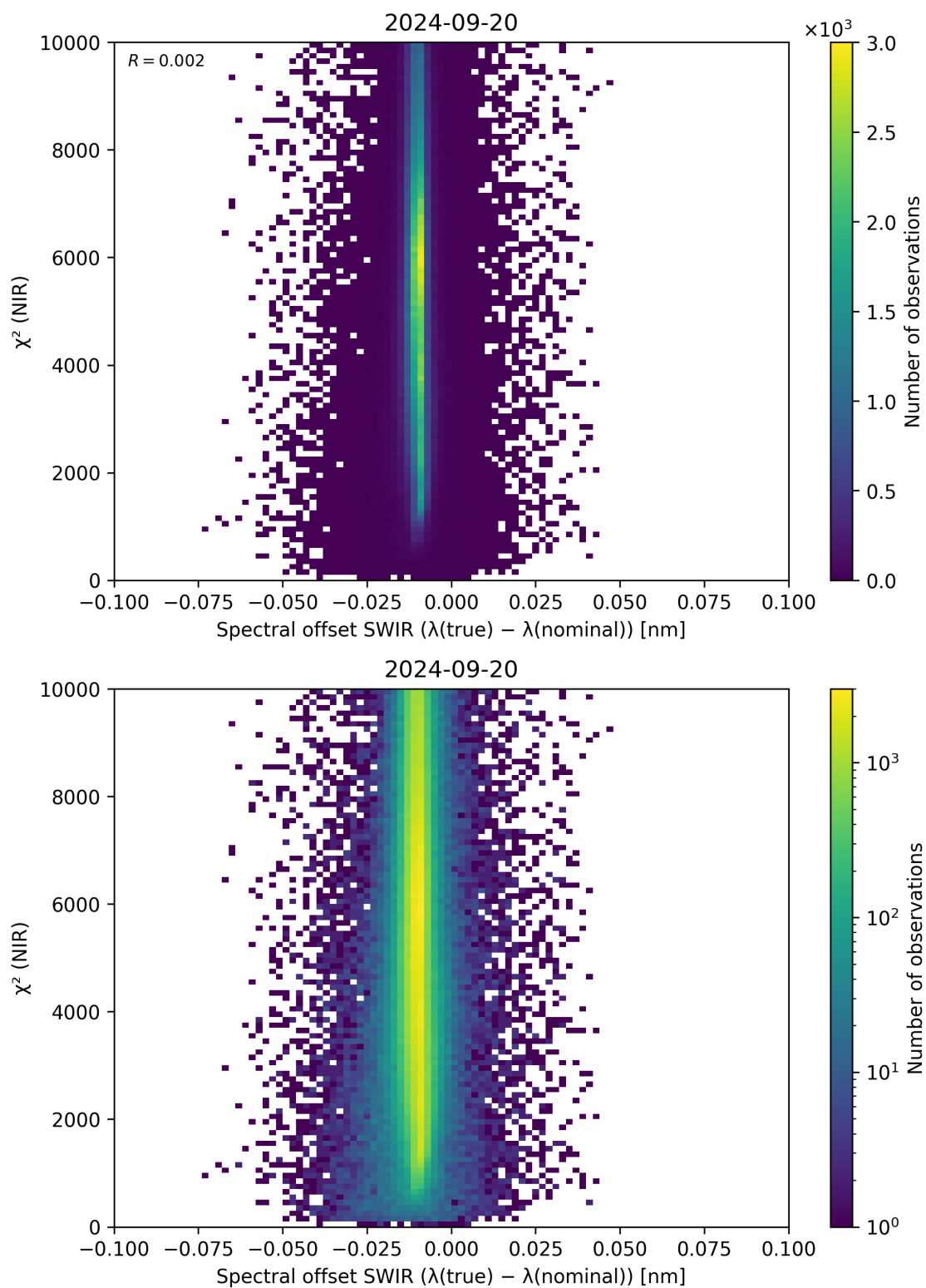
Figure 117: Scatter density plot of “Spectral offset SWIR ( \lambda_{\text{true}} - \lambda_{\text{nominal}} )” against “ \chi^2 (NIR)” for 2024-09-19 to 2024-09-21.
