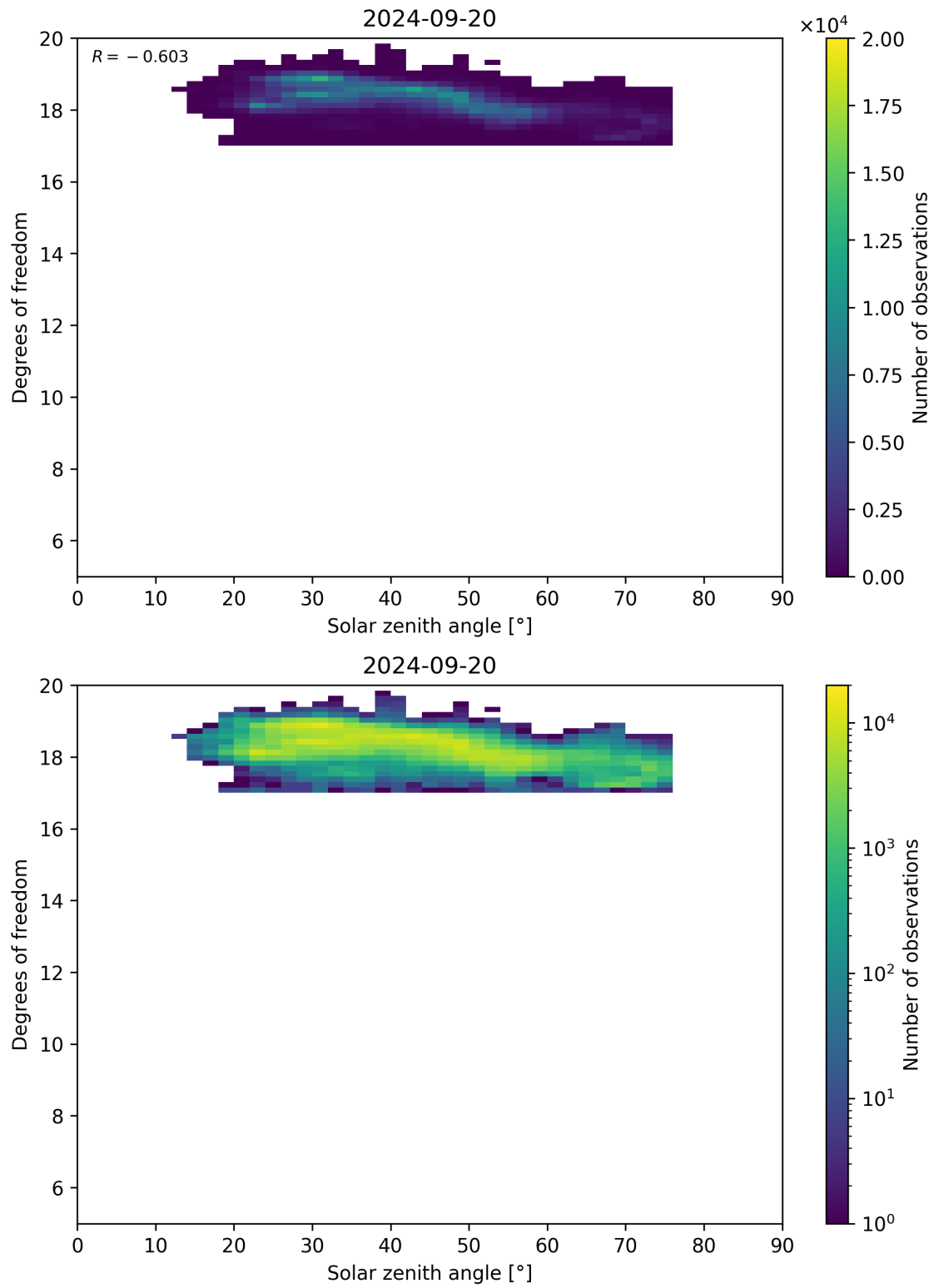
Figure 96: Scatter density plot of “Solar zenith angle” against “Degrees of freedom” for 2024-09-19 to 2024-09-21.
