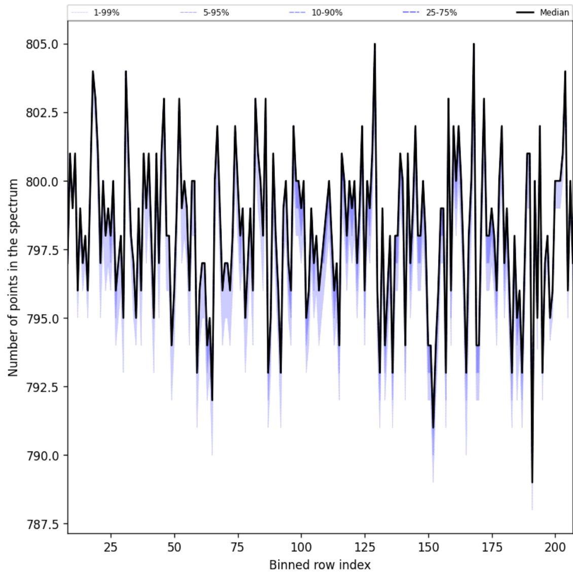
Figure 37: Along track statistics of “Number of points in the spectrum” for 2024-09-19 to 2024-09-21
