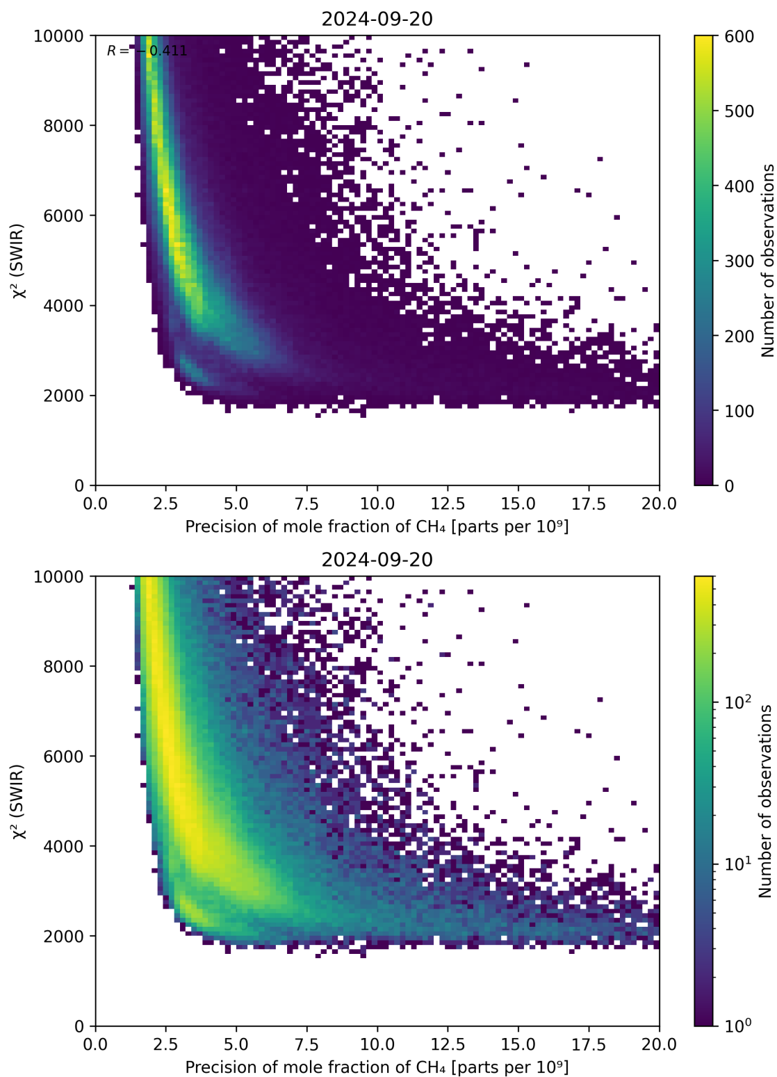
Figure 79: Scatter density plot of “Precision of mole fraction of \text{CH}_4 ” against “ \chi^2 (SWIR)” for 2024-09-19 to 2024-09-21.
