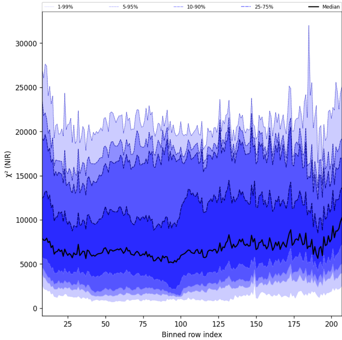
Figure 40: Along track statistics of “ \chi^2 (NIR)” for 2024-09-19 to 2024-09-21
