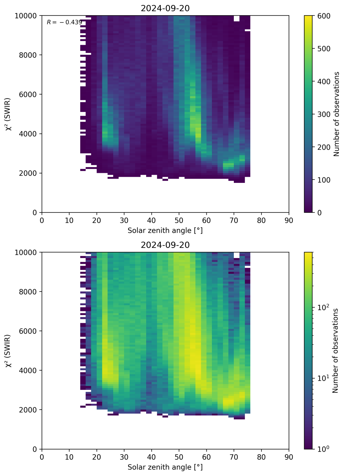
Figure 95: Scatter density plot of “Solar zenith angle” against “ \chi^2 (SWIR)” for 2024-09-19 to 2024-09-21.
