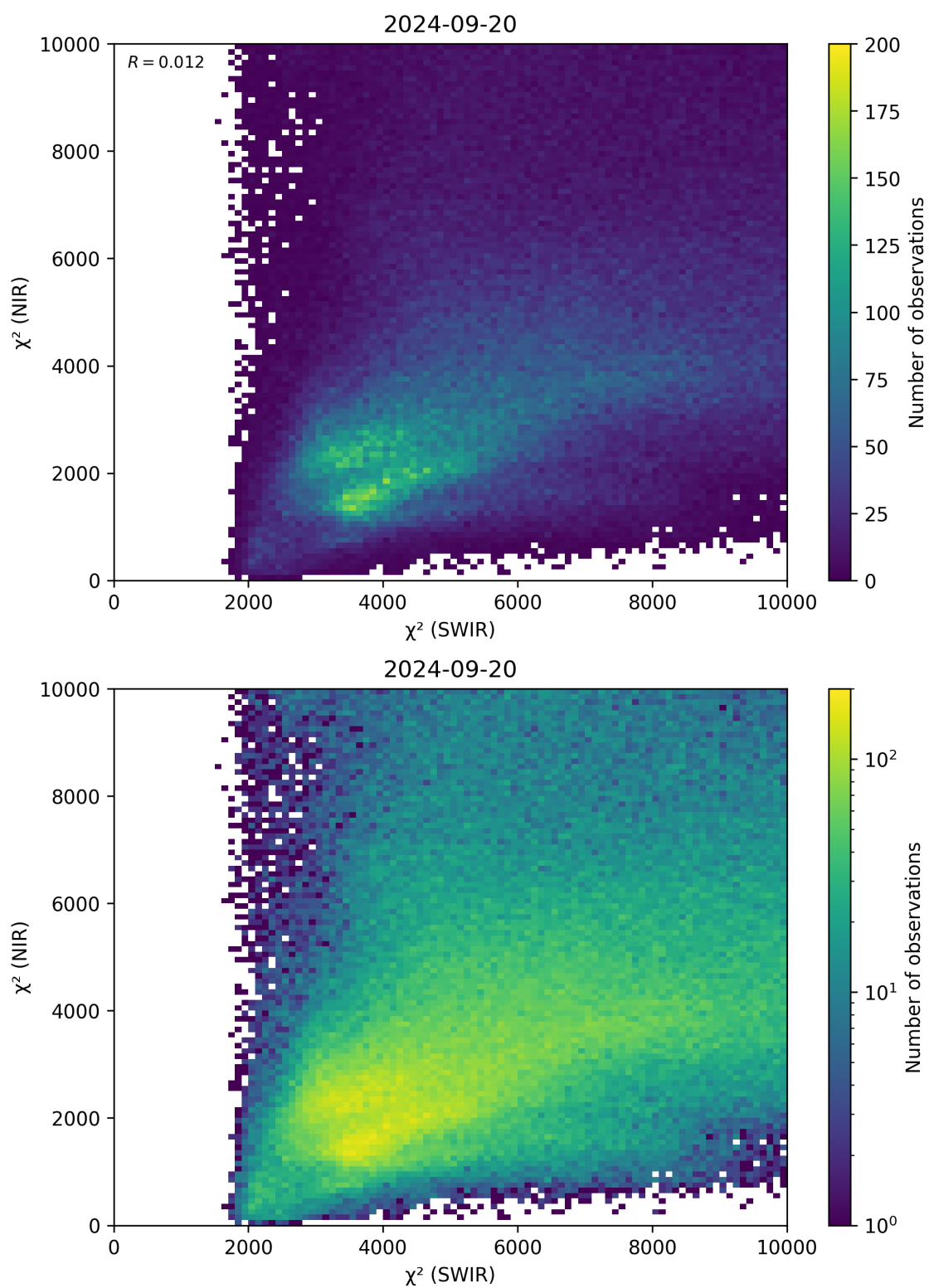
Figure 47: Scatter density plot of “ \chi^2 (SWIR)” against “ \chi^2 (NIR)” for 2024-09-19 to 2024-09-21.
