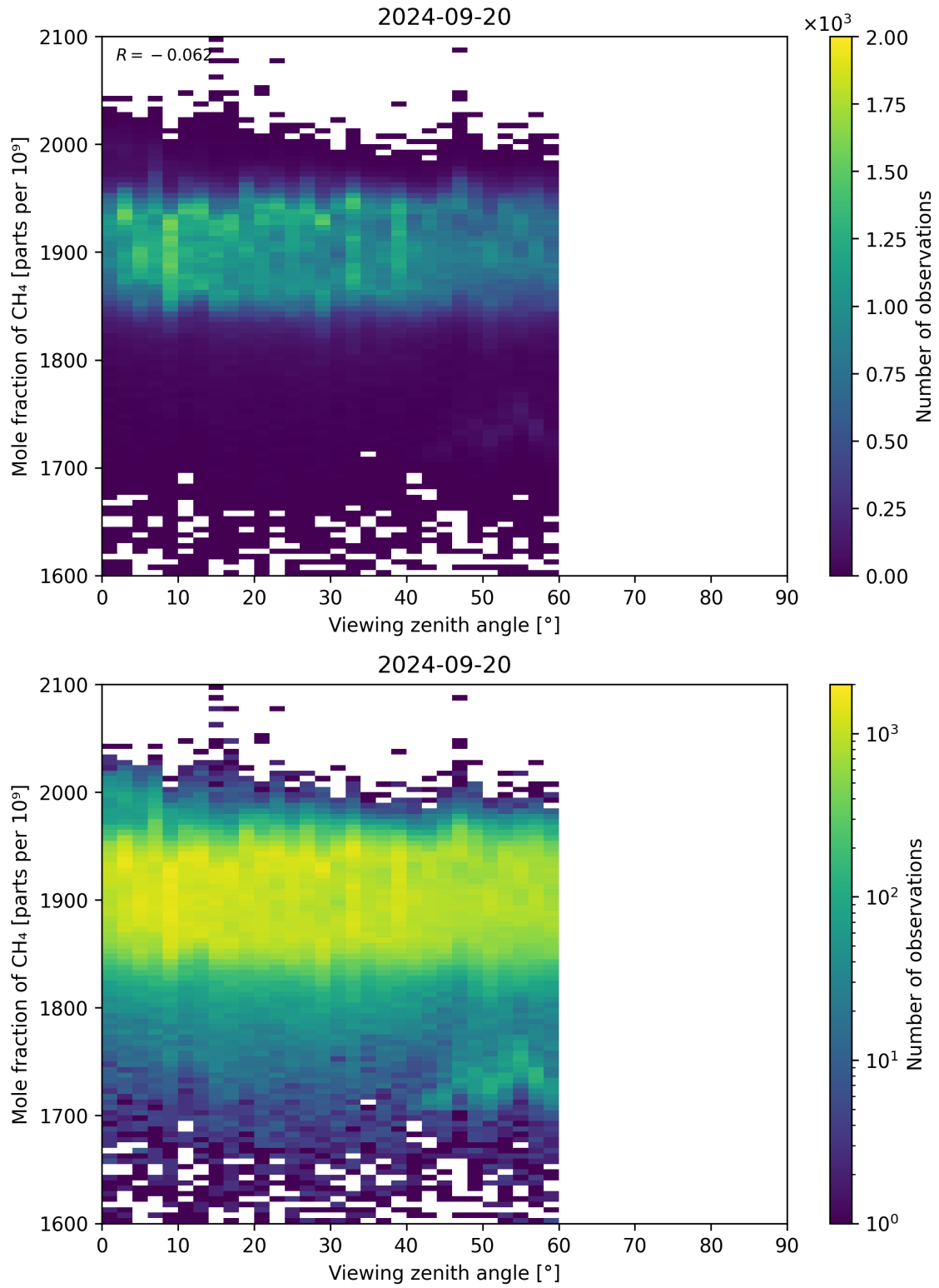
Figure 110: Scatter density plot of “Viewing zenith angle” against “Mole fraction of CH 4 ” for 2024-09-19 to 2024-09-21.
