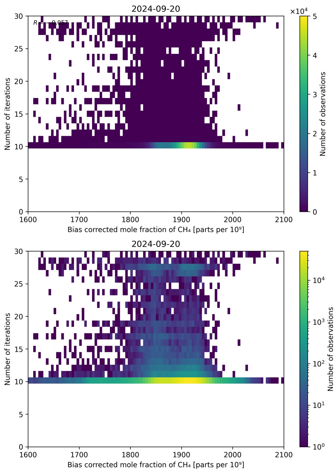
Figure 67: Scatter density plot of “Bias corrected mole fraction of CH 4 ” against “Number of iterations” for 2024-09-19 to 2024-09-21.
