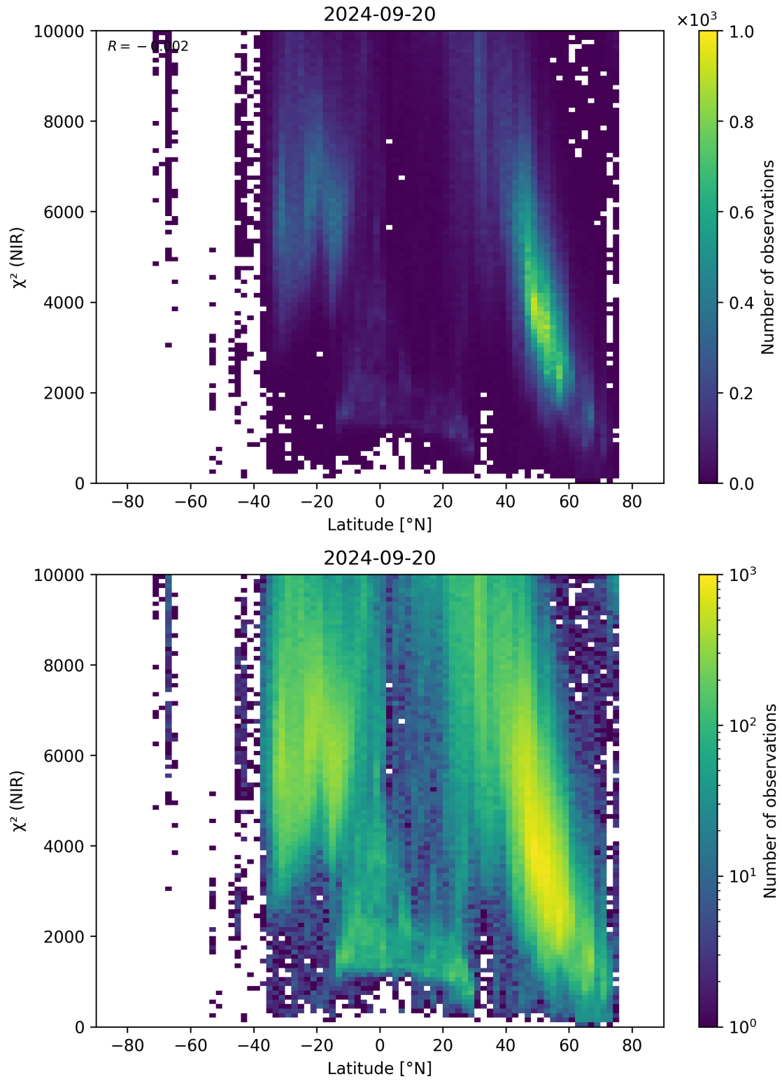
Figure 53: Scatter density plot of “Latitude” against “ \chi^2 (NIR)” for 2024-09-19 to 2024-09-21.
