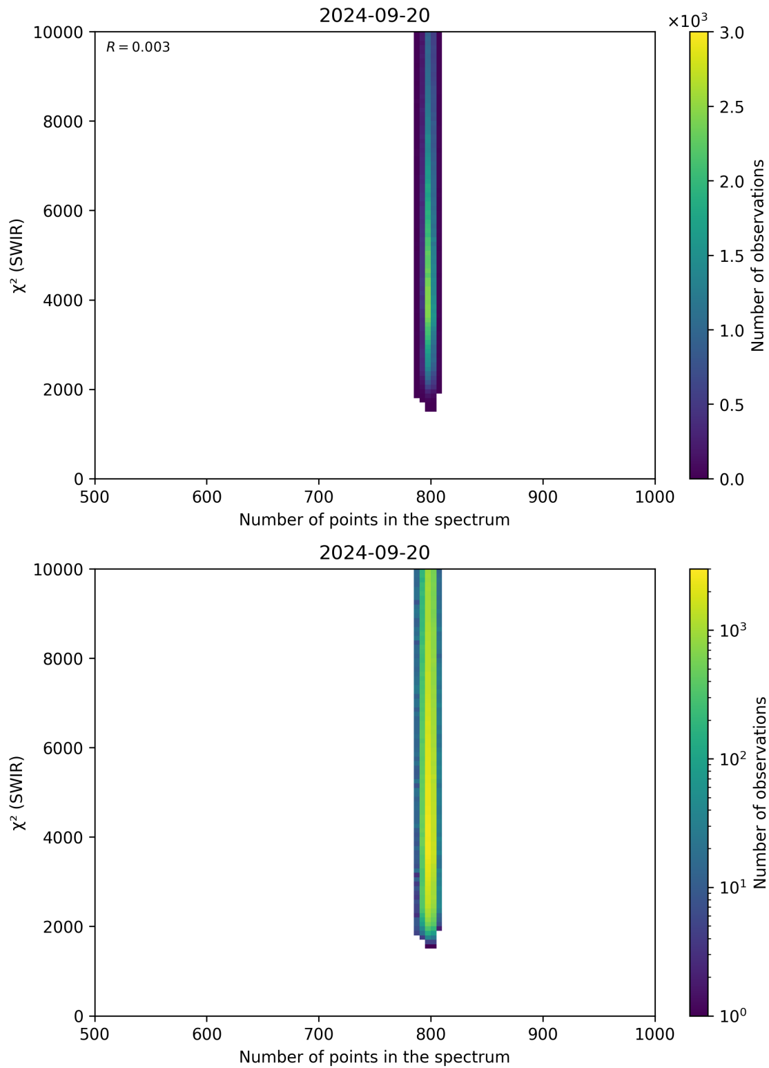
Figure 89: Scatter density plot of “Number of points in the spectrum” against “ \chi^2 (SWIR)” for 2024-09-19 to 2024-09-21.
