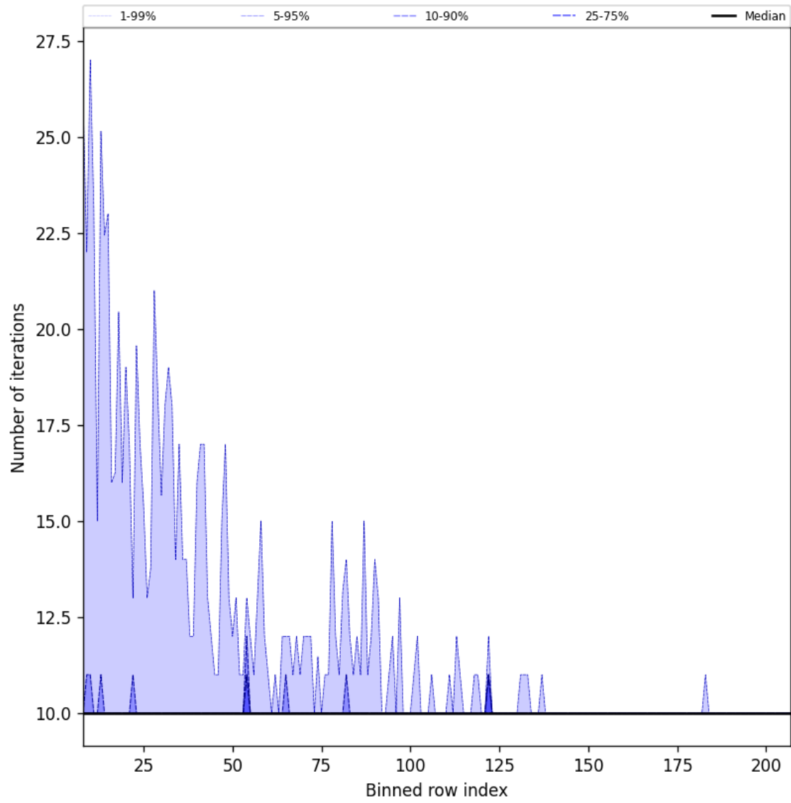
Figure 42: Along track statistics of “Number of iterations” for 2024-09-19 to 2024-09-21
