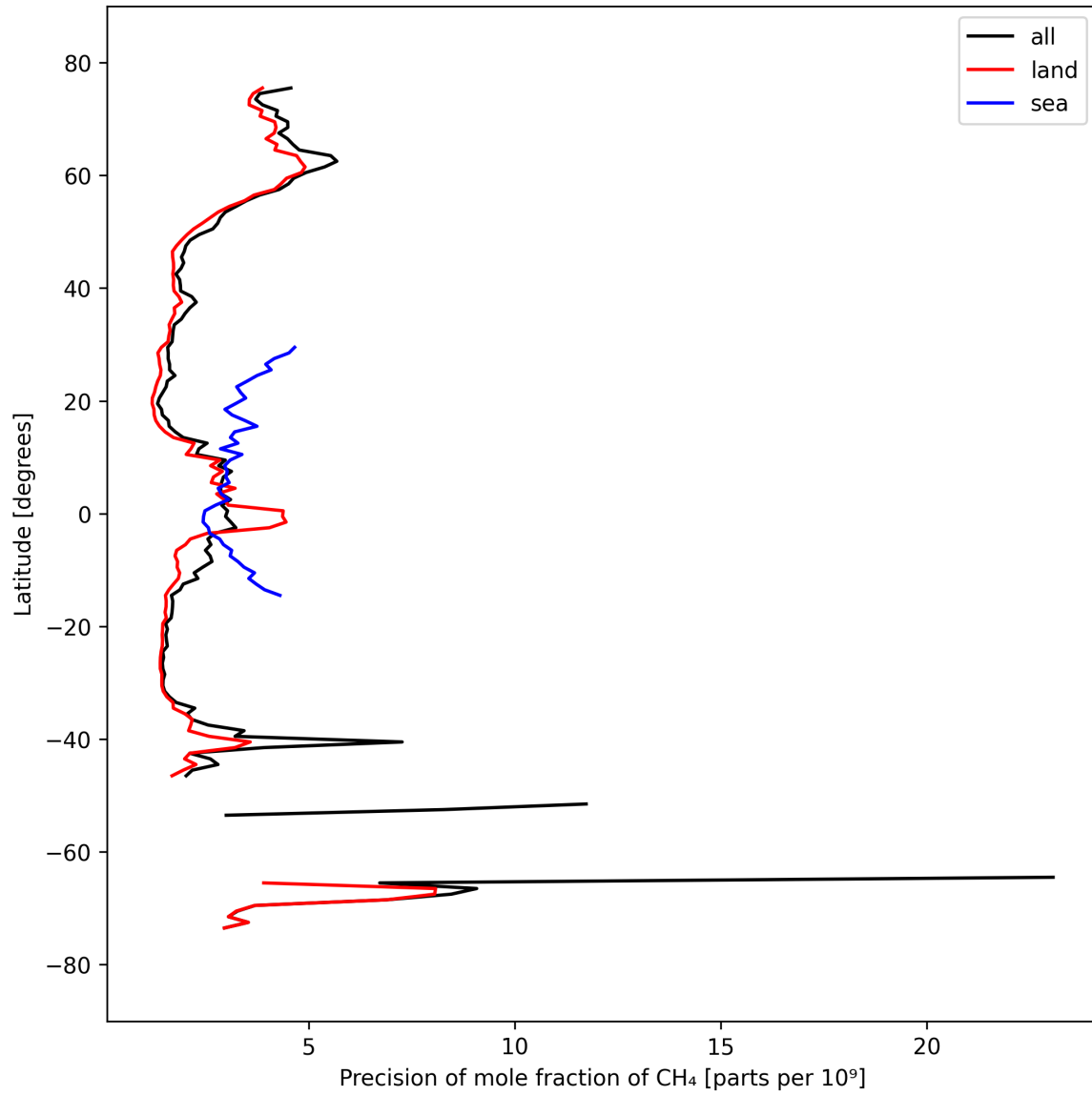
Figure 13: Zonal average of “Precision of mole fraction of CH 4 ” for 2024-09-19 to 2024-09-21.
