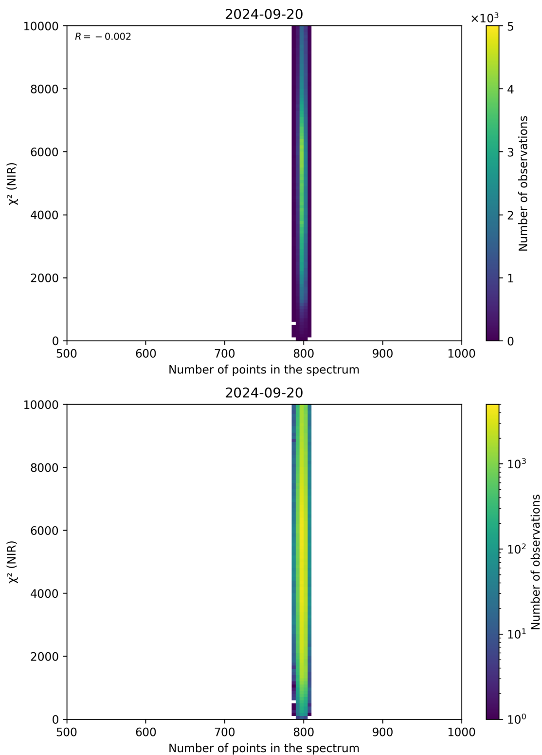
Figure 88: Scatter density plot of “Number of points in the spectrum” against “ \chi^2 (NIR)” for 2024-09-19 to 2024-09-21.
