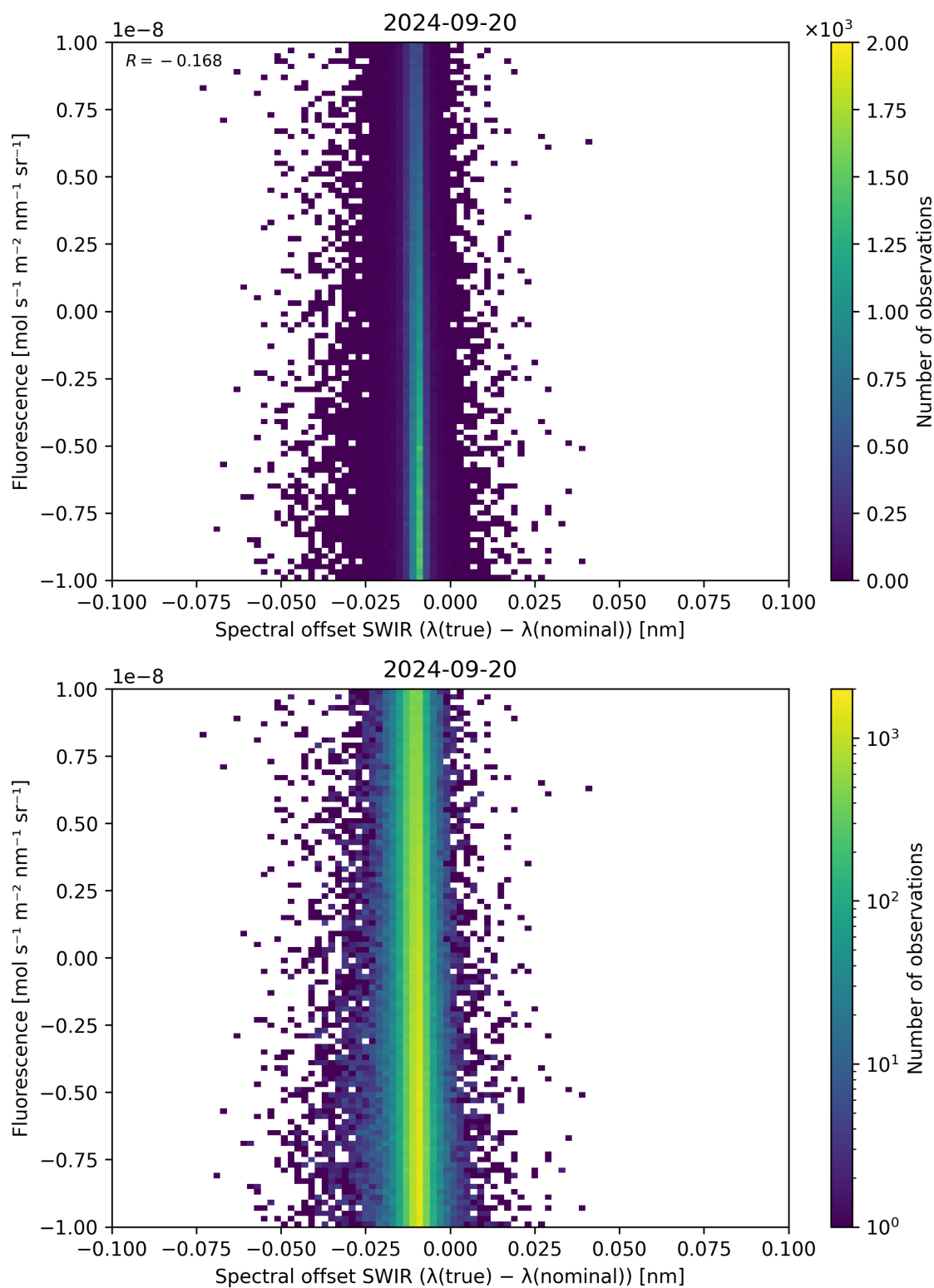
Figure 120: Scatter density plot of “Spectral offset SWIR ( \lambda_{\text{true}} - \lambda_{\text{nominal}} )” against “Fluorescence” for 2024-09-19 to 2024-09-21.
