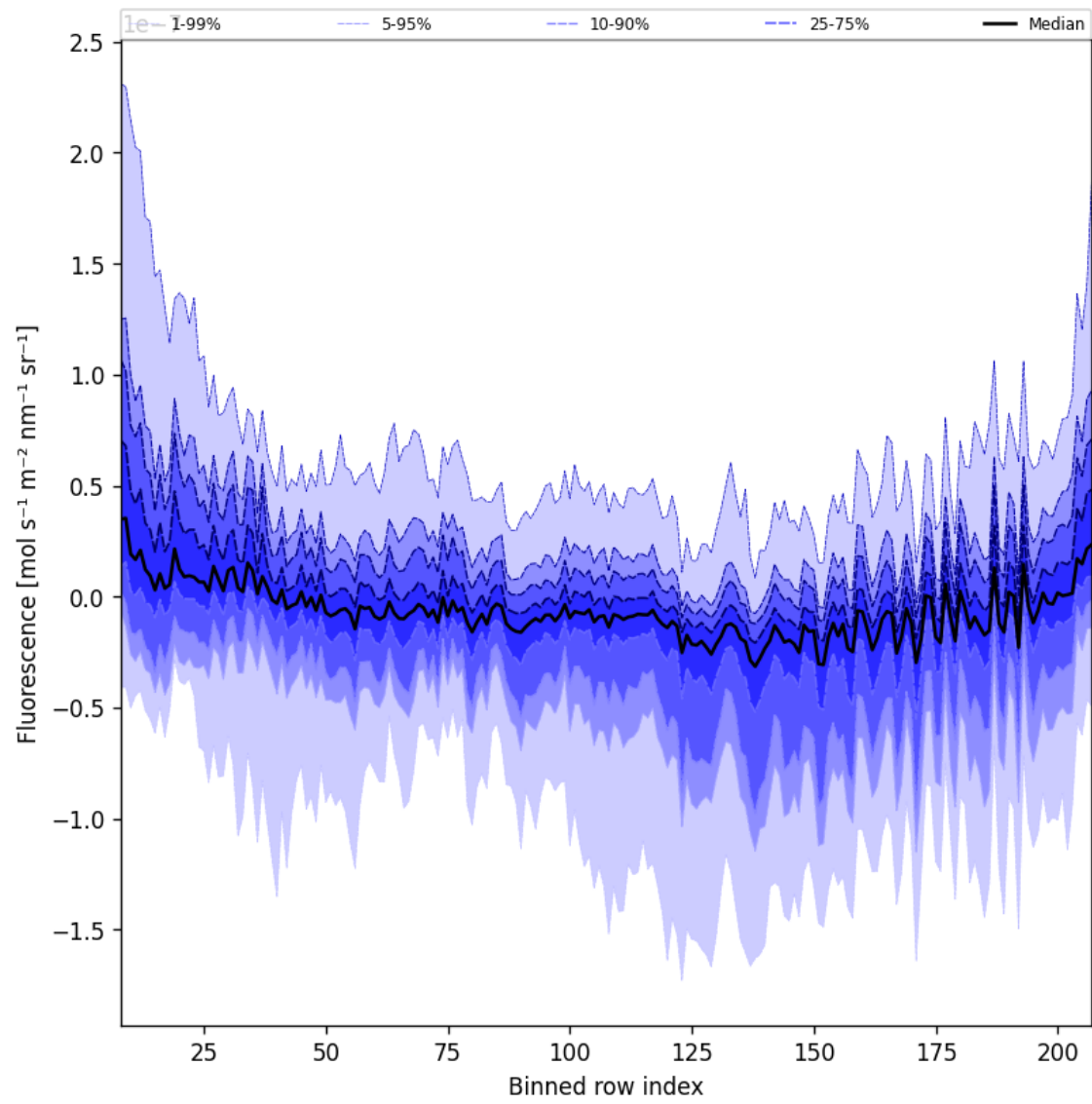
Figure 43: Along track statistics of “Fluorescence” for 2024-09-19 to 2024-09-21
