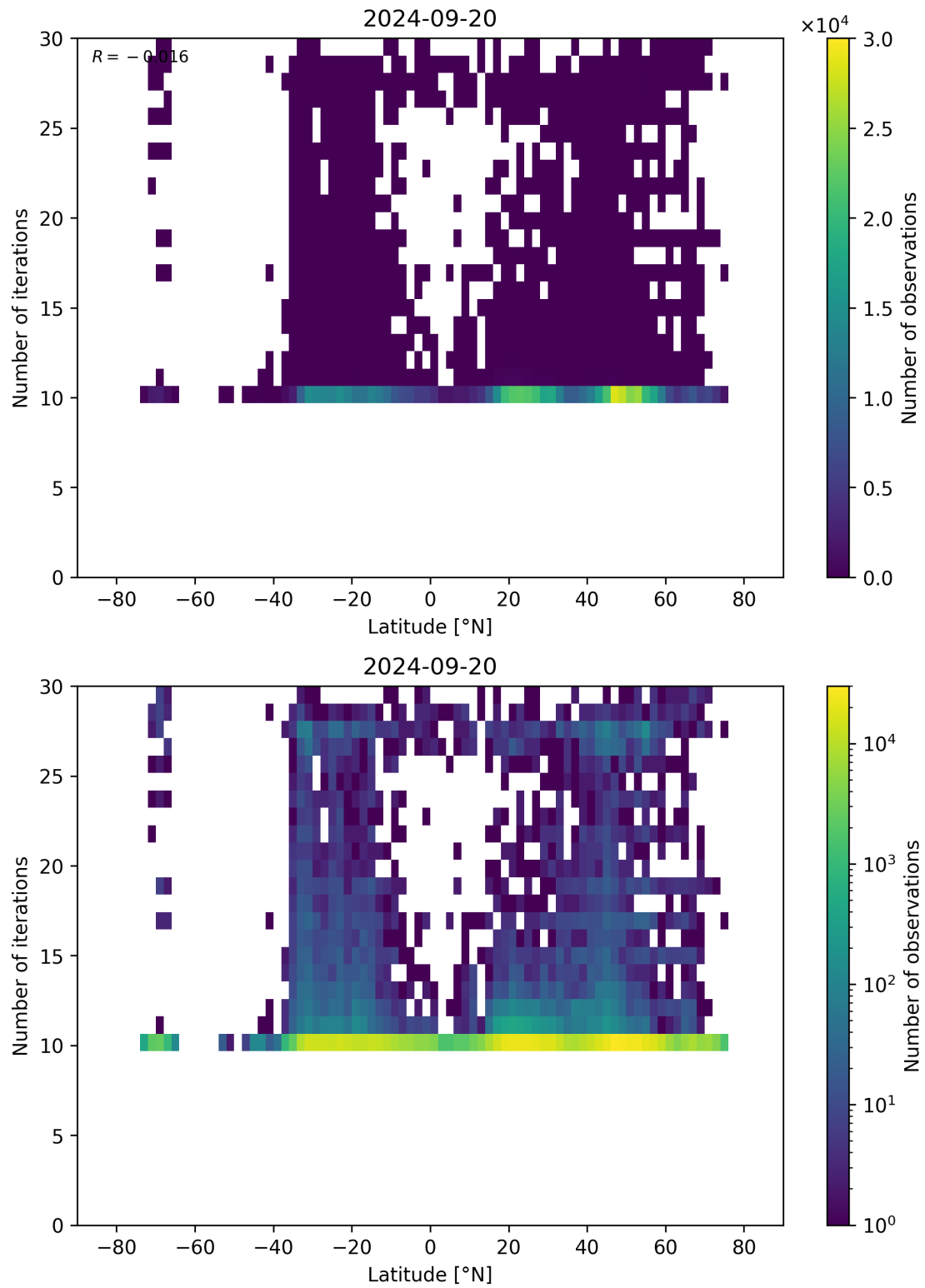
Figure 60: Scatter density plot of “Latitude” against “Number of iterations” for 2024-09-19 to 2024-09-21.
