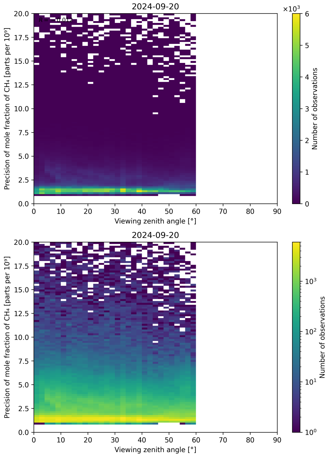
Figure 112: Scatter density plot of “Viewing zenith angle” against “Precision of mole fraction of CH 4 ” for 2024-09-19 to 2024-09-21.
