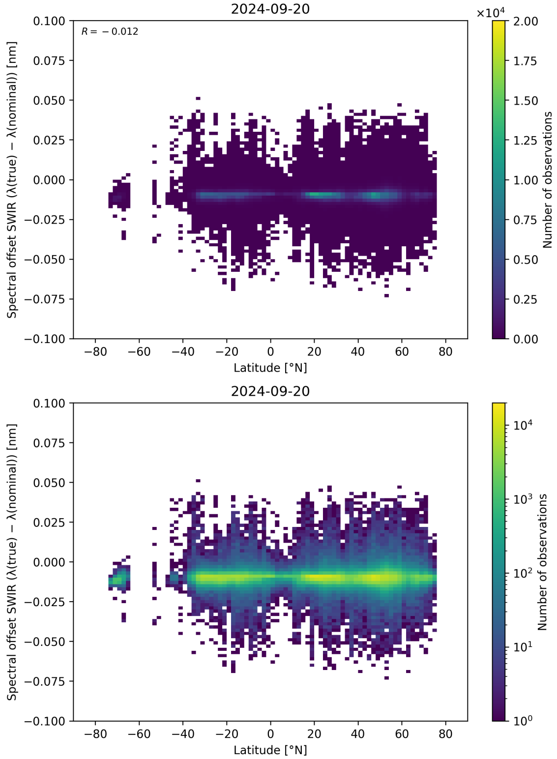
Figure 62: Scatter density plot of “Latitude” against “Spectral offset SWIR ( \lambda_{\text{true}} - \lambda_{\text{nominal}} )” for 2024-09-19 to 2024-09-21.
