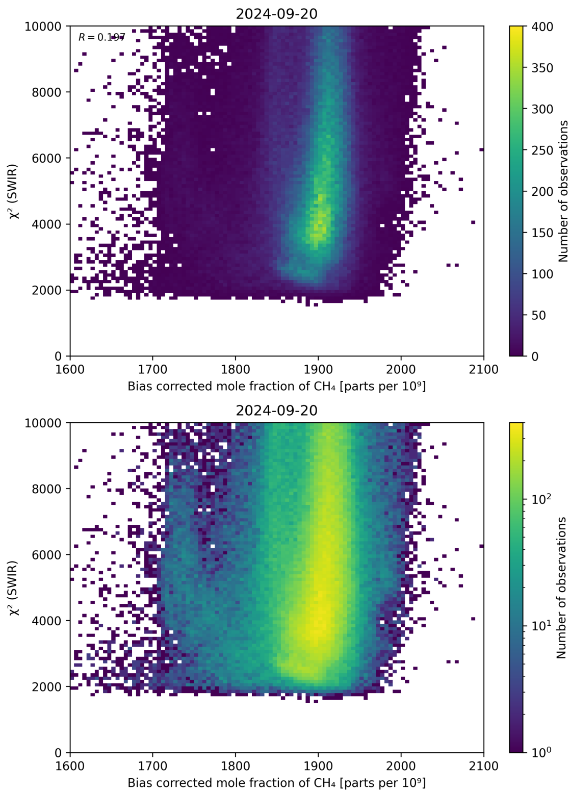
Figure 64: Scatter density plot of “Bias corrected mole fraction of \text{CH}_4 ” against “ \chi^2 (SWIR)” for 2024-09-19 to 2024-09-21.
