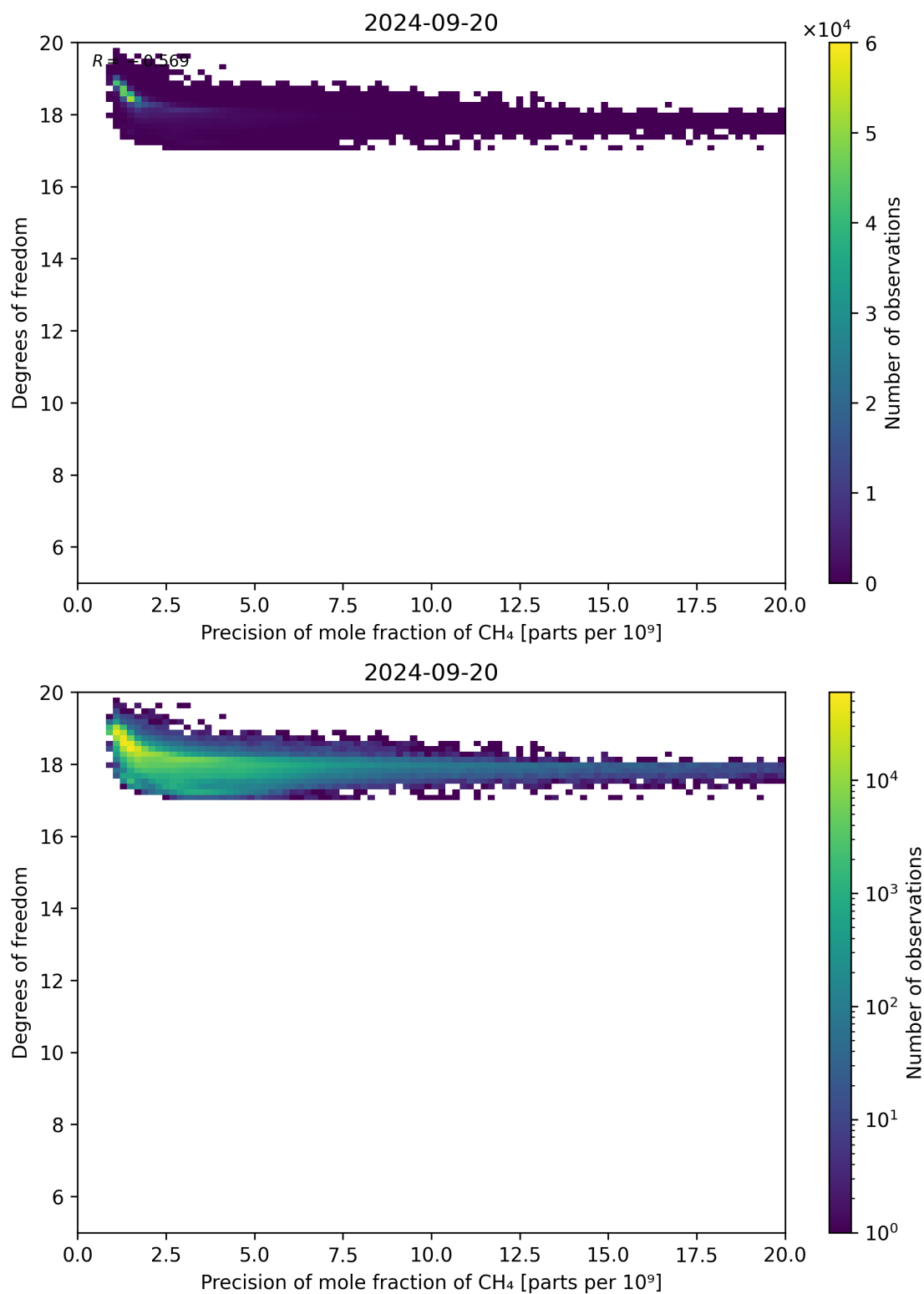
Figure 80: Scatter density plot of “Precision of mole fraction of CH 4 ” against “Degrees of freedom” for 2024-09-19 to 2024-09-21.
