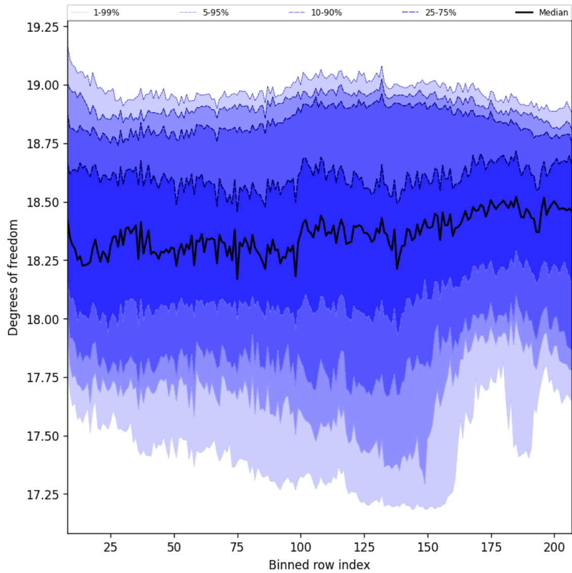
Figure 41: Along track statistics of “Degrees of freedom” for 2024-09-19 to 2024-09-21
