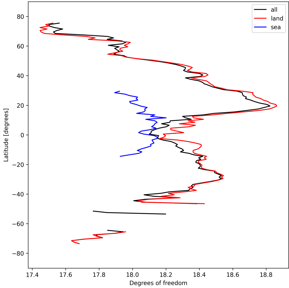
Figure 19: Zonal average of “Degrees of freedom” for 2024-09-19 to 2024-09-21.
