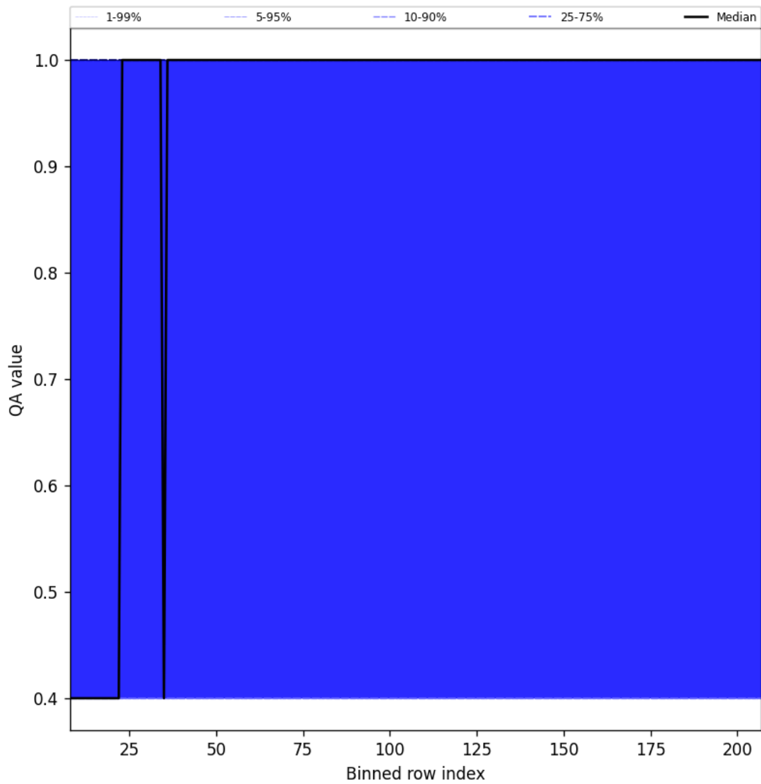
Figure 33: Along track statistics of “QA value” for 2024-09-19 to 2024-09-21
