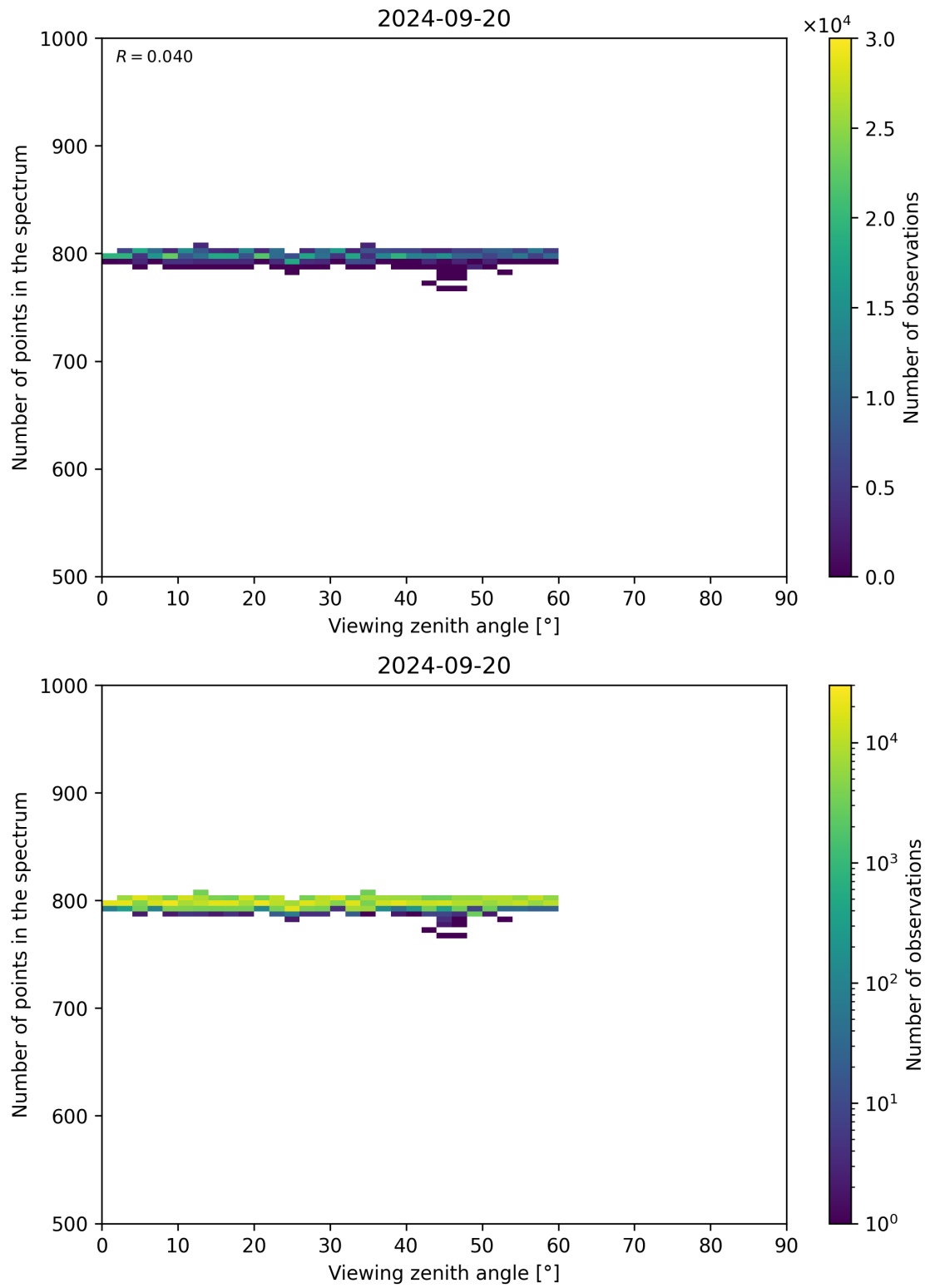
Figure 114: Scatter density plot of “Viewing zenith angle” against “Number of points in the spectrum” for 2024-09-19 to 2024-09-21.
