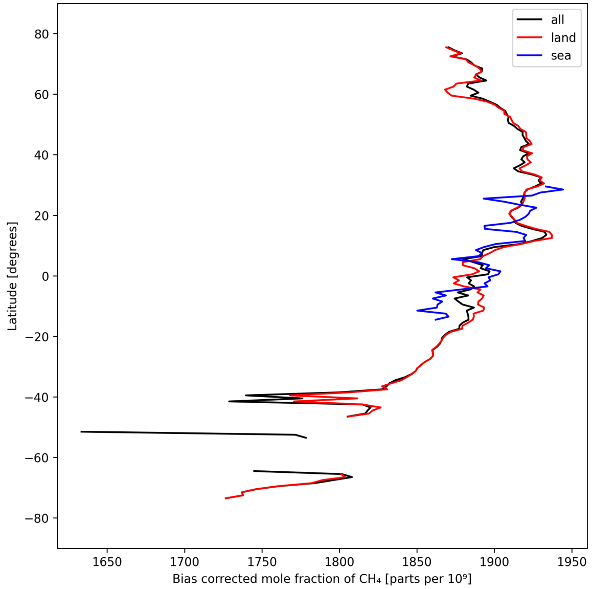
Figure 14: Zonal average of “Bias corrected mole fraction of CH 4 ” for 2024-09-19 to 2024-09-21.
