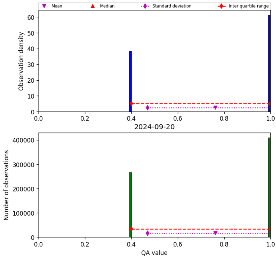
Figure 22: Histogram of “QA value” for 2024-09-19 to 2024-09-21
