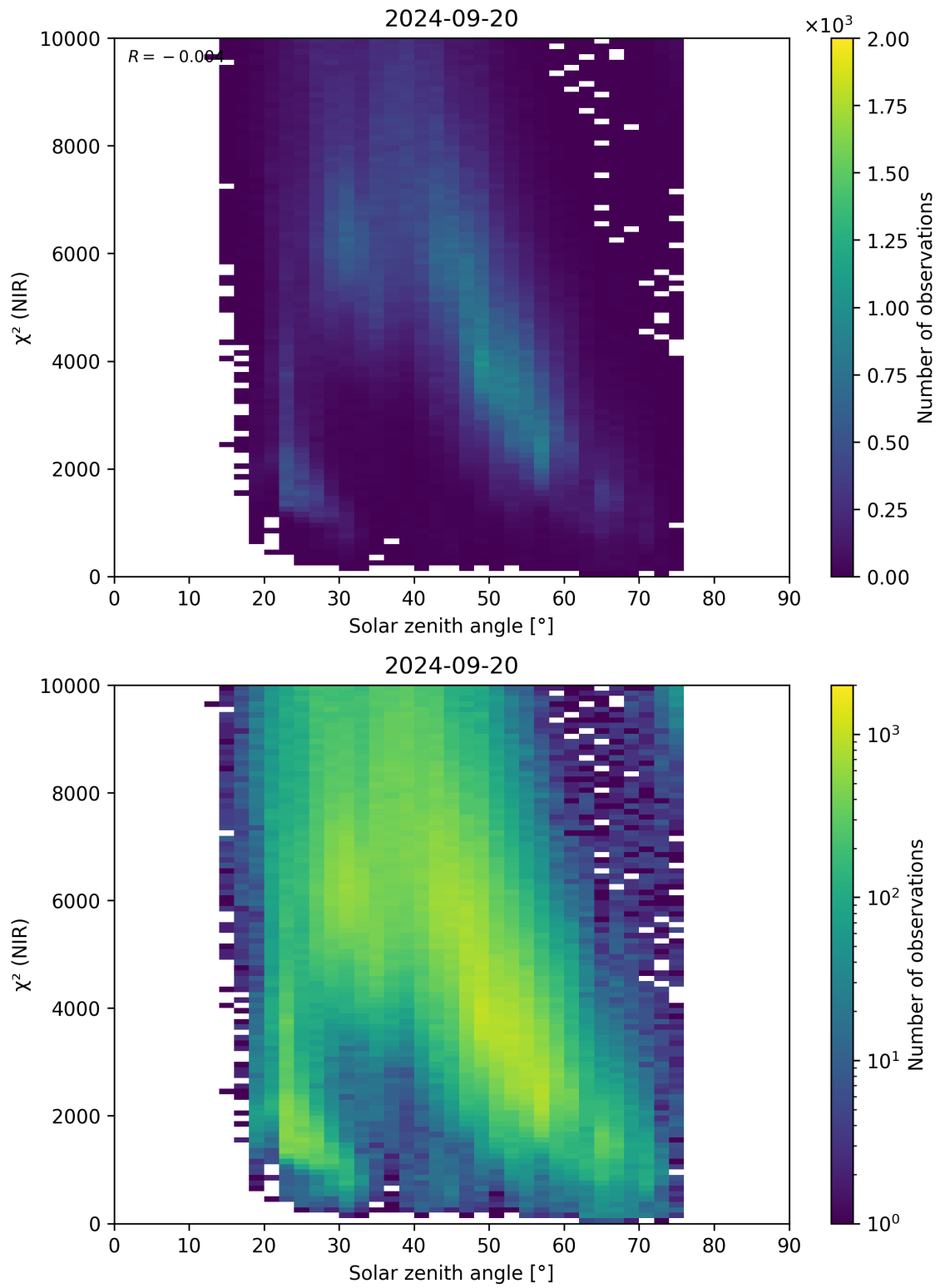
Figure 94: Scatter density plot of “Solar zenith angle” against “ \chi^2 (NIR)” for 2024-09-19 to 2024-09-21.
