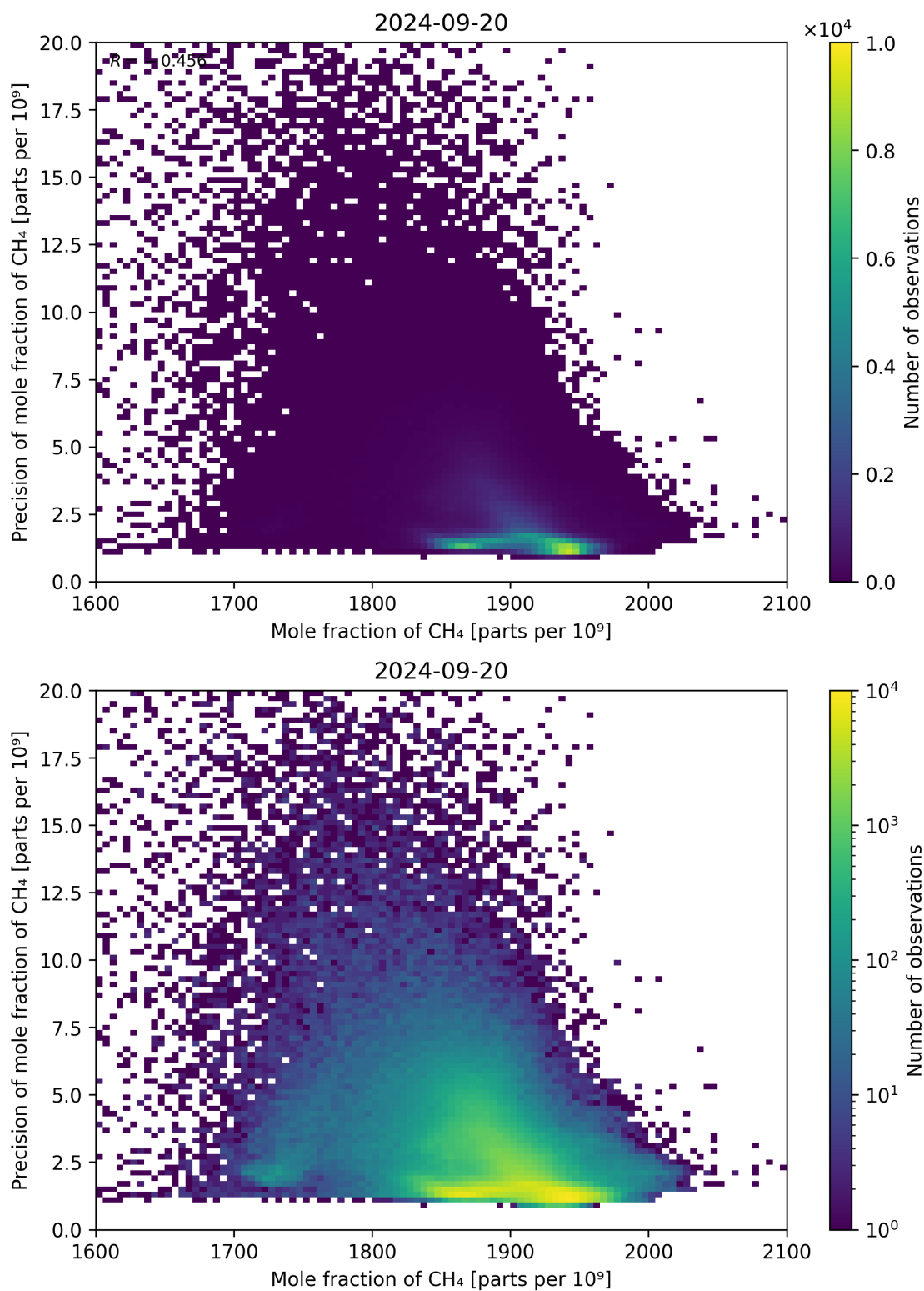
Figure 75: Scatter density plot of “Mole fraction of CH 4 ” against “Precision of mole fraction of CH 4 ” for 2024-09-19 to 2024-09-21.
