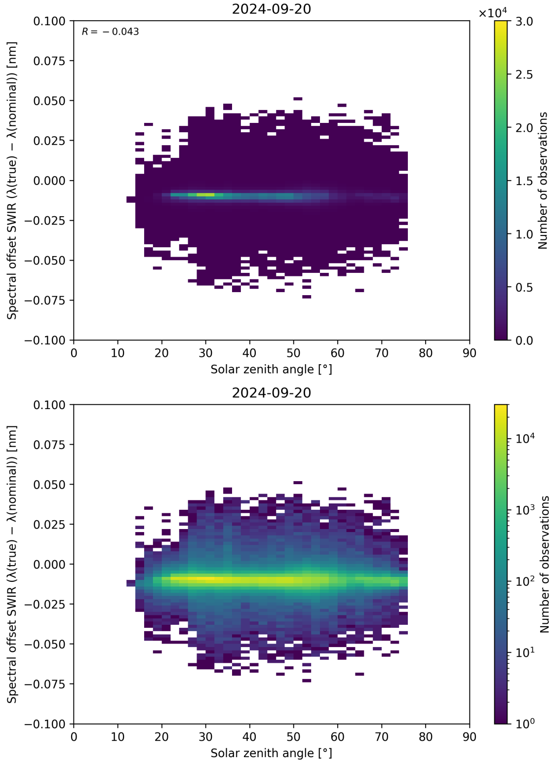
Figure 104: Scatter density plot of “Solar zenith angle” against “Spectral offset SWIR ( \lambda_{\text{true}} - \lambda_{\text{nominal}} )” for 2024-09-19 to 2024-09-21.
