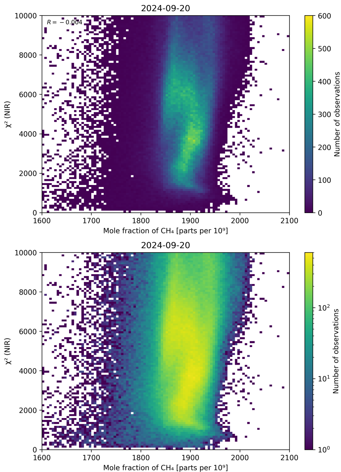
Figure 70: Scatter density plot of “Mole fraction of CH 4 ” against “ \chi^2 (NIR)” for 2024-09-19 to 2024-09-21.
