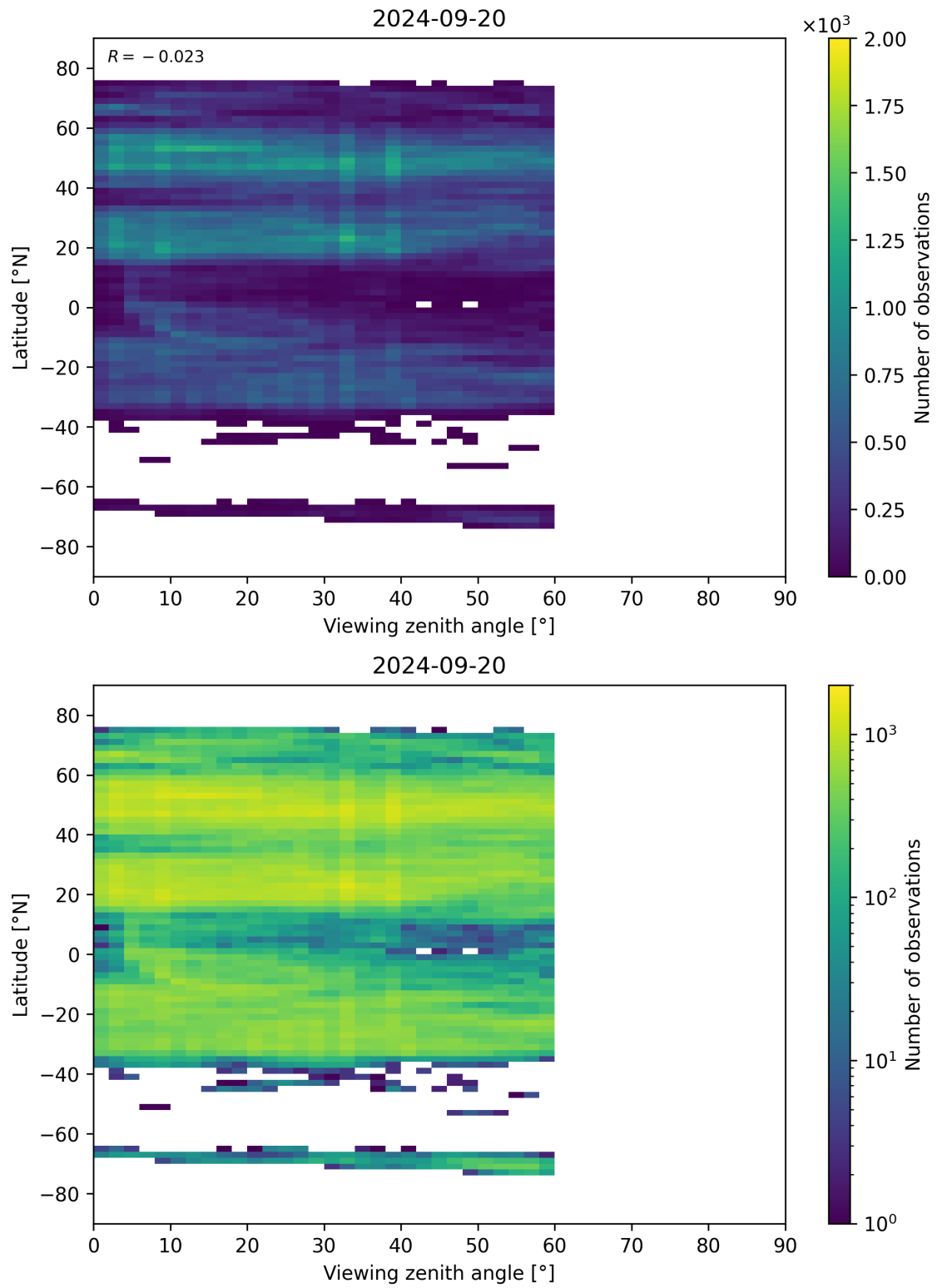
Figure 109: Scatter density plot of “Viewing zenith angle” against “Latitude” for 2024-09-19 to 2024-09-21.
