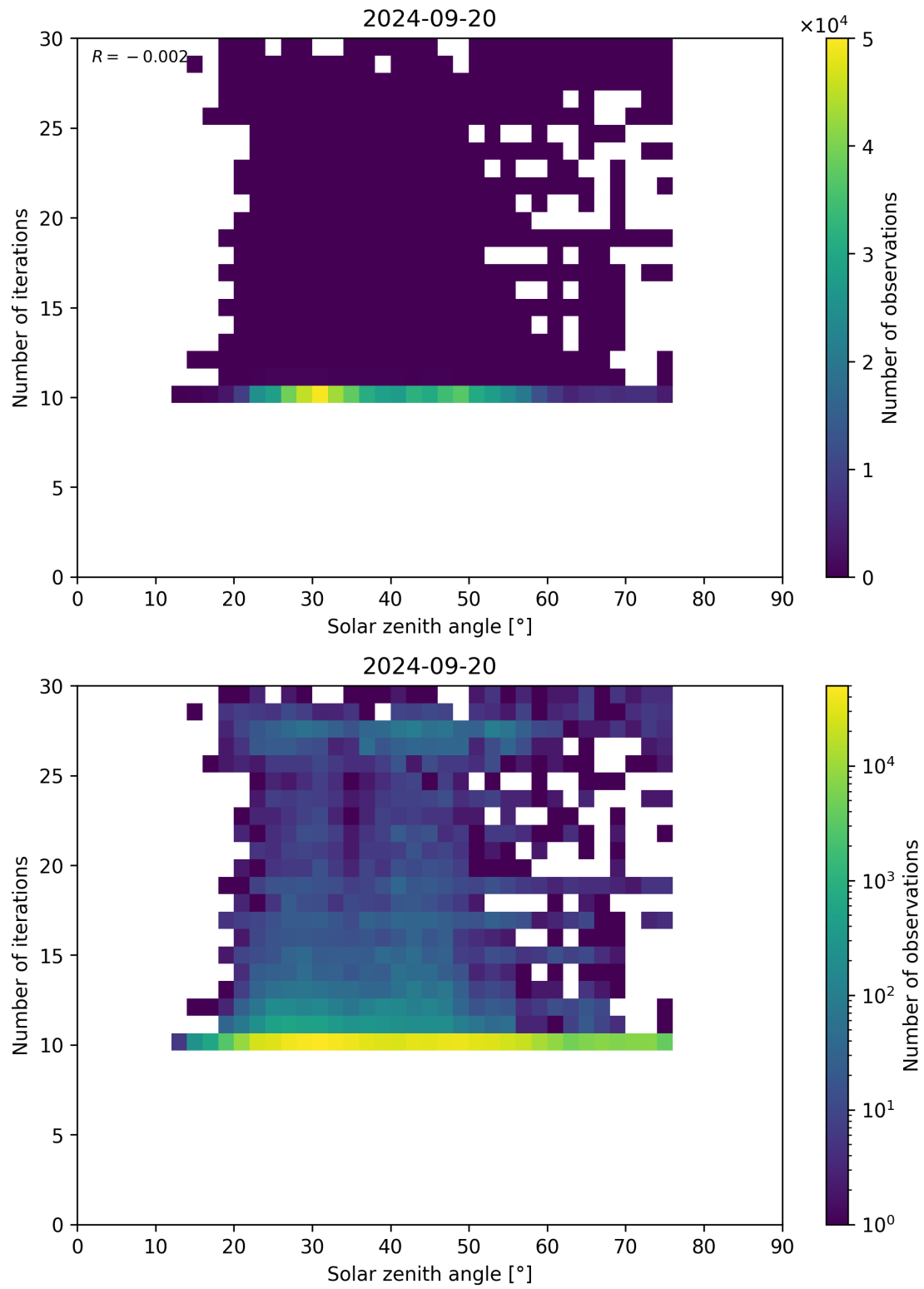
Figure 102: Scatter density plot of “Solar zenith angle” against “Number of iterations” for 2024-09-19 to 2024-09-21.
