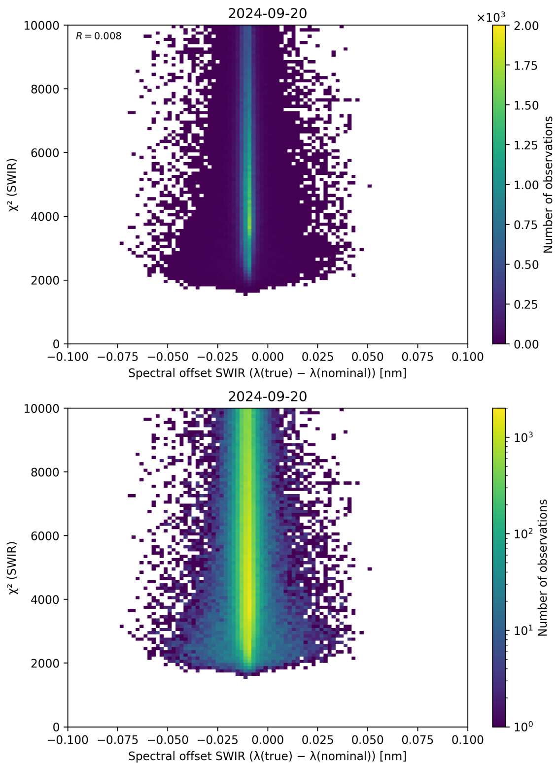
Figure 118: Scatter density plot of “Spectral offset SWIR ( \lambda_{\text{true}} - \lambda_{\text{nominal}} )” against “ \chi^2 (SWIR)” for 2024-09-19 to 2024-09-21.
