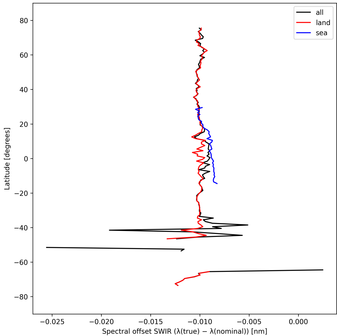
Figure 16: Zonal average of “Spectral offset SWIR ( \lambda_{\text{true}} - \lambda_{\text{nominal}} )” for 2024-09-19 to 2024-09-21.
