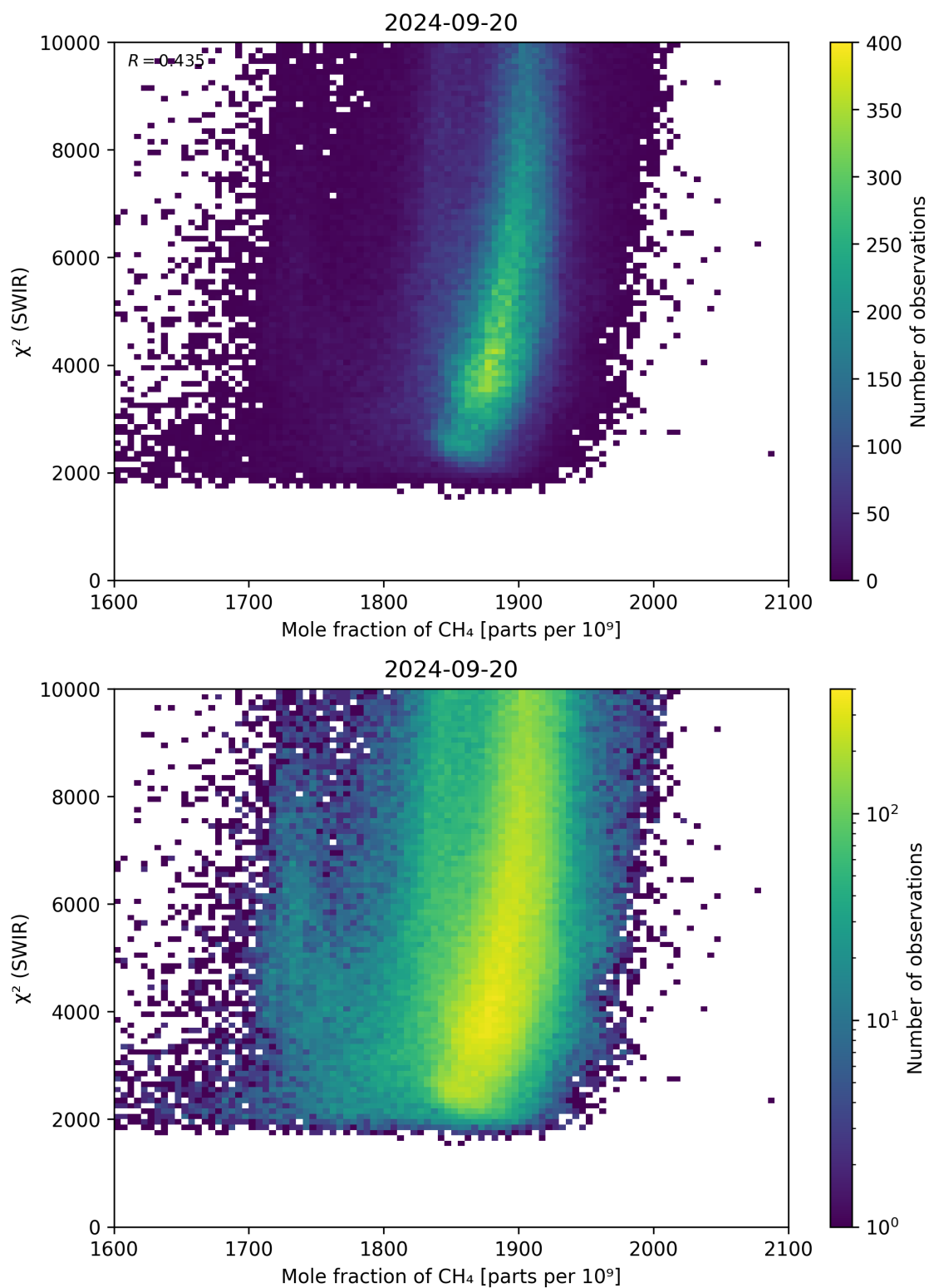
Figure 71: Scatter density plot of “Mole fraction of \text{CH}_4 ” against “ \chi^2 (SWIR)” for 2024-09-19 to 2024-09-21.
