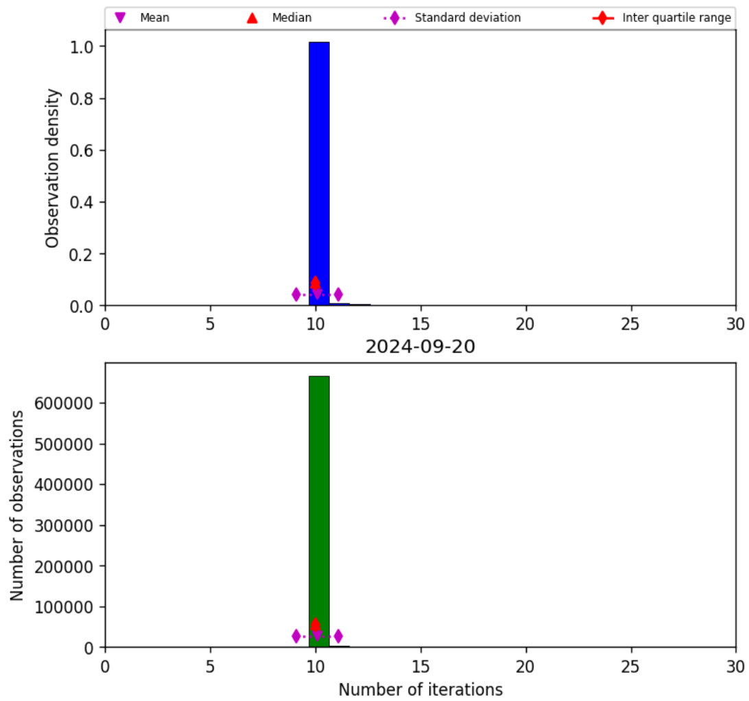
Figure 31: Histogram of “Number of iterations” for 2024-09-19 to 2024-09-21
