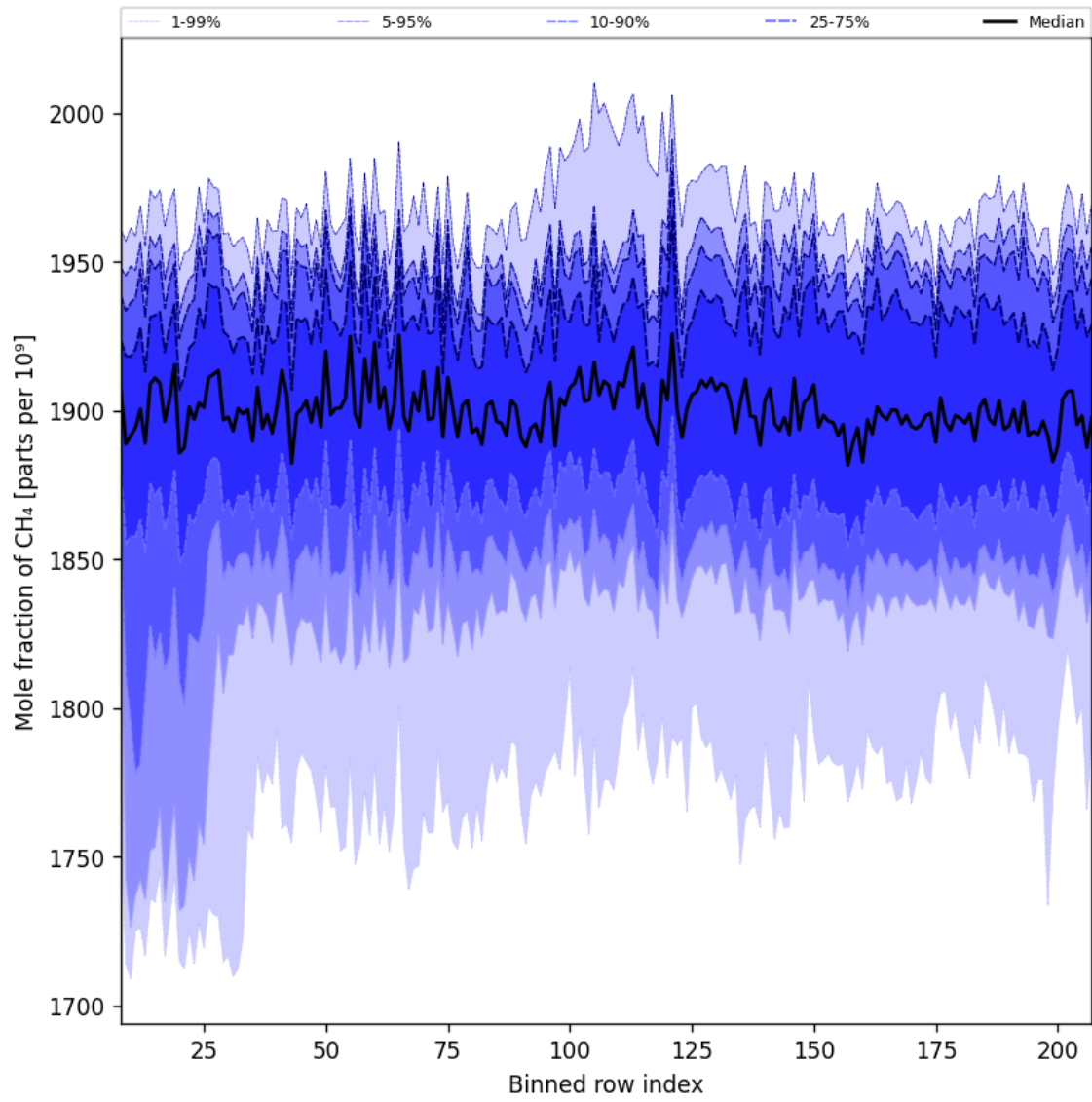
Figure 34: Along track statistics of “Mole fraction of CH 4 ” for 2024-09-19 to 2024-09-21
