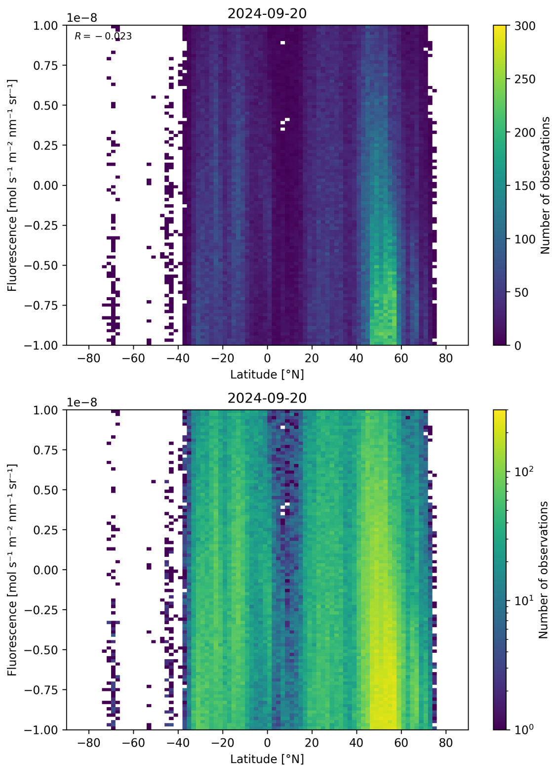
Figure 56: Scatter density plot of “Latitude” against “Fluorescence” for 2024-09-19 to 2024-09-21.
