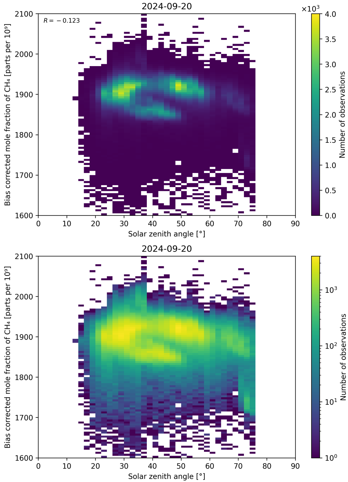
Figure 100: Scatter density plot of “Solar zenith angle” against “Bias corrected mole fraction of \text{CH}_4 ” for 2024-09-19 to 2024-09-21.
