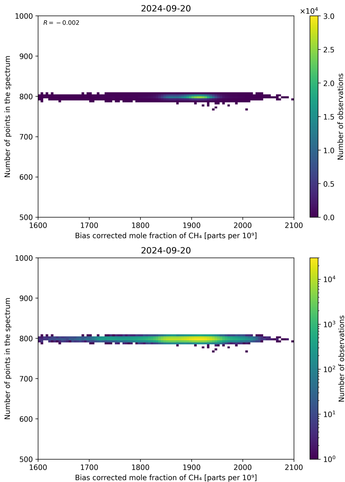
Figure 68: Scatter density plot of “Bias corrected mole fraction of CH 4 ” against “Number of points in the spectrum” for 2024-09-19 to 2024-09-21.
