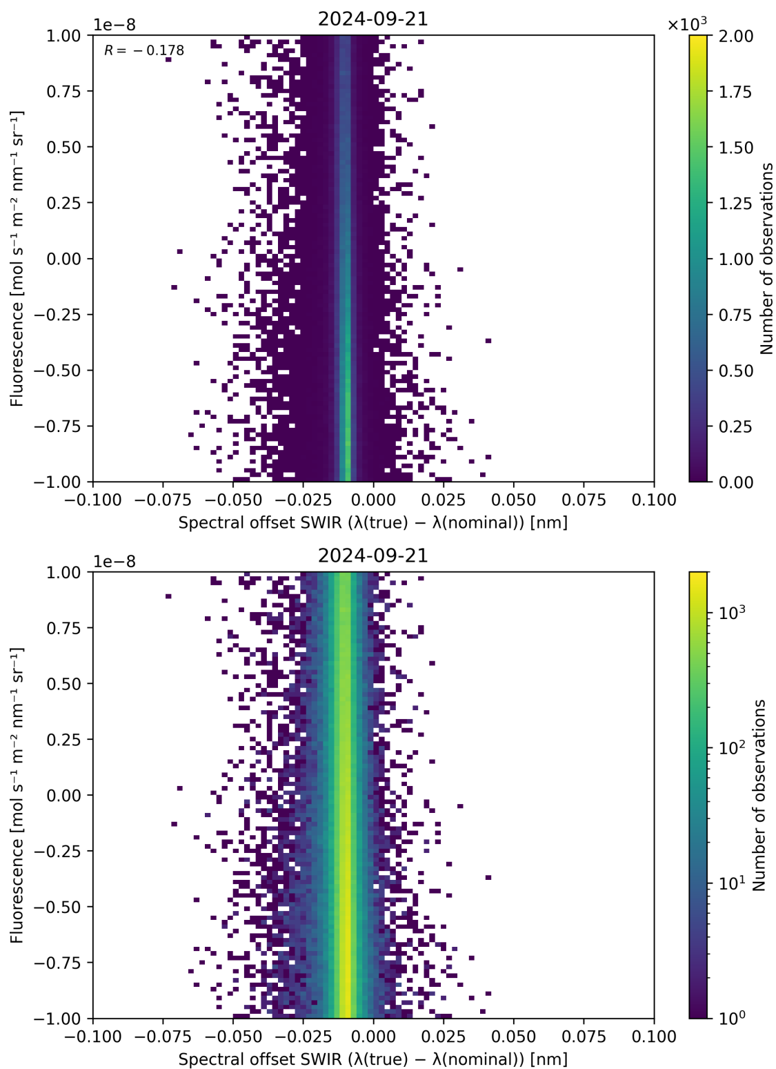
Figure 120: Scatter density plot of “Spectral offset SWIR ( \lambda_{\text{true}} - \lambda_{\text{nominal}} )” against “Fluorescence” for 2024-09-20 to 2024-09-22.
