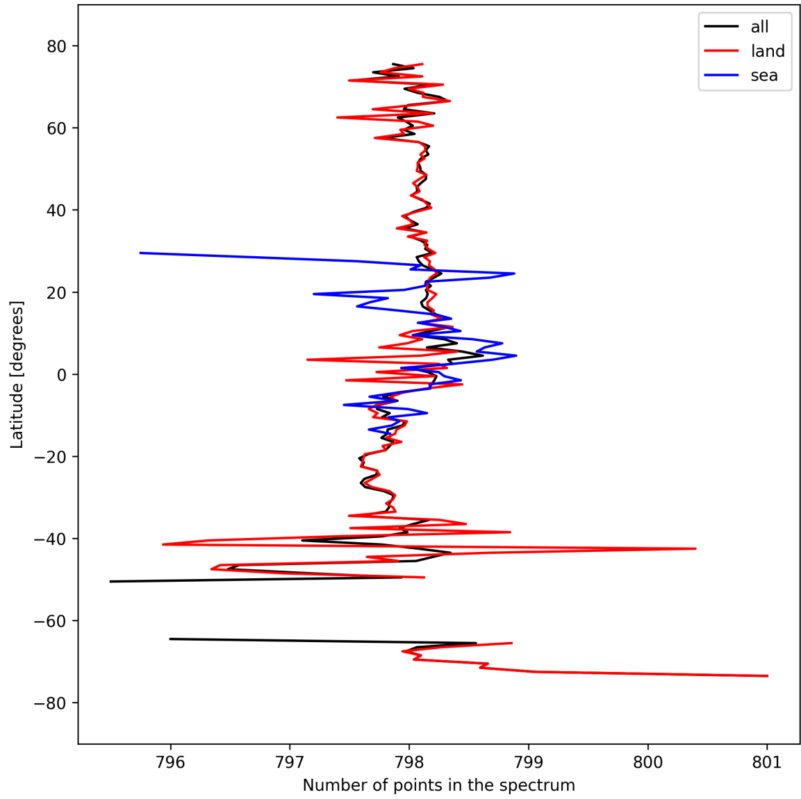
Figure 15: Zonal average of “Number of points in the spectrum” for 2024-09-20 to 2024-09-22.
