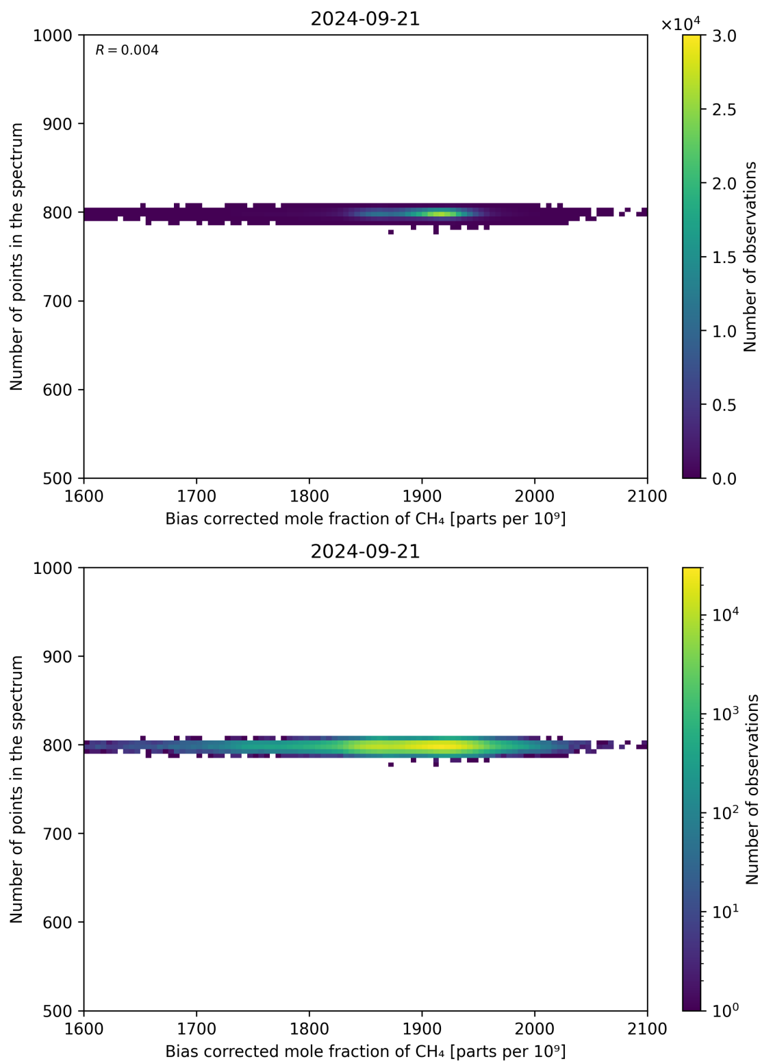
Figure 68: Scatter density plot of “Bias corrected mole fraction of \text{CH}_4 ” against “Number of points in the spectrum” for 2024-09-20 to 2024-09-22.
