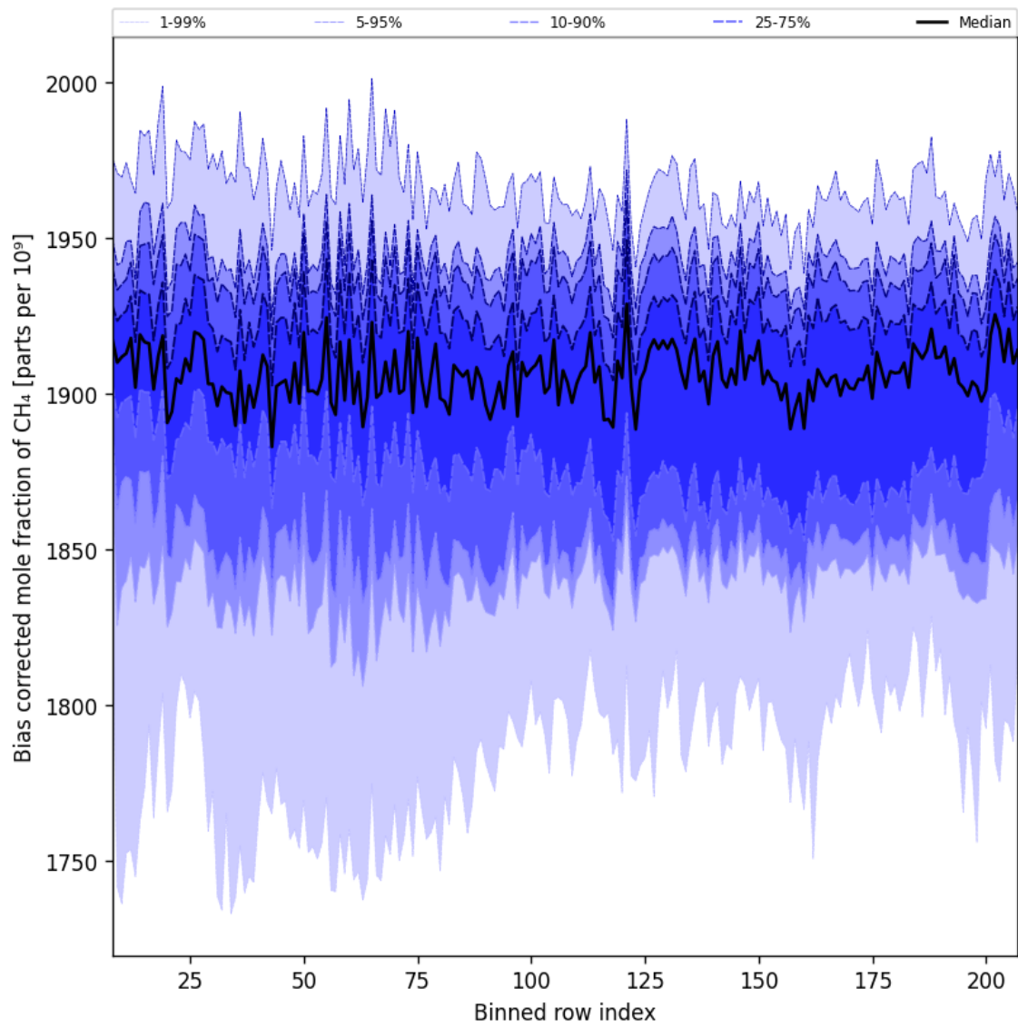
Figure 36: Along track statistics of “Bias corrected mole fraction of CH 4 ” for 2024-09-20 to 2024-09-22
