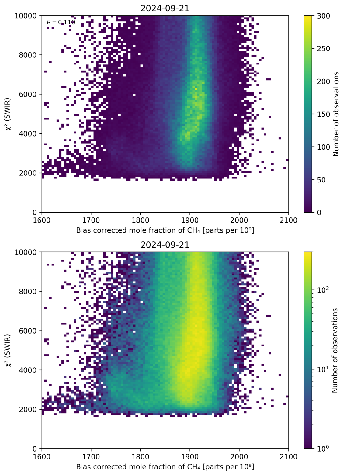
Figure 64: Scatter density plot of “Bias corrected mole fraction of \text{CH}_4 ” against “ \chi^2 (SWIR)” for 2024-09-20 to 2024-09-22.
