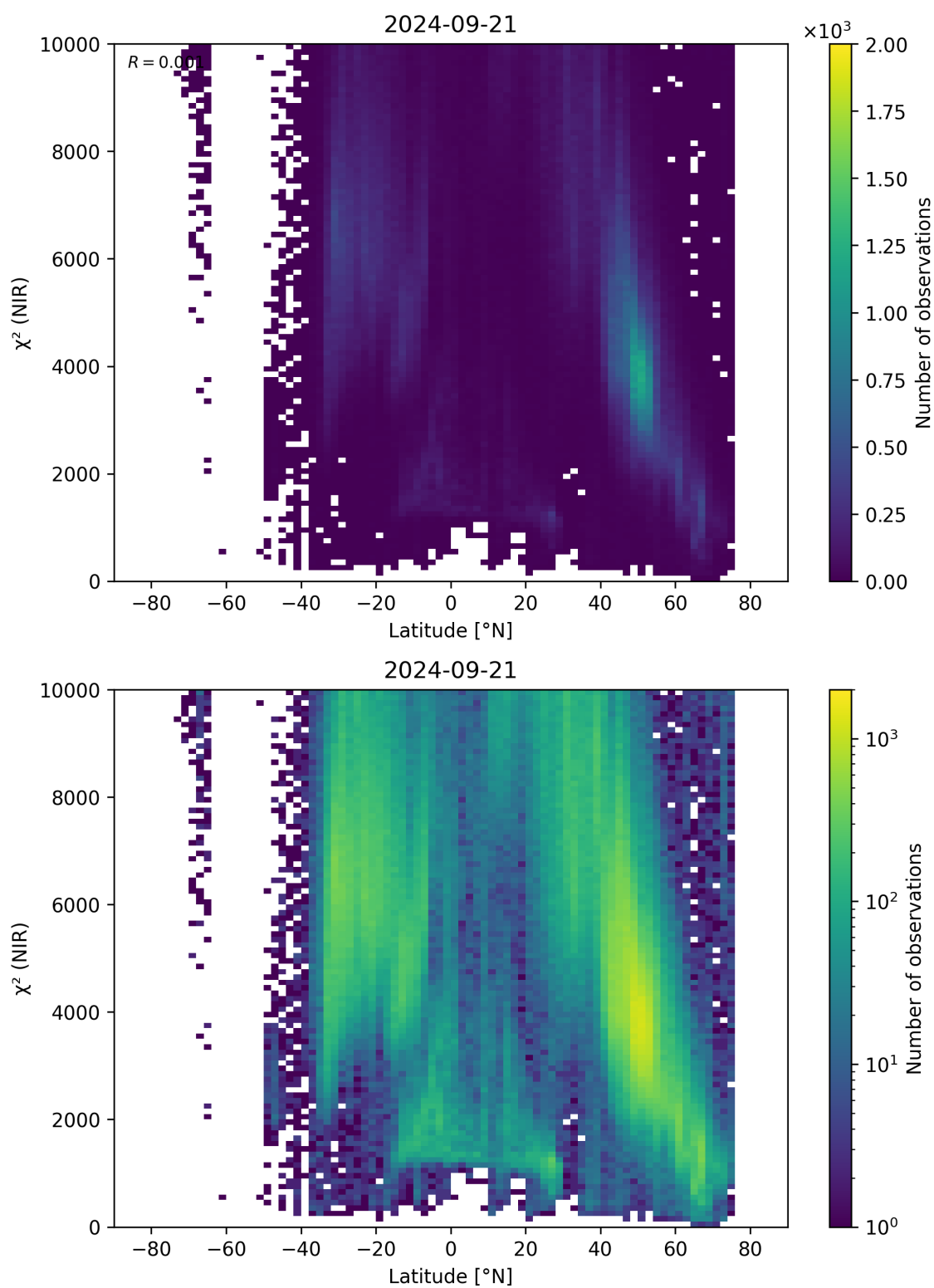
Figure 53: Scatter density plot of “Latitude” against “ \chi^2 (NIR)” for 2024-09-20 to 2024-09-22.
