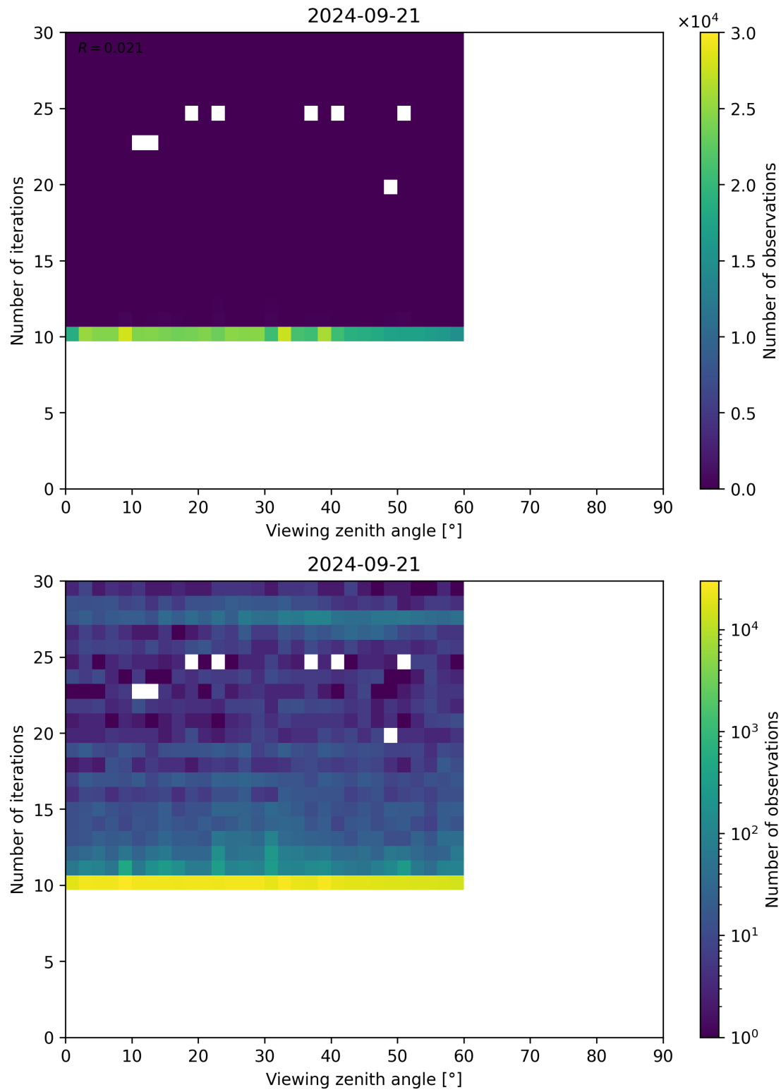
Figure 113: Scatter density plot of “Viewing zenith angle” against “Number of iterations” for 2024-09-20 to 2024-09-22.
