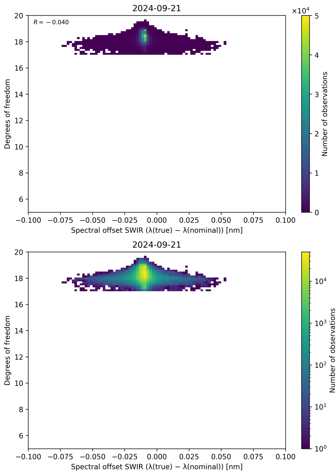
Figure 119: Scatter density plot of “Spectral offset SWIR ( \lambda_{\text{true}} - \lambda_{\text{nominal}} )” against “Degrees of freedom” for 2024-09-20 to 2024-09-22.
