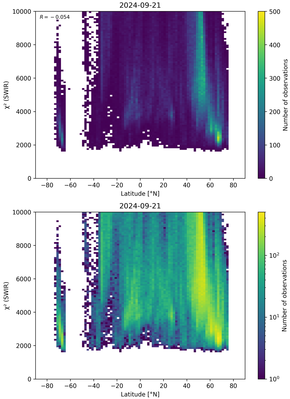
Figure 54: Scatter density plot of “Latitude” against “ \chi^2 (SWIR)” for 2024-09-20 to 2024-09-22.
