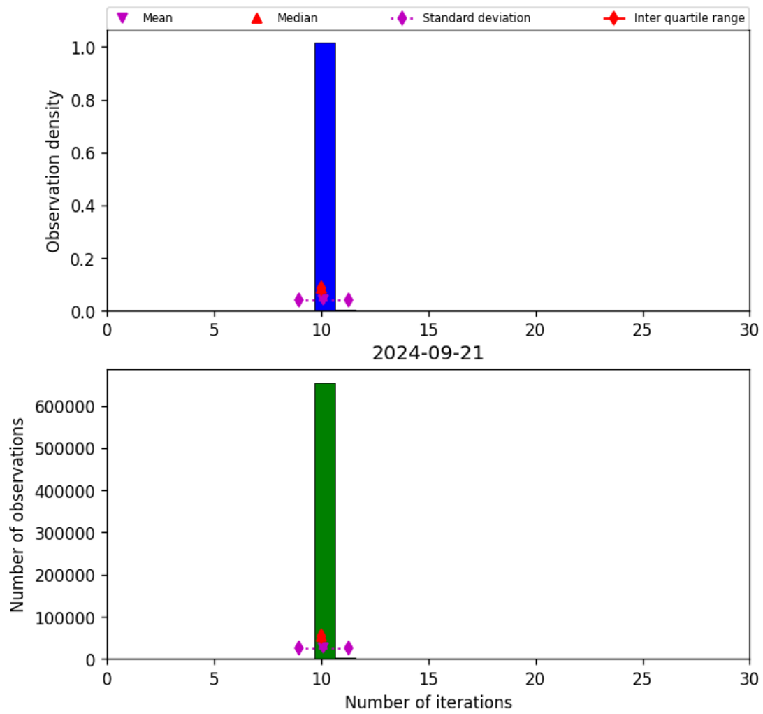
Figure 31: Histogram of “Number of iterations” for 2024-09-20 to 2024-09-22
