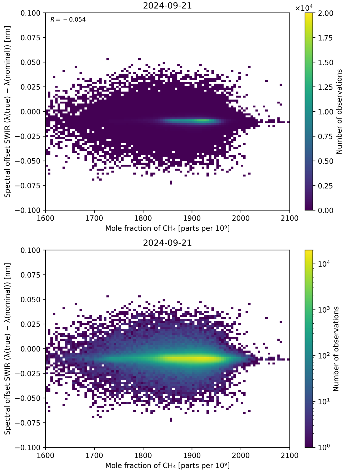
Figure 86: Scatter density plot of “Mole fraction of \text{CH}_4 ” against “Spectral offset SWIR ( \lambda_{\text{true}} - \lambda_{\text{nominal}} )” for 2024-09-20 to 2024-09-22.
