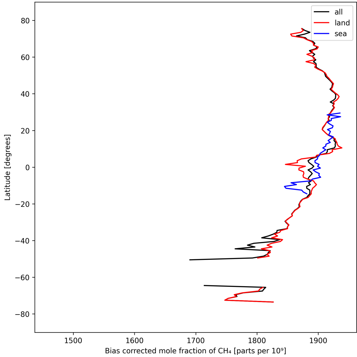
Figure 14: Zonal average of “Bias corrected mole fraction of CH 4 ” for 2024-09-20 to 2024-09-22.
