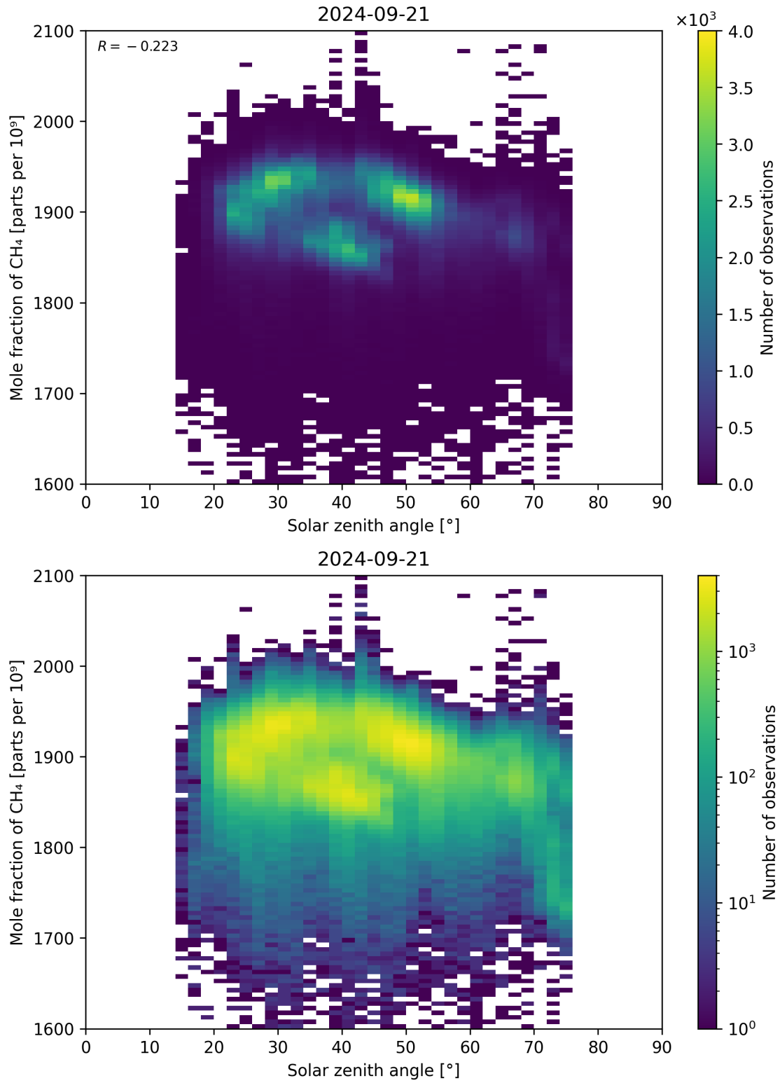
Figure 99: Scatter density plot of “Solar zenith angle” against “Mole fraction of \text{CH}_4 ” for 2024-09-20 to 2024-09-22.
