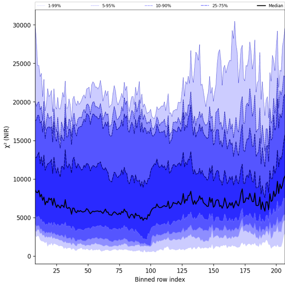
Figure 40: Along track statistics of “ \chi^2 (NIR)” for 2024-09-20 to 2024-09-22
