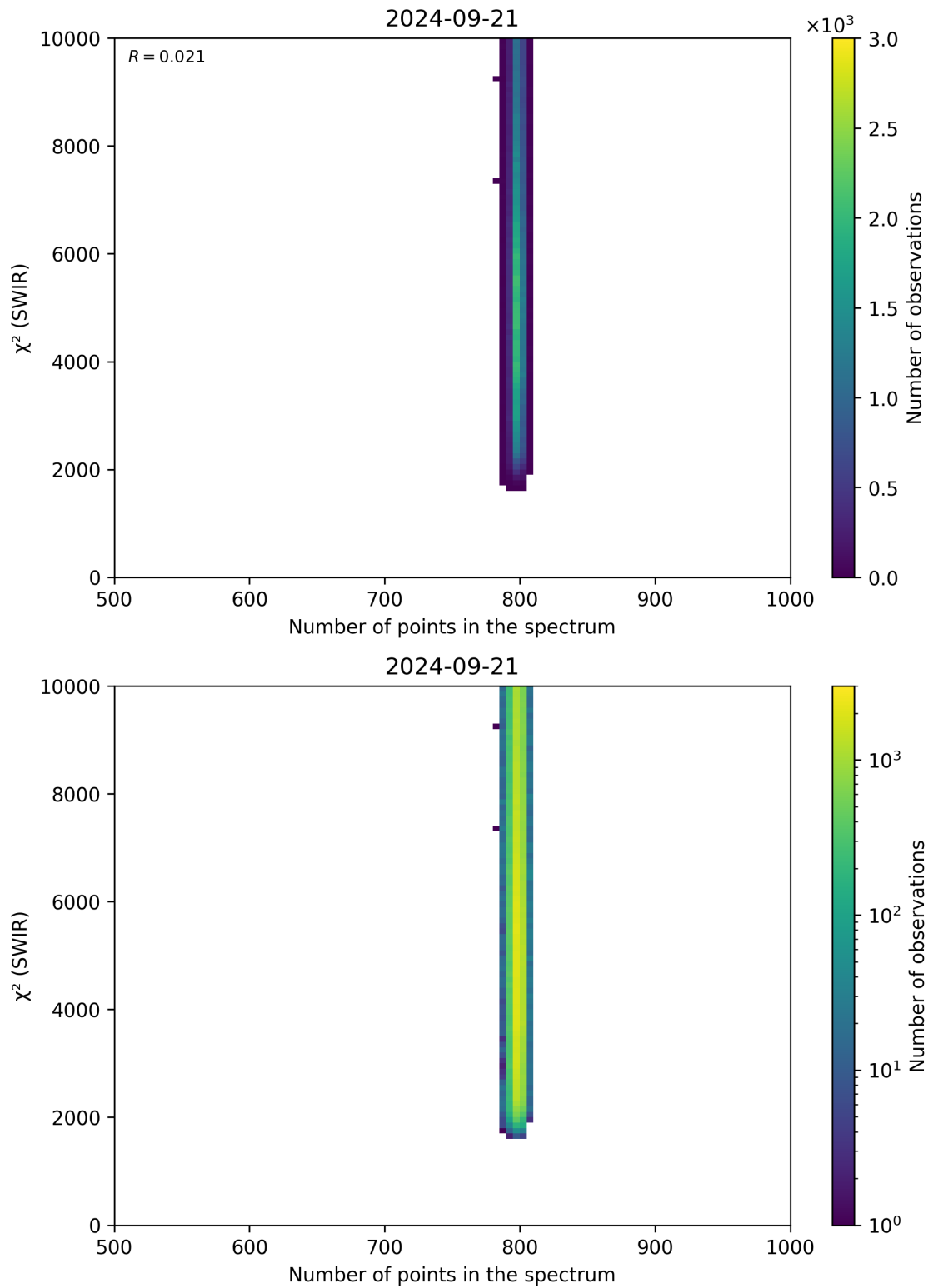
Figure 89: Scatter density plot of “Number of points in the spectrum” against “ \chi^2 (SWIR)” for 2024-09-20 to 2024-09-22.
