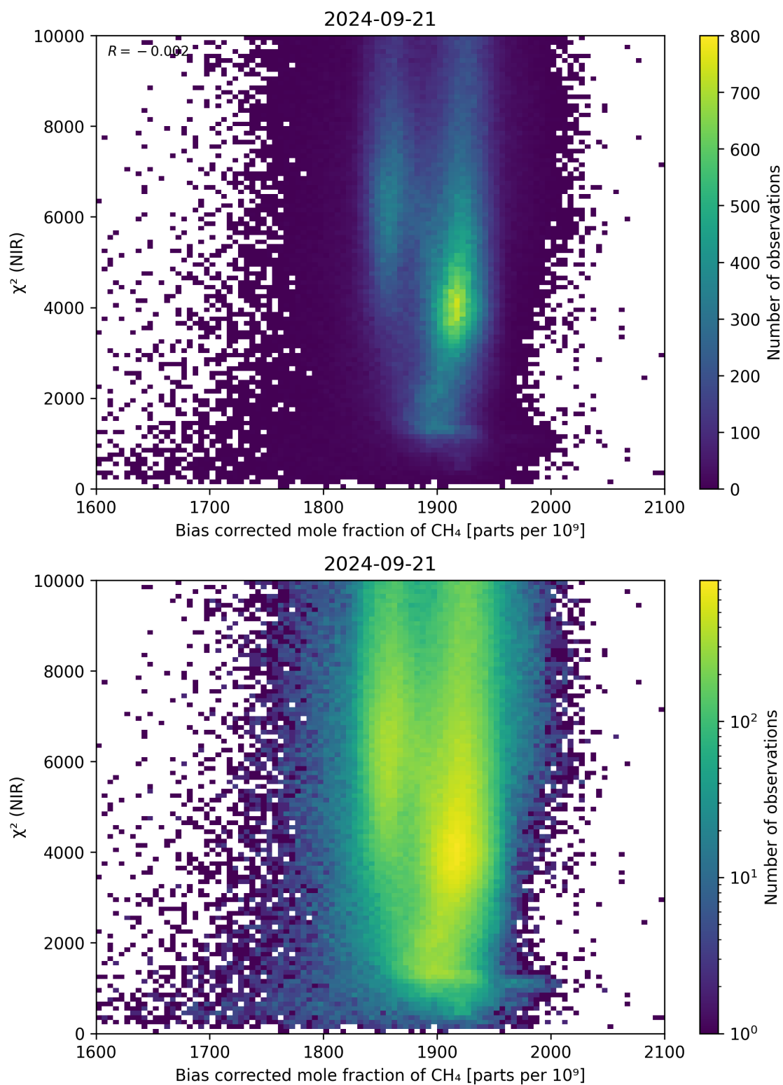
Figure 63: Scatter density plot of “Bias corrected mole fraction of \text{CH}_4 ” against “ \chi^2 (NIR)” for 2024-09-20 to 2024-09-22.
