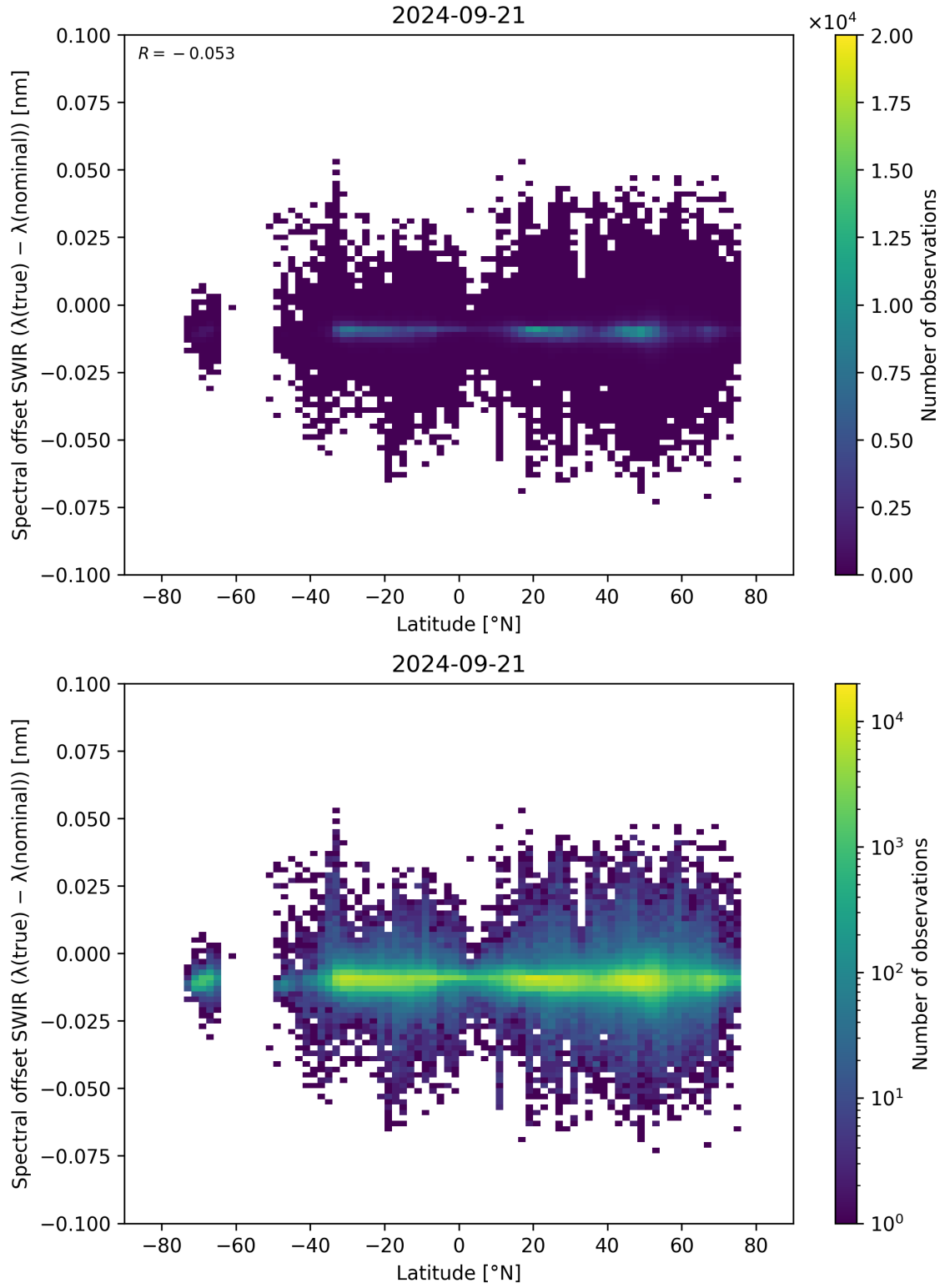
Figure 62: Scatter density plot of “Latitude” against “Spectral offset SWIR ( \lambda_{\text{true}} - \lambda_{\text{nominal}} )” for 2024-09-20 to 2024-09-22.
