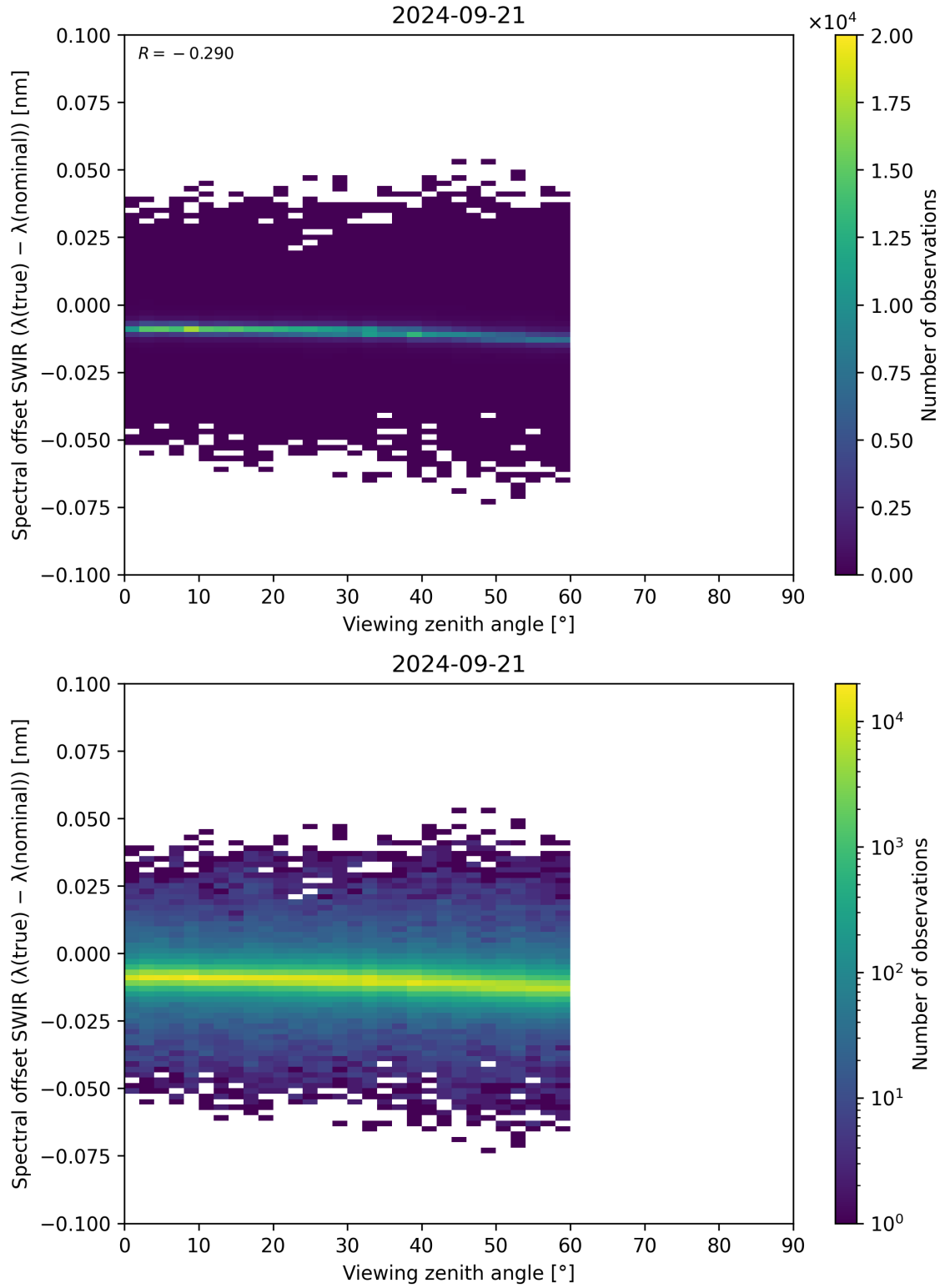
Figure 116: Scatter density plot of “Viewing zenith angle” against “Spectral offset SWIR ( \lambda_{\text{true}} - \lambda_{\text{nominal}} )” for 2024-09-20 to 2024-09-22.
