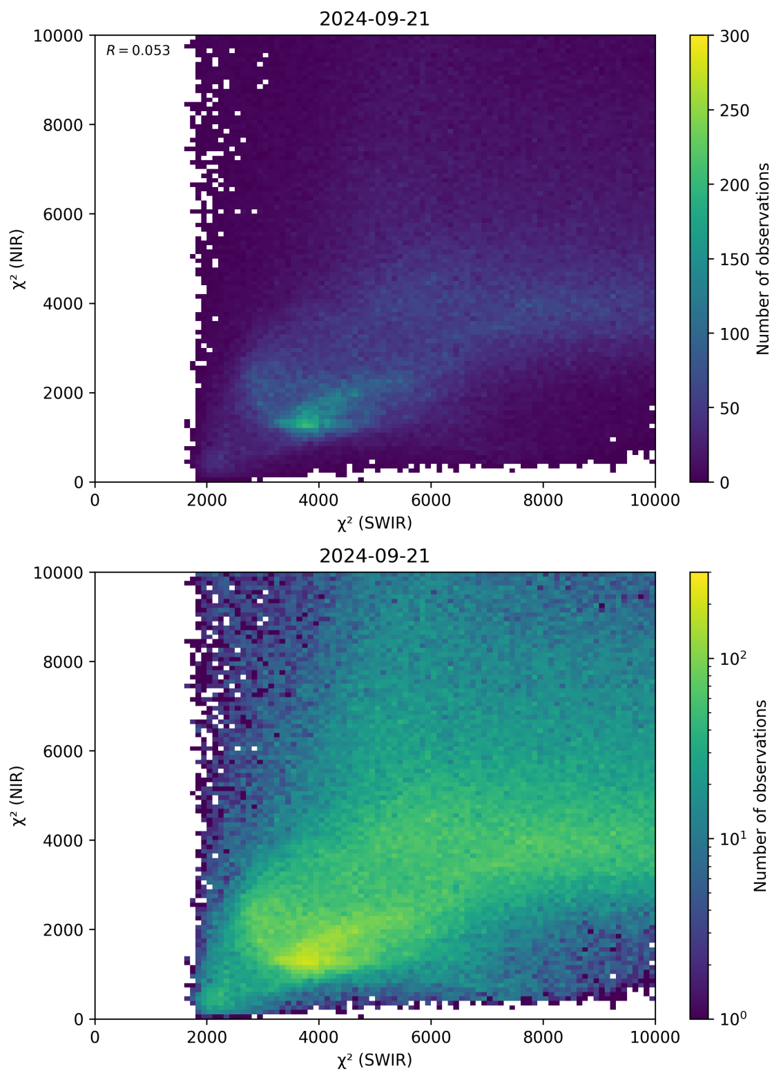
Figure 47: Scatter density plot of “ \chi^2 (SWIR)” against “ \chi^2 (NIR)” for 2024-09-20 to 2024-09-22.
