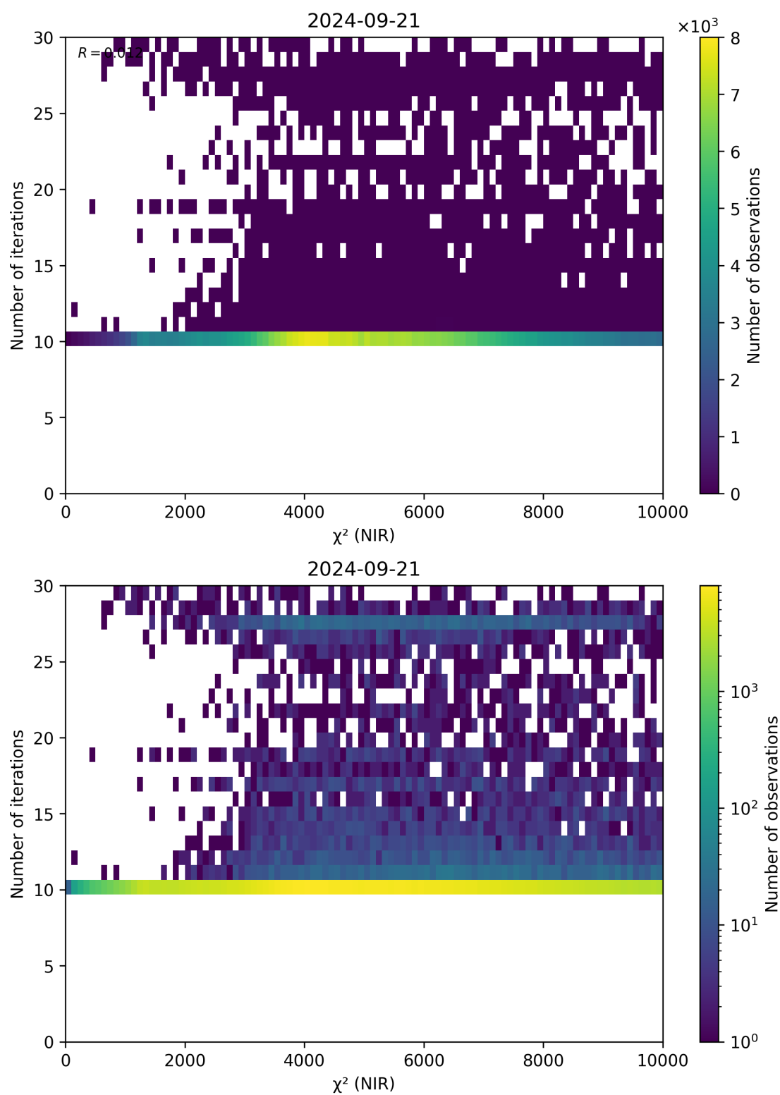
Figure 46: Scatter density plot of “ \chi^2 (NIR)” against “Number of iterations” for 2024-09-20 to 2024-09-22.
