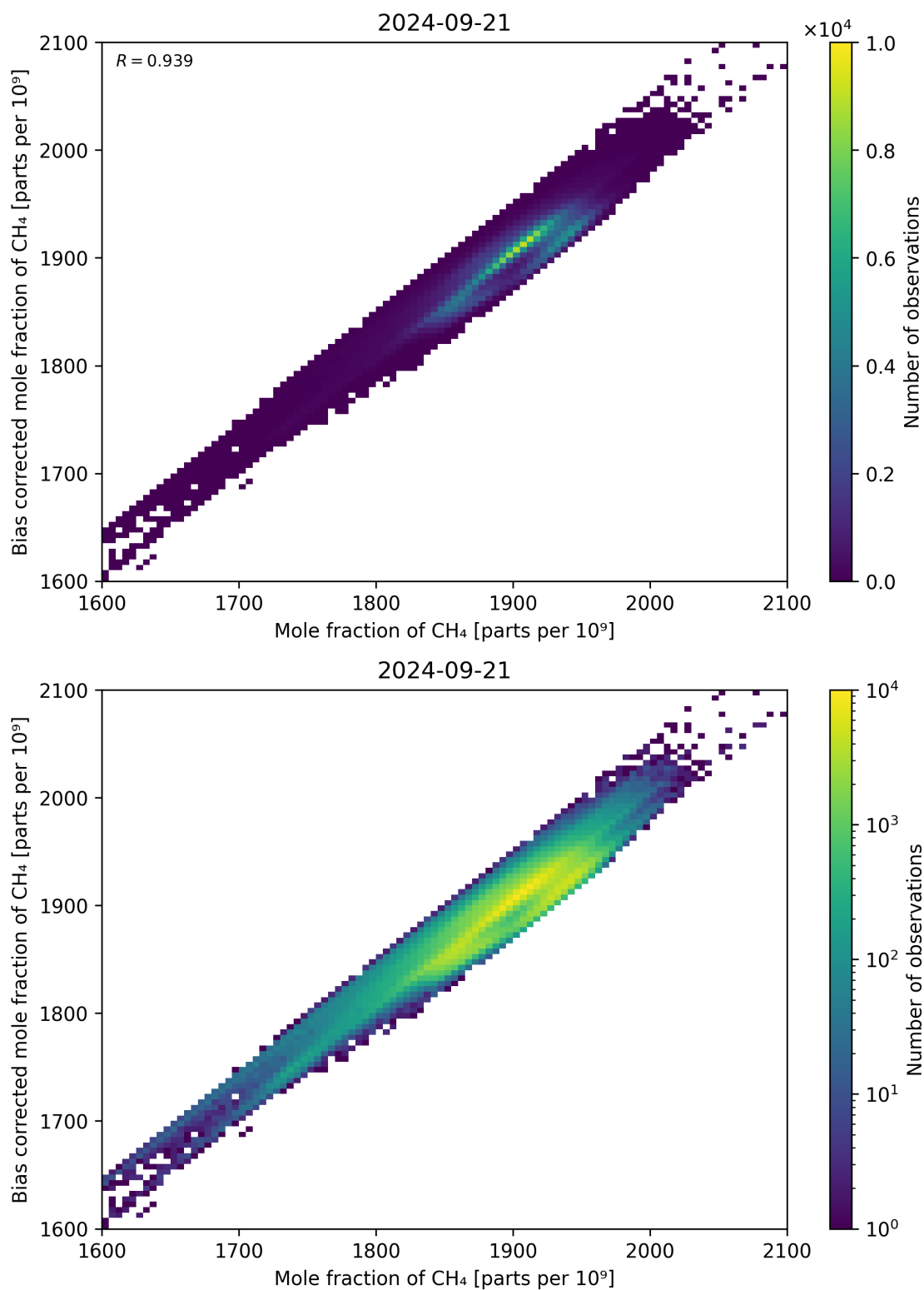
Figure 74: Scatter density plot of “Mole fraction of CH 4 ” against “Bias corrected mole fraction of CH 4 ” for 2024-09-20 to 2024-09-22.
