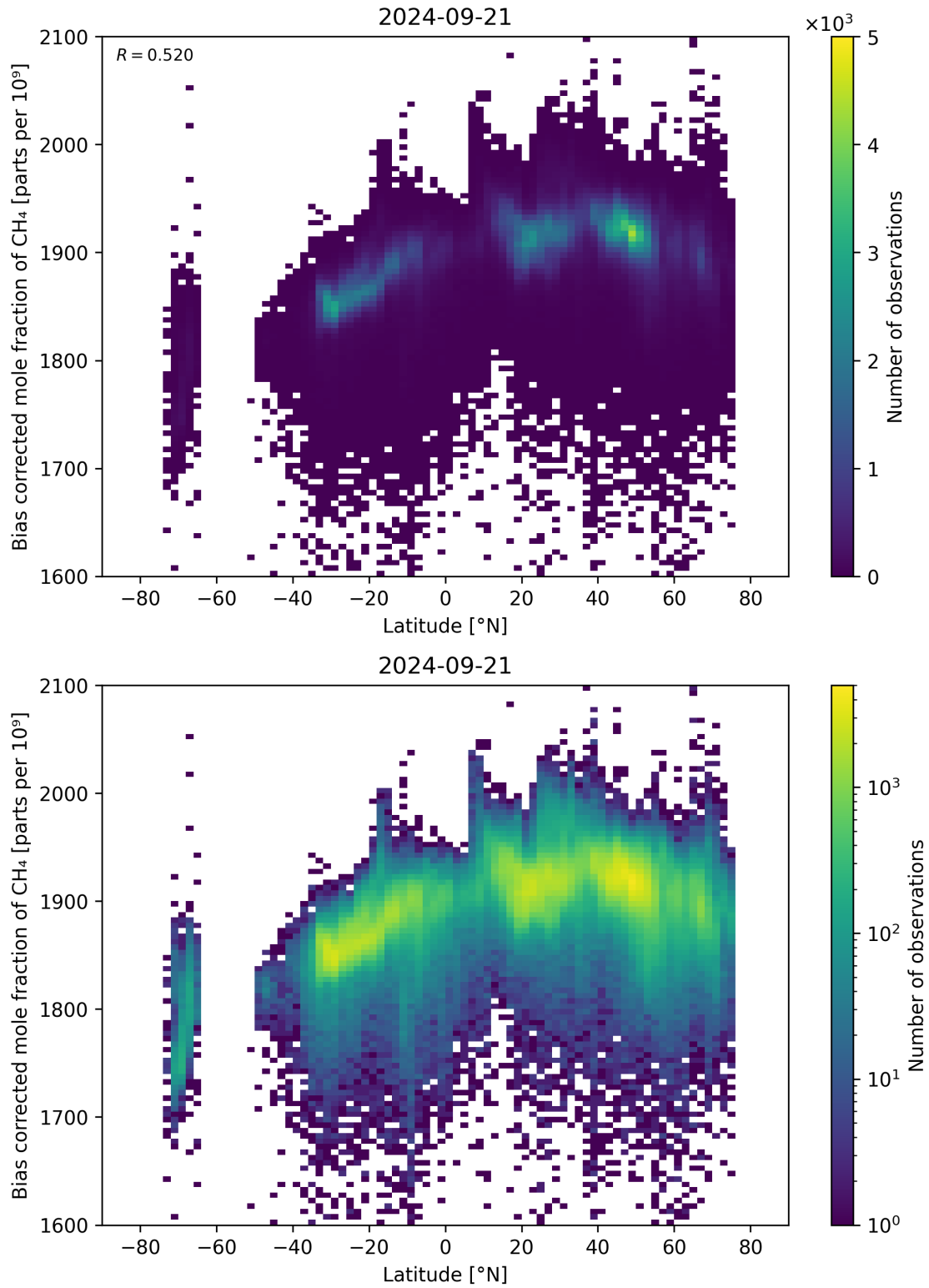
Figure 58: Scatter density plot of “Latitude” against “Bias corrected mole fraction of \text{CH}_4 ” for 2024-09-20 to 2024-09-22.
