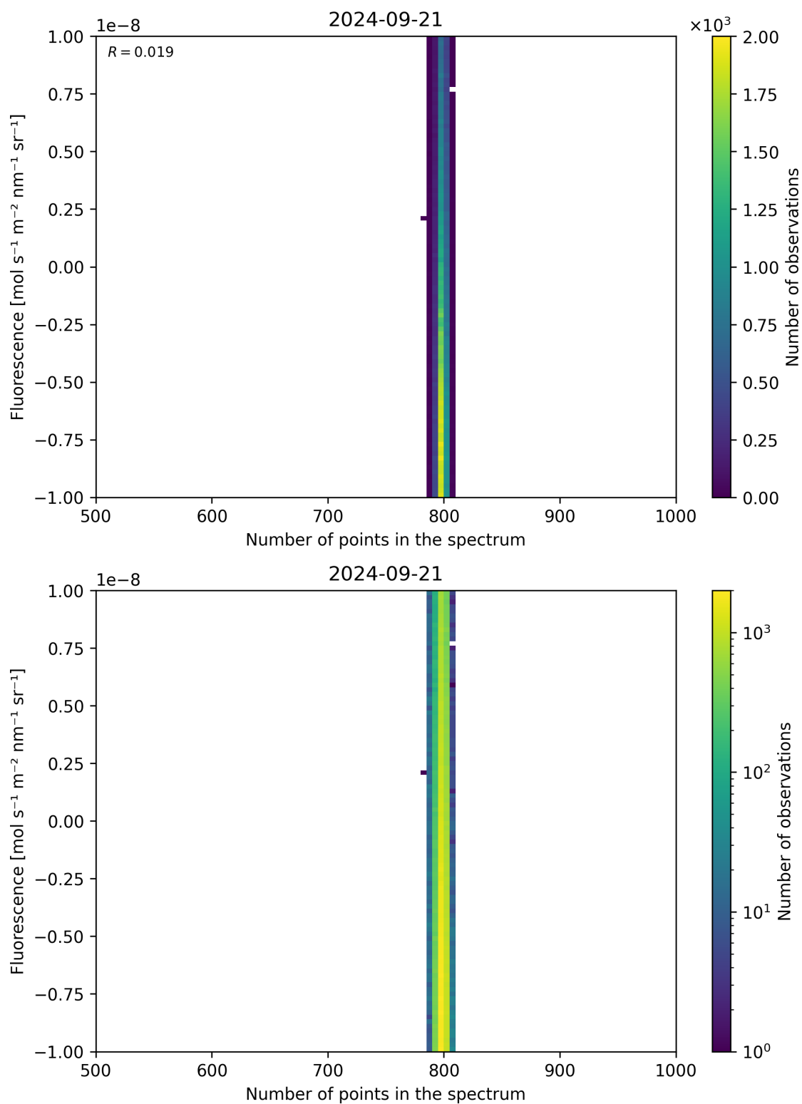
Figure 91: Scatter density plot of “Number of points in the spectrum” against “Fluorescence” for 2024-09-20 to 2024-09-22.
