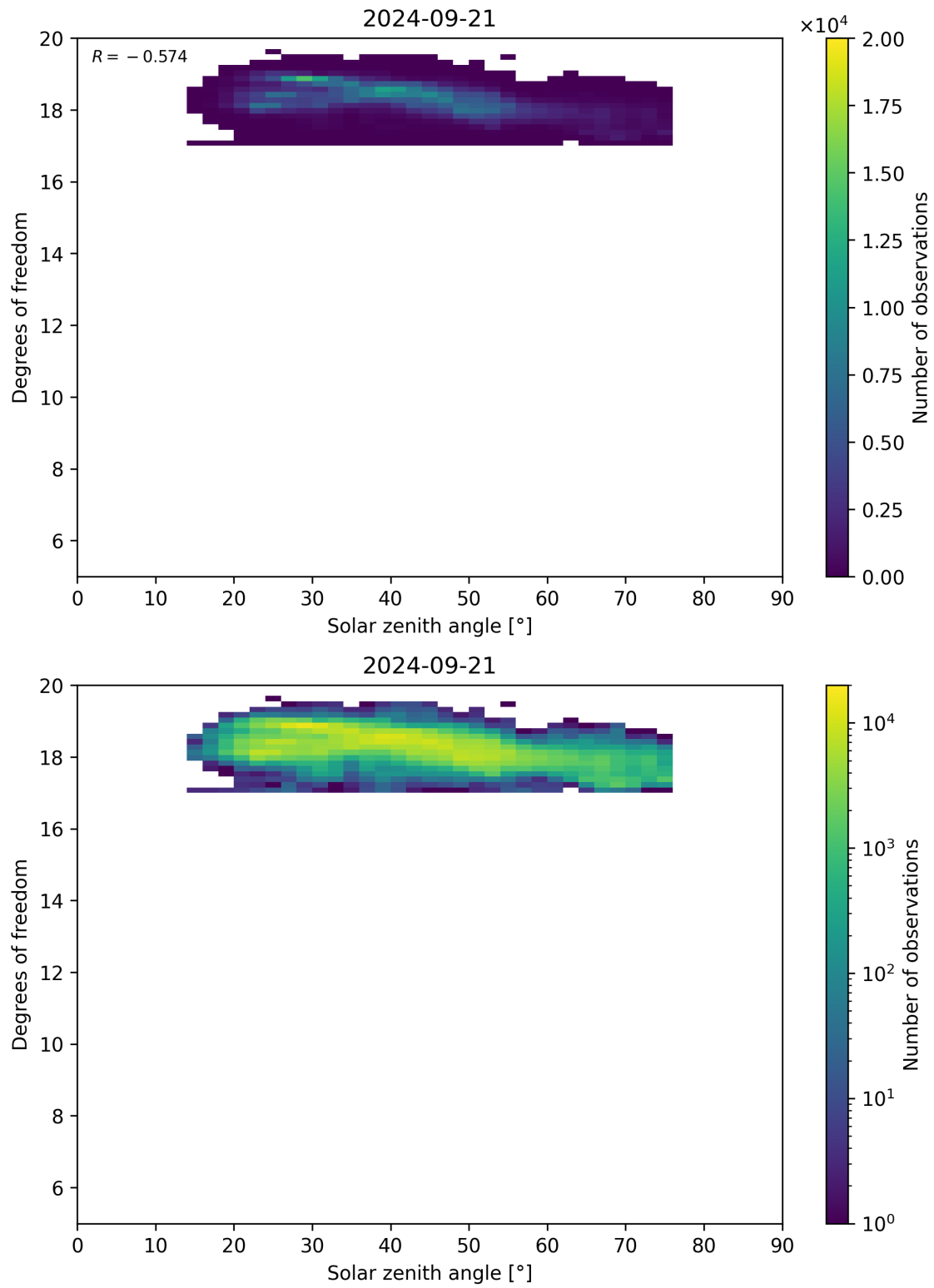
Figure 96: Scatter density plot of “Solar zenith angle” against “Degrees of freedom” for 2024-09-20 to 2024-09-22.
