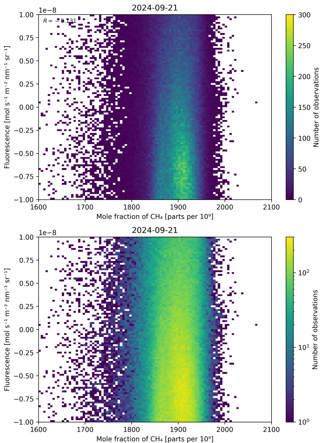
Figure 73: Scatter density plot of “Mole fraction of \text{CH}_4 ” against “Fluorescence” for 2024-09-20 to 2024-09-22.
