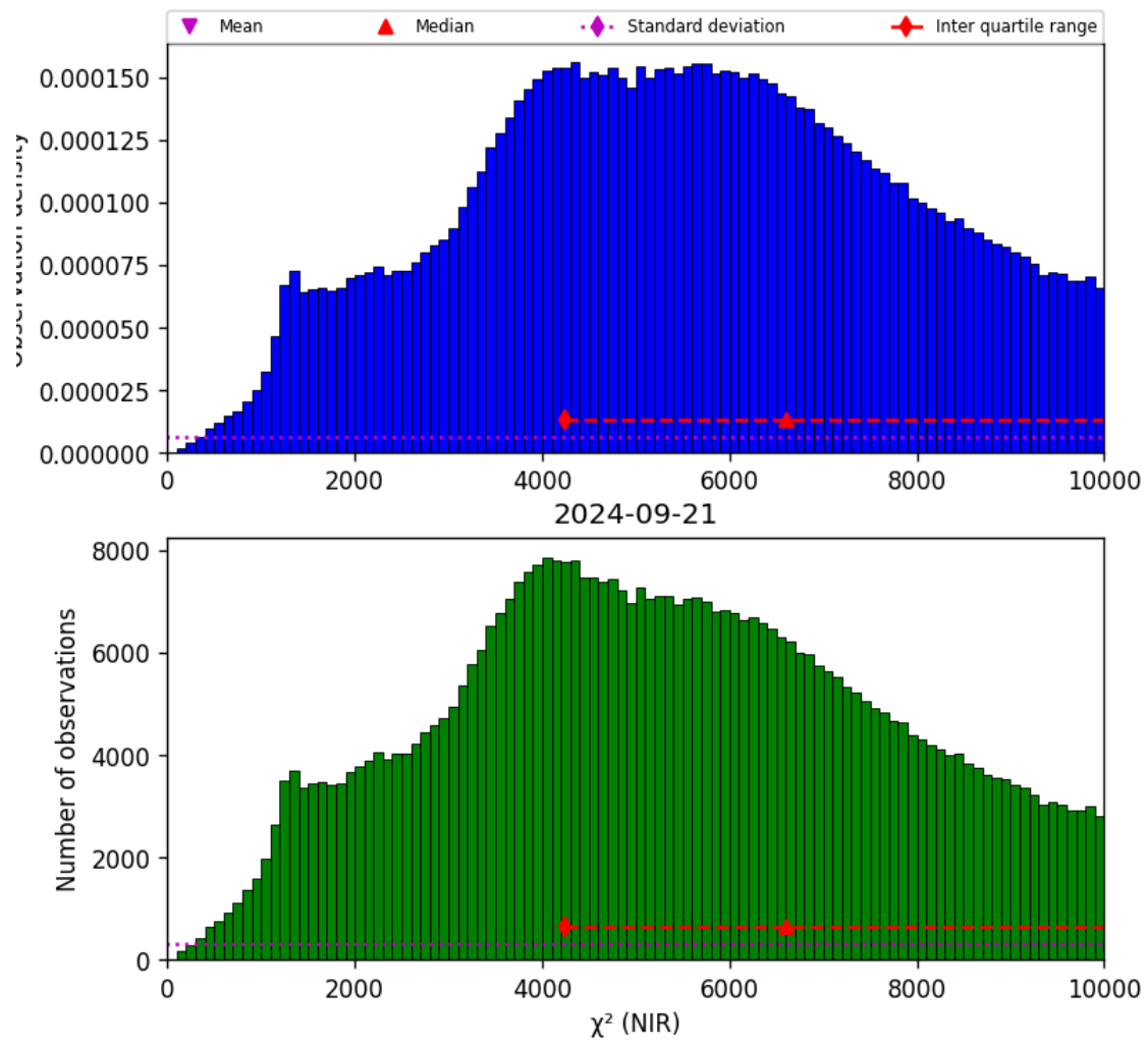
Figure 29: Histogram of “ \chi^2 (NIR)” for 2024-09-20 to 2024-09-22
