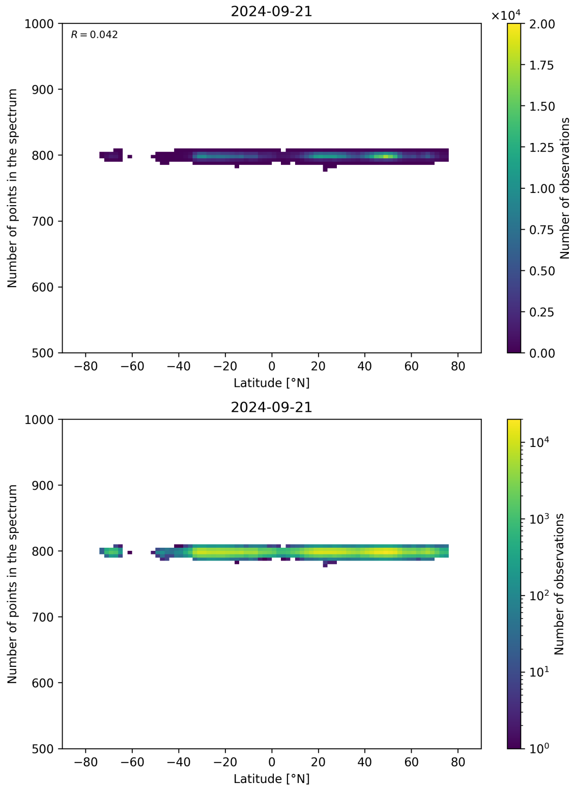
Figure 61: Scatter density plot of “Latitude” against “Number of points in the spectrum” for 2024-09-20 to 2024-09-22.
