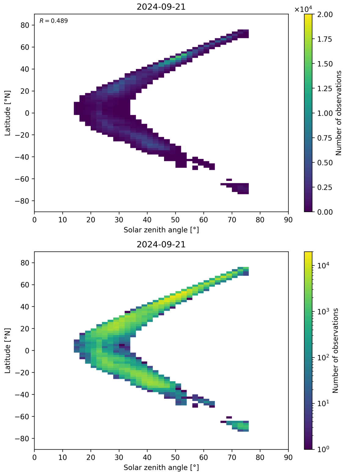
Figure 98: Scatter density plot of “Solar zenith angle” against “Latitude” for 2024-09-20 to 2024-09-22.
