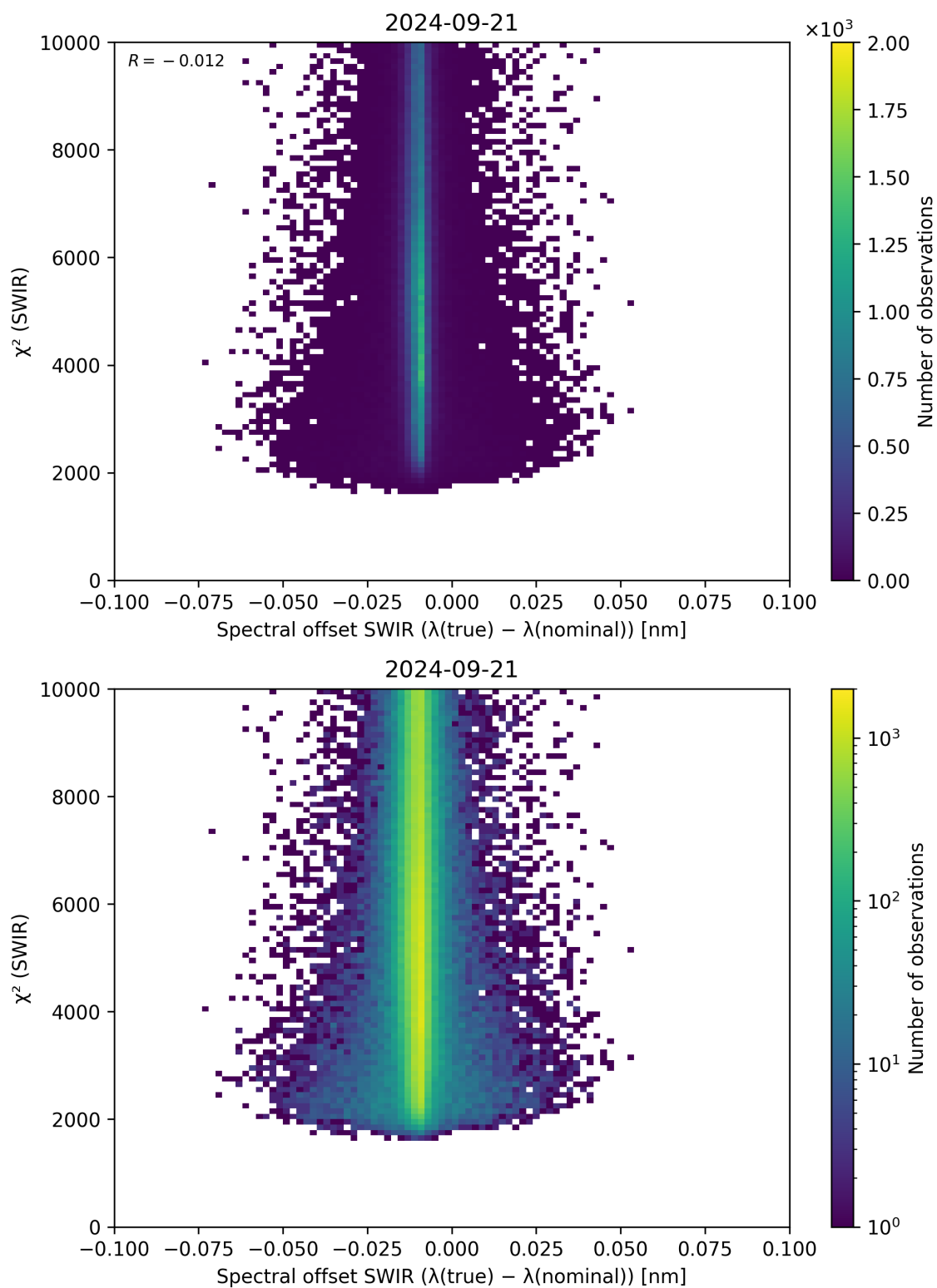
Figure 118: Scatter density plot of “Spectral offset SWIR ( \lambda_{\text{true}} - \lambda_{\text{nominal}} )” against “ \chi^2 (SWIR)” for 2024-09-20 to 2024-09-22.
