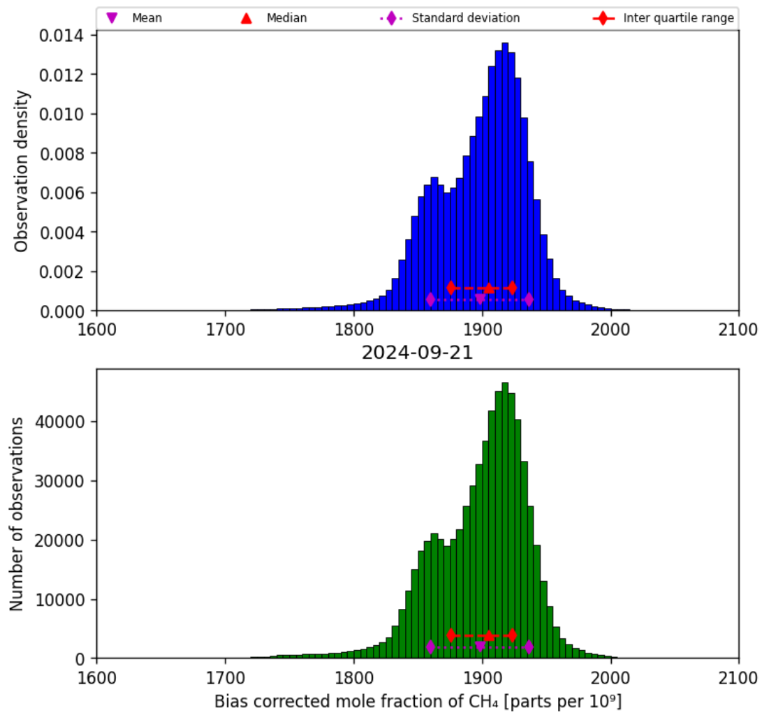
Figure 25: Histogram of “Bias corrected mole fraction of CH 4 ” for 2024-09-20 to 2024-09-22
