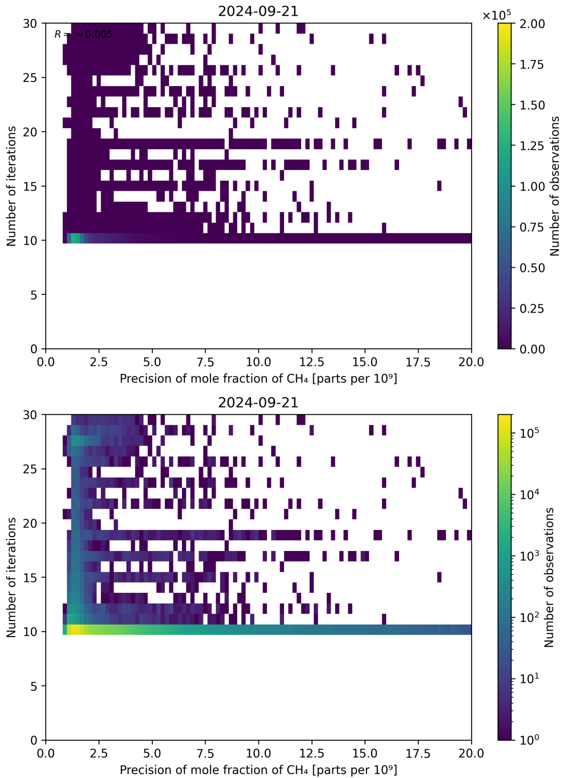
Figure 83: Scatter density plot of “Precision of mole fraction of CH 4 ” against “Number of iterations” for 2024-09-20 to 2024-09-22.
