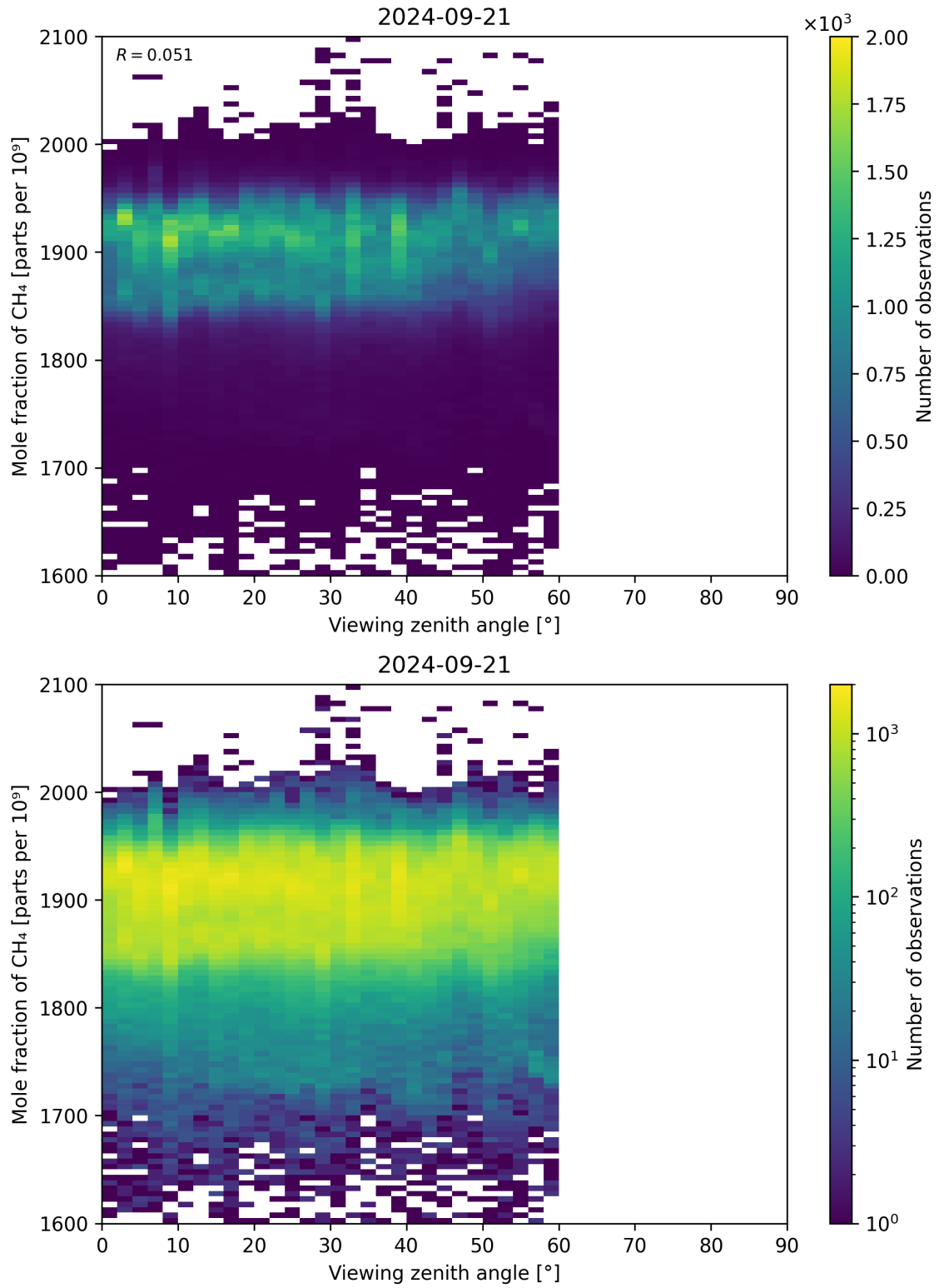
Figure 110: Scatter density plot of “Viewing zenith angle” against “Mole fraction of CH 4 ” for 2024-09-20 to 2024-09-22.
