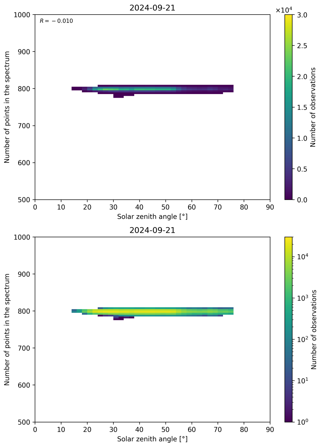
Figure 103: Scatter density plot of “Solar zenith angle” against “Number of points in the spectrum” for 2024-09-20 to 2024-09-22.
