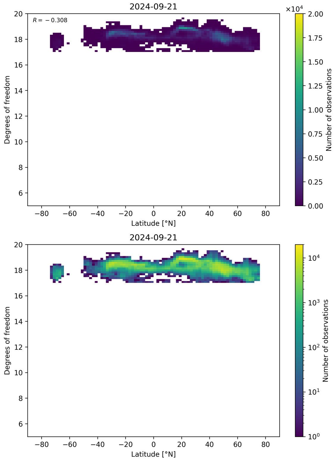
Figure 55: Scatter density plot of “Latitude” against “Degrees of freedom” for 2024-09-20 to 2024-09-22.
