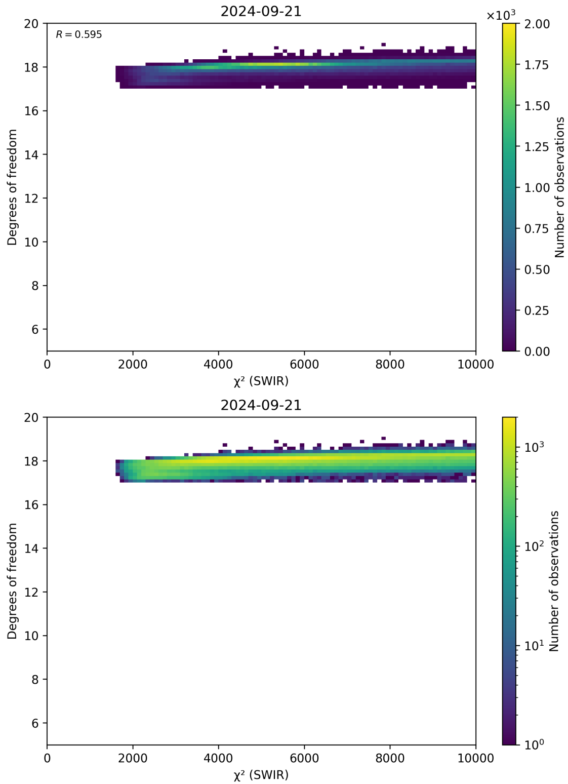
Figure 48: Scatter density plot of “ \chi^2 (SWIR)” against “Degrees of freedom” for 2024-09-20 to 2024-09-22.
