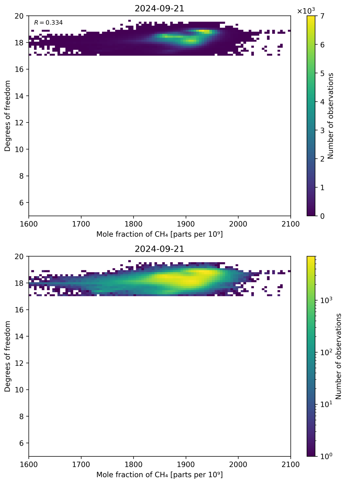
Figure 72: Scatter density plot of “Mole fraction of CH 4 ” against “Degrees of freedom” for 2024-09-20 to 2024-09-22.
