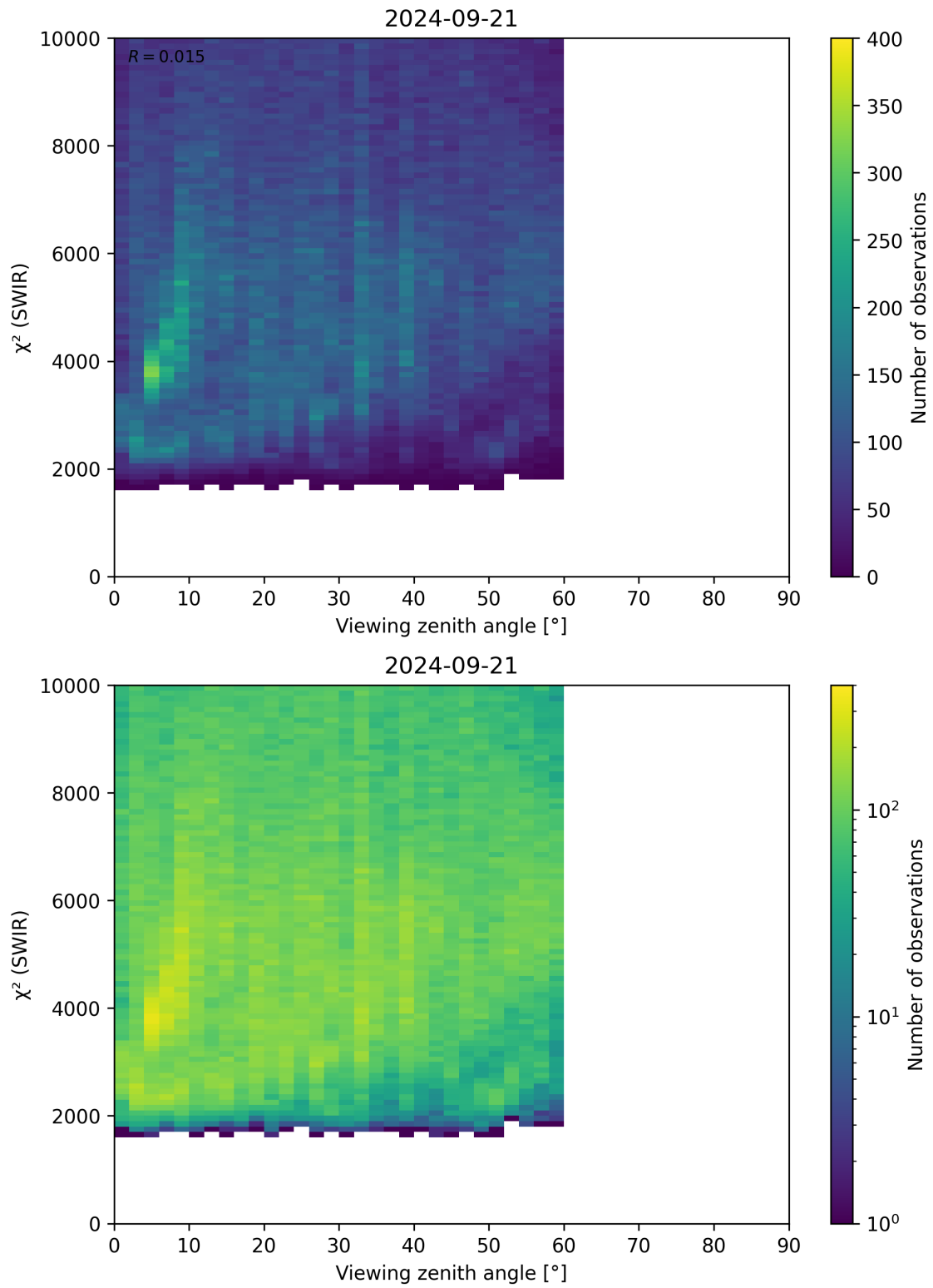
Figure 106: Scatter density plot of “Viewing zenith angle” against “ \chi^2 (SWIR)” for 2024-09-20 to 2024-09-22.
