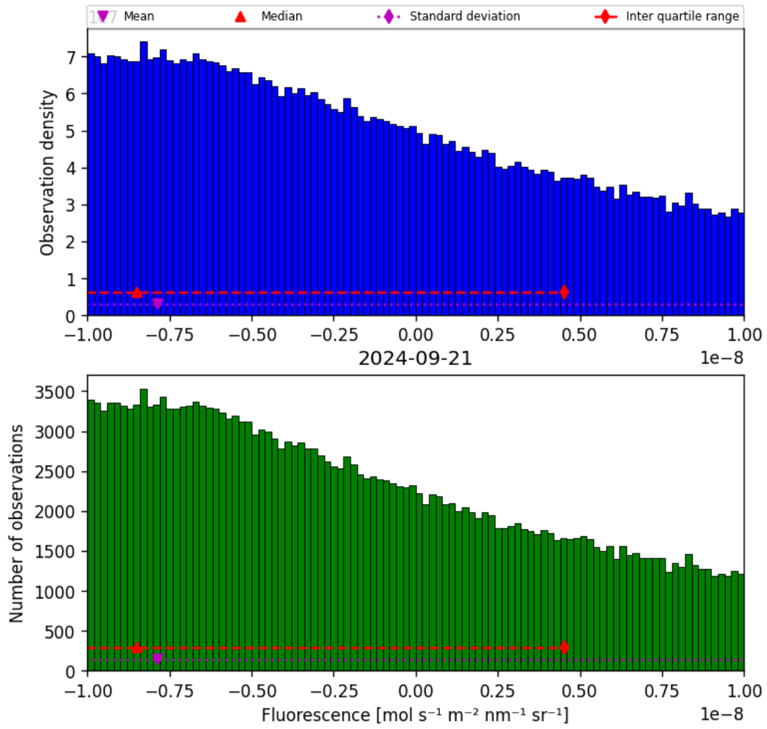
Figure 32: Histogram of “Fluorescence” for 2024-09-20 to 2024-09-22
