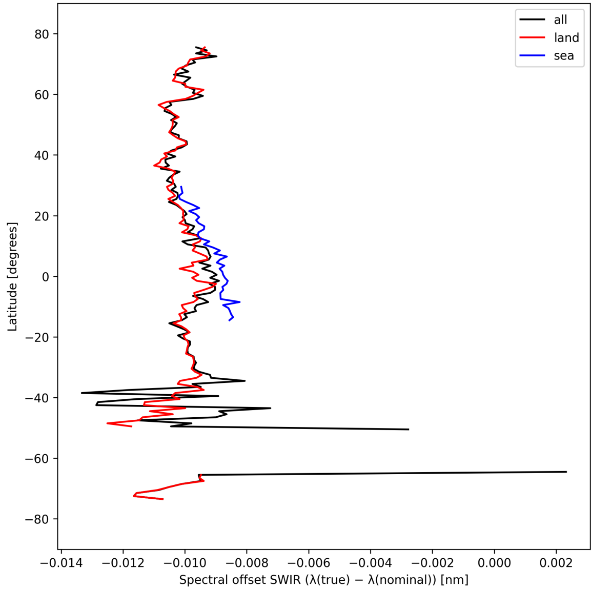
Figure 16: Zonal average of “Spectral offset SWIR ( \lambda_{\text{true}} - \lambda_{\text{nominal}} )” for 2024-09-20 to 2024-09-22.
