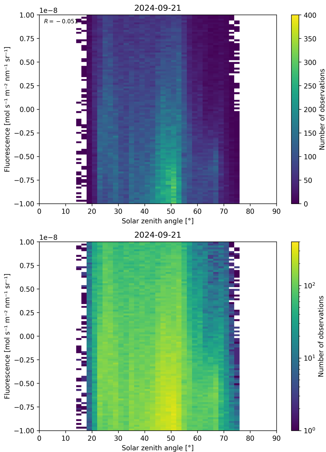
Figure 97: Scatter density plot of “Solar zenith angle” against “Fluorescence” for 2024-09-20 to 2024-09-22.
