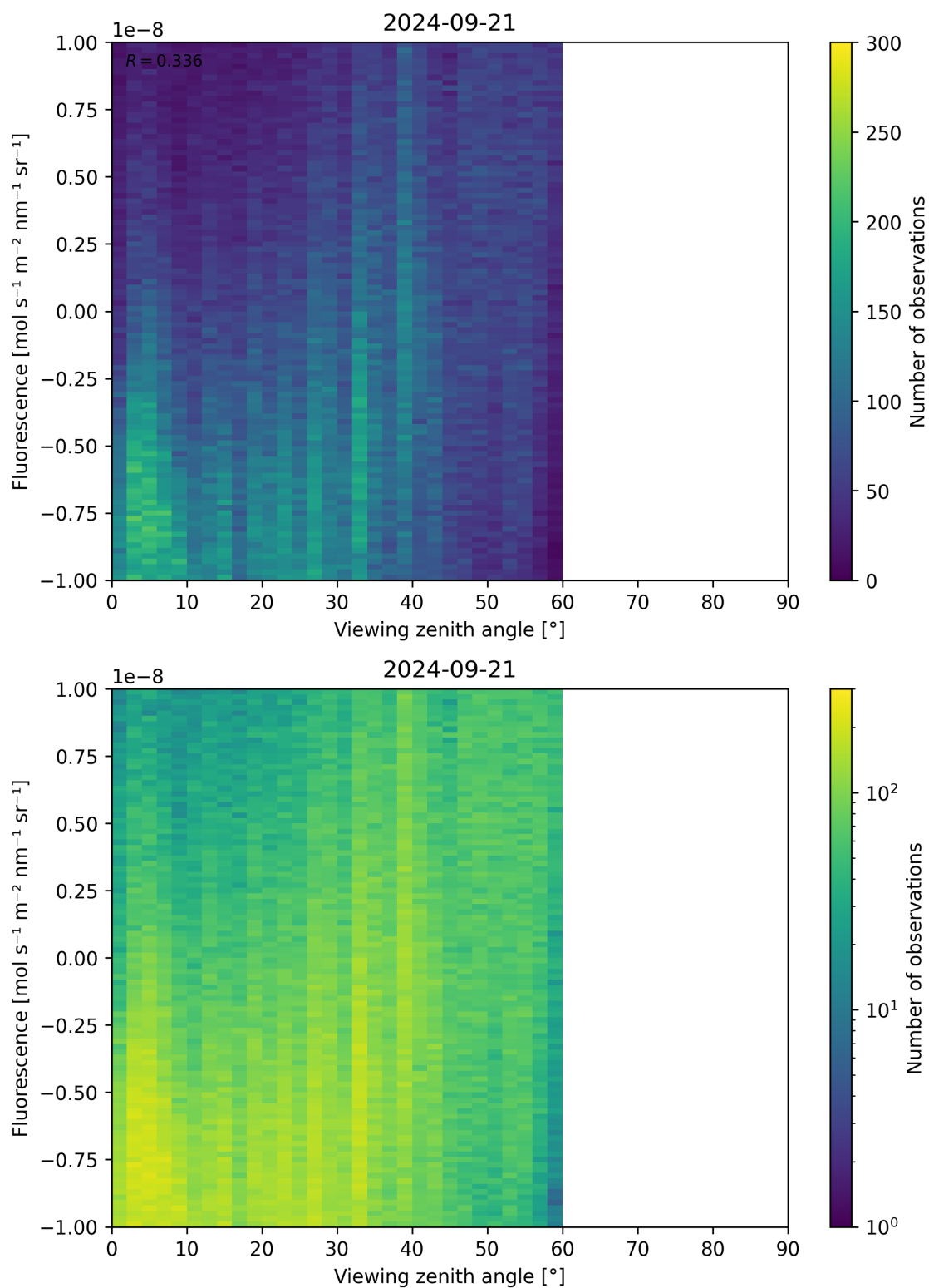
Figure 108: Scatter density plot of “Viewing zenith angle” against “Fluorescence” for 2024-09-20 to 2024-09-22.
