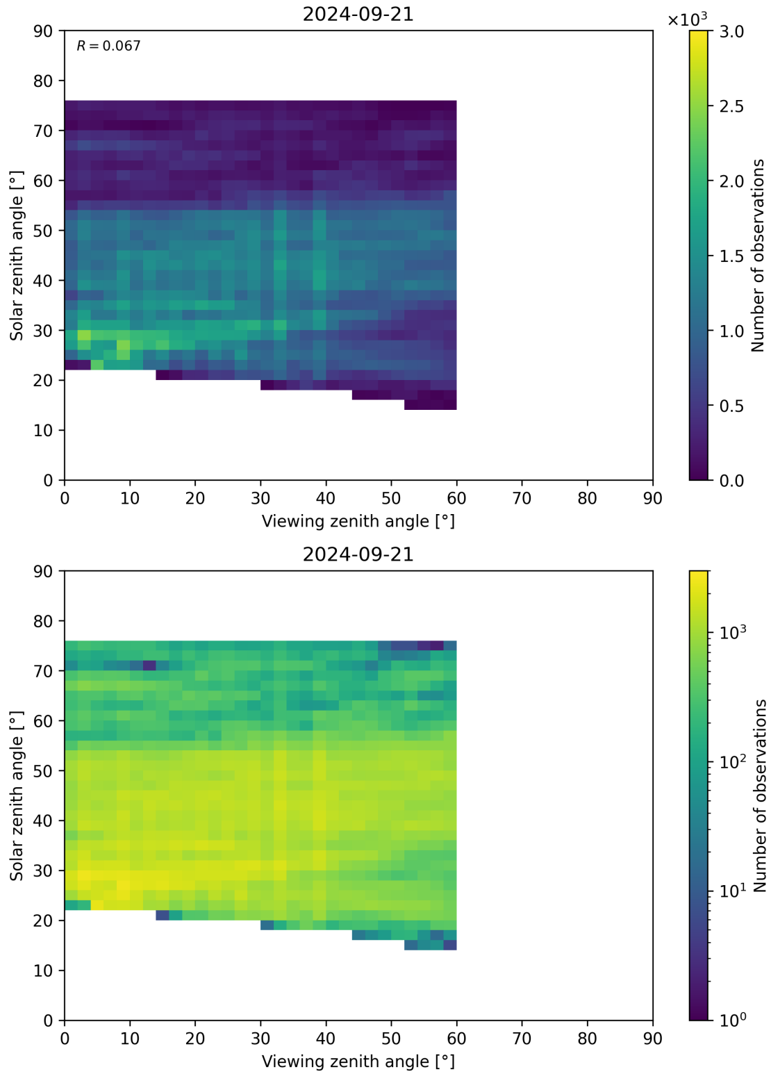
Figure 115: Scatter density plot of “Viewing zenith angle” against “Solar zenith angle” for 2024-09-20 to 2024-09-22.
