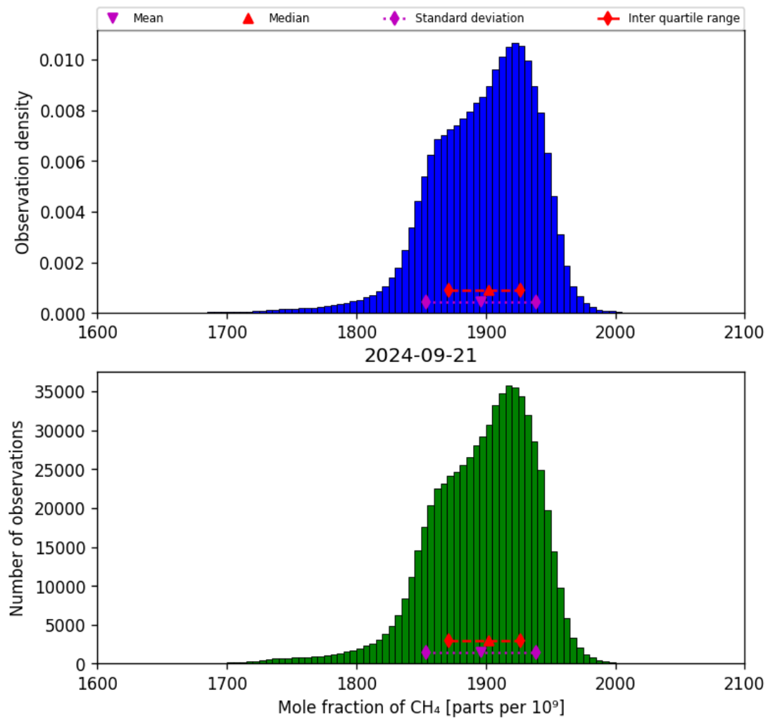
Figure 23: Histogram of “Mole fraction of CH 4 ” for 2024-09-20 to 2024-09-22
