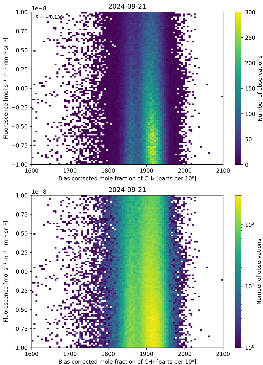
Figure 66: Scatter density plot of “Bias corrected mole fraction of CH 4 ” against “Fluorescence” for 2024-09-20 to 2024-09-22.
