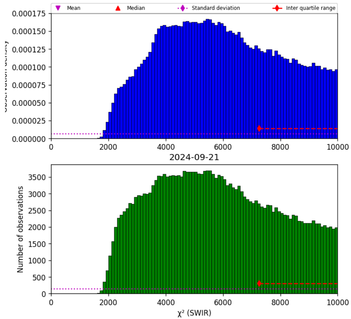
Figure 28: Histogram of “ \chi^2 (SWIR)” for 2024-09-20 to 2024-09-22
