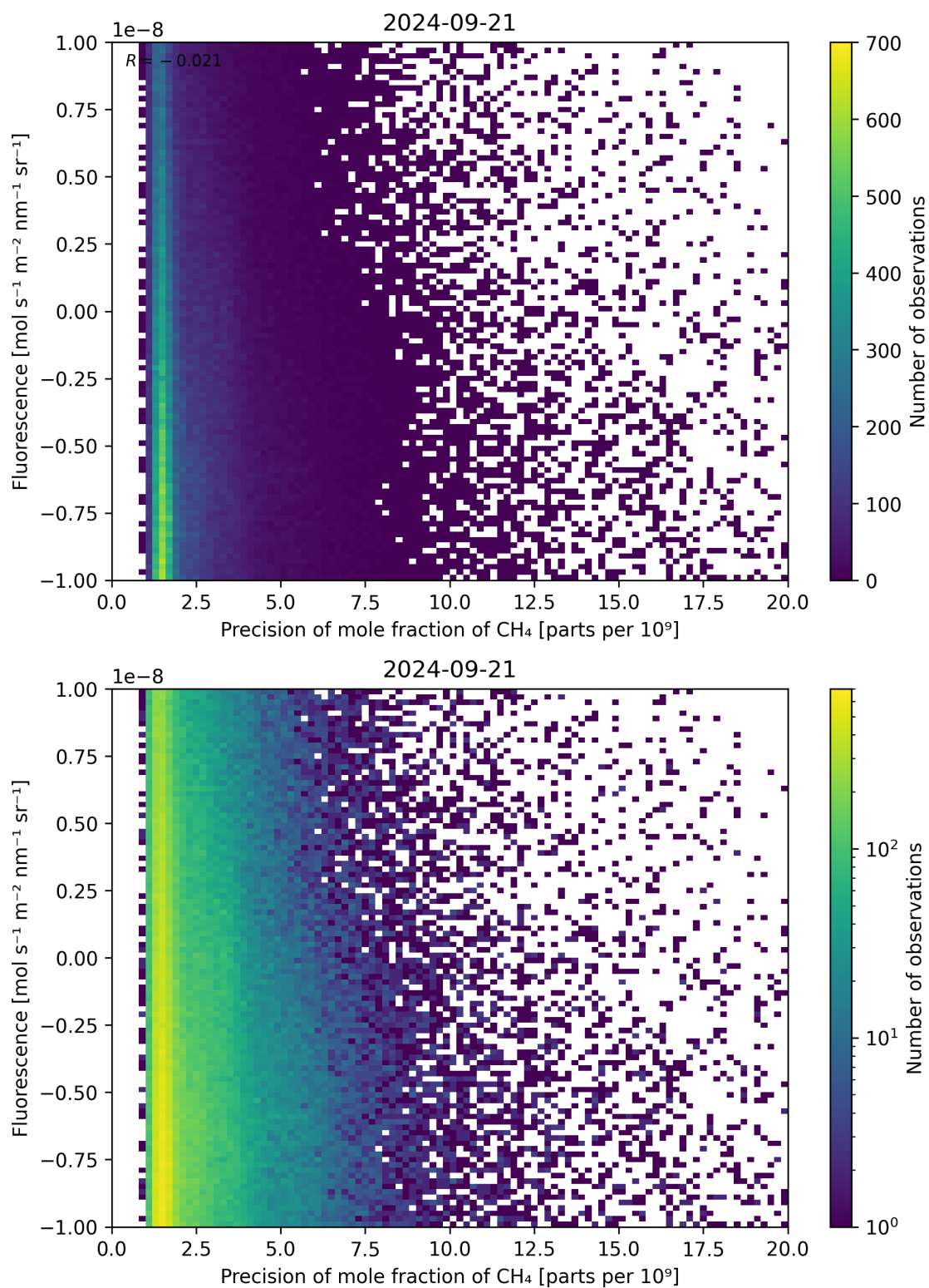
Figure 81: Scatter density plot of “Precision of mole fraction of \text{CH}_4 ” against “Fluorescence” for 2024-09-20 to 2024-09-22.
