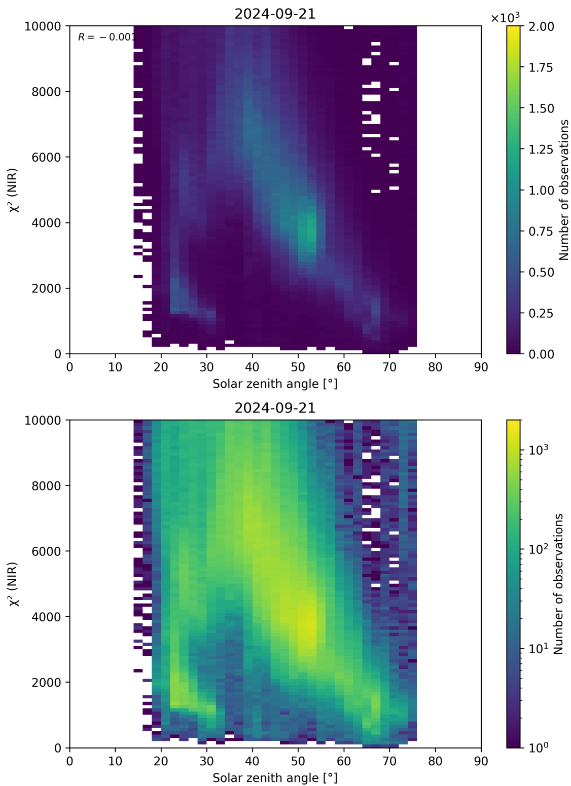
Figure 94: Scatter density plot of “Solar zenith angle” against “ \chi^2 (NIR)” for 2024-09-20 to 2024-09-22.
