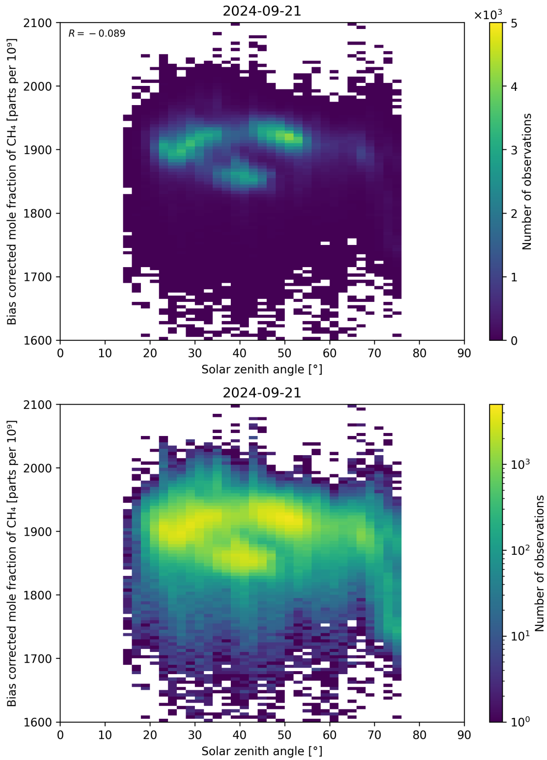
Figure 100: Scatter density plot of “Solar zenith angle” against “Bias corrected mole fraction of \text{CH}_4 ” for 2024-09-20 to 2024-09-22.
