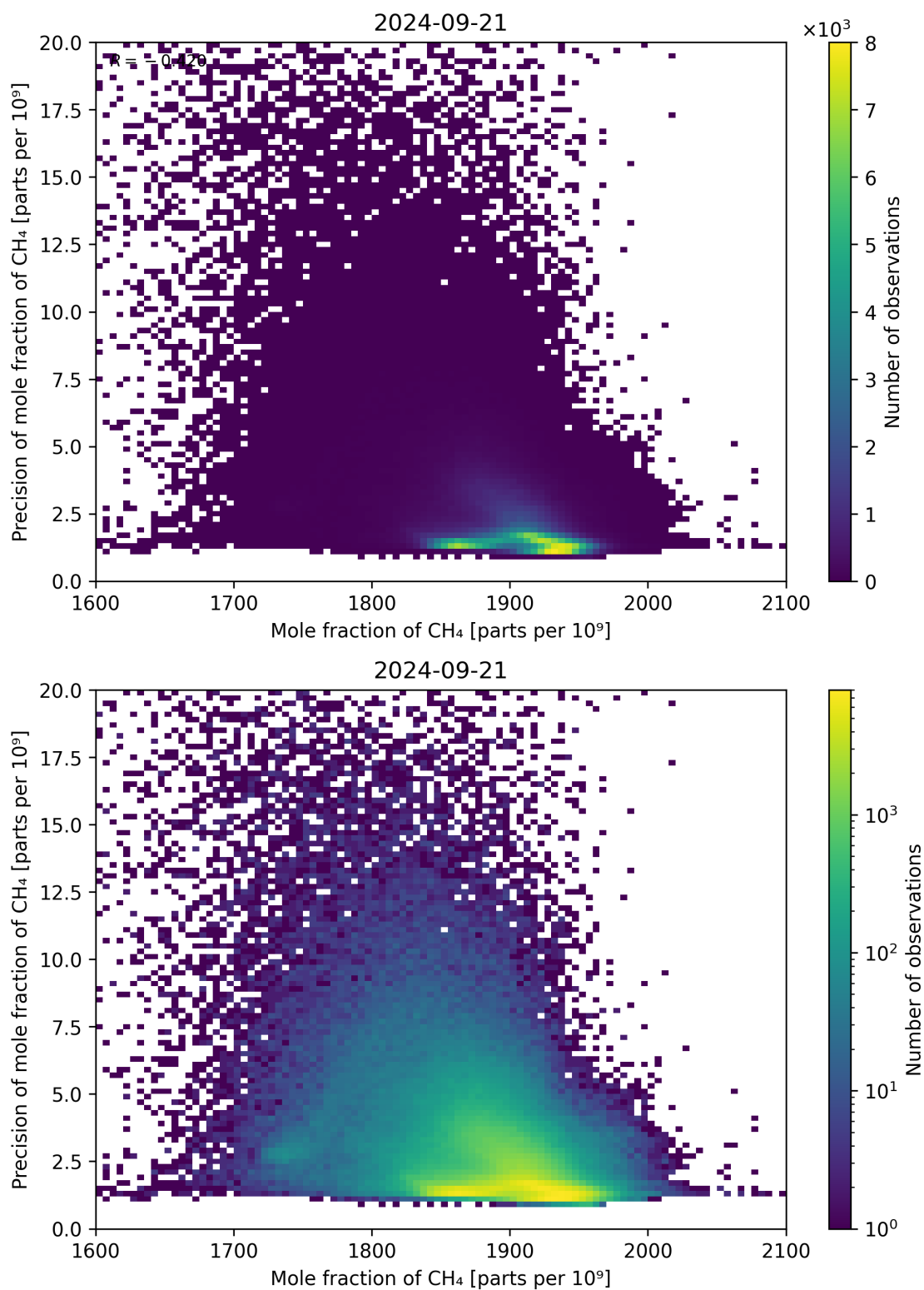
Figure 75: Scatter density plot of “Mole fraction of CH 4 ” against “Precision of mole fraction of CH 4 ” for 2024-09-20 to 2024-09-22.
