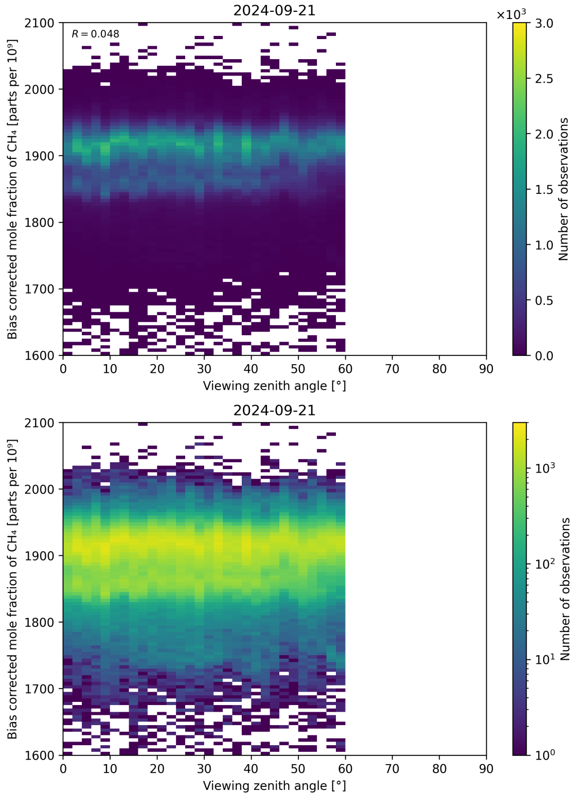
Figure 111: Scatter density plot of “Viewing zenith angle” against “Bias corrected mole fraction of CH 4 ” for 2024-09-20 to 2024-09-22.
