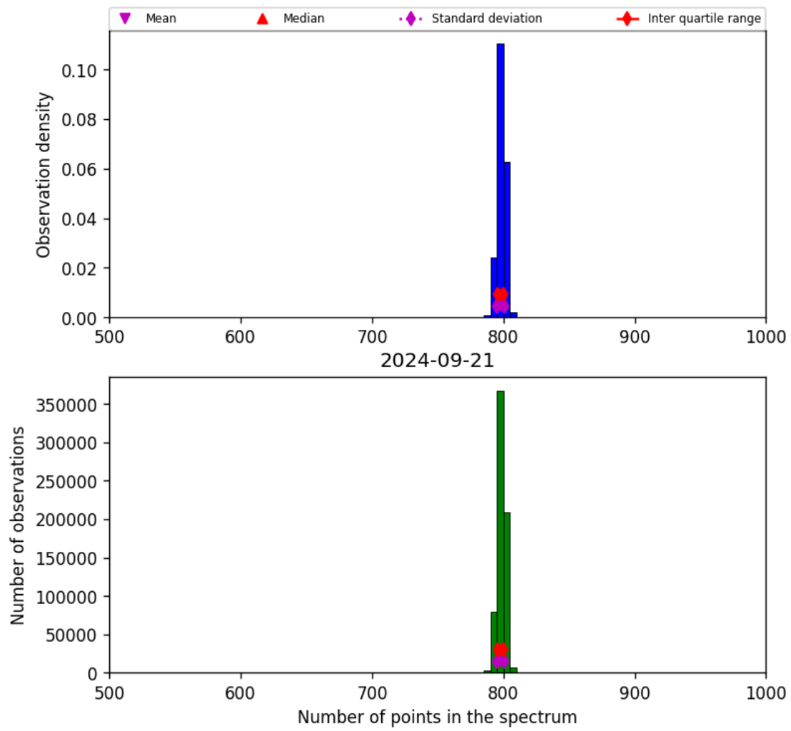
Figure 26: Histogram of “Number of points in the spectrum” for 2024-09-20 to 2024-09-22
