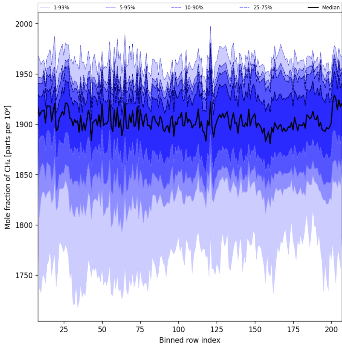
Figure 34: Along track statistics of “Mole fraction of CH 4 ” for 2024-09-20 to 2024-09-22
