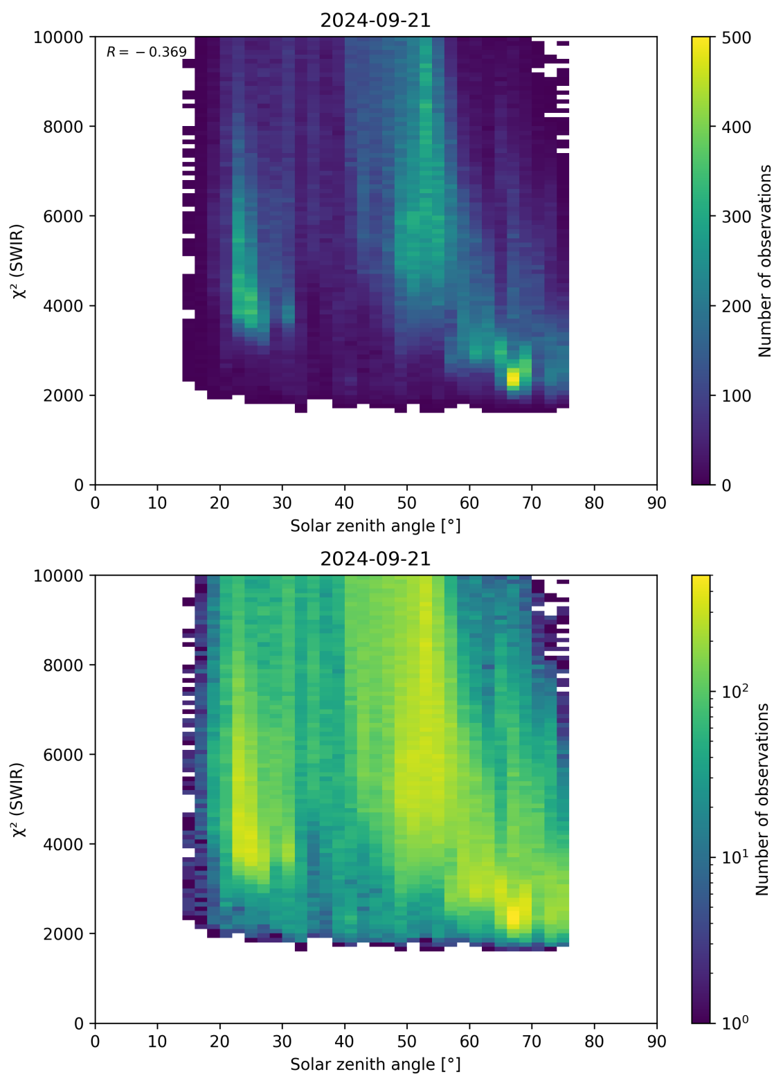
Figure 95: Scatter density plot of “Solar zenith angle” against “ \chi^2 (SWIR)” for 2024-09-20 to 2024-09-22.
