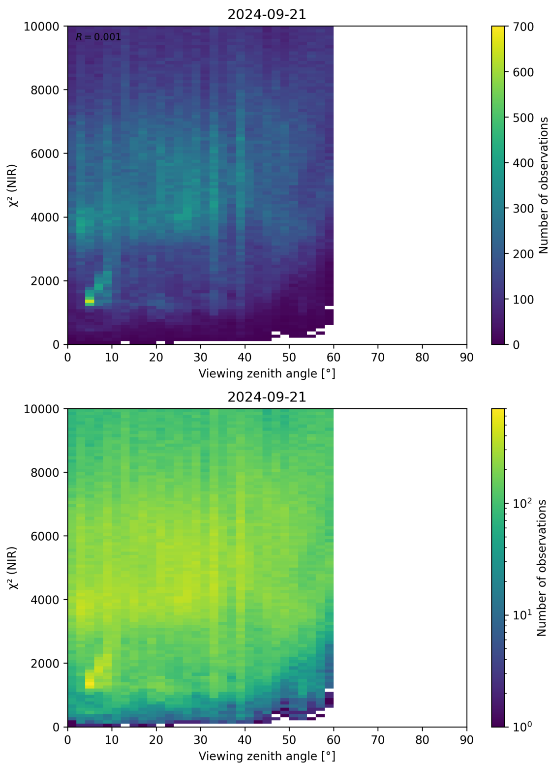
Figure 105: Scatter density plot of “Viewing zenith angle” against “ \chi^2 (NIR)” for 2024-09-20 to 2024-09-22.
