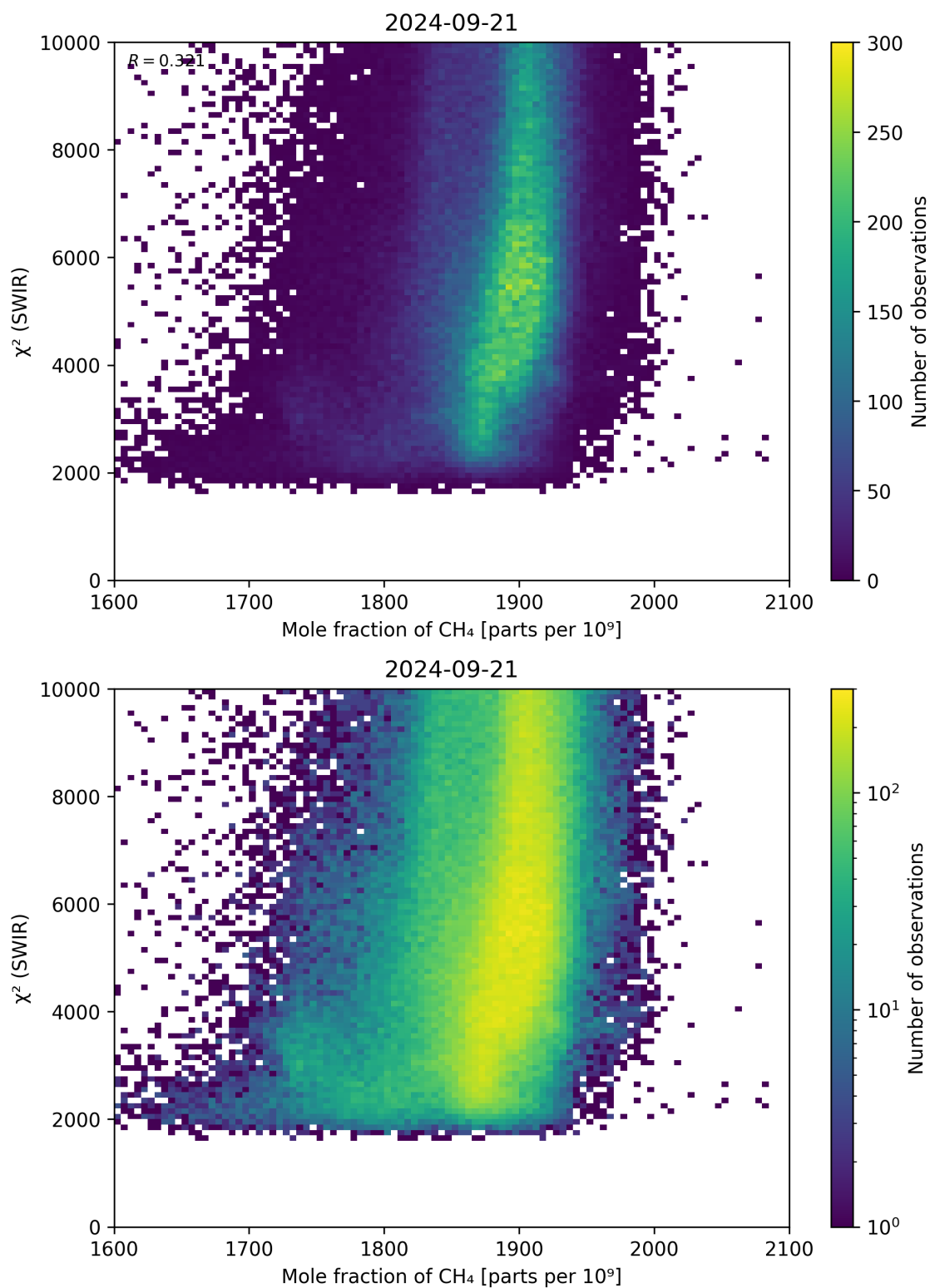
Figure 71: Scatter density plot of “Mole fraction of \text{CH}_4 ” against “ \chi^2 (SWIR)” for 2024-09-20 to 2024-09-22.
