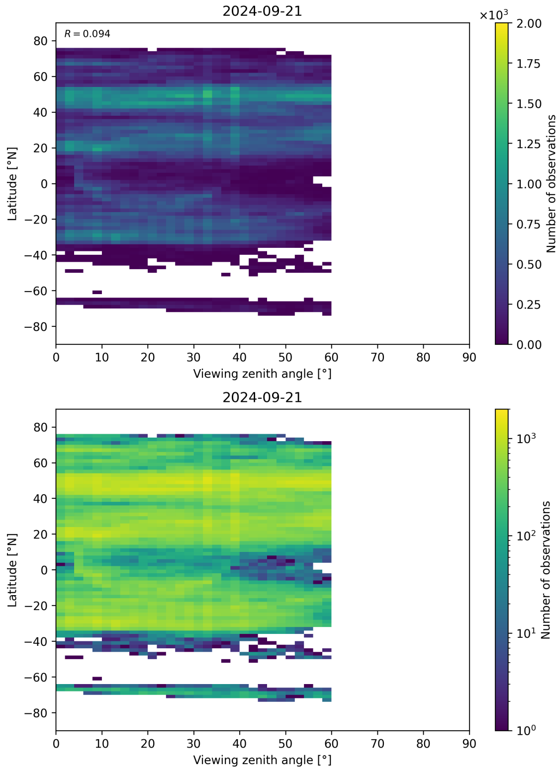
Figure 109: Scatter density plot of “Viewing zenith angle” against “Latitude” for 2024-09-20 to 2024-09-22.
