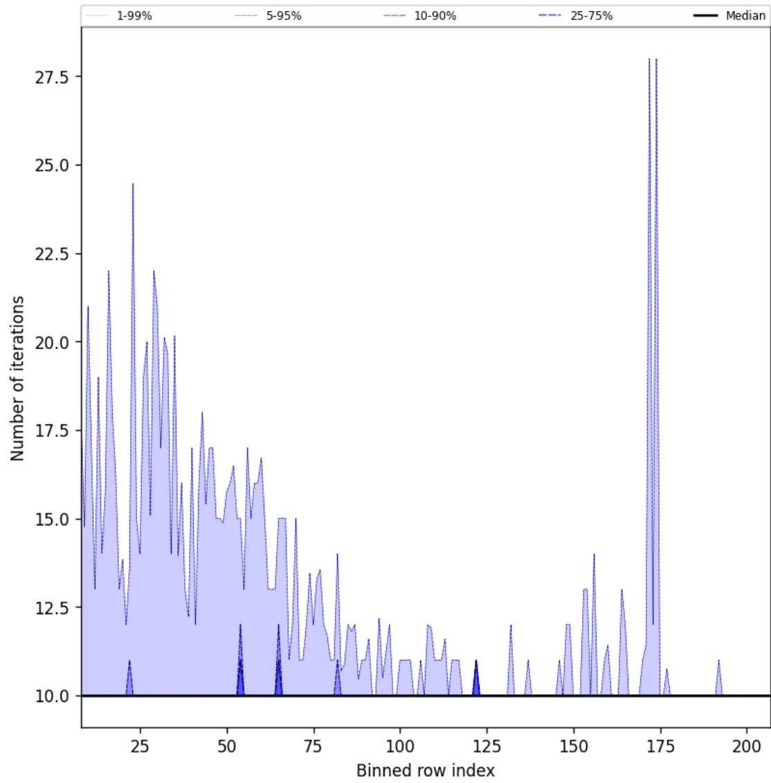
Figure 42: Along track statistics of “Number of iterations” for 2024-09-20 to 2024-09-22
