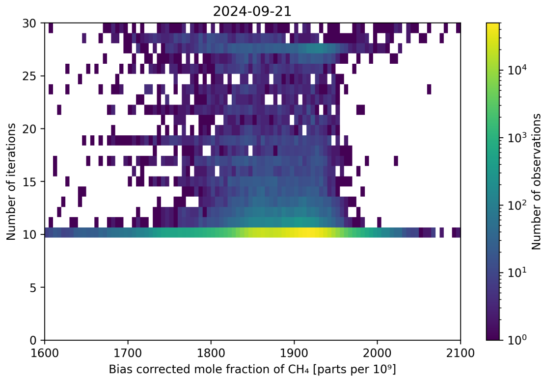
Figure 67: Scatter density plot of “Bias corrected mole fraction of \text{CH}_4 ” against “Number of iterations” for 2024-09-20 to 2024-09-22.
