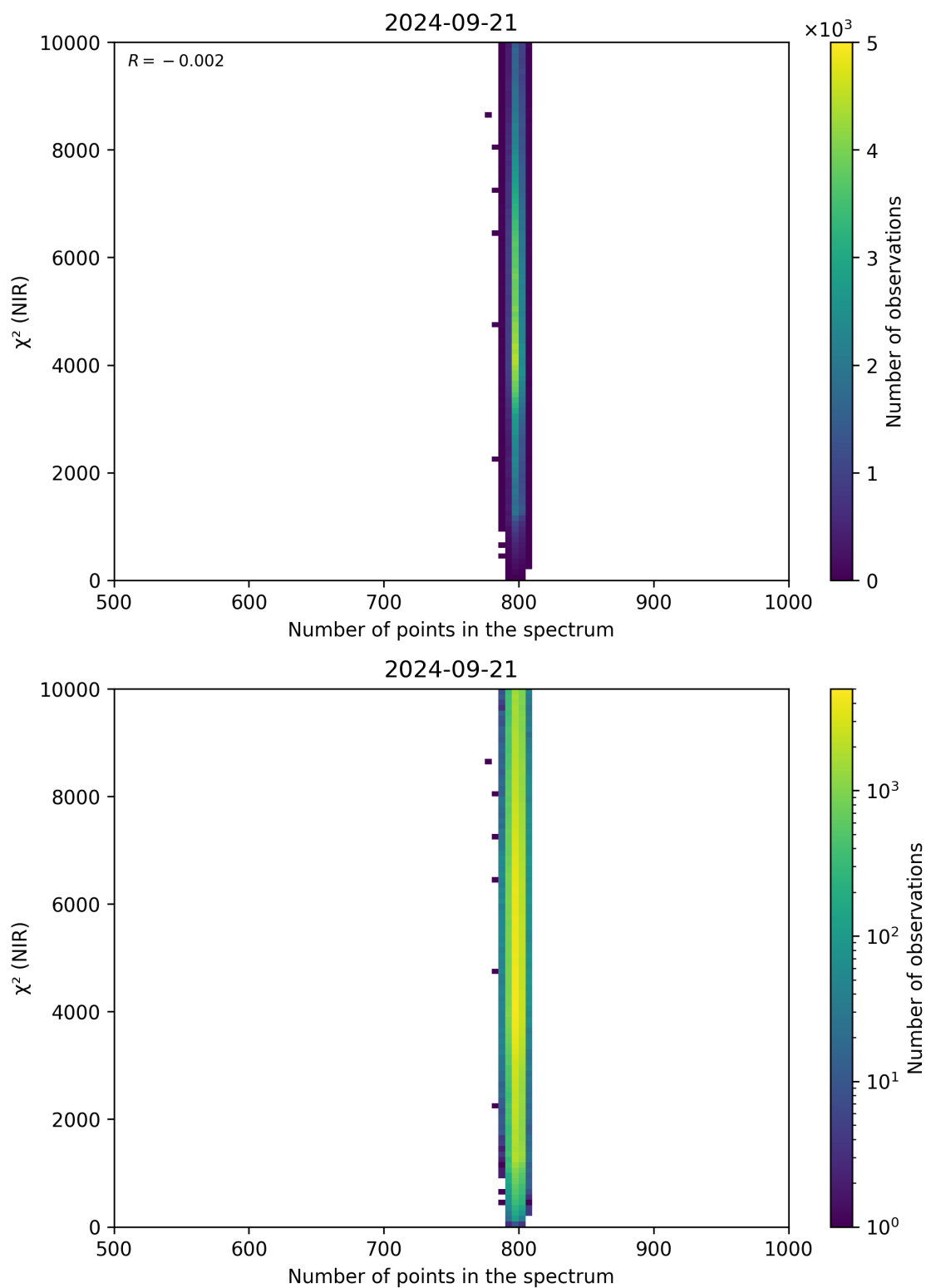
Figure 88: Scatter density plot of “Number of points in the spectrum” against “ \chi^2 (NIR)” for 2024-09-20 to 2024-09-22.
