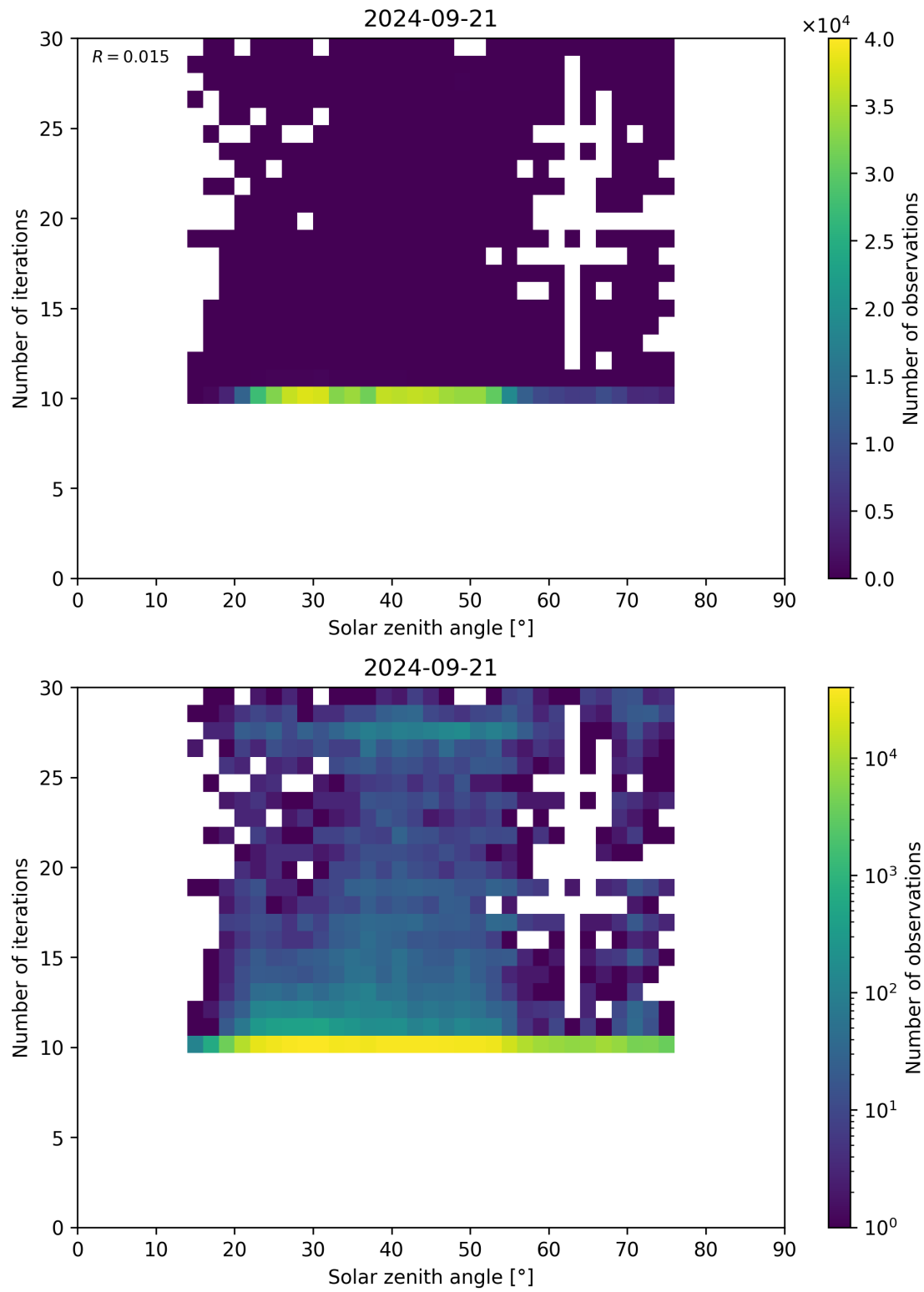
Figure 102: Scatter density plot of “Solar zenith angle” against “Number of iterations” for 2024-09-20 to 2024-09-22.
