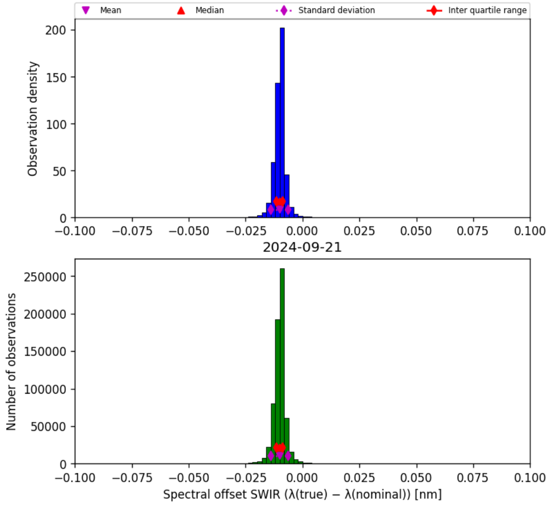
Figure 27: Histogram of “Spectral offset SWIR ( \lambda_{\text{true}} - \lambda_{\text{nominal}} )” for 2024-09-20 to 2024-09-22
