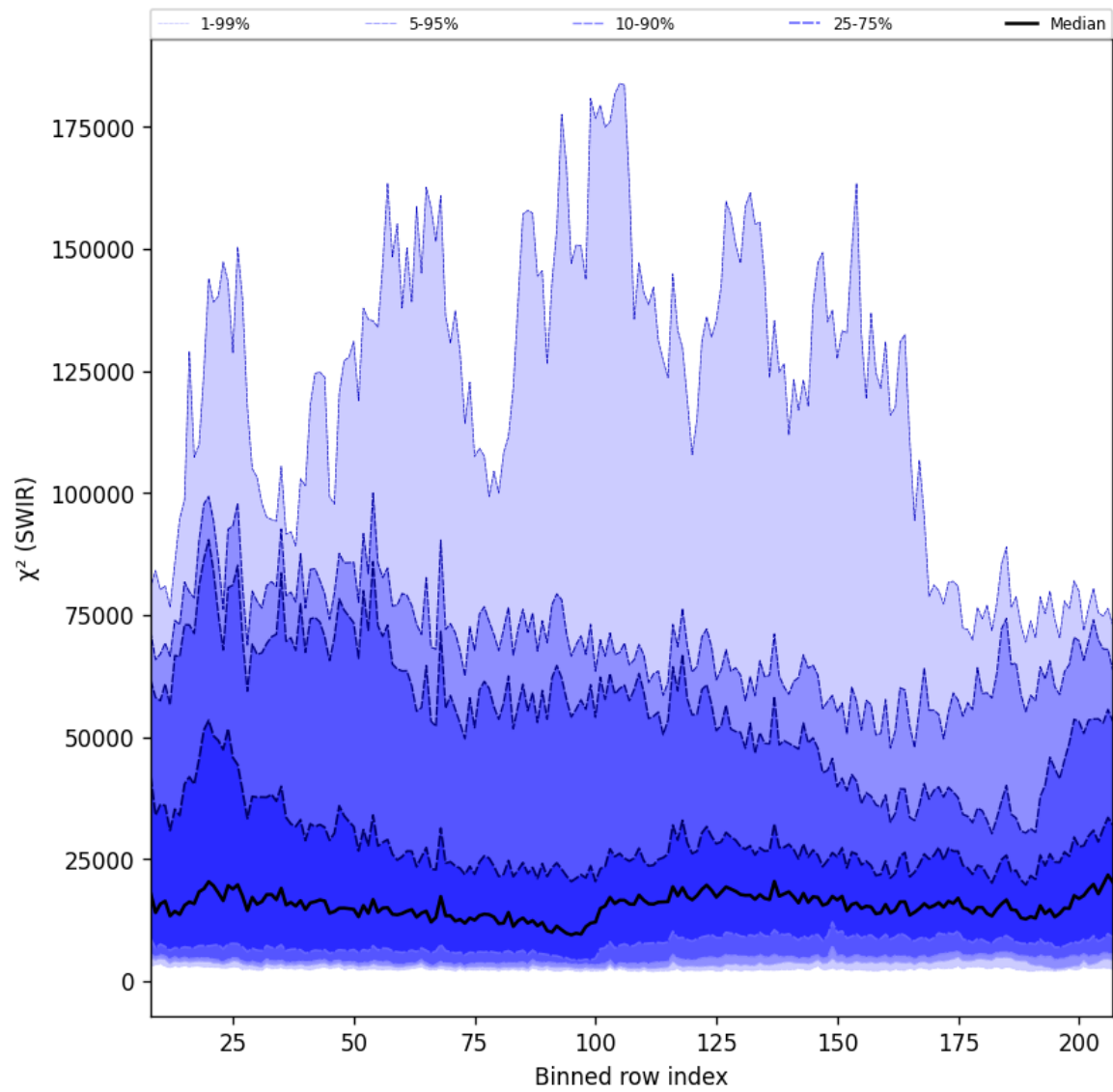
Figure 39: Along track statistics of “ \chi^2 (SWIR)” for 2024-09-20 to 2024-09-22
