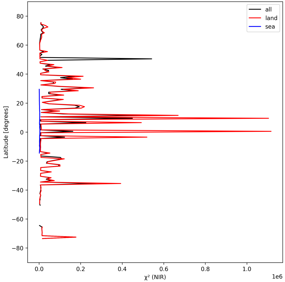
Figure 18: Zonal average of “ \chi^2 (NIR)” for 2024-09-20 to 2024-09-22.
