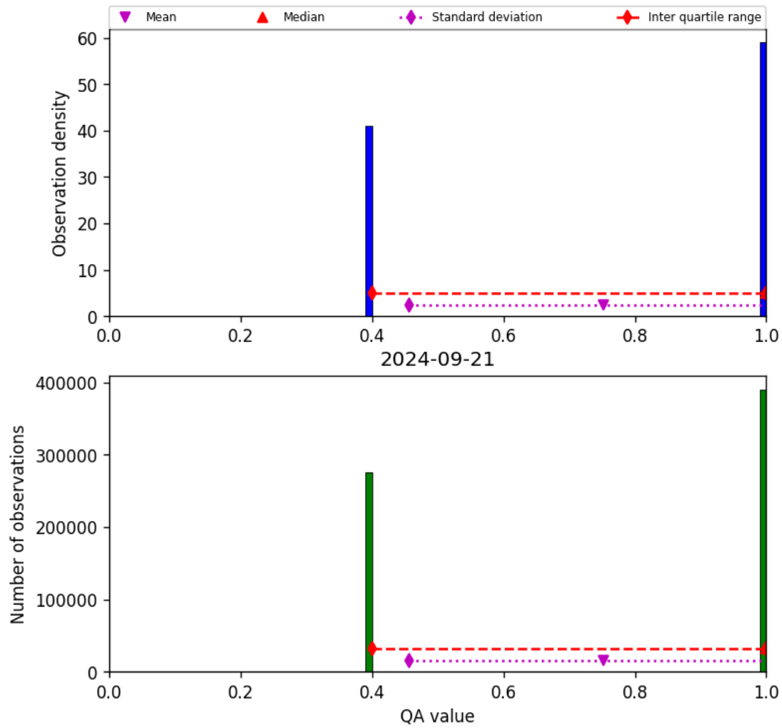
Figure 22: Histogram of “QA value” for 2024-09-20 to 2024-09-22
