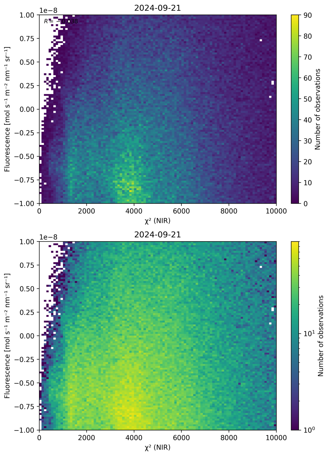
Figure 45: Scatter density plot of “ \chi^2 (NIR)” against “Fluorescence” for 2024-09-20 to 2024-09-22.
