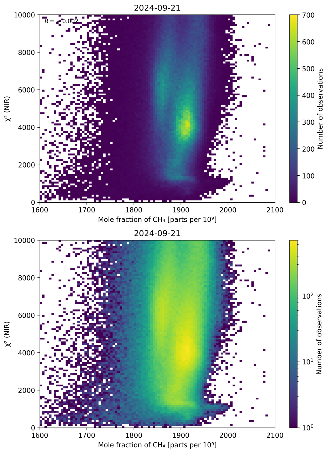
Figure 70: Scatter density plot of “Mole fraction of CH 4 ” against “ \chi^2 (NIR)” for 2024-09-20 to 2024-09-22.
