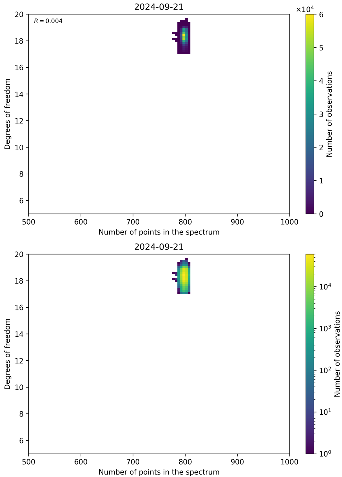
Figure 90: Scatter density plot of “Number of points in the spectrum” against “Degrees of freedom” for 2024-09-20 to 2024-09-22.
