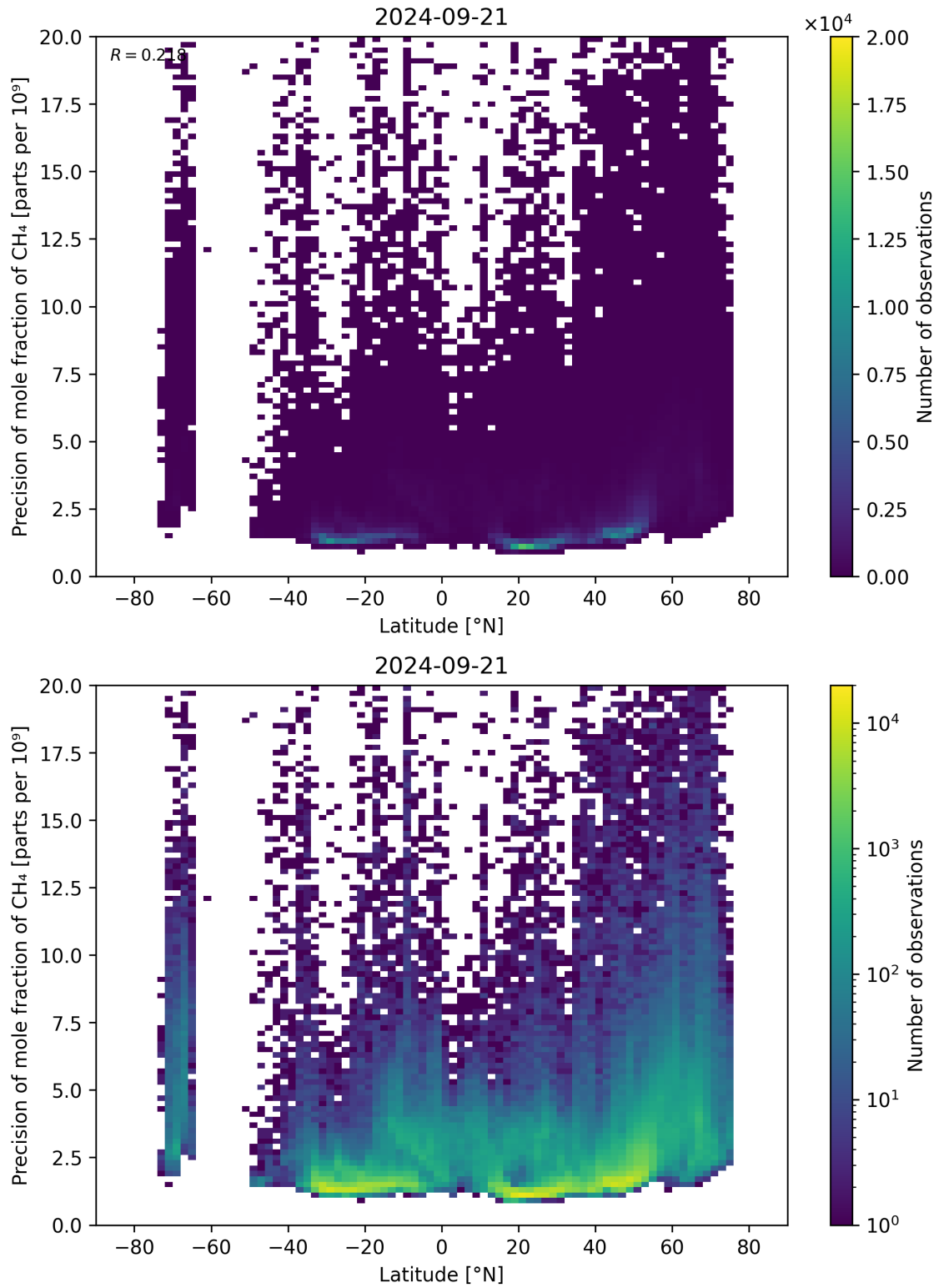
Figure 59: Scatter density plot of “Latitude” against “Precision of mole fraction of CH 4 ” for 2024-09-20 to 2024-09-22.
