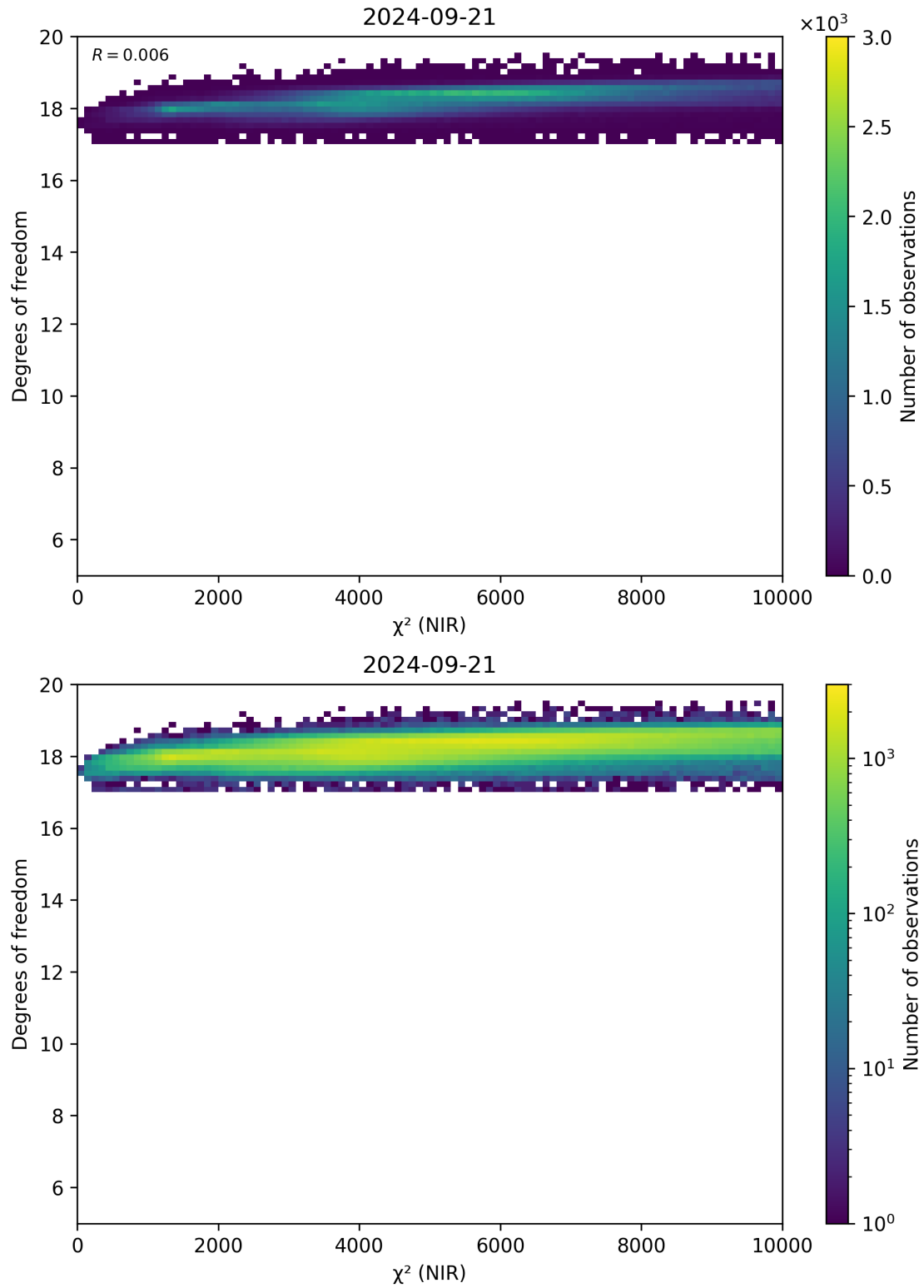
Figure 44: Scatter density plot of “ \chi^2 (NIR)” against “Degrees of freedom” for 2024-09-20 to 2024-09-22.
