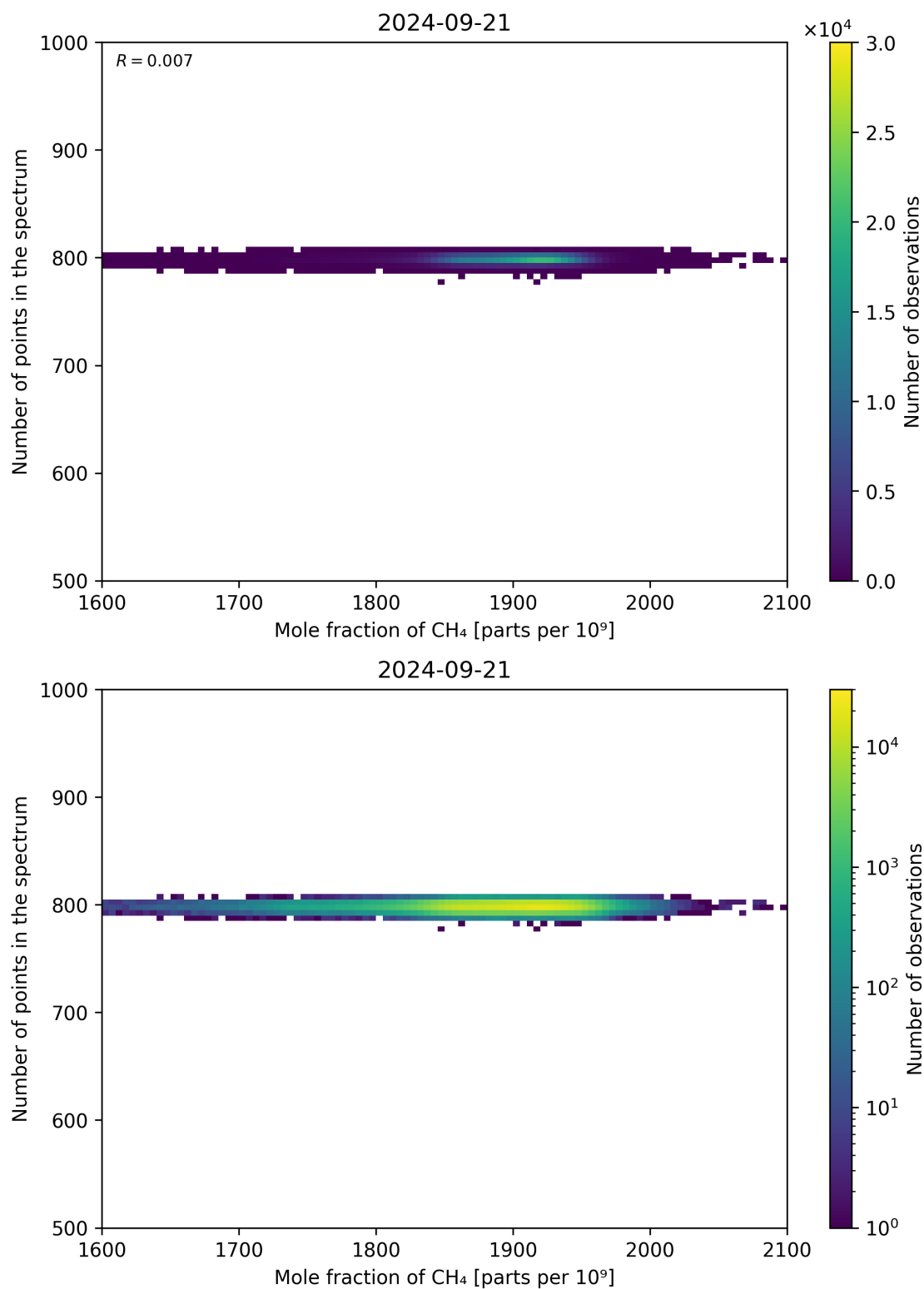
Figure 77: Scatter density plot of “Mole fraction of CH 4 ” against “Number of points in the spectrum” for 2024-09-20 to 2024-09-22.
