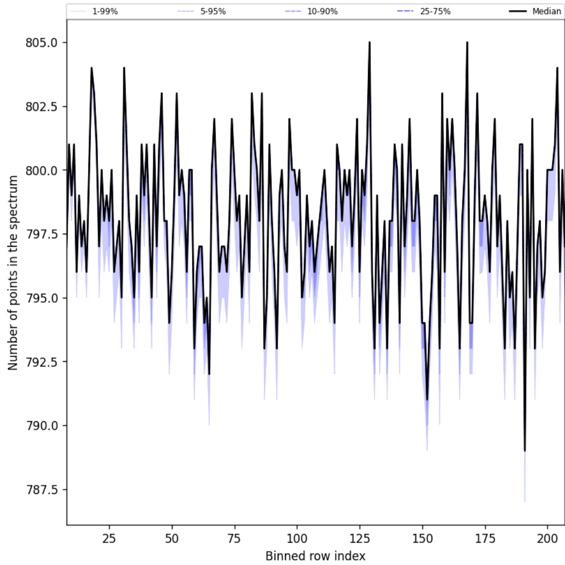
Figure 37: Along track statistics of “Number of points in the spectrum” for 2024-09-20 to 2024-09-22
