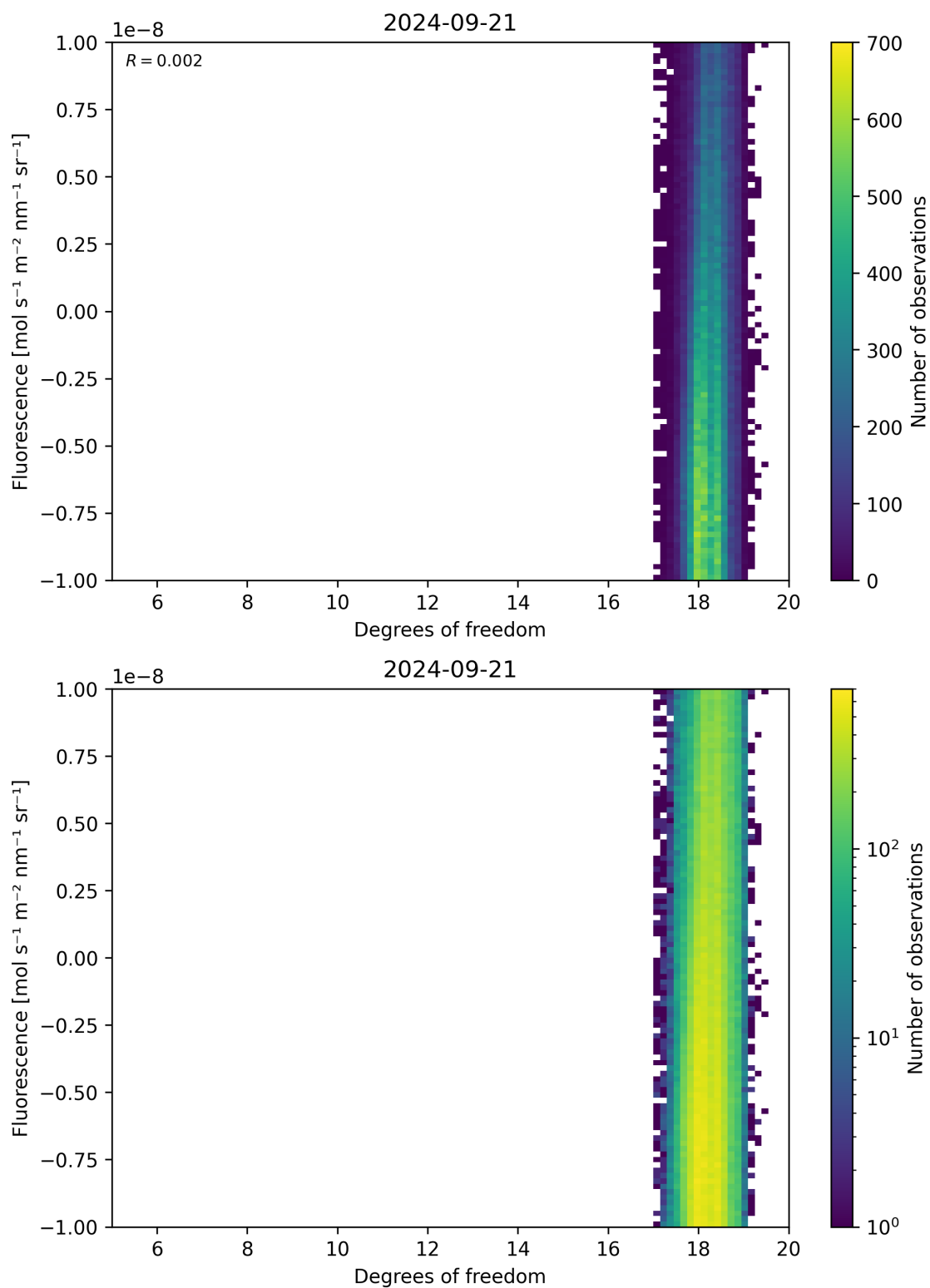
Figure 51: Scatter density plot of “Degrees of freedom” against “Fluorescence” for 2024-09-20 to 2024-09-22.
