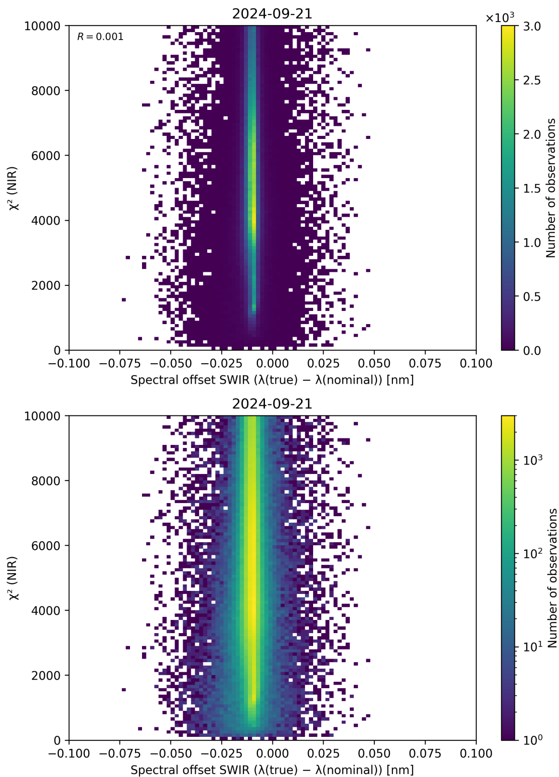
Figure 117: Scatter density plot of “Spectral offset SWIR ( \lambda_{\text{true}} - \lambda_{\text{nominal}} )” against “ \chi^2 (NIR)” for 2024-09-20 to 2024-09-22.
