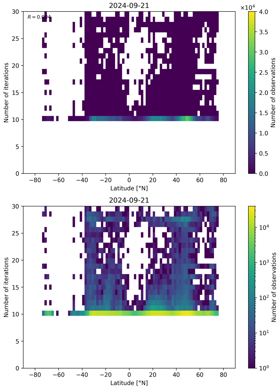
Figure 60: Scatter density plot of “Latitude” against “Number of iterations” for 2024-09-20 to 2024-09-22.
