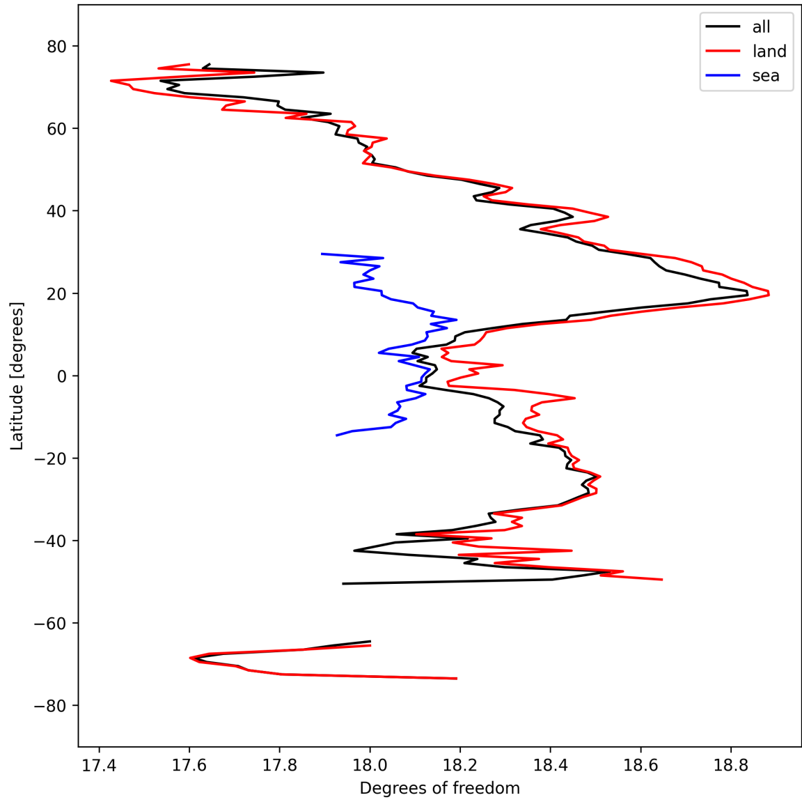
Figure 19: Zonal average of “Degrees of freedom” for 2024-09-20 to 2024-09-22.
