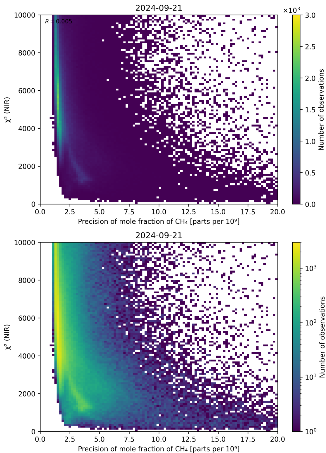
Figure 78: Scatter density plot of “Precision of mole fraction of \text{CH}_4 ” against “ \chi^2 (NIR)” for 2024-09-20 to 2024-09-22.
