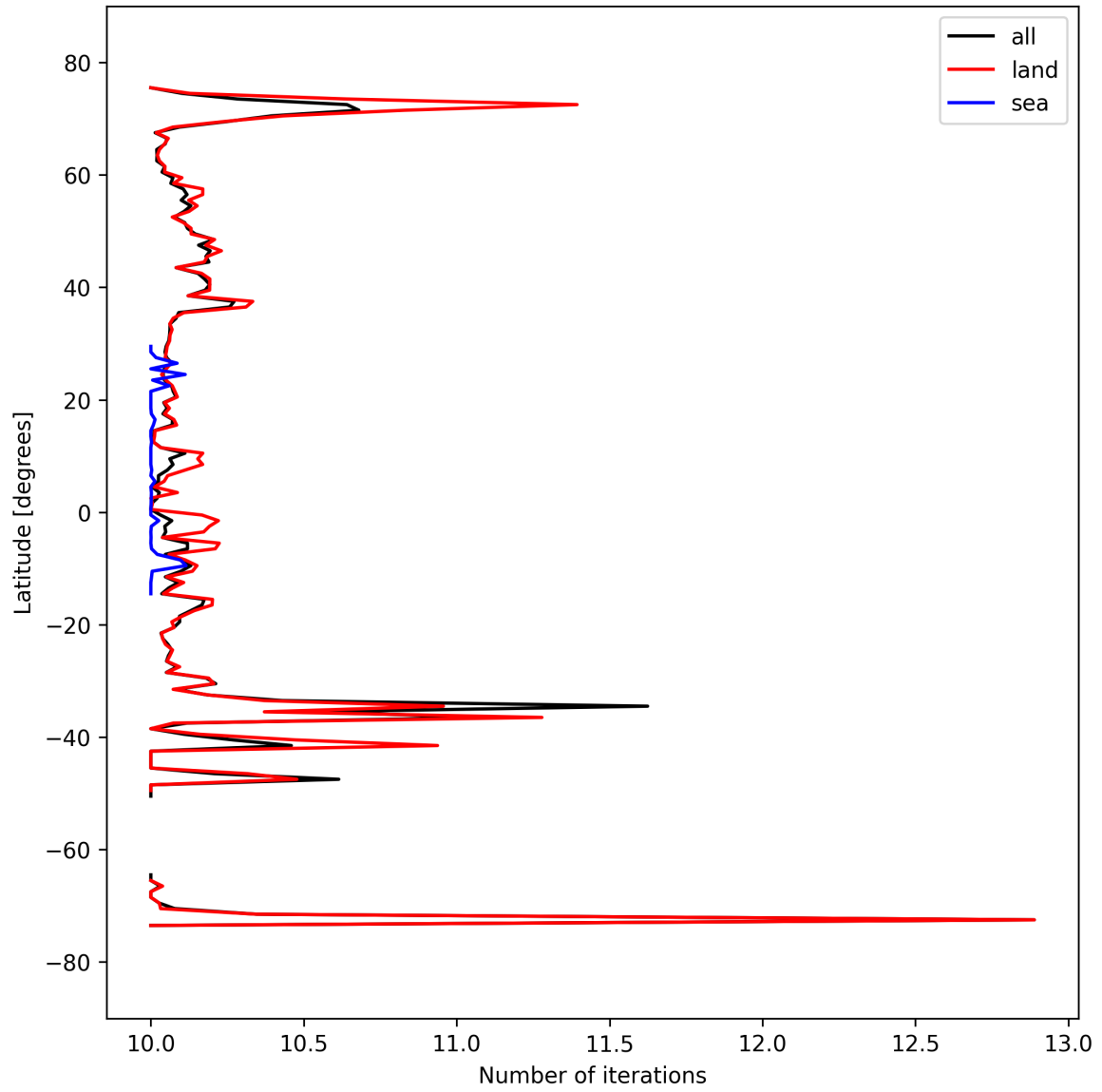
Figure 20: Zonal average of “Number of iterations” for 2024-09-20 to 2024-09-22.
