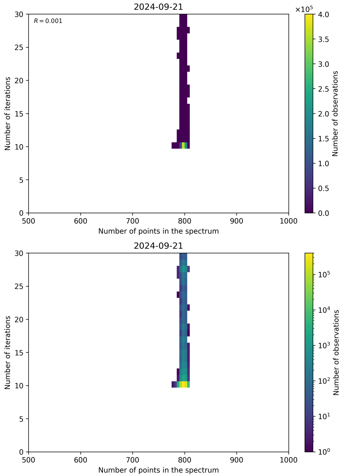
Figure 92: Scatter density plot of “Number of points in the spectrum” against “Number of iterations” for 2024-09-20 to 2024-09-22.
