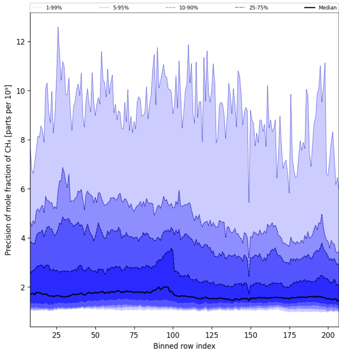
Figure 35: Along track statistics of “Precision of mole fraction of CH 4 ” for 2024-09-20 to 2024-09-22
