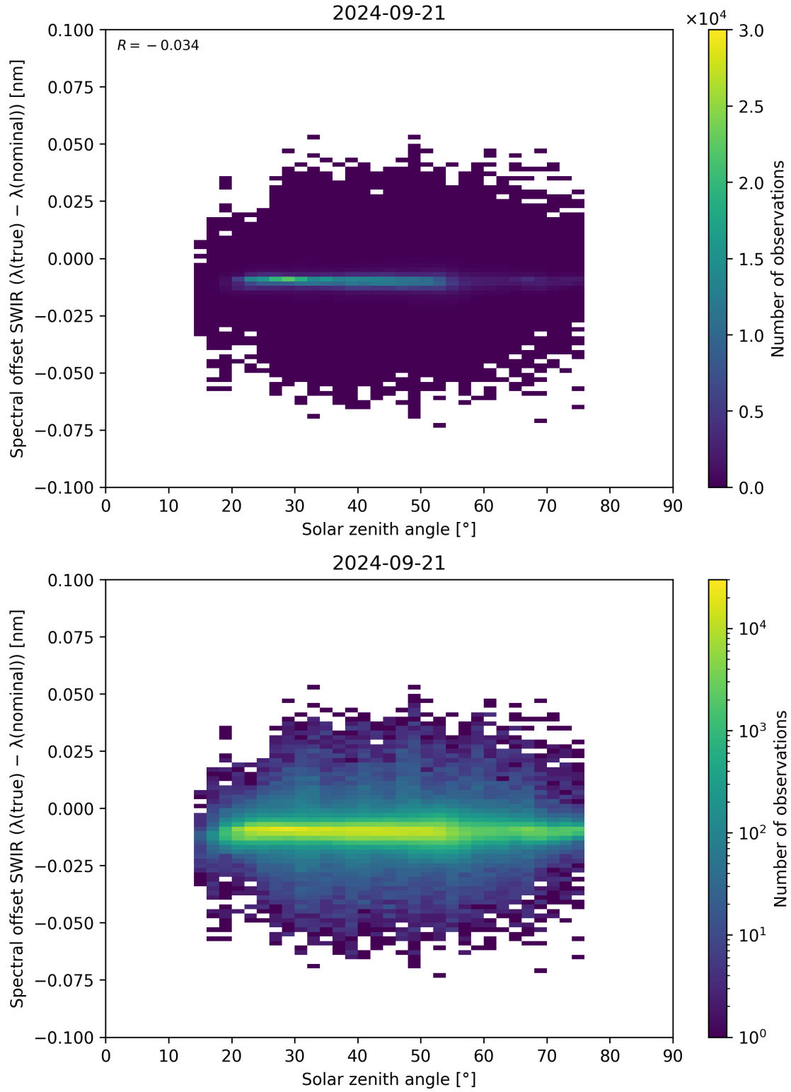
Figure 104: Scatter density plot of “Solar zenith angle” against “Spectral offset SWIR ( \lambda_{\text{true}} - \lambda_{\text{nominal}} )” for 2024-09-20 to 2024-09-22.
