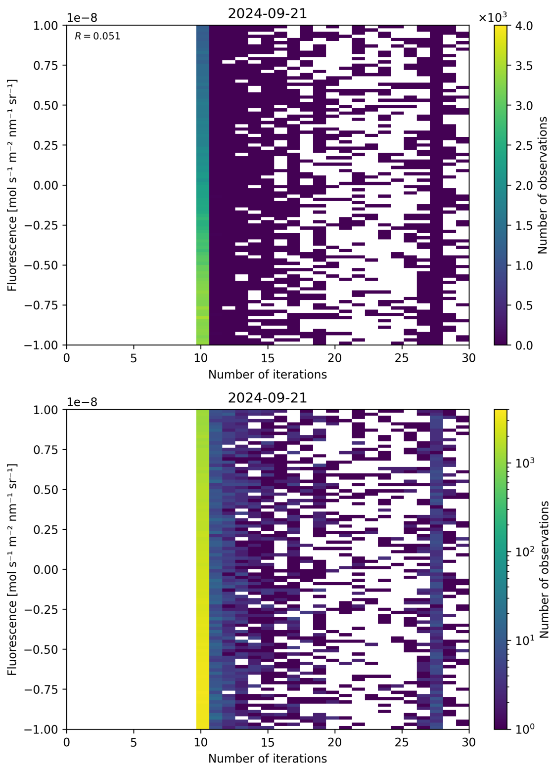
Figure 87: Scatter density plot of “Number of iterations” against “Fluorescence” for 2024-09-20 to 2024-09-22.
