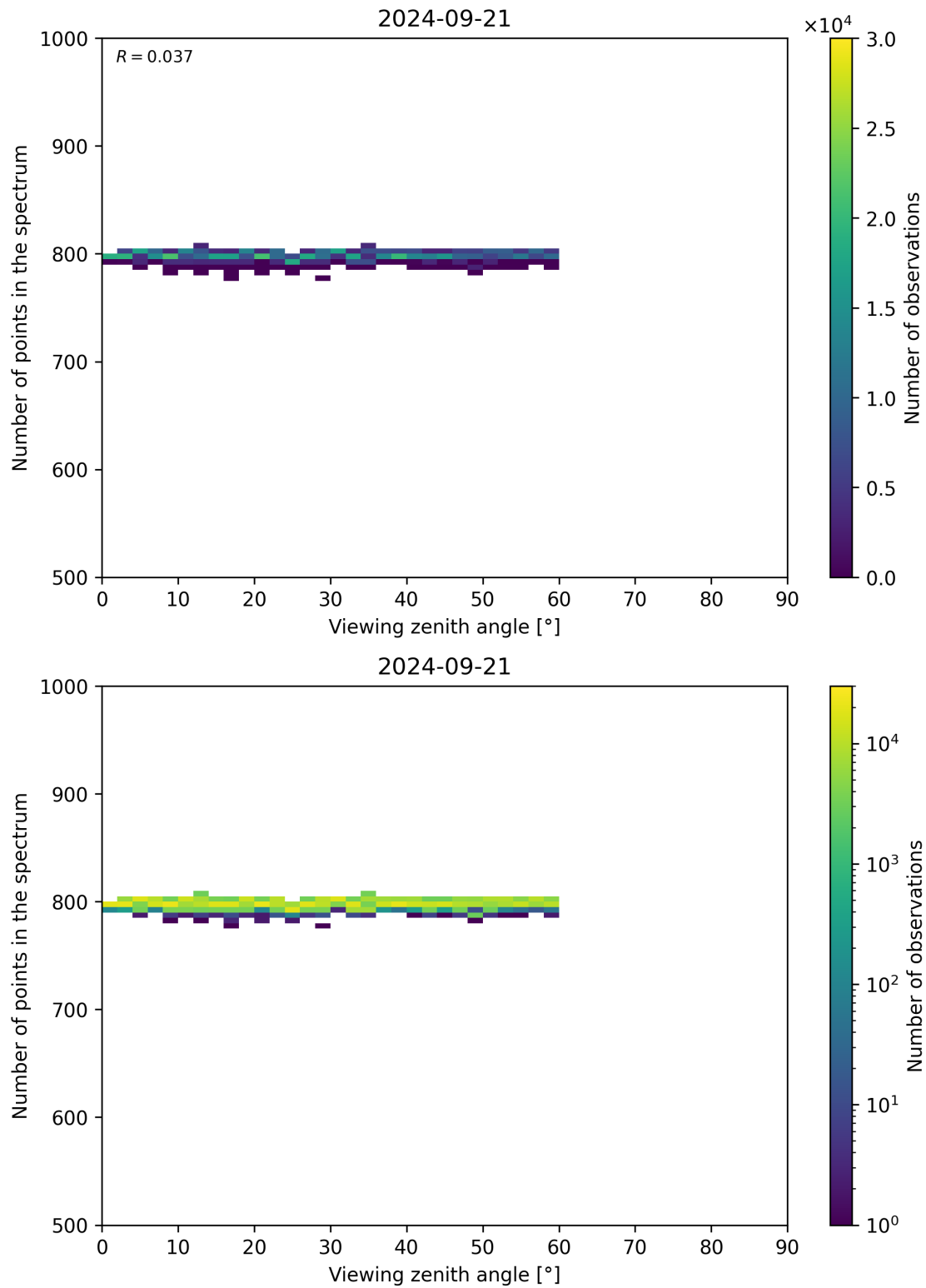
Figure 114: Scatter density plot of “Viewing zenith angle” against “Number of points in the spectrum” for 2024-09-20 to 2024-09-22.
