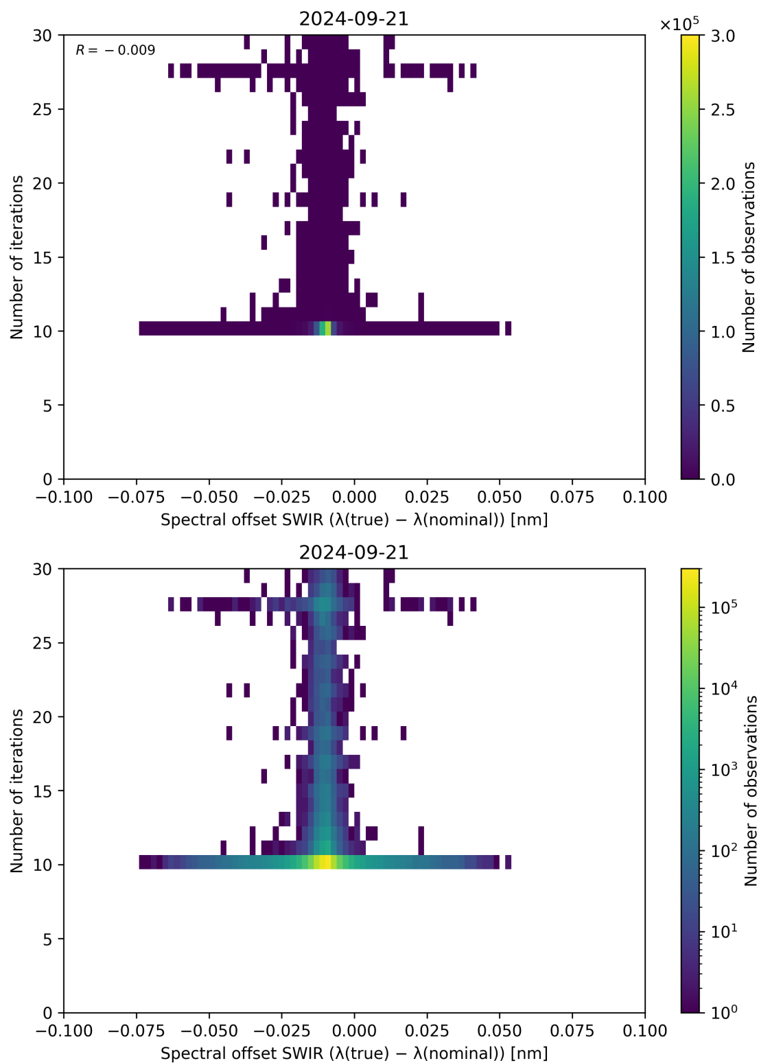
Figure 121: Scatter density plot of “Spectral offset SWIR ( \lambda_{\text{true}} - \lambda_{\text{nominal}} )” against “Number of iterations” for 2024-09-20 to 2024-09-22.
