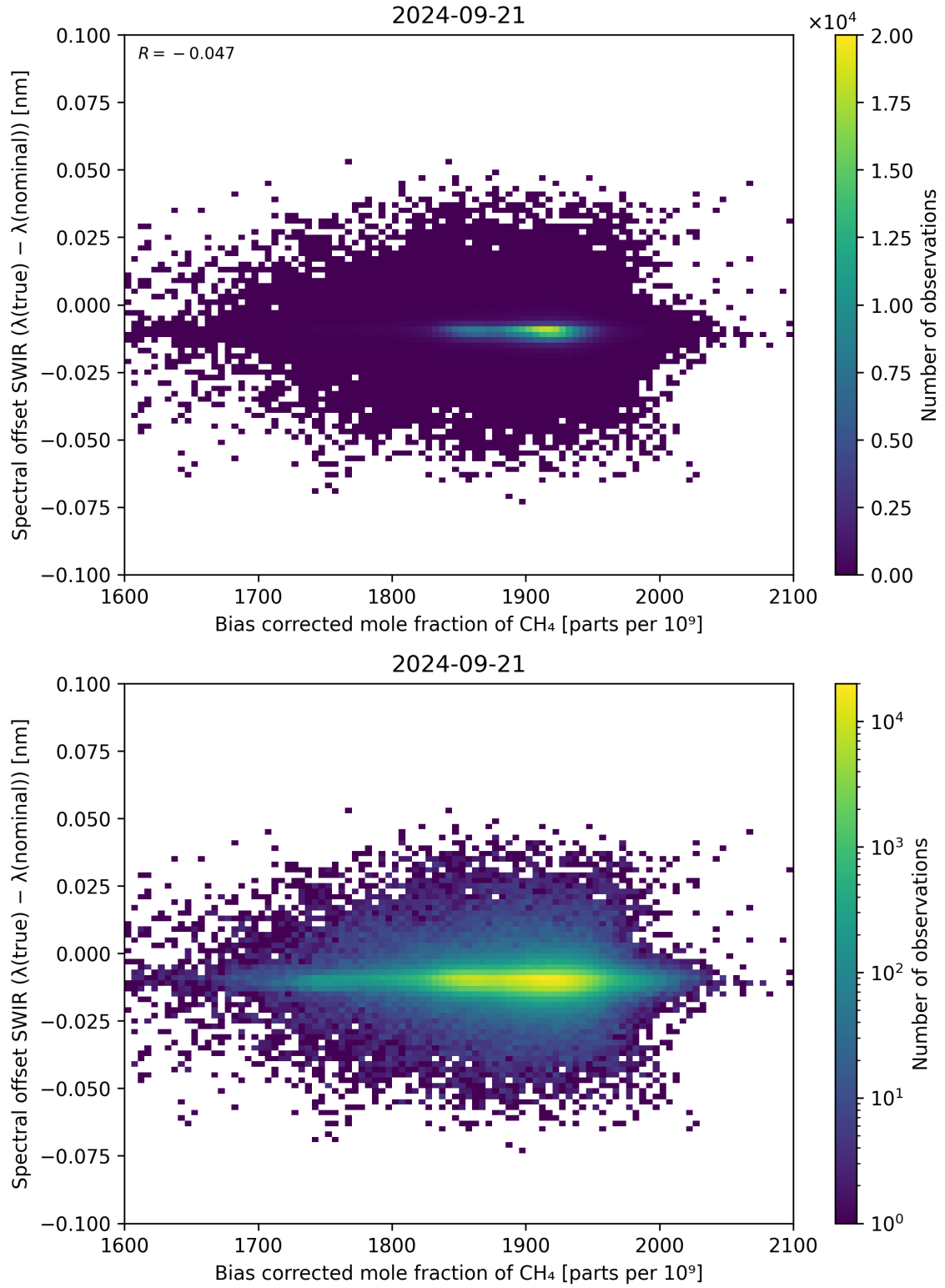
Figure 69: Scatter density plot of “Bias corrected mole fraction of \text{CH}_4 ” against “Spectral offset SWIR ( \lambda_{\text{true}} - \lambda_{\text{nominal}} )” for 2024-09-20 to 2024-09-22.
