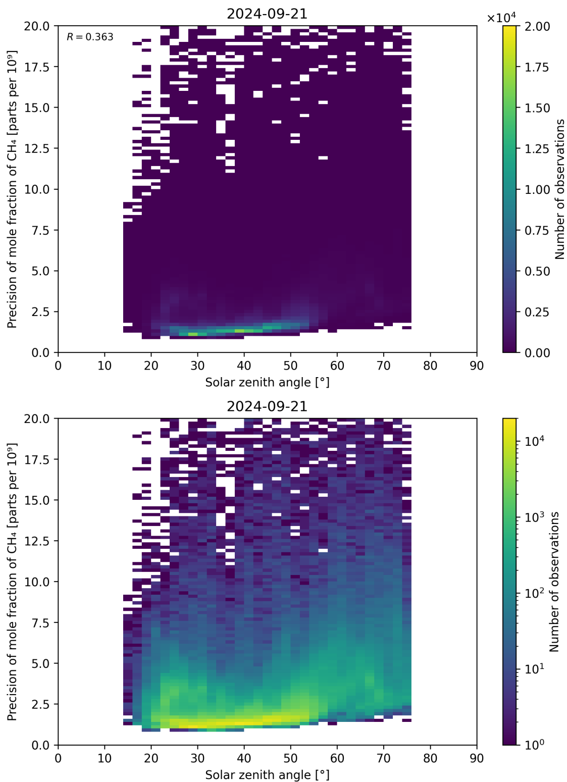
Figure 101: Scatter density plot of “Solar zenith angle” against “Precision of mole fraction of \text{CH}_4 ” for 2024-09-20 to 2024-09-22.
