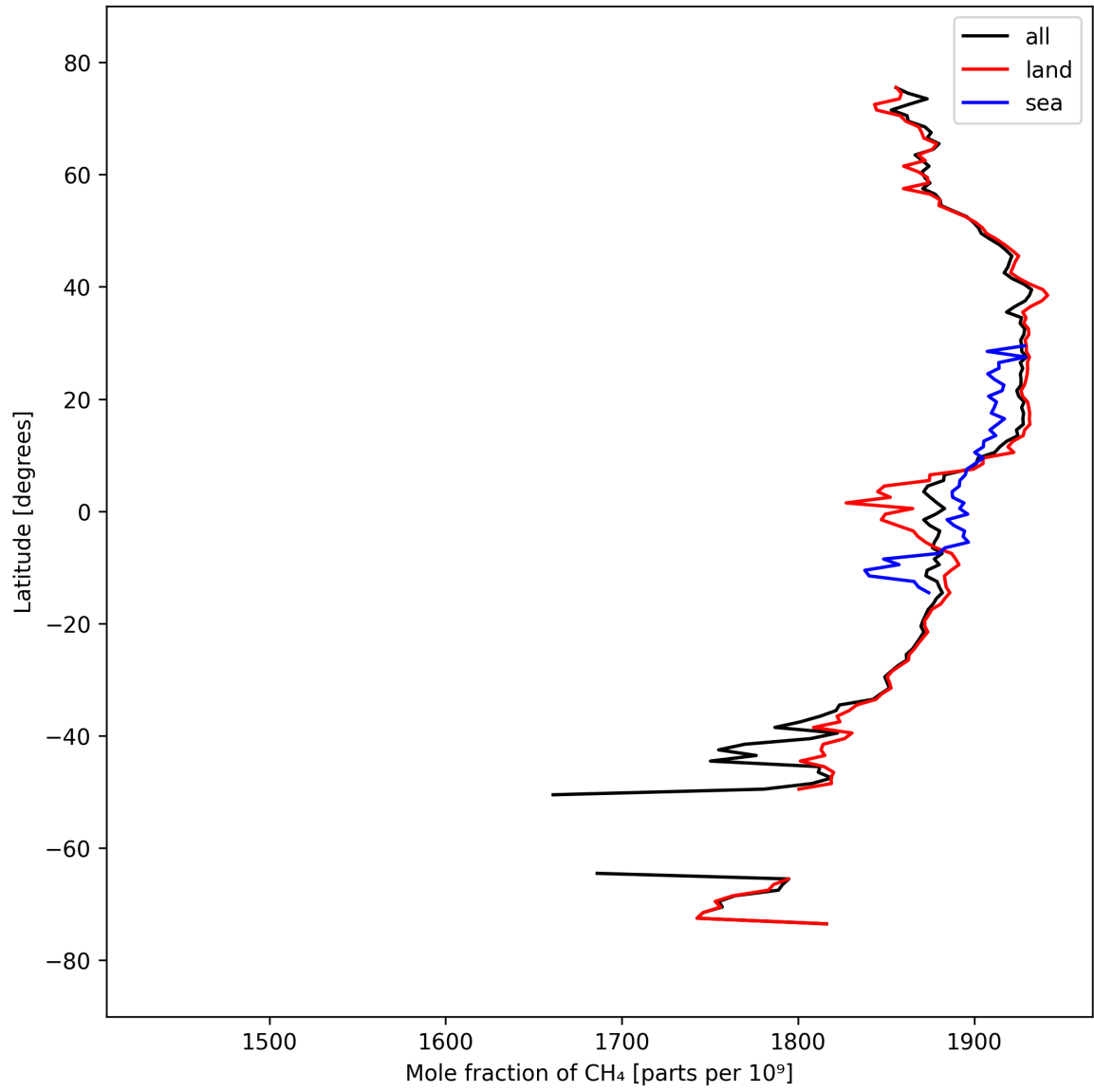
Figure 12: Zonal average of “Mole fraction of CH 4 ” for 2024-09-20 to 2024-09-22.
