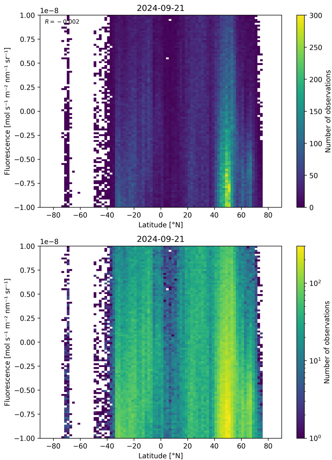
Figure 56: Scatter density plot of “Latitude” against “Fluorescence” for 2024-09-20 to 2024-09-22.
