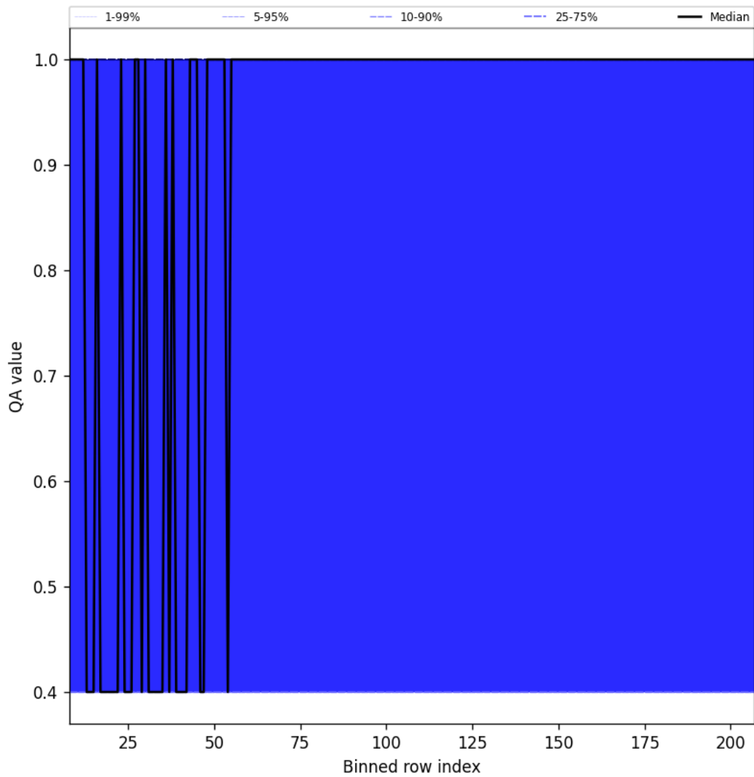
Figure 33: Along track statistics of “QA value” for 2024-09-20 to 2024-09-22
