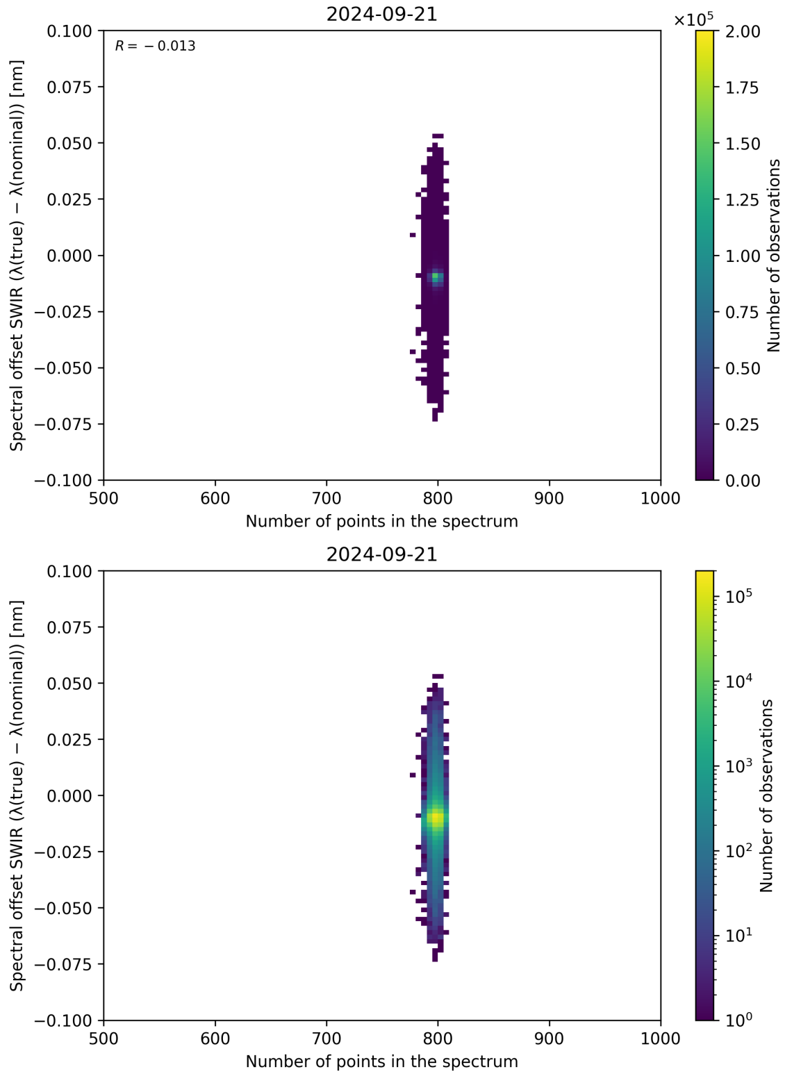
Figure 93: Scatter density plot of “Number of points in the spectrum” against “Spectral offset SWIR ( \lambda_{\text{true}} - \lambda_{\text{nominal}} )” for 2024-09-20 to 2024-09-22.
