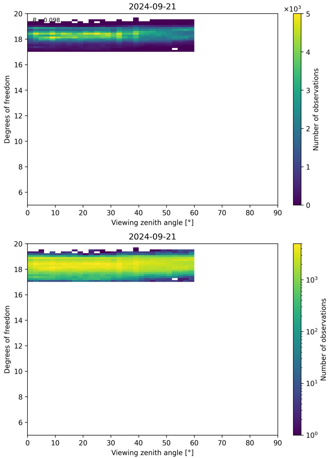
Figure 107: Scatter density plot of “Viewing zenith angle” against “Degrees of freedom” for 2024-09-20 to 2024-09-22.
