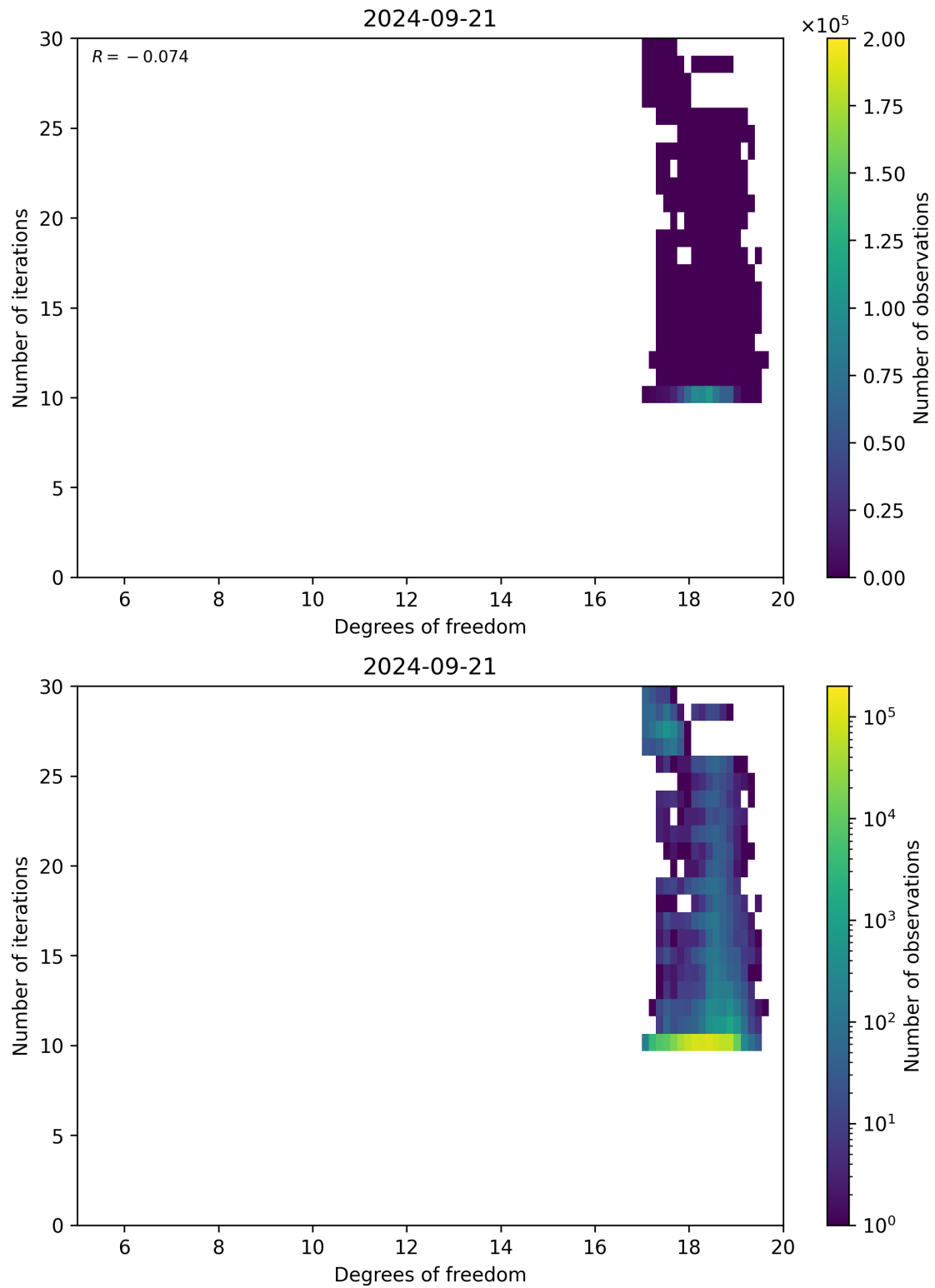
Figure 52: Scatter density plot of “Degrees of freedom” against “Number of iterations” for 2024-09-20 to 2024-09-22.
