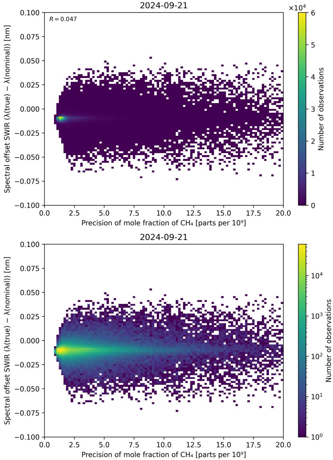
Figure 85: Scatter density plot of “Precision of mole fraction of \text{CH}_4 ” against “Spectral offset SWIR ( \lambda_{\text{true}} - \lambda_{\text{nominal}} )” for 2024-09-20 to 2024-09-22.
