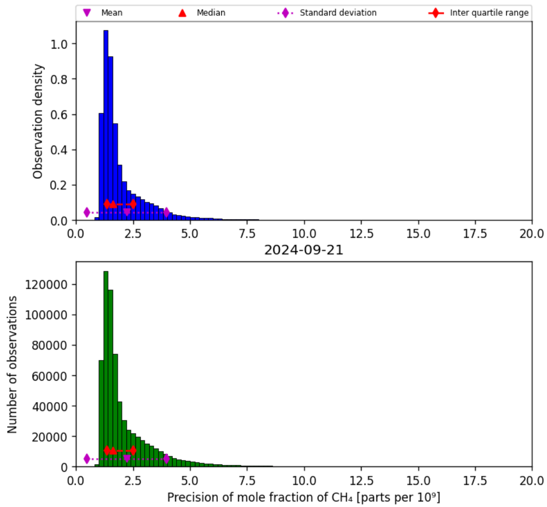
Figure 24: Histogram of “Precision of mole fraction of CH 4 ” for 2024-09-20 to 2024-09-22
