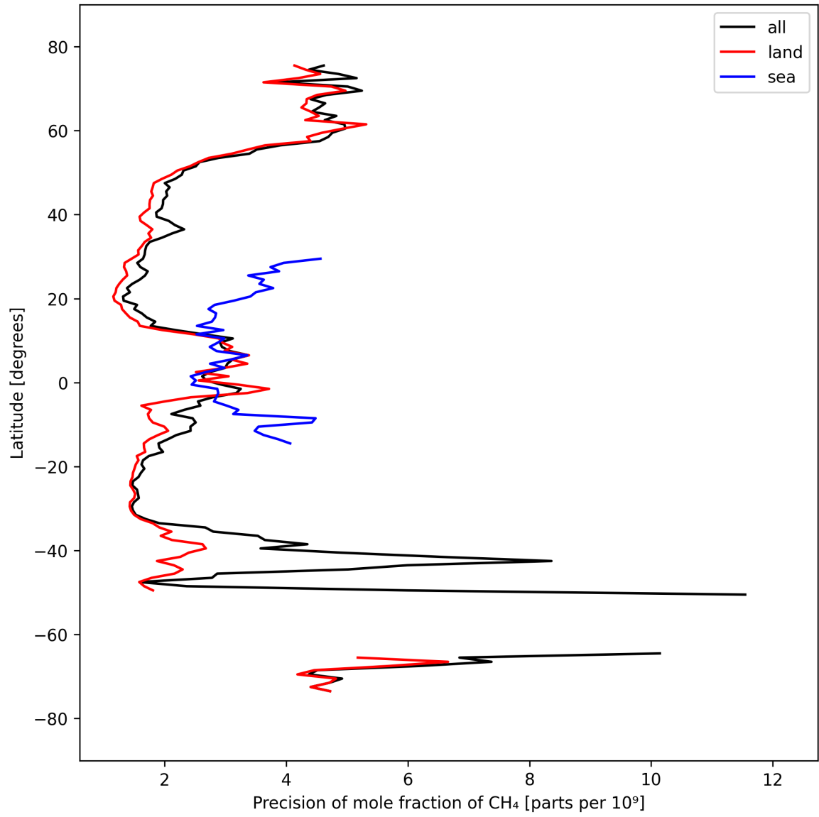
Figure 13: Zonal average of “Precision of mole fraction of CH 4 ” for 2024-09-20 to 2024-09-22.
