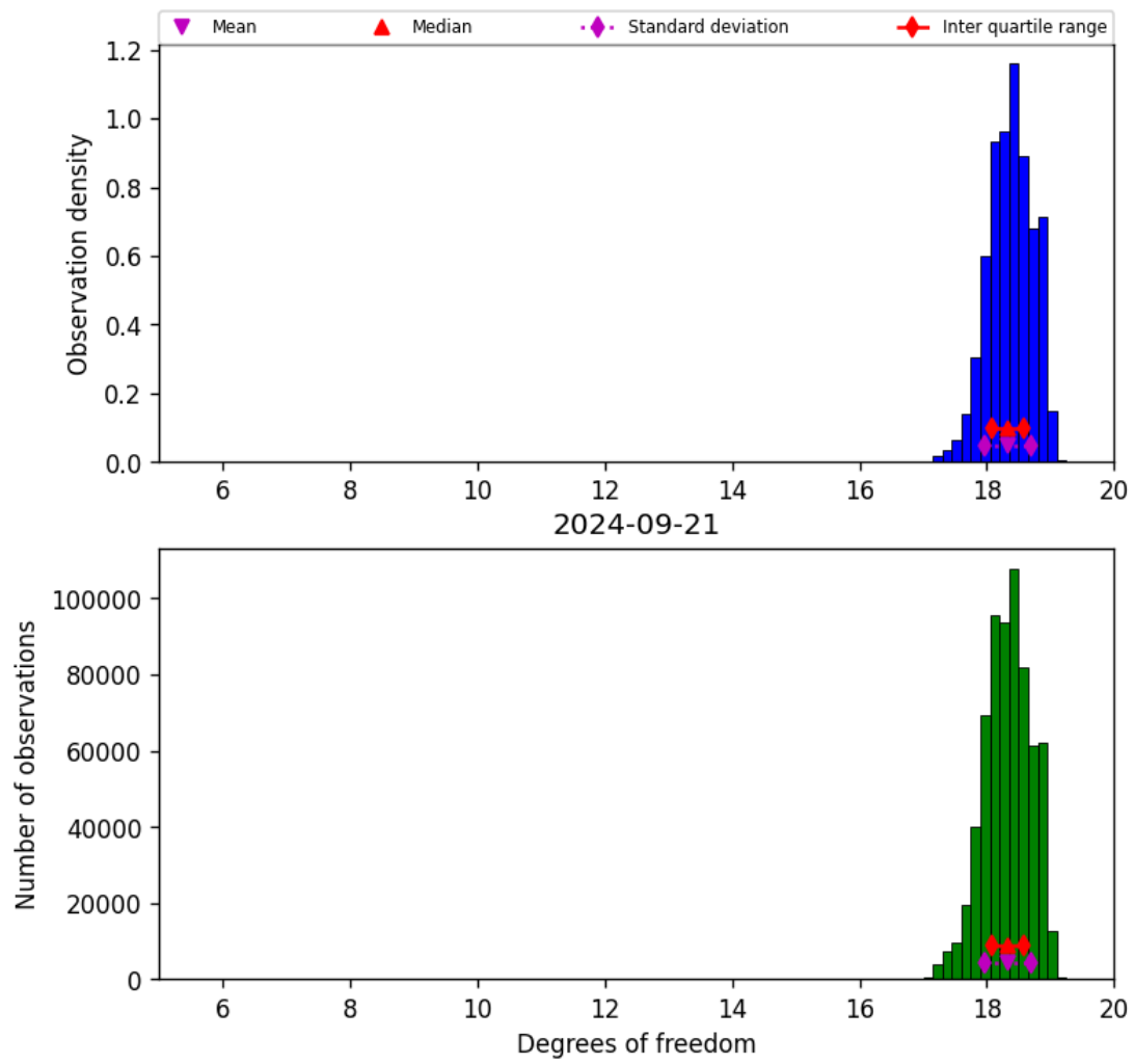
Figure 30: Histogram of “Degrees of freedom” for 2024-09-20 to 2024-09-22
