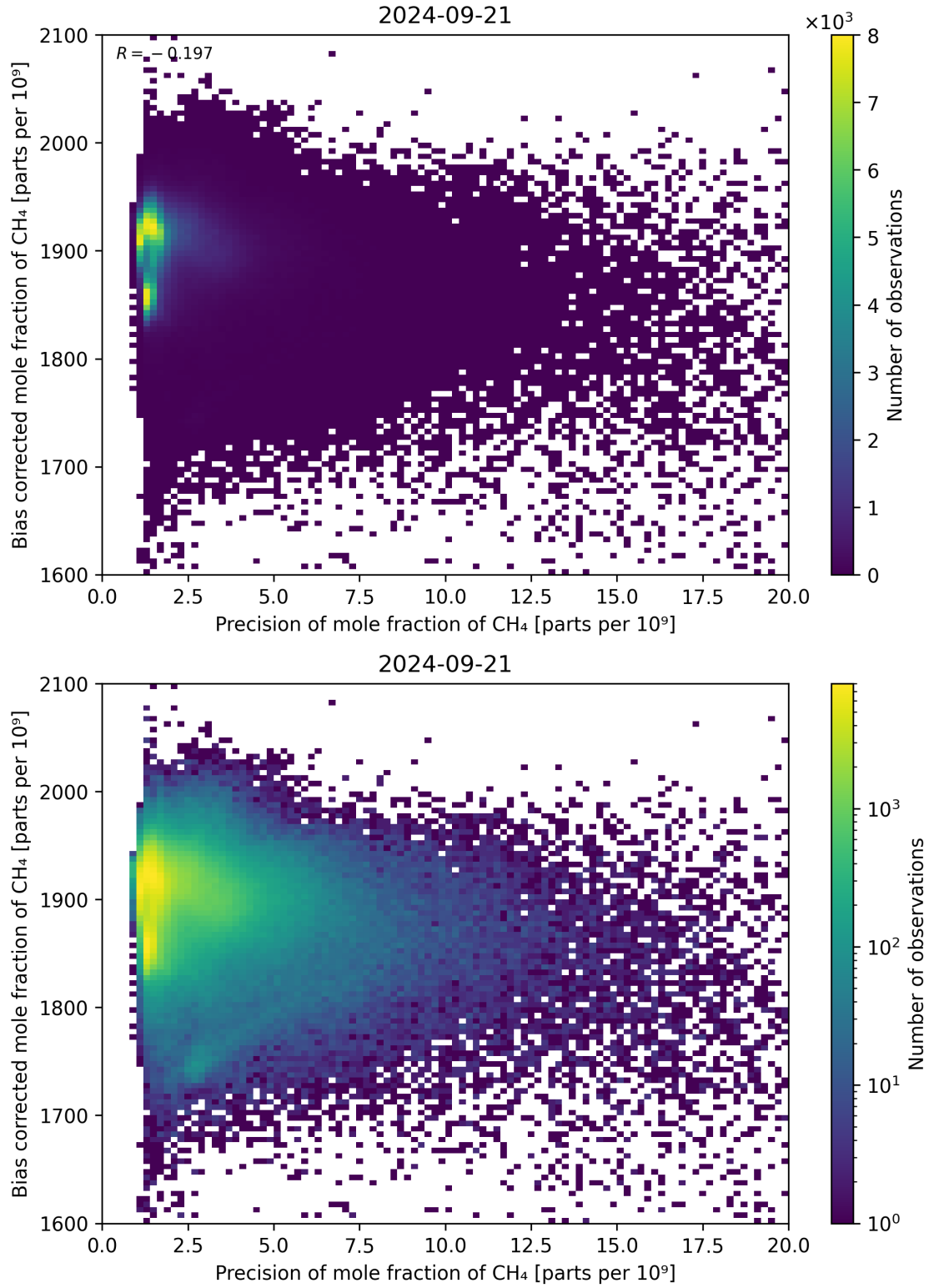
Figure 82: Scatter density plot of “Precision of mole fraction of CH 4 ” against “Bias corrected mole fraction of CH 4 ” for 2024-09-20 to 2024-09-22.
