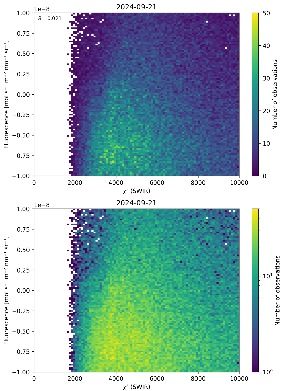
Figure 49: Scatter density plot of “ \chi^2 (SWIR)” against “Fluorescence” for 2024-09-20 to 2024-09-22.
