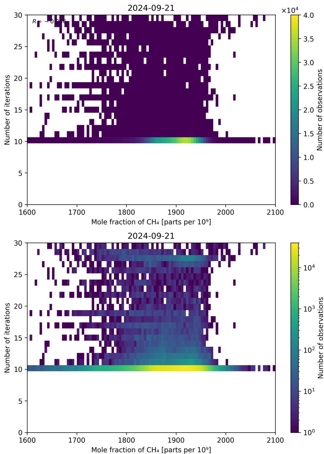
Figure 76: Scatter density plot of “Mole fraction of CH 4 ” against “Number of iterations” for 2024-09-20 to 2024-09-22.
