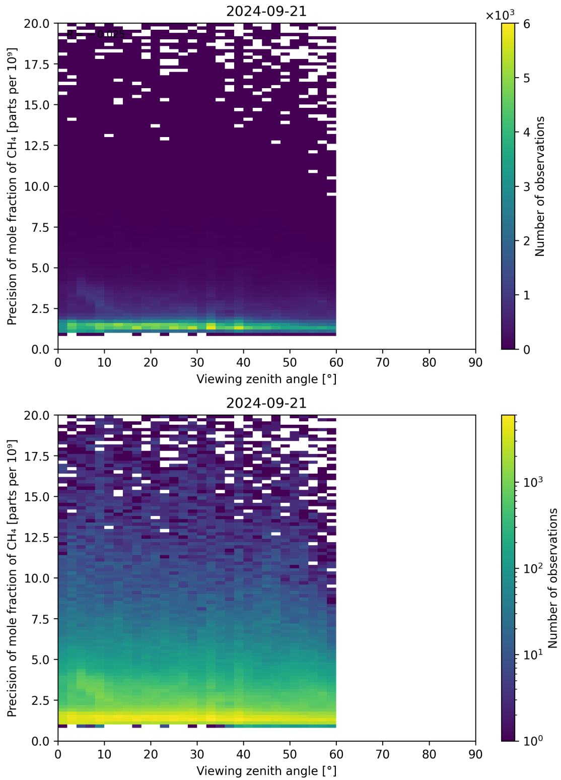
Figure 112: Scatter density plot of “Viewing zenith angle” against “Precision of mole fraction of CH 4 ” for 2024-09-20 to 2024-09-22.
