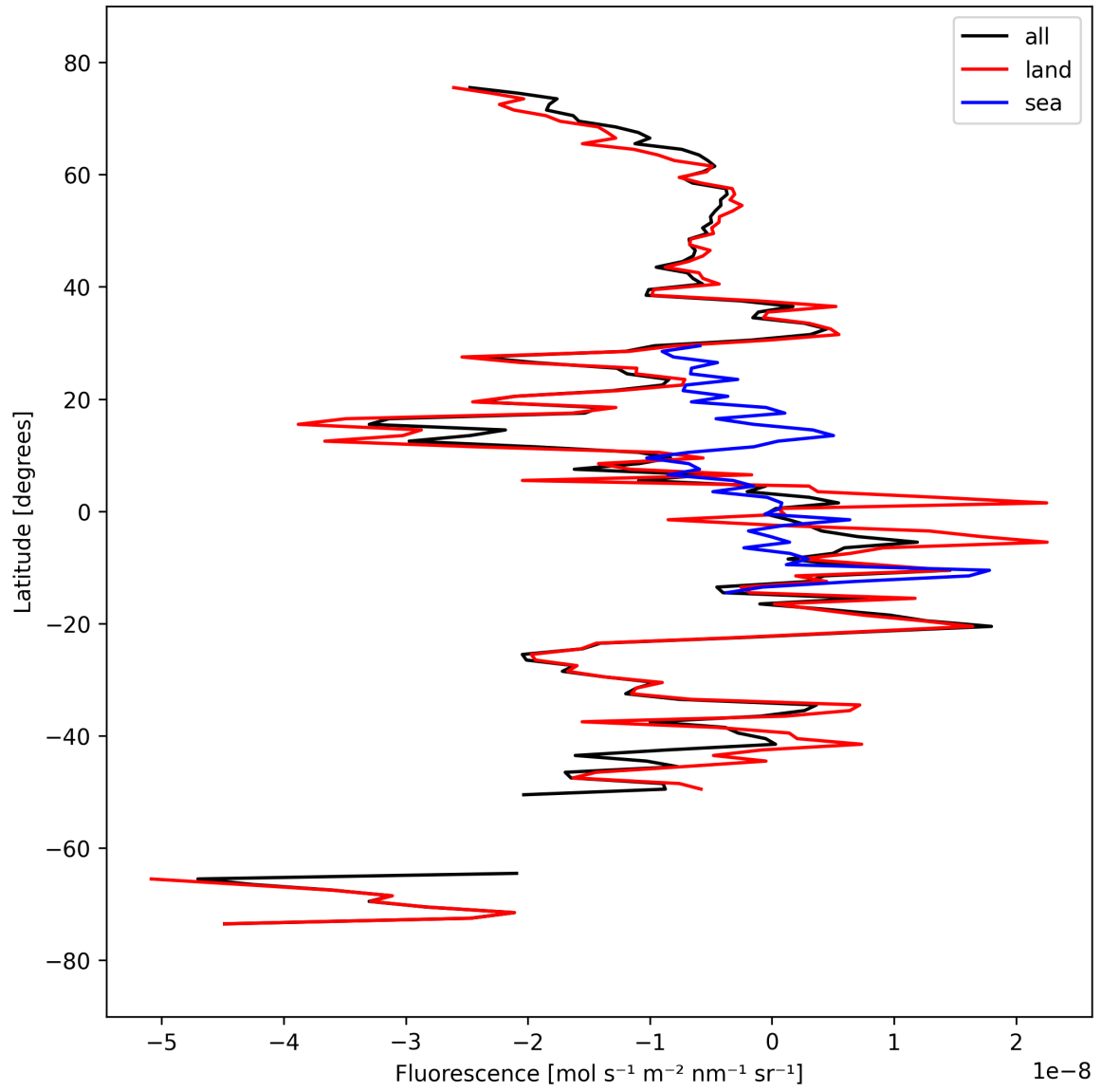
Figure 21: Zonal average of “Fluorescence” for 2024-09-20 to 2024-09-22.
