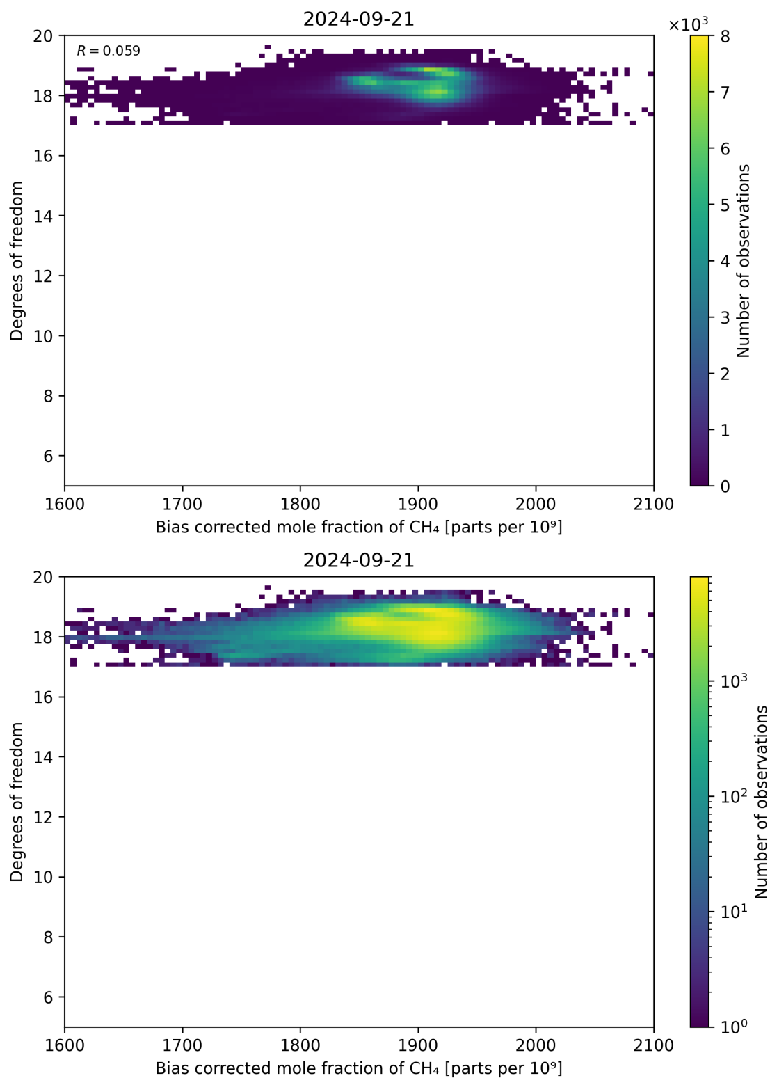
Figure 65: Scatter density plot of “Bias corrected mole fraction of CH 4 ” against “Degrees of freedom” for 2024-09-20 to 2024-09-22.
