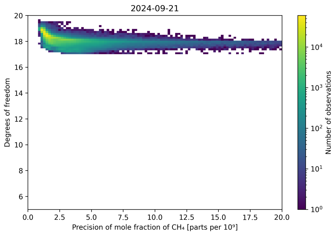
Figure 80: Scatter density plot of “Precision of mole fraction of CH 4 ” against “Degrees of freedom” for 2024-09-20 to 2024-09-22.
