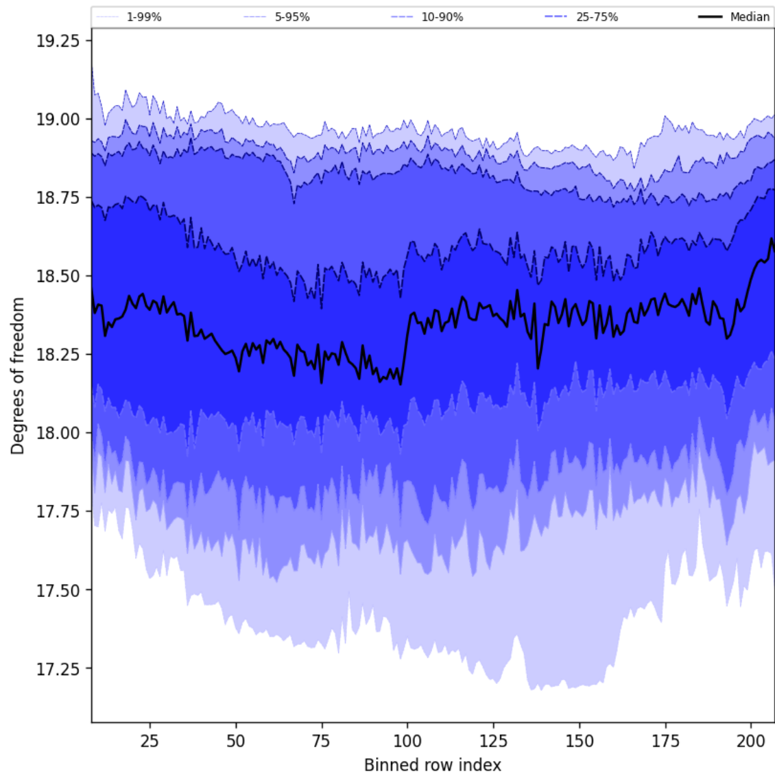
Figure 41: Along track statistics of “Degrees of freedom” for 2024-09-20 to 2024-09-22
