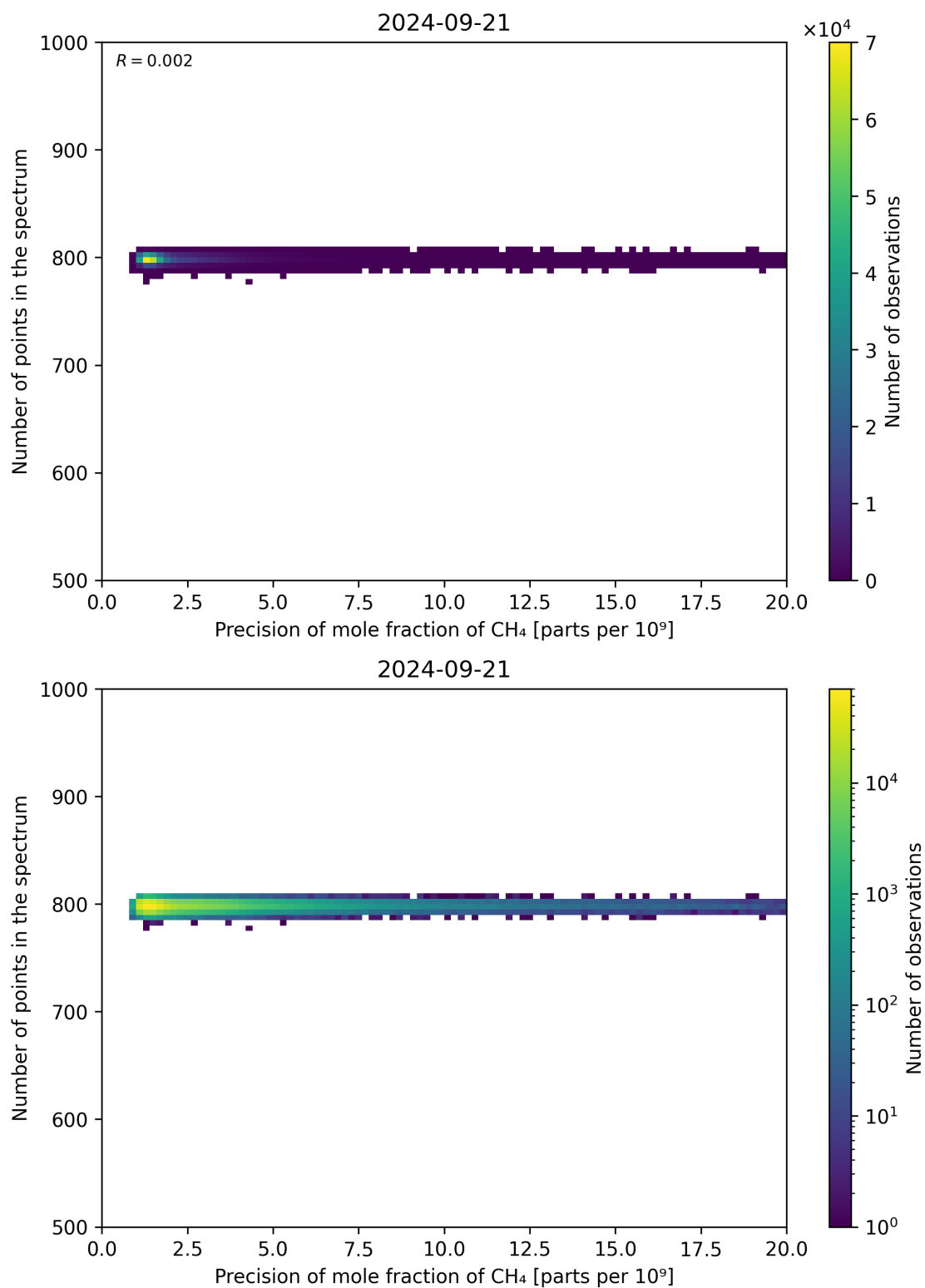
Figure 84: Scatter density plot of “Precision of mole fraction of CH 4 ” against “Number of points in the spectrum” for 2024-09-20 to 2024-09-22.
