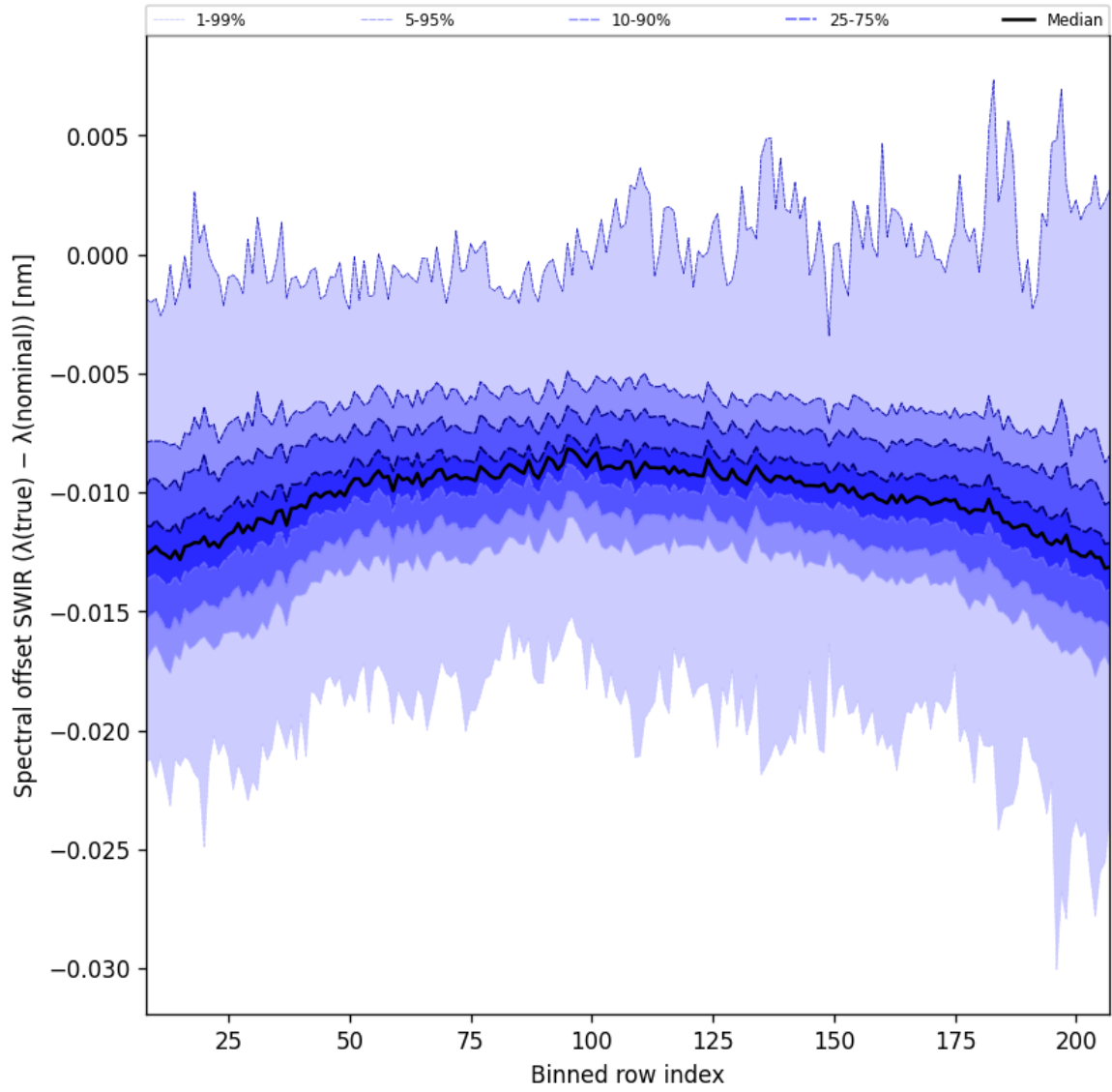
Figure 38: Along track statistics of “Spectral offset SWIR ( \lambda_{\text{true}} - \lambda_{\text{nominal}} )” for 2024-09-20 to 2024-09-22
