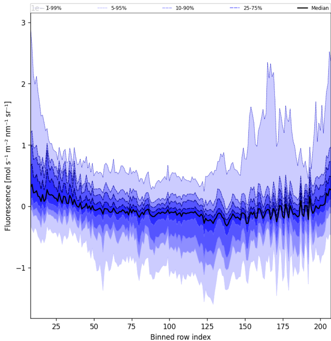
Figure 43: Along track statistics of “Fluorescence” for 2024-09-20 to 2024-09-22
