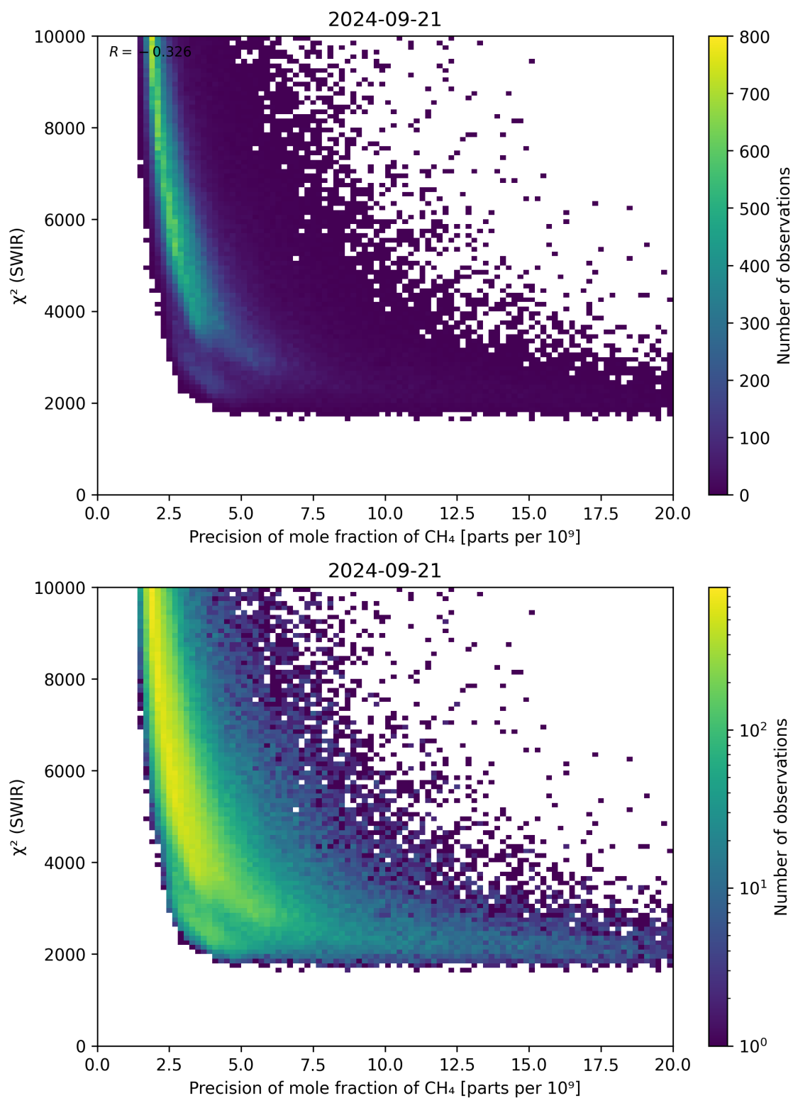
Figure 79: Scatter density plot of “Precision of mole fraction of \text{CH}_4 ” against “ \chi^2 (SWIR)” for 2024-09-20 to 2024-09-22.
