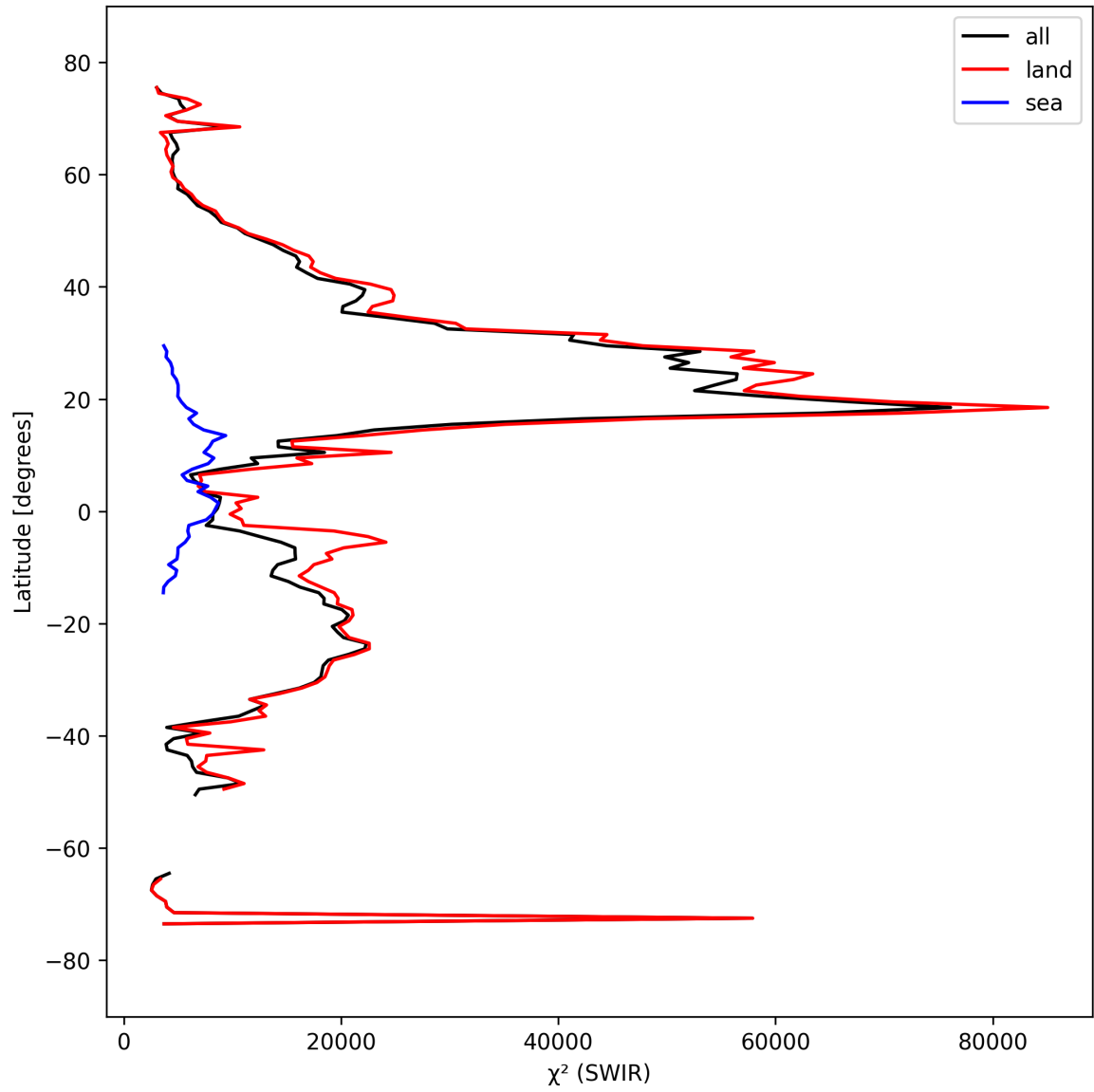
Figure 17: Zonal average of “ \chi^2 (SWIR)” for 2024-09-20 to 2024-09-22.
