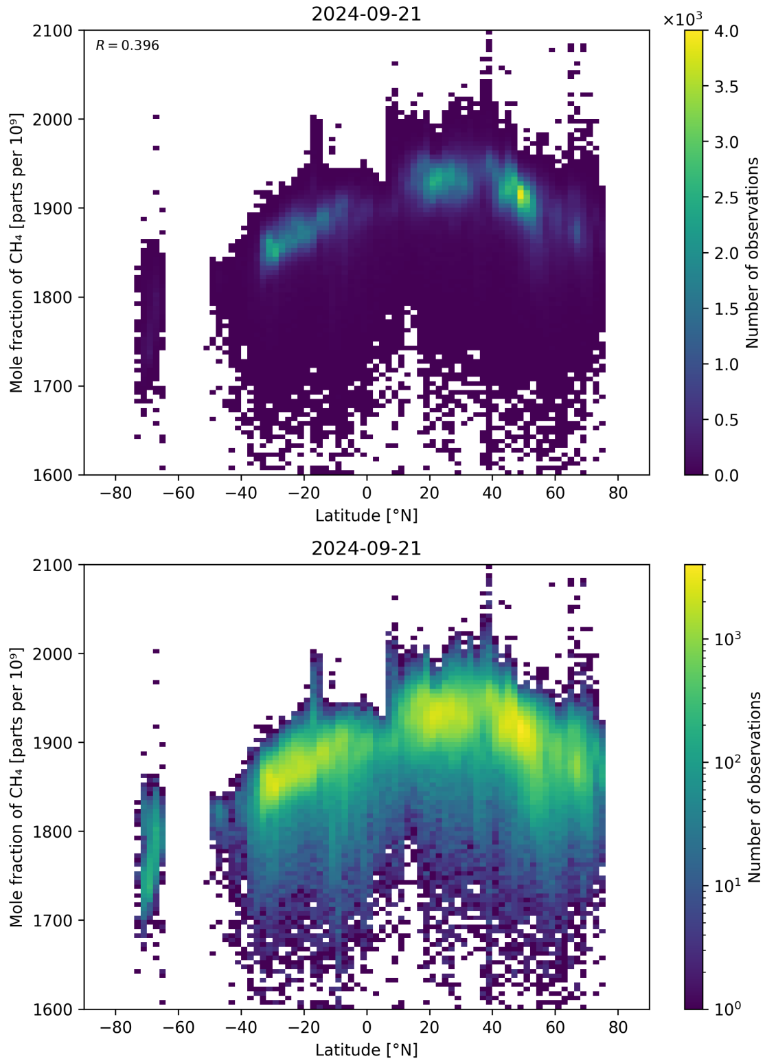
Figure 57: Scatter density plot of “Latitude” against “Mole fraction of CH 4 ” for 2024-09-20 to 2024-09-22.
