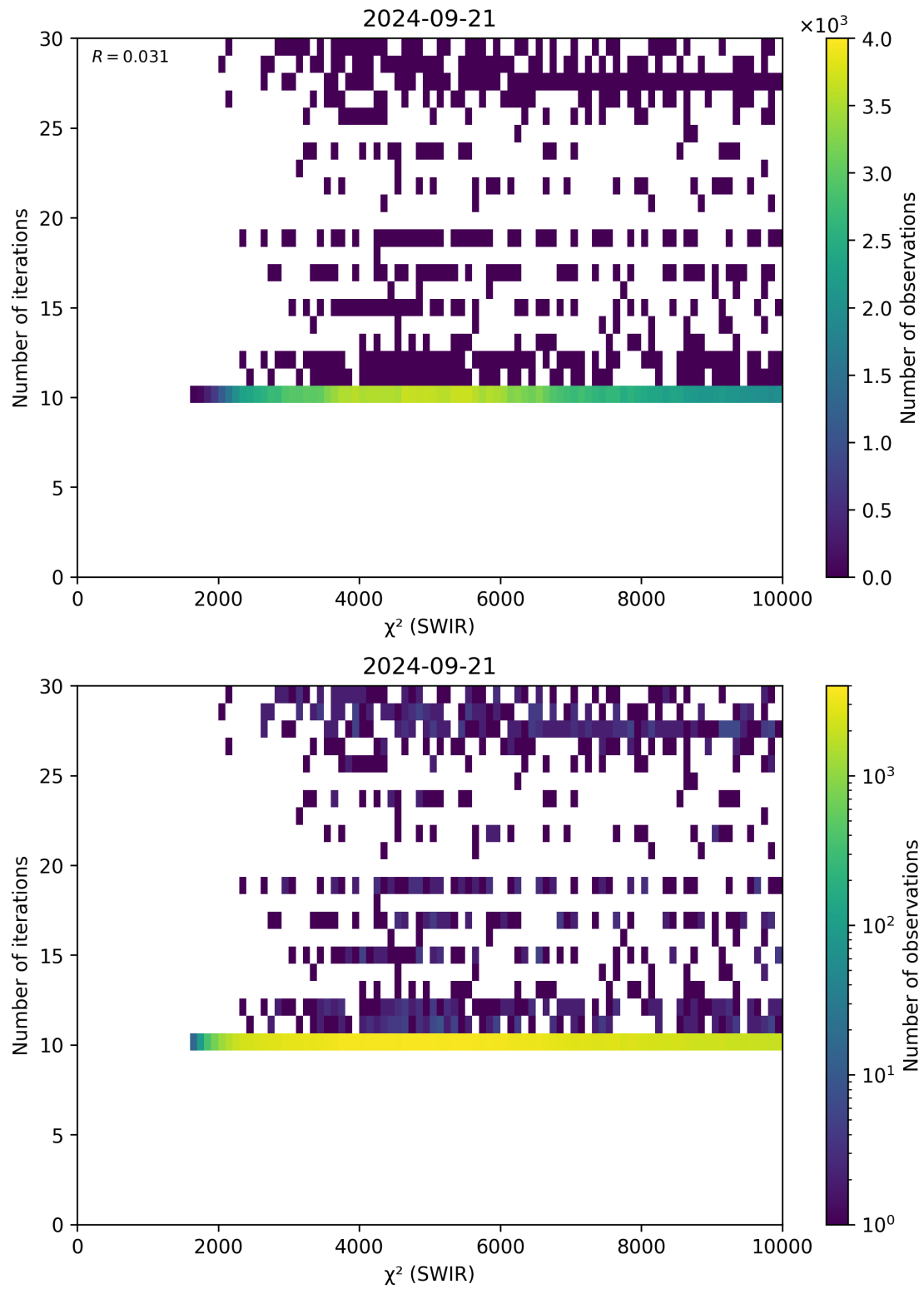
Figure 50: Scatter density plot of “ \chi^2 (SWIR)” against “Number of iterations” for 2024-09-20 to 2024-09-22.
