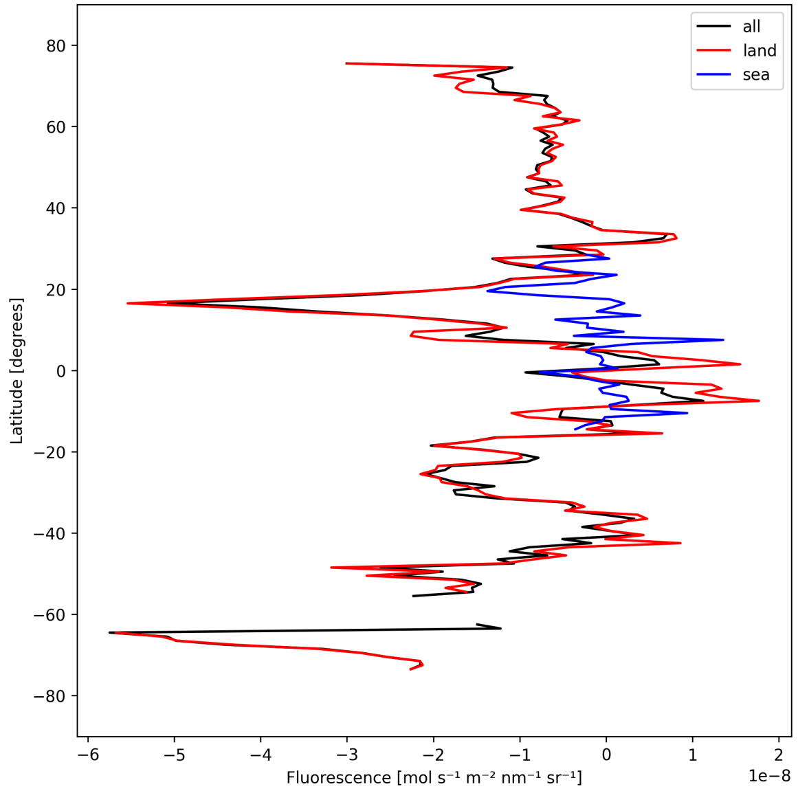
Figure 21: Zonal average of “Fluorescence” for 2024-09-22 to 2024-09-23.
