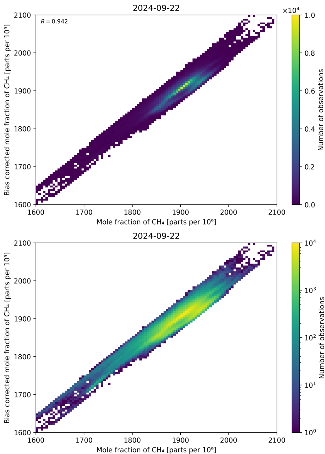
Figure 74: Scatter density plot of “Mole fraction of CH 4 ” against “Bias corrected mole fraction of CH 4 ” for 2024-09-22 to 2024-09-23.
