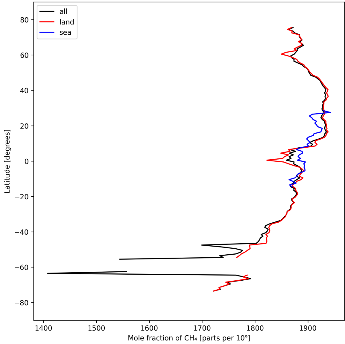
Figure 12: Zonal average of “Mole fraction of CH 4 ” for 2024-09-22 to 2024-09-23.
