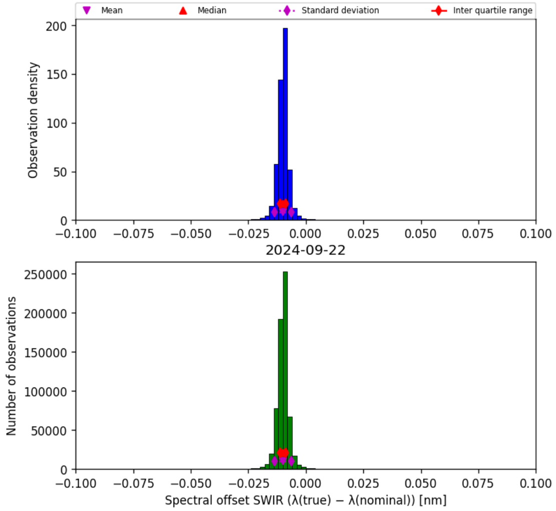
Figure 27: Histogram of “Spectral offset SWIR ( \lambda_{\text{true}} - \lambda_{\text{nominal}} )” for 2024-09-22 to 2024-09-23
