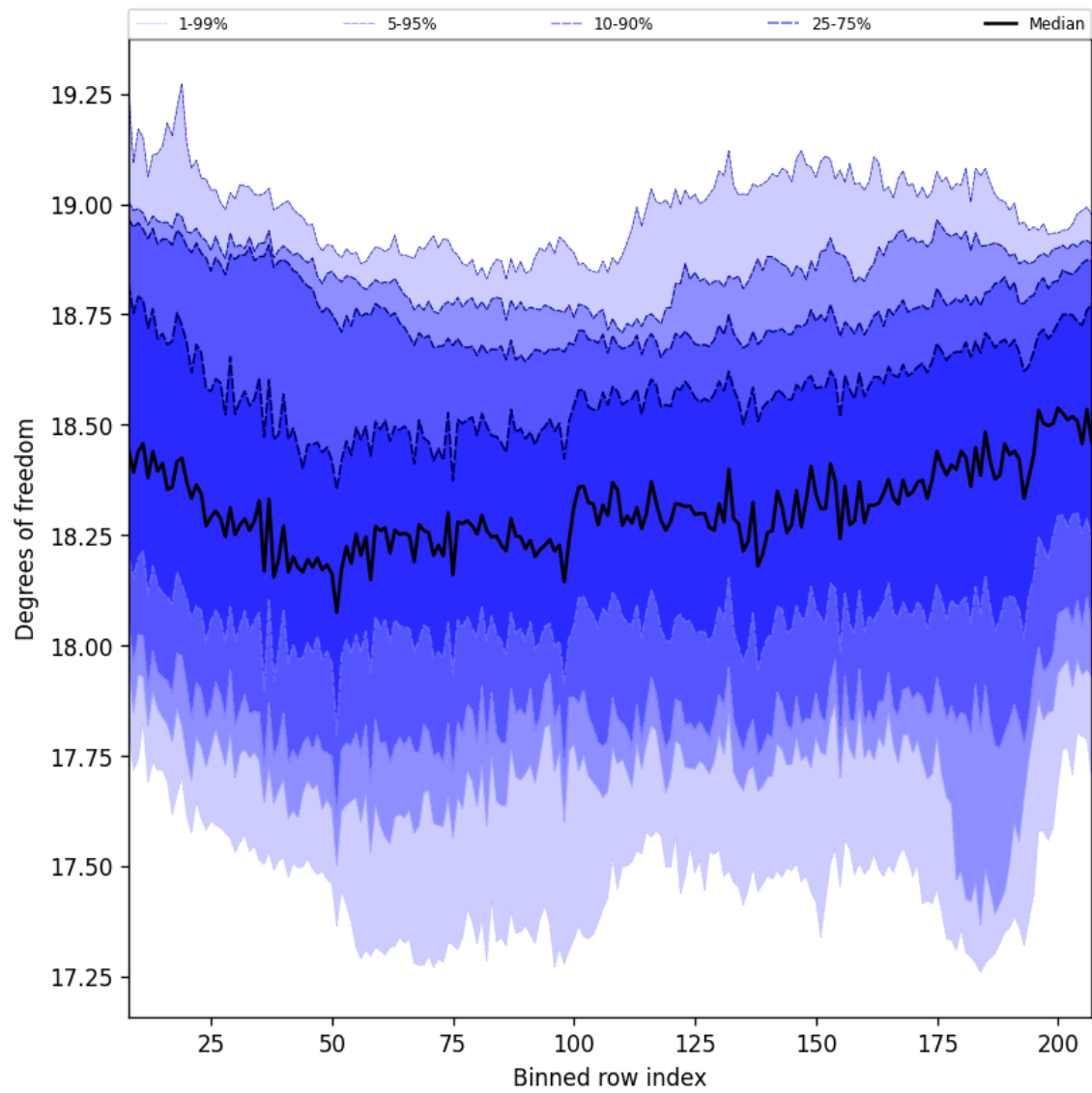
Figure 41: Along track statistics of “Degrees of freedom” for 2024-09-22 to 2024-09-23
