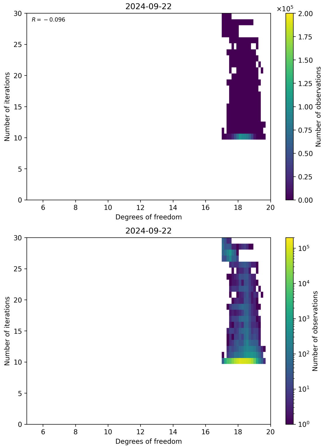
Figure 52: Scatter density plot of “Degrees of freedom” against “Number of iterations” for 2024-09-22 to 2024-09-23.
