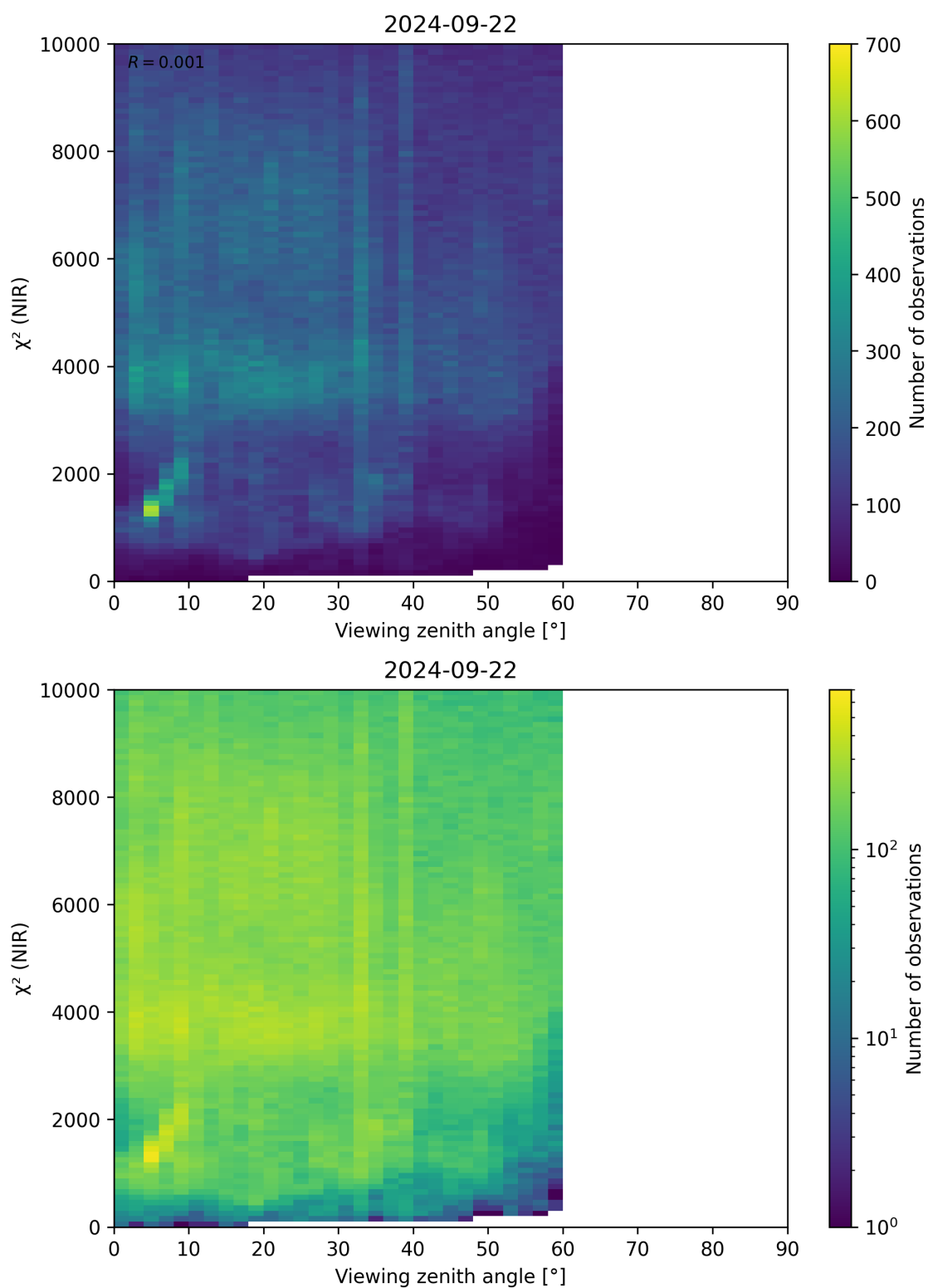
Figure 105: Scatter density plot of “Viewing zenith angle” against “ \chi^2 (NIR)” for 2024-09-22 to 2024-09-23.
