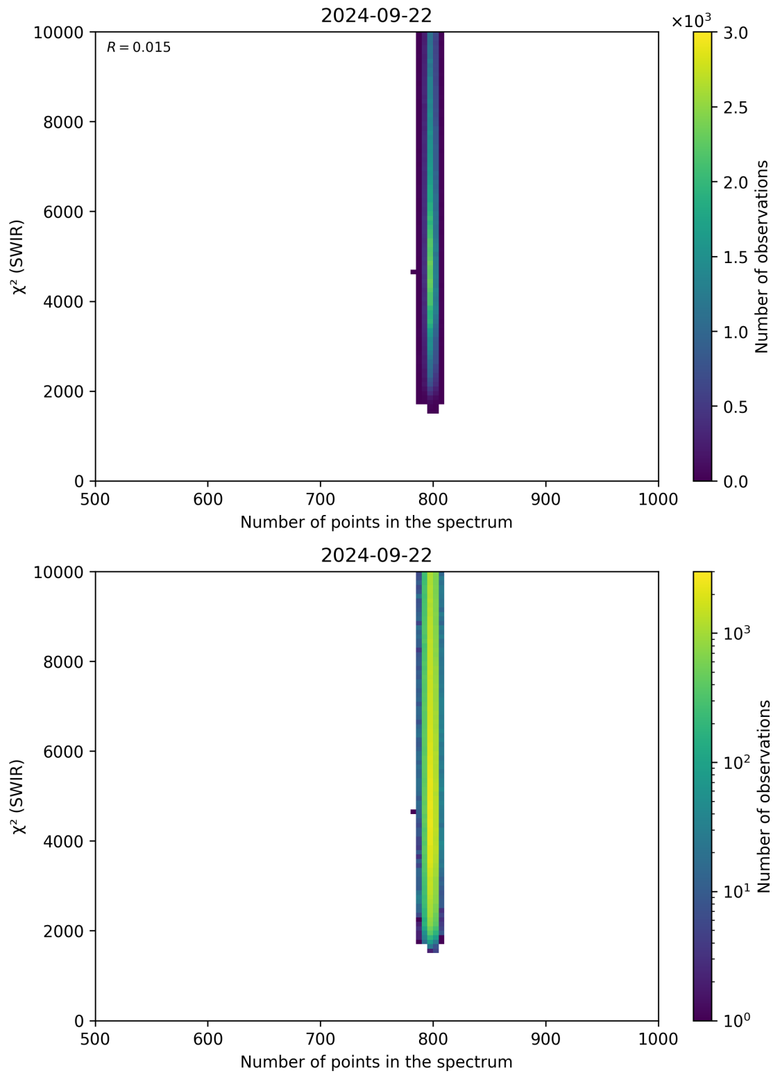
Figure 89: Scatter density plot of “Number of points in the spectrum” against “ \chi^2 (SWIR)” for 2024-09-22 to 2024-09-23.
