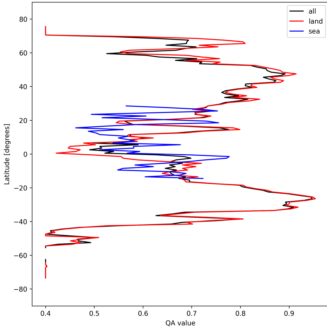
Figure 11: Zonal average of “QA value” for 2024-09-22 to 2024-09-23.
