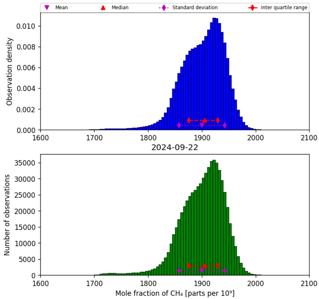
Figure 23: Histogram of “Mole fraction of CH 4 ” for 2024-09-22 to 2024-09-23
