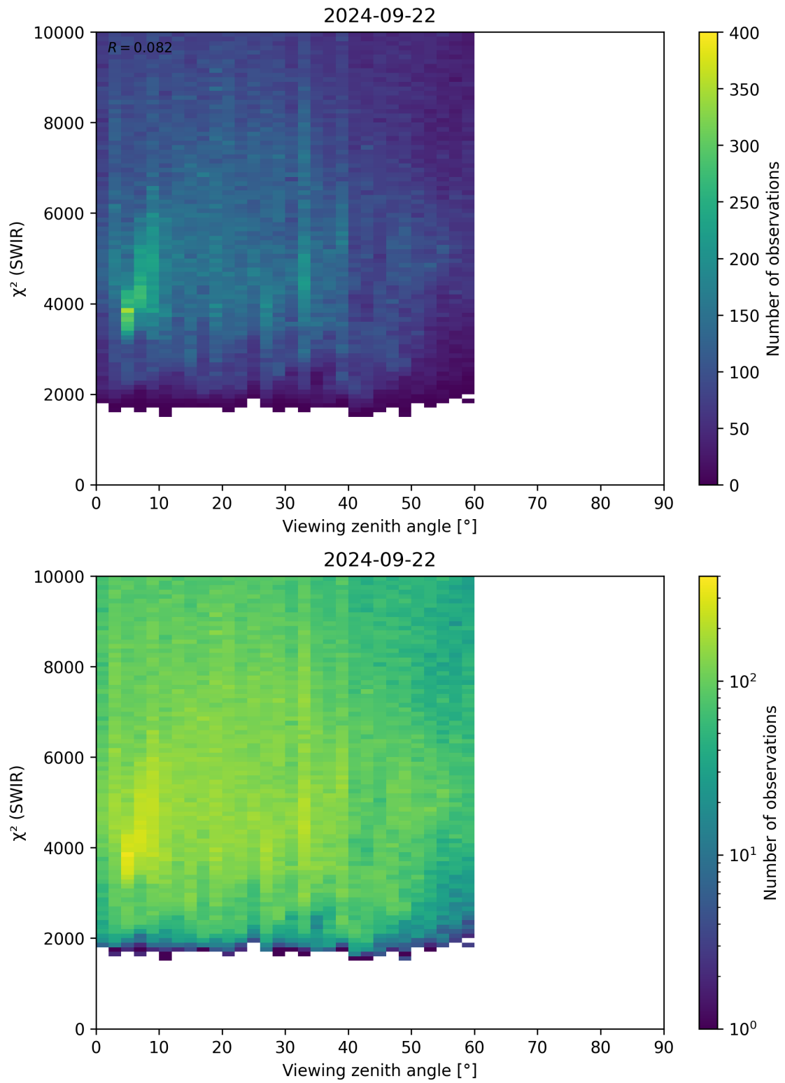
Figure 106: Scatter density plot of “Viewing zenith angle” against “ \chi^2 (SWIR)” for 2024-09-22 to 2024-09-23.
