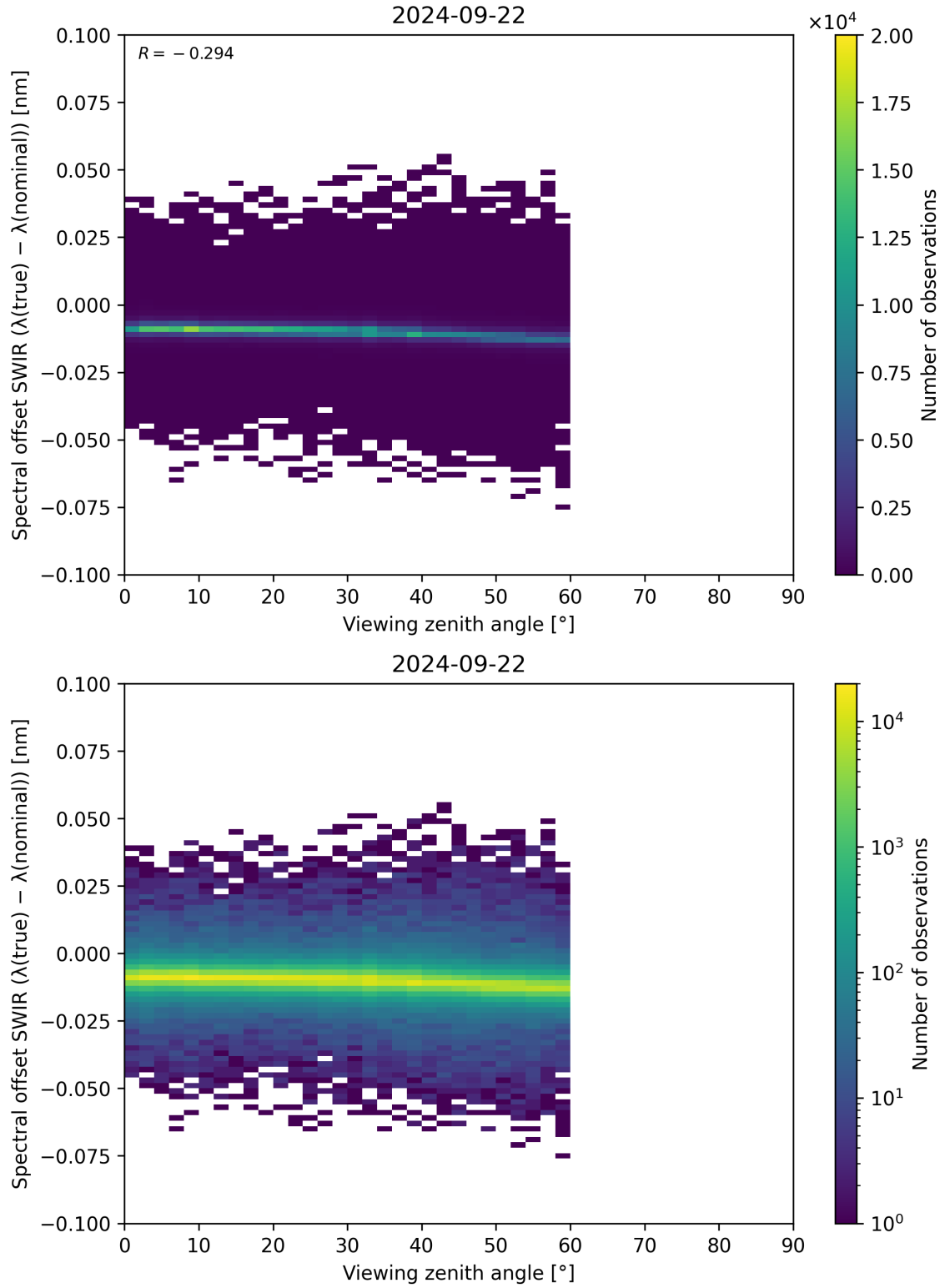
Figure 116: Scatter density plot of “Viewing zenith angle” against “Spectral offset SWIR ( \lambda_{\text{true}} - \lambda_{\text{nominal}} )” for 2024-09-22 to 2024-09-23.
