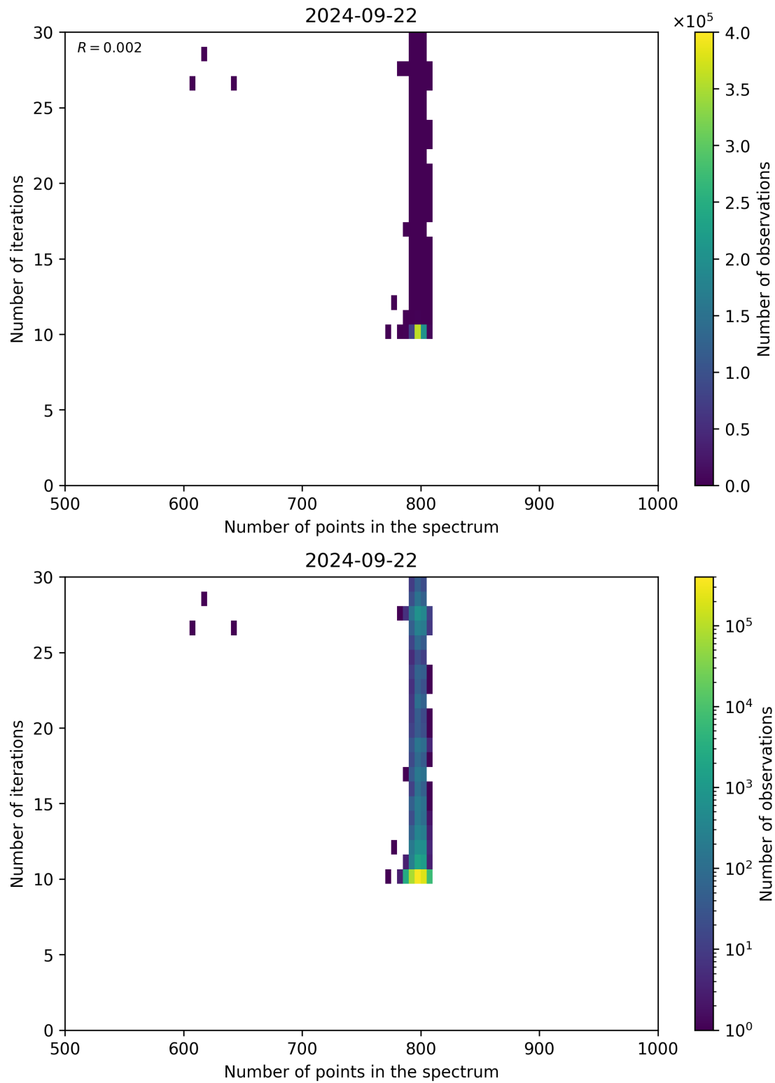
Figure 92: Scatter density plot of “Number of points in the spectrum” against “Number of iterations” for 2024-09-22 to 2024-09-23.
