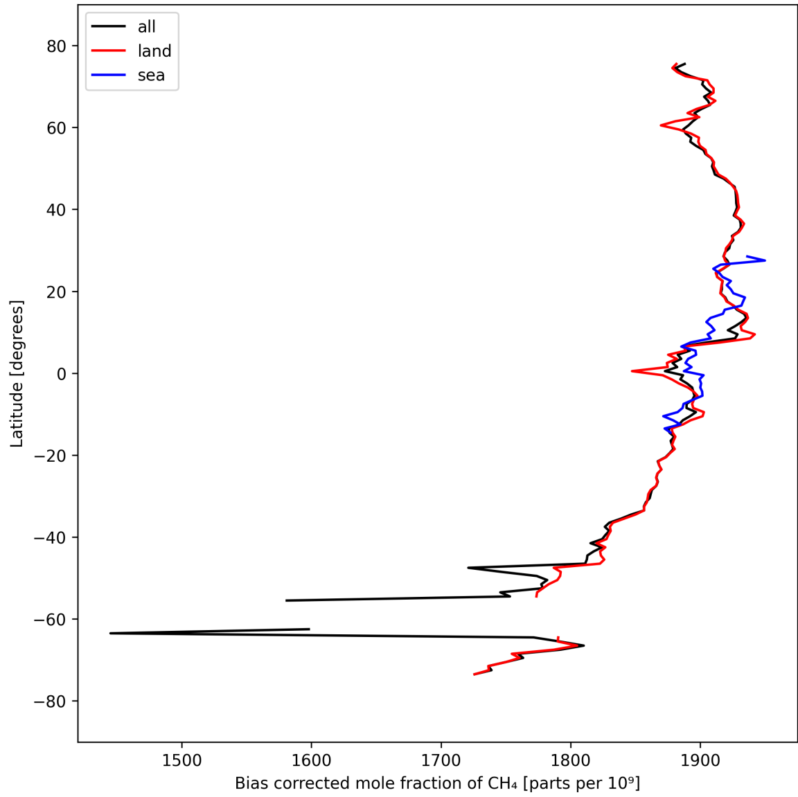
Figure 14: Zonal average of “Bias corrected mole fraction of CH 4 ” for 2024-09-22 to 2024-09-23.
