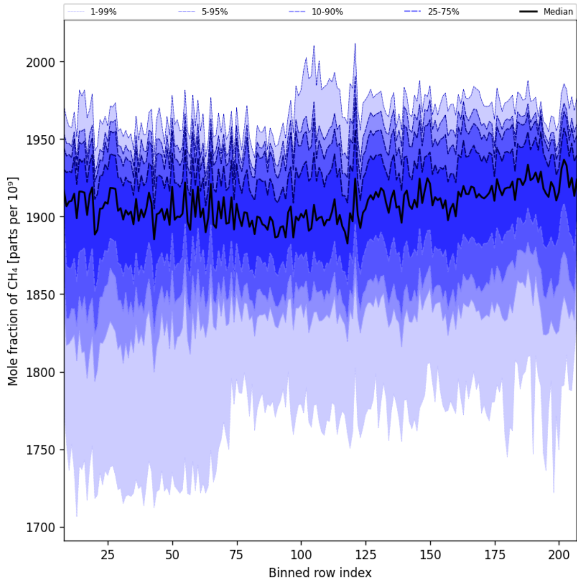
Figure 34: Along track statistics of “Mole fraction of CH 4 ” for 2024-09-22 to 2024-09-23
