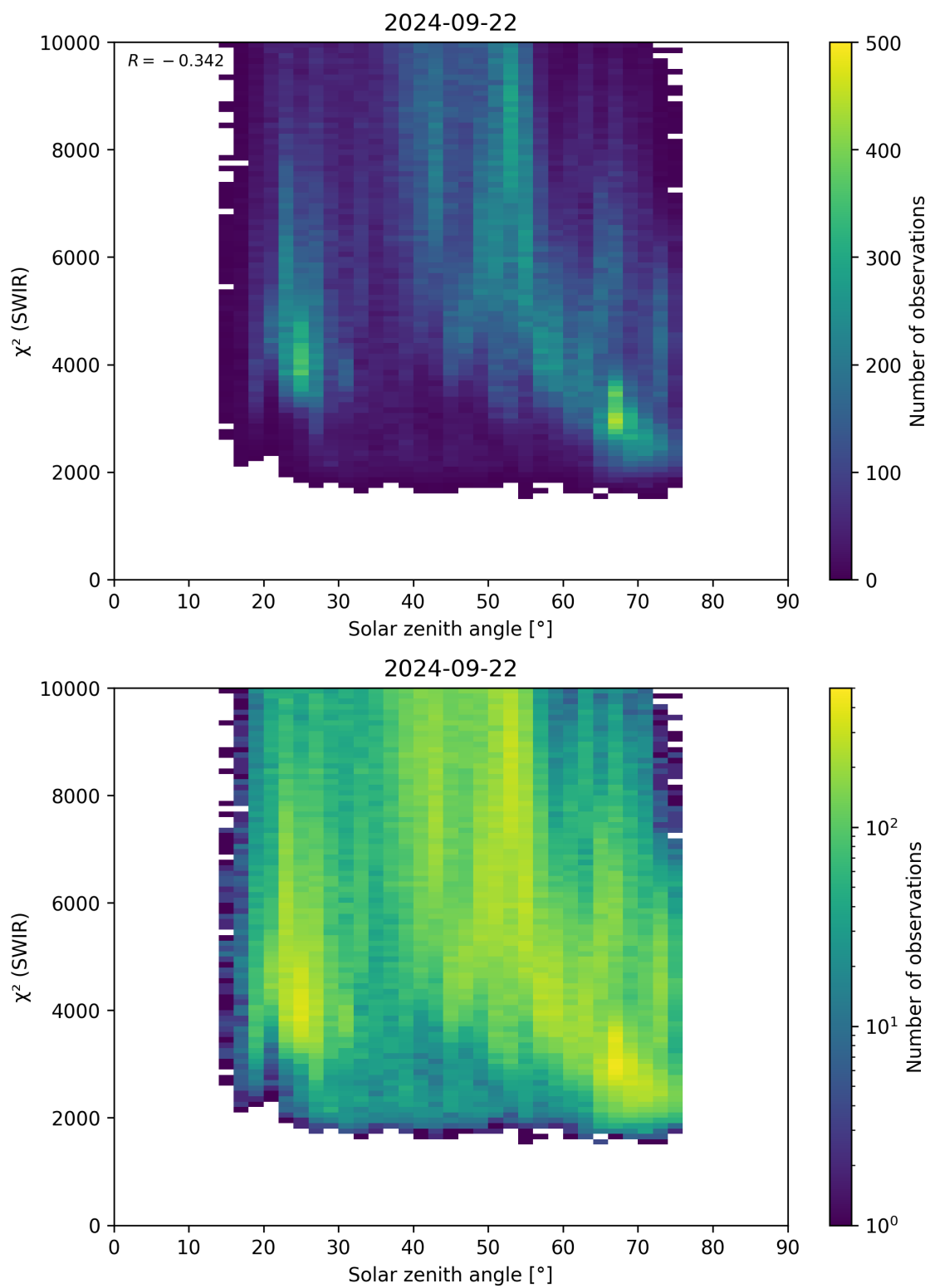
Figure 95: Scatter density plot of “Solar zenith angle” against “ \chi^2 (SWIR)” for 2024-09-22 to 2024-09-23.
