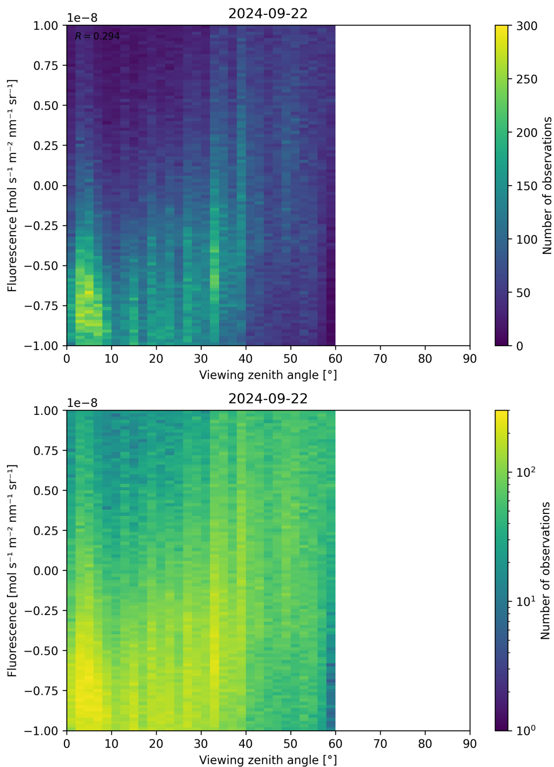
Figure 108: Scatter density plot of “Viewing zenith angle” against “Fluorescence” for 2024-09-22 to 2024-09-23.
