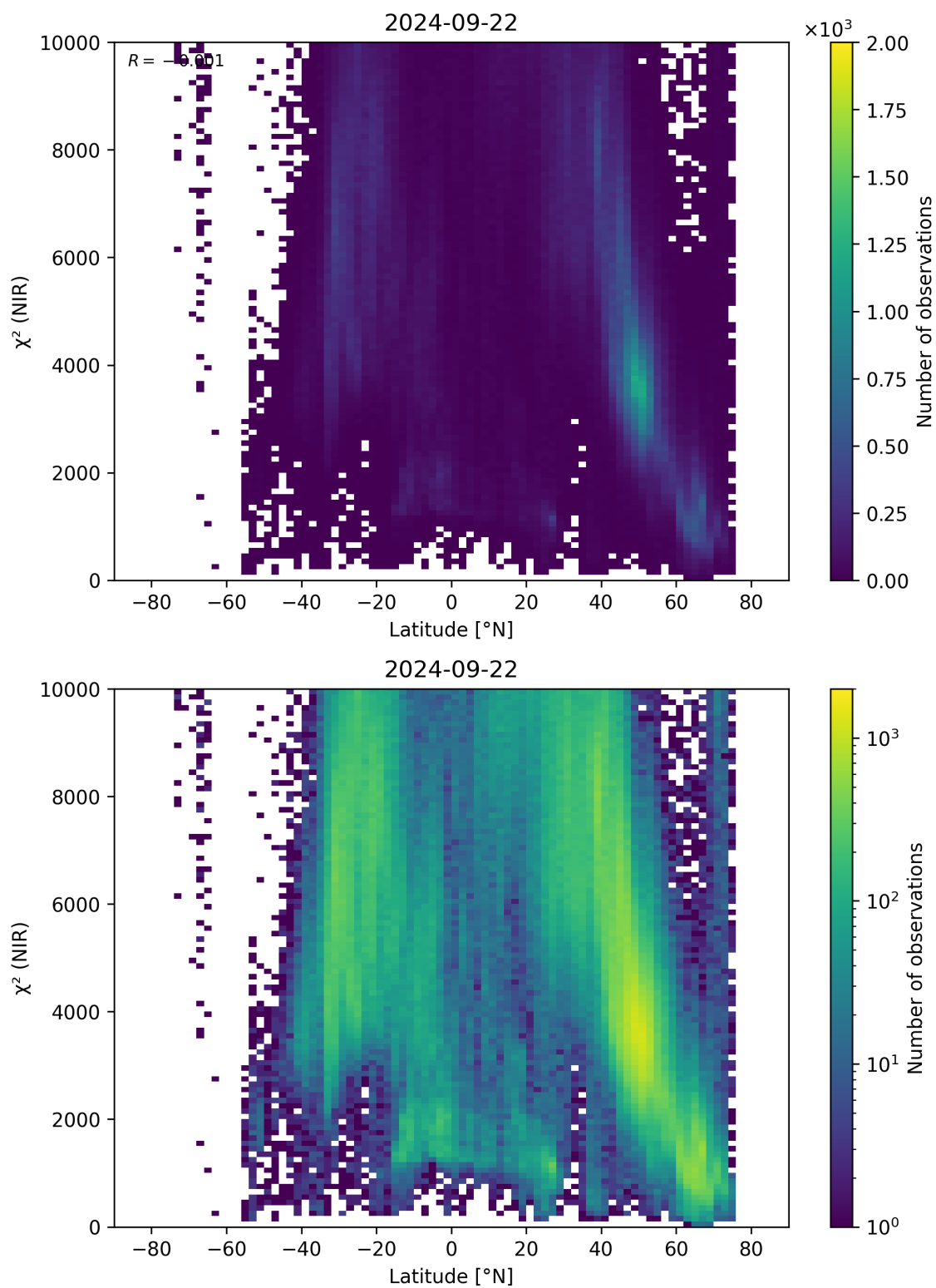
Figure 53: Scatter density plot of “Latitude” against “ \chi^2 (NIR)” for 2024-09-22 to 2024-09-23.
