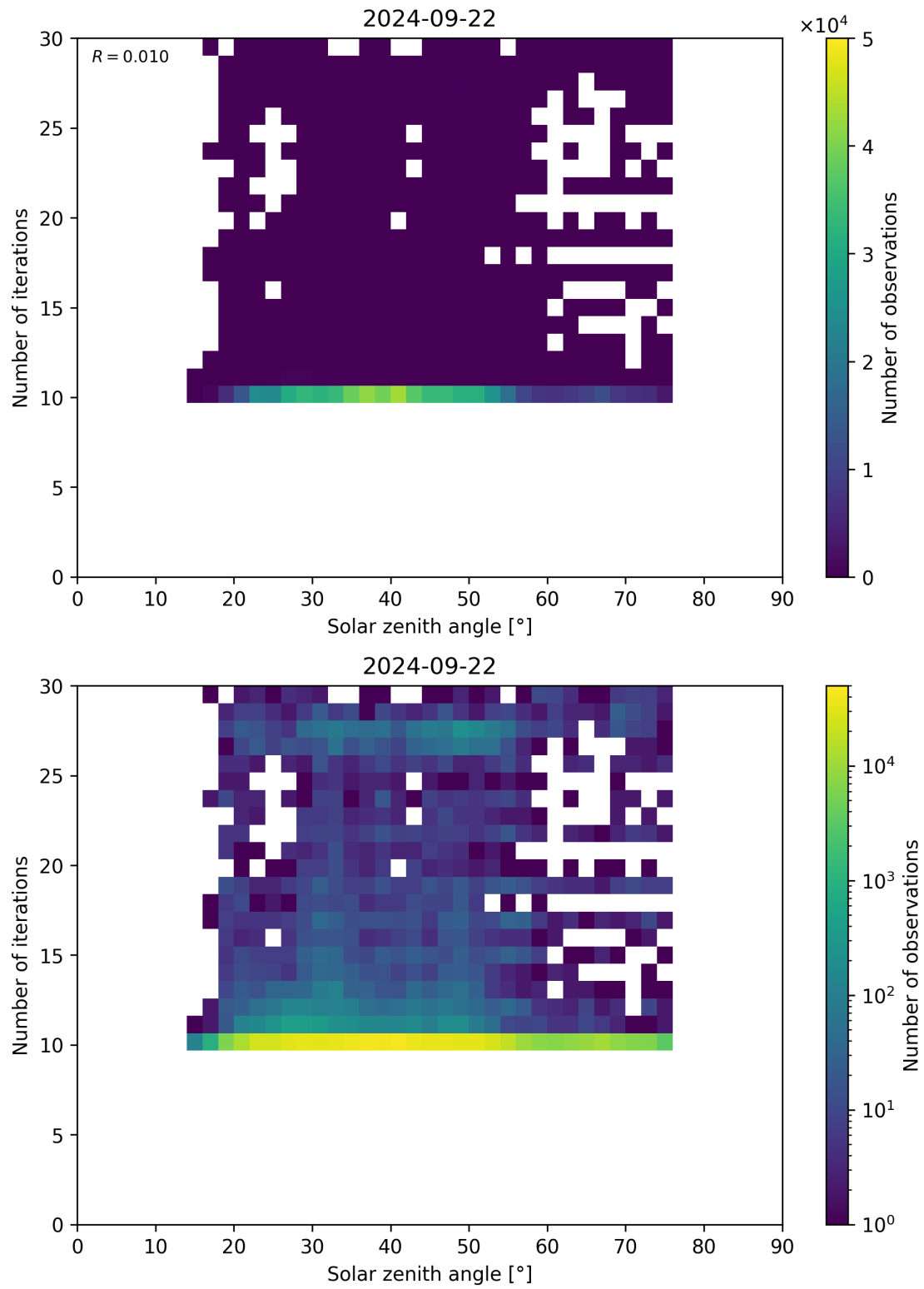
Figure 102: Scatter density plot of “Solar zenith angle” against “Number of iterations” for 2024-09-22 to 2024-09-23.
