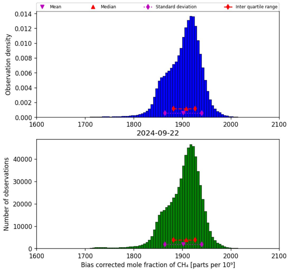
Figure 25: Histogram of “Bias corrected mole fraction of CH 4 ” for 2024-09-22 to 2024-09-23
