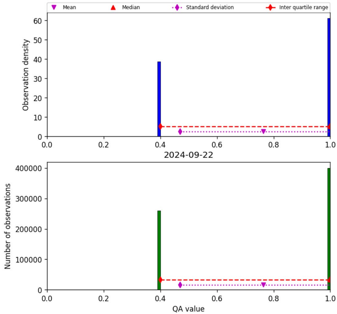
Figure 22: Histogram of “QA value” for 2024-09-22 to 2024-09-23
