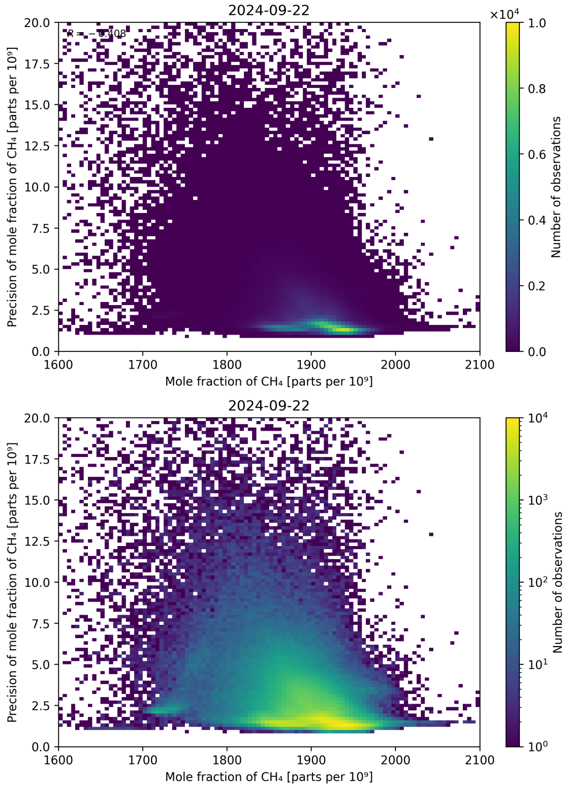
Figure 75: Scatter density plot of “Mole fraction of CH 4 ” against “Precision of mole fraction of CH 4 ” for 2024-09-22 to 2024-09-23.
