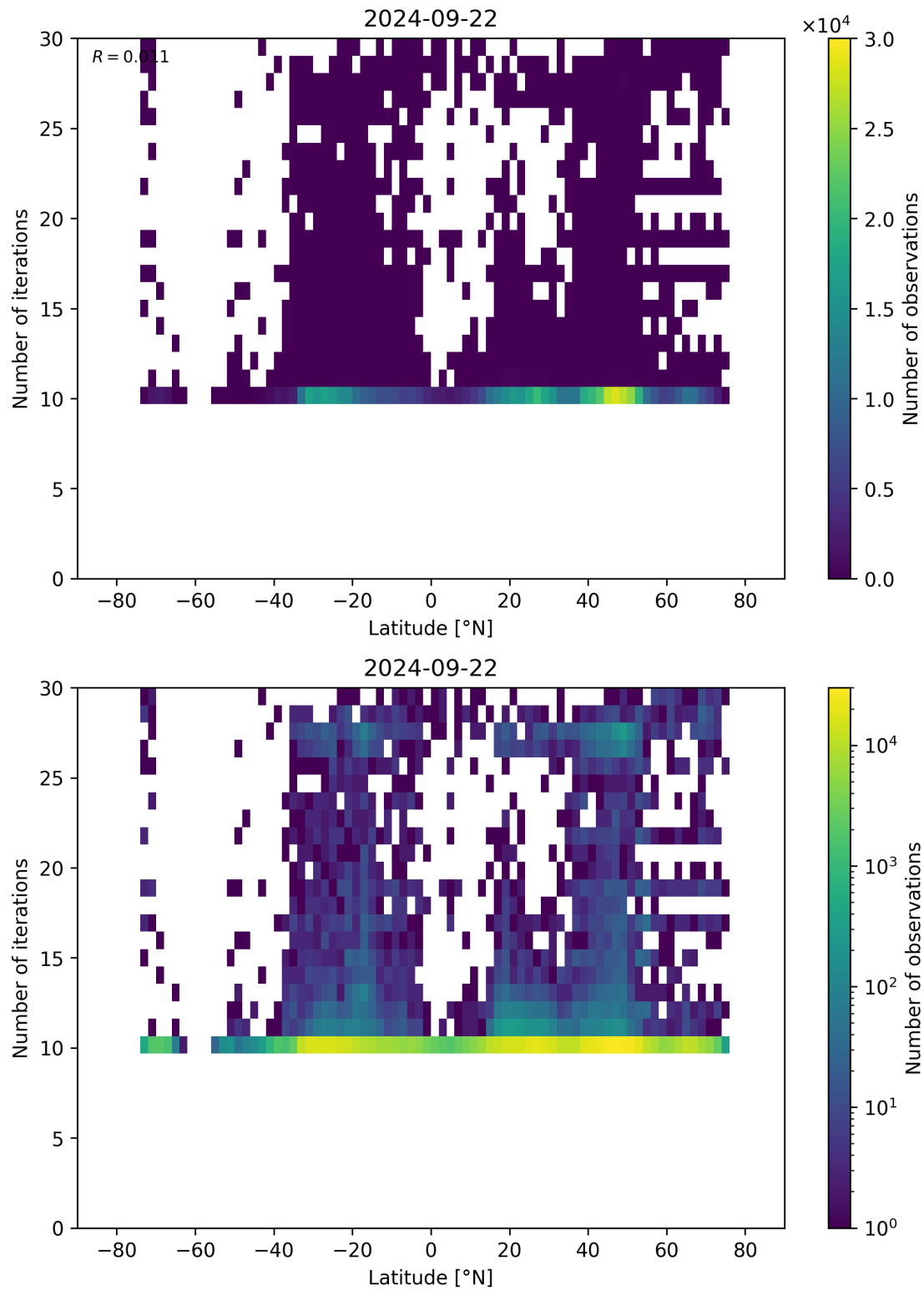
Figure 60: Scatter density plot of “Latitude” against “Number of iterations” for 2024-09-22 to 2024-09-23.
