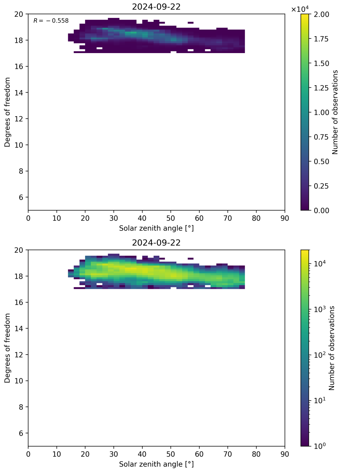
Figure 96: Scatter density plot of “Solar zenith angle” against “Degrees of freedom” for 2024-09-22 to 2024-09-23.
