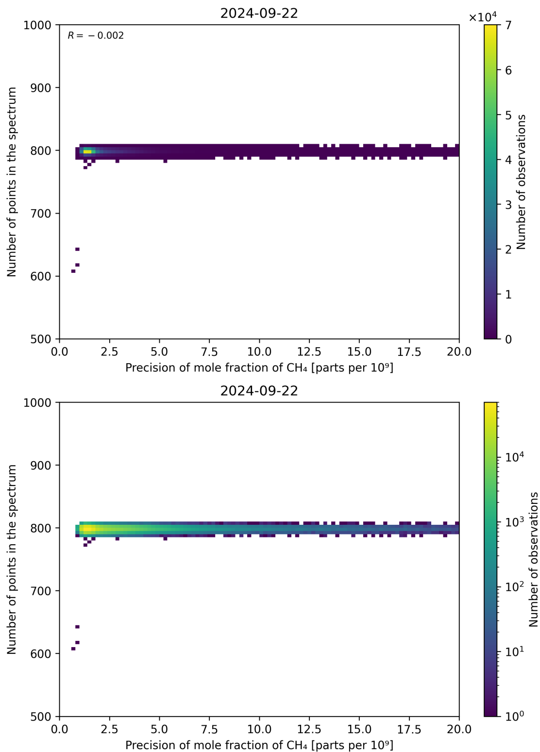
Figure 84: Scatter density plot of “Precision of mole fraction of CH 4 ” against “Number of points in the spectrum” for 2024-09-22 to 2024-09-23.
