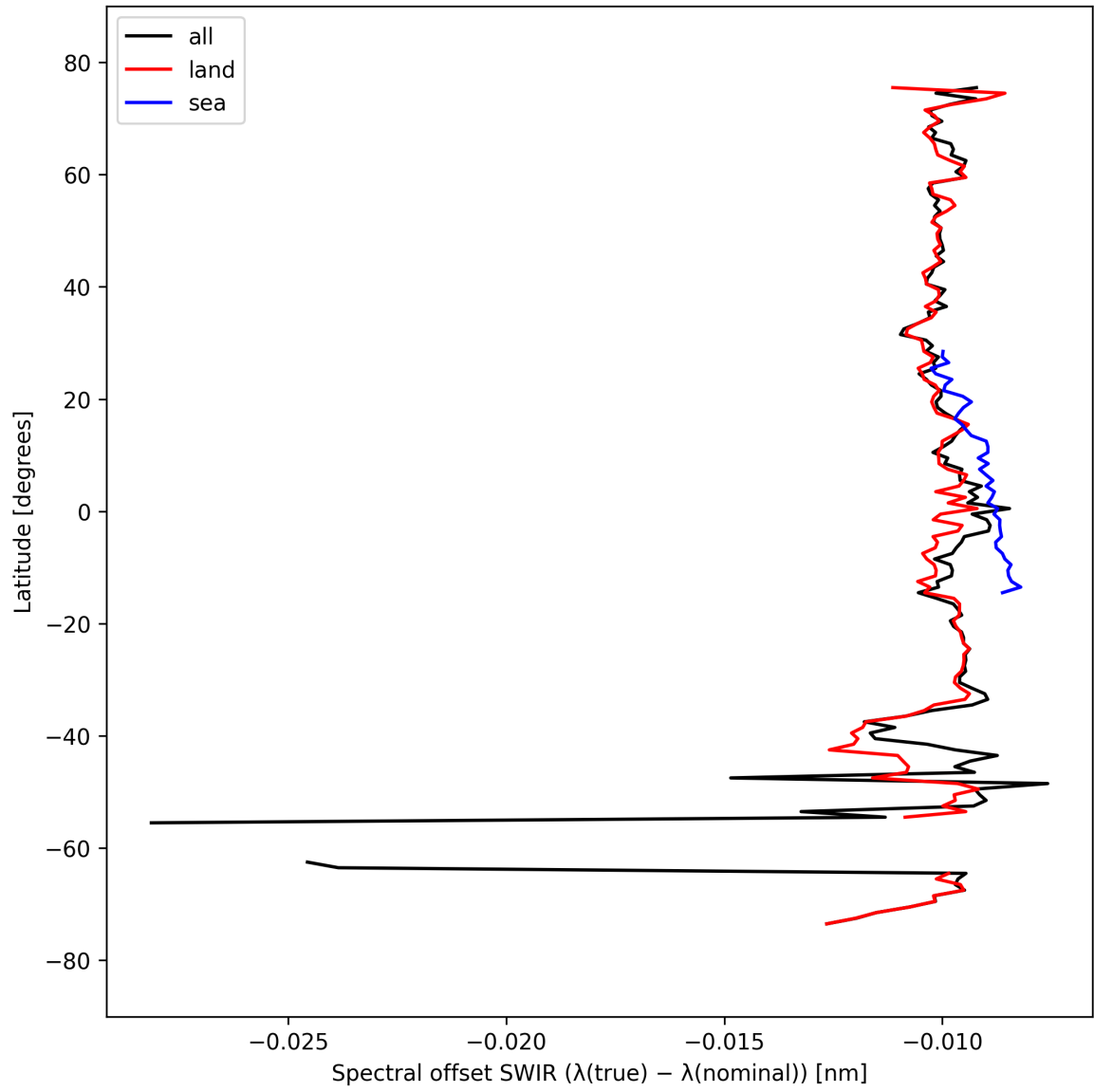
Figure 16: Zonal average of “Spectral offset SWIR ( \lambda_{\text{true}} - \lambda_{\text{nominal}} )” for 2024-09-22 to 2024-09-23.
