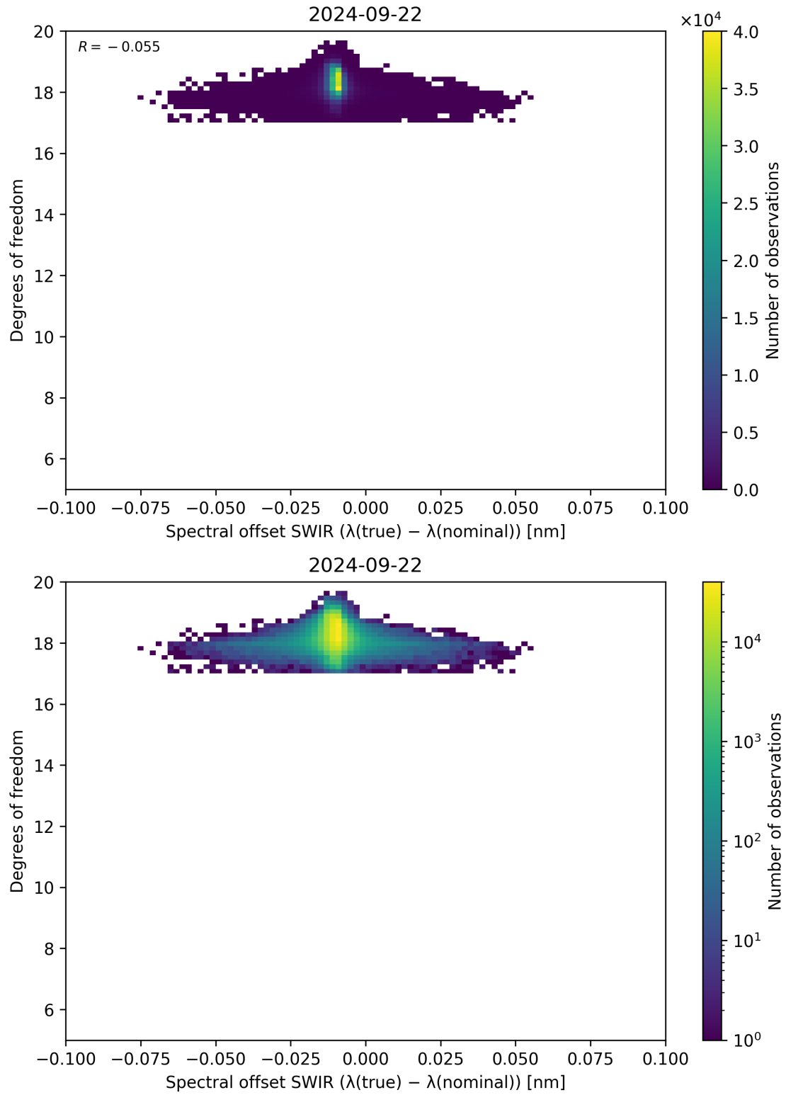
Figure 119: Scatter density plot of “Spectral offset SWIR ( \lambda_{\text{true}} - \lambda_{\text{nominal}} )” against “Degrees of freedom” for 2024-09-22 to 2024-09-23.
