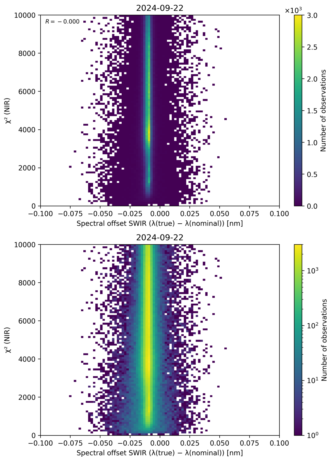
Figure 117: Scatter density plot of “Spectral offset SWIR ( \lambda_{\text{true}} - \lambda_{\text{nominal}} )” against “ \chi^2 (NIR)” for 2024-09-22 to 2024-09-23.
