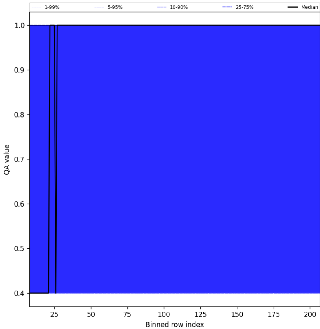
Figure 33: Along track statistics of “QA value” for 2024-09-22 to 2024-09-23
