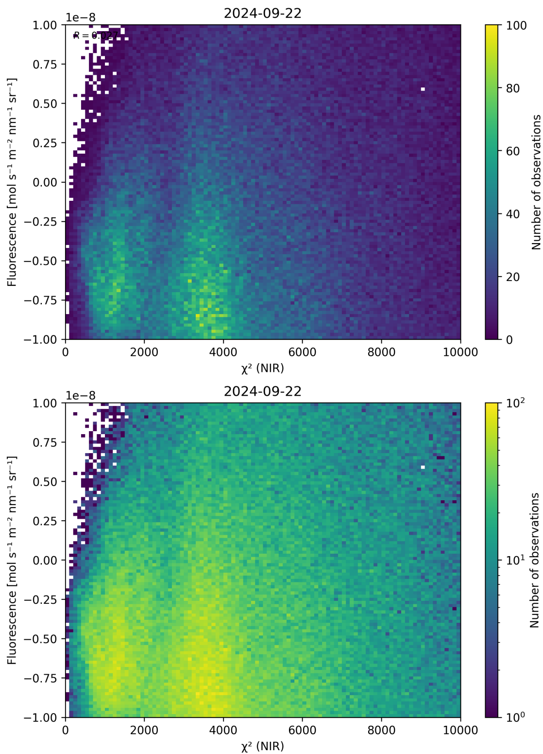
Figure 45: Scatter density plot of “ \chi^2 (NIR)” against “Fluorescence” for 2024-09-22 to 2024-09-23.
