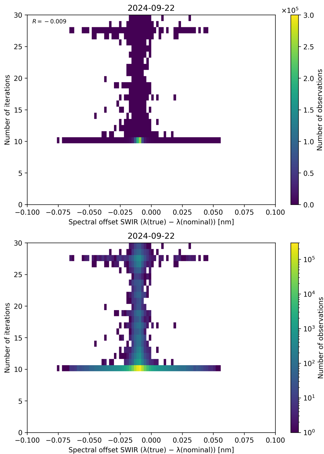
Figure 121: Scatter density plot of “Spectral offset SWIR ( \lambda_{\text{true}} - \lambda_{\text{nominal}} )” against “Number of iterations” for 2024-09-22 to 2024-09-23.
