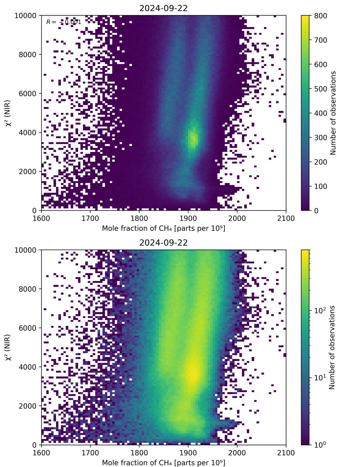
Figure 70: Scatter density plot of “Mole fraction of \text{CH}_4 ” against “ \chi^2 (NIR)” for 2024-09-22 to 2024-09-23.
