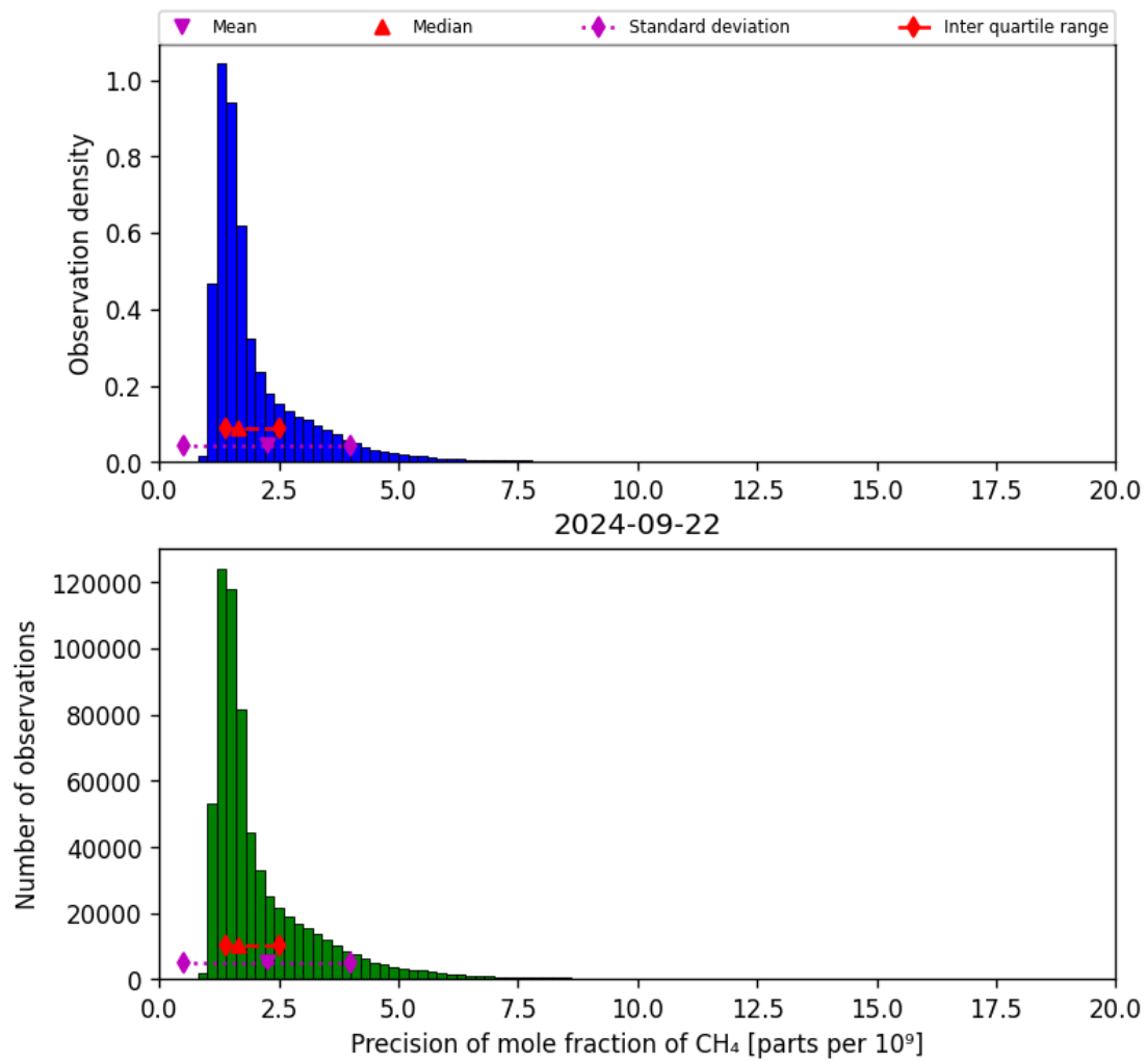
Figure 24: Histogram of “Precision of mole fraction of CH 4 ” for 2024-09-22 to 2024-09-23
