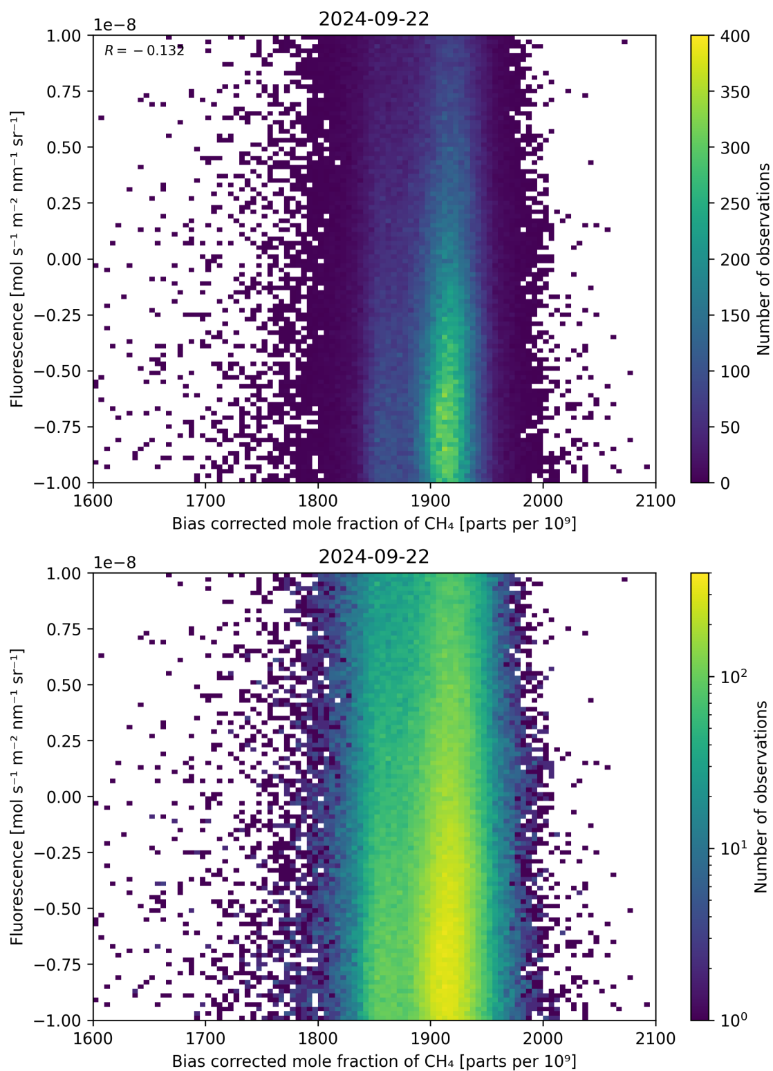
Figure 66: Scatter density plot of “Bias corrected mole fraction of \text{CH}_4 ” against “Fluorescence” for 2024-09-22 to 2024-09-23.
