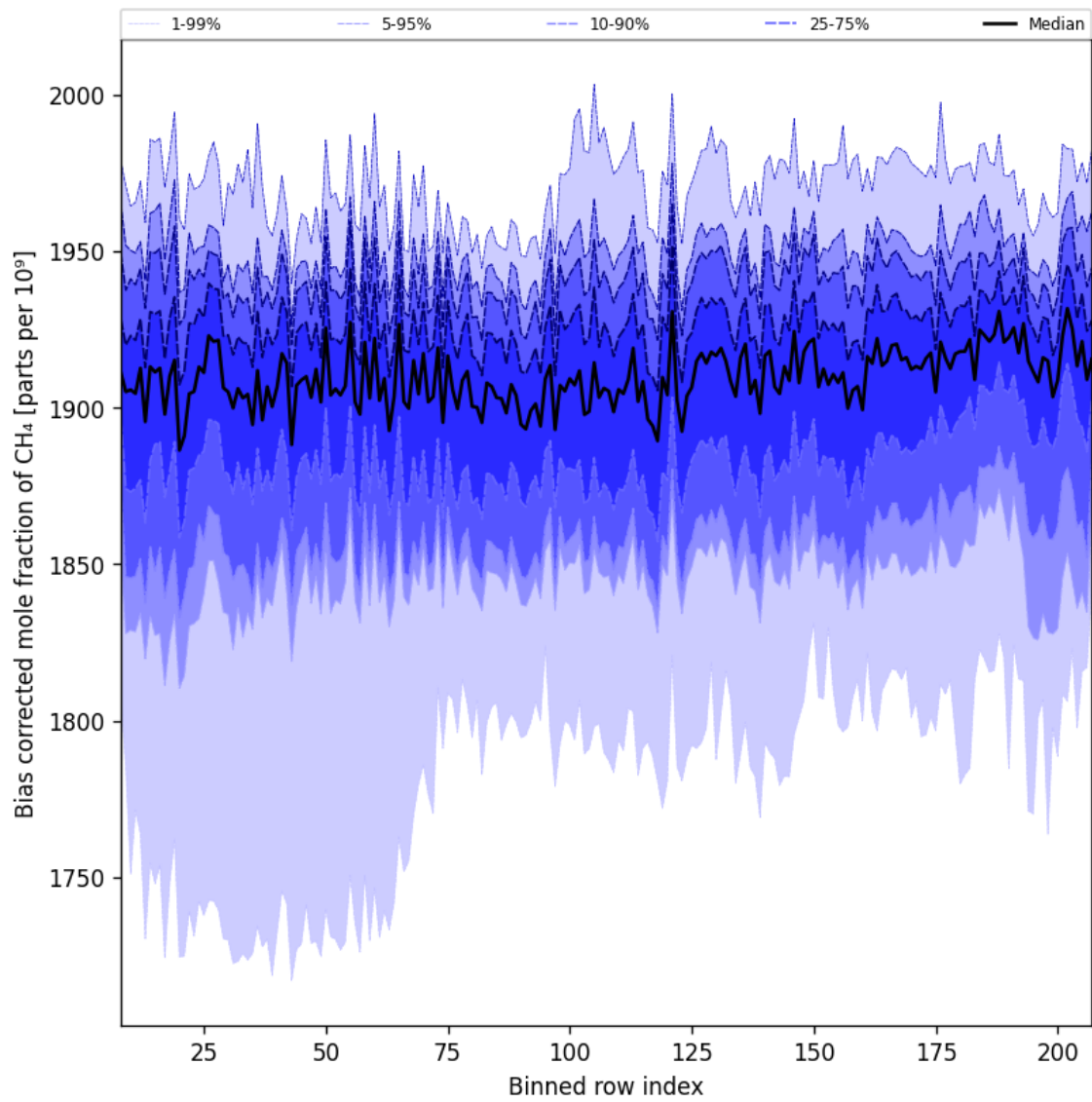
Figure 36: Along track statistics of “Bias corrected mole fraction of CH 4 ” for 2024-09-22 to 2024-09-23
