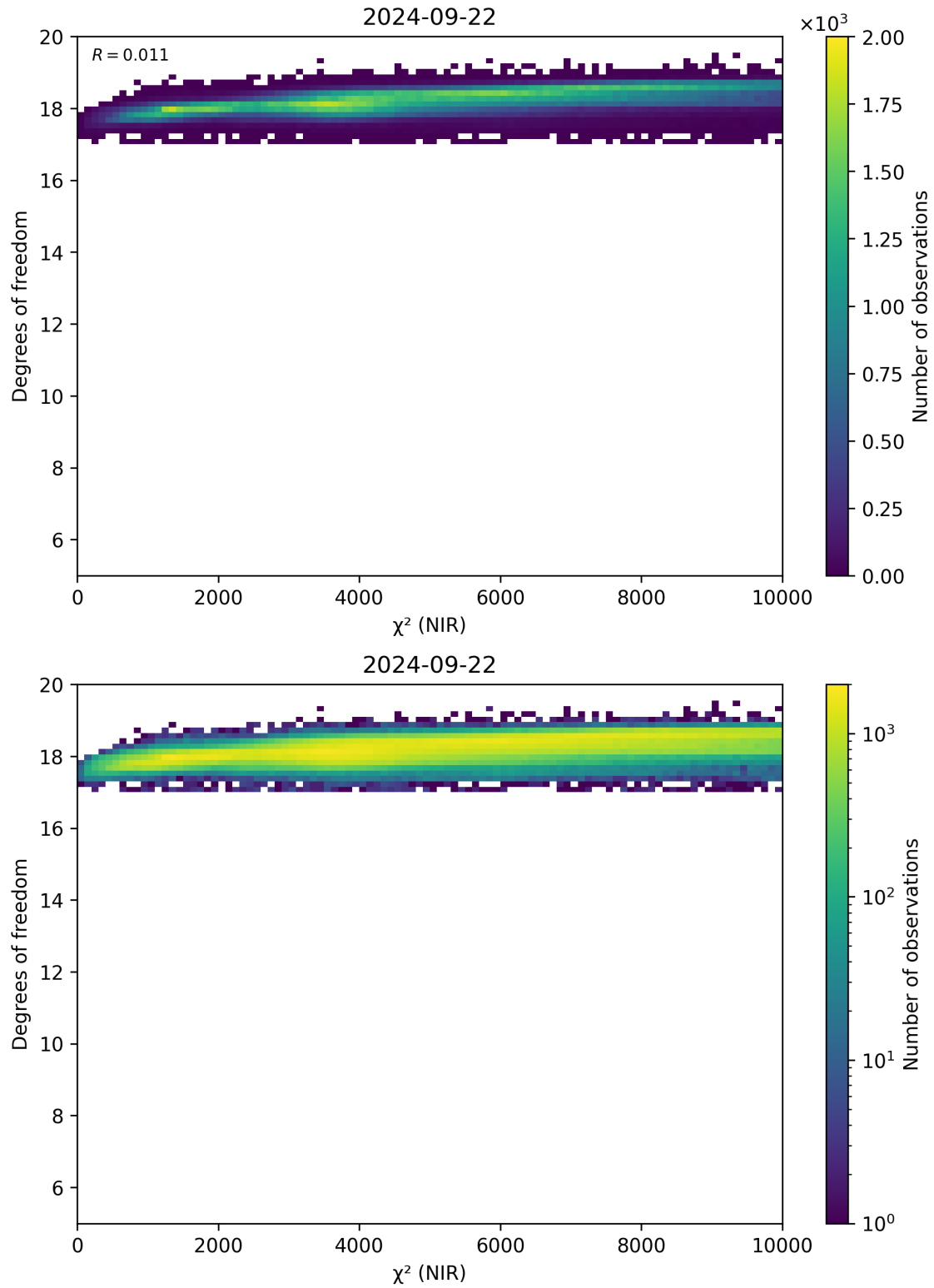
Figure 44: Scatter density plot of “ \chi^2 (NIR)” against “Degrees of freedom” for 2024-09-22 to 2024-09-23.
