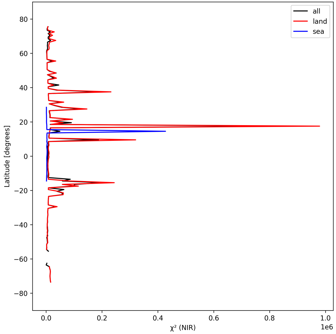
Figure 18: Zonal average of “ \chi^2 (NIR)” for 2024-09-22 to 2024-09-23.
