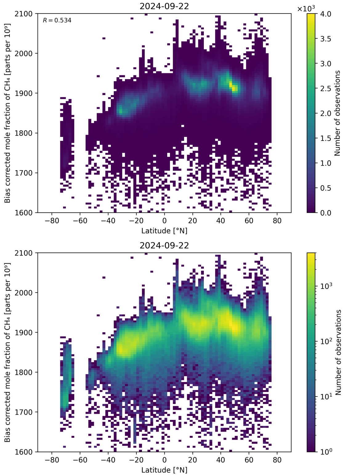
Figure 58: Scatter density plot of “Latitude” against “Bias corrected mole fraction of CH 4 ” for 2024-09-22 to 2024-09-23.
