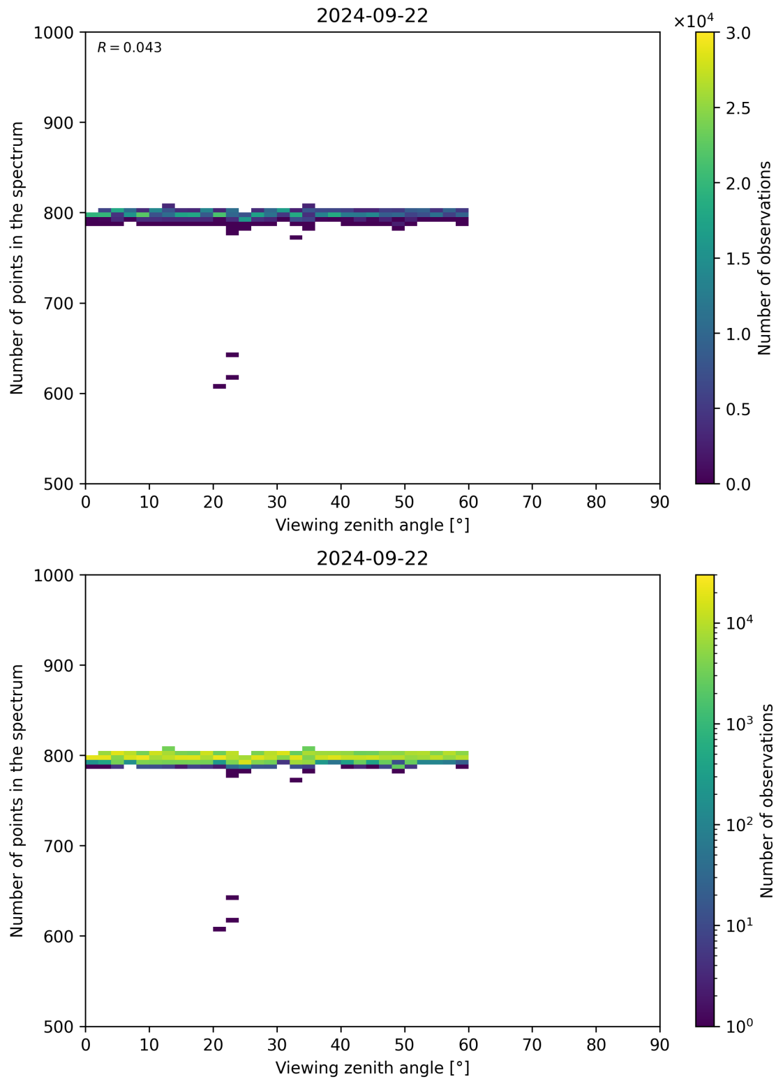
Figure 114: Scatter density plot of “Viewing zenith angle” against “Number of points in the spectrum” for 2024-09-22 to 2024-09-23.
