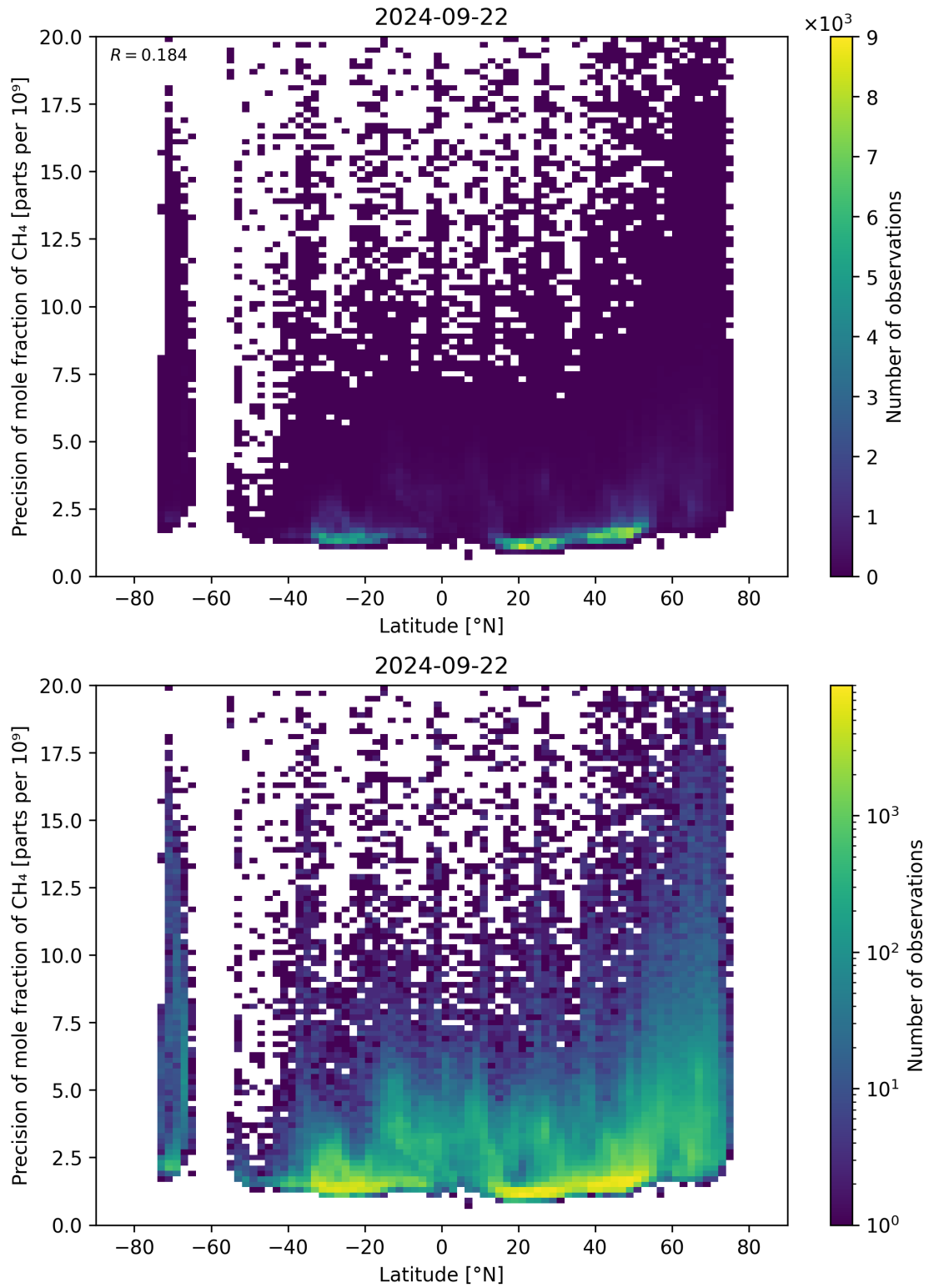
Figure 59: Scatter density plot of “Latitude” against “Precision of mole fraction of CH 4 ” for 2024-09-22 to 2024-09-23.
