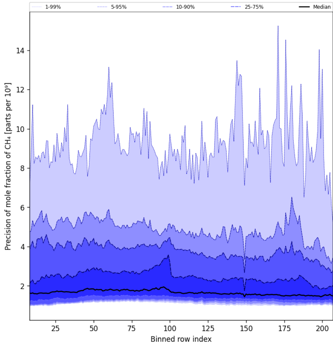
Figure 35: Along track statistics of “Precision of mole fraction of CH 4 ” for 2024-09-22 to 2024-09-23
