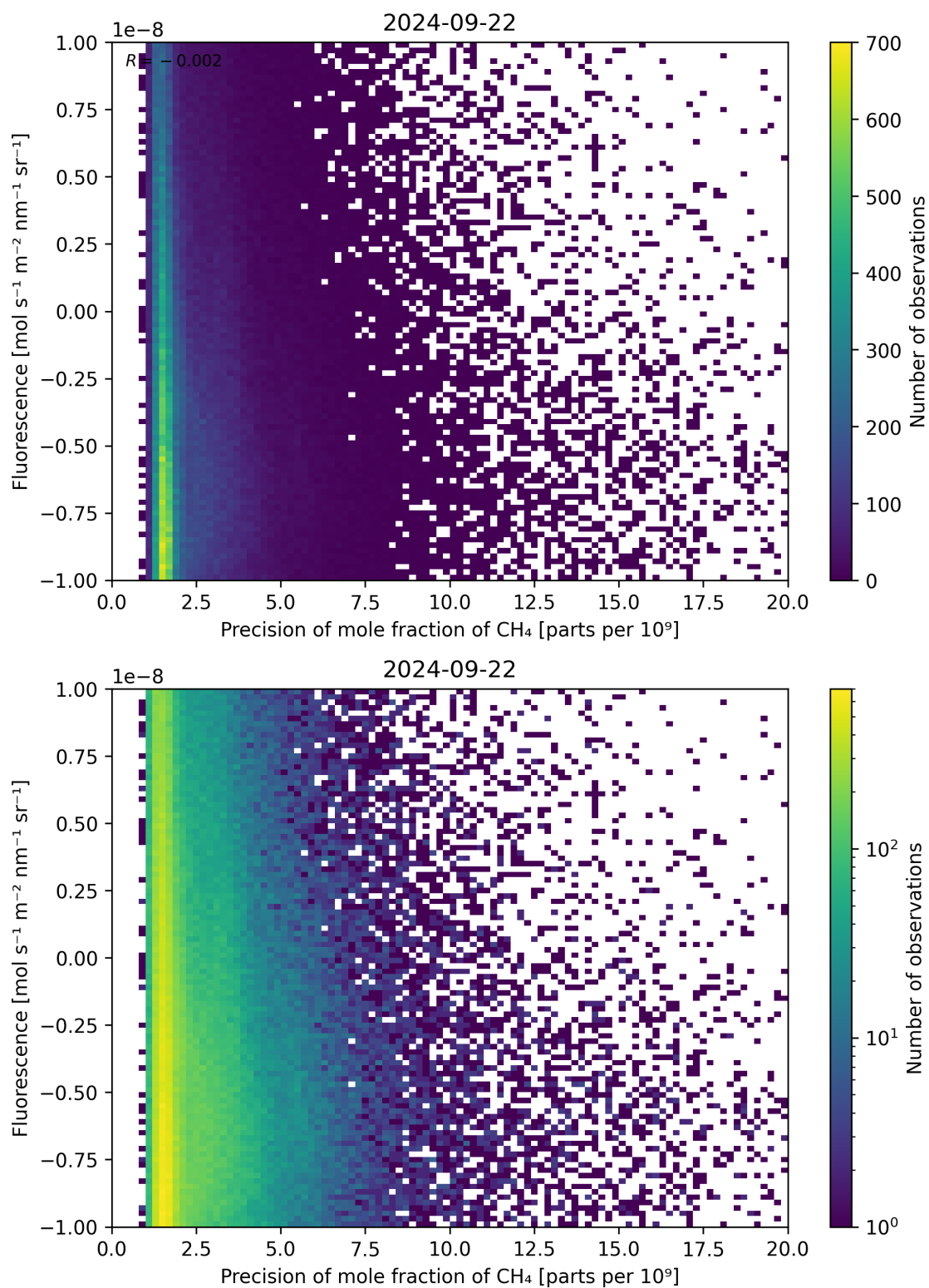
Figure 81: Scatter density plot of “Precision of mole fraction of CH 4 ” against “Fluorescence” for 2024-09-22 to 2024-09-23.
