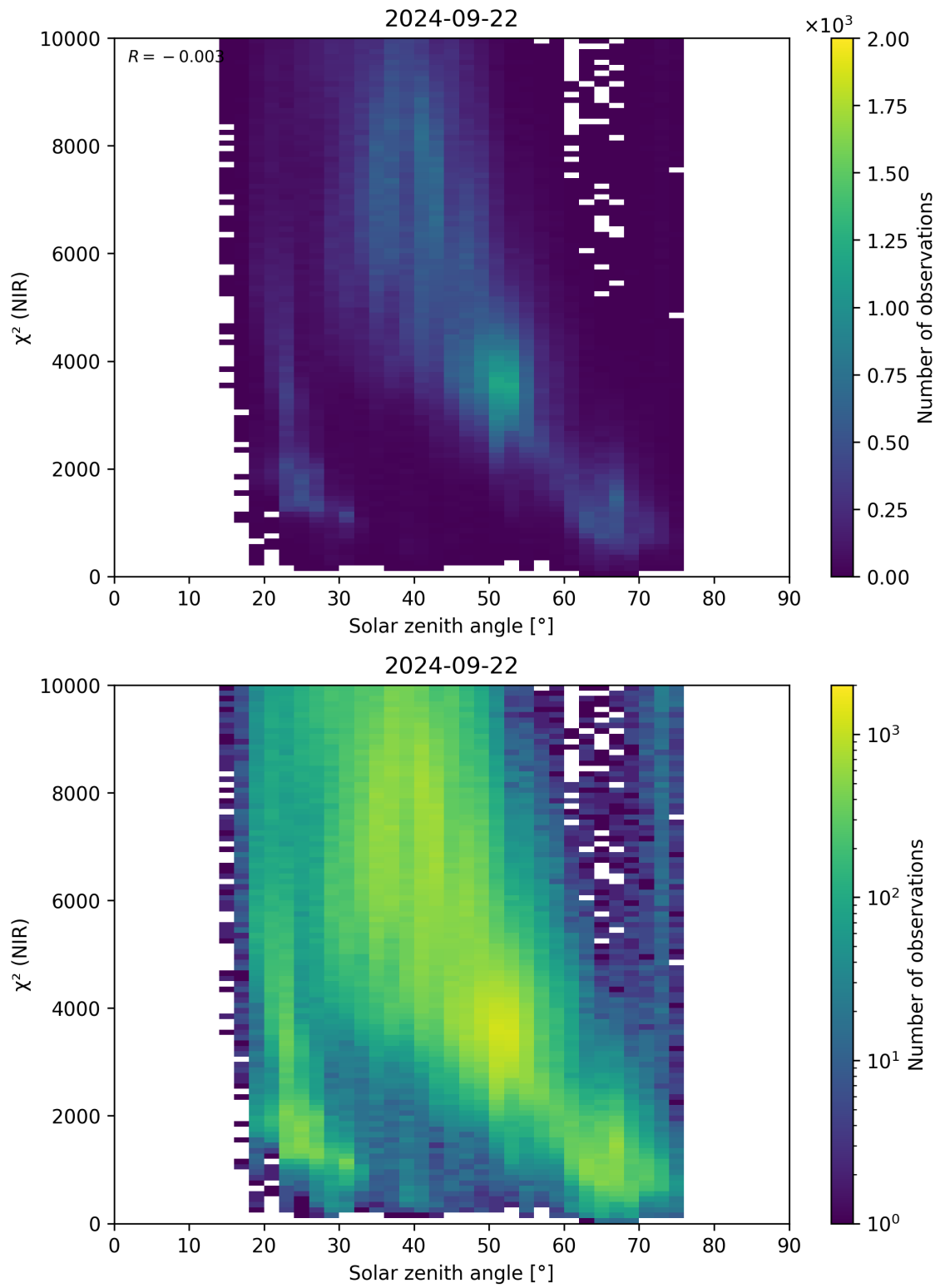
Figure 94: Scatter density plot of “Solar zenith angle” against “ \chi^2 (NIR)” for 2024-09-22 to 2024-09-23.
