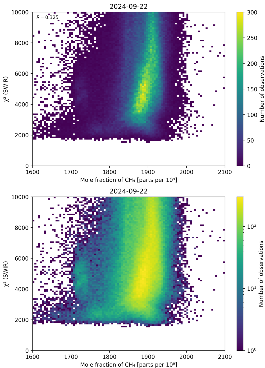
Figure 71: Scatter density plot of “Mole fraction of \text{CH}_4 ” against “ \chi^2 (SWIR)” for 2024-09-22 to 2024-09-23.
