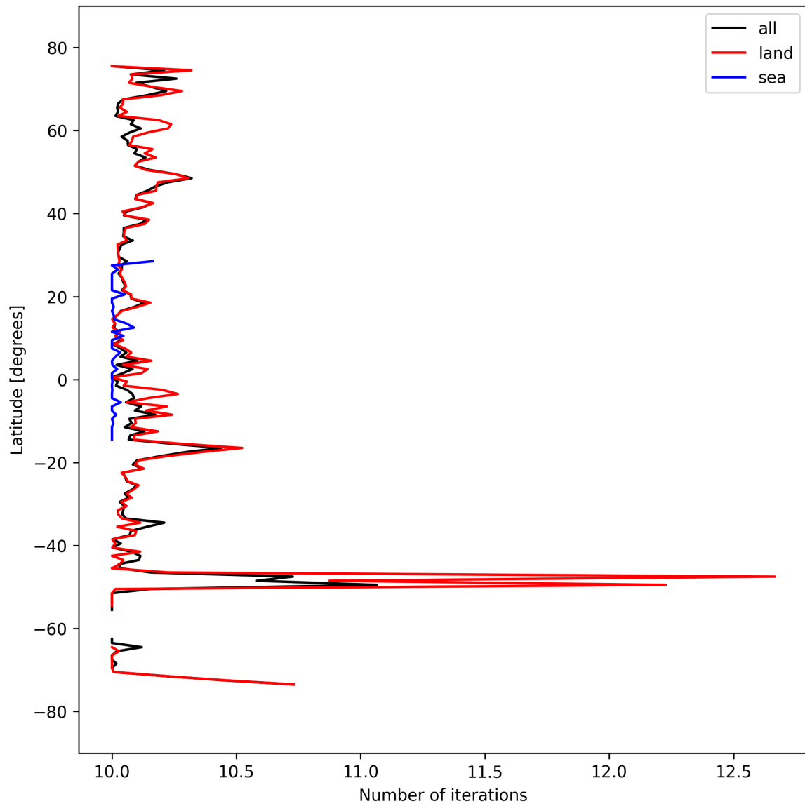
Figure 20: Zonal average of “Number of iterations” for 2024-09-22 to 2024-09-23.
