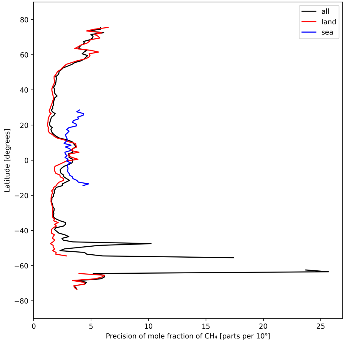
Figure 13: Zonal average of “Precision of mole fraction of \text{CH}_4 ” for 2024-09-22 to 2024-09-23.
