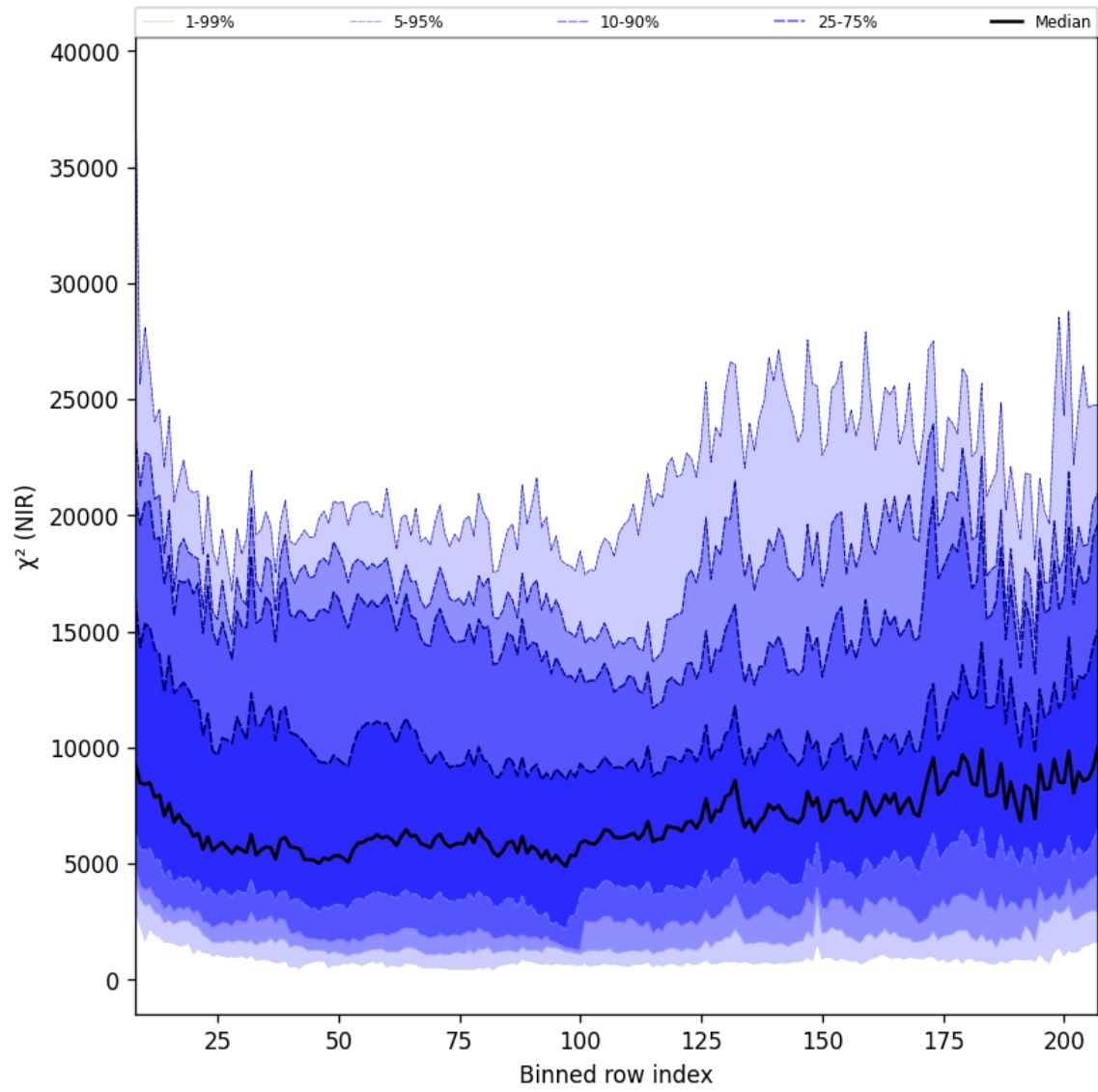
Figure 40: Along track statistics of “ \chi^2 (NIR)” for 2024-09-22 to 2024-09-23
