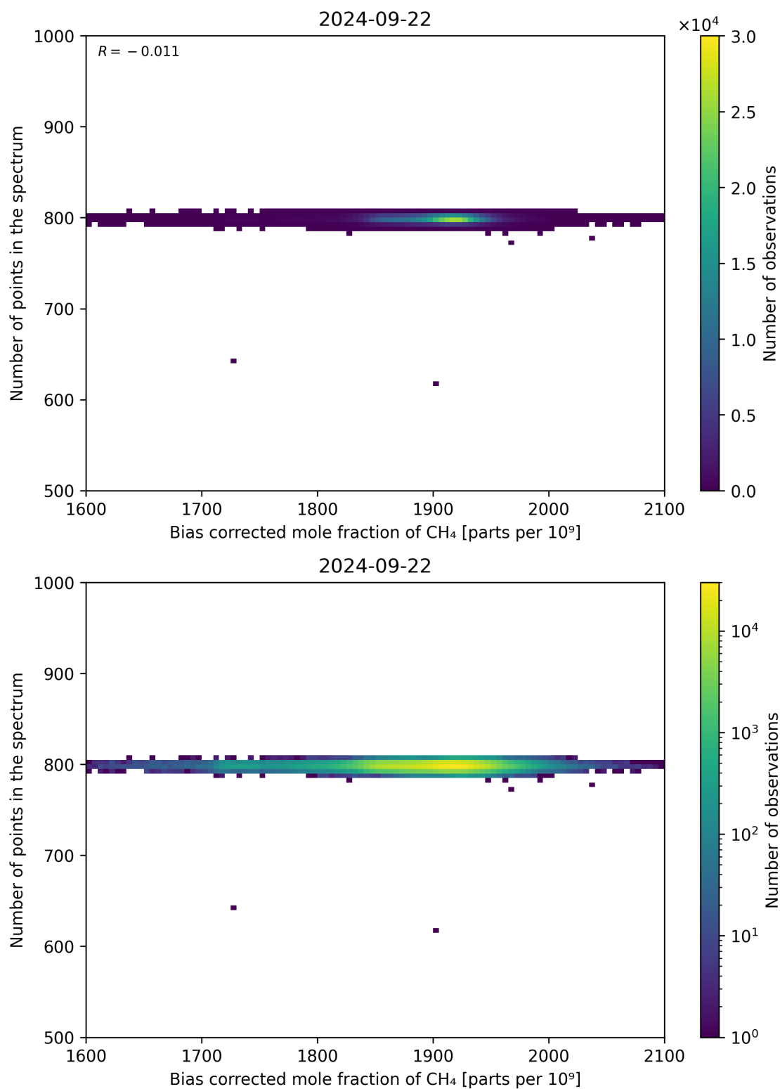
Figure 68: Scatter density plot of “Bias corrected mole fraction of CH 4 ” against “Number of points in the spectrum” for 2024-09-22 to 2024-09-23.
