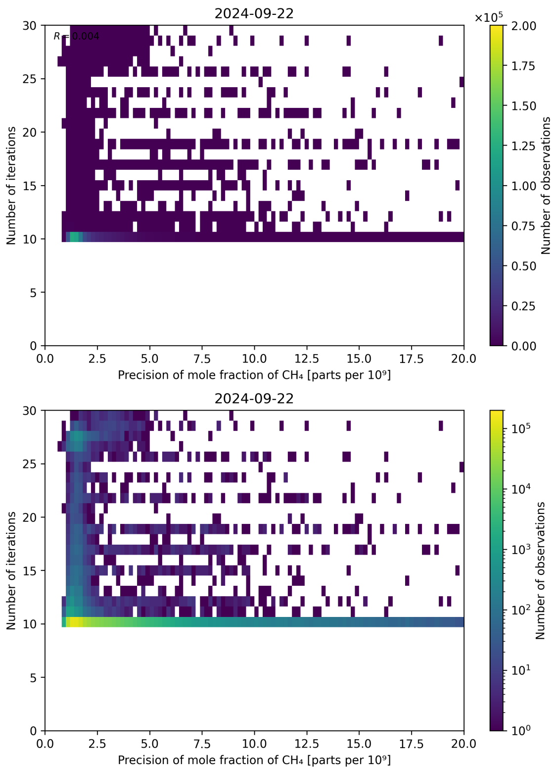
Figure 83: Scatter density plot of “Precision of mole fraction of CH 4 ” against “Number of iterations” for 2024-09-22 to 2024-09-23.
