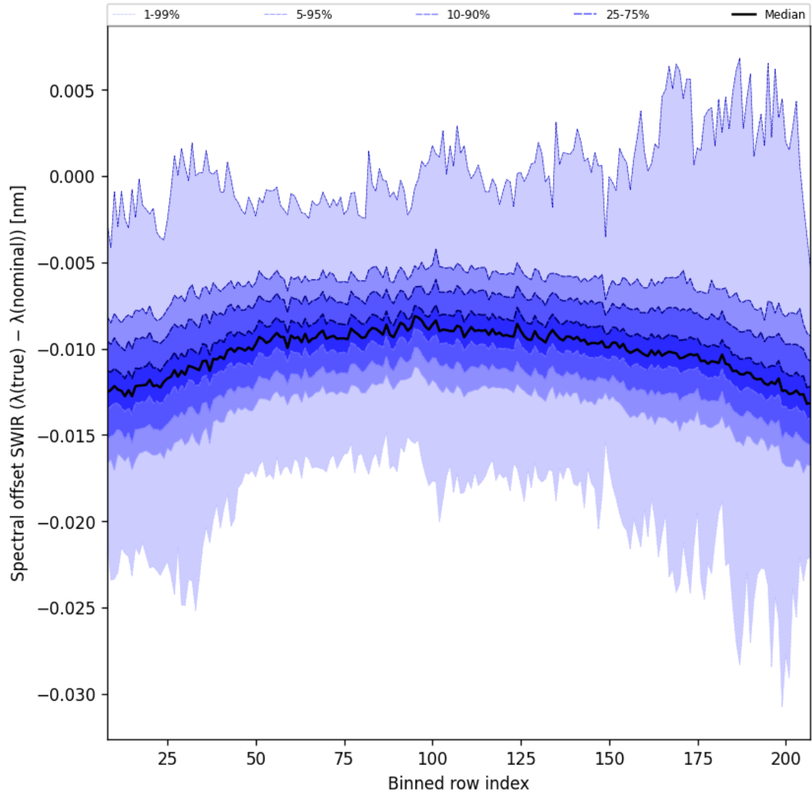
Figure 38: Along track statistics of “Spectral offset SWIR ( \lambda_{\text{true}} - \lambda_{\text{nominal}} )” for 2024-09-22 to 2024-09-23
