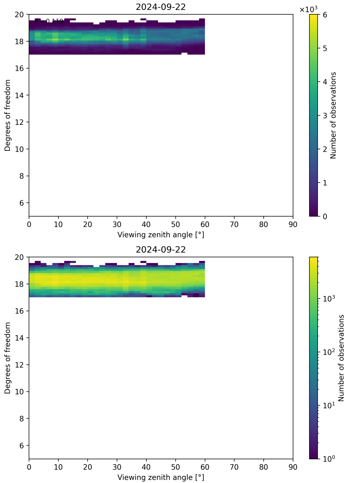
Figure 107: Scatter density plot of “Viewing zenith angle” against “Degrees of freedom” for 2024-09-22 to 2024-09-23.
