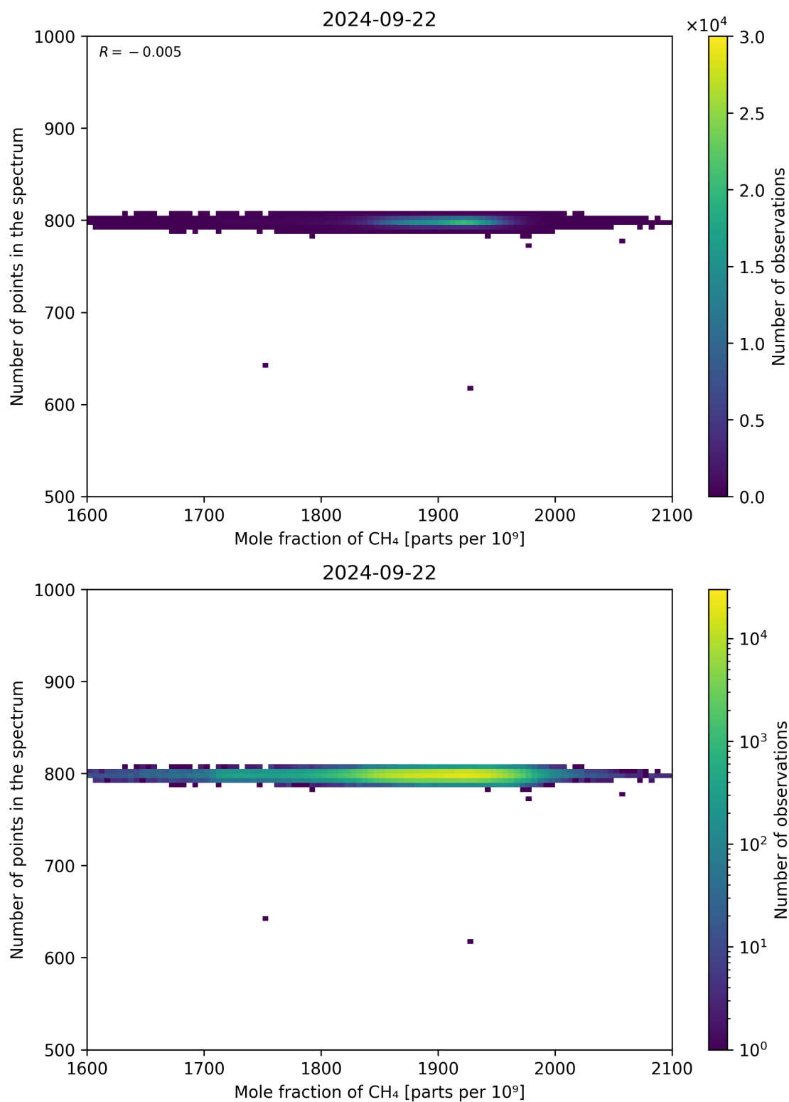
Figure 77: Scatter density plot of “Mole fraction of CH 4 ” against “Number of points in the spectrum” for 2024-09-22 to 2024-09-23.
