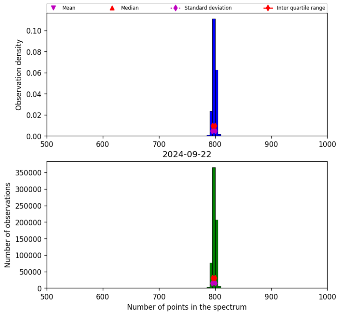
Figure 26: Histogram of “Number of points in the spectrum” for 2024-09-22 to 2024-09-23
