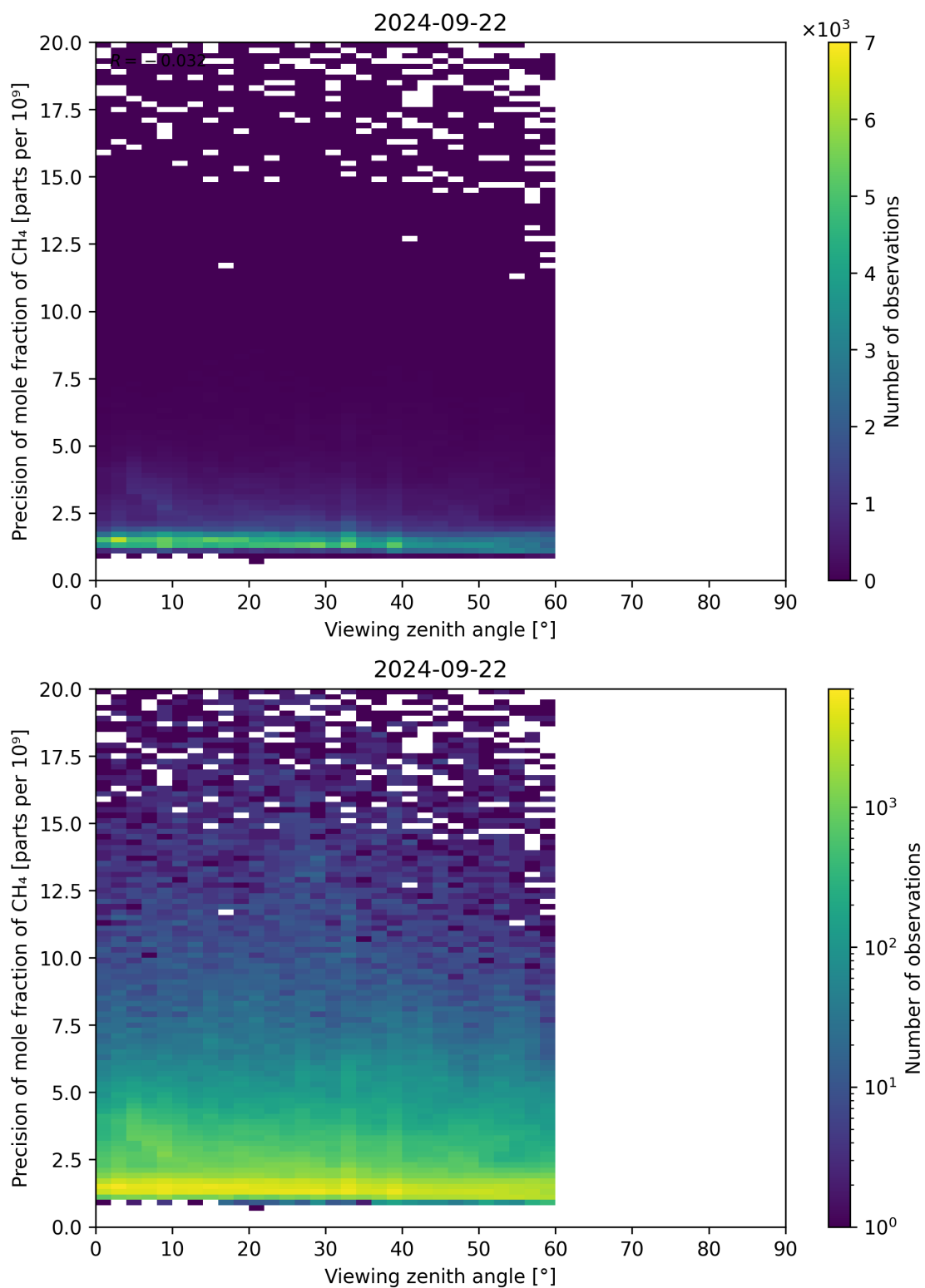
Figure 112: Scatter density plot of “Viewing zenith angle” against “Precision of mole fraction of \text{CH}_4 ” for 2024-09-22 to 2024-09-23.
