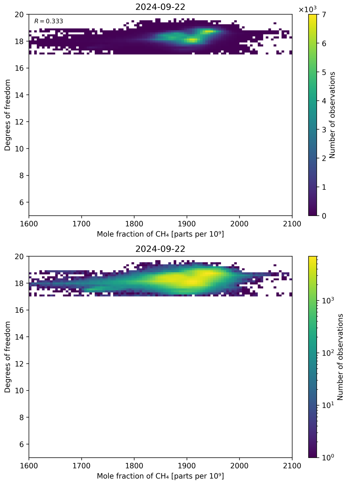
Figure 72: Scatter density plot of “Mole fraction of CH 4 ” against “Degrees of freedom” for 2024-09-22 to 2024-09-23.
