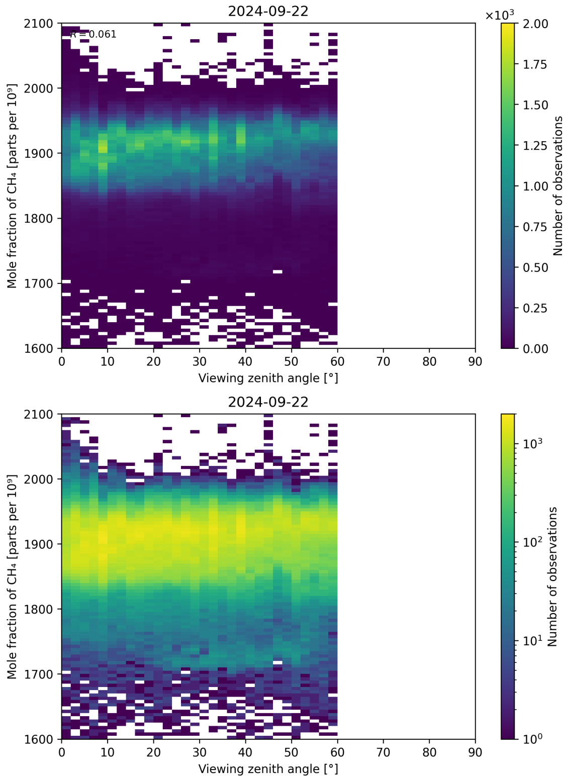
Figure 110: Scatter density plot of “Viewing zenith angle” against “Mole fraction of CH 4 ” for 2024-09-22 to 2024-09-23.
