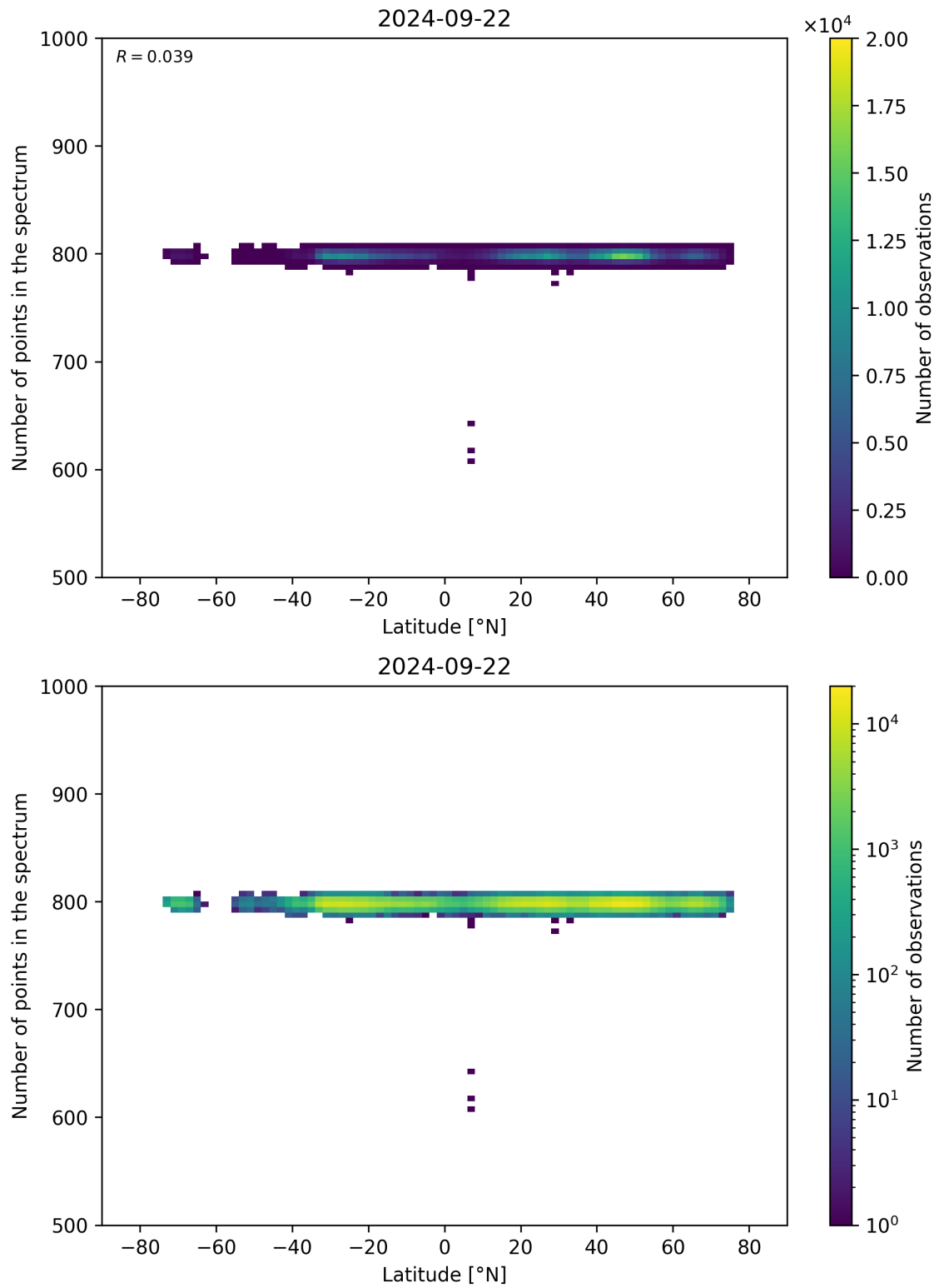
Figure 61: Scatter density plot of “Latitude” against “Number of points in the spectrum” for 2024-09-22 to 2024-09-23.
