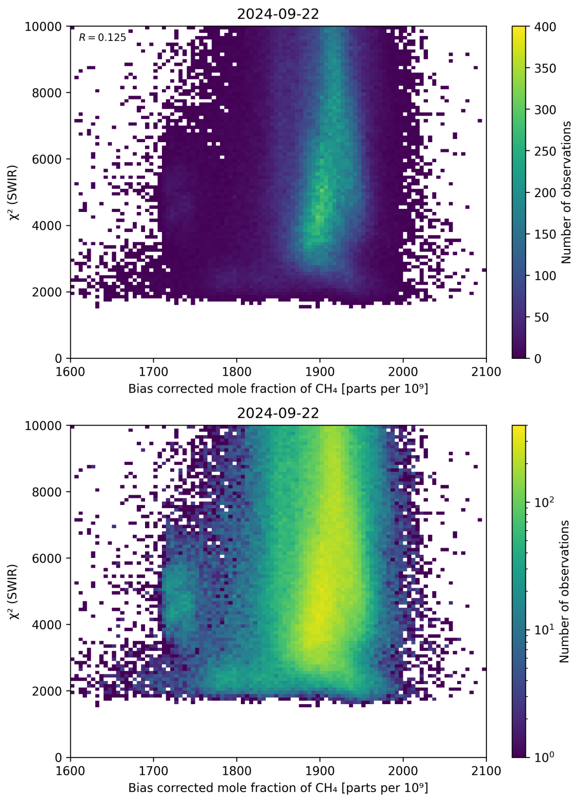
Figure 64: Scatter density plot of “Bias corrected mole fraction of \text{CH}_4 ” against “ \chi^2 (SWIR)” for 2024-09-22 to 2024-09-23.
