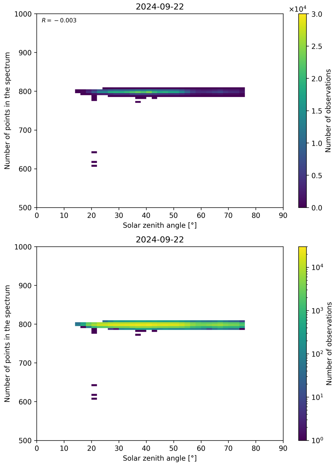
Figure 103: Scatter density plot of “Solar zenith angle” against “Number of points in the spectrum” for 2024-09-22 to 2024-09-23.
