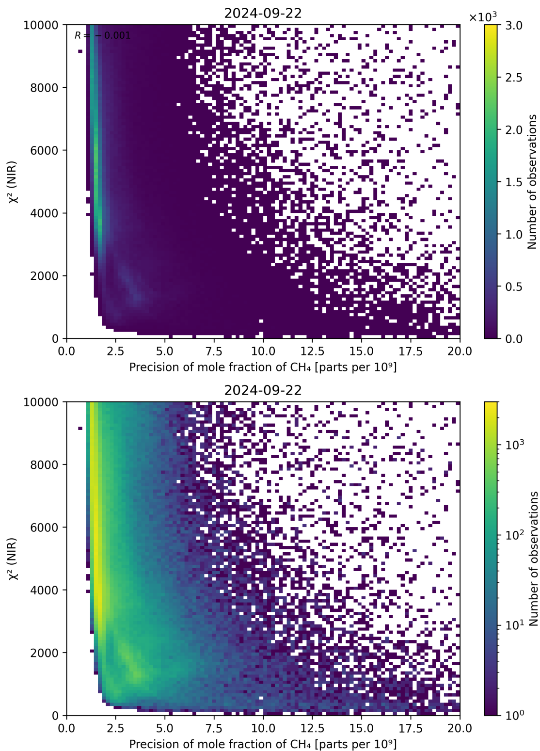
Figure 78: Scatter density plot of “Precision of mole fraction of \text{CH}_4 ” against “ \chi^2 (NIR)” for 2024-09-22 to 2024-09-23.
