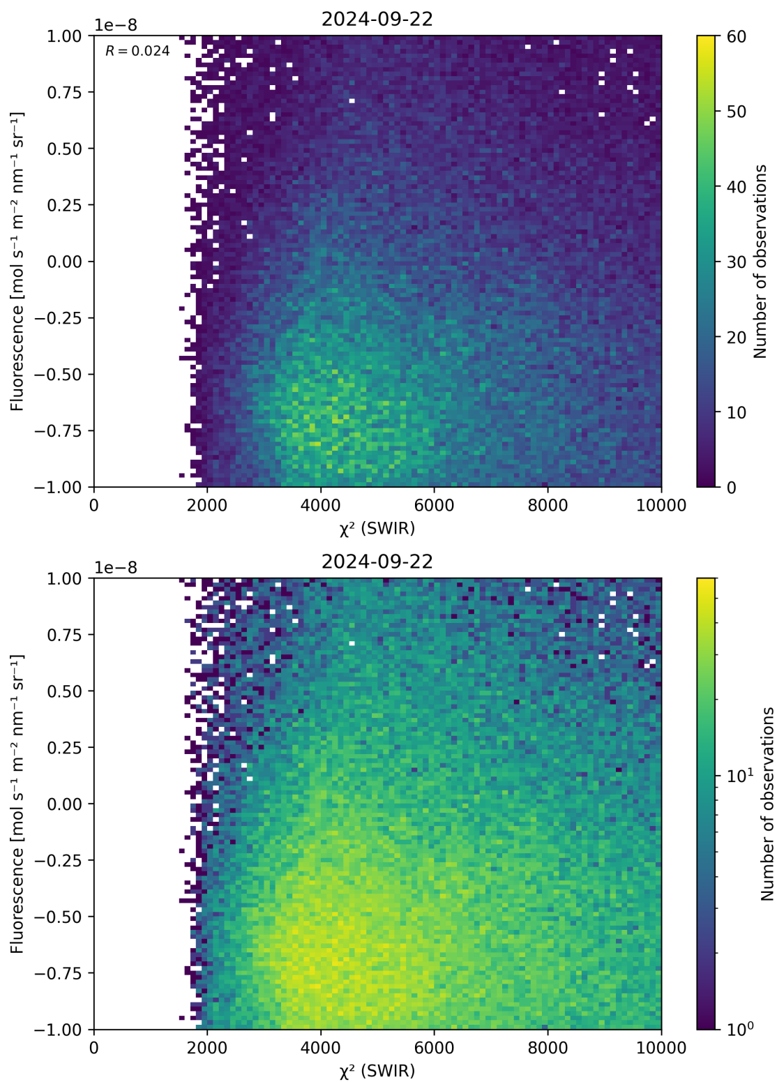
Figure 49: Scatter density plot of “ \chi^2 (SWIR)” against “Fluorescence” for 2024-09-22 to 2024-09-23.
