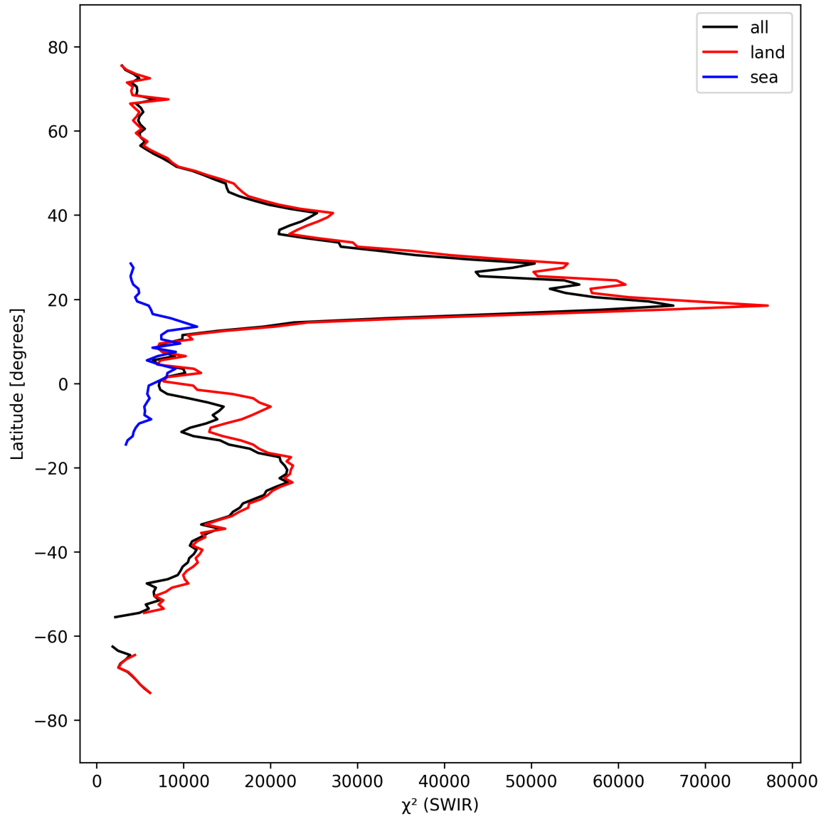
Figure 17: Zonal average of “ \chi^2 (SWIR)” for 2024-09-22 to 2024-09-23.
