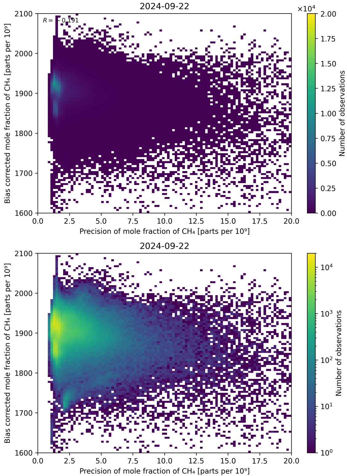
Figure 82: Scatter density plot of “Precision of mole fraction of CH 4 ” against “Bias corrected mole fraction of CH 4 ” for 2024-09-22 to 2024-09-23.
