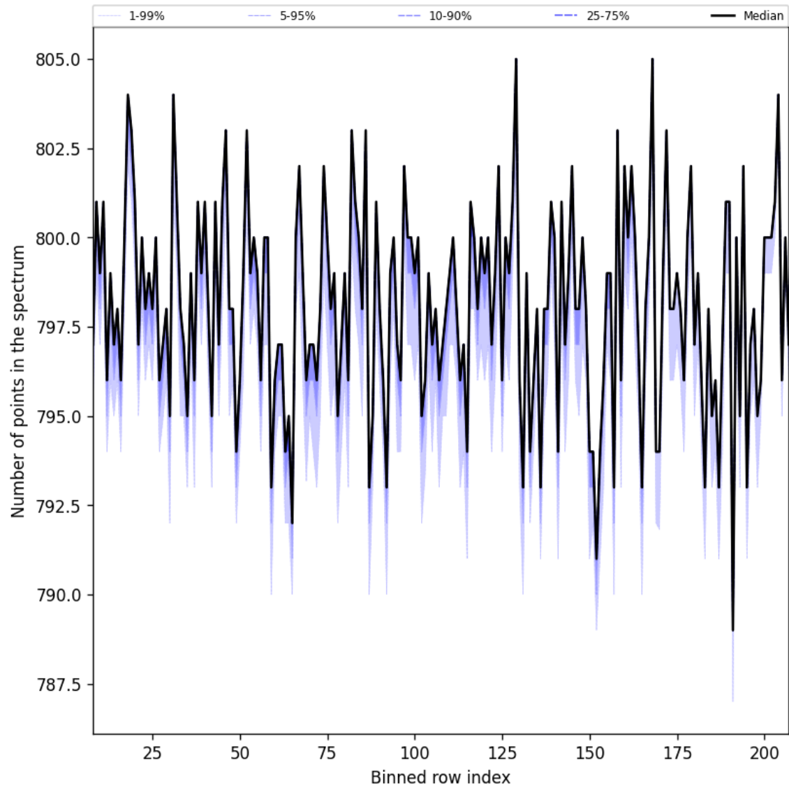
Figure 37: Along track statistics of “Number of points in the spectrum” for 2024-09-22 to 2024-09-23
