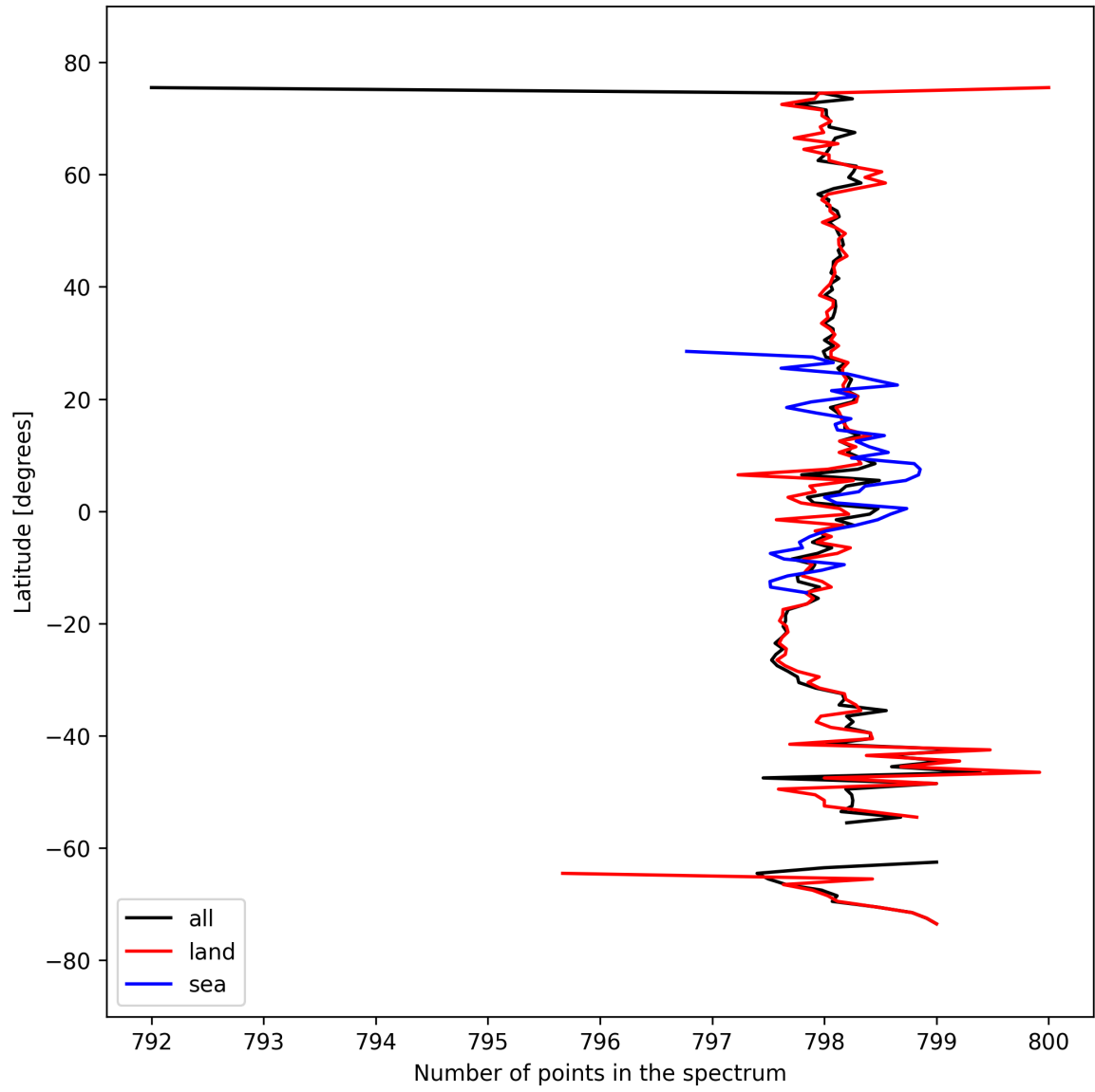
Figure 15: Zonal average of “Number of points in the spectrum” for 2024-09-22 to 2024-09-23.
