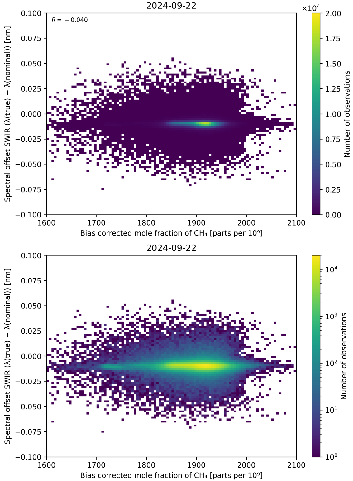
Figure 69: Scatter density plot of “Bias corrected mole fraction of \text{CH}_4 ” against “Spectral offset SWIR ( \lambda_{\text{true}} - \lambda_{\text{nominal}} )” for 2024-09-22 to 2024-09-23.
