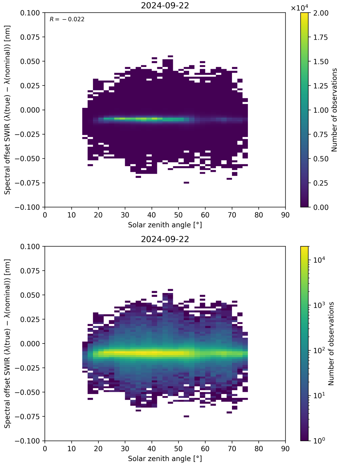
Figure 104: Scatter density plot of “Solar zenith angle” against “Spectral offset SWIR ( \lambda_{\text{true}} - \lambda_{\text{nominal}} )” for 2024-09-22 to 2024-09-23.
