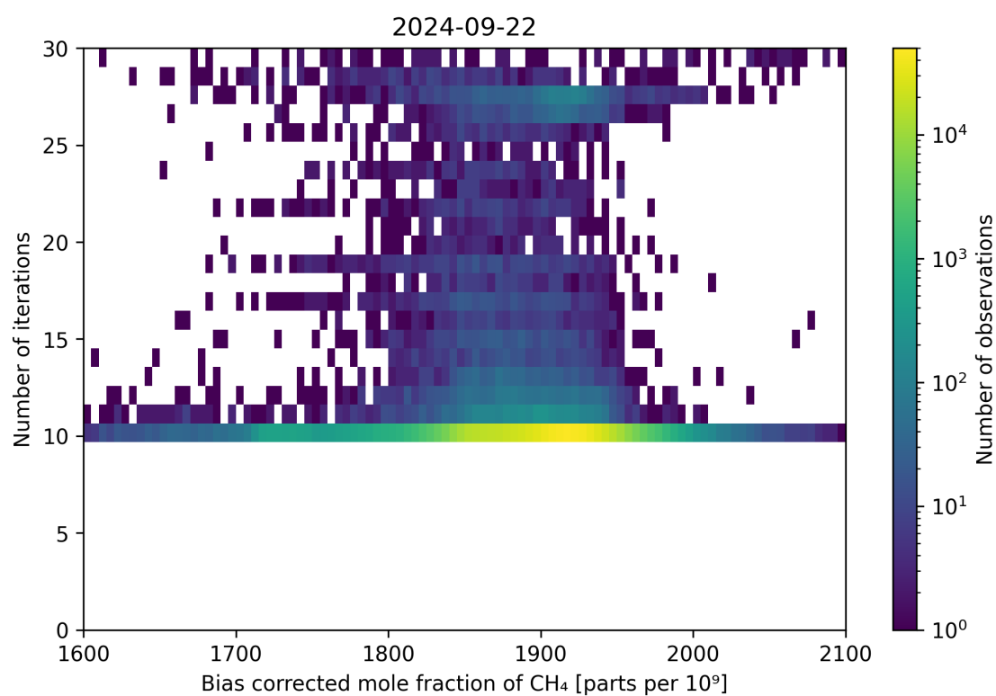
Figure 67: Scatter density plot of “Bias corrected mole fraction of \text{CH}_4 ” against “Number of iterations” for 2024-09-22 to 2024-09-23.
