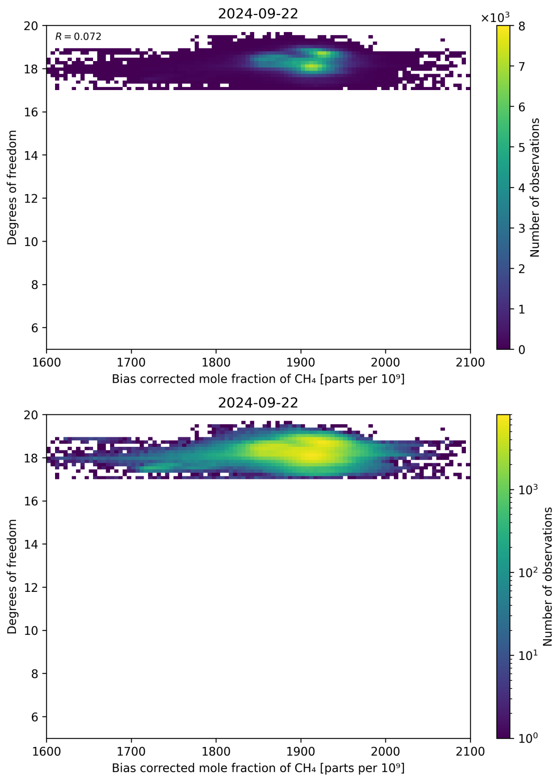
Figure 65: Scatter density plot of “Bias corrected mole fraction of CH 4 ” against “Degrees of freedom” for 2024-09-22 to 2024-09-23.
