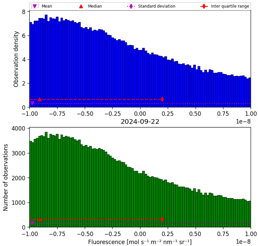
Figure 32: Histogram of “Fluorescence” for 2024-09-22 to 2024-09-23
