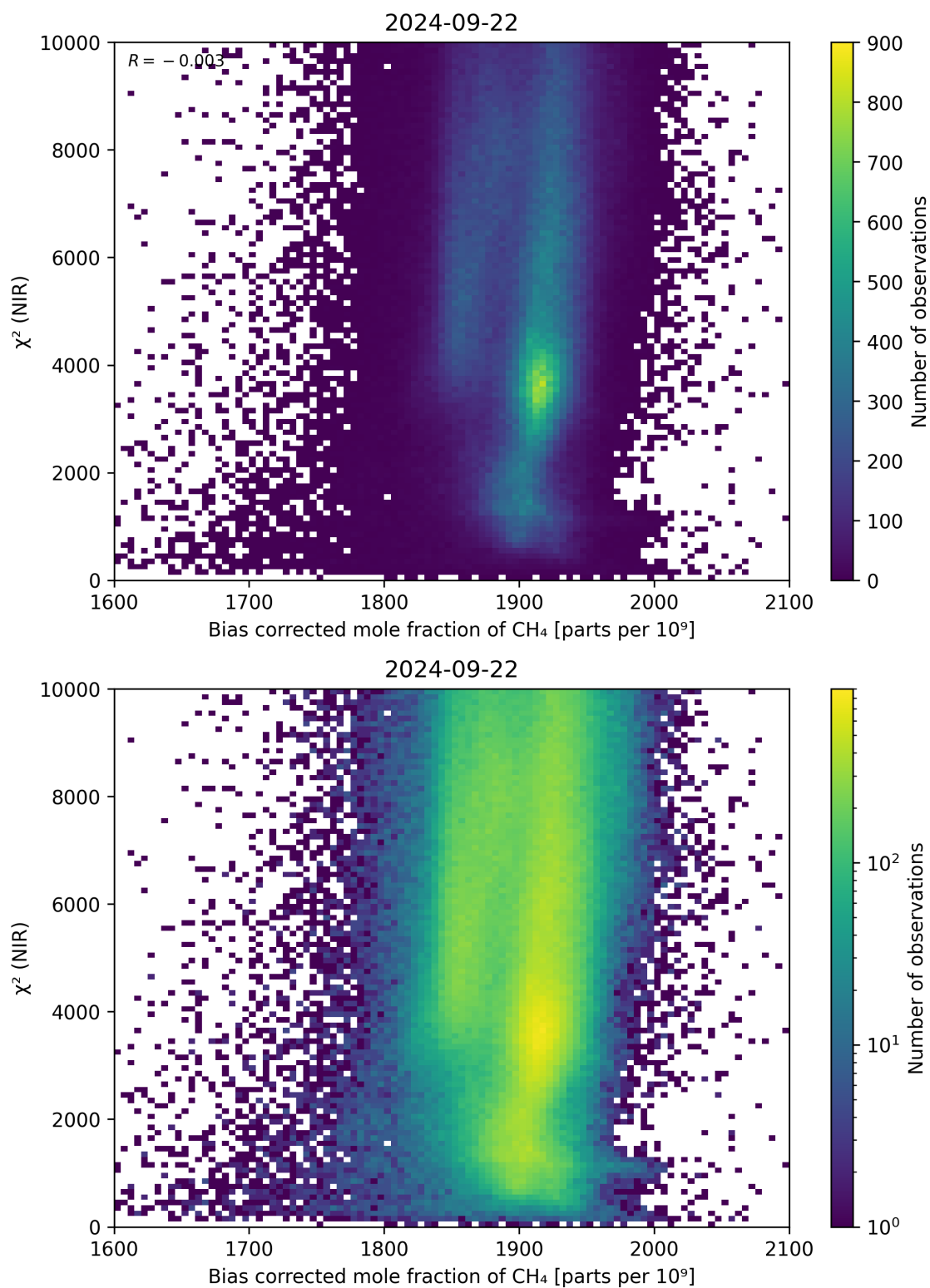
Figure 63: Scatter density plot of “Bias corrected mole fraction of CH 4 ” against “ \chi^2 (NIR)” for 2024-09-22 to 2024-09-23.
