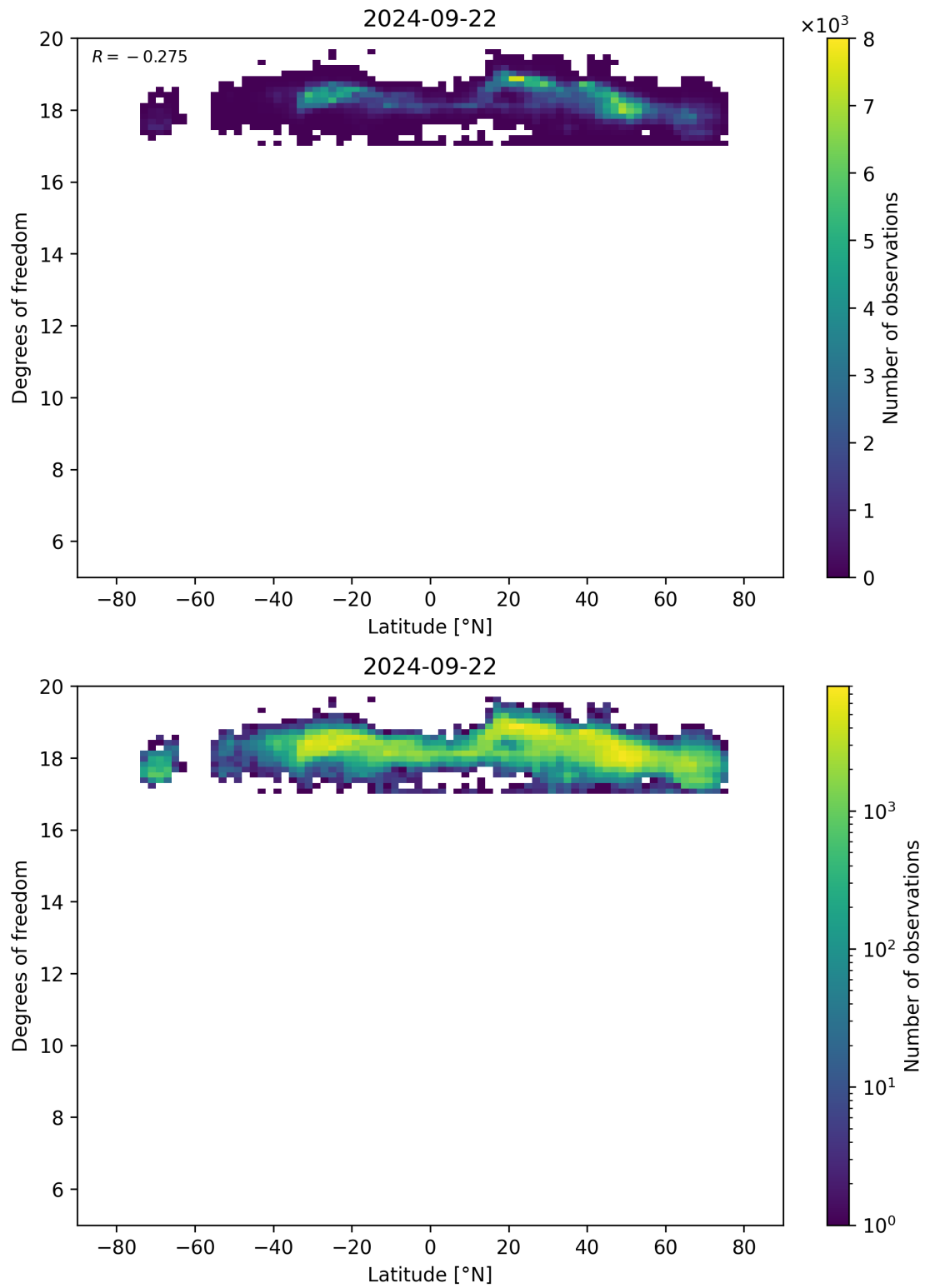
Figure 55: Scatter density plot of “Latitude” against “Degrees of freedom” for 2024-09-22 to 2024-09-23.
