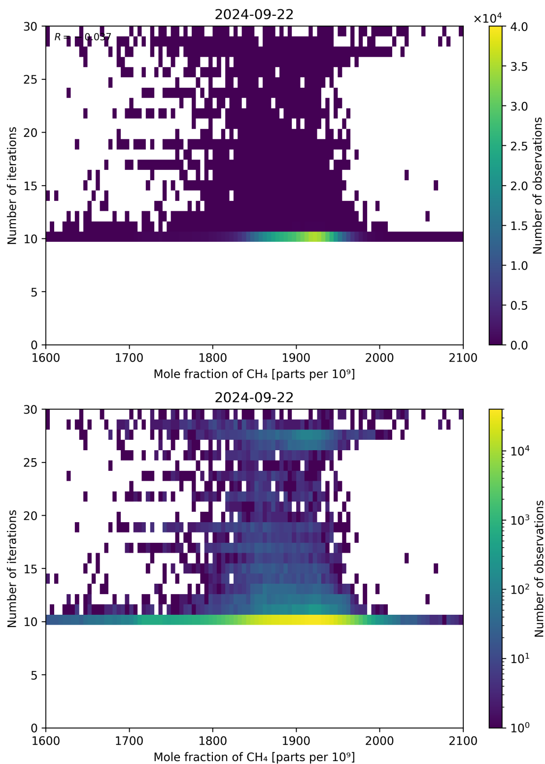
Figure 76: Scatter density plot of “Mole fraction of CH 4 ” against “Number of iterations” for 2024-09-22 to 2024-09-23.
