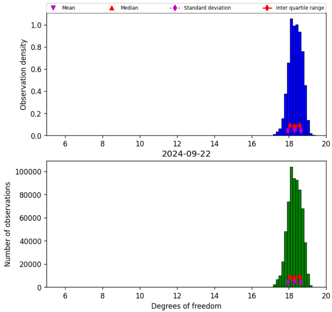
Figure 30: Histogram of “Degrees of freedom” for 2024-09-22 to 2024-09-23
