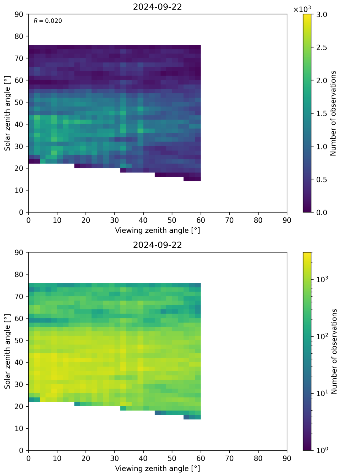
Figure 115: Scatter density plot of “Viewing zenith angle” against “Solar zenith angle” for 2024-09-22 to 2024-09-23.
