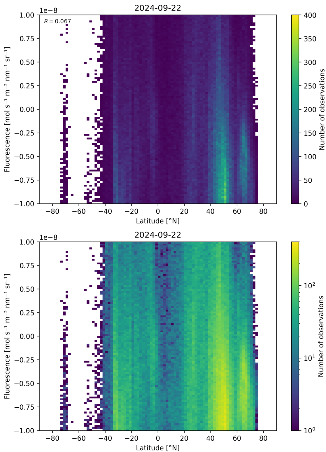
Figure 56: Scatter density plot of “Latitude” against “Fluorescence” for 2024-09-22 to 2024-09-23.
