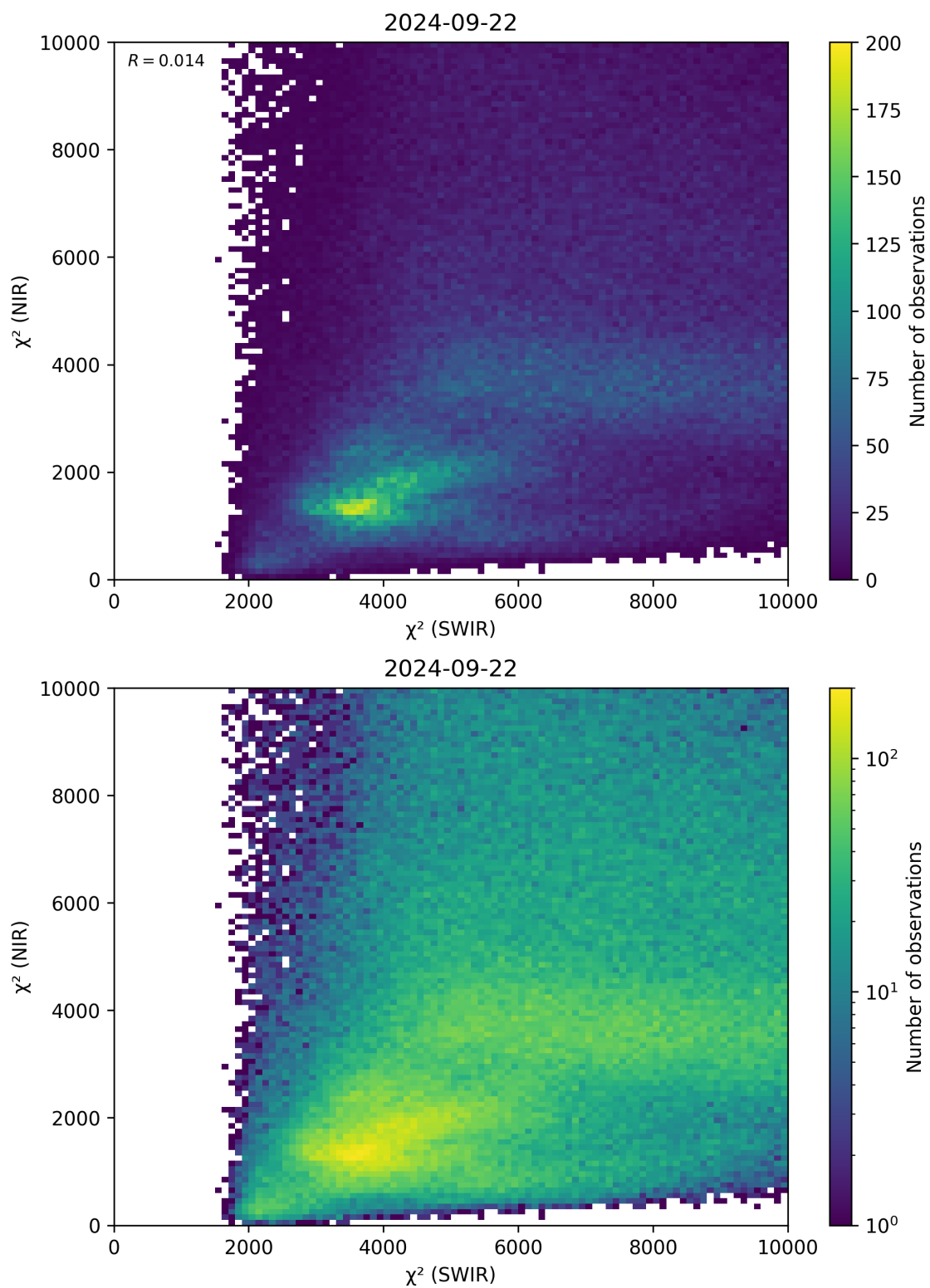
Figure 47: Scatter density plot of “ \chi^2 (SWIR)” against “ \chi^2 (NIR)” for 2024-09-22 to 2024-09-23.
