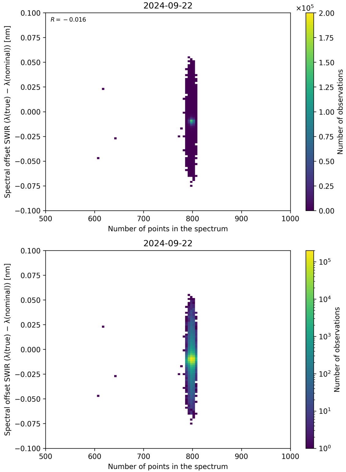
Figure 93: Scatter density plot of “Number of points in the spectrum” against “Spectral offset SWIR ( \lambda_{\text{true}} - \lambda_{\text{nominal}} )” for 2024-09-22 to 2024-09-23.
