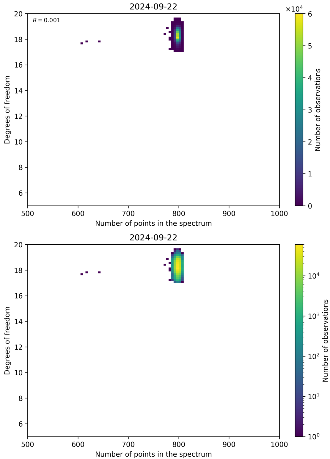
Figure 90: Scatter density plot of “Number of points in the spectrum” against “Degrees of freedom” for 2024-09-22 to 2024-09-23.
