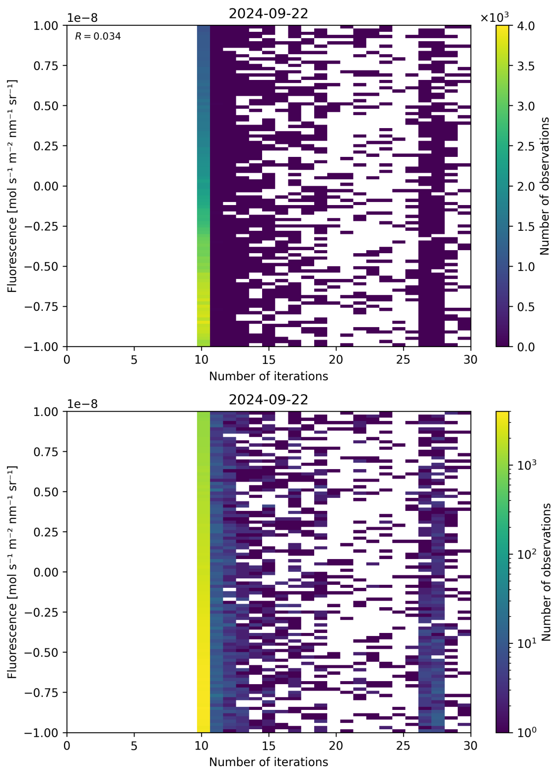
Figure 87: Scatter density plot of “Number of iterations” against “Fluorescence” for 2024-09-22 to 2024-09-23.
