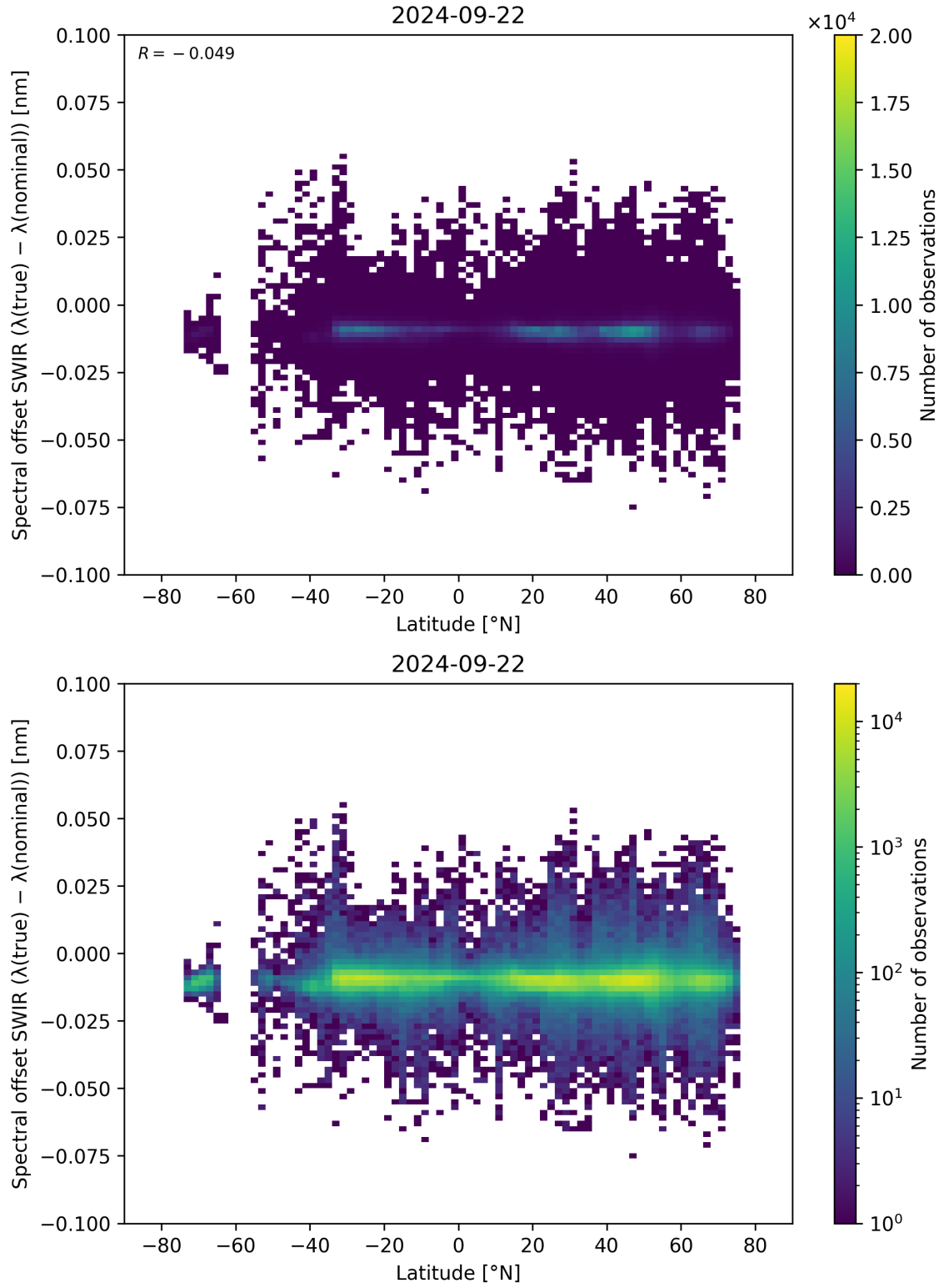
Figure 62: Scatter density plot of “Latitude” against “Spectral offset SWIR ( \lambda_{\text{true}} - \lambda_{\text{nominal}} )” for 2024-09-22 to 2024-09-23.
