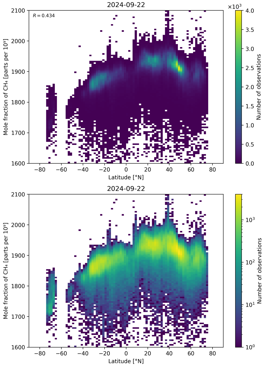
Figure 57: Scatter density plot of “Latitude” against “Mole fraction of \text{CH}_4 ” for 2024-09-22 to 2024-09-23.
