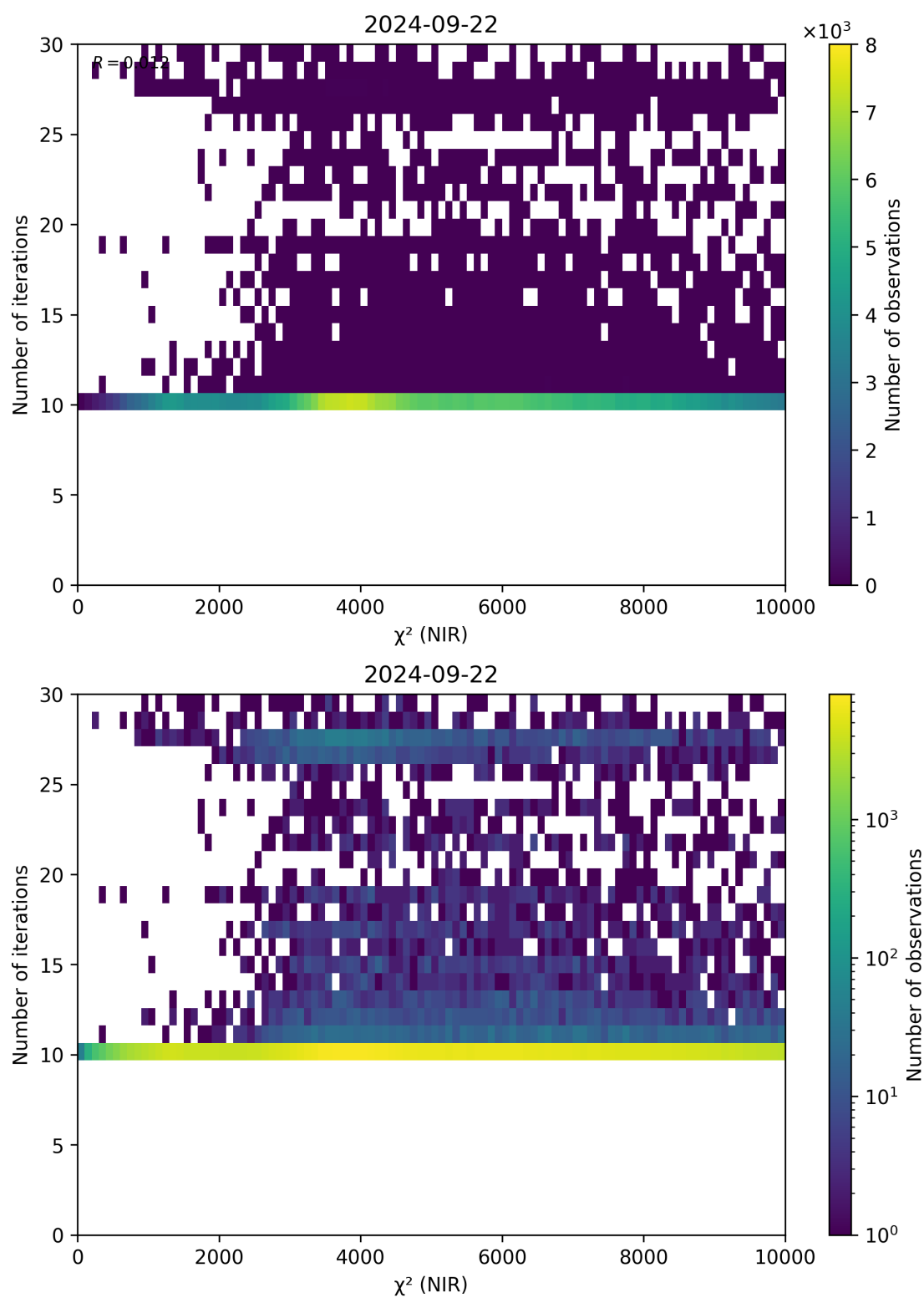
Figure 46: Scatter density plot of “ \chi^2 (NIR)” against “Number of iterations” for 2024-09-22 to 2024-09-23.
