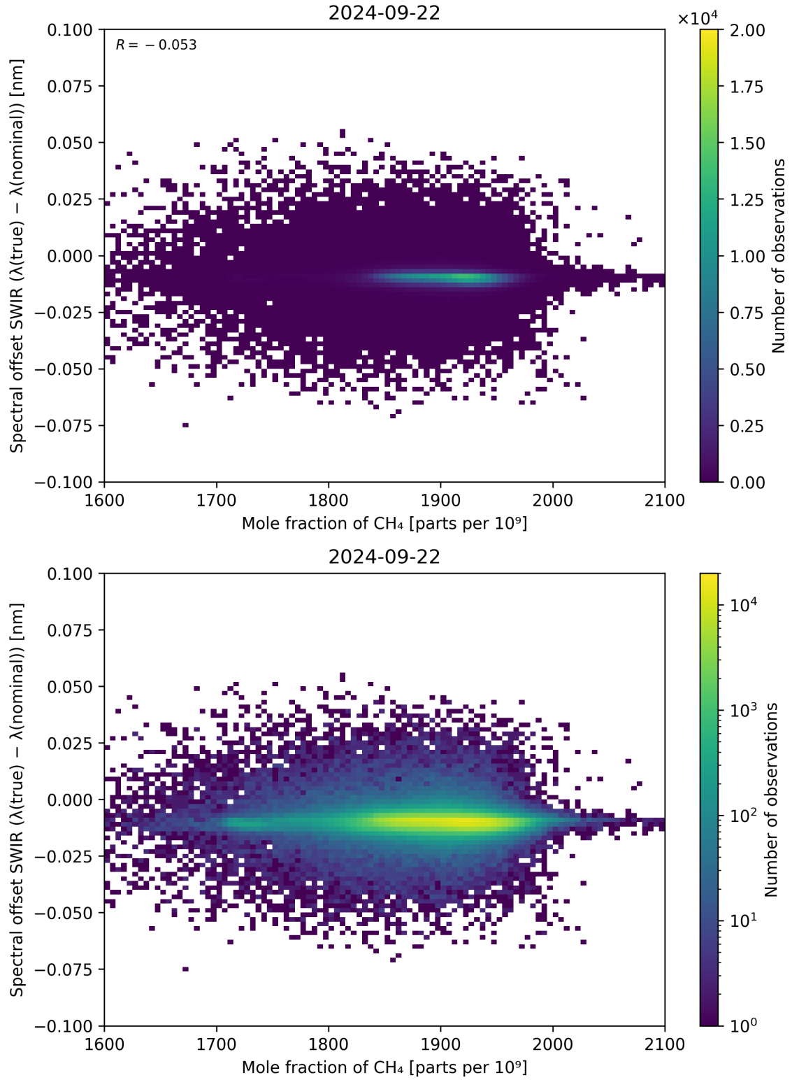
Figure 86: Scatter density plot of “Mole fraction of CH 4 ” against “Spectral offset SWIR ( \lambda_{\text{true}} - \lambda_{\text{nominal}} )” for 2024-09-22 to 2024-09-23.
