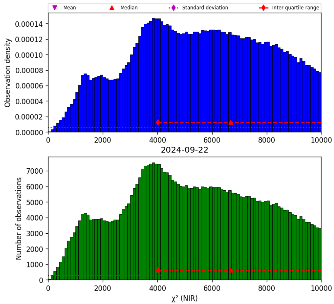
Figure 29: Histogram of " \chi^2 (NIR)" for 2024-09-22 to 2024-09-23
