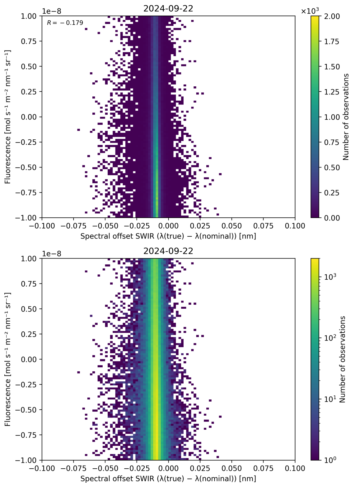
Figure 120: Scatter density plot of “Spectral offset SWIR ( \lambda_{\text{true}} - \lambda_{\text{nominal}} )” against “Fluorescence” for 2024-09-22 to 2024-09-23.
