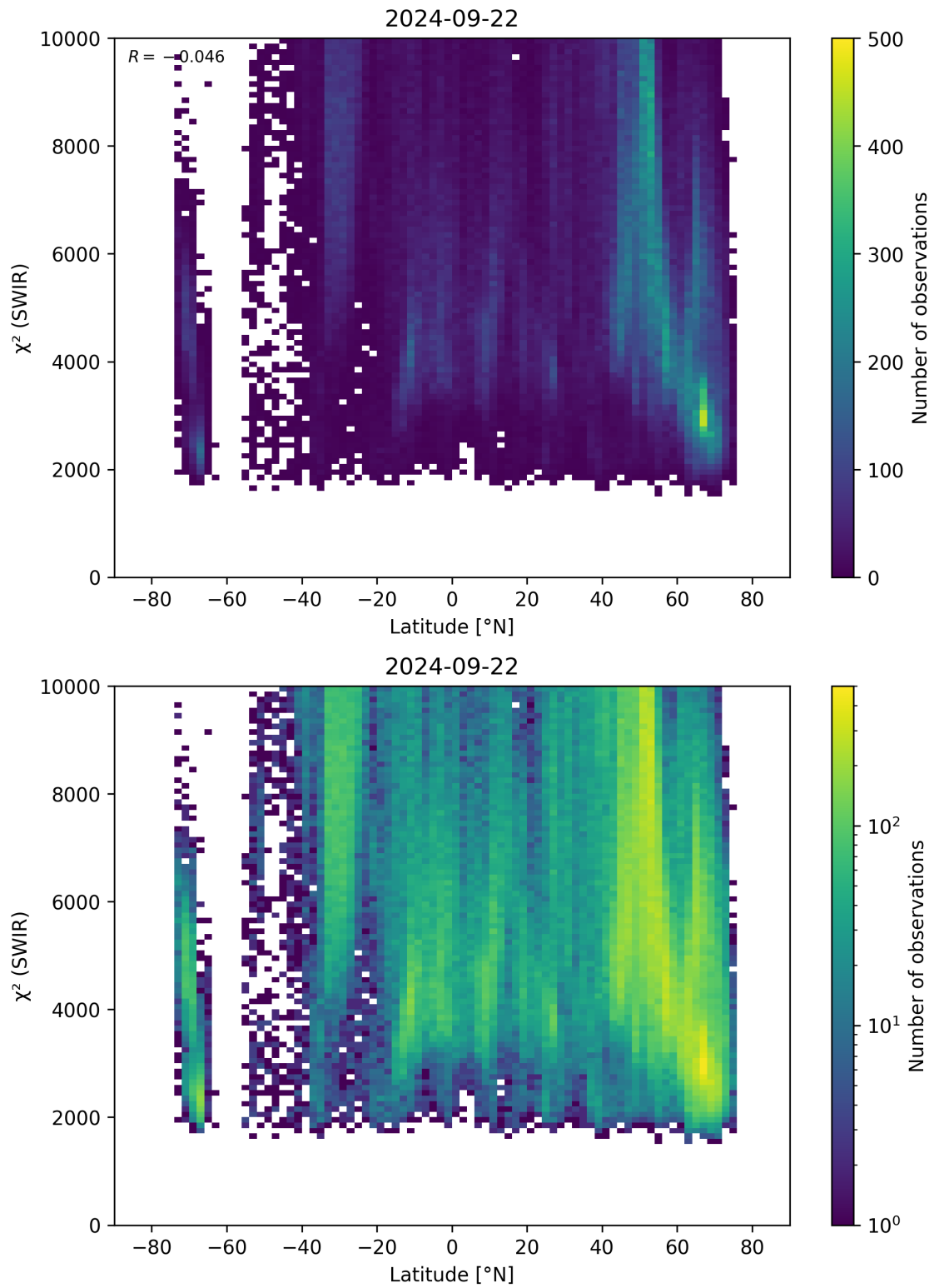
Figure 54: Scatter density plot of “Latitude” against “ \chi^2 (SWIR)” for 2024-09-22 to 2024-09-23.
