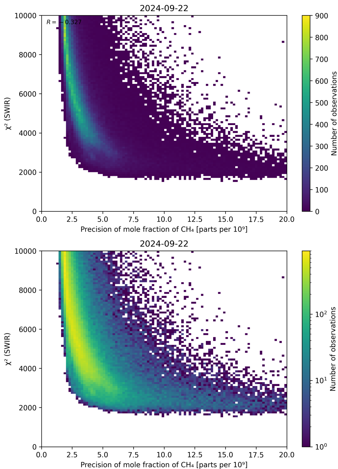
Figure 79: Scatter density plot of “Precision of mole fraction of \text{CH}_4 ” against “ \chi^2 (SWIR)” for 2024-09-22 to 2024-09-23.
