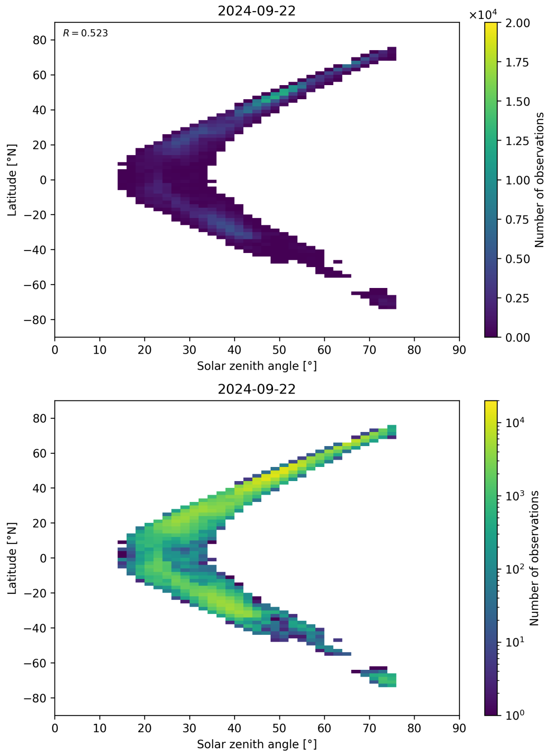
Figure 98: Scatter density plot of “Solar zenith angle” against “Latitude” for 2024-09-22 to 2024-09-23.
