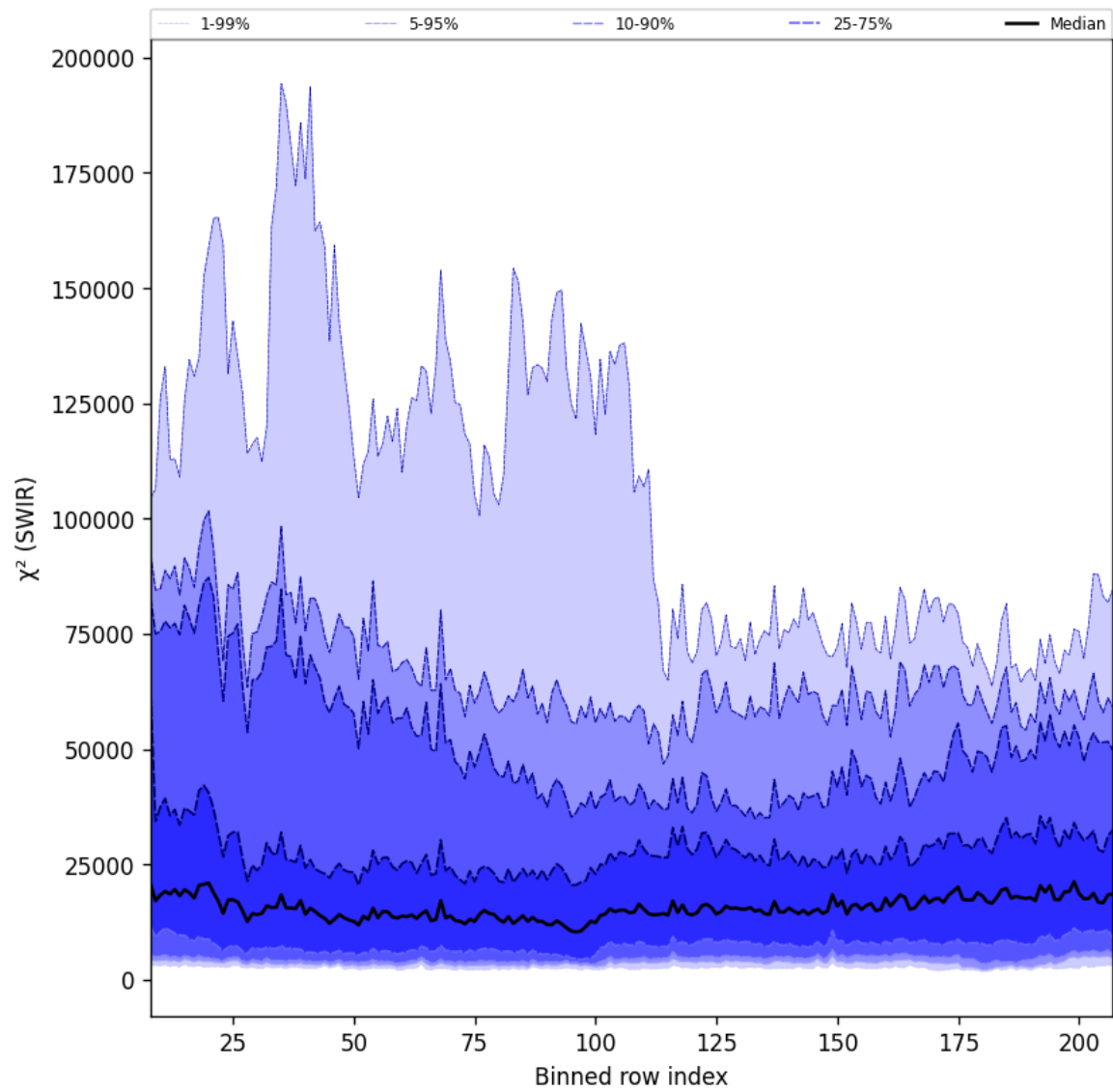
Figure 39: Along track statistics of “ \chi^2 (SWIR)” for 2024-09-22 to 2024-09-23
