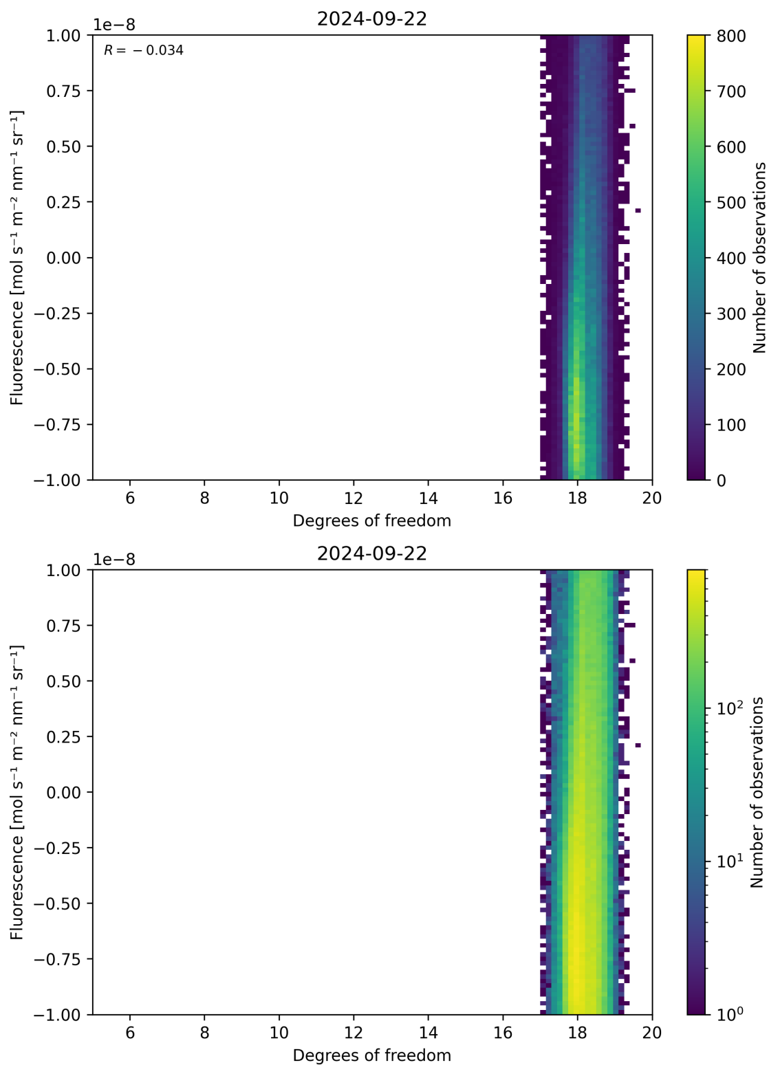
Figure 51: Scatter density plot of “Degrees of freedom” against “Fluorescence” for 2024-09-22 to 2024-09-23.
