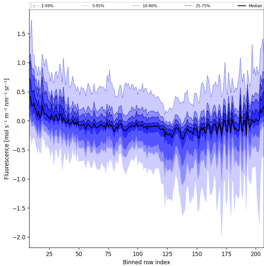
Figure 43: Along track statistics of "Fluorescence" for 2024-09-22 to 2024-09-23
