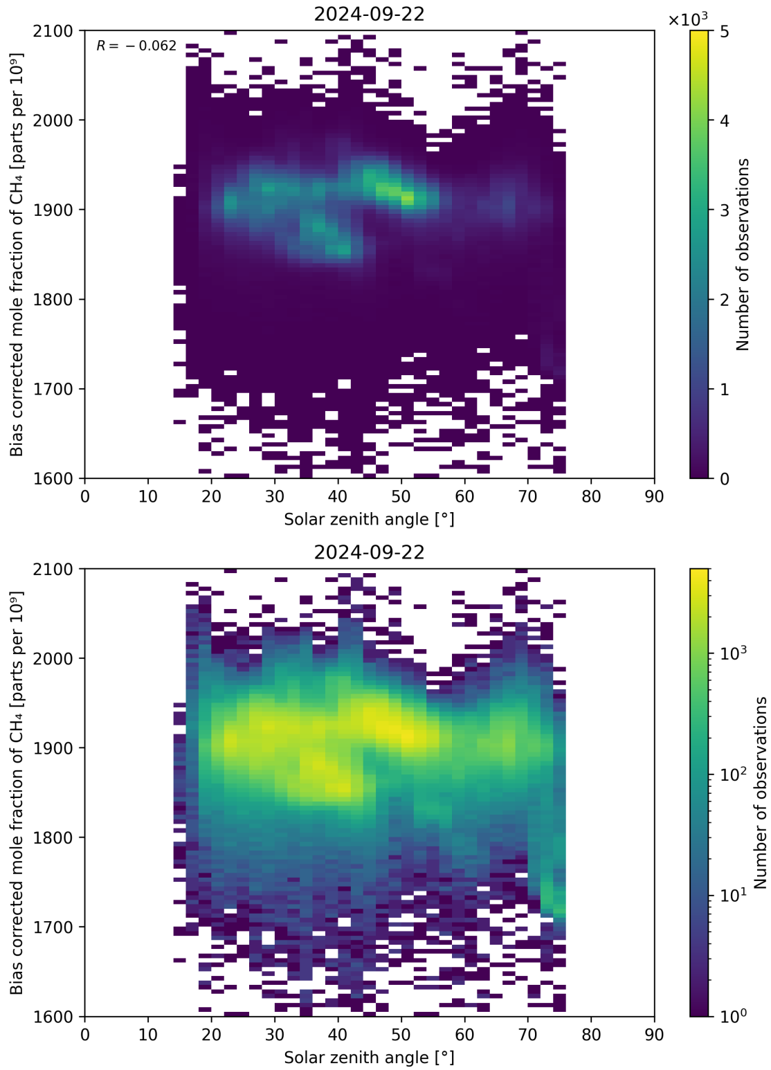
Figure 100: Scatter density plot of “Solar zenith angle” against “Bias corrected mole fraction of \text{CH}_4 ” for 2024-09-22 to 2024-09-23.
