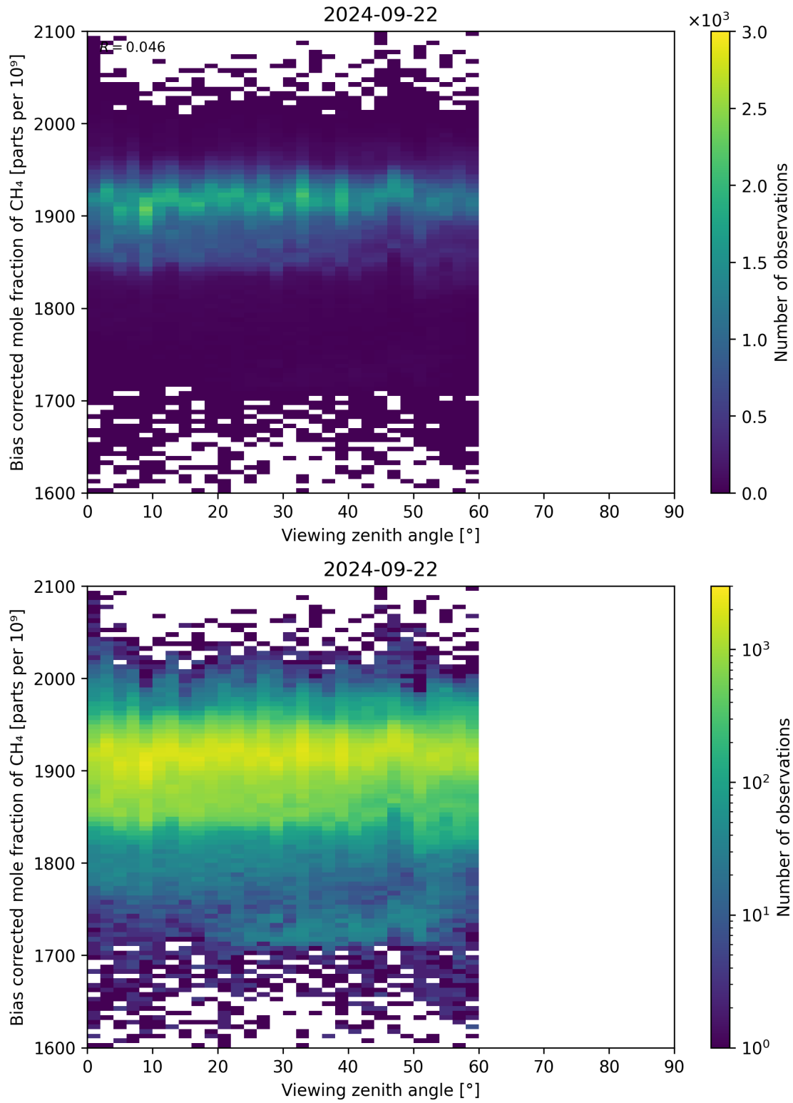
Figure 111: Scatter density plot of “Viewing zenith angle” against “Bias corrected mole fraction of CH 4 ” for 2024-09-22 to 2024-09-23.
