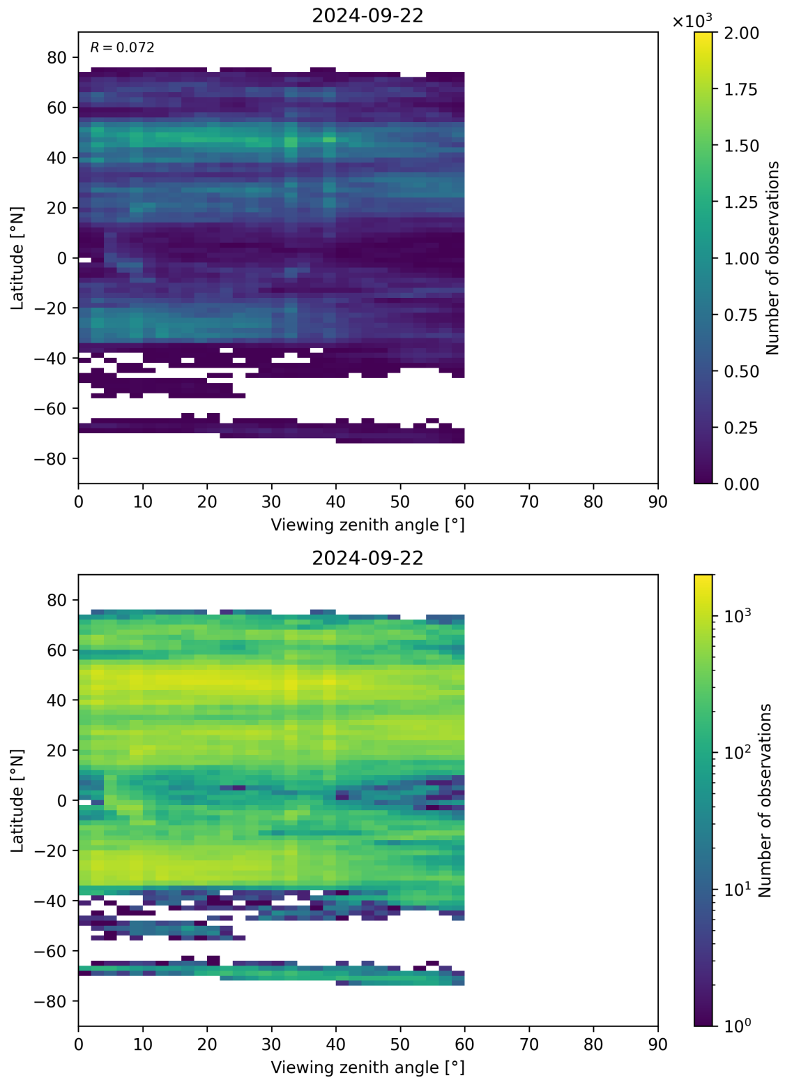
Figure 109: Scatter density plot of “Viewing zenith angle” against “Latitude” for 2024-09-22 to 2024-09-23.
