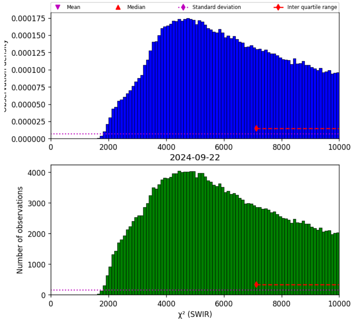
Figure 28: Histogram of “ \chi^2 (SWIR)” for 2024-09-22 to 2024-09-23
