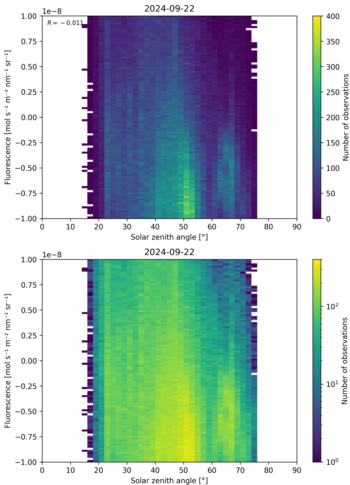
Figure 97: Scatter density plot of “Solar zenith angle” against “Fluorescence” for 2024-09-22 to 2024-09-23.
