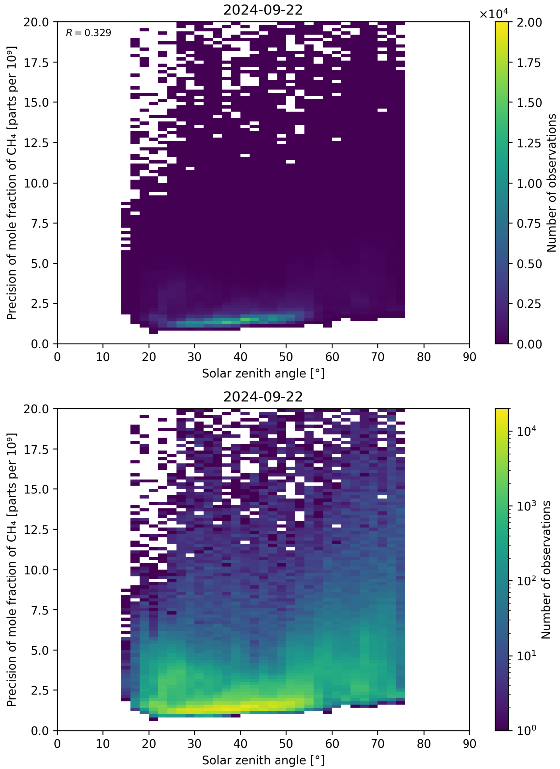
Figure 101: Scatter density plot of “Solar zenith angle” against “Precision of mole fraction of \text{CH}_4 ” for 2024-09-22 to 2024-09-23.
