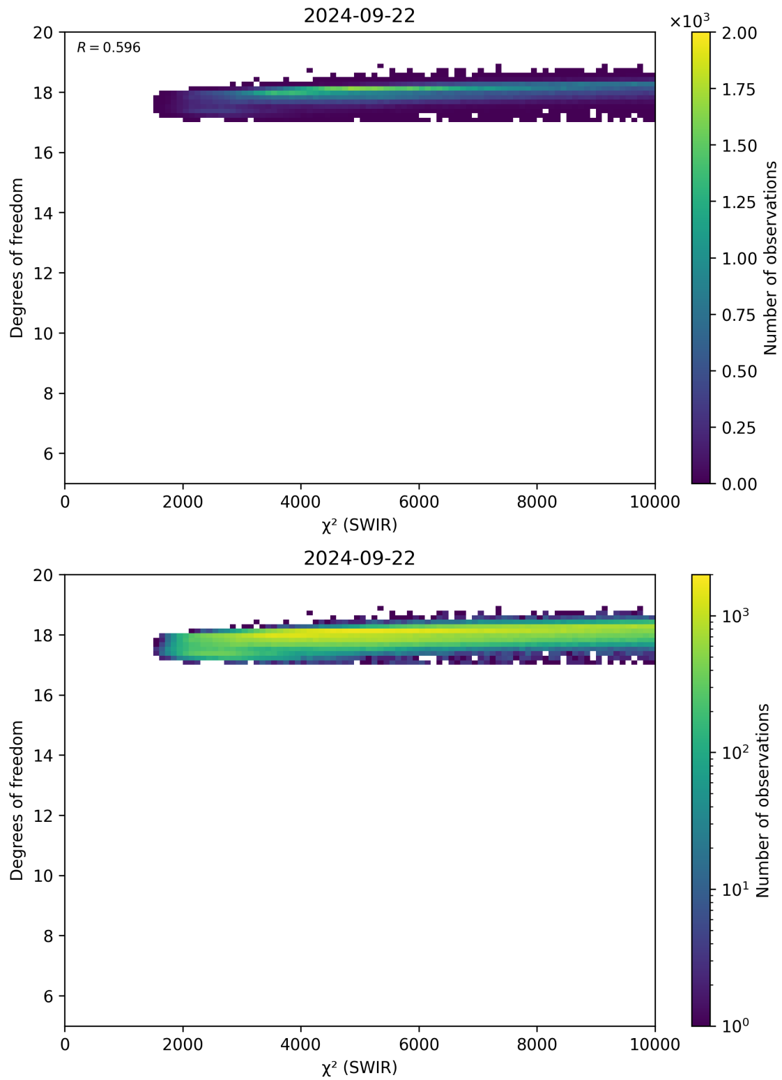
Figure 48: Scatter density plot of “ \chi^2 (SWIR)” against “Degrees of freedom” for 2024-09-22 to 2024-09-23.
