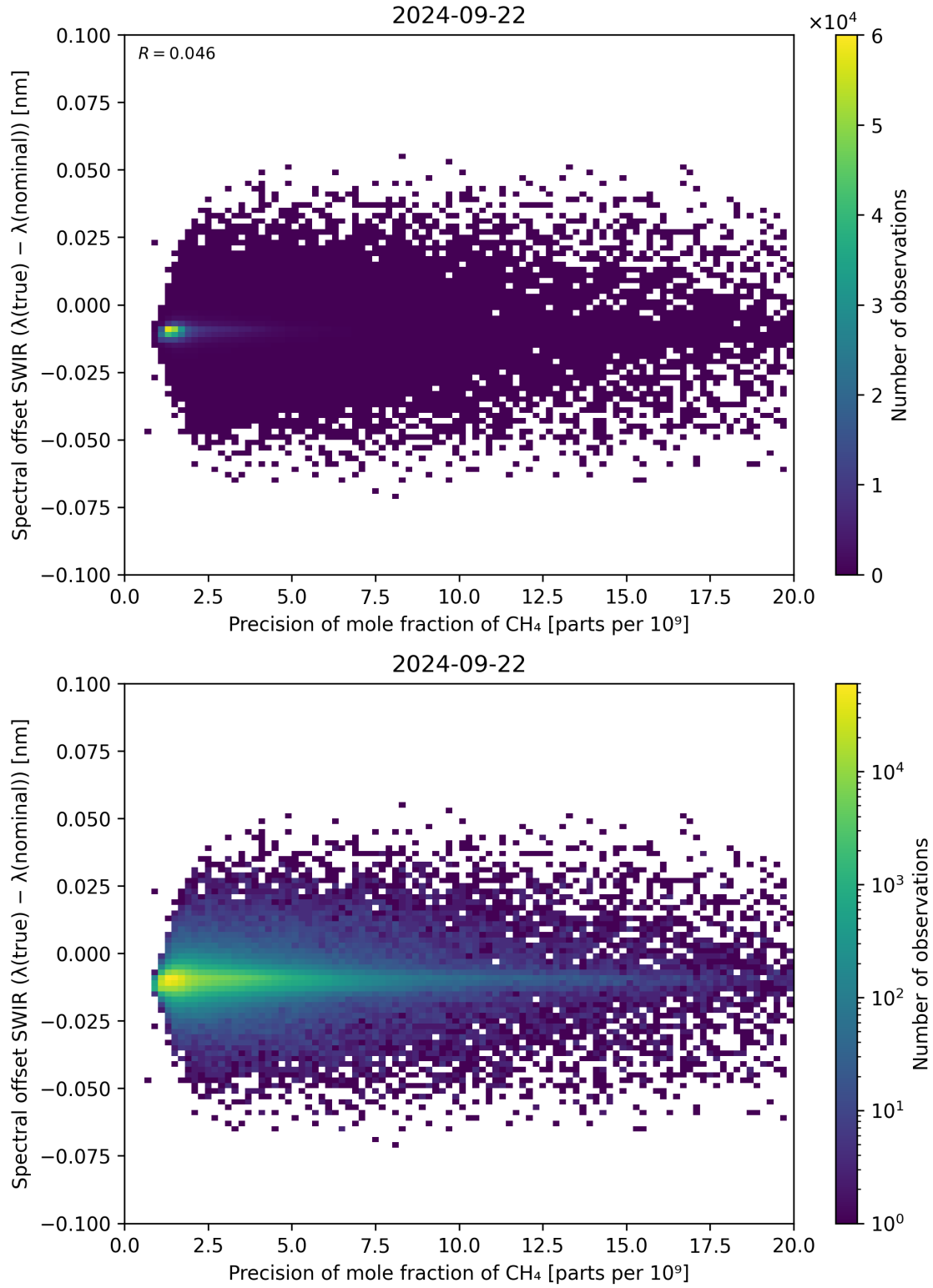
Figure 85: Scatter density plot of “Precision of mole fraction of CH 4 ” against “Spectral offset SWIR ( \lambda_{\text{true}} - \lambda_{\text{nominal}} )” for 2024-09-22 to 2024-09-23.
