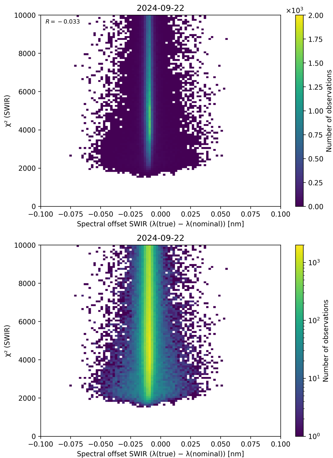
Figure 118: Scatter density plot of “Spectral offset SWIR ( \lambda_{\text{true}} - \lambda_{\text{nominal}} )” against “ \chi^2 (SWIR)” for 2024-09-22 to 2024-09-23.
