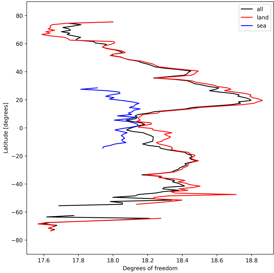
Figure 19: Zonal average of “Degrees of freedom” for 2024-09-22 to 2024-09-23.
