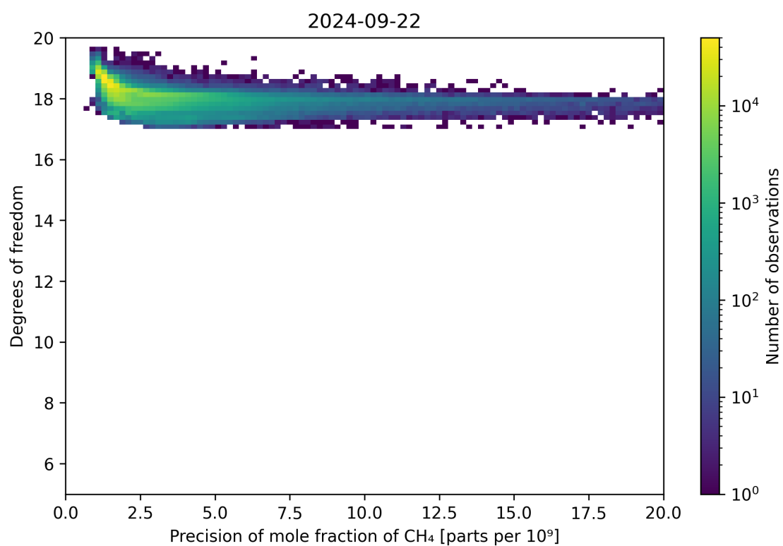
Figure 80: Scatter density plot of “Precision of mole fraction of CH 4 ” against “Degrees of freedom” for 2024-09-22 to 2024-09-23.
