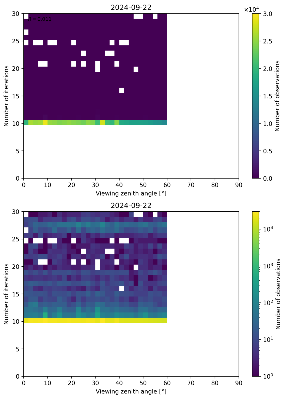
Figure 113: Scatter density plot of “Viewing zenith angle” against “Number of iterations” for 2024-09-22 to 2024-09-23.
