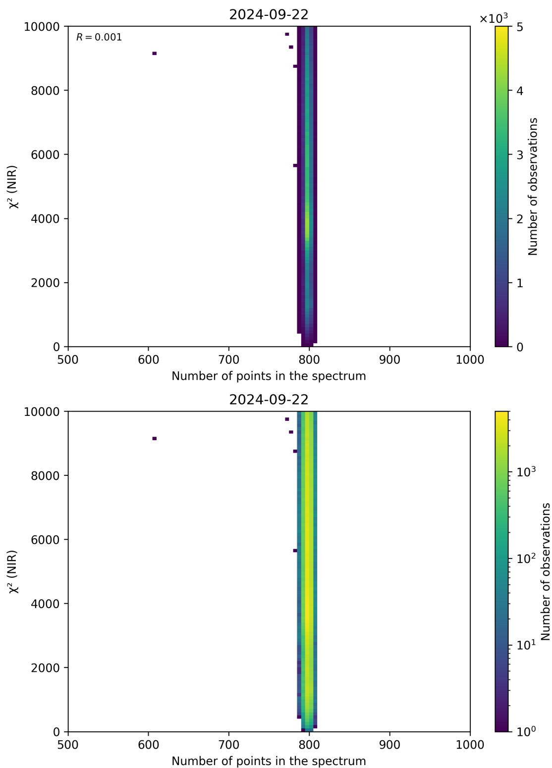
Figure 88: Scatter density plot of “Number of points in the spectrum” against “ \chi^2 (NIR)” for 2024-09-22 to 2024-09-23.
