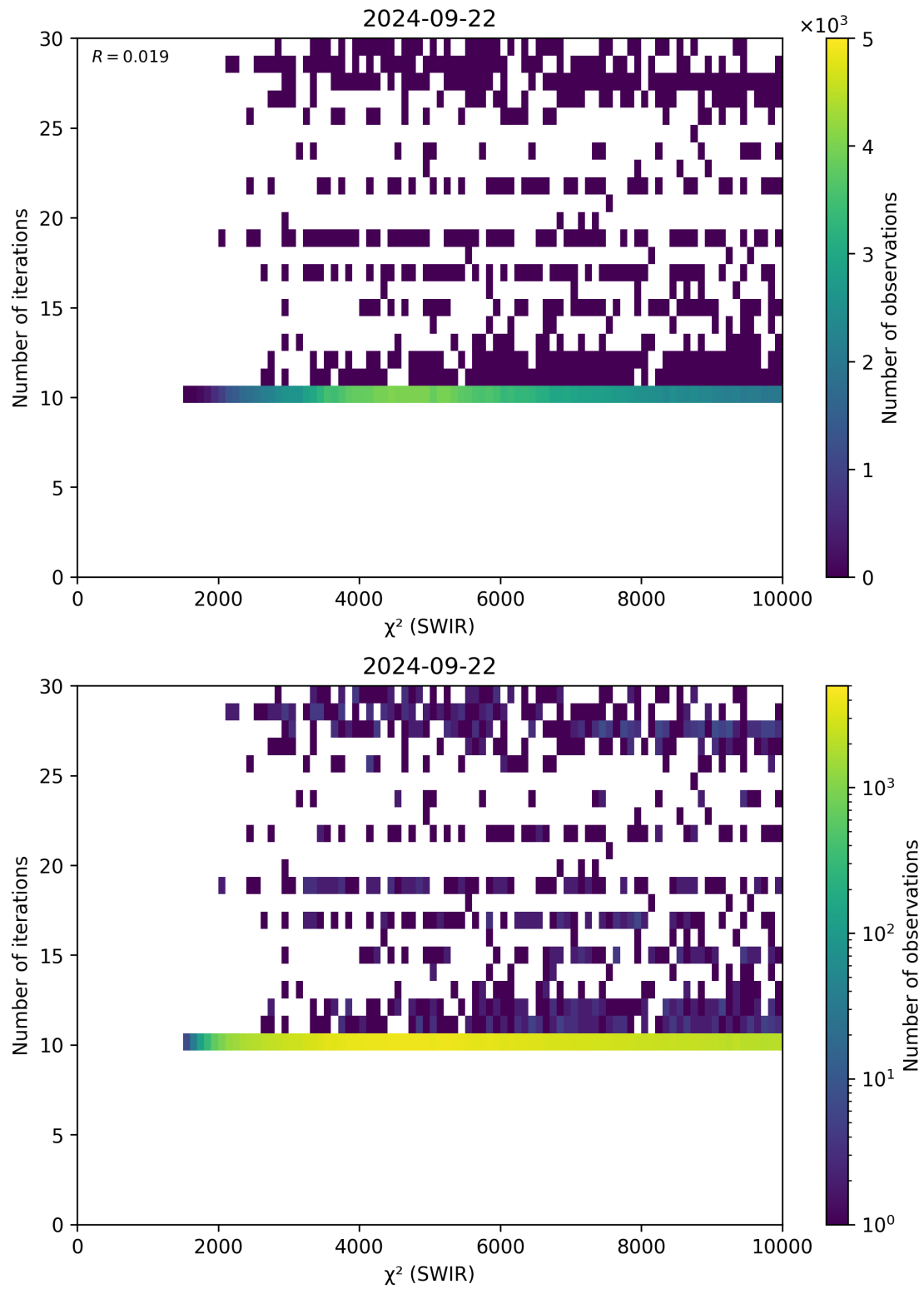
Figure 50: Scatter density plot of “ \chi^2 (SWIR)” against “Number of iterations” for 2024-09-22 to 2024-09-23.
