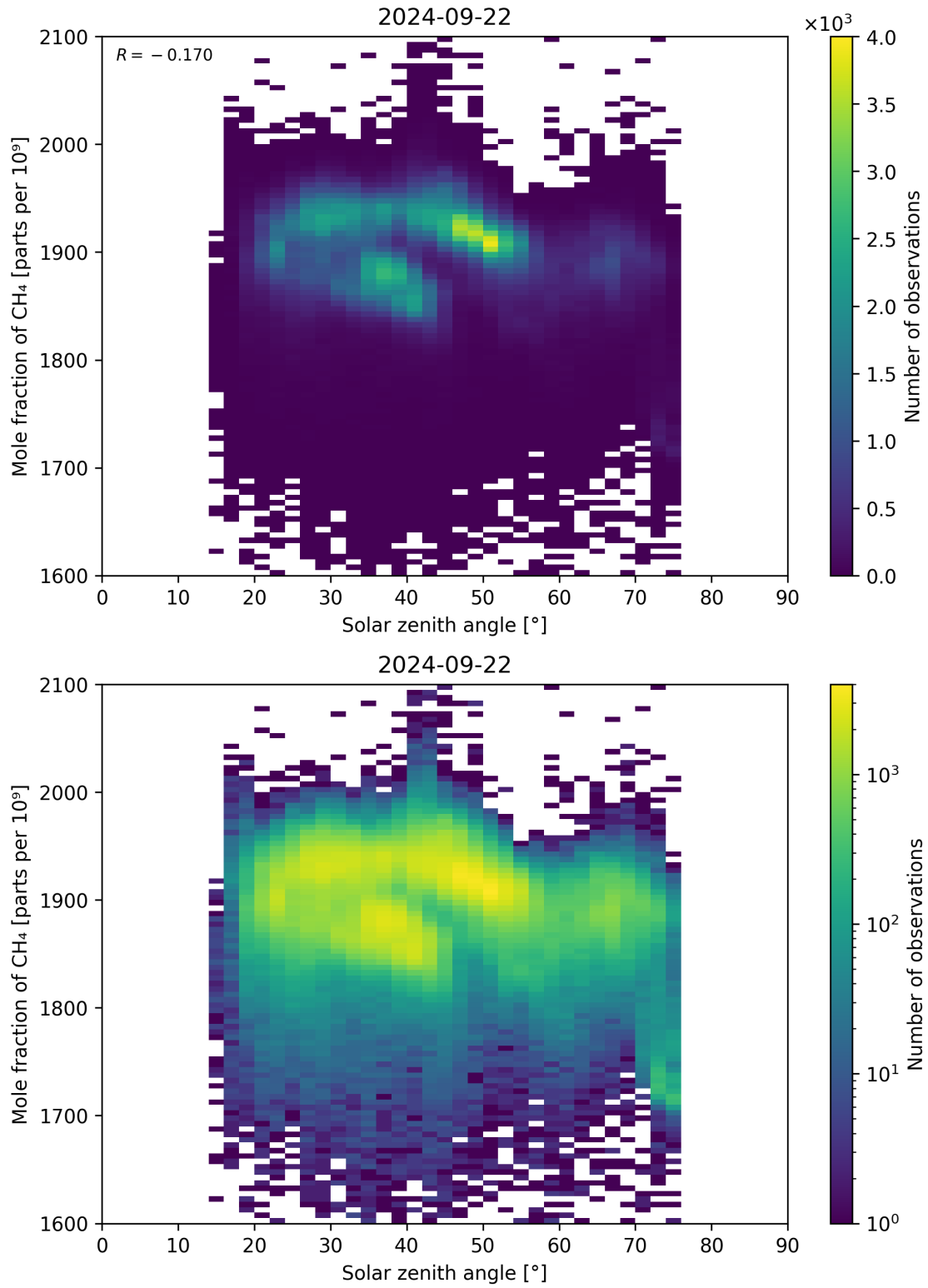
Figure 99: Scatter density plot of “Solar zenith angle” against “Mole fraction of CH 4 ” for 2024-09-22 to 2024-09-23.
