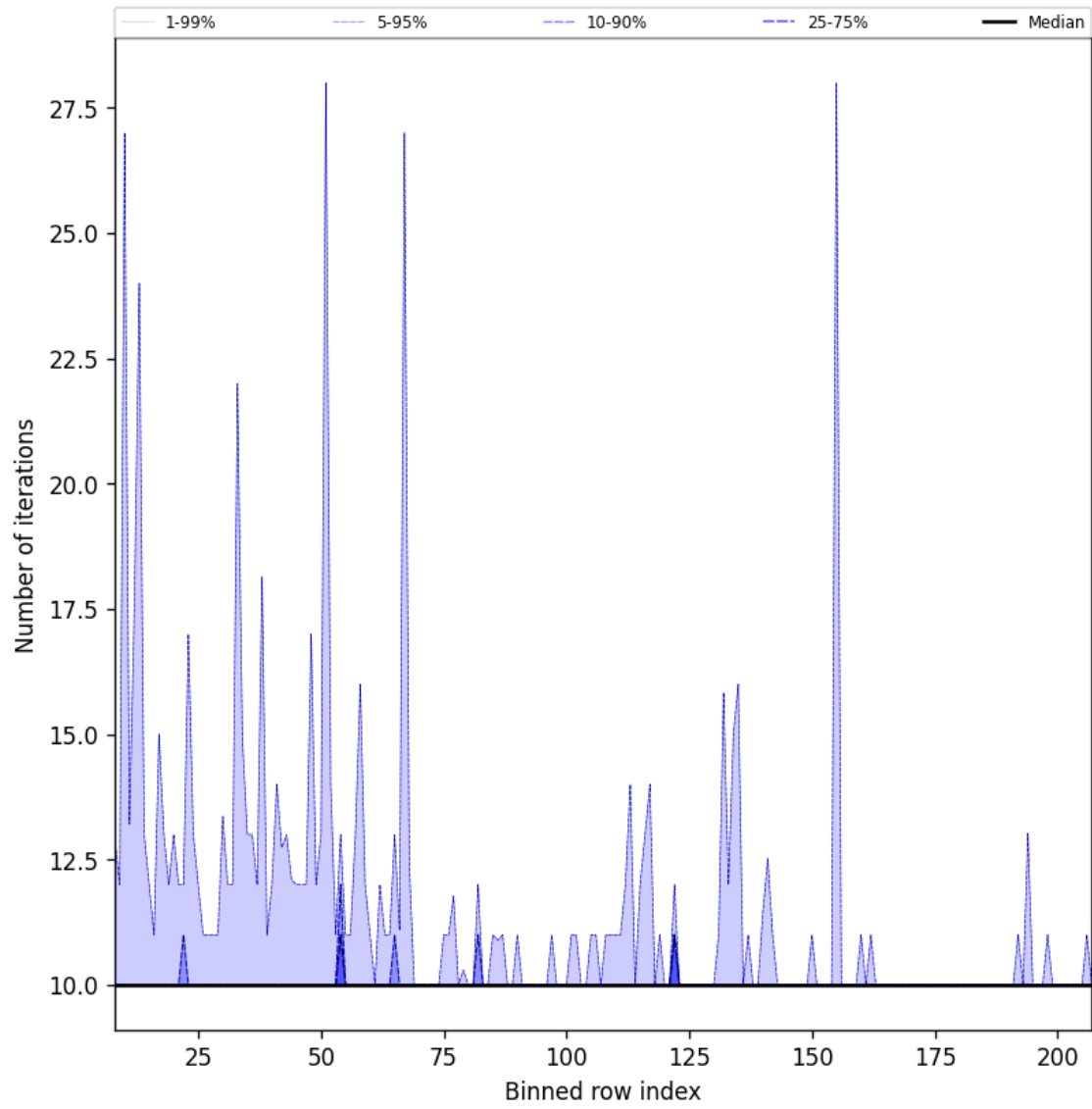
Figure 42: Along track statistics of “Number of iterations” for 2024-09-22 to 2024-09-23
