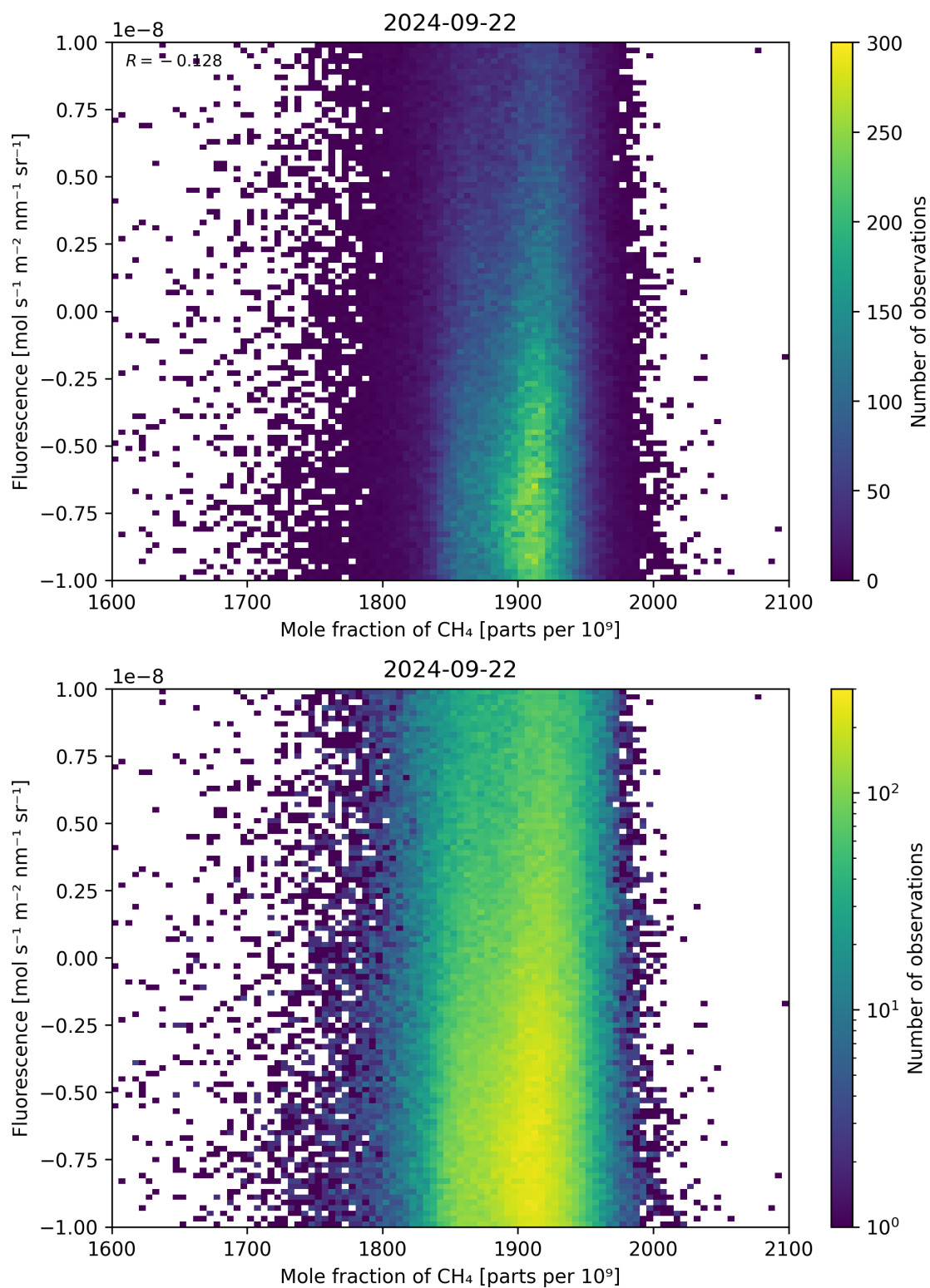
Figure 73: Scatter density plot of “Mole fraction of \text{CH}_4 ” against “Fluorescence” for 2024-09-22 to 2024-09-23.
