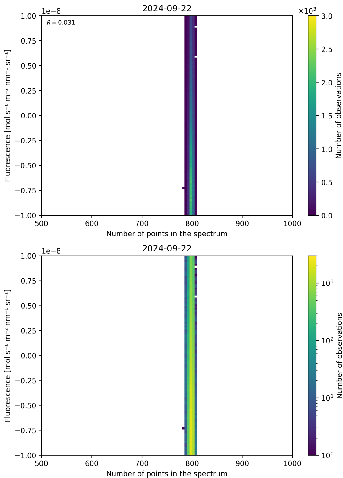
Figure 91: Scatter density plot of “Number of points in the spectrum” against “Fluorescence” for 2024-09-22 to 2024-09-23.
