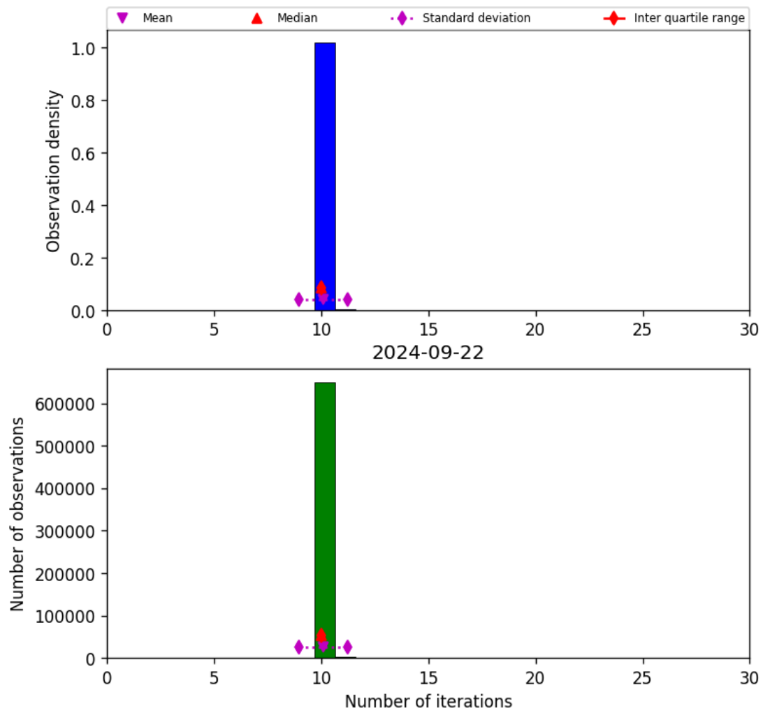
Figure 31: Histogram of “Number of iterations” for 2024-09-22 to 2024-09-23
