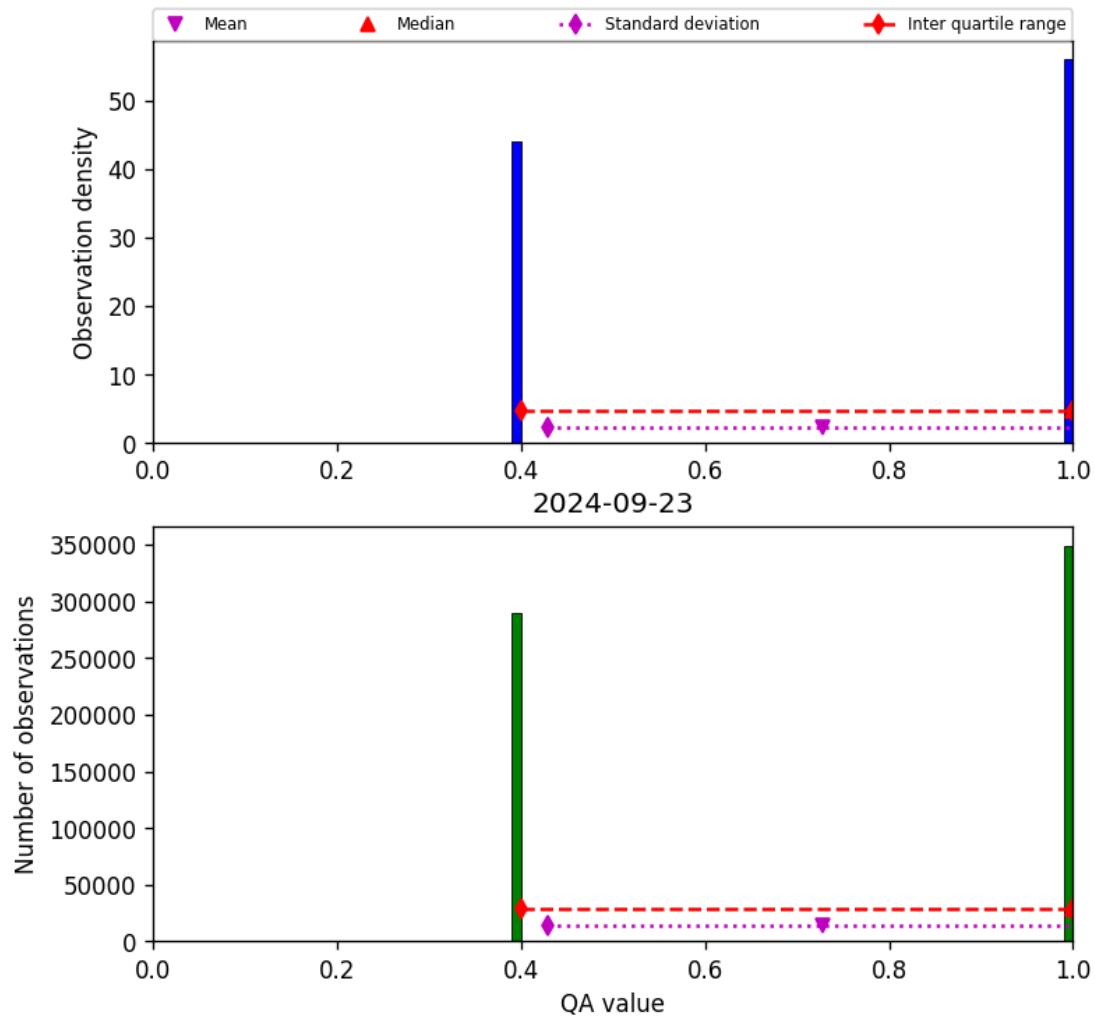
Figure 22: Histogram of “QA value” for 2024-09-22 to 2024-09-24
