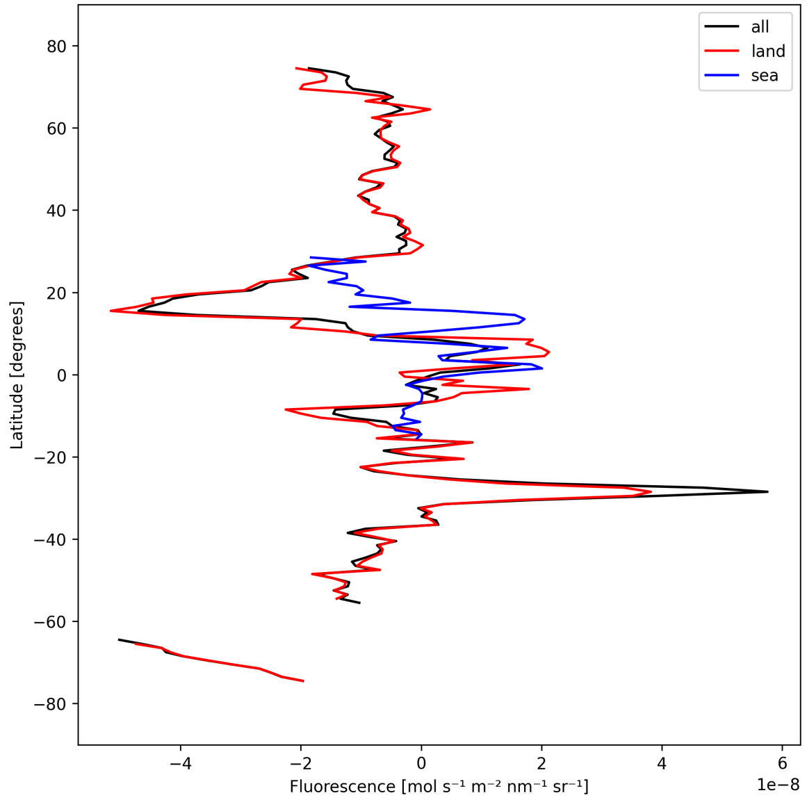
Figure 21: Zonal average of “Fluorescence” for 2024-09-22 to 2024-09-24.
