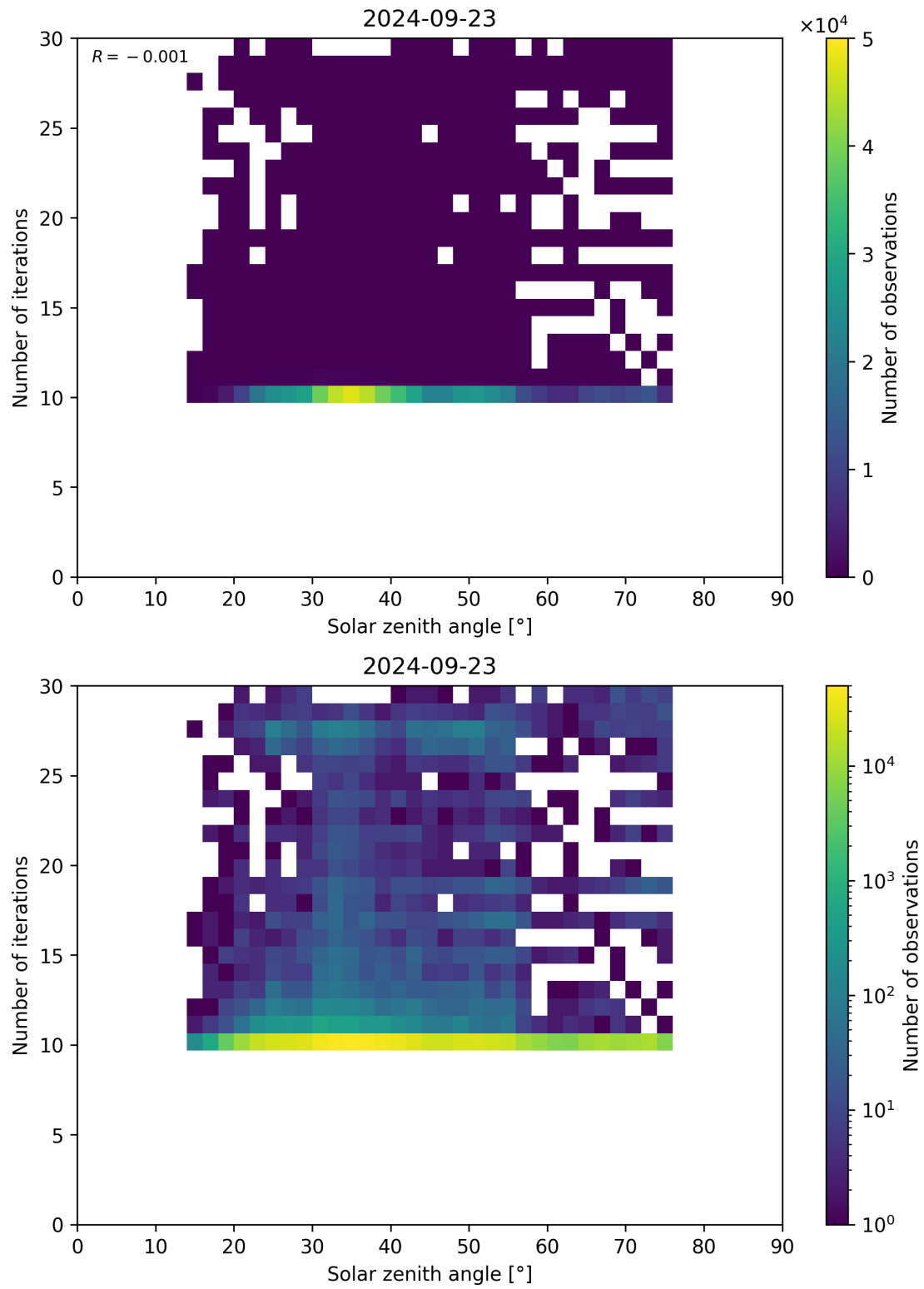
Figure 102: Scatter density plot of “Solar zenith angle” against “Number of iterations” for 2024-09-22 to 2024-09-24.
