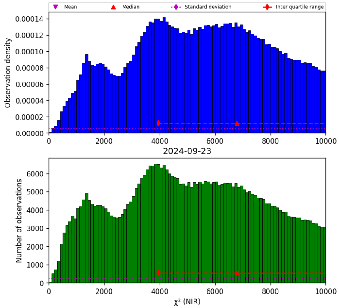
Figure 29: Histogram of " \chi^2 (NIR)" for 2024-09-22 to 2024-09-24
