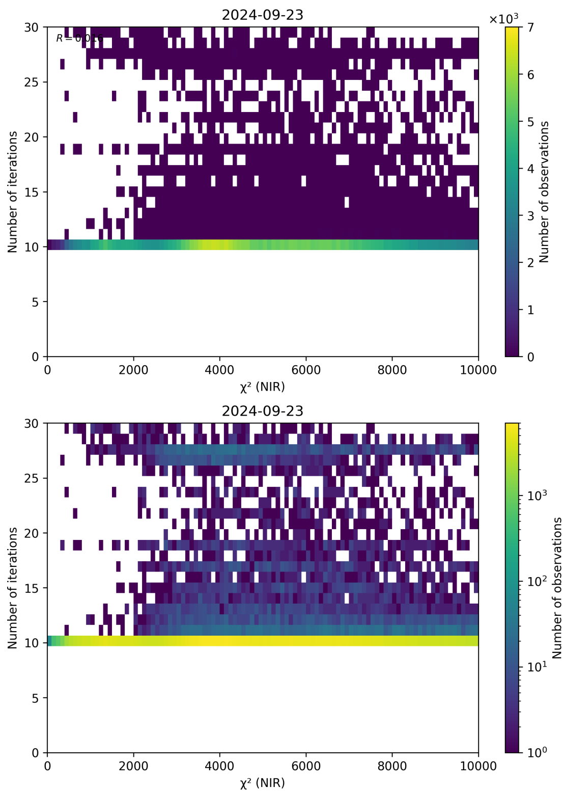
Figure 46: Scatter density plot of “ \chi^2 (NIR)” against “Number of iterations” for 2024-09-22 to 2024-09-24.
