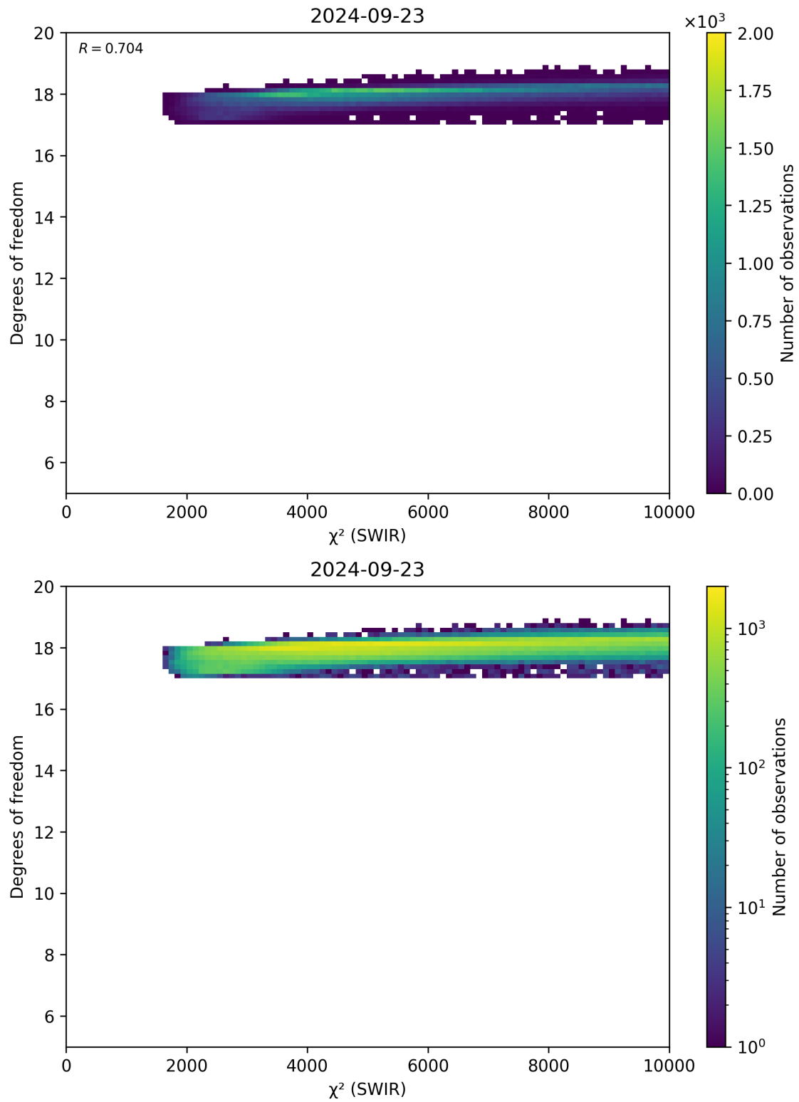
Figure 48: Scatter density plot of “ \chi^2 (SWIR)” against “Degrees of freedom” for 2024-09-22 to 2024-09-24.
