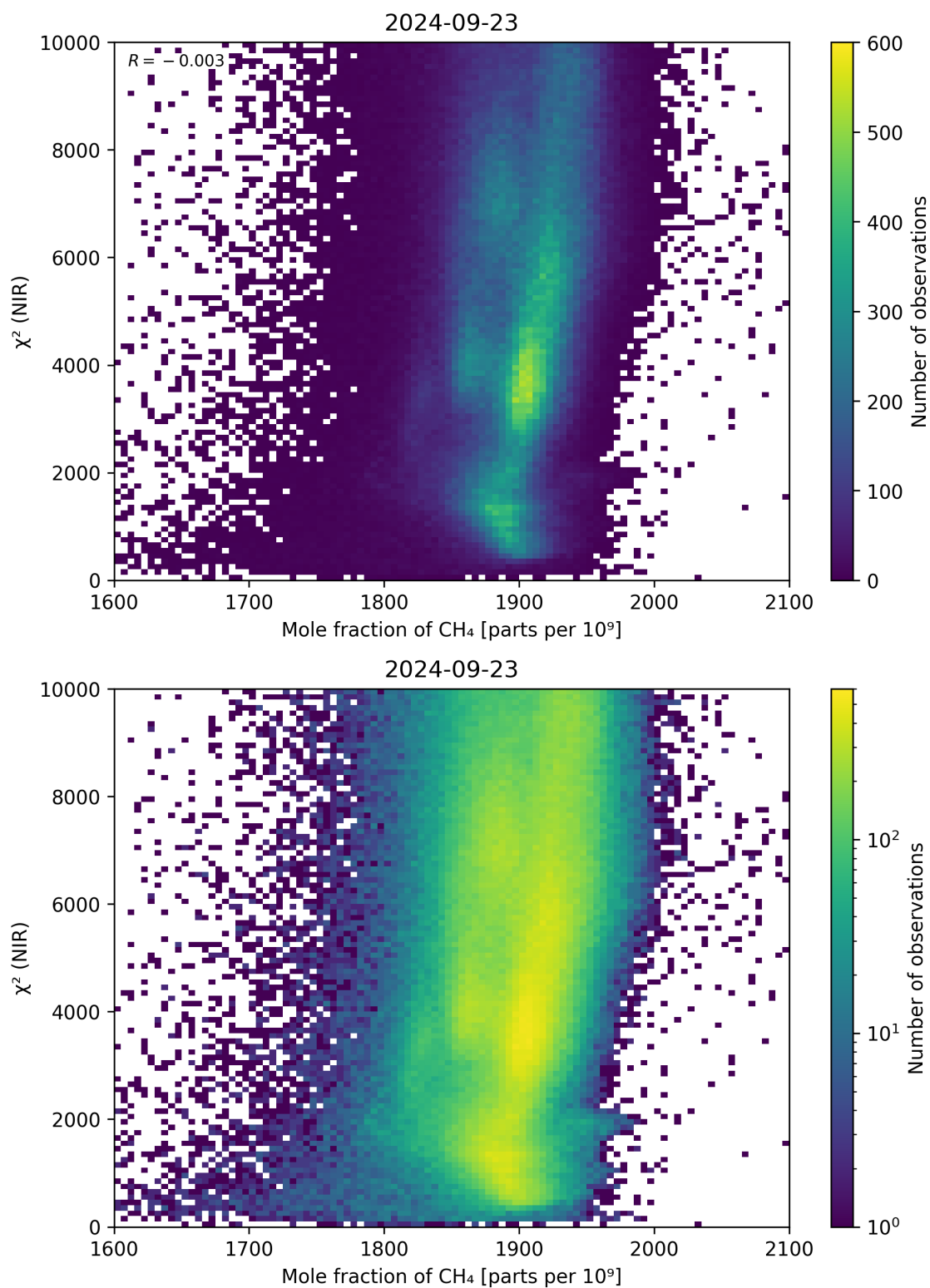
Figure 70: Scatter density plot of “Mole fraction of CH 4 ” against “ \chi^2 (NIR)” for 2024-09-22 to 2024-09-24.
