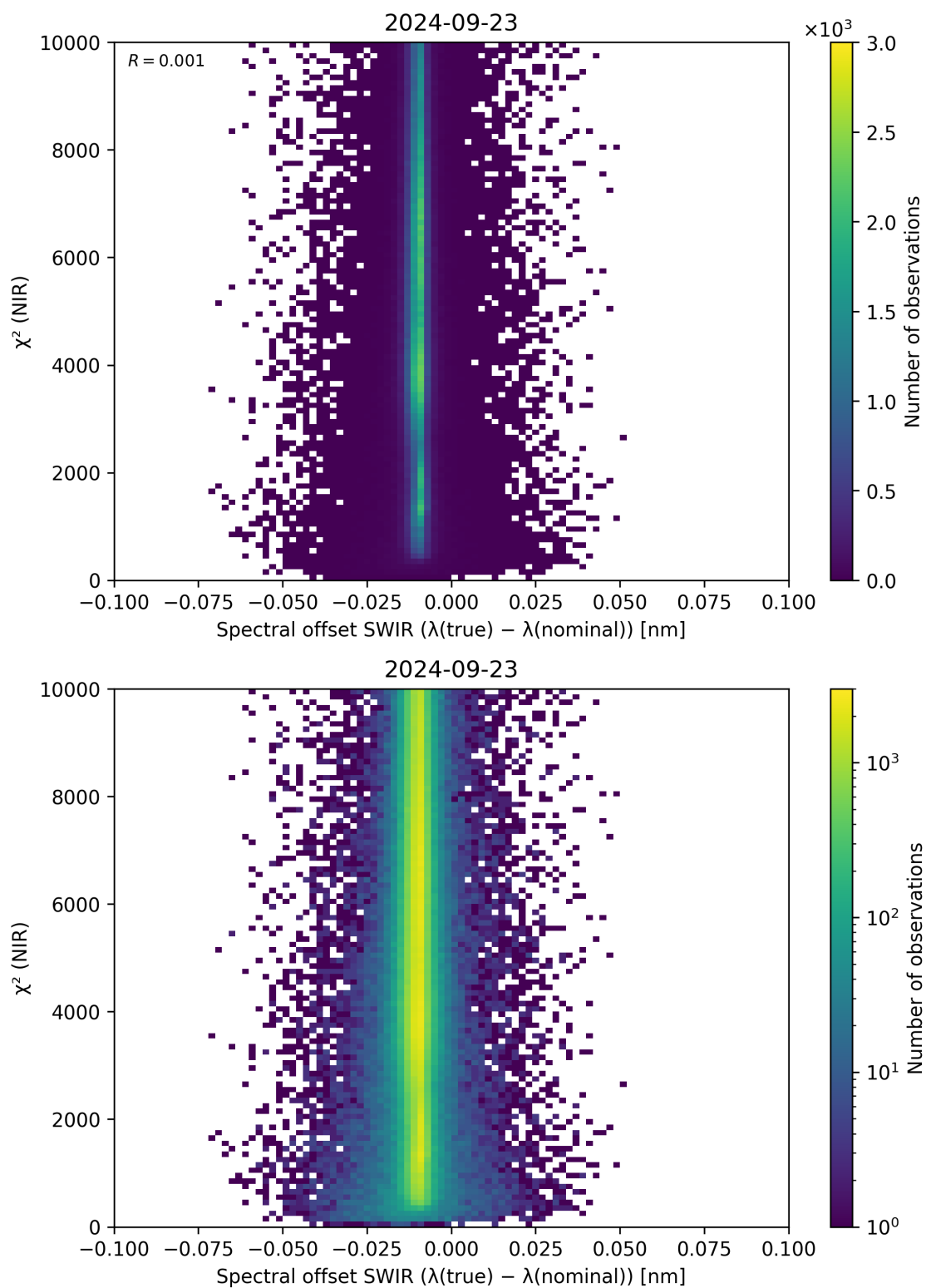
Figure 117: Scatter density plot of “Spectral offset SWIR ( \lambda_{\text{true}} - \lambda_{\text{nominal}} )” against “ \chi^2 (NIR)” for 2024-09-22 to 2024-09-24.
