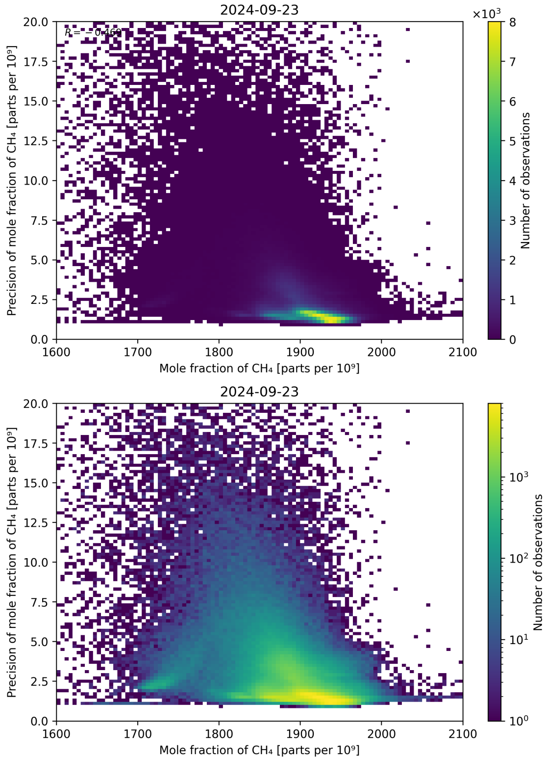
Figure 75: Scatter density plot of “Mole fraction of CH 4 ” against “Precision of mole fraction of CH 4 ” for 2024-09-22 to 2024-09-24.
