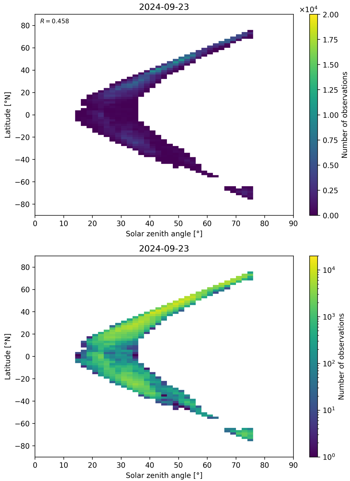
Figure 98: Scatter density plot of “Solar zenith angle” against “Latitude” for 2024-09-22 to 2024-09-24.
