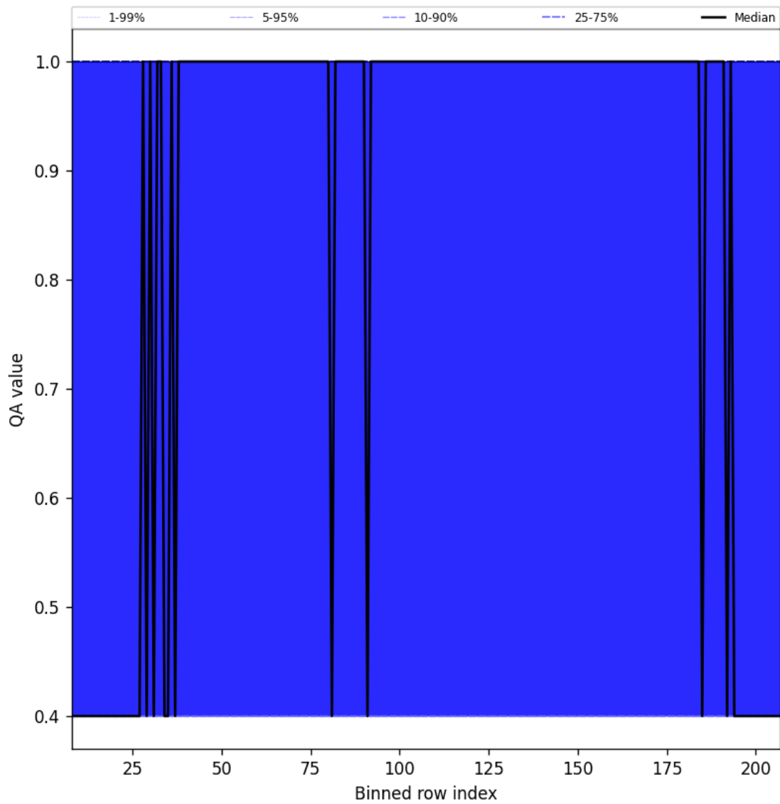
Figure 33: Along track statistics of “QA value” for 2024-09-22 to 2024-09-24
