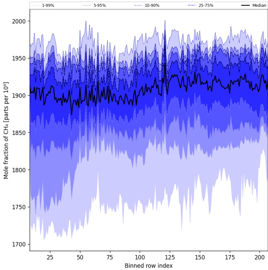
Figure 34: Along track statistics of “Mole fraction of CH 4 ” for 2024-09-22 to 2024-09-24
