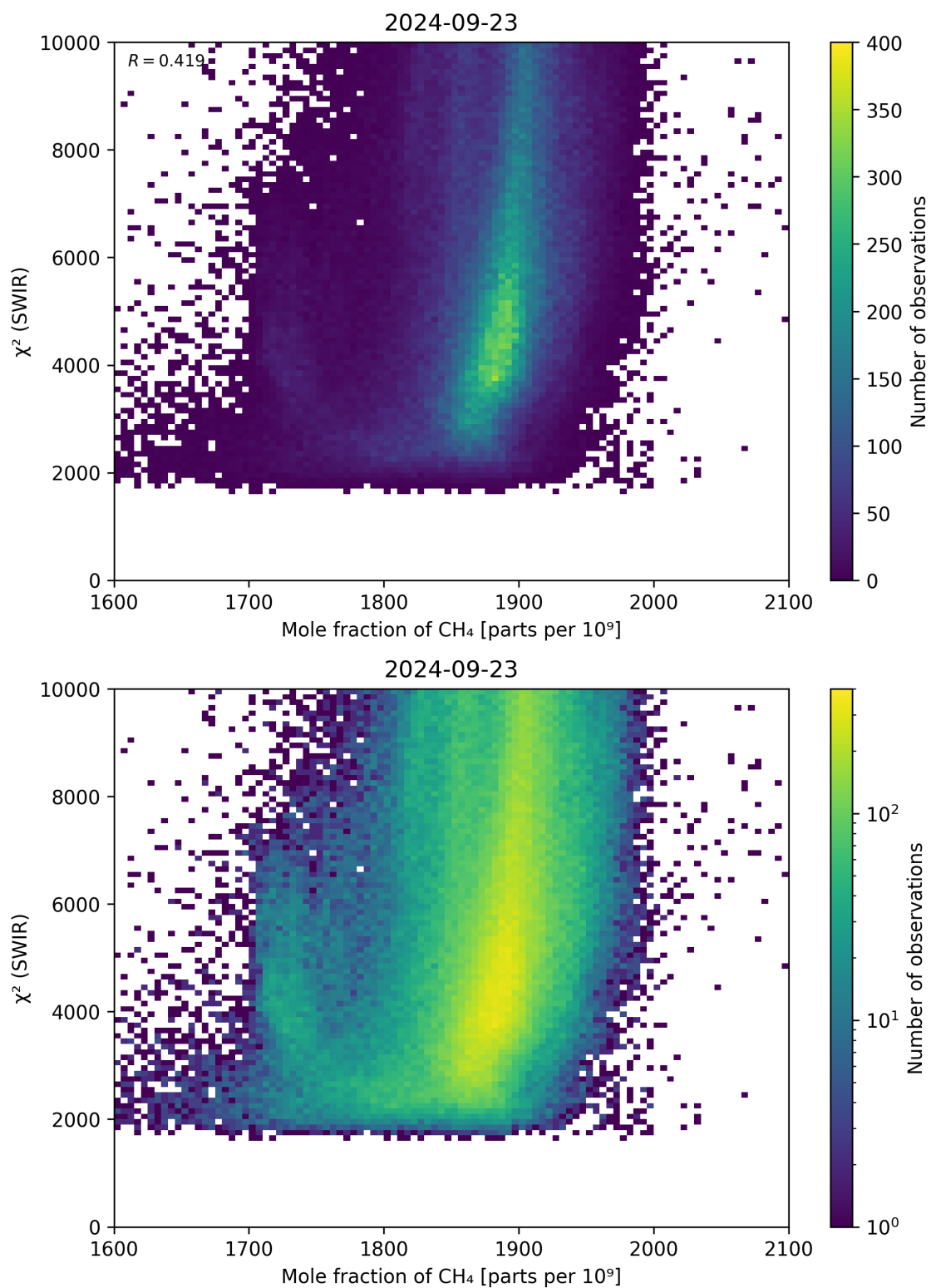
Figure 71: Scatter density plot of “Mole fraction of \text{CH}_4 ” against “ \chi^2 (SWIR)” for 2024-09-22 to 2024-09-24.
