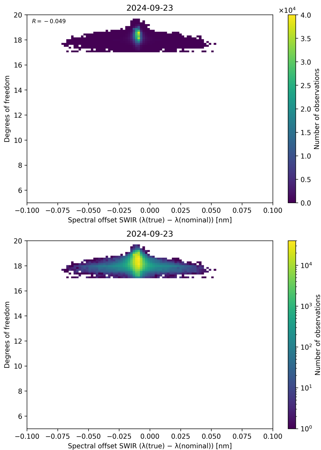
Figure 119: Scatter density plot of “Spectral offset SWIR ( \lambda_{\text{true}} - \lambda_{\text{nominal}} )” against “Degrees of freedom” for 2024-09-22 to 2024-09-24.
