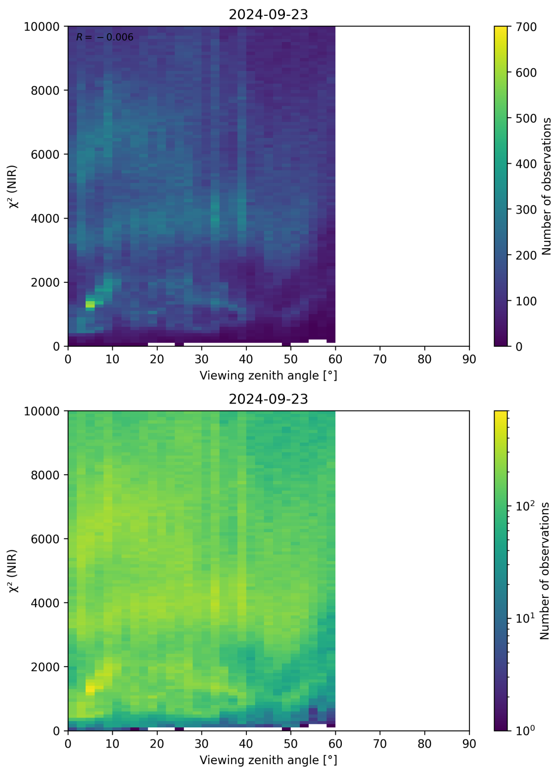
Figure 105: Scatter density plot of “Viewing zenith angle” against “ \chi^2 (NIR)” for 2024-09-22 to 2024-09-24.
