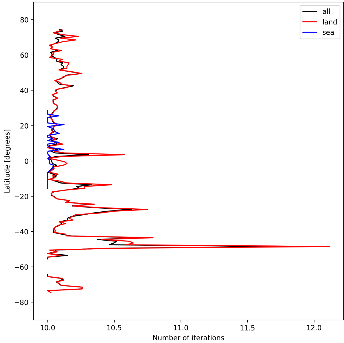
Figure 20: Zonal average of “Number of iterations” for 2024-09-22 to 2024-09-24.
