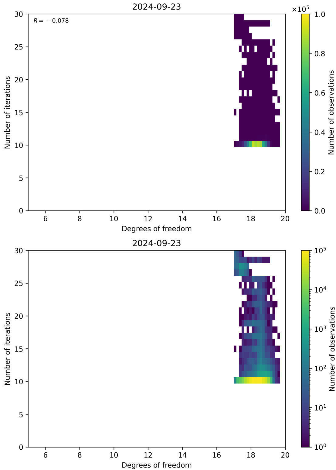
Figure 52: Scatter density plot of “Degrees of freedom” against “Number of iterations” for 2024-09-22 to 2024-09-24.
