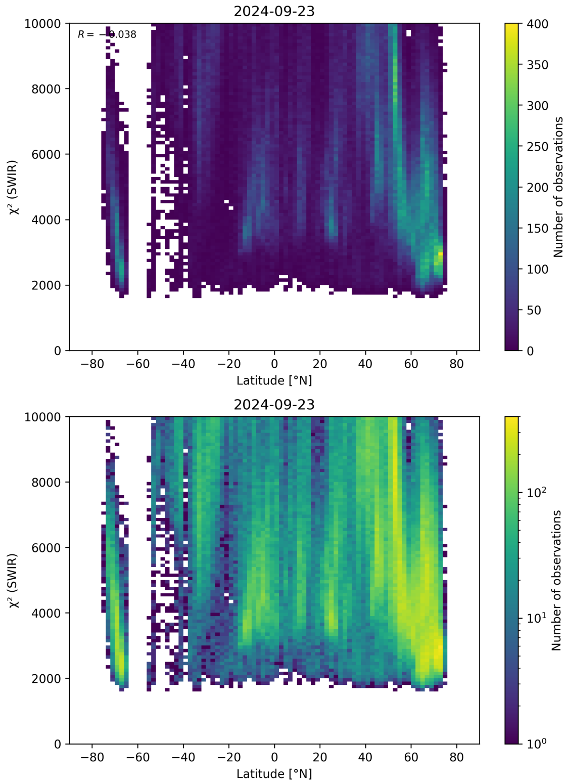
Figure 54: Scatter density plot of “Latitude” against “ \chi^2 (SWIR)” for 2024-09-22 to 2024-09-24.
