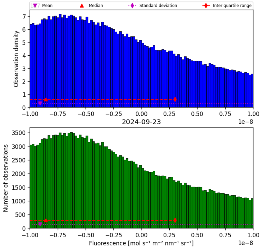
Figure 32: Histogram of “Fluorescence” for 2024-09-22 to 2024-09-24
