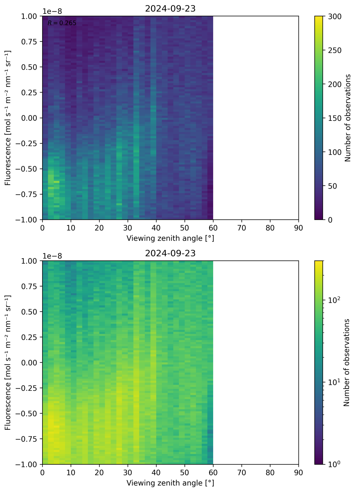
Figure 108: Scatter density plot of “Viewing zenith angle” against “Fluorescence” for 2024-09-22 to 2024-09-24.
