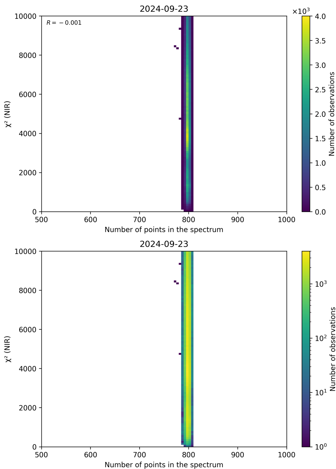
Figure 88: Scatter density plot of “Number of points in the spectrum” against “ \chi^2 (NIR)” for 2024-09-22 to 2024-09-24.
