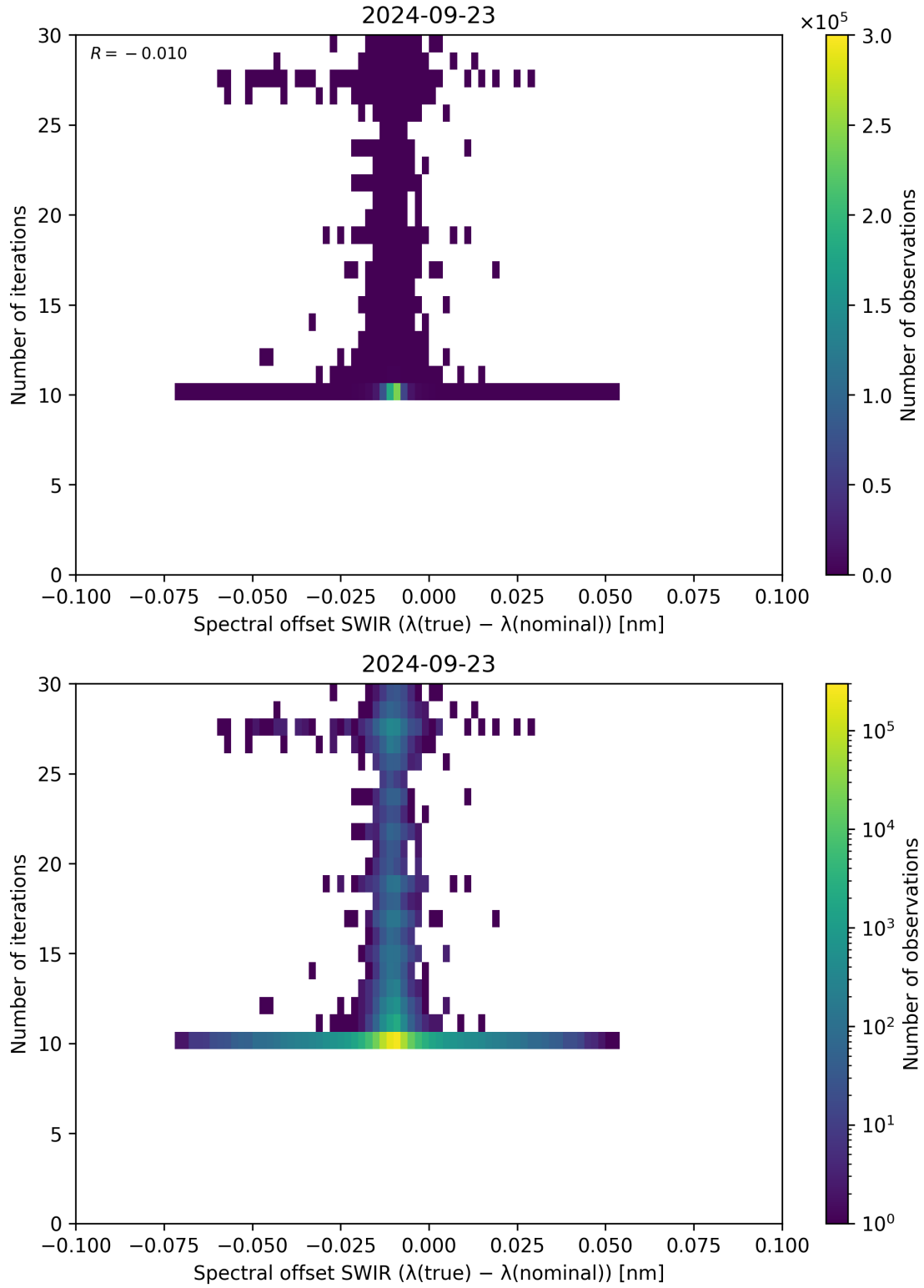
Figure 121: Scatter density plot of “Spectral offset SWIR ( \lambda_{\text{true}} - \lambda_{\text{nominal}} )” against “Number of iterations” for 2024-09-22 to 2024-09-24.
