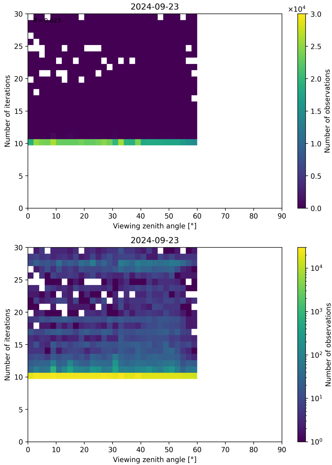
Figure 113: Scatter density plot of “Viewing zenith angle” against “Number of iterations” for 2024-09-22 to 2024-09-24.
