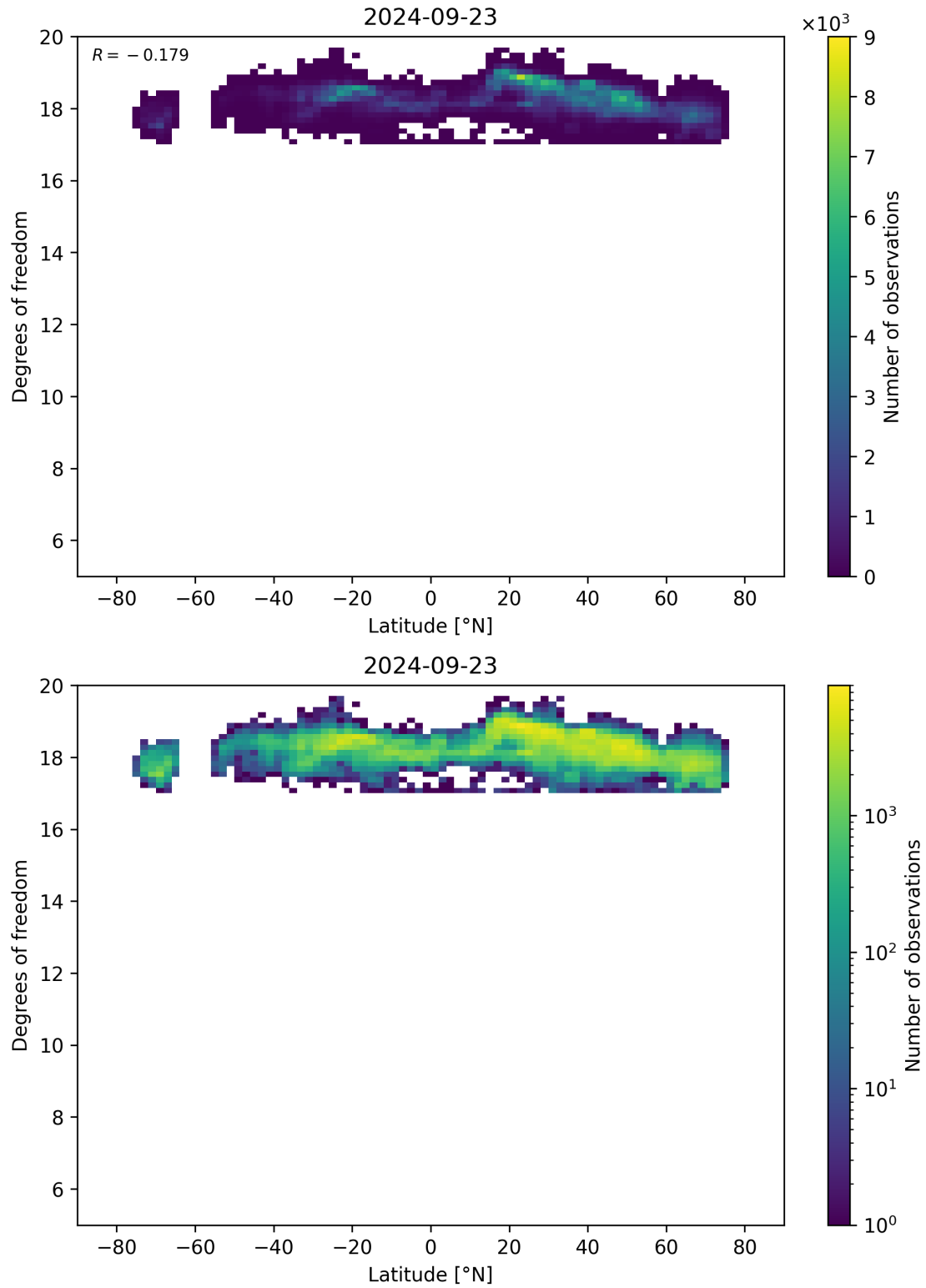
Figure 55: Scatter density plot of “Latitude” against “Degrees of freedom” for 2024-09-22 to 2024-09-24.
