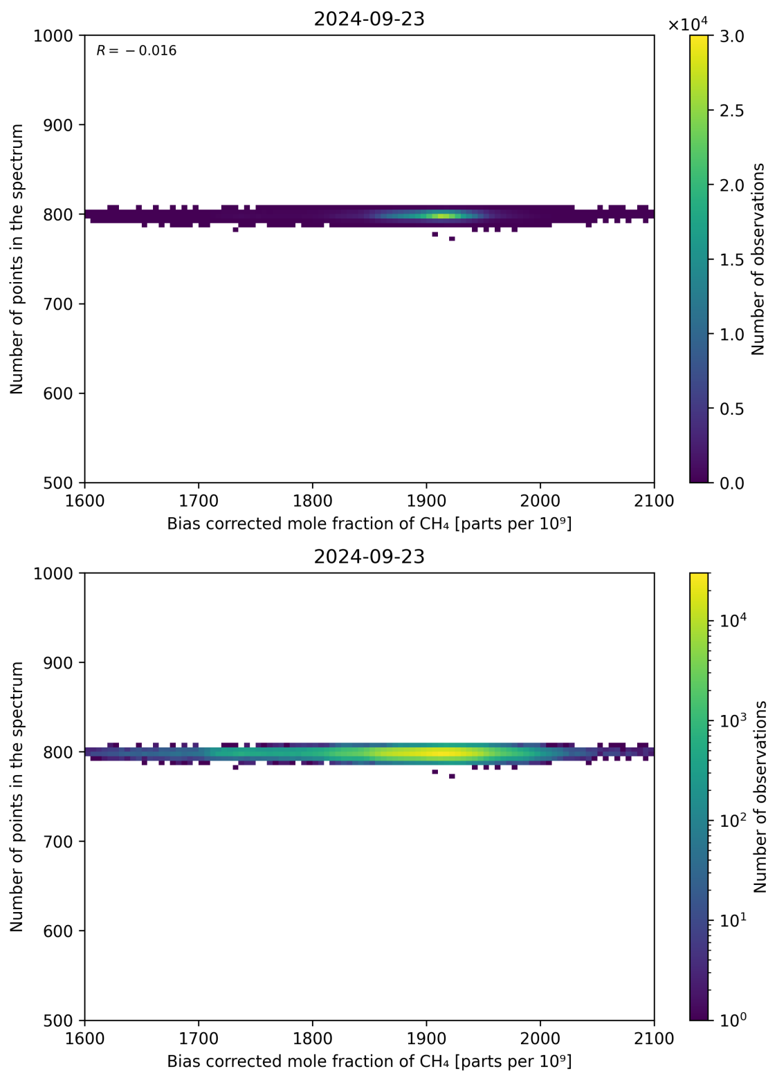
Figure 68: Scatter density plot of “Bias corrected mole fraction of CH 4 ” against “Number of points in the spectrum” for 2024-09-22 to 2024-09-24.
