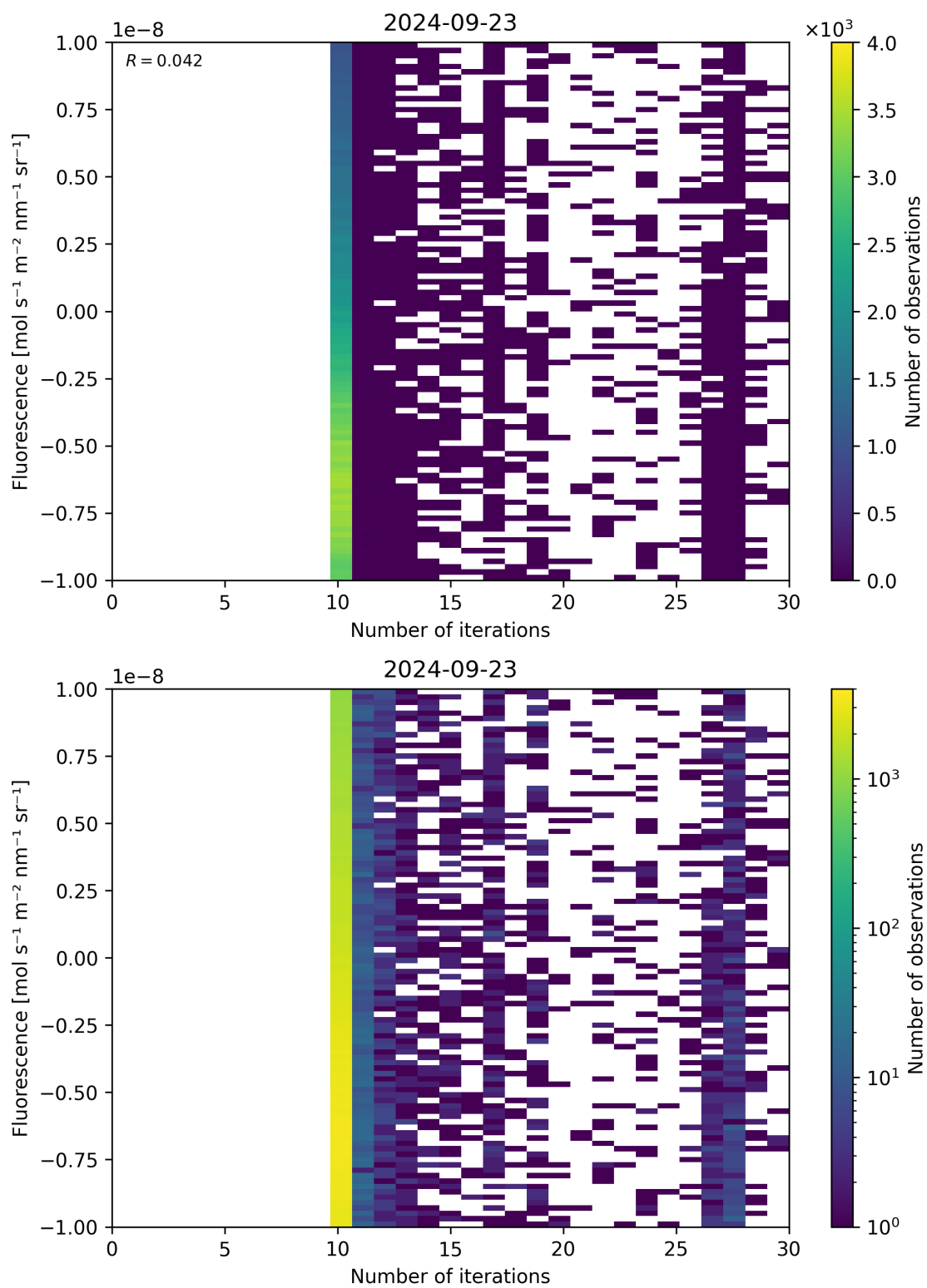
Figure 87: Scatter density plot of “Number of iterations” against “Fluorescence” for 2024-09-22 to 2024-09-24.
