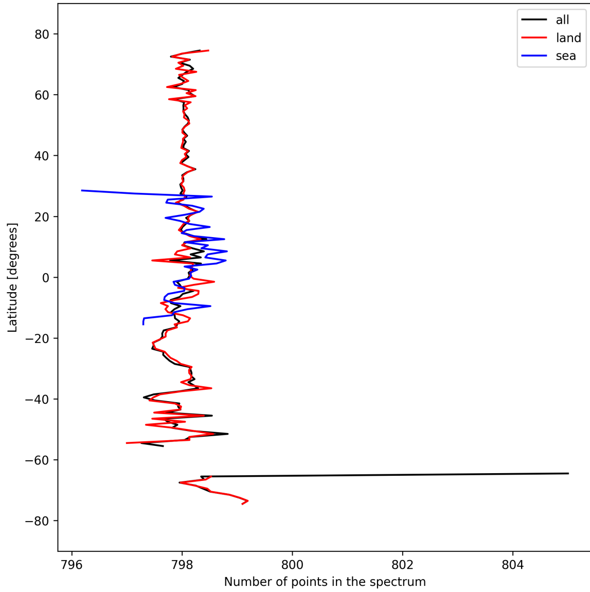
Figure 15: Zonal average of “Number of points in the spectrum” for 2024-09-22 to 2024-09-24.
