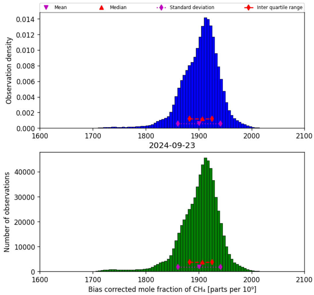
Figure 25: Histogram of “Bias corrected mole fraction of CH 4 ” for 2024-09-22 to 2024-09-24
