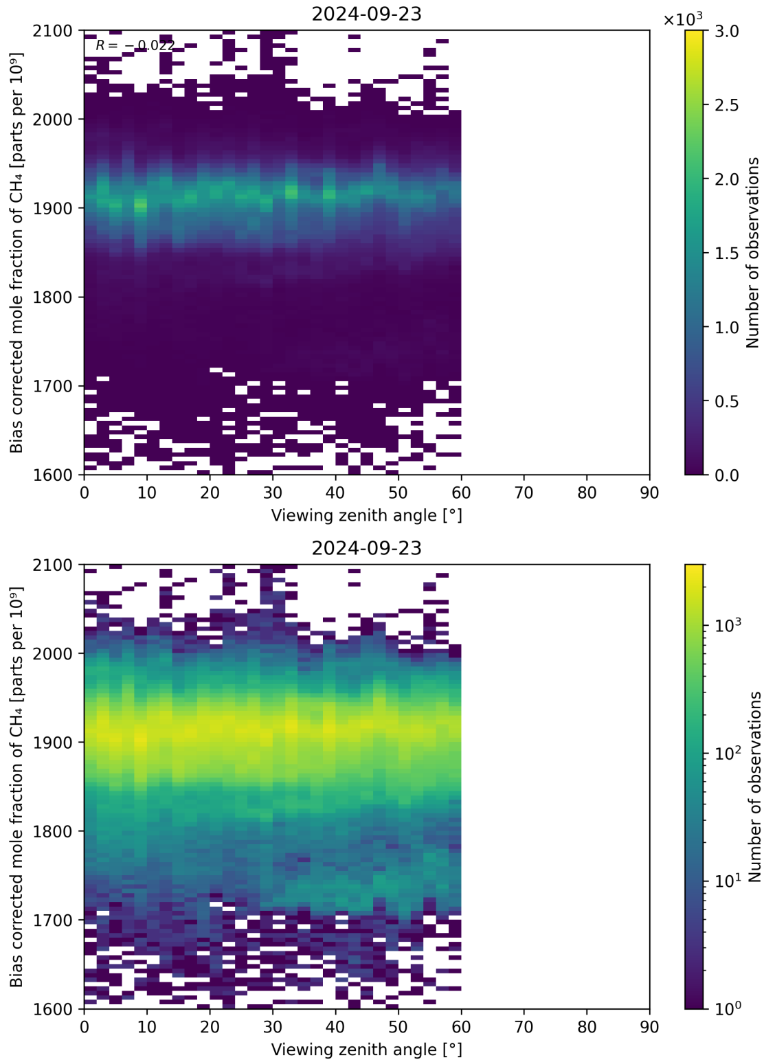
Figure 111: Scatter density plot of “Viewing zenith angle” against “Bias corrected mole fraction of CH 4 ” for 2024-09-22 to 2024-09-24.
