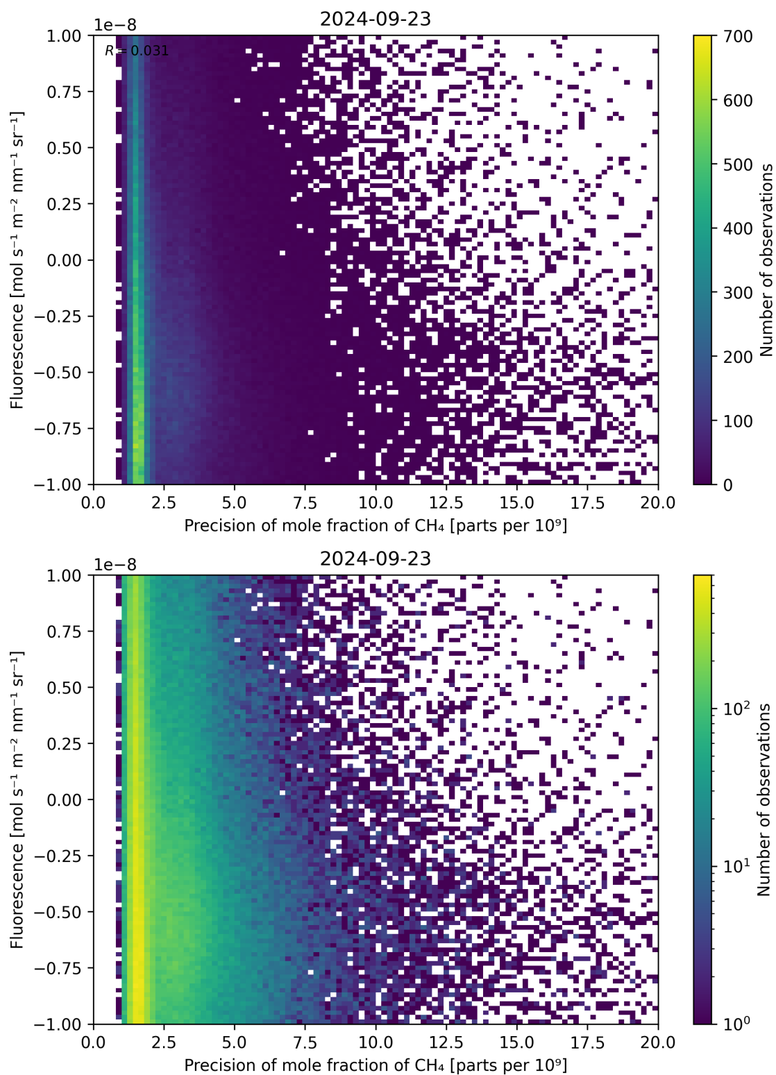
Figure 81: Scatter density plot of “Precision of mole fraction of \text{CH}_4 ” against “Fluorescence” for 2024-09-22 to 2024-09-24.
