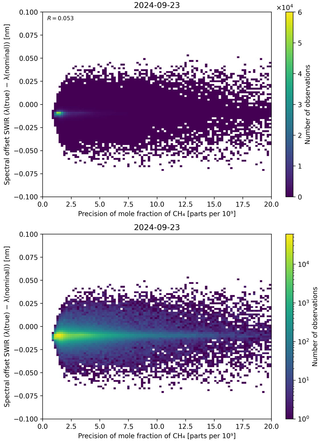
Figure 85: Scatter density plot of “Precision of mole fraction of \text{CH}_4 ” against “Spectral offset SWIR ( \lambda_{\text{true}} - \lambda_{\text{nominal}} )” for 2024-09-22 to 2024-09-24.
