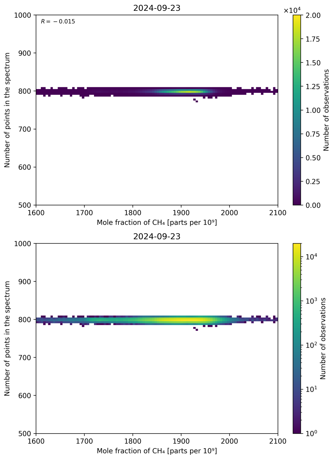
Figure 77: Scatter density plot of “Mole fraction of CH 4 ” against “Number of points in the spectrum” for 2024-09-22 to 2024-09-24.
