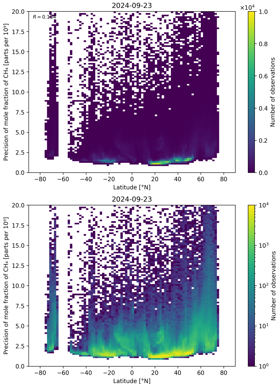
Figure 59: Scatter density plot of “Latitude” against “Precision of mole fraction of \text{CH}_4 ” for 2024-09-22 to 2024-09-24.
