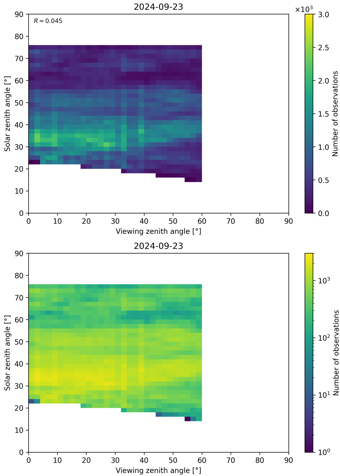
Figure 115: Scatter density plot of “Viewing zenith angle” against “Solar zenith angle” for 2024-09-22 to 2024-09-24.
