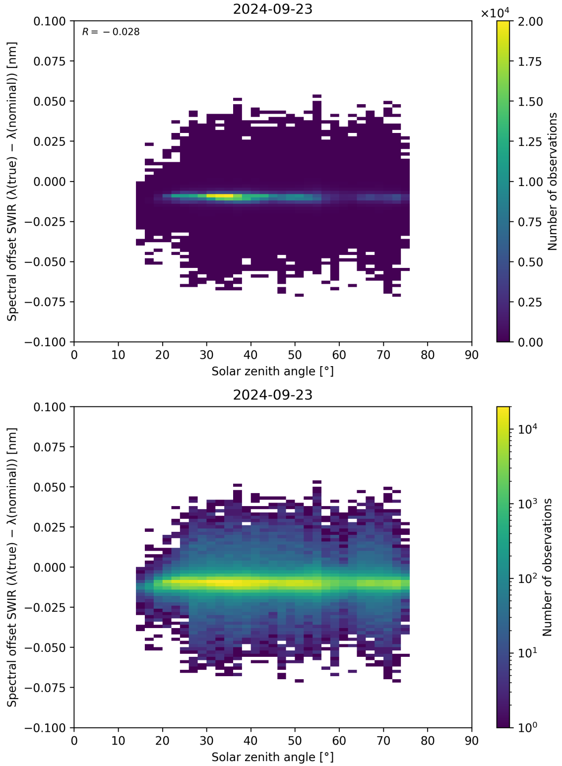
Figure 104: Scatter density plot of “Solar zenith angle” against “Spectral offset SWIR ( \lambda_{\text{true}} - \lambda_{\text{nominal}} )” for 2024-09-22 to 2024-09-24.
