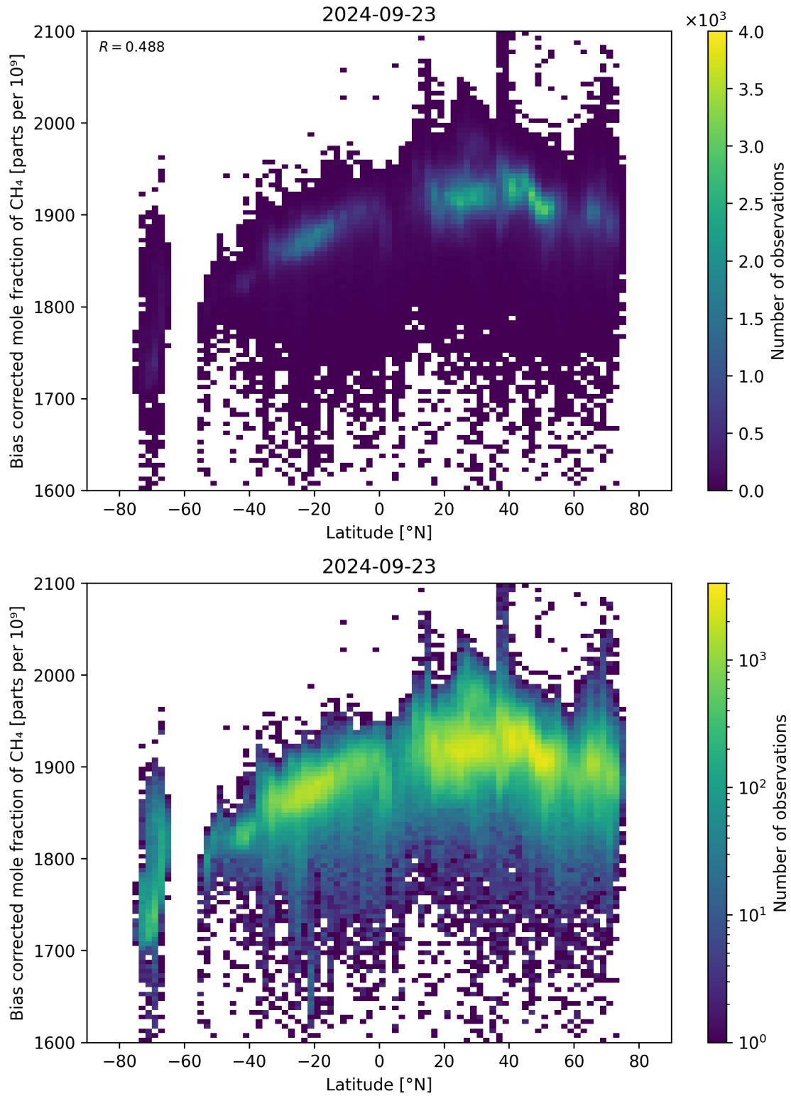
Figure 58: Scatter density plot of “Latitude” against “Bias corrected mole fraction of CH 4 ” for 2024-09-22 to 2024-09-24.
