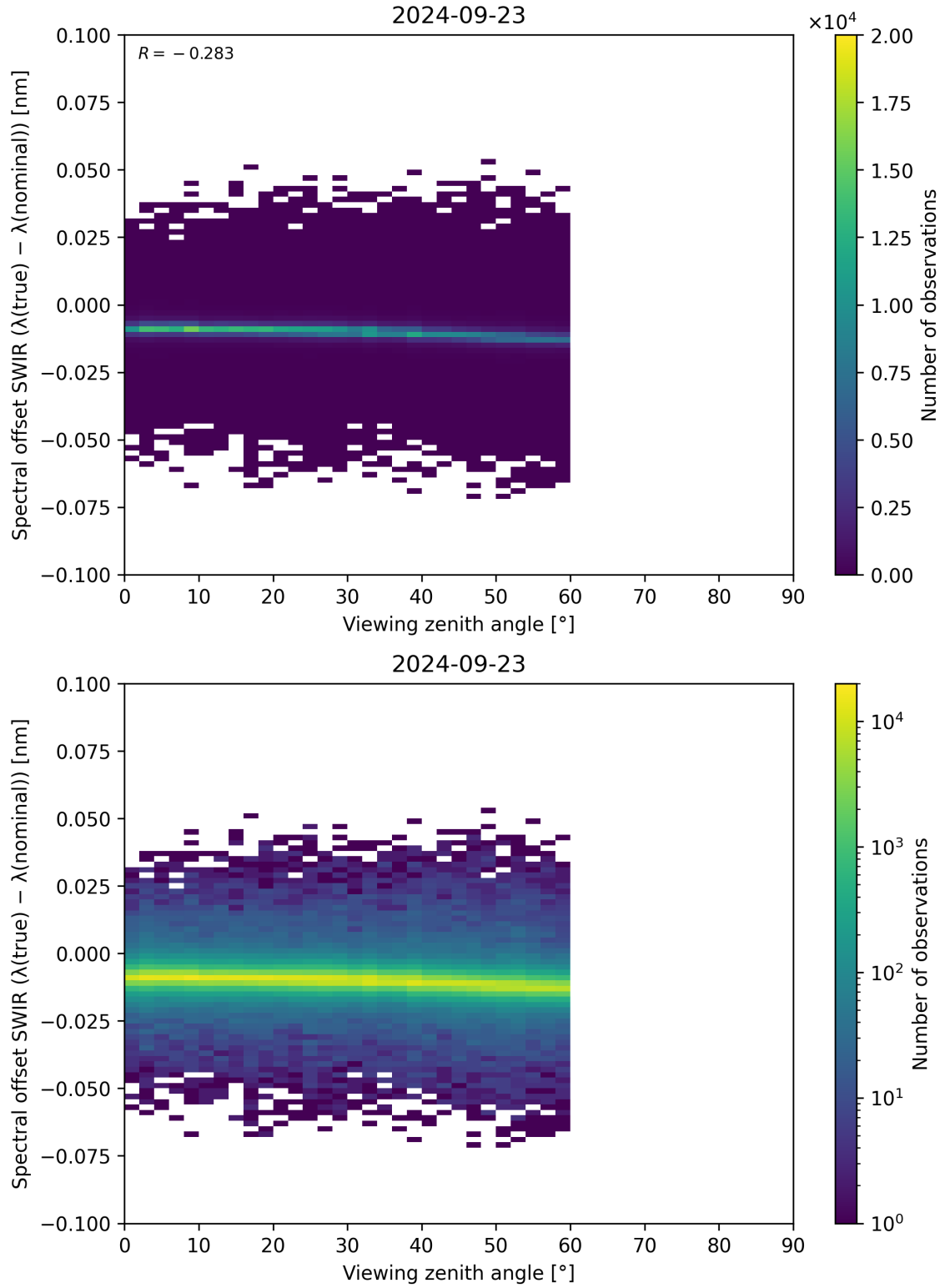
Figure 116: Scatter density plot of “Viewing zenith angle” against “Spectral offset SWIR ( \lambda_{\text{true}} - \lambda_{\text{nominal}} )” for 2024-09-22 to 2024-09-24.
