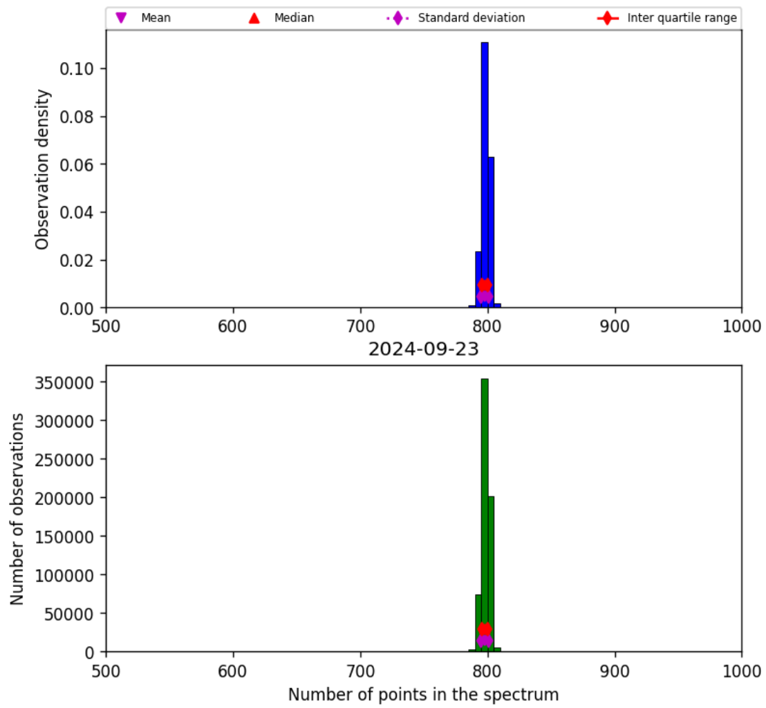
Figure 26: Histogram of “Number of points in the spectrum” for 2024-09-22 to 2024-09-24
