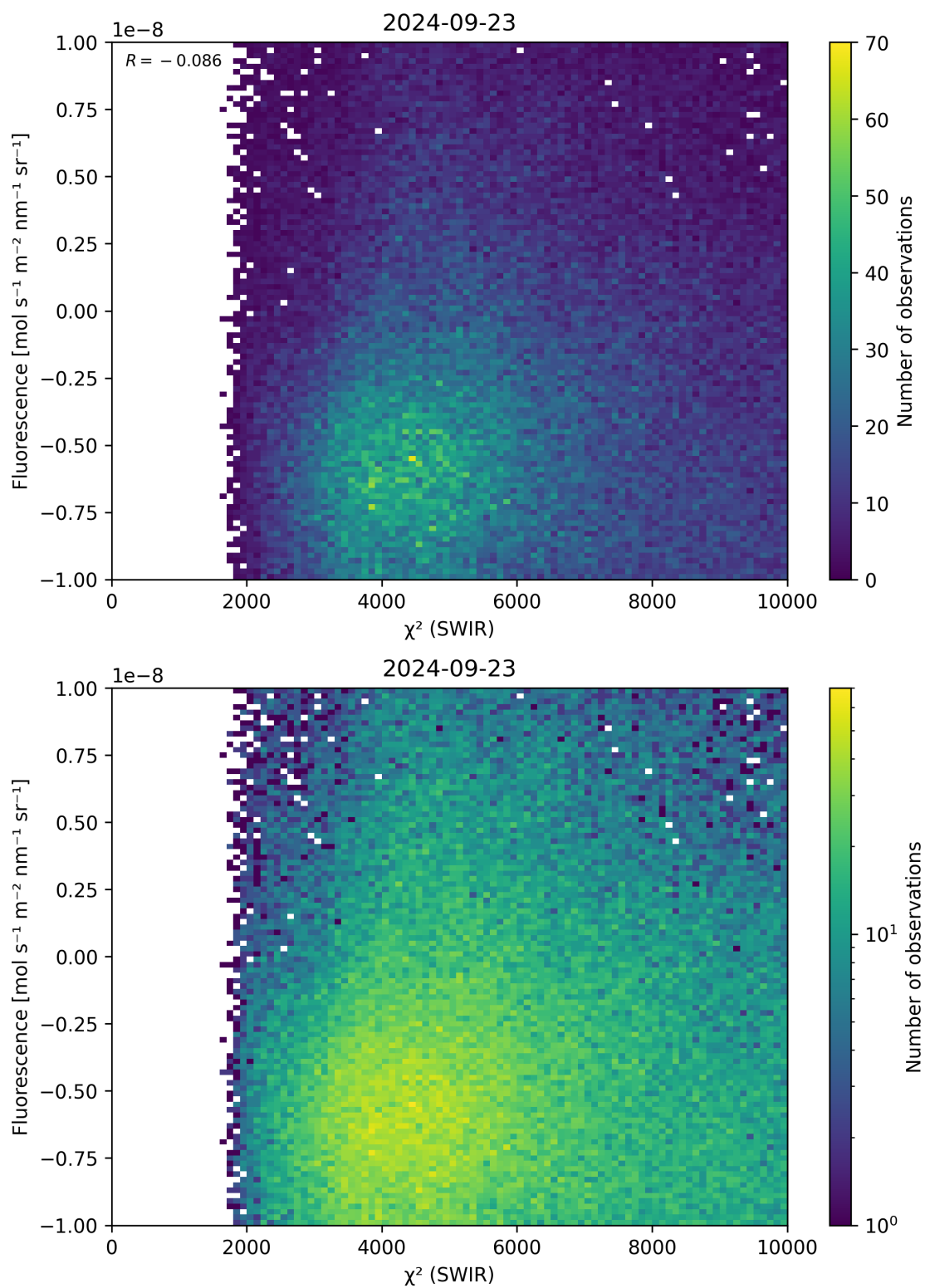
Figure 49: Scatter density plot of “ \chi^2 (SWIR)” against “Fluorescence” for 2024-09-22 to 2024-09-24.
