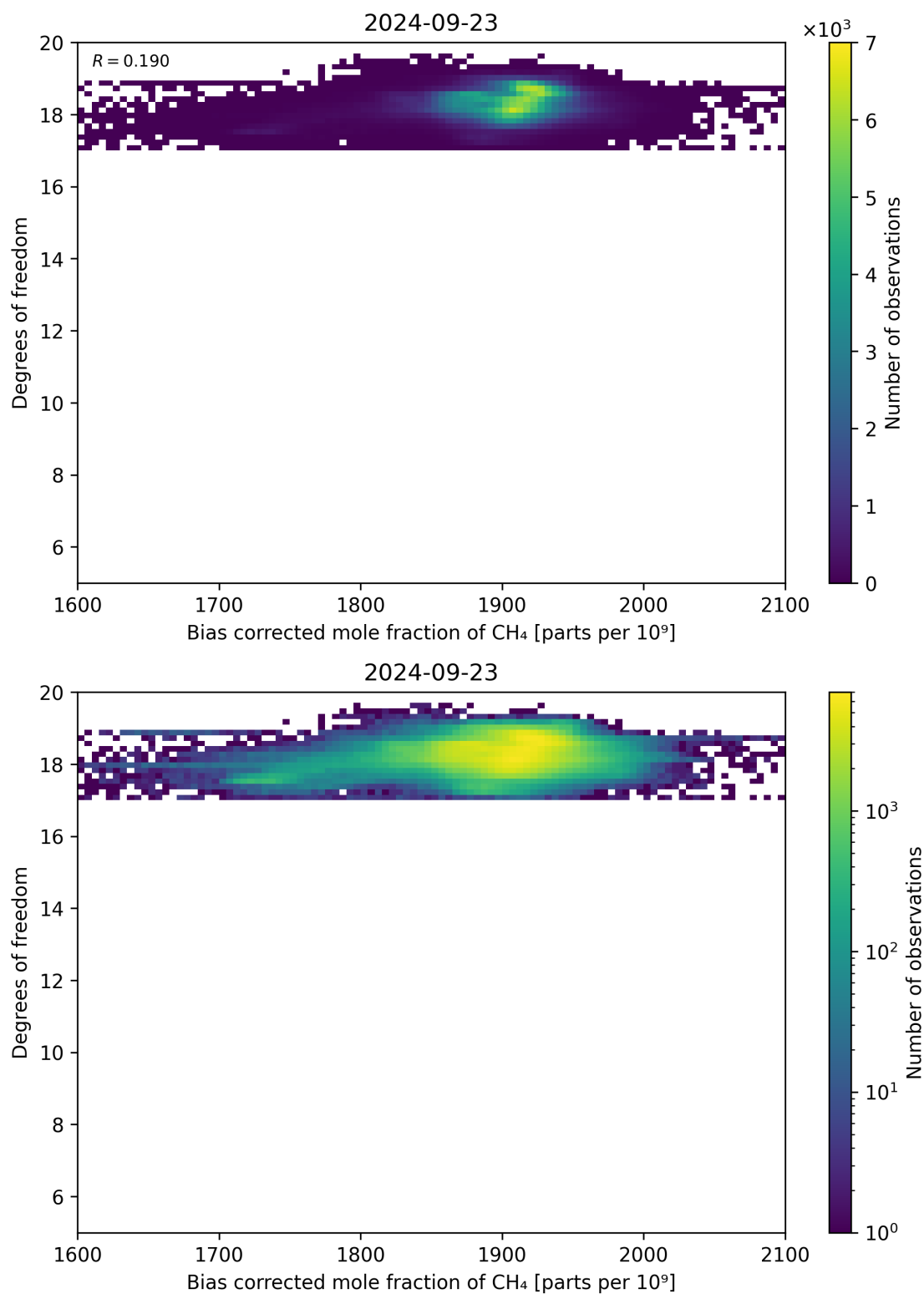
Figure 65: Scatter density plot of “Bias corrected mole fraction of CH 4 ” against “Degrees of freedom” for 2024-09-22 to 2024-09-24.
