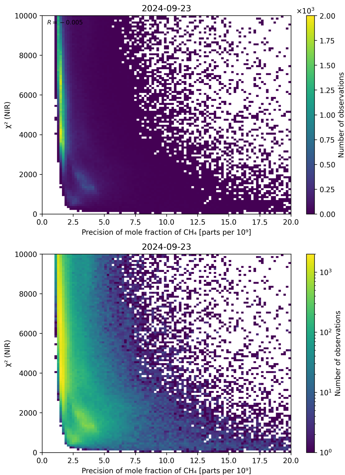
Figure 78: Scatter density plot of “Precision of mole fraction of CH 4 ” against “ \chi^2 (NIR)” for 2024-09-22 to 2024-09-24.
