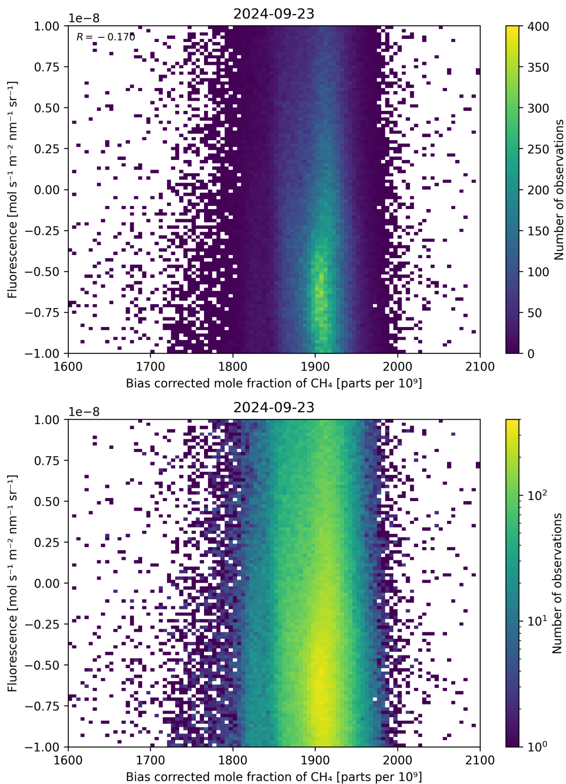
Figure 66: Scatter density plot of “Bias corrected mole fraction of \text{CH}_4 ” against “Fluorescence” for 2024-09-22 to 2024-09-24.
