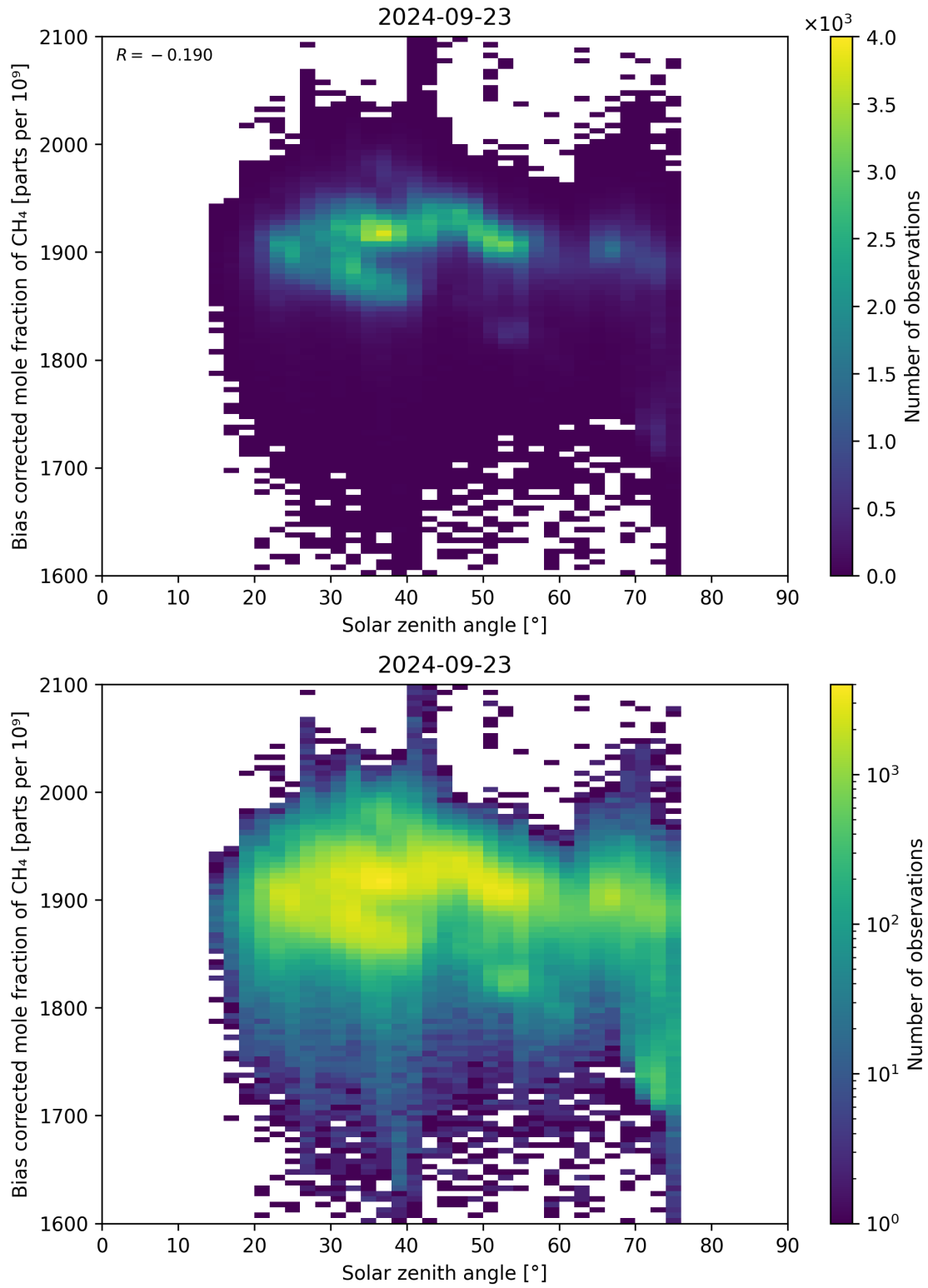
Figure 100: Scatter density plot of “Solar zenith angle” against “Bias corrected mole fraction of \text{CH}_4 ” for 2024-09-22 to 2024-09-24.
