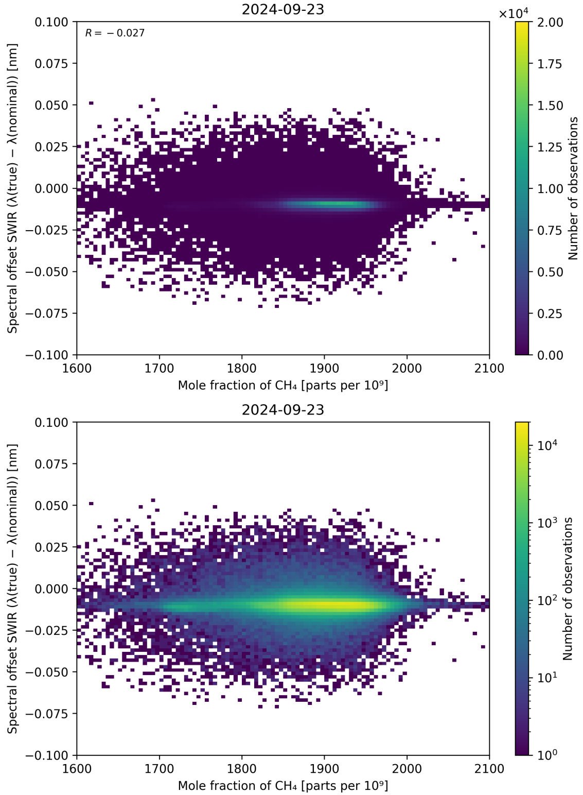
Figure 86: Scatter density plot of “Mole fraction of CH 4 ” against “Spectral offset SWIR ( \lambda_{\text{true}} - \lambda_{\text{nominal}} )” for 2024-09-22 to 2024-09-24.
