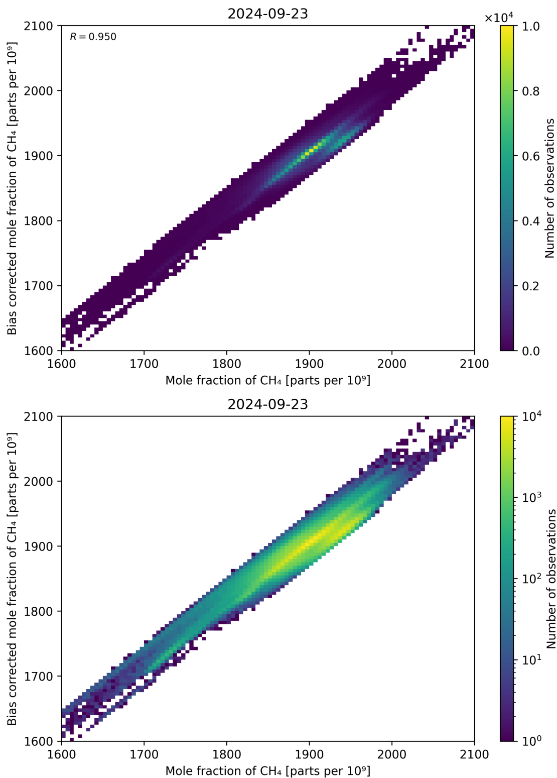
Figure 74: Scatter density plot of “Mole fraction of CH 4 ” against “Bias corrected mole fraction of CH 4 ” for 2024-09-22 to 2024-09-24.
