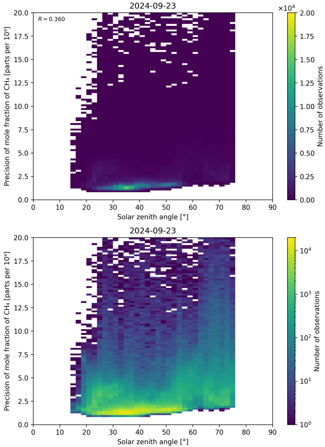
Figure 101: Scatter density plot of “Solar zenith angle” against “Precision of mole fraction of CH 4 ” for 2024-09-22 to 2024-09-24.
