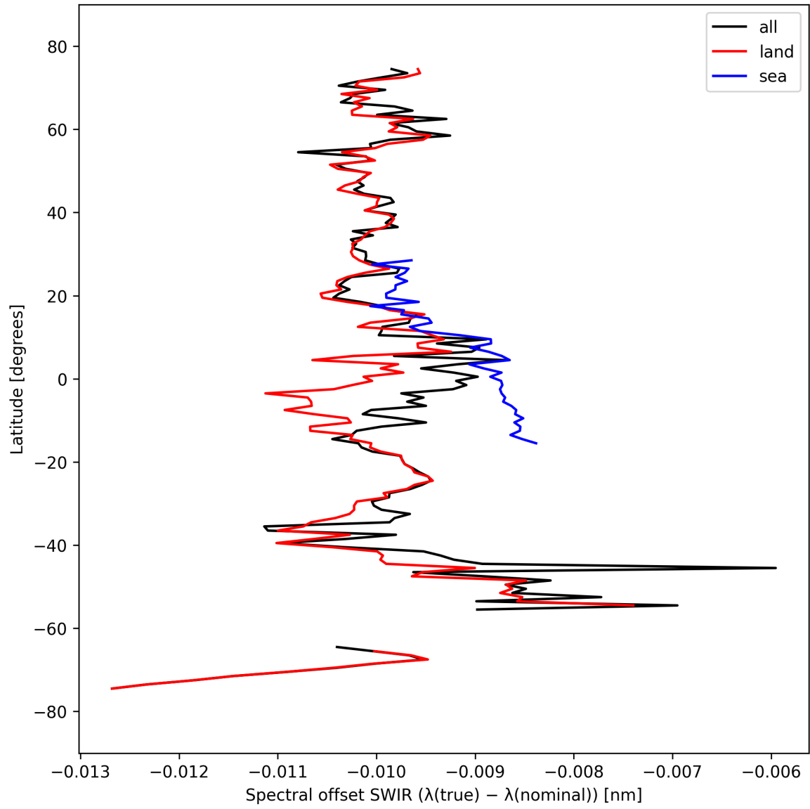
Figure 16: Zonal average of “Spectral offset SWIR ( \lambda_{\text{true}} - \lambda_{\text{nominal}} )” for 2024-09-22 to 2024-09-24.
