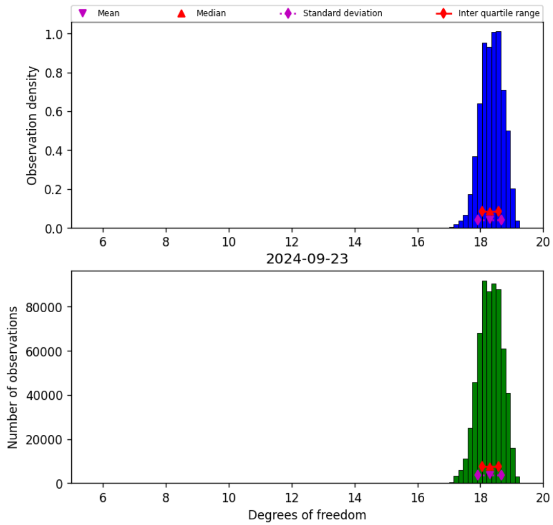
Figure 30: Histogram of “Degrees of freedom” for 2024-09-22 to 2024-09-24
