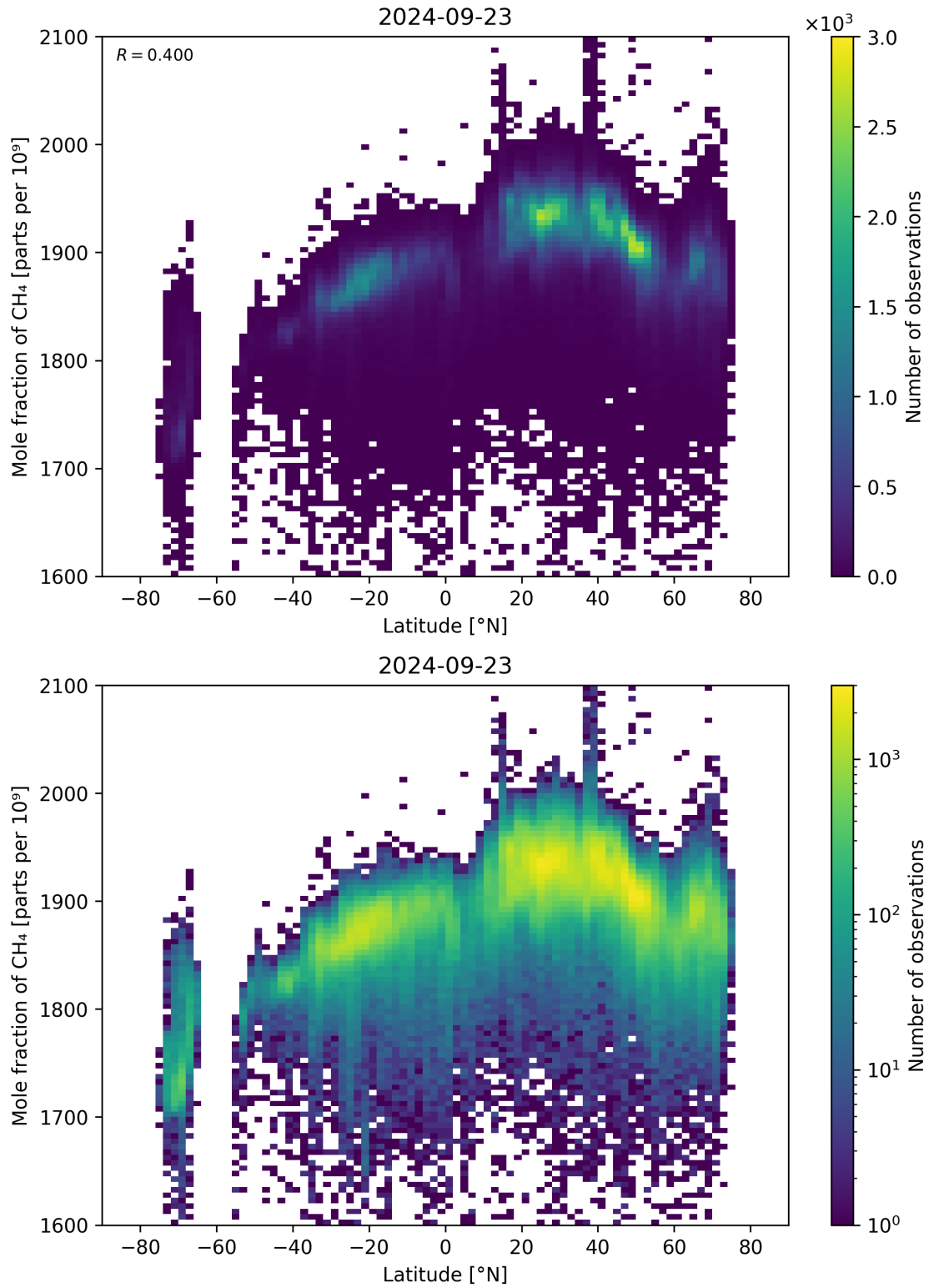
Figure 57: Scatter density plot of “Latitude” against “Mole fraction of \text{CH}_4 ” for 2024-09-22 to 2024-09-24.
