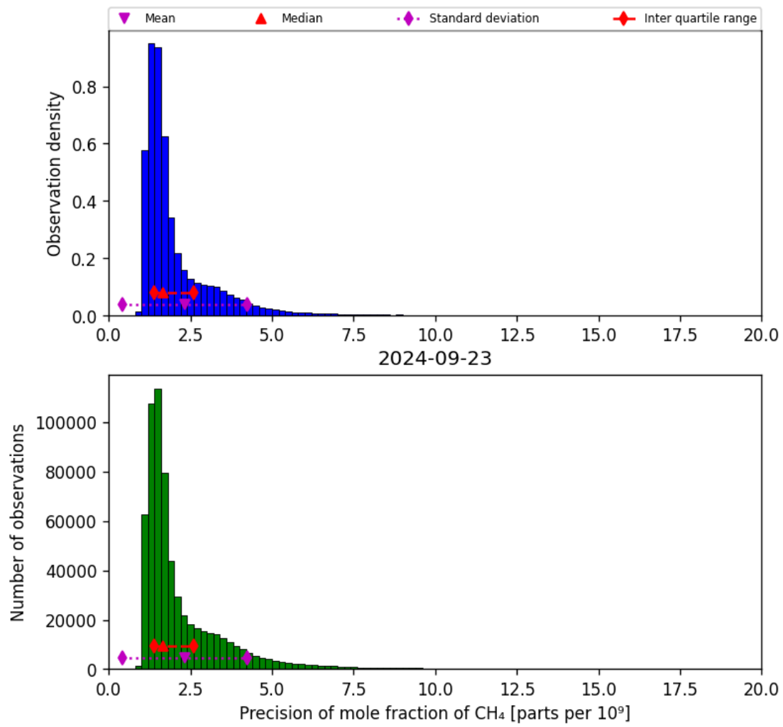
Figure 24: Histogram of “Precision of mole fraction of CH 4 ” for 2024-09-22 to 2024-09-24
