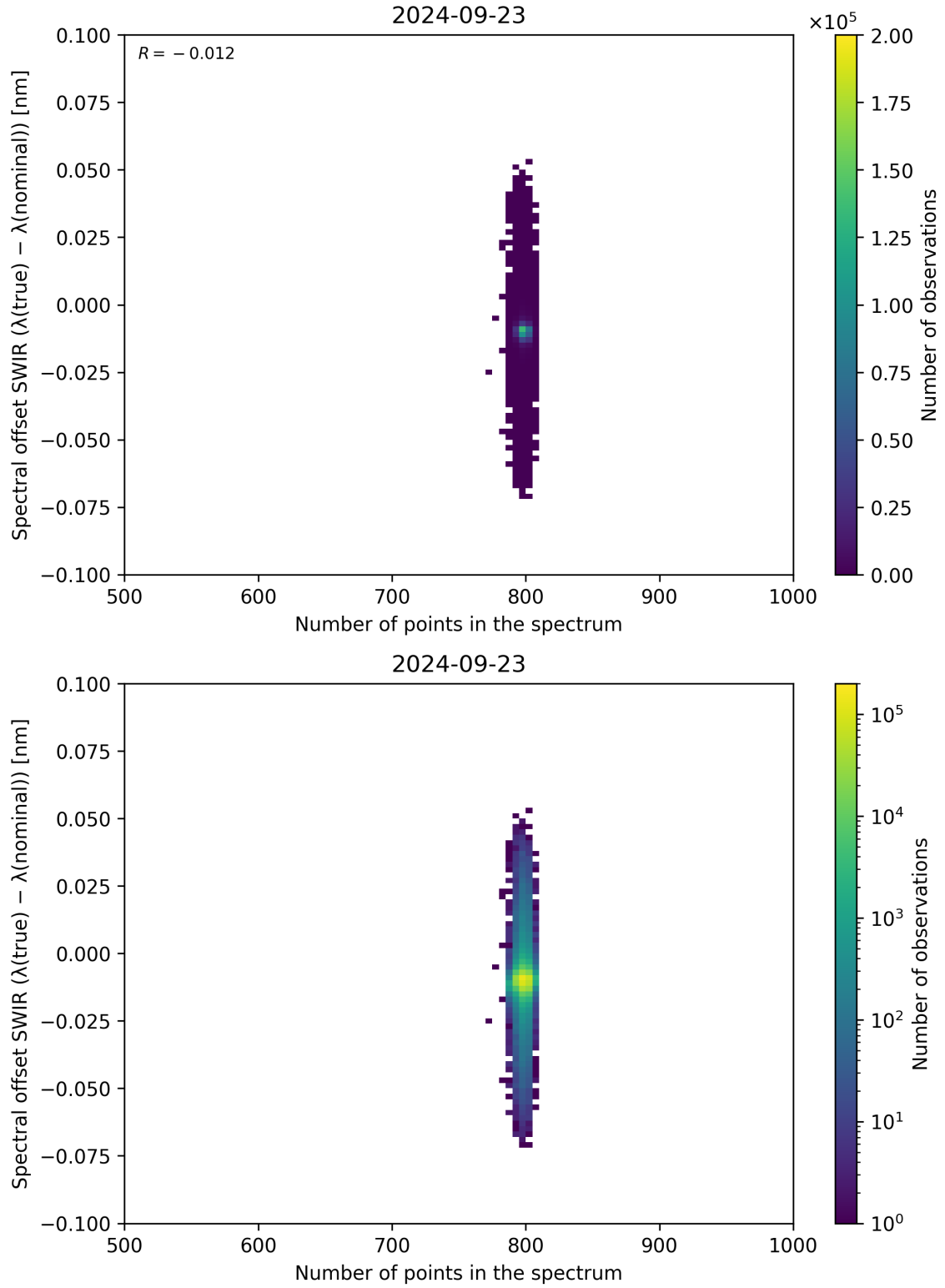
Figure 93: Scatter density plot of “Number of points in the spectrum” against “Spectral offset SWIR ( \lambda_{\text{true}} - \lambda_{\text{nominal}} )” for 2024-09-22 to 2024-09-24.
