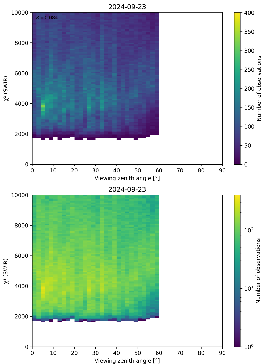
Figure 106: Scatter density plot of “Viewing zenith angle” against “ \chi^2 (SWIR)” for 2024-09-22 to 2024-09-24.
