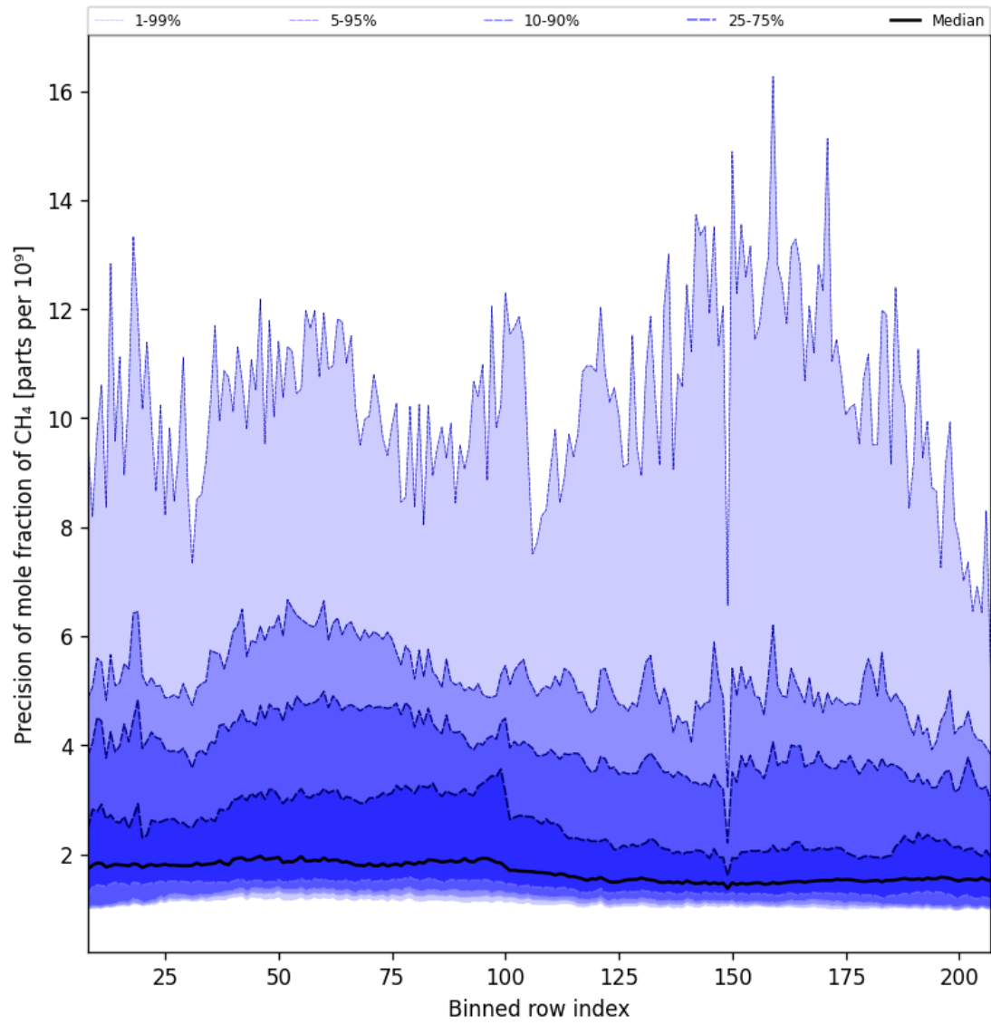
Figure 35: Along track statistics of “Precision of mole fraction of CH 4 ” for 2024-09-22 to 2024-09-24
