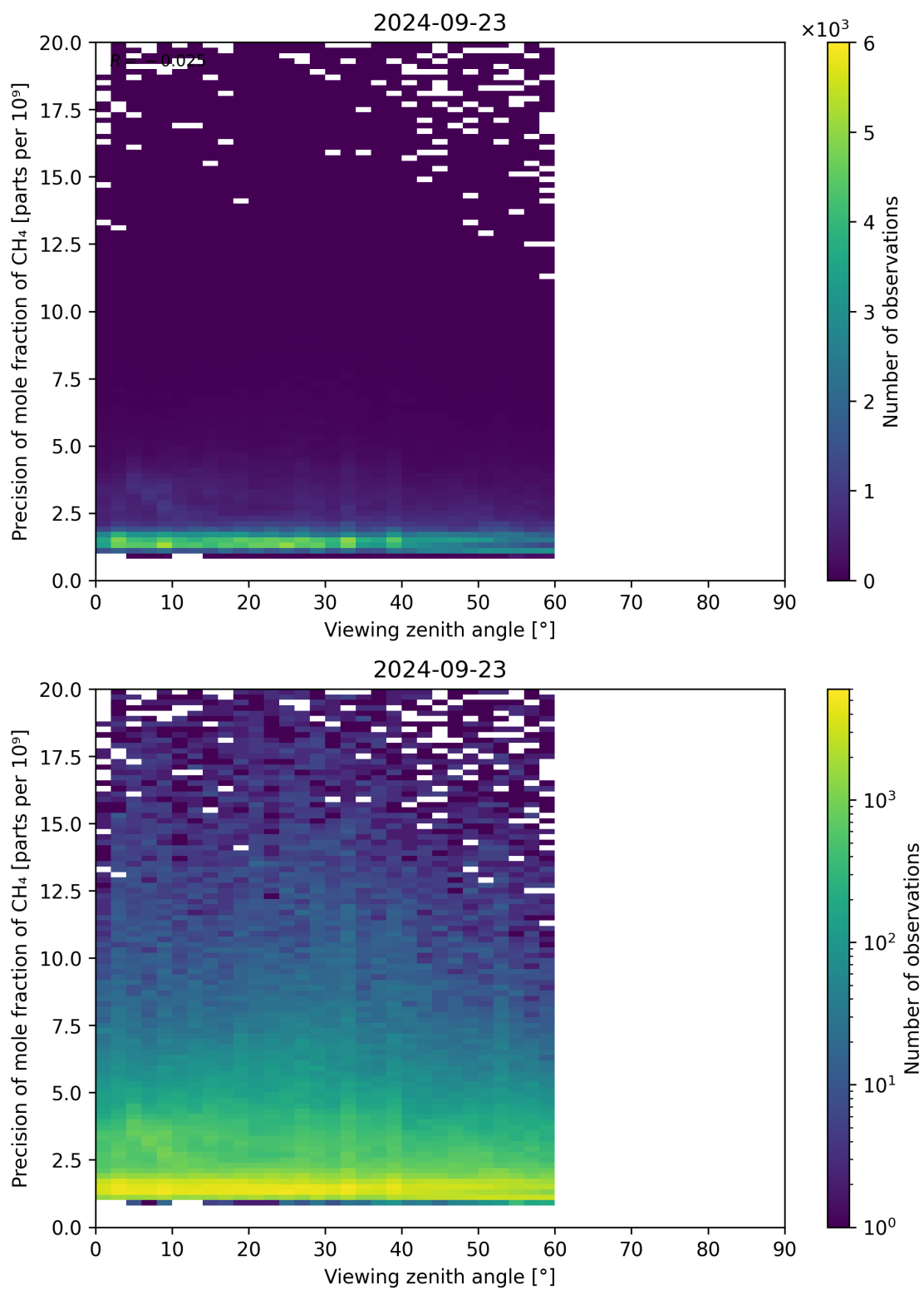
Figure 112: Scatter density plot of “Viewing zenith angle” against “Precision of mole fraction of CH 4 ” for 2024-09-22 to 2024-09-24.
