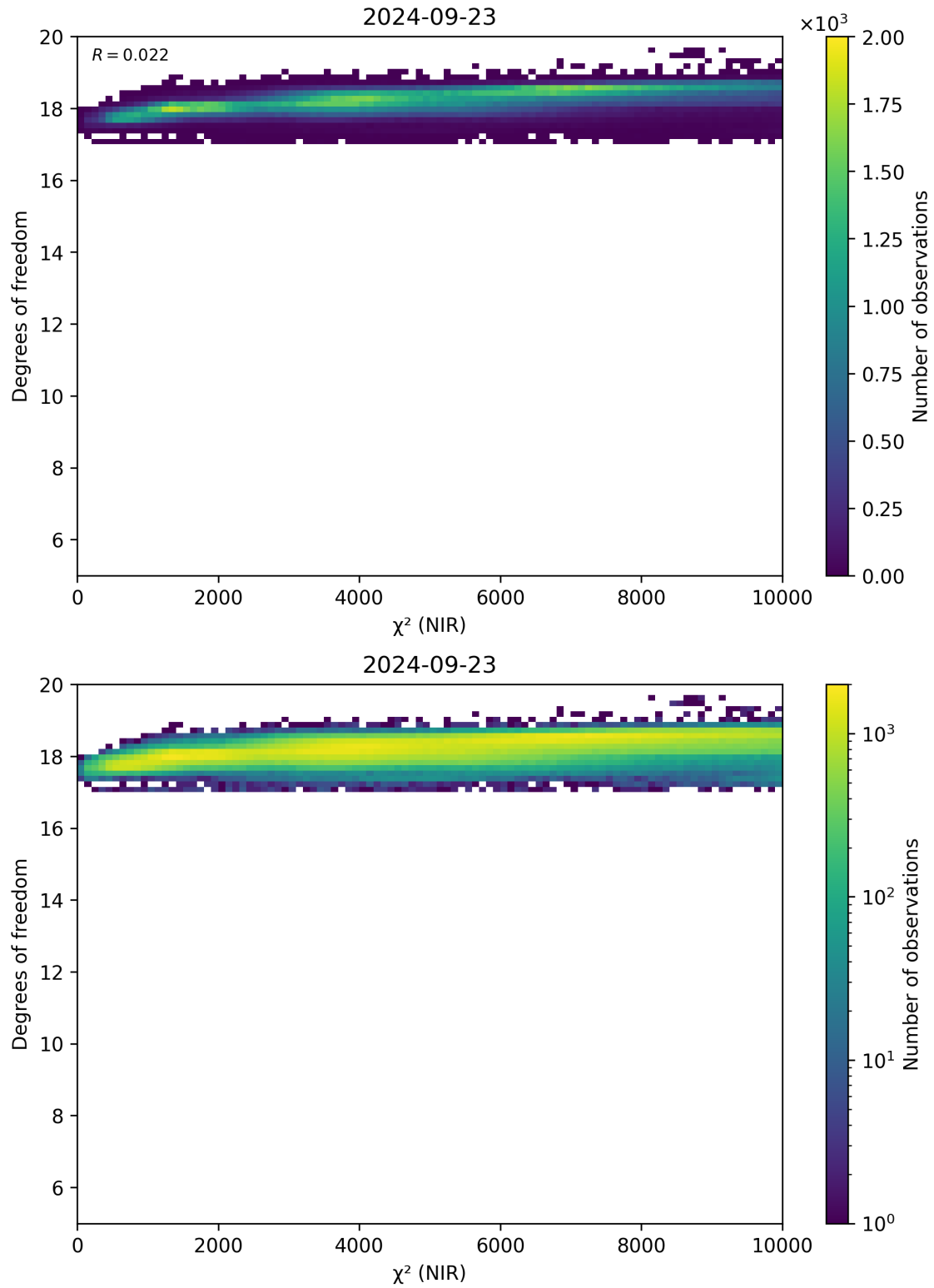
Figure 44: Scatter density plot of “ \chi^2 (NIR)” against “Degrees of freedom” for 2024-09-22 to 2024-09-24.
