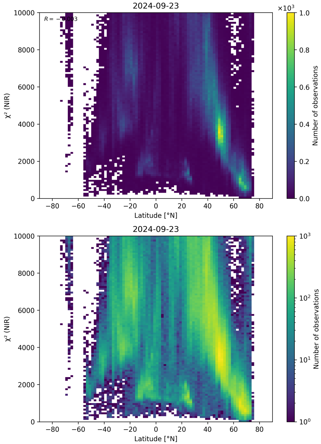
Figure 53: Scatter density plot of “Latitude” against “ \chi^2 (NIR)” for 2024-09-22 to 2024-09-24.
