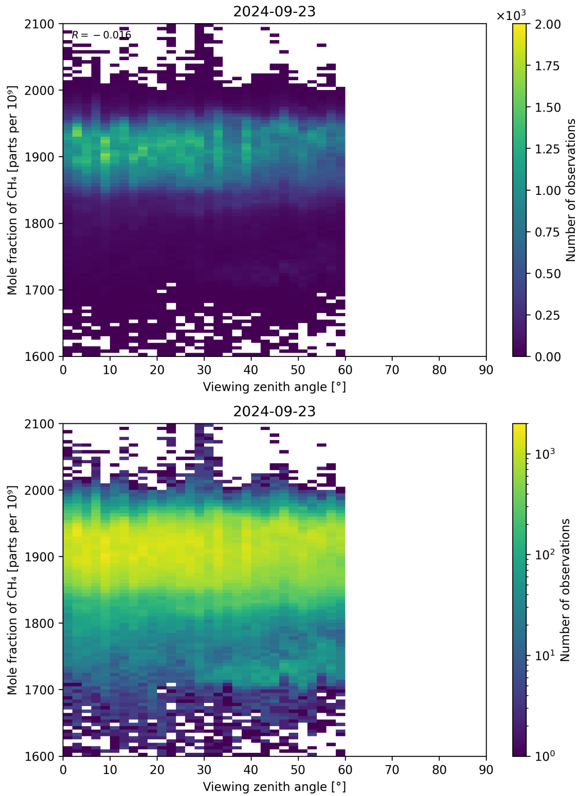
Figure 110: Scatter density plot of “Viewing zenith angle” against “Mole fraction of CH 4 ” for 2024-09-22 to 2024-09-24.
