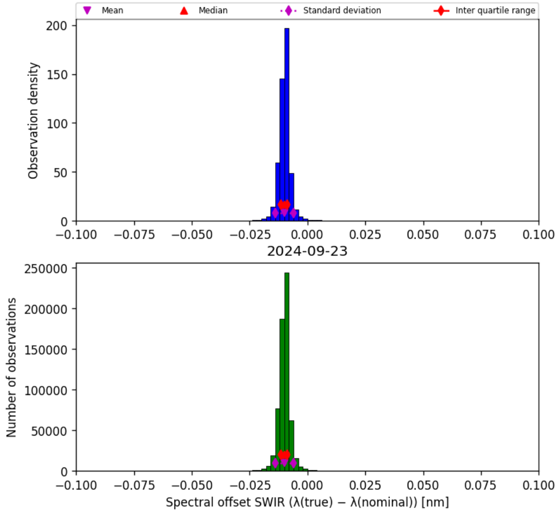
Figure 27: Histogram of “Spectral offset SWIR ( \lambda_{\text{true}} - \lambda_{\text{nominal}} )” for 2024-09-22 to 2024-09-24
