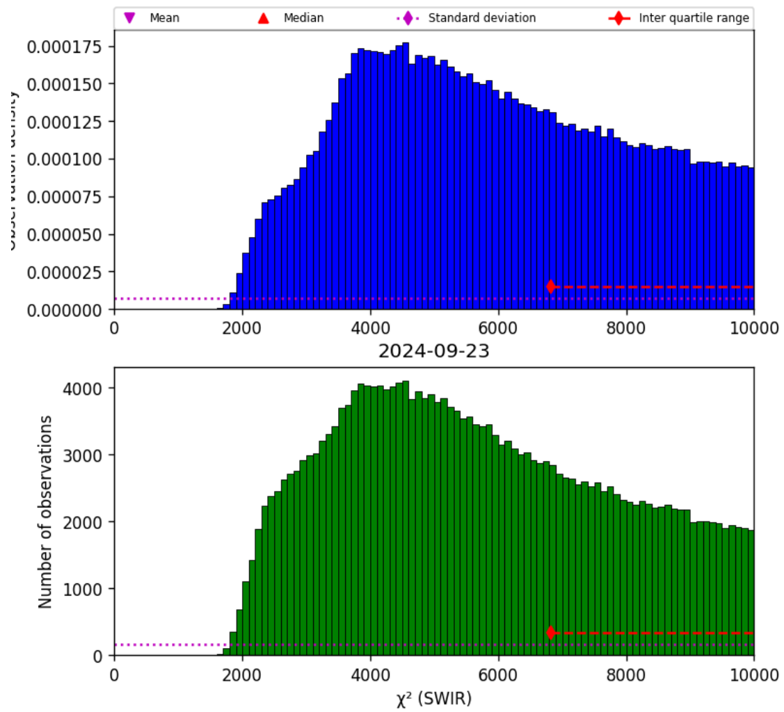
Figure 28: Histogram of " \chi^2 (SWIR)" for 2024-09-22 to 2024-09-24
