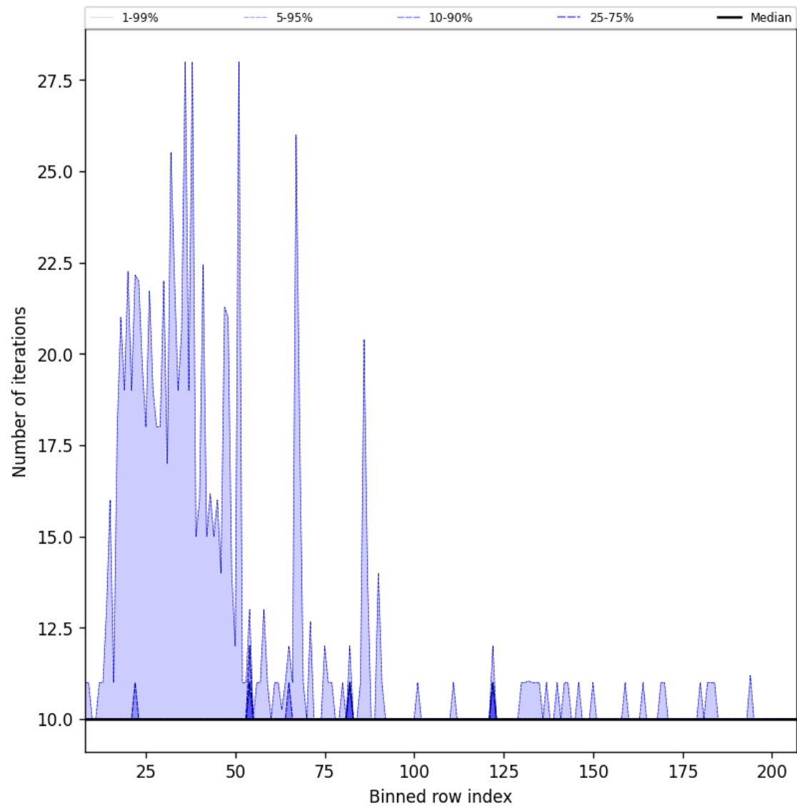
Figure 42: Along track statistics of “Number of iterations” for 2024-09-22 to 2024-09-24
