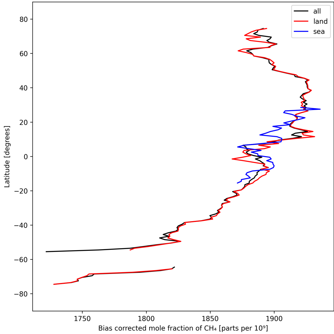
Figure 14: Zonal average of “Bias corrected mole fraction of \text{CH}_4 ” for 2024-09-22 to 2024-09-24.
