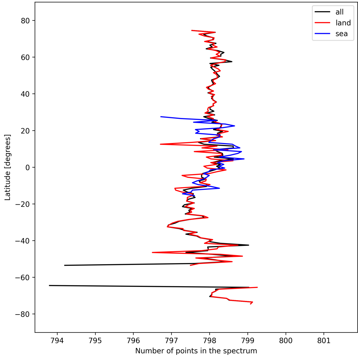
Figure 15: Zonal average of “Number of points in the spectrum” for 2024-09-23 to 2024-09-25.
