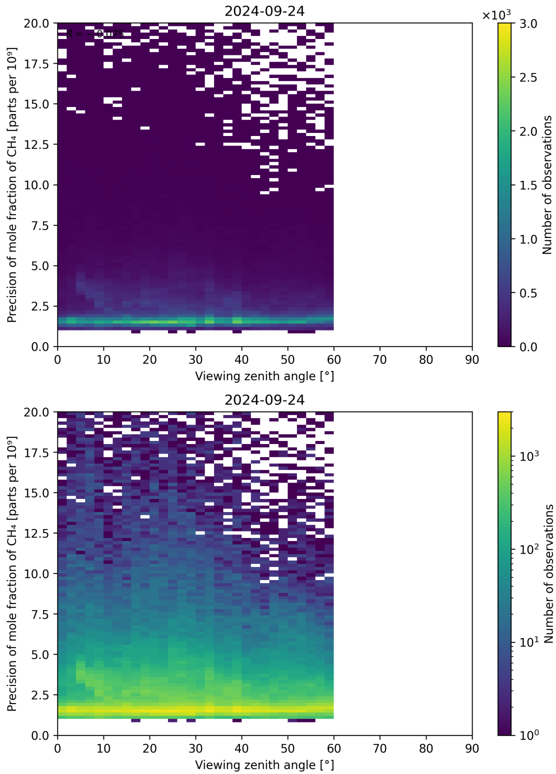
Figure 112: Scatter density plot of “Viewing zenith angle” against “Precision of mole fraction of CH 4 ” for 2024-09-23 to 2024-09-25.
