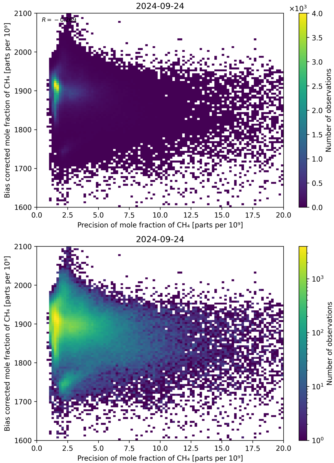
Figure 82: Scatter density plot of “Precision of mole fraction of CH 4 ” against “Bias corrected mole fraction of CH 4 ” for 2024-09-23 to 2024-09-25.
