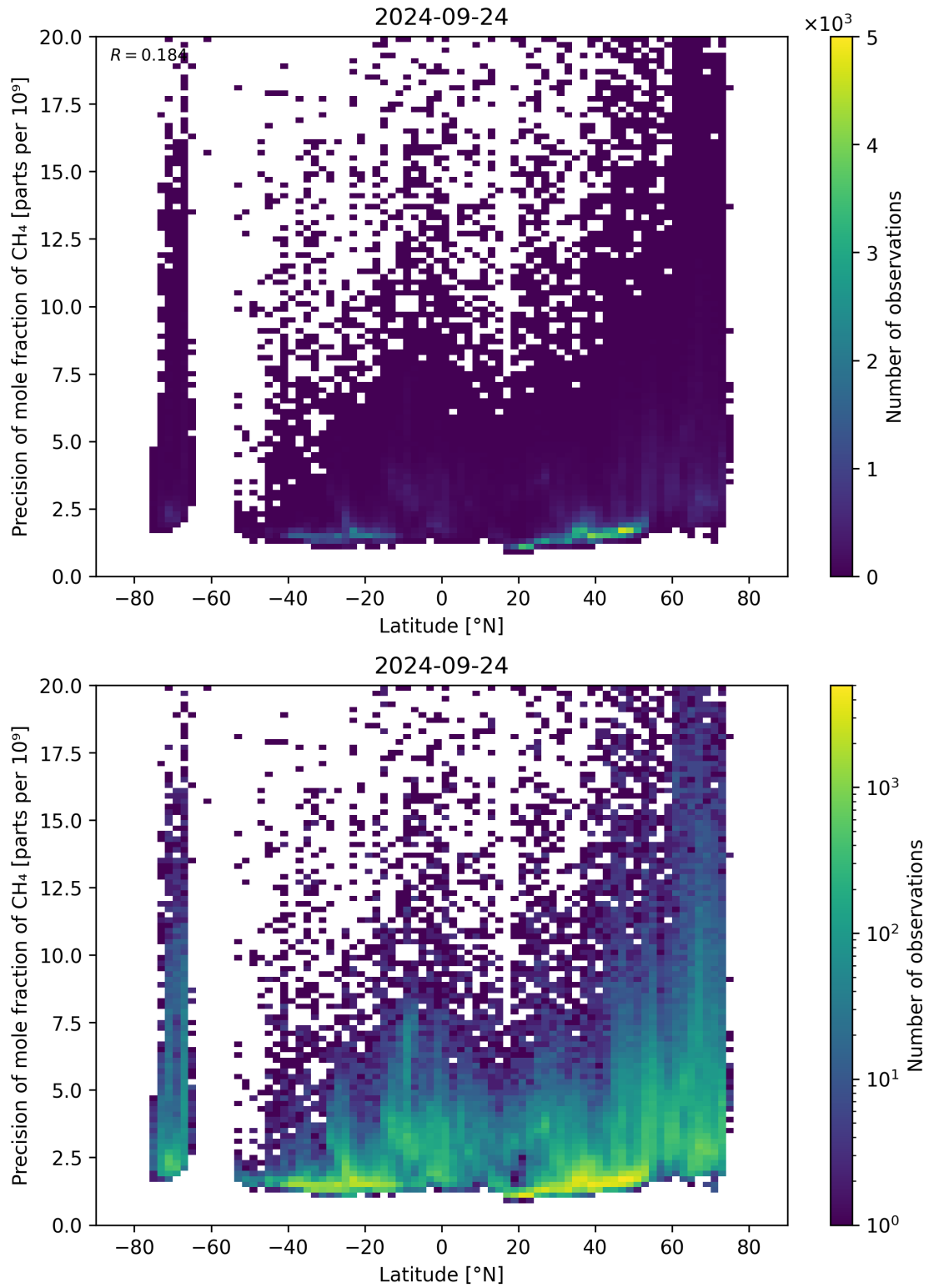
Figure 59: Scatter density plot of “Latitude” against “Precision of mole fraction of \text{CH}_4 ” for 2024-09-23 to 2024-09-25.
