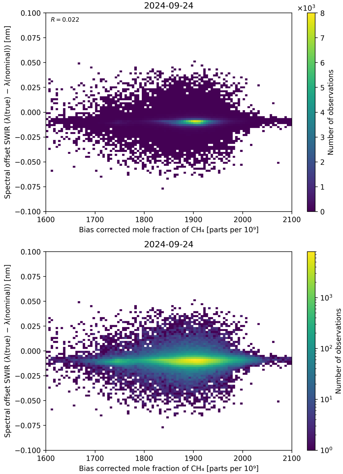
Figure 69: Scatter density plot of “Bias corrected mole fraction of \text{CH}_4 ” against “Spectral offset SWIR ( \lambda_{\text{true}} - \lambda_{\text{nominal}} )” for 2024-09-23 to 2024-09-25.
