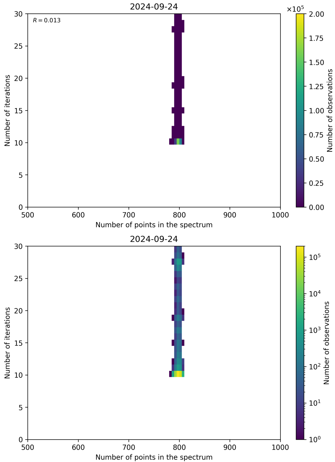
Figure 92: Scatter density plot of “Number of points in the spectrum” against “Number of iterations” for 2024-09-23 to 2024-09-25.
