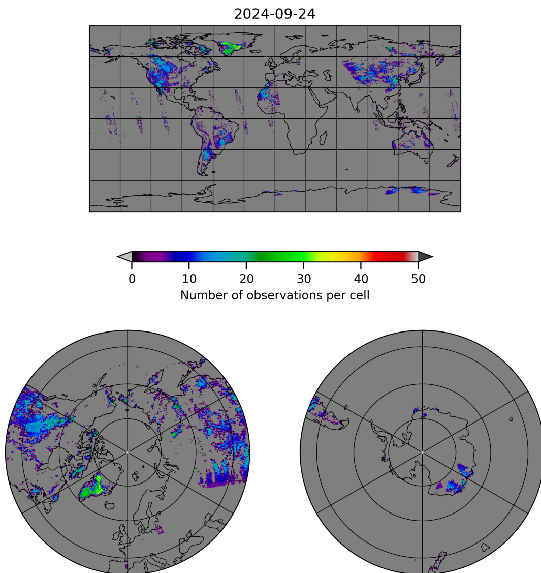
Figure 10: Map of the number of observations for 2024-09-23 to 2024-09-25
