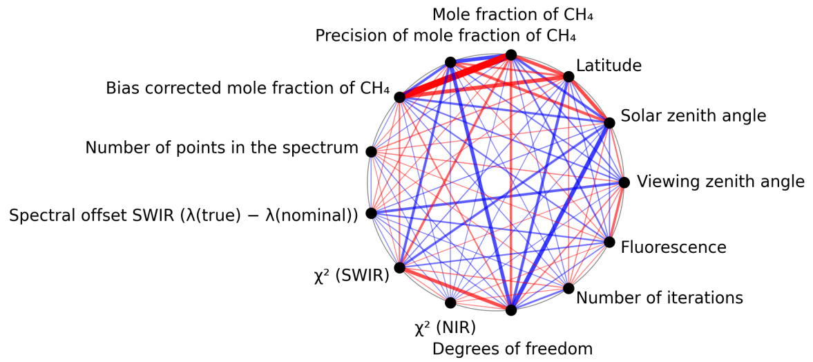
Figure 1: Map of correlation graph for 2024-09-23 to 2024-09-25.
