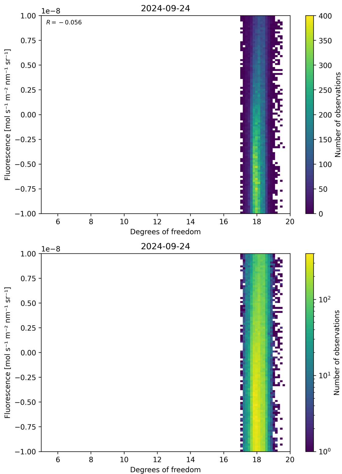
Figure 51: Scatter density plot of “Degrees of freedom” against “Fluorescence” for 2024-09-23 to 2024-09-25.
