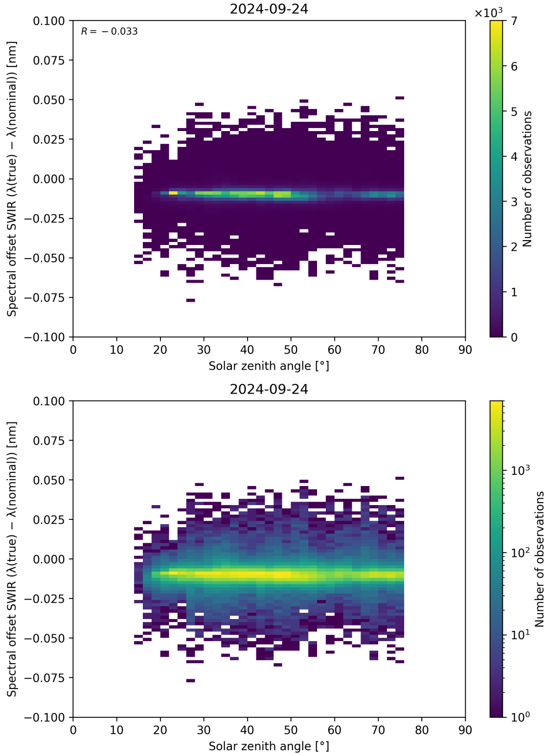
Figure 104: Scatter density plot of “Solar zenith angle” against “Spectral offset SWIR ( \lambda_{\text{true}} - \lambda_{\text{nominal}} )” for 2024-09-23 to 2024-09-25.
