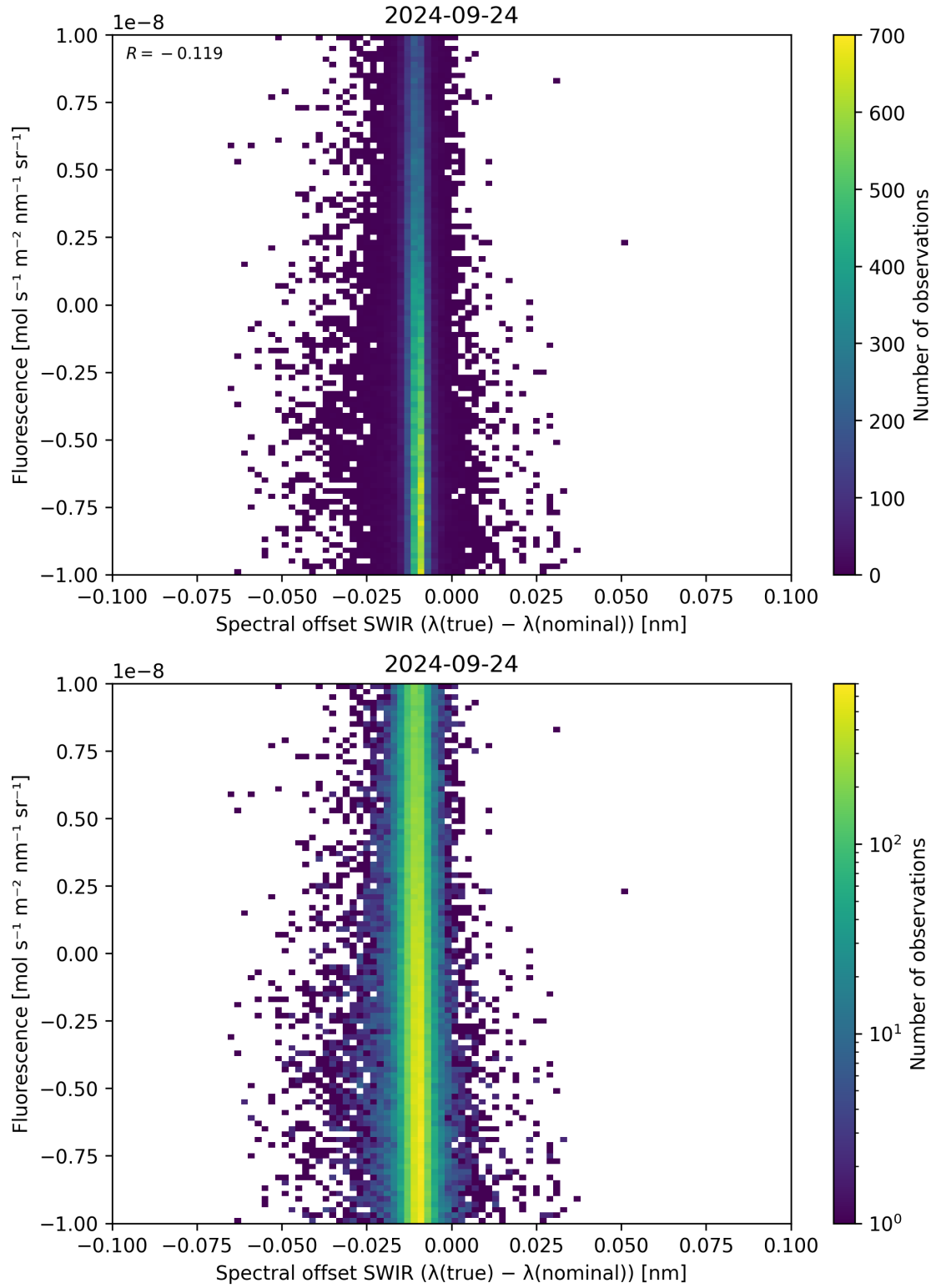
Figure 120: Scatter density plot of “Spectral offset SWIR ( \lambda_{\text{true}} - \lambda_{\text{nominal}} )” against “Fluorescence” for 2024-09-23 to 2024-09-25.
