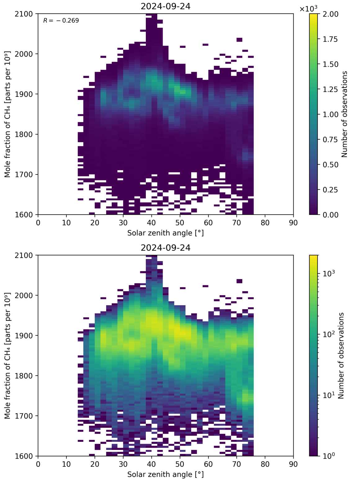
Figure 99: Scatter density plot of “Solar zenith angle” against “Mole fraction of CH 4 ” for 2024-09-23 to 2024-09-25.
