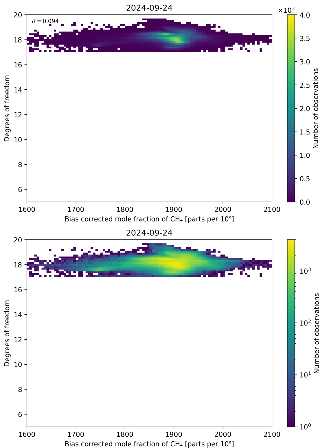
Figure 65: Scatter density plot of “Bias corrected mole fraction of CH 4 ” against “Degrees of freedom” for 2024-09-23 to 2024-09-25.
