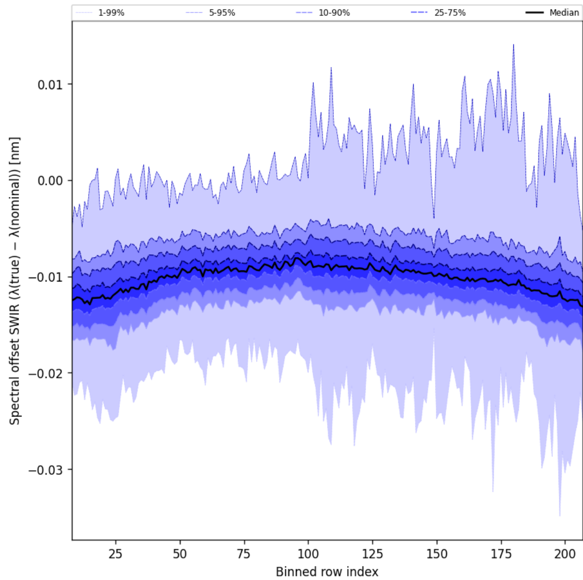
Figure 38: Along track statistics of “Spectral offset SWIR ( \lambda_{\text{true}} - \lambda_{\text{nominal}} )” for 2024-09-23 to 2024-09-25
