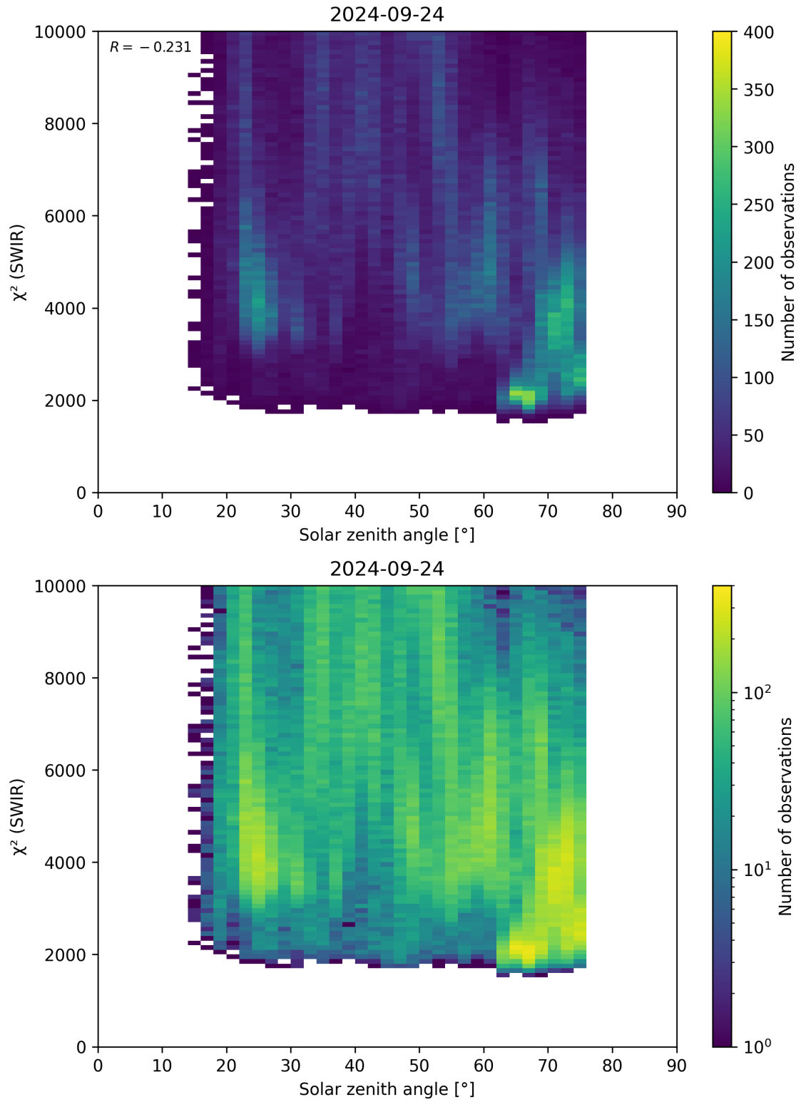
Figure 95: Scatter density plot of “Solar zenith angle” against “ \chi^2 (SWIR)” for 2024-09-23 to 2024-09-25.
