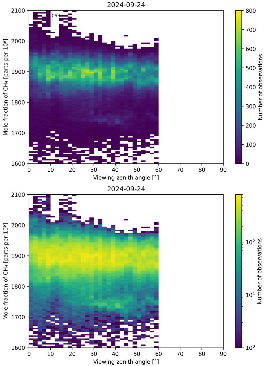
Figure 110: Scatter density plot of “Viewing zenith angle” against “Mole fraction of CH 4 ” for 2024-09-23 to 2024-09-25.
