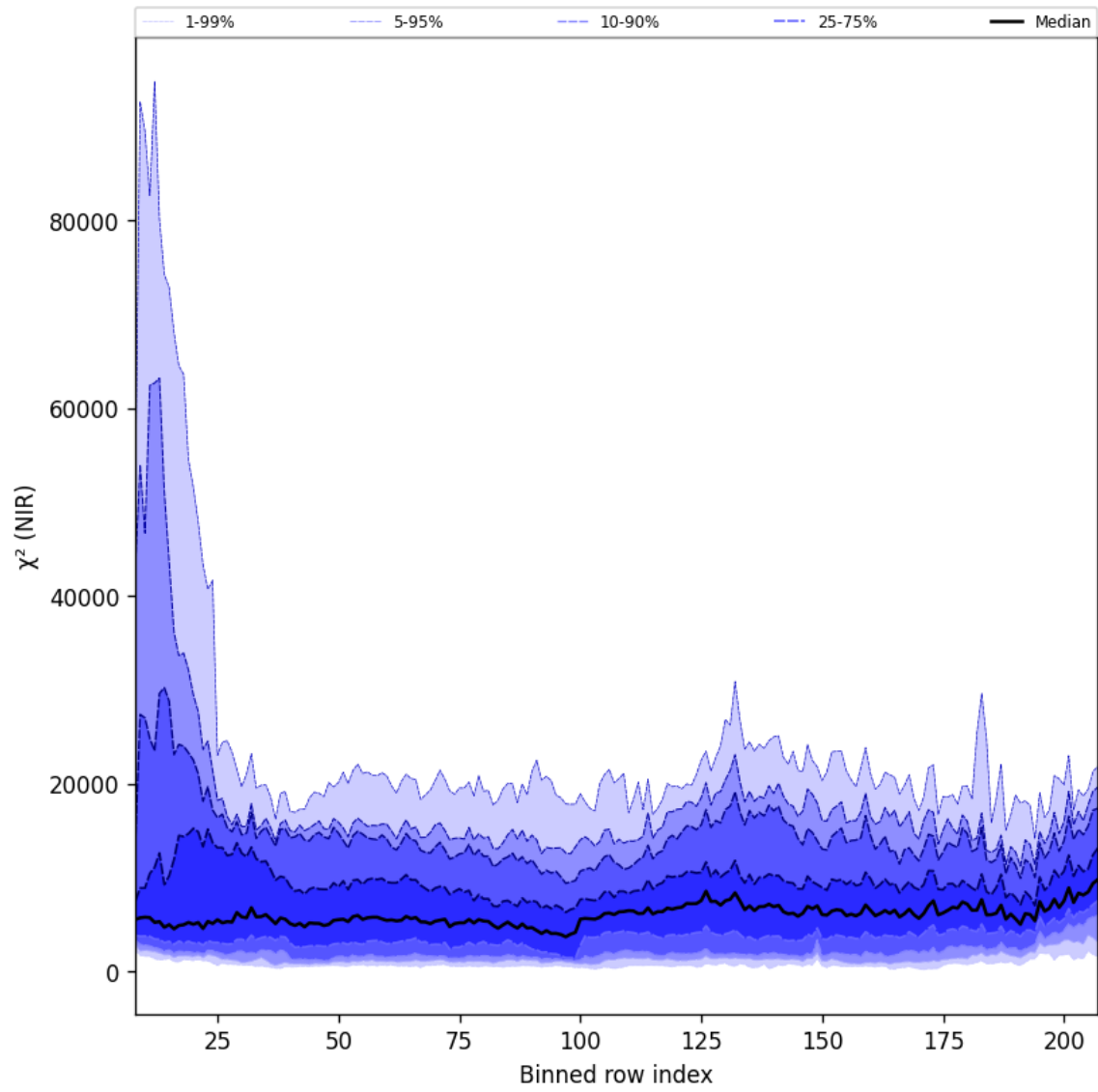
Figure 40: Along track statistics of “ \chi^2 (NIR)” for 2024-09-23 to 2024-09-25
