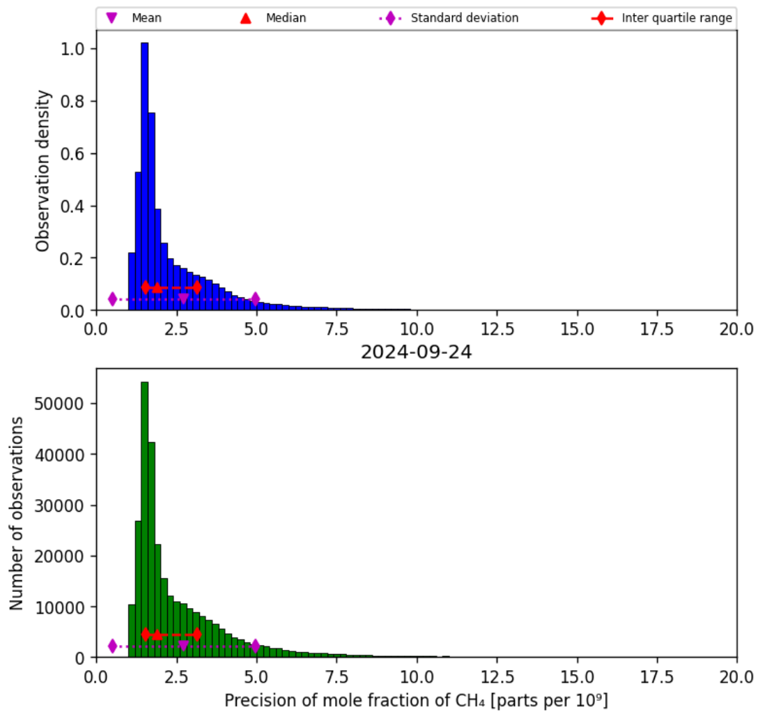
Figure 24: Histogram of “Precision of mole fraction of CH 4 ” for 2024-09-23 to 2024-09-25
