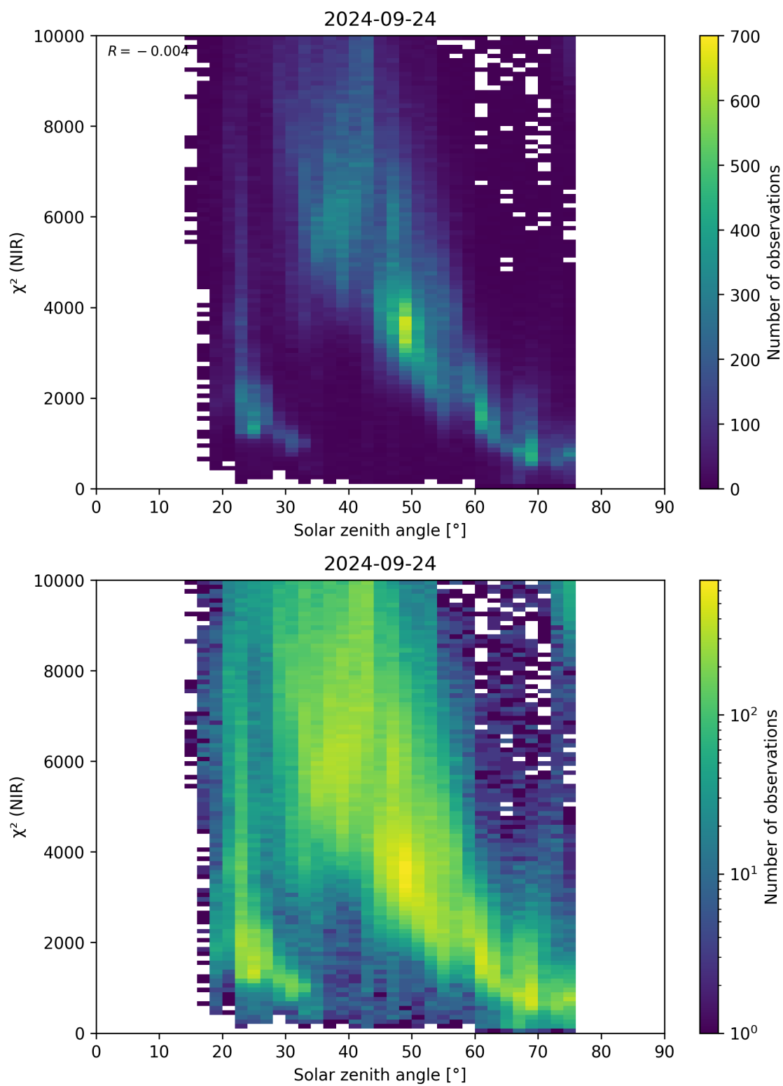
Figure 94: Scatter density plot of “Solar zenith angle” against “ \chi^2 (NIR)” for 2024-09-23 to 2024-09-25.
