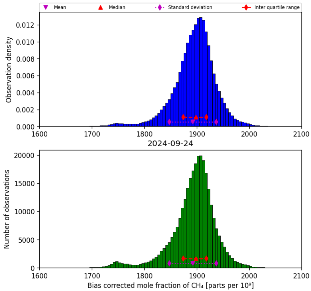
Figure 25: Histogram of “Bias corrected mole fraction of CH 4 ” for 2024-09-23 to 2024-09-25
