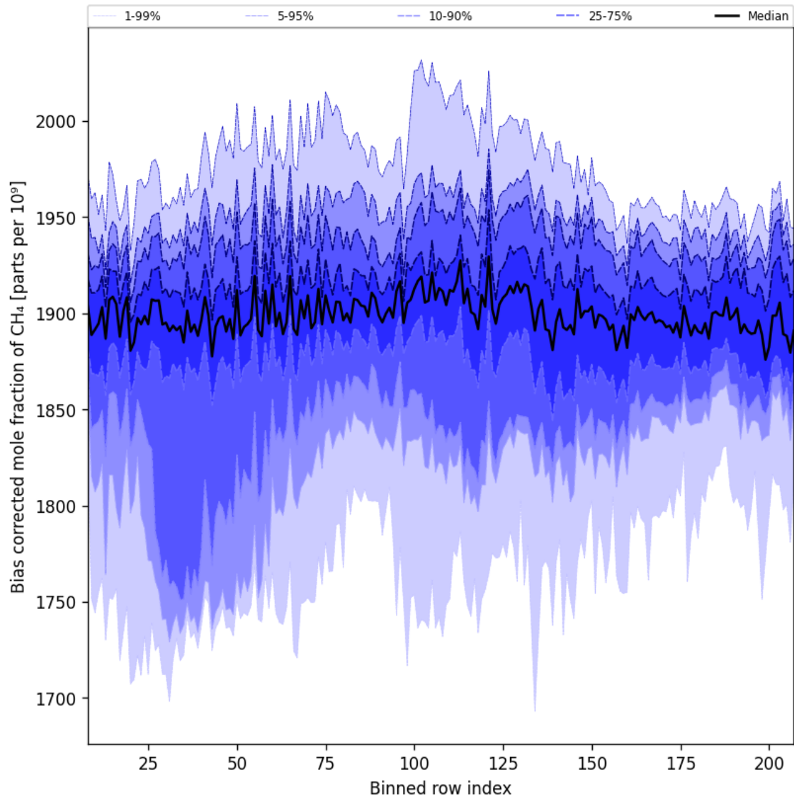
Figure 36: Along track statistics of “Bias corrected mole fraction of CH 4 ” for 2024-09-23 to 2024-09-25
