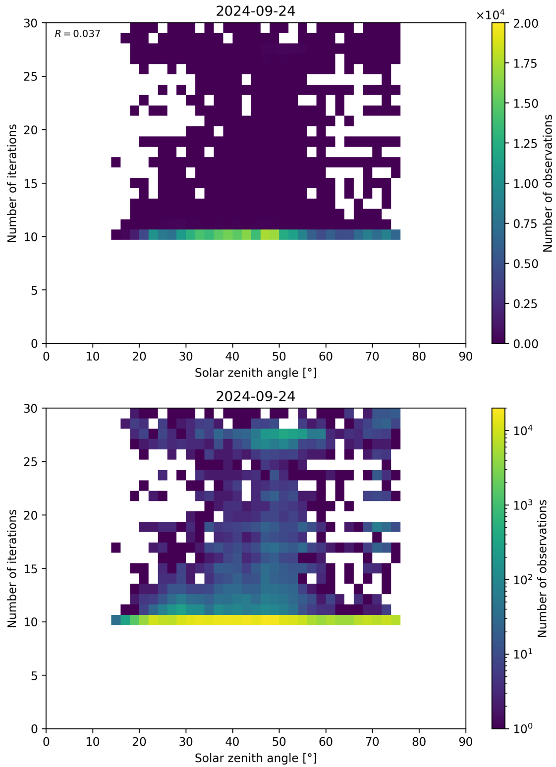
Figure 102: Scatter density plot of “Solar zenith angle” against “Number of iterations” for 2024-09-23 to 2024-09-25.
