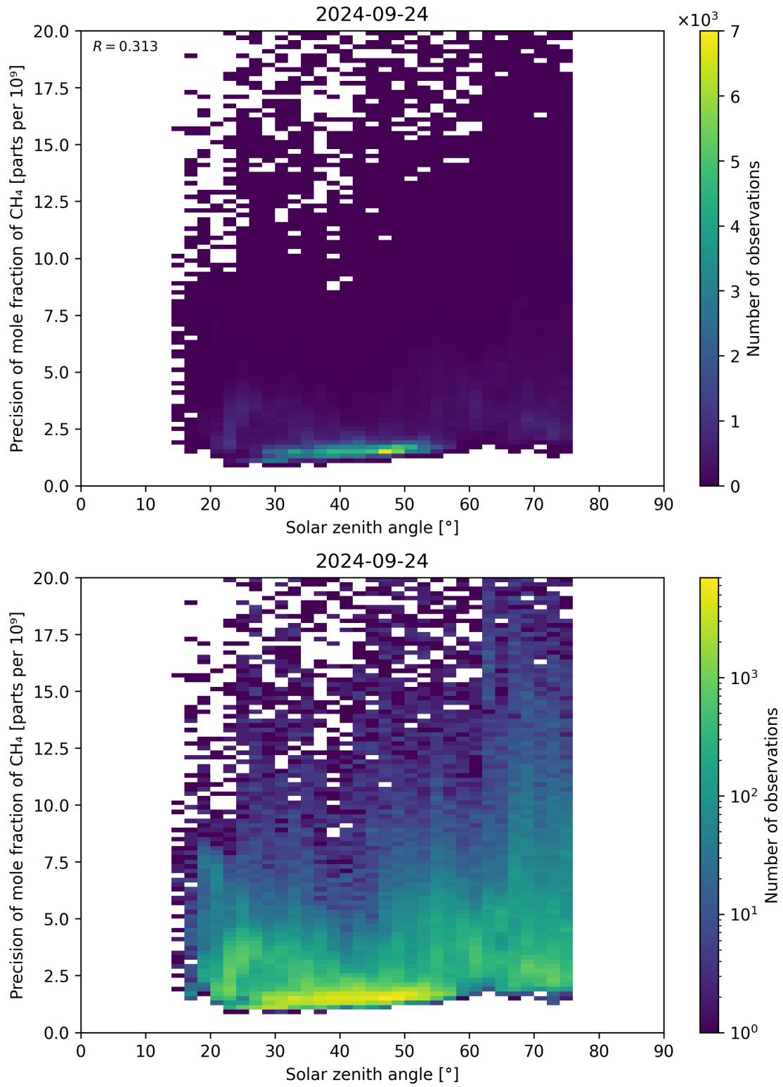
Figure 101: Scatter density plot of “Solar zenith angle” against “Precision of mole fraction of CH 4 ” for 2024-09-23 to 2024-09-25.
