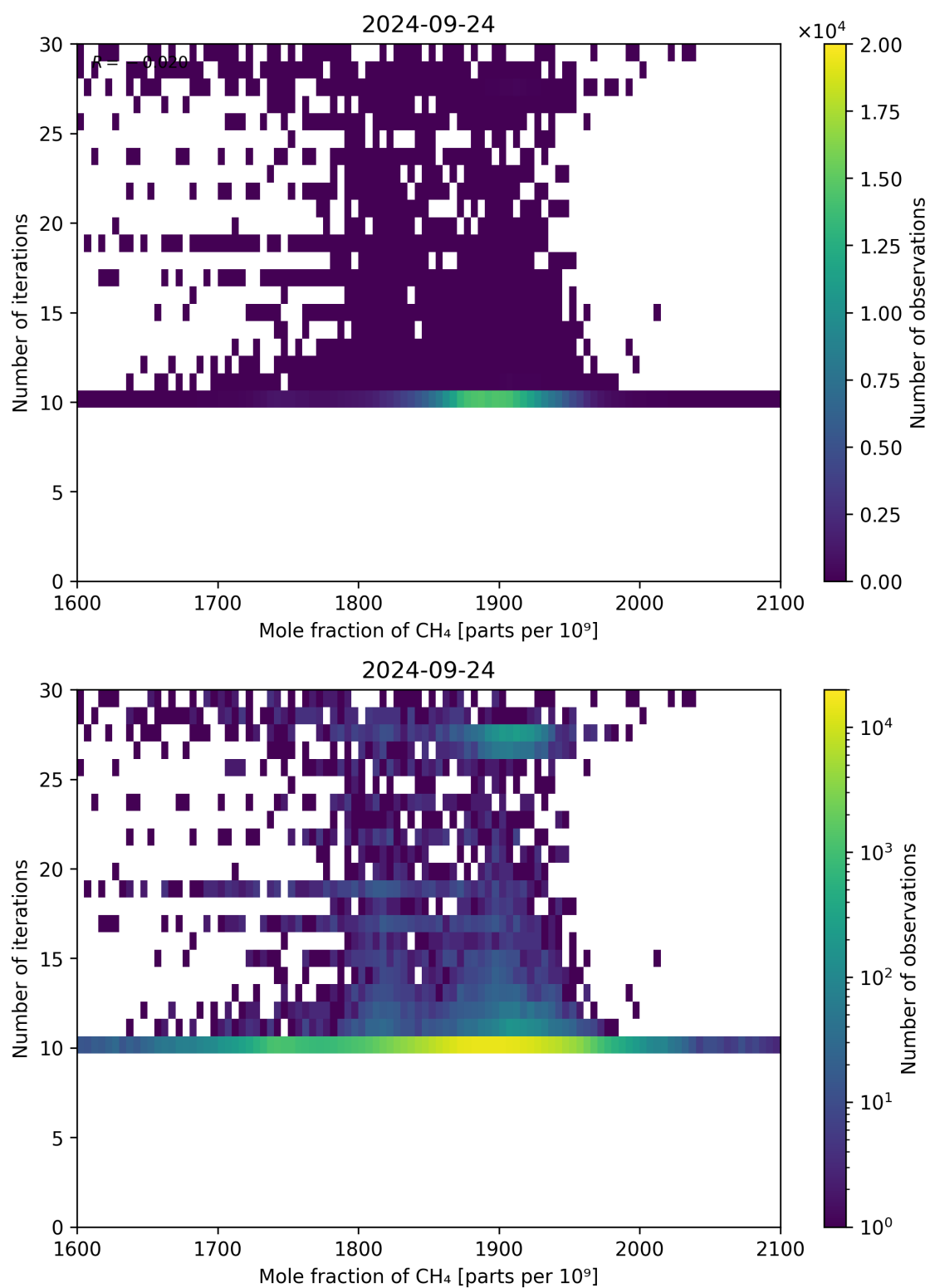
Figure 76: Scatter density plot of “Mole fraction of CH 4 ” against “Number of iterations” for 2024-09-23 to 2024-09-25.
