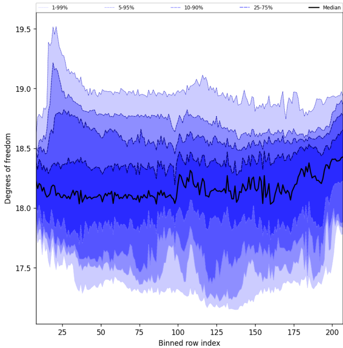
Figure 41: Along track statistics of “Degrees of freedom” for 2024-09-23 to 2024-09-25
