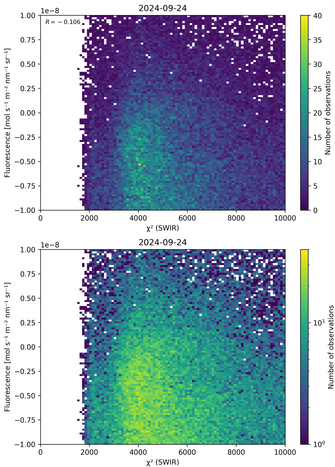
Figure 49: Scatter density plot of “ \chi^2 (SWIR)” against “Fluorescence” for 2024-09-23 to 2024-09-25.
