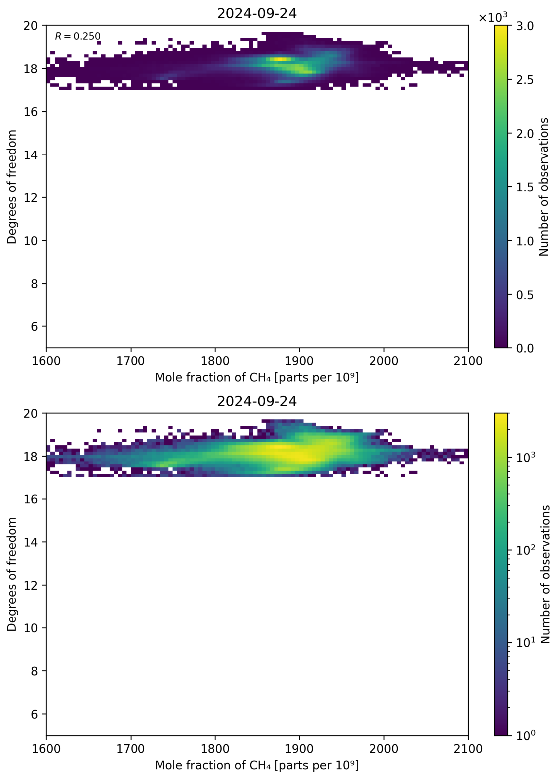
Figure 72: Scatter density plot of “Mole fraction of CH 4 ” against “Degrees of freedom” for 2024-09-23 to 2024-09-25.
