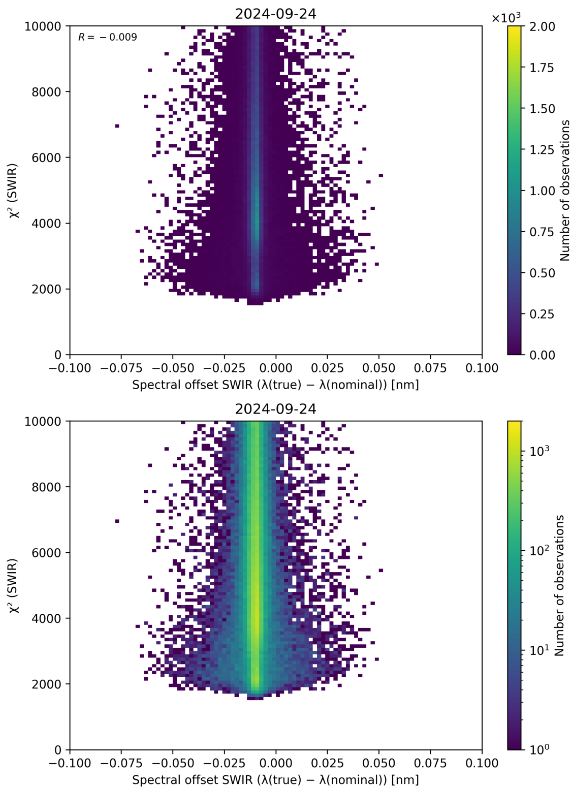
Figure 118: Scatter density plot of “Spectral offset SWIR ( \lambda_{\text{true}} - \lambda_{\text{nominal}} )” against “ \chi^2 (SWIR)” for 2024-09-23 to 2024-09-25.
