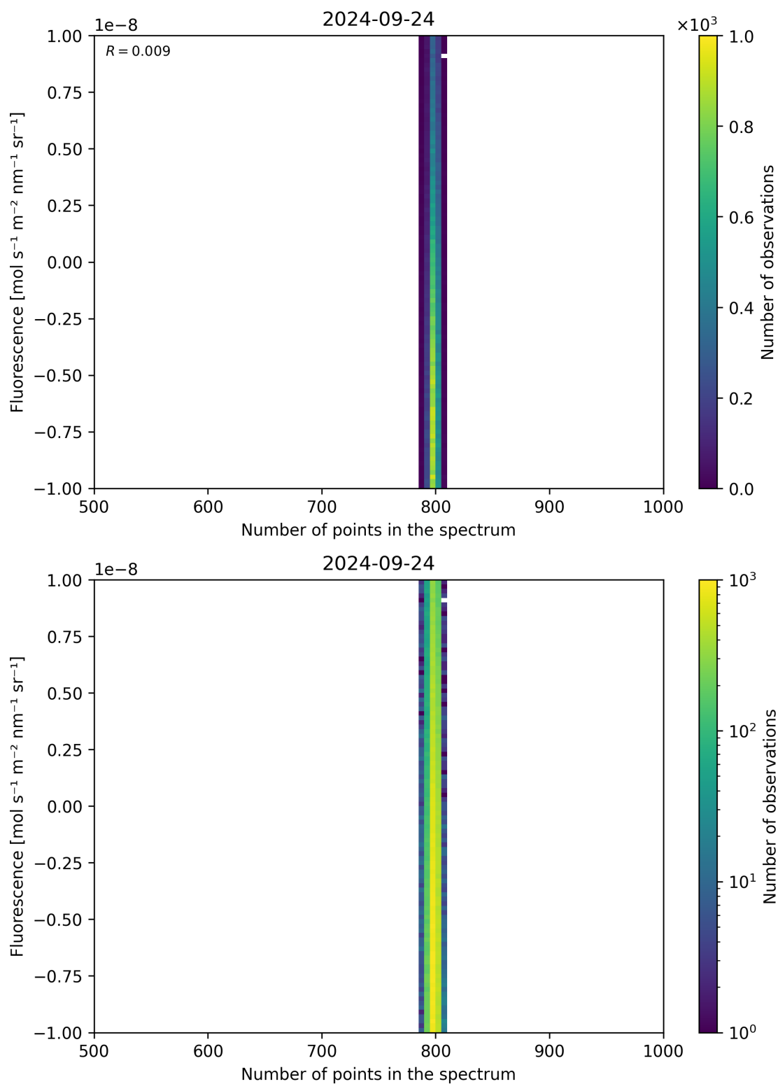
Figure 91: Scatter density plot of “Number of points in the spectrum” against “Fluorescence” for 2024-09-23 to 2024-09-25.
