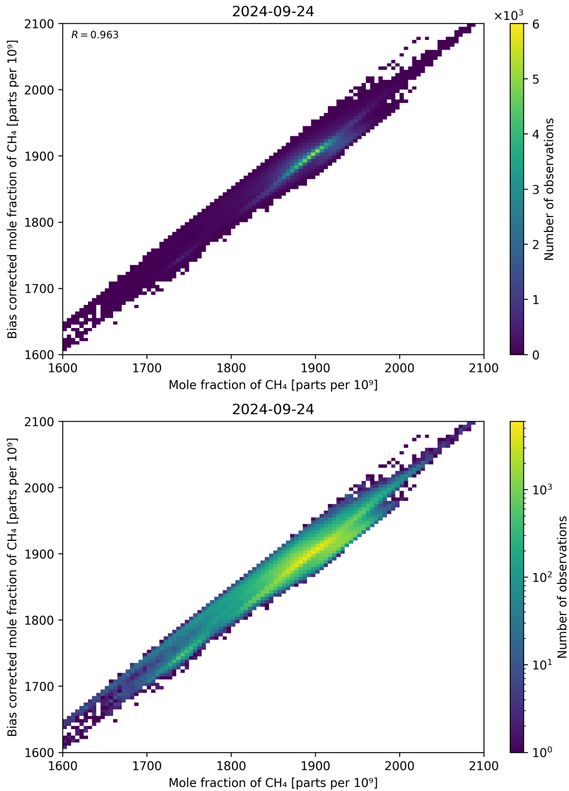
Figure 74: Scatter density plot of “Mole fraction of CH 4 ” against “Bias corrected mole fraction of CH 4 ” for 2024-09-23 to 2024-09-25.
