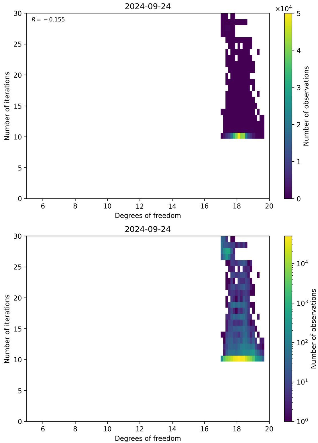
Figure 52: Scatter density plot of “Degrees of freedom” against “Number of iterations” for 2024-09-23 to 2024-09-25.
