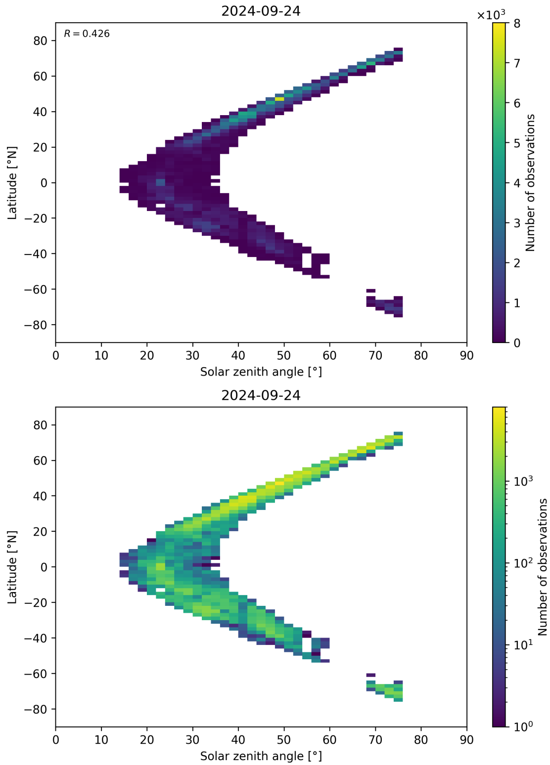
Figure 98: Scatter density plot of “Solar zenith angle” against “Latitude” for 2024-09-23 to 2024-09-25.
