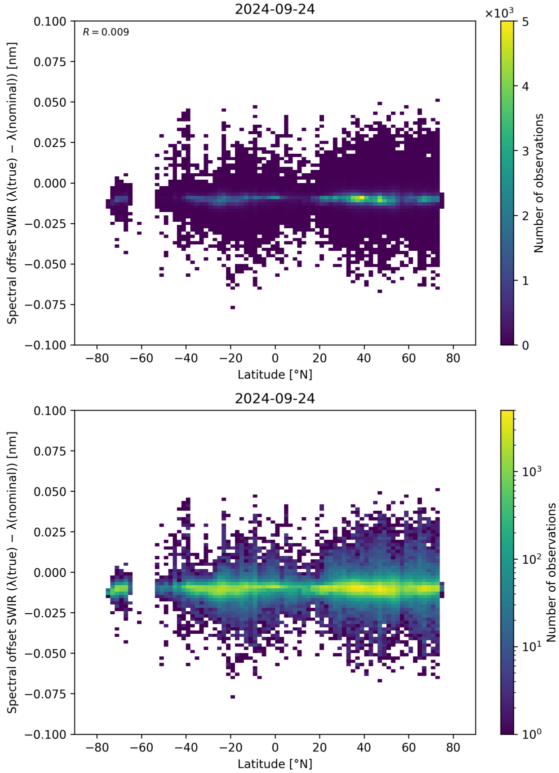
Figure 62: Scatter density plot of “Latitude” against “Spectral offset SWIR ( \lambda_{\text{true}} - \lambda_{\text{nominal}} )” for 2024-09-23 to 2024-09-25.
