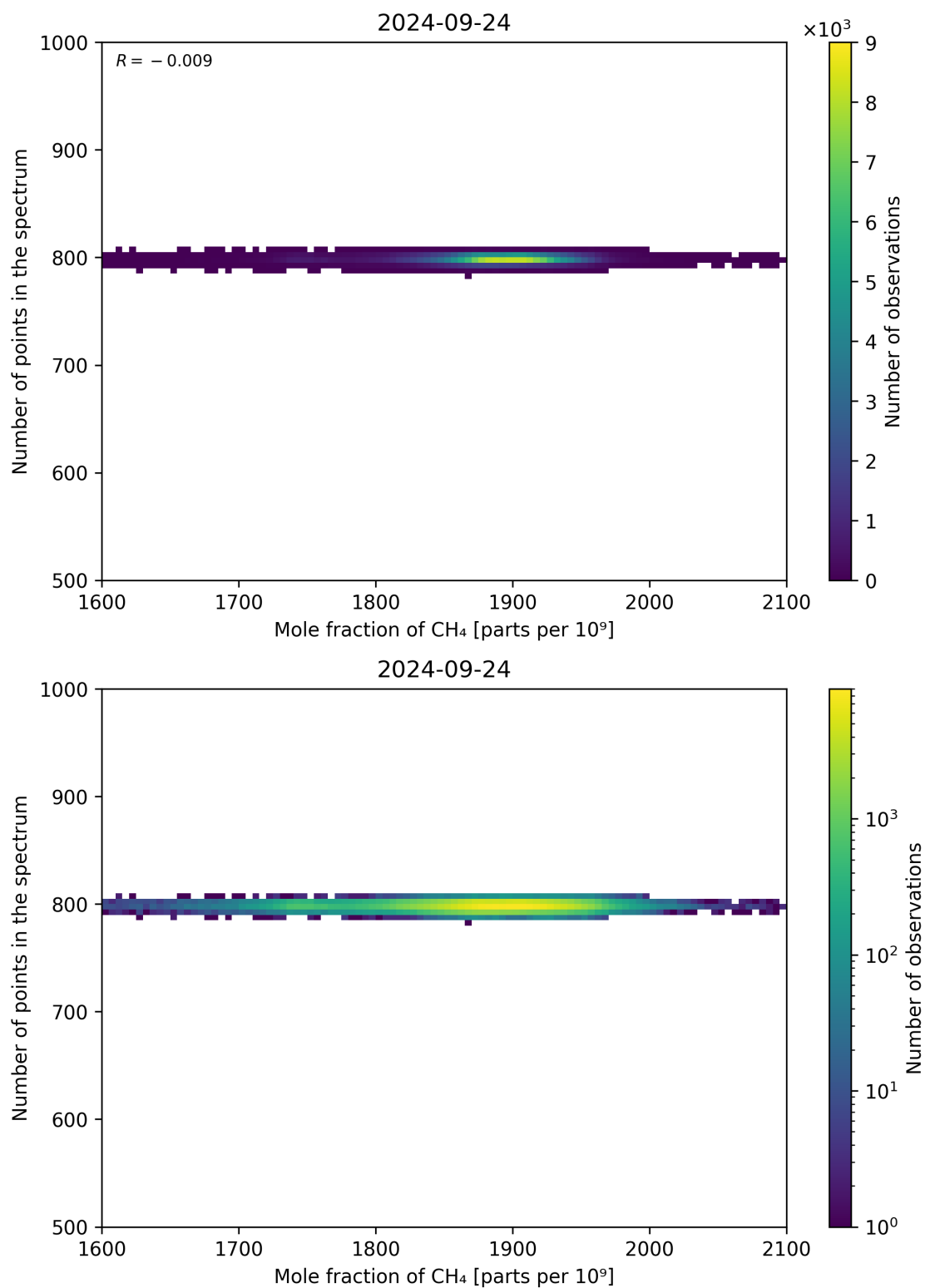
Figure 77: Scatter density plot of “Mole fraction of CH 4 ” against “Number of points in the spectrum” for 2024-09-23 to 2024-09-25.
