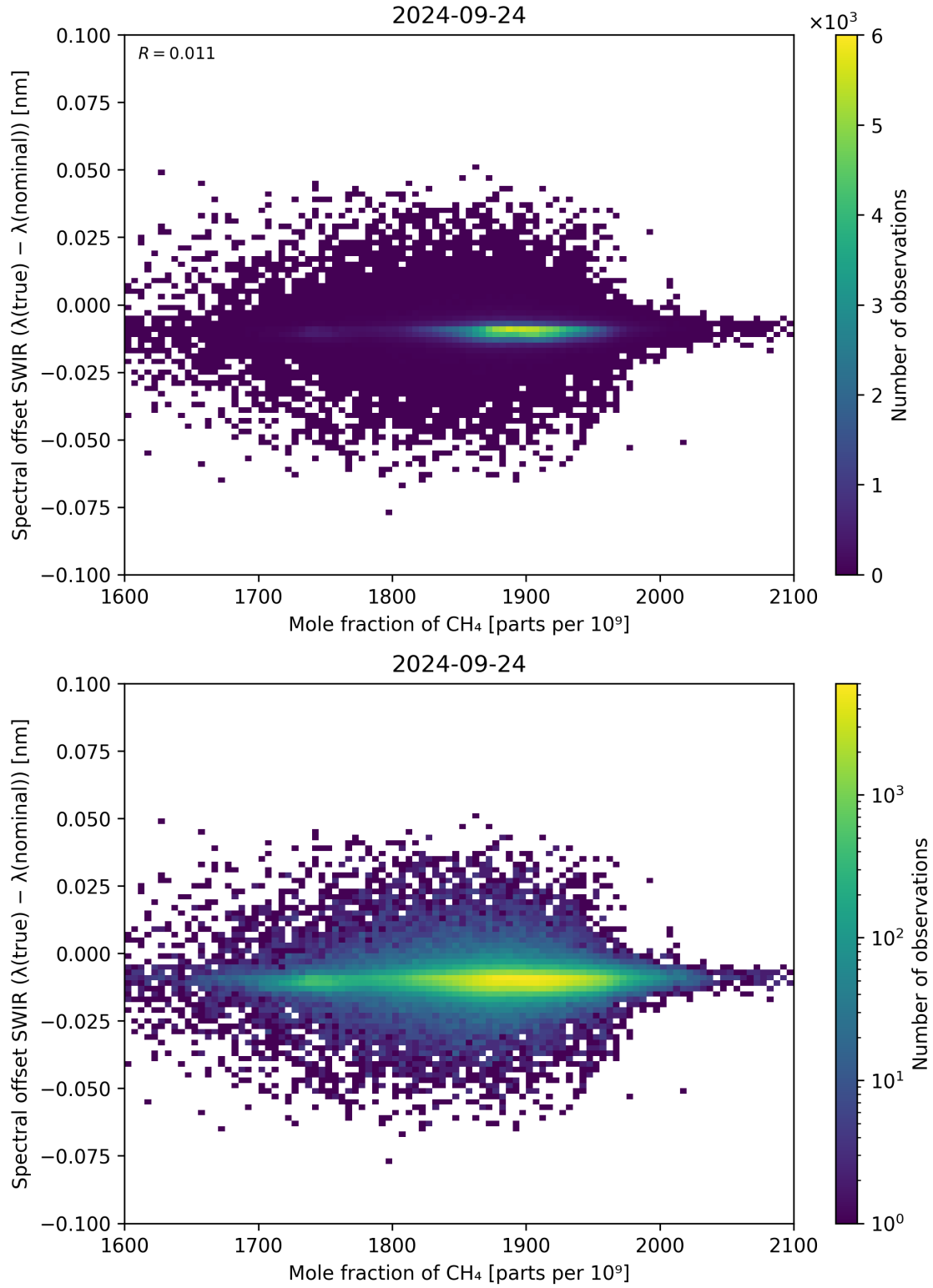
Figure 86: Scatter density plot of “Mole fraction of \text{CH}_4 ” against “Spectral offset SWIR ( \lambda_{\text{true}} - \lambda_{\text{nominal}} )” for 2024-09-23 to 2024-09-25.
