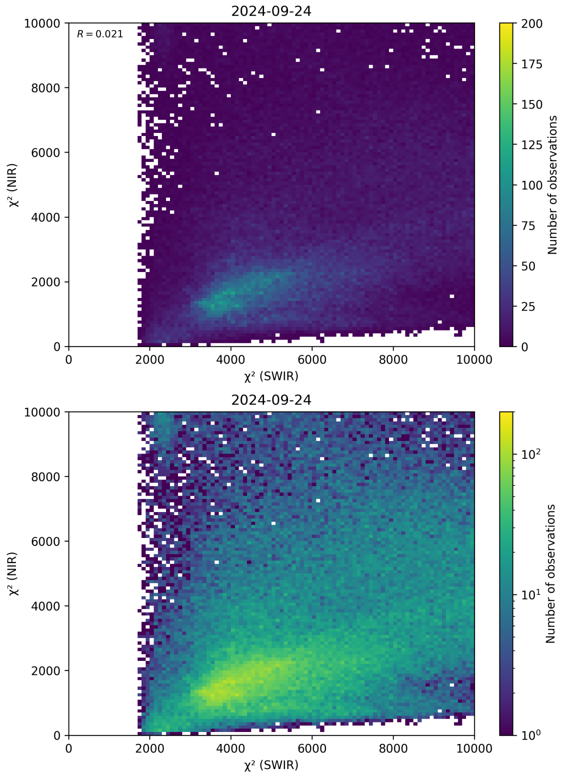
Figure 47: Scatter density plot of “ \chi^2 (SWIR)” against “ \chi^2 (NIR)” for 2024-09-23 to 2024-09-25.
