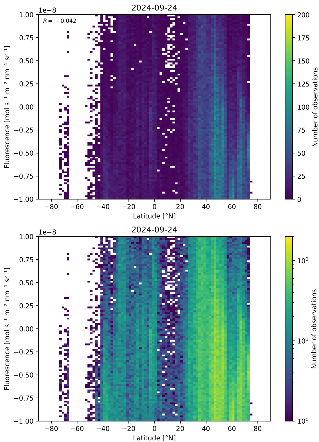
Figure 56: Scatter density plot of “Latitude” against “Fluorescence” for 2024-09-23 to 2024-09-25.
