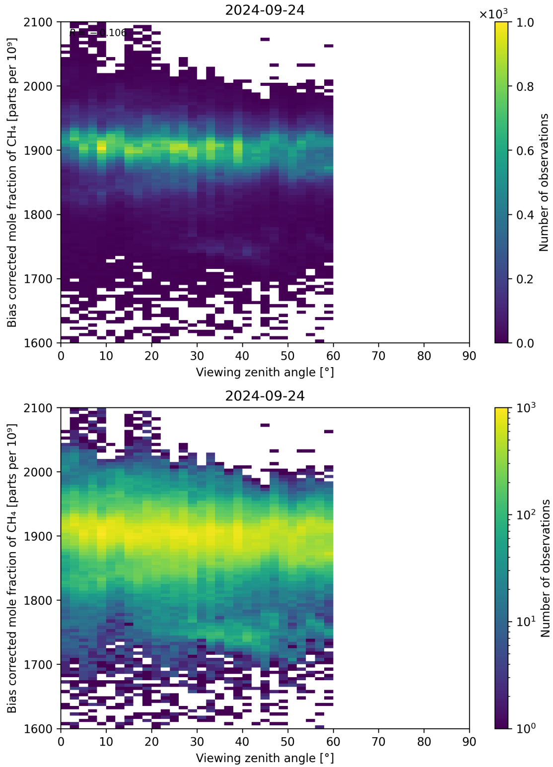
Figure 111: Scatter density plot of “Viewing zenith angle” against “Bias corrected mole fraction of CH 4 ” for 2024-09-23 to 2024-09-25.
