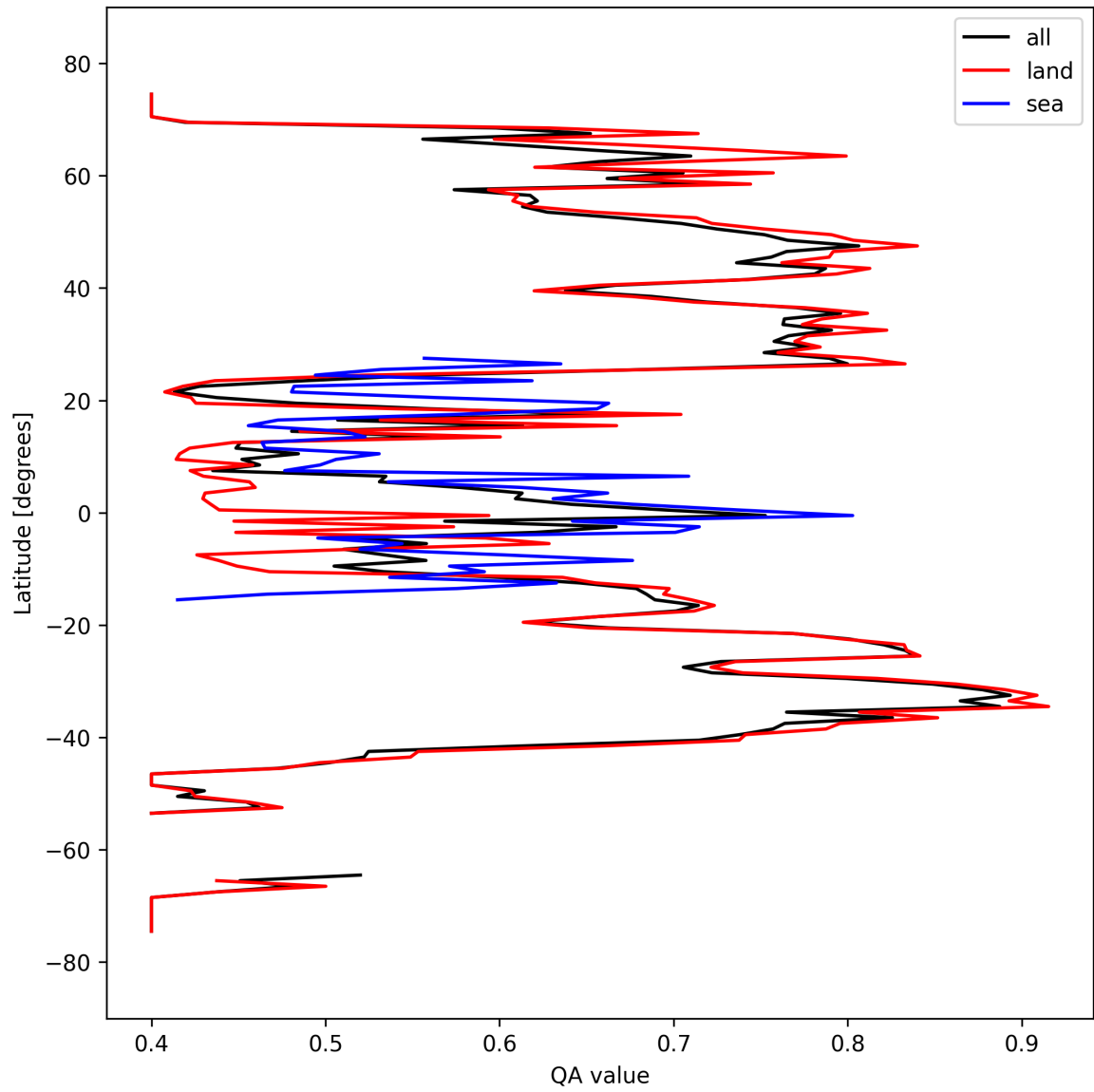
Figure 11: Zonal average of “QA value” for 2024-09-23 to 2024-09-25.
