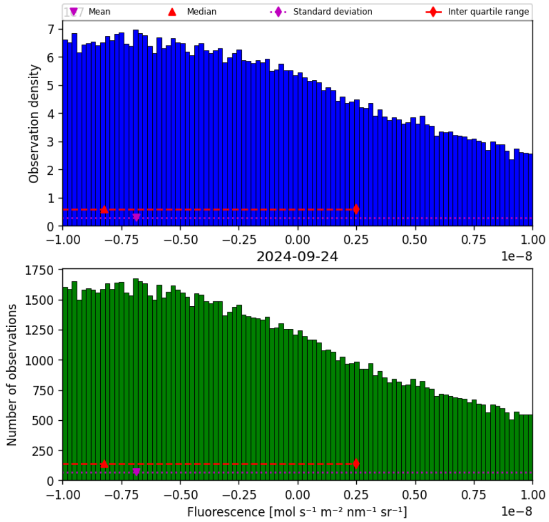
Figure 32: Histogram of “Fluorescence” for 2024-09-23 to 2024-09-25
