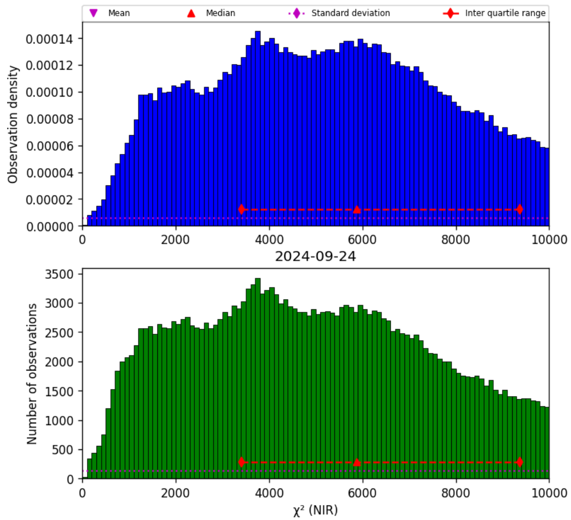
Figure 29: Histogram of “ \chi^2 (NIR)” for 2024-09-23 to 2024-09-25
