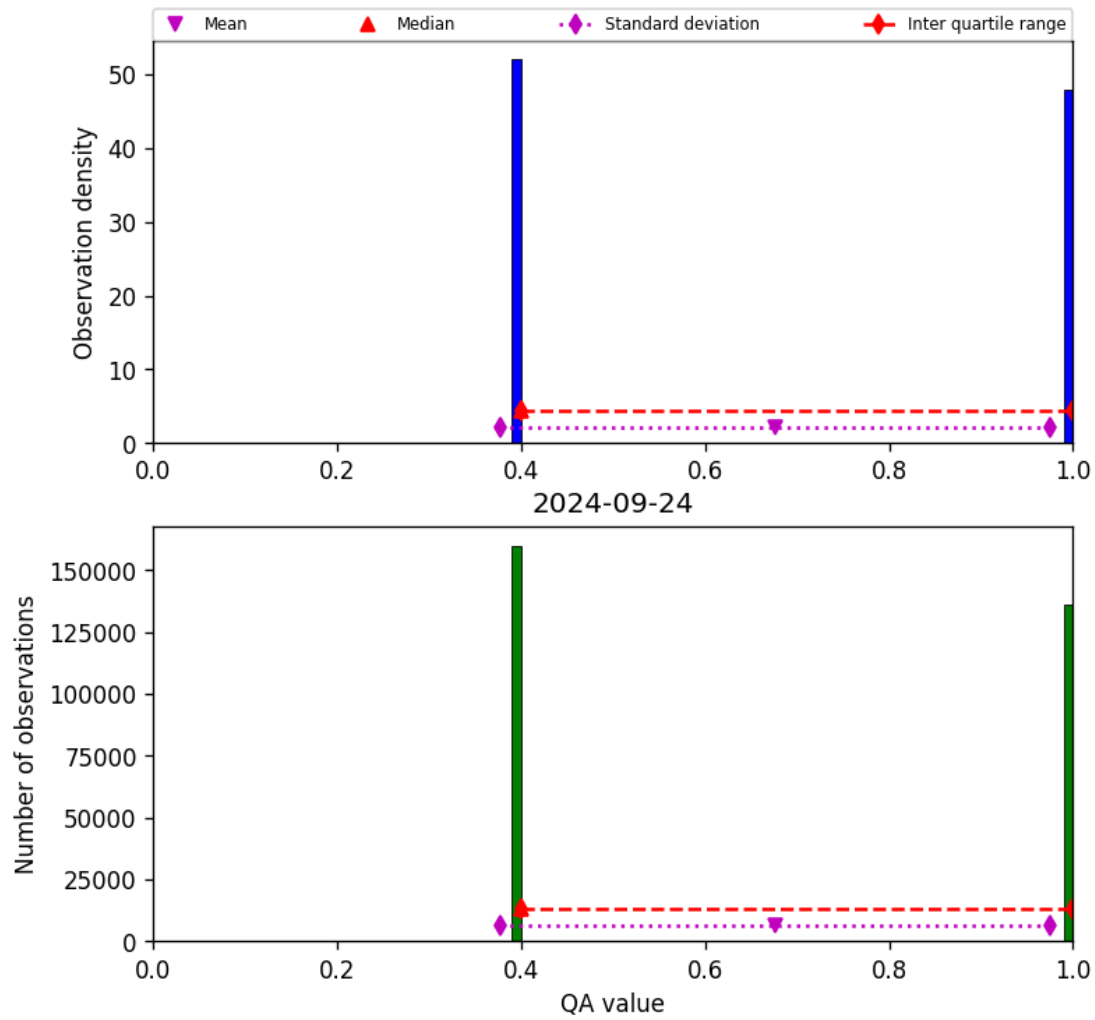
Figure 22: Histogram of “QA value” for 2024-09-23 to 2024-09-25
