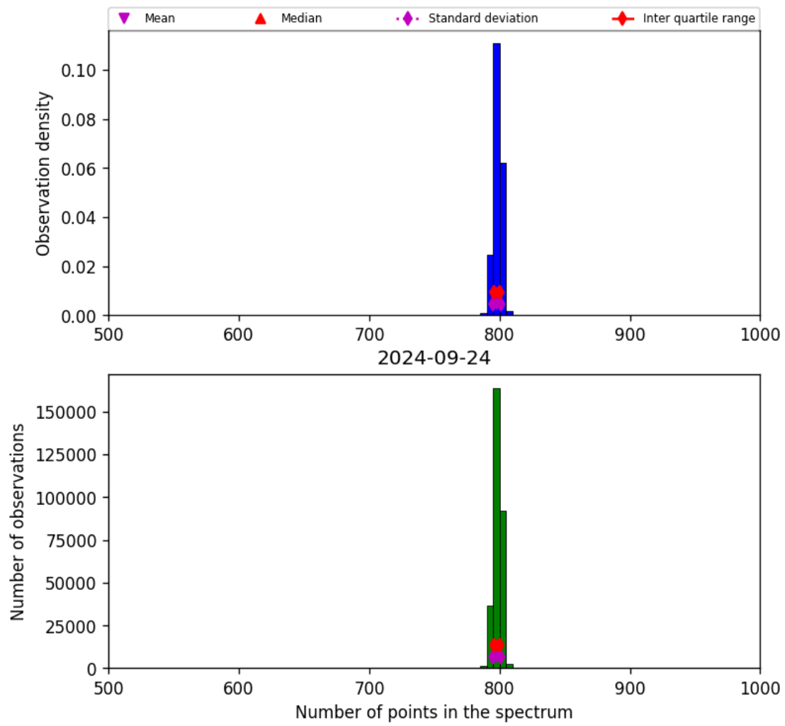
Figure 26: Histogram of “Number of points in the spectrum” for 2024-09-23 to 2024-09-25
