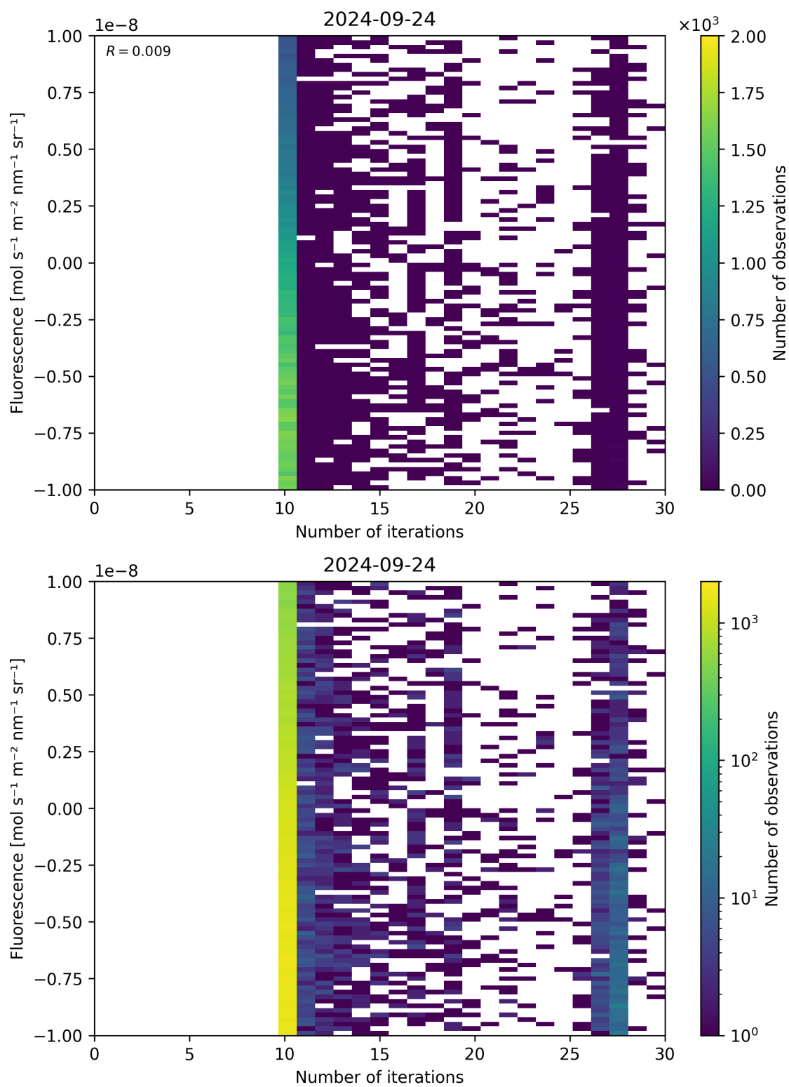
Figure 87: Scatter density plot of “Number of iterations” against “Fluorescence” for 2024-09-23 to 2024-09-25.
