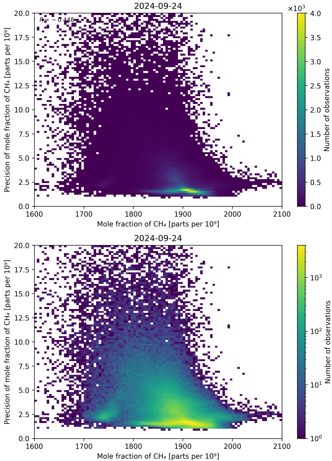
Figure 75: Scatter density plot of “Mole fraction of CH 4 ” against “Precision of mole fraction of CH 4 ” for 2024-09-23 to 2024-09-25.
