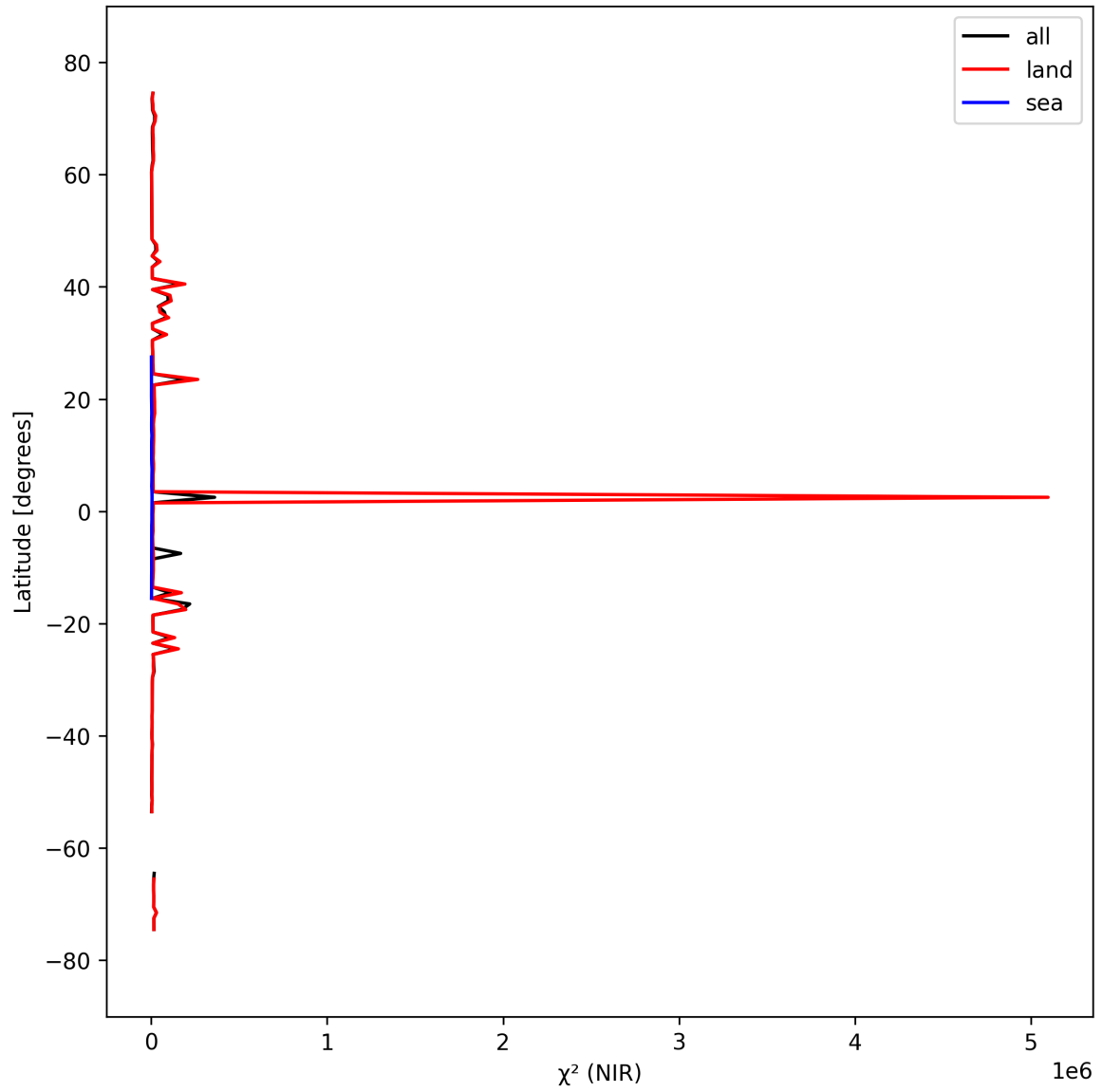
Figure 18: Zonal average of “ \chi^2 (NIR)” for 2024-09-23 to 2024-09-25.
