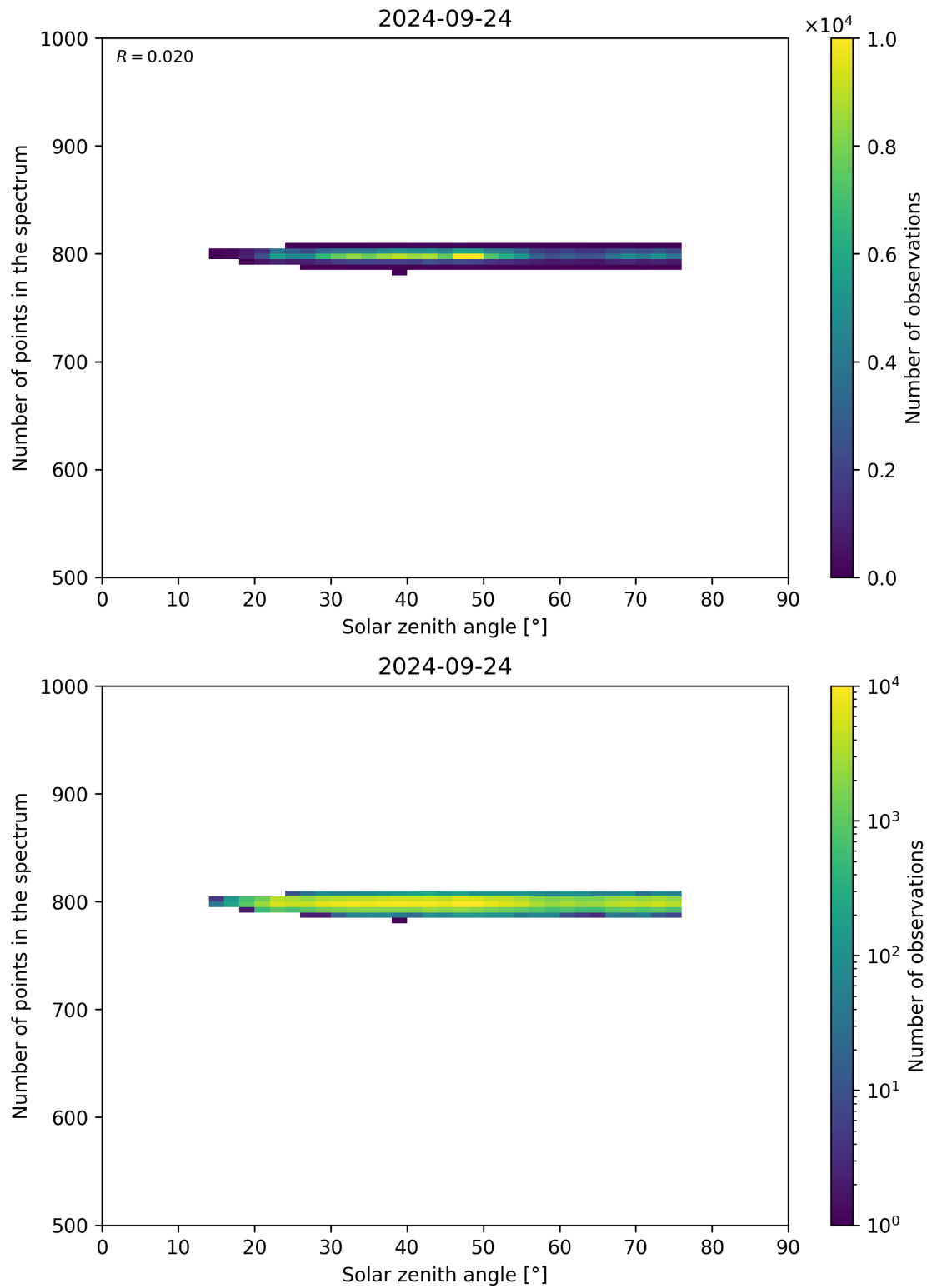
Figure 103: Scatter density plot of “Solar zenith angle” against “Number of points in the spectrum” for 2024-09-23 to 2024-09-25.
