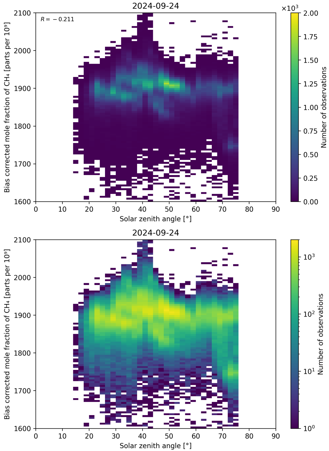
Figure 100: Scatter density plot of “Solar zenith angle” against “Bias corrected mole fraction of CH 4 ” for 2024-09-23 to 2024-09-25.
