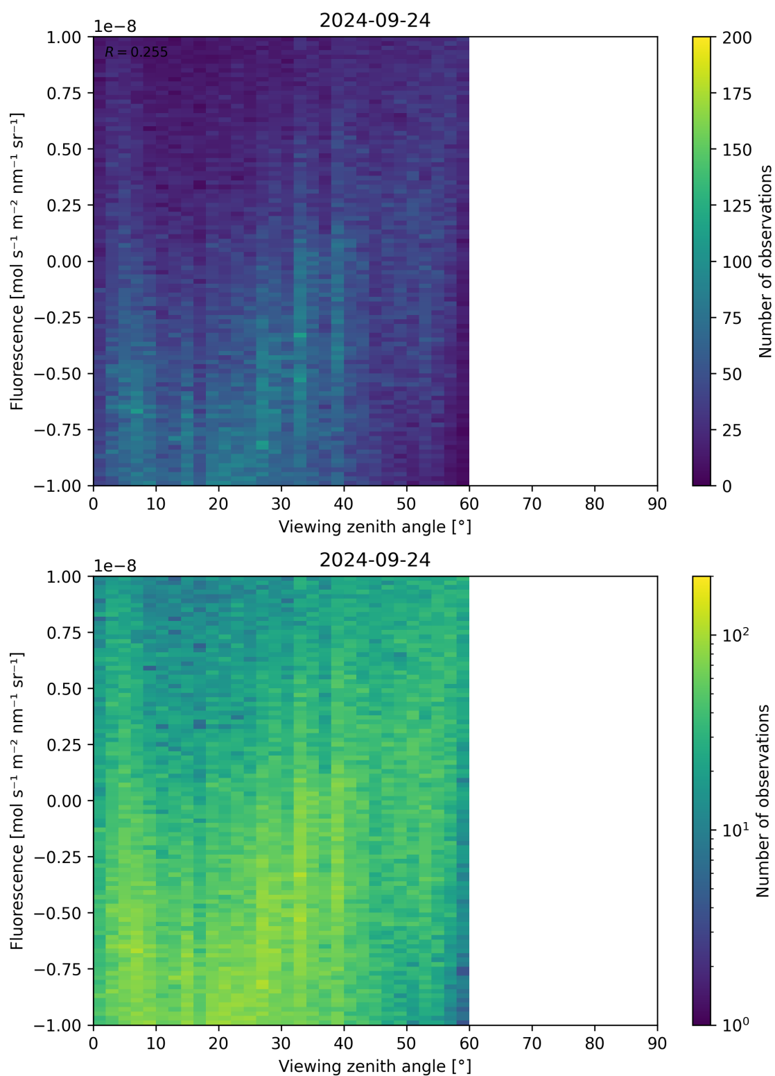
Figure 108: Scatter density plot of “Viewing zenith angle” against “Fluorescence” for 2024-09-23 to 2024-09-25.
