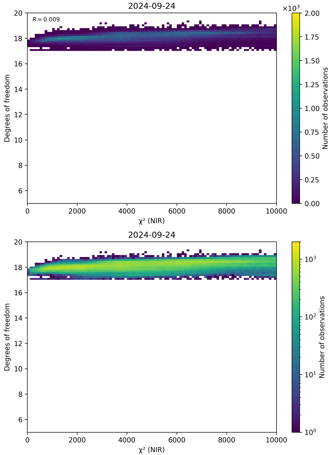
Figure 44: Scatter density plot of “ \chi^2 (NIR)” against “Degrees of freedom” for 2024-09-23 to 2024-09-25.
