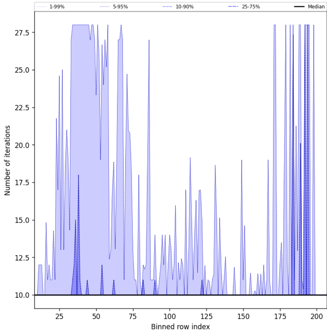
Figure 42: Along track statistics of “Number of iterations” for 2024-09-23 to 2024-09-25
