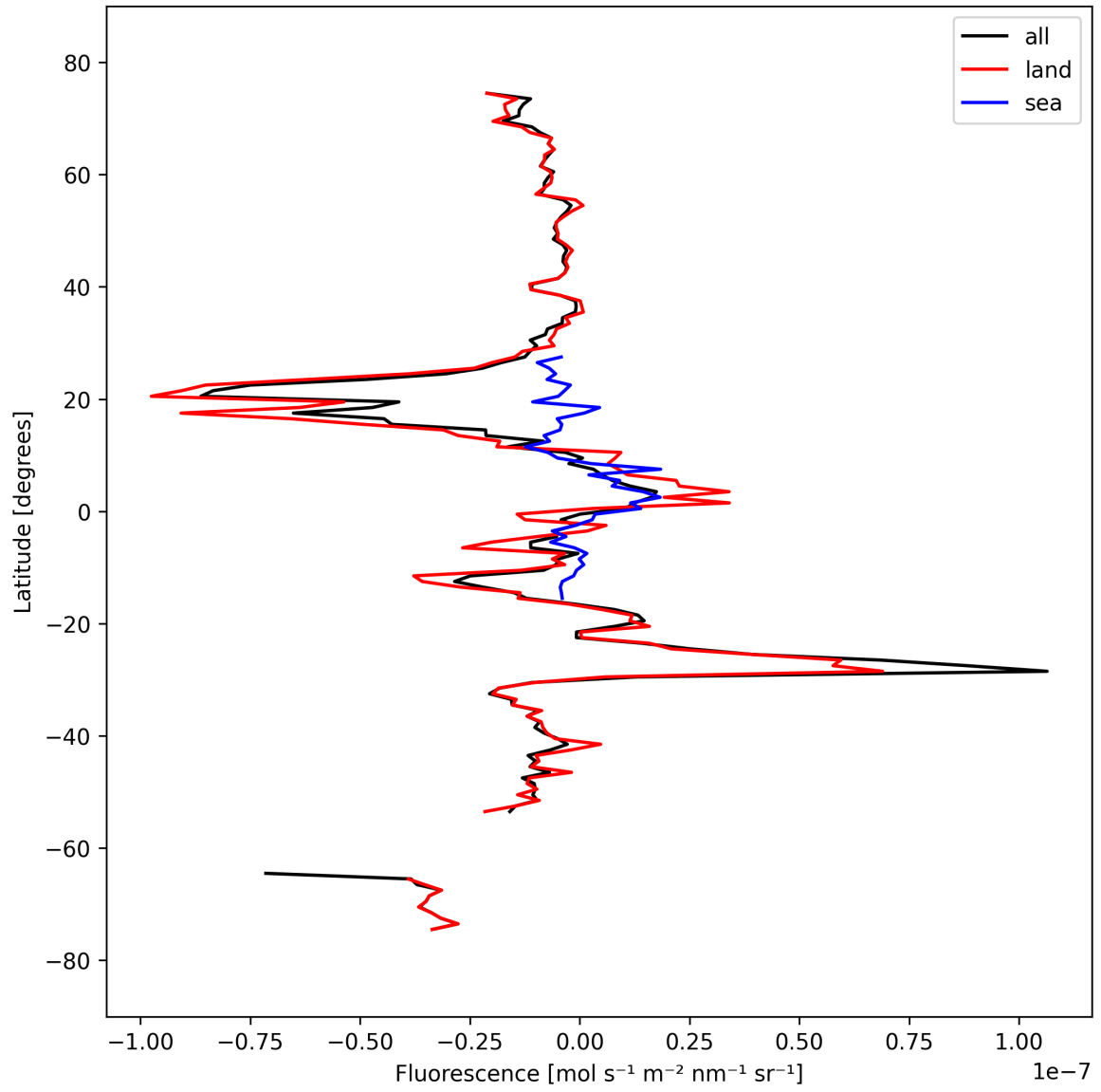
Figure 21: Zonal average of “Fluorescence” for 2024-09-23 to 2024-09-25.
