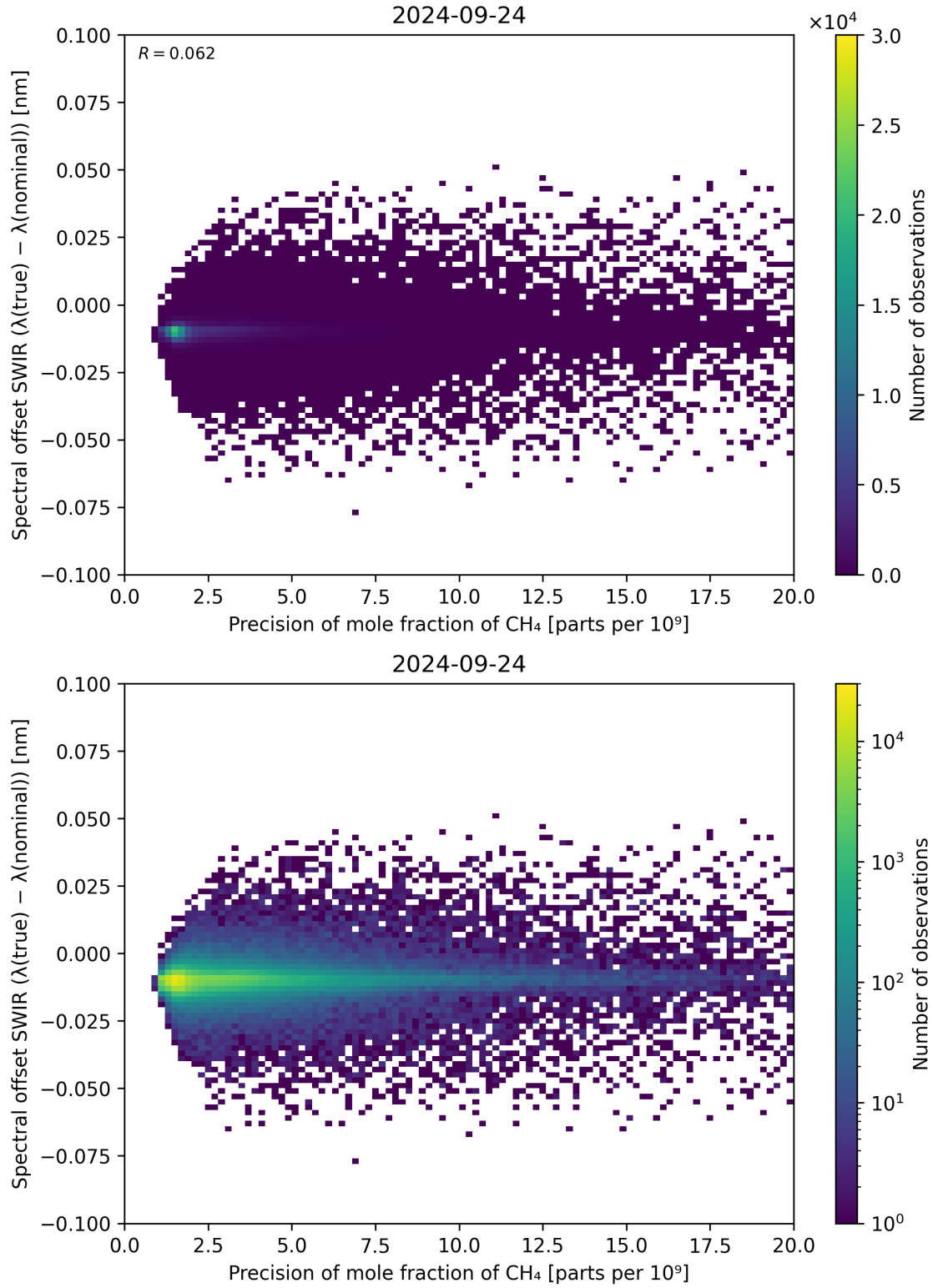
Figure 85: Scatter density plot of “Precision of mole fraction of CH 4 ” against “Spectral offset SWIR ( \lambda_{\text{true}} - \lambda_{\text{nominal}} )” for 2024-09-23 to 2024-09-25.
