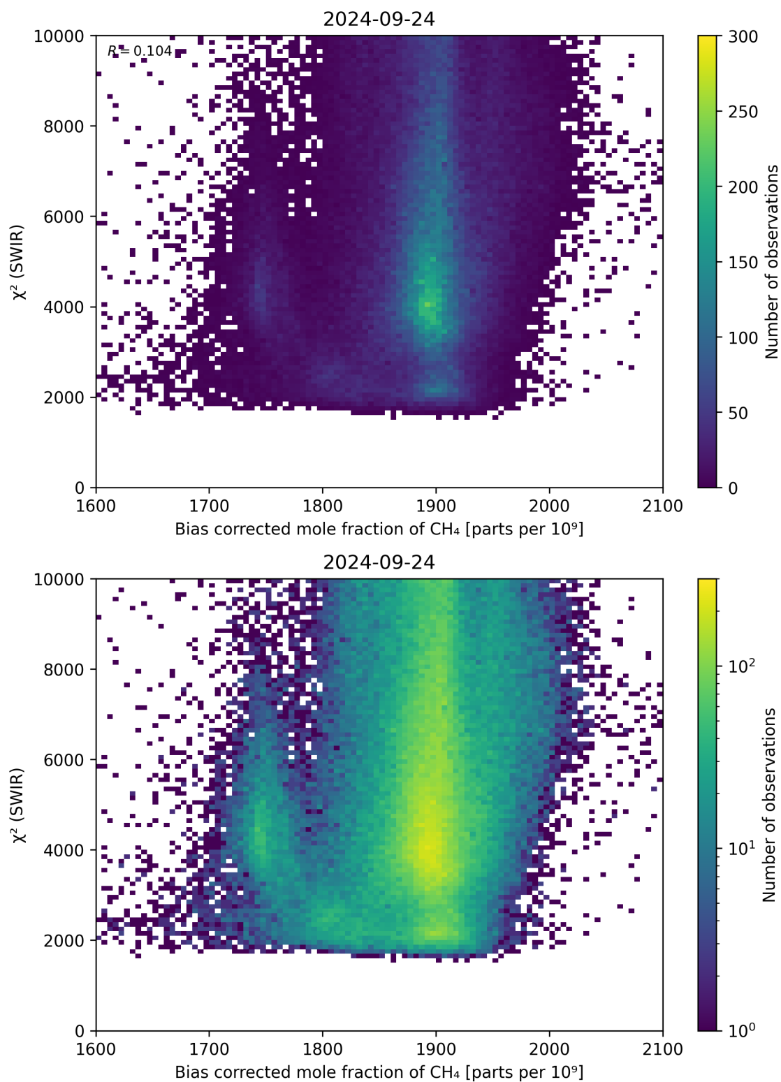
Figure 64: Scatter density plot of “Bias corrected mole fraction of \text{CH}_4 ” against “ \chi^2 (SWIR)” for 2024-09-23 to 2024-09-25.
