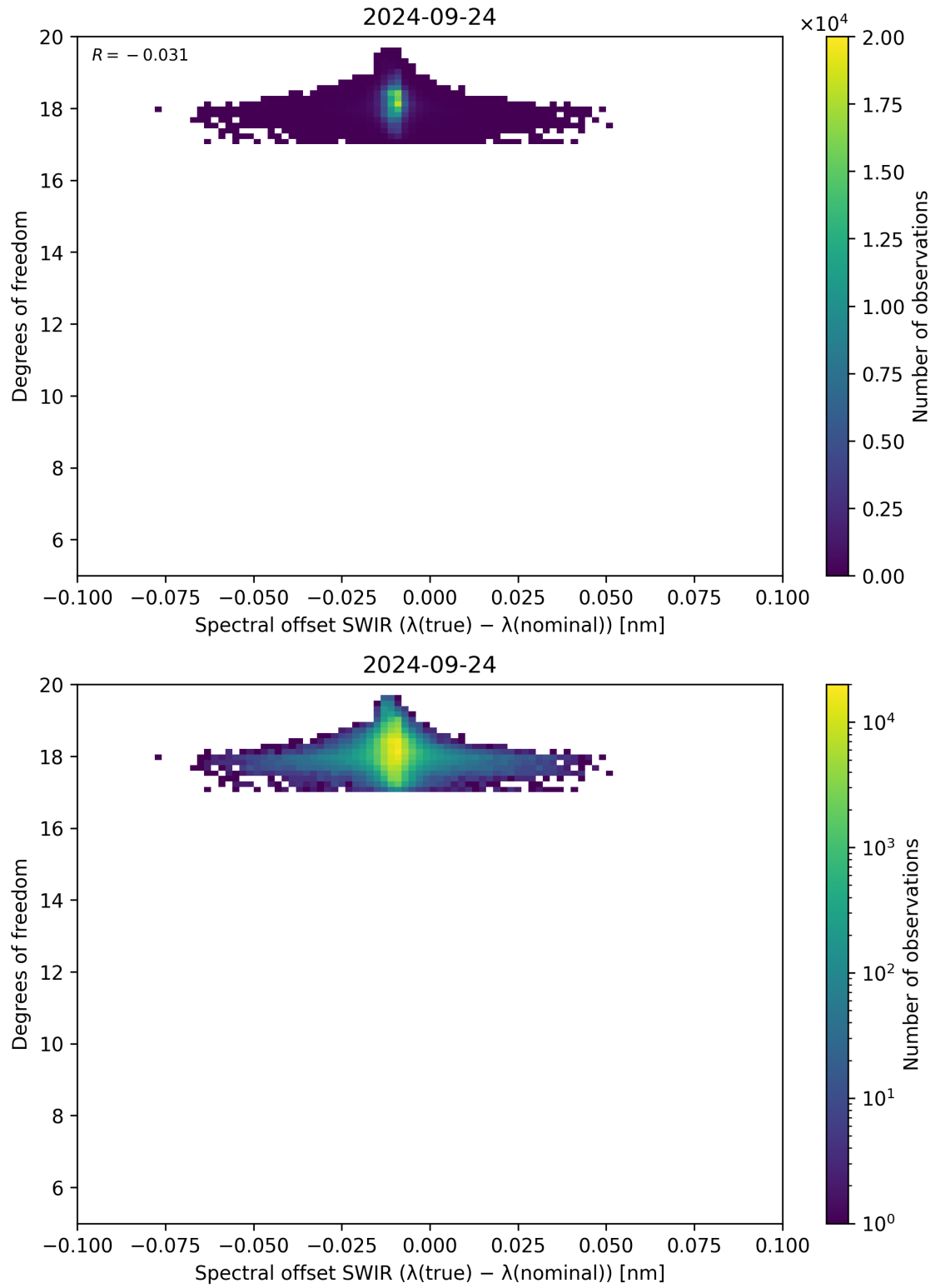
Figure 119: Scatter density plot of “Spectral offset SWIR ( \lambda_{\text{true}} - \lambda_{\text{nominal}} )” against “Degrees of freedom” for 2024-09-23 to 2024-09-25.
