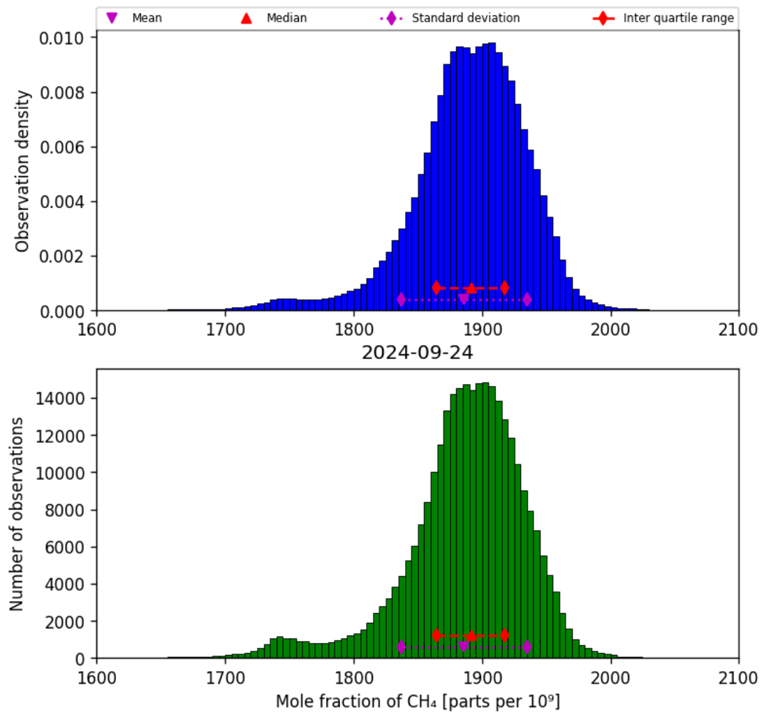
Figure 23: Histogram of “Mole fraction of CH 4 ” for 2024-09-23 to 2024-09-25
