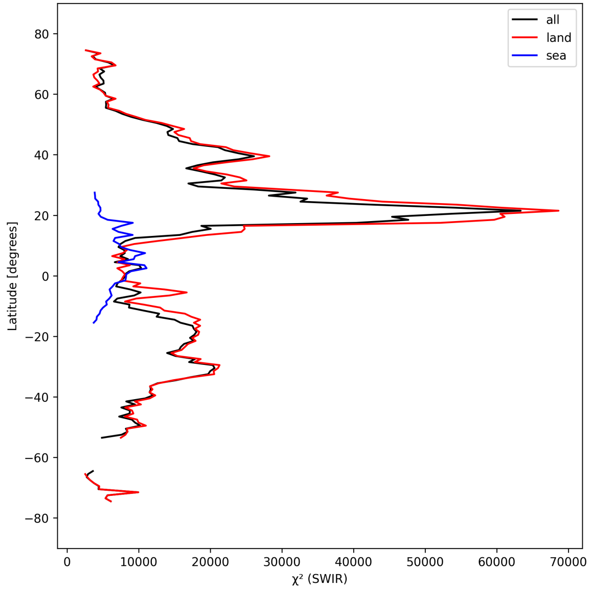
Figure 17: Zonal average of “ \chi^2 (SWIR)” for 2024-09-23 to 2024-09-25.
