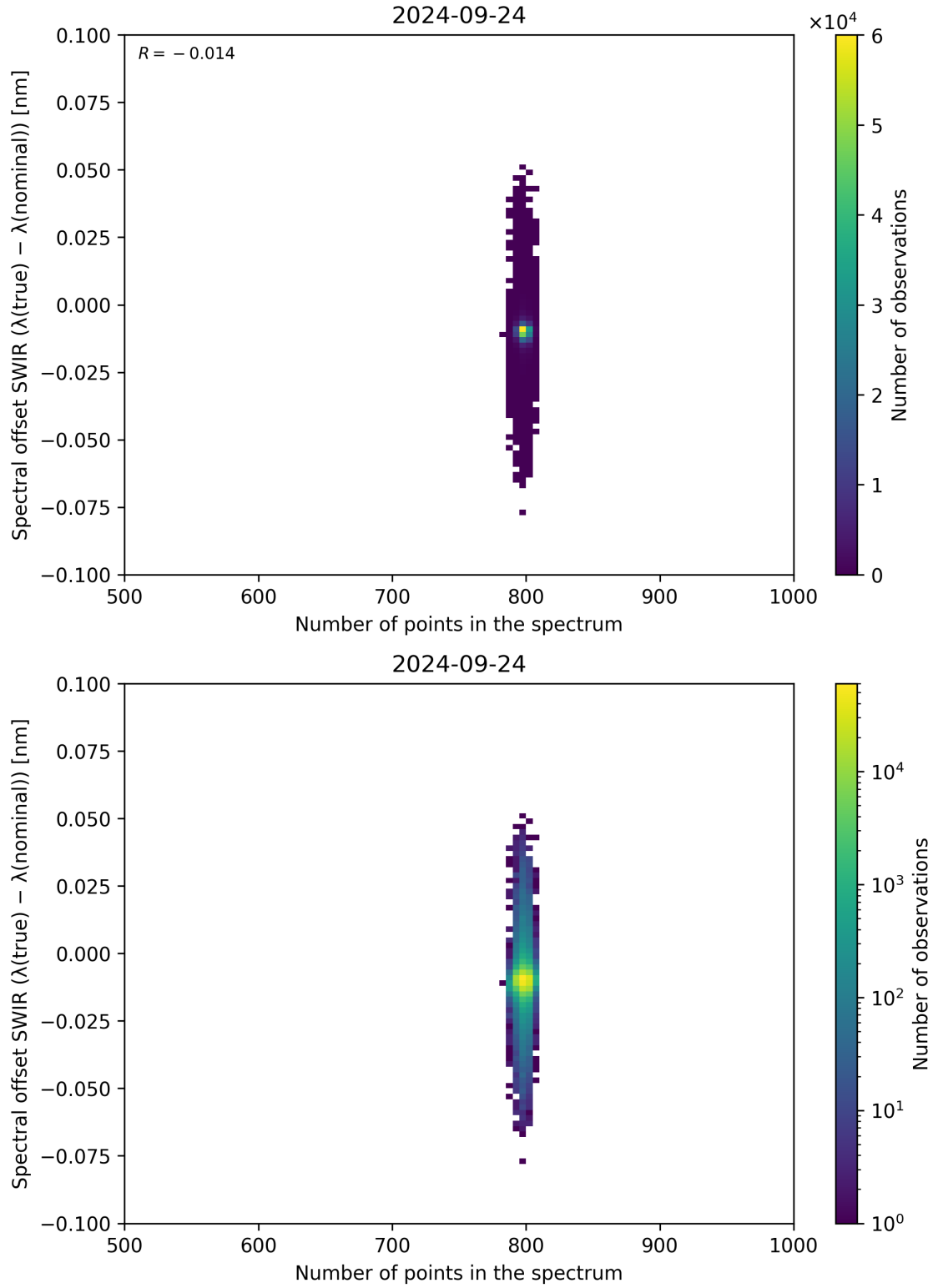
Figure 93: Scatter density plot of “Number of points in the spectrum” against “Spectral offset SWIR ( \lambda_{\text{true}} - \lambda_{\text{nominal}} )” for 2024-09-23 to 2024-09-25.
