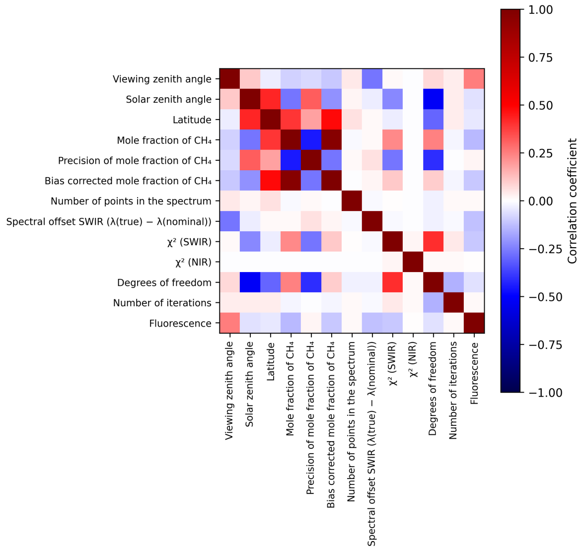
Figure 2: Map of correlation matrix for 2024-09-23 to 2024-09-25.
