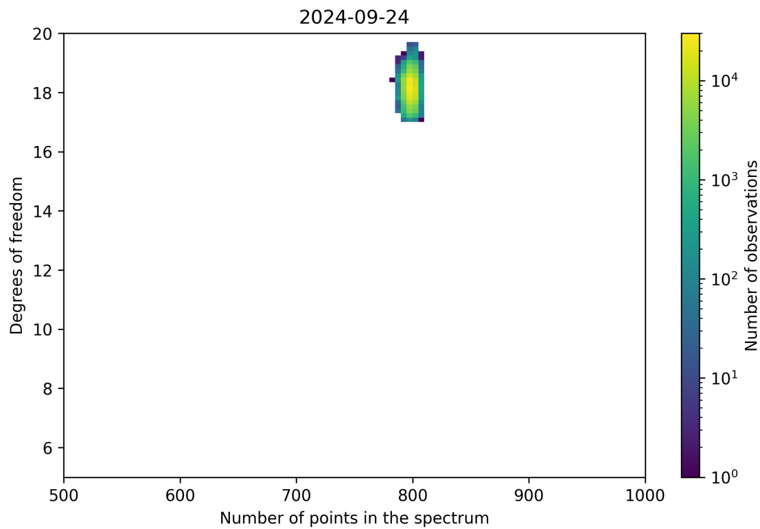
Figure 90: Scatter density plot of “Number of points in the spectrum” against “Degrees of freedom” for 2024-09-23 to 2024-09-25.
