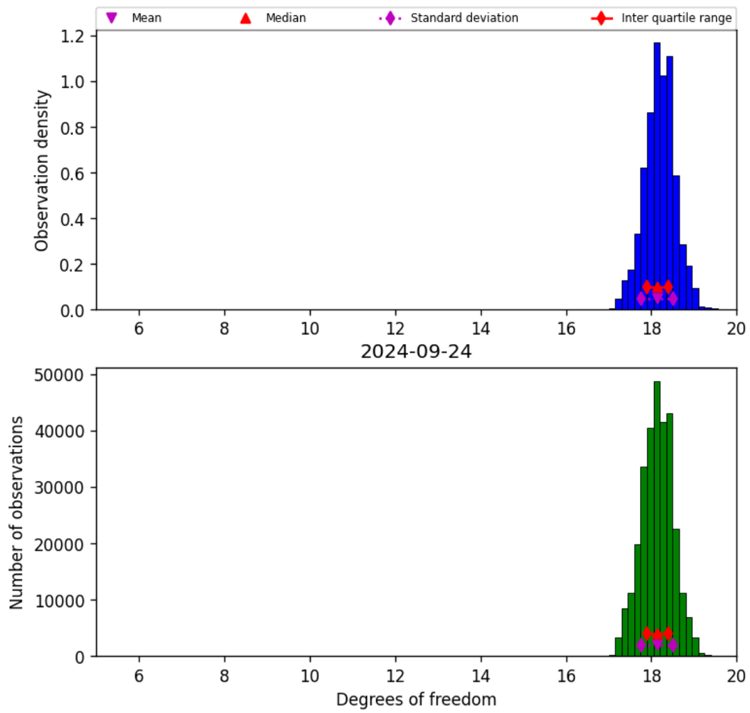
Figure 30: Histogram of “Degrees of freedom” for 2024-09-23 to 2024-09-25
