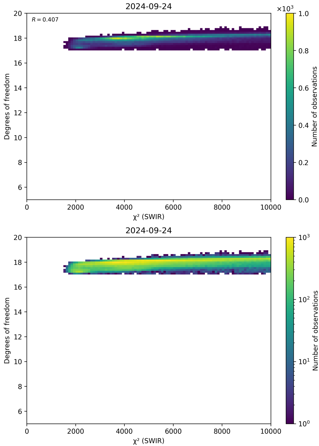
Figure 48: Scatter density plot of “ \chi^2 (SWIR)” against “Degrees of freedom” for 2024-09-23 to 2024-09-25.
