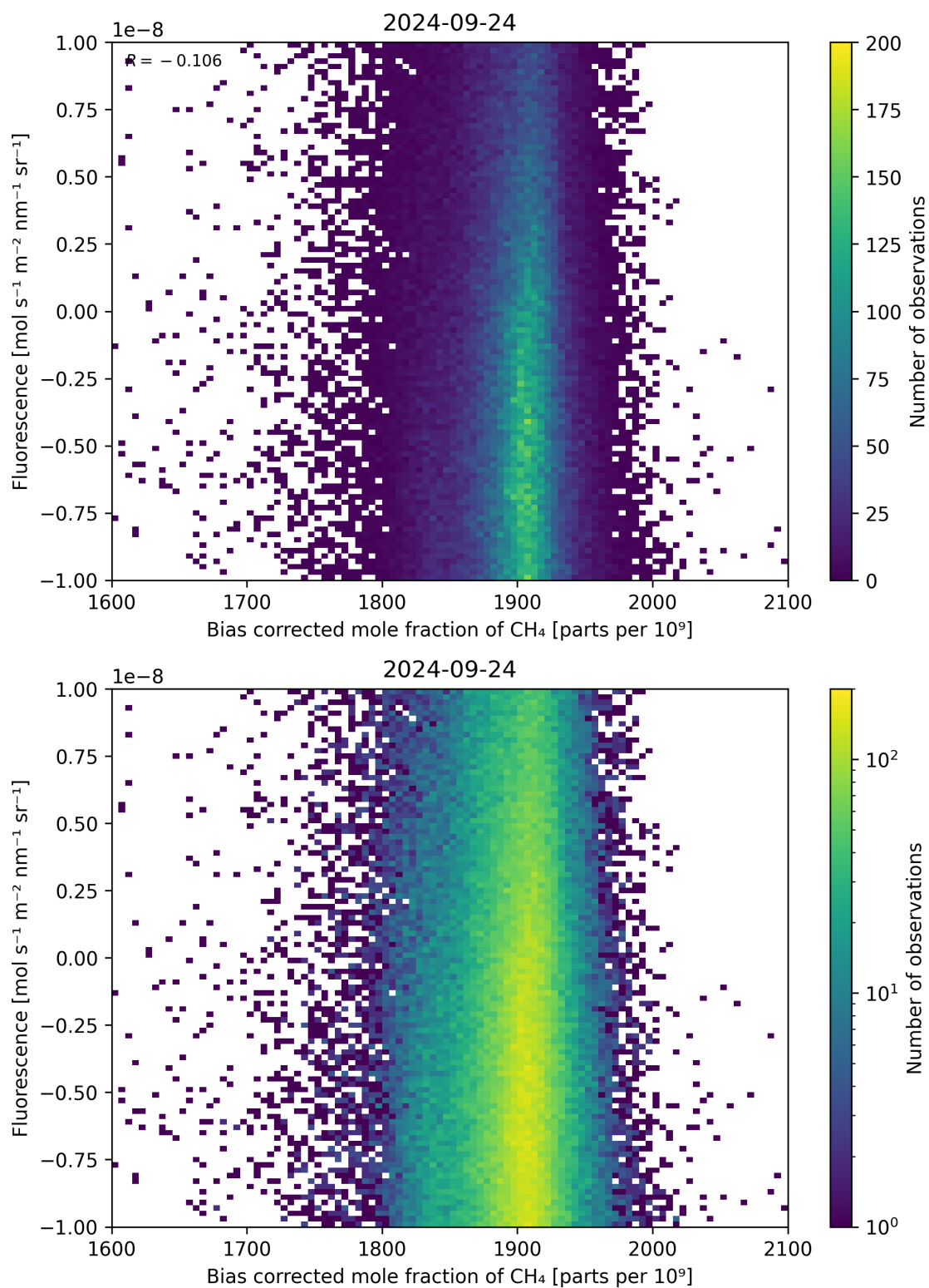
Figure 66: Scatter density plot of “Bias corrected mole fraction of \text{CH}_4 ” against “Fluorescence” for 2024-09-23 to 2024-09-25.
