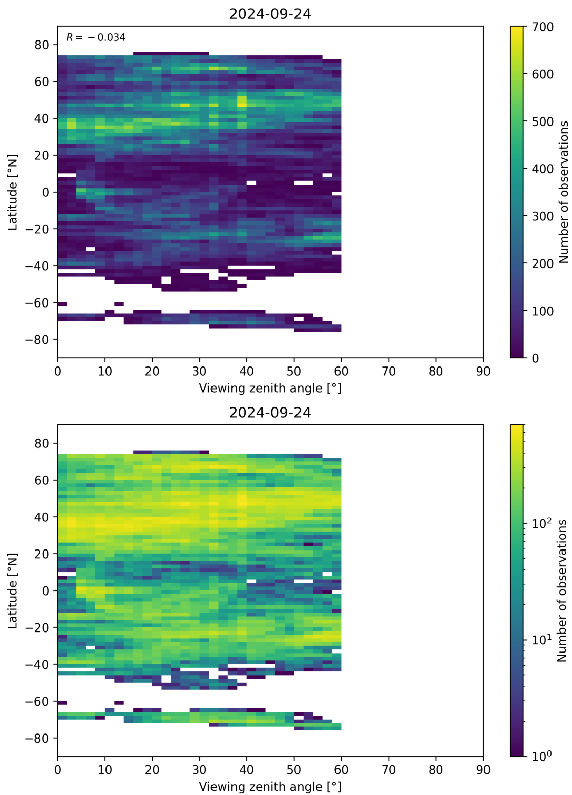
Figure 109: Scatter density plot of “Viewing zenith angle” against “Latitude” for 2024-09-23 to 2024-09-25.
