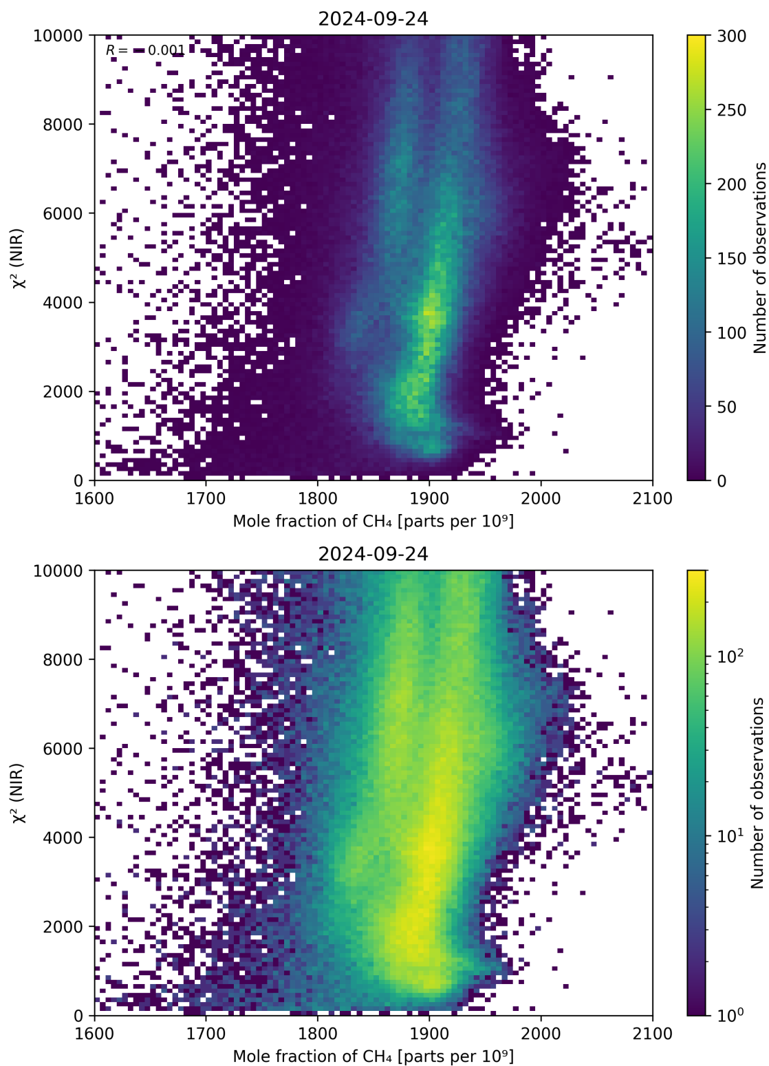
Figure 70: Scatter density plot of “Mole fraction of CH 4 ” against “ \chi^2 (NIR)” for 2024-09-23 to 2024-09-25.
