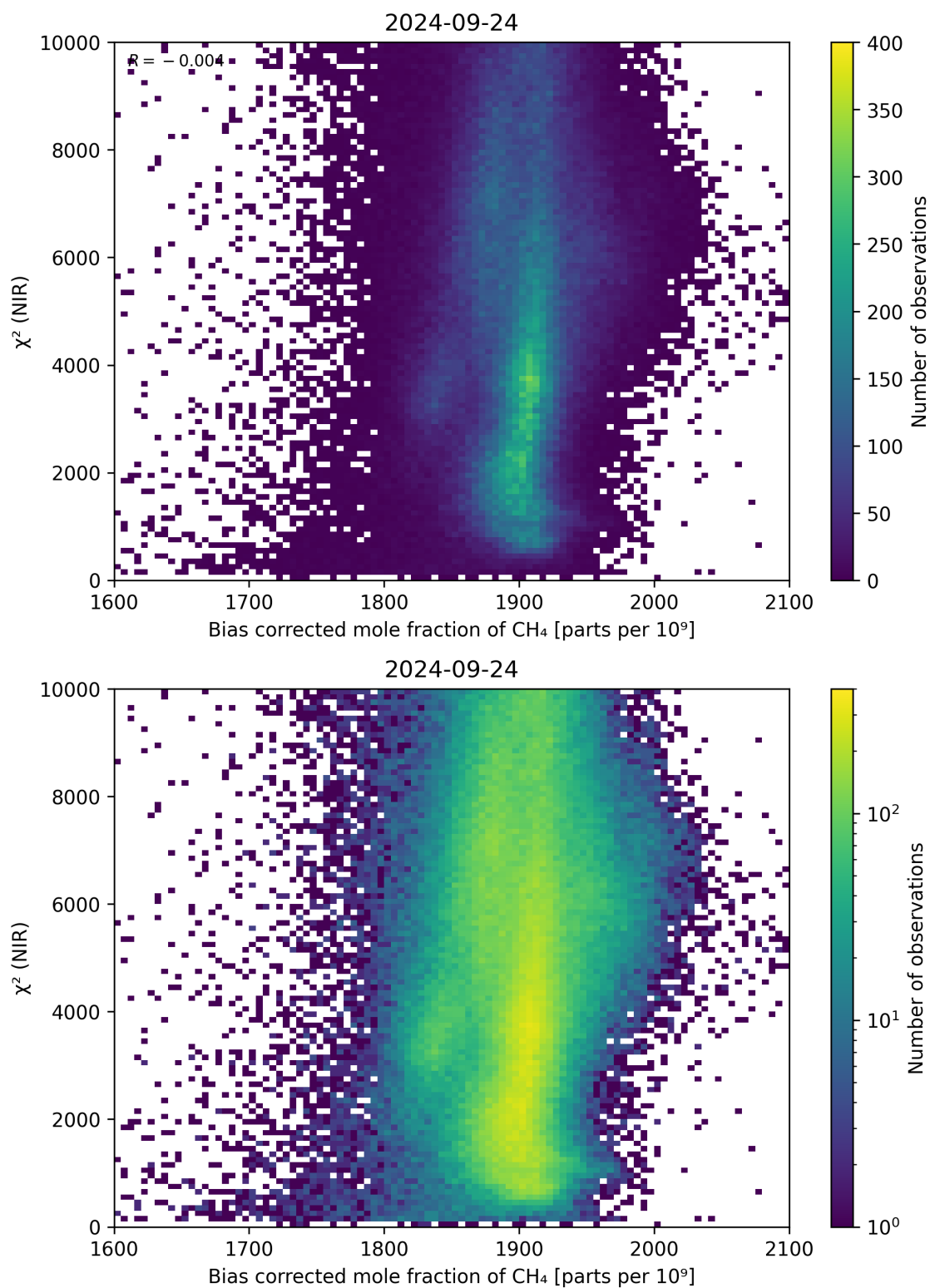
Figure 63: Scatter density plot of “Bias corrected mole fraction of CH 4 ” against “ \chi^2 (NIR)” for 2024-09-23 to 2024-09-25.
