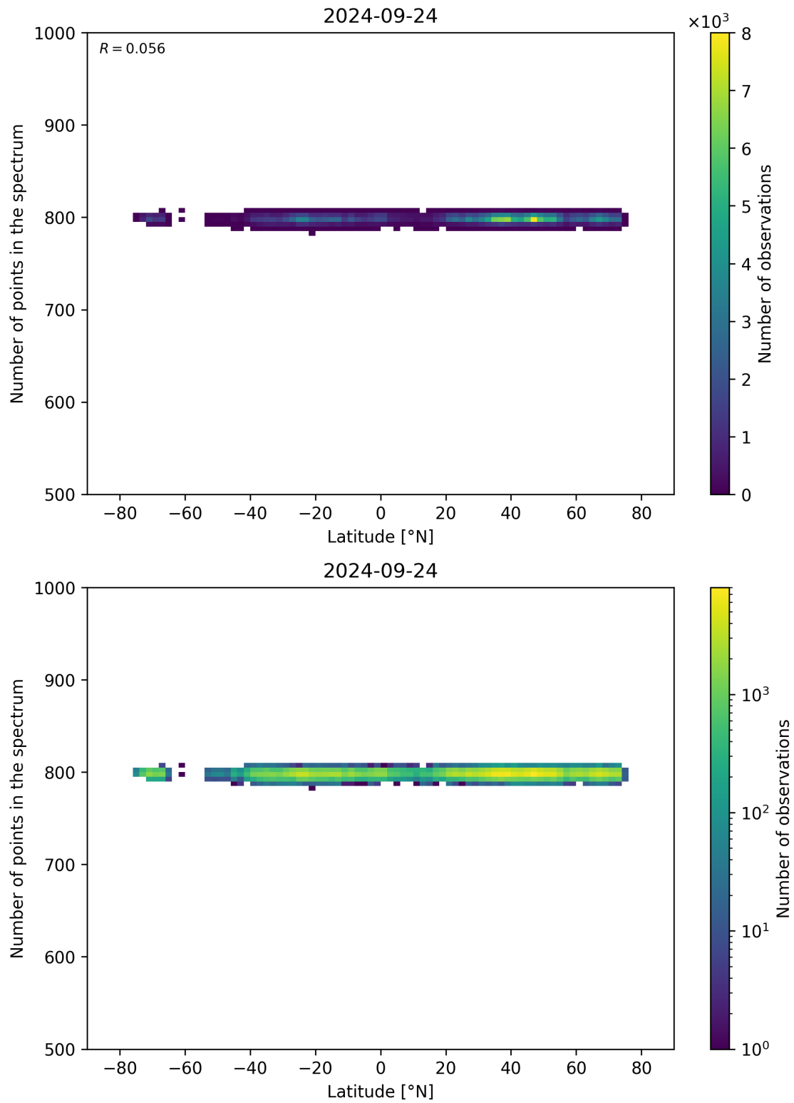
Figure 61: Scatter density plot of “Latitude” against “Number of points in the spectrum” for 2024-09-23 to 2024-09-25.
