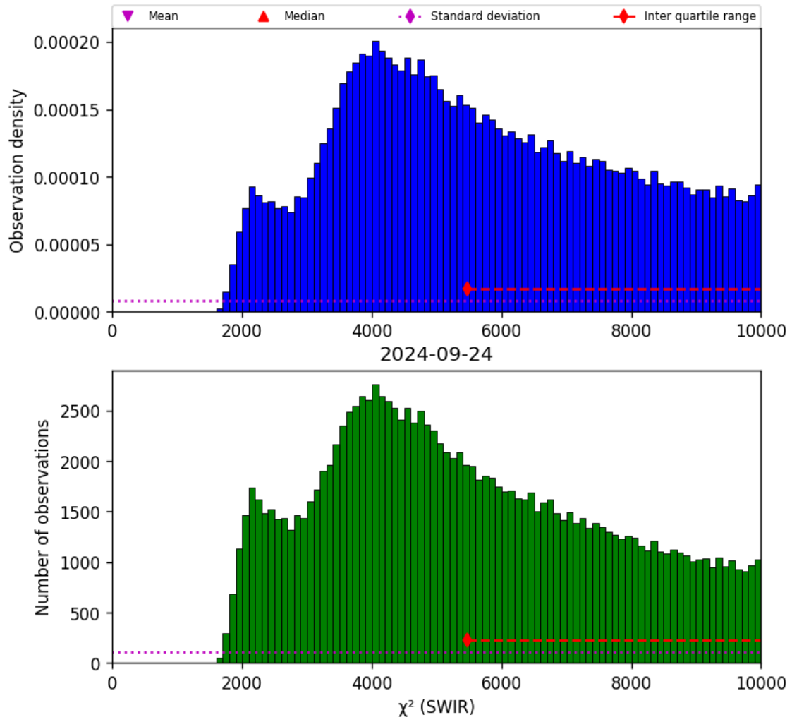
Figure 28: Histogram of “ \chi^2 (SWIR)” for 2024-09-23 to 2024-09-25
