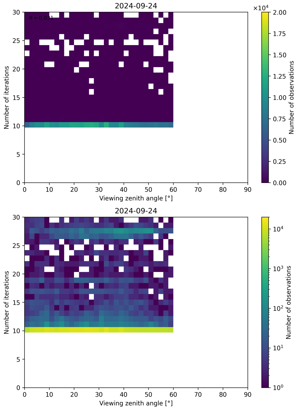
Figure 113: Scatter density plot of “Viewing zenith angle” against “Number of iterations” for 2024-09-23 to 2024-09-25.
