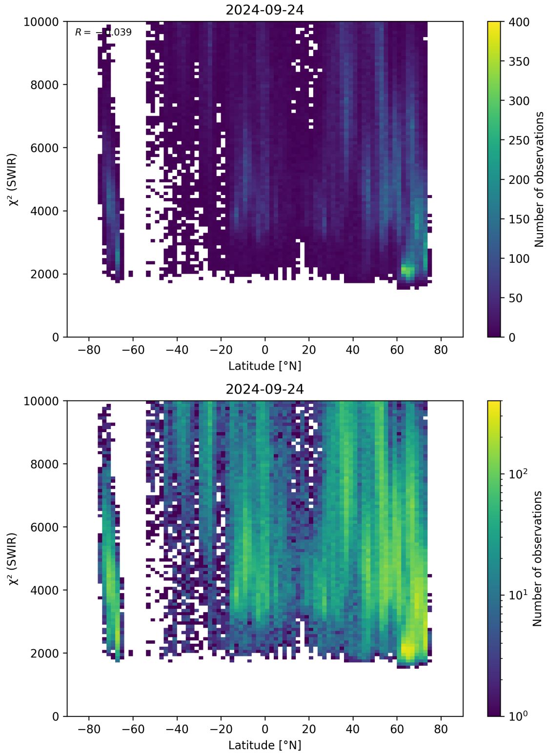
Figure 54: Scatter density plot of “Latitude” against “ \chi^2 (SWIR)” for 2024-09-23 to 2024-09-25.
