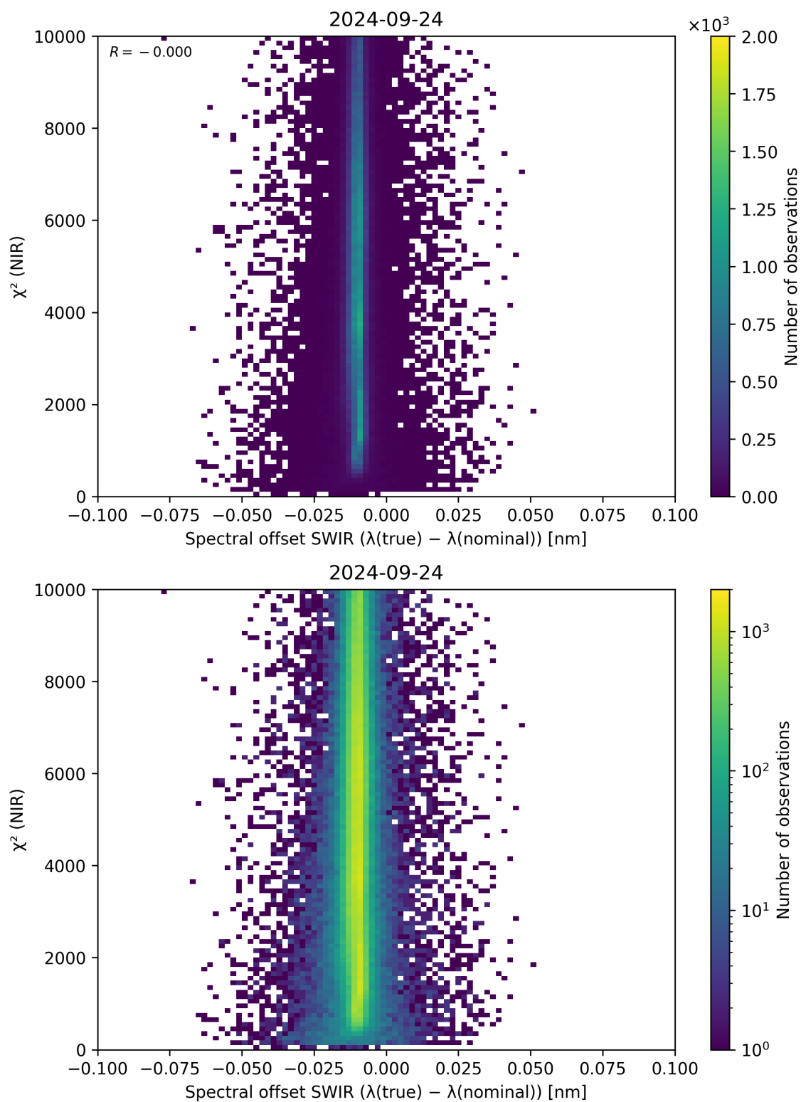
Figure 117: Scatter density plot of “Spectral offset SWIR ( \lambda_{\text{true}} - \lambda_{\text{nominal}} )” against “ \chi^2 (NIR)” for 2024-09-23 to 2024-09-25.
