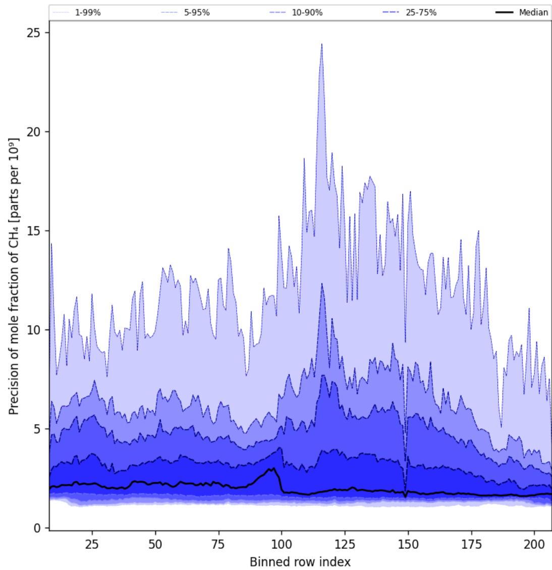
Figure 35: Along track statistics of “Precision of mole fraction of CH 4 ” for 2024-09-23 to 2024-09-25
