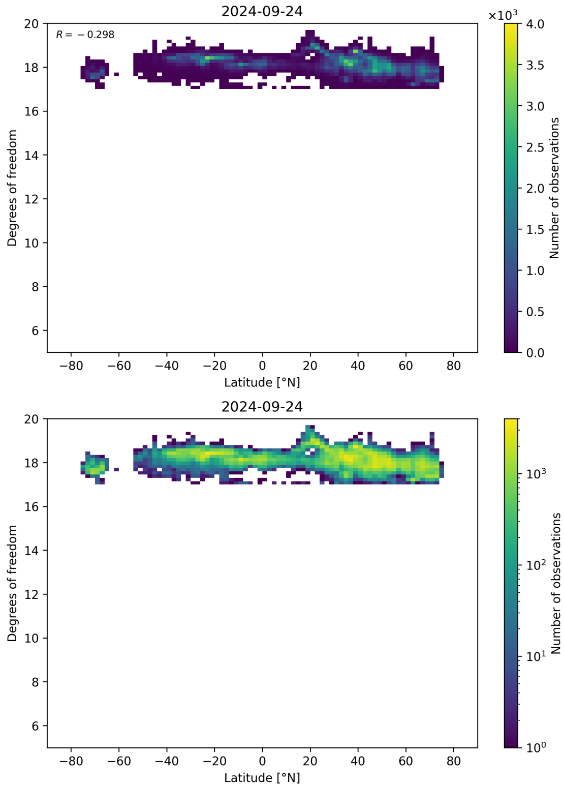
Figure 55: Scatter density plot of “Latitude” against “Degrees of freedom” for 2024-09-23 to 2024-09-25.
