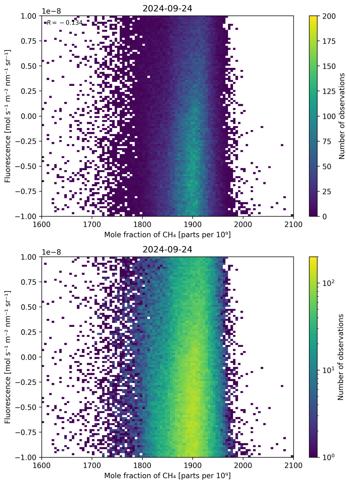
Figure 73: Scatter density plot of “Mole fraction of \text{CH}_4 ” against “Fluorescence” for 2024-09-23 to 2024-09-25.
