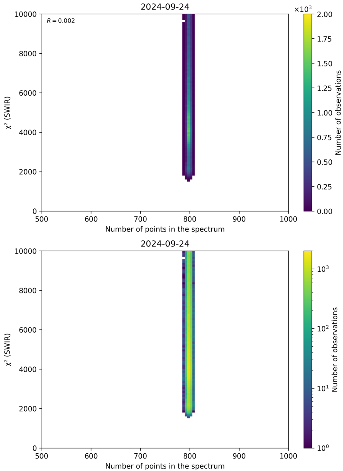
Figure 89: Scatter density plot of “Number of points in the spectrum” against “ \chi^2 (SWIR)” for 2024-09-23 to 2024-09-25.
