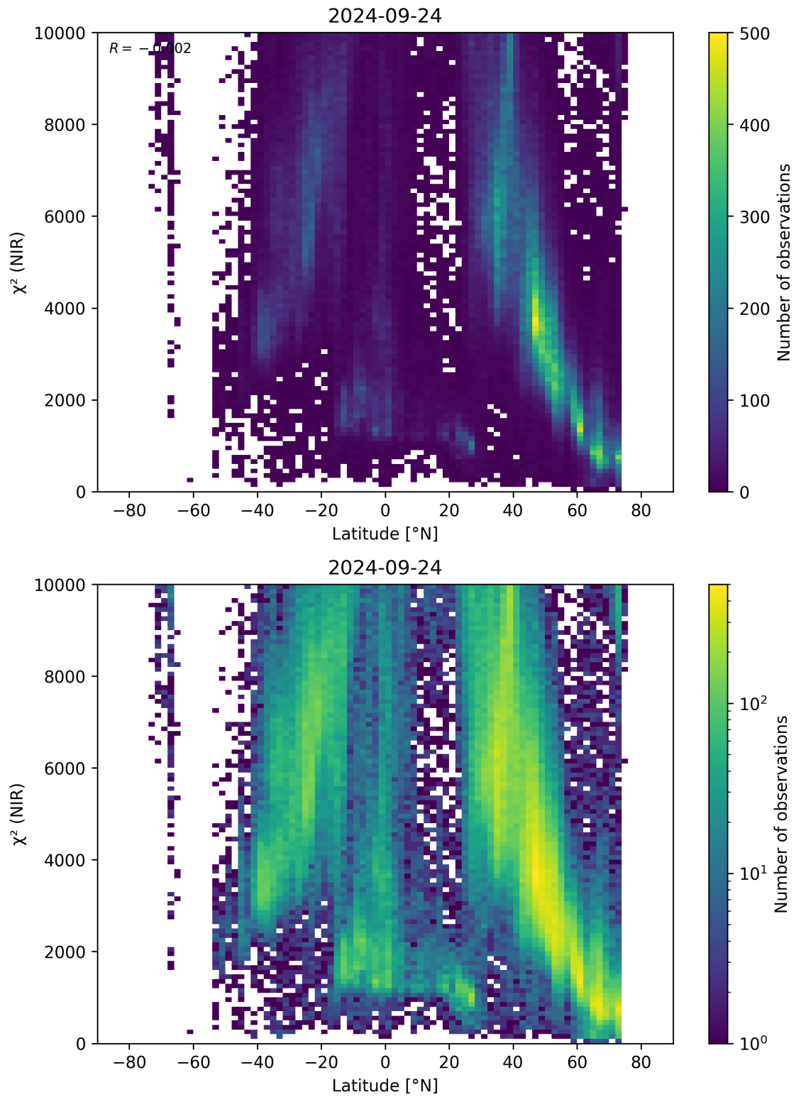
Figure 53: Scatter density plot of “Latitude” against “ \chi^2 (NIR)” for 2024-09-23 to 2024-09-25.
