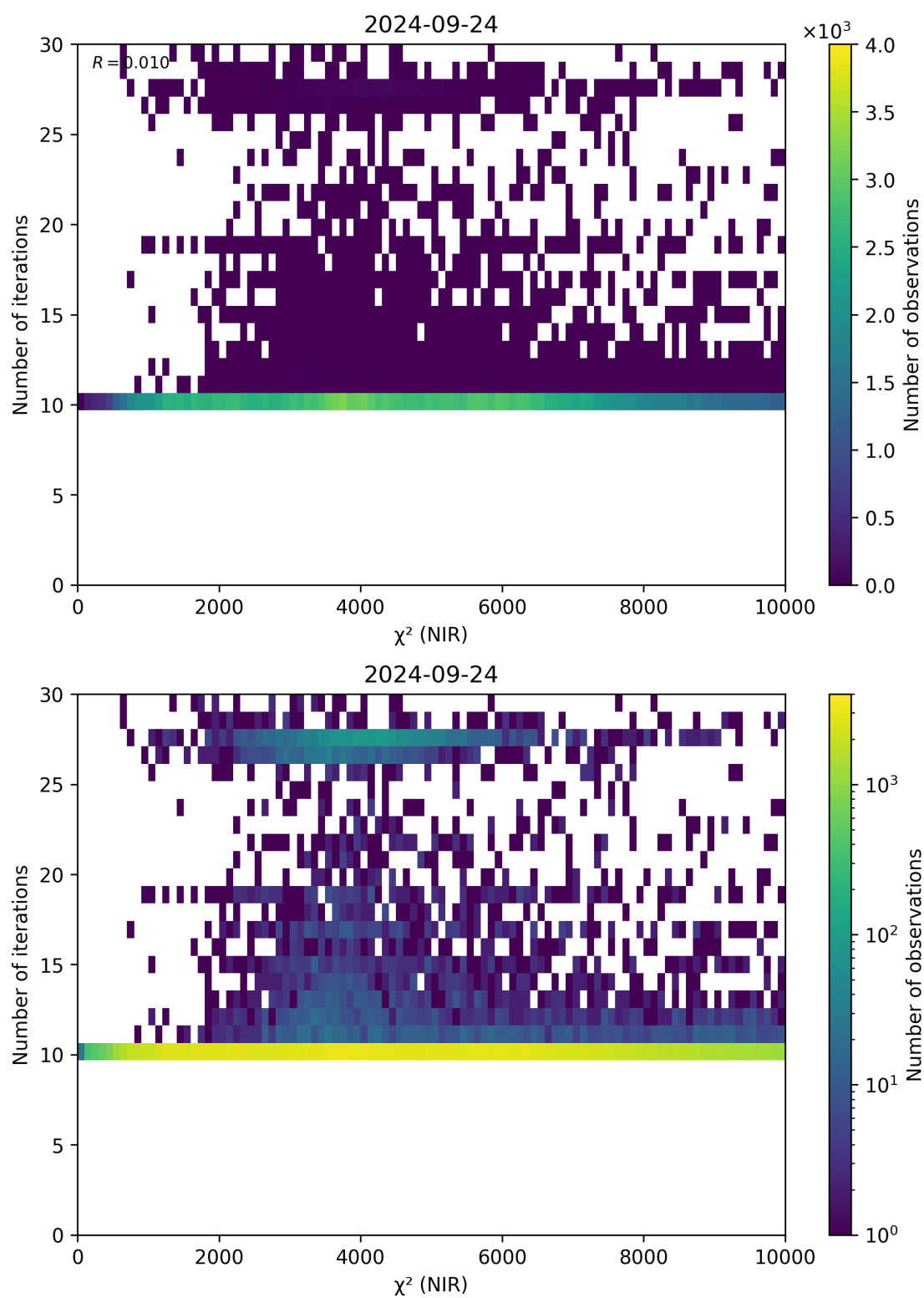
Figure 46: Scatter density plot of “ \chi^2 (NIR)” against “Number of iterations” for 2024-09-23 to 2024-09-25.
