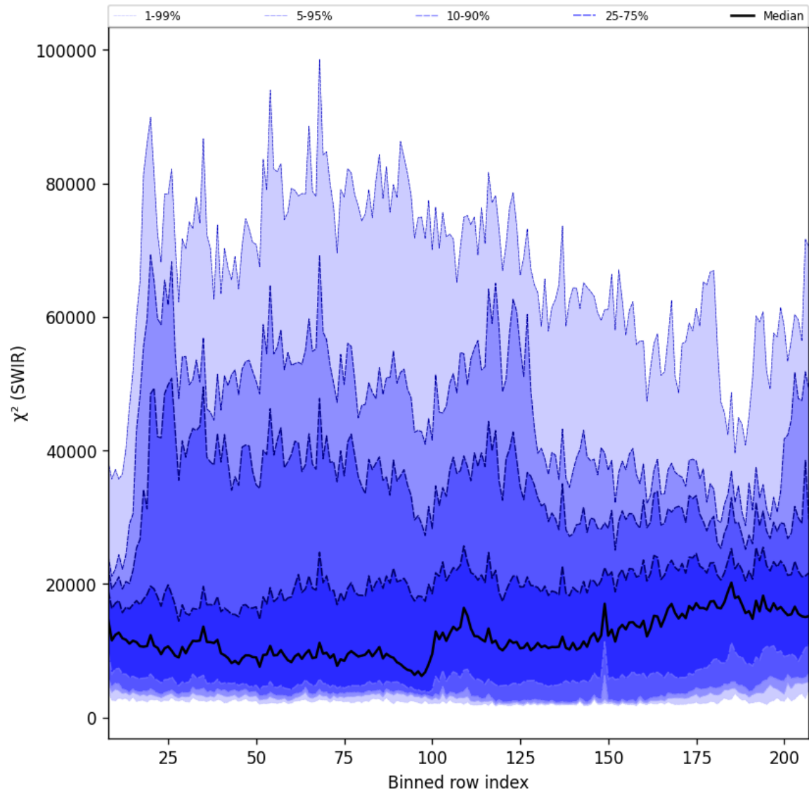
Figure 39: Along track statistics of “ \chi^2 (SWIR)” for 2024-09-23 to 2024-09-25
