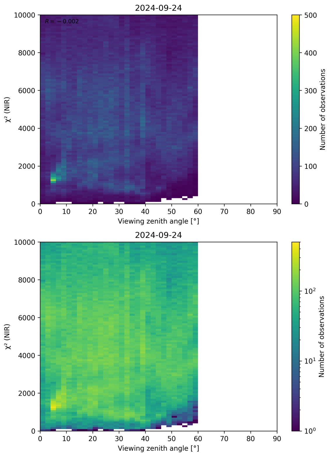
Figure 105: Scatter density plot of “Viewing zenith angle” against “ \chi^2 (NIR)” for 2024-09-23 to 2024-09-25.
