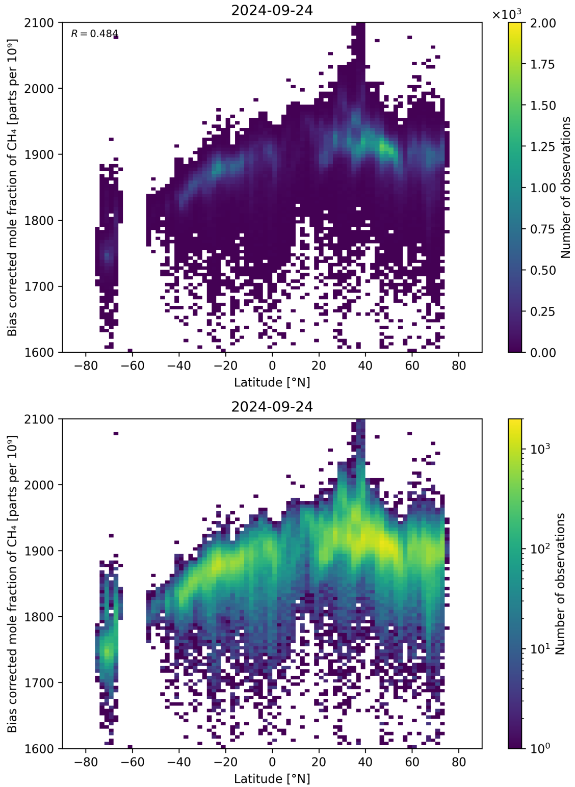
Figure 58: Scatter density plot of “Latitude” against “Bias corrected mole fraction of CH 4 ” for 2024-09-23 to 2024-09-25.
