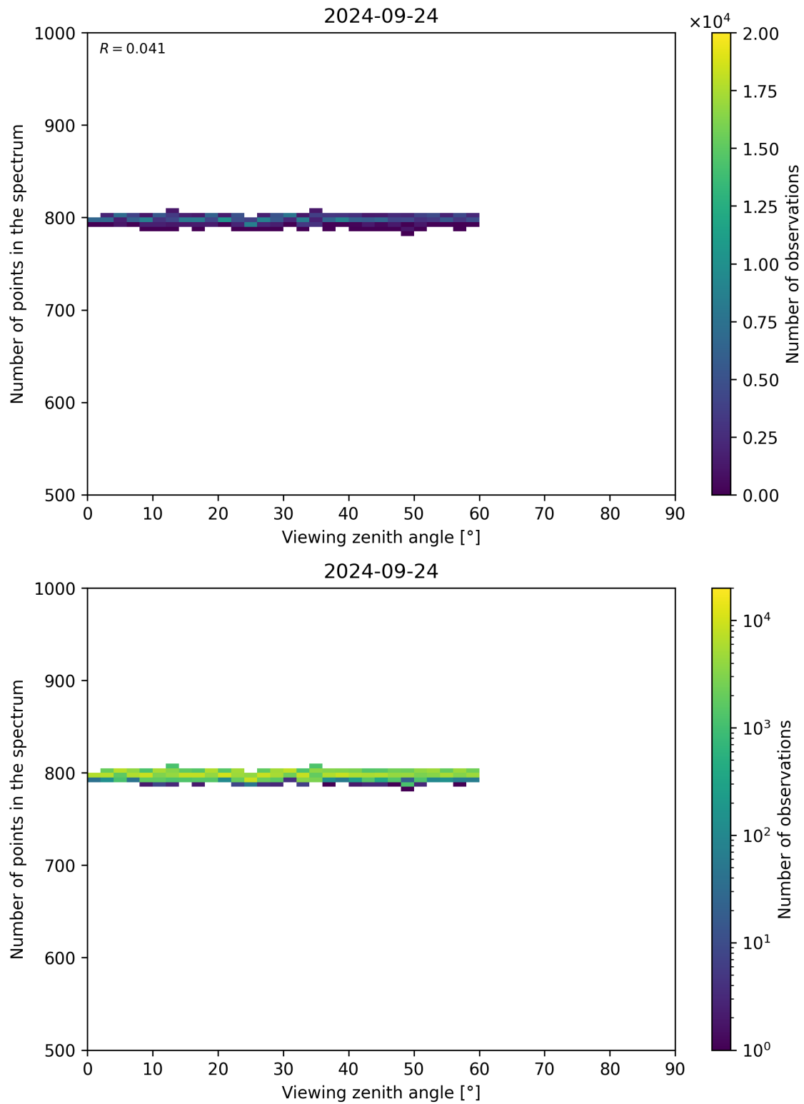
Figure 114: Scatter density plot of “Viewing zenith angle” against “Number of points in the spectrum” for 2024-09-23 to 2024-09-25.
