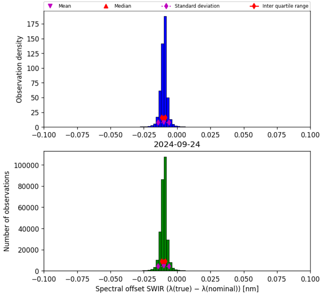
Figure 27: Histogram of “Spectral offset SWIR ( \lambda_{\text{true}} - \lambda_{\text{nominal}} )” for 2024-09-23 to 2024-09-25
