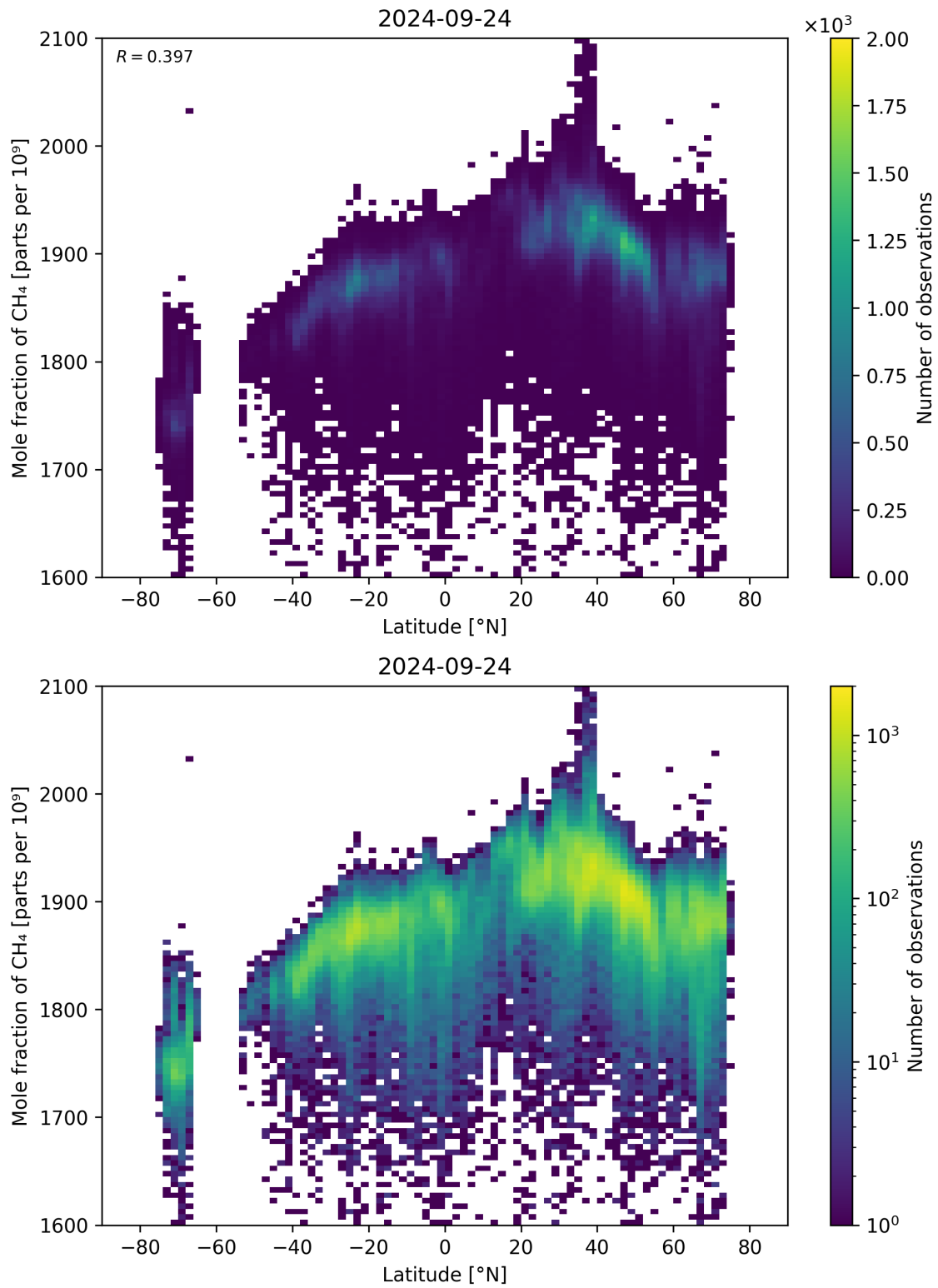
Figure 57: Scatter density plot of “Latitude” against “Mole fraction of CH 4 ” for 2024-09-23 to 2024-09-25.
