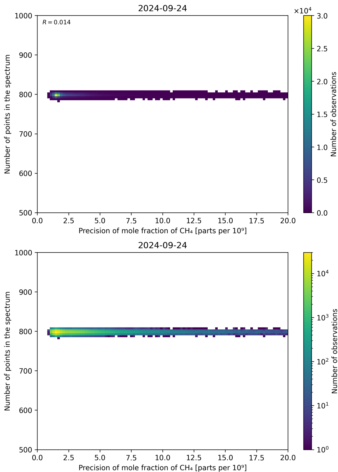
Figure 84: Scatter density plot of “Precision of mole fraction of CH 4 ” against “Number of points in the spectrum” for 2024-09-23 to 2024-09-25.
