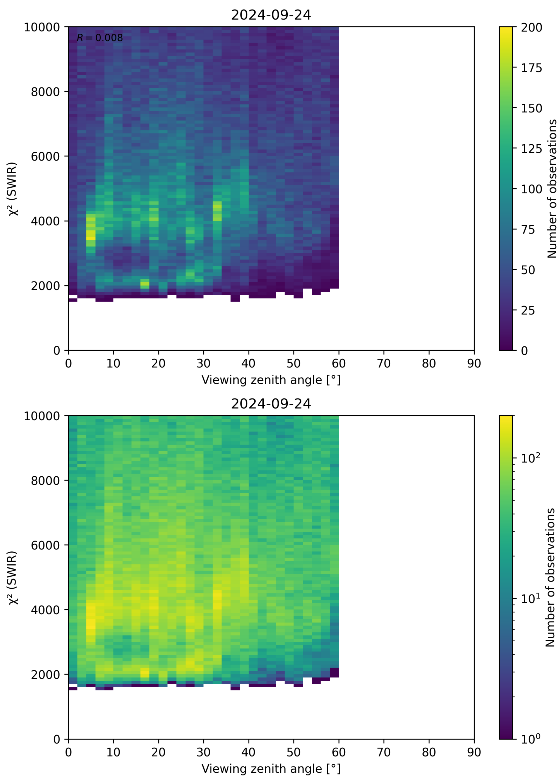
Figure 106: Scatter density plot of “Viewing zenith angle” against “ \chi^2 (SWIR)” for 2024-09-23 to 2024-09-25.
