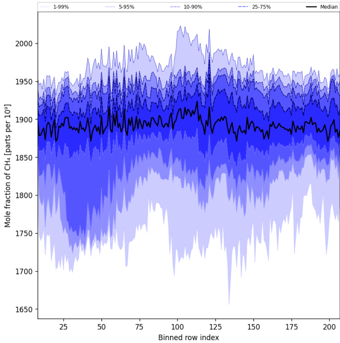
Figure 34: Along track statistics of “Mole fraction of CH 4 ” for 2024-09-23 to 2024-09-25
