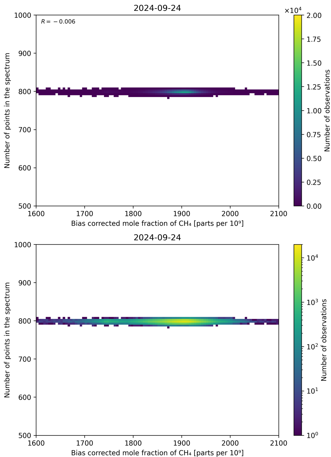
Figure 68: Scatter density plot of “Bias corrected mole fraction of CH 4 ” against “Number of points in the spectrum” for 2024-09-23 to 2024-09-25.
