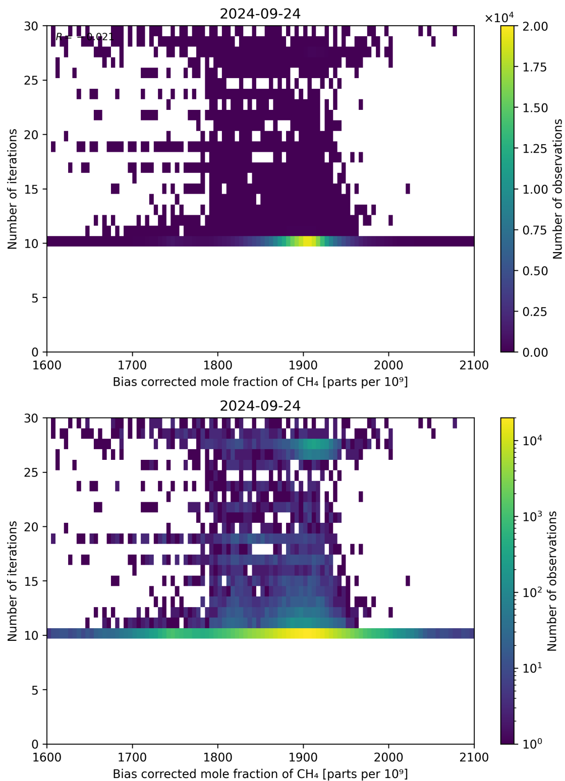
Figure 67: Scatter density plot of “Bias corrected mole fraction of CH 4 ” against “Number of iterations” for 2024-09-23 to 2024-09-25.
