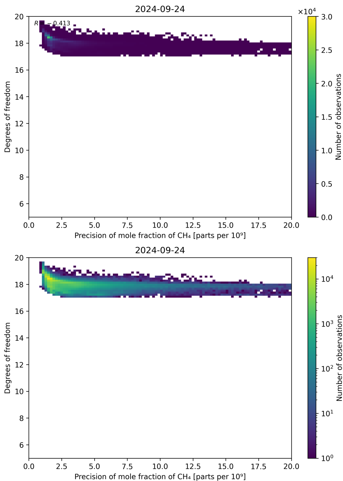
Figure 80: Scatter density plot of “Precision of mole fraction of CH 4 ” against “Degrees of freedom” for 2024-09-23 to 2024-09-25.
