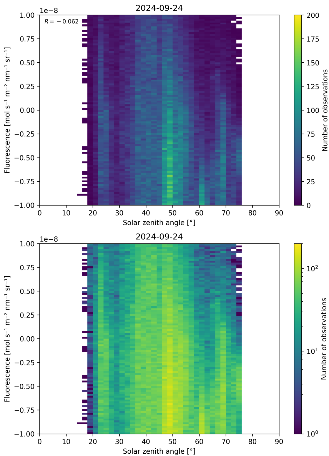
Figure 97: Scatter density plot of “Solar zenith angle” against “Fluorescence” for 2024-09-23 to 2024-09-25.
