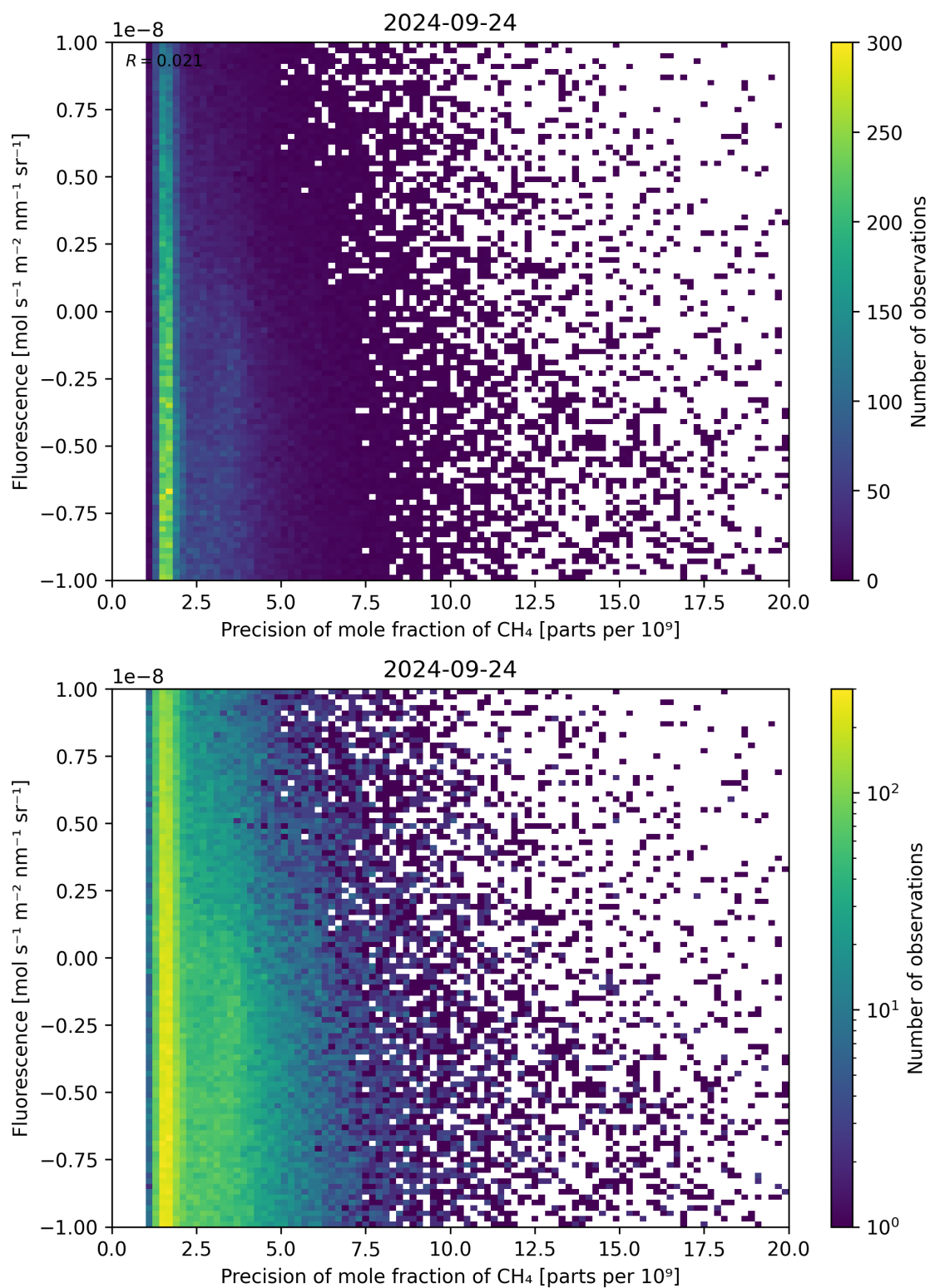
Figure 81: Scatter density plot of “Precision of mole fraction of \text{CH}_4 ” against “Fluorescence” for 2024-09-23 to 2024-09-25.
