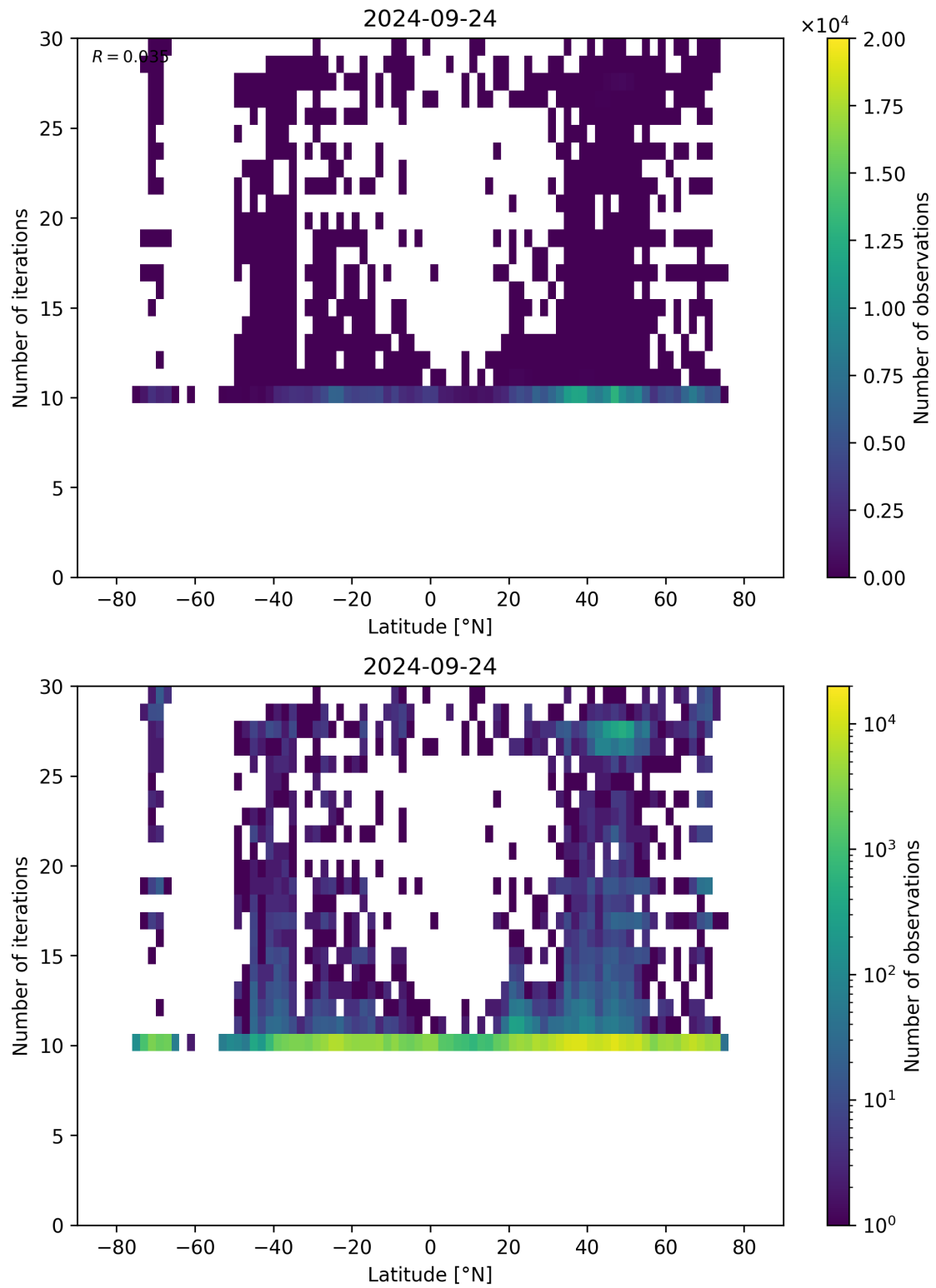
Figure 60: Scatter density plot of “Latitude” against “Number of iterations” for 2024-09-23 to 2024-09-25.
