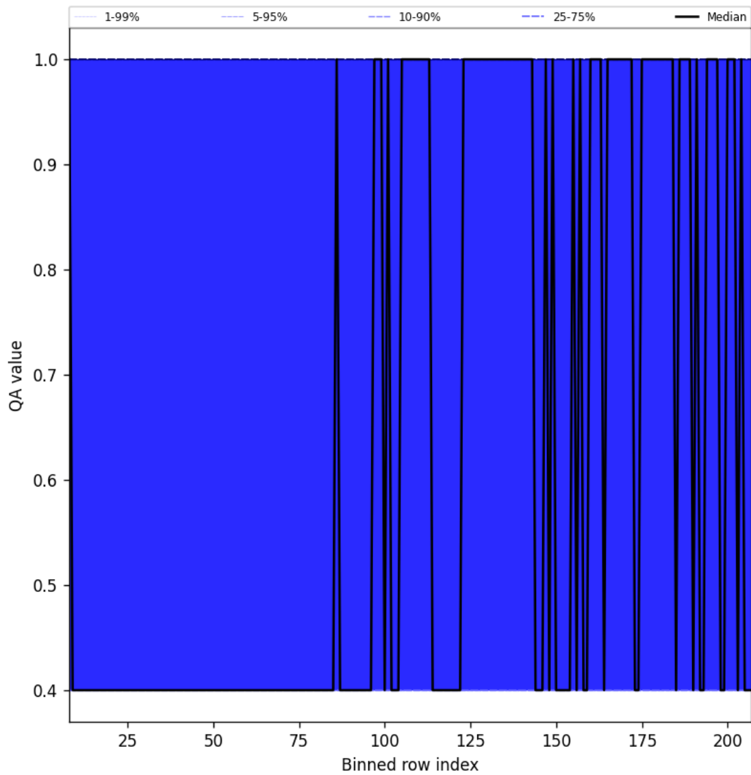
Figure 33: Along track statistics of “QA value” for 2024-09-23 to 2024-09-25
