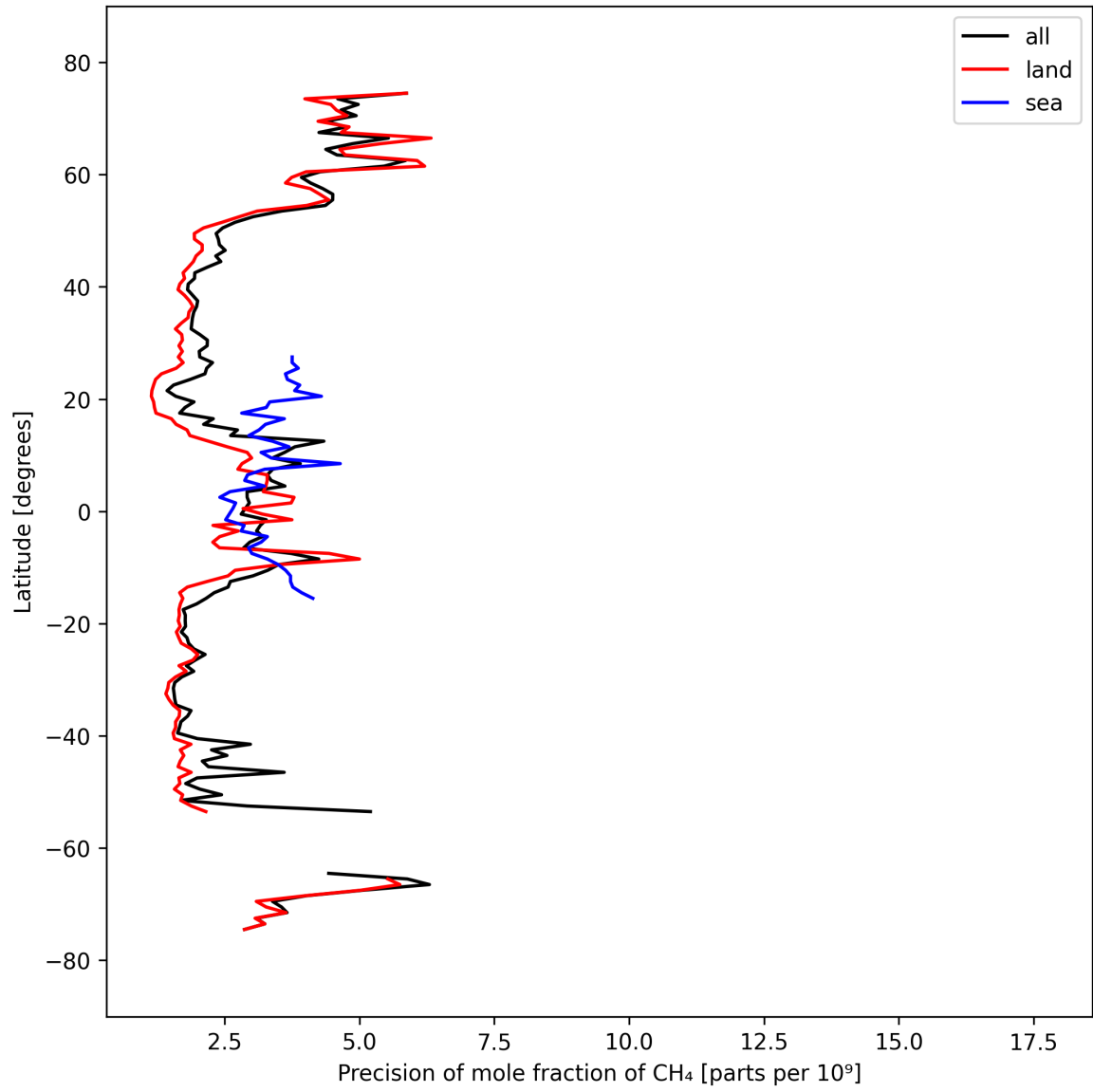
Figure 13: Zonal average of “Precision of mole fraction of CH 4 ” for 2024-09-23 to 2024-09-25.
