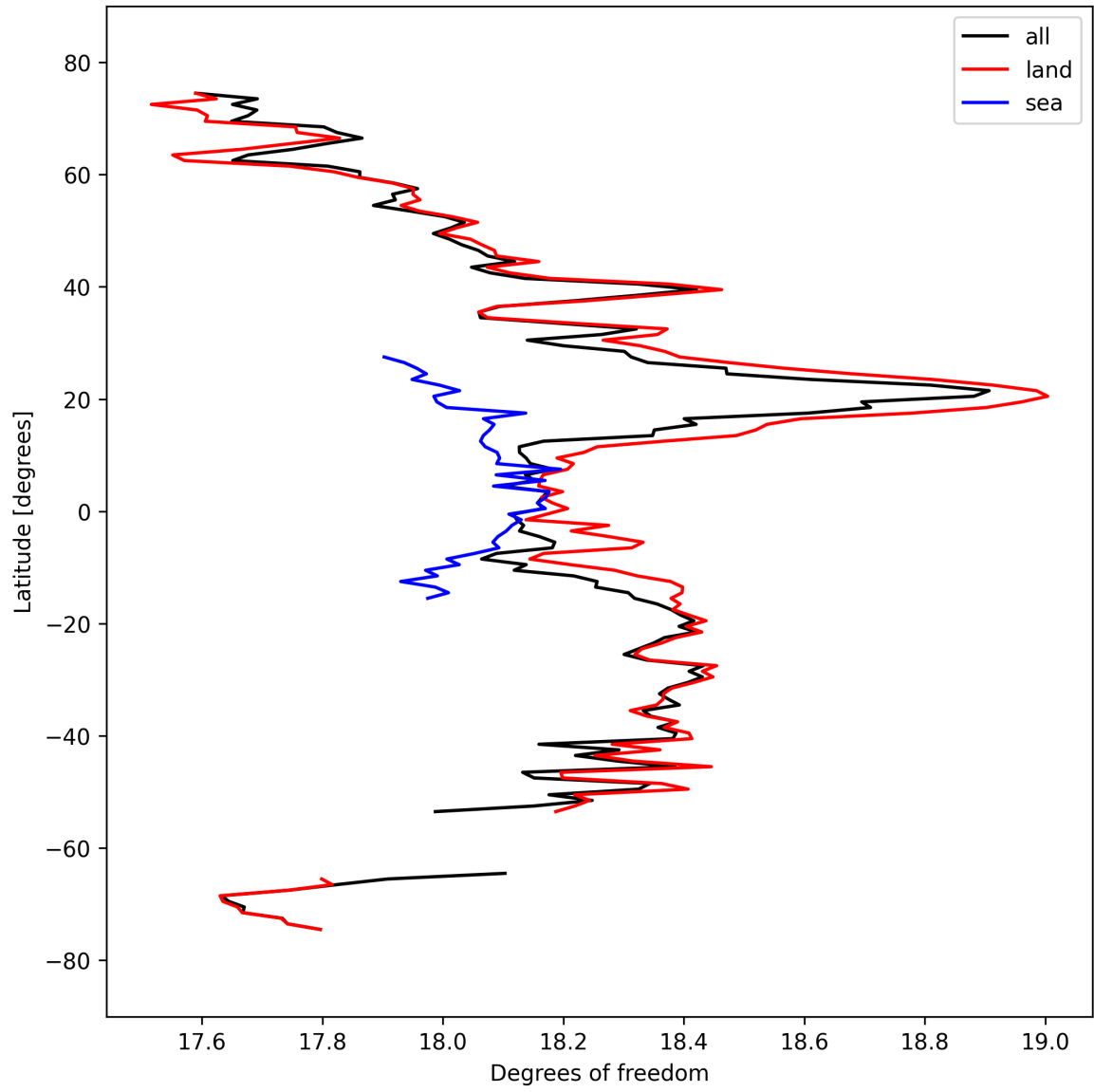
Figure 19: Zonal average of “Degrees of freedom” for 2024-09-23 to 2024-09-25.
