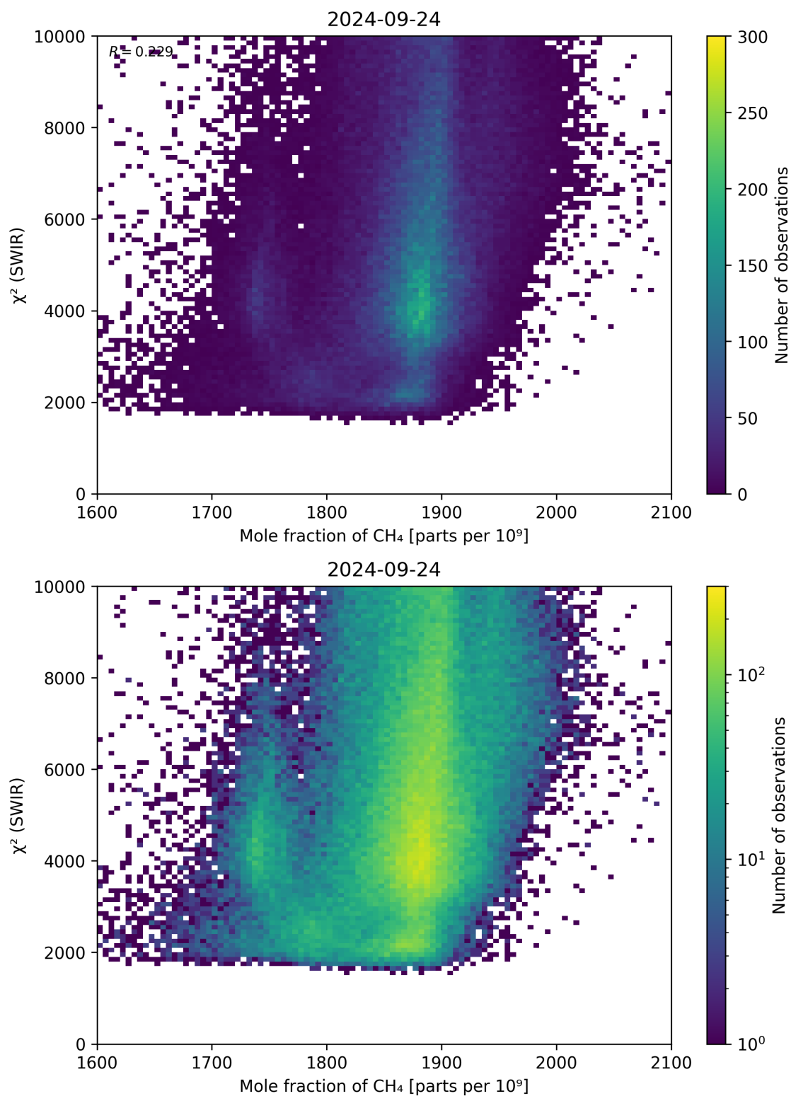
Figure 71: Scatter density plot of “Mole fraction of \text{CH}_4 ” against “ \chi^2 (SWIR)” for 2024-09-23 to 2024-09-25.
