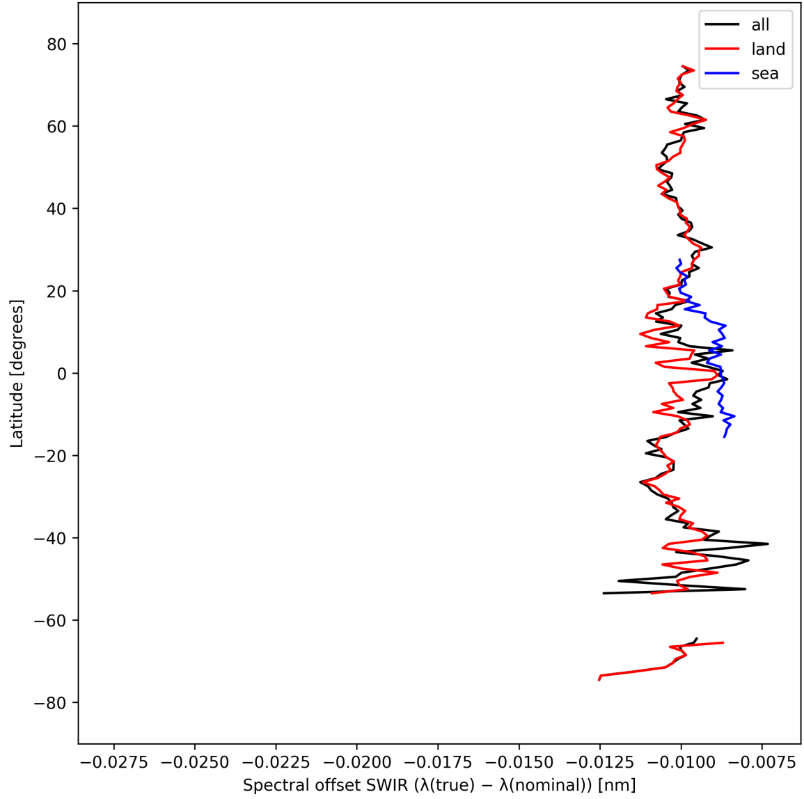
Figure 16: Zonal average of “Spectral offset SWIR ( \lambda_{\text{true}} - \lambda_{\text{nominal}} )” for 2024-09-23 to 2024-09-25.
