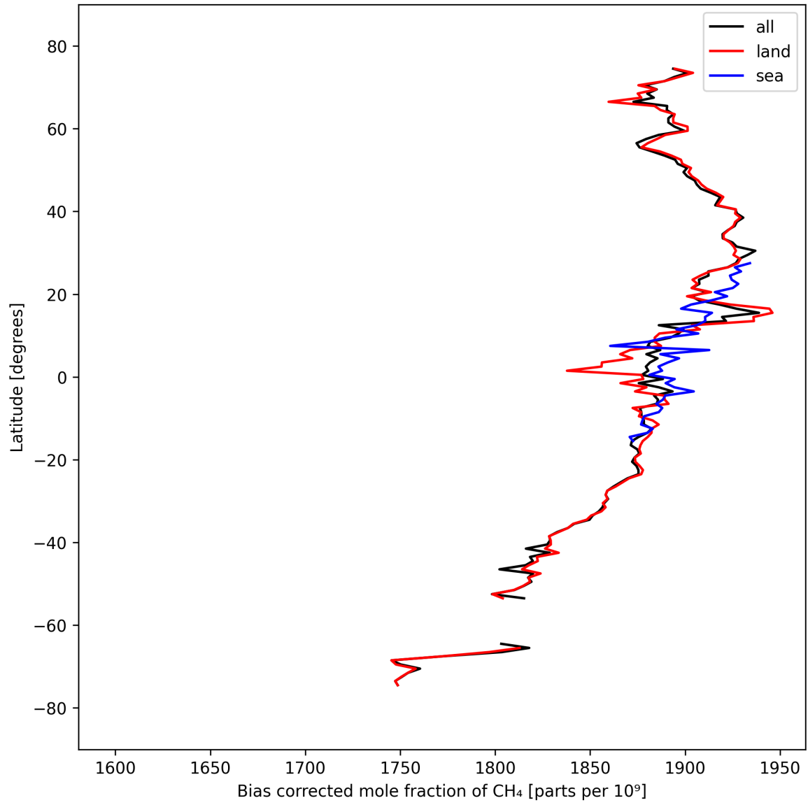
Figure 14: Zonal average of “Bias corrected mole fraction of \text{CH}_4 ” for 2024-09-23 to 2024-09-25.
