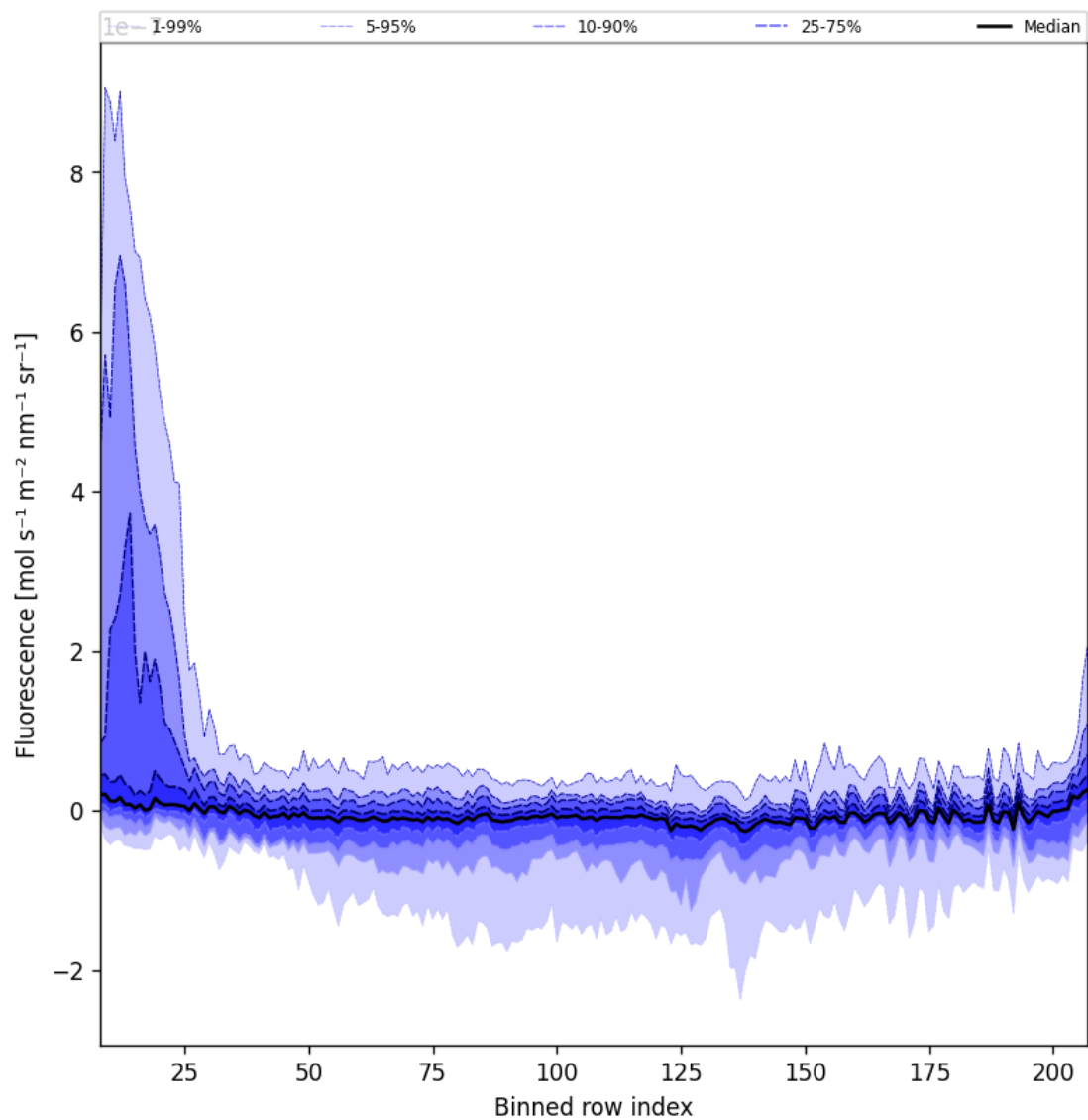
Figure 43: Along track statistics of “Fluorescence” for 2024-09-23 to 2024-09-25
