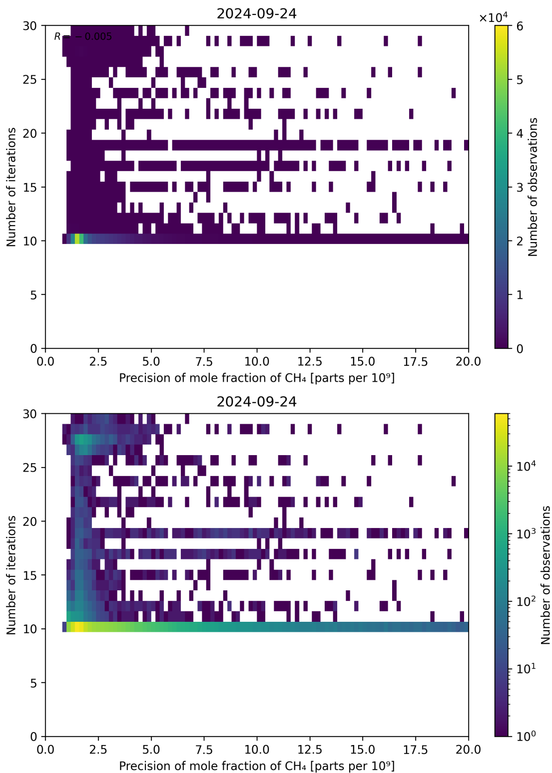
Figure 83: Scatter density plot of “Precision of mole fraction of CH 4 ” against “Number of iterations” for 2024-09-23 to 2024-09-25.
