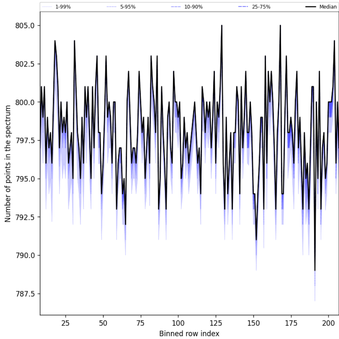
Figure 37: Along track statistics of “Number of points in the spectrum” for 2024-09-23 to 2024-09-25
