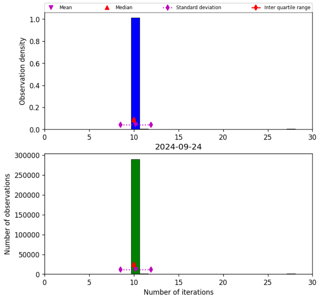
Figure 31: Histogram of “Number of iterations” for 2024-09-23 to 2024-09-25
