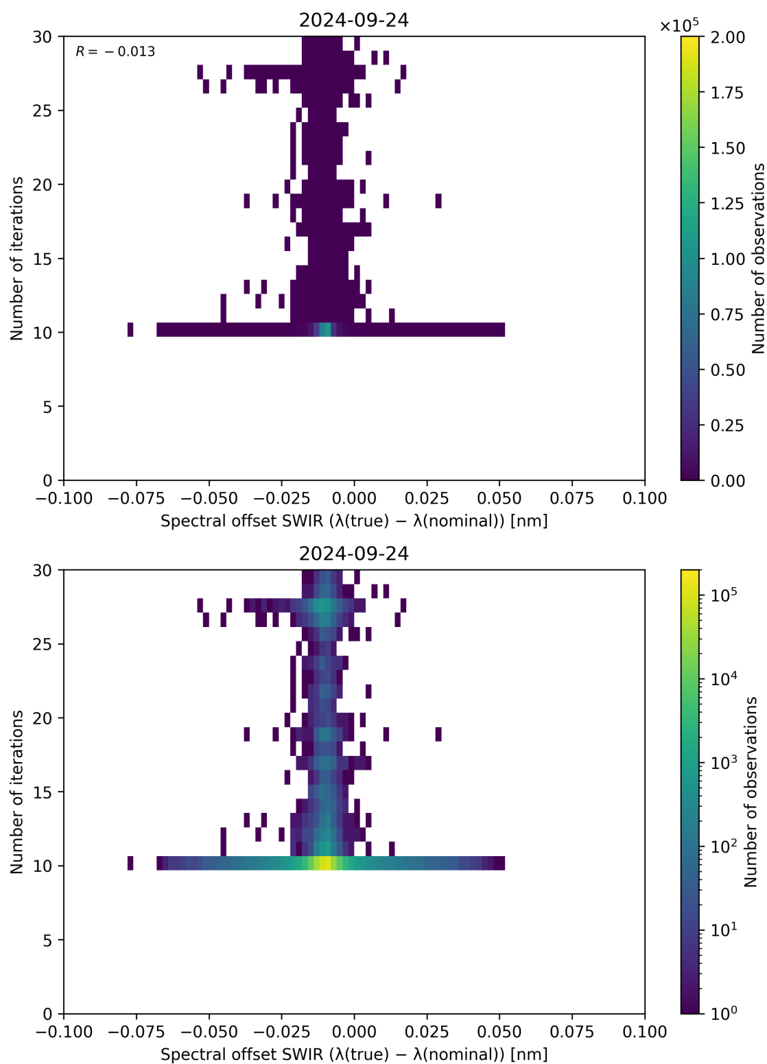
Figure 121: Scatter density plot of “Spectral offset SWIR ( \lambda_{\text{true}} - \lambda_{\text{nominal}} )” against “Number of iterations” for 2024-09-23 to 2024-09-25.
