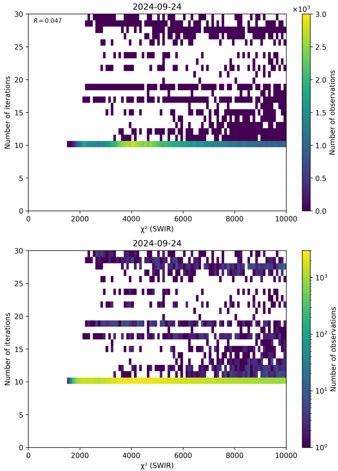
Figure 50: Scatter density plot of “ \chi^2 (SWIR)” against “Number of iterations” for 2024-09-23 to 2024-09-25.
