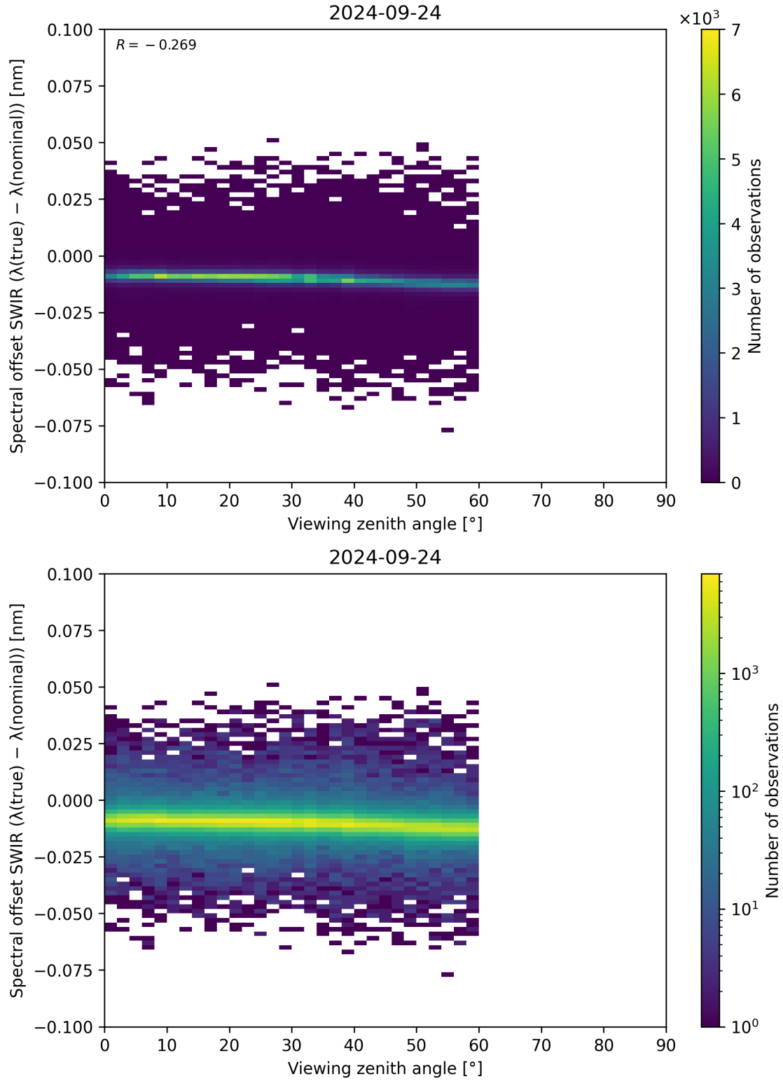
Figure 116: Scatter density plot of “Viewing zenith angle” against “Spectral offset SWIR ( \lambda_{\text{true}} - \lambda_{\text{nominal}} )” for 2024-09-23 to 2024-09-25.
