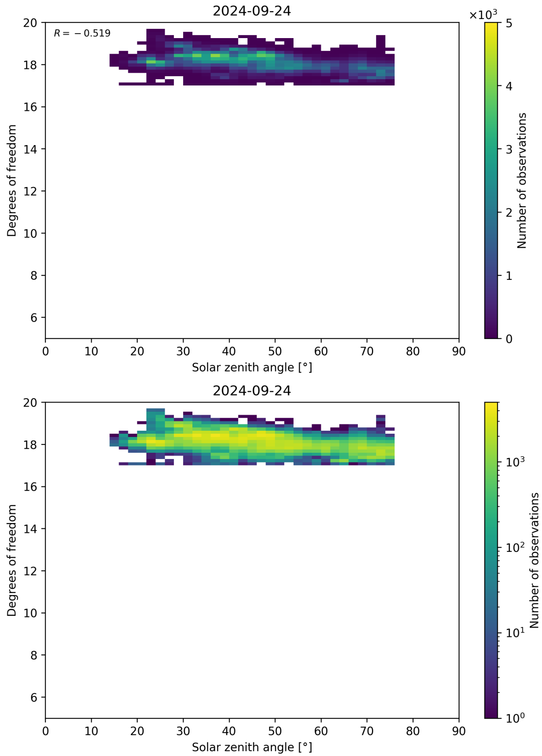
Figure 96: Scatter density plot of “Solar zenith angle” against “Degrees of freedom” for 2024-09-23 to 2024-09-25.
