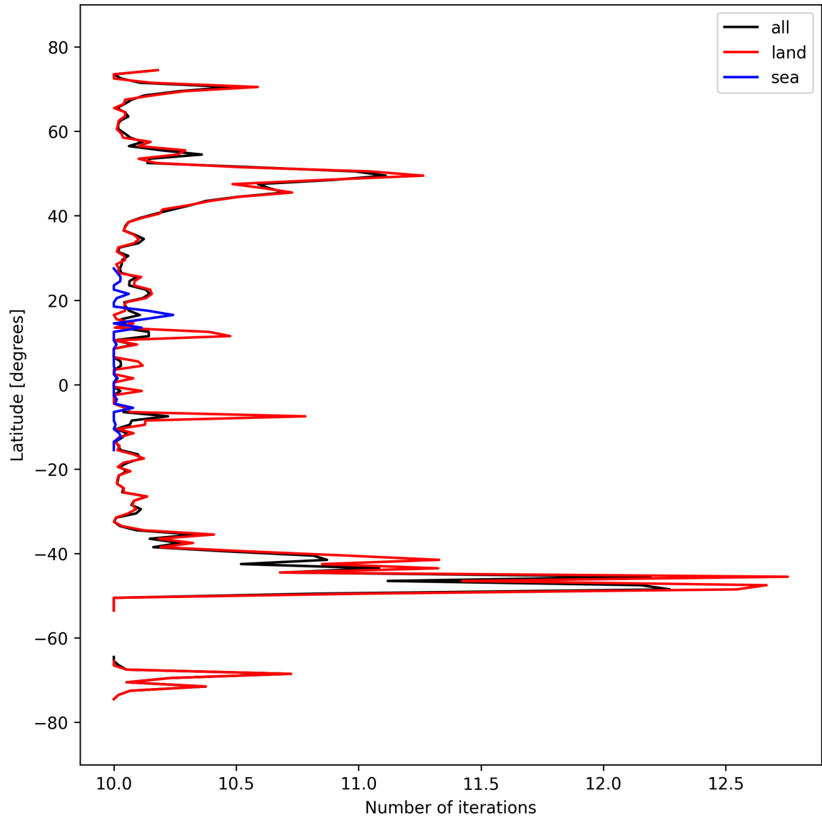
Figure 20: Zonal average of “Number of iterations” for 2024-09-23 to 2024-09-25.
