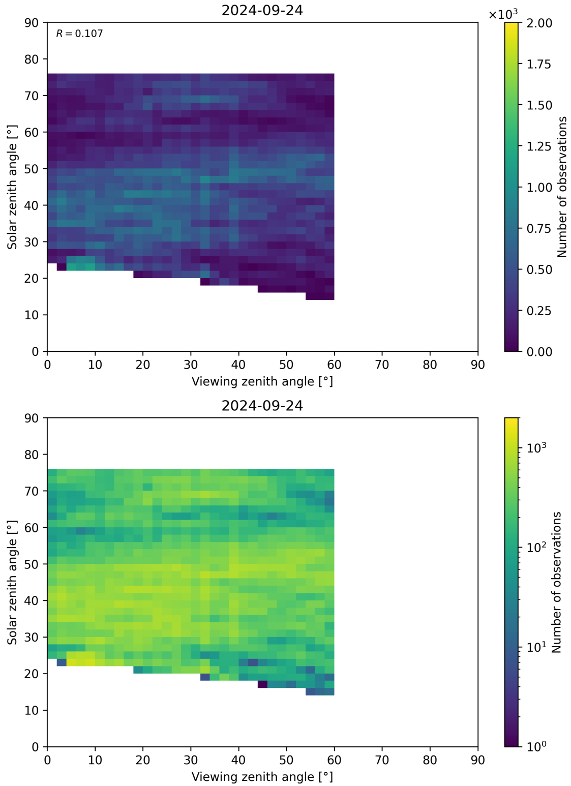
Figure 115: Scatter density plot of “Viewing zenith angle” against “Solar zenith angle” for 2024-09-23 to 2024-09-25.
