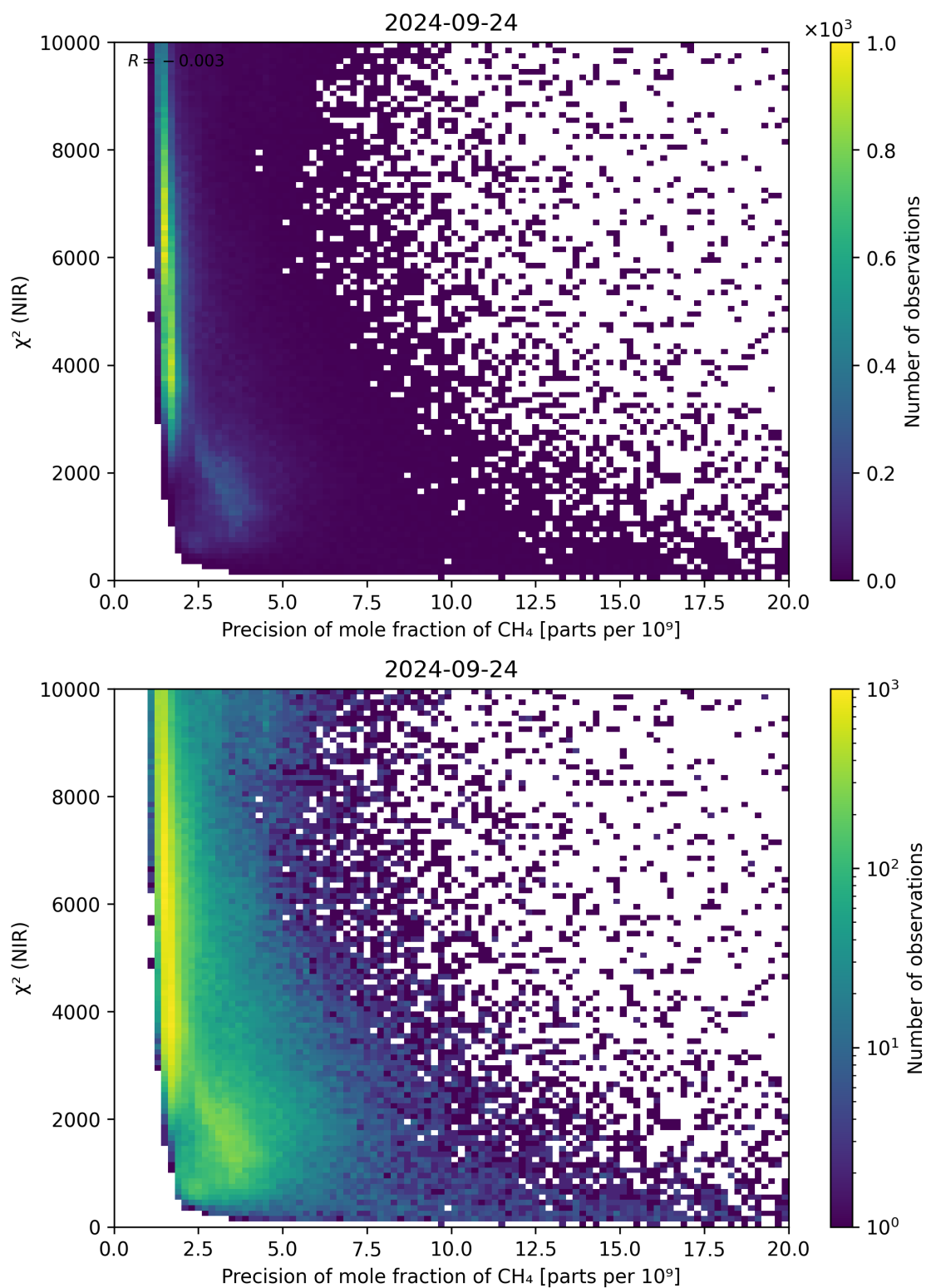
Figure 78: Scatter density plot of “Precision of mole fraction of CH 4 ” against “ \chi^2 (NIR)” for 2024-09-23 to 2024-09-25.
