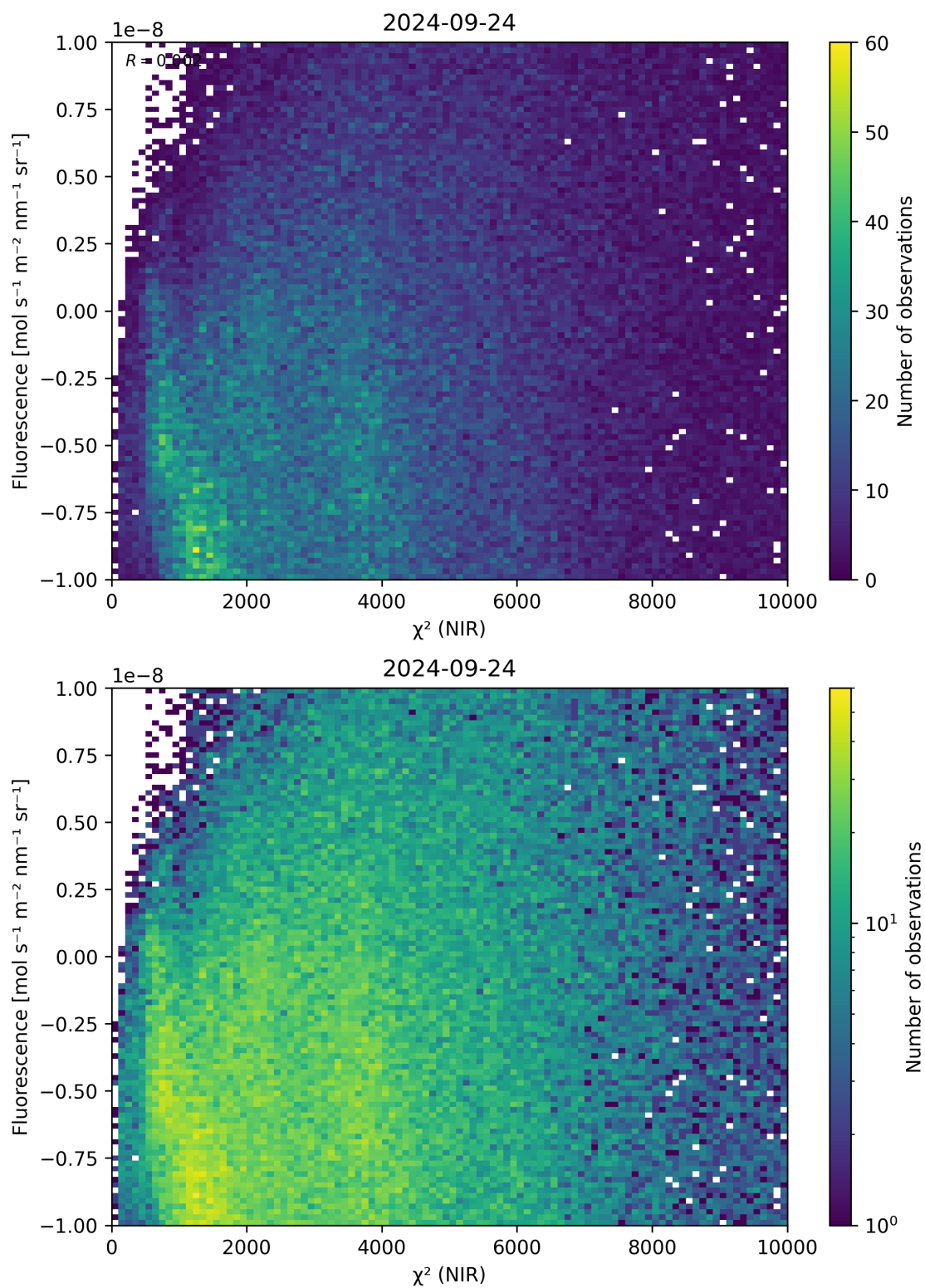
Figure 45: Scatter density plot of “ \chi^2 (NIR)” against “Fluorescence” for 2024-09-23 to 2024-09-25.
