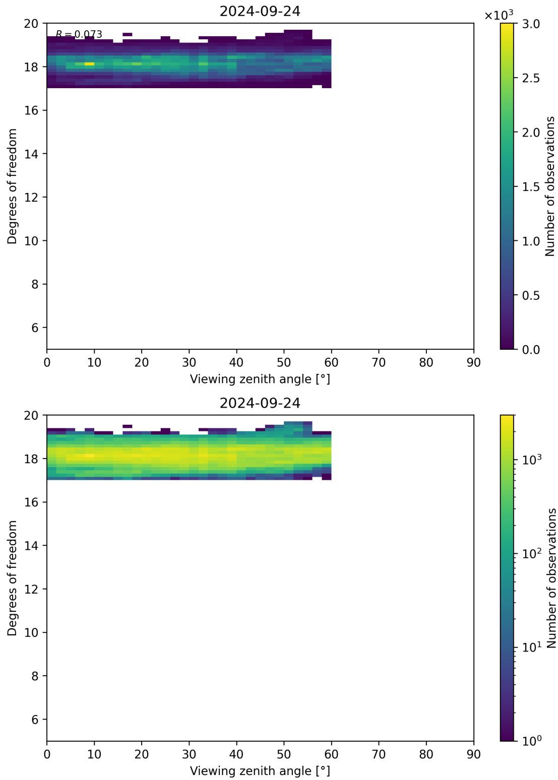
Figure 107: Scatter density plot of “Viewing zenith angle” against “Degrees of freedom” for 2024-09-23 to 2024-09-25.
