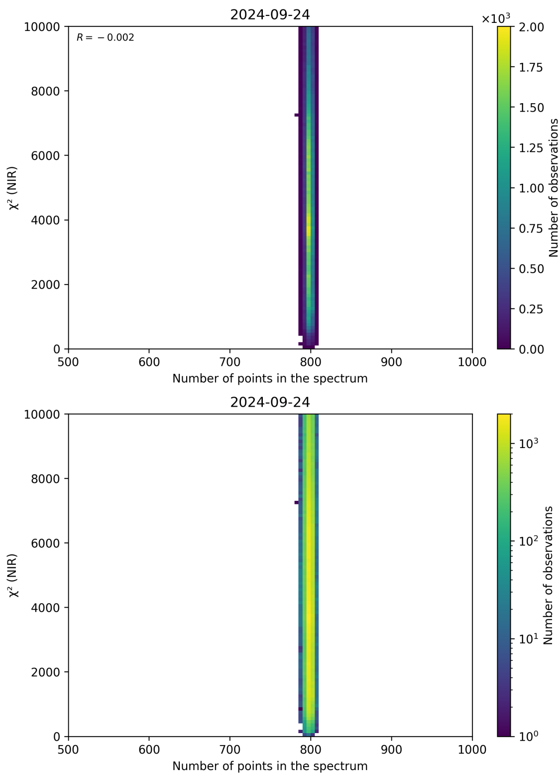
Figure 88: Scatter density plot of “Number of points in the spectrum” against “ \chi^2 (NIR)” for 2024-09-23 to 2024-09-25.
