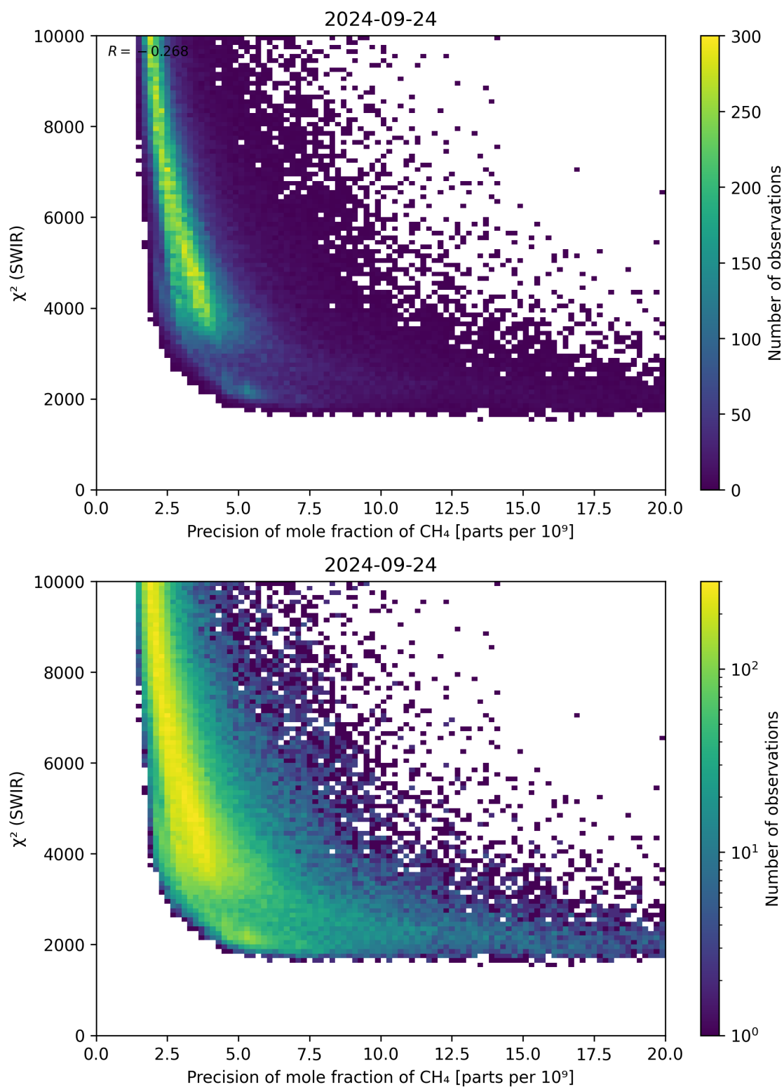
Figure 79: Scatter density plot of “Precision of mole fraction of \text{CH}_4 ” against “ \chi^2 (SWIR)” for 2024-09-23 to 2024-09-25.
