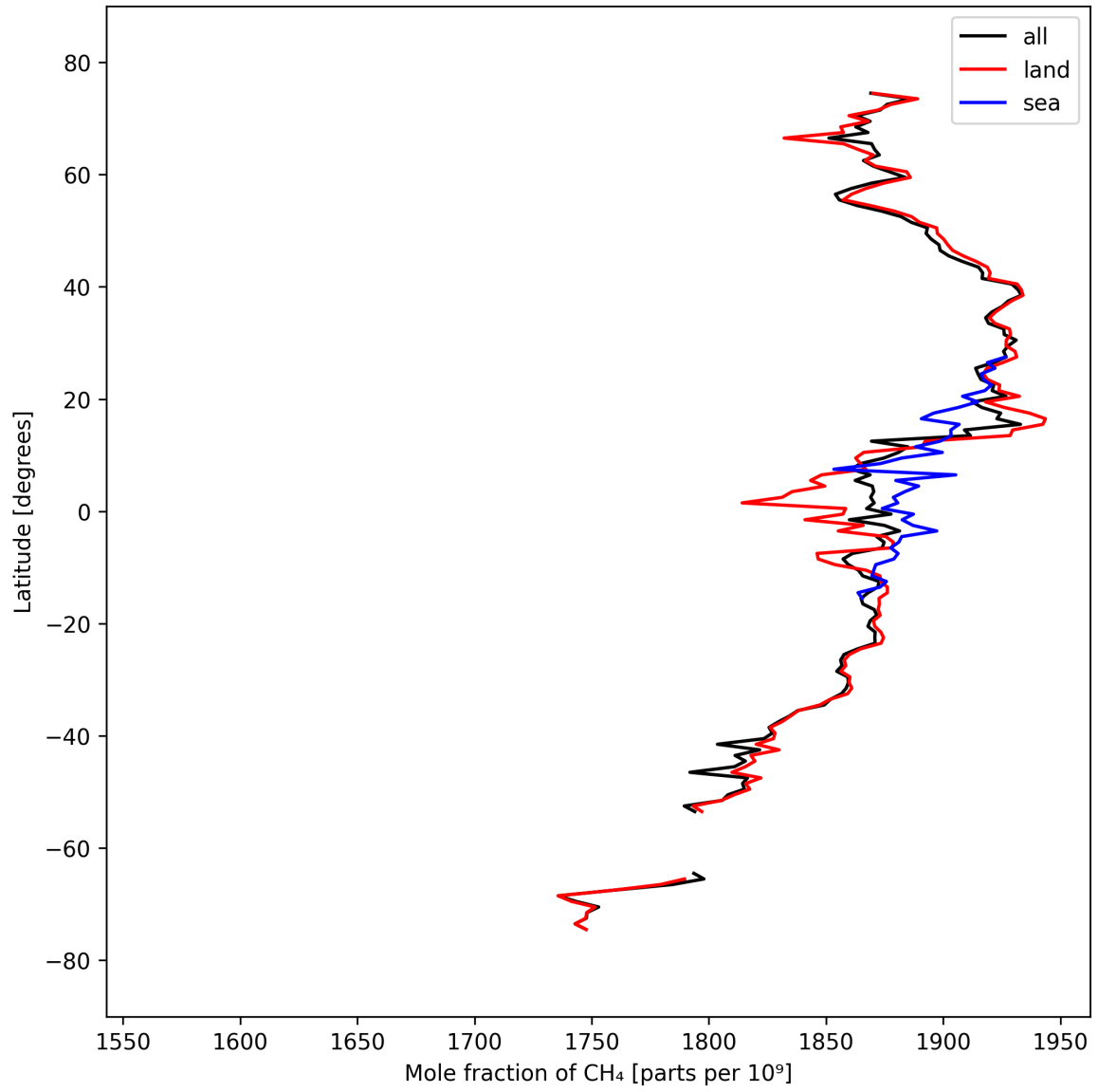
Figure 12: Zonal average of “Mole fraction of CH 4 ” for 2024-09-23 to 2024-09-25.
