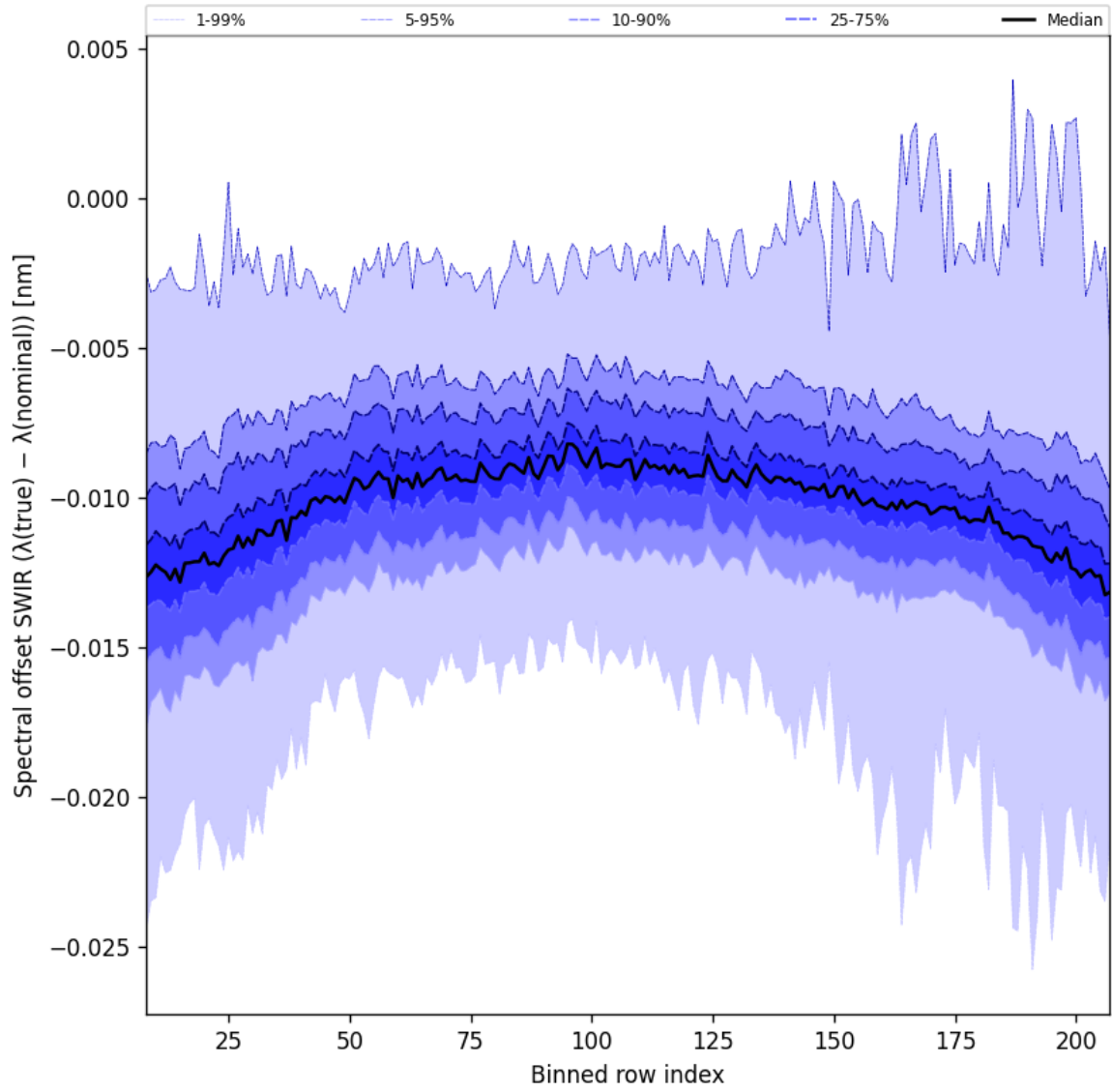
Figure 38: Along track statistics of “Spectral offset SWIR ( \lambda_{\text{true}} - \lambda_{\text{nominal}} )” for 2024-09-24 to 2024-09-26
