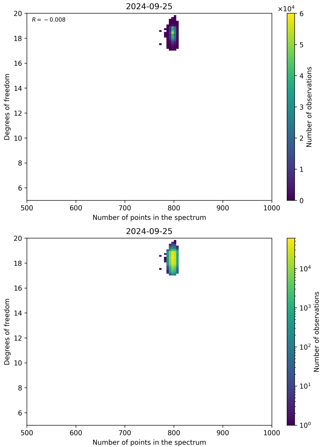
Figure 90: Scatter density plot of “Number of points in the spectrum” against “Degrees of freedom” for 2024-09-24 to 2024-09-26.
