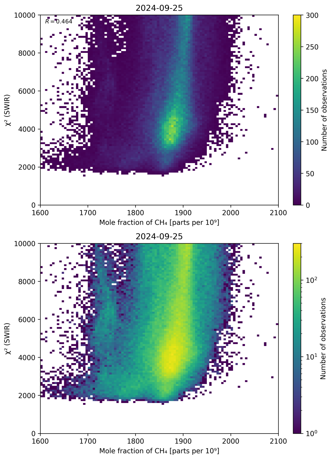
Figure 71: Scatter density plot of “Mole fraction of \text{CH}_4 ” against “ \chi^2 (SWIR)” for 2024-09-24 to 2024-09-26.
