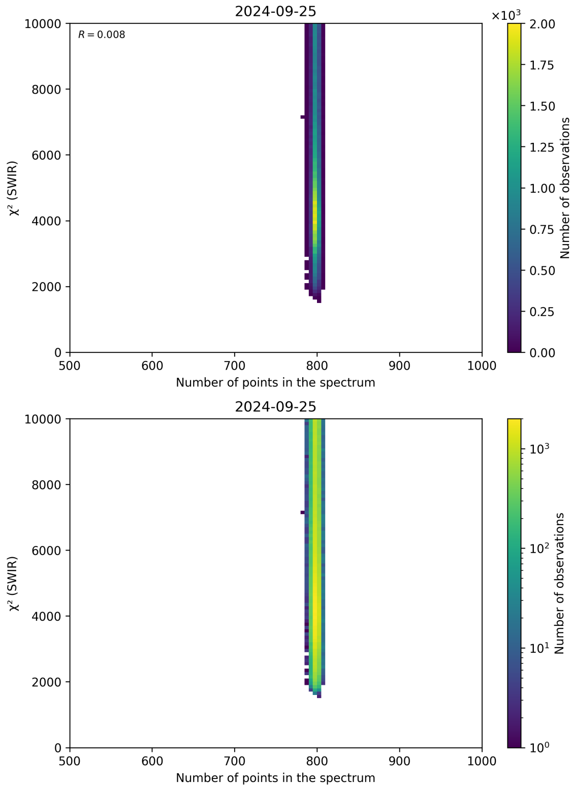
Figure 89: Scatter density plot of “Number of points in the spectrum” against “ \chi^2 (SWIR)” for 2024-09-24 to 2024-09-26.
