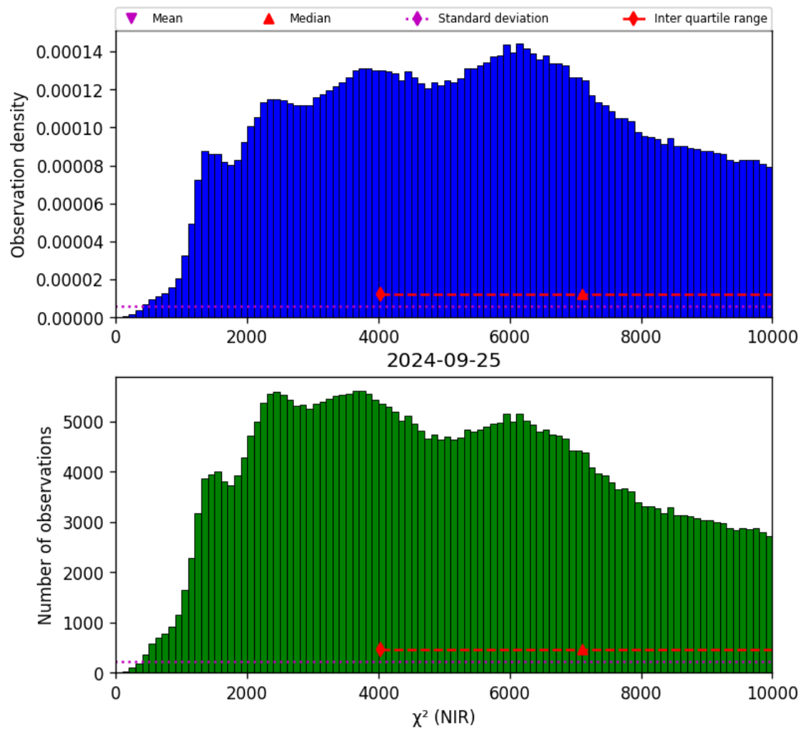
Figure 29: Histogram of “ \chi^2 (NIR)” for 2024-09-24 to 2024-09-26
