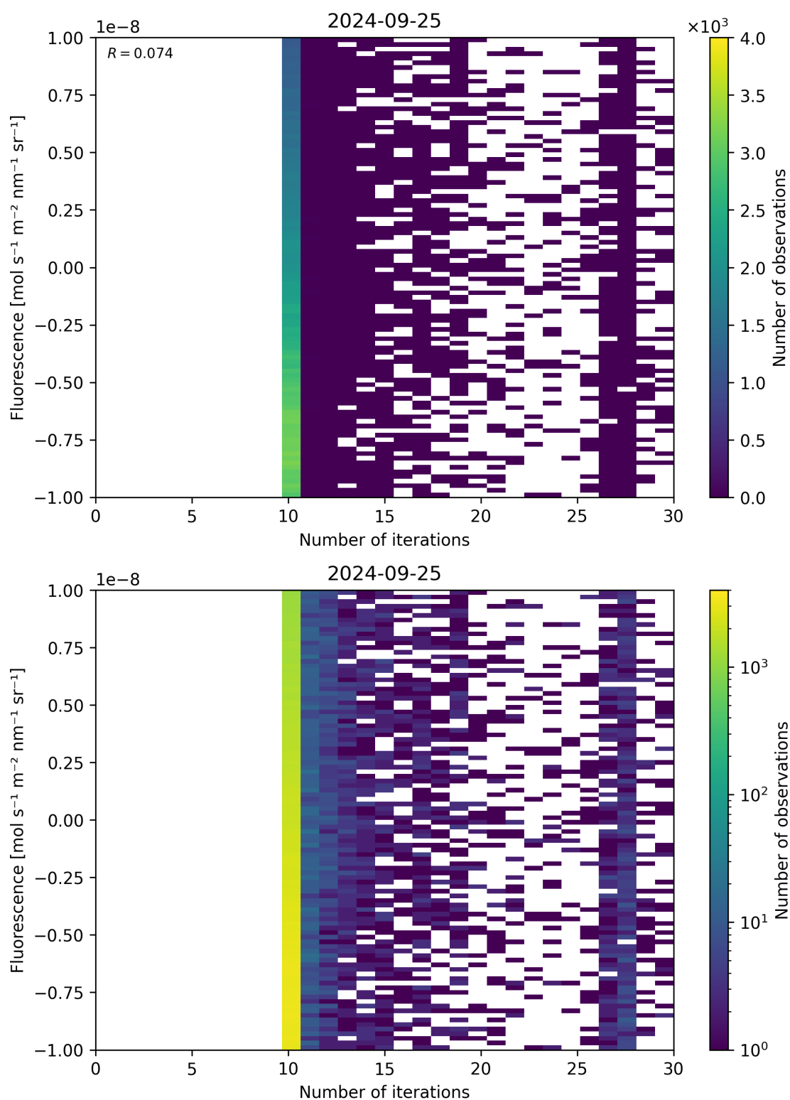
Figure 87: Scatter density plot of “Number of iterations” against “Fluorescence” for 2024-09-24 to 2024-09-26.
