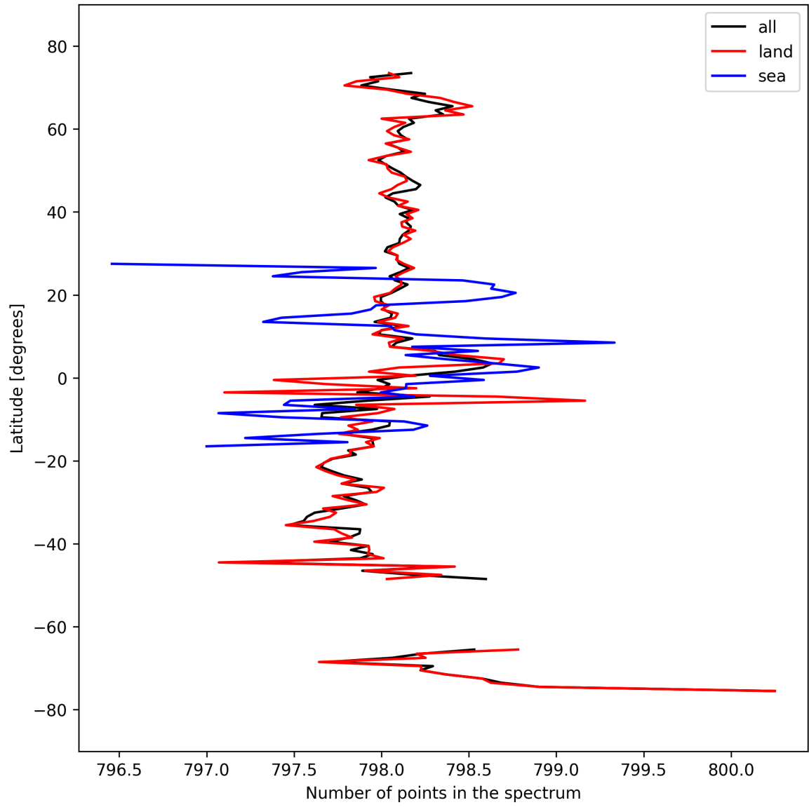
Figure 15: Zonal average of “Number of points in the spectrum” for 2024-09-24 to 2024-09-26.
