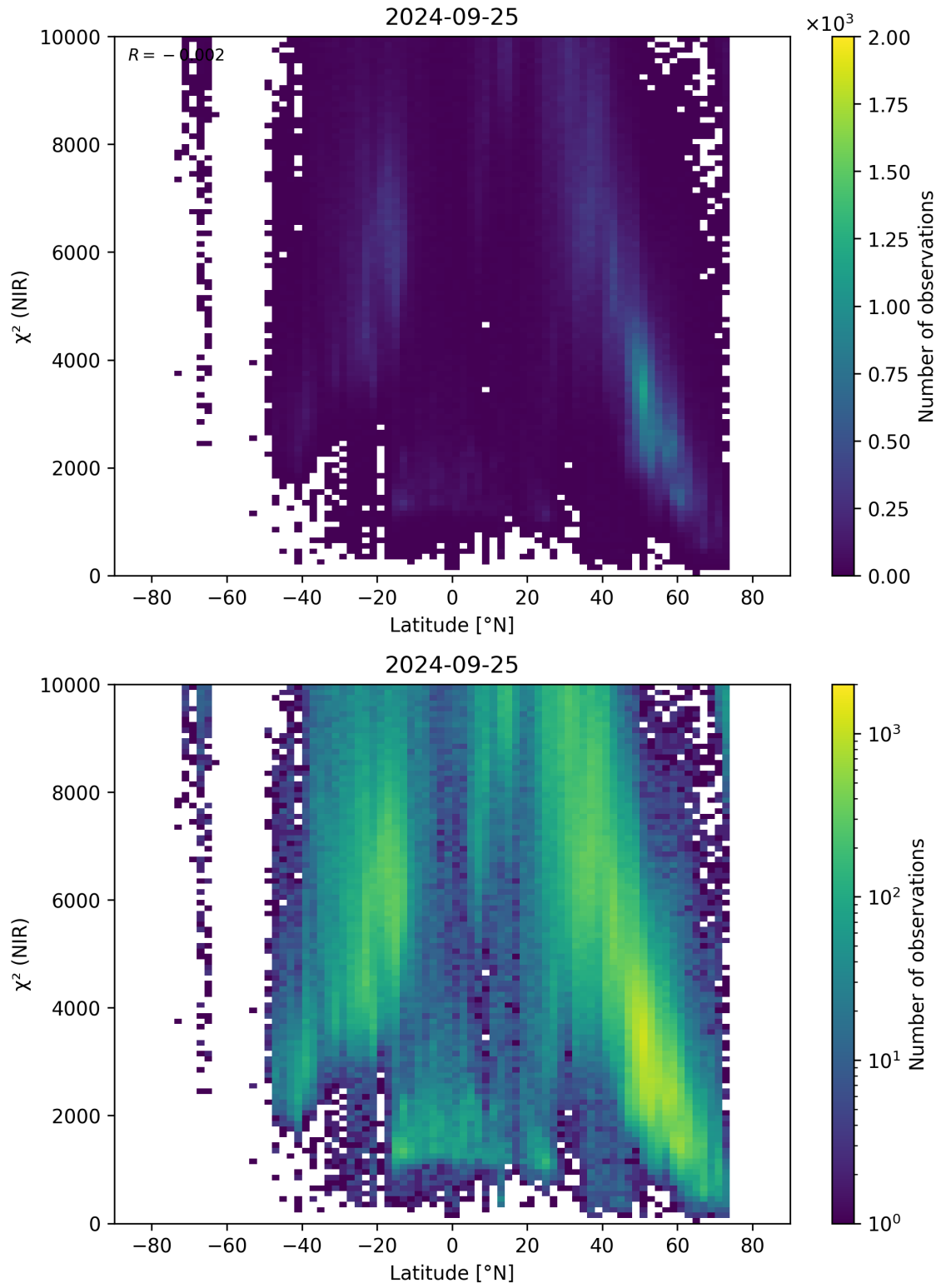
Figure 53: Scatter density plot of “Latitude” against “ \chi^2 (NIR)” for 2024-09-24 to 2024-09-26.
