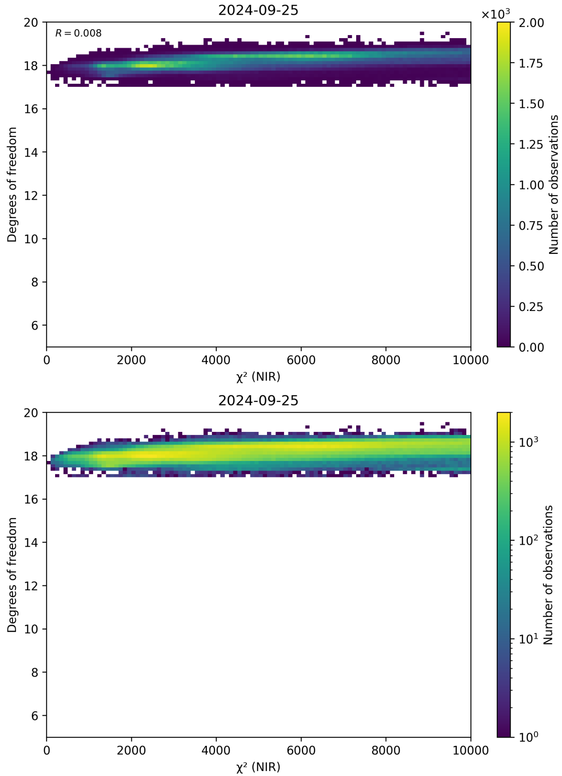
Figure 44: Scatter density plot of “ \chi^2 (NIR)” against “Degrees of freedom” for 2024-09-24 to 2024-09-26.
