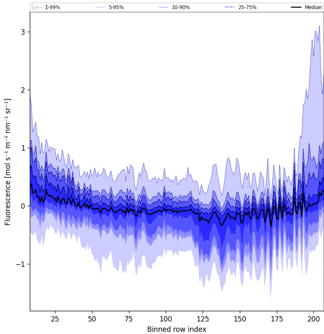
Figure 43: Along track statistics of “Fluorescence” for 2024-09-24 to 2024-09-26
