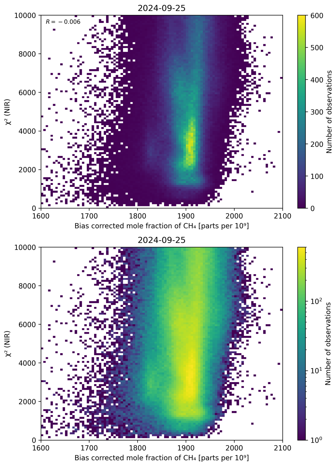
Figure 63: Scatter density plot of “Bias corrected mole fraction of CH 4 ” against “ \chi^2 (NIR)” for 2024-09-24 to 2024-09-26.
