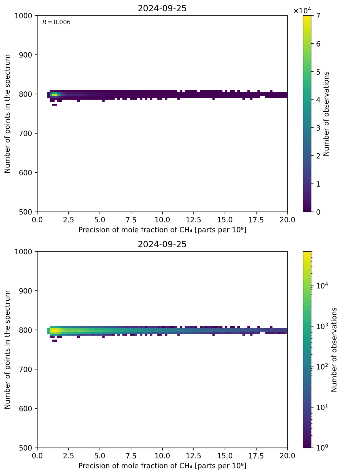
Figure 84: Scatter density plot of “Precision of mole fraction of CH 4 ” against “Number of points in the spectrum” for 2024-09-24 to 2024-09-26.
