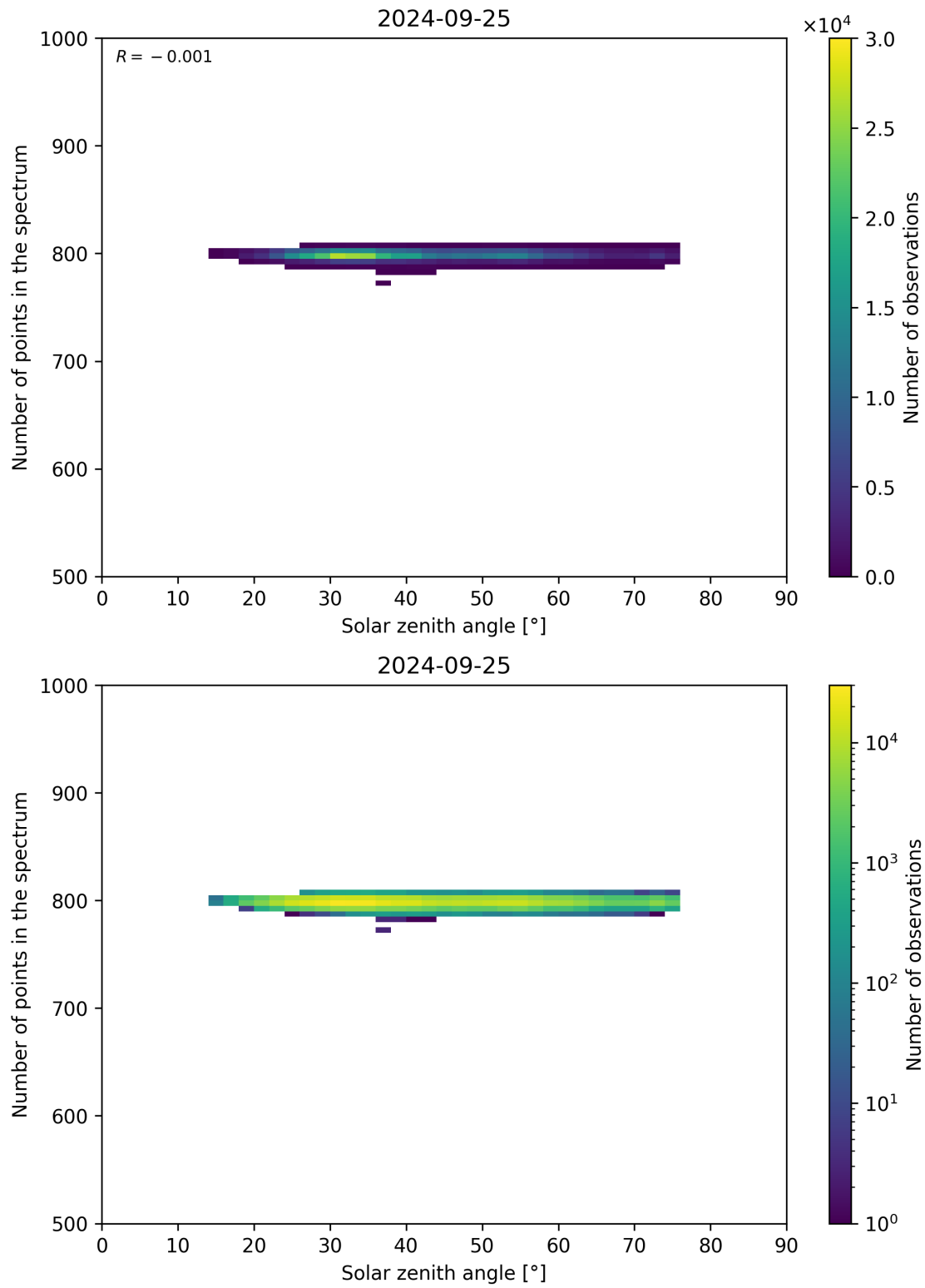
Figure 103: Scatter density plot of “Solar zenith angle” against “Number of points in the spectrum” for 2024-09-24 to 2024-09-26.
