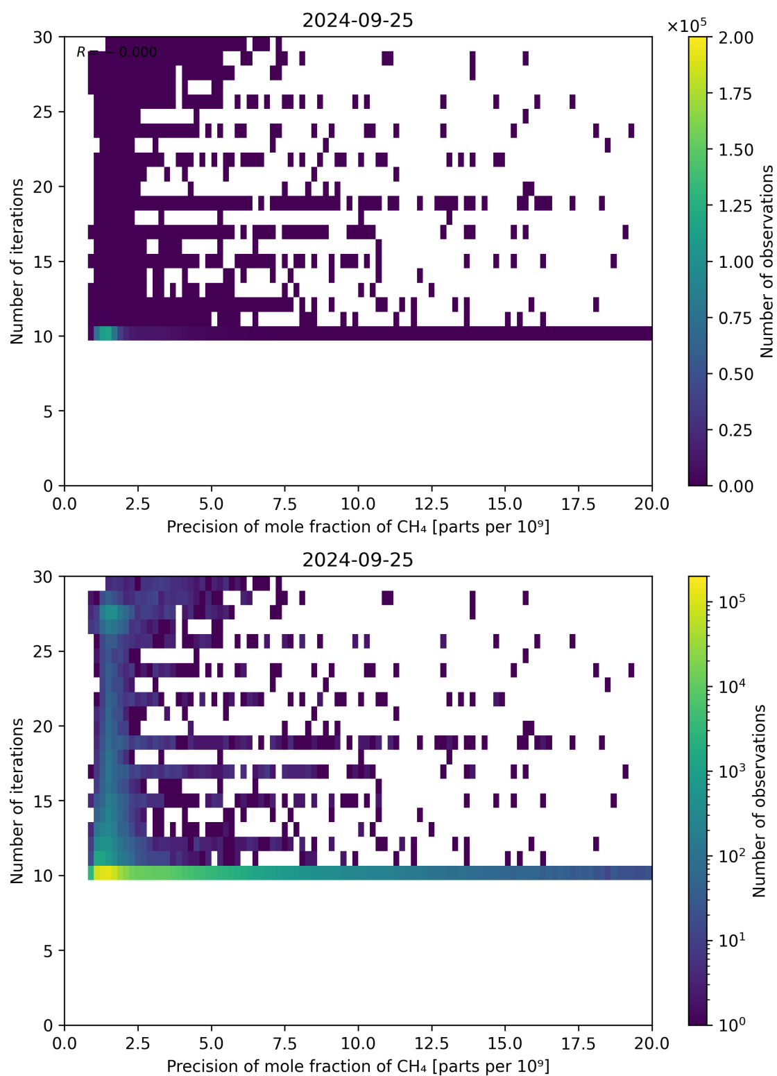
Figure 83: Scatter density plot of “Precision of mole fraction of CH 4 ” against “Number of iterations” for 2024-09-24 to 2024-09-26.
