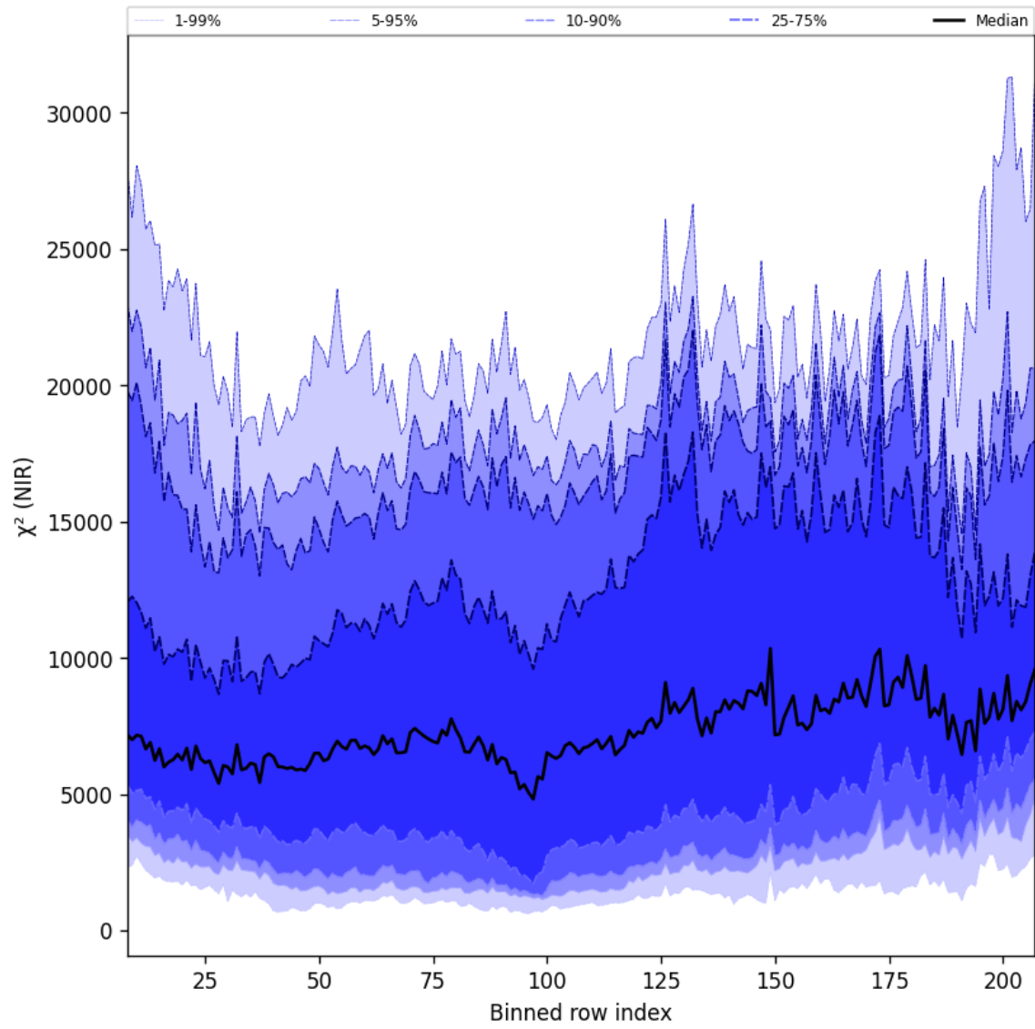
Figure 40: Along track statistics of “ \chi^2 (NIR)” for 2024-09-24 to 2024-09-26
