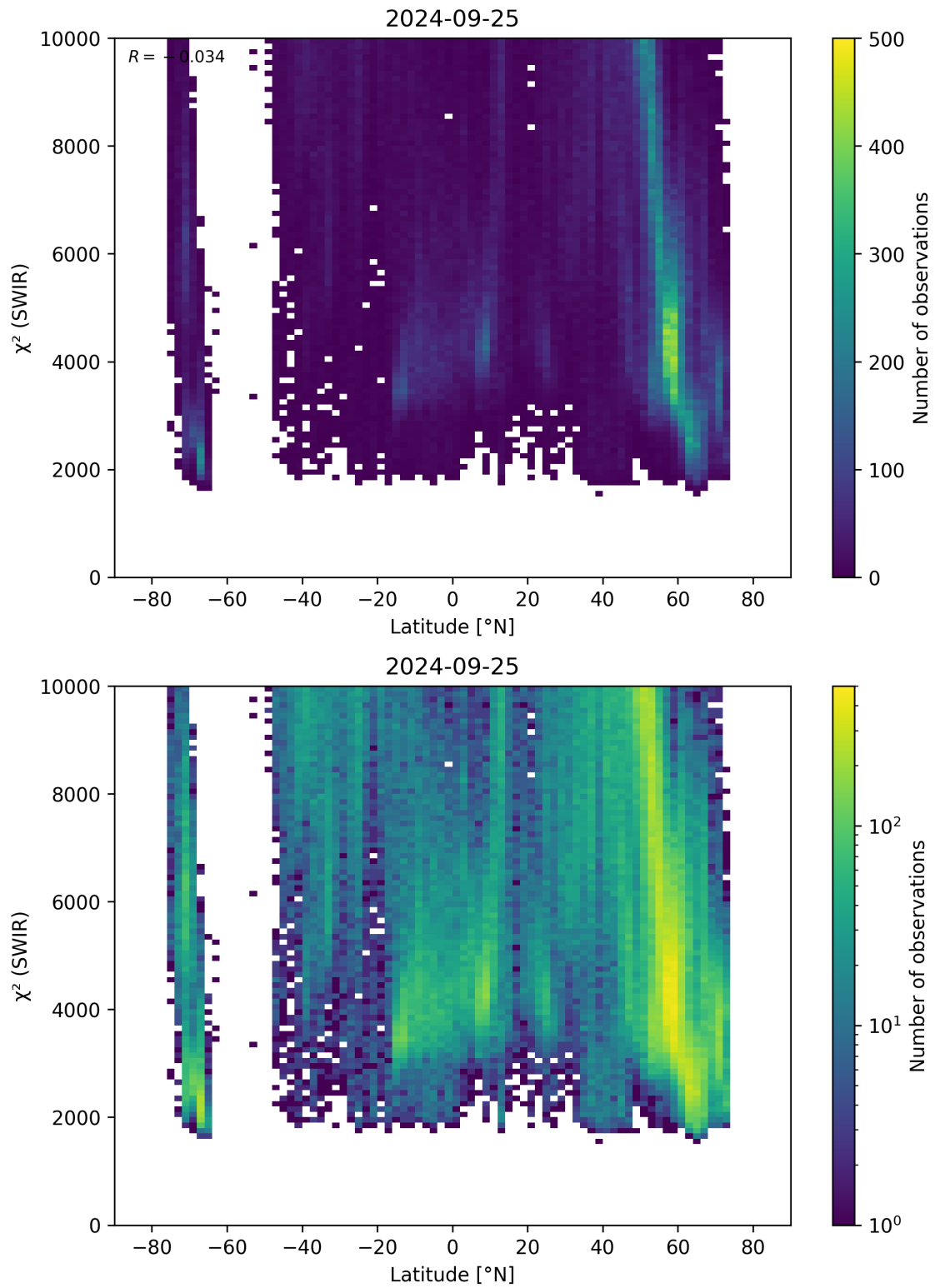
Figure 54: Scatter density plot of “Latitude” against “ \chi^2 (SWIR)” for 2024-09-24 to 2024-09-26.
