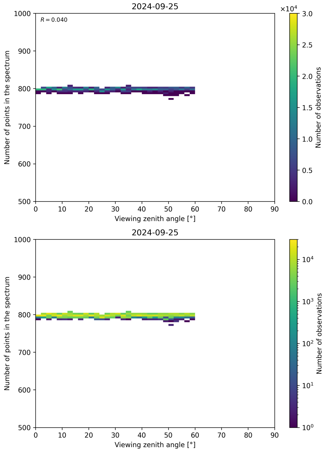
Figure 114: Scatter density plot of “Viewing zenith angle” against “Number of points in the spectrum” for 2024-09-24 to 2024-09-26.
