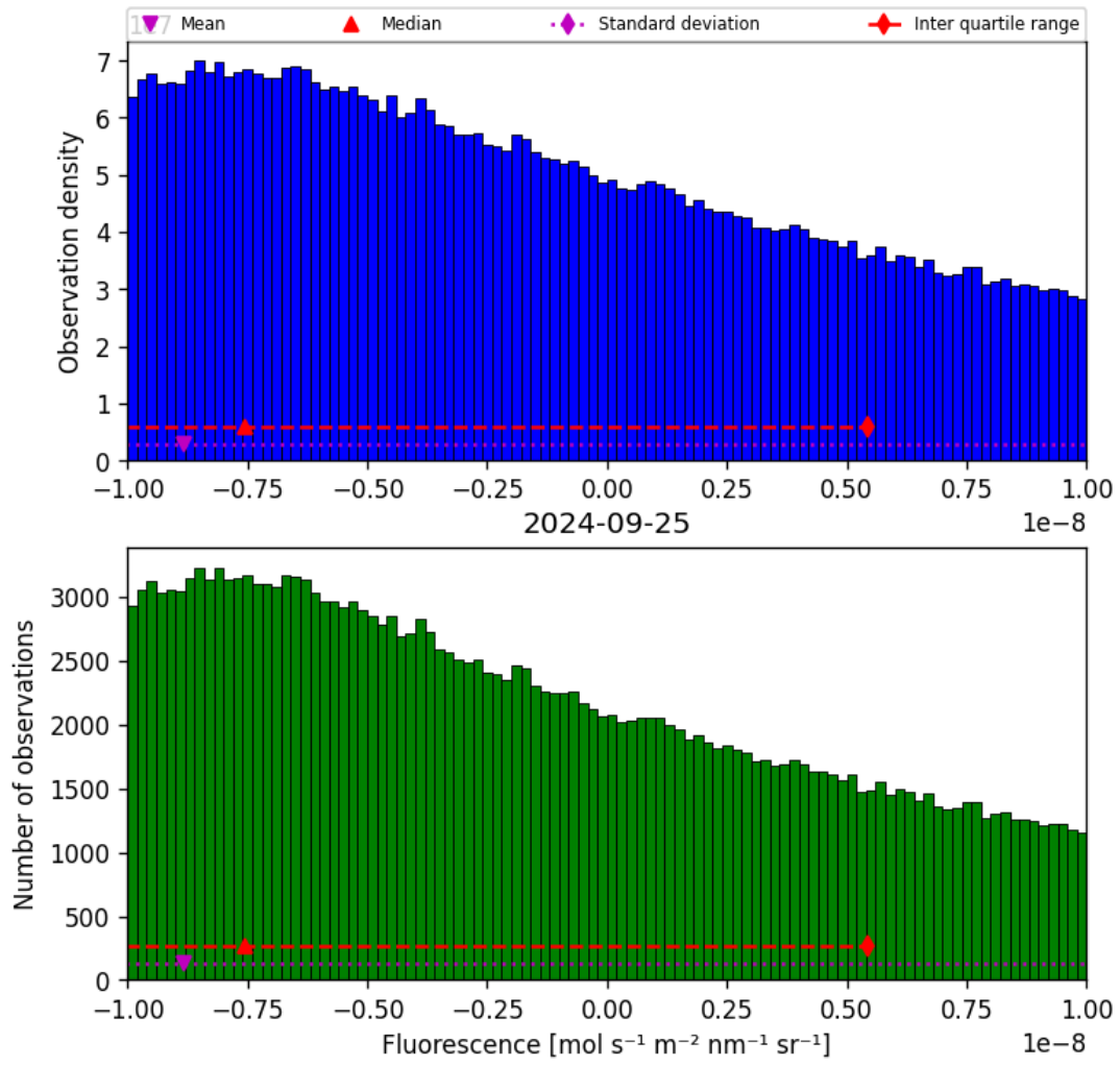
Figure 32: Histogram of “Fluorescence” for 2024-09-24 to 2024-09-26
