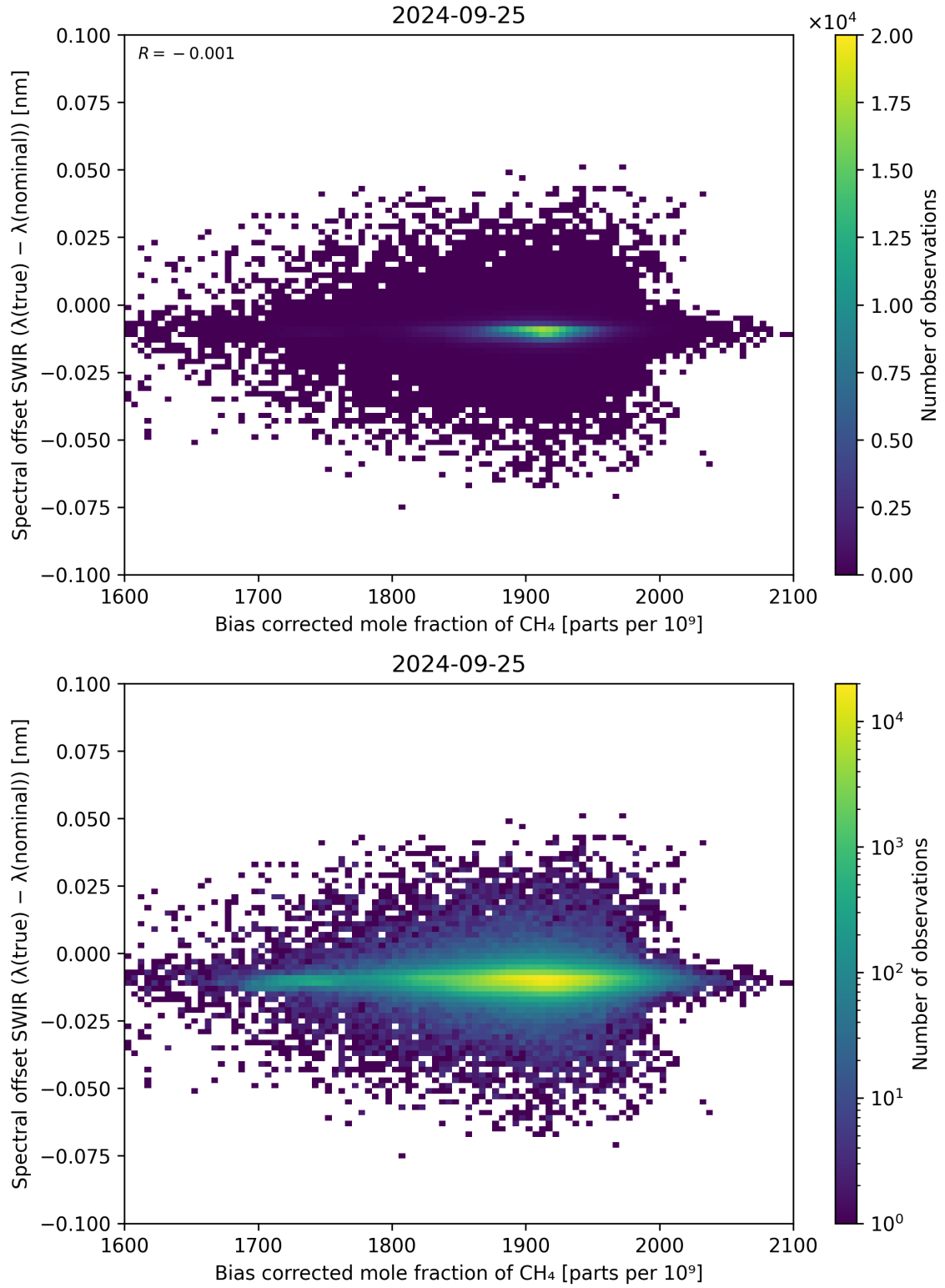
Figure 69: Scatter density plot of “Bias corrected mole fraction of CH 4 ” against “Spectral offset SWIR ( \lambda_{\text{true}} - \lambda_{\text{nominal}} )” for 2024-09-24 to 2024-09-26.
