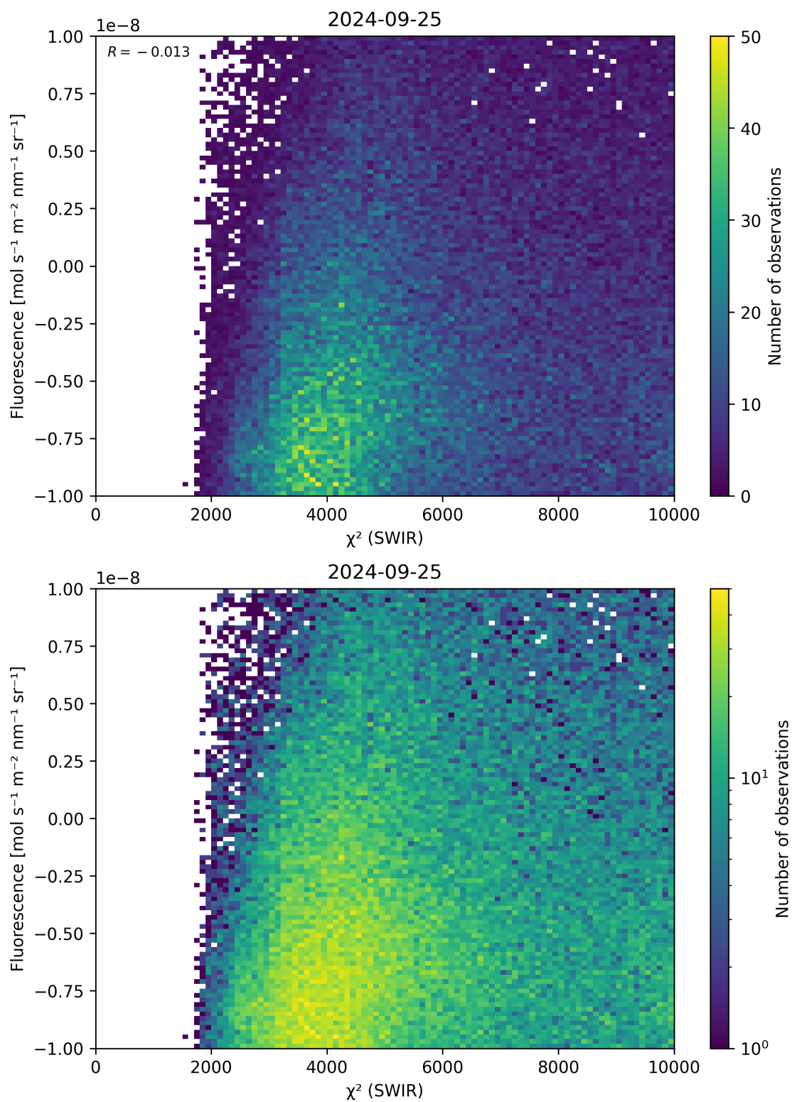
Figure 49: Scatter density plot of “ \chi^2 (SWIR)” against “Fluorescence” for 2024-09-24 to 2024-09-26.
