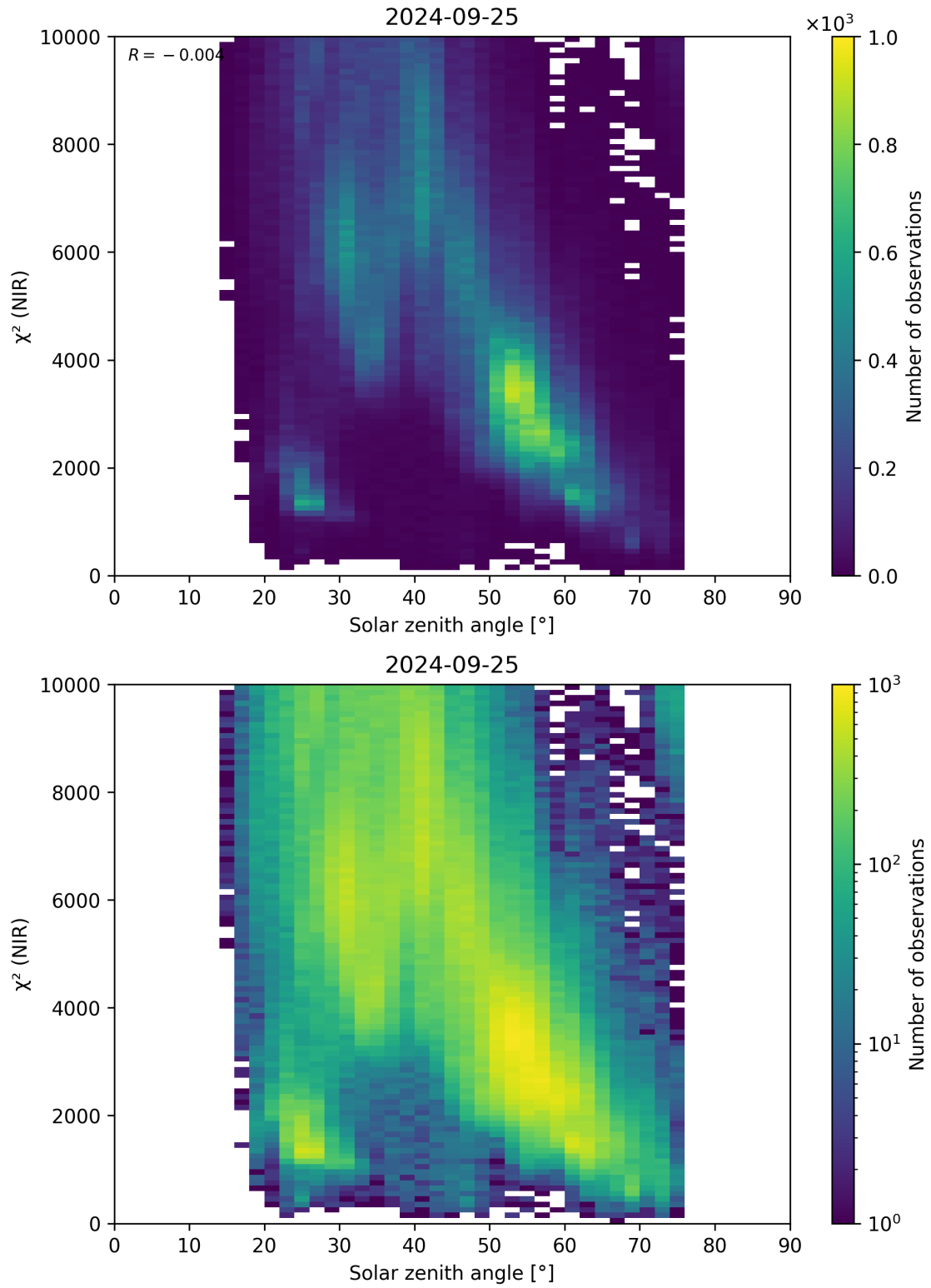
Figure 94: Scatter density plot of “Solar zenith angle” against “ \chi^2 (NIR)” for 2024-09-24 to 2024-09-26.
