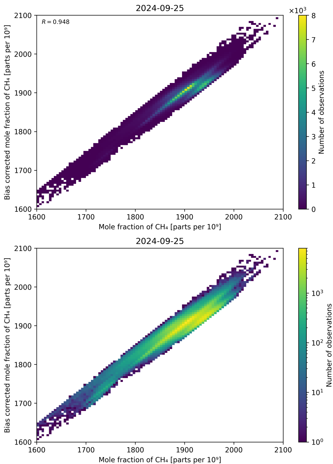
Figure 74: Scatter density plot of “Mole fraction of CH 4 ” against “Bias corrected mole fraction of CH 4 ” for 2024-09-24 to 2024-09-26.
