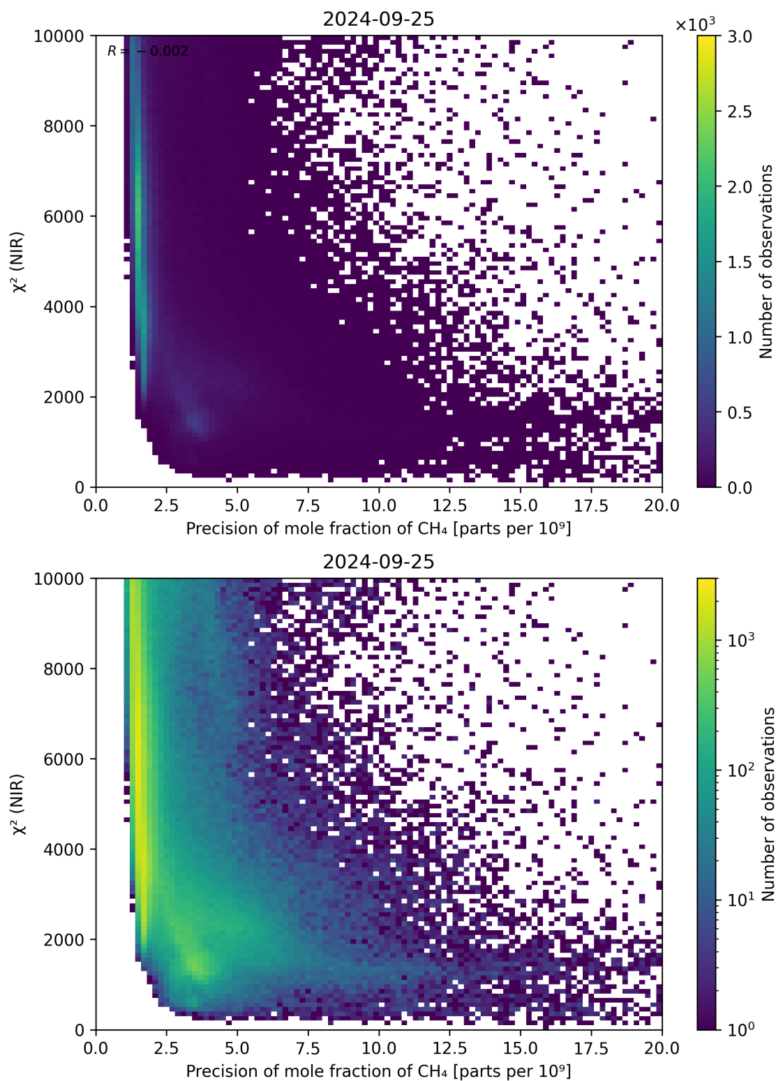
Figure 78: Scatter density plot of “Precision of mole fraction of \text{CH}_4 ” against “ \chi^2 (NIR)” for 2024-09-24 to 2024-09-26.
