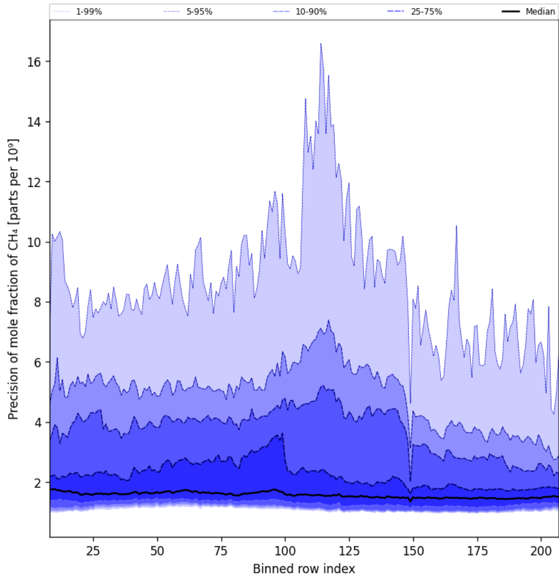
Figure 35: Along track statistics of “Precision of mole fraction of CH 4 ” for 2024-09-24 to 2024-09-26
