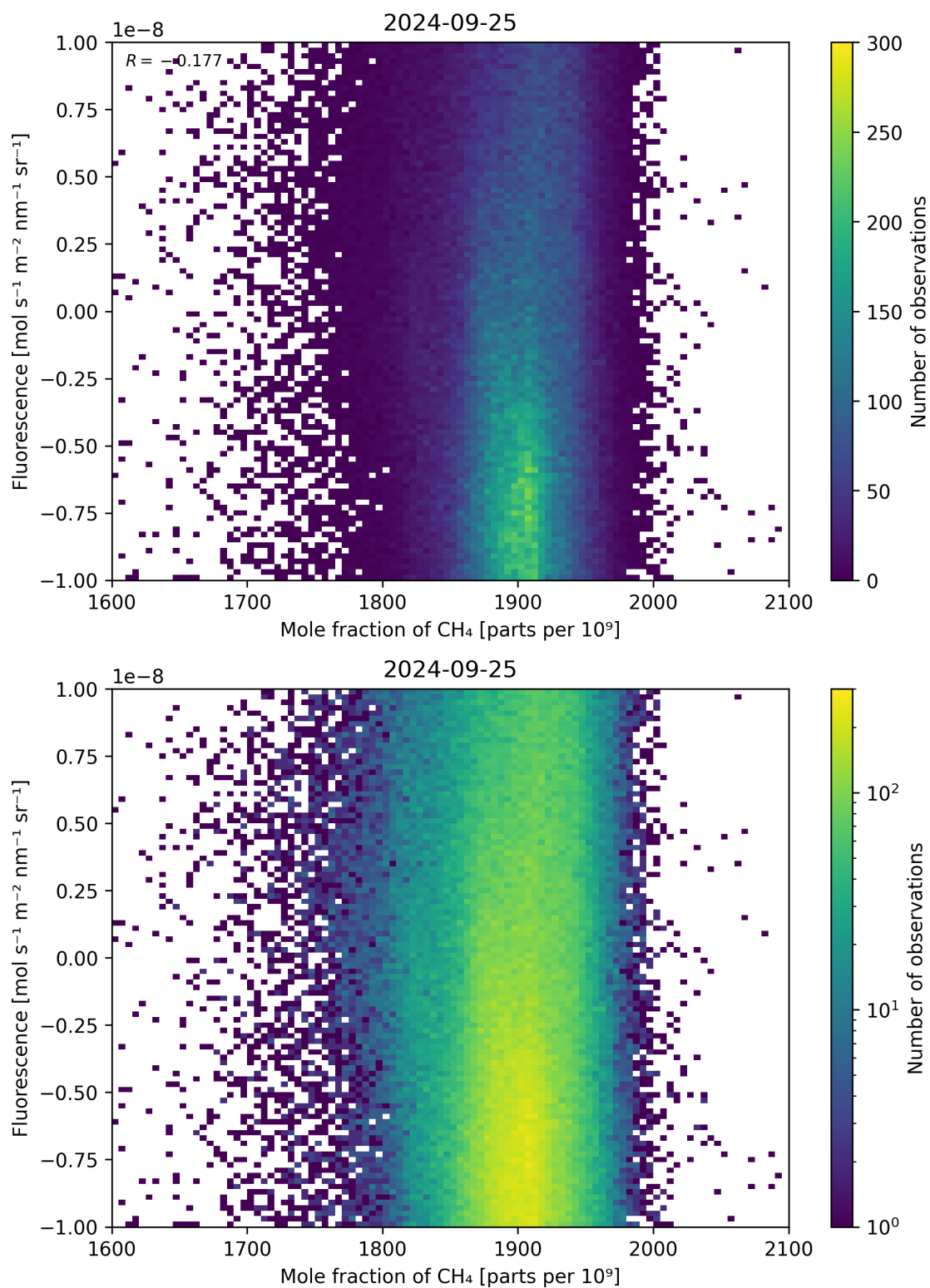
Figure 73: Scatter density plot of “Mole fraction of \text{CH}_4 ” against “Fluorescence” for 2024-09-24 to 2024-09-26.
