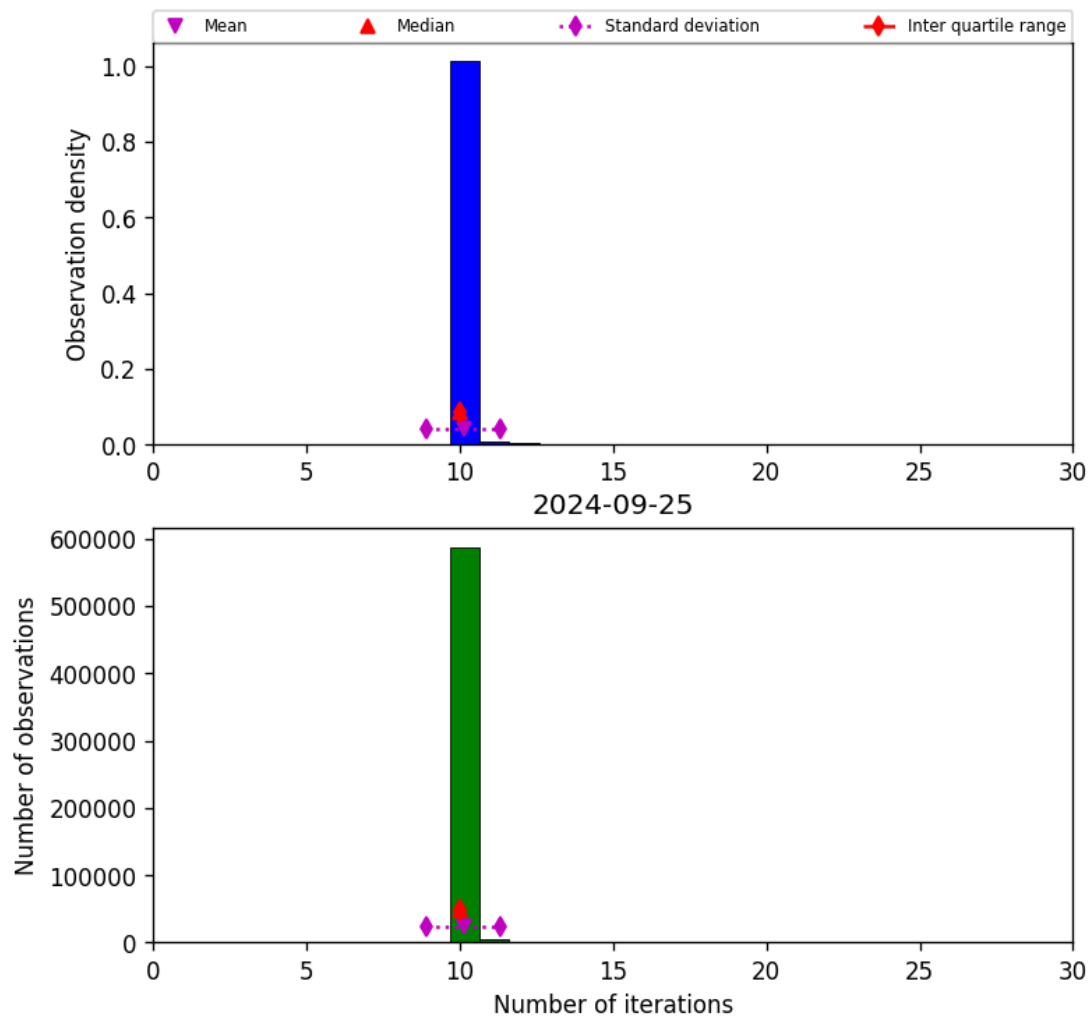
Figure 31: Histogram of “Number of iterations” for 2024-09-24 to 2024-09-26
