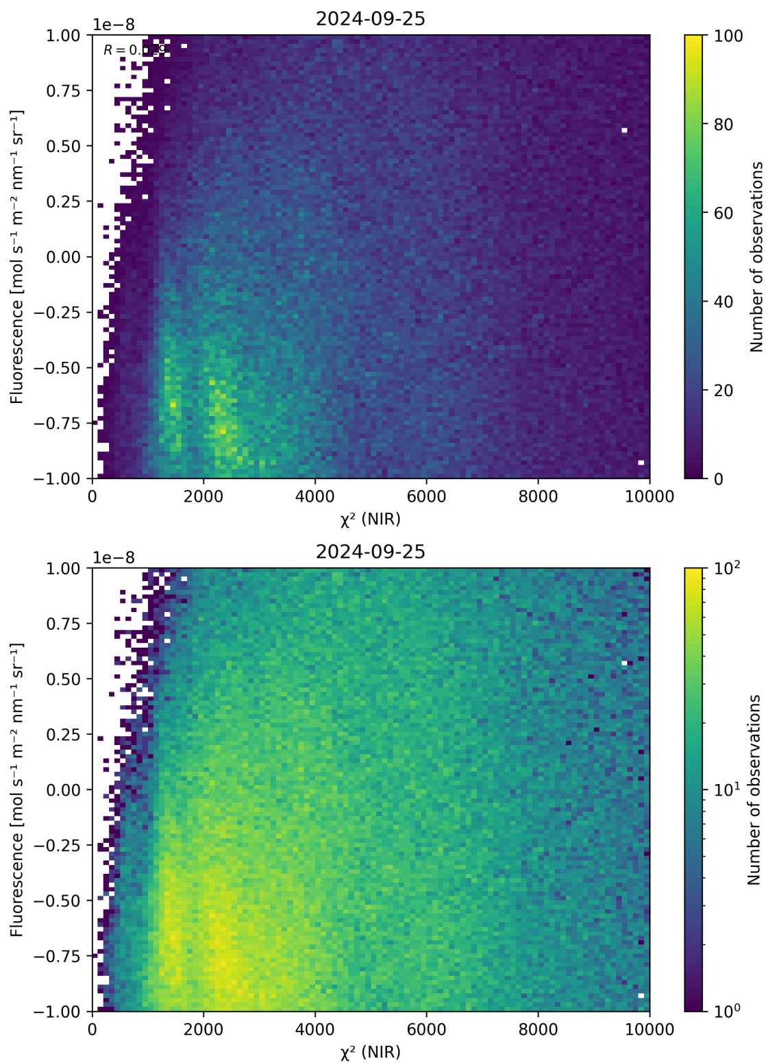
Figure 45: Scatter density plot of “ \chi^2 (NIR)” against “Fluorescence” for 2024-09-24 to 2024-09-26.
