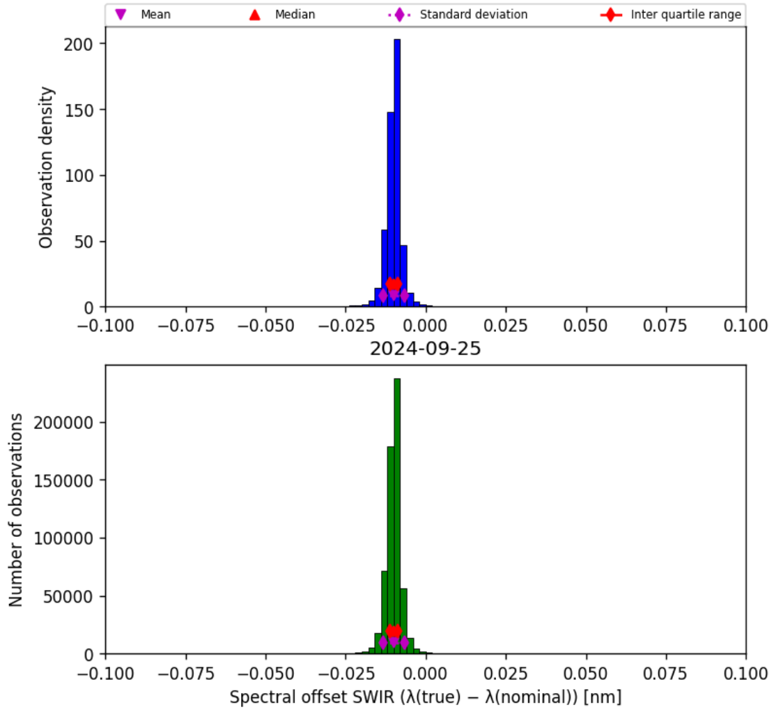
Figure 27: Histogram of “Spectral offset SWIR ( \lambda_{\text{true}} - \lambda_{\text{nominal}} )” for 2024-09-24 to 2024-09-26
