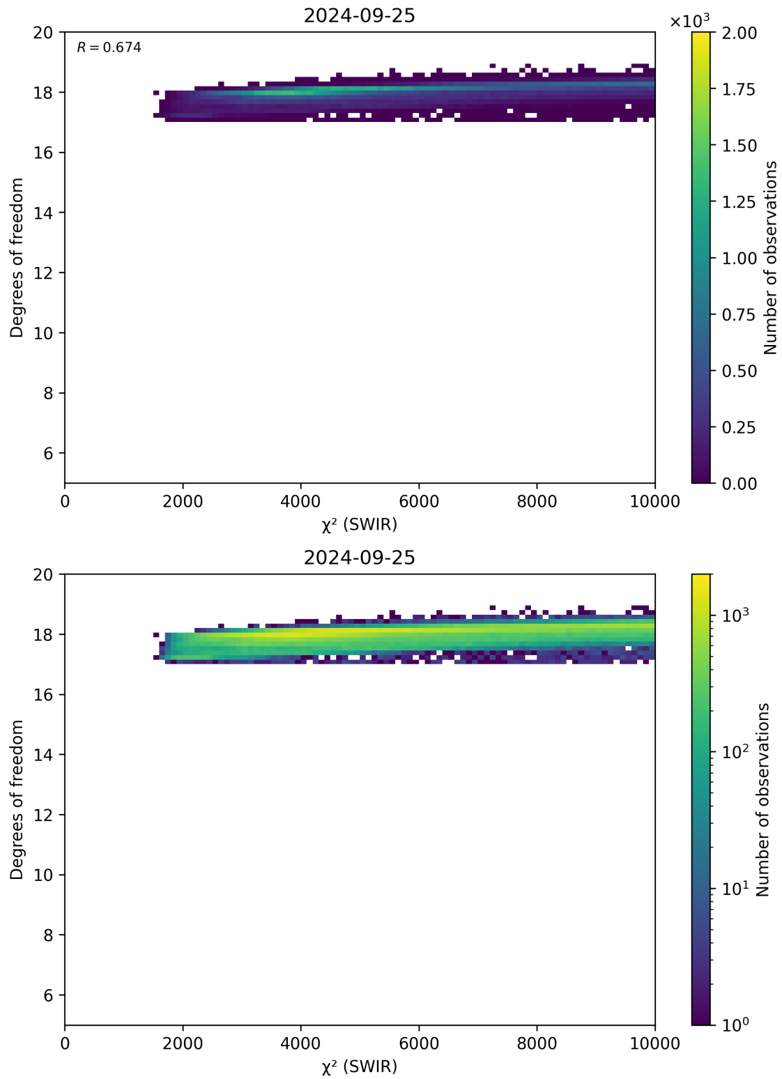
Figure 48: Scatter density plot of “ \chi^2 (SWIR)” against “Degrees of freedom” for 2024-09-24 to 2024-09-26.
