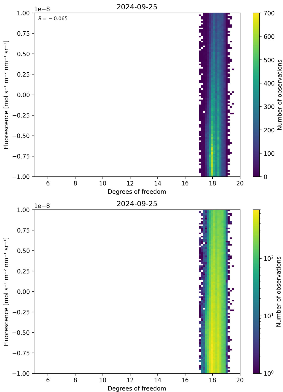
Figure 51: Scatter density plot of “Degrees of freedom” against “Fluorescence” for 2024-09-24 to 2024-09-26.
