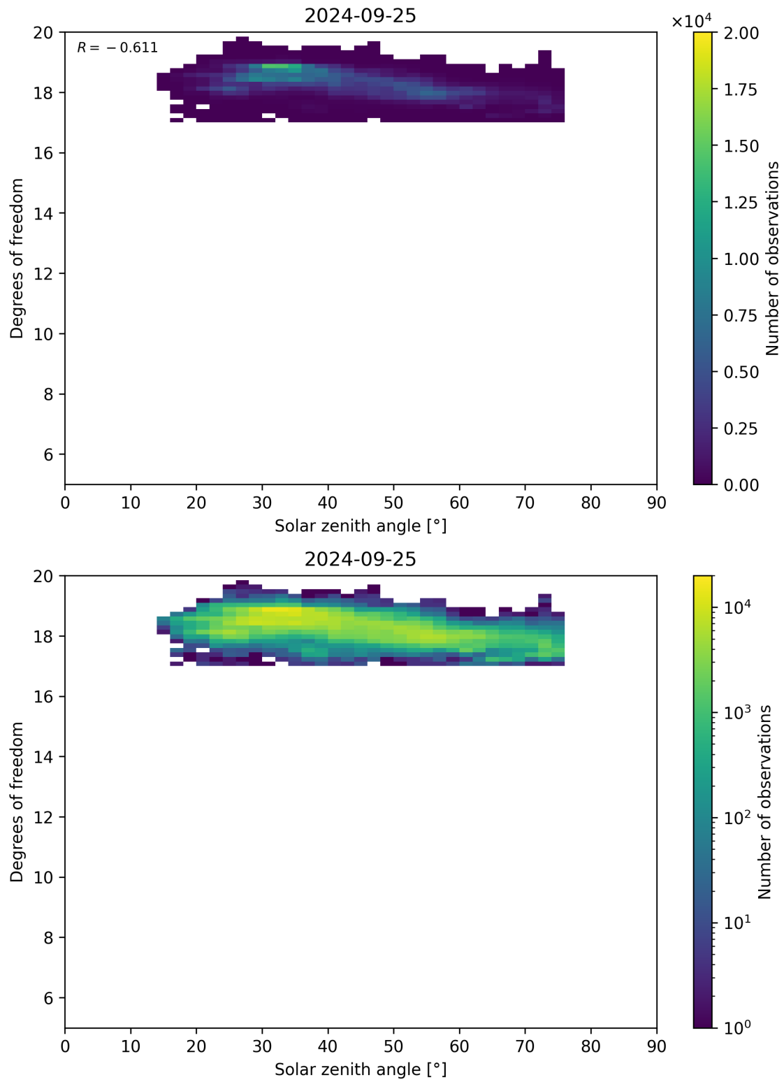
Figure 96: Scatter density plot of “Solar zenith angle” against “Degrees of freedom” for 2024-09-24 to 2024-09-26.
