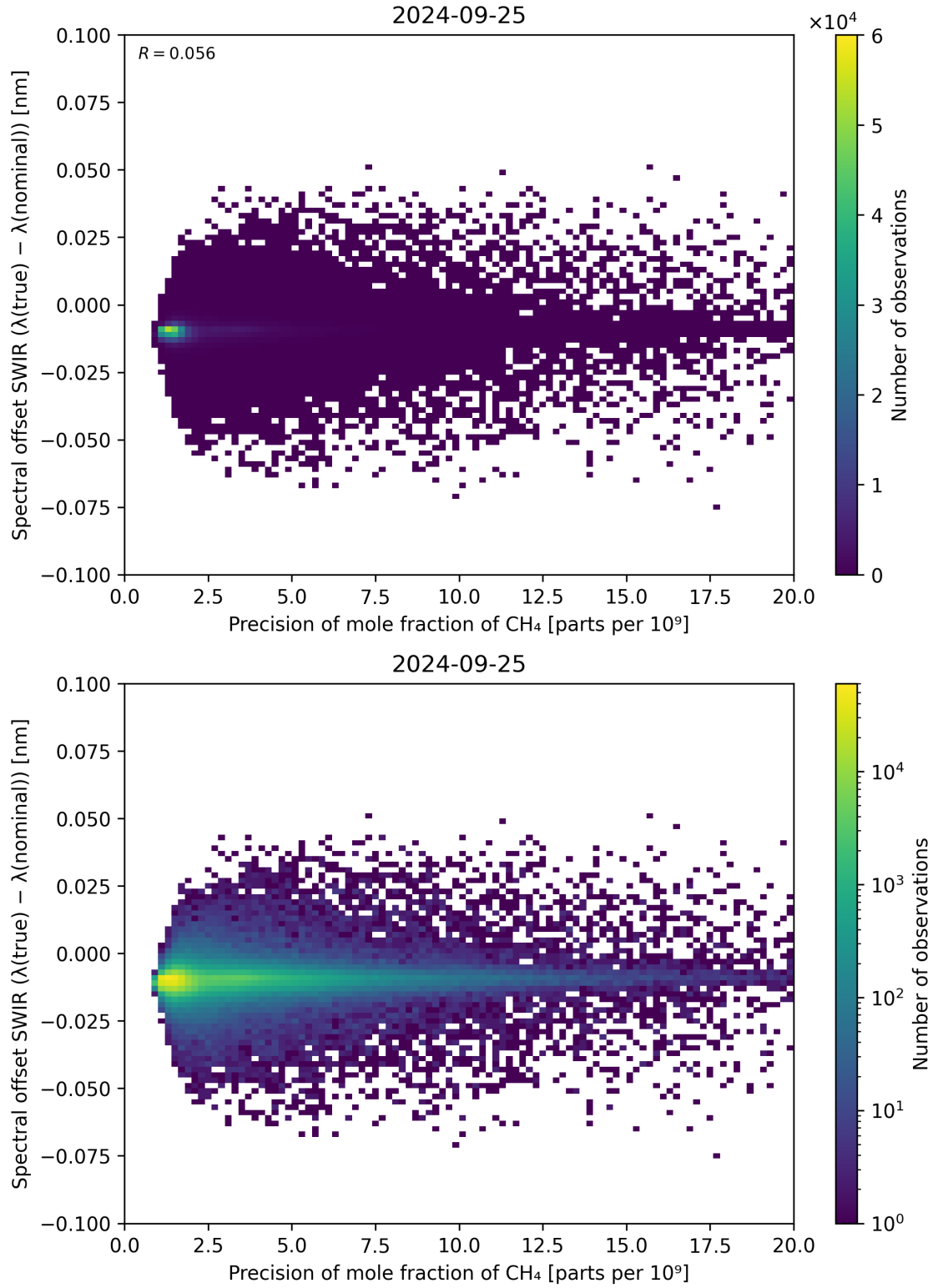
Figure 85: Scatter density plot of “Precision of mole fraction of \text{CH}_4 ” against “Spectral offset SWIR ( \lambda_{\text{true}} - \lambda_{\text{nominal}} )” for 2024-09-24 to 2024-09-26.
