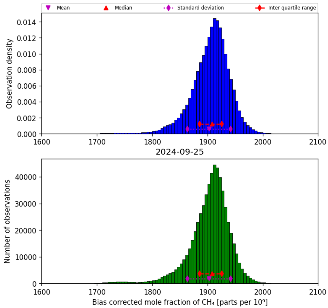
Figure 25: Histogram of “Bias corrected mole fraction of CH 4 ” for 2024-09-24 to 2024-09-26
