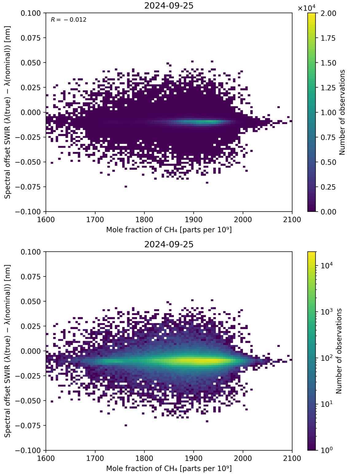
Figure 86: Scatter density plot of “Mole fraction of CH 4 ” against “Spectral offset SWIR ( \lambda_{\text{true}} - \lambda_{\text{nominal}} )” for 2024-09-24 to 2024-09-26.
