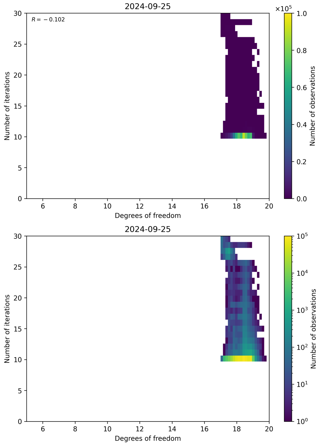
Figure 52: Scatter density plot of “Degrees of freedom” against “Number of iterations” for 2024-09-24 to 2024-09-26.
