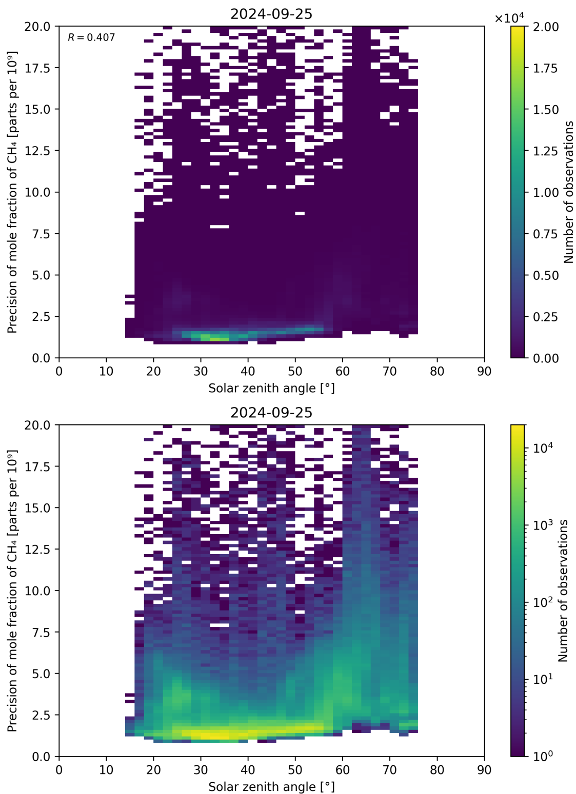
Figure 101: Scatter density plot of “Solar zenith angle” against “Precision of mole fraction of \text{CH}_4 ” for 2024-09-24 to 2024-09-26.
