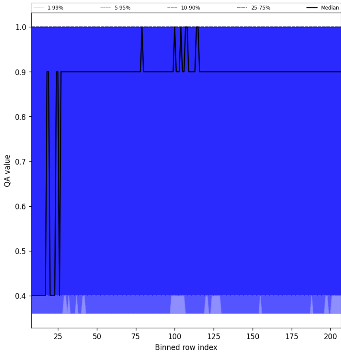
Figure 33: Along track statistics of “QA value” for 2024-09-24 to 2024-09-26
