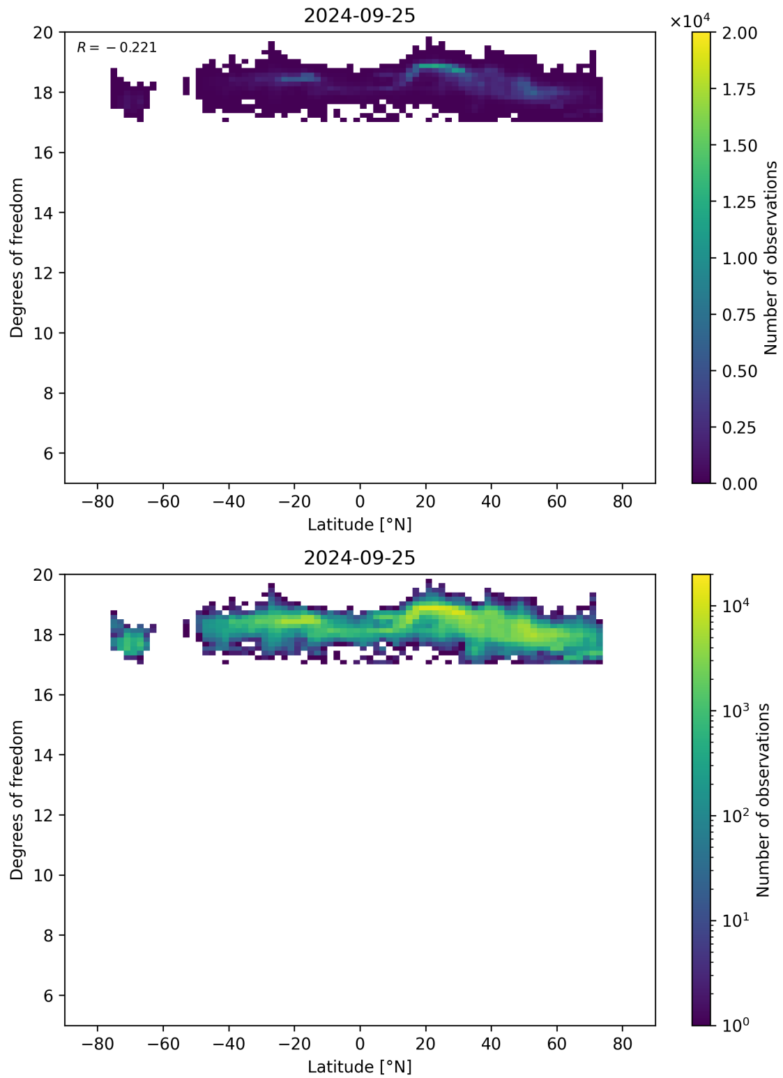
Figure 55: Scatter density plot of “Latitude” against “Degrees of freedom” for 2024-09-24 to 2024-09-26.
