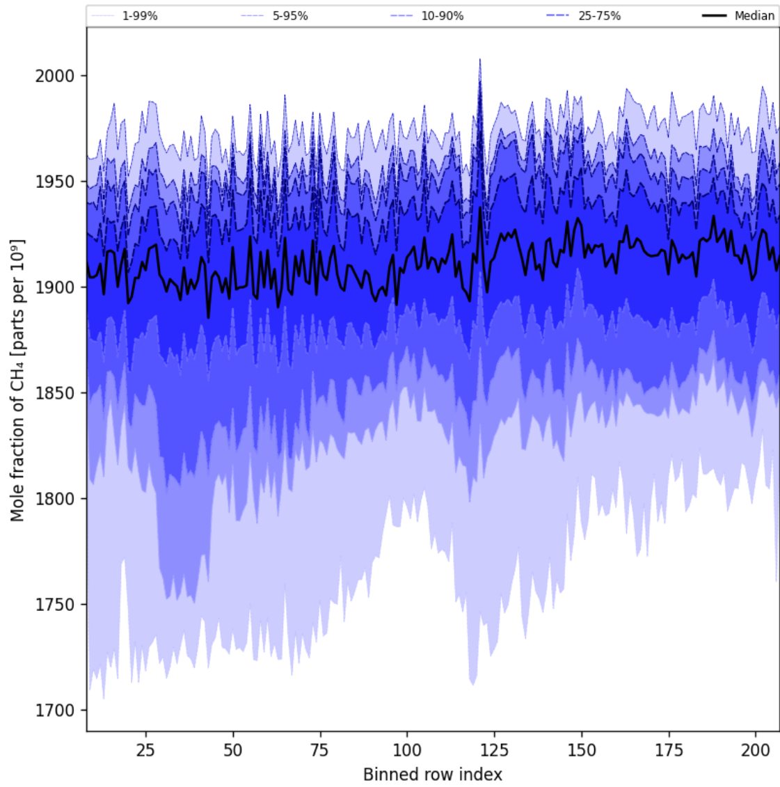
Figure 34: Along track statistics of “Mole fraction of CH 4 ” for 2024-09-24 to 2024-09-26
