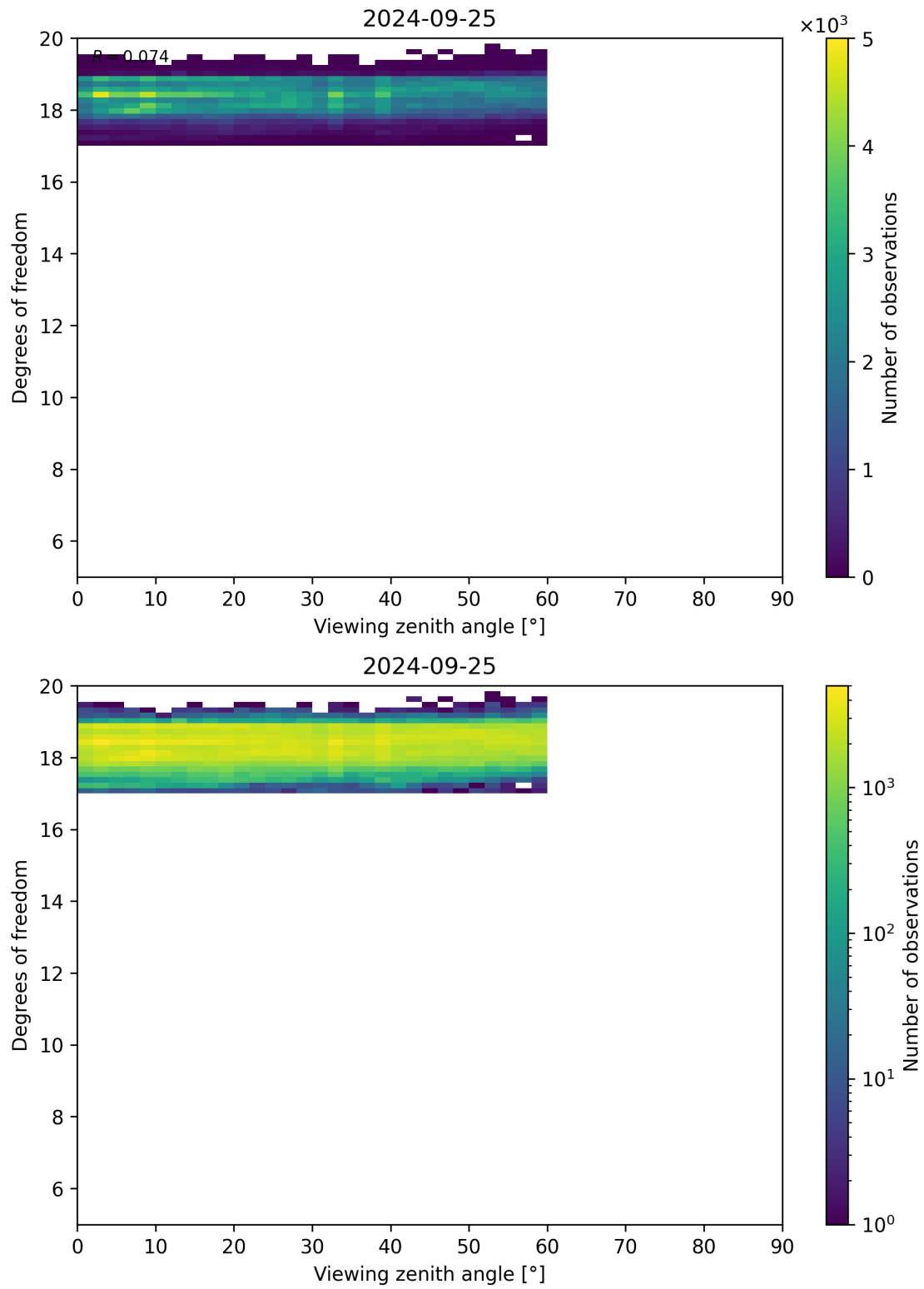
Figure 107: Scatter density plot of “Viewing zenith angle” against “Degrees of freedom” for 2024-09-24 to 2024-09-26.
