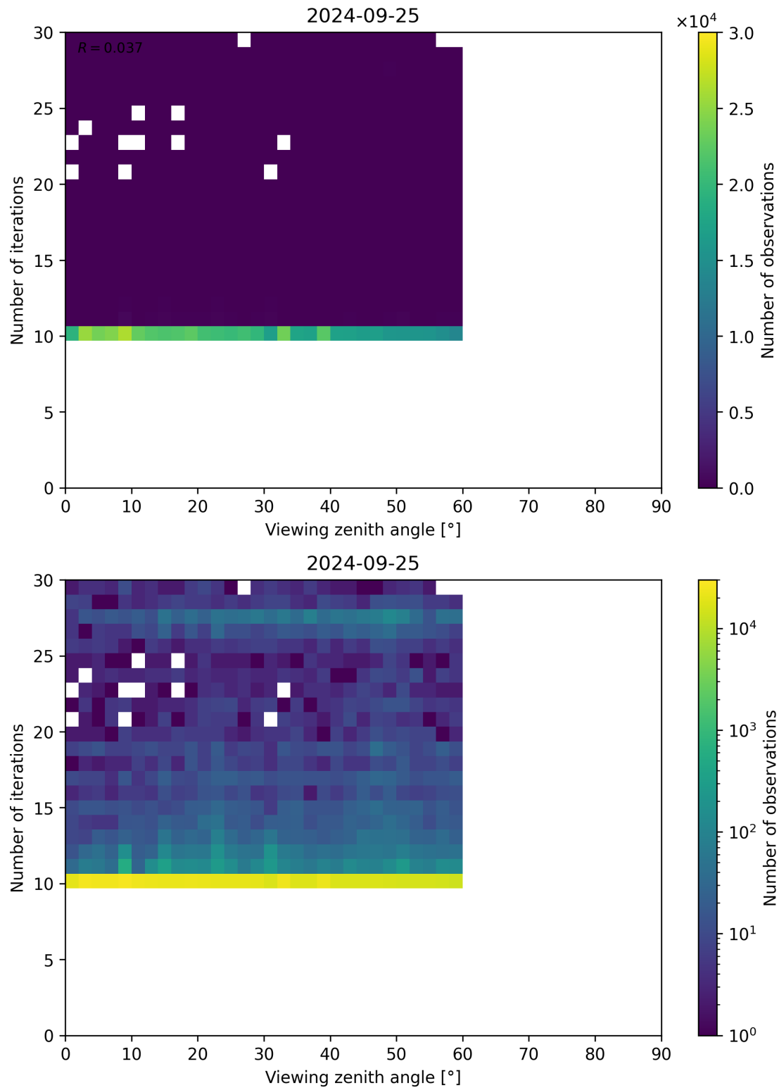
Figure 113: Scatter density plot of “Viewing zenith angle” against “Number of iterations” for 2024-09-24 to 2024-09-26.
