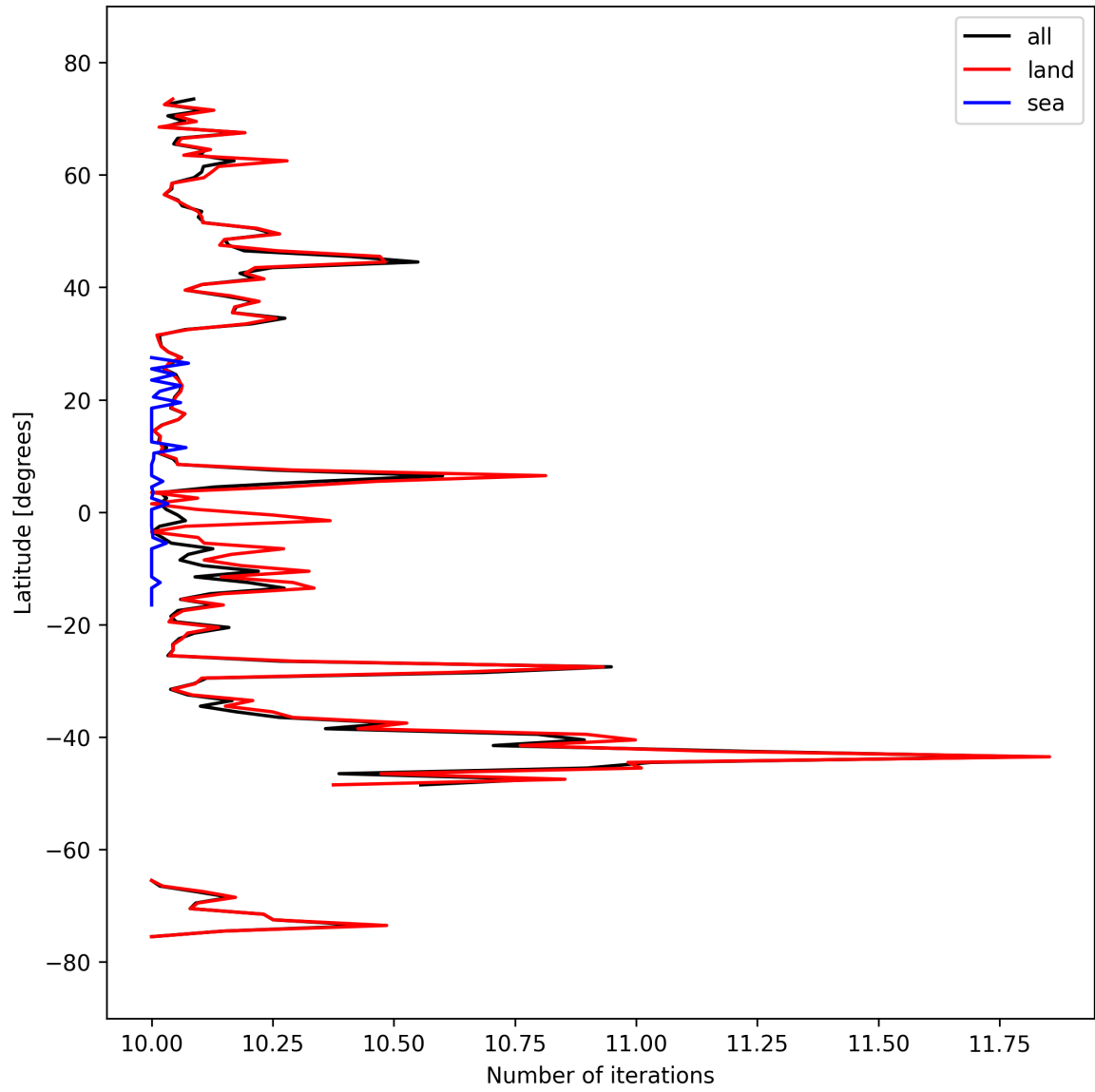
Figure 20: Zonal average of “Number of iterations” for 2024-09-24 to 2024-09-26.
