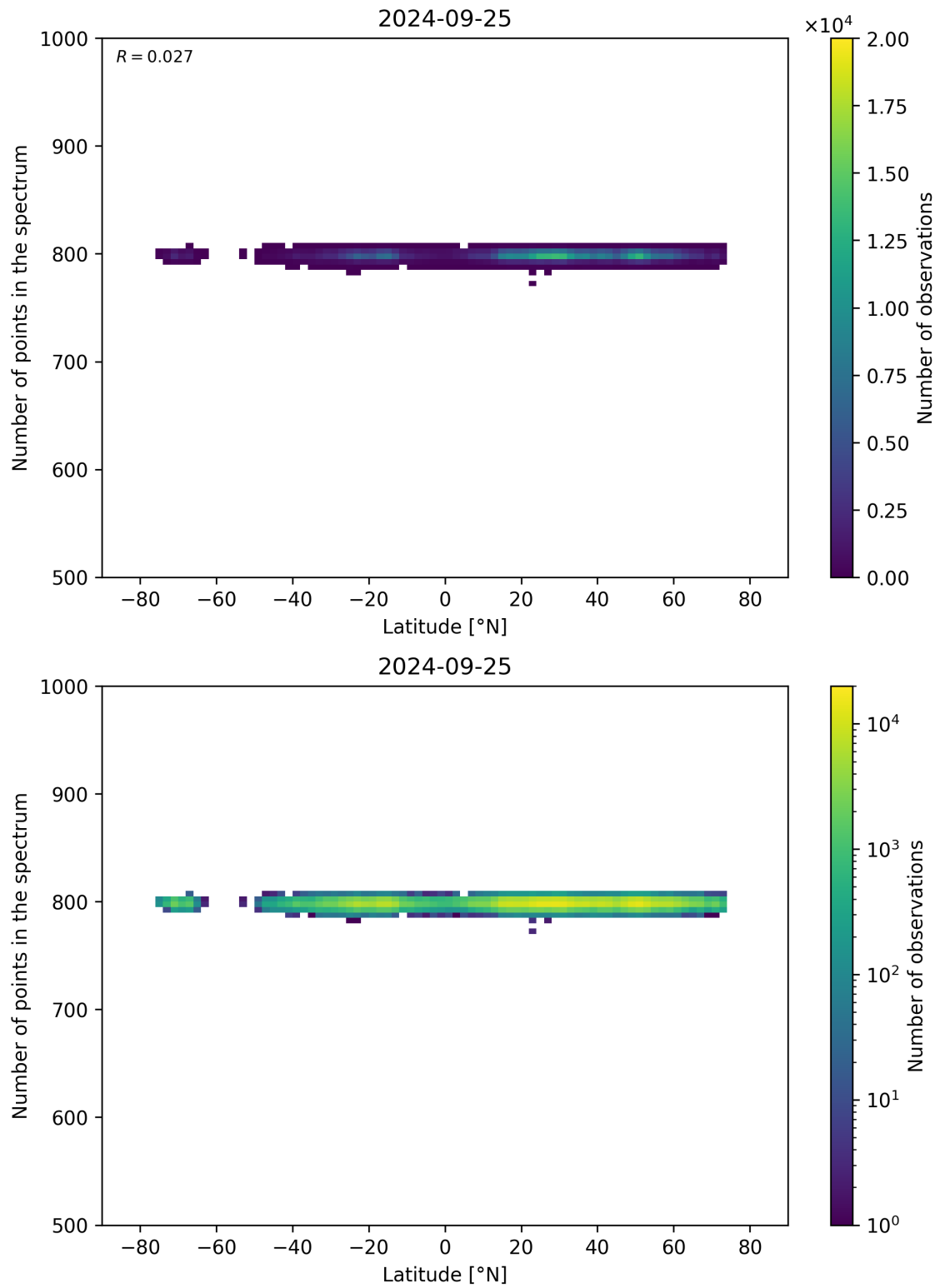
Figure 61: Scatter density plot of “Latitude” against “Number of points in the spectrum” for 2024-09-24 to 2024-09-26.
