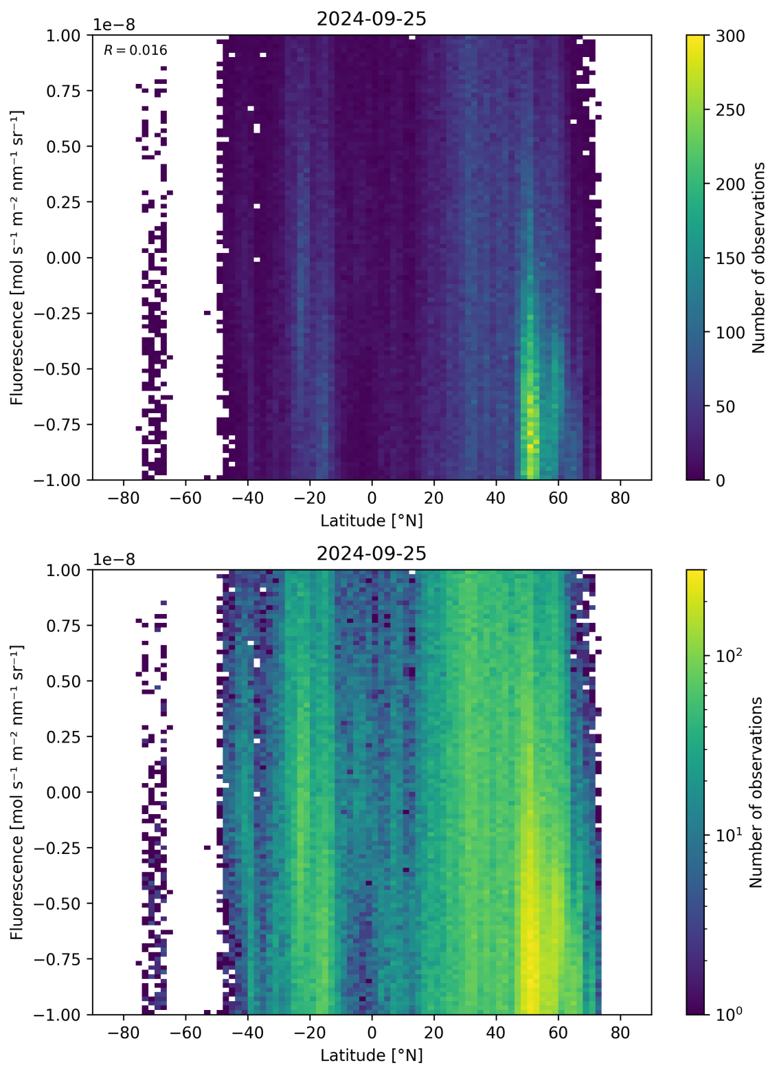
Figure 56: Scatter density plot of “Latitude” against “Fluorescence” for 2024-09-24 to 2024-09-26.
