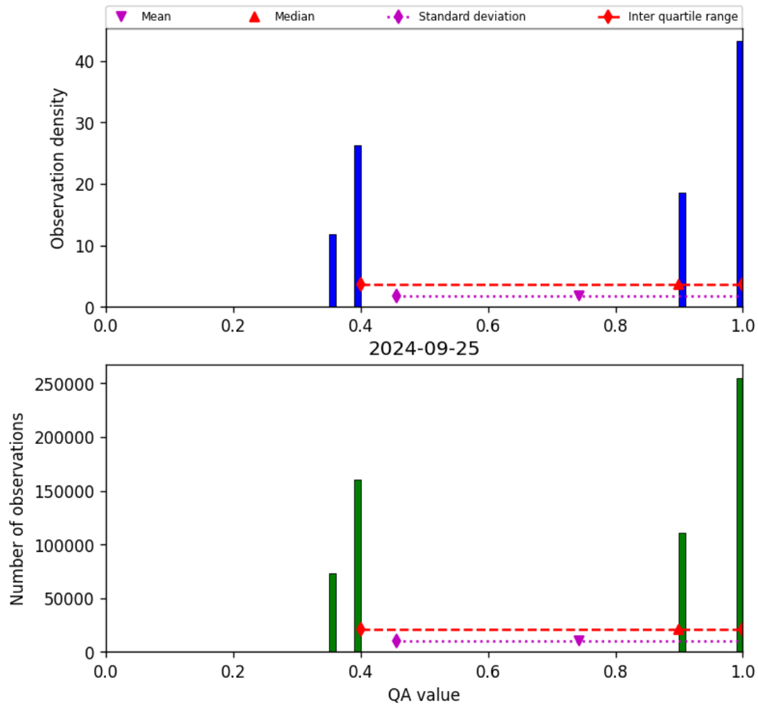
Figure 22: Histogram of “QA value” for 2024-09-24 to 2024-09-26
