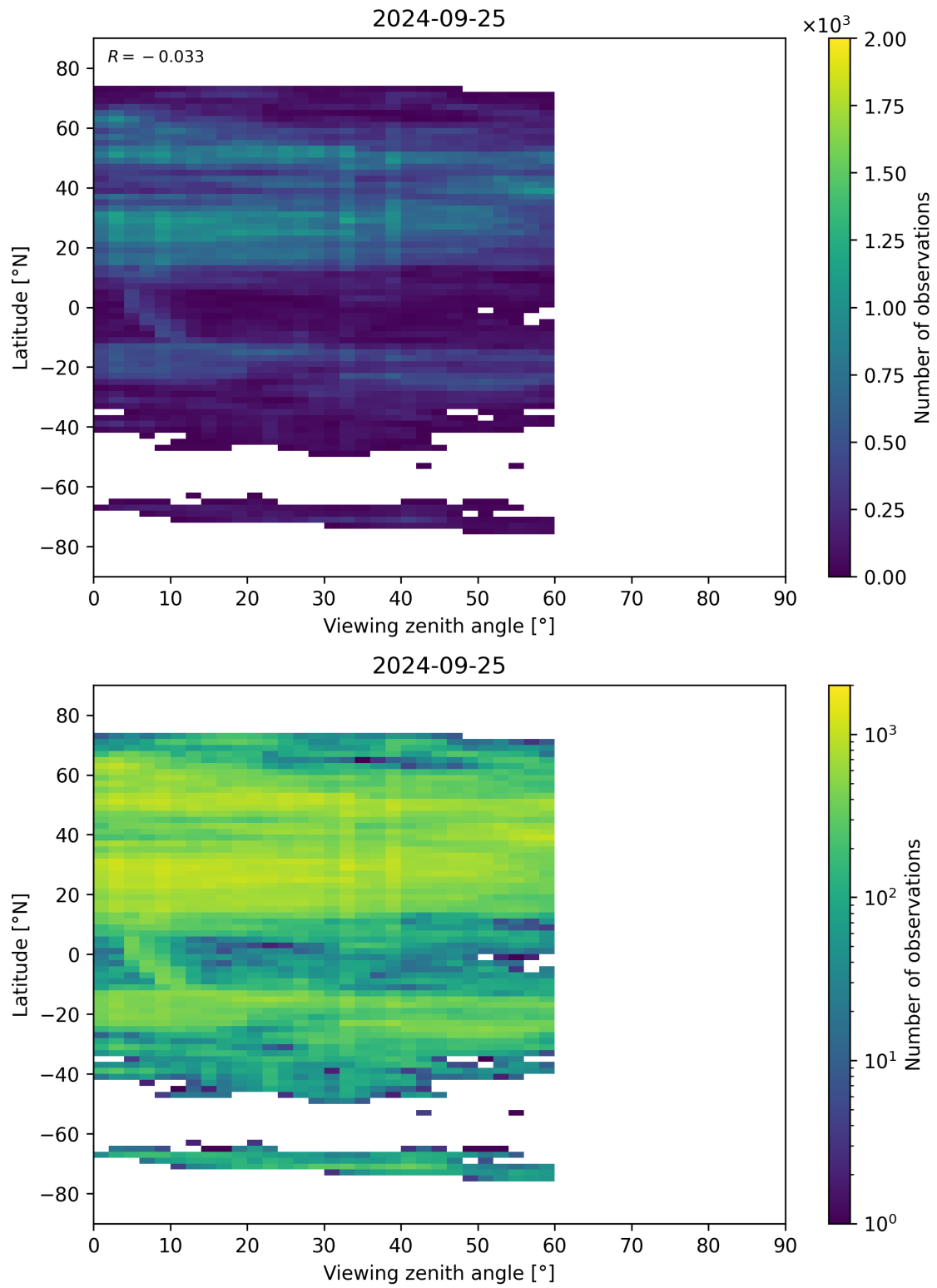
Figure 109: Scatter density plot of “Viewing zenith angle” against “Latitude” for 2024-09-24 to 2024-09-26.
