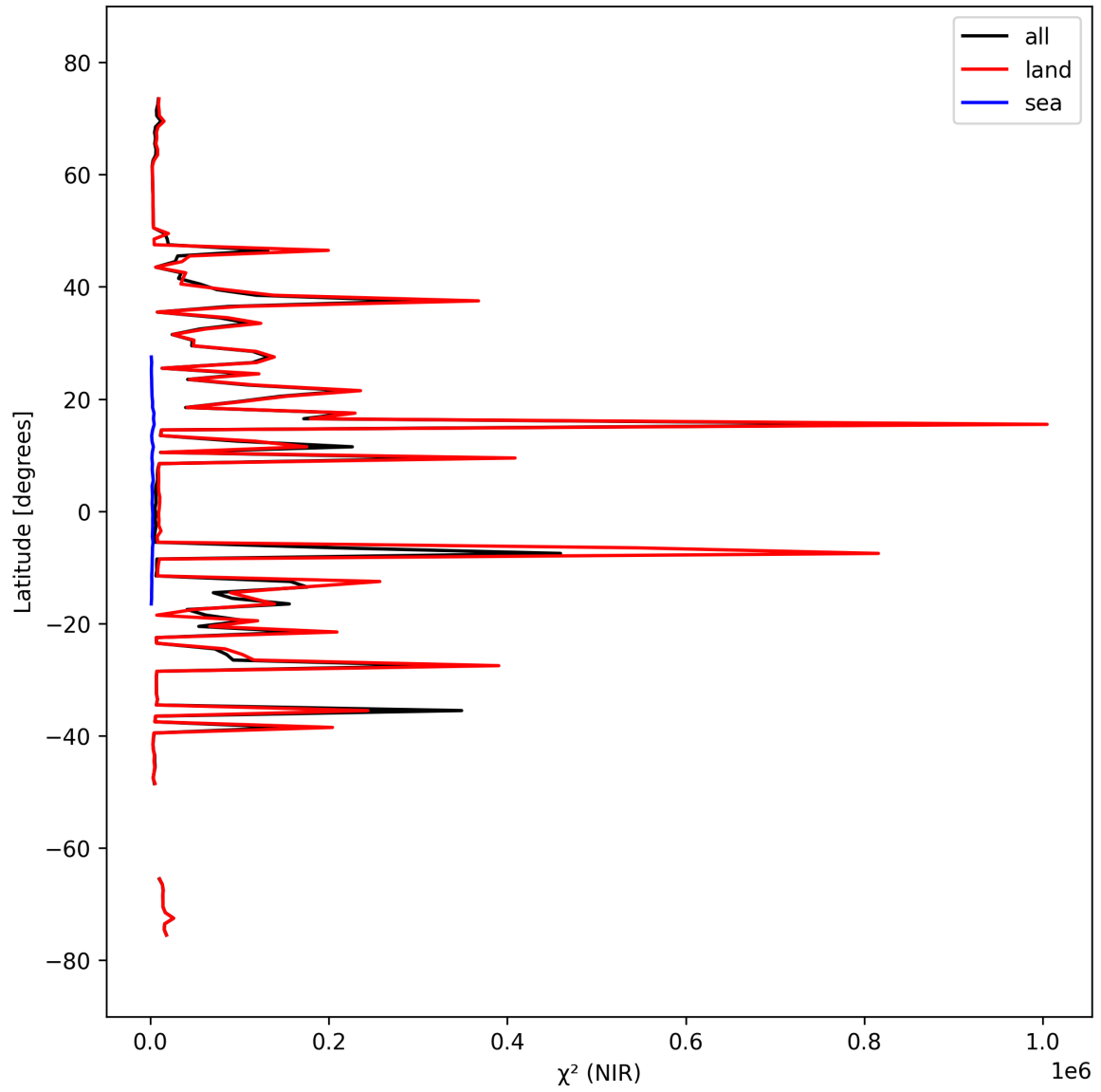
Figure 18: Zonal average of “ \chi^2 (NIR)” for 2024-09-24 to 2024-09-26.
