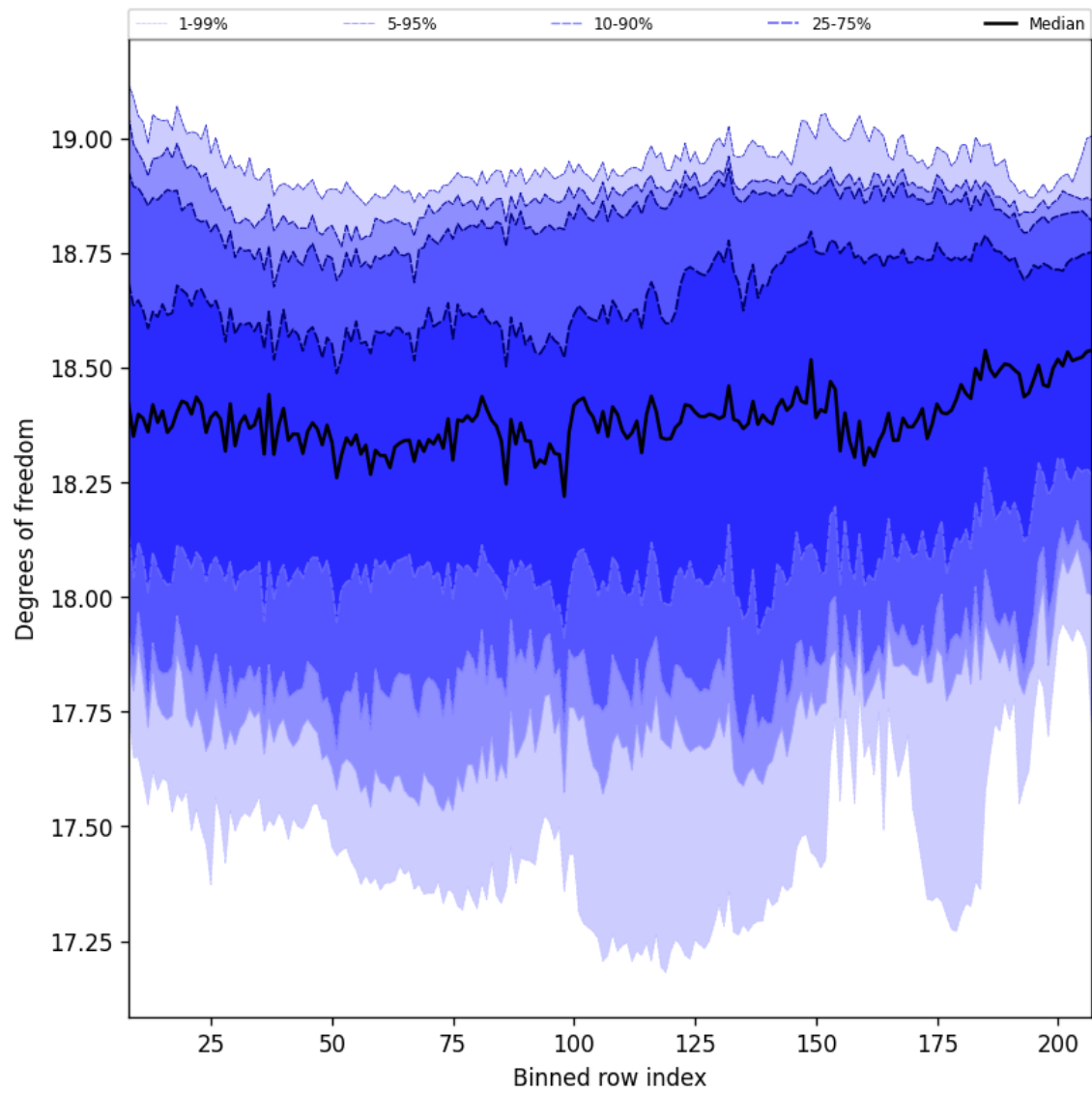
Figure 41: Along track statistics of “Degrees of freedom” for 2024-09-24 to 2024-09-26
