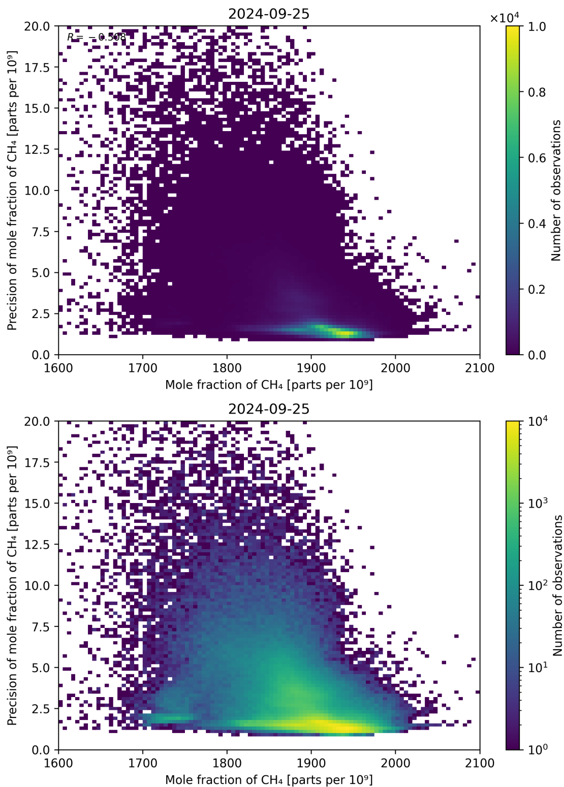
Figure 75: Scatter density plot of “Mole fraction of CH 4 ” against “Precision of mole fraction of CH 4 ” for 2024-09-24 to 2024-09-26.
