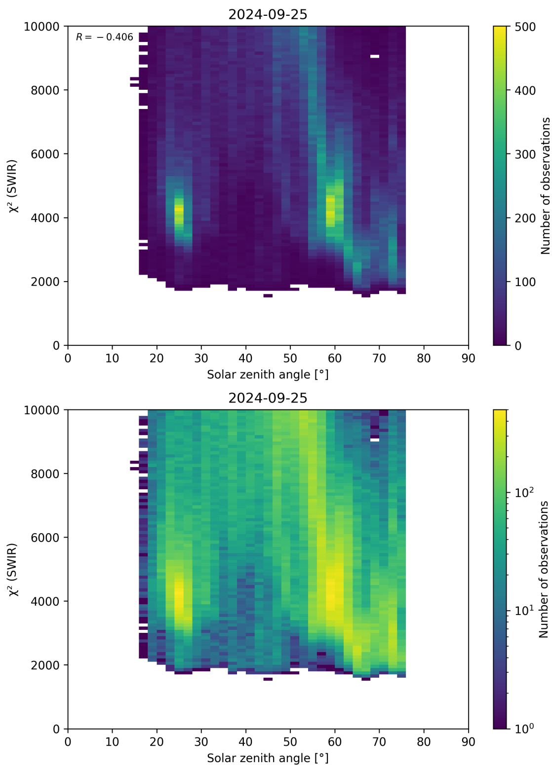
Figure 95: Scatter density plot of “Solar zenith angle” against “ \chi^2 (SWIR)” for 2024-09-24 to 2024-09-26.
