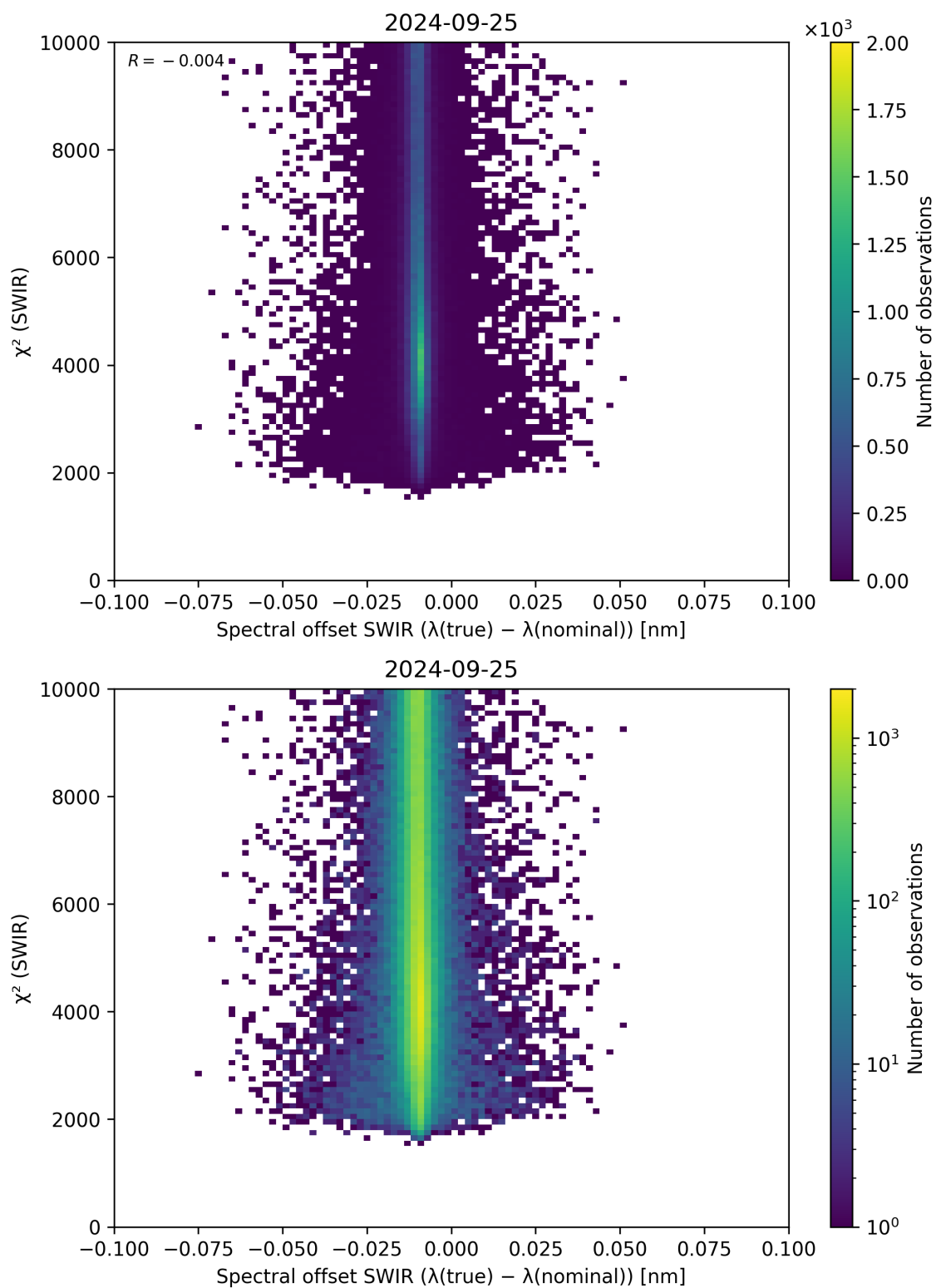
Figure 118: Scatter density plot of “Spectral offset SWIR ( \lambda_{\text{true}} - \lambda_{\text{nominal}} )” against “ \chi^2 (SWIR)” for 2024-09-24 to 2024-09-26.
