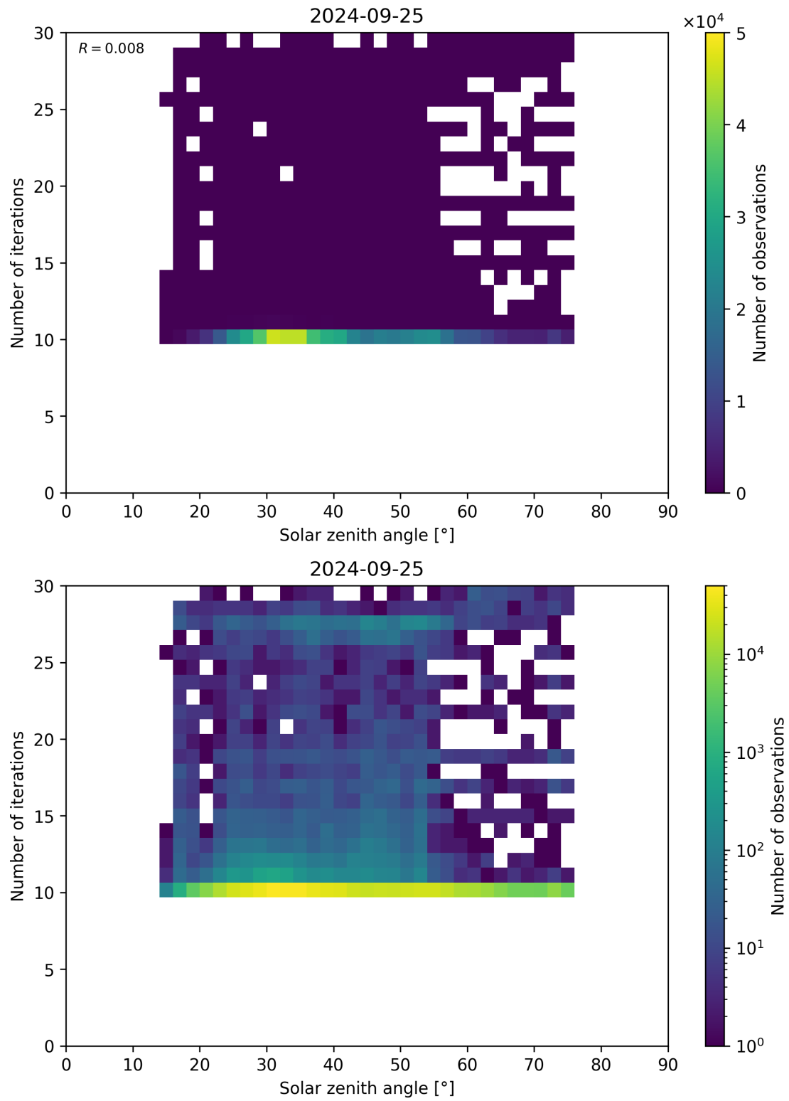
Figure 102: Scatter density plot of “Solar zenith angle” against “Number of iterations” for 2024-09-24 to 2024-09-26.
