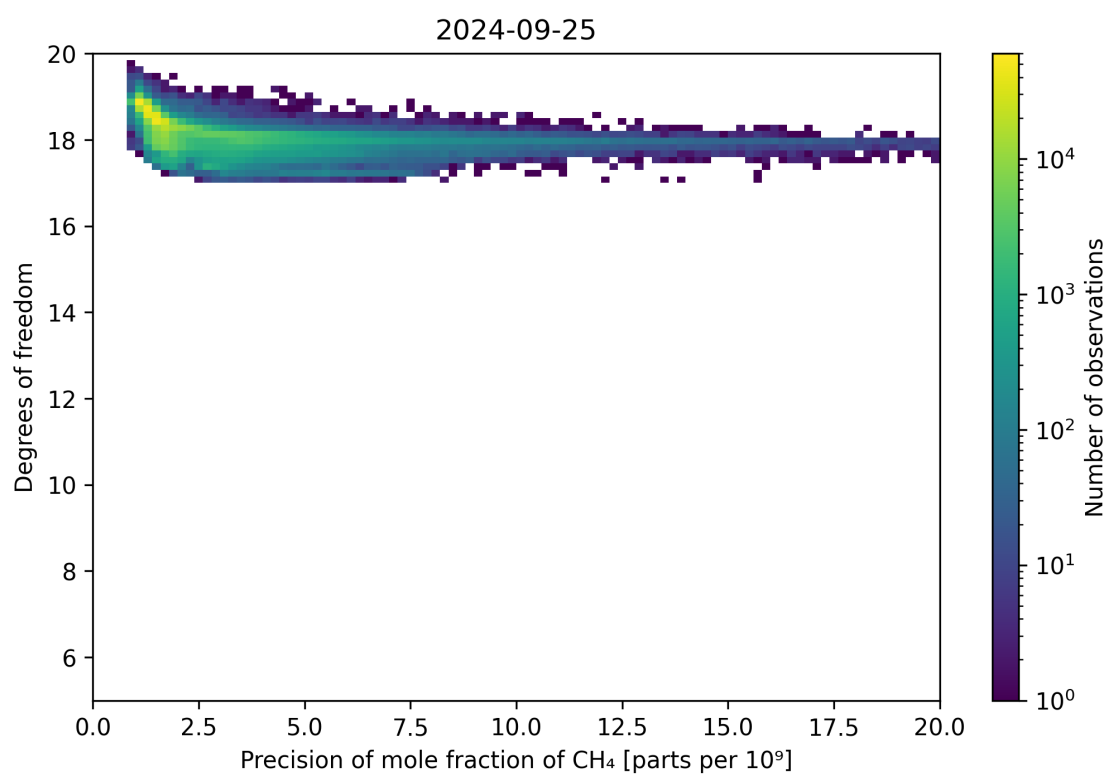
Figure 80: Scatter density plot of “Precision of mole fraction of CH 4 ” against “Degrees of freedom” for 2024-09-24 to 2024-09-26.
