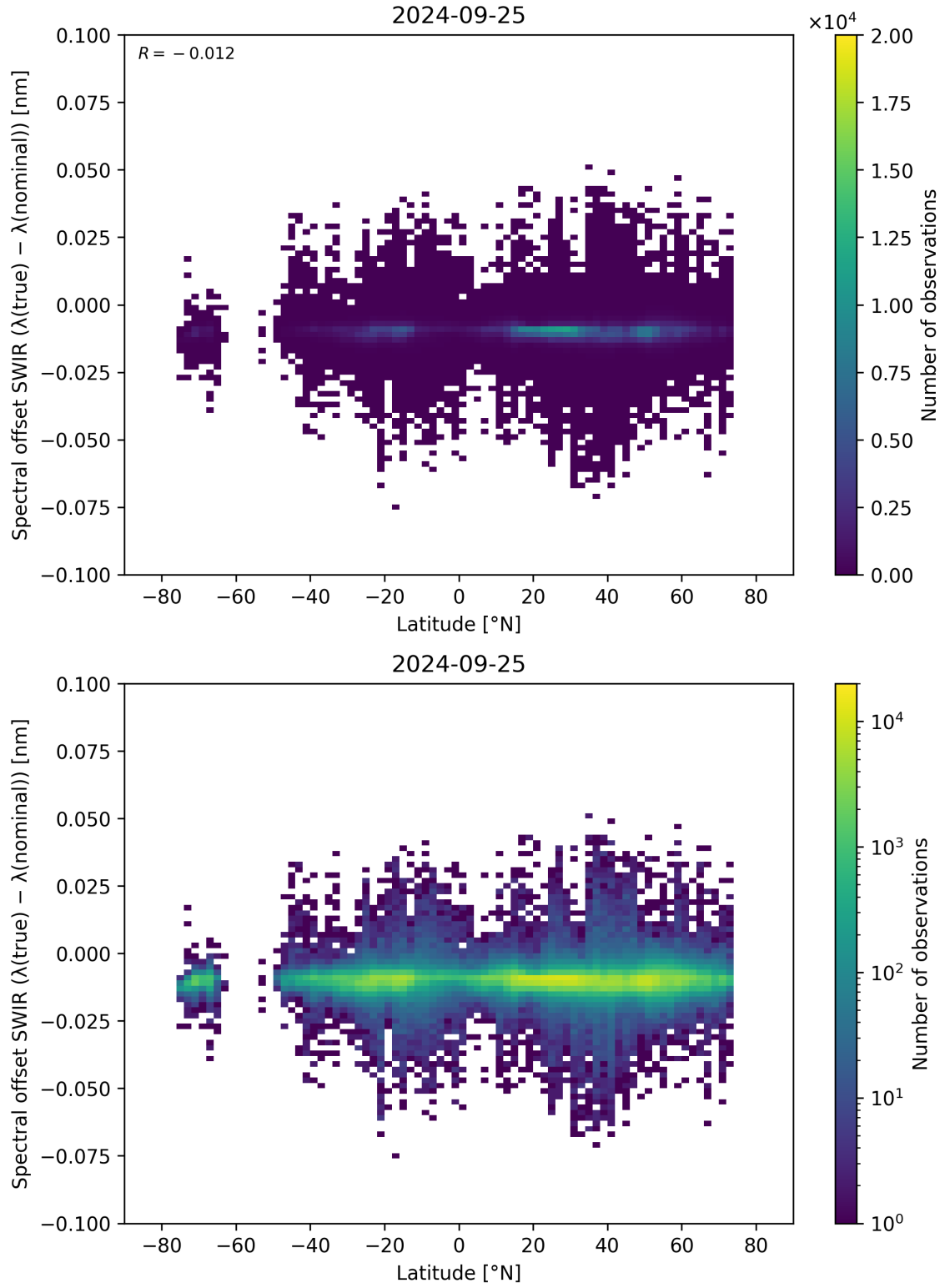
Figure 62: Scatter density plot of “Latitude” against “Spectral offset SWIR ( \lambda_{\text{true}} - \lambda_{\text{nominal}} )” for 2024-09-24 to 2024-09-26.
