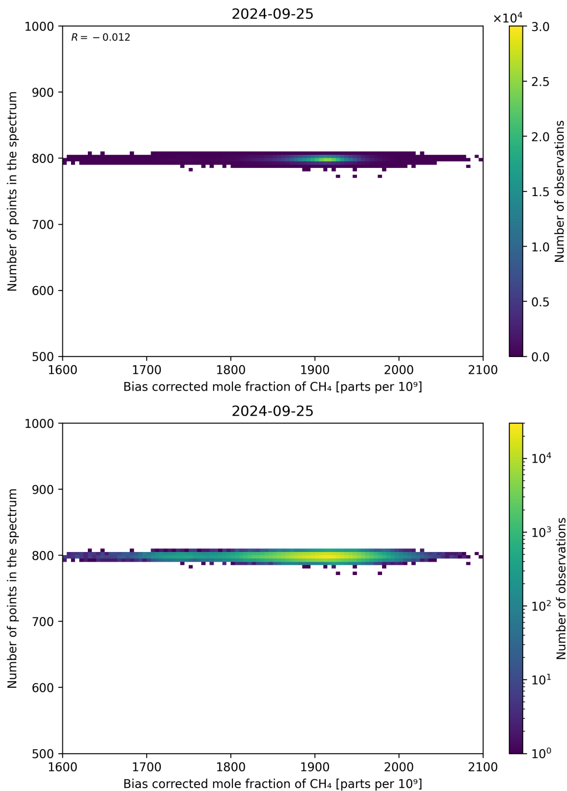
Figure 68: Scatter density plot of “Bias corrected mole fraction of CH 4 ” against “Number of points in the spectrum” for 2024-09-24 to 2024-09-26.
