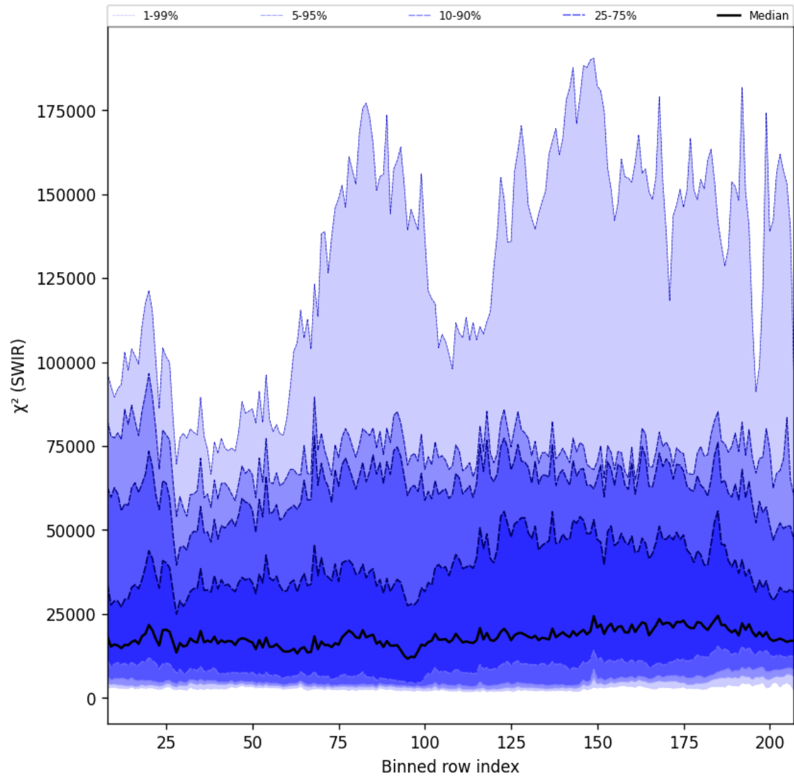
Figure 39: Along track statistics of “ \chi^2 (SWIR)” for 2024-09-24 to 2024-09-26
