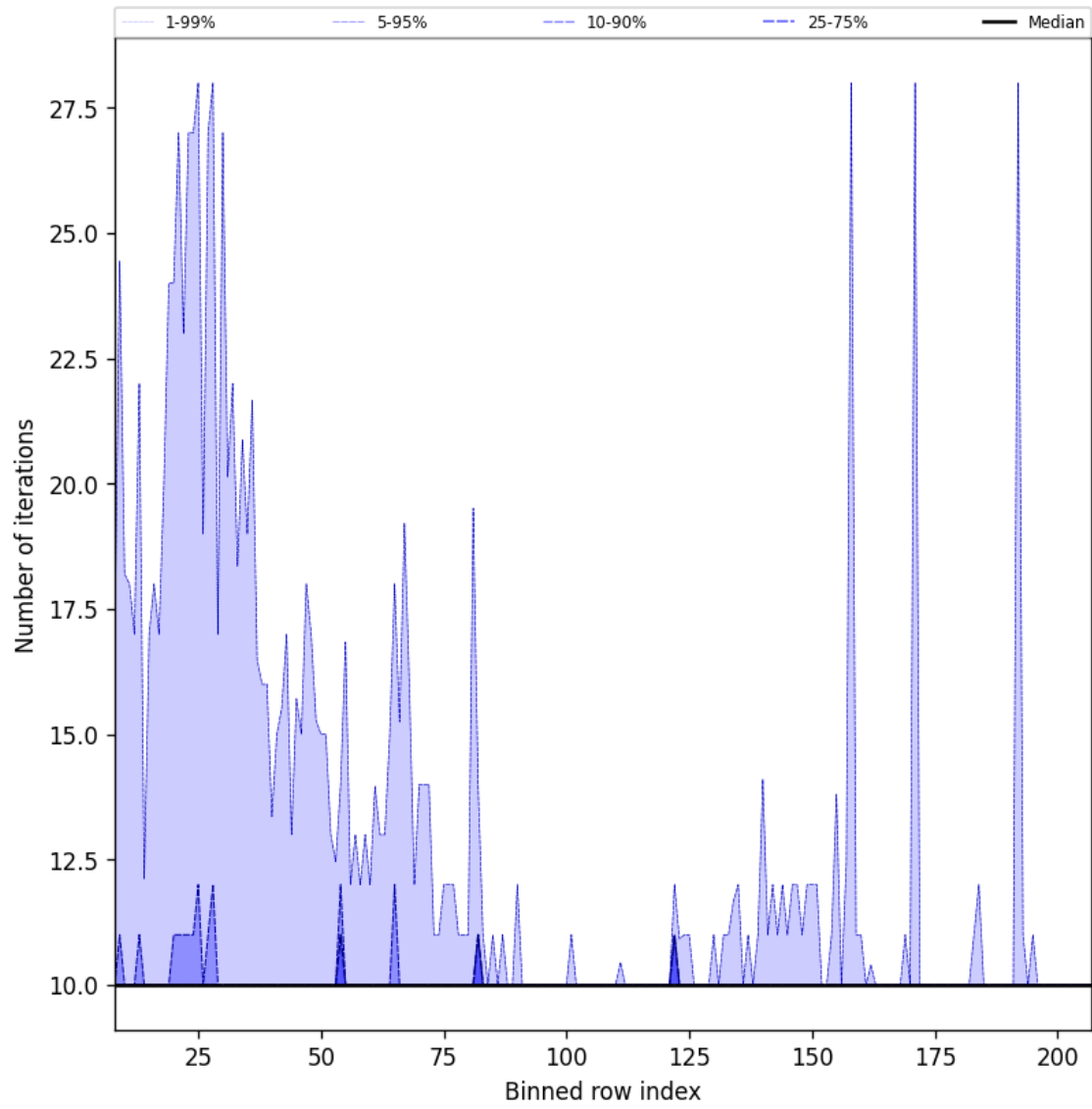
Figure 42: Along track statistics of “Number of iterations” for 2024-09-24 to 2024-09-26
