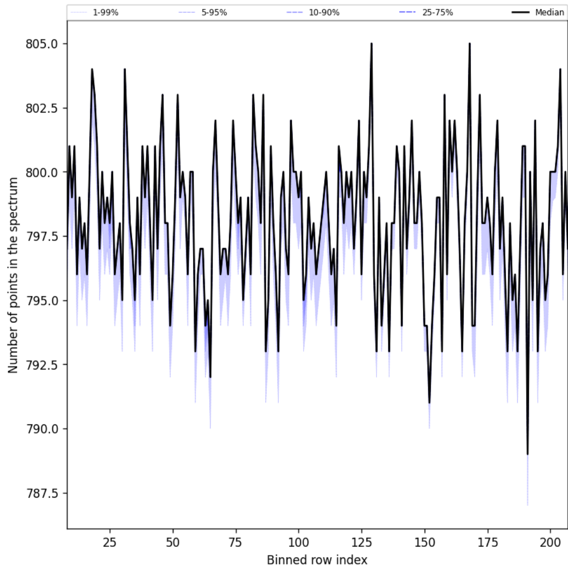
Figure 37: Along track statistics of “Number of points in the spectrum” for 2024-09-24 to 2024-09-26
