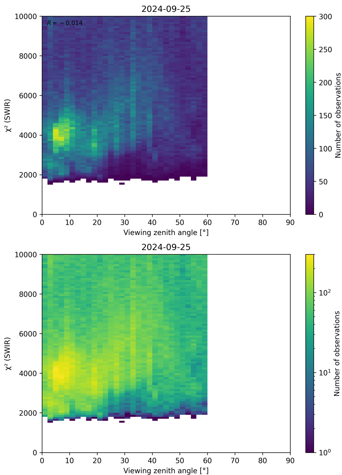
Figure 106: Scatter density plot of “Viewing zenith angle” against “ \chi^2 (SWIR)” for 2024-09-24 to 2024-09-26.
