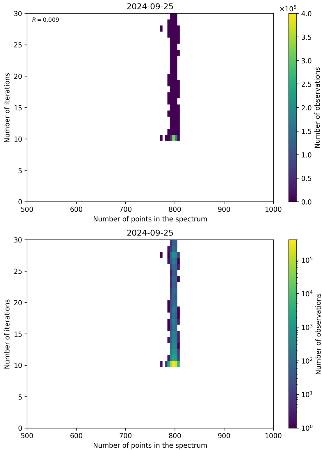
Figure 92: Scatter density plot of “Number of points in the spectrum” against “Number of iterations” for 2024-09-24 to 2024-09-26.
