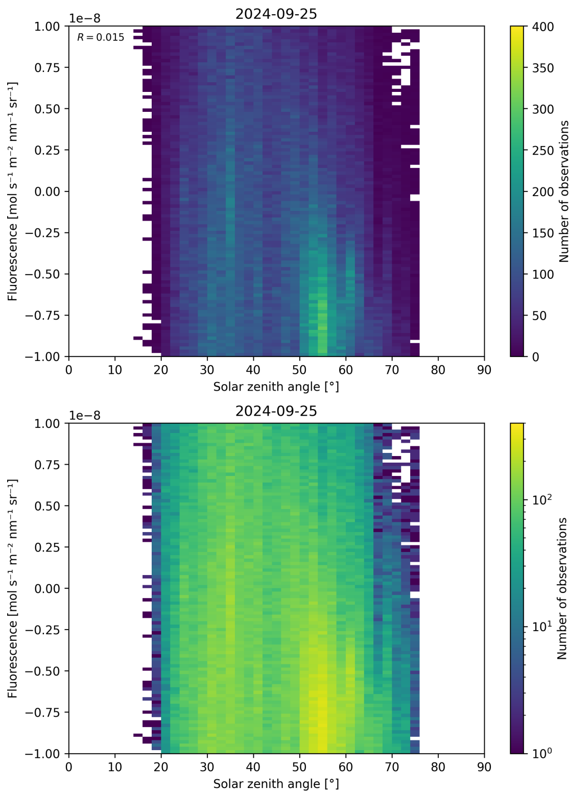
Figure 97: Scatter density plot of “Solar zenith angle” against “Fluorescence” for 2024-09-24 to 2024-09-26.
