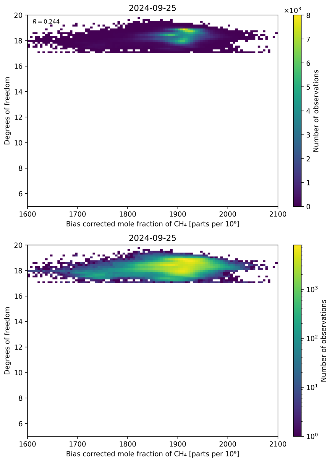
Figure 65: Scatter density plot of “Bias corrected mole fraction of CH 4 ” against “Degrees of freedom” for 2024-09-24 to 2024-09-26.
