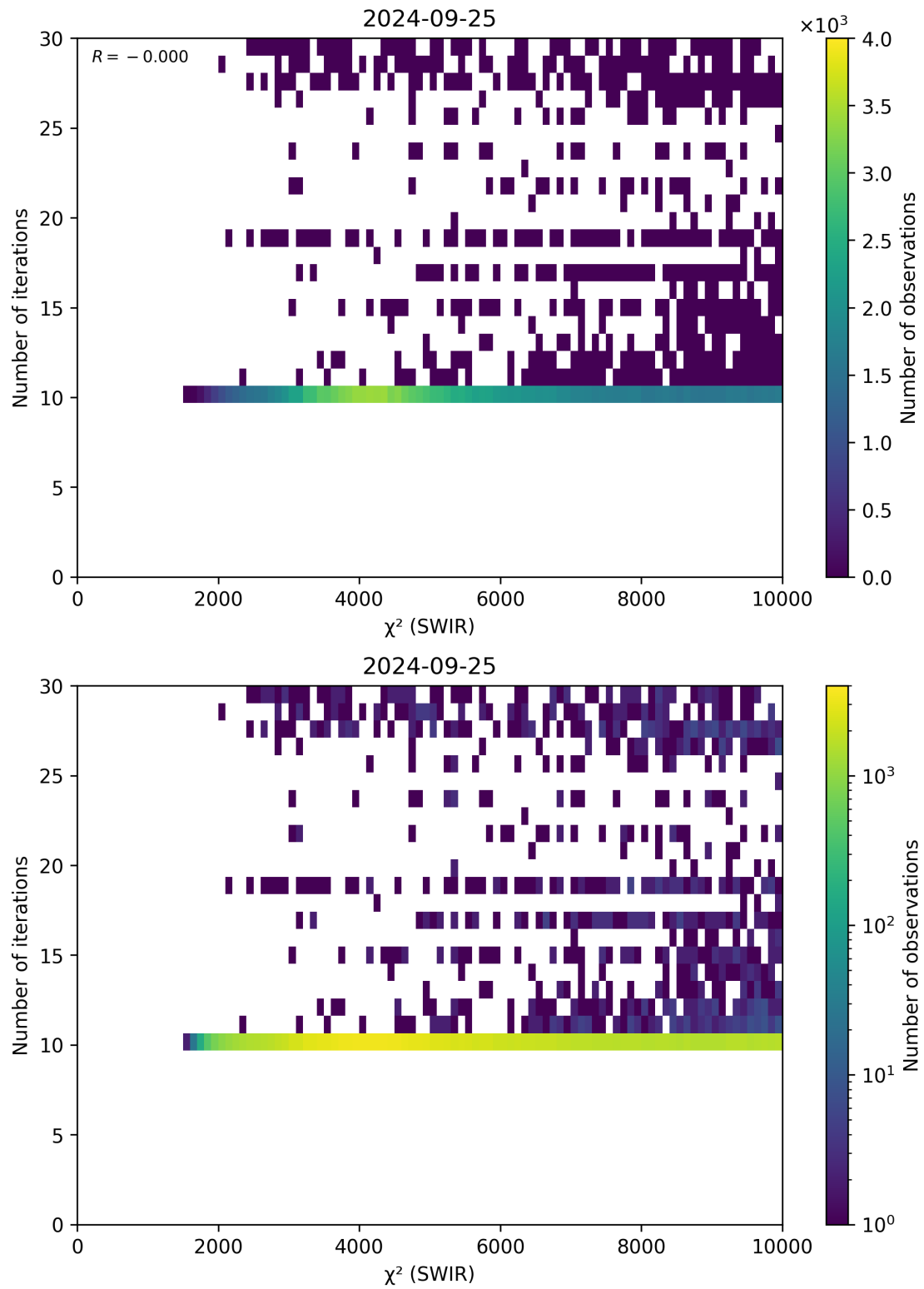
Figure 50: Scatter density plot of “ \chi^2 (SWIR)” against “Number of iterations” for 2024-09-24 to 2024-09-26.
