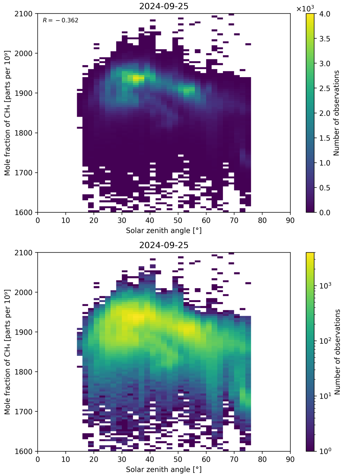
Figure 99: Scatter density plot of “Solar zenith angle” against “Mole fraction of CH 4 ” for 2024-09-24 to 2024-09-26.
