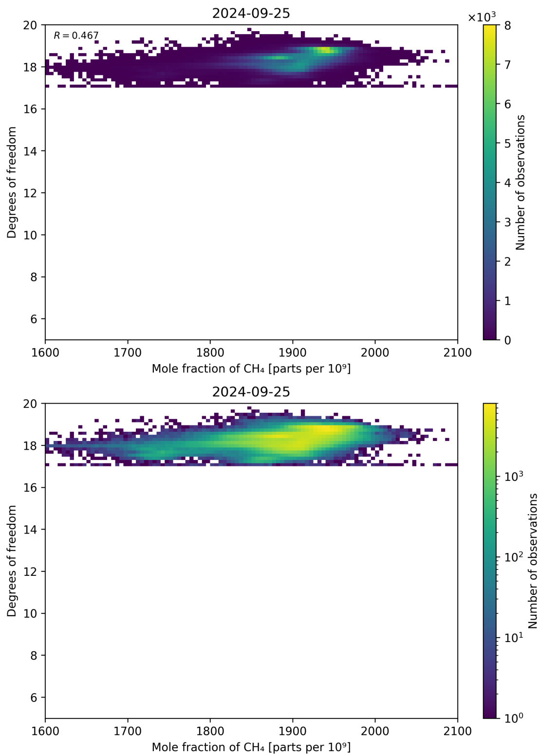
Figure 72: Scatter density plot of “Mole fraction of CH 4 ” against “Degrees of freedom” for 2024-09-24 to 2024-09-26.
