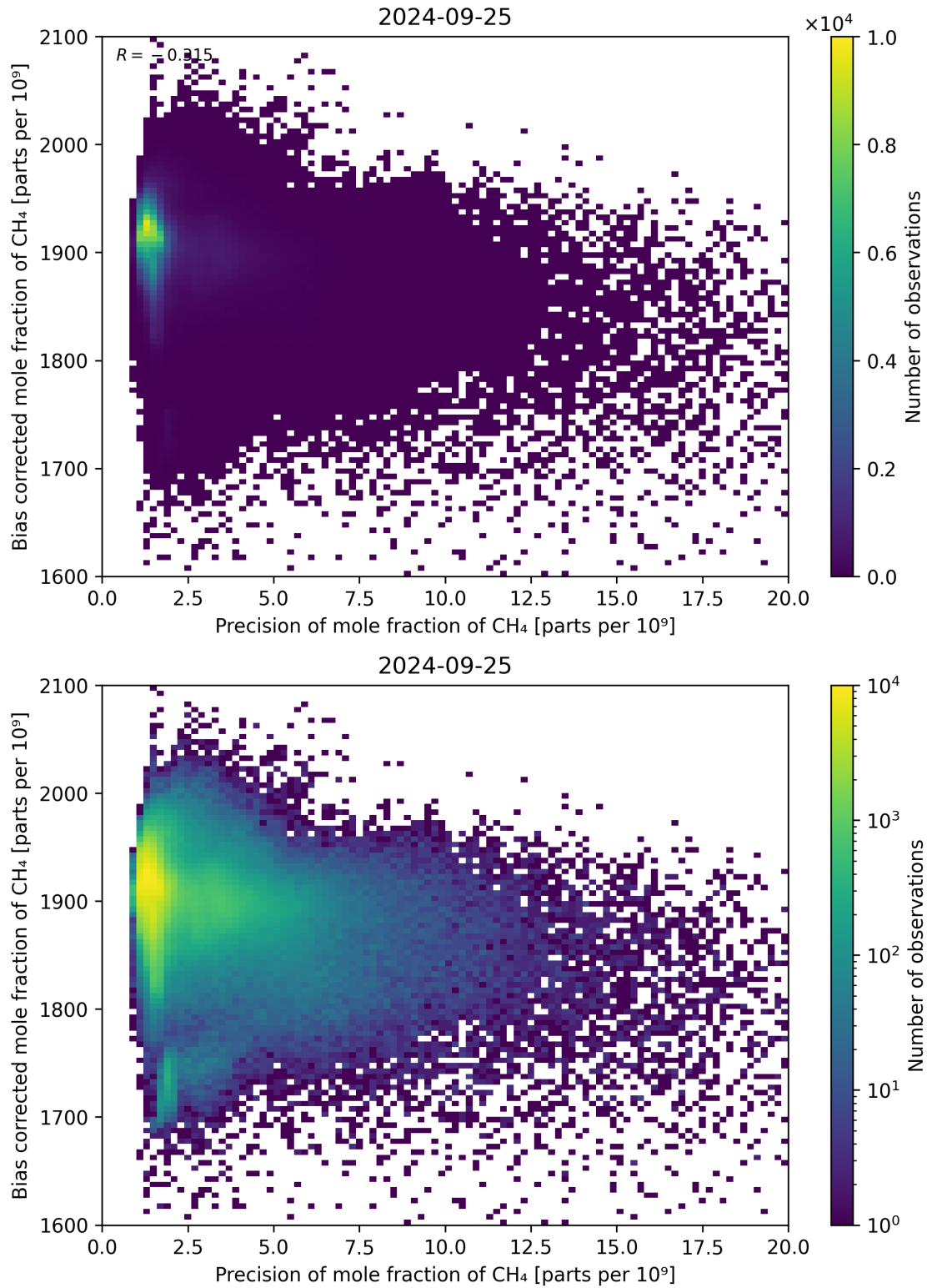
Figure 82: Scatter density plot of “Precision of mole fraction of CH 4 ” against “Bias corrected mole fraction of CH 4 ” for 2024-09-24 to 2024-09-26.
