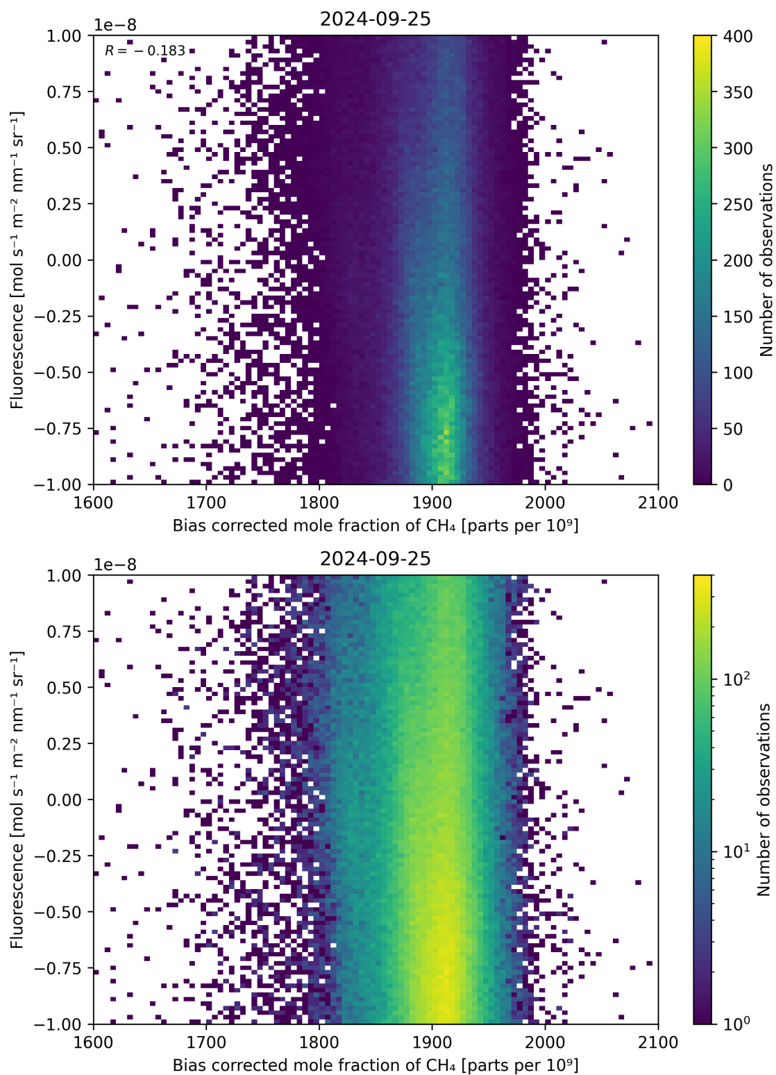
Figure 66: Scatter density plot of “Bias corrected mole fraction of \text{CH}_4 ” against “Fluorescence” for 2024-09-24 to 2024-09-26.
