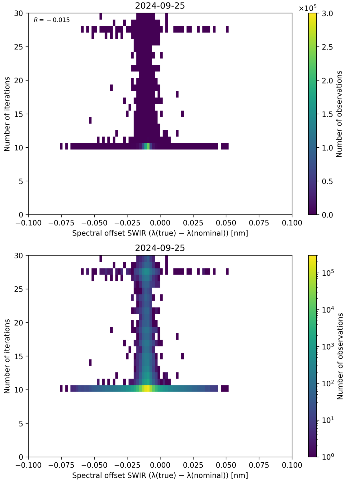
Figure 121: Scatter density plot of “Spectral offset SWIR ( \lambda_{\text{true}} - \lambda_{\text{nominal}} )” against “Number of iterations” for 2024-09-24 to 2024-09-26.
