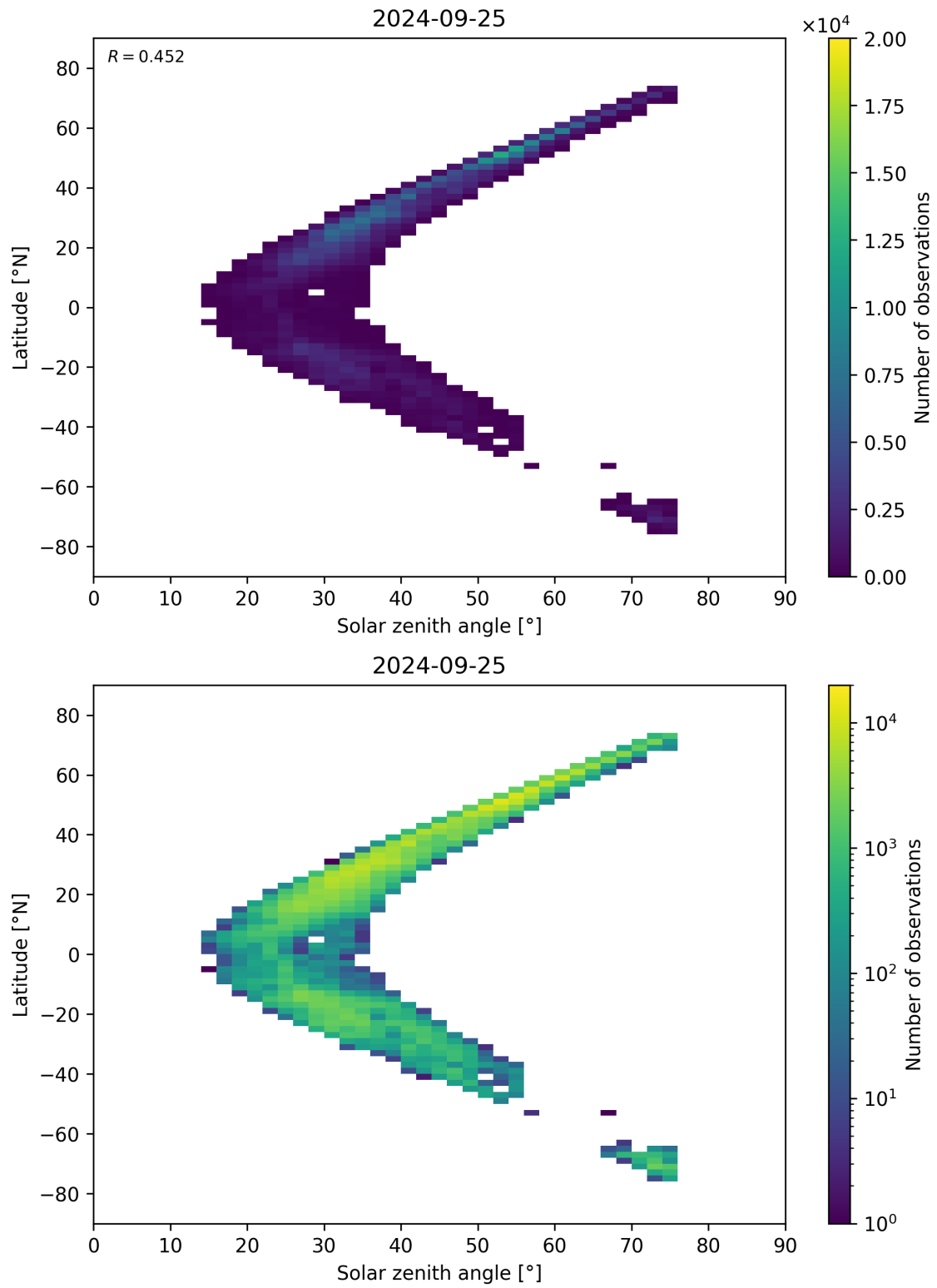
Figure 98: Scatter density plot of “Solar zenith angle” against “Latitude” for 2024-09-24 to 2024-09-26.
