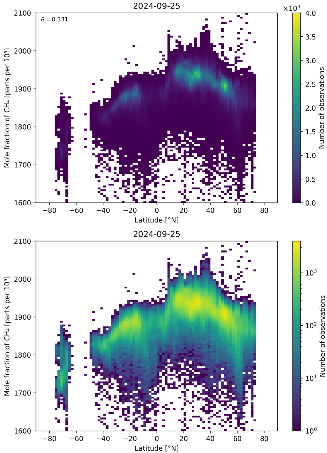
Figure 57: Scatter density plot of “Latitude” against “Mole fraction of CH 4 ” for 2024-09-24 to 2024-09-26.
