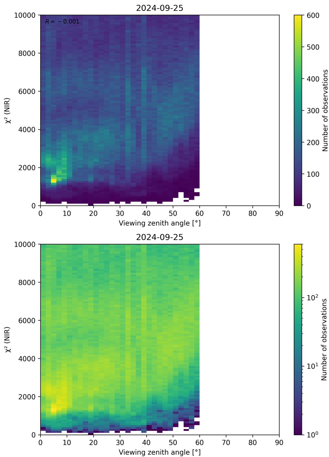
Figure 105: Scatter density plot of “Viewing zenith angle” against “ \chi^2 (NIR)” for 2024-09-24 to 2024-09-26.
