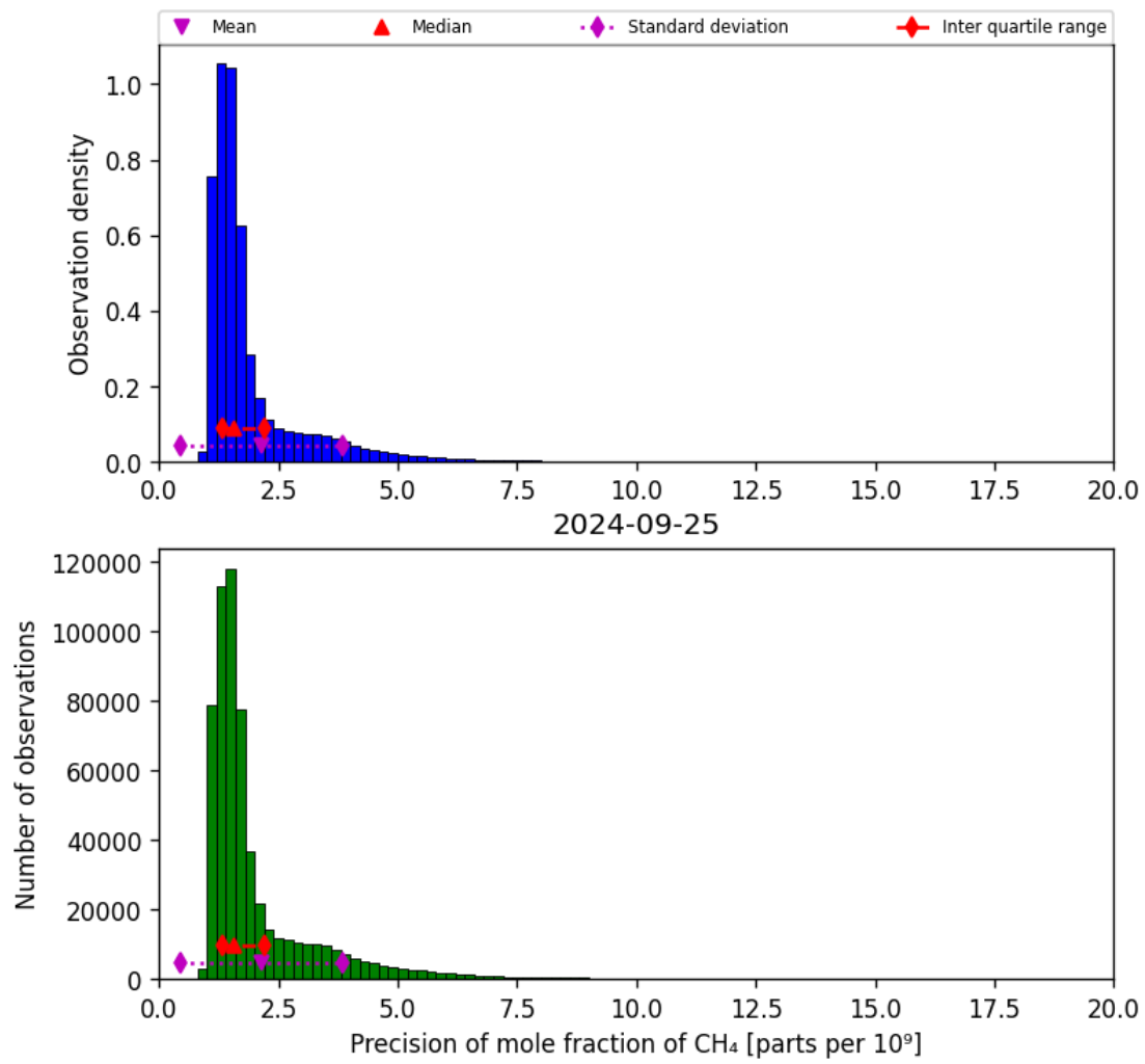
Figure 24: Histogram of “Precision of mole fraction of CH 4 ” for 2024-09-24 to 2024-09-26
