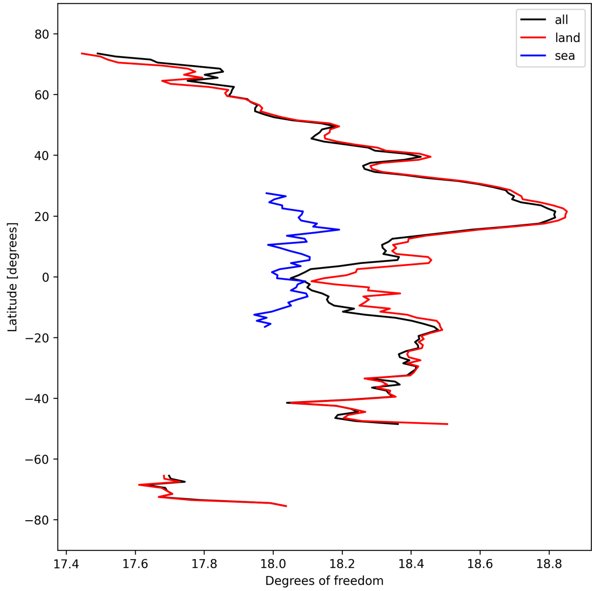
Figure 19: Zonal average of “Degrees of freedom” for 2024-09-24 to 2024-09-26.
