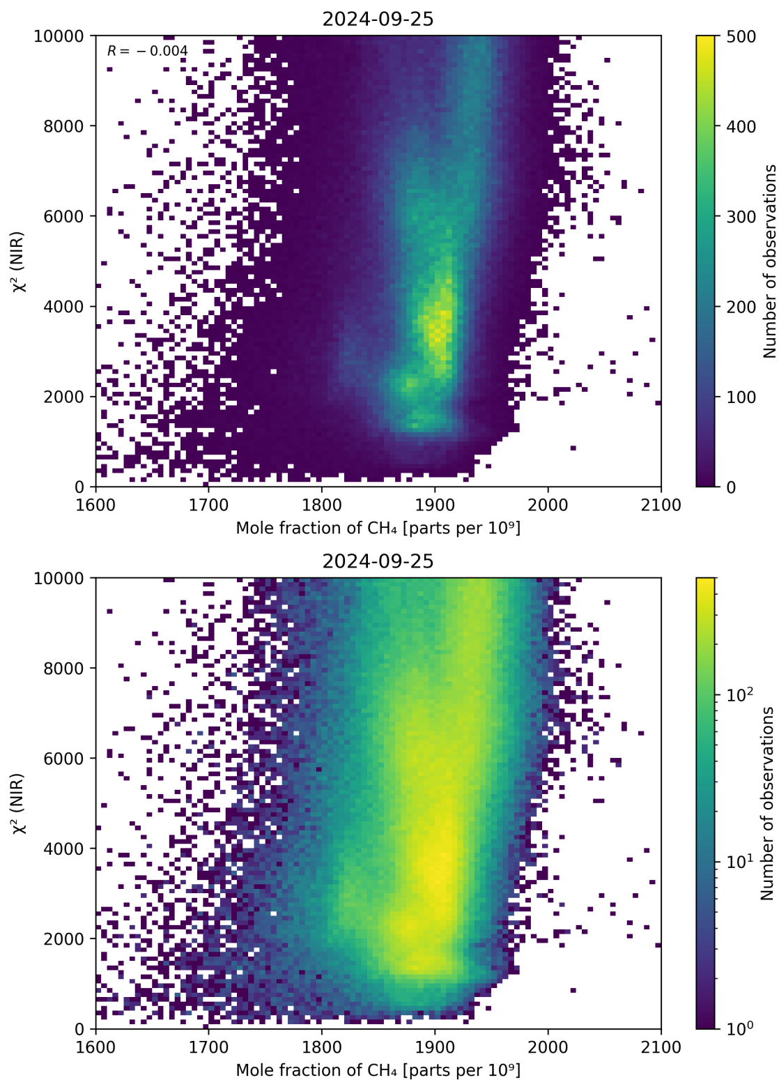
Figure 70: Scatter density plot of “Mole fraction of CH 4 ” against “ \chi^2 (NIR)” for 2024-09-24 to 2024-09-26.
