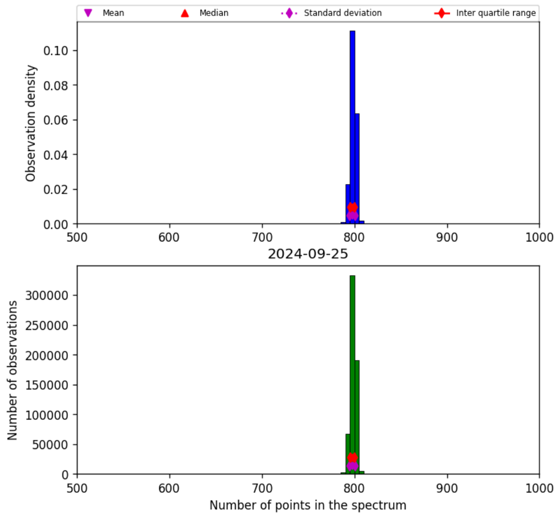
Figure 26: Histogram of “Number of points in the spectrum” for 2024-09-24 to 2024-09-26
