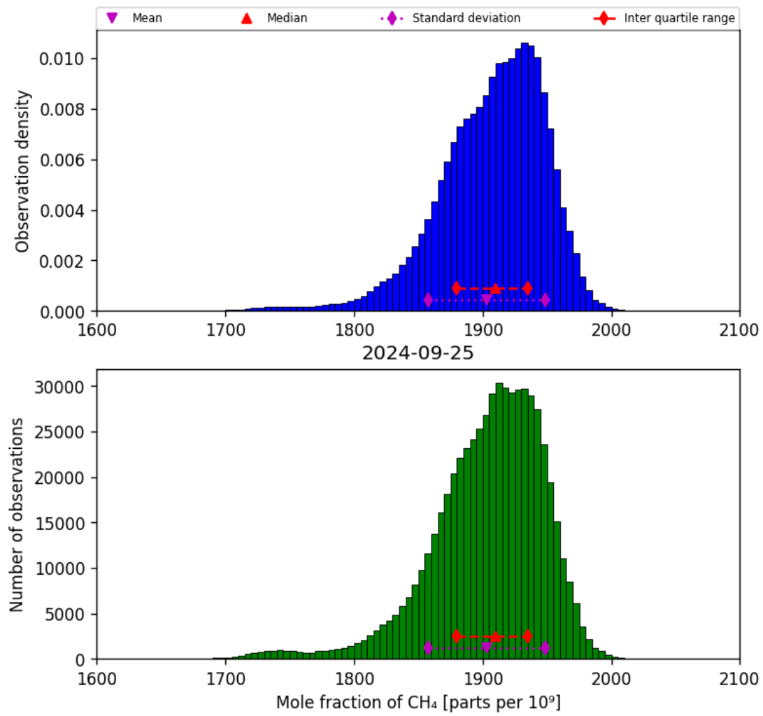
Figure 23: Histogram of “Mole fraction of CH 4 ” for 2024-09-24 to 2024-09-26
