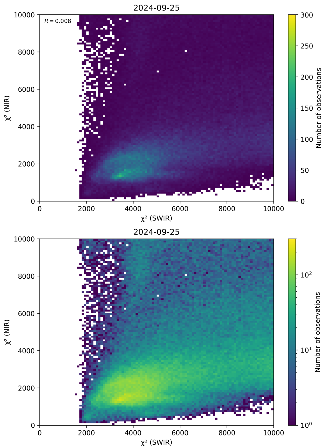
Figure 47: Scatter density plot of “ \chi^2 (SWIR)” against “ \chi^2 (NIR)” for 2024-09-24 to 2024-09-26.
