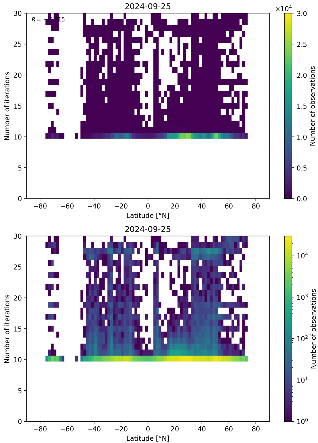
Figure 60: Scatter density plot of “Latitude” against “Number of iterations” for 2024-09-24 to 2024-09-26.
