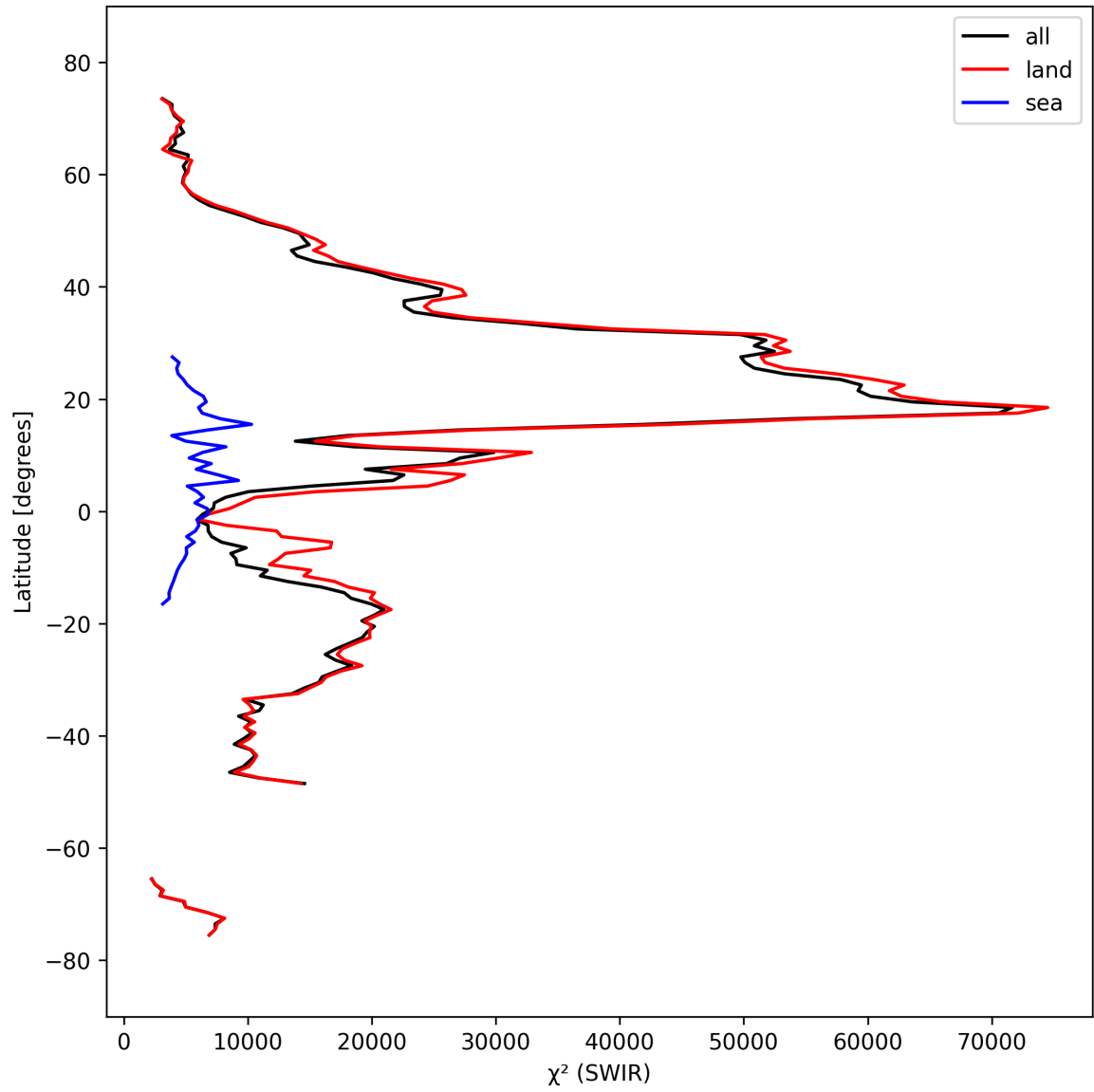
Figure 17: Zonal average of “ \chi^2 (SWIR)” for 2024-09-24 to 2024-09-26.
