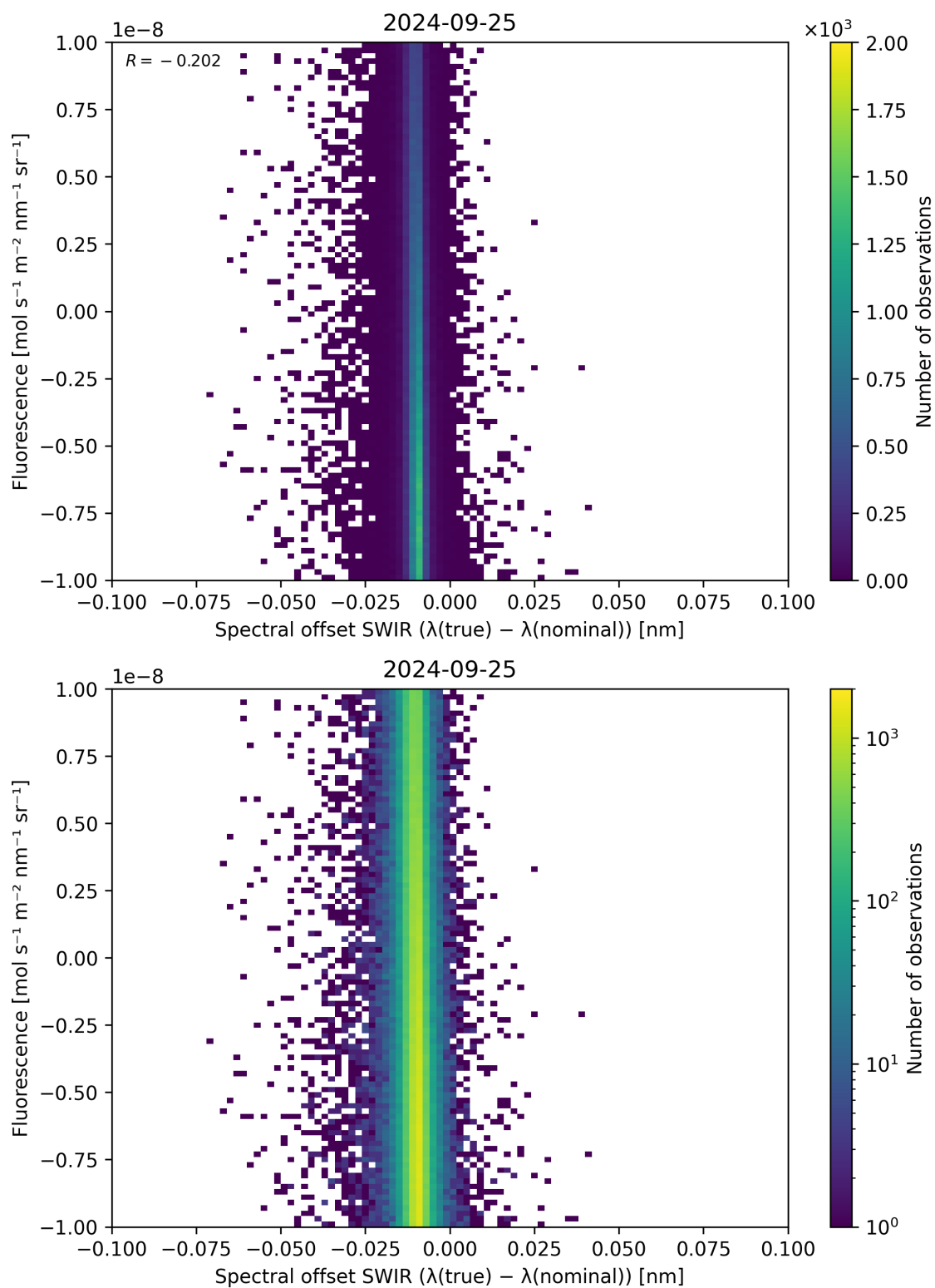
Figure 120: Scatter density plot of “Spectral offset SWIR ( \lambda_{\text{true}} - \lambda_{\text{nominal}} )” against “Fluorescence” for 2024-09-24 to 2024-09-26.
