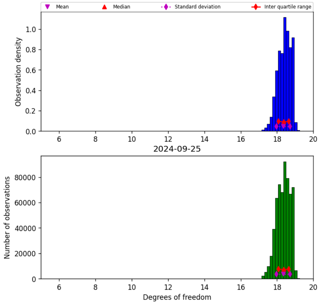
Figure 30: Histogram of “Degrees of freedom” for 2024-09-24 to 2024-09-26
