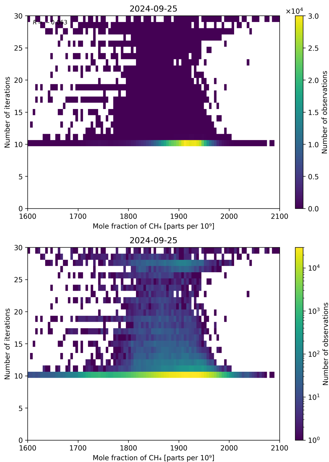
Figure 76: Scatter density plot of “Mole fraction of CH 4 ” against “Number of iterations” for 2024-09-24 to 2024-09-26.
