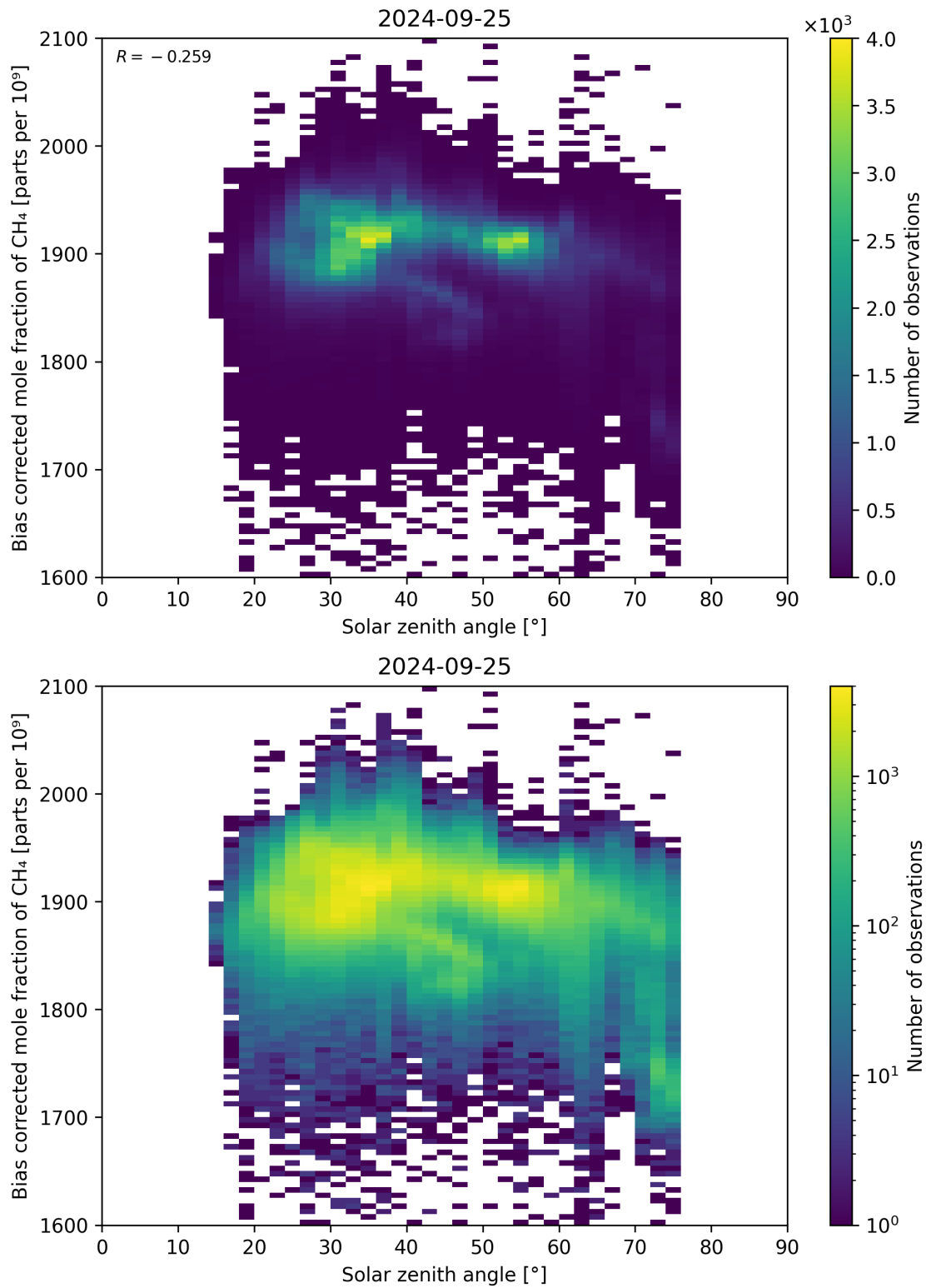
Figure 100: Scatter density plot of “Solar zenith angle” against “Bias corrected mole fraction of CH 4 ” for 2024-09-24 to 2024-09-26.
