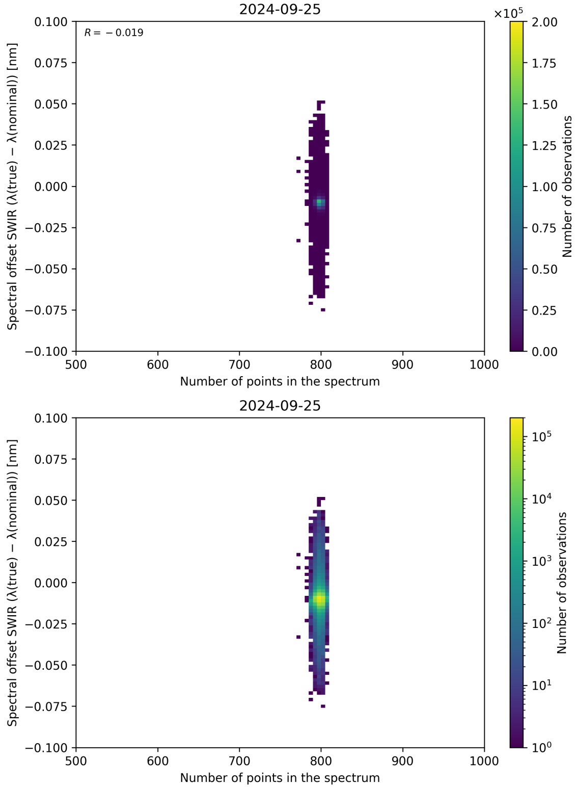
Figure 93: Scatter density plot of “Number of points in the spectrum” against “Spectral offset SWIR ( \lambda_{\text{true}} - \lambda_{\text{nominal}} )” for 2024-09-24 to 2024-09-26.
