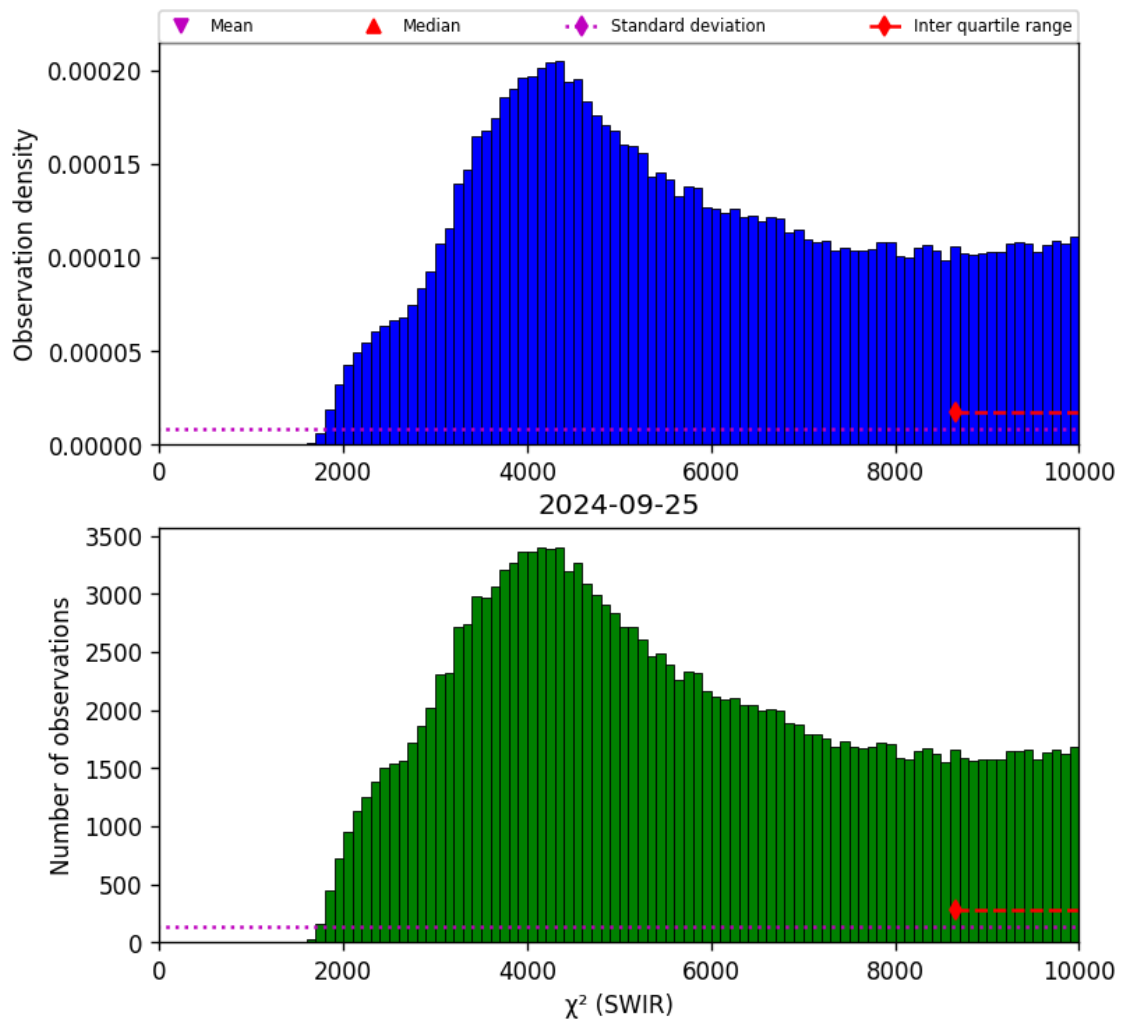
Figure 28: Histogram of " \chi^2 (SWIR)" for 2024-09-24 to 2024-09-26
