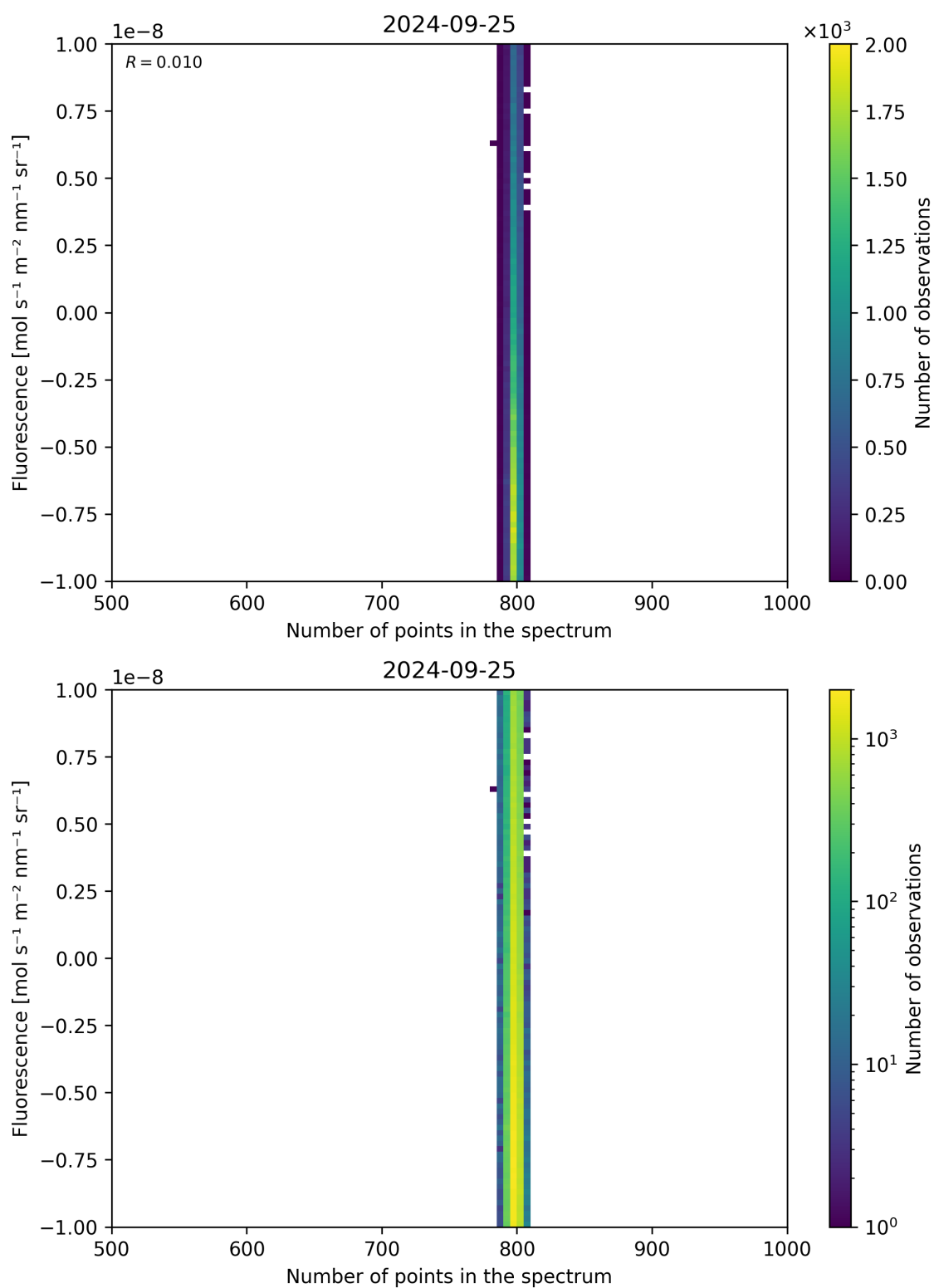
Figure 91: Scatter density plot of “Number of points in the spectrum” against “Fluorescence” for 2024-09-24 to 2024-09-26.
