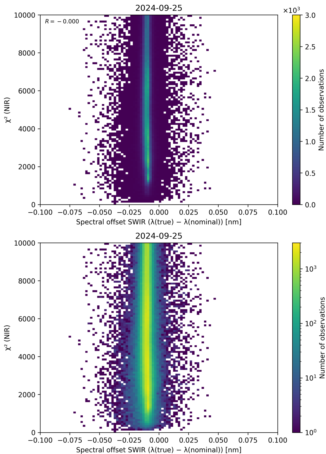
Figure 117: Scatter density plot of “Spectral offset SWIR ( \lambda_{\text{true}} - \lambda_{\text{nominal}} )” against “ \chi^2 (NIR)” for 2024-09-24 to 2024-09-26.
