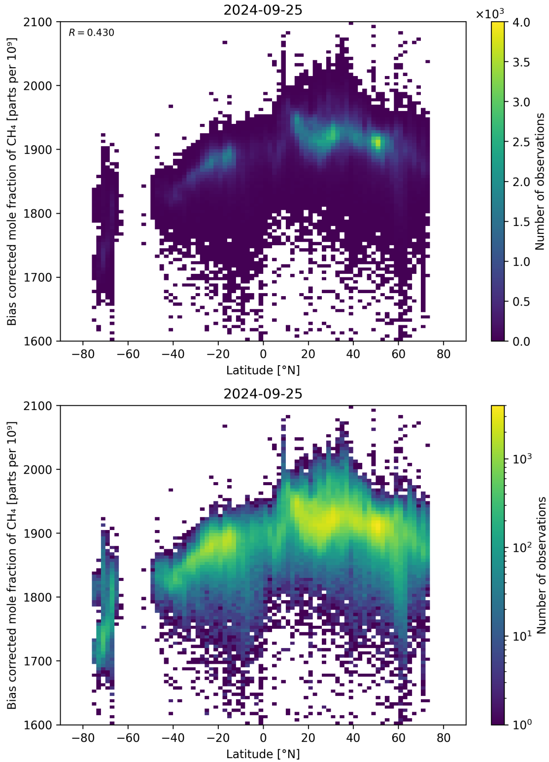
Figure 58: Scatter density plot of “Latitude” against “Bias corrected mole fraction of CH 4 ” for 2024-09-24 to 2024-09-26.
