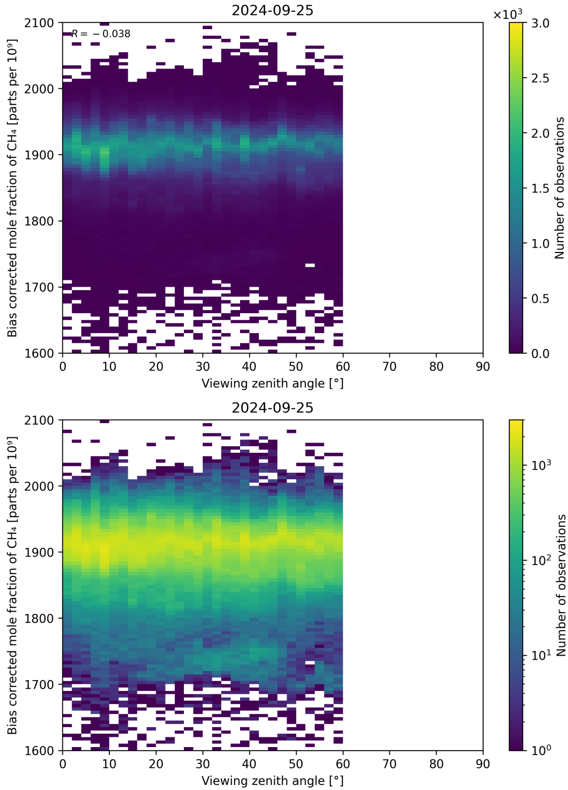
Figure 111: Scatter density plot of “Viewing zenith angle” against “Bias corrected mole fraction of CH 4 ” for 2024-09-24 to 2024-09-26.
