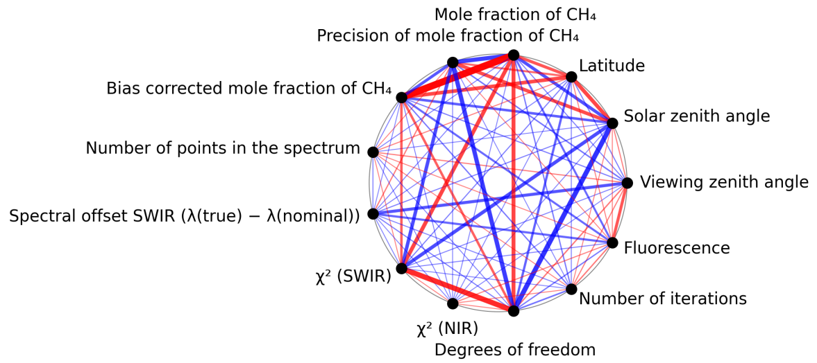
Figure 1: Map of correlation graph for 2024-09-24 to 2024-09-26.
