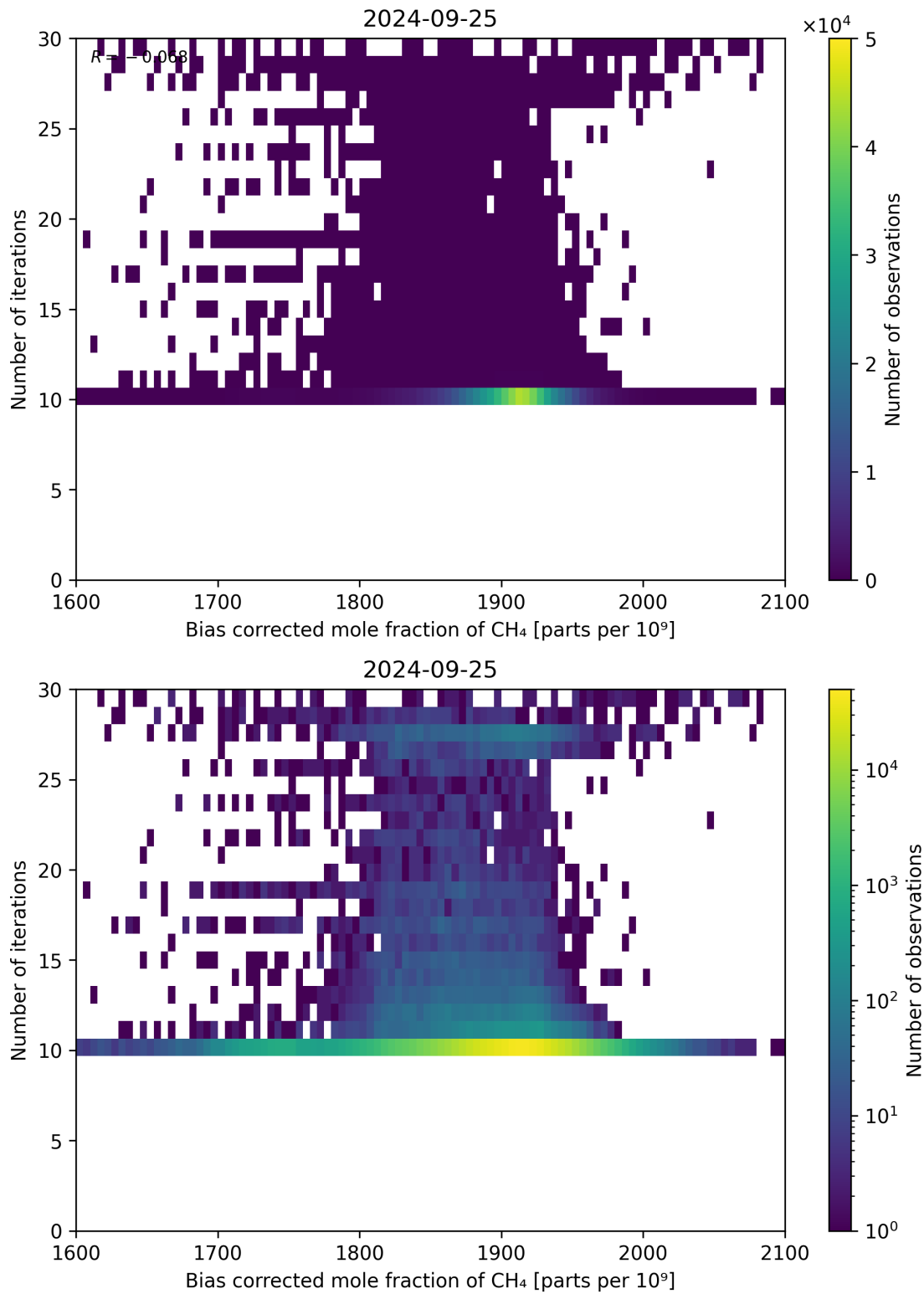
Figure 67: Scatter density plot of “Bias corrected mole fraction of CH 4 ” against “Number of iterations” for 2024-09-24 to 2024-09-26.
