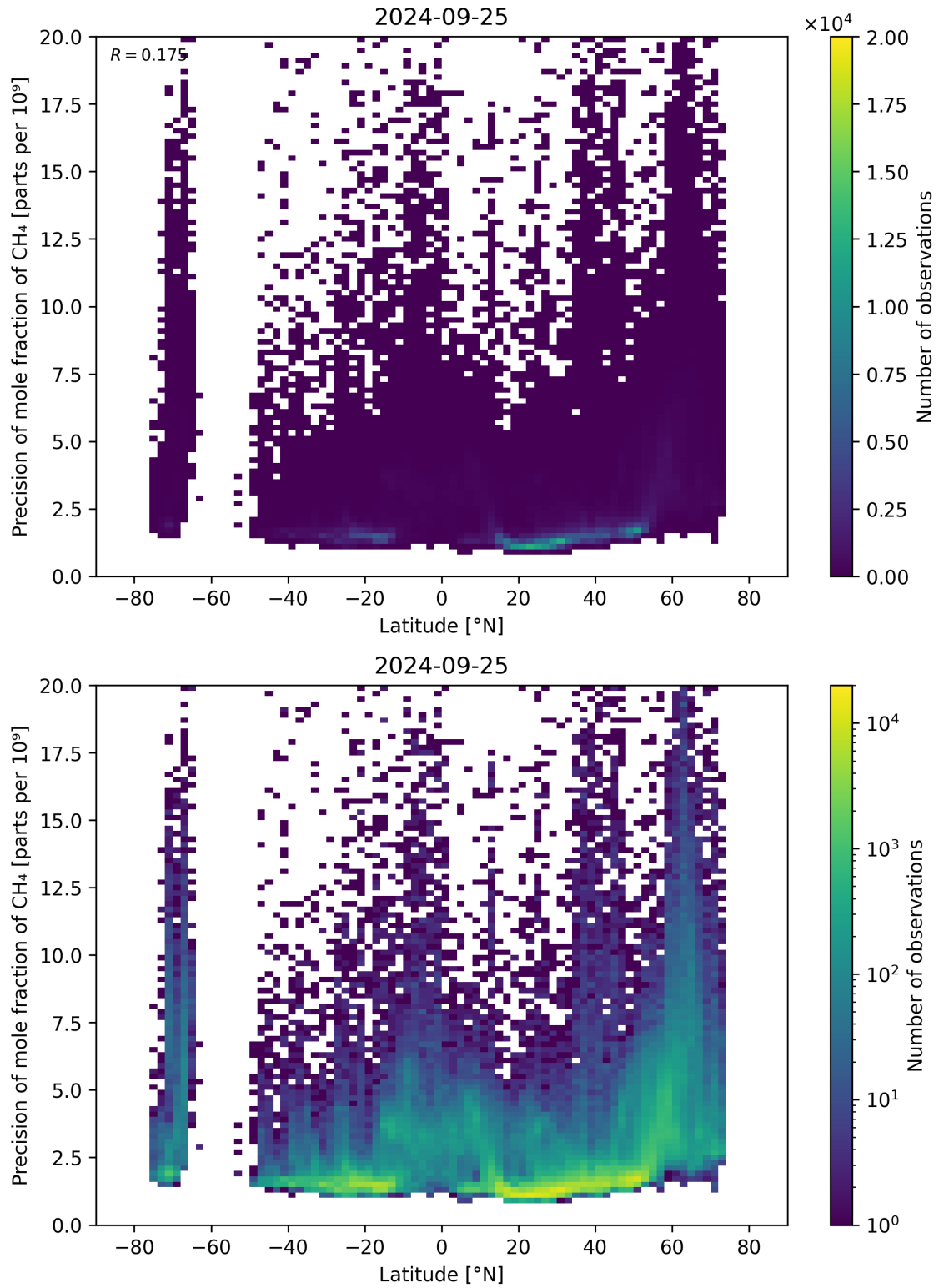
Figure 59: Scatter density plot of “Latitude” against “Precision of mole fraction of \text{CH}_4 ” for 2024-09-24 to 2024-09-26.
