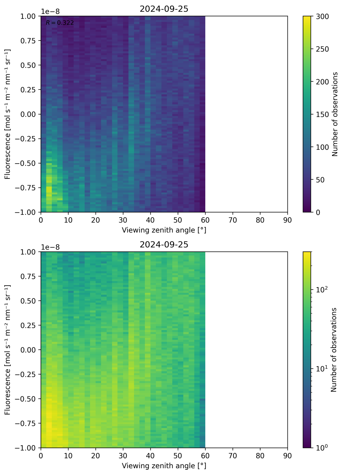
Figure 108: Scatter density plot of “Viewing zenith angle” against “Fluorescence” for 2024-09-24 to 2024-09-26.
