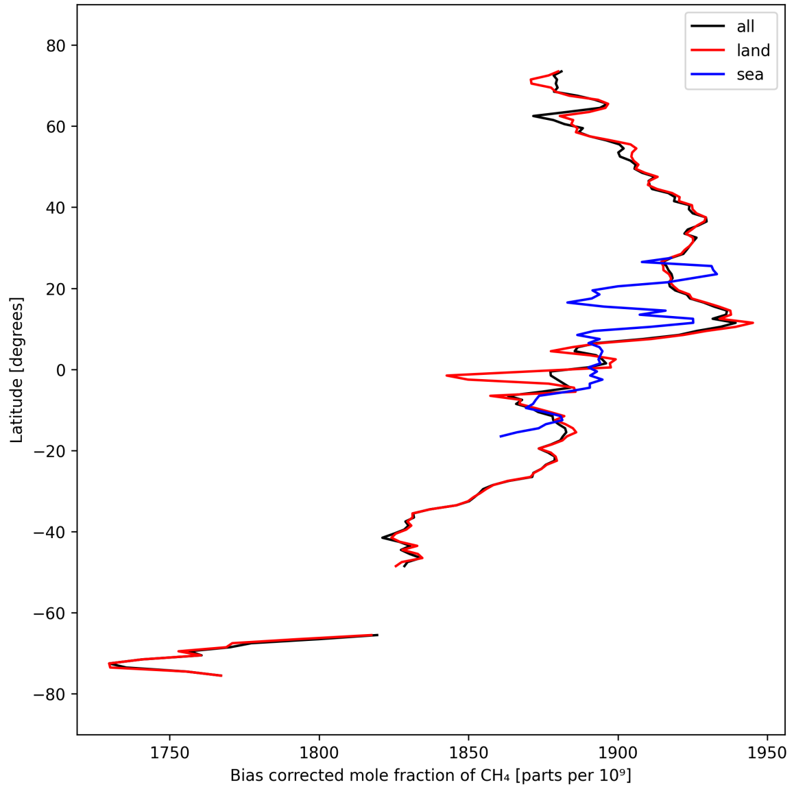
Figure 14: Zonal average of “Bias corrected mole fraction of CH 4 ” for 2024-09-24 to 2024-09-26.
