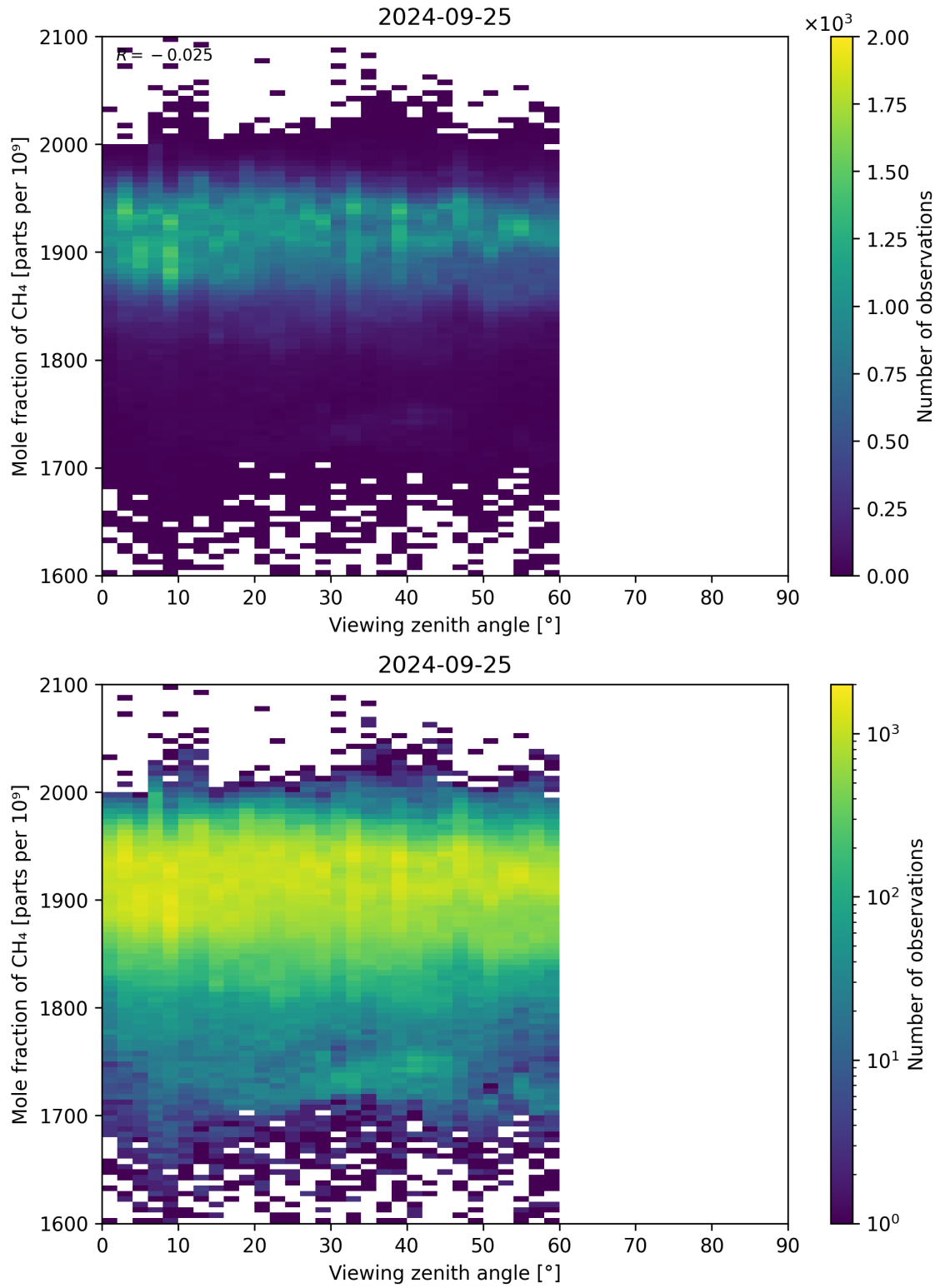
Figure 110: Scatter density plot of “Viewing zenith angle” against “Mole fraction of CH 4 ” for 2024-09-24 to 2024-09-26.
