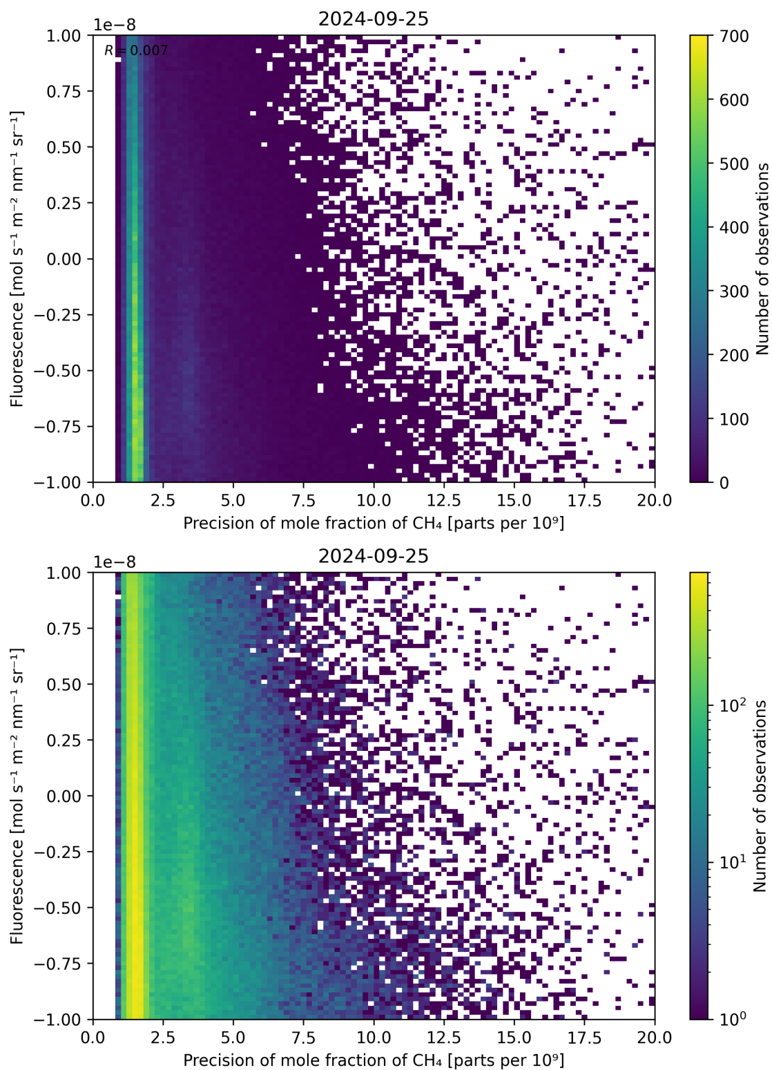
Figure 81: Scatter density plot of “Precision of mole fraction of \text{CH}_4 ” against “Fluorescence” for 2024-09-24 to 2024-09-26.
