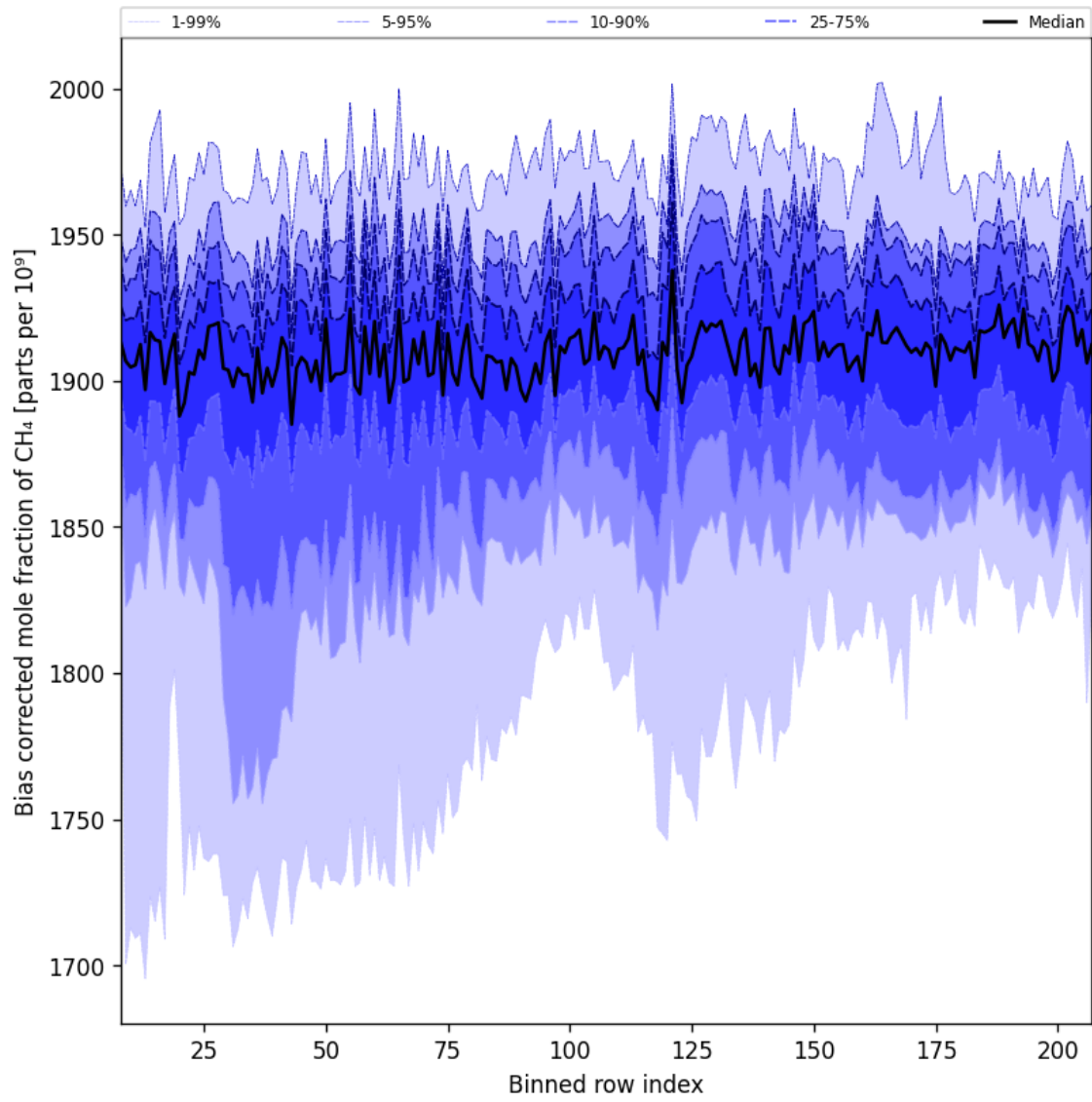
Figure 36: Along track statistics of “Bias corrected mole fraction of CH 4 ” for 2024-09-24 to 2024-09-26
