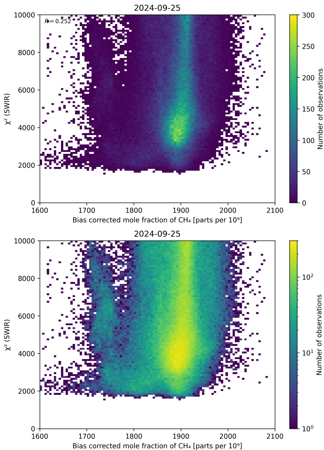
Figure 64: Scatter density plot of “Bias corrected mole fraction of \text{CH}_4 ” against “ \chi^2 (SWIR)” for 2024-09-24 to 2024-09-26.
