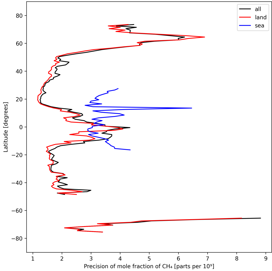
Figure 13: Zonal average of “Precision of mole fraction of CH 4 ” for 2024-09-24 to 2024-09-26.
