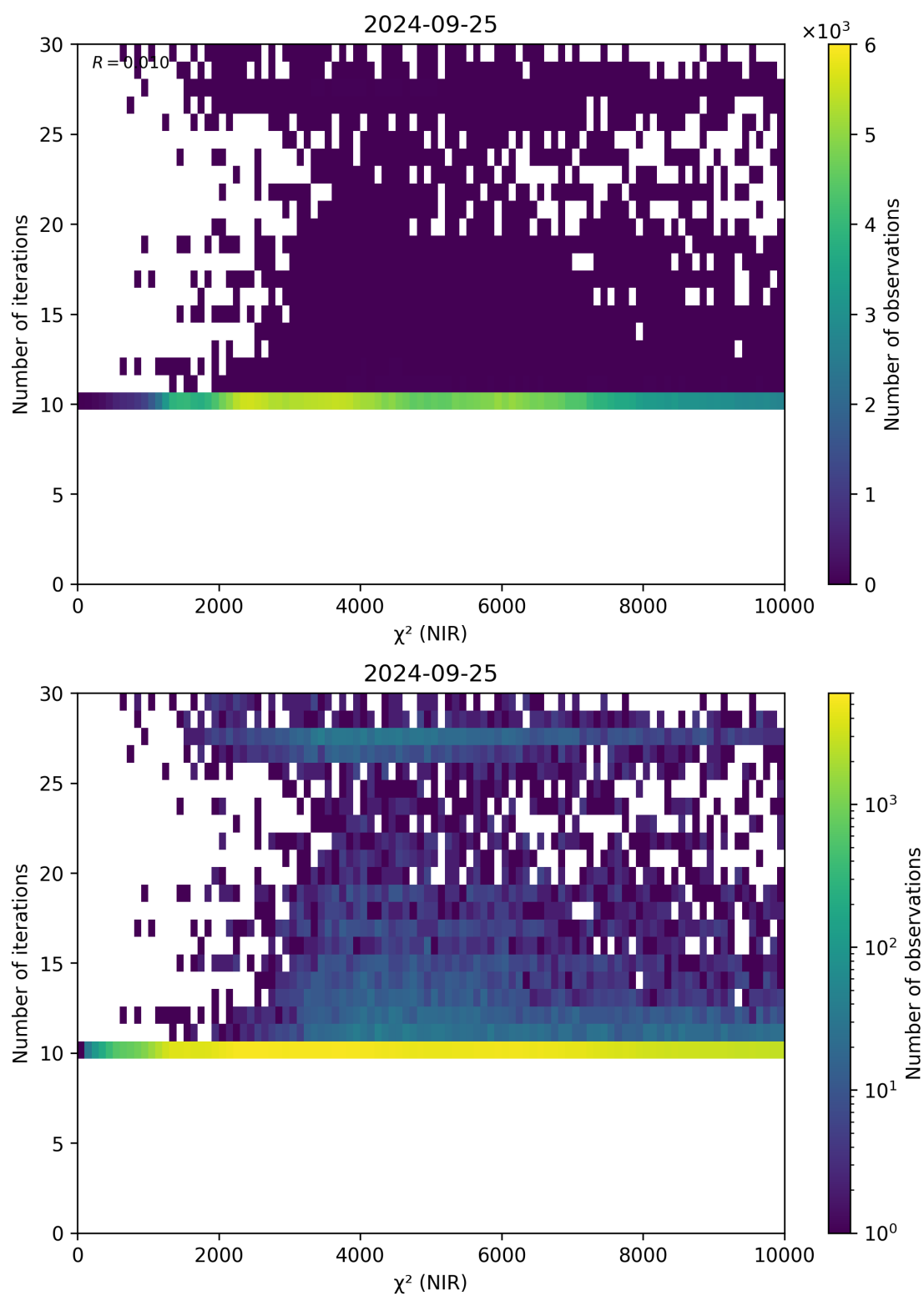
Figure 46: Scatter density plot of “ \chi^2 (NIR)” against “Number of iterations” for 2024-09-24 to 2024-09-26.
