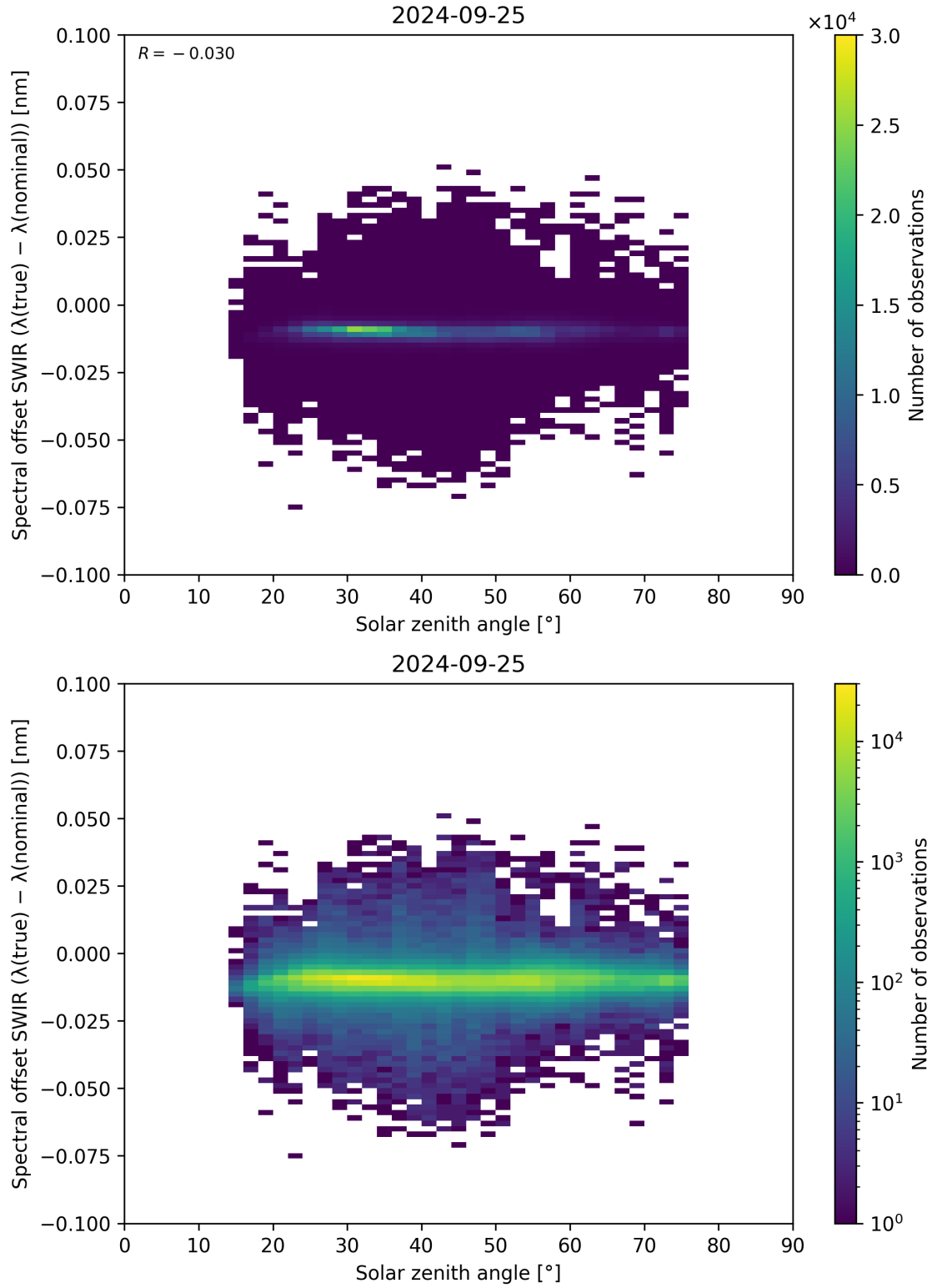
Figure 104: Scatter density plot of “Solar zenith angle” against “Spectral offset SWIR ( \lambda_{\text{true}} - \lambda_{\text{nominal}} )” for 2024-09-24 to 2024-09-26.
