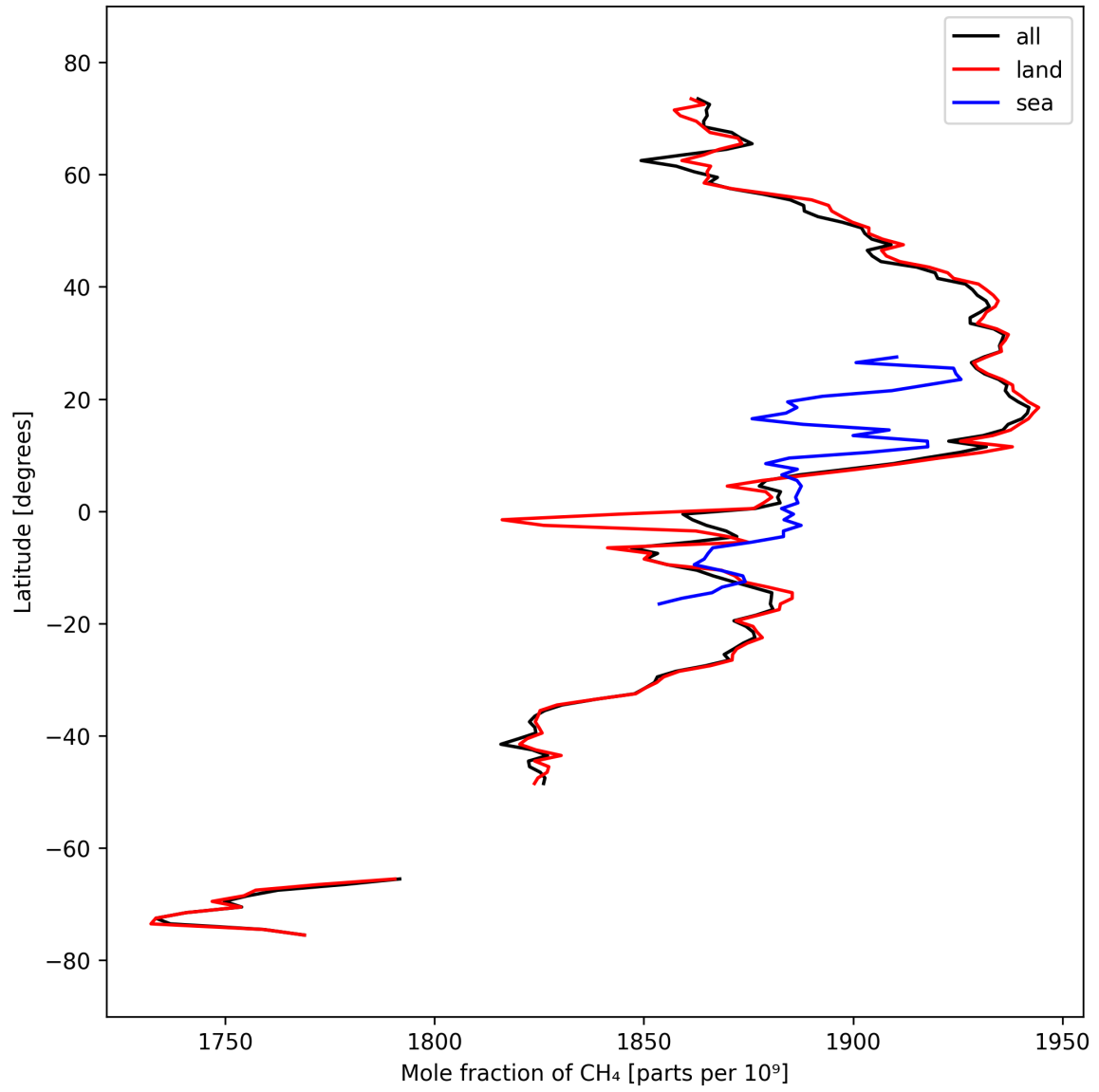
Figure 12: Zonal average of “Mole fraction of \text{CH}_4 ” for 2024-09-24 to 2024-09-26.
