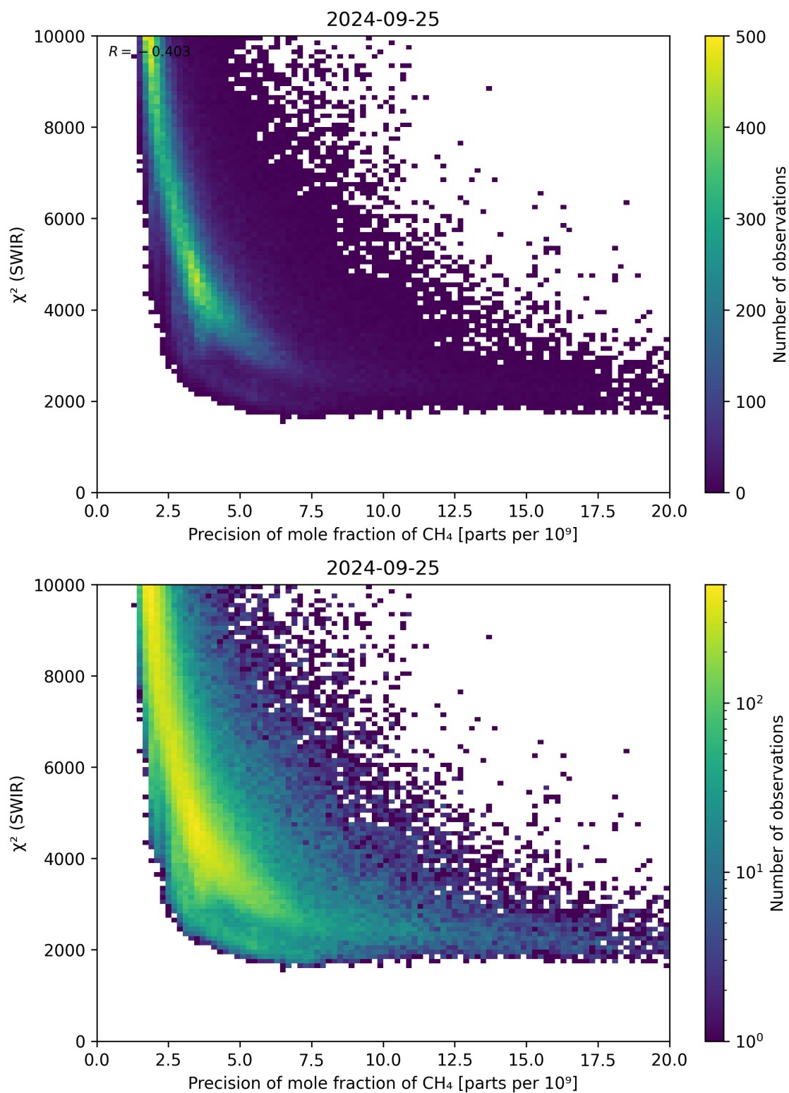
Figure 79: Scatter density plot of “Precision of mole fraction of \text{CH}_4 ” against “ \chi^2 (SWIR)” for 2024-09-24 to 2024-09-26.
