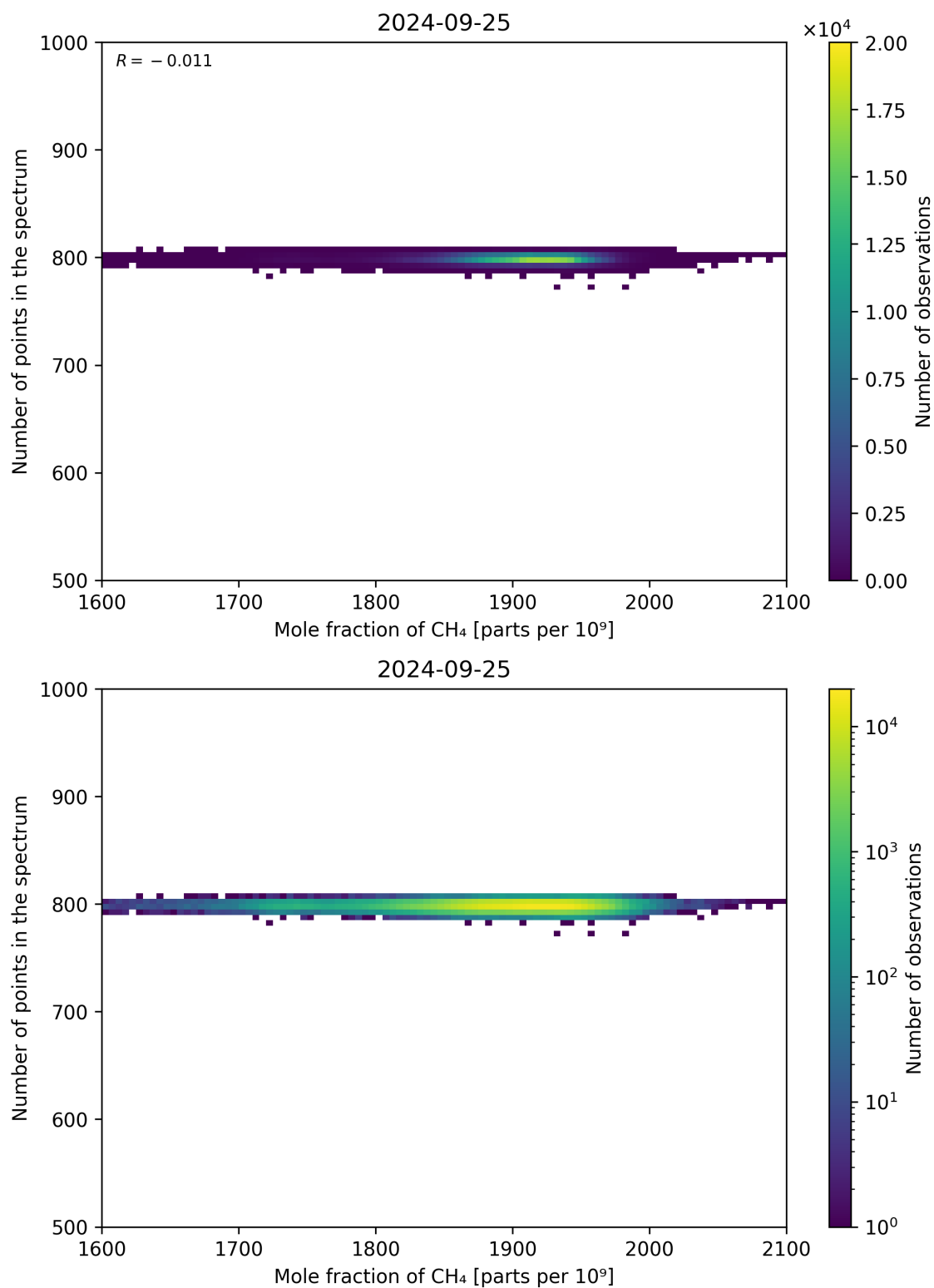
Figure 77: Scatter density plot of “Mole fraction of CH 4 ” against “Number of points in the spectrum” for 2024-09-24 to 2024-09-26.
