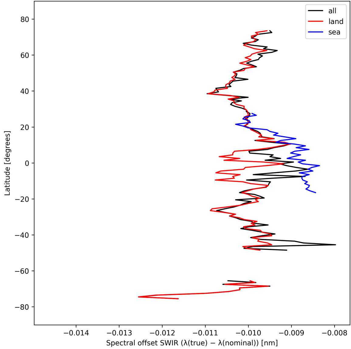
Figure 16: Zonal average of “Spectral offset SWIR ( \lambda_{\text{true}} - \lambda_{\text{nominal}} )” for 2024-09-24 to 2024-09-26.
