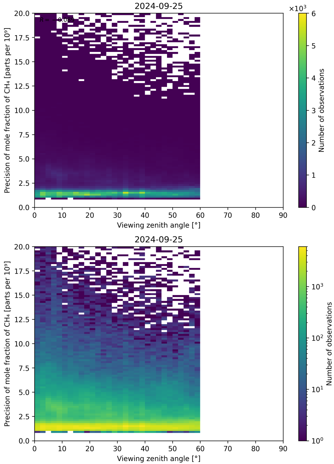
Figure 112: Scatter density plot of “Viewing zenith angle” against “Precision of mole fraction of CH 4 ” for 2024-09-24 to 2024-09-26.
