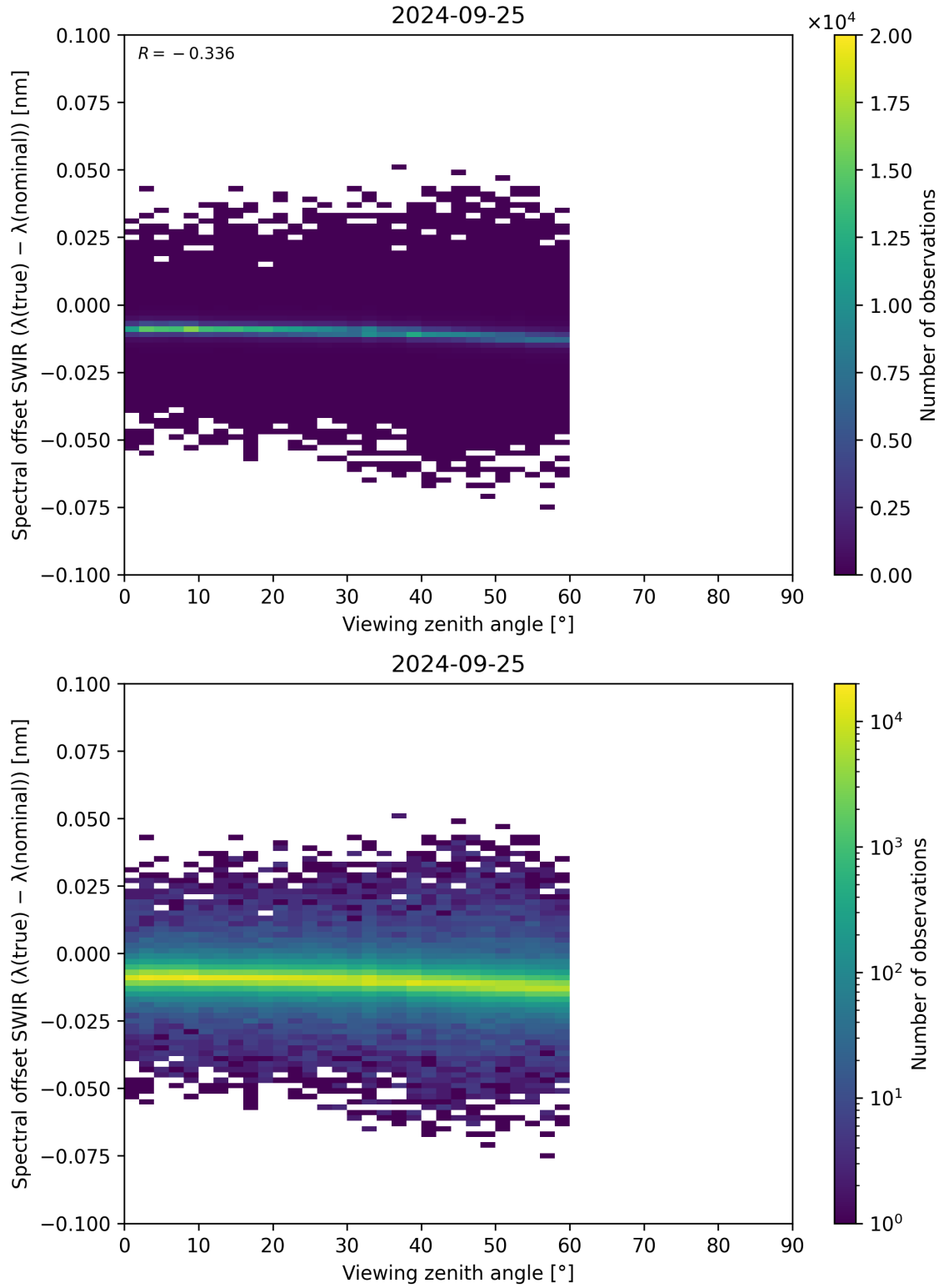
Figure 116: Scatter density plot of “Viewing zenith angle” against “Spectral offset SWIR ( \lambda_{\text{true}} - \lambda_{\text{nominal}} )” for 2024-09-24 to 2024-09-26.
