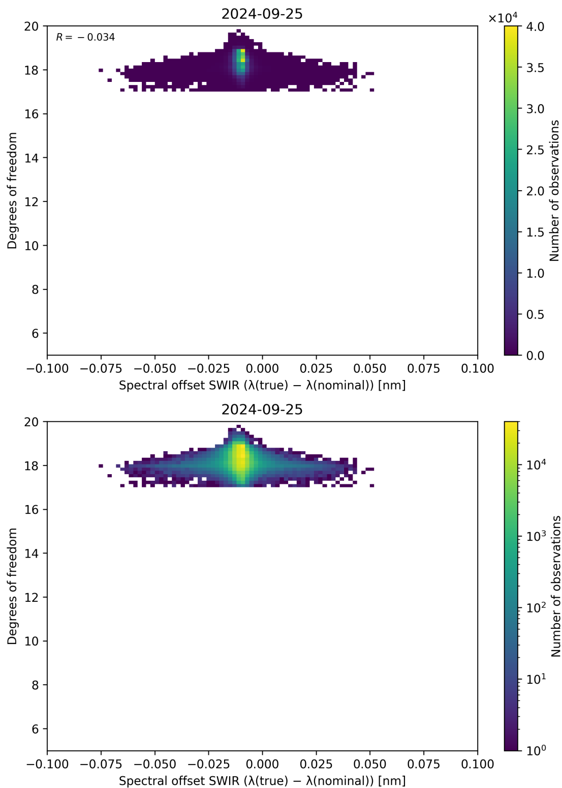
Figure 119: Scatter density plot of “Spectral offset SWIR ( \lambda_{\text{true}} - \lambda_{\text{nominal}} )” against “Degrees of freedom” for 2024-09-24 to 2024-09-26.
