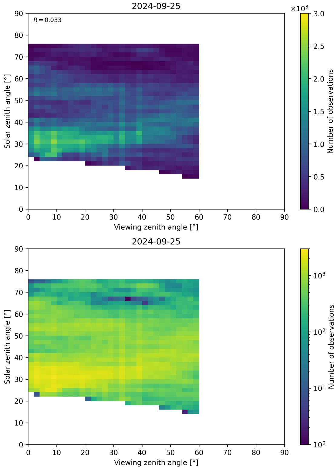
Figure 115: Scatter density plot of “Viewing zenith angle” against “Solar zenith angle” for 2024-09-24 to 2024-09-26.
