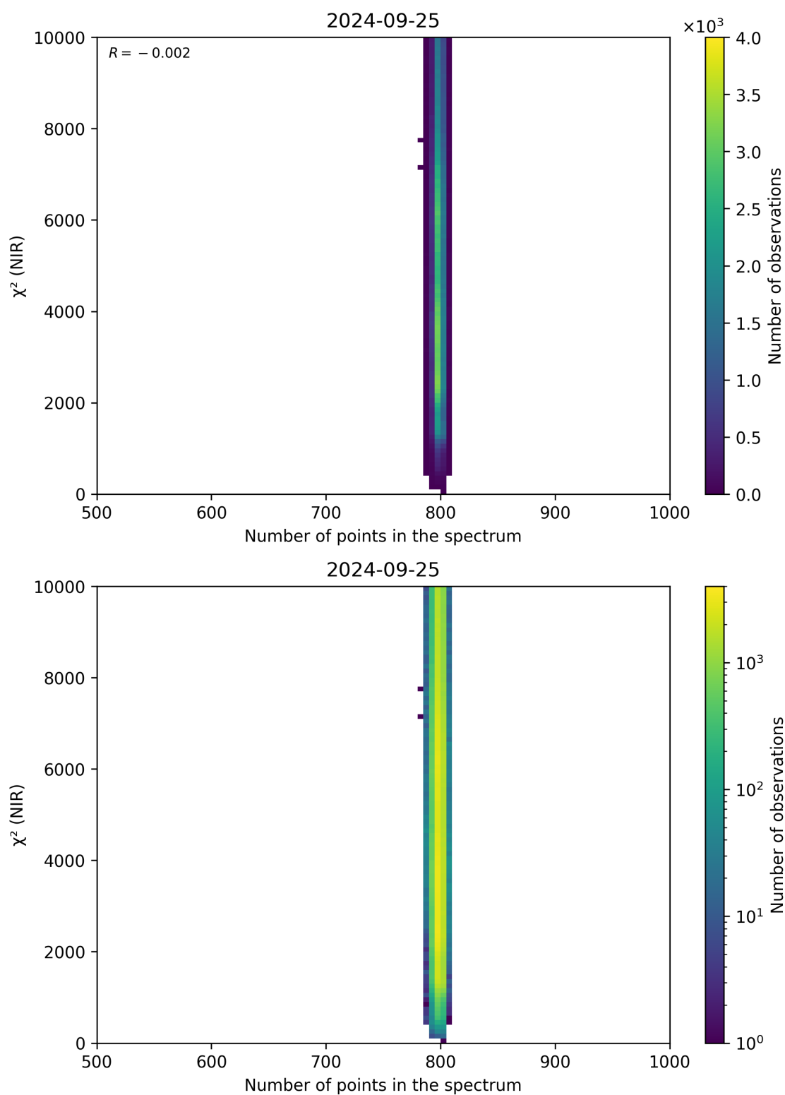
Figure 88: Scatter density plot of “Number of points in the spectrum” against “ \chi^2 (NIR)” for 2024-09-24 to 2024-09-26.
