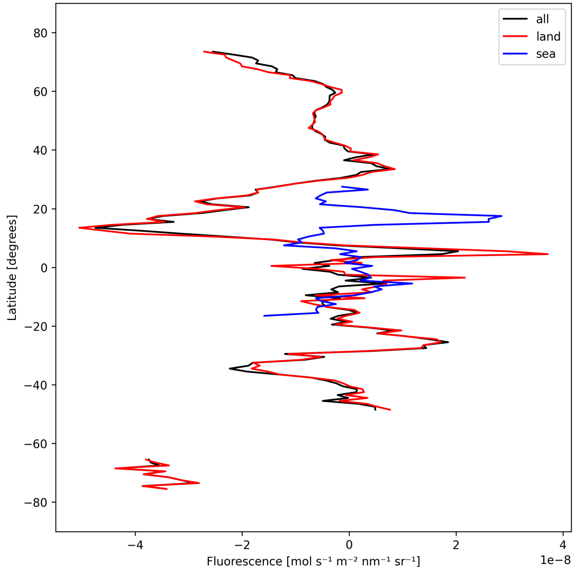
Figure 21: Zonal average of “Fluorescence” for 2024-09-24 to 2024-09-26.
