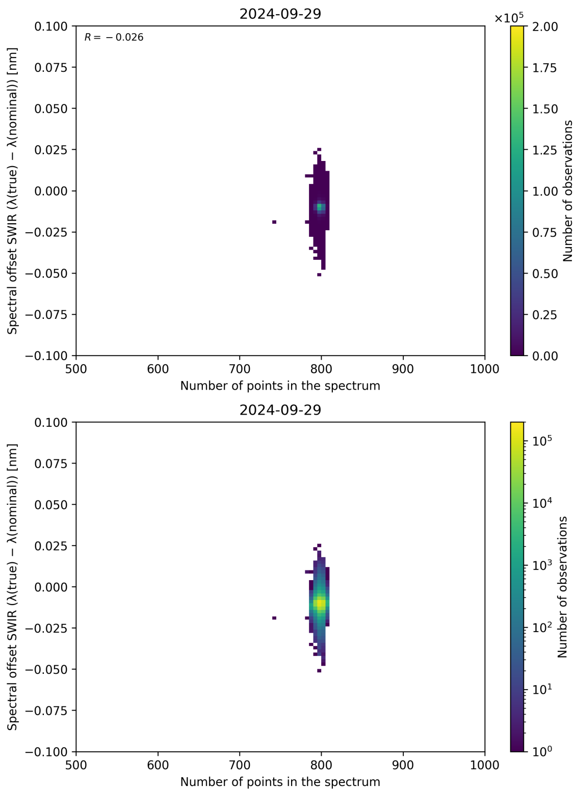
Figure 93: Scatter density plot of “Number of points in the spectrum” against “Spectral offset SWIR ( \lambda_{\text{true}} - \lambda_{\text{nominal}} )” for 2024-09-28 to 2024-09-30.
