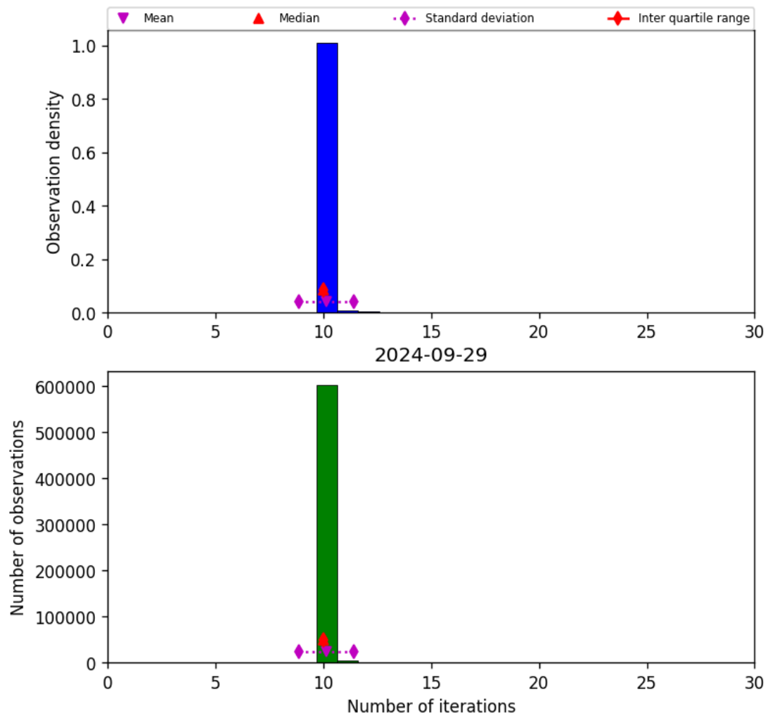
Figure 31: Histogram of “Number of iterations” for 2024-09-28 to 2024-09-30
