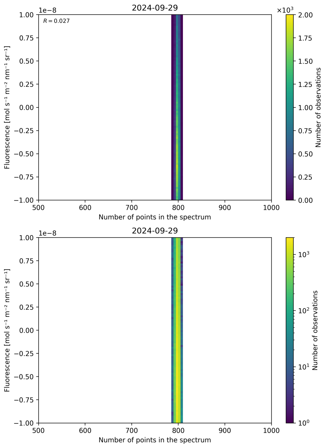
Figure 91: Scatter density plot of “Number of points in the spectrum” against “Fluorescence” for 2024-09-28 to 2024-09-30.
