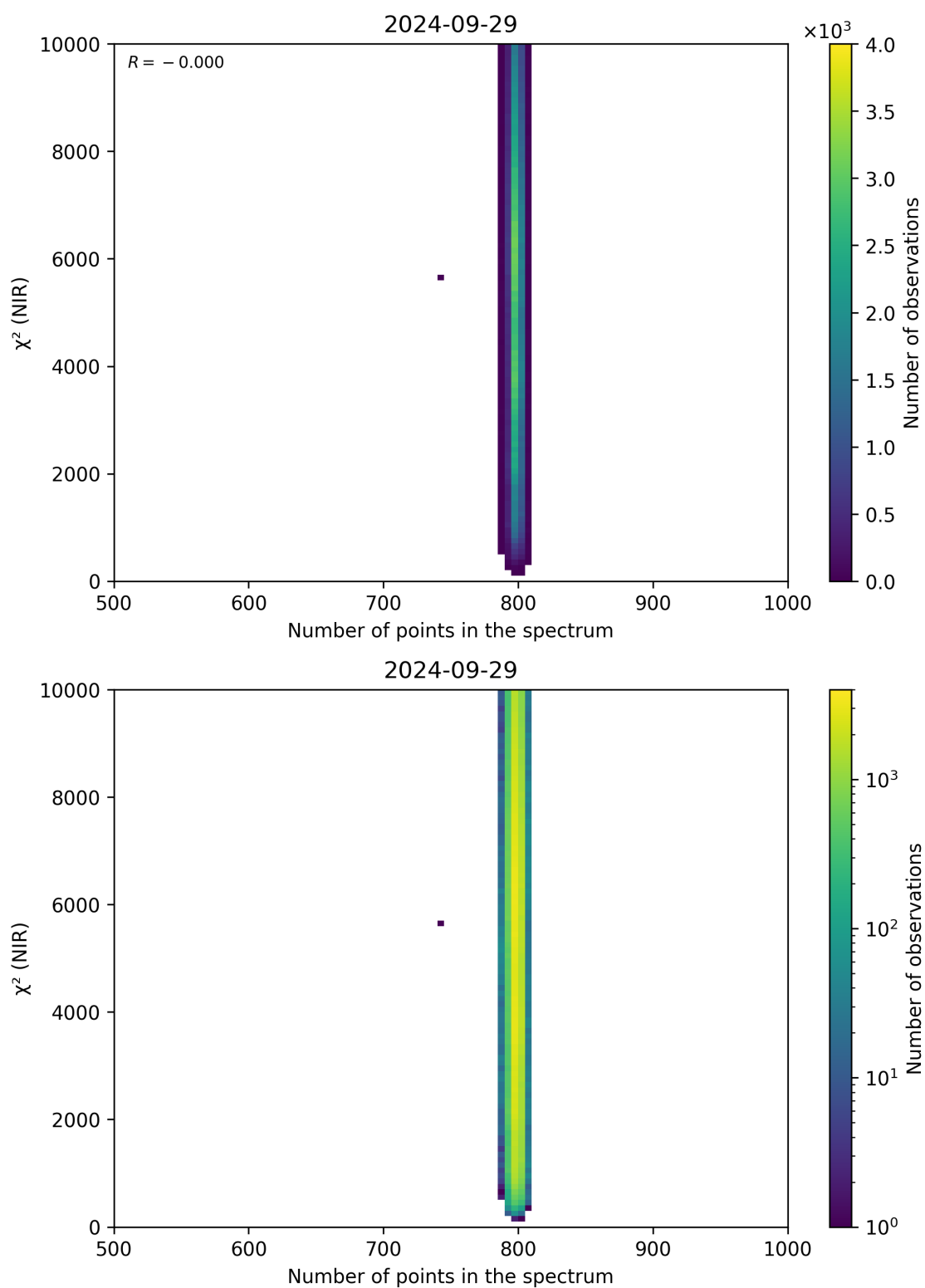
Figure 88: Scatter density plot of “Number of points in the spectrum” against “ \chi^2 (NIR)” for 2024-09-28 to 2024-09-30.
