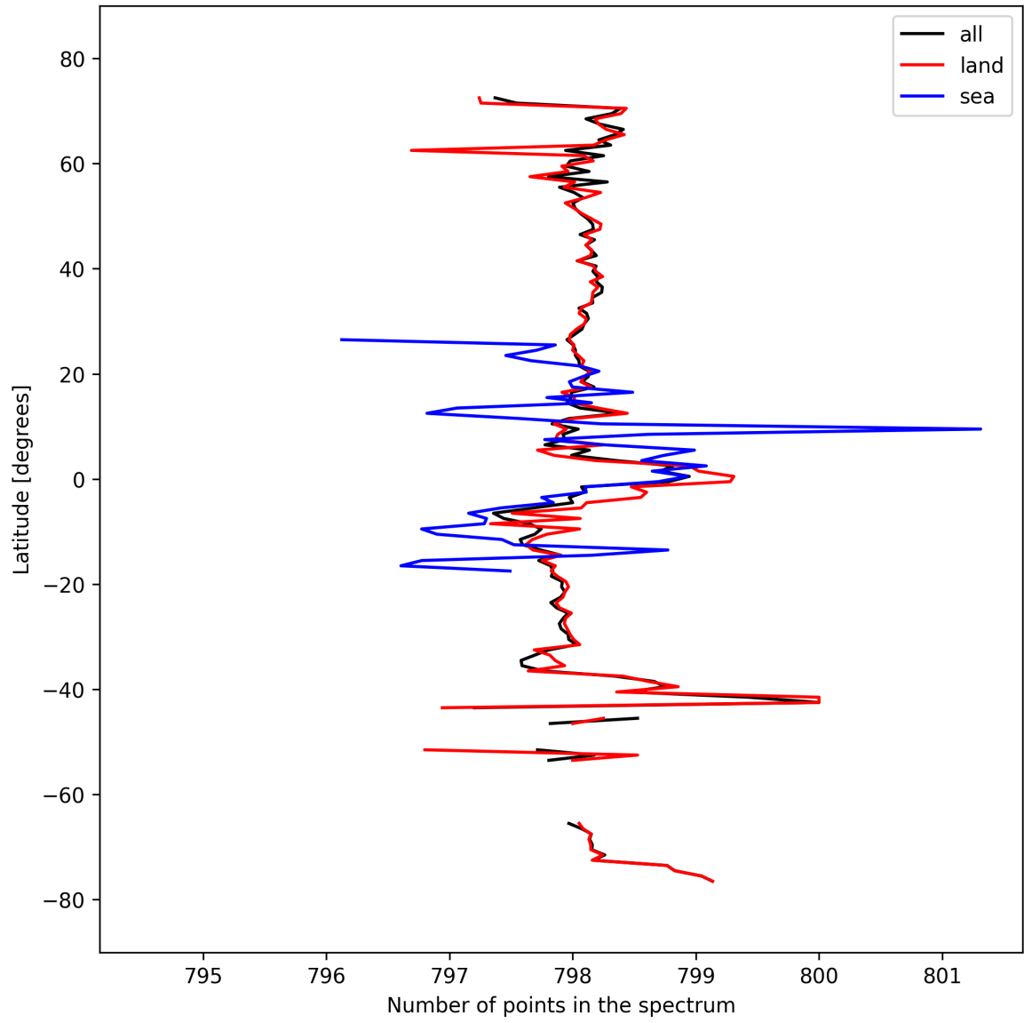
Figure 15: Zonal average of “Number of points in the spectrum” for 2024-09-28 to 2024-09-30.
