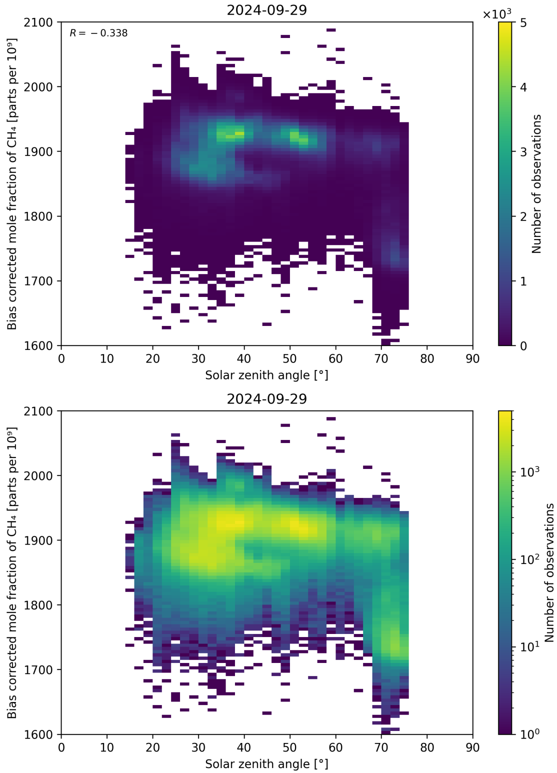
Figure 100: Scatter density plot of “Solar zenith angle” against “Bias corrected mole fraction of \text{CH}_4 ” for 2024-09-28 to 2024-09-30.
