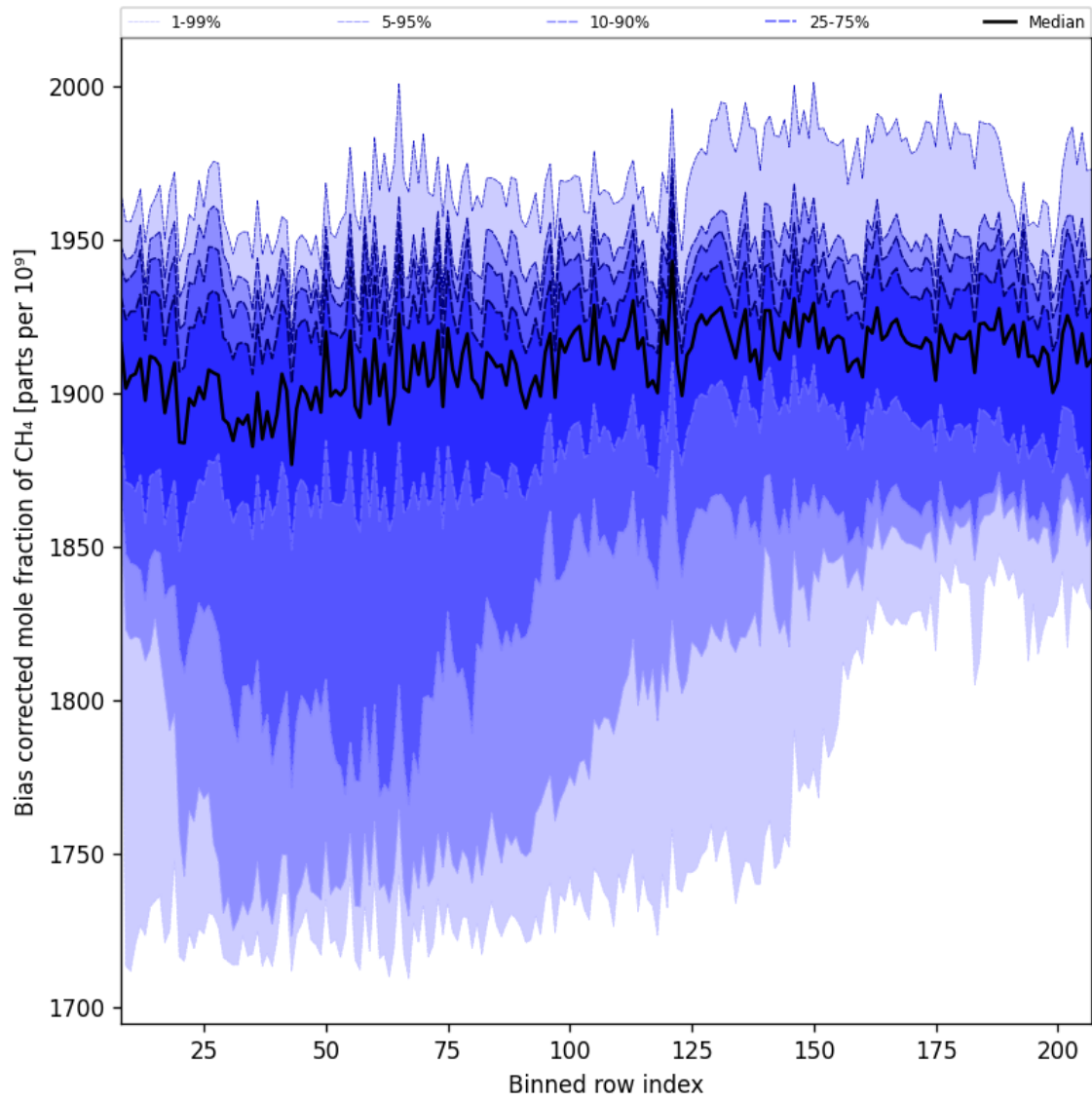
Figure 36: Along track statistics of “Bias corrected mole fraction of CH 4 ” for 2024-09-28 to 2024-09-30
