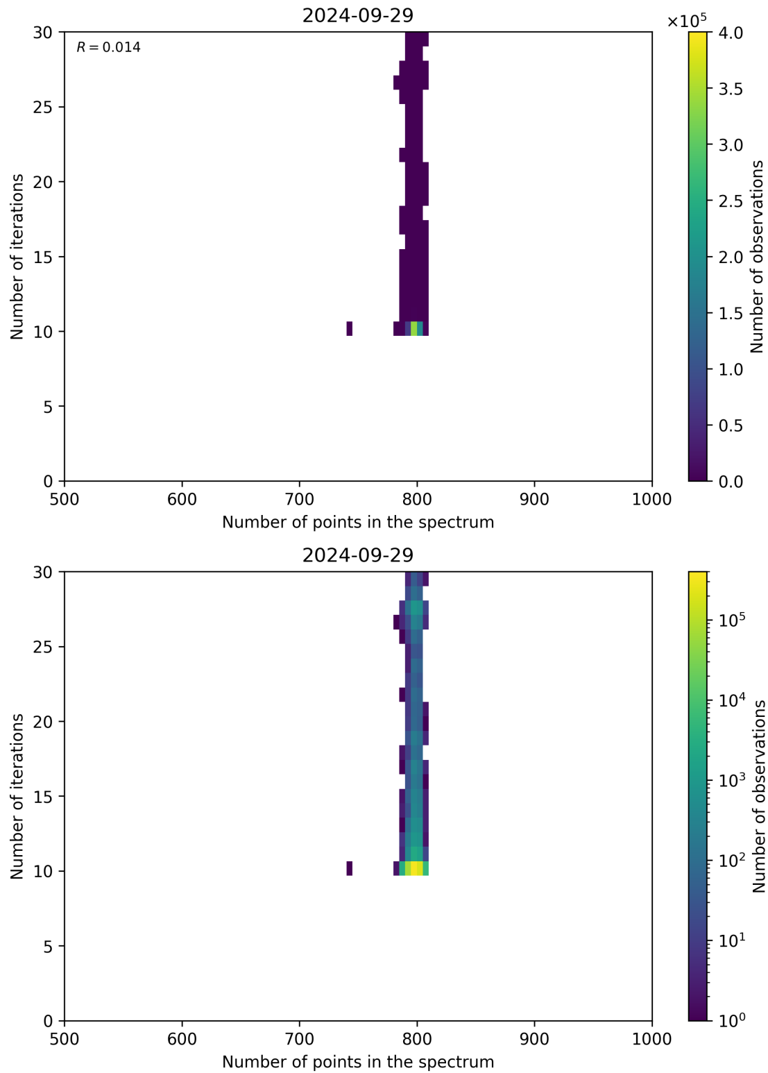
Figure 92: Scatter density plot of “Number of points in the spectrum” against “Number of iterations” for 2024-09-28 to 2024-09-30.
