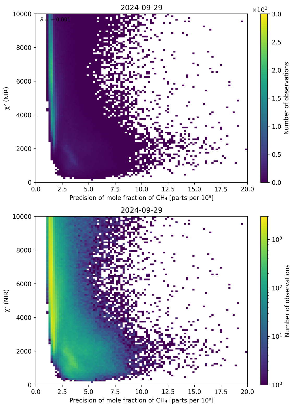
Figure 78: Scatter density plot of “Precision of mole fraction of CH 4 ” against “ \chi^2 (NIR)” for 2024-09-28 to 2024-09-30.
