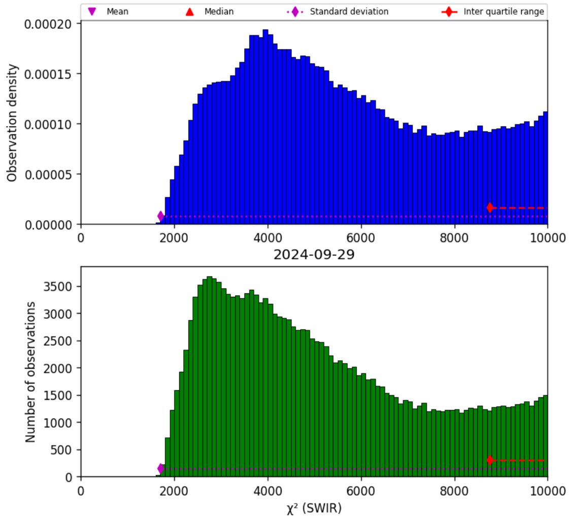
Figure 28: Histogram of “ \chi^2 (SWIR)” for 2024-09-28 to 2024-09-30
