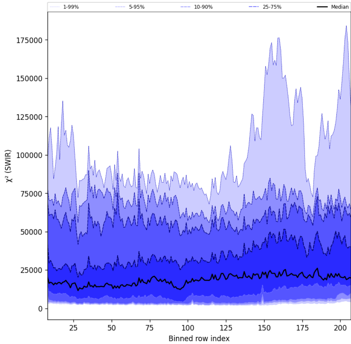
Figure 39: Along track statistics of “ \chi^2 (SWIR)” for 2024-09-28 to 2024-09-30
