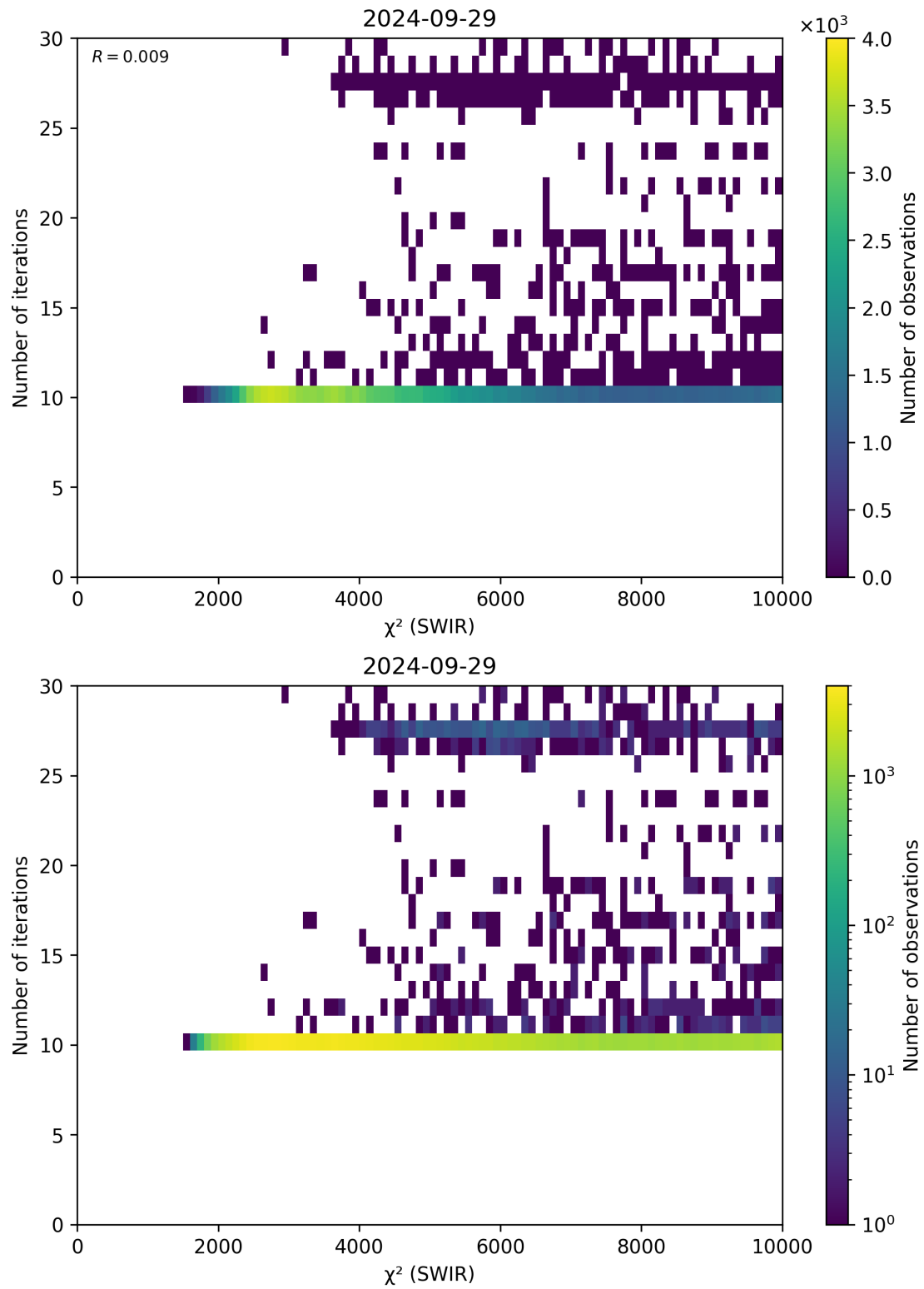
Figure 50: Scatter density plot of “ \chi^2 (SWIR)” against “Number of iterations” for 2024-09-28 to 2024-09-30.
