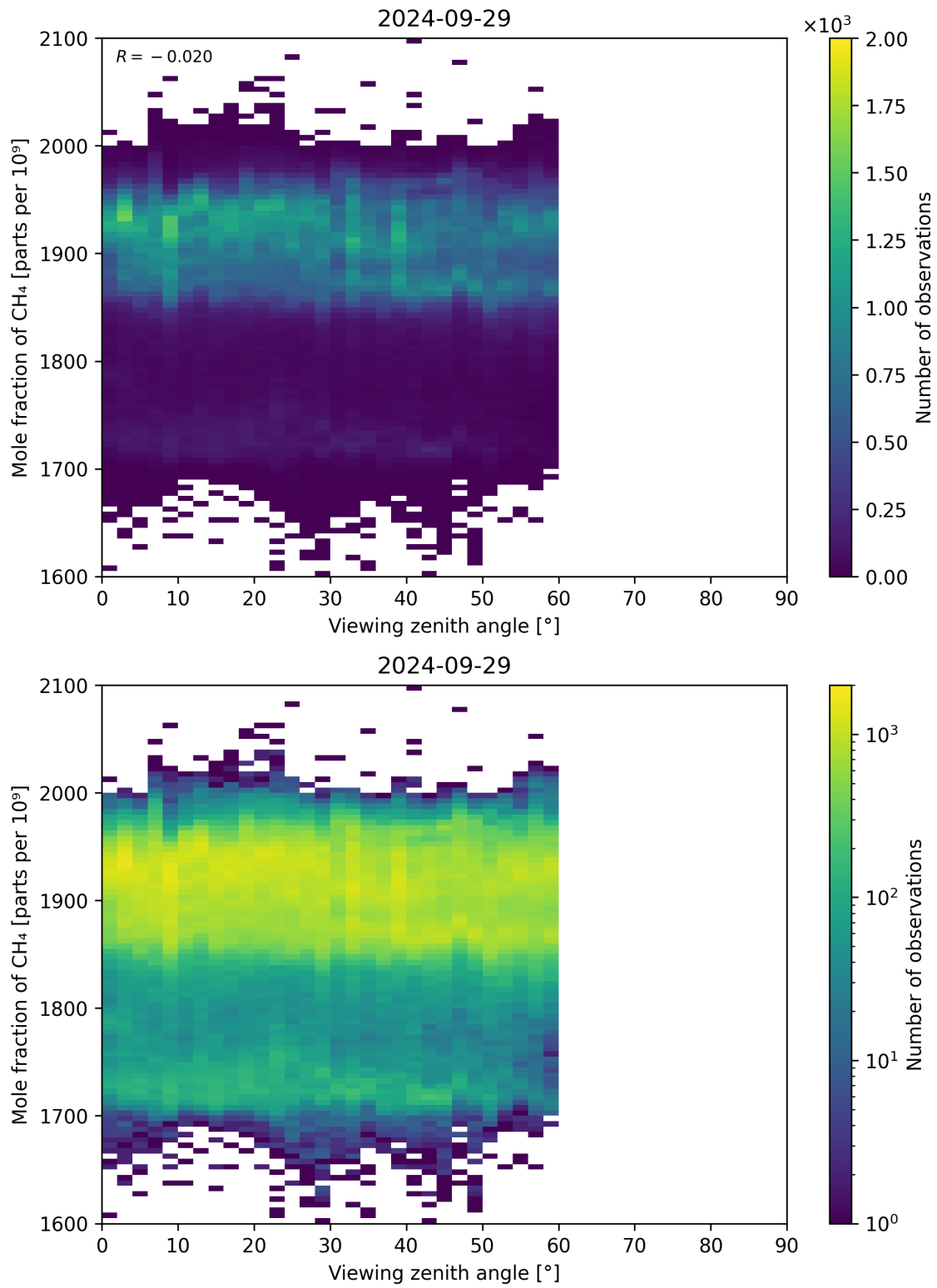
Figure 110: Scatter density plot of “Viewing zenith angle” against “Mole fraction of CH 4 ” for 2024-09-28 to 2024-09-30.
