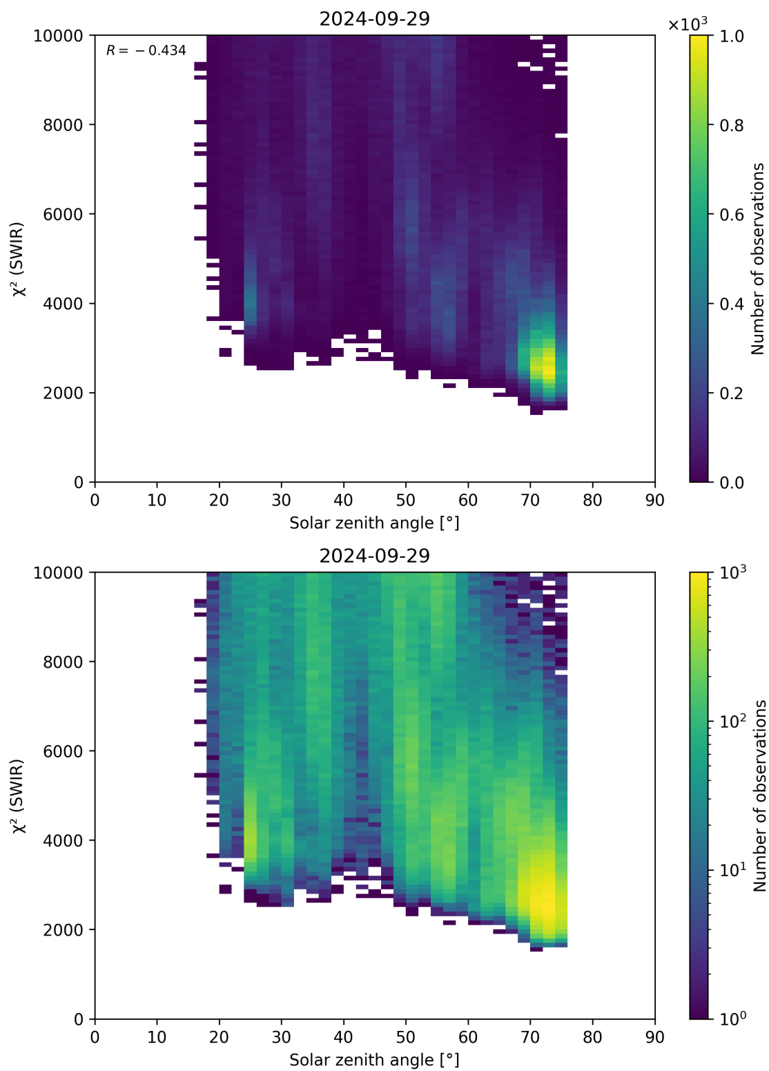
Figure 95: Scatter density plot of “Solar zenith angle” against “ \chi^2 (SWIR)” for 2024-09-28 to 2024-09-30.
