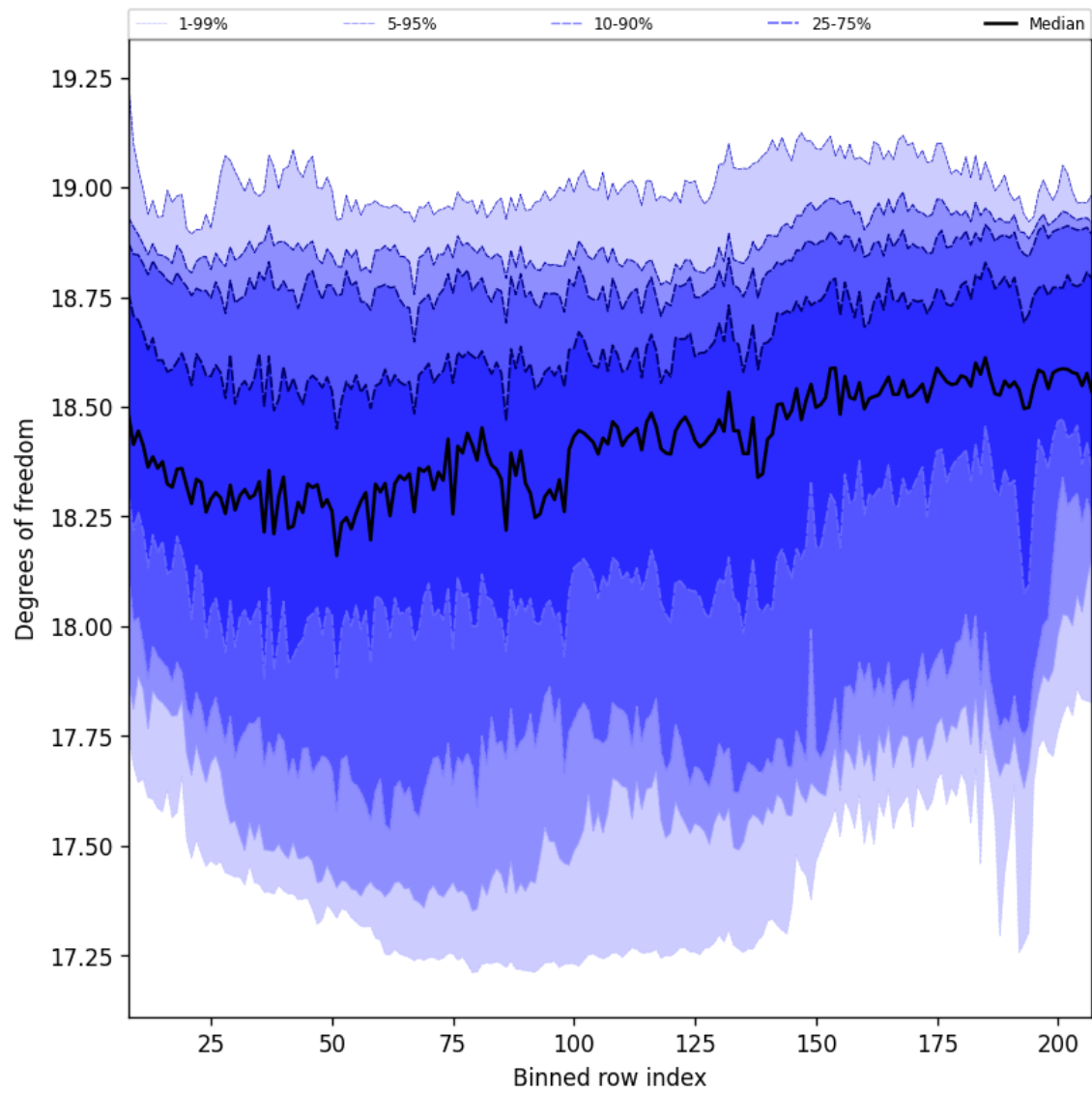
Figure 41: Along track statistics of “Degrees of freedom” for 2024-09-28 to 2024-09-30
