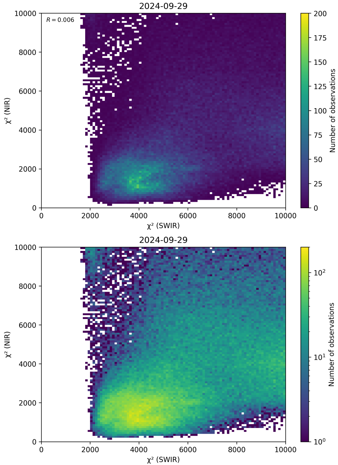
Figure 47: Scatter density plot of “ \chi^2 (SWIR)” against “ \chi^2 (NIR)” for 2024-09-28 to 2024-09-30.
