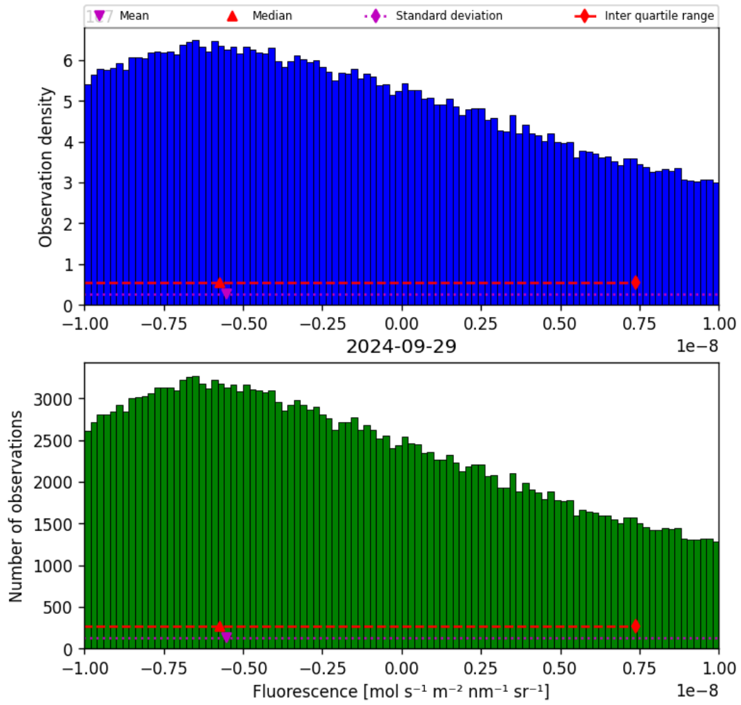
Figure 32: Histogram of “Fluorescence” for 2024-09-28 to 2024-09-30
