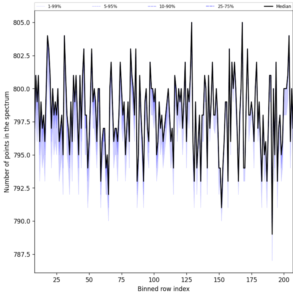
Figure 37: Along track statistics of “Number of points in the spectrum” for 2024-09-28 to 2024-09-30
