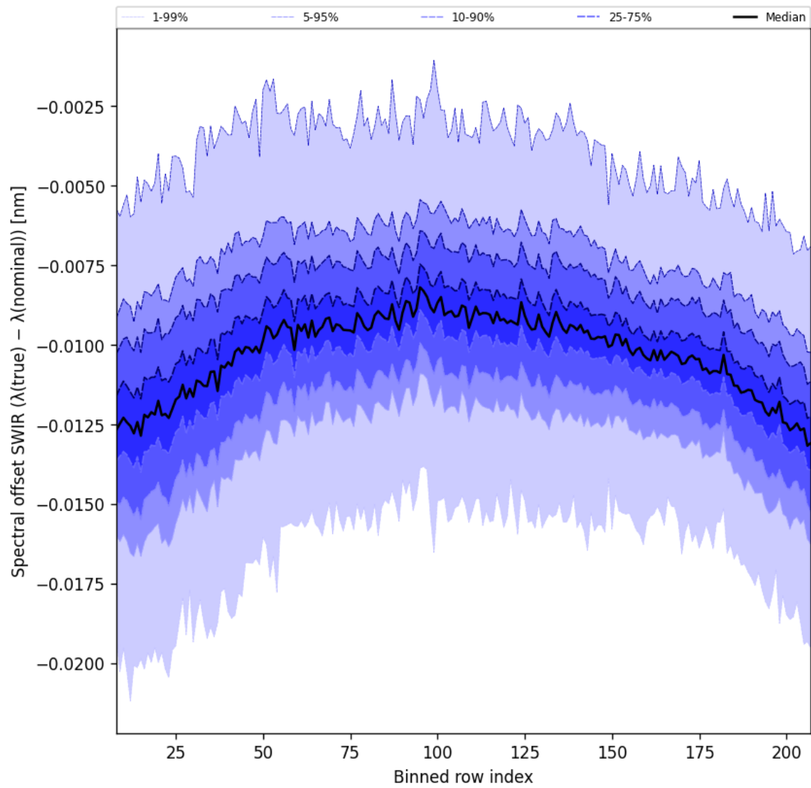
Figure 38: Along track statistics of “Spectral offset SWIR ( \lambda_{\text{true}} - \lambda_{\text{nominal}} )” for 2024-09-28 to 2024-09-30
