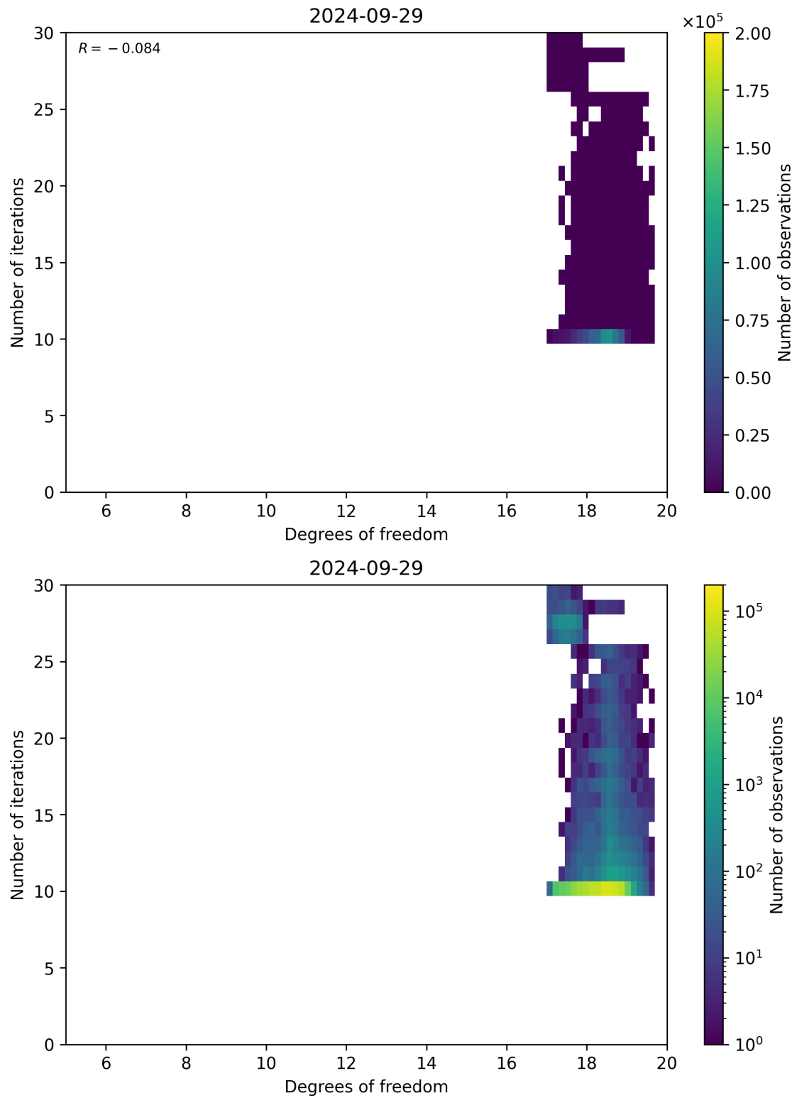
Figure 52: Scatter density plot of “Degrees of freedom” against “Number of iterations” for 2024-09-28 to 2024-09-30.
