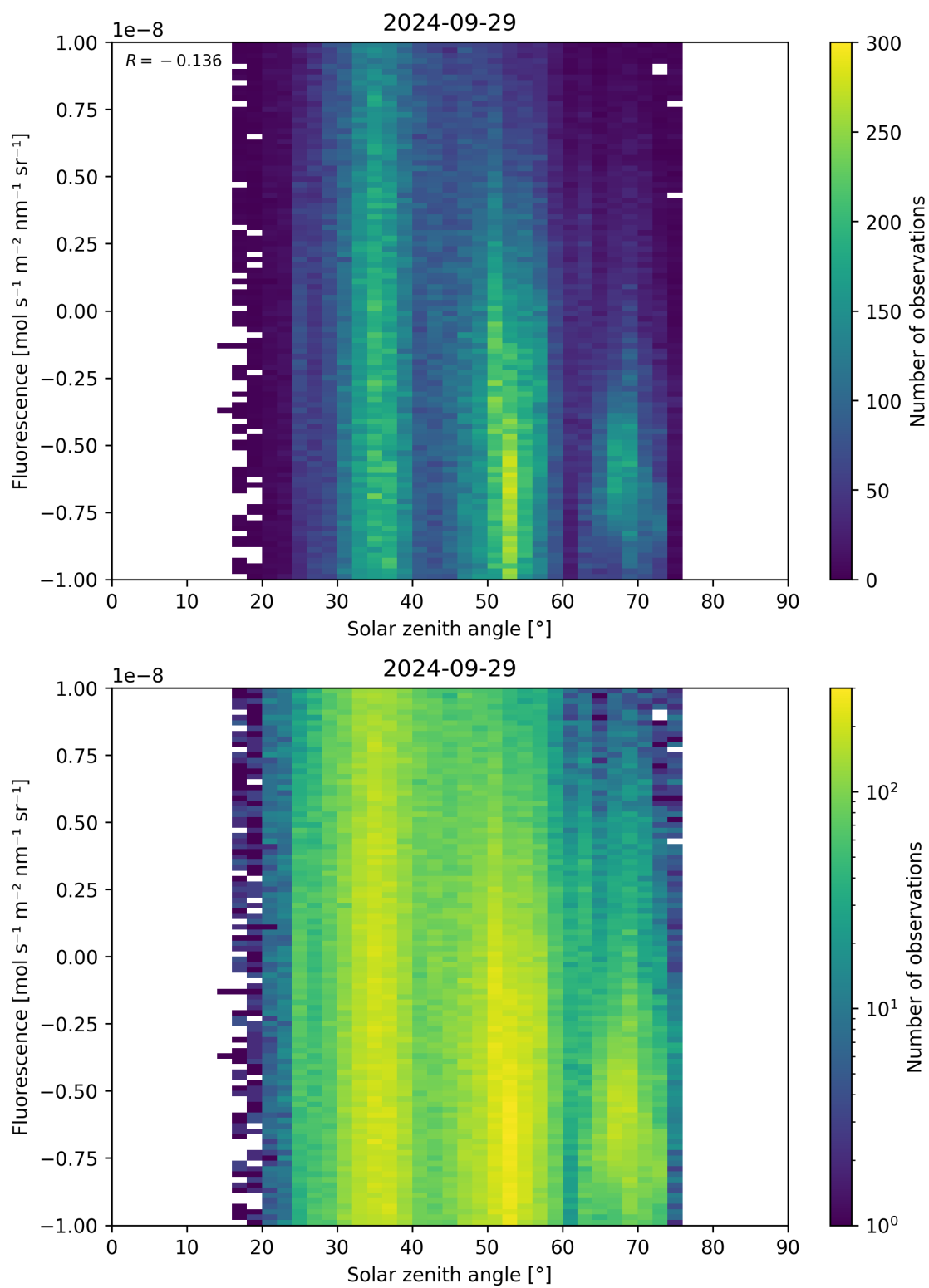
Figure 97: Scatter density plot of “Solar zenith angle” against “Fluorescence” for 2024-09-28 to 2024-09-30.
