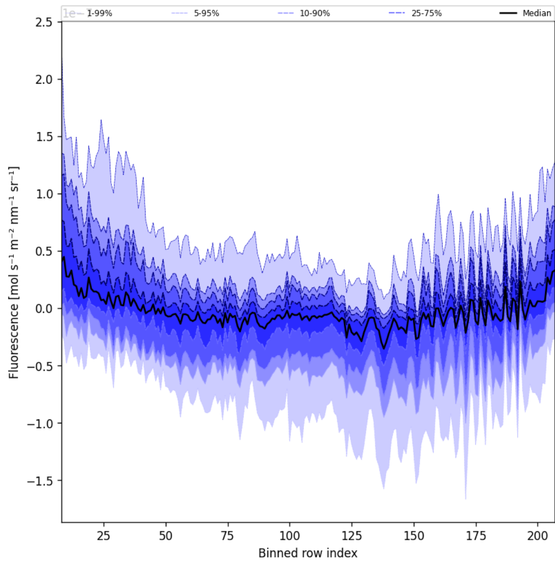
Figure 43: Along track statistics of “Fluorescence” for 2024-09-28 to 2024-09-30
