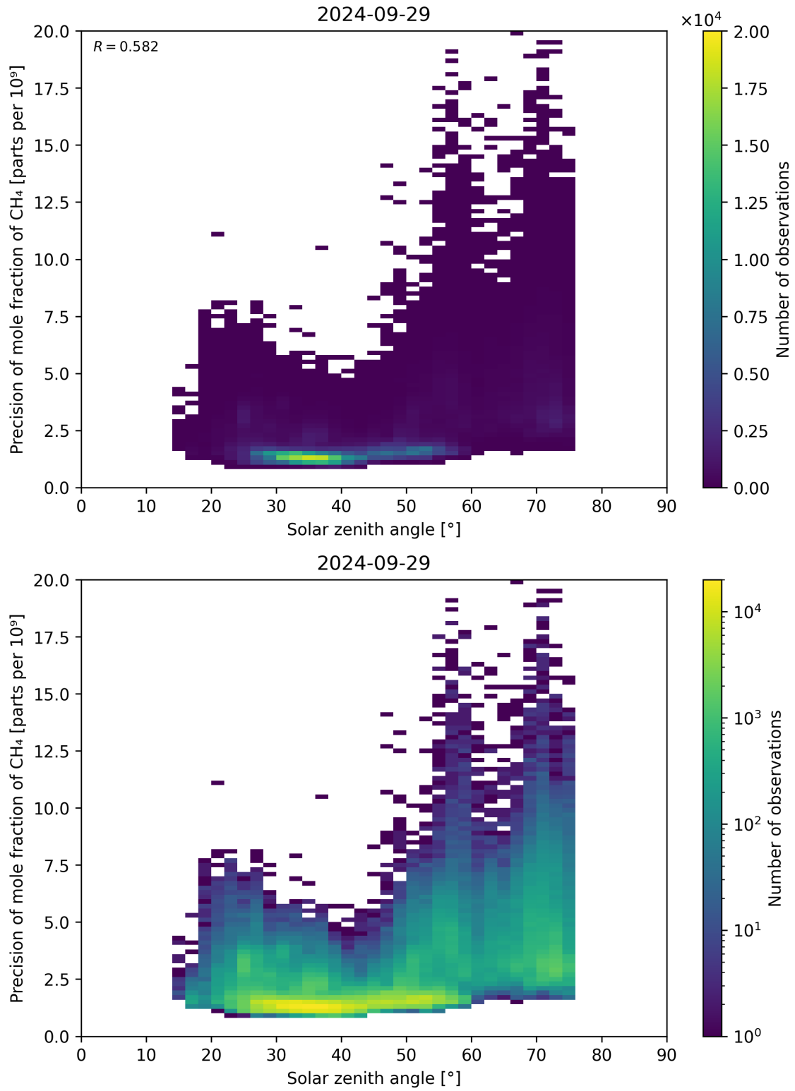
Figure 101: Scatter density plot of “Solar zenith angle” against “Precision of mole fraction of \text{CH}_4 ” for 2024-09-28 to 2024-09-30.
