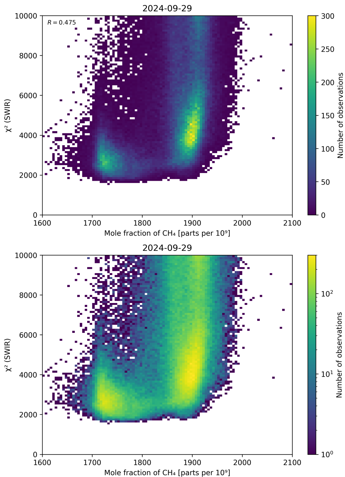
Figure 71: Scatter density plot of “Mole fraction of \text{CH}_4 ” against “ \chi^2 (SWIR)” for 2024-09-28 to 2024-09-30.
