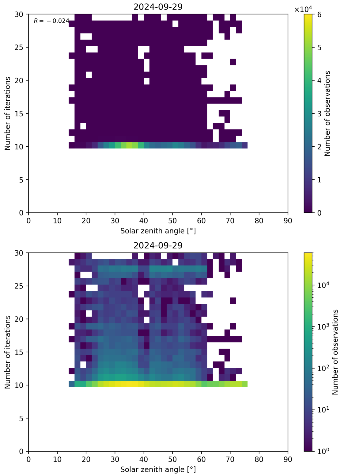
Figure 102: Scatter density plot of “Solar zenith angle” against “Number of iterations” for 2024-09-28 to 2024-09-30.
