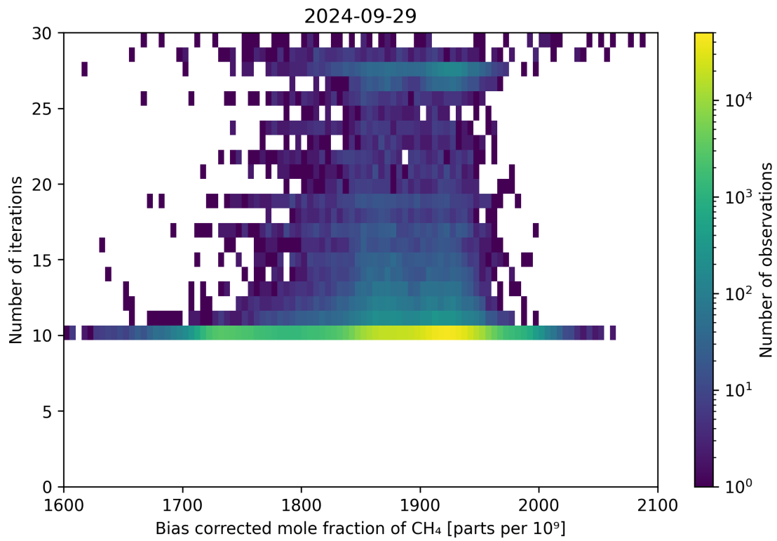
Figure 67: Scatter density plot of “Bias corrected mole fraction of CH 4 ” against “Number of iterations” for 2024-09-28 to 2024-09-30.
