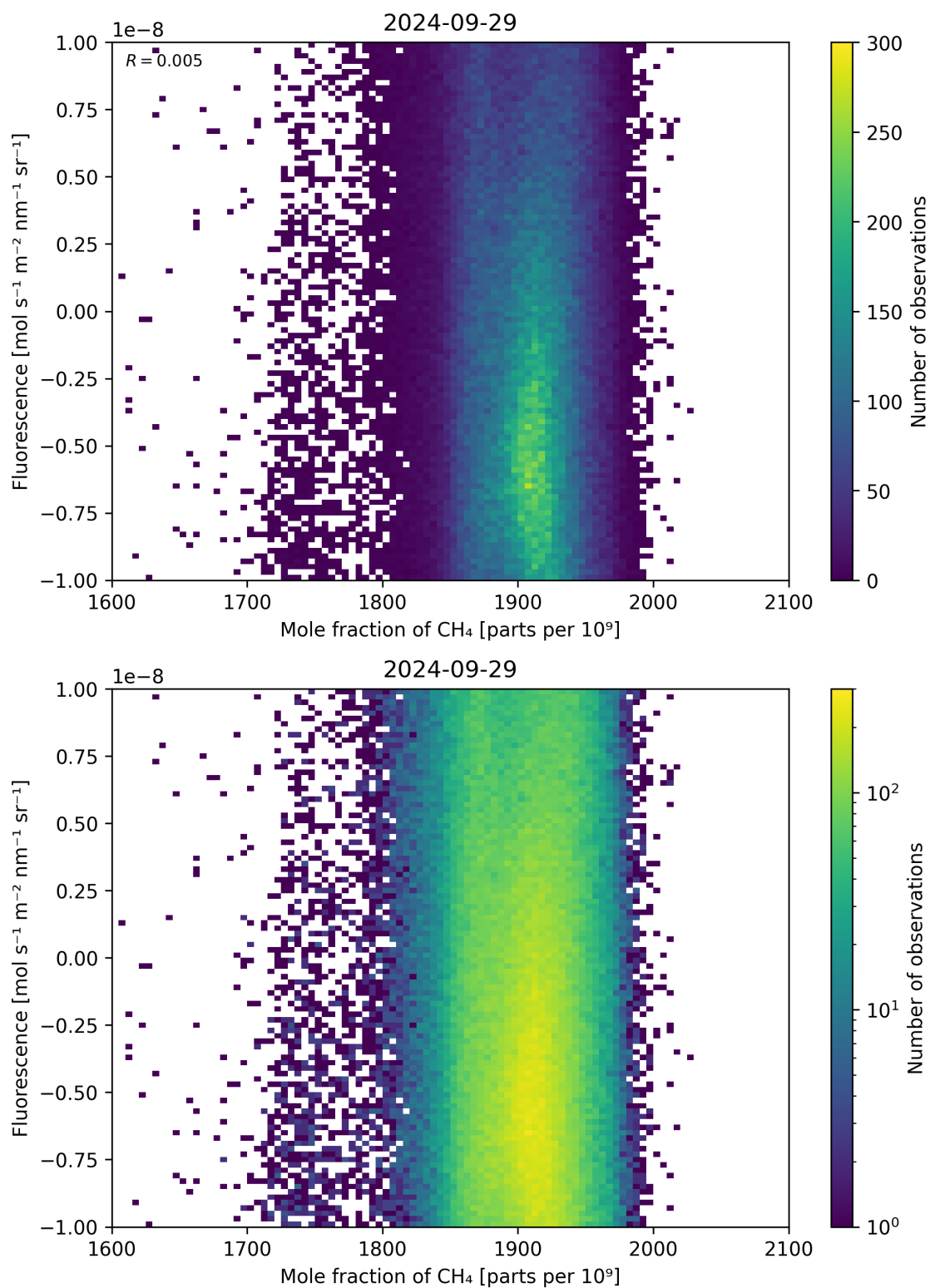
Figure 73: Scatter density plot of “Mole fraction of \text{CH}_4 ” against “Fluorescence” for 2024-09-28 to 2024-09-30.
