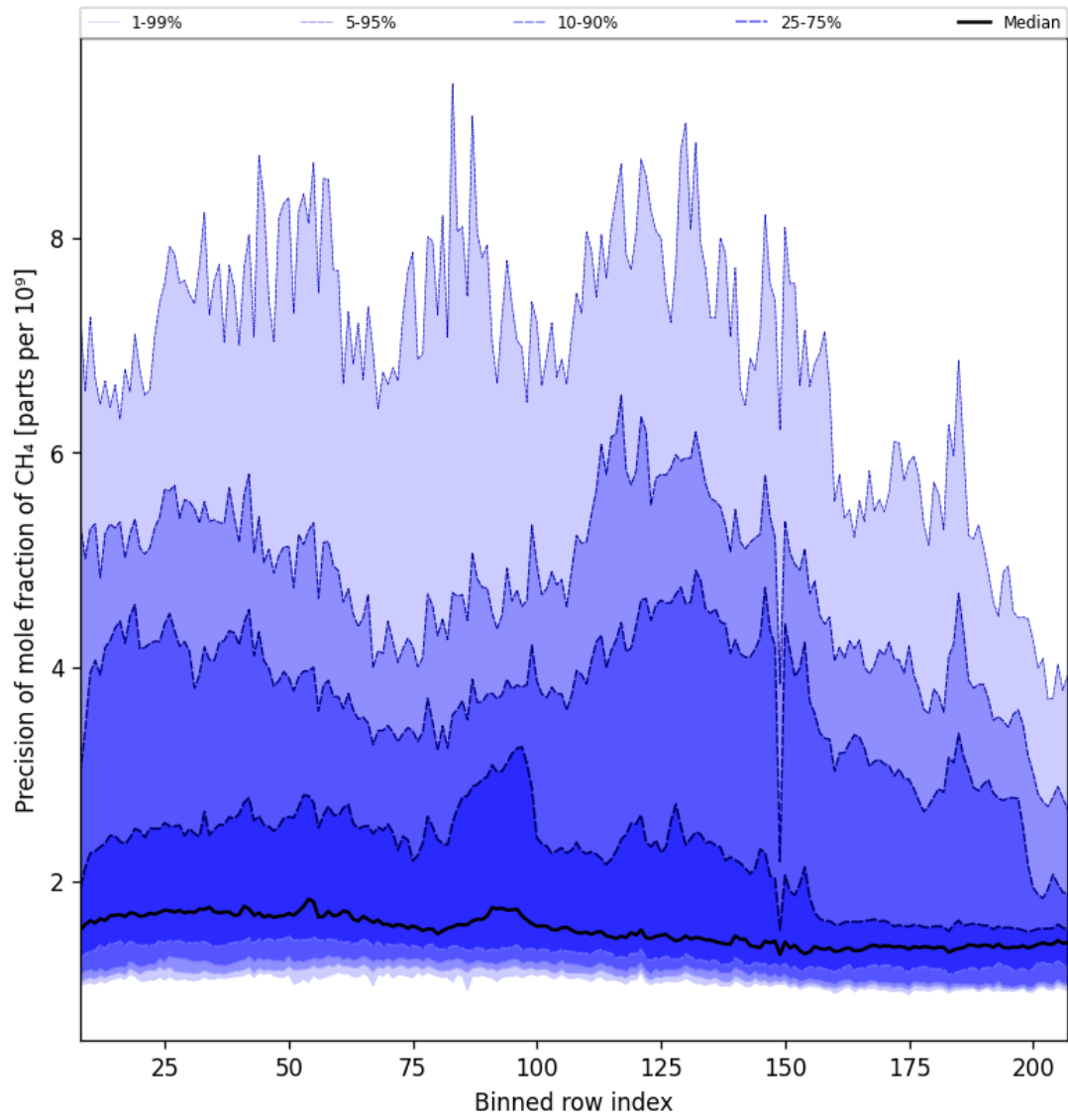
Figure 35: Along track statistics of “Precision of mole fraction of CH 4 ” for 2024-09-28 to 2024-09-30
