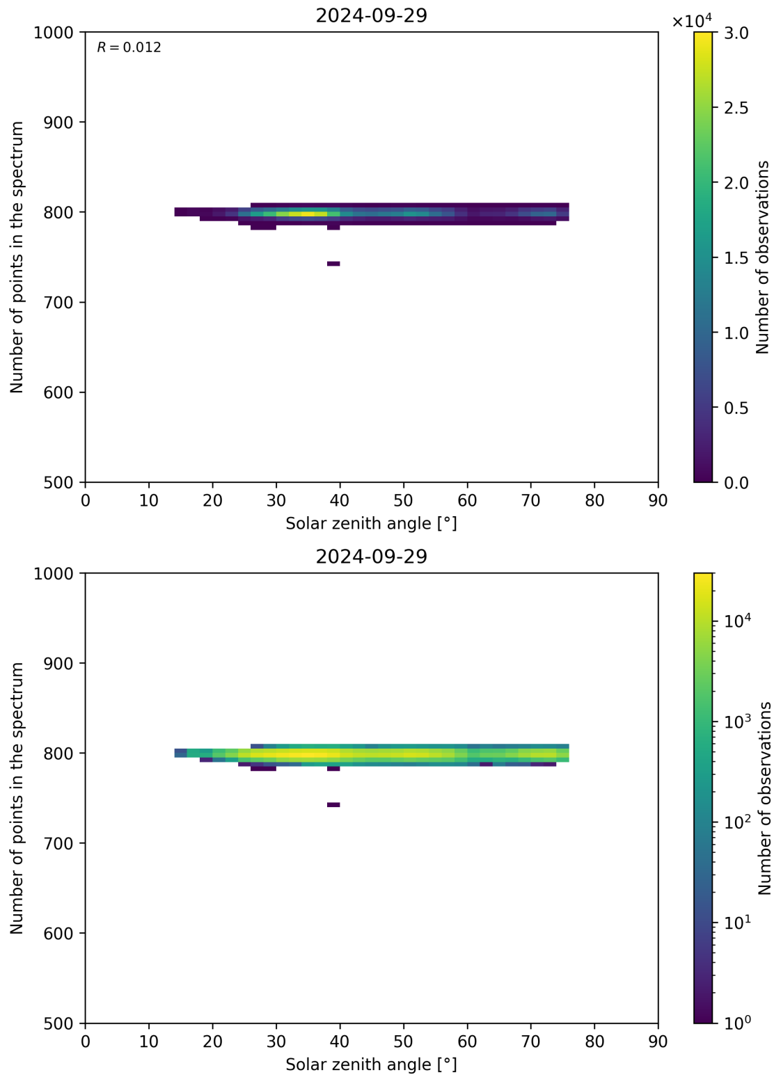
Figure 103: Scatter density plot of “Solar zenith angle” against “Number of points in the spectrum” for 2024-09-28 to 2024-09-30.
