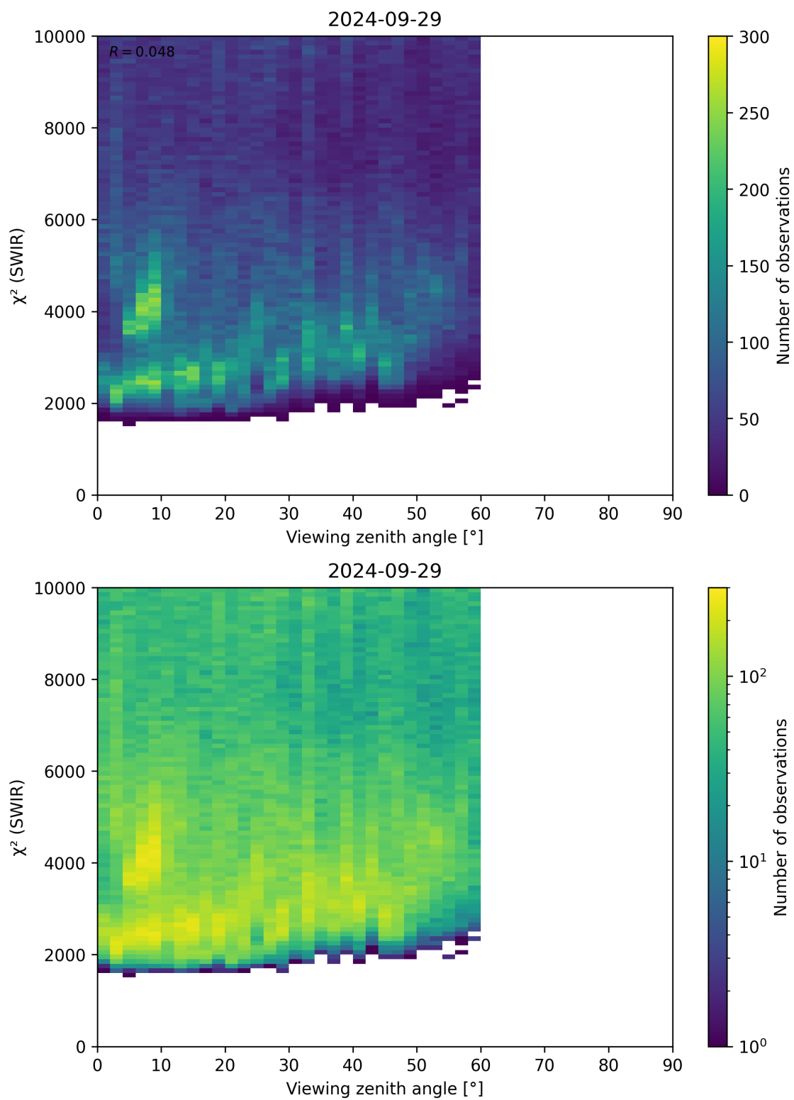
Figure 106: Scatter density plot of “Viewing zenith angle” against “ \chi^2 (SWIR)” for 2024-09-28 to 2024-09-30.
