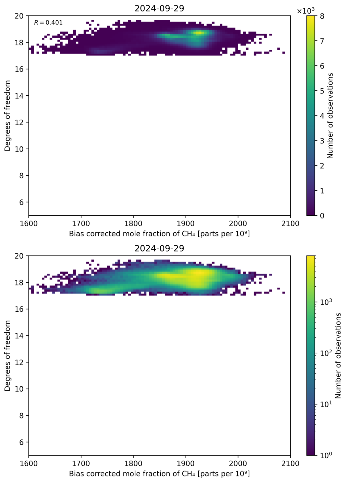
Figure 65: Scatter density plot of “Bias corrected mole fraction of CH 4 ” against “Degrees of freedom” for 2024-09-28 to 2024-09-30.
