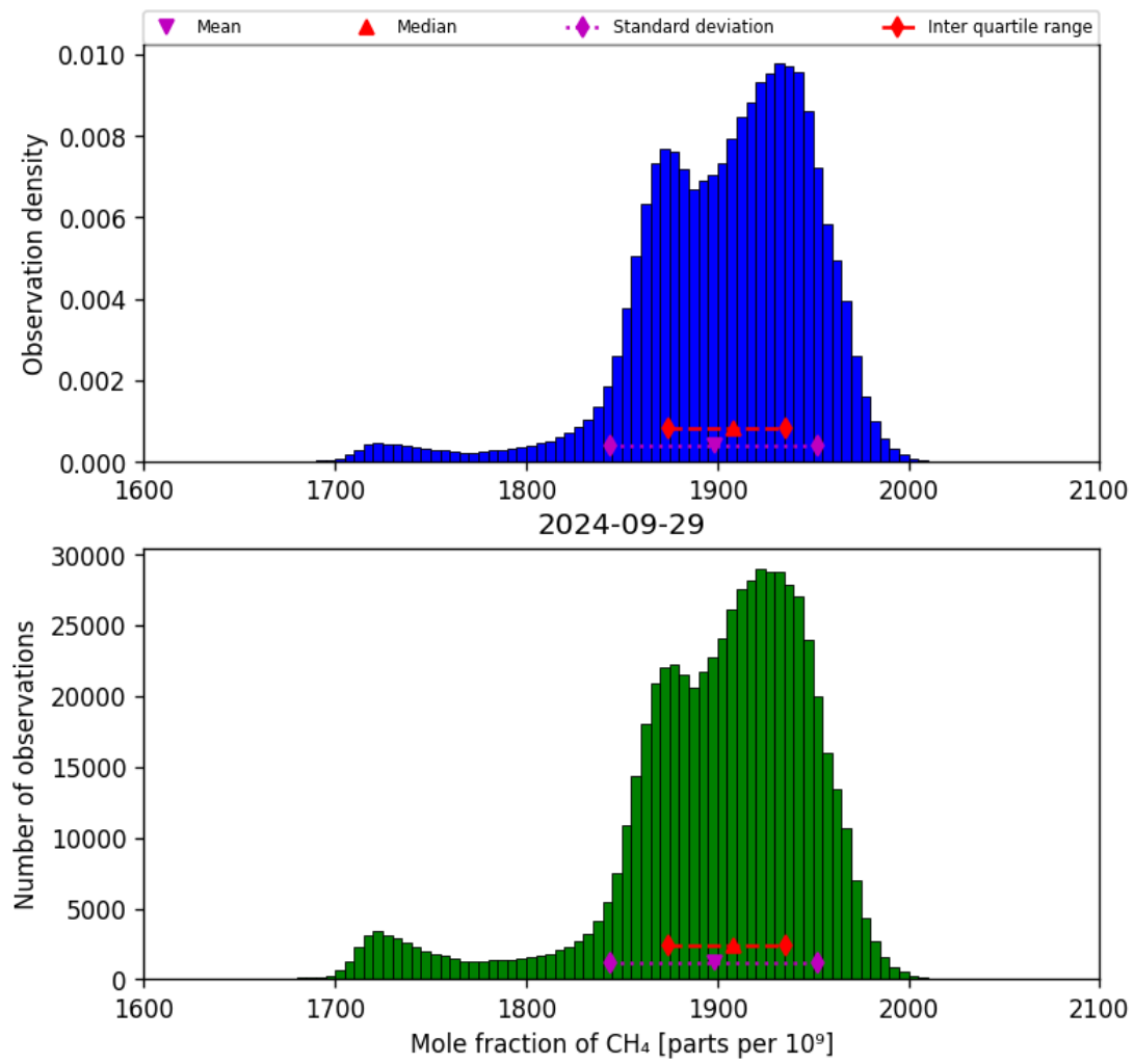
Figure 23: Histogram of “Mole fraction of CH 4 ” for 2024-09-28 to 2024-09-30
