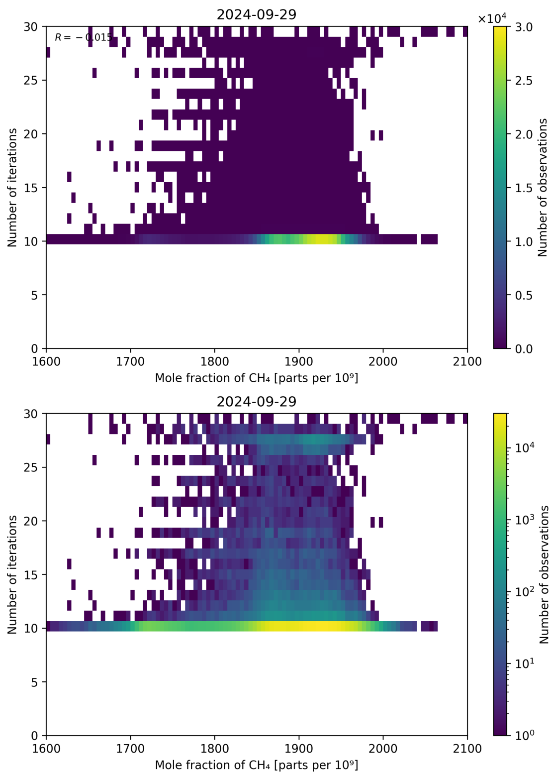
Figure 76: Scatter density plot of “Mole fraction of CH 4 ” against “Number of iterations” for 2024-09-28 to 2024-09-30.
