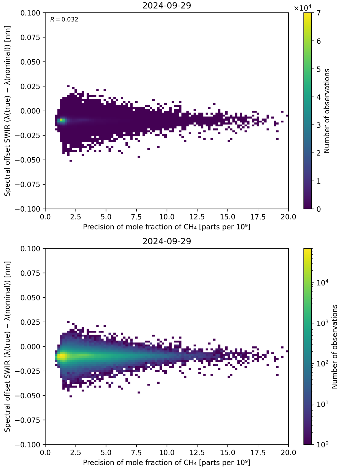
Figure 85: Scatter density plot of “Precision of mole fraction of CH 4 ” against “Spectral offset SWIR ( \lambda_{\text{true}} - \lambda_{\text{nominal}} )” for 2024-09-28 to 2024-09-30.
