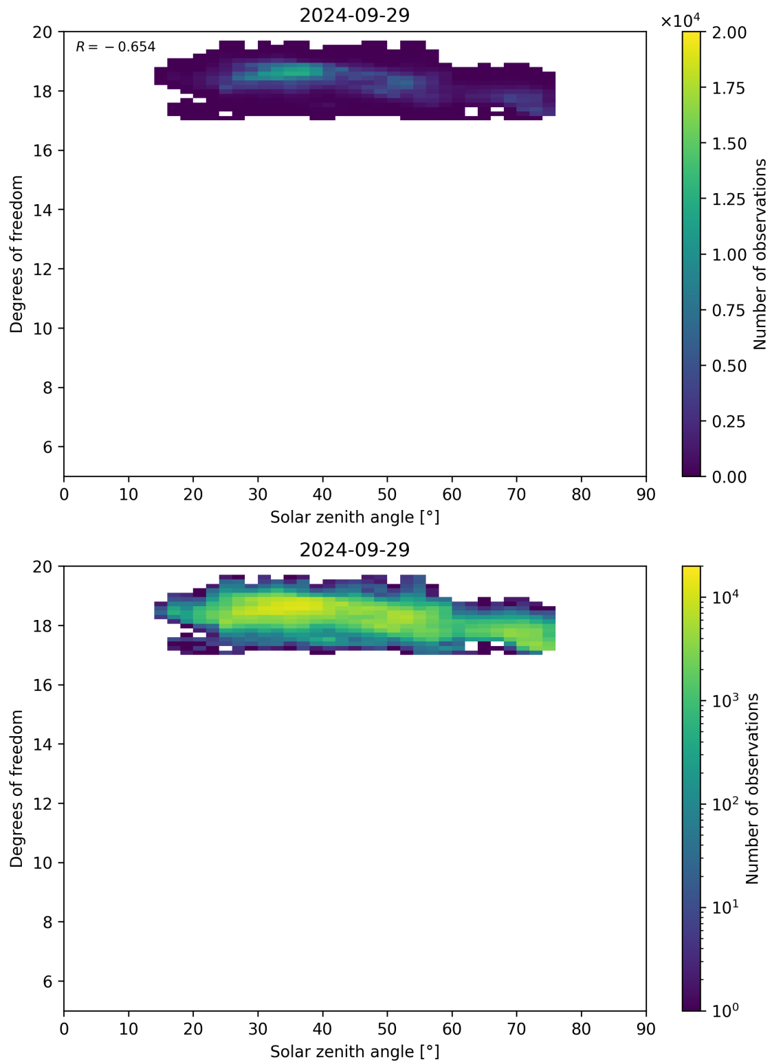
Figure 96: Scatter density plot of “Solar zenith angle” against “Degrees of freedom” for 2024-09-28 to 2024-09-30.
