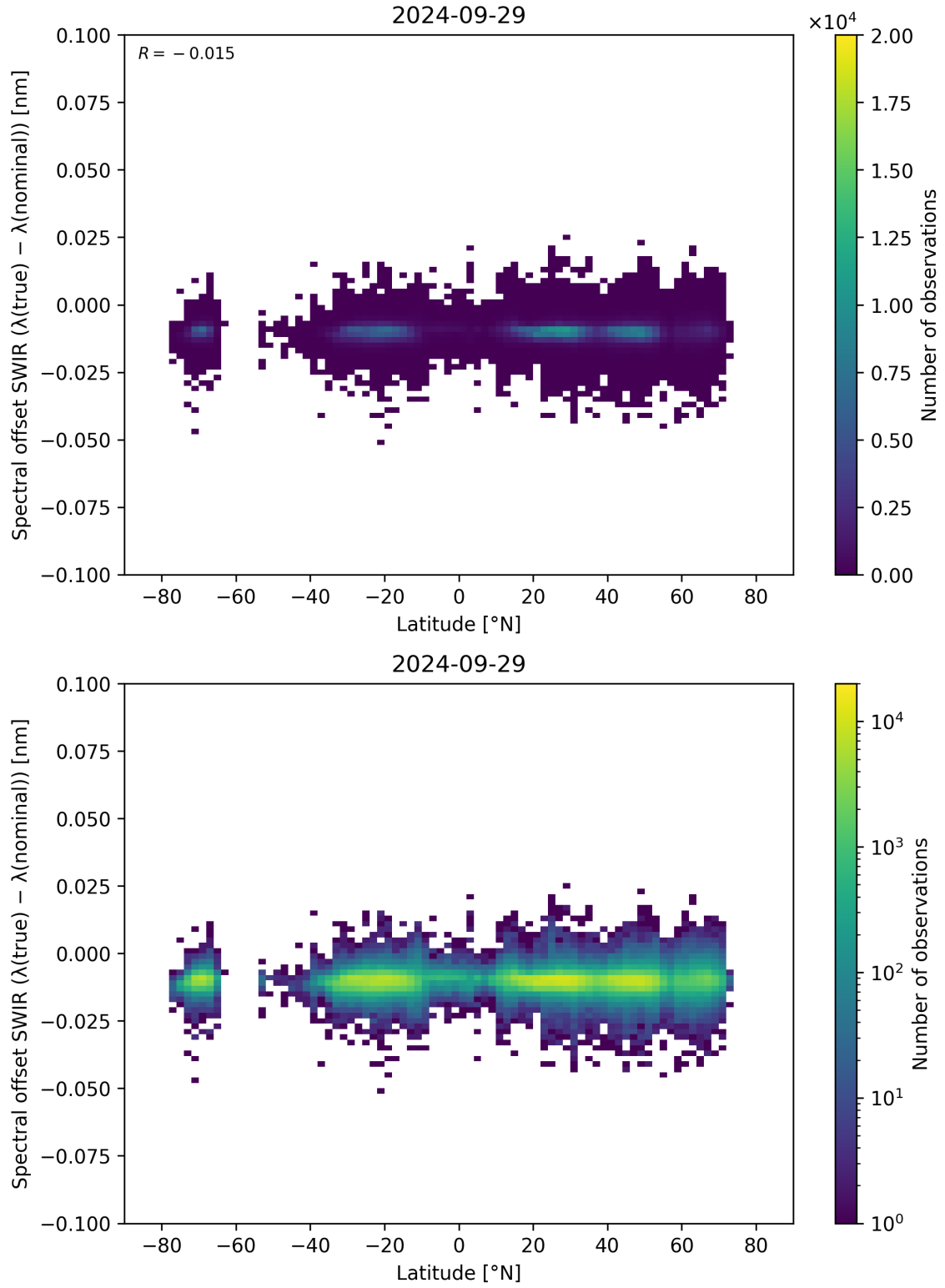
Figure 62: Scatter density plot of “Latitude” against “Spectral offset SWIR ( \lambda_{\text{true}} - \lambda_{\text{nominal}} )” for 2024-09-28 to 2024-09-30.
