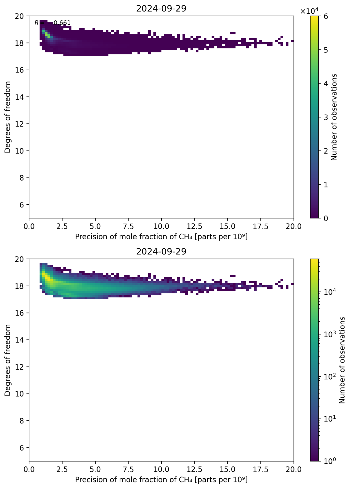
Figure 80: Scatter density plot of “Precision of mole fraction of CH 4 ” against “Degrees of freedom” for 2024-09-28 to 2024-09-30.
