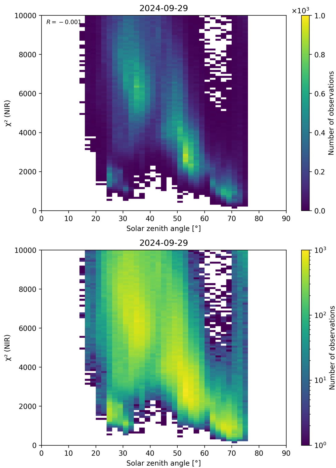
Figure 94: Scatter density plot of “Solar zenith angle” against “ \chi^2 (NIR)” for 2024-09-28 to 2024-09-30.
