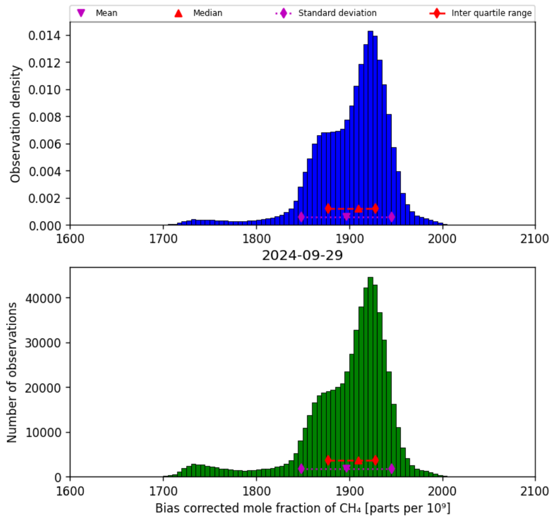
Figure 25: Histogram of “Bias corrected mole fraction of CH 4 ” for 2024-09-28 to 2024-09-30
