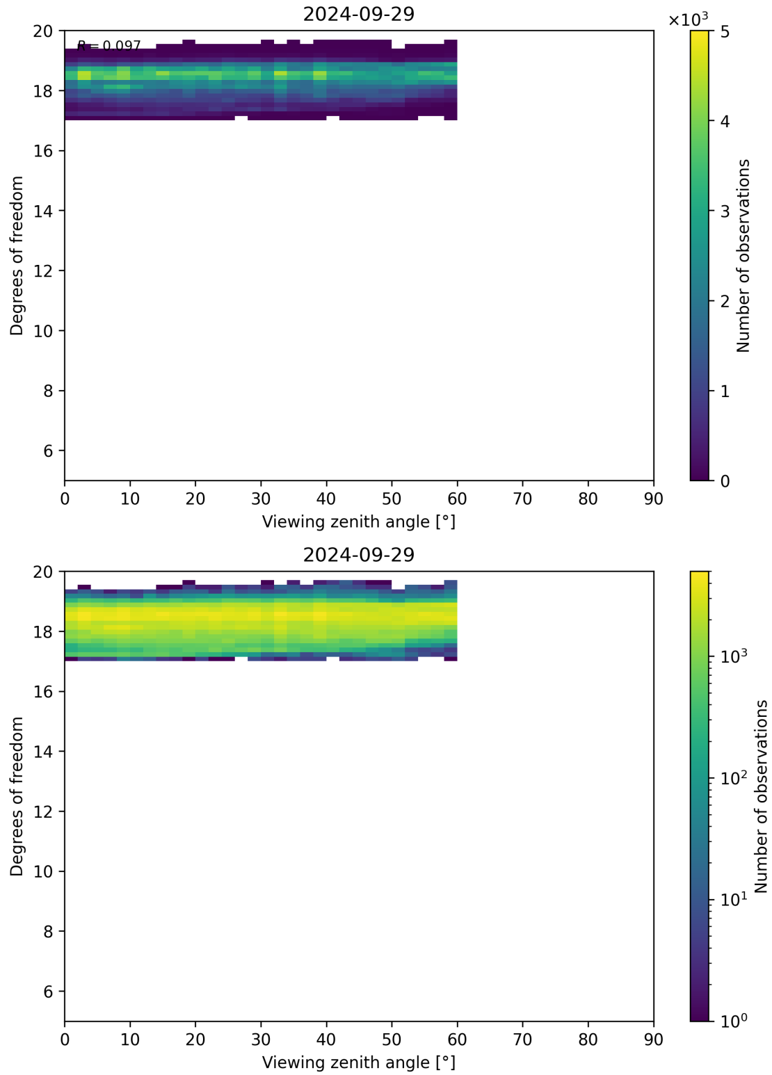
Figure 107: Scatter density plot of “Viewing zenith angle” against “Degrees of freedom” for 2024-09-28 to 2024-09-30.
