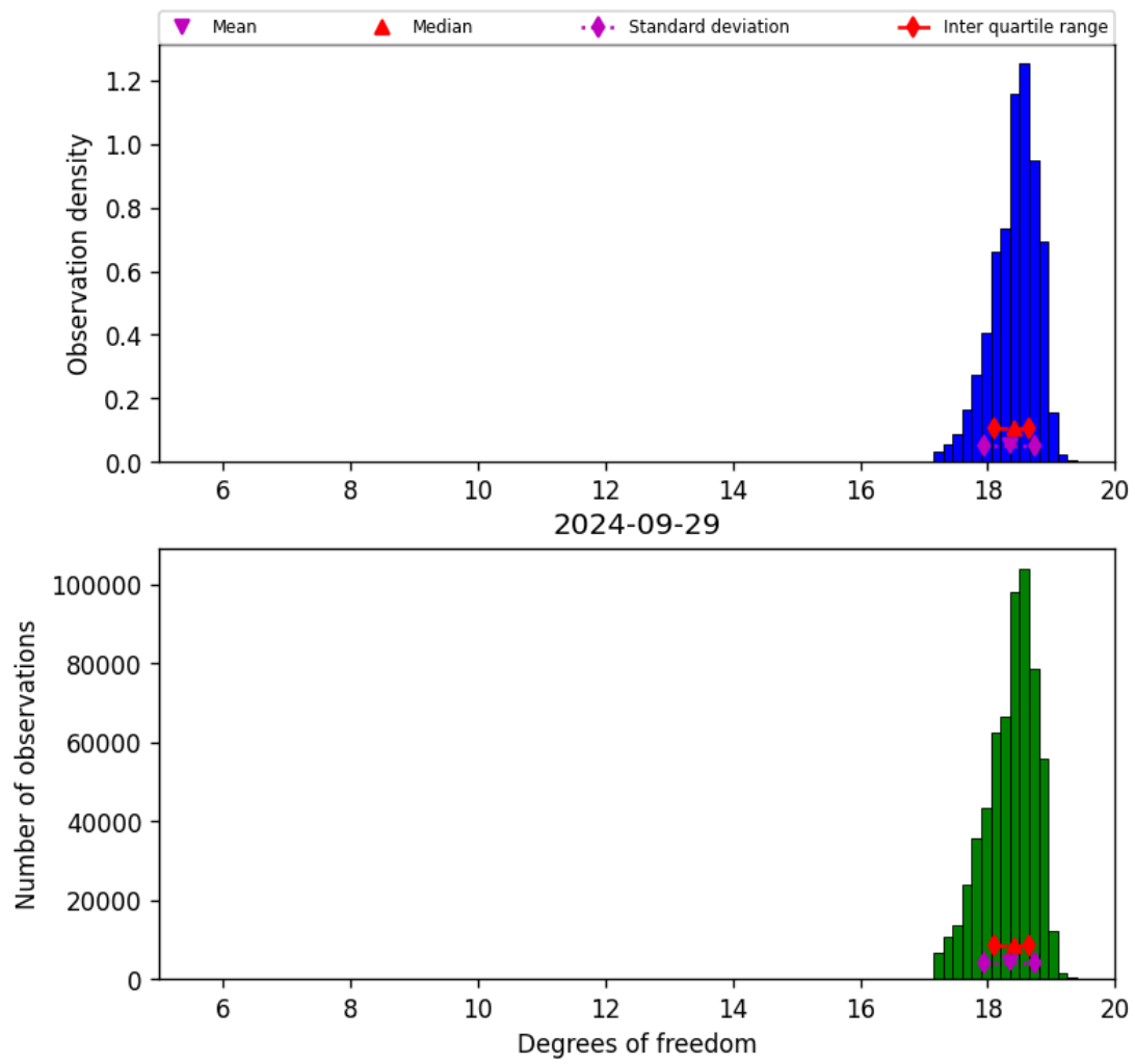
Figure 30: Histogram of “Degrees of freedom” for 2024-09-28 to 2024-09-30
