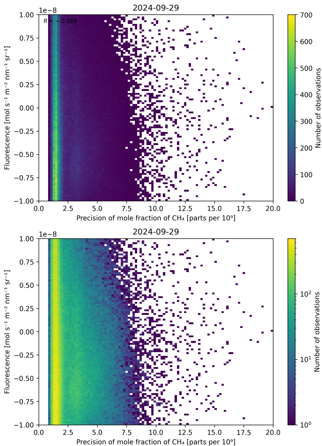
Figure 81: Scatter density plot of “Precision of mole fraction of \text{CH}_4 ” against “Fluorescence” for 2024-09-28 to 2024-09-30.
