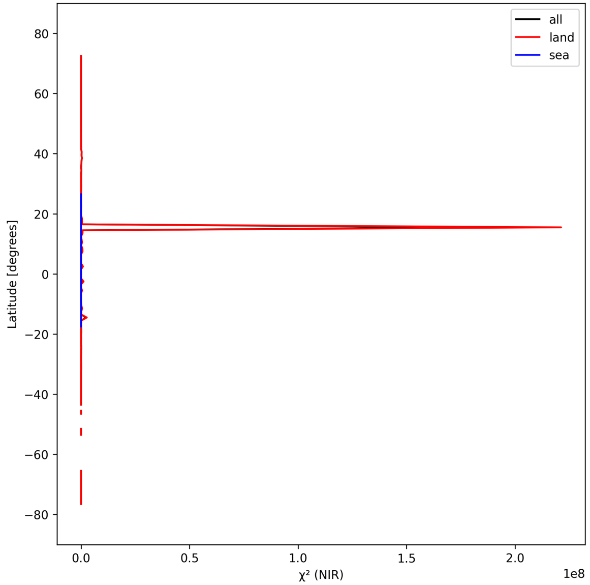
Figure 18: Zonal average of “ \chi^2 (NIR)” for 2024-09-28 to 2024-09-30.
