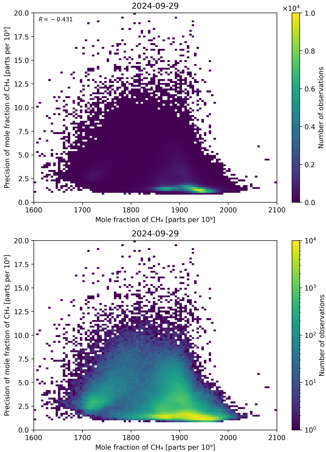
Figure 75: Scatter density plot of “Mole fraction of CH 4 ” against “Precision of mole fraction of CH 4 ” for 2024-09-28 to 2024-09-30.
