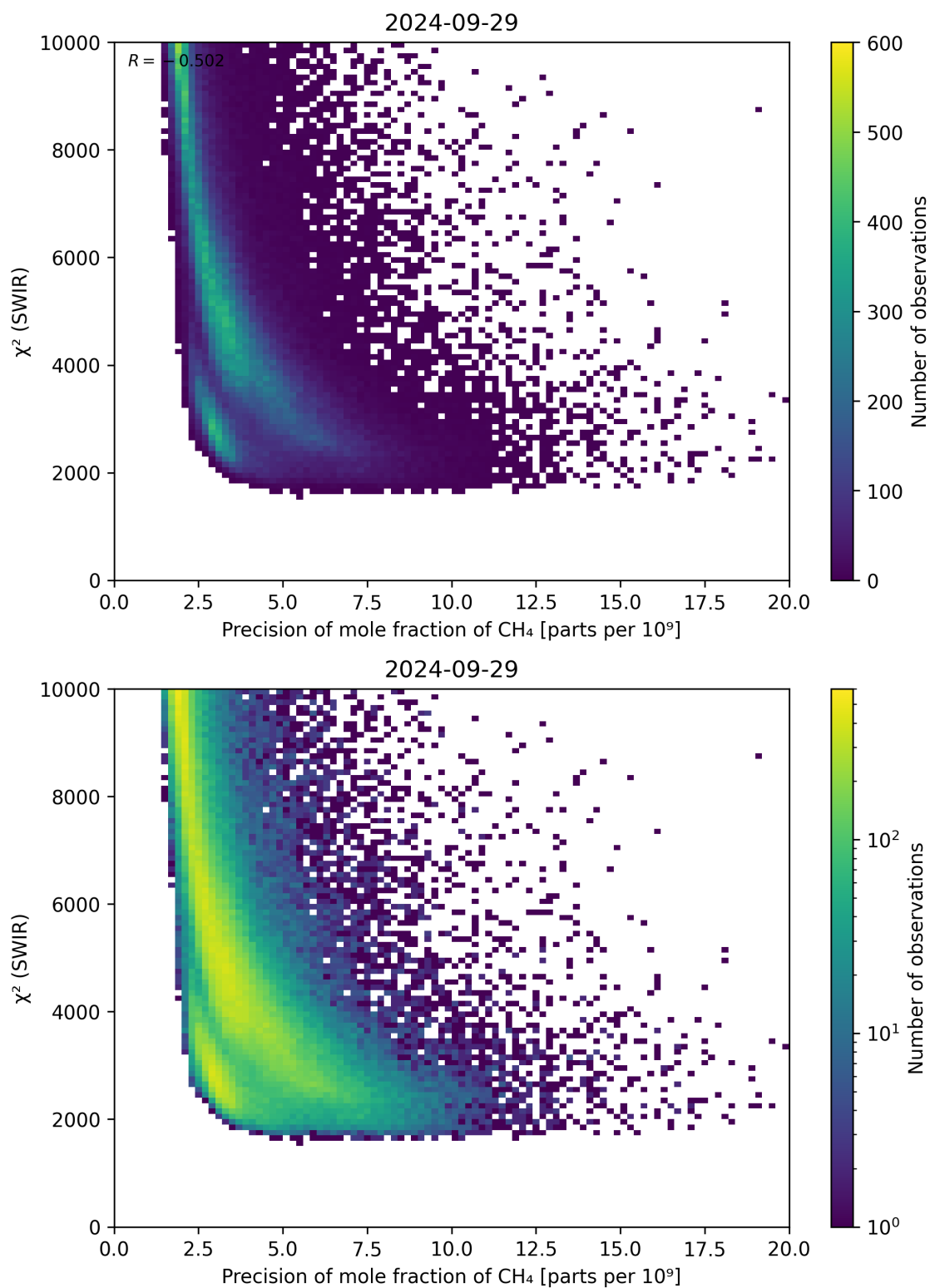
Figure 79: Scatter density plot of “Precision of mole fraction of \text{CH}_4 ” against “ \chi^2 (SWIR)” for 2024-09-28 to 2024-09-30.
