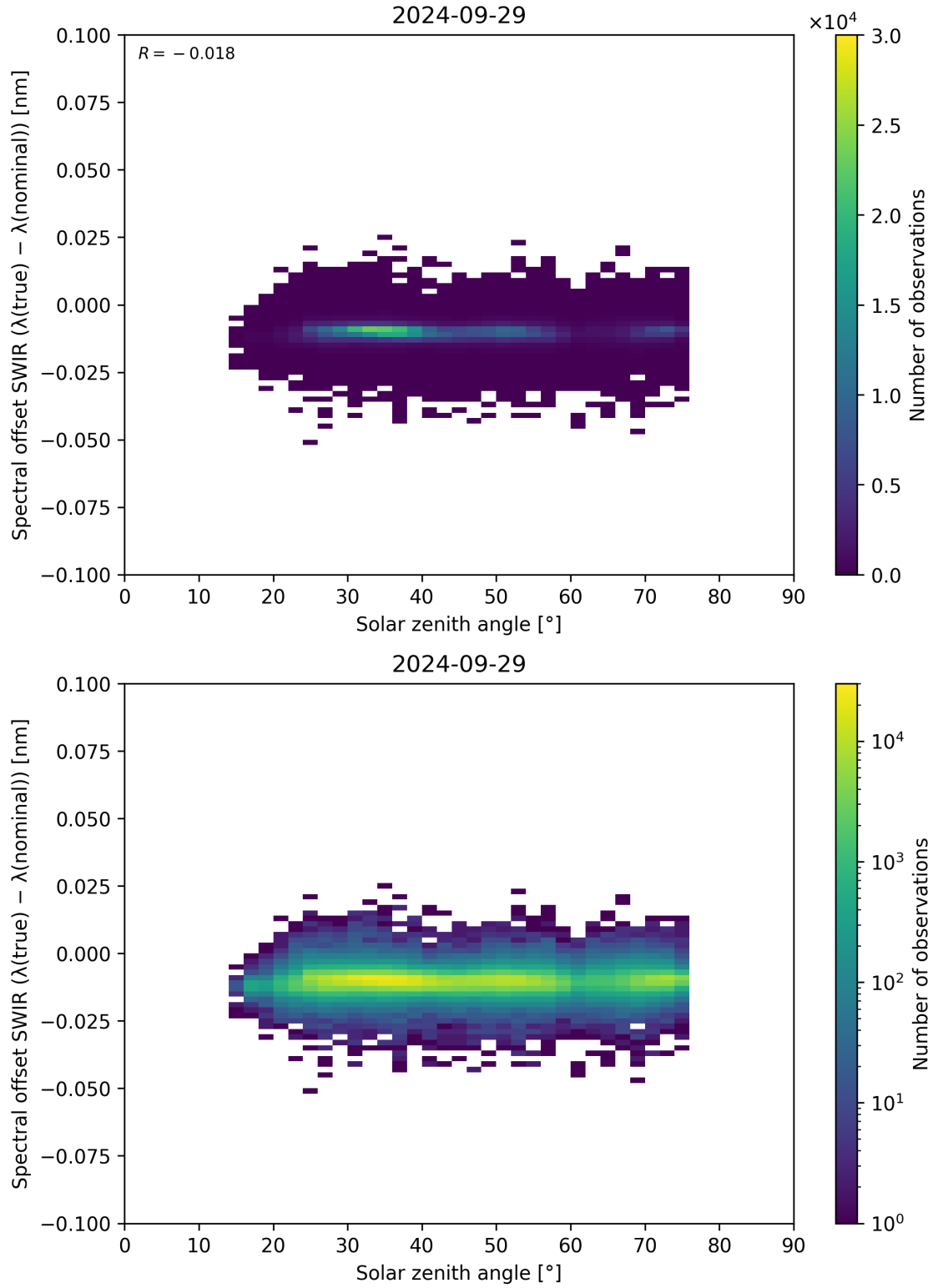
Figure 104: Scatter density plot of “Solar zenith angle” against “Spectral offset SWIR ( \lambda_{\text{true}} - \lambda_{\text{nominal}} )” for 2024-09-28 to 2024-09-30.
