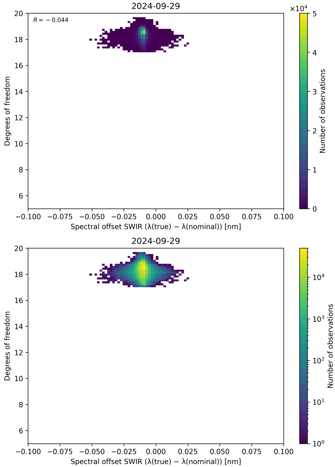
Figure 119: Scatter density plot of “Spectral offset SWIR ( \lambda_{\text{true}} - \lambda_{\text{nominal}} )” against “Degrees of freedom” for 2024-09-28 to 2024-09-30.
