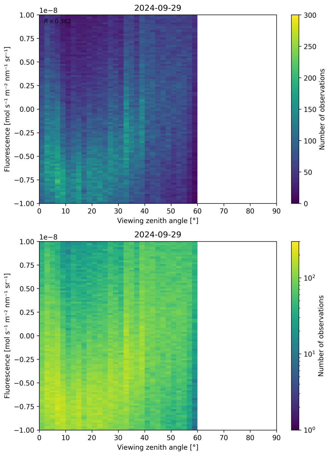
Figure 108: Scatter density plot of “Viewing zenith angle” against “Fluorescence” for 2024-09-28 to 2024-09-30.
