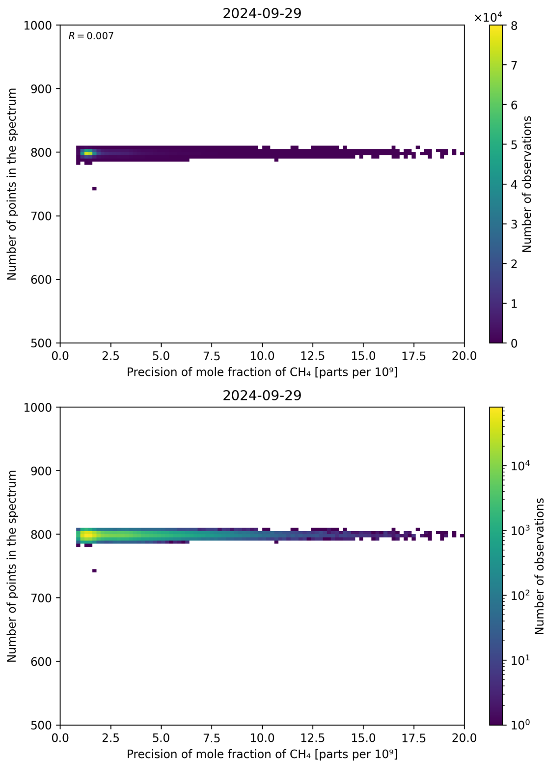
Figure 84: Scatter density plot of “Precision of mole fraction of CH 4 ” against “Number of points in the spectrum” for 2024-09-28 to 2024-09-30.
