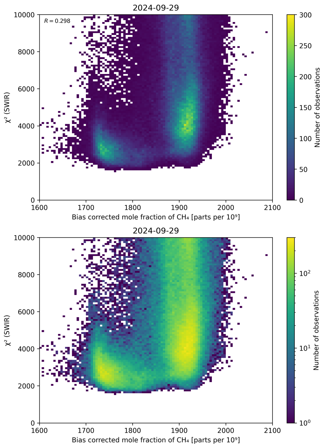
Figure 64: Scatter density plot of “Bias corrected mole fraction of \text{CH}_4 ” against “ \chi^2 (SWIR)” for 2024-09-28 to 2024-09-30.
