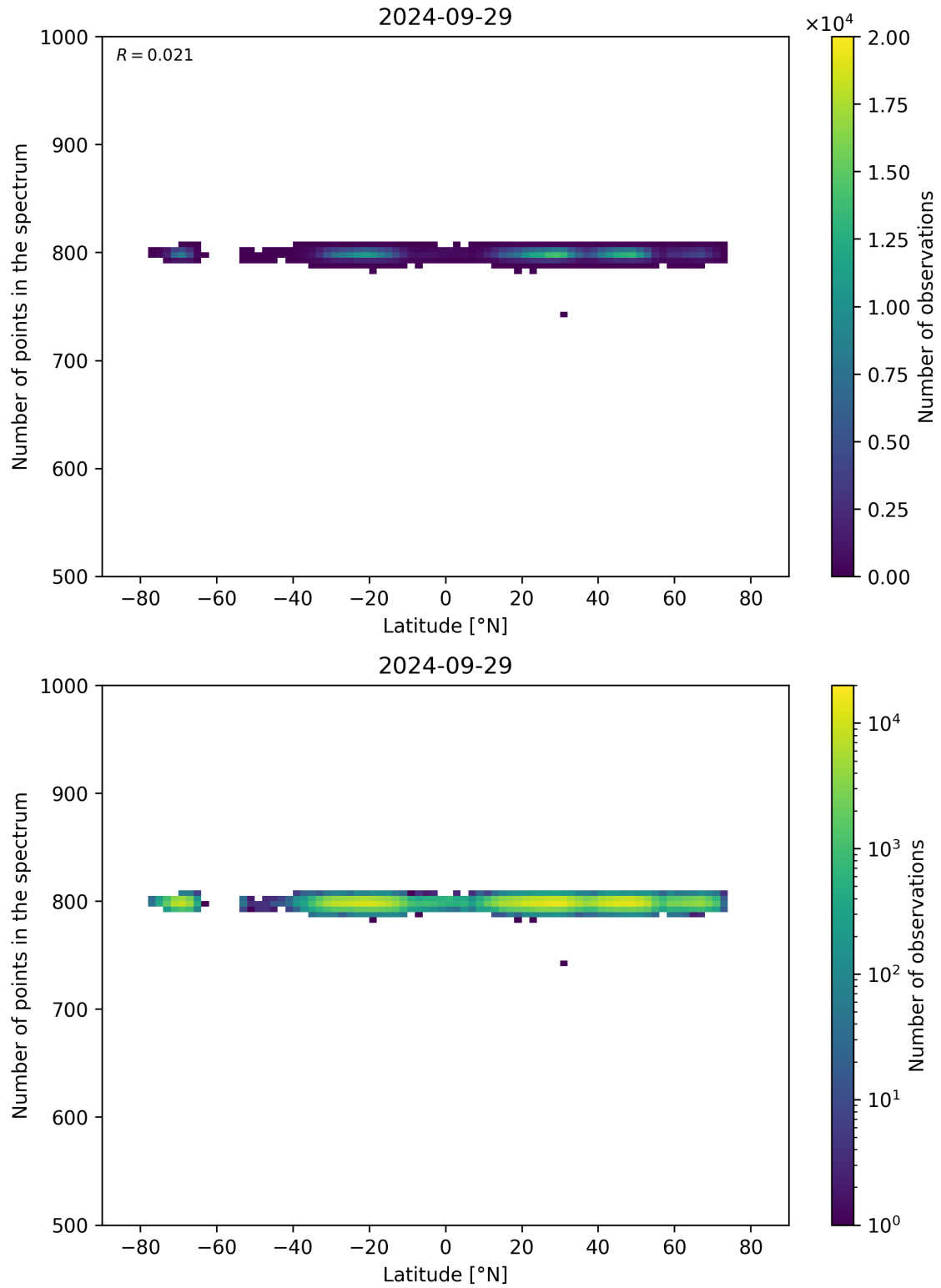
Figure 61: Scatter density plot of “Latitude” against “Number of points in the spectrum” for 2024-09-28 to 2024-09-30.
