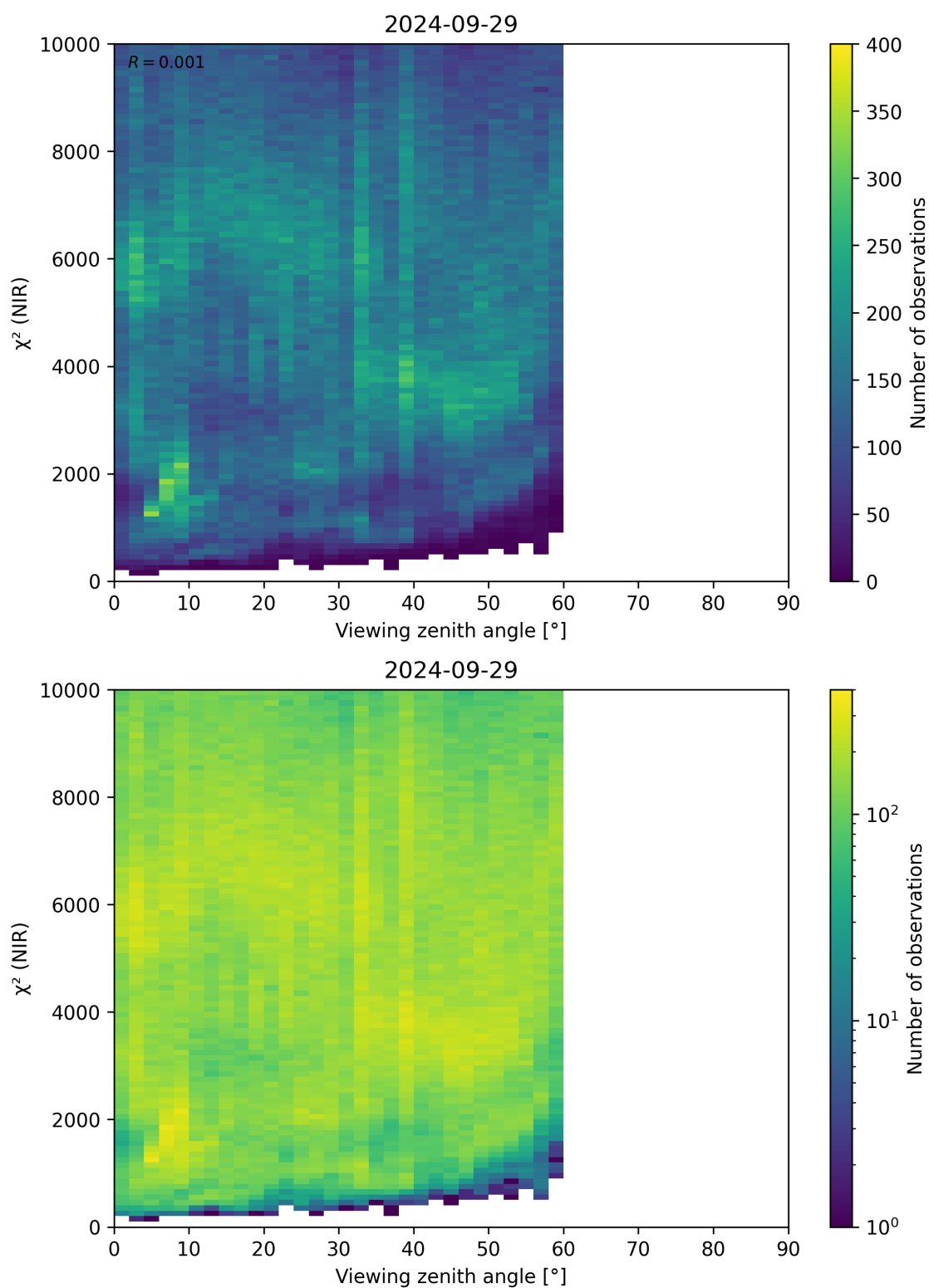
Figure 105: Scatter density plot of “Viewing zenith angle” against “ \chi^2 (NIR)” for 2024-09-28 to 2024-09-30.
