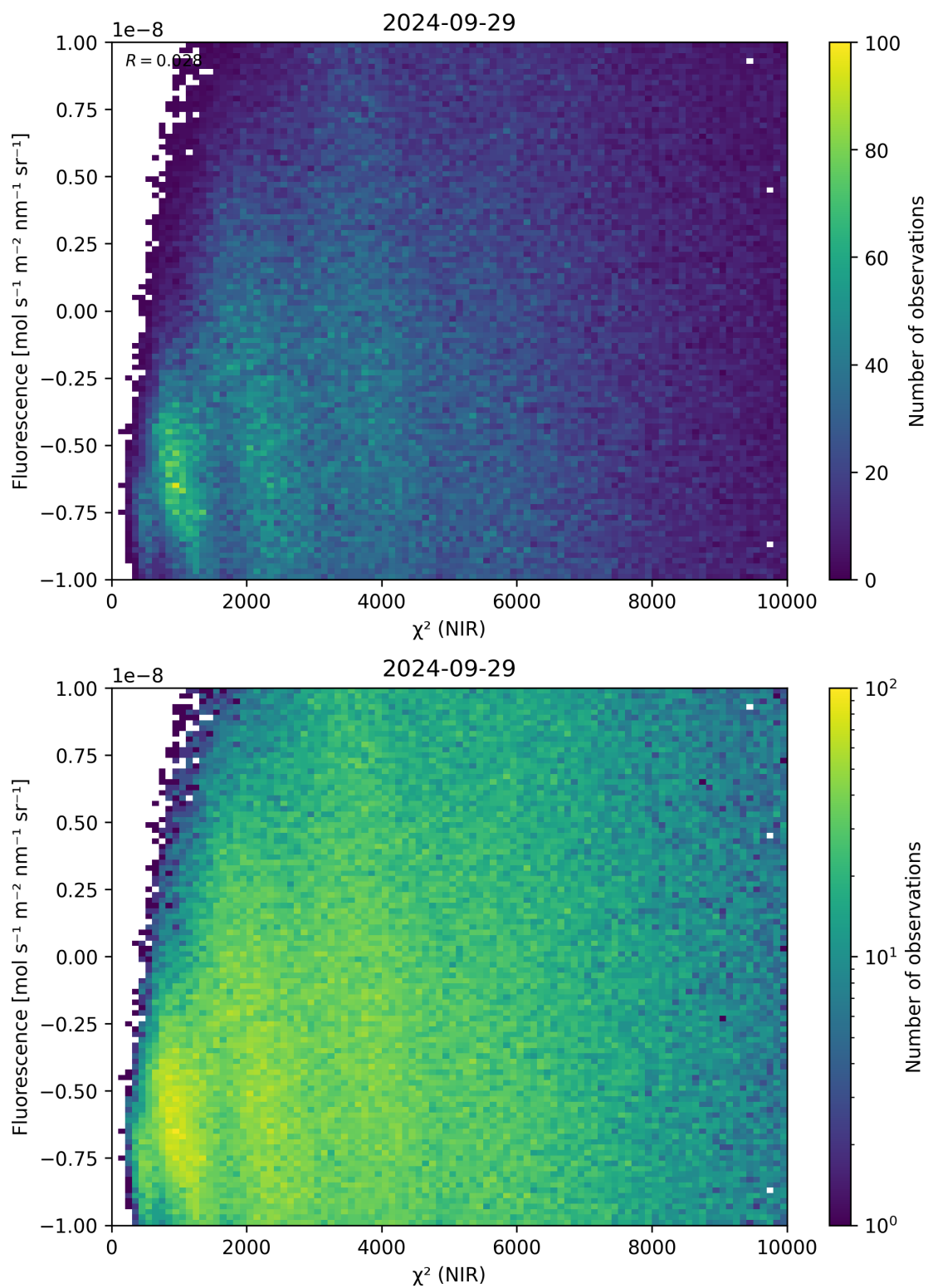
Figure 45: Scatter density plot of “ \chi^2 (NIR)” against “Fluorescence” for 2024-09-28 to 2024-09-30.
