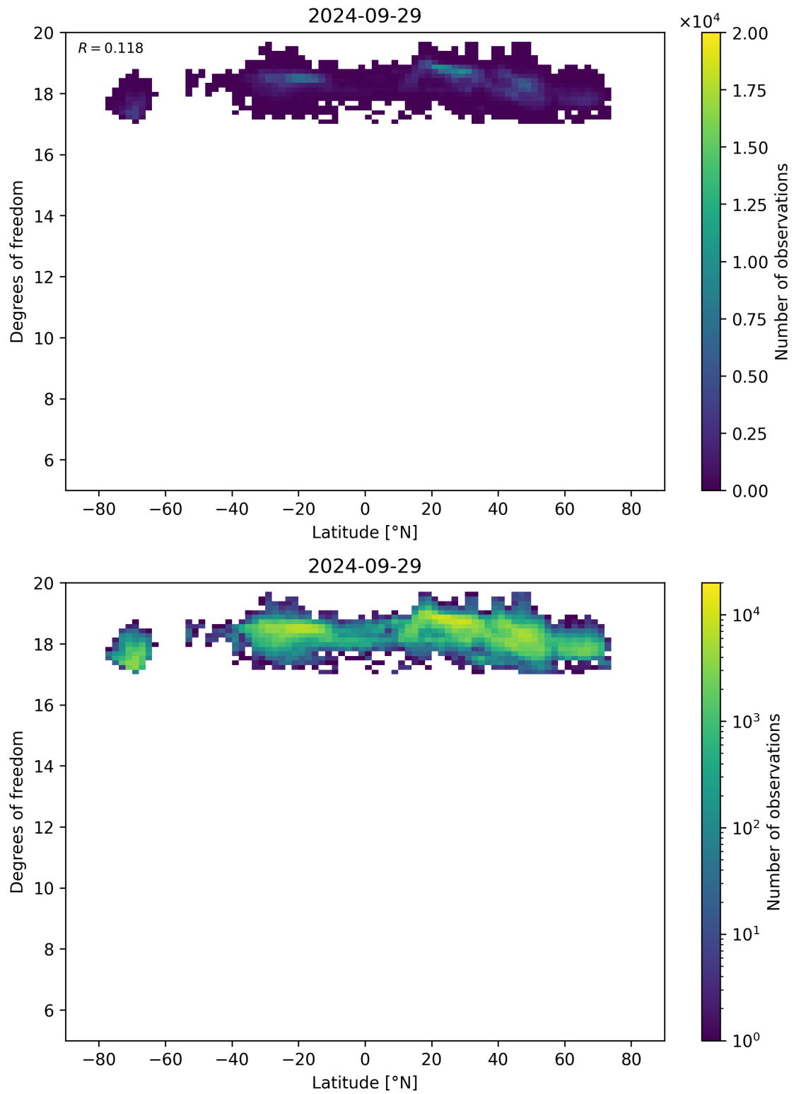
Figure 55: Scatter density plot of “Latitude” against “Degrees of freedom” for 2024-09-28 to 2024-09-30.
