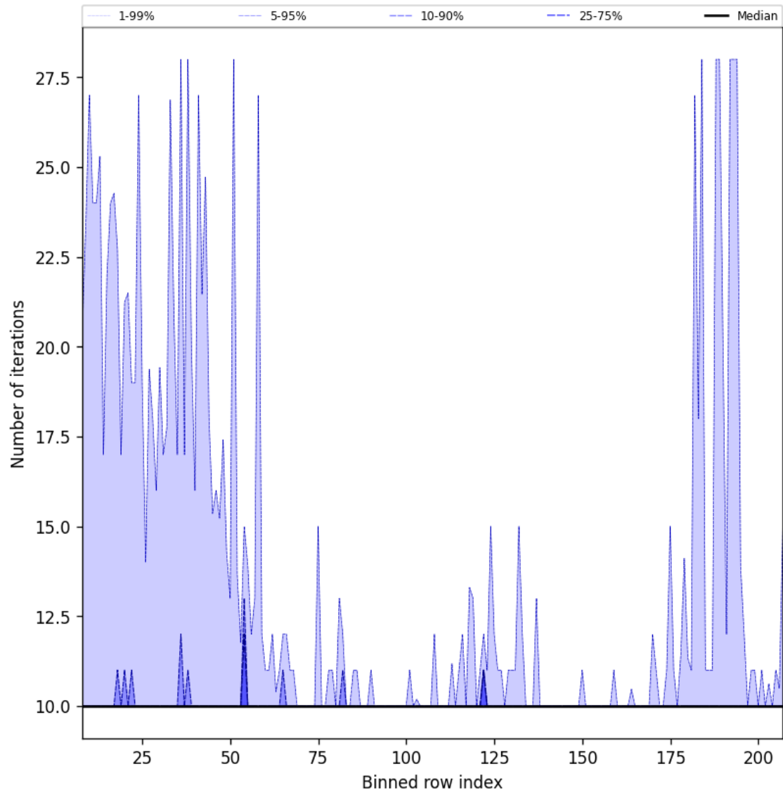
Figure 42: Along track statistics of “Number of iterations” for 2024-09-28 to 2024-09-30
