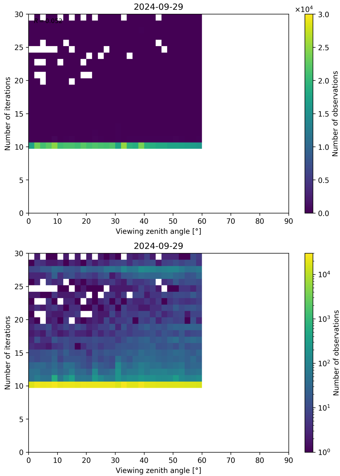
Figure 113: Scatter density plot of “Viewing zenith angle” against “Number of iterations” for 2024-09-28 to 2024-09-30.
