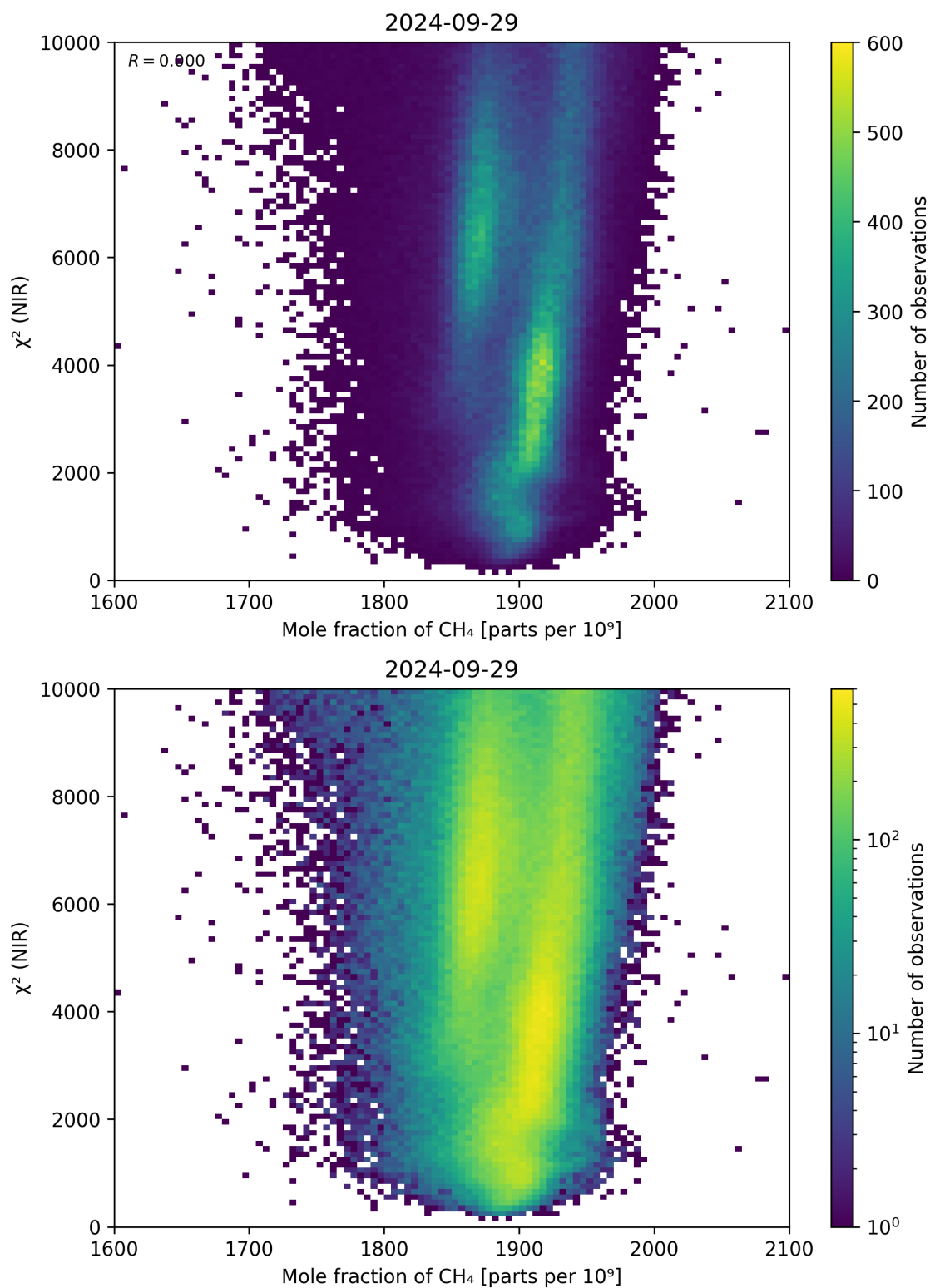
Figure 70: Scatter density plot of “Mole fraction of CH 4 ” against “ \chi^2 (NIR)” for 2024-09-28 to 2024-09-30.
