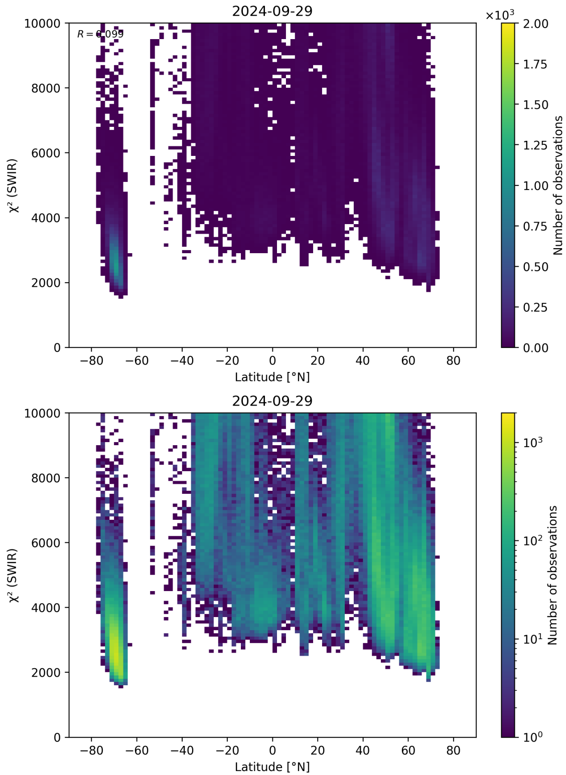
Figure 54: Scatter density plot of “Latitude” against “ \chi^2 (SWIR)” for 2024-09-28 to 2024-09-30.
