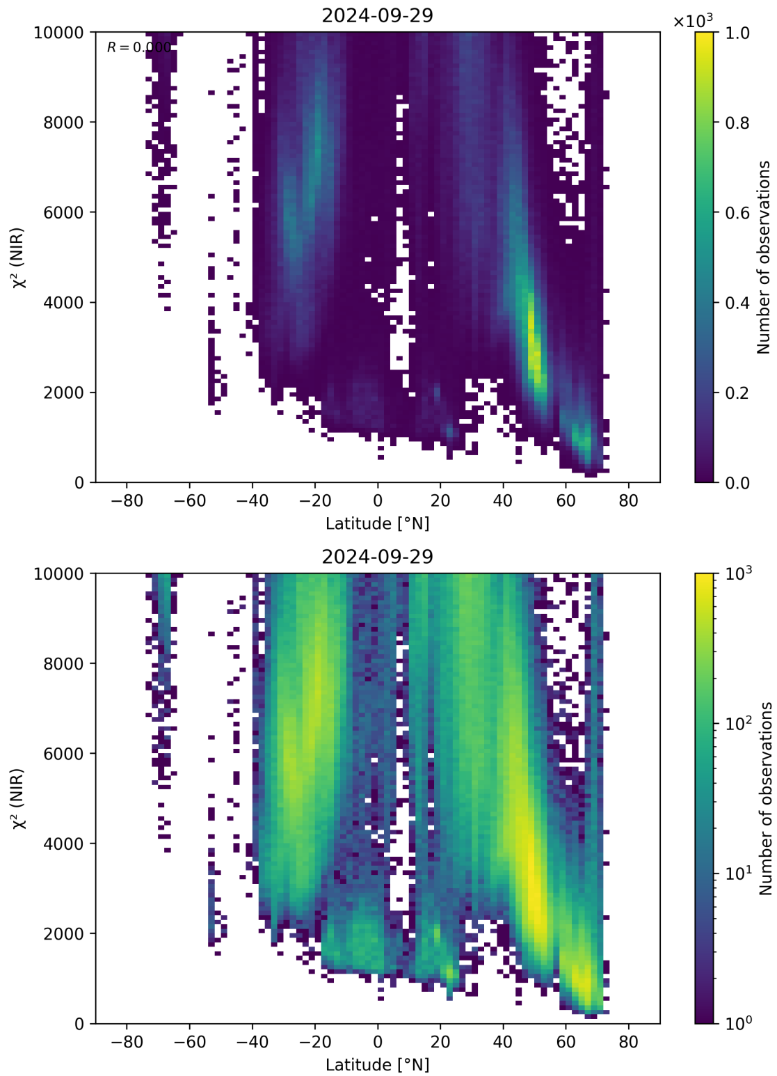
Figure 53: Scatter density plot of “Latitude” against “ \chi^2 (NIR)” for 2024-09-28 to 2024-09-30.
