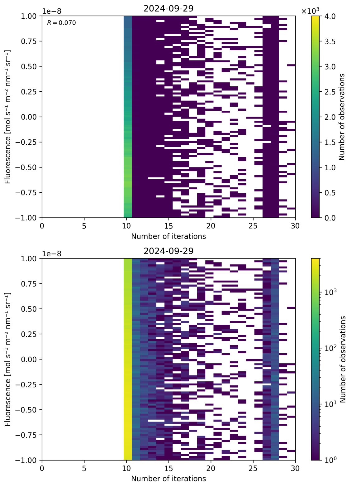
Figure 87: Scatter density plot of “Number of iterations” against “Fluorescence” for 2024-09-28 to 2024-09-30.
