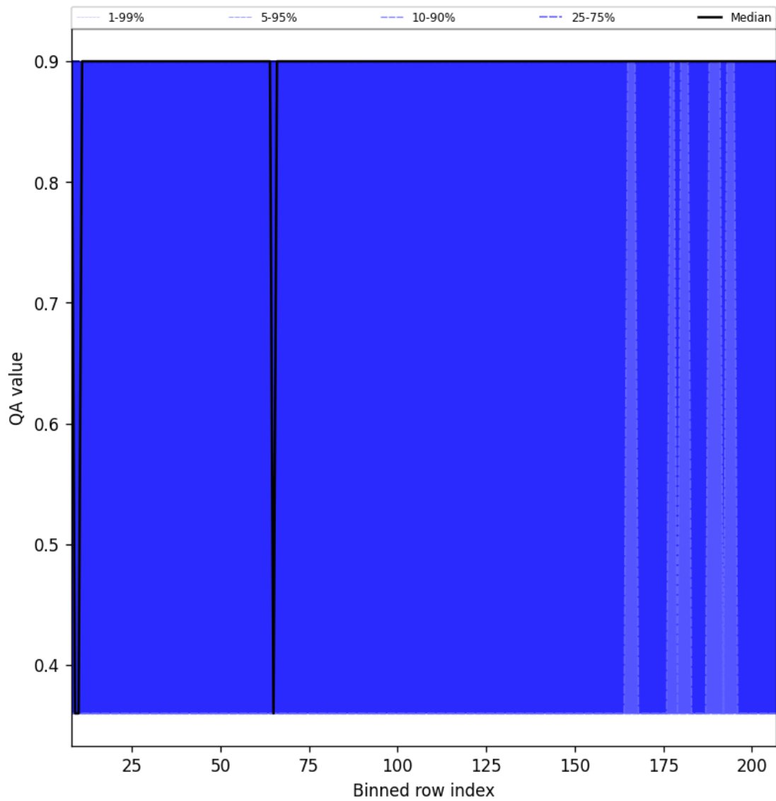
Figure 33: Along track statistics of “QA value” for 2024-09-28 to 2024-09-30
