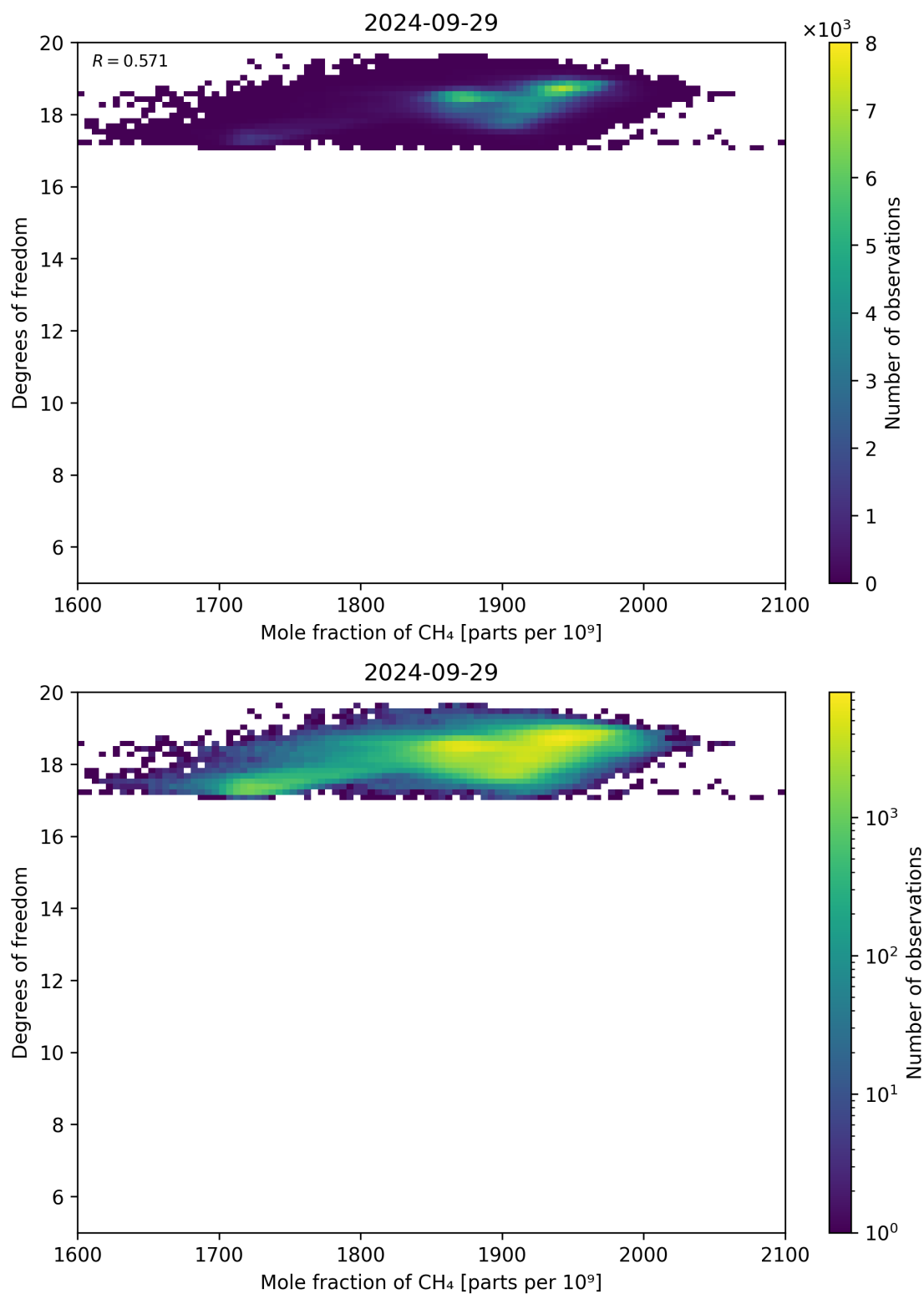
Figure 72: Scatter density plot of “Mole fraction of CH 4 ” against “Degrees of freedom” for 2024-09-28 to 2024-09-30.
