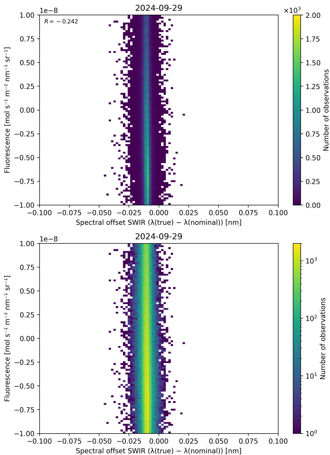
Figure 120: Scatter density plot of “Spectral offset SWIR ( \lambda_{\text{true}} - \lambda_{\text{nominal}} )” against “Fluorescence” for 2024-09-28 to 2024-09-30.
