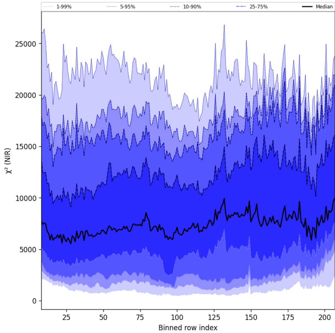
Figure 40: Along track statistics of “ \chi^2 (NIR)” for 2024-09-28 to 2024-09-30
