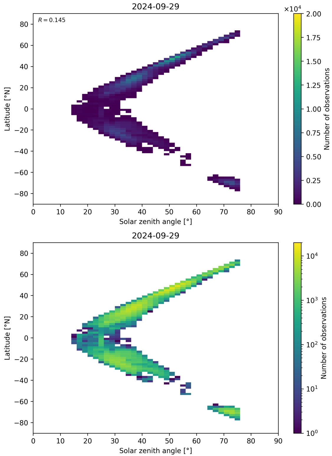
Figure 98: Scatter density plot of “Solar zenith angle” against “Latitude” for 2024-09-28 to 2024-09-30.
