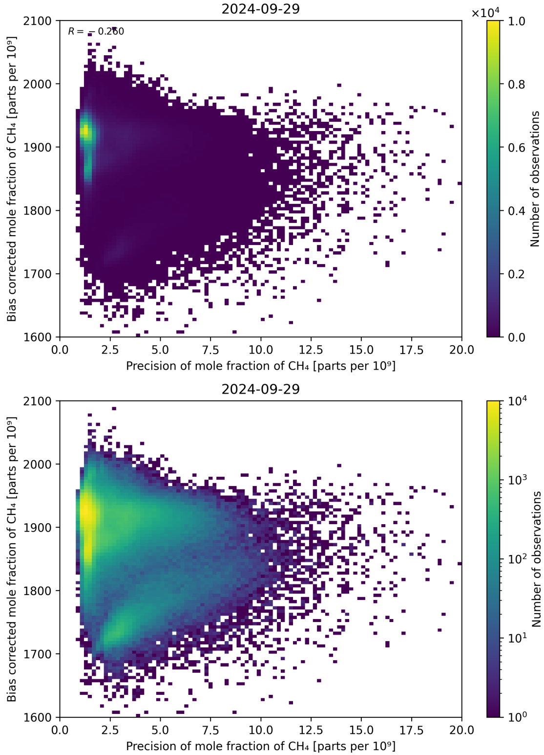
Figure 82: Scatter density plot of “Precision of mole fraction of CH 4 ” against “Bias corrected mole fraction of CH 4 ” for 2024-09-28 to 2024-09-30.
