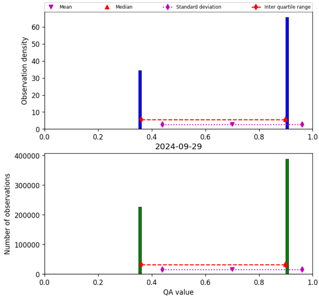
Figure 22: Histogram of “QA value” for 2024-09-28 to 2024-09-30
