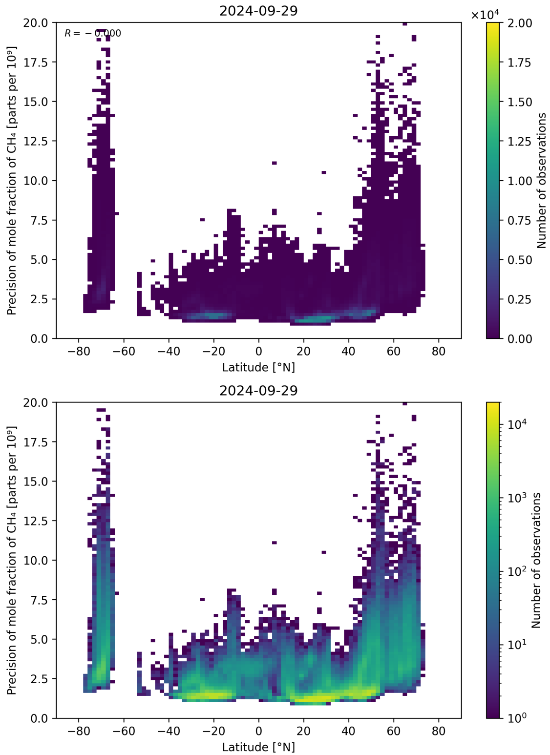
Figure 59: Scatter density plot of “Latitude” against “Precision of mole fraction of \text{CH}_4 ” for 2024-09-28 to 2024-09-30.
