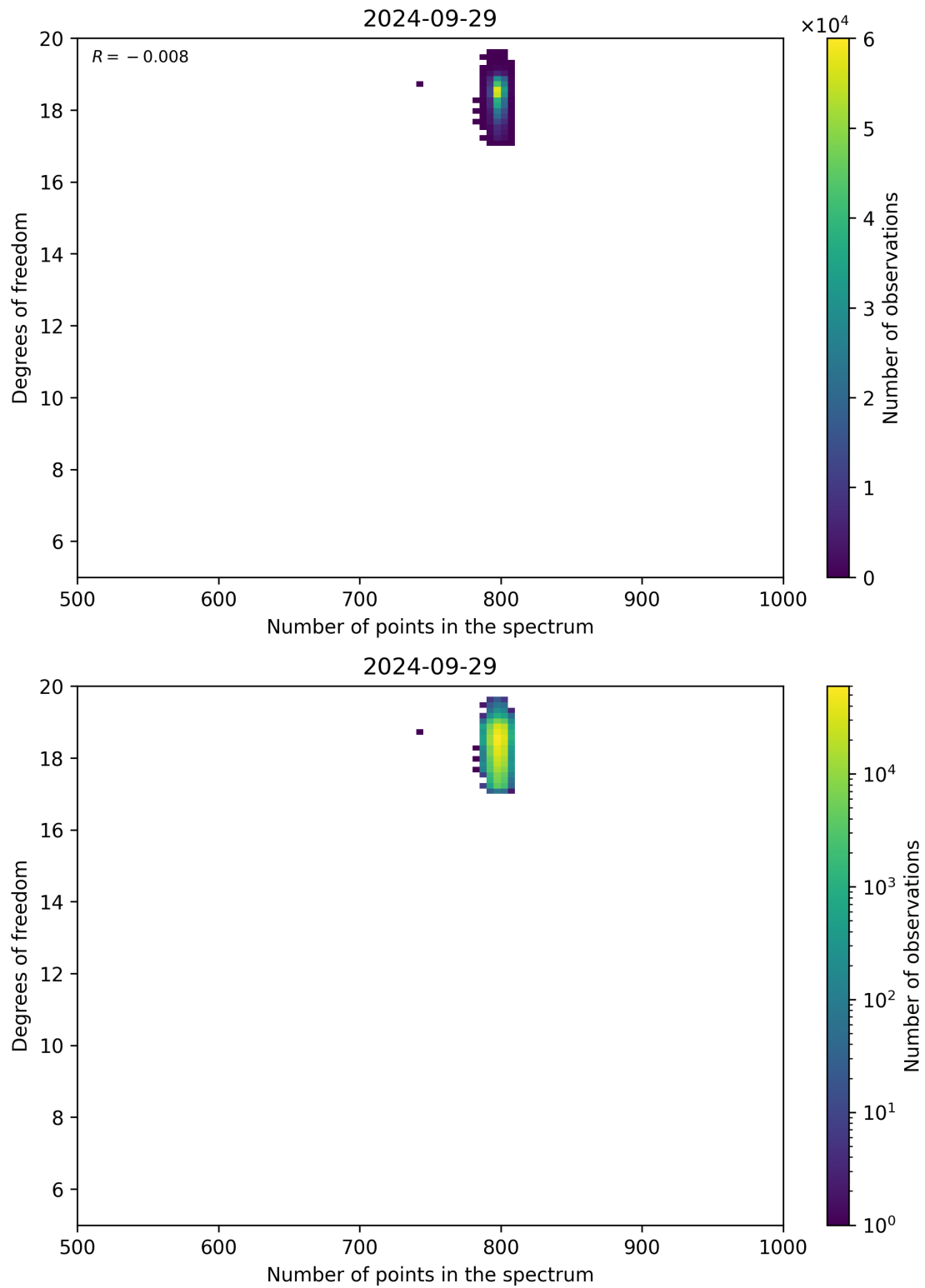
Figure 90: Scatter density plot of “Number of points in the spectrum” against “Degrees of freedom” for 2024-09-28 to 2024-09-30.
