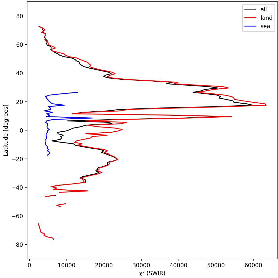
Figure 17: Zonal average of “ \chi^2 (SWIR)” for 2024-09-28 to 2024-09-30.
