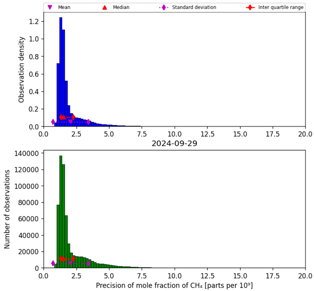
Figure 24: Histogram of “Precision of mole fraction of CH 4 ” for 2024-09-28 to 2024-09-30
