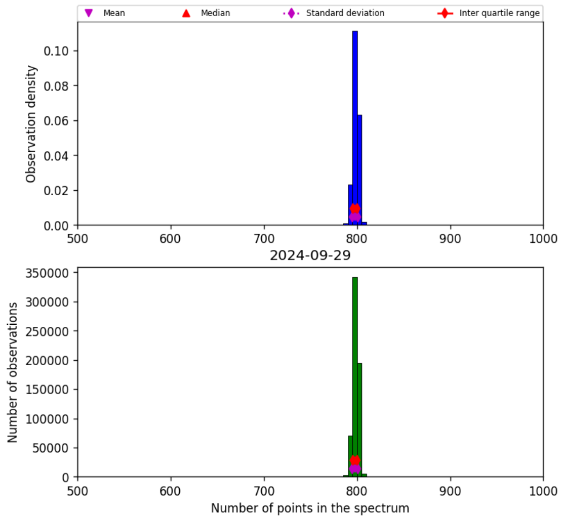
Figure 26: Histogram of “Number of points in the spectrum” for 2024-09-28 to 2024-09-30
