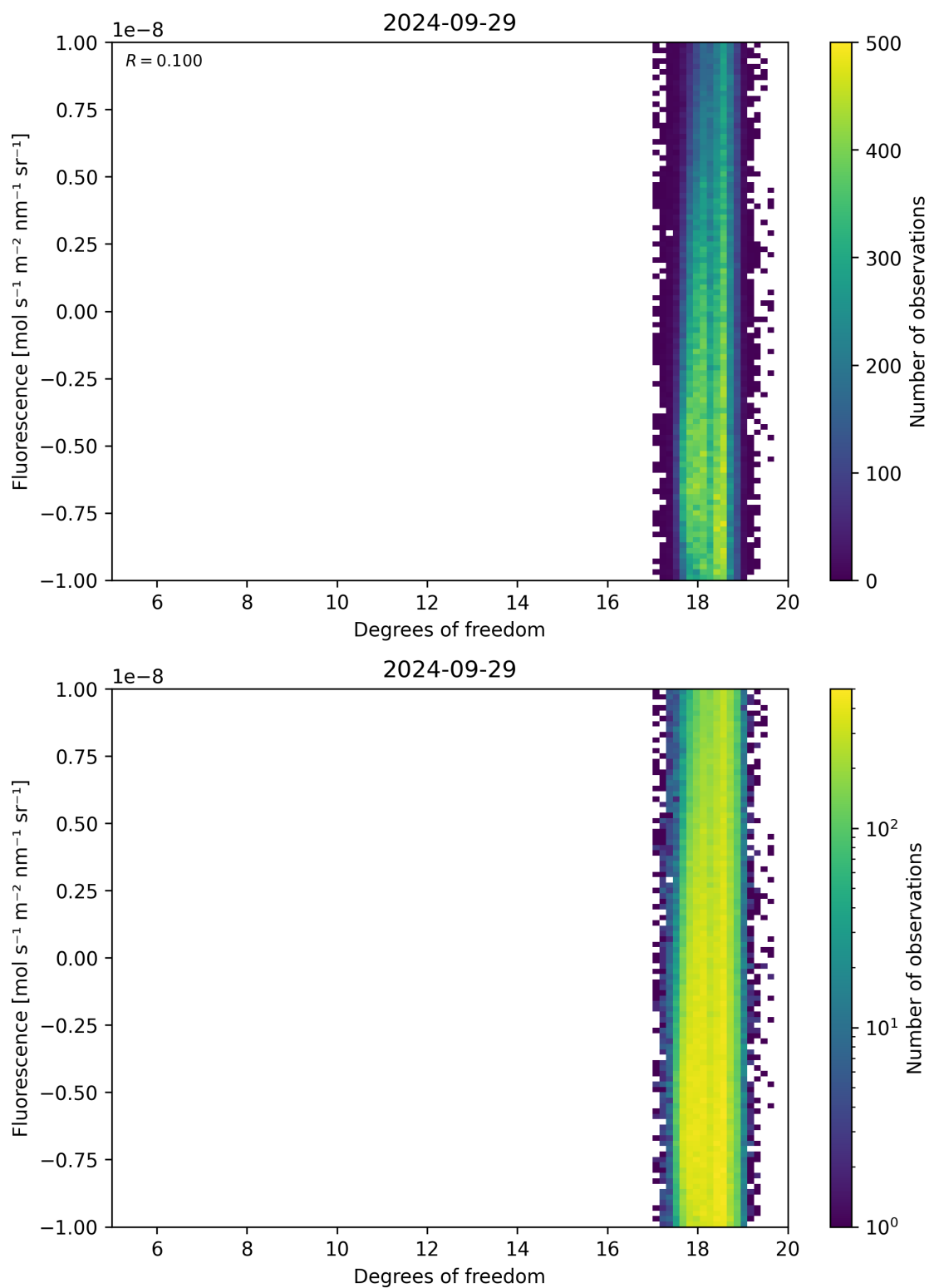
Figure 51: Scatter density plot of “Degrees of freedom” against “Fluorescence” for 2024-09-28 to 2024-09-30.
