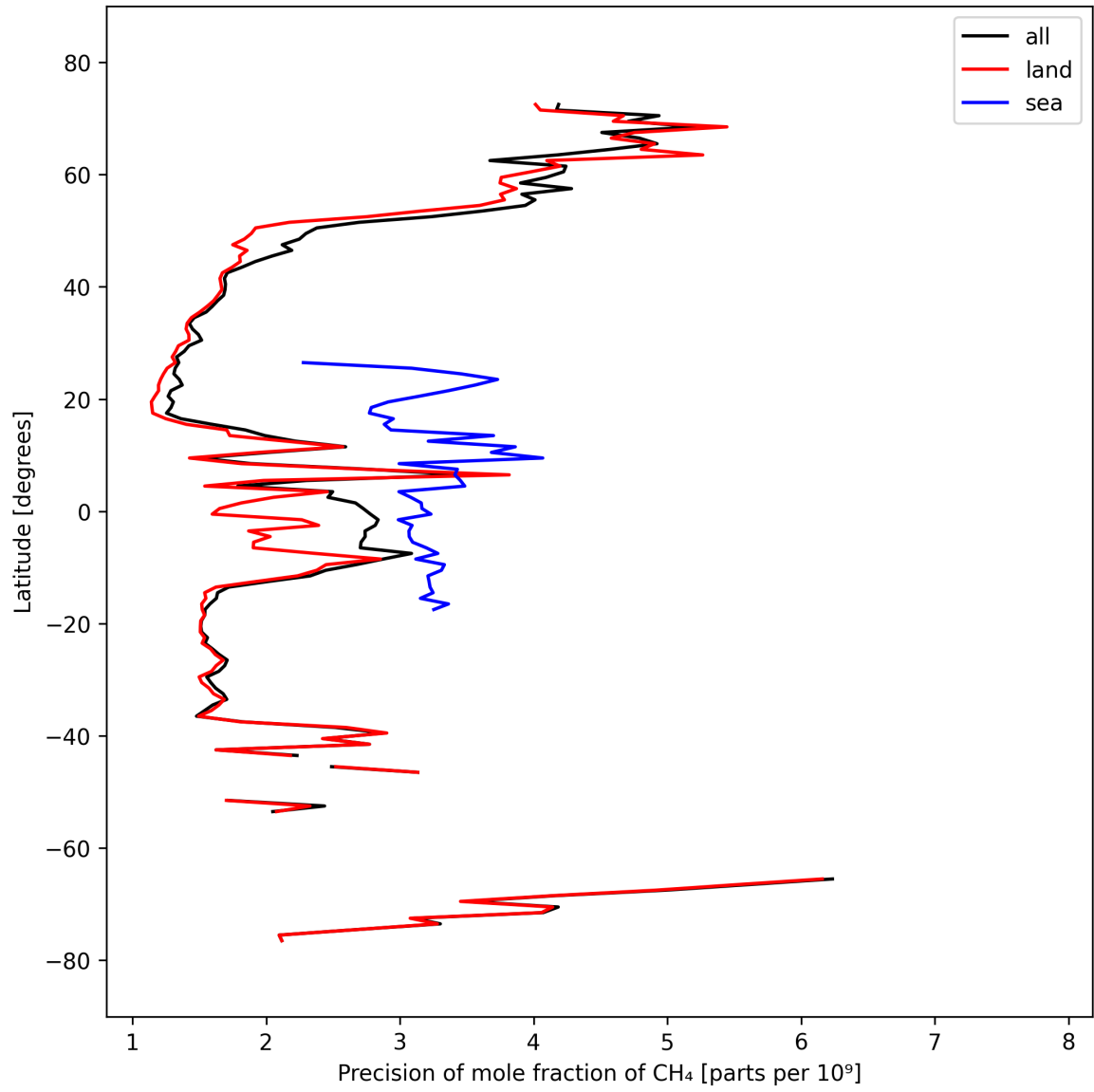
Figure 13: Zonal average of “Precision of mole fraction of CH 4 ” for 2024-09-28 to 2024-09-30.
