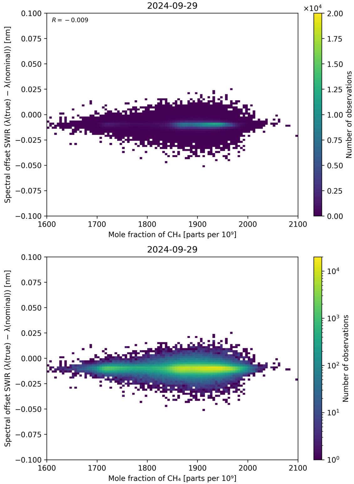
Figure 86: Scatter density plot of “Mole fraction of CH 4 ” against “Spectral offset SWIR ( \lambda_{\text{true}} - \lambda_{\text{nominal}} )” for 2024-09-28 to 2024-09-30.
