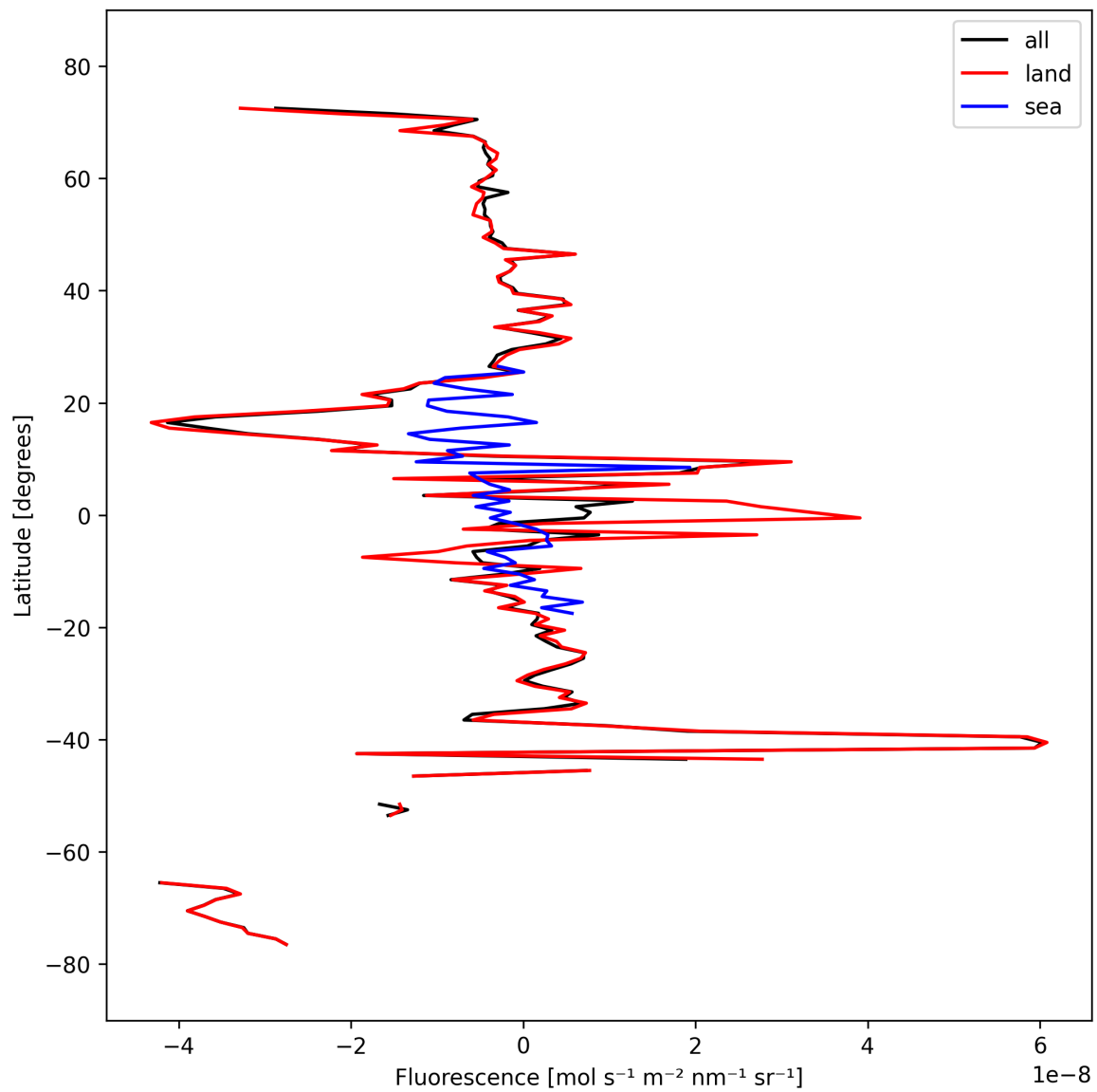
Figure 21: Zonal average of “Fluorescence” for 2024-09-28 to 2024-09-30.
