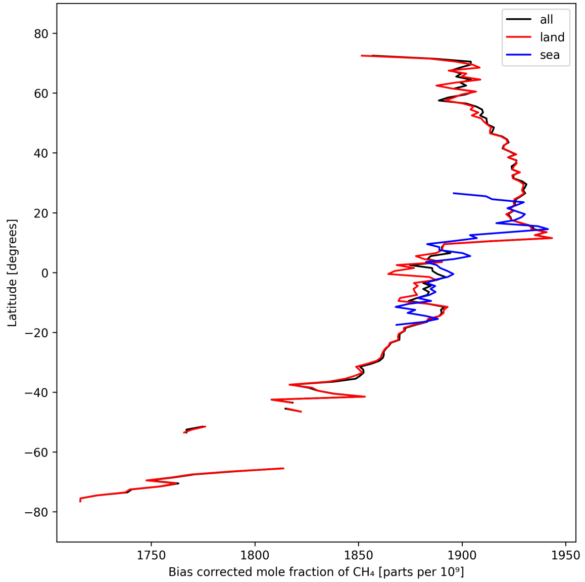
Figure 14: Zonal average of “Bias corrected mole fraction of \text{CH}_4 ” for 2024-09-28 to 2024-09-30.
