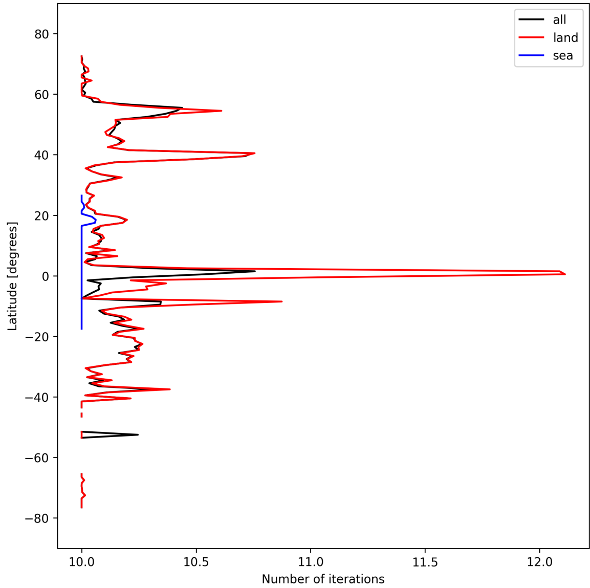
Figure 20: Zonal average of “Number of iterations” for 2024-09-28 to 2024-09-30.
