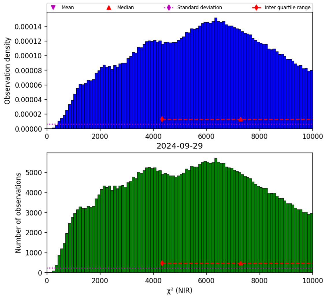
Figure 29: Histogram of “ \chi^2 (NIR)” for 2024-09-28 to 2024-09-30
