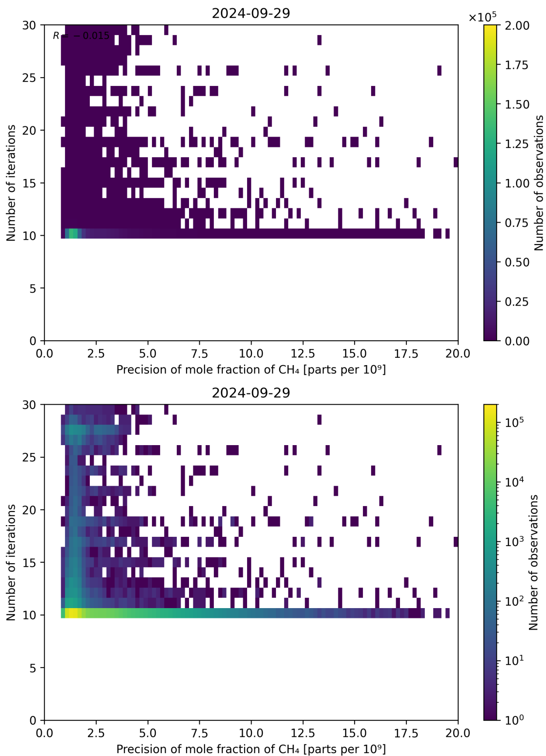
Figure 83: Scatter density plot of “Precision of mole fraction of CH 4 ” against “Number of iterations” for 2024-09-28 to 2024-09-30.
