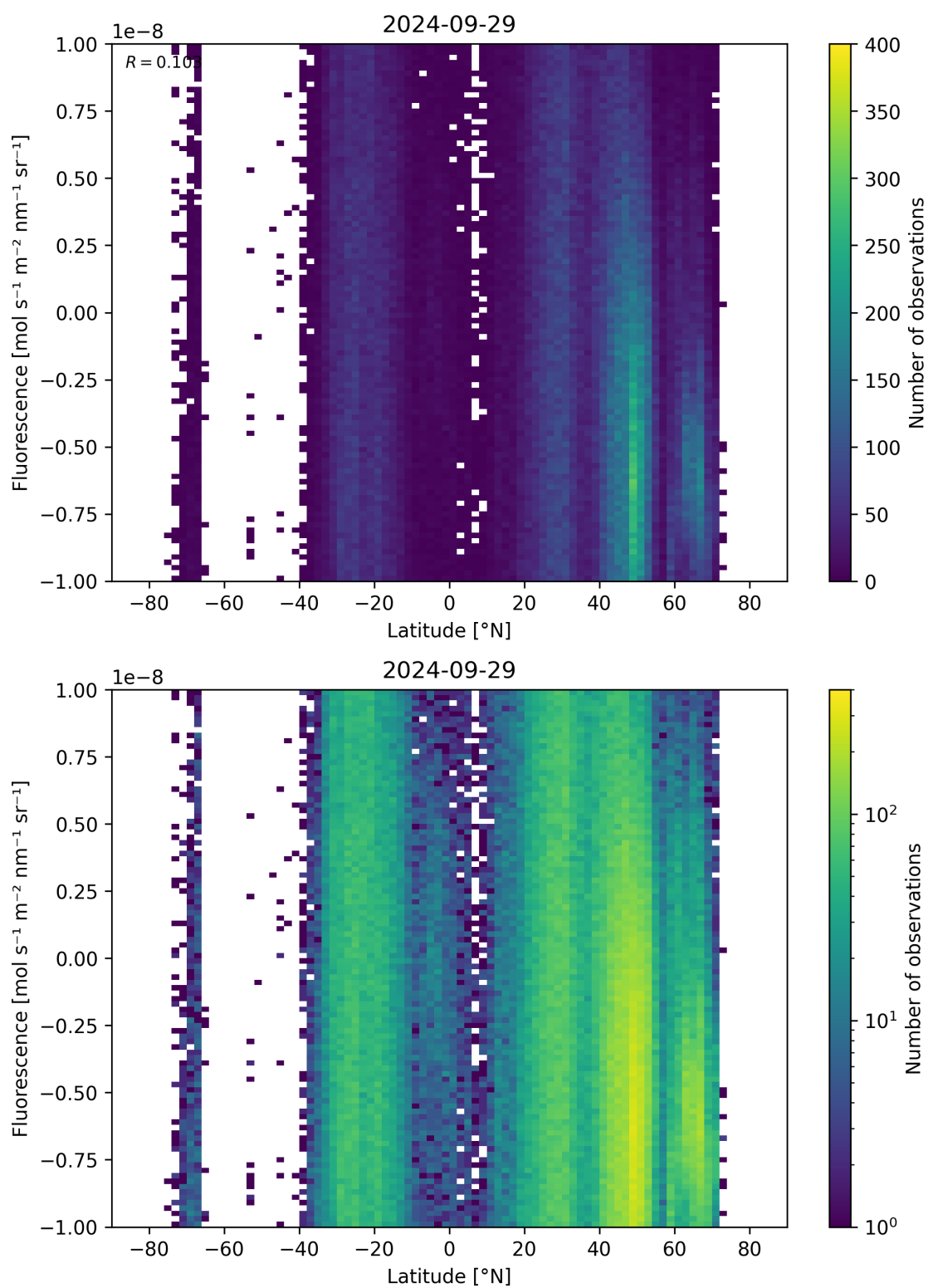
Figure 56: Scatter density plot of “Latitude” against “Fluorescence” for 2024-09-28 to 2024-09-30.
