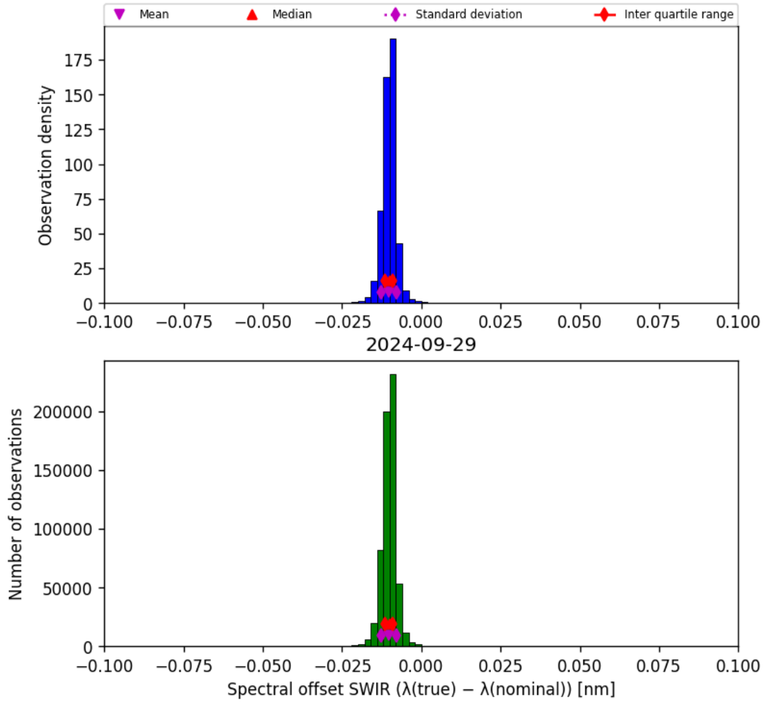
Figure 27: Histogram of “Spectral offset SWIR ( \lambda_{\text{true}} - \lambda_{\text{nominal}} )” for 2024-09-28 to 2024-09-30
