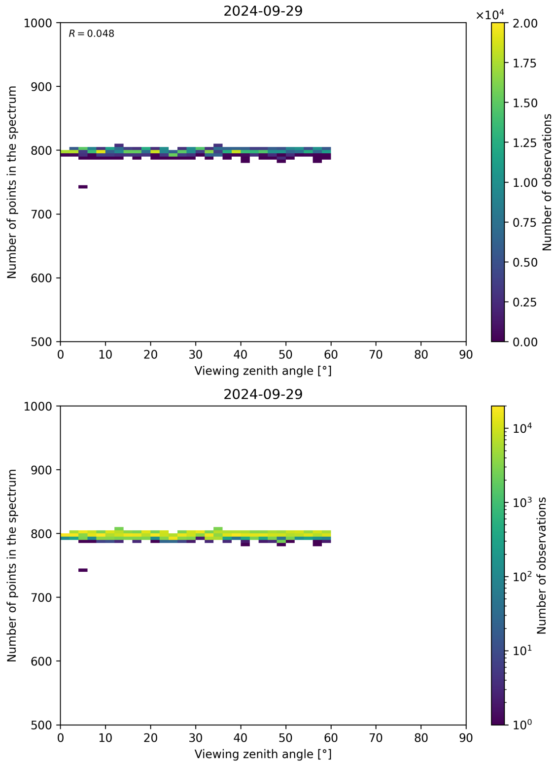
Figure 114: Scatter density plot of “Viewing zenith angle” against “Number of points in the spectrum” for 2024-09-28 to 2024-09-30.
