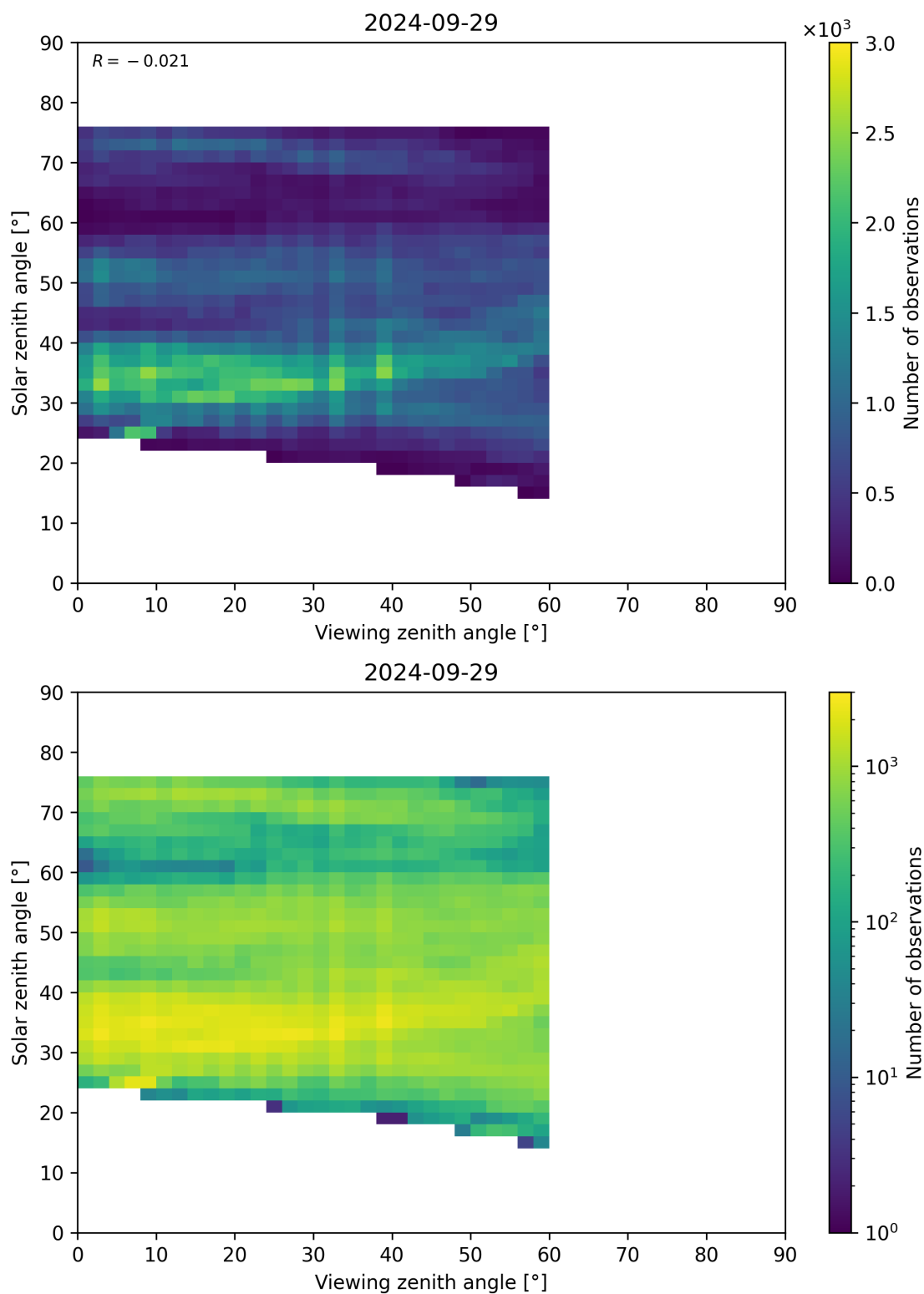
Figure 115: Scatter density plot of “Viewing zenith angle” against “Solar zenith angle” for 2024-09-28 to 2024-09-30.
