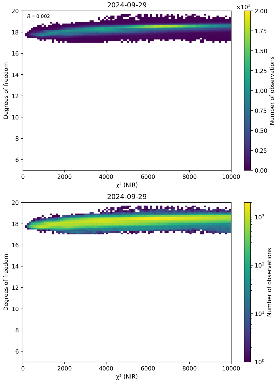
Figure 44: Scatter density plot of “ \chi^2 (NIR)” against “Degrees of freedom” for 2024-09-28 to 2024-09-30.
