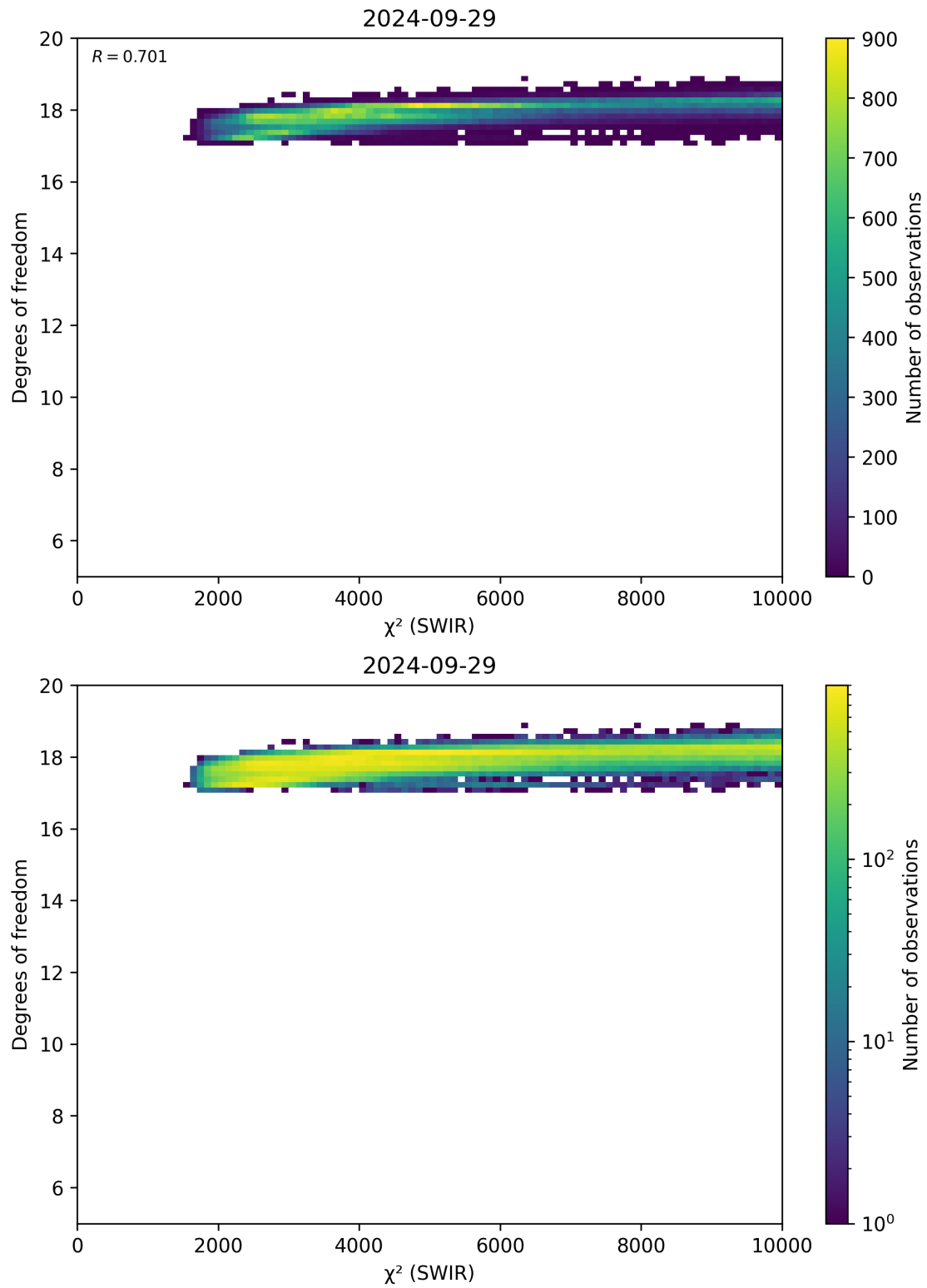
Figure 48: Scatter density plot of “ \chi^2 (SWIR)” against “Degrees of freedom” for 2024-09-28 to 2024-09-30.
