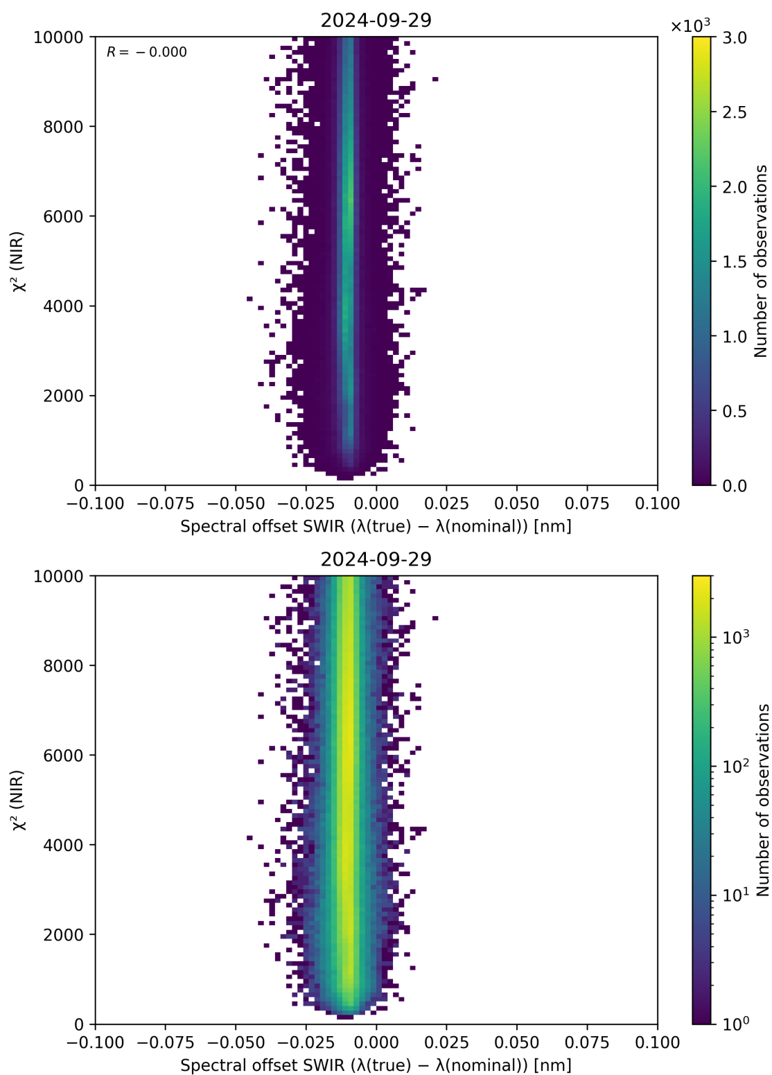
Figure 117: Scatter density plot of “Spectral offset SWIR ( \lambda_{\text{true}} - \lambda_{\text{nominal}} )” against “ \chi^2 (NIR)” for 2024-09-28 to 2024-09-30.
