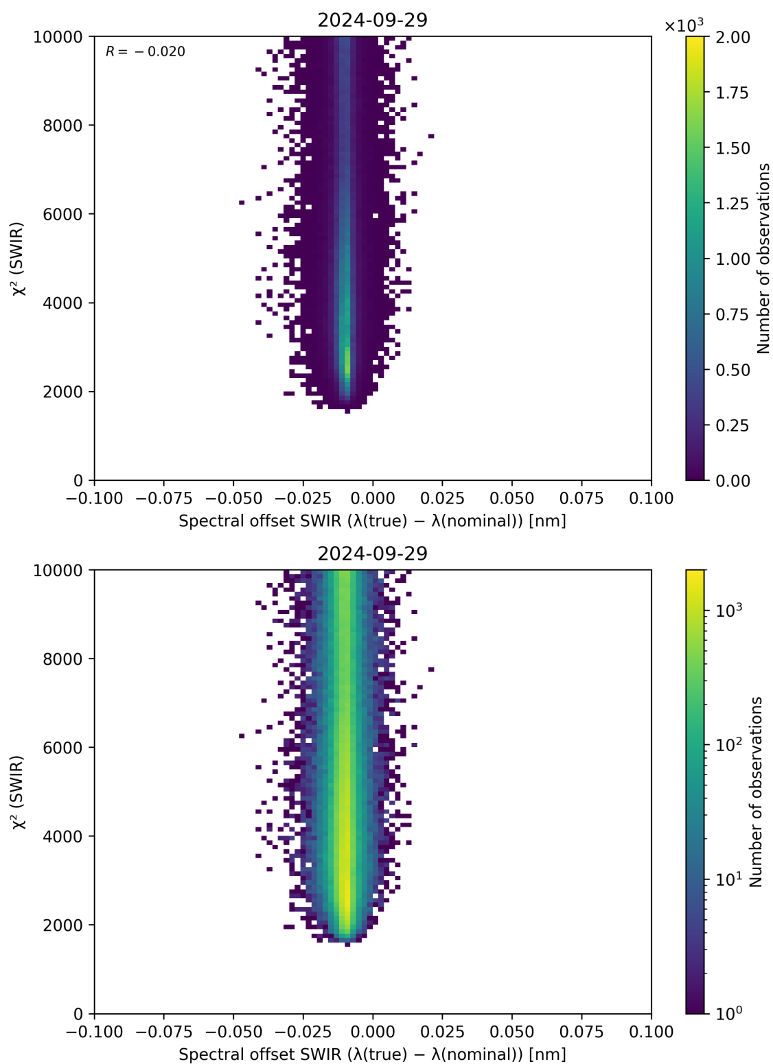
Figure 118: Scatter density plot of “Spectral offset SWIR ( \lambda_{\text{true}} - \lambda_{\text{nominal}} )” against “ \chi^2 (SWIR)” for 2024-09-28 to 2024-09-30.
