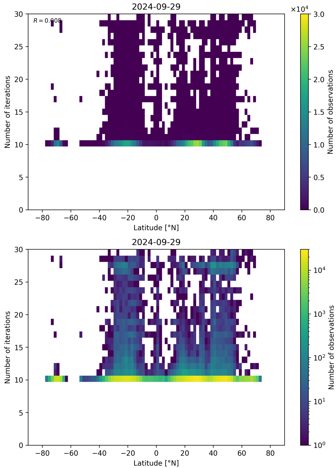
Figure 60: Scatter density plot of “Latitude” against “Number of iterations” for 2024-09-28 to 2024-09-30.
