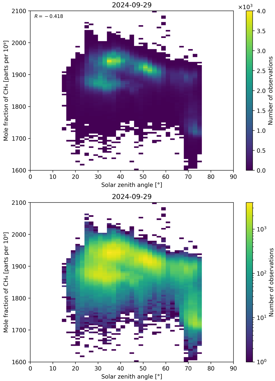
Figure 99: Scatter density plot of “Solar zenith angle” against “Mole fraction of CH 4 ” for 2024-09-28 to 2024-09-30.
