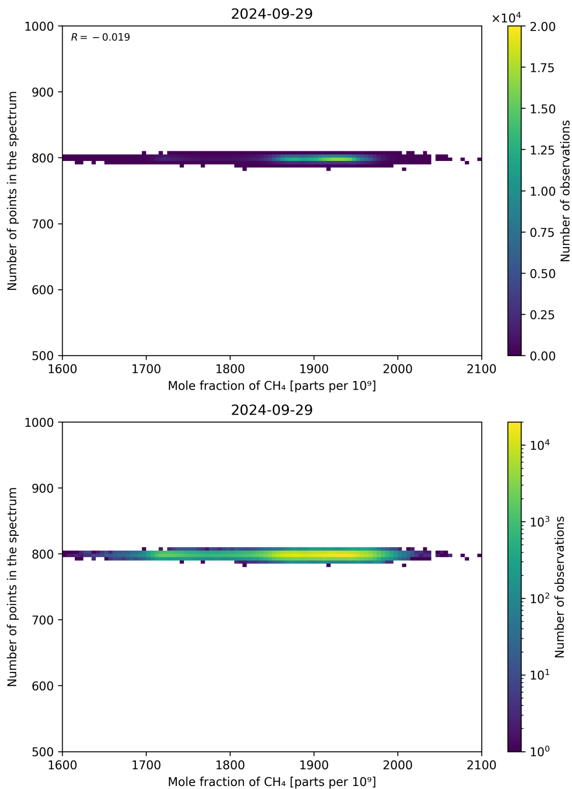
Figure 77: Scatter density plot of “Mole fraction of CH 4 ” against “Number of points in the spectrum” for 2024-09-28 to 2024-09-30.
