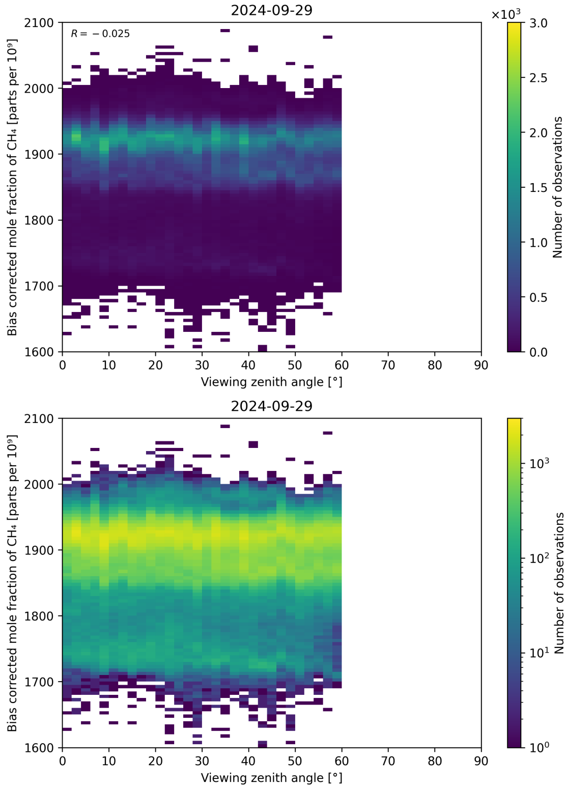
Figure 111: Scatter density plot of “Viewing zenith angle” against “Bias corrected mole fraction of CH 4 ” for 2024-09-28 to 2024-09-30.
