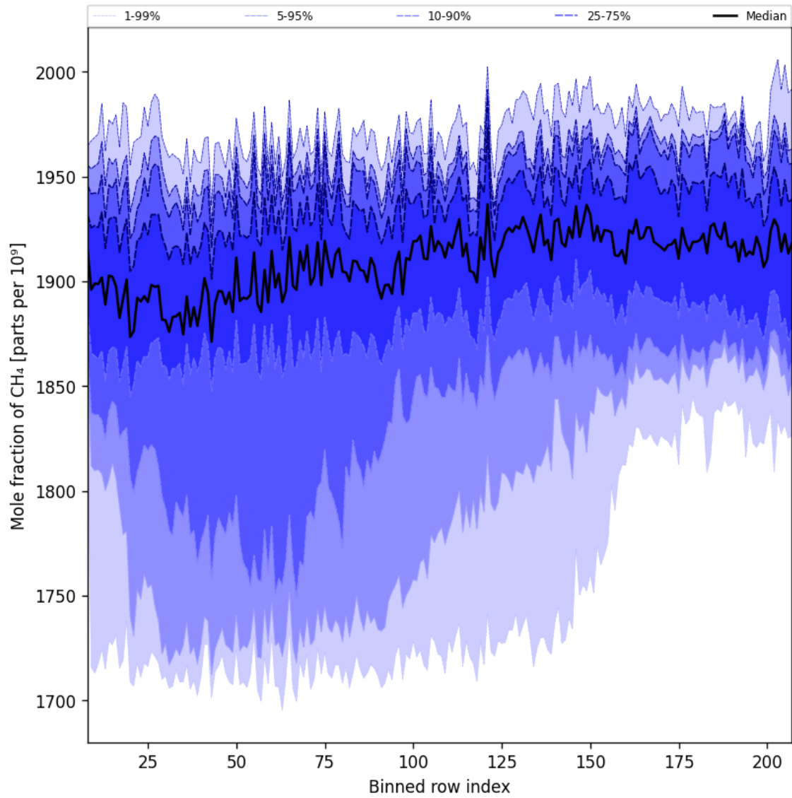
Figure 34: Along track statistics of “Mole fraction of CH 4 ” for 2024-09-28 to 2024-09-30
