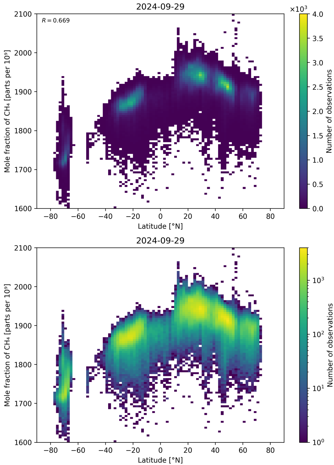
Figure 57: Scatter density plot of “Latitude” against “Mole fraction of CH 4 ” for 2024-09-28 to 2024-09-30.
