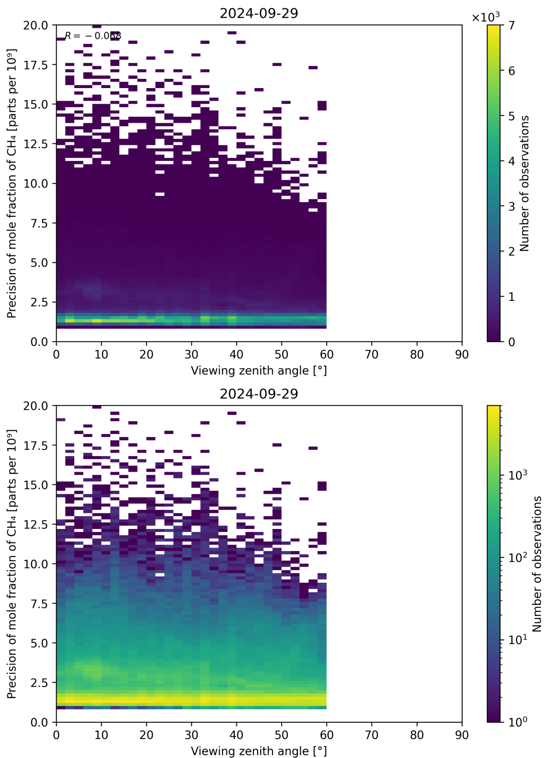
Figure 112: Scatter density plot of “Viewing zenith angle” against “Precision of mole fraction of CH 4 ” for 2024-09-28 to 2024-09-30.
