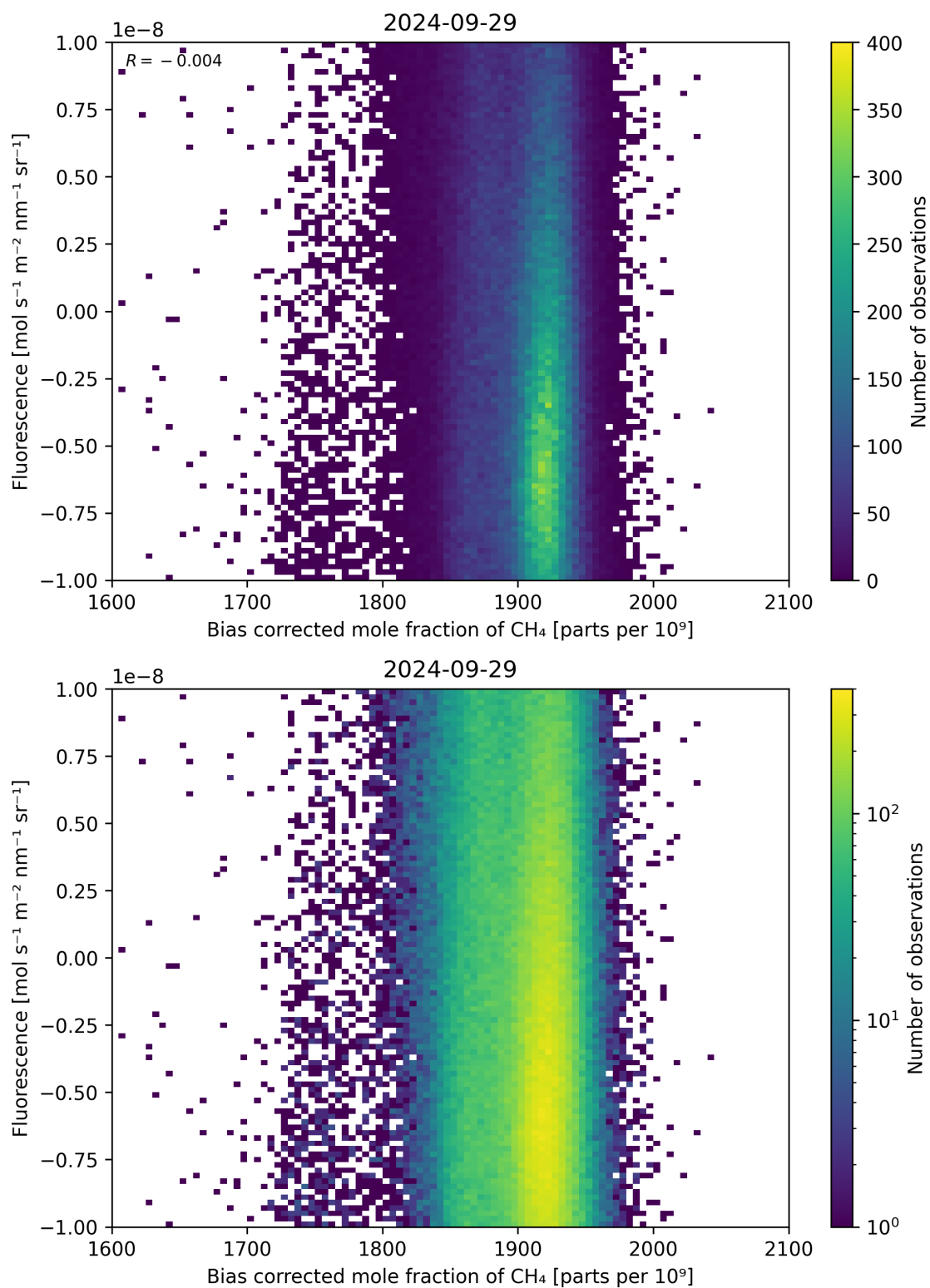
Figure 66: Scatter density plot of “Bias corrected mole fraction of \text{CH}_4 ” against “Fluorescence” for 2024-09-28 to 2024-09-30.
