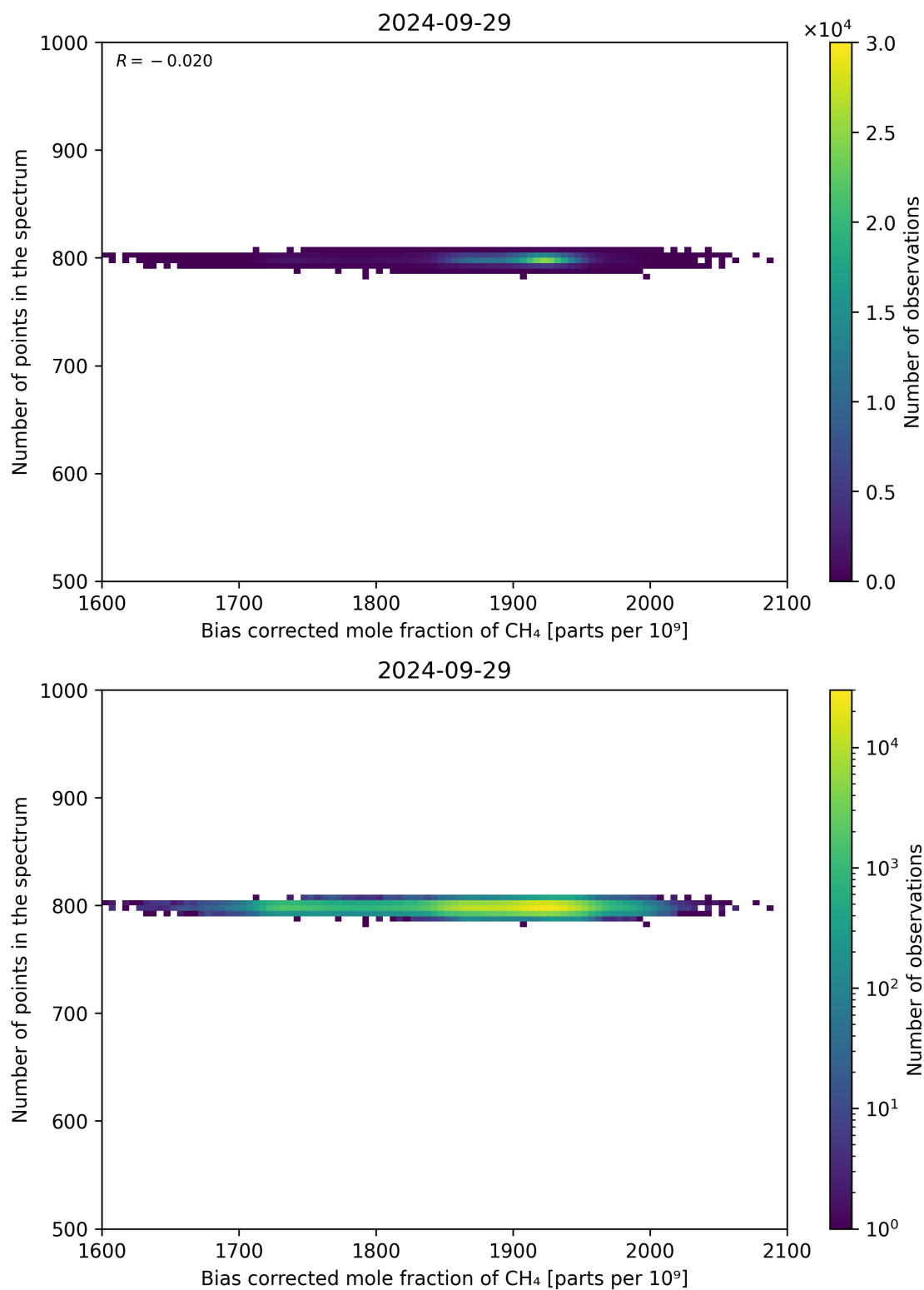
Figure 68: Scatter density plot of “Bias corrected mole fraction of CH 4 ” against “Number of points in the spectrum” for 2024-09-28 to 2024-09-30.
