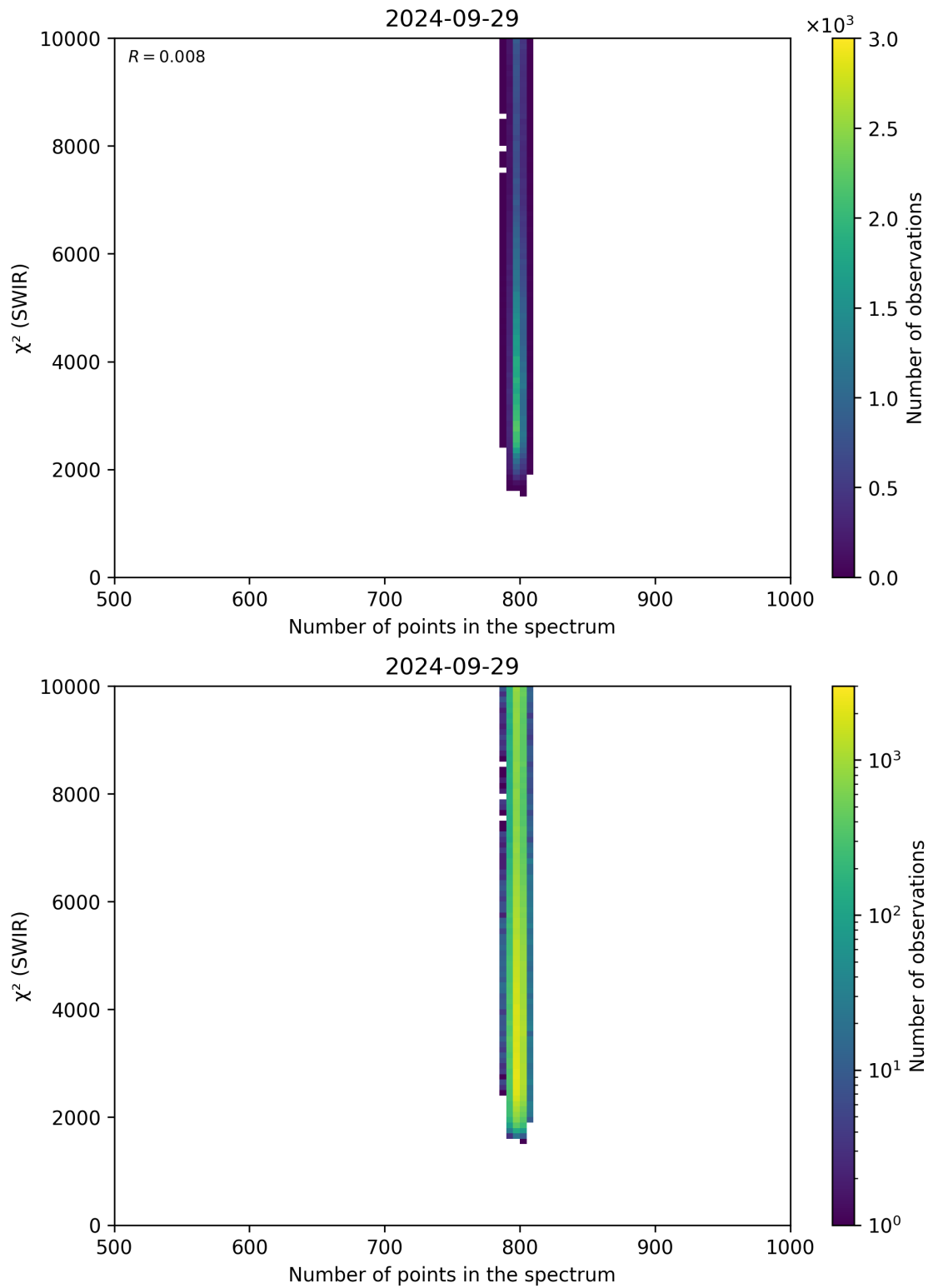
Figure 89: Scatter density plot of “Number of points in the spectrum” against “ \chi^2 (SWIR)” for 2024-09-28 to 2024-09-30.
