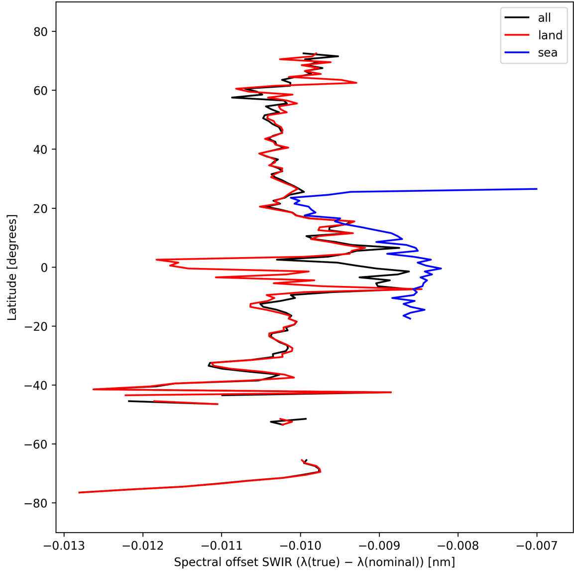
Figure 16: Zonal average of “Spectral offset SWIR ( \lambda_{\text{true}} - \lambda_{\text{nominal}} )” for 2024-09-28 to 2024-09-30.
