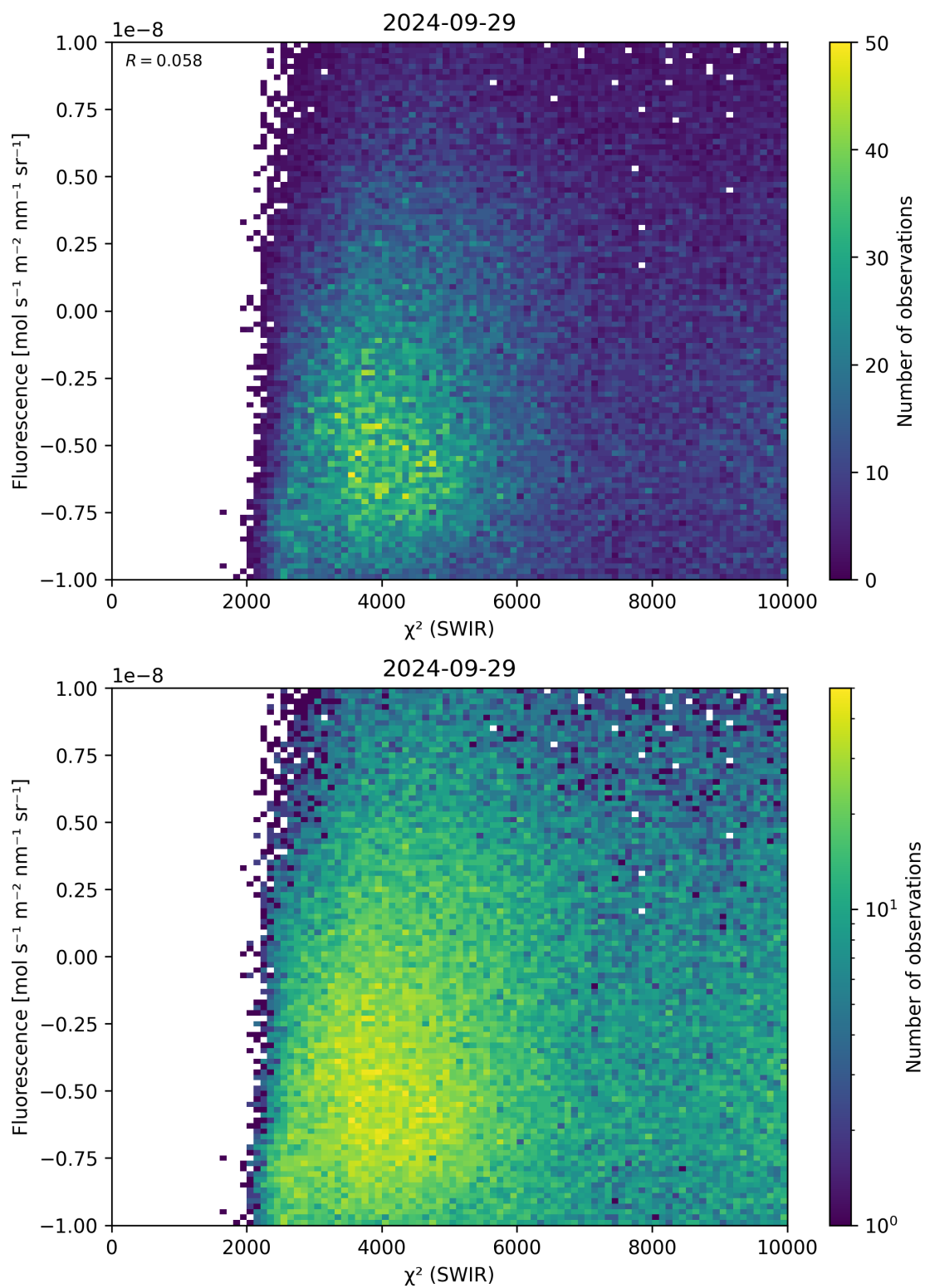
Figure 49: Scatter density plot of “ \chi^2 (SWIR)” against “Fluorescence” for 2024-09-28 to 2024-09-30.
