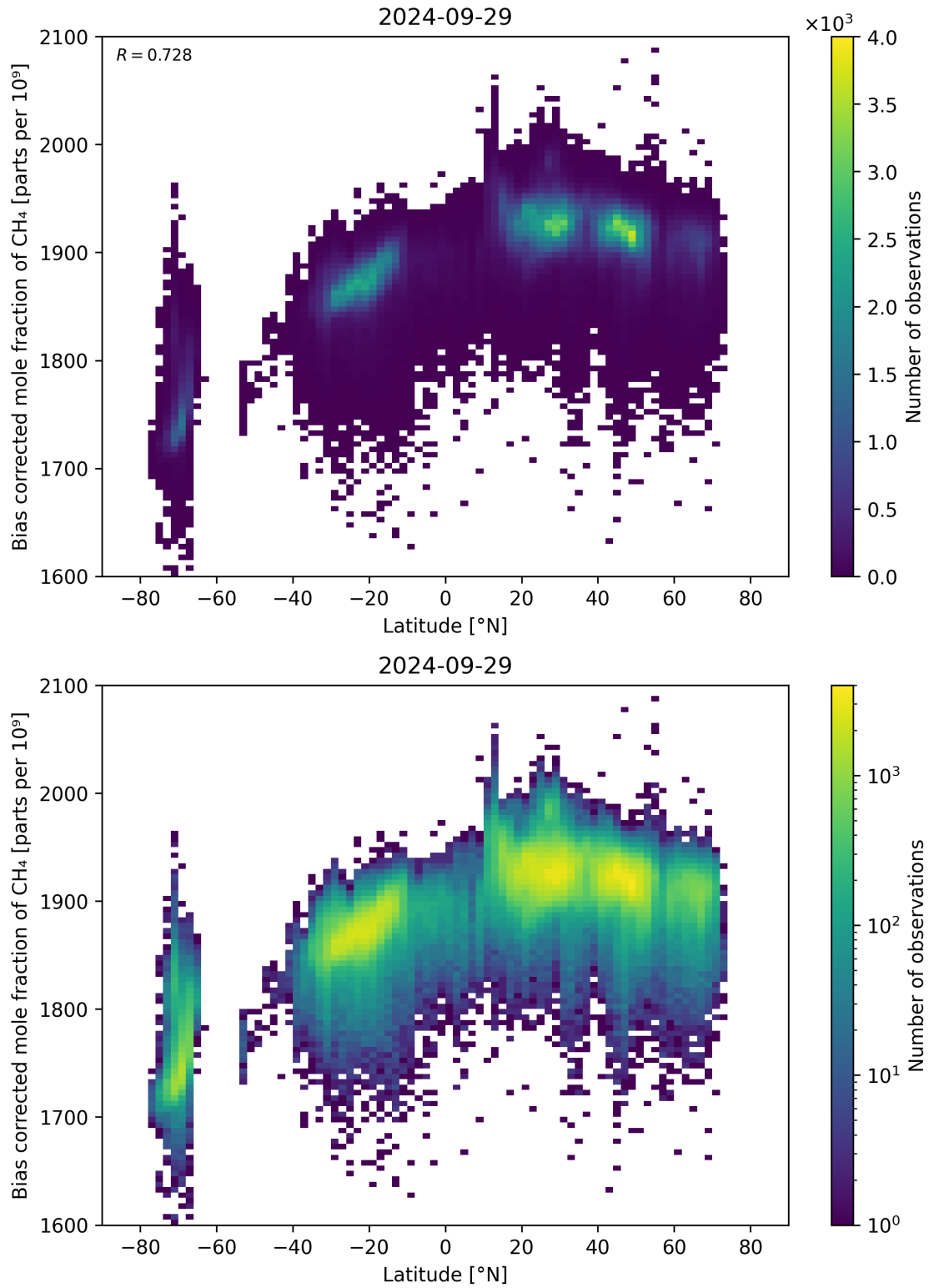
Figure 58: Scatter density plot of “Latitude” against “Bias corrected mole fraction of \text{CH}_4 ” for 2024-09-28 to 2024-09-30.
