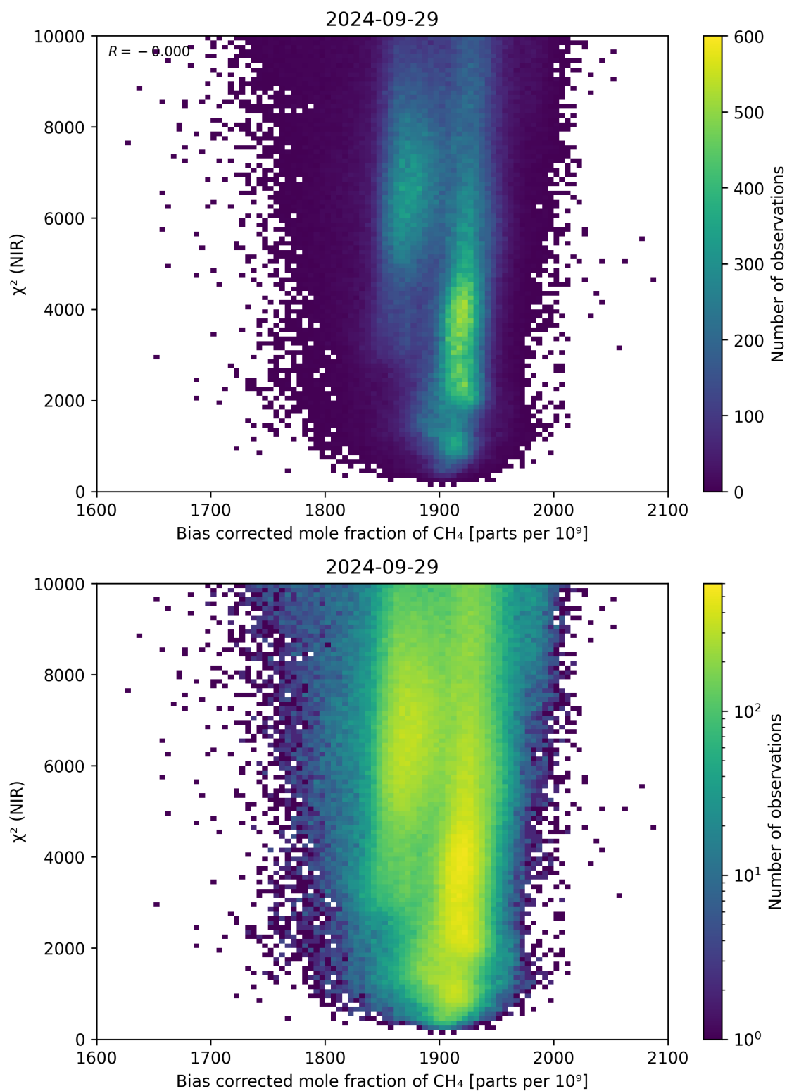
Figure 63: Scatter density plot of “Bias corrected mole fraction of CH 4 ” against “ \chi^2 (NIR)” for 2024-09-28 to 2024-09-30.
