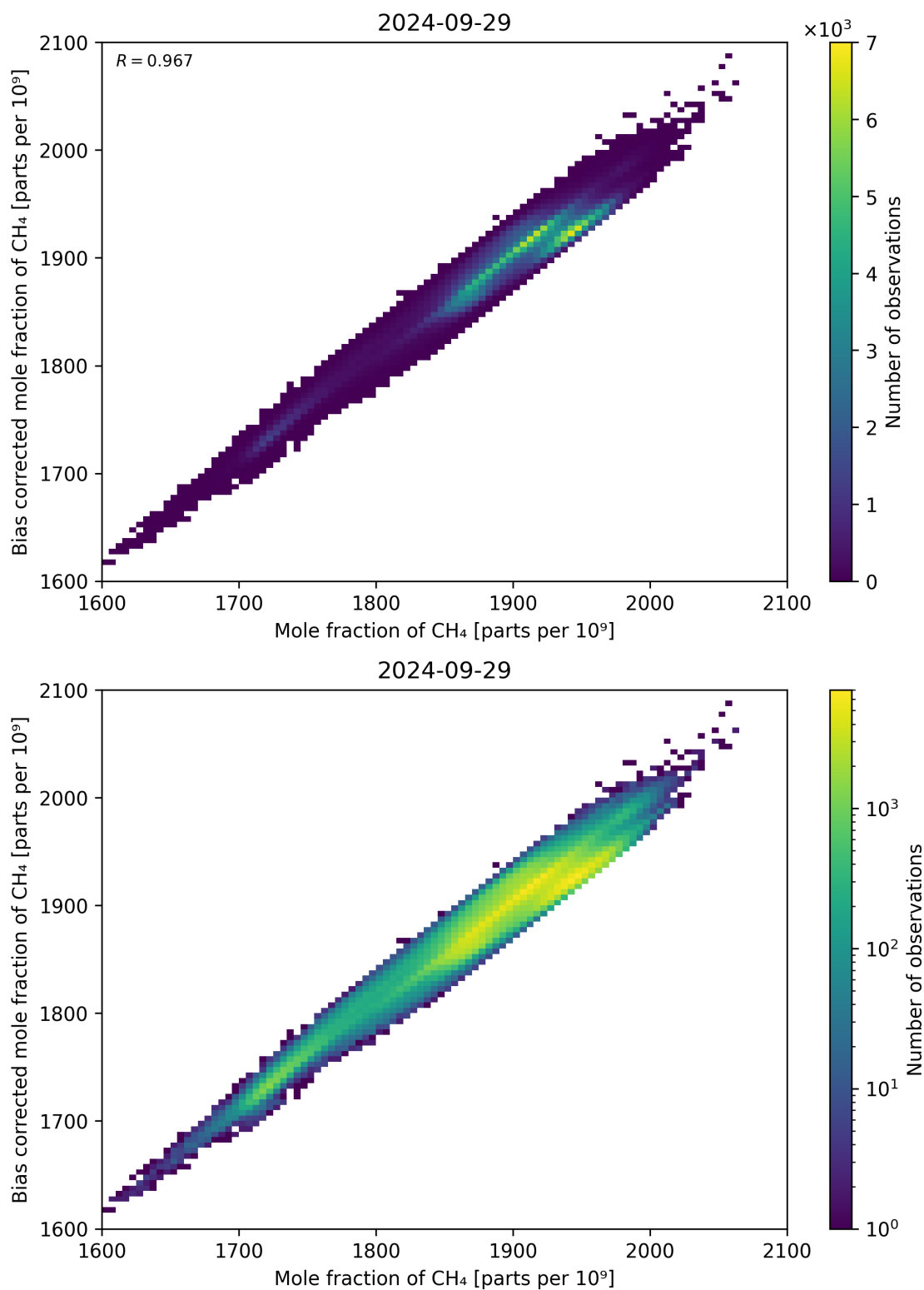
Figure 74: Scatter density plot of “Mole fraction of CH 4 ” against “Bias corrected mole fraction of CH 4 ” for 2024-09-28 to 2024-09-30.
