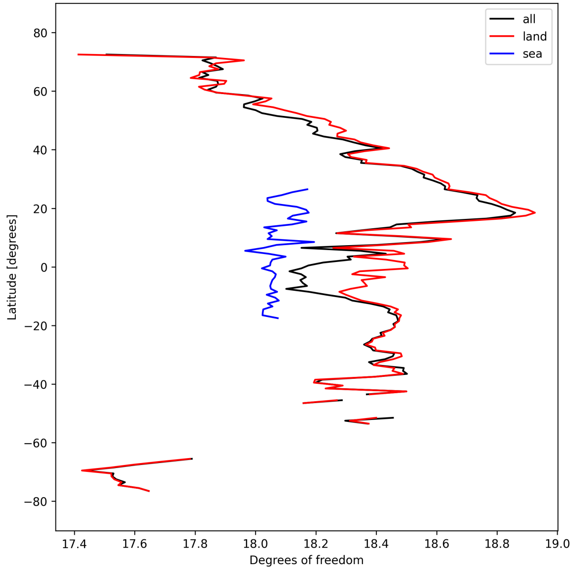
Figure 19: Zonal average of “Degrees of freedom” for 2024-09-28 to 2024-09-30.
