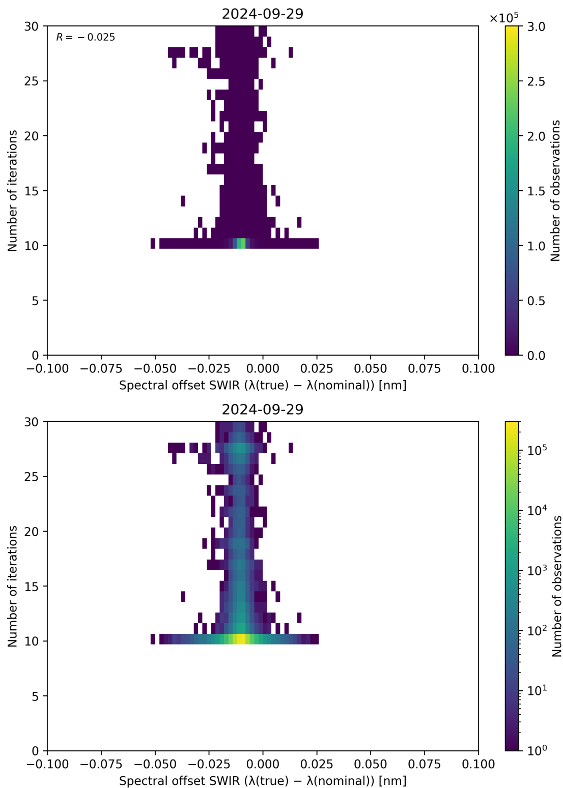
Figure 121: Scatter density plot of “Spectral offset SWIR ( \lambda_{\text{true}} - \lambda_{\text{nominal}} )” against “Number of iterations” for 2024-09-28 to 2024-09-30.
