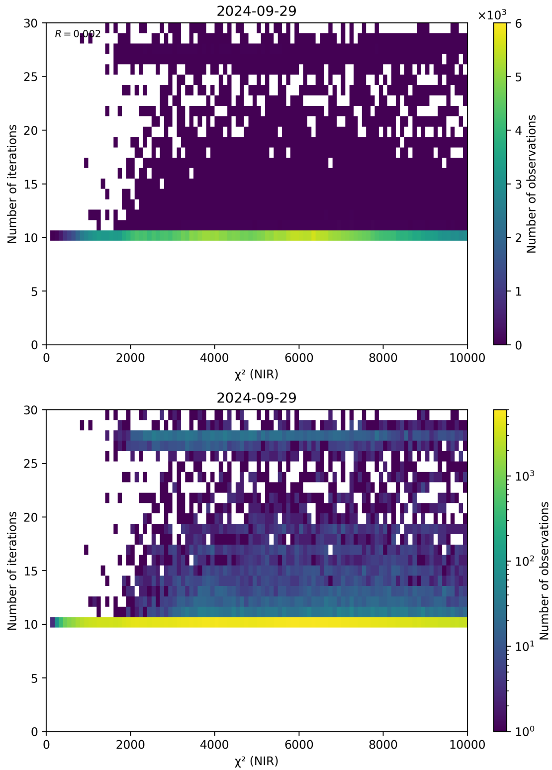
Figure 46: Scatter density plot of “ \chi^2 (NIR)” against “Number of iterations” for 2024-09-28 to 2024-09-30.
