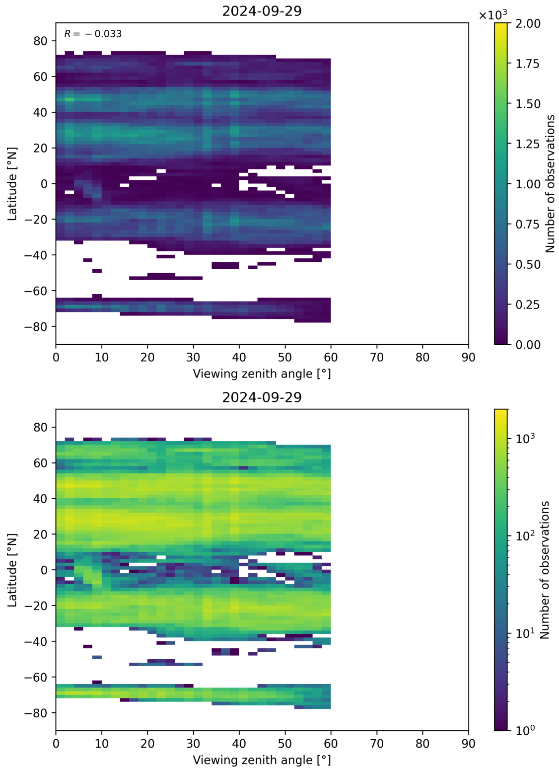
Figure 109: Scatter density plot of “Viewing zenith angle” against “Latitude” for 2024-09-28 to 2024-09-30.
