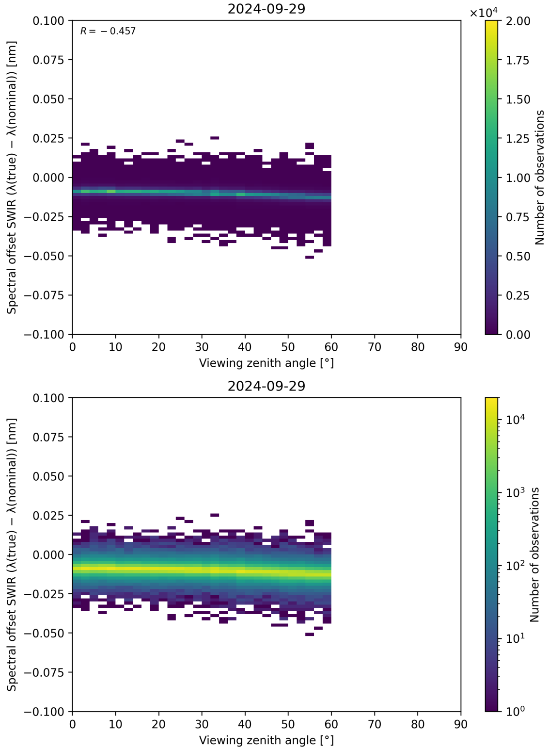
Figure 116: Scatter density plot of “Viewing zenith angle” against “Spectral offset SWIR ( \lambda_{\text{true}} - \lambda_{\text{nominal}} )” for 2024-09-28 to 2024-09-30.
