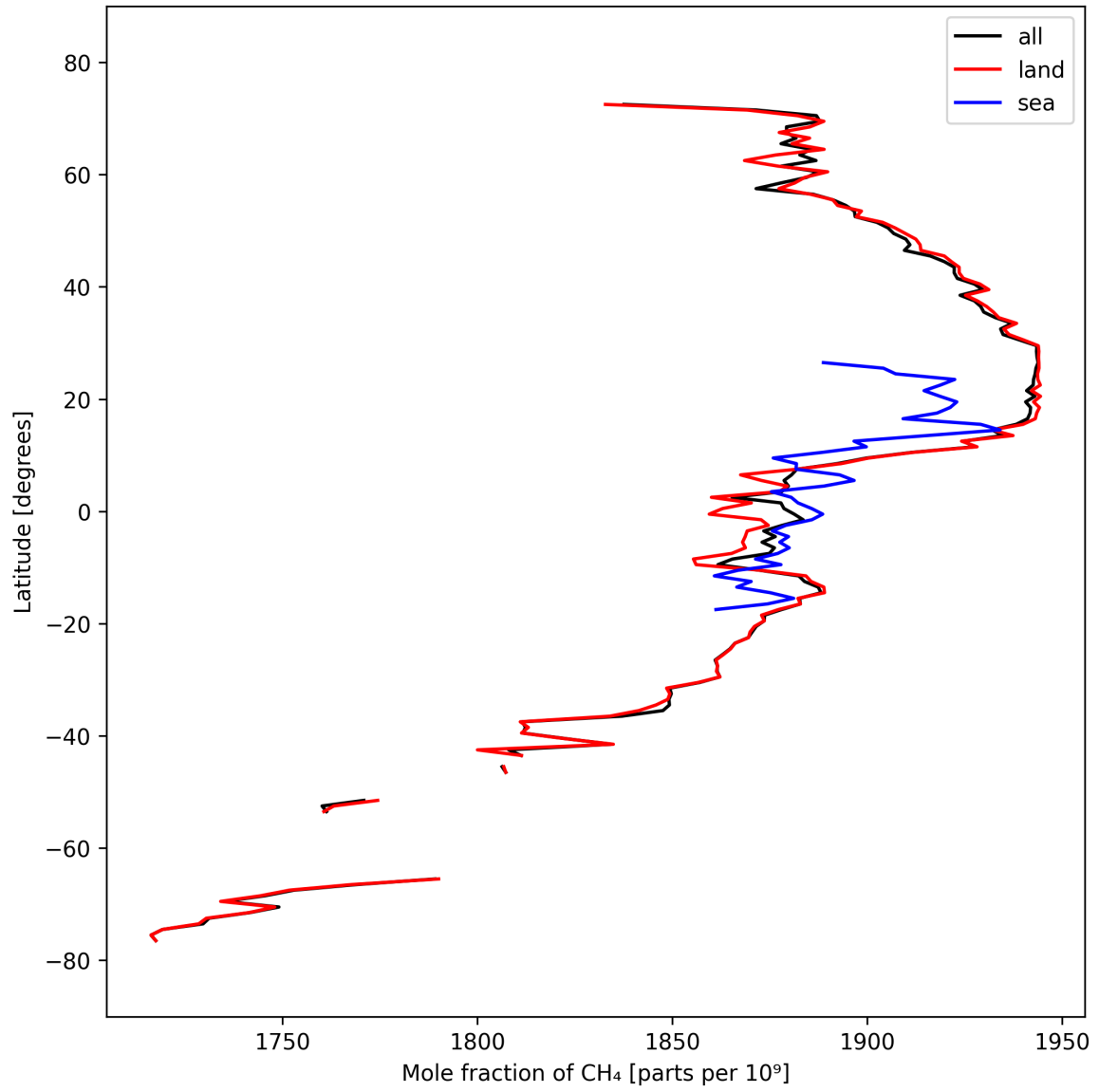
Figure 12: Zonal average of “Mole fraction of CH 4 ” for 2024-09-28 to 2024-09-30.
