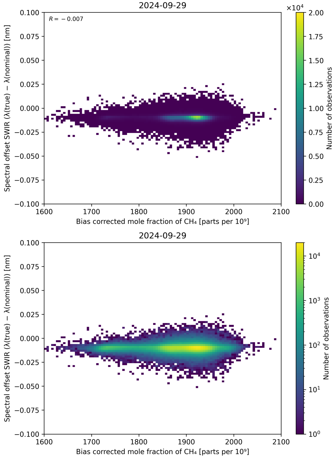
Figure 69: Scatter density plot of “Bias corrected mole fraction of \text{CH}_4 ” against “Spectral offset SWIR ( \lambda_{\text{true}} - \lambda_{\text{nominal}} )” for 2024-09-28 to 2024-09-30.
