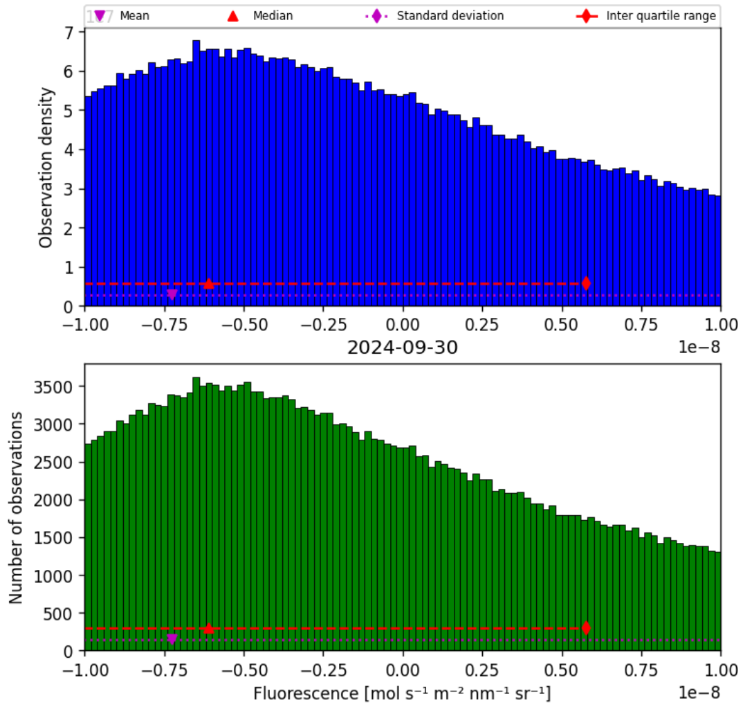
Figure 32: Histogram of “Fluorescence” for 2024-09-29 to 2024-10-01
