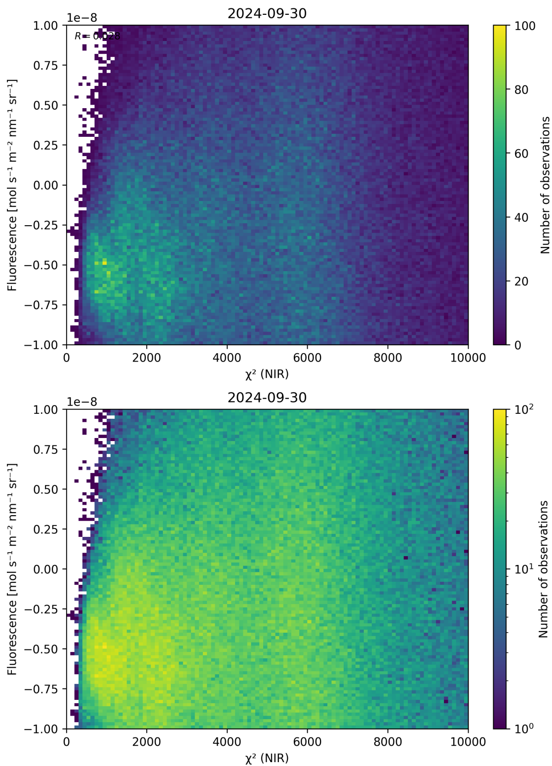
Figure 45: Scatter density plot of “ \chi^2 (NIR)” against “Fluorescence” for 2024-09-29 to 2024-10-01.
