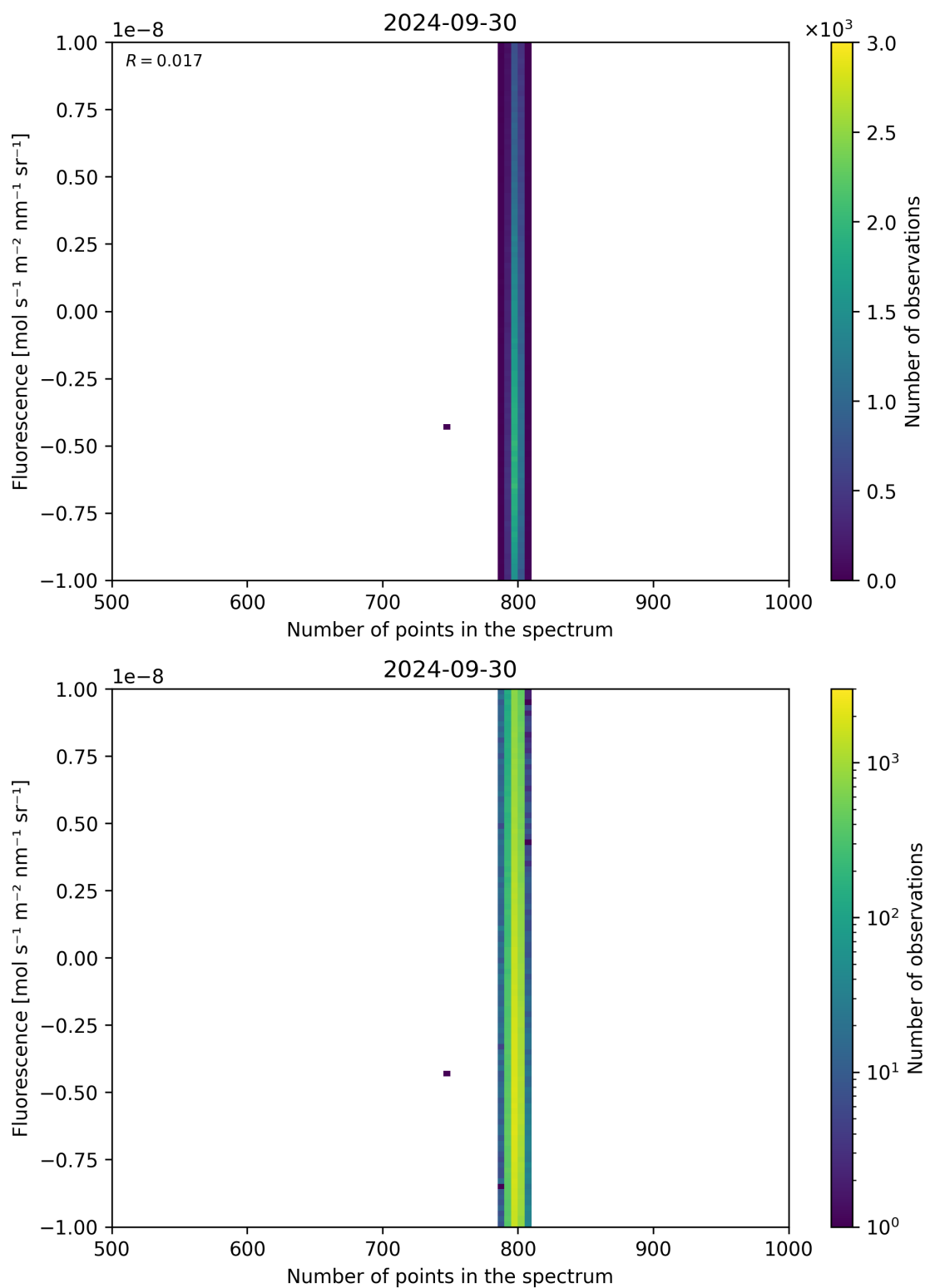
Figure 91: Scatter density plot of “Number of points in the spectrum” against “Fluorescence” for 2024-09-29 to 2024-10-01.
