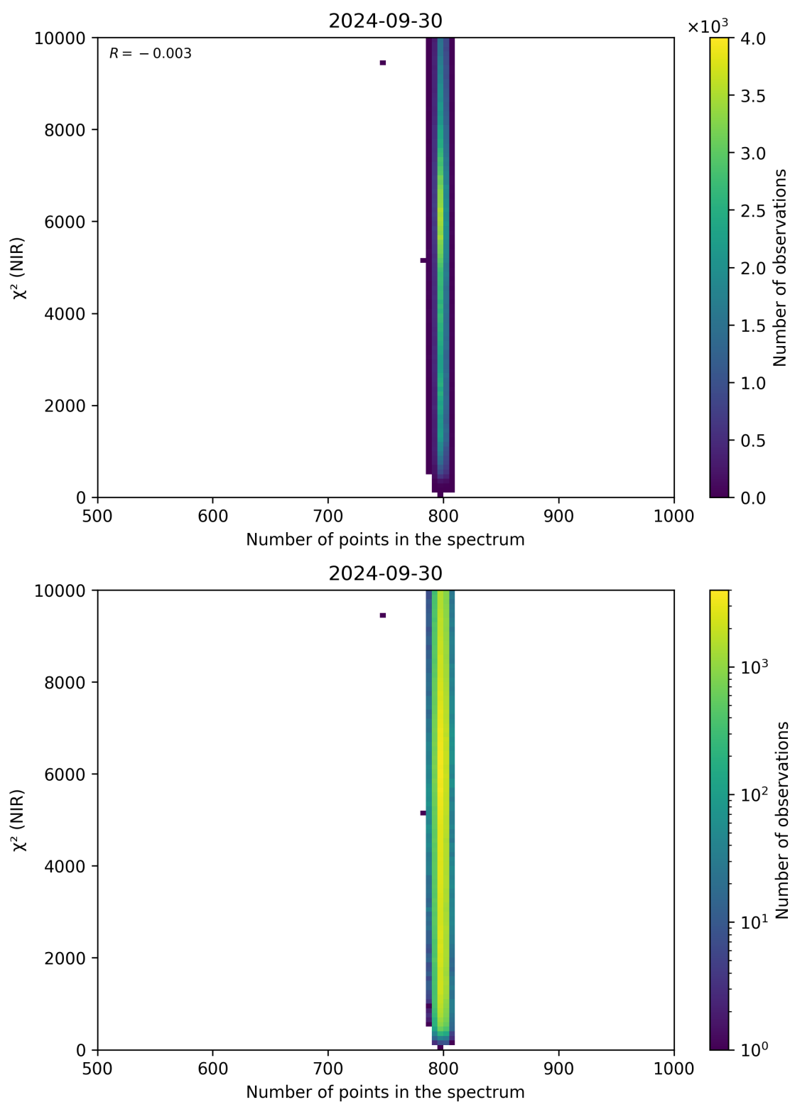
Figure 88: Scatter density plot of “Number of points in the spectrum” against “ \chi^2 (NIR)” for 2024-09-29 to 2024-10-01.
