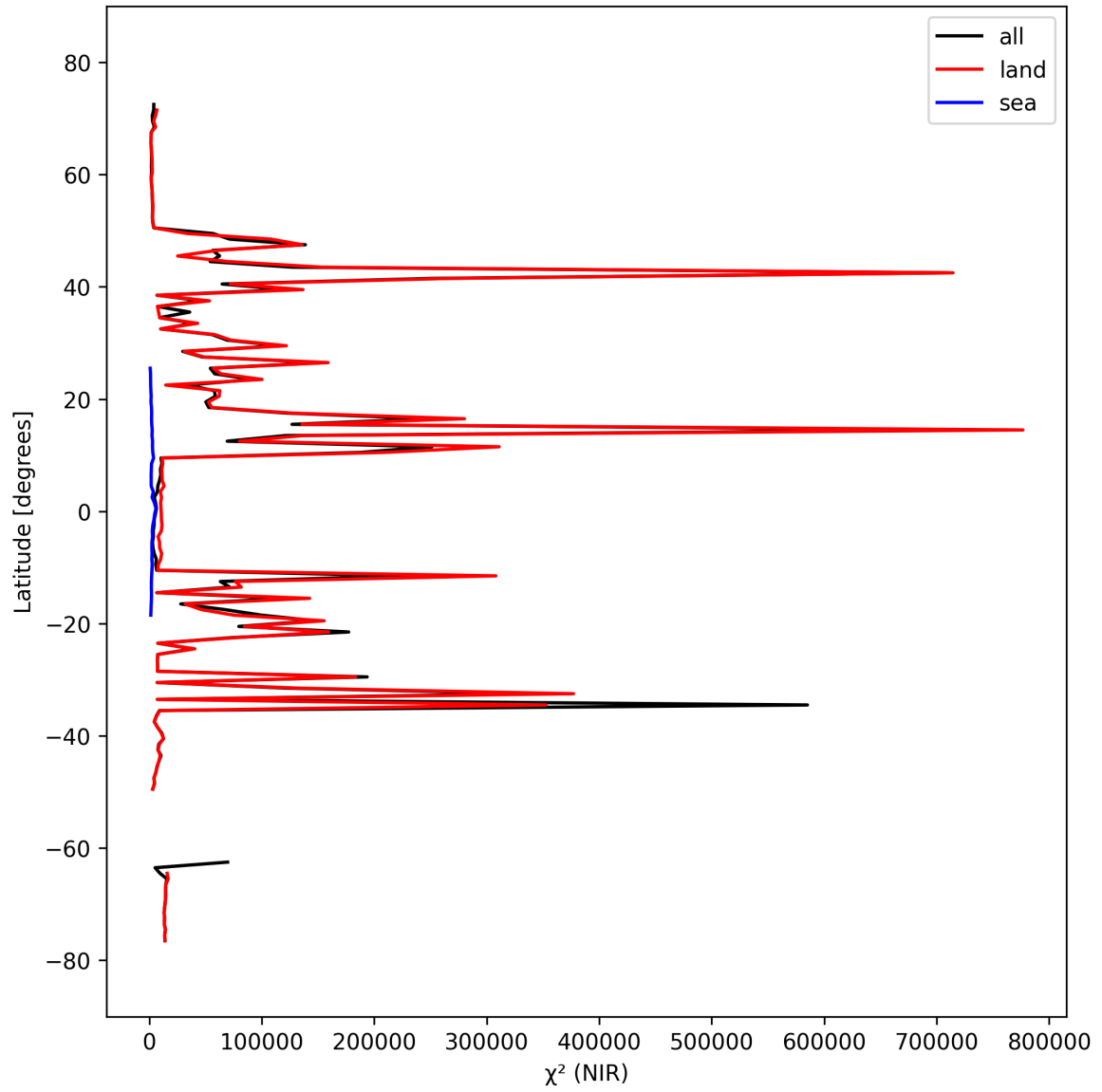
Figure 18: Zonal average of “ \chi^2 (NIR)” for 2024-09-29 to 2024-10-01.
