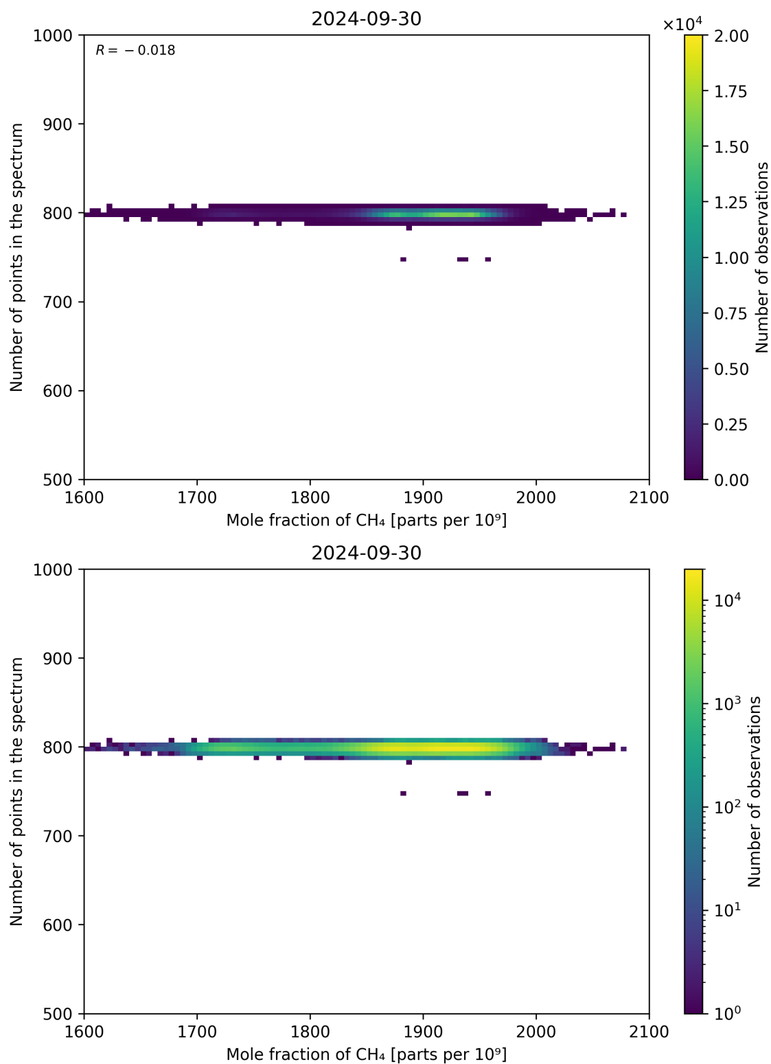
Figure 77: Scatter density plot of “Mole fraction of CH 4 ” against “Number of points in the spectrum” for 2024-09-29 to 2024-10-01.
