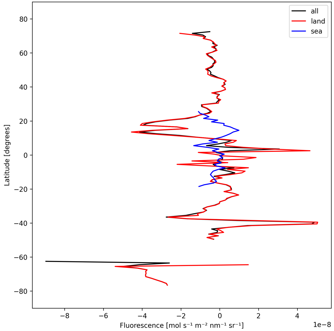
Figure 21: Zonal average of “Fluorescence” for 2024-09-29 to 2024-10-01.
