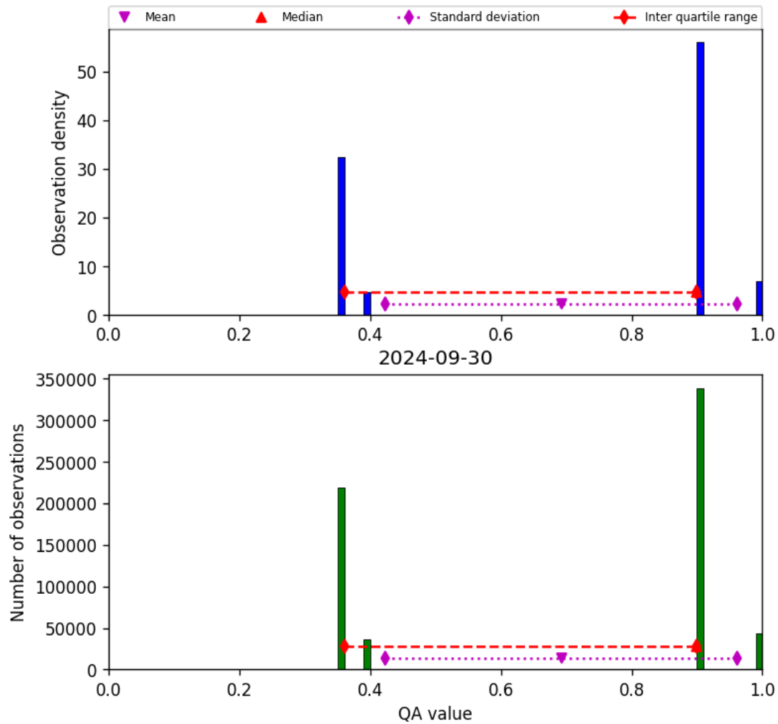
Figure 22: Histogram of “QA value” for 2024-09-29 to 2024-10-01
