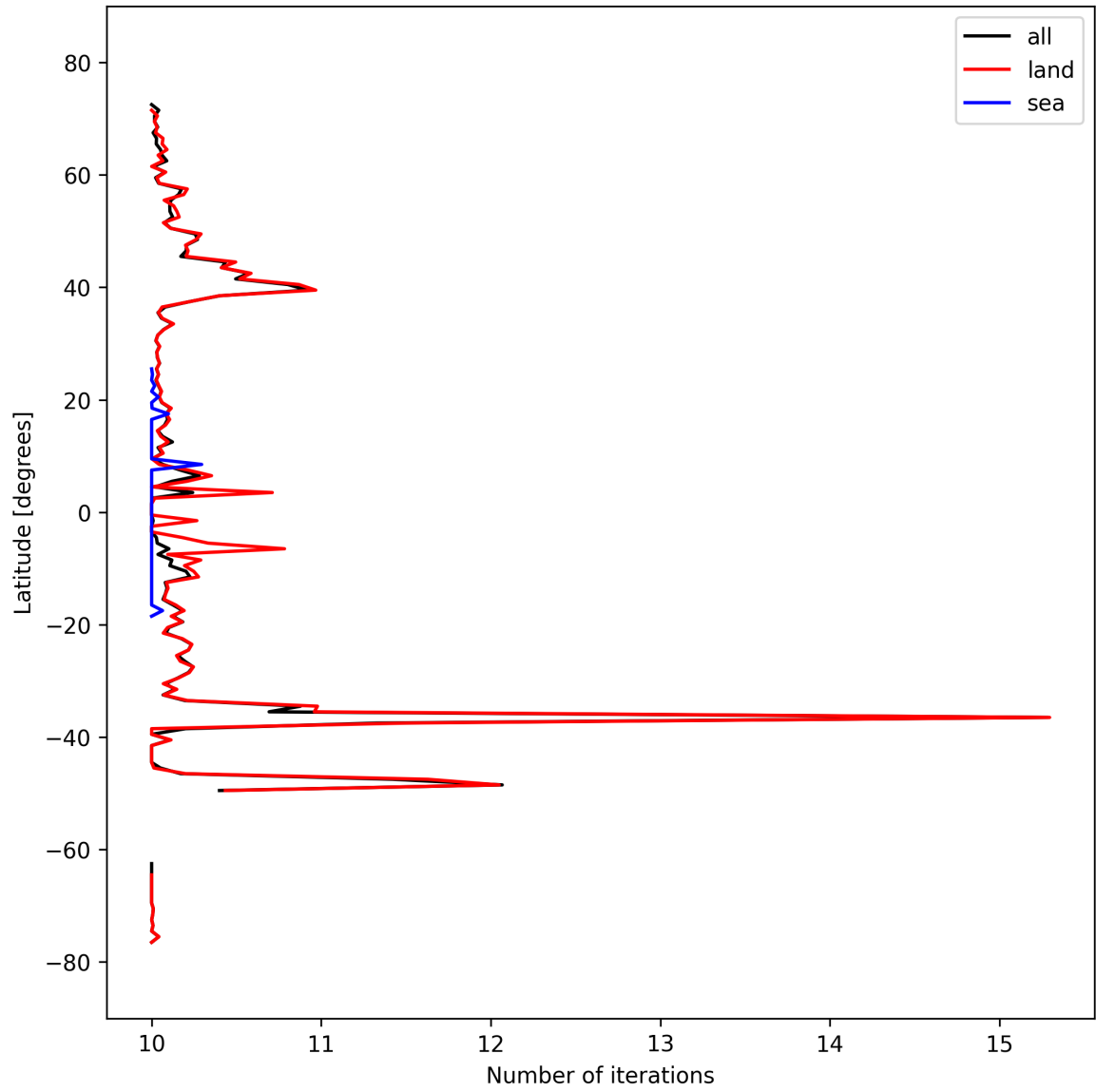
Figure 20: Zonal average of “Number of iterations” for 2024-09-29 to 2024-10-01.
