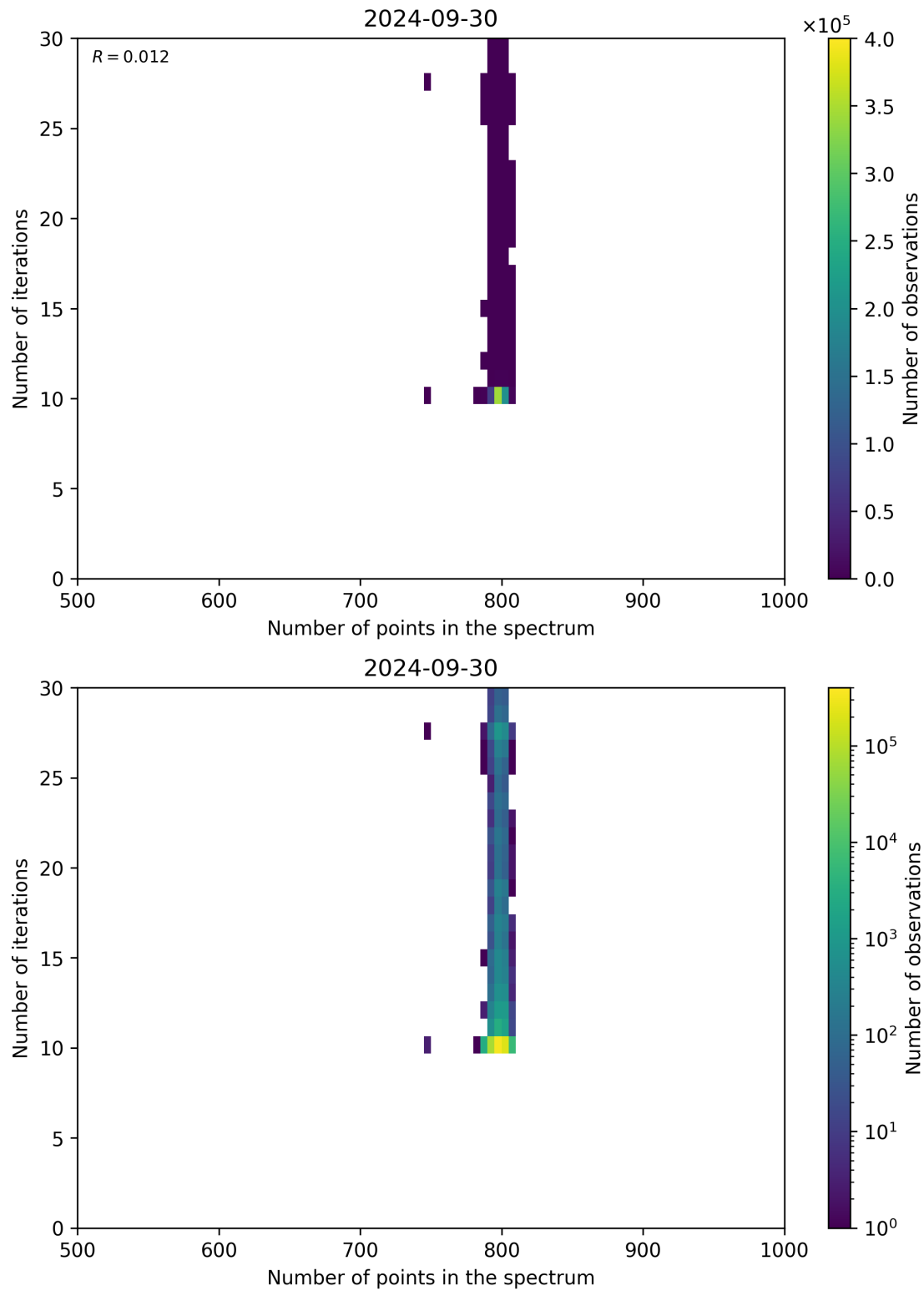
Figure 92: Scatter density plot of “Number of points in the spectrum” against “Number of iterations” for 2024-09-29 to 2024-10-01.
