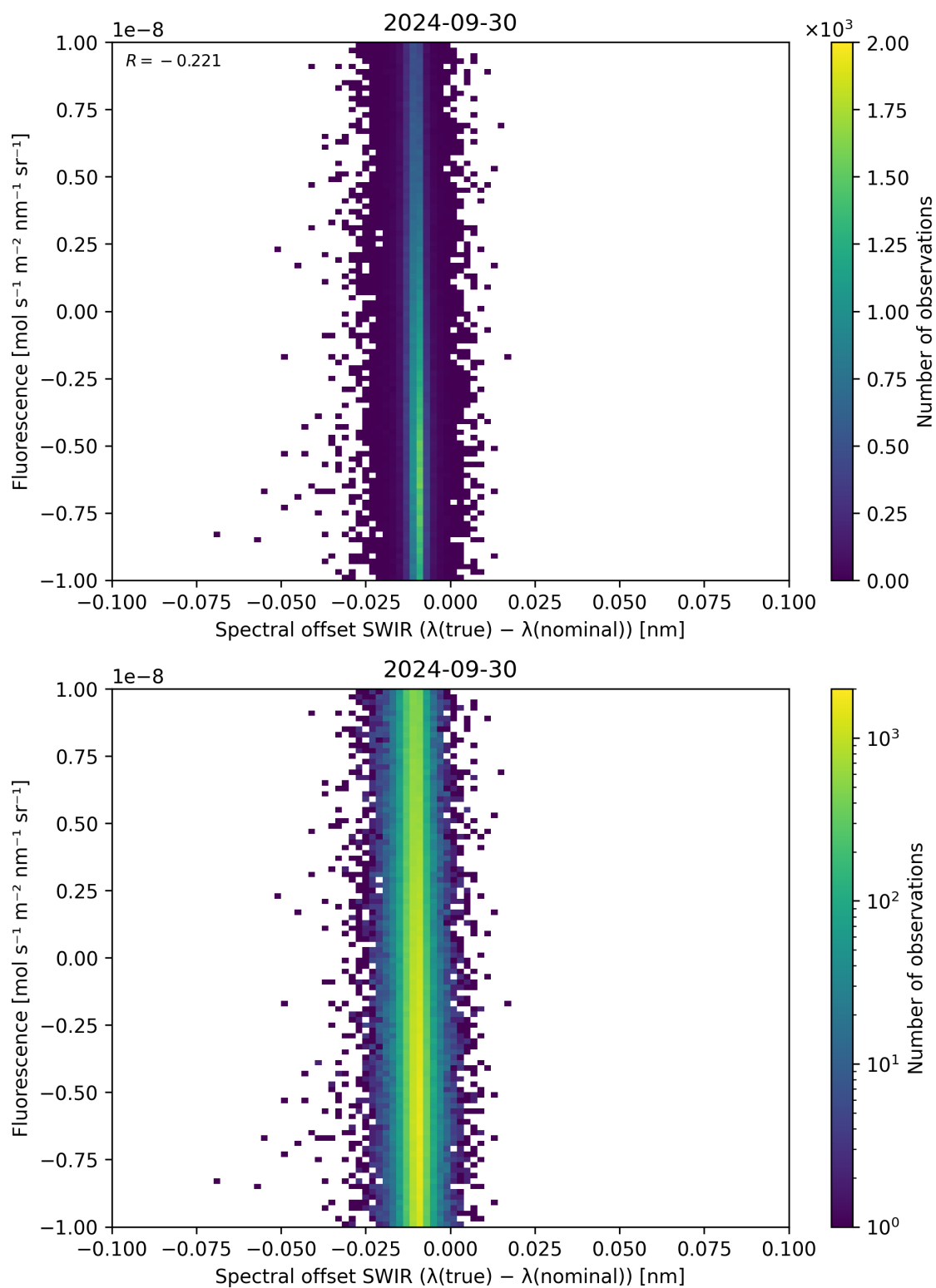
Figure 120: Scatter density plot of “Spectral offset SWIR ( \lambda_{\text{true}} - \lambda_{\text{nominal}} )” against “Fluorescence” for 2024-09-29 to 2024-10-01.
