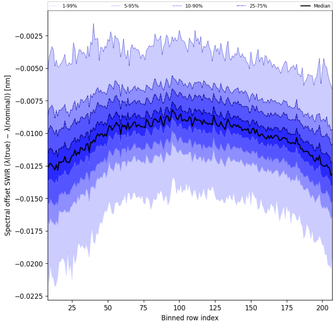
Figure 38: Along track statistics of “Spectral offset SWIR ( \lambda_{\text{true}} - \lambda_{\text{nominal}} )” for 2024-09-29 to 2024-10-01
