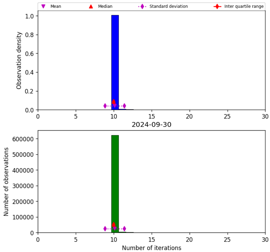
Figure 31: Histogram of “Number of iterations” for 2024-09-29 to 2024-10-01
