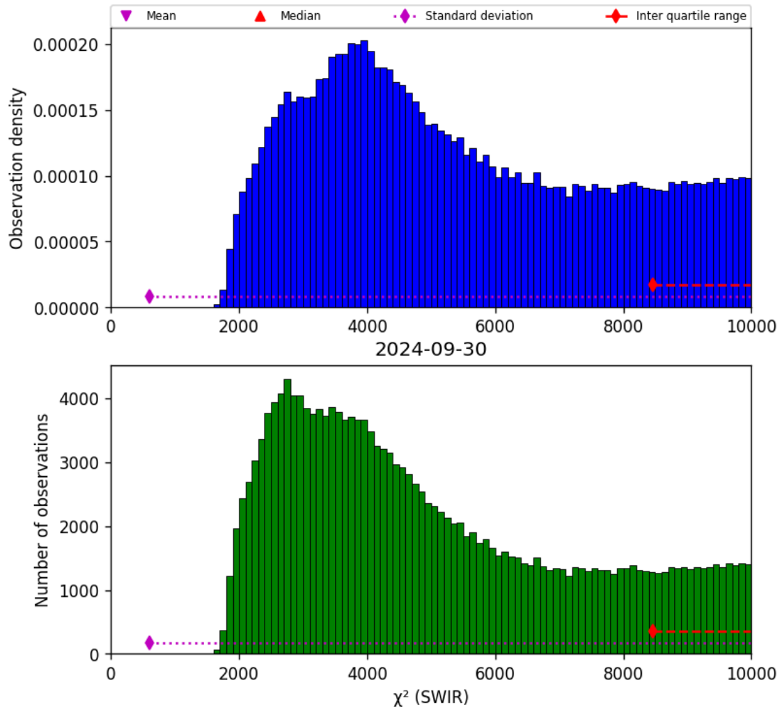
Figure 28: Histogram of " \chi^2 (SWIR)" for 2024-09-29 to 2024-10-01
