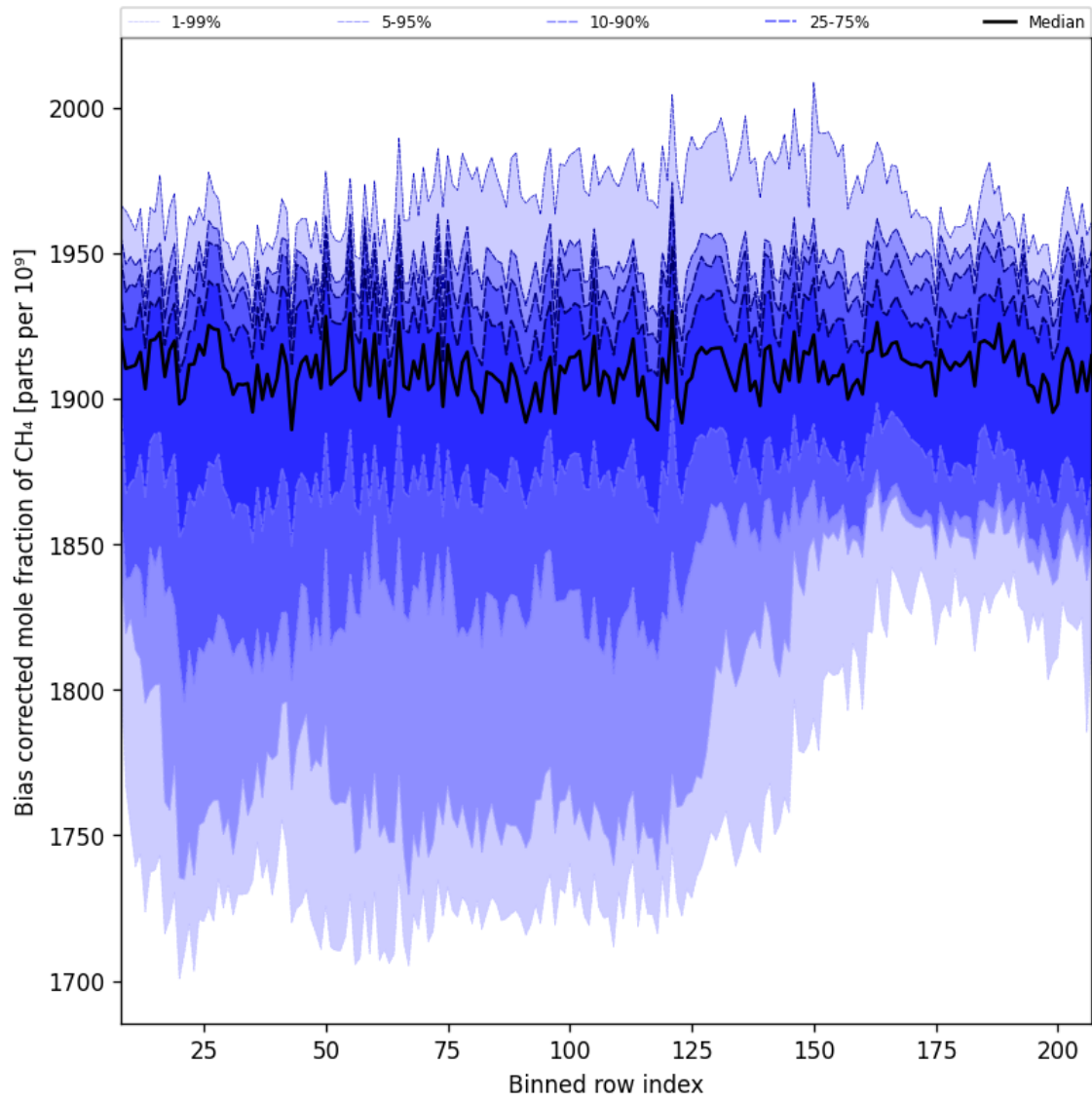
Figure 36: Along track statistics of “Bias corrected mole fraction of CH 4 ” for 2024-09-29 to 2024-10-01
