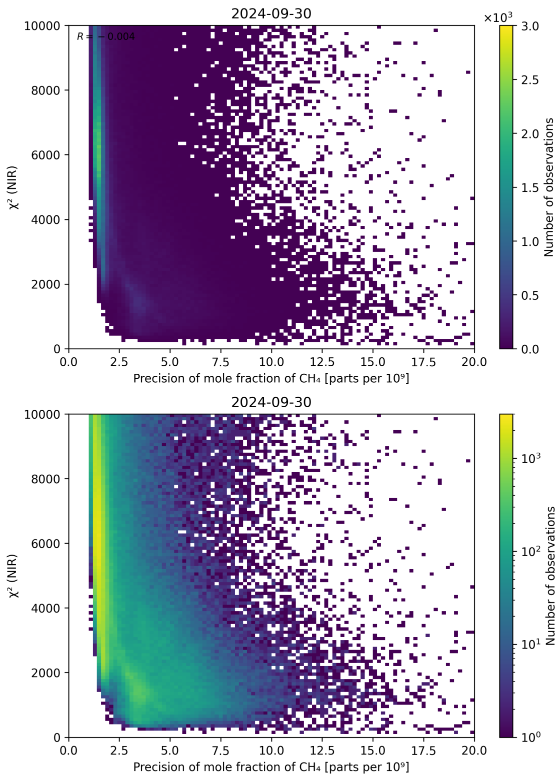
Figure 78: Scatter density plot of “Precision of mole fraction of CH 4 ” against “ \chi^2 (NIR)” for 2024-09-29 to 2024-10-01.
