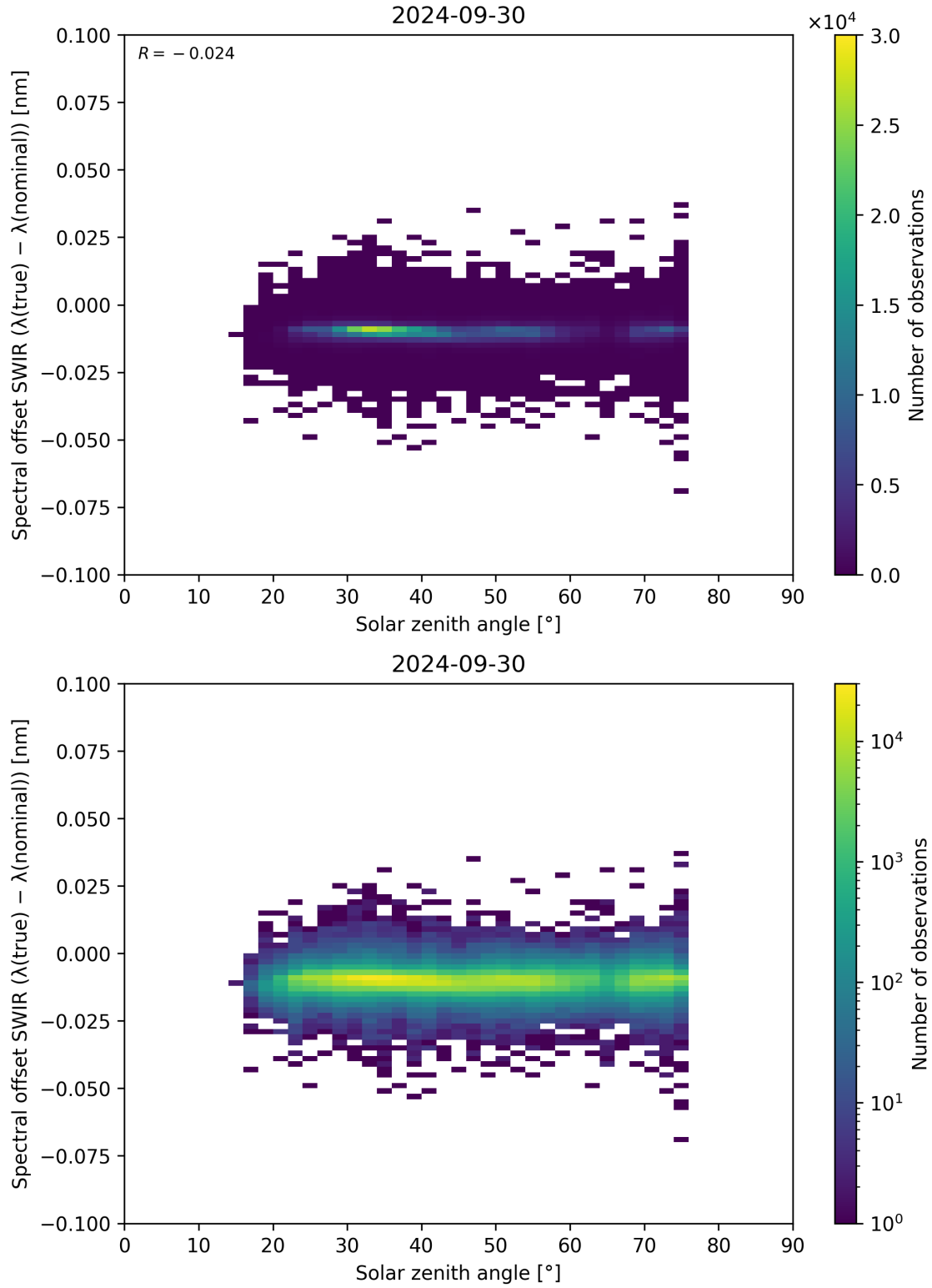
Figure 104: Scatter density plot of “Solar zenith angle” against “Spectral offset SWIR ( \lambda_{\text{true}} - \lambda_{\text{nominal}} )” for 2024-09-29 to 2024-10-01.
