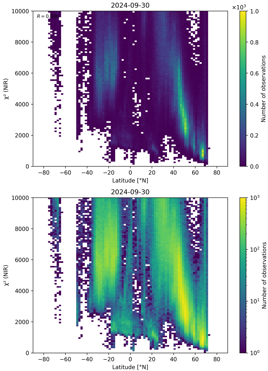
Figure 53: Scatter density plot of “Latitude” against “ \chi^2 (NIR)” for 2024-09-29 to 2024-10-01.
