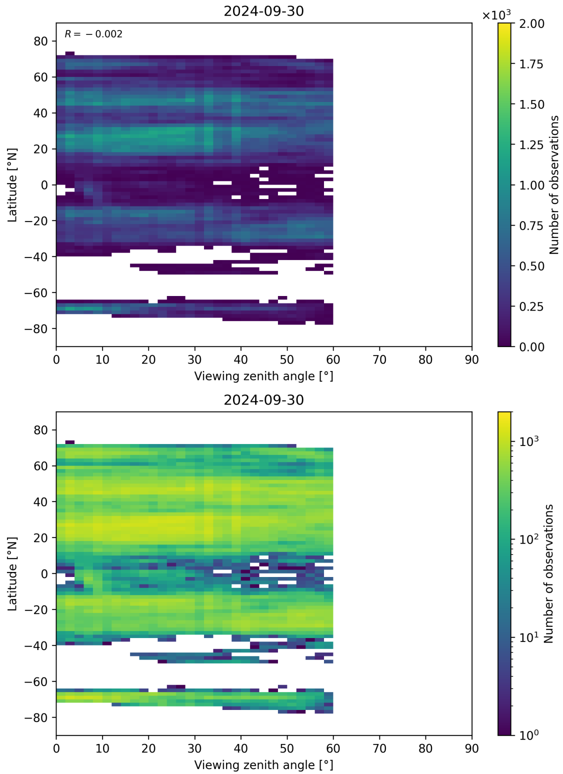
Figure 109: Scatter density plot of “Viewing zenith angle” against “Latitude” for 2024-09-29 to 2024-10-01.
