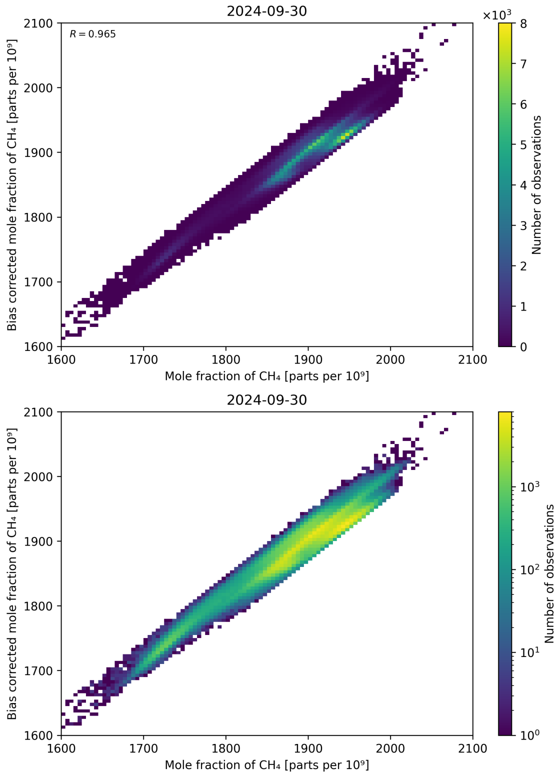
Figure 74: Scatter density plot of “Mole fraction of CH 4 ” against “Bias corrected mole fraction of CH 4 ” for 2024-09-29 to 2024-10-01.
