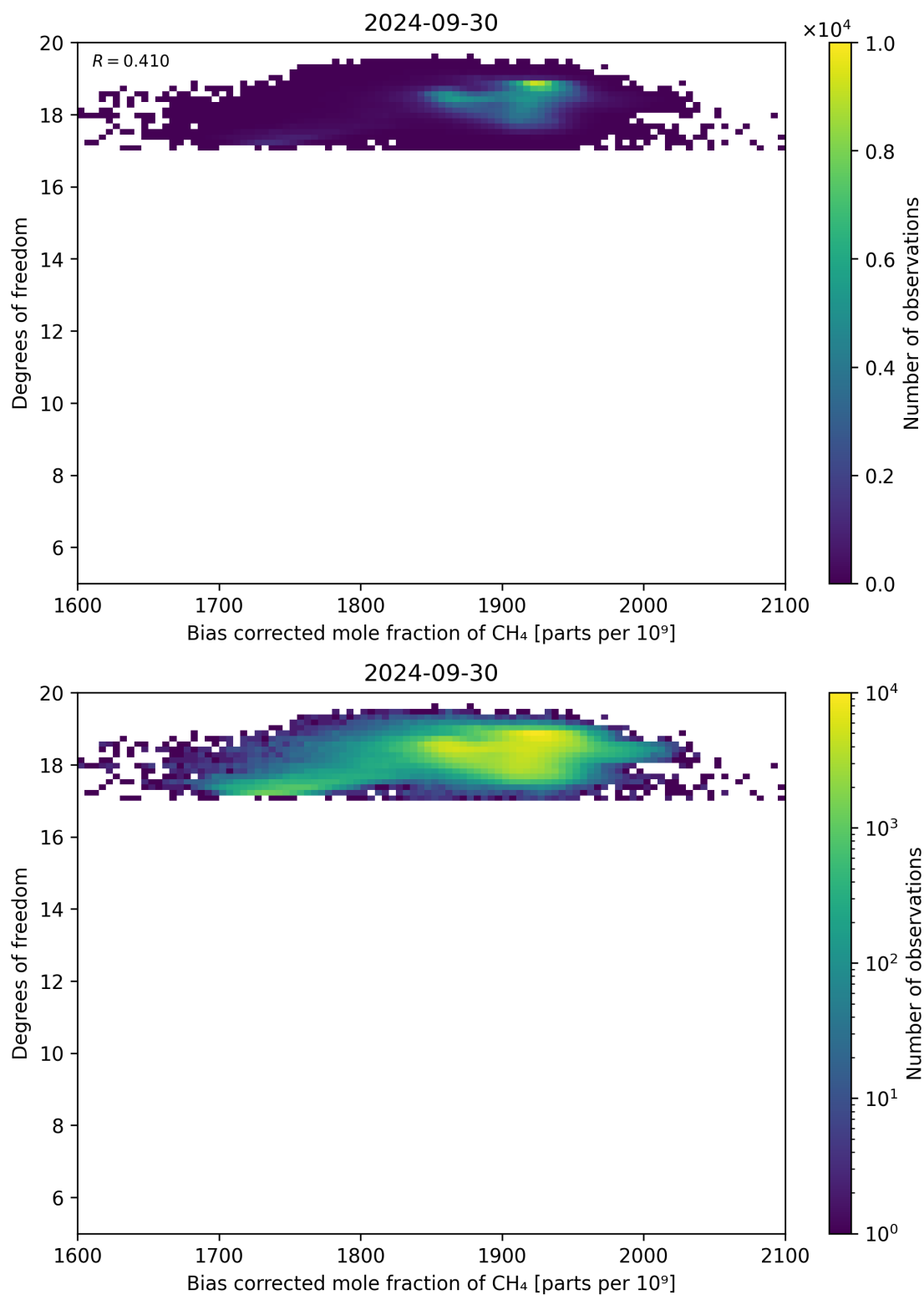
Figure 65: Scatter density plot of “Bias corrected mole fraction of CH 4 ” against “Degrees of freedom” for 2024-09-29 to 2024-10-01.
