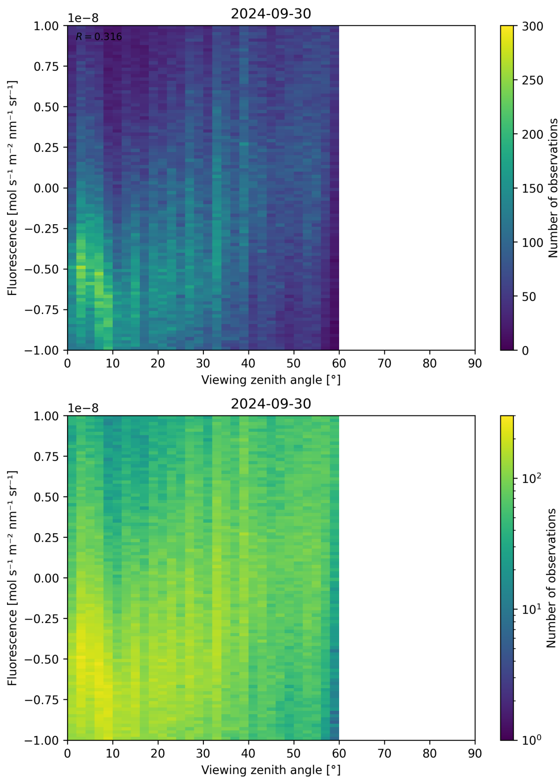
Figure 108: Scatter density plot of “Viewing zenith angle” against “Fluorescence” for 2024-09-29 to 2024-10-01.
