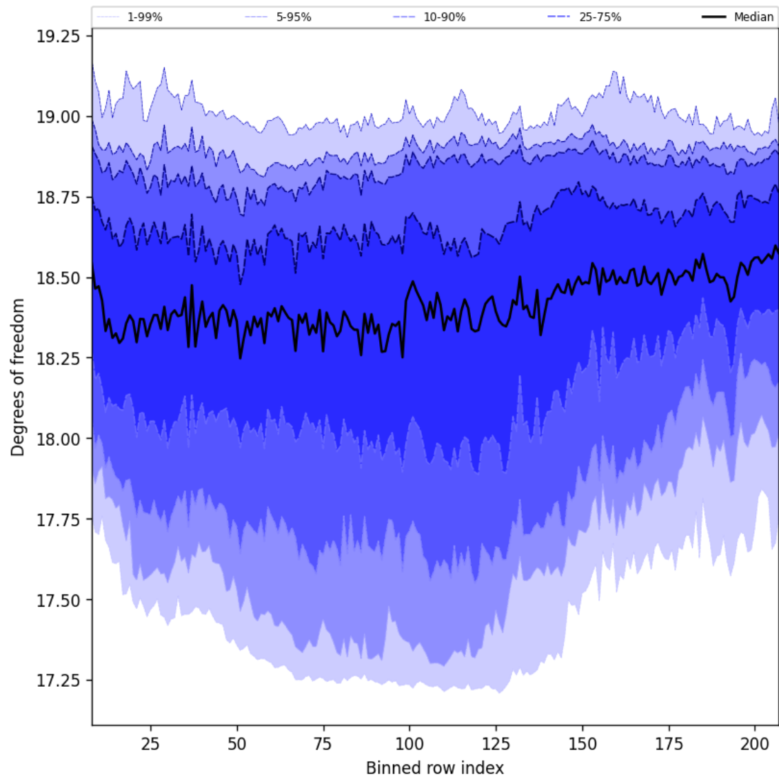
Figure 41: Along track statistics of “Degrees of freedom” for 2024-09-29 to 2024-10-01
