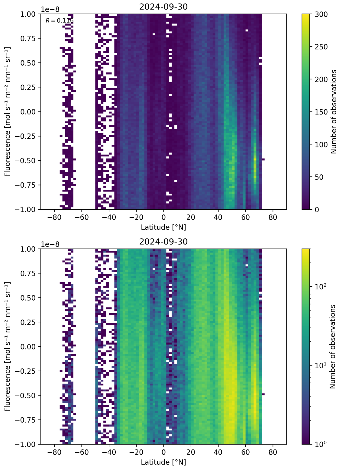
Figure 56: Scatter density plot of “Latitude” against “Fluorescence” for 2024-09-29 to 2024-10-01.
