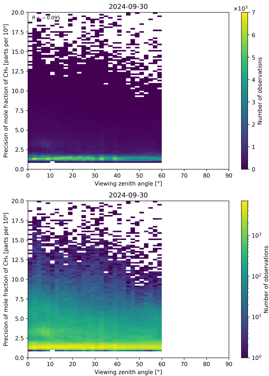
Figure 112: Scatter density plot of “Viewing zenith angle” against “Precision of mole fraction of CH 4 ” for 2024-09-29 to 2024-10-01.
