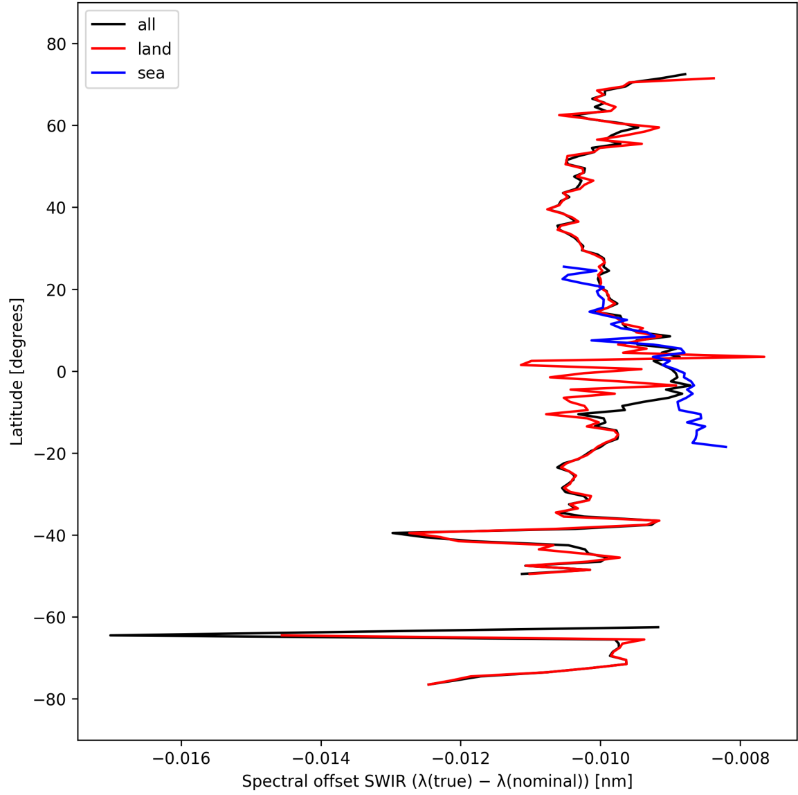
Figure 16: Zonal average of “Spectral offset SWIR ( \lambda_{\text{true}} - \lambda_{\text{nominal}} )” for 2024-09-29 to 2024-10-01.
