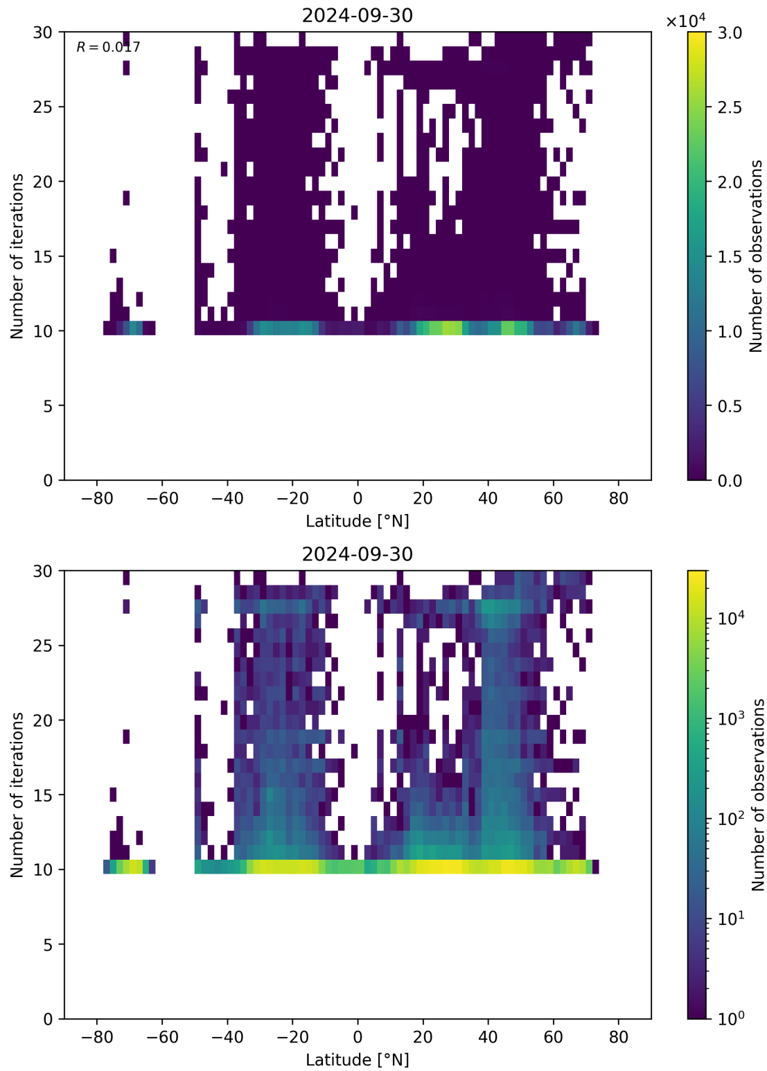
Figure 60: Scatter density plot of “Latitude” against “Number of iterations” for 2024-09-29 to 2024-10-01.
