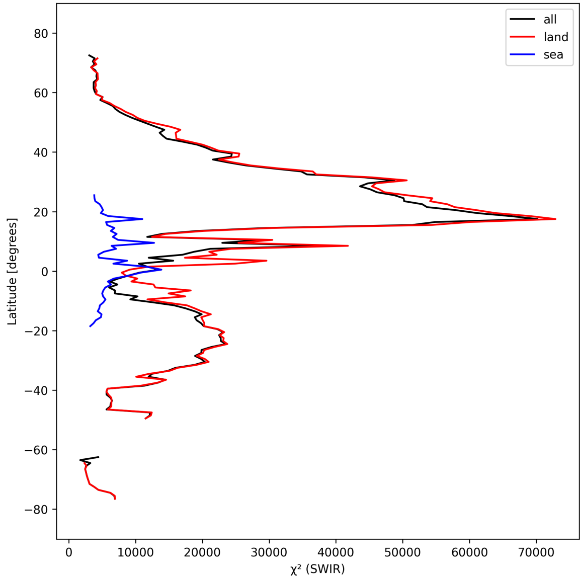
Figure 17: Zonal average of “ \chi^2 (SWIR)” for 2024-09-29 to 2024-10-01.
