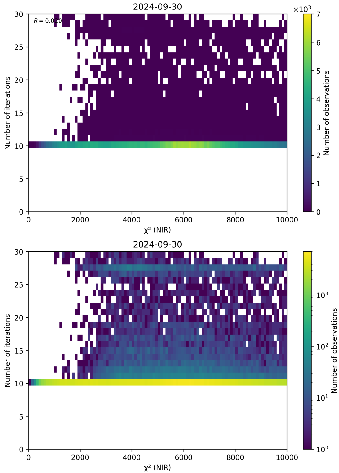
Figure 46: Scatter density plot of “ \chi^2 (NIR)” against “Number of iterations” for 2024-09-29 to 2024-10-01.
