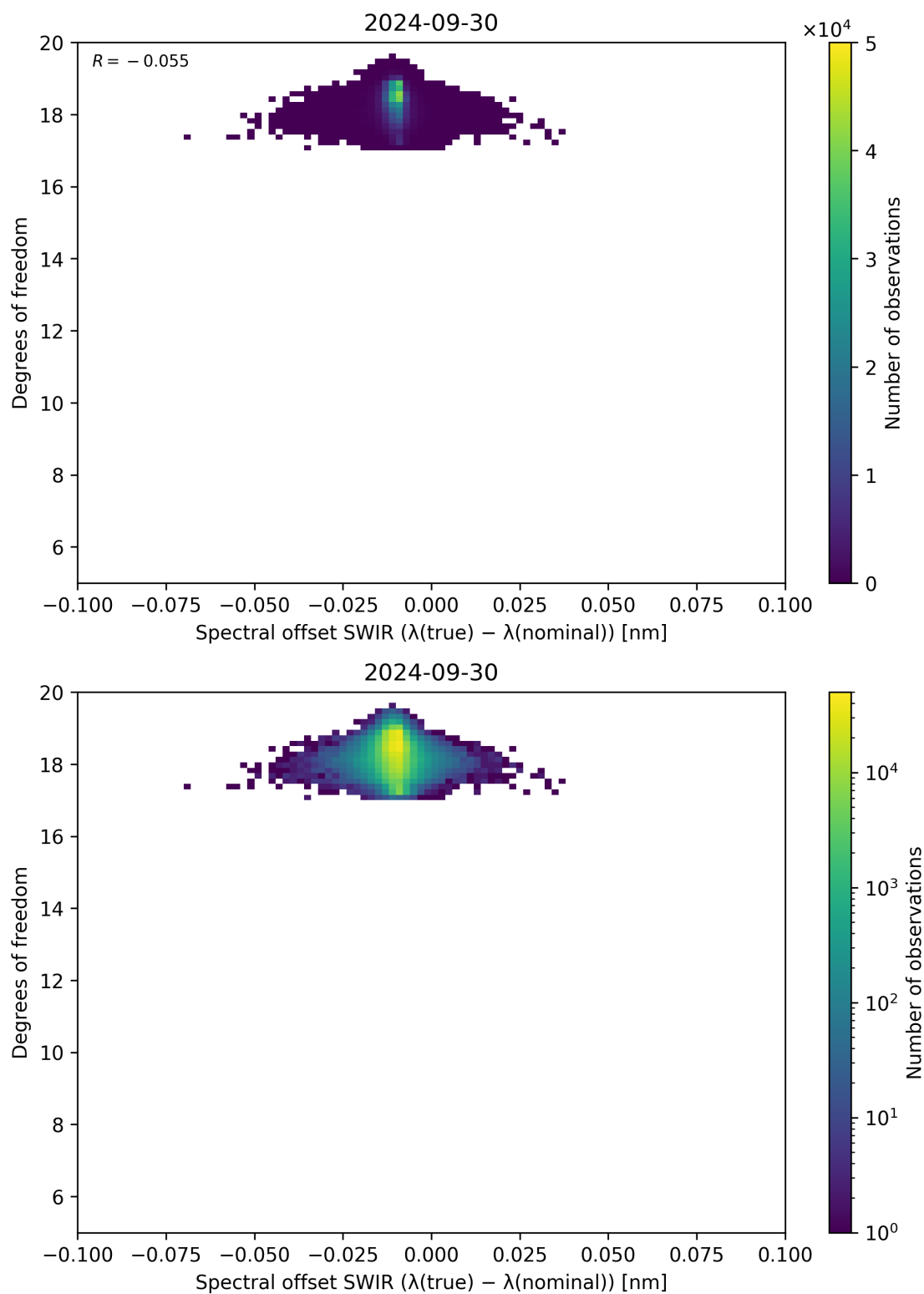
Figure 119: Scatter density plot of “Spectral offset SWIR ( \lambda_{\text{true}} - \lambda_{\text{nominal}} )” against “Degrees of freedom” for 2024-09-29 to 2024-10-01.
