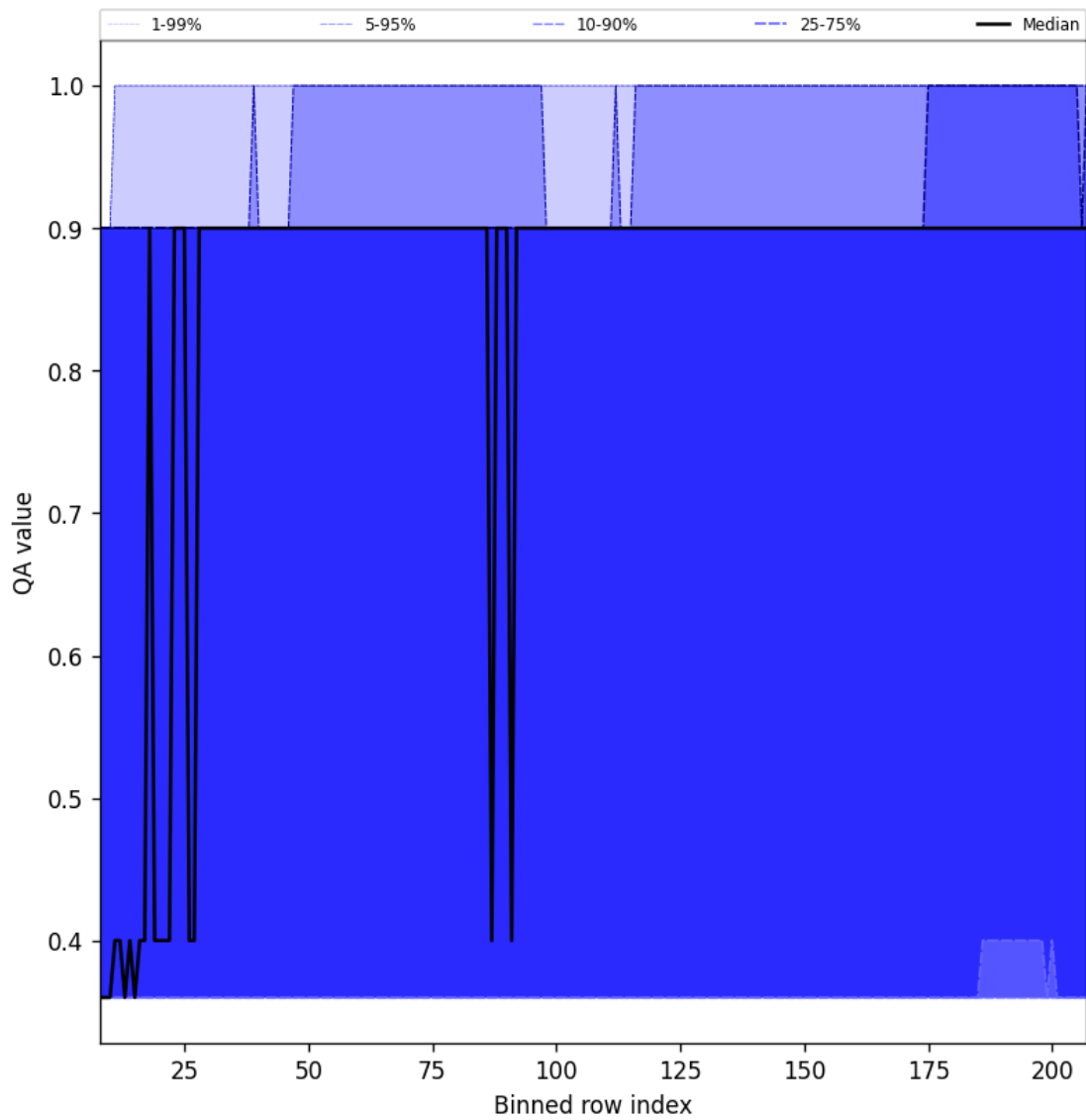
Figure 33: Along track statistics of “QA value” for 2024-09-29 to 2024-10-01
