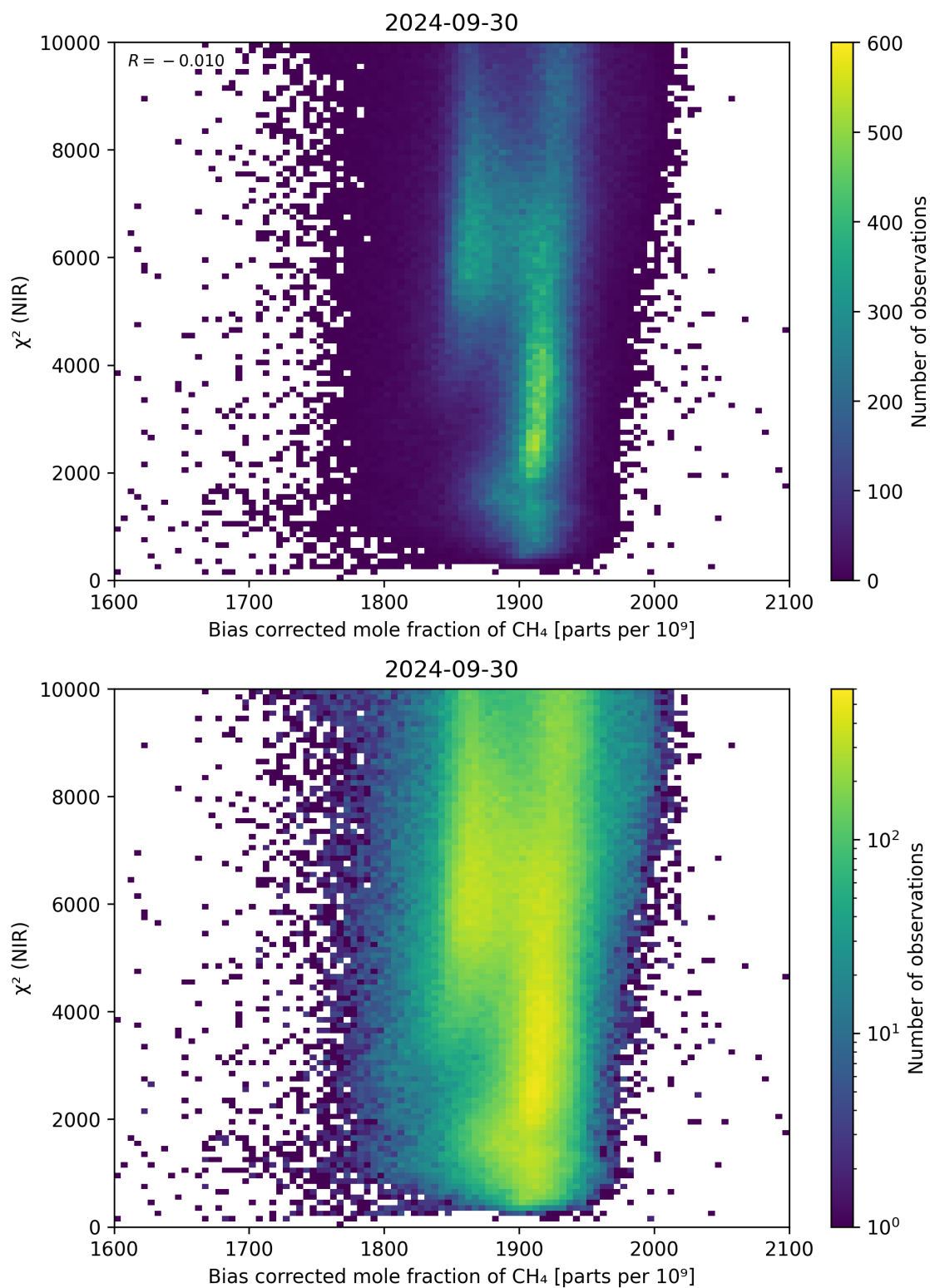
Figure 63: Scatter density plot of “Bias corrected mole fraction of CH 4 ” against “ \chi^2 (NIR)” for 2024-09-29 to 2024-10-01.
