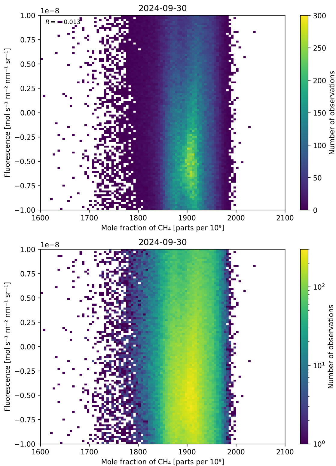
Figure 73: Scatter density plot of “Mole fraction of \text{CH}_4 ” against “Fluorescence” for 2024-09-29 to 2024-10-01.
