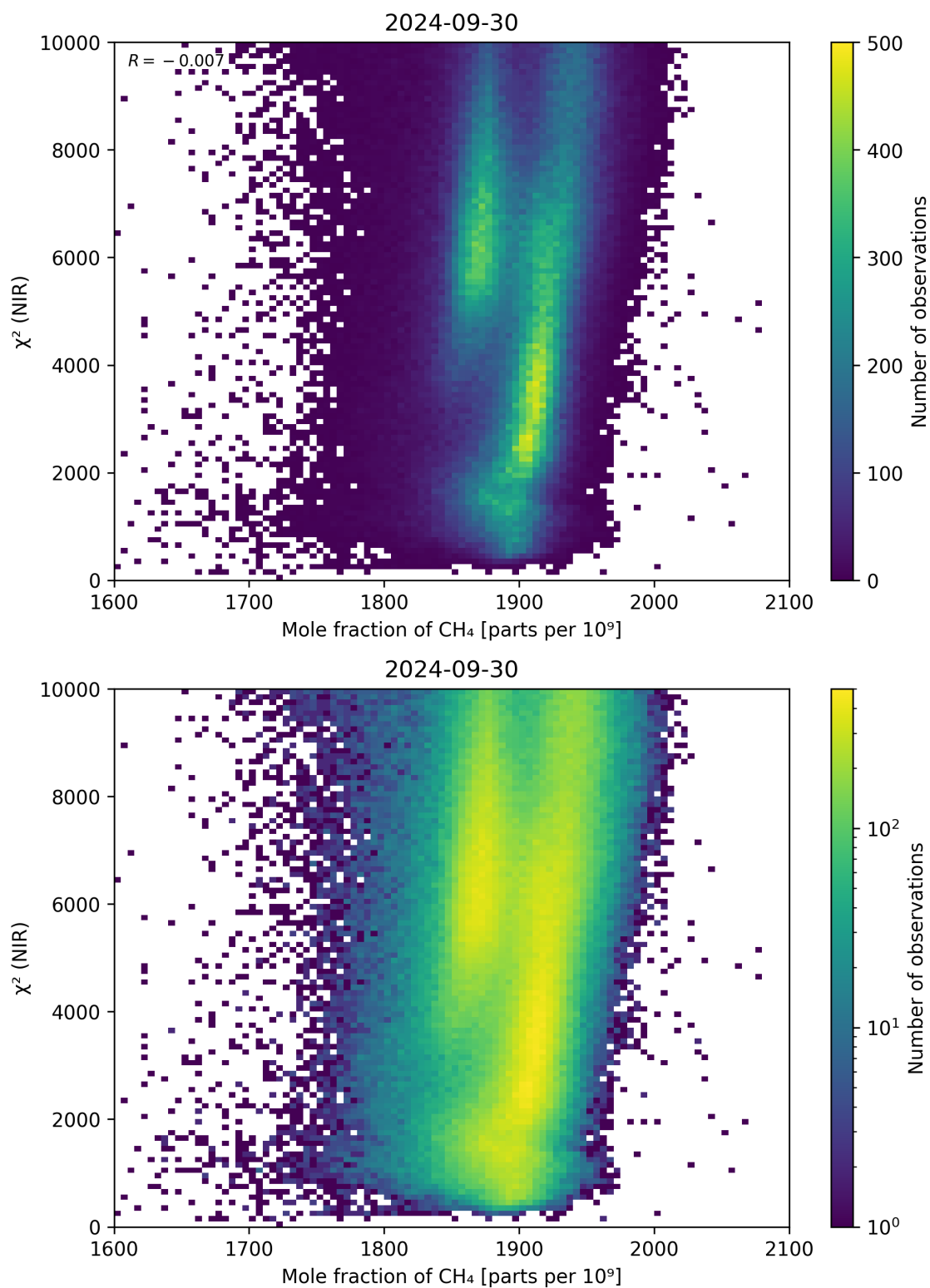
Figure 70: Scatter density plot of “Mole fraction of \text{CH}_4 ” against “ \chi^2 (NIR)” for 2024-09-29 to 2024-10-01.
