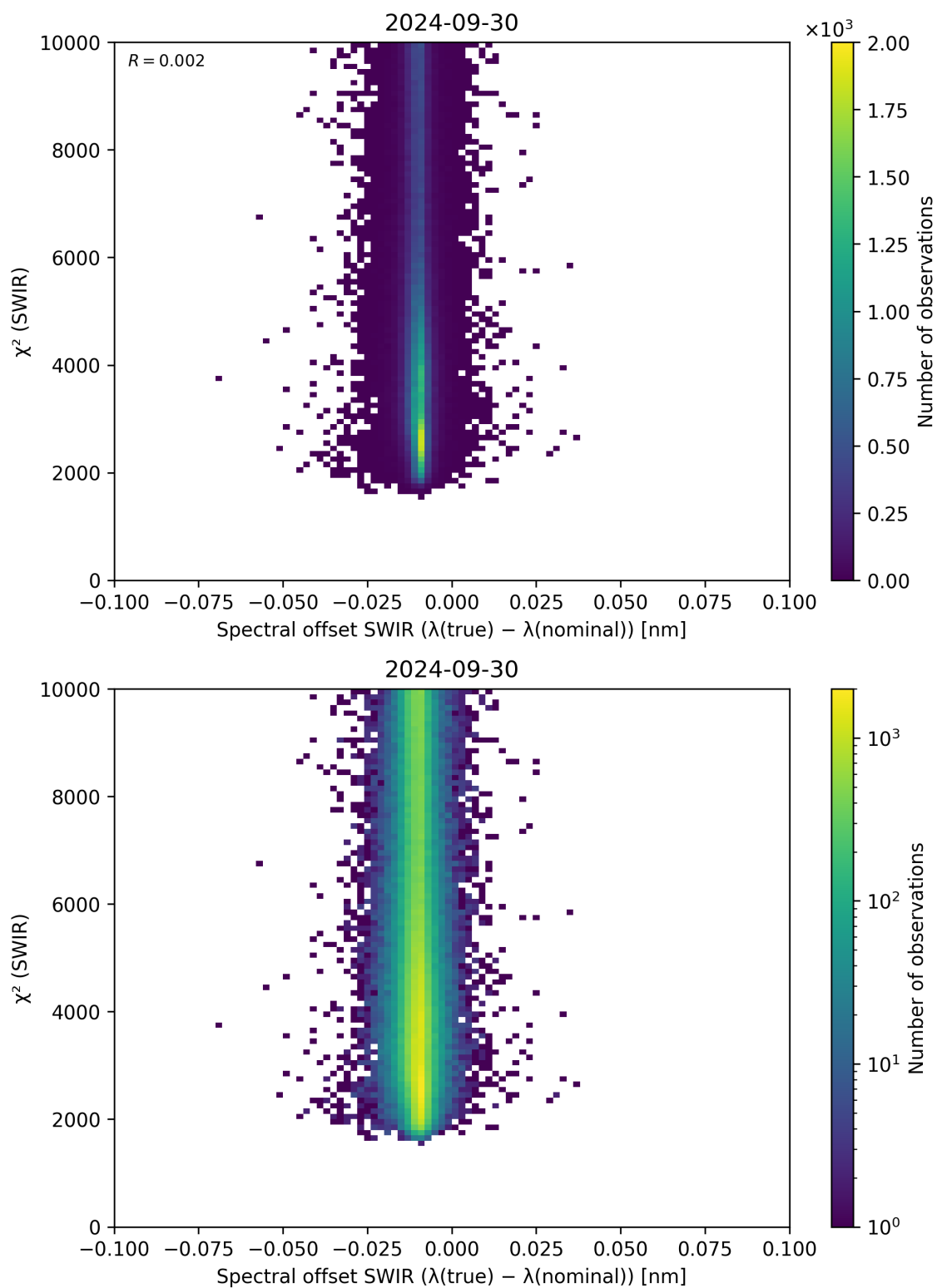
Figure 118: Scatter density plot of “Spectral offset SWIR ( \lambda_{\text{true}} - \lambda_{\text{nominal}} )” against “ \chi^2 (SWIR)” for 2024-09-29 to 2024-10-01.
