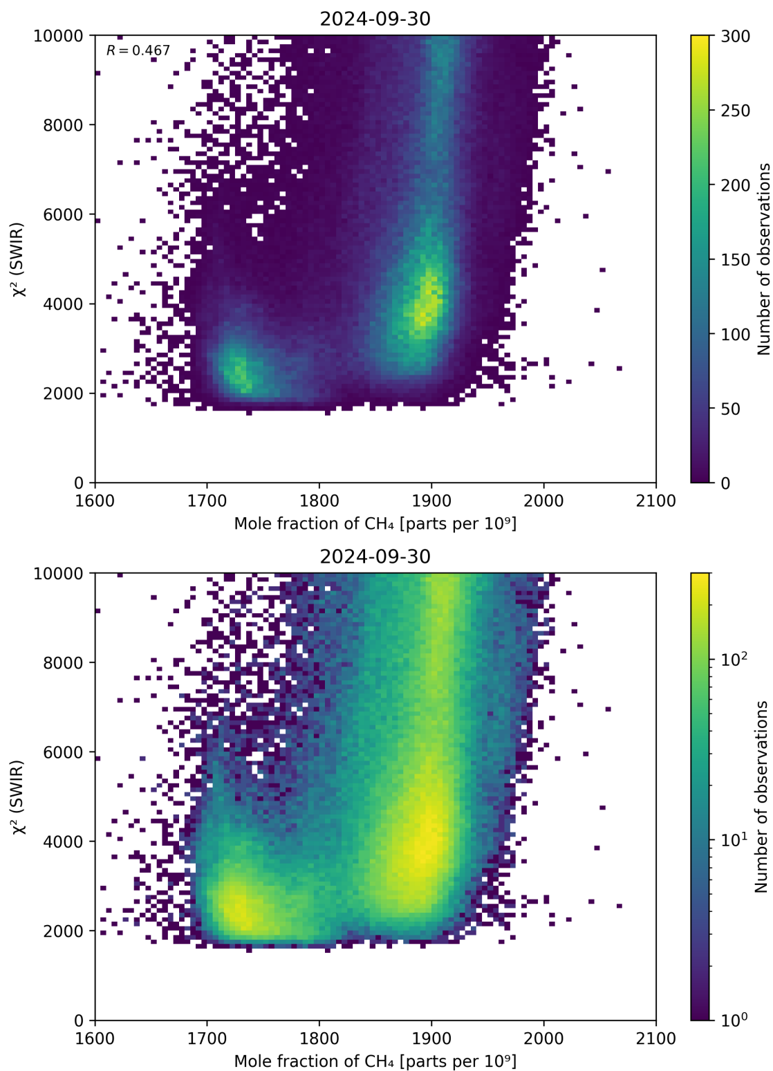
Figure 71: Scatter density plot of “Mole fraction of \text{CH}_4 ” against “ \chi^2 (SWIR)” for 2024-09-29 to 2024-10-01.
