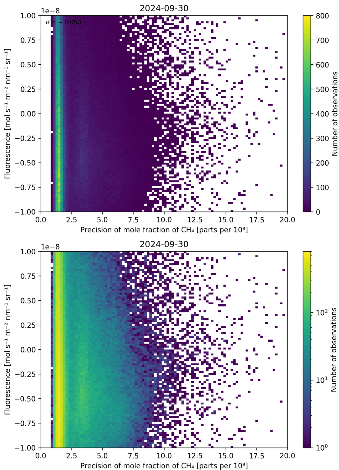
Figure 81: Scatter density plot of “Precision of mole fraction of \text{CH}_4 ” against “Fluorescence” for 2024-09-29 to 2024-10-01.
