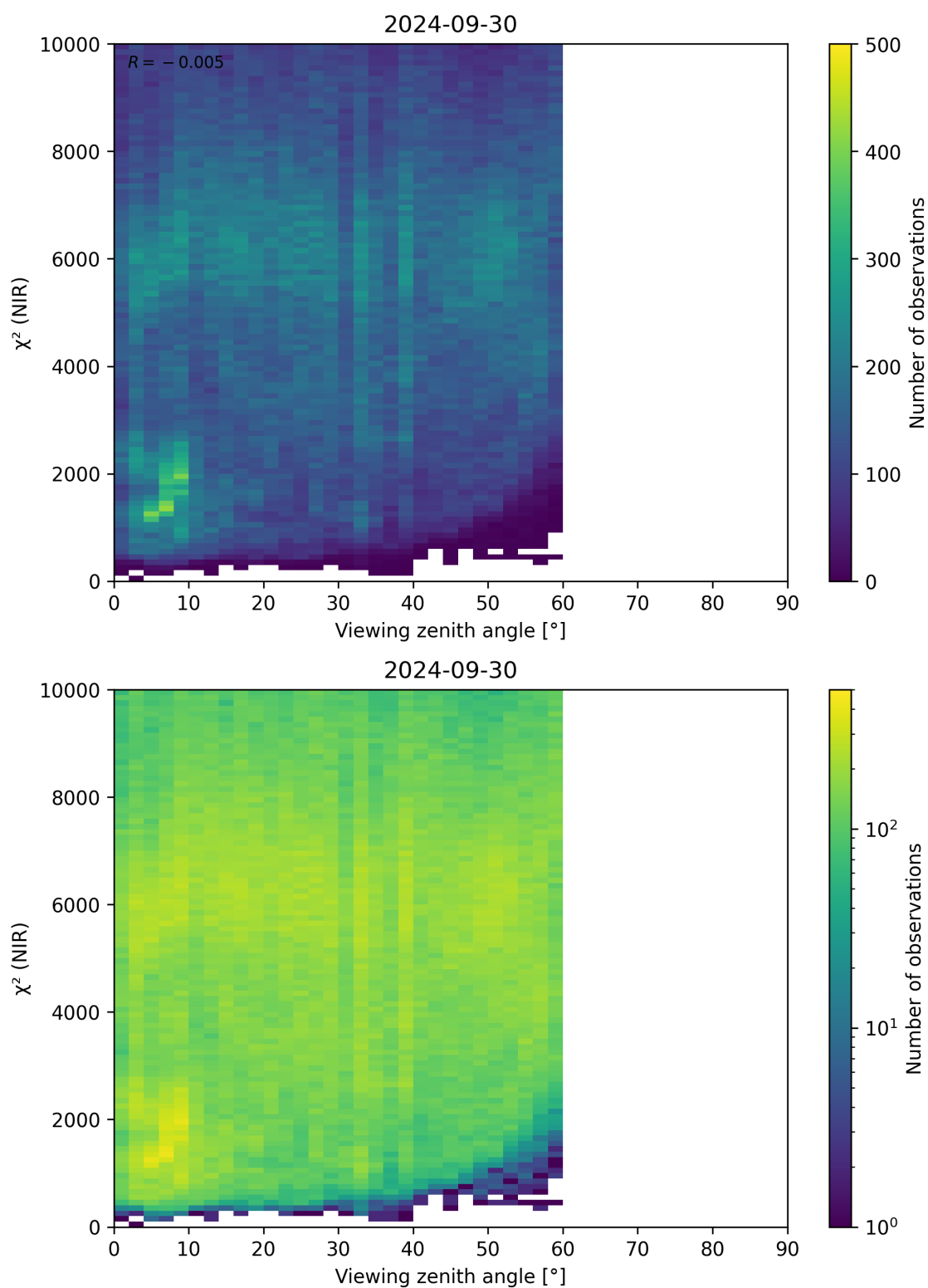
Figure 105: Scatter density plot of “Viewing zenith angle” against “ \chi^2 (NIR)” for 2024-09-29 to 2024-10-01.
