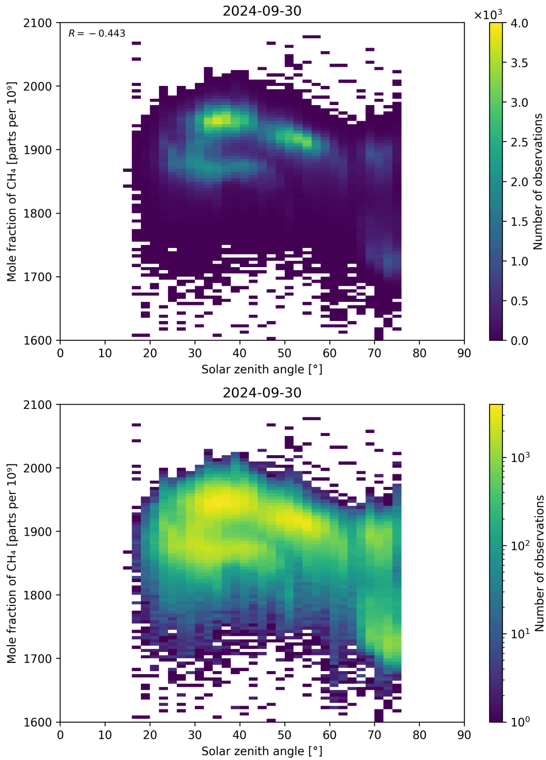
Figure 99: Scatter density plot of “Solar zenith angle” against “Mole fraction of \text{CH}_4 ” for 2024-09-29 to 2024-10-01.
