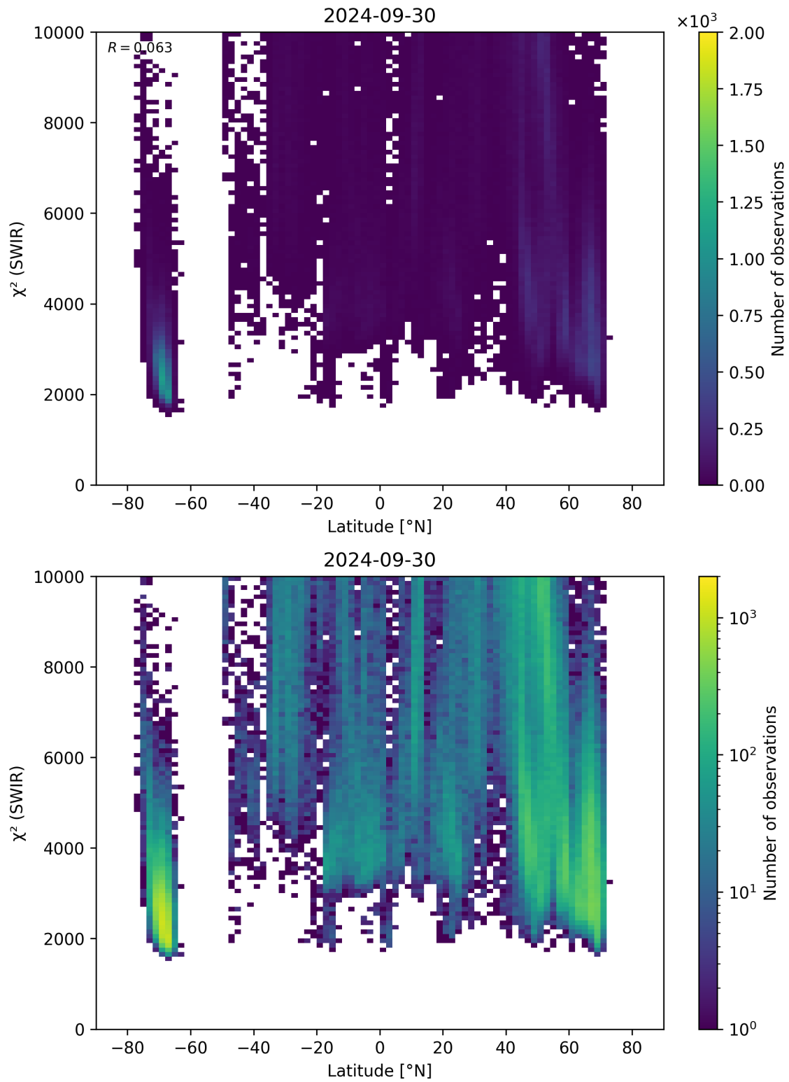
Figure 54: Scatter density plot of “Latitude” against “ \chi^2 (SWIR)” for 2024-09-29 to 2024-10-01.
