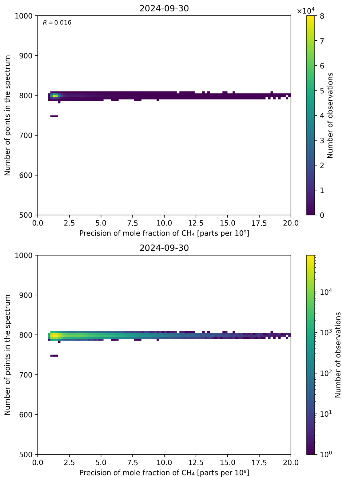
Figure 84: Scatter density plot of “Precision of mole fraction of CH 4 ” against “Number of points in the spectrum” for 2024-09-29 to 2024-10-01.
