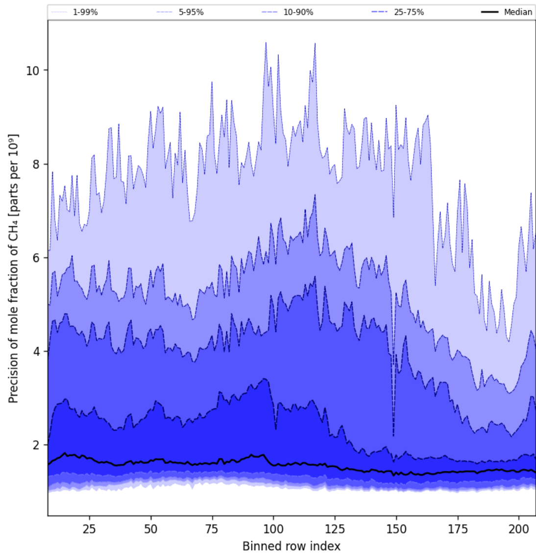
Figure 35: Along track statistics of “Precision of mole fraction of CH 4 ” for 2024-09-29 to 2024-10-01
