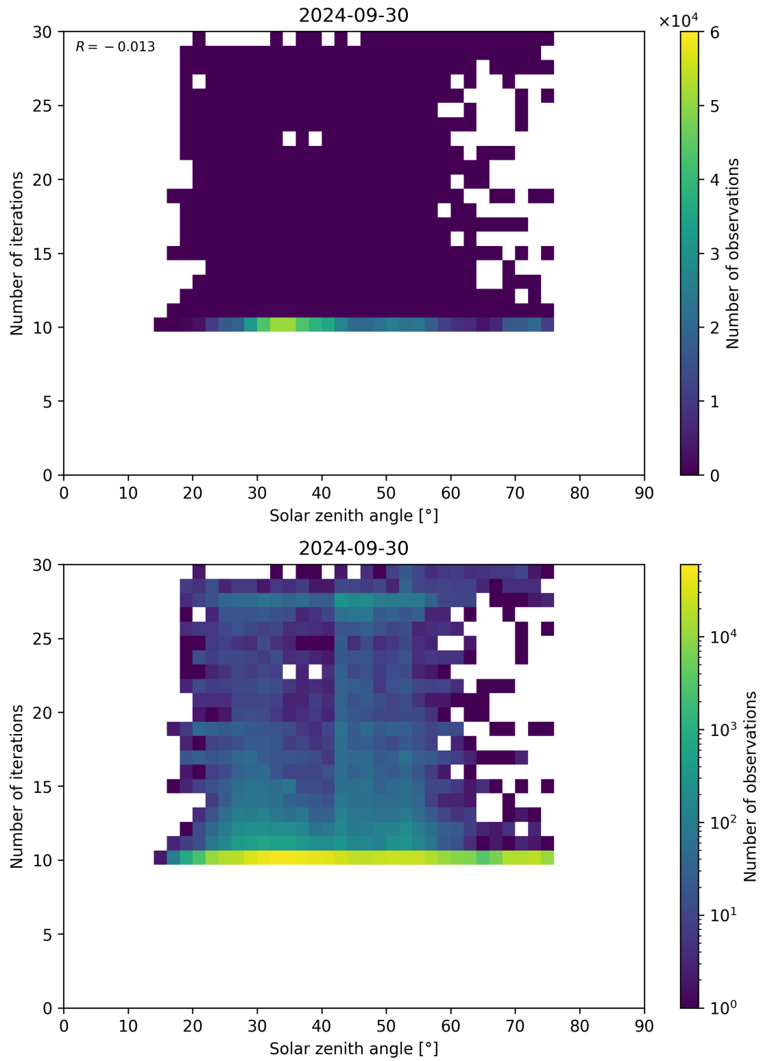
Figure 102: Scatter density plot of “Solar zenith angle” against “Number of iterations” for 2024-09-29 to 2024-10-01.
