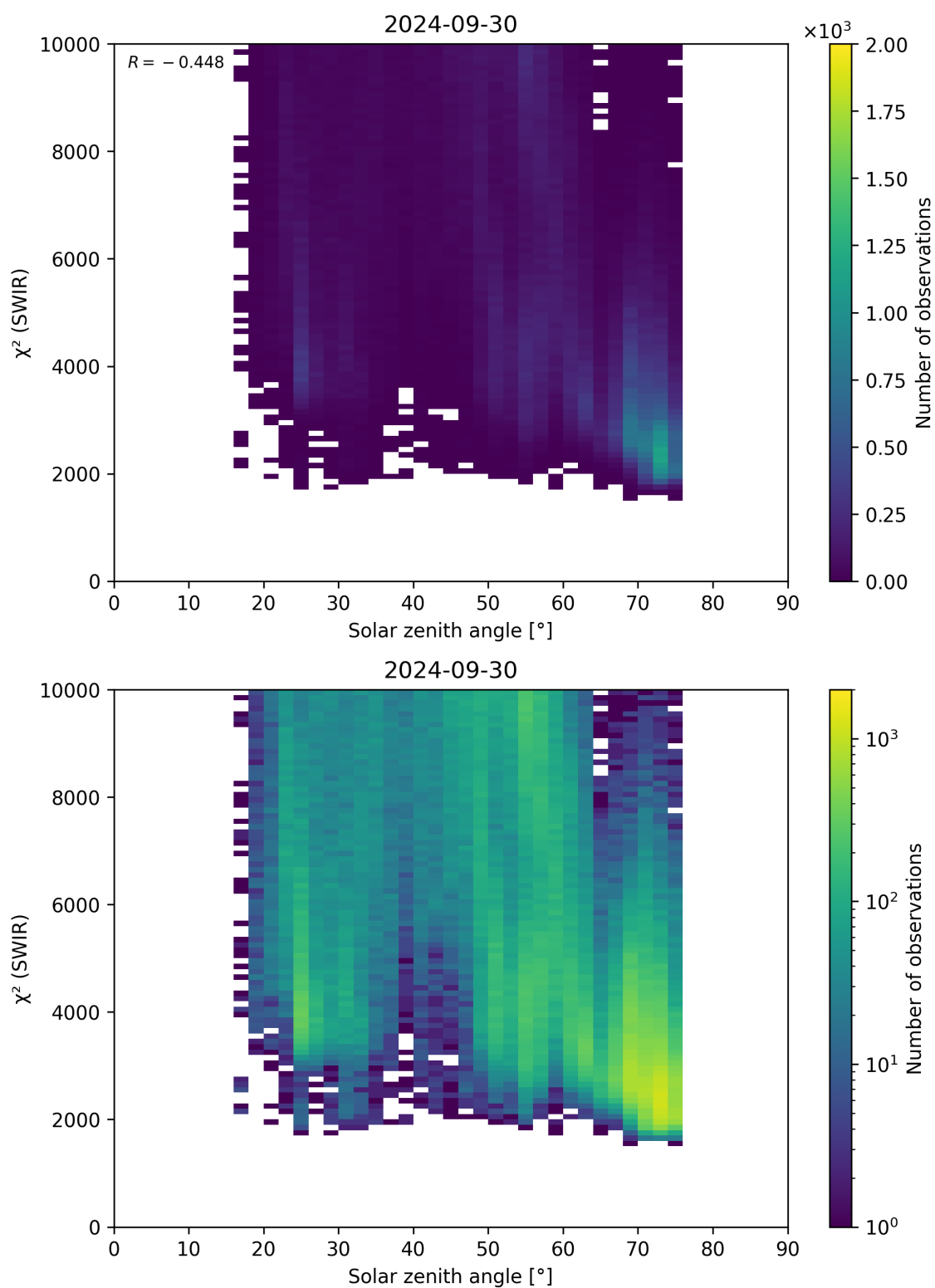
Figure 95: Scatter density plot of “Solar zenith angle” against “ \chi^2 (SWIR)” for 2024-09-29 to 2024-10-01.
