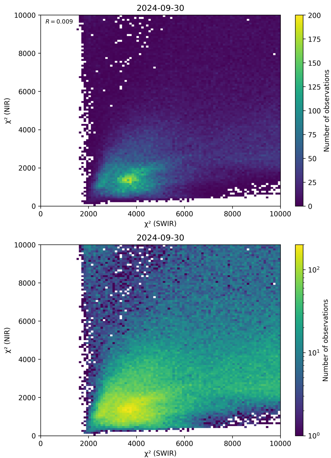
Figure 47: Scatter density plot of “ \chi^2 (SWIR)” against “ \chi^2 (NIR)” for 2024-09-29 to 2024-10-01.
