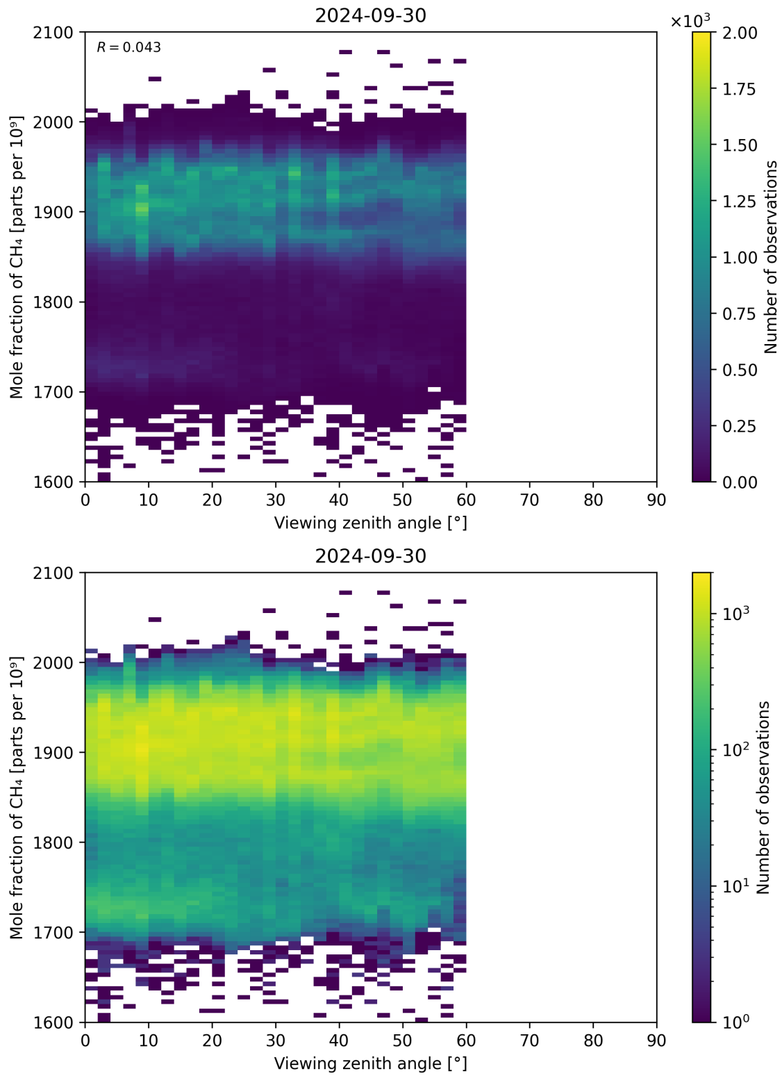
Figure 110: Scatter density plot of “Viewing zenith angle” against “Mole fraction of CH 4 ” for 2024-09-29 to 2024-10-01.
