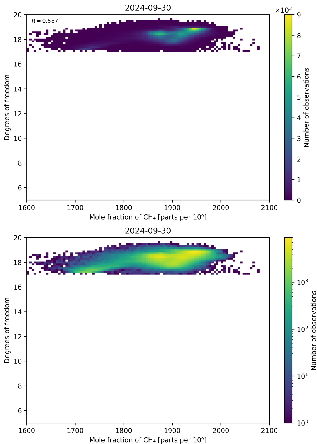
Figure 72: Scatter density plot of “Mole fraction of CH 4 ” against “Degrees of freedom” for 2024-09-29 to 2024-10-01.
