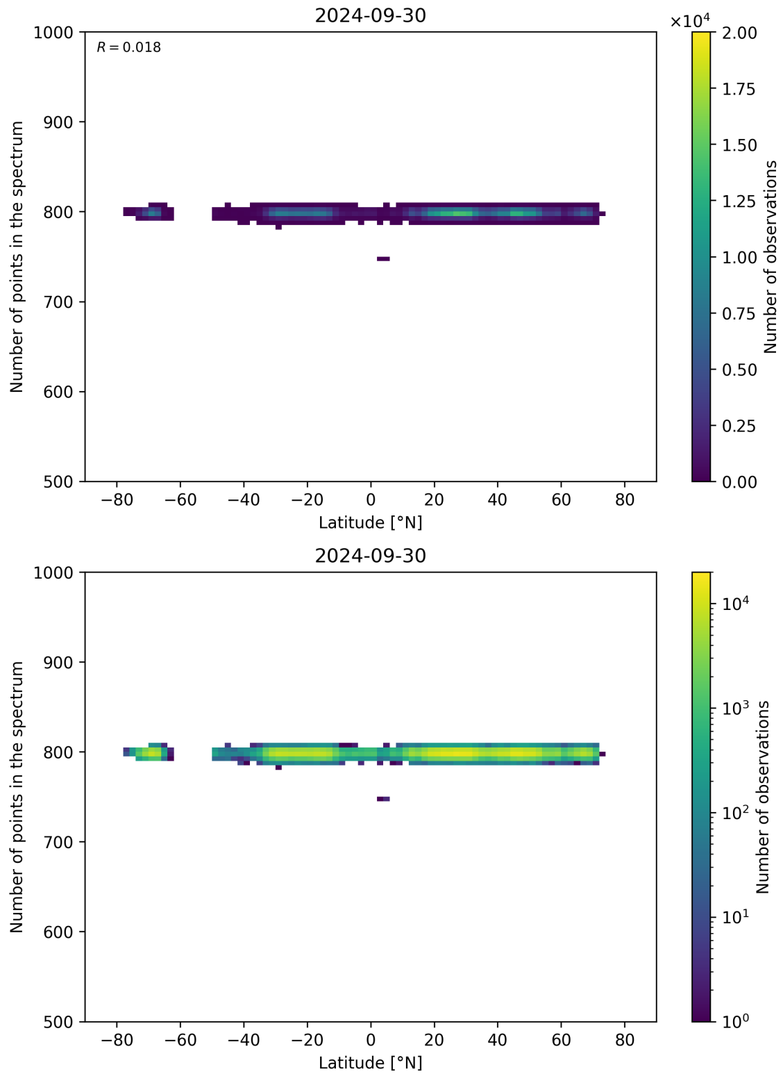
Figure 61: Scatter density plot of “Latitude” against “Number of points in the spectrum” for 2024-09-29 to 2024-10-01.
