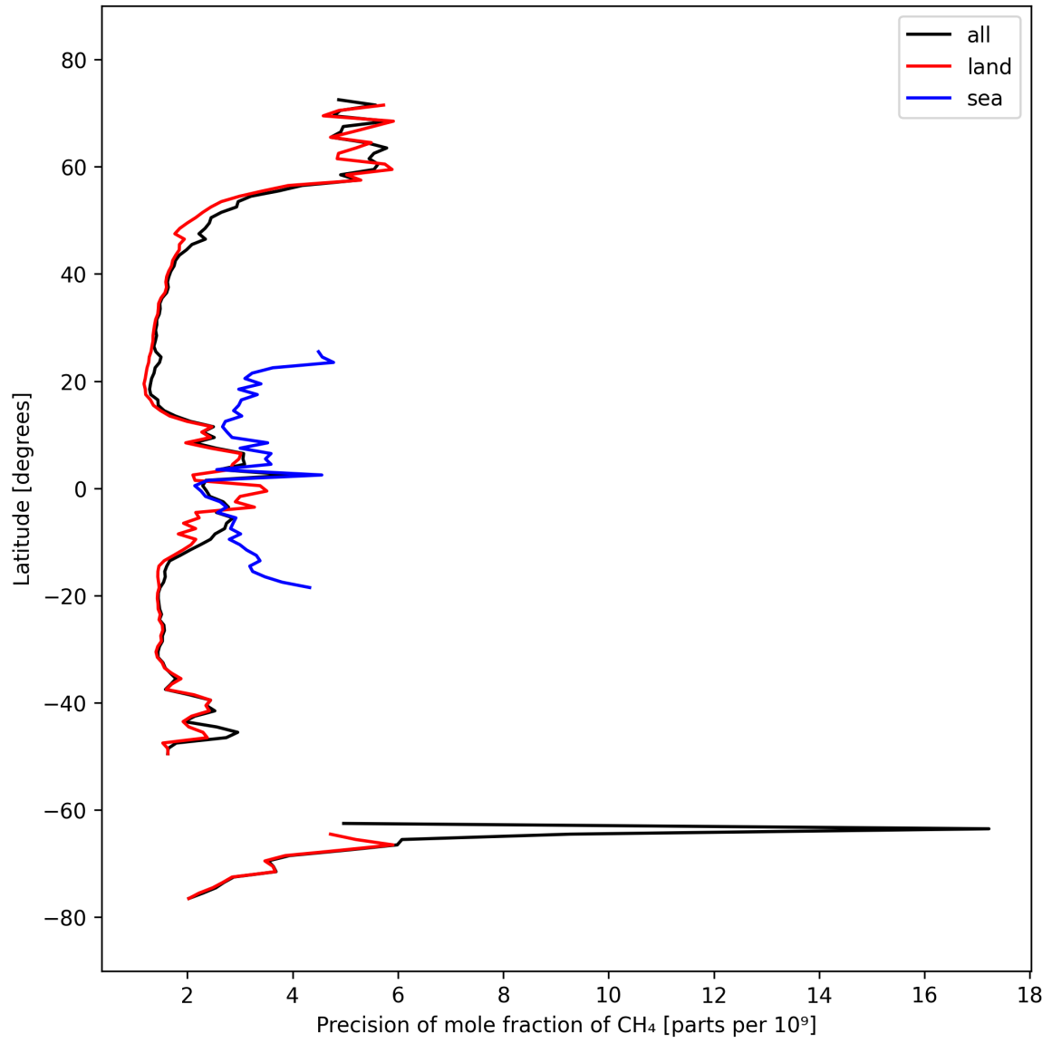
Figure 13: Zonal average of “Precision of mole fraction of CH 4 ” for 2024-09-29 to 2024-10-01.
