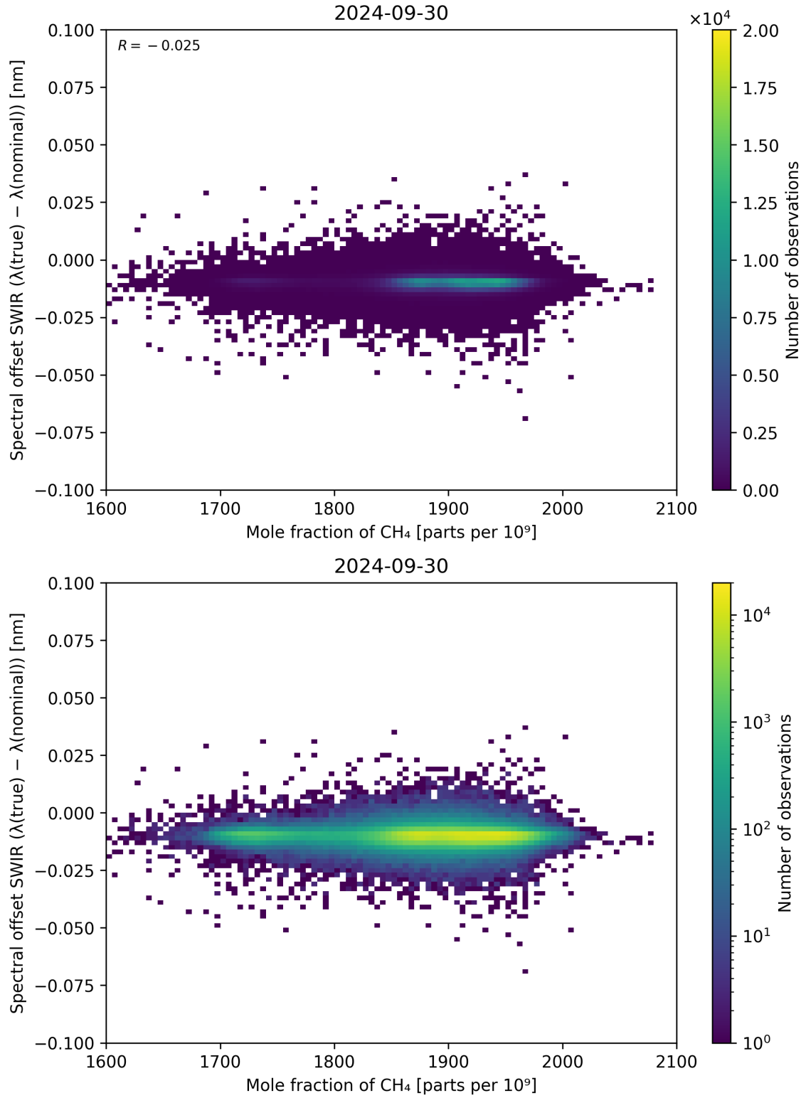
Figure 86: Scatter density plot of “Mole fraction of \text{CH}_4 ” against “Spectral offset SWIR ( \lambda_{\text{true}} - \lambda_{\text{nominal}} )” for 2024-09-29 to 2024-10-01.
