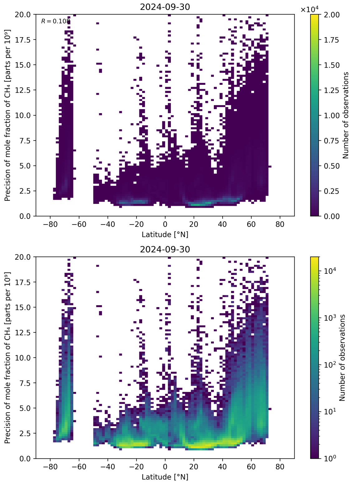
Figure 59: Scatter density plot of “Latitude” against “Precision of mole fraction of \text{CH}_4 ” for 2024-09-29 to 2024-10-01.
