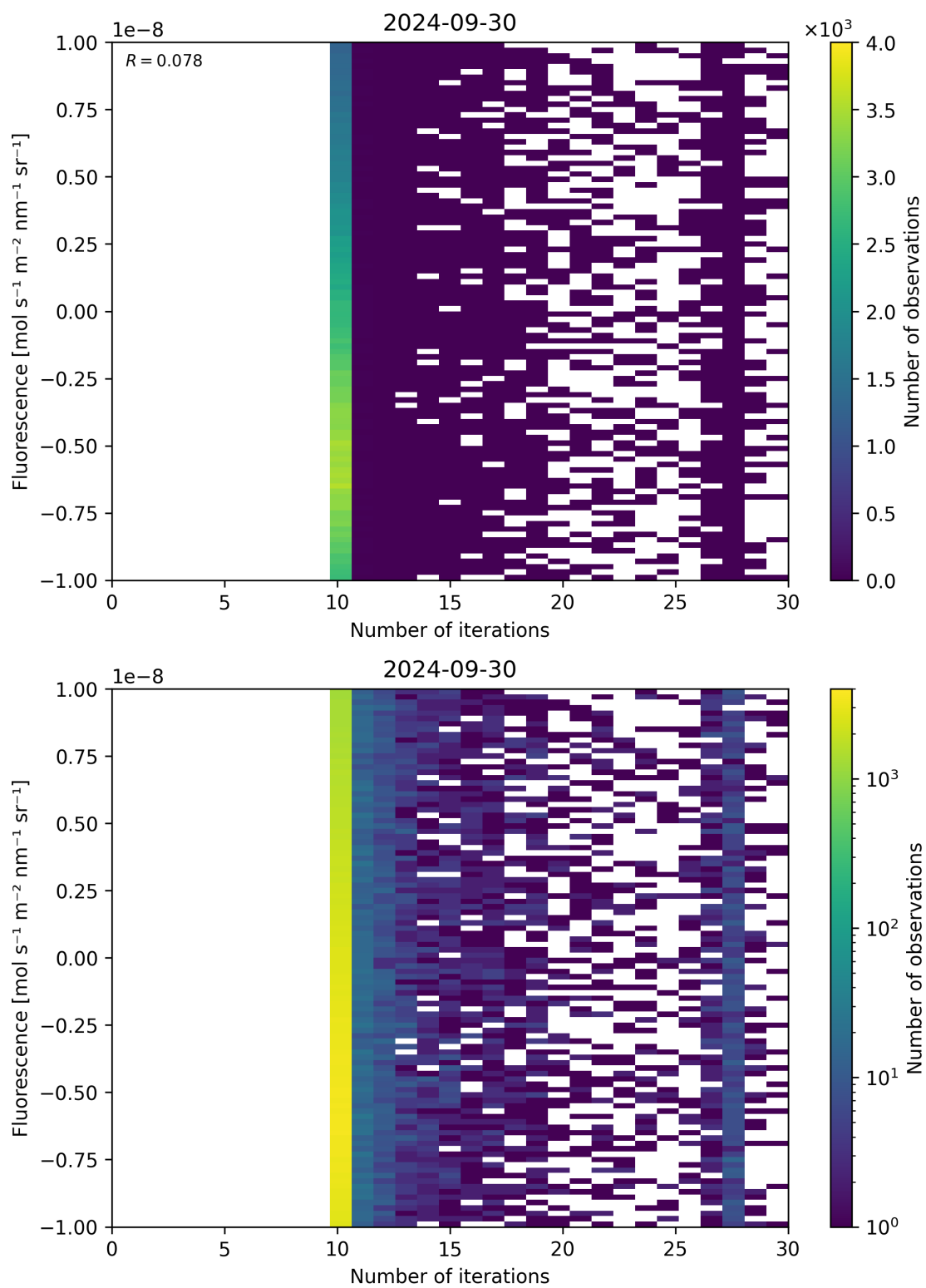
Figure 87: Scatter density plot of “Number of iterations” against “Fluorescence” for 2024-09-29 to 2024-10-01.
