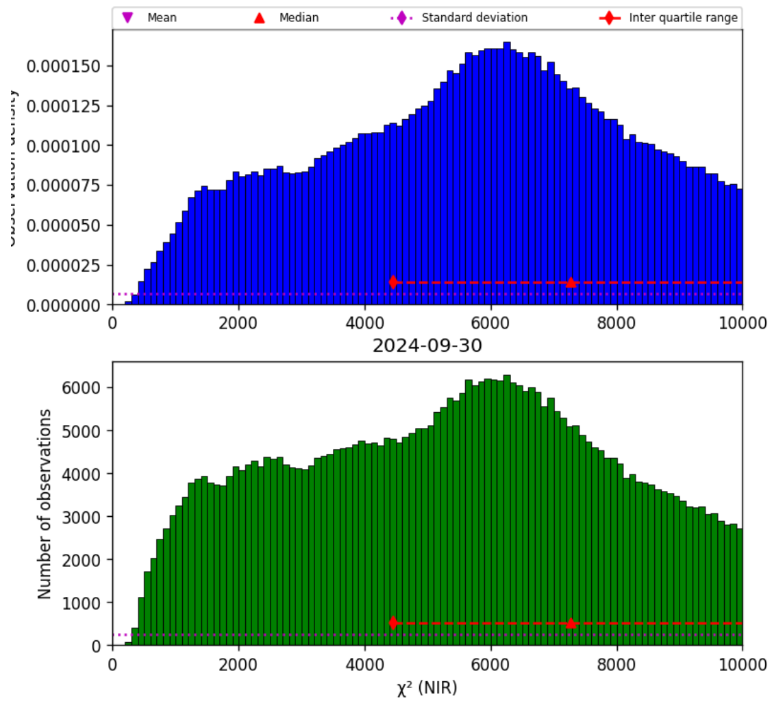
Figure 29: Histogram of “ \chi^2 (NIR)” for 2024-09-29 to 2024-10-01
