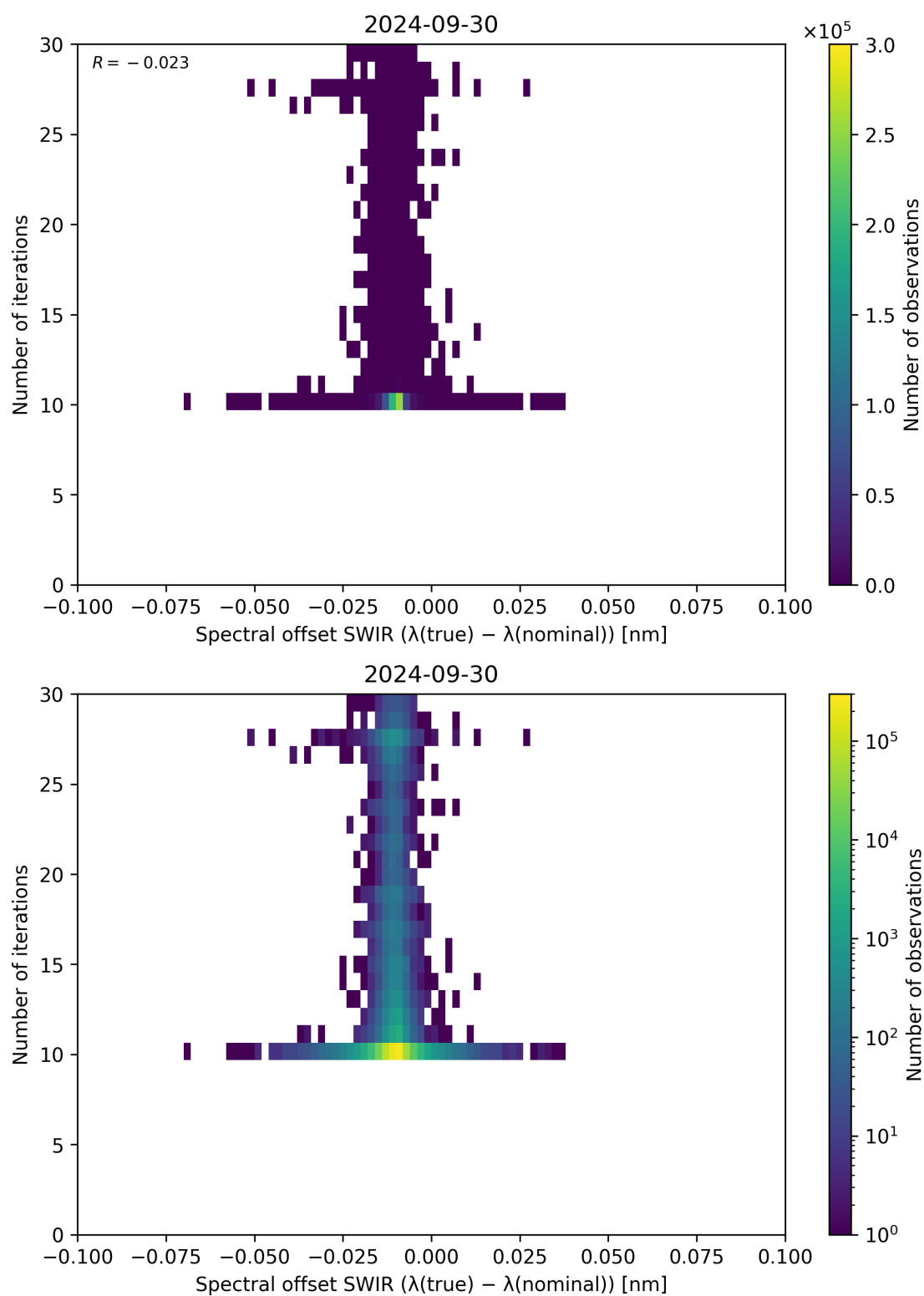
Figure 121: Scatter density plot of “Spectral offset SWIR ( \lambda_{\text{true}} - \lambda_{\text{nominal}} )” against “Number of iterations” for 2024-09-29 to 2024-10-01.
