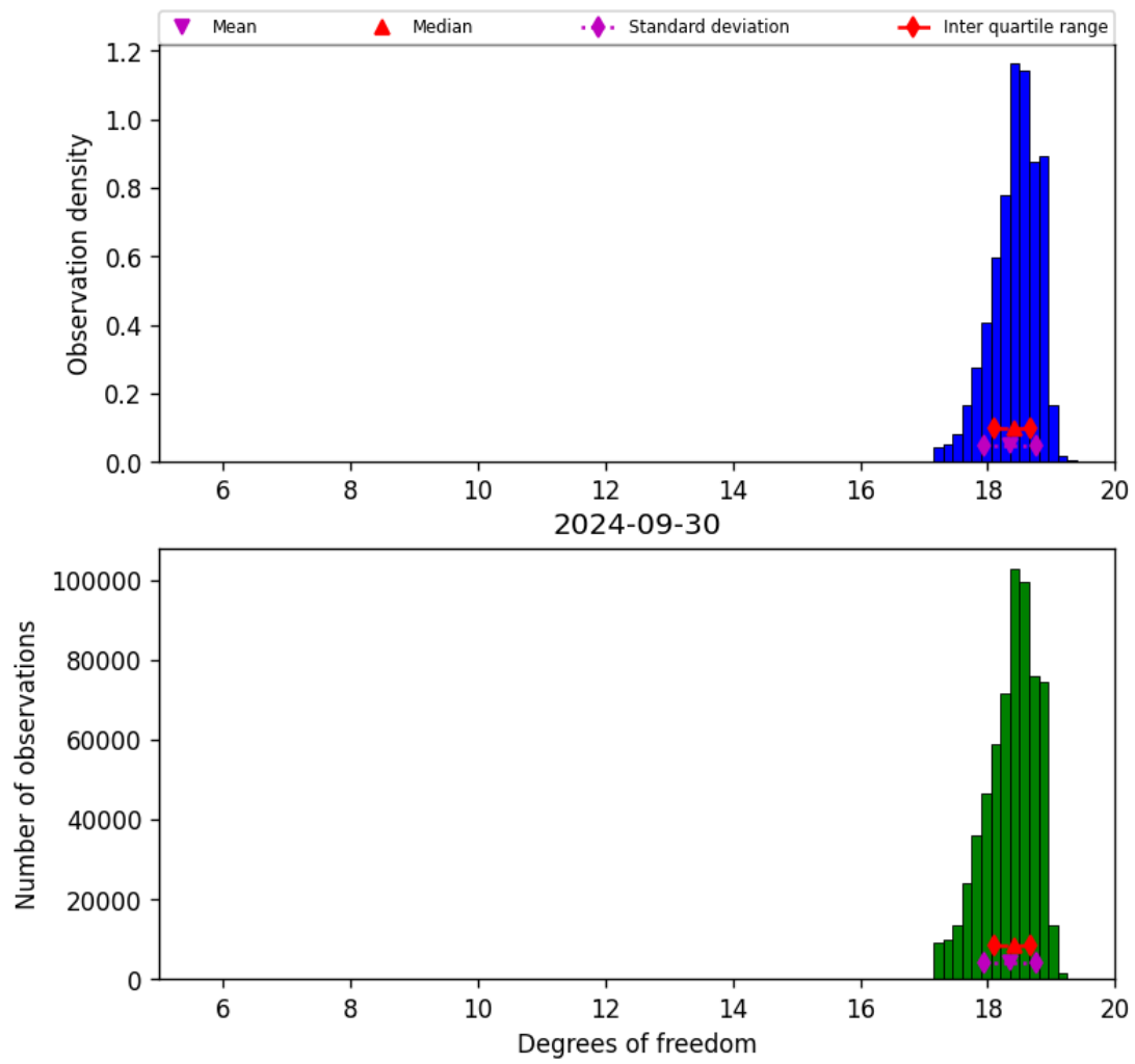
Figure 30: Histogram of “Degrees of freedom” for 2024-09-29 to 2024-10-01
