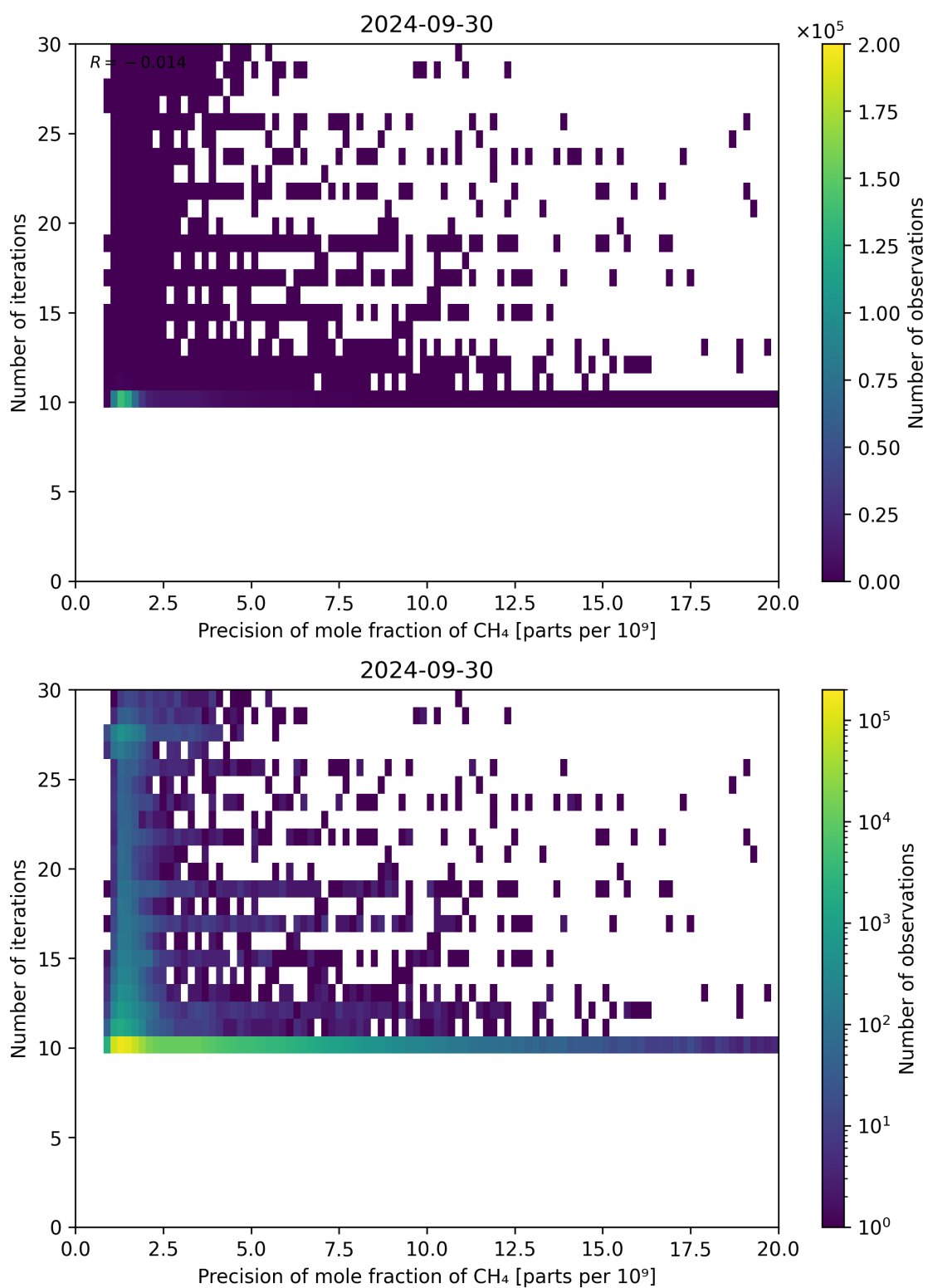
Figure 83: Scatter density plot of “Precision of mole fraction of CH 4 ” against “Number of iterations” for 2024-09-29 to 2024-10-01.
