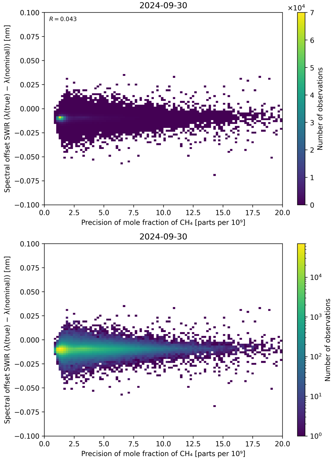
Figure 85: Scatter density plot of “Precision of mole fraction of \text{CH}_4 ” against “Spectral offset SWIR ( \lambda_{\text{true}} - \lambda_{\text{nominal}} )” for 2024-09-29 to 2024-10-01.
