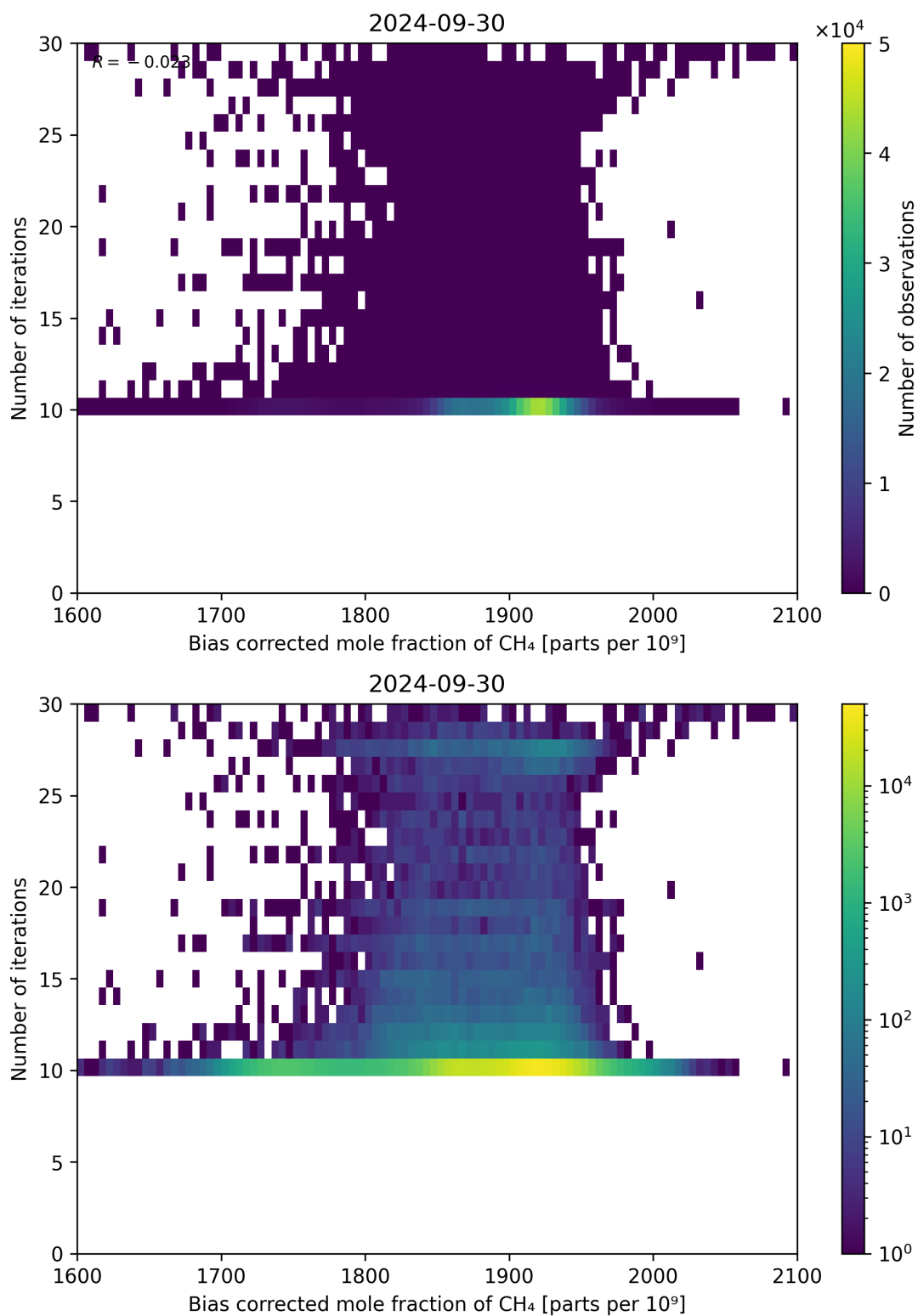
Figure 67: Scatter density plot of “Bias corrected mole fraction of CH 4 ” against “Number of iterations” for 2024-09-29 to 2024-10-01.
