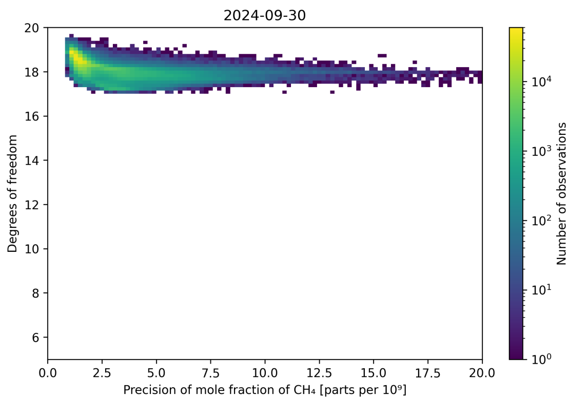
Figure 80: Scatter density plot of “Precision of mole fraction of CH 4 ” against “Degrees of freedom” for 2024-09-29 to 2024-10-01.
