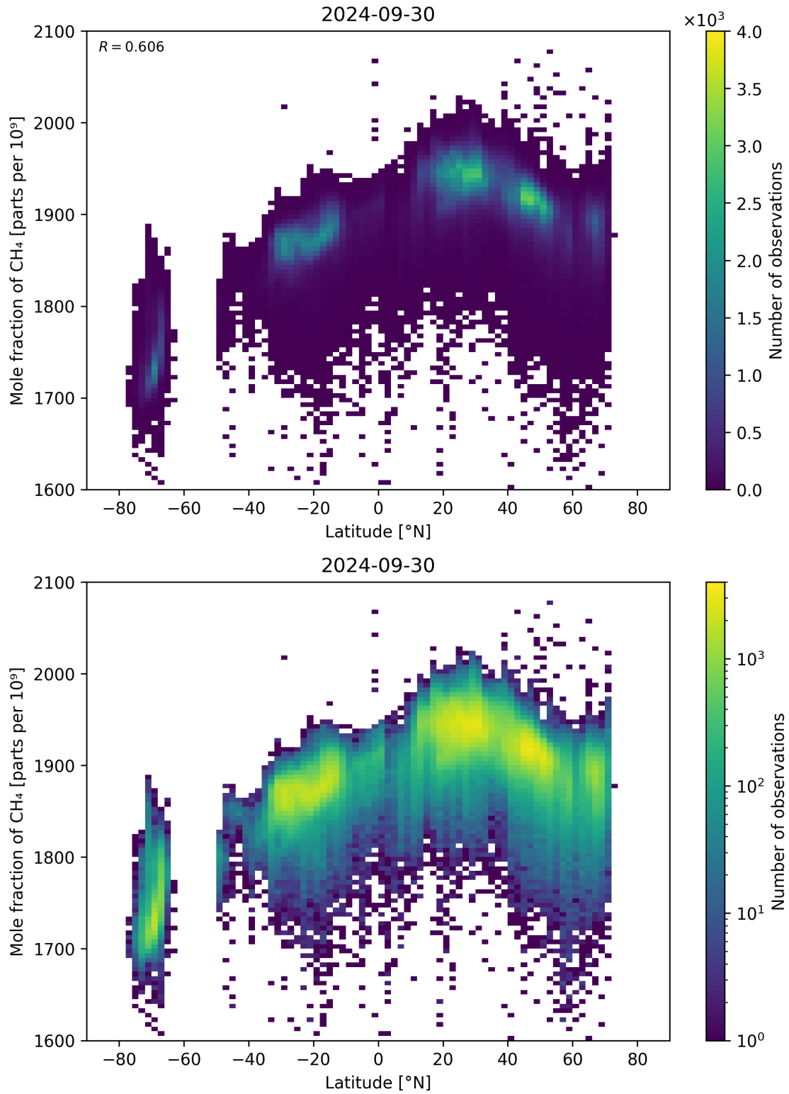
Figure 57: Scatter density plot of “Latitude” against “Mole fraction of CH 4 ” for 2024-09-29 to 2024-10-01.
