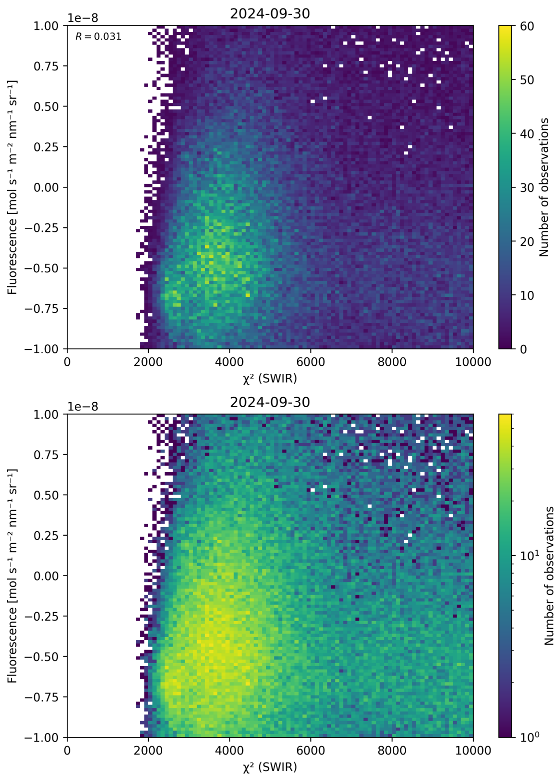
Figure 49: Scatter density plot of “ \chi^2 (SWIR)” against “Fluorescence” for 2024-09-29 to 2024-10-01.
