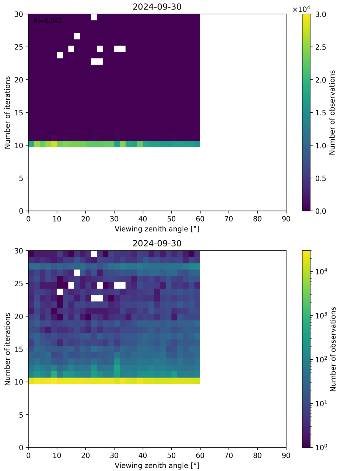
Figure 113: Scatter density plot of “Viewing zenith angle” against “Number of iterations” for 2024-09-29 to 2024-10-01.
