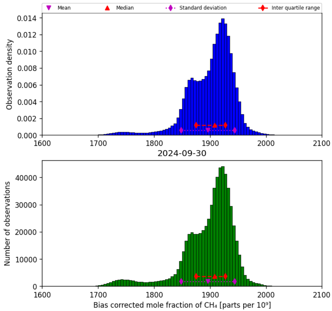
Figure 25: Histogram of “Bias corrected mole fraction of CH 4 ” for 2024-09-29 to 2024-10-01
