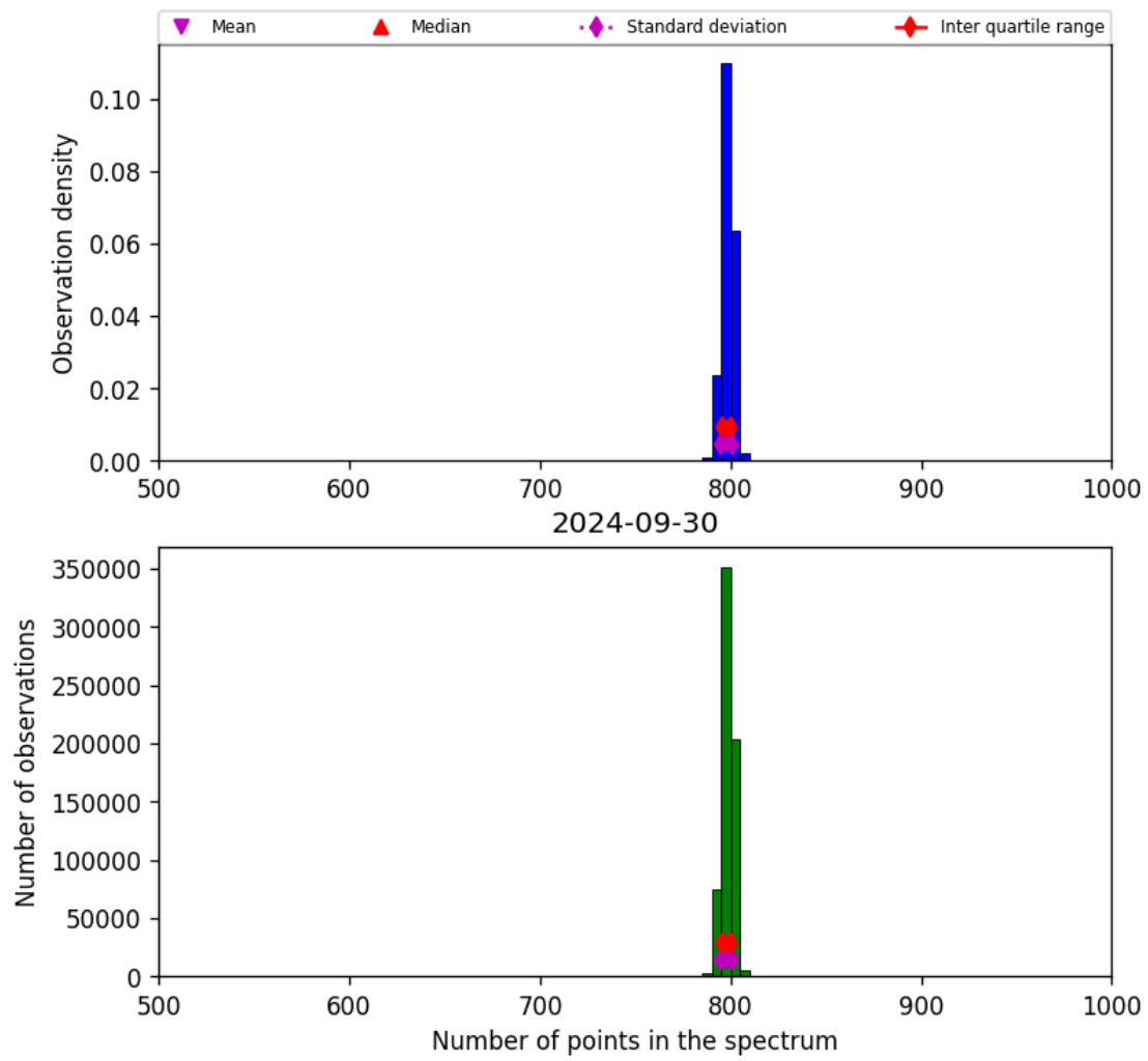
Figure 26: Histogram of “Number of points in the spectrum” for 2024-09-29 to 2024-10-01
