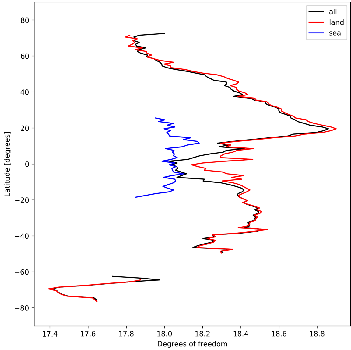
Figure 19: Zonal average of “Degrees of freedom” for 2024-09-29 to 2024-10-01.
