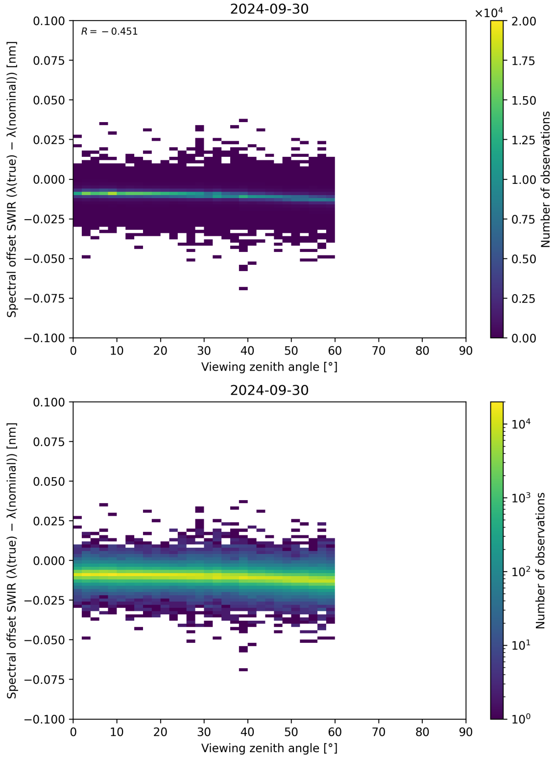
Figure 116: Scatter density plot of “Viewing zenith angle” against “Spectral offset SWIR ( \lambda_{\text{true}} - \lambda_{\text{nominal}} )” for 2024-09-29 to 2024-10-01.
