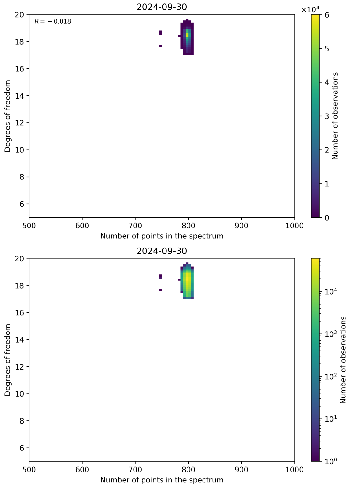
Figure 90: Scatter density plot of “Number of points in the spectrum” against “Degrees of freedom” for 2024-09-29 to 2024-10-01.
