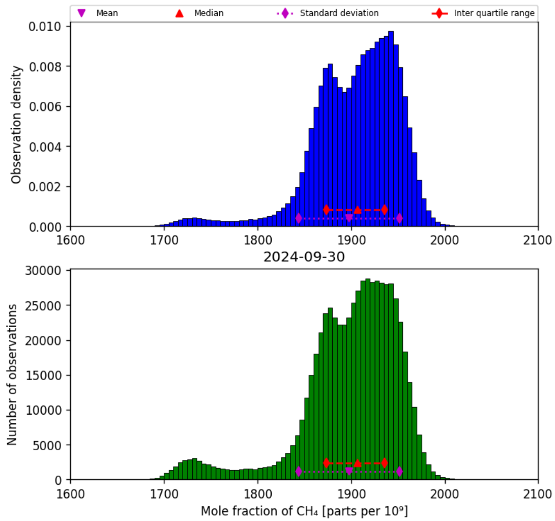
Figure 23: Histogram of “Mole fraction of CH 4 ” for 2024-09-29 to 2024-10-01
