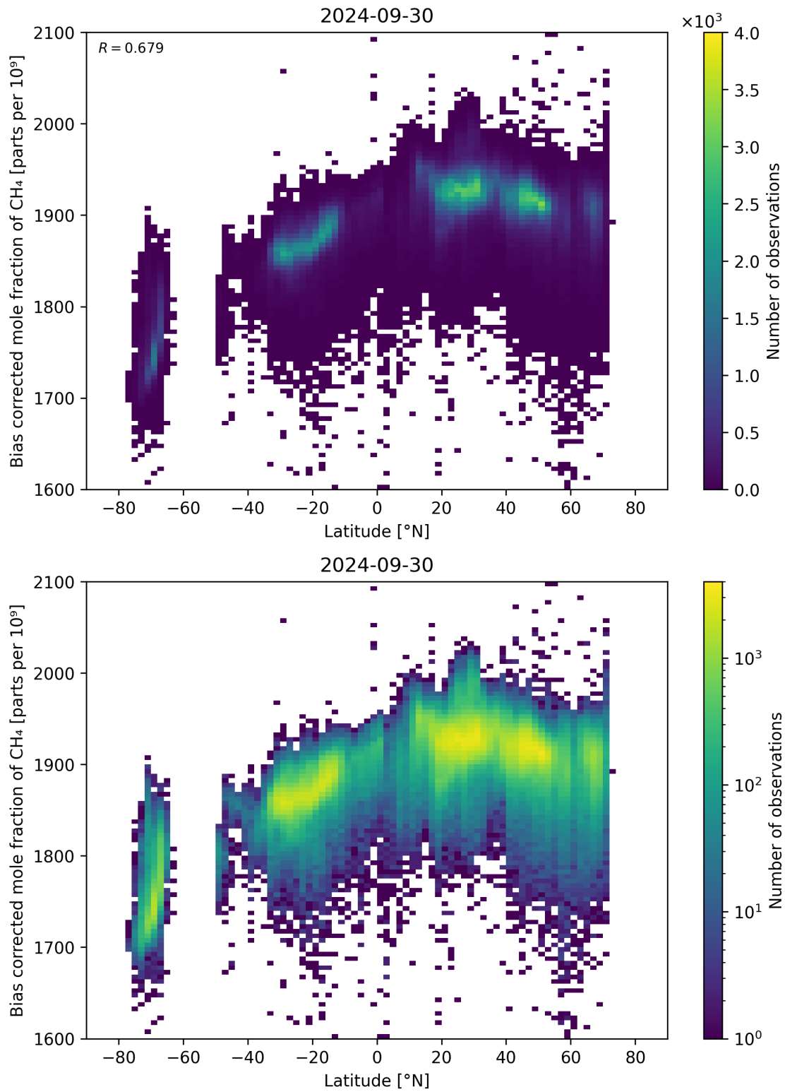
Figure 58: Scatter density plot of “Latitude” against “Bias corrected mole fraction of CH 4 ” for 2024-09-29 to 2024-10-01.
