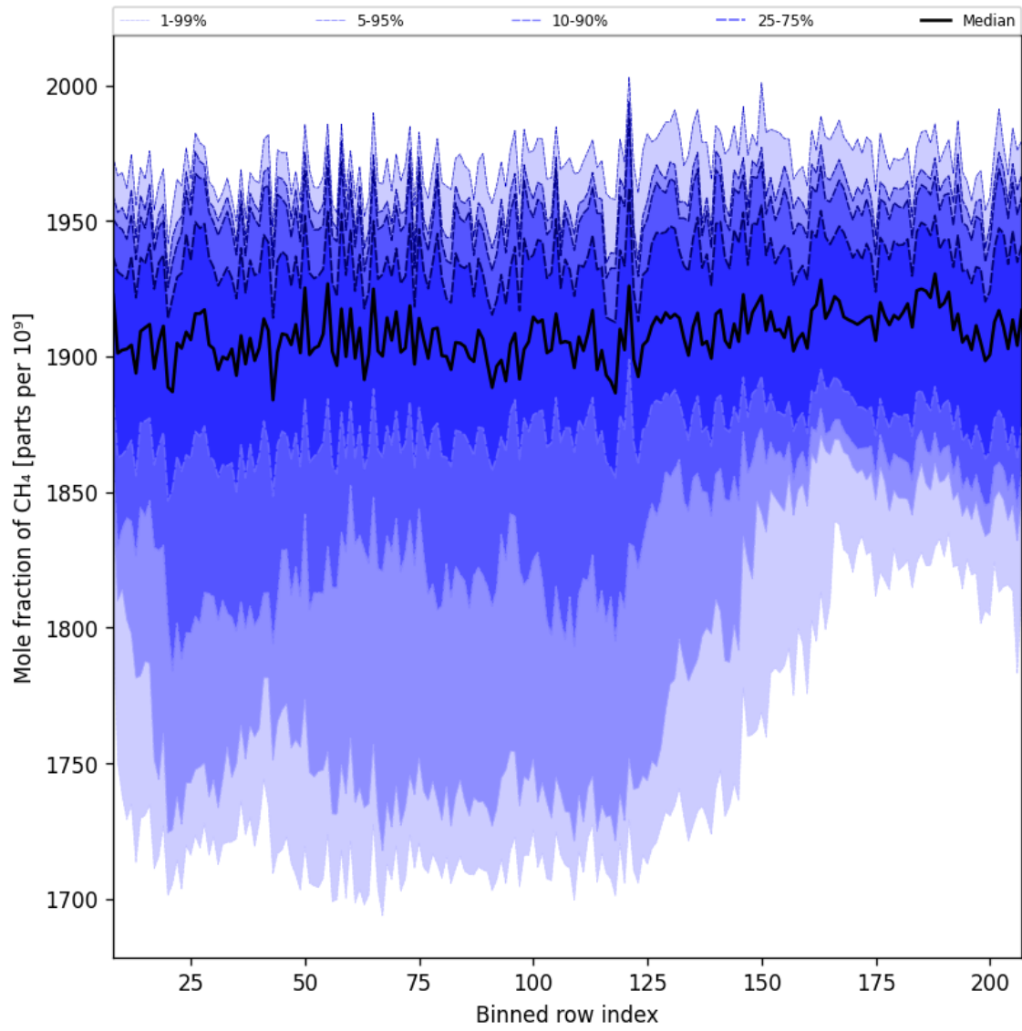
Figure 34: Along track statistics of “Mole fraction of CH 4 ” for 2024-09-29 to 2024-10-01
