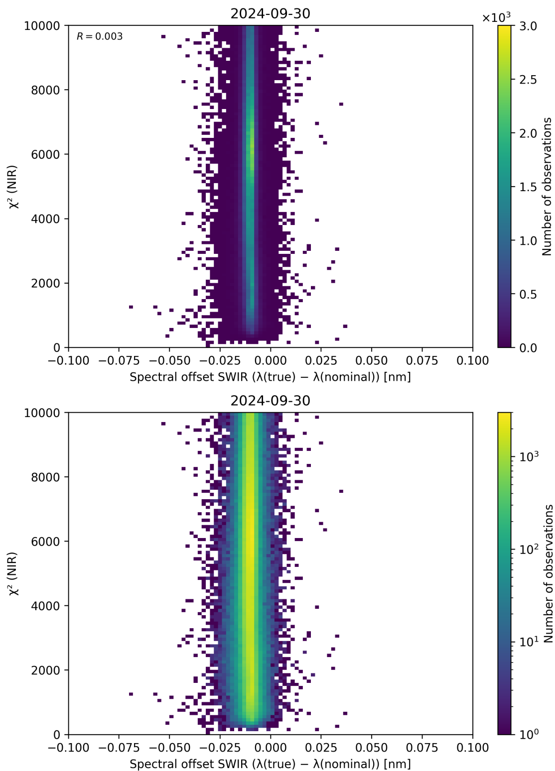
Figure 117: Scatter density plot of “Spectral offset SWIR ( \lambda_{\text{true}} - \lambda_{\text{nominal}} )” against “ \chi^2 (NIR)” for 2024-09-29 to 2024-10-01.
