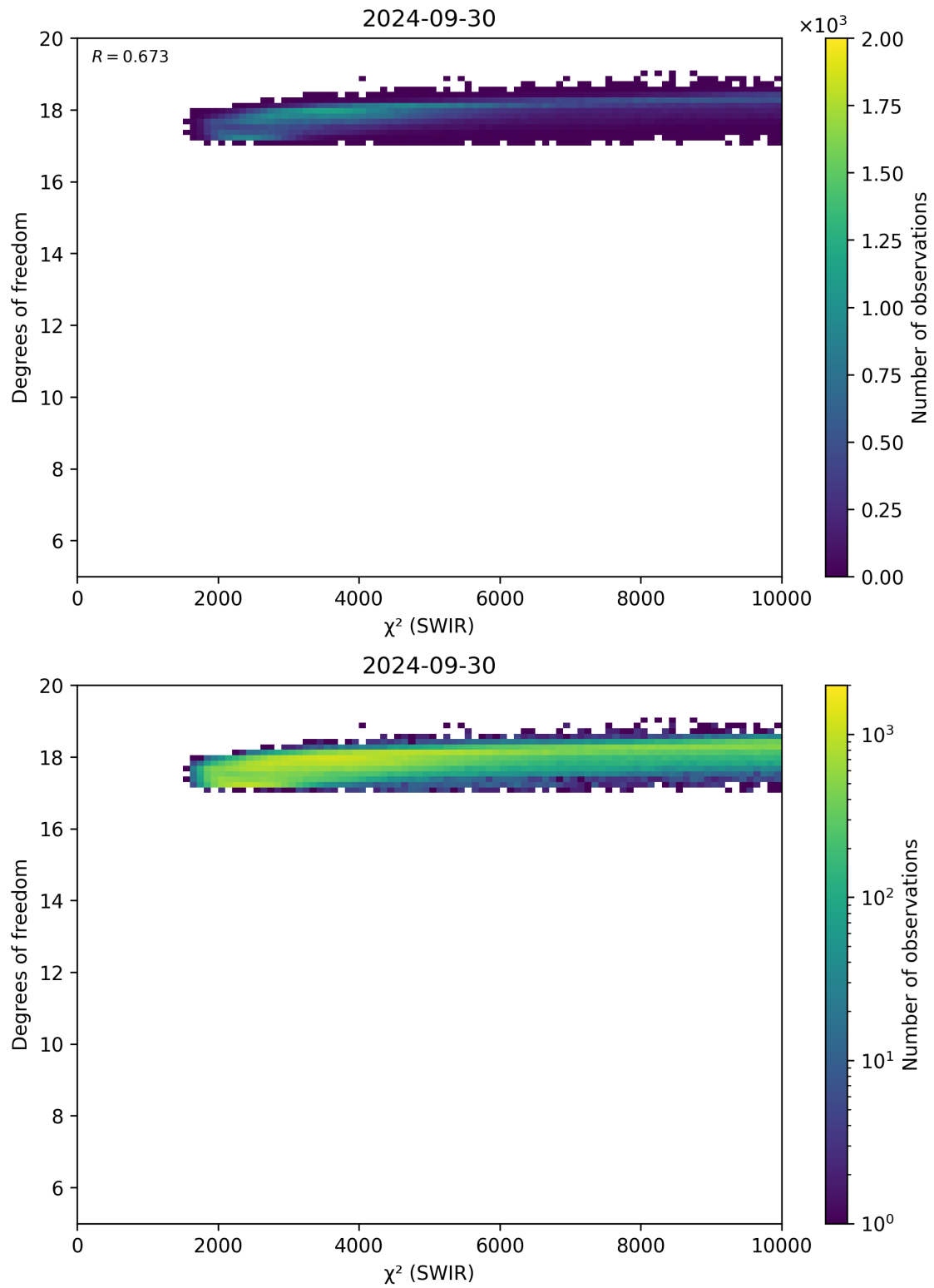
Figure 48: Scatter density plot of “ \chi^2 (SWIR)” against “Degrees of freedom” for 2024-09-29 to 2024-10-01.
