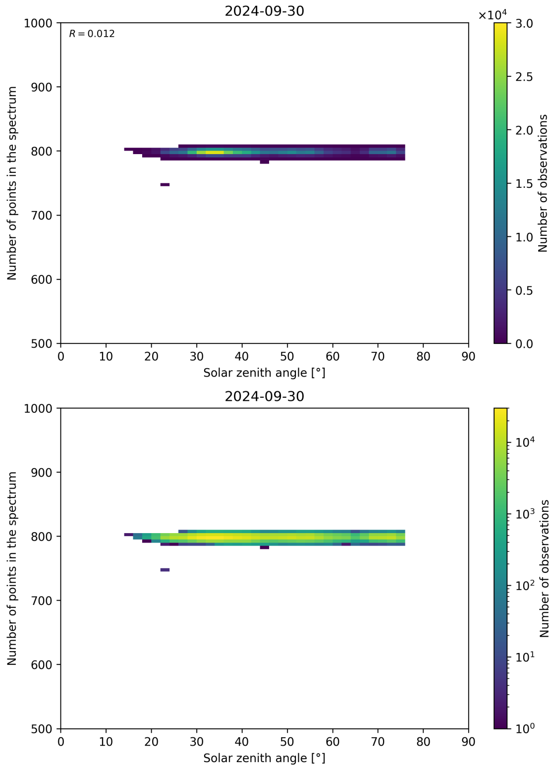
Figure 103: Scatter density plot of “Solar zenith angle” against “Number of points in the spectrum” for 2024-09-29 to 2024-10-01.
