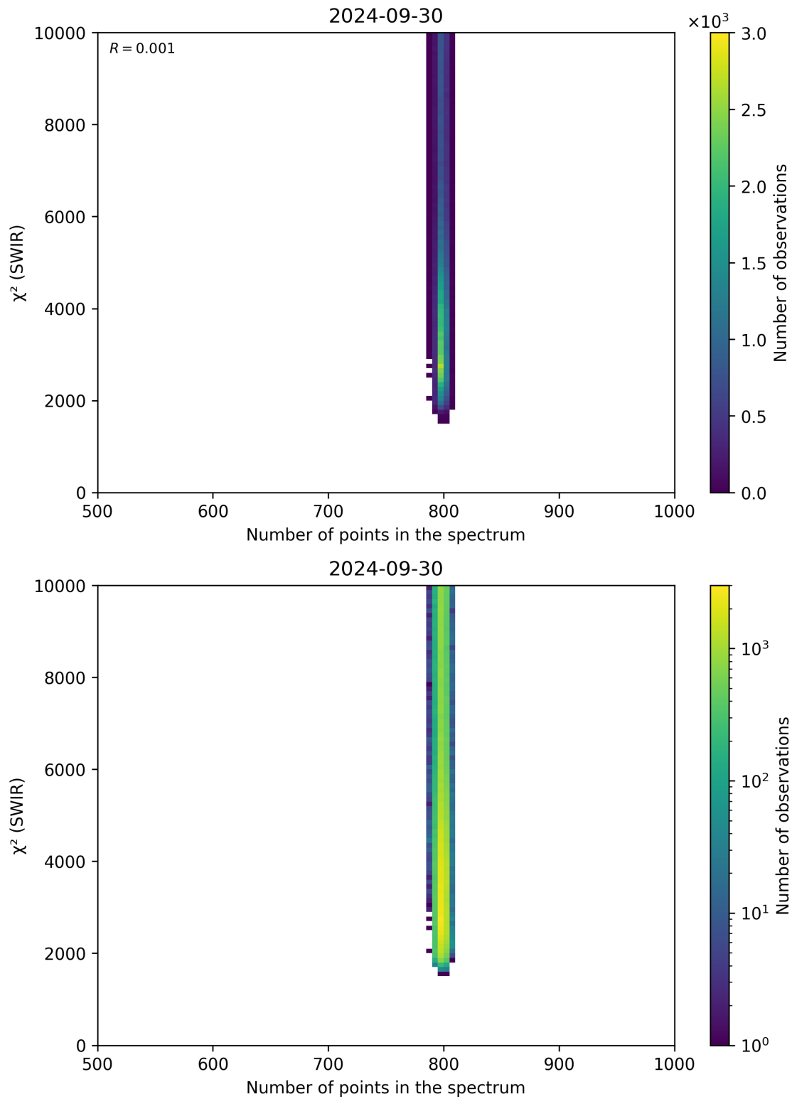
Figure 89: Scatter density plot of “Number of points in the spectrum” against “ \chi^2 (SWIR)” for 2024-09-29 to 2024-10-01.
