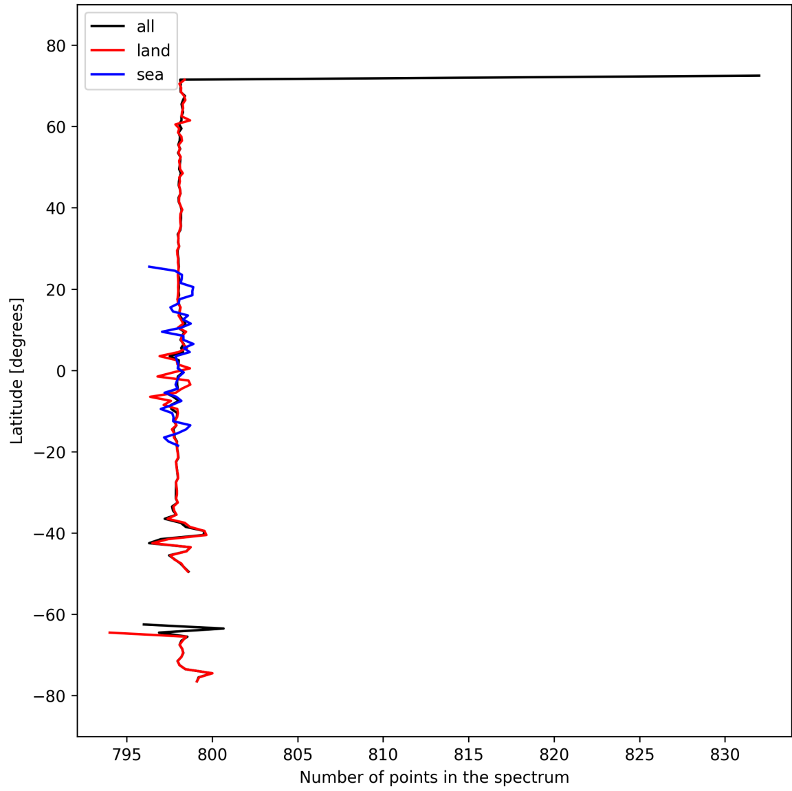
Figure 15: Zonal average of “Number of points in the spectrum” for 2024-09-29 to 2024-10-01.
