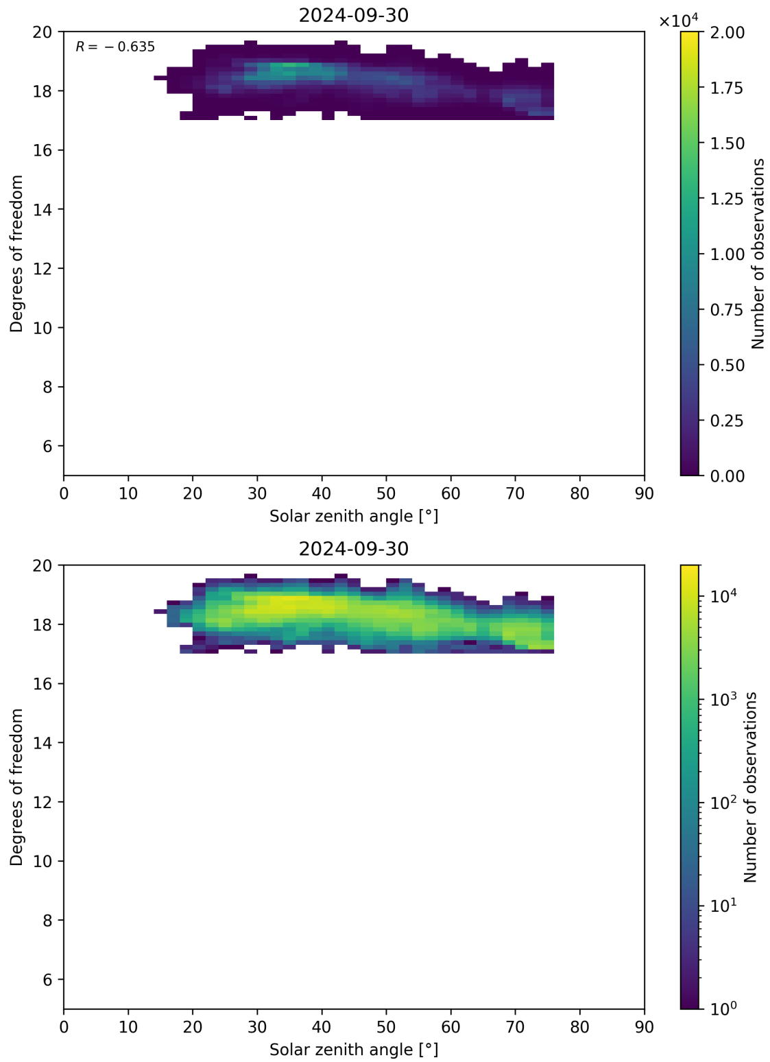
Figure 96: Scatter density plot of “Solar zenith angle” against “Degrees of freedom” for 2024-09-29 to 2024-10-01.
