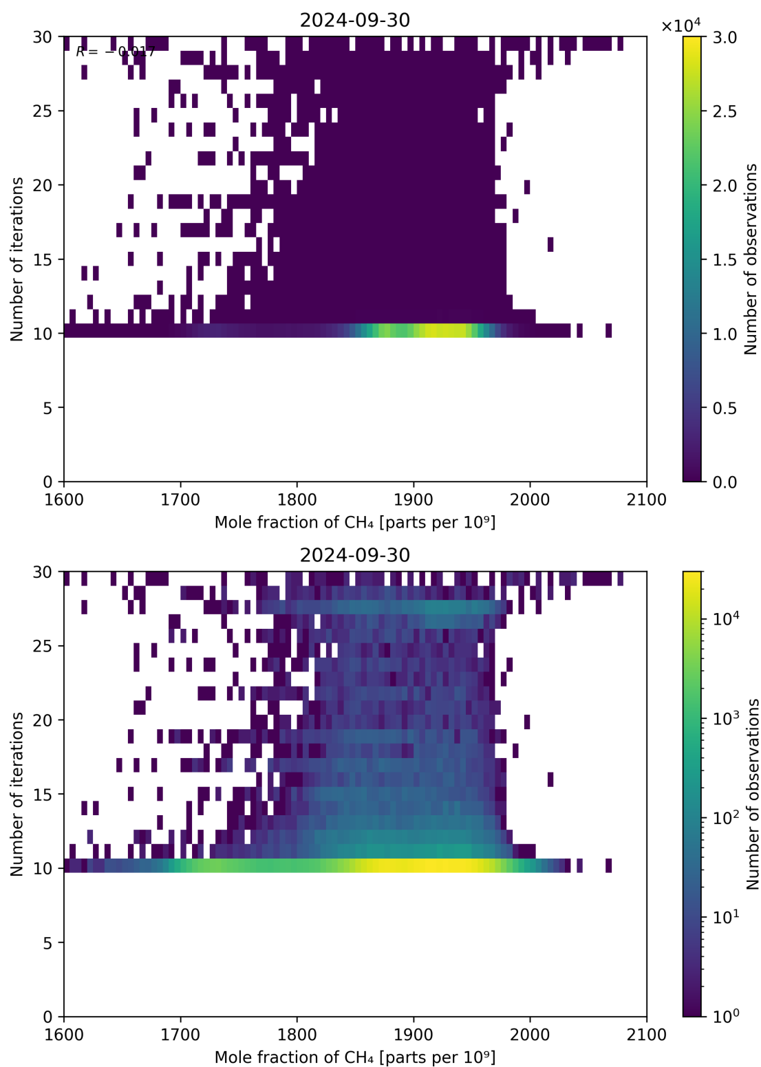
Figure 76: Scatter density plot of “Mole fraction of CH 4 ” against “Number of iterations” for 2024-09-29 to 2024-10-01.
