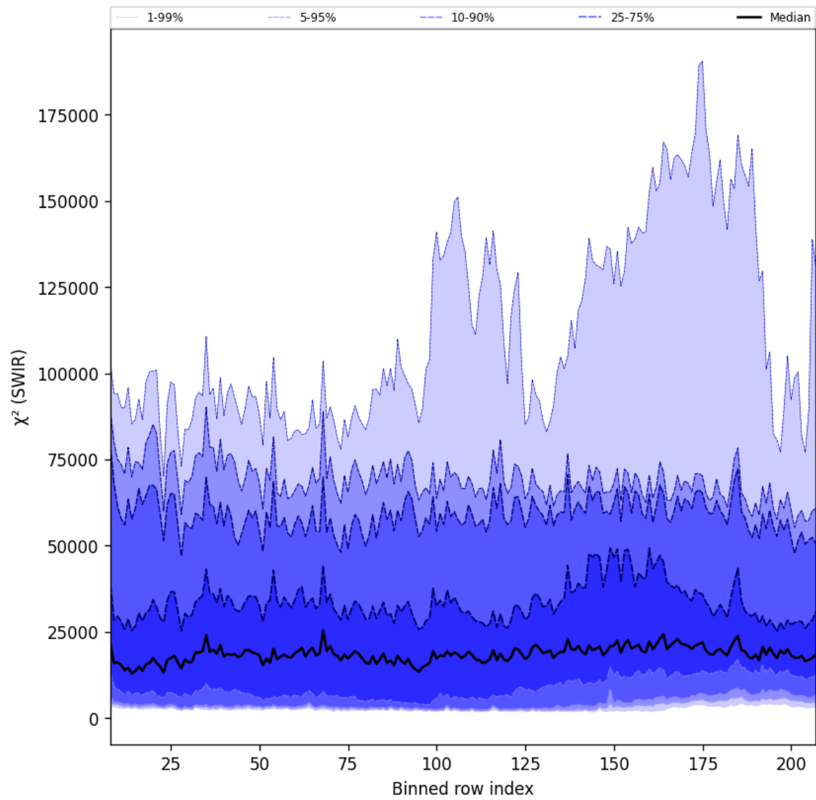
Figure 39: Along track statistics of “ \chi^2 (SWIR)” for 2024-09-29 to 2024-10-01
