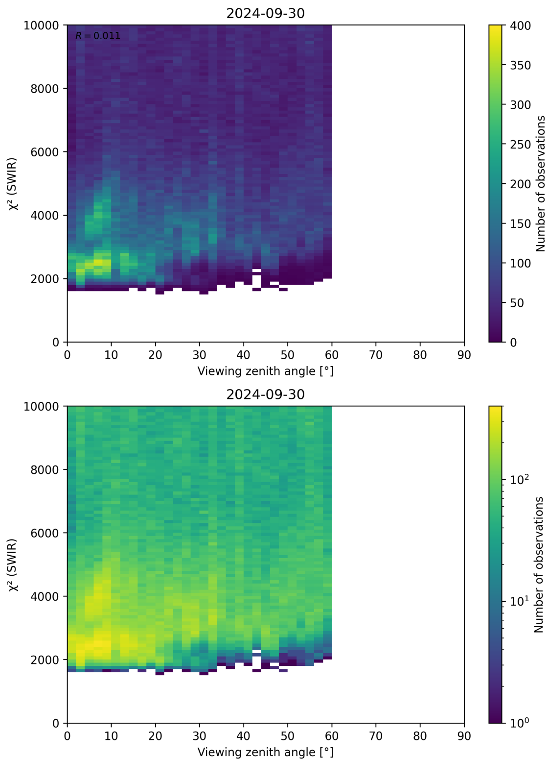
Figure 106: Scatter density plot of “Viewing zenith angle” against “ \chi^2 (SWIR)” for 2024-09-29 to 2024-10-01.
