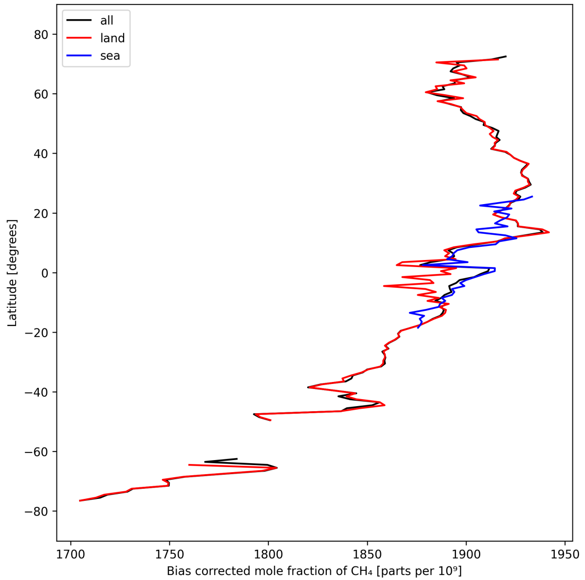
Figure 14: Zonal average of “Bias corrected mole fraction of CH 4 ” for 2024-09-29 to 2024-10-01.
