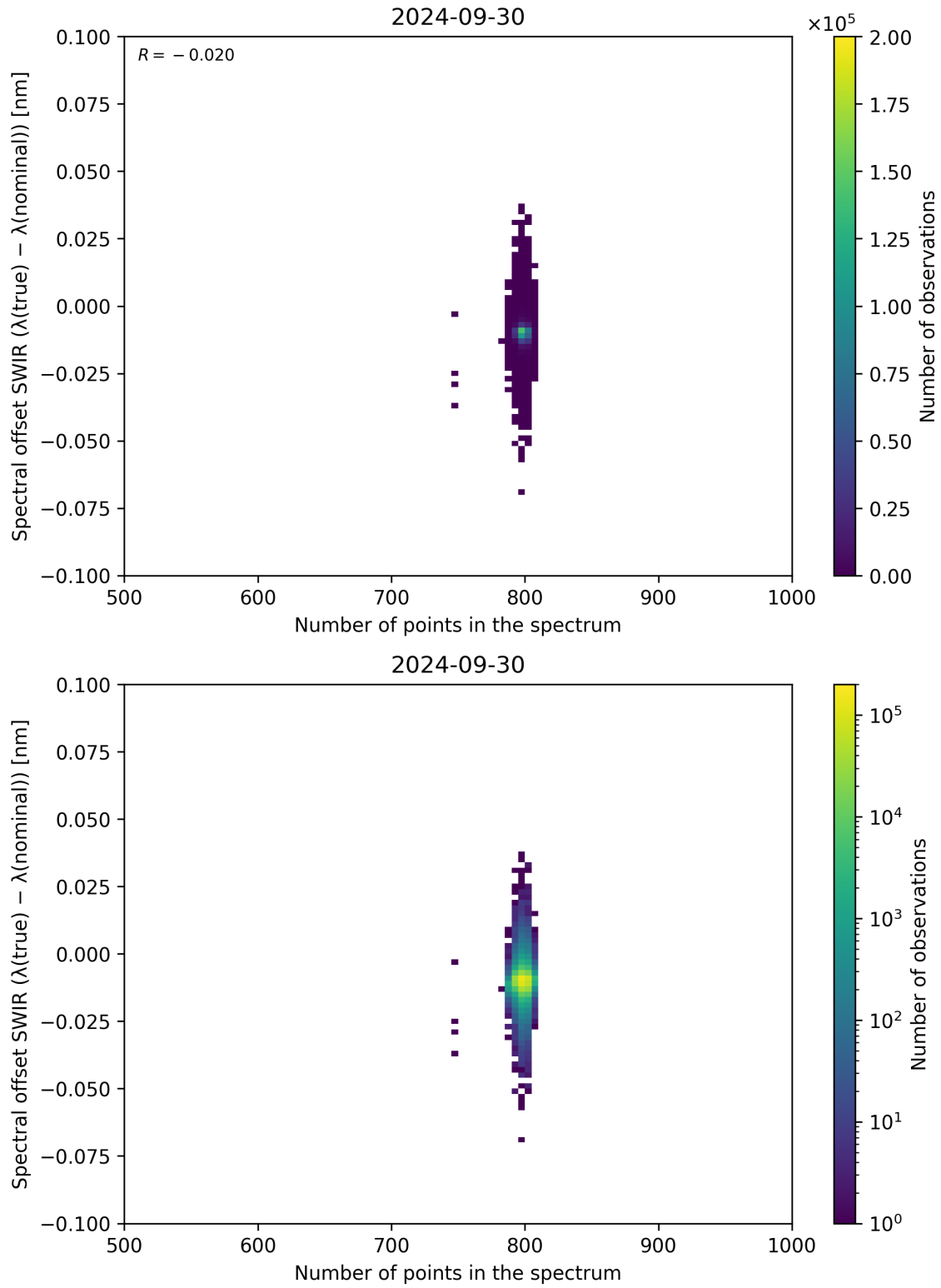
Figure 93: Scatter density plot of “Number of points in the spectrum” against “Spectral offset SWIR ( \lambda_{\text{true}} - \lambda_{\text{nominal}} )” for 2024-09-29 to 2024-10-01.
