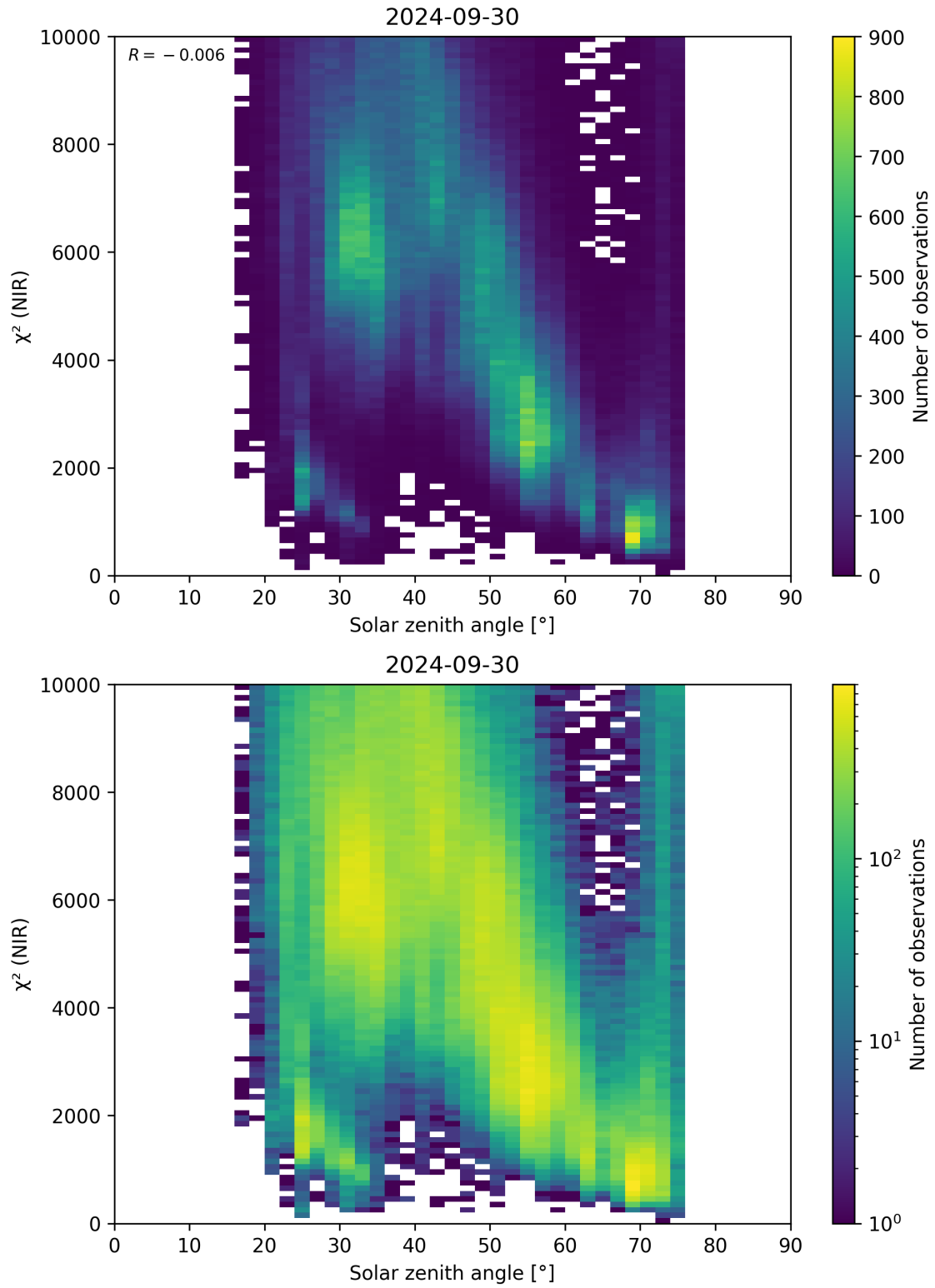
Figure 94: Scatter density plot of “Solar zenith angle” against “ \chi^2 (NIR)” for 2024-09-29 to 2024-10-01.
