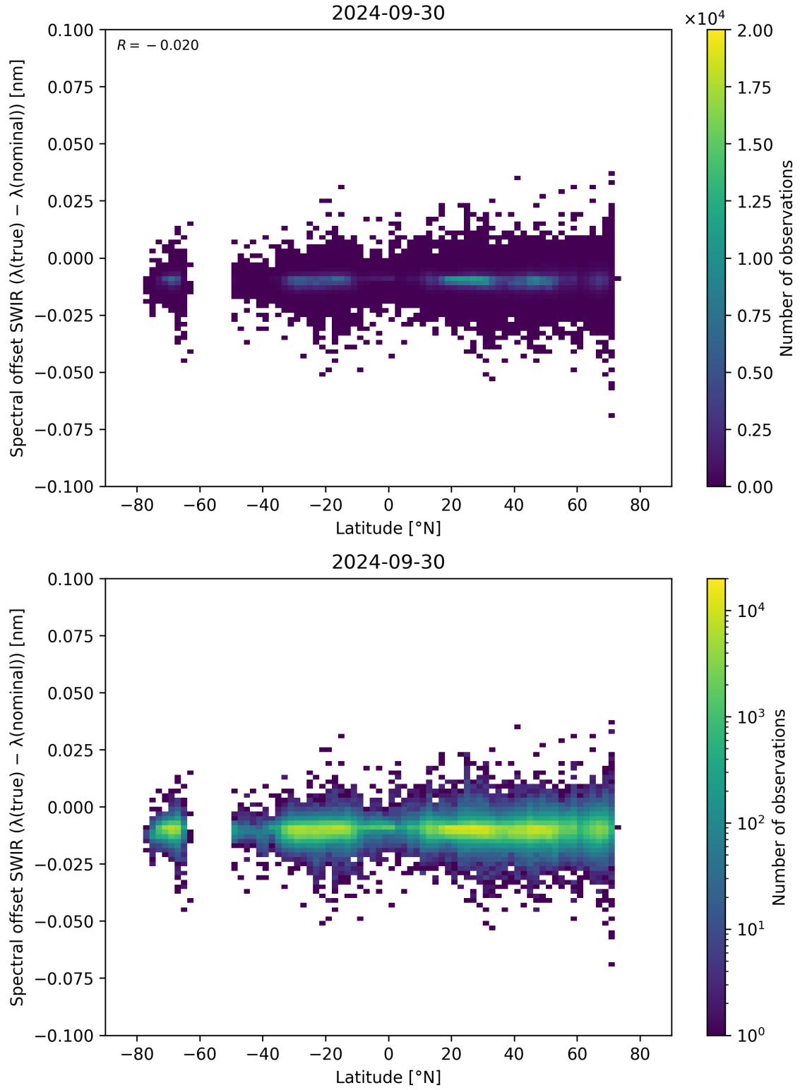
Figure 62: Scatter density plot of “Latitude” against “Spectral offset SWIR ( \lambda_{\text{true}} - \lambda_{\text{nominal}} )” for 2024-09-29 to 2024-10-01.
