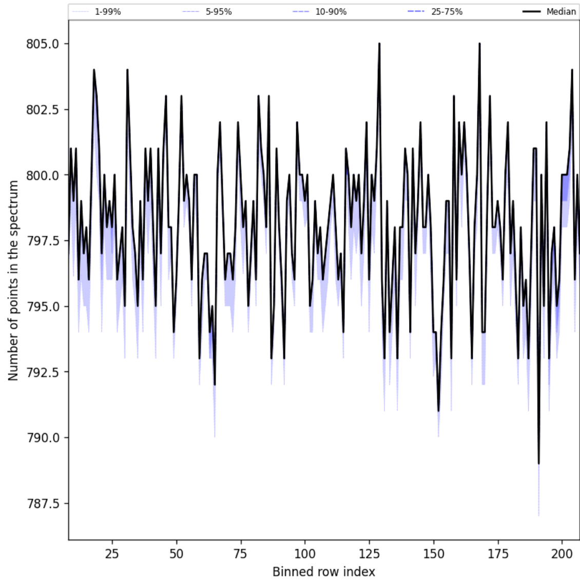
Figure 37: Along track statistics of “Number of points in the spectrum” for 2024-09-29 to 2024-10-01
