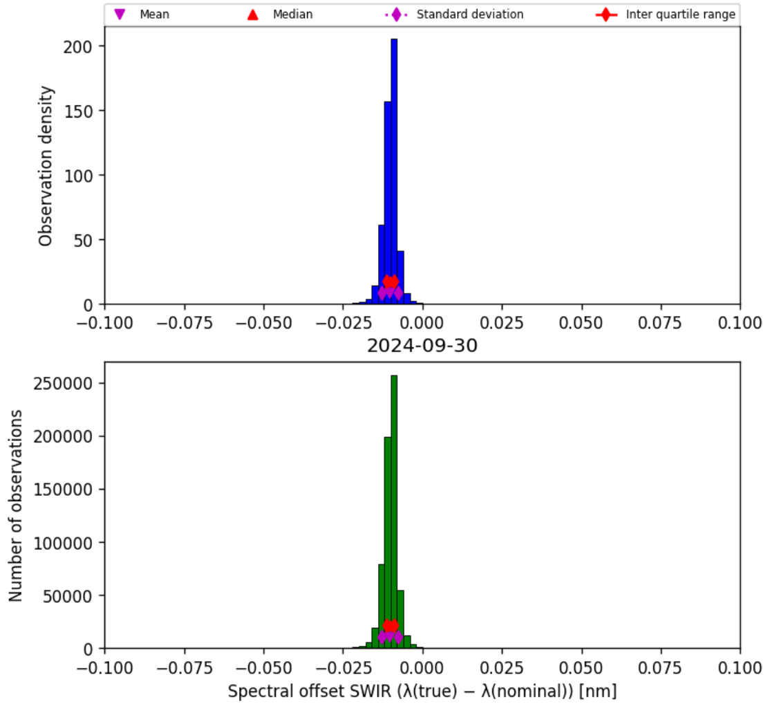
Figure 27: Histogram of “Spectral offset SWIR ( \lambda_{\text{true}} - \lambda_{\text{nominal}} )” for 2024-09-29 to 2024-10-01
