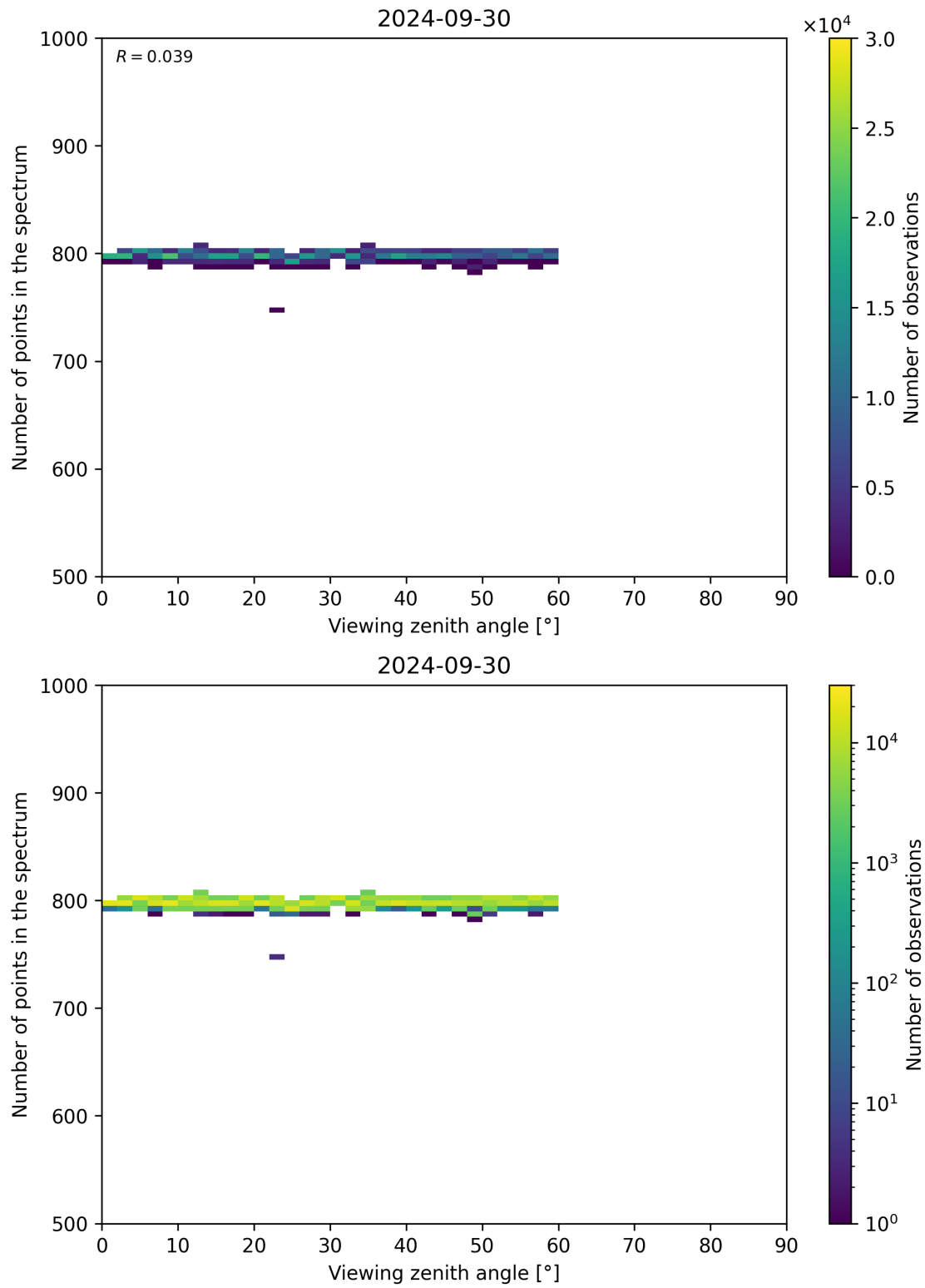
Figure 114: Scatter density plot of “Viewing zenith angle” against “Number of points in the spectrum” for 2024-09-29 to 2024-10-01.
