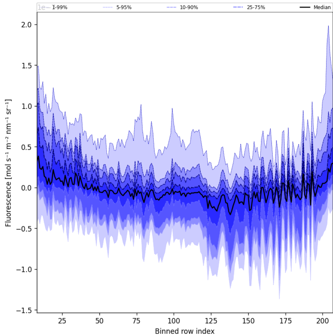
Figure 43: Along track statistics of “Fluorescence” for 2024-09-29 to 2024-10-01
