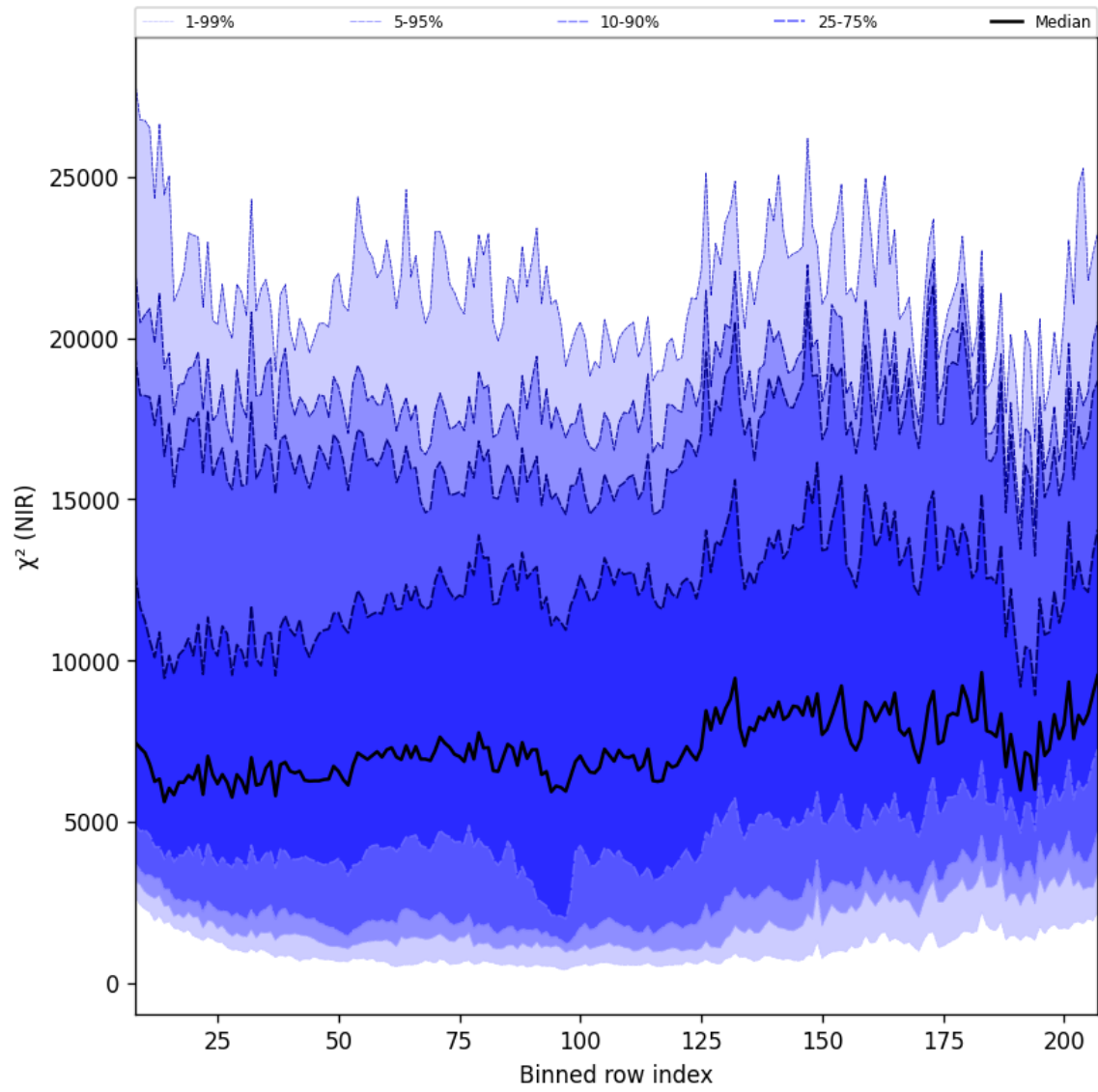
Figure 40: Along track statistics of “ \chi^2 (NIR)” for 2024-09-29 to 2024-10-01
