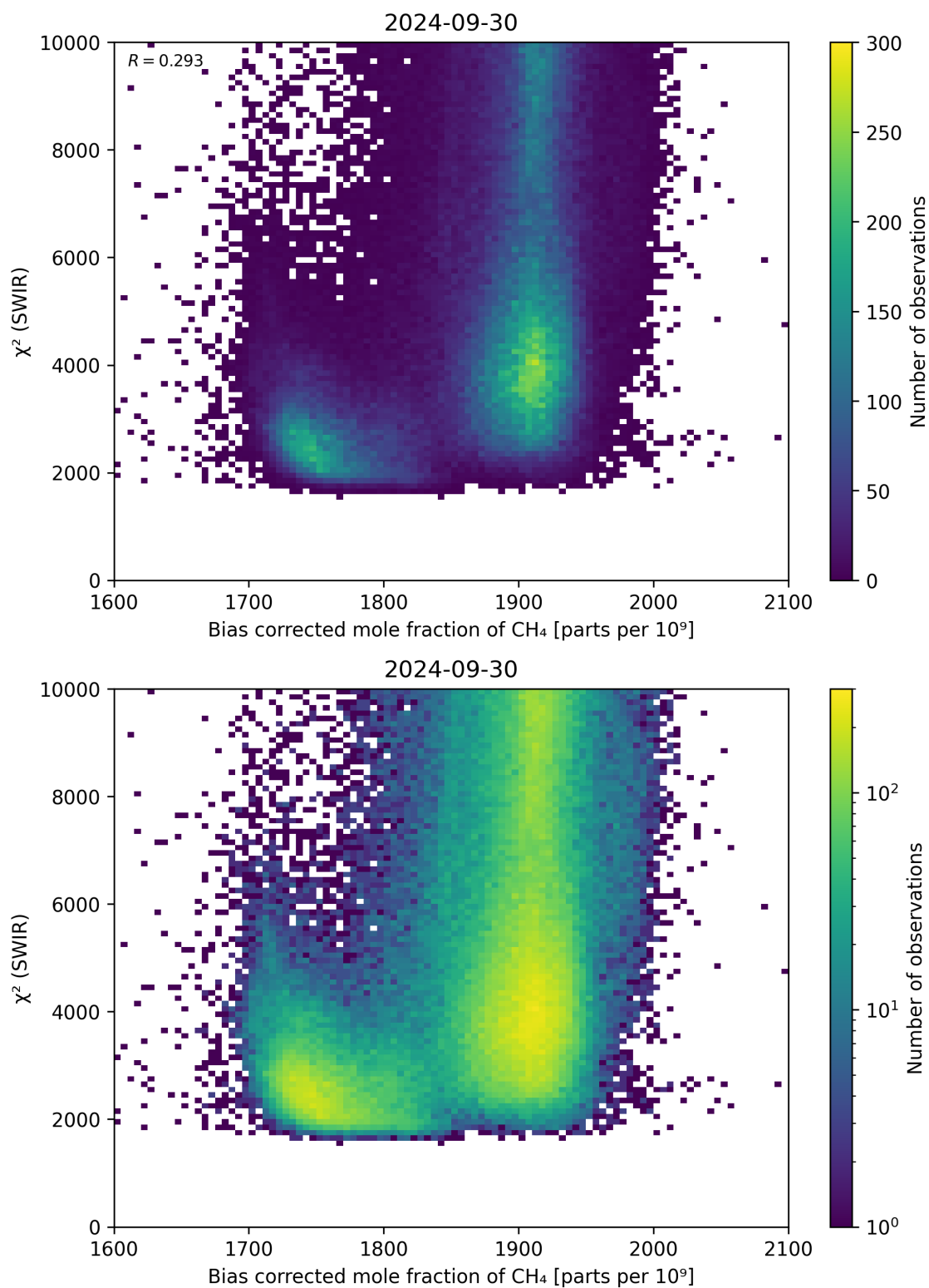
Figure 64: Scatter density plot of “Bias corrected mole fraction of \text{CH}_4 ” against “ \chi^2 (SWIR)” for 2024-09-29 to 2024-10-01.
