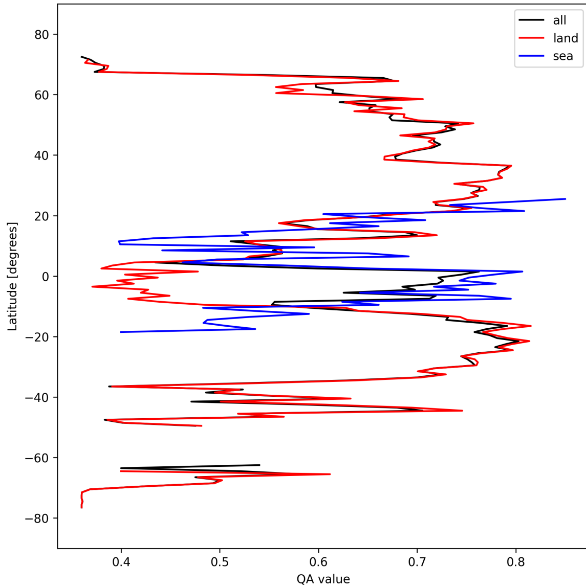
Figure 11: Zonal average of “QA value” for 2024-09-29 to 2024-10-01.
