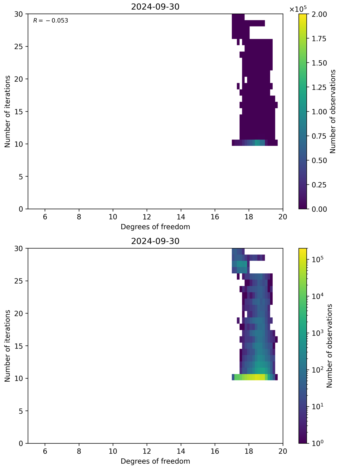
Figure 52: Scatter density plot of “Degrees of freedom” against “Number of iterations” for 2024-09-29 to 2024-10-01.
