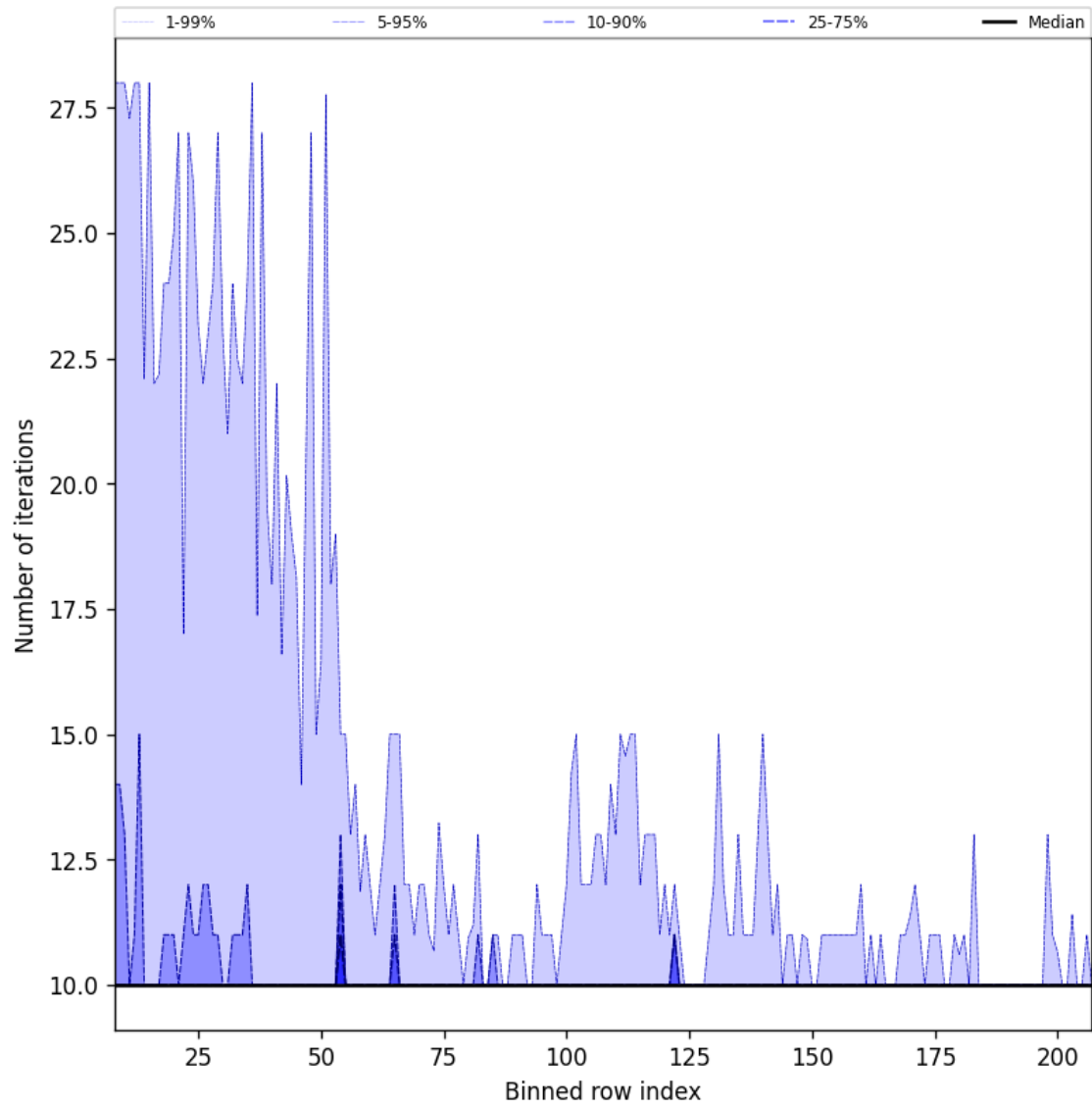
Figure 42: Along track statistics of “Number of iterations” for 2024-09-29 to 2024-10-01
