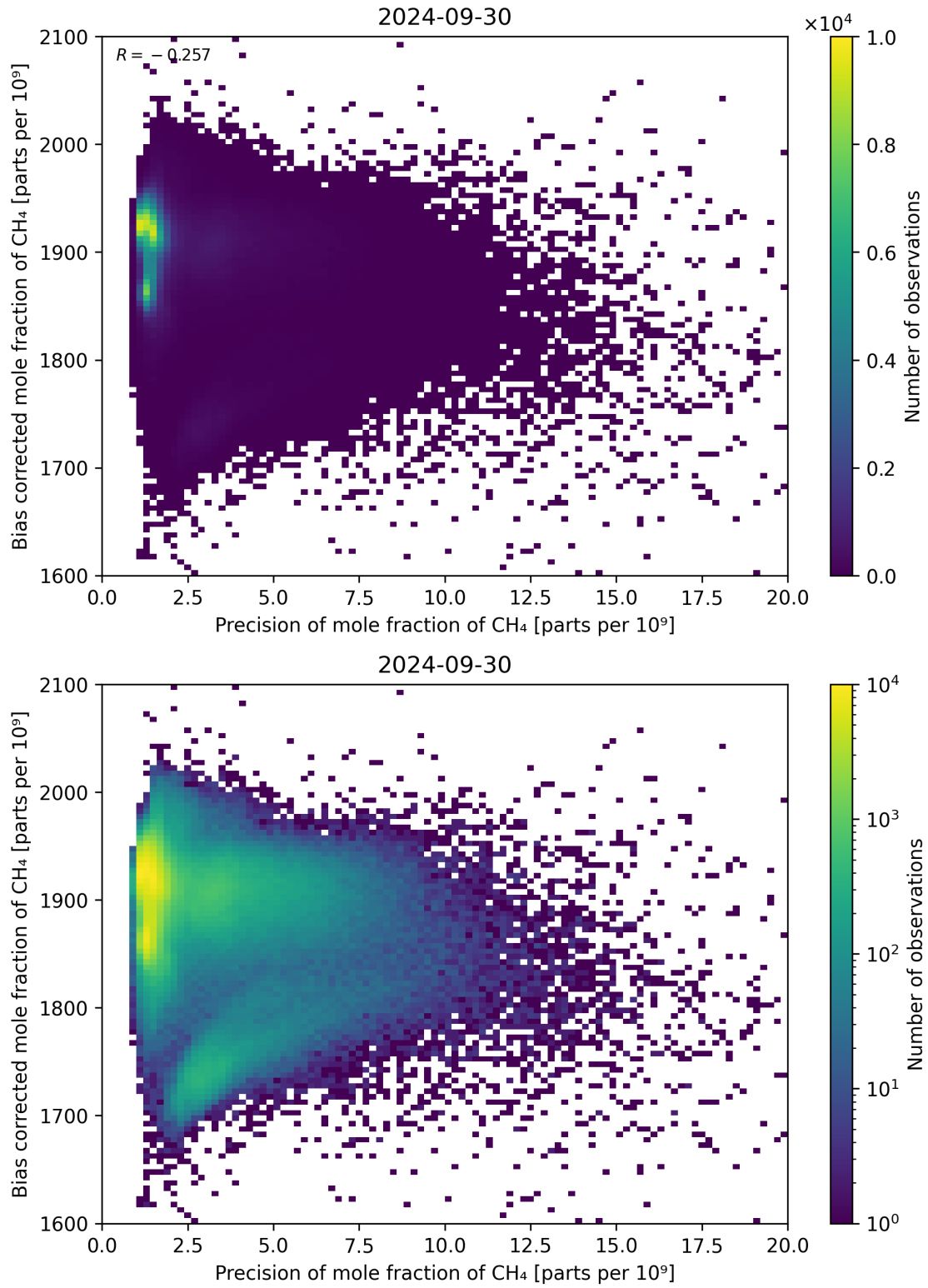
Figure 82: Scatter density plot of “Precision of mole fraction of CH 4 ” against “Bias corrected mole fraction of CH 4 ” for 2024-09-29 to 2024-10-01.
