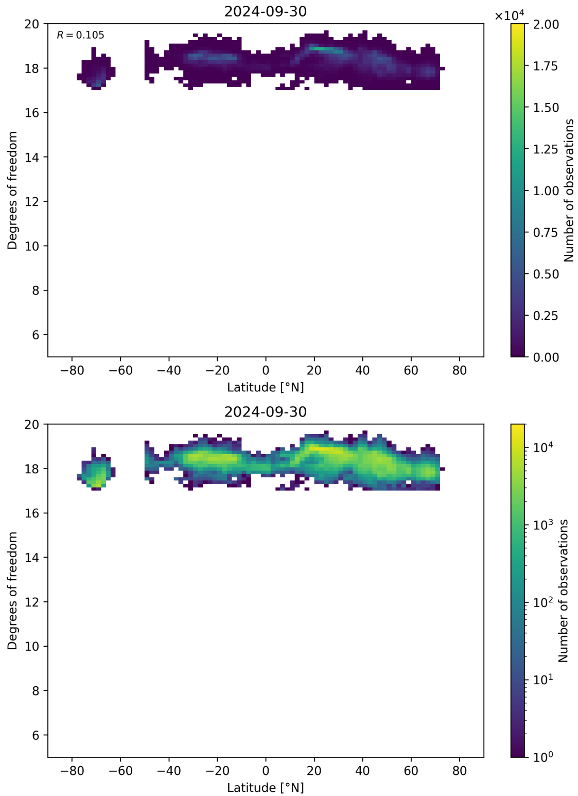
Figure 55: Scatter density plot of “Latitude” against “Degrees of freedom” for 2024-09-29 to 2024-10-01.
