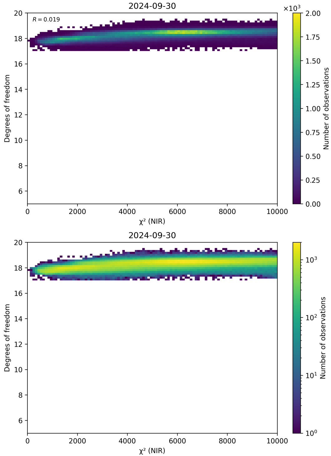
Figure 44: Scatter density plot of “ \chi^2 (NIR)” against “Degrees of freedom” for 2024-09-29 to 2024-10-01.
