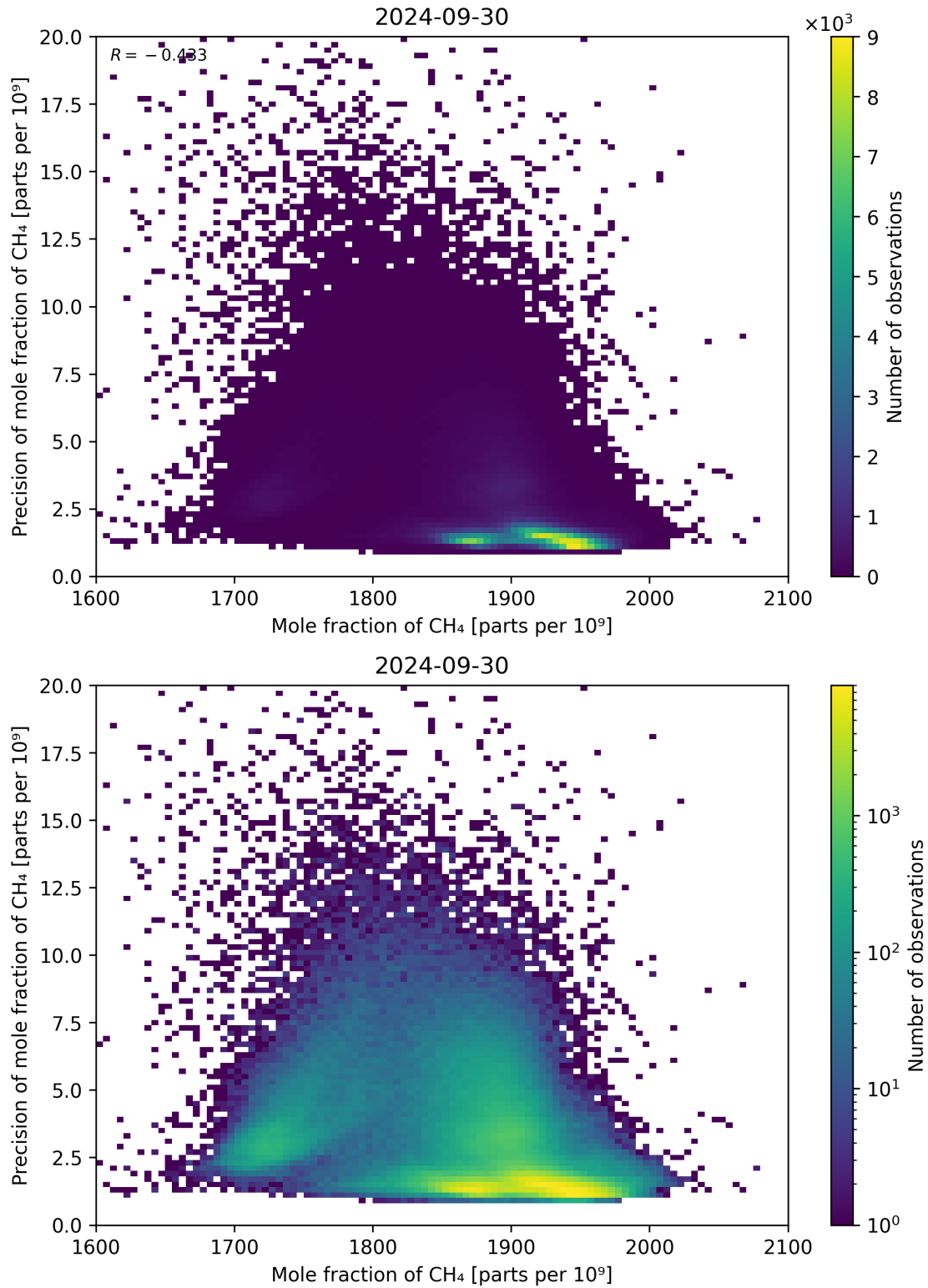
Figure 75: Scatter density plot of “Mole fraction of CH 4 ” against “Precision of mole fraction of CH 4 ” for 2024-09-29 to 2024-10-01.
