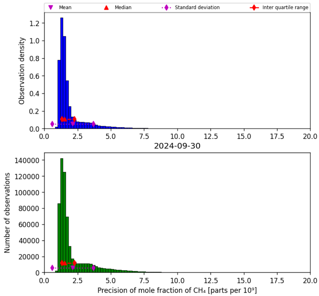
Figure 24: Histogram of “Precision of mole fraction of CH 4 ” for 2024-09-29 to 2024-10-01
