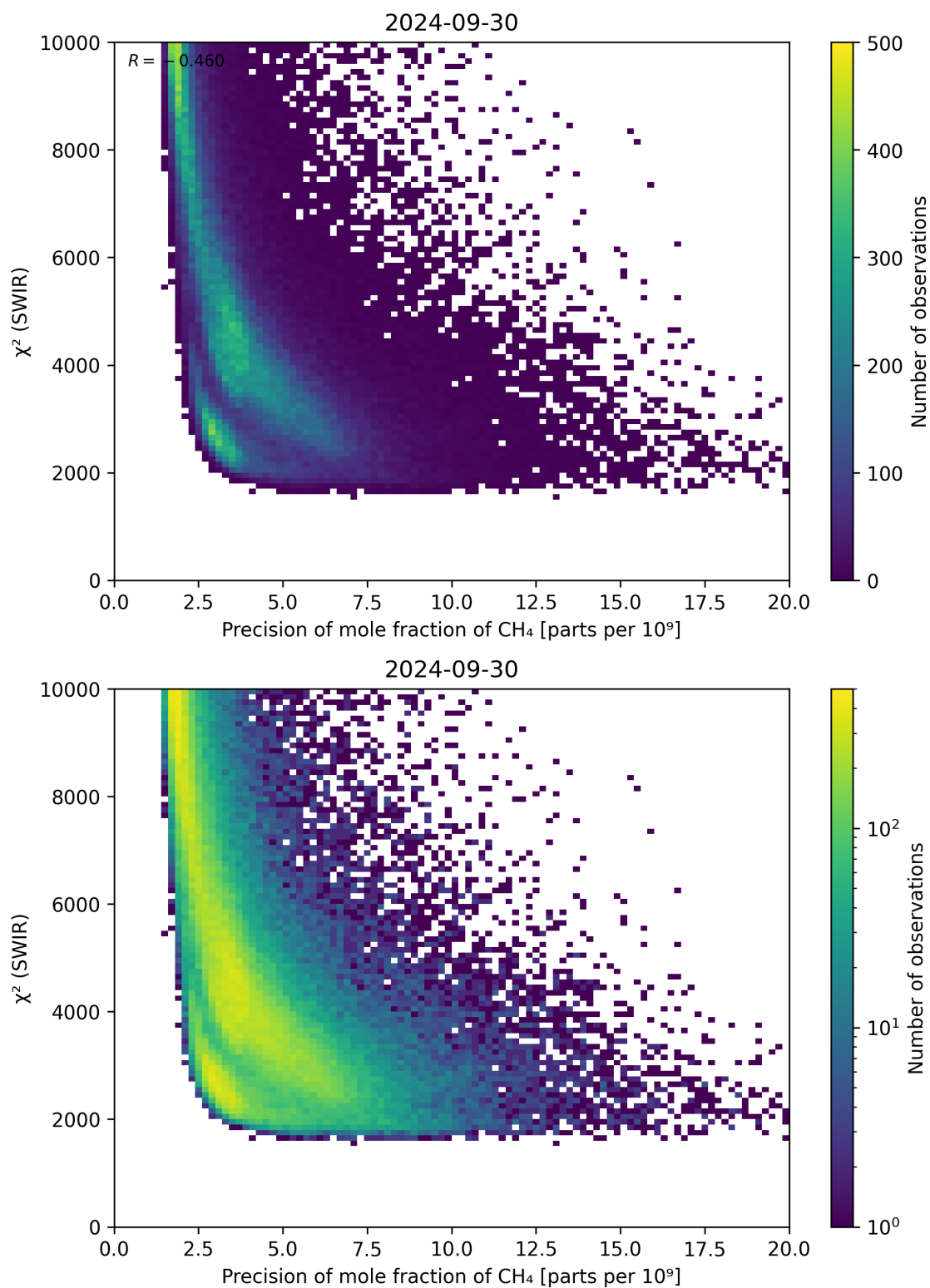
Figure 79: Scatter density plot of “Precision of mole fraction of \text{CH}_4 ” against “ \chi^2 (SWIR)” for 2024-09-29 to 2024-10-01.
