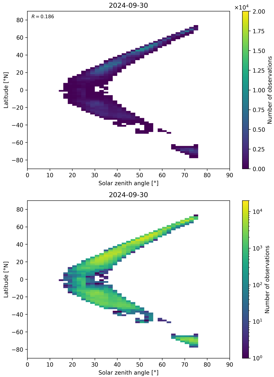
Figure 98: Scatter density plot of “Solar zenith angle” against “Latitude” for 2024-09-29 to 2024-10-01.
