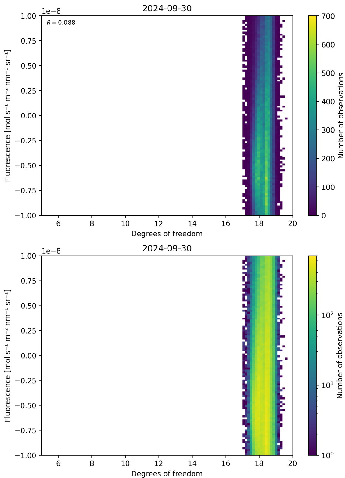
Figure 51: Scatter density plot of “Degrees of freedom” against “Fluorescence” for 2024-09-29 to 2024-10-01.
