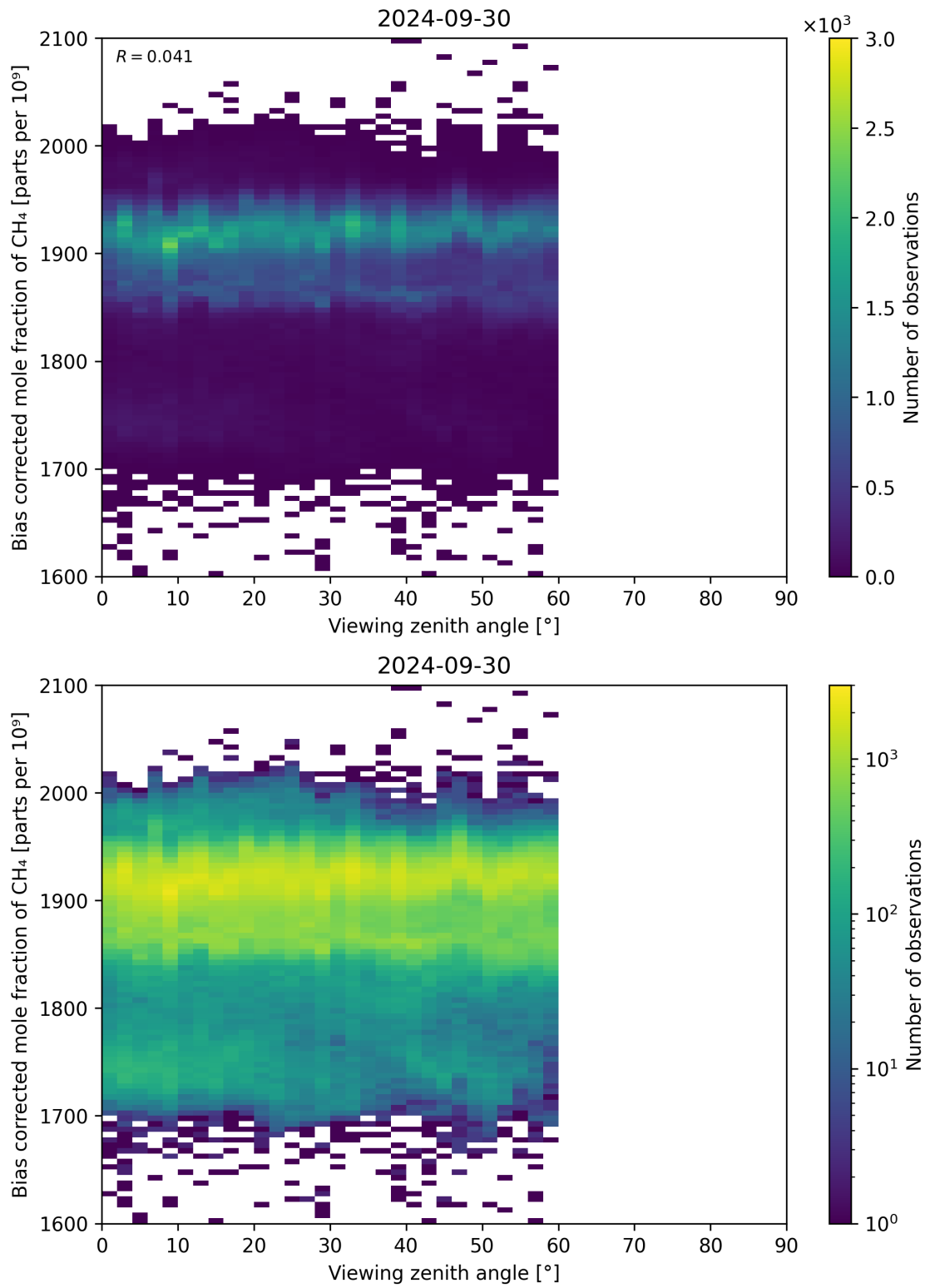
Figure 111: Scatter density plot of “Viewing zenith angle” against “Bias corrected mole fraction of CH 4 ” for 2024-09-29 to 2024-10-01.
