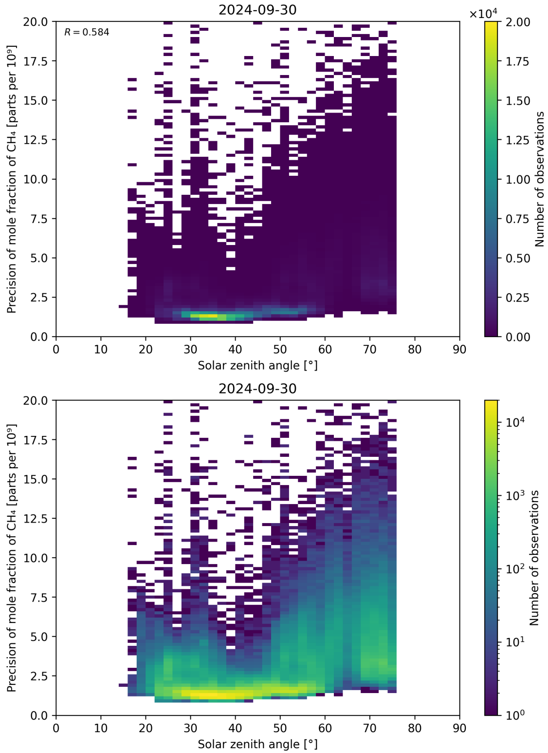
Figure 101: Scatter density plot of “Solar zenith angle” against “Precision of mole fraction of \text{CH}_4 ” for 2024-09-29 to 2024-10-01.
