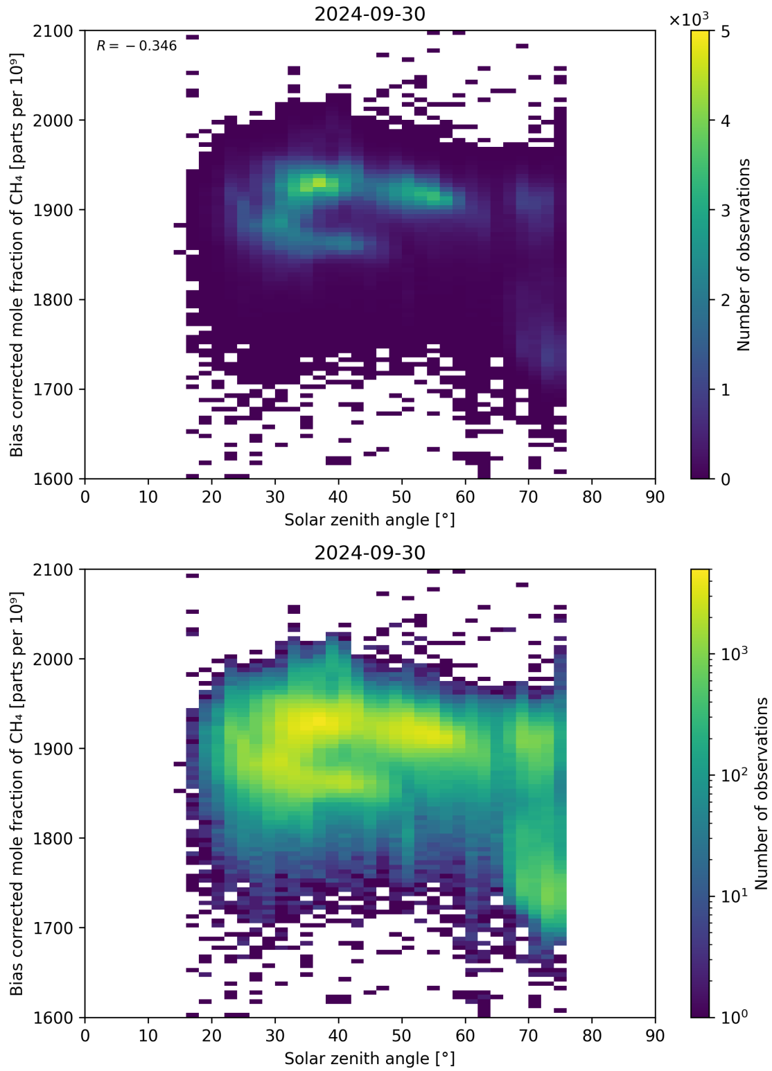
Figure 100: Scatter density plot of “Solar zenith angle” against “Bias corrected mole fraction of \text{CH}_4 ” for 2024-09-29 to 2024-10-01.
