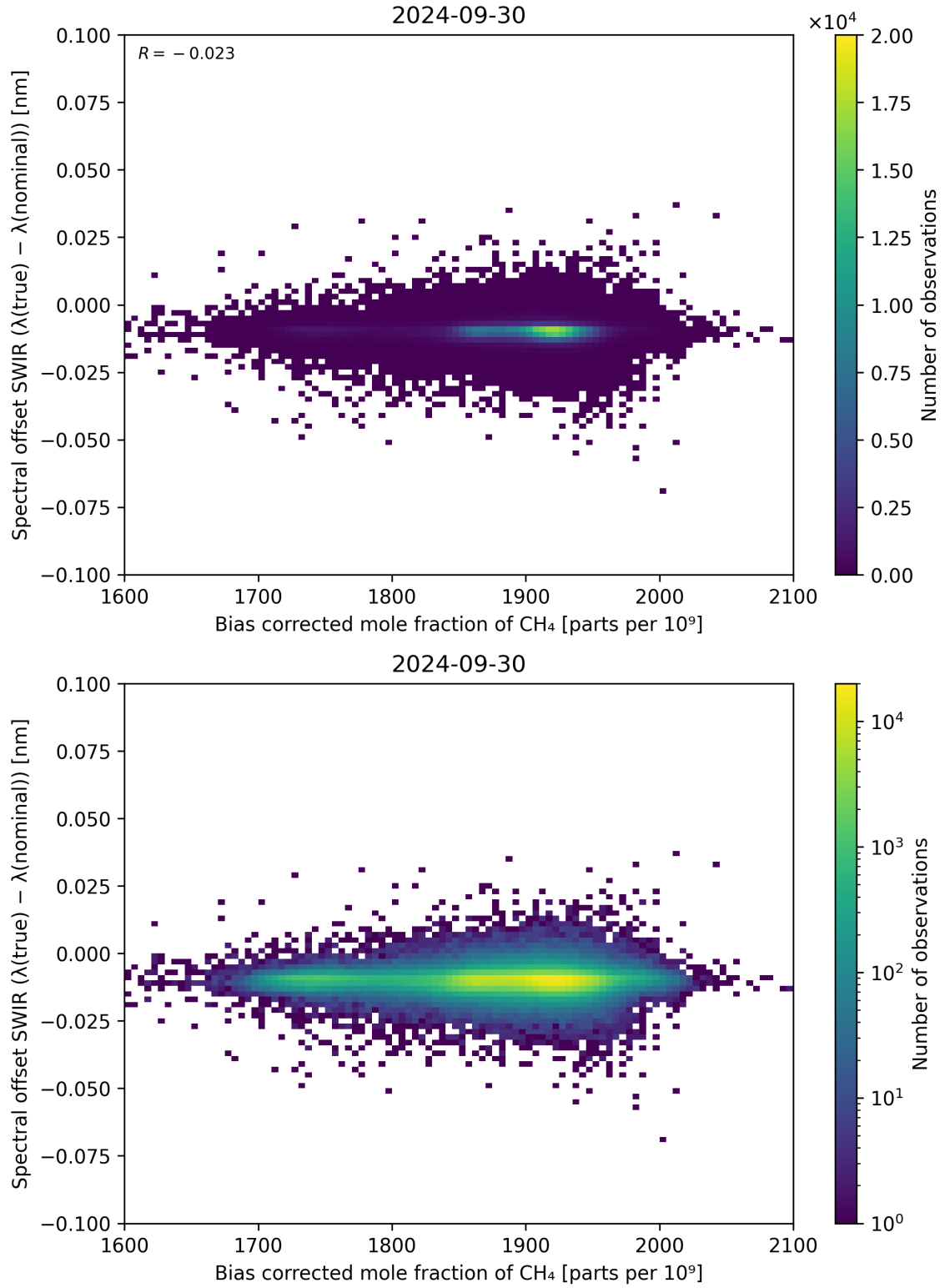
Figure 69: Scatter density plot of “Bias corrected mole fraction of \text{CH}_4 ” against “Spectral offset SWIR ( \lambda_{\text{true}} - \lambda_{\text{nominal}} )” for 2024-09-29 to 2024-10-01.
