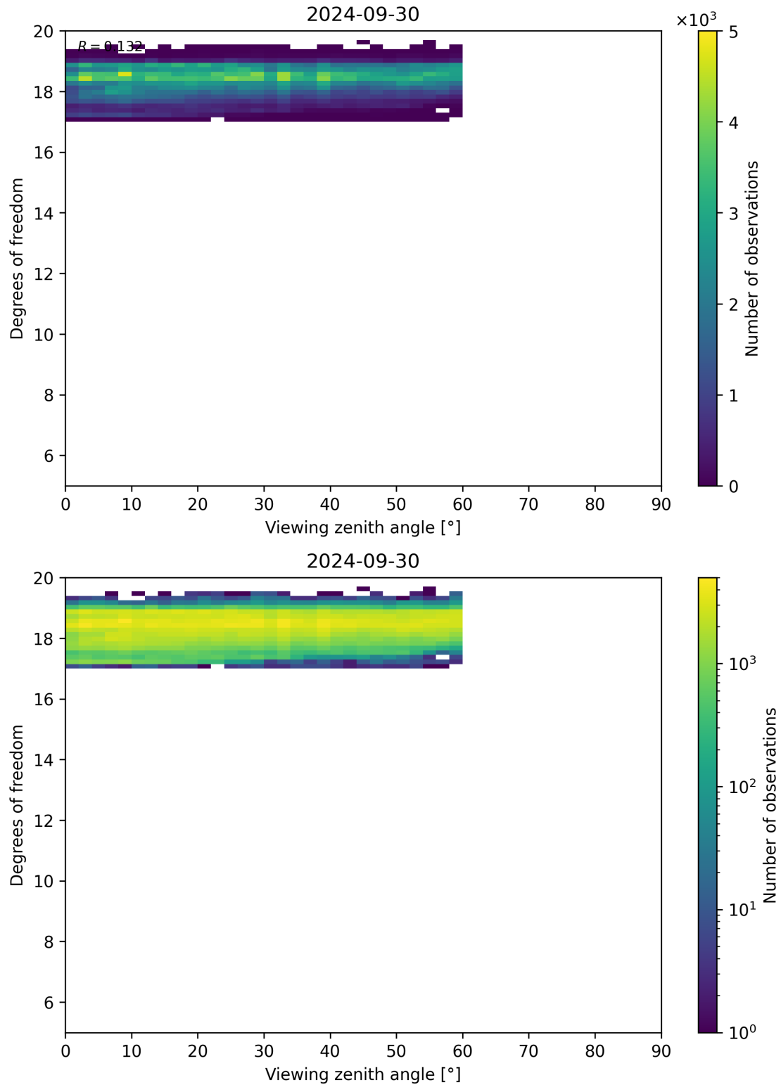
Figure 107: Scatter density plot of “Viewing zenith angle” against “Degrees of freedom” for 2024-09-29 to 2024-10-01.
