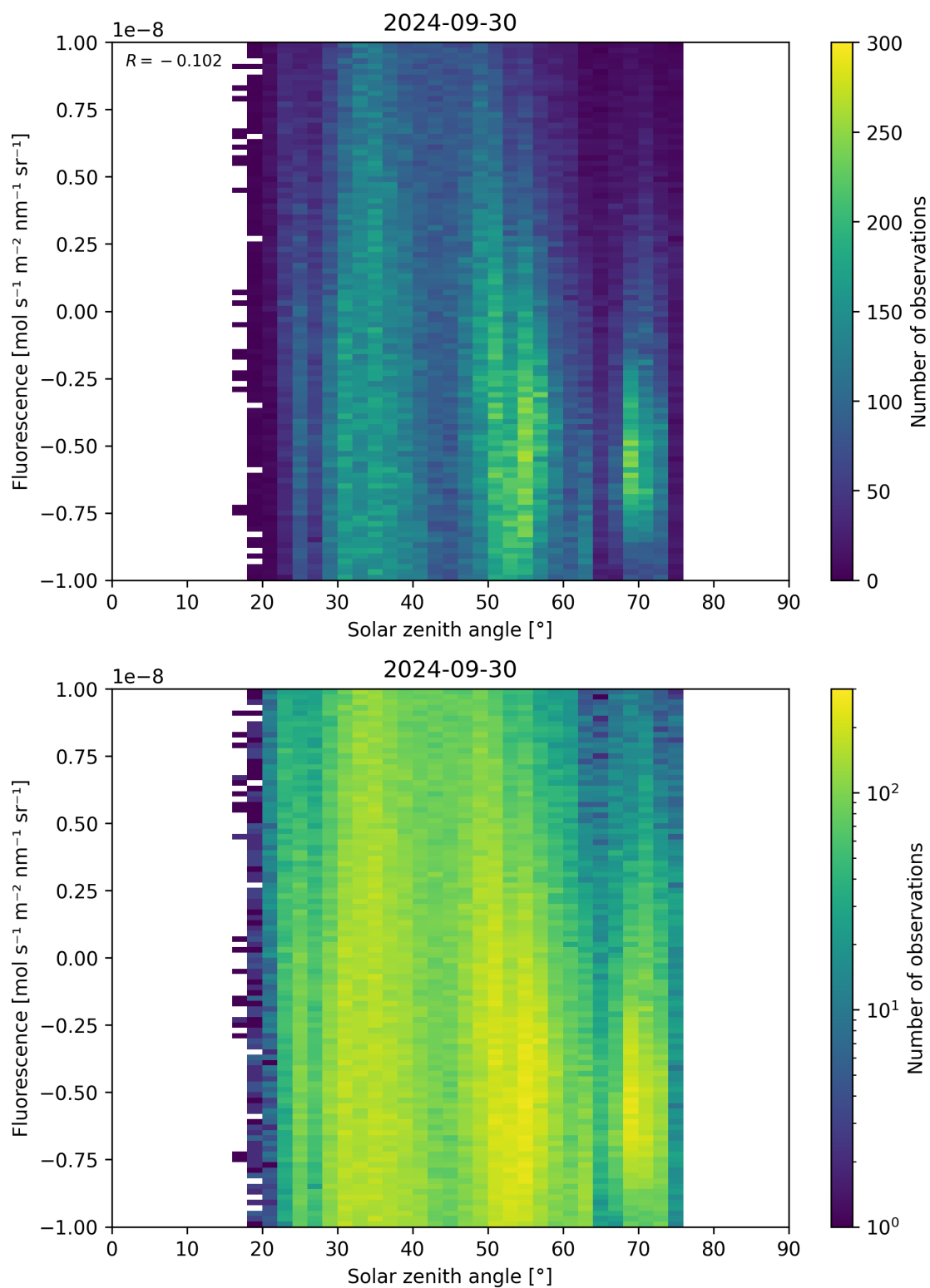
Figure 97: Scatter density plot of “Solar zenith angle” against “Fluorescence” for 2024-09-29 to 2024-10-01.
