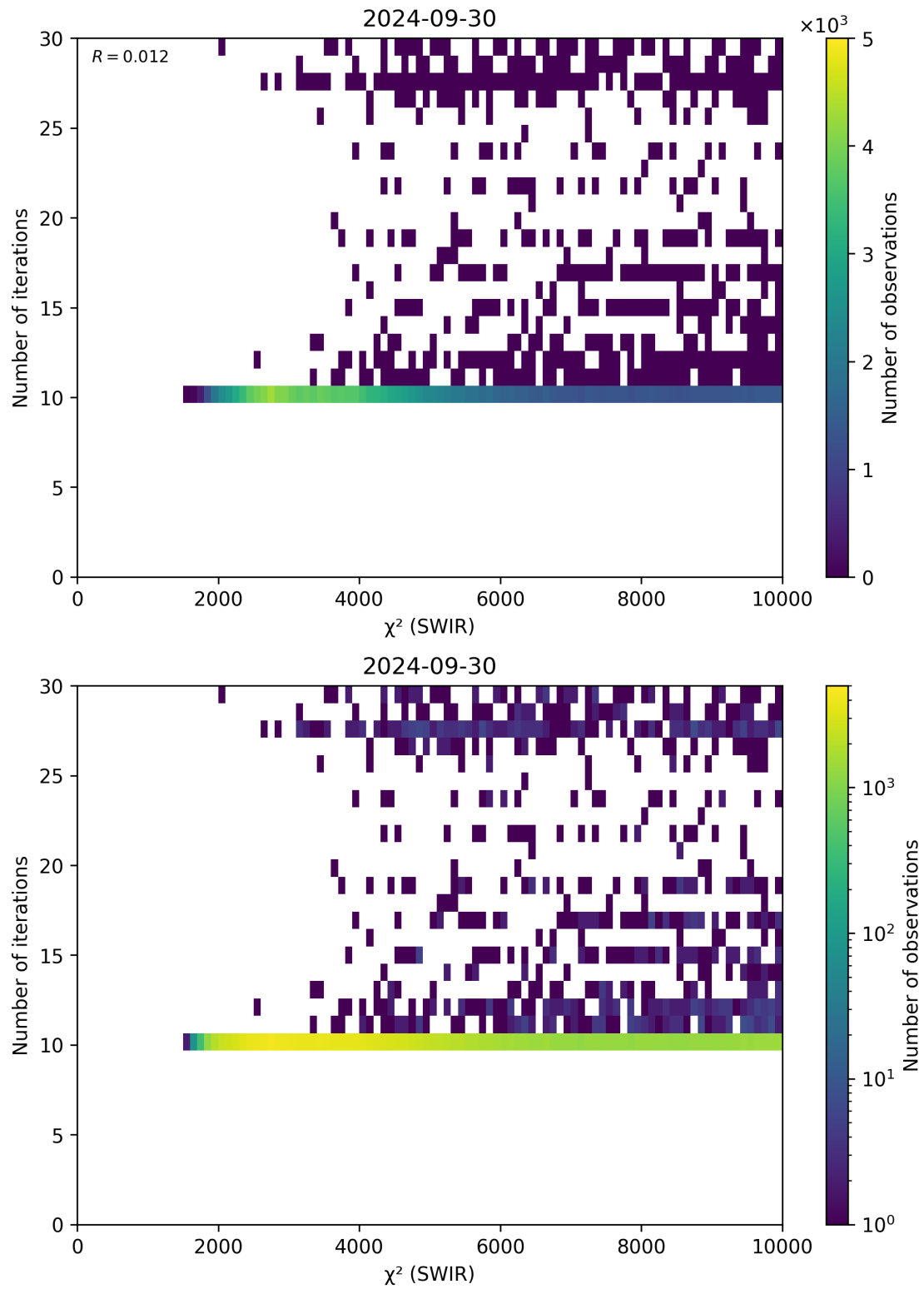
Figure 50: Scatter density plot of “ \chi^2 (SWIR)” against “Number of iterations” for 2024-09-29 to 2024-10-01.
