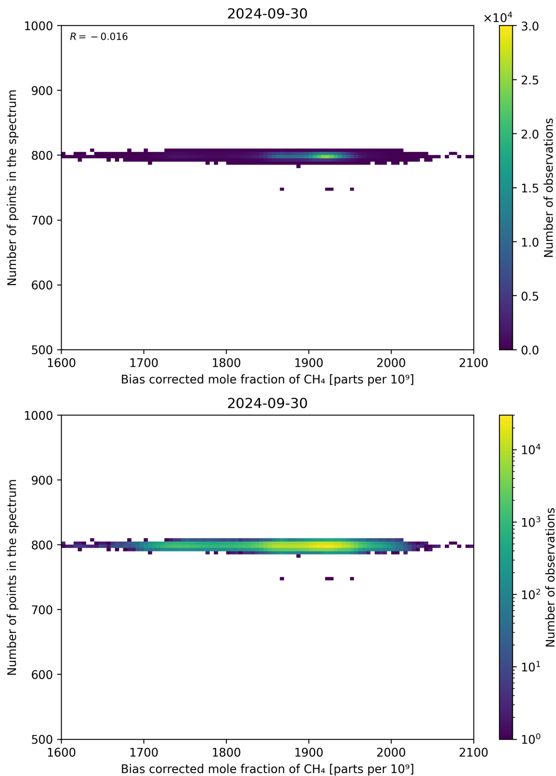
Figure 68: Scatter density plot of “Bias corrected mole fraction of CH 4 ” against “Number of points in the spectrum” for 2024-09-29 to 2024-10-01.
