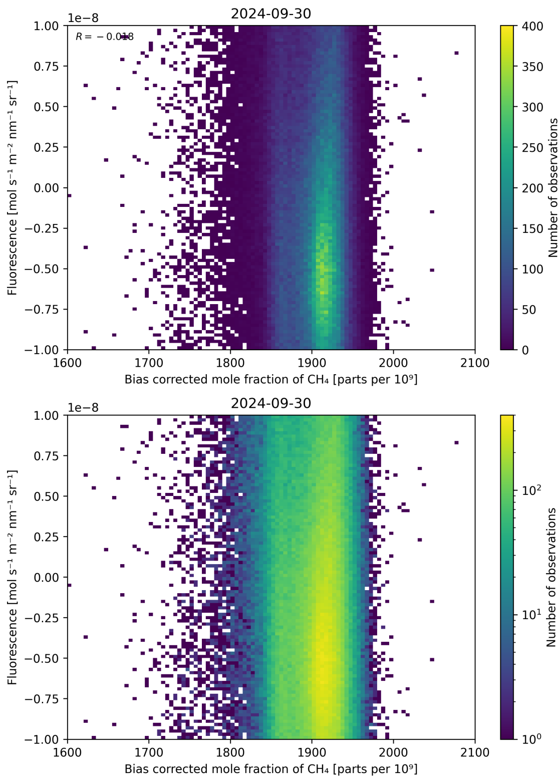
Figure 66: Scatter density plot of “Bias corrected mole fraction of \text{CH}_4 ” against “Fluorescence” for 2024-09-29 to 2024-10-01.
