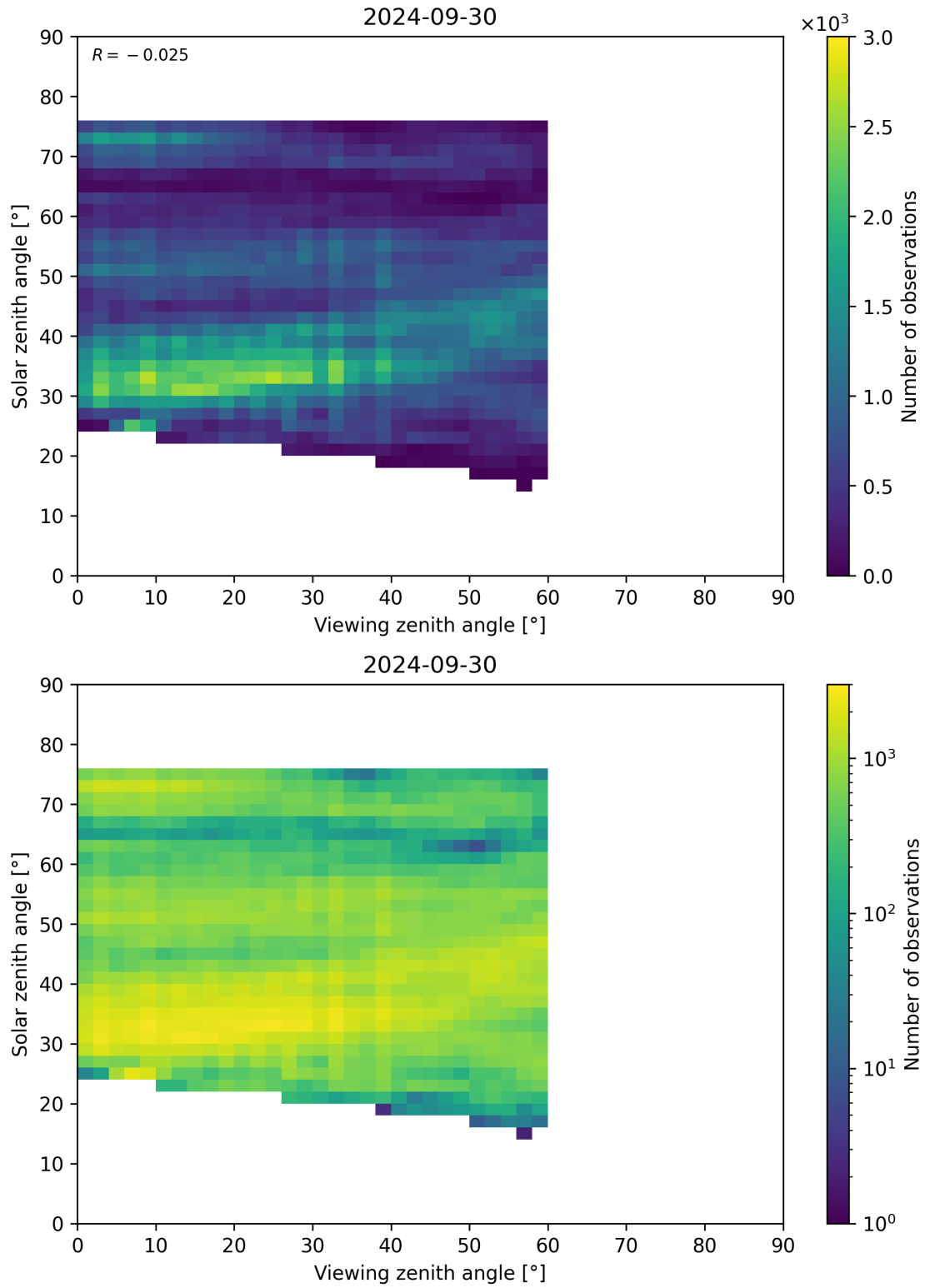
Figure 115: Scatter density plot of “Viewing zenith angle” against “Solar zenith angle” for 2024-09-29 to 2024-10-01.
