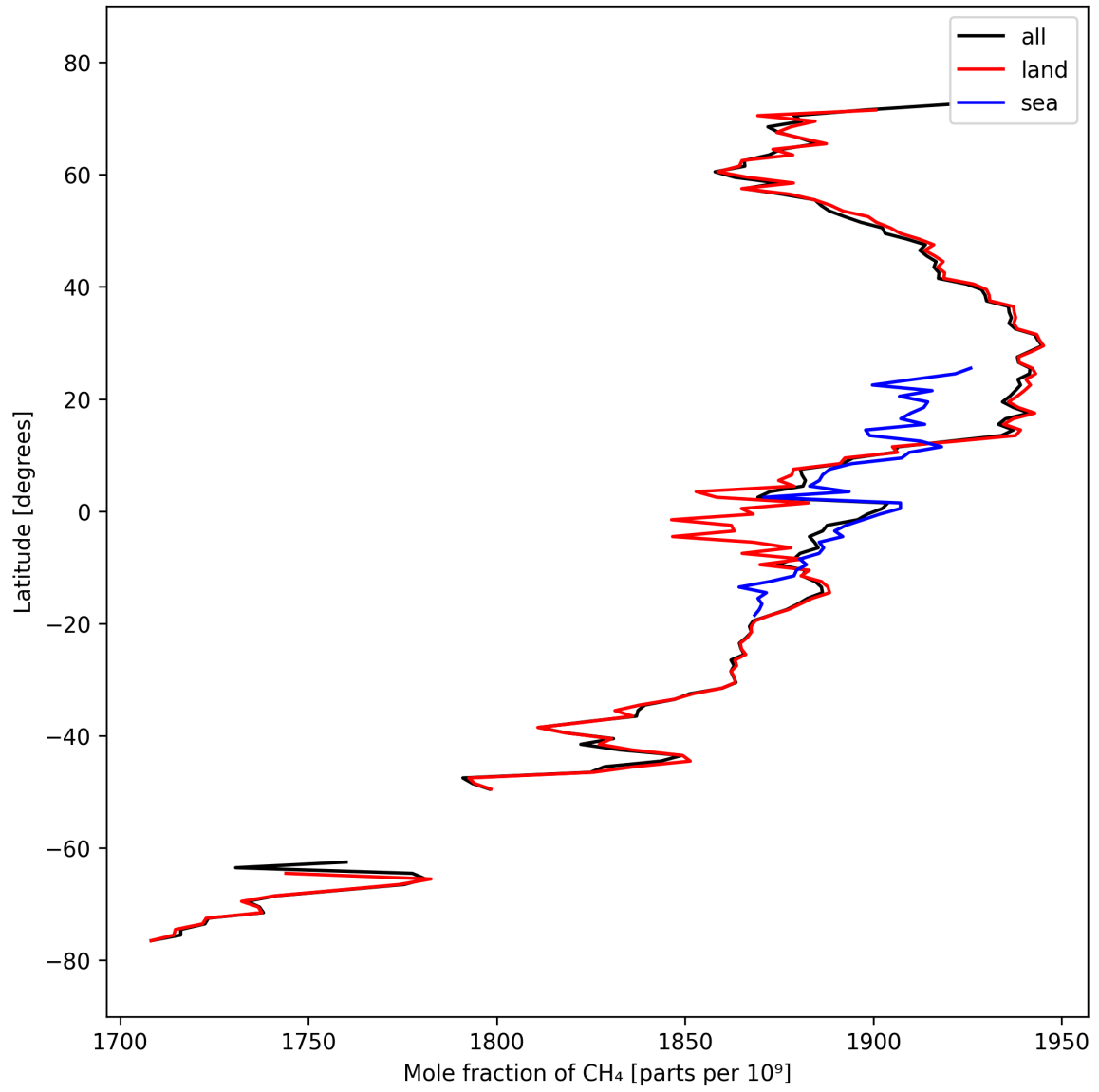
Figure 12: Zonal average of “Mole fraction of CH 4 ” for 2024-09-29 to 2024-10-01.
