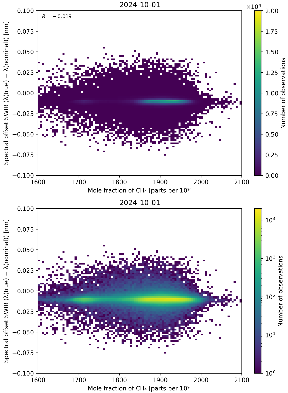
Figure 86: Scatter density plot of “Mole fraction of CH 4 ” against “Spectral offset SWIR ( \lambda_{\text{true}} - \lambda_{\text{nominal}} )” for 2024-09-30 to 2024-10-02.
