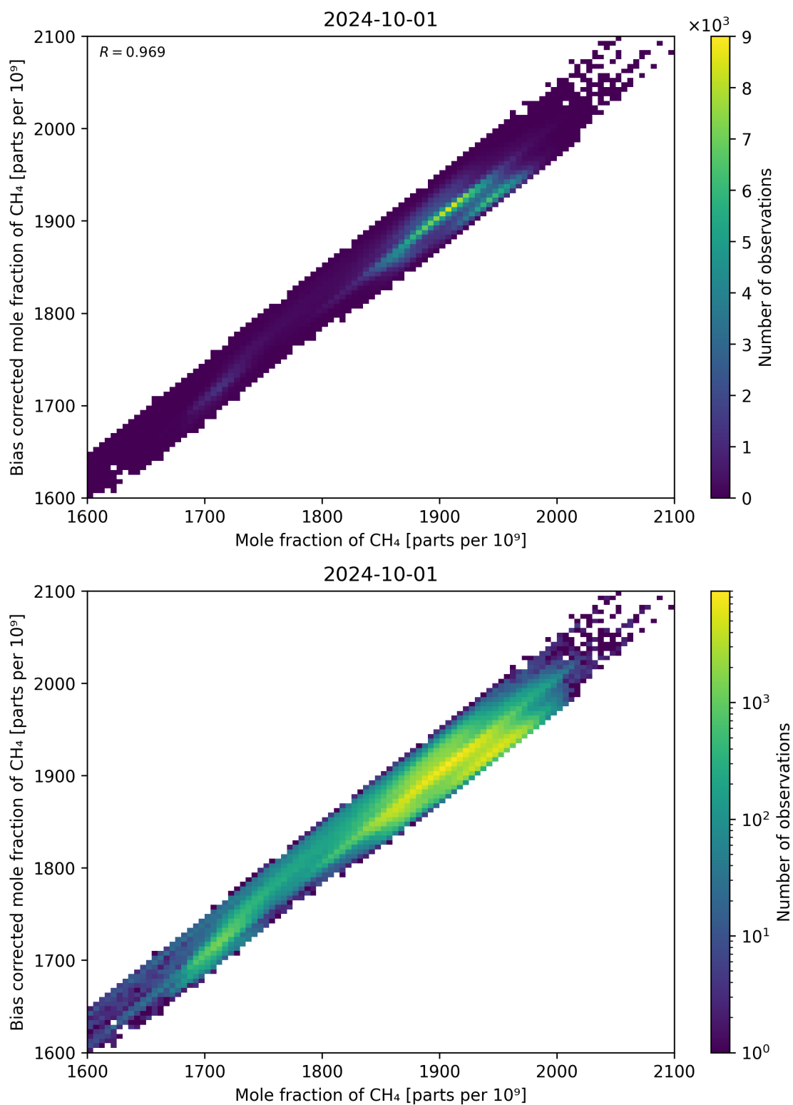
Figure 74: Scatter density plot of “Mole fraction of CH 4 ” against “Bias corrected mole fraction of CH 4 ” for 2024-09-30 to 2024-10-02.
