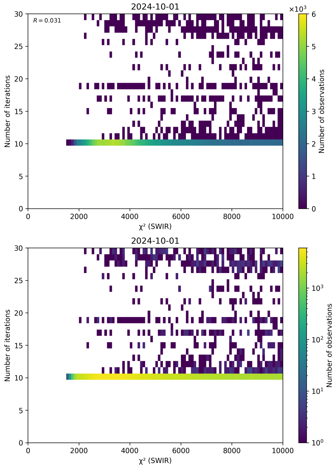
Figure 50: Scatter density plot of “ \chi^2 (SWIR)” against “Number of iterations” for 2024-09-30 to 2024-10-02.
