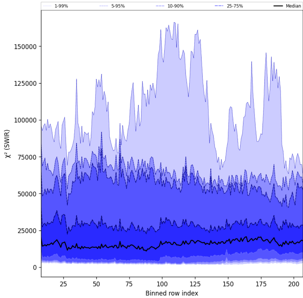
Figure 39: Along track statistics of “ \chi^2 (SWIR)” for 2024-09-30 to 2024-10-02
