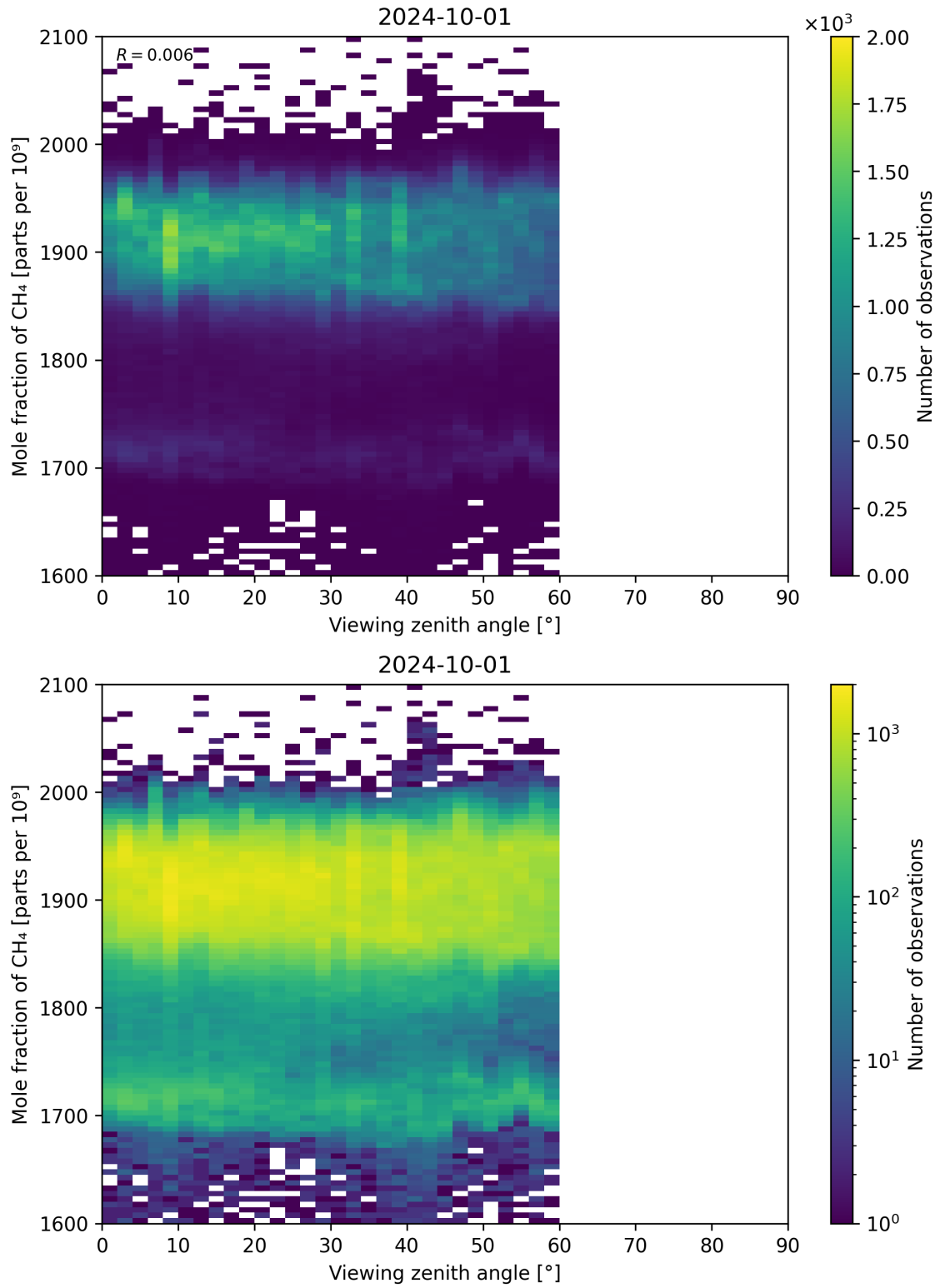
Figure 110: Scatter density plot of “Viewing zenith angle” against “Mole fraction of CH 4 ” for 2024-09-30 to 2024-10-02.
