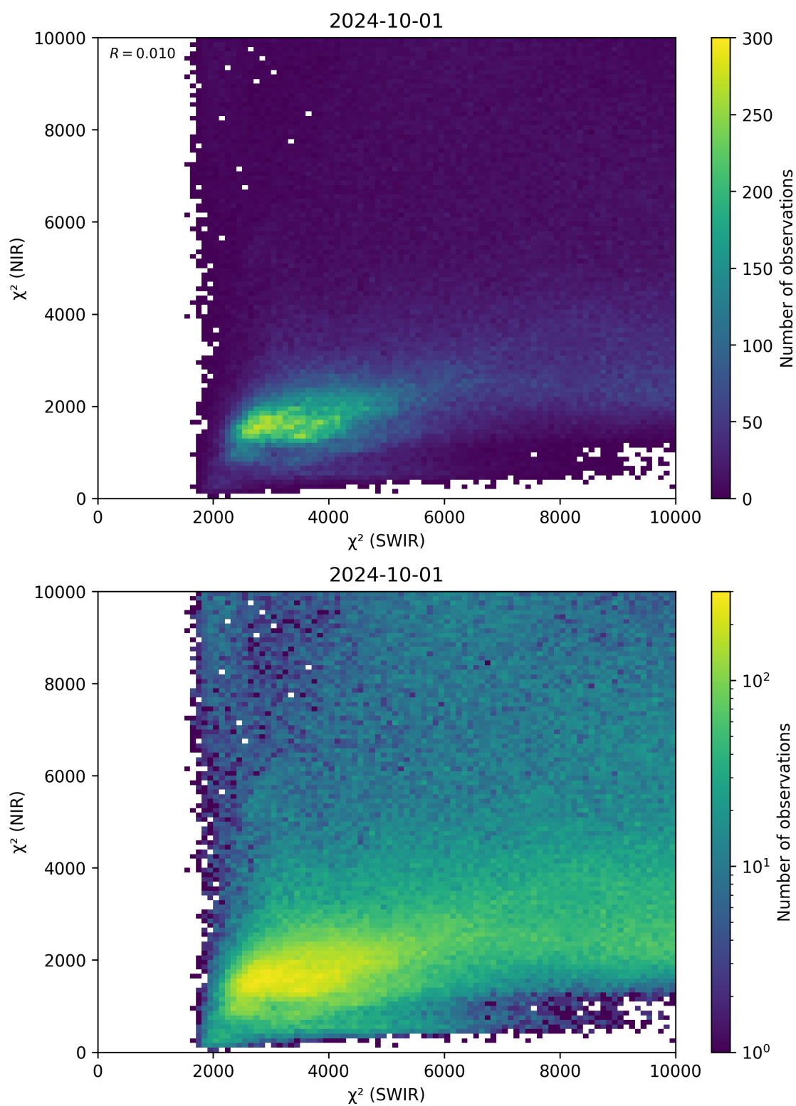
Figure 47: Scatter density plot of “ \chi^2 (SWIR)” against “ \chi^2 (NIR)” for 2024-09-30 to 2024-10-02.
