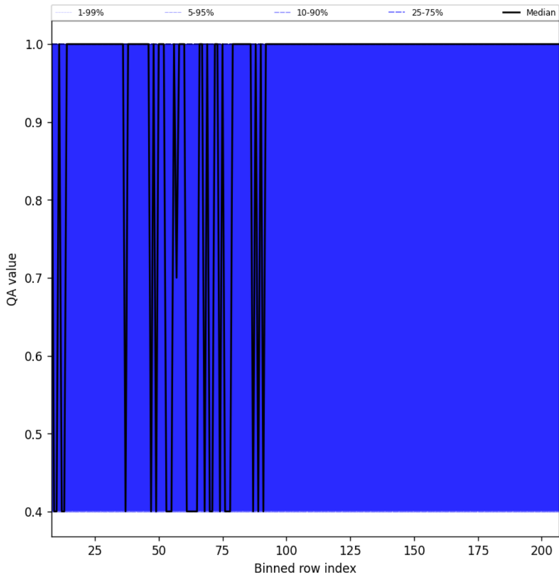
Figure 33: Along track statistics of “QA value” for 2024-09-30 to 2024-10-02
