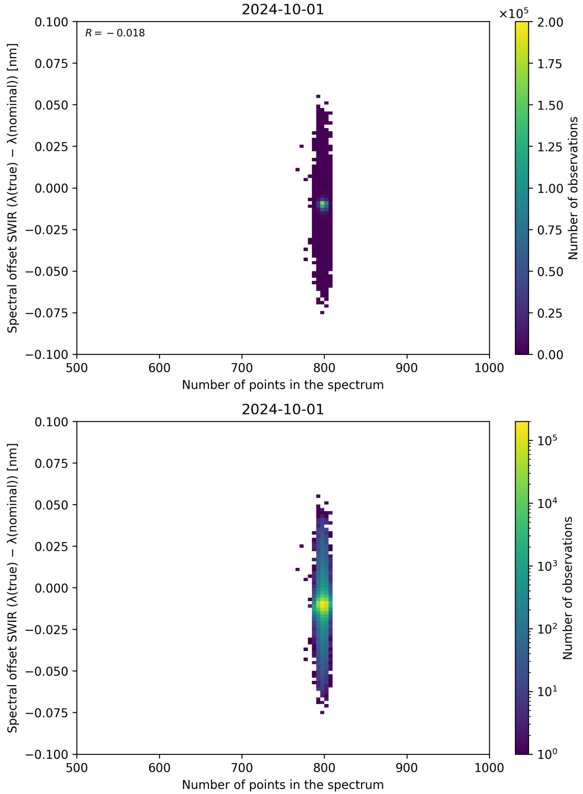
Figure 93: Scatter density plot of “Number of points in the spectrum” against “Spectral offset SWIR ( \lambda_{\text{true}} - \lambda_{\text{nominal}} )” for 2024-09-30 to 2024-10-02.
