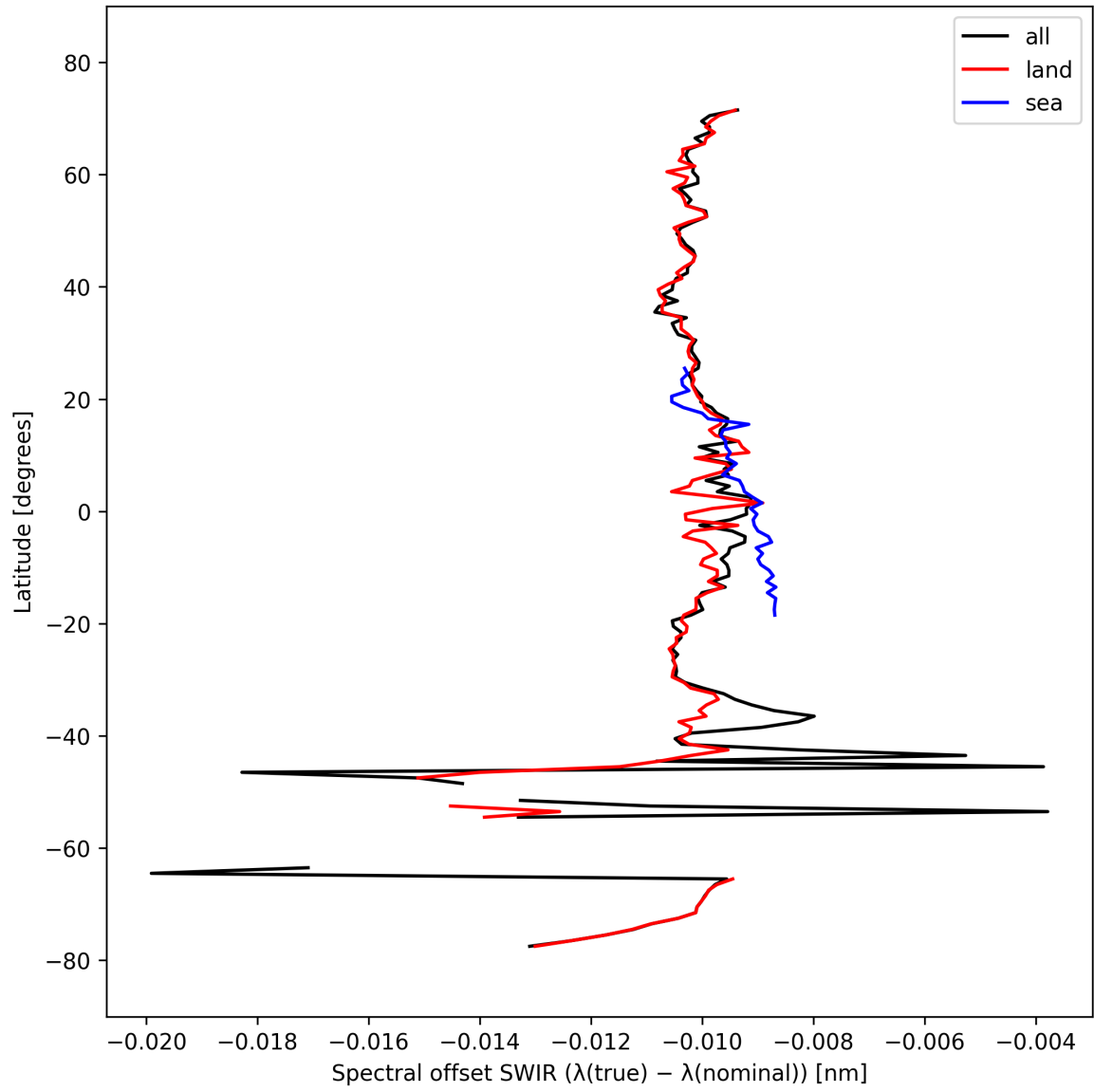
Figure 16: Zonal average of “Spectral offset SWIR ( \lambda_{\text{true}} - \lambda_{\text{nominal}} )” for 2024-09-30 to 2024-10-02.
