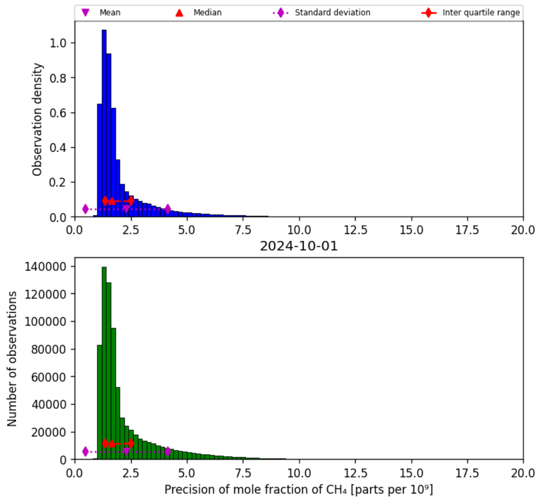
Figure 24: Histogram of “Precision of mole fraction of CH 4 ” for 2024-09-30 to 2024-10-02
