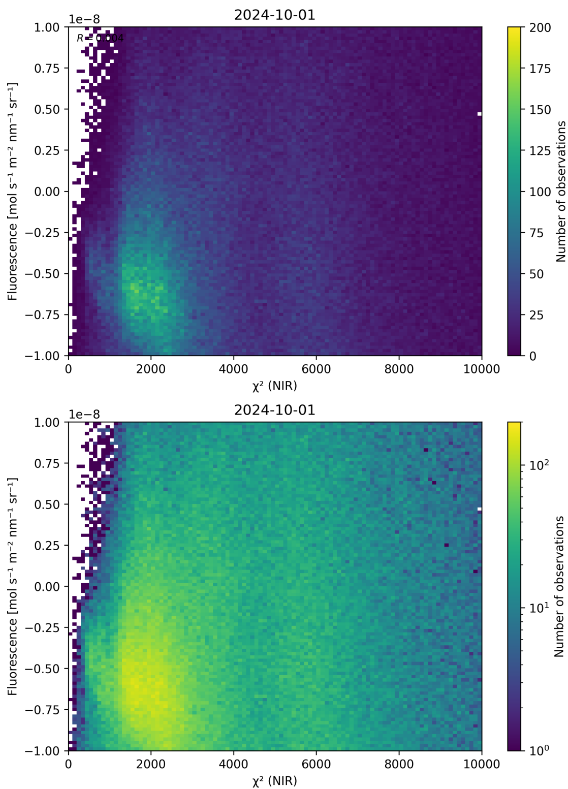
Figure 45: Scatter density plot of “ \chi^2 (NIR)” against “Fluorescence” for 2024-09-30 to 2024-10-02.
