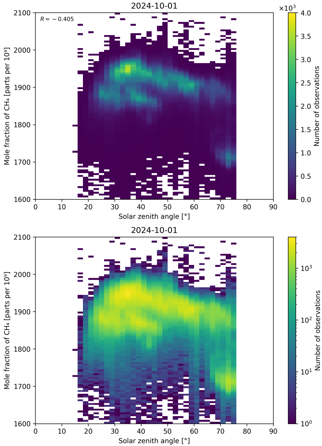
Figure 99: Scatter density plot of “Solar zenith angle” against “Mole fraction of \text{CH}_4 ” for 2024-09-30 to 2024-10-02.
