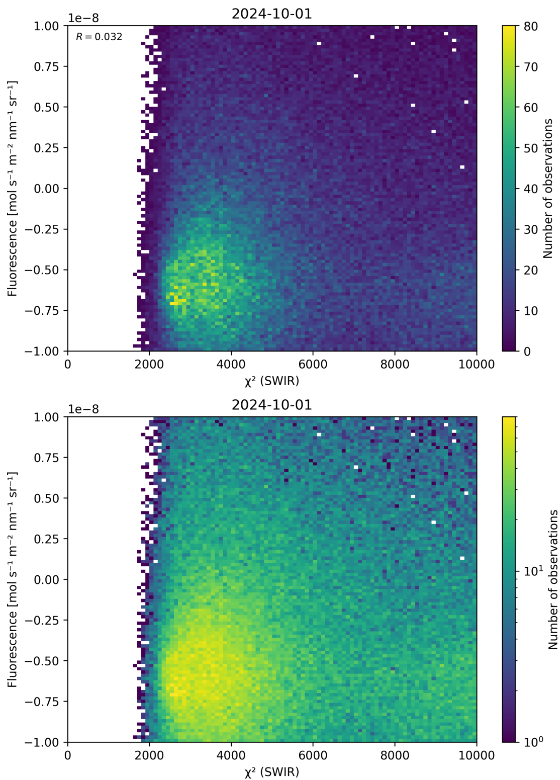
Figure 49: Scatter density plot of “ \chi^2 (SWIR)” against “Fluorescence” for 2024-09-30 to 2024-10-02.
