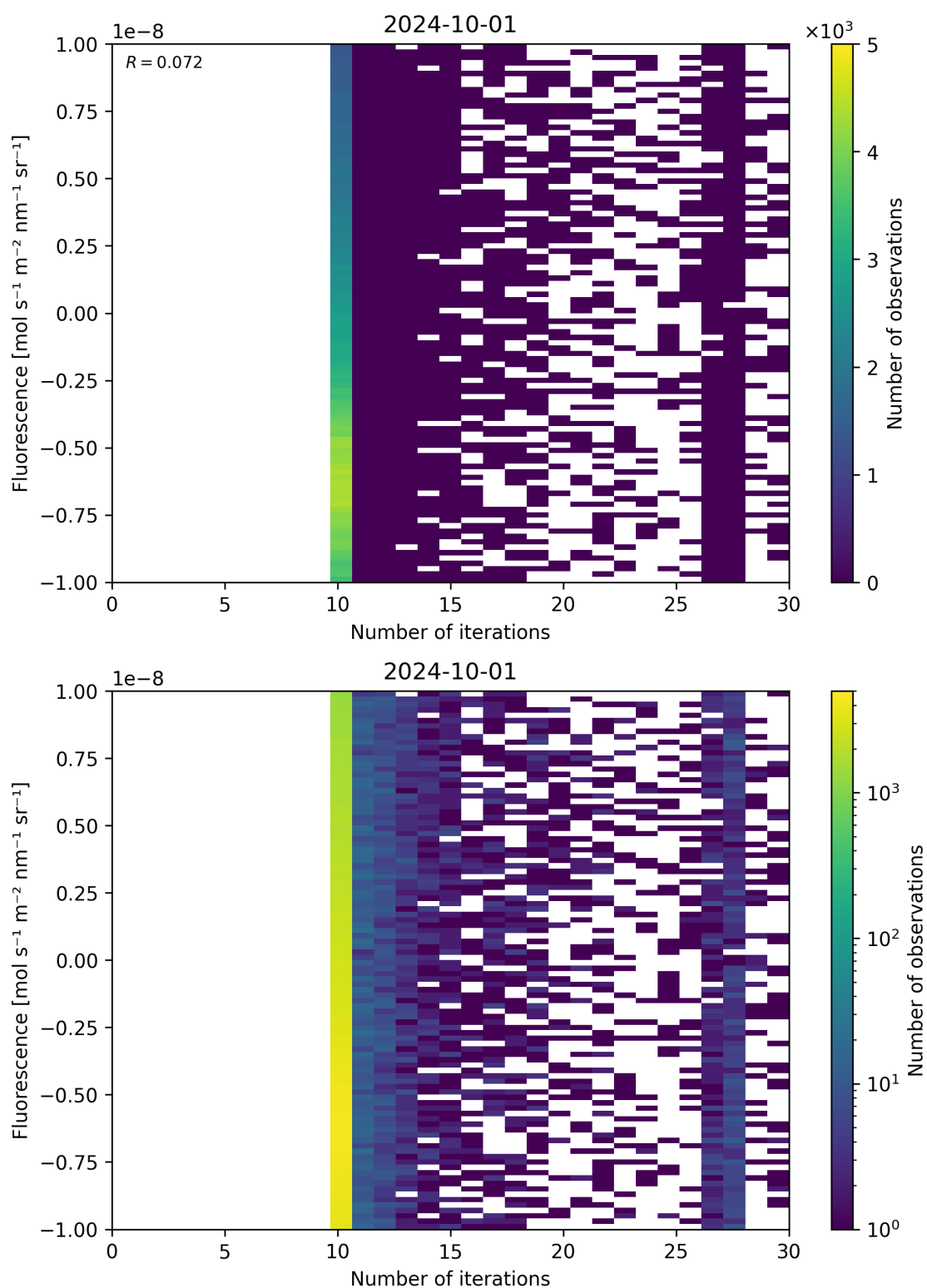
Figure 87: Scatter density plot of “Number of iterations” against “Fluorescence” for 2024-09-30 to 2024-10-02.
