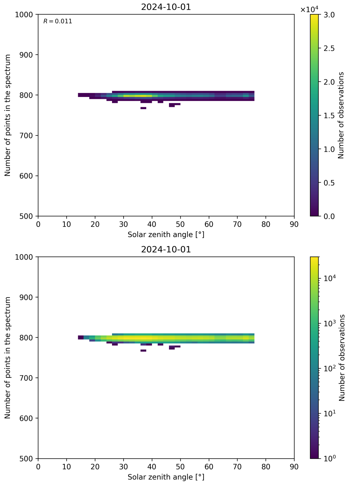
Figure 103: Scatter density plot of “Solar zenith angle” against “Number of points in the spectrum” for 2024-09-30 to 2024-10-02.
