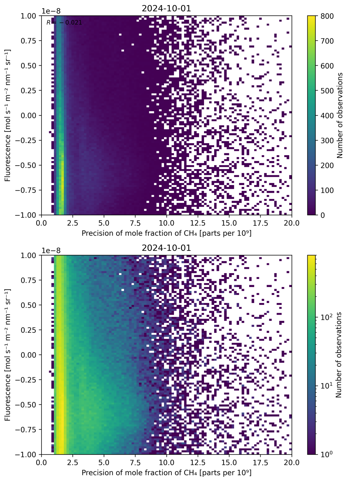
Figure 81: Scatter density plot of “Precision of mole fraction of \text{CH}_4 ” against “Fluorescence” for 2024-09-30 to 2024-10-02.
