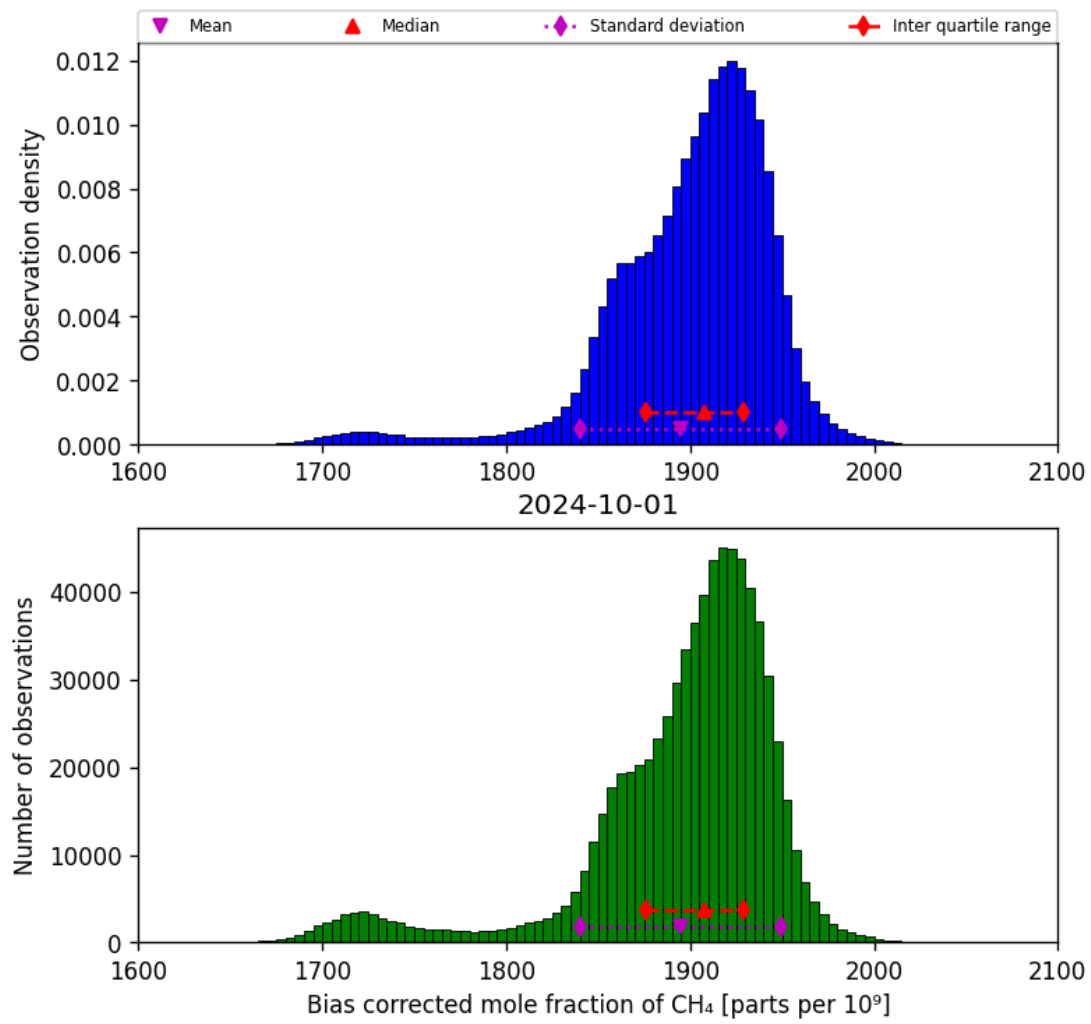
Figure 25: Histogram of “Bias corrected mole fraction of CH 4 ” for 2024-09-30 to 2024-10-02
