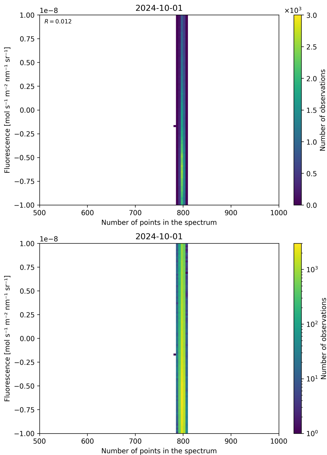
Figure 91: Scatter density plot of “Number of points in the spectrum” against “Fluorescence” for 2024-09-30 to 2024-10-02.
