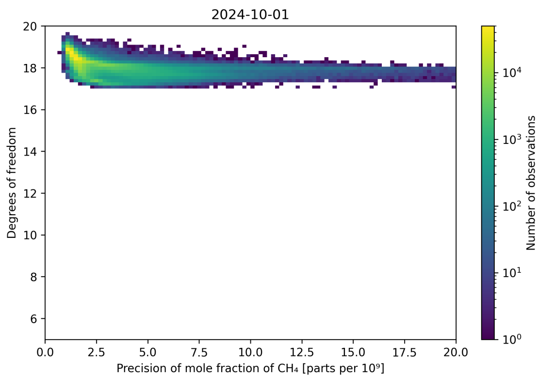
Figure 80: Scatter density plot of “Precision of mole fraction of CH 4 ” against “Degrees of freedom” for 2024-09-30 to 2024-10-02.
