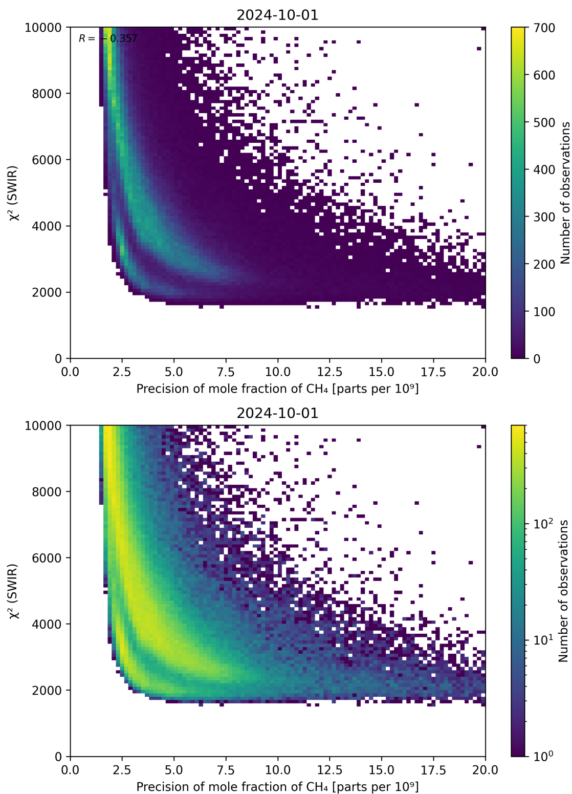
Figure 79: Scatter density plot of “Precision of mole fraction of \text{CH}_4 ” against “ \chi^2 (SWIR)” for 2024-09-30 to 2024-10-02.
