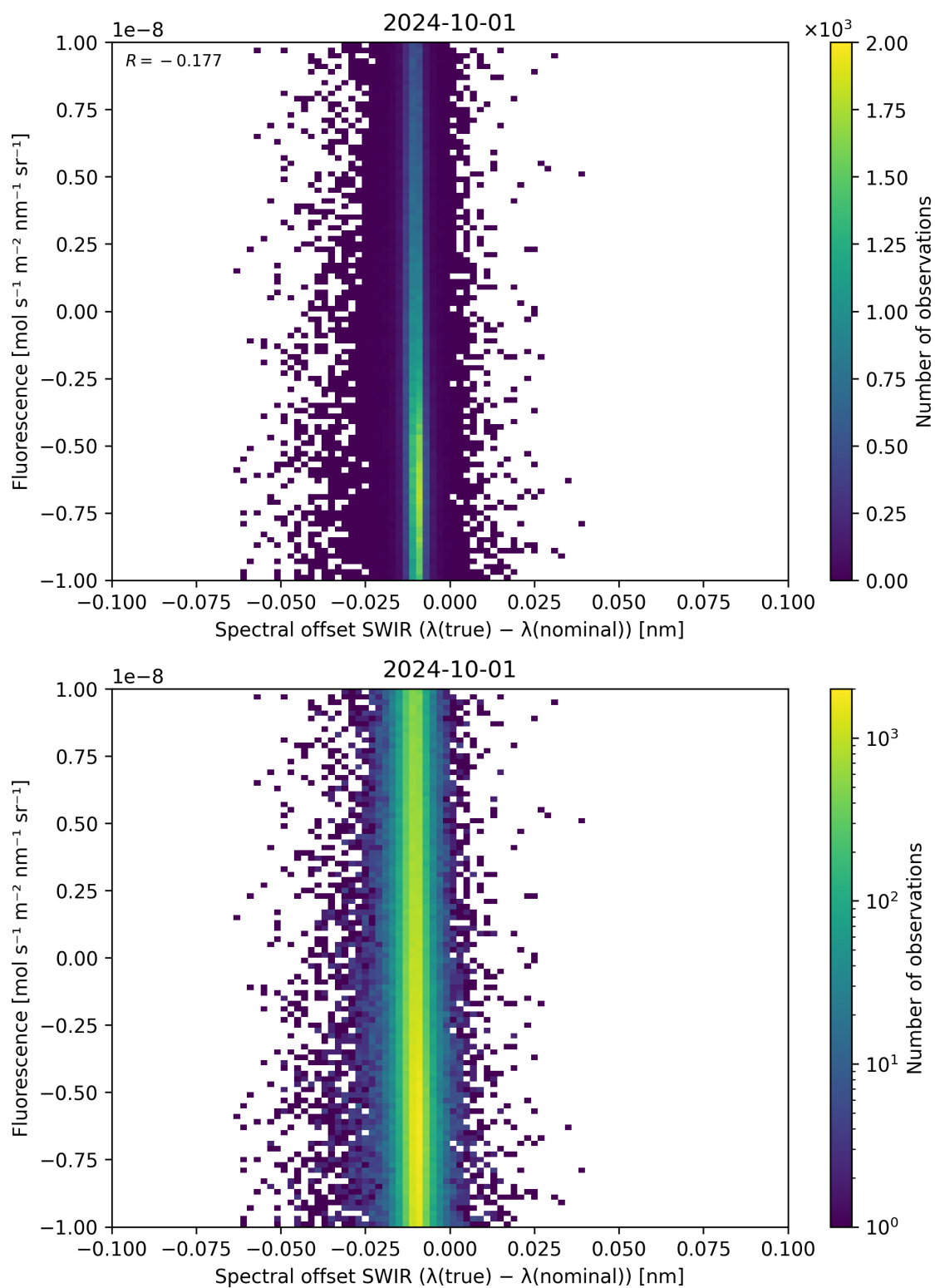
Figure 120: Scatter density plot of “Spectral offset SWIR ( \lambda_{\text{true}} - \lambda_{\text{nominal}} )” against “Fluorescence” for 2024-09-30 to 2024-10-02.
