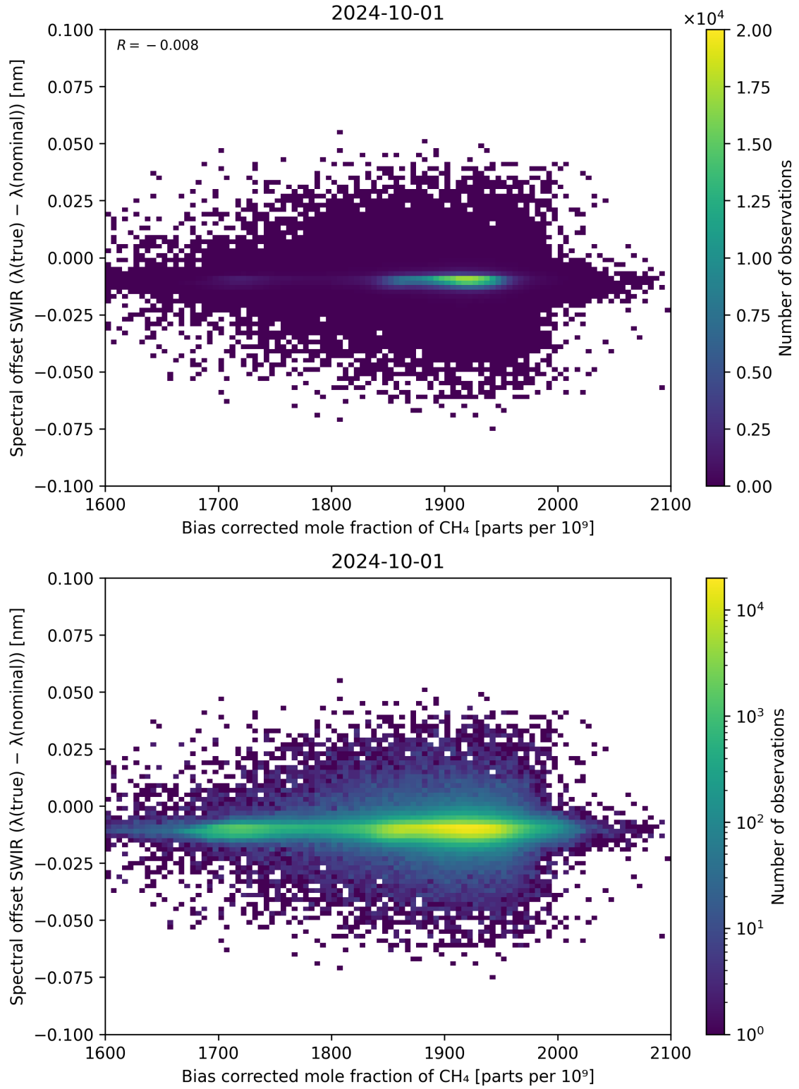
Figure 69: Scatter density plot of “Bias corrected mole fraction of \text{CH}_4 ” against “Spectral offset SWIR ( \lambda_{\text{true}} - \lambda_{\text{nominal}} )” for 2024-09-30 to 2024-10-02.
