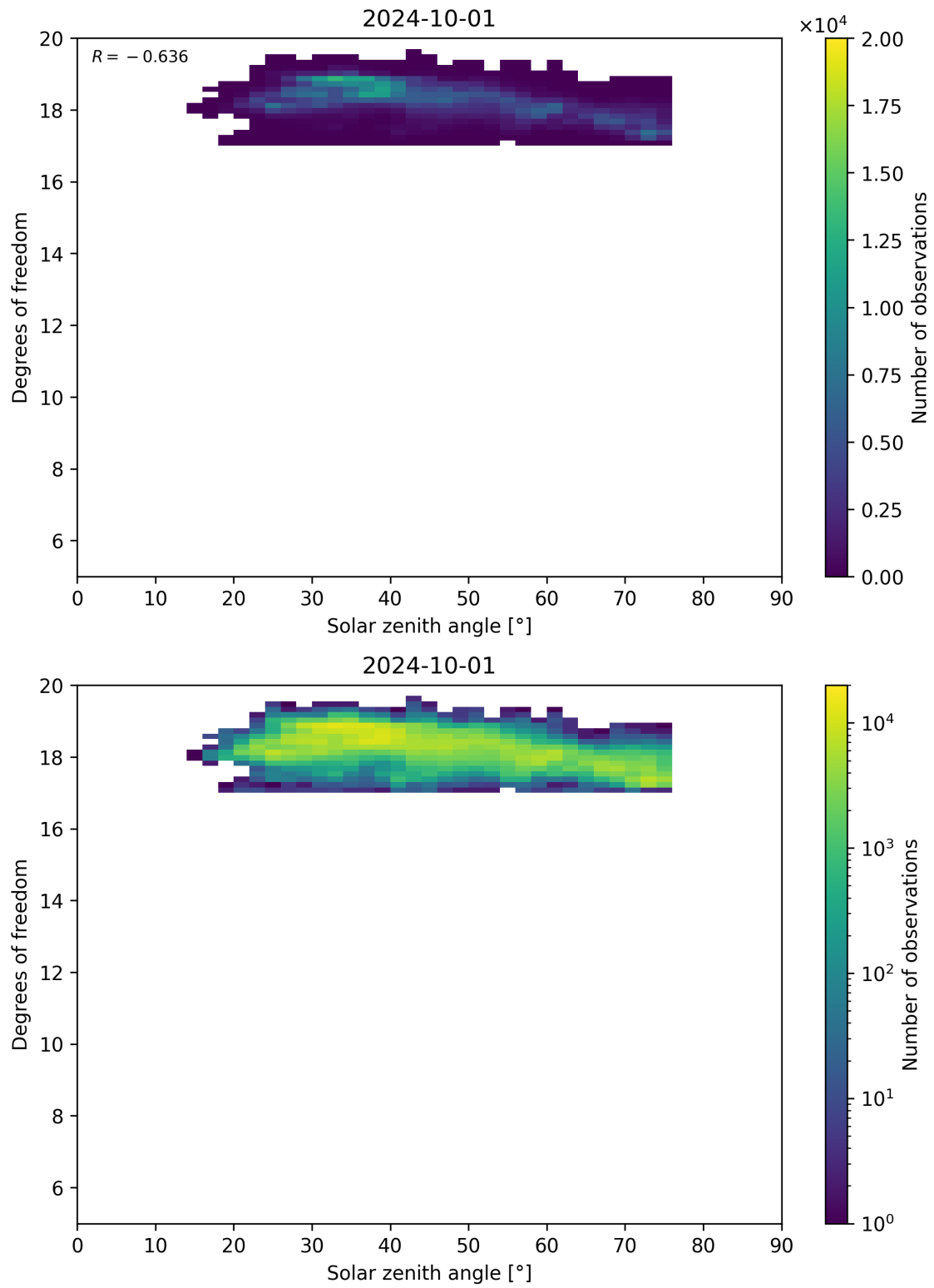
Figure 96: Scatter density plot of “Solar zenith angle” against “Degrees of freedom” for 2024-09-30 to 2024-10-02.
