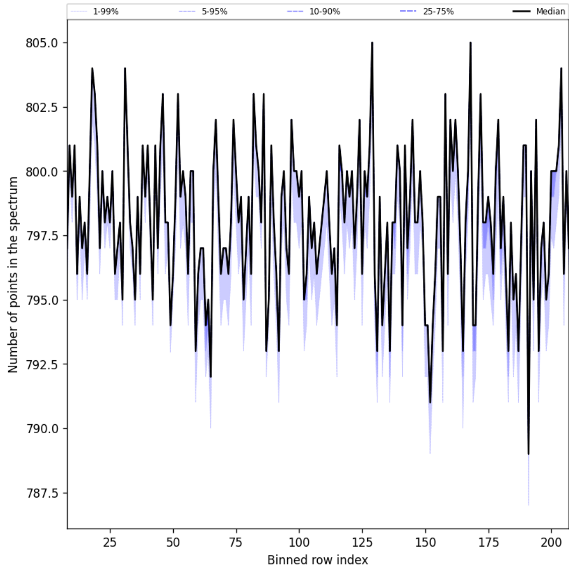
Figure 37: Along track statistics of “Number of points in the spectrum” for 2024-09-30 to 2024-10-02
