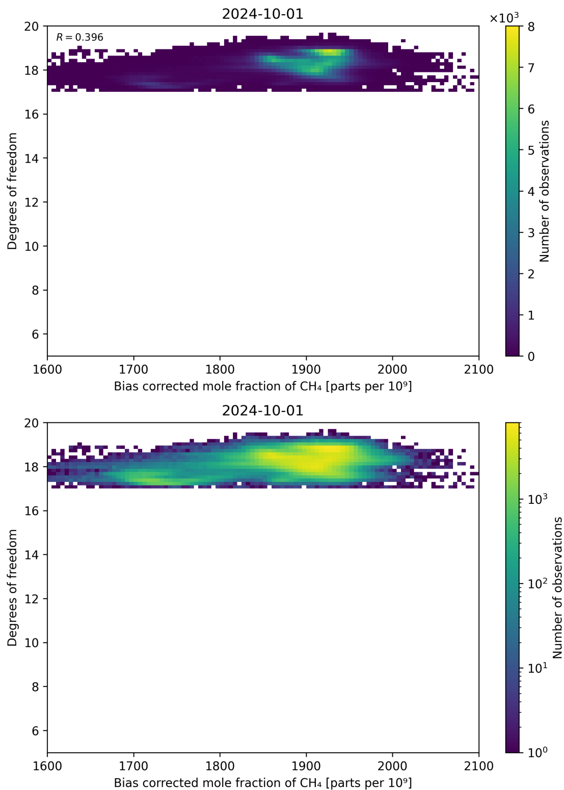
Figure 65: Scatter density plot of “Bias corrected mole fraction of CH 4 ” against “Degrees of freedom” for 2024-09-30 to 2024-10-02.
