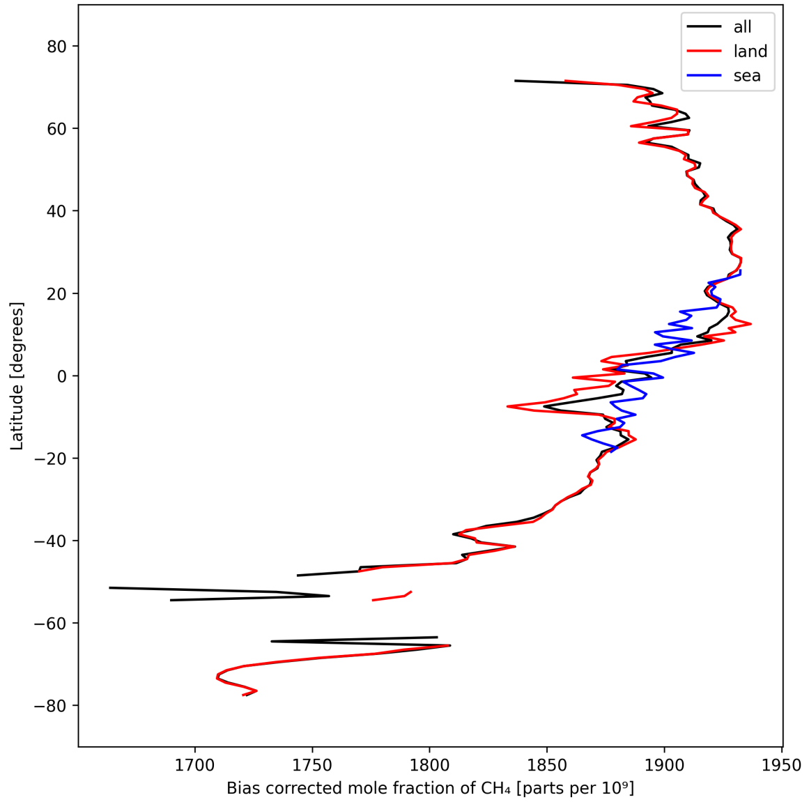
Figure 14: Zonal average of “Bias corrected mole fraction of CH 4 ” for 2024-09-30 to 2024-10-02.
