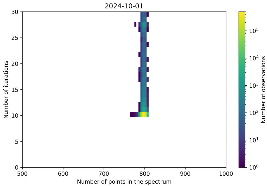
Figure 92: Scatter density plot of “Number of points in the spectrum” against “Number of iterations” for 2024-09-30 to 2024-10-02.
