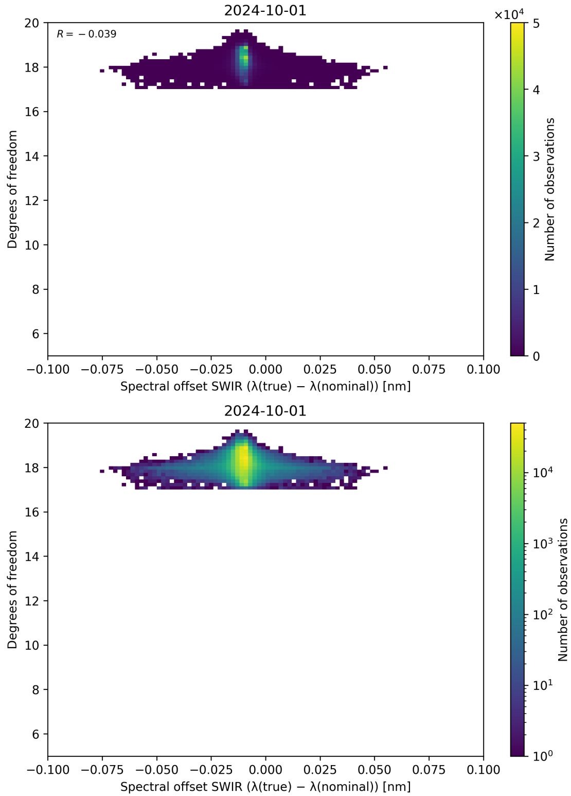
Figure 119: Scatter density plot of “Spectral offset SWIR ( \lambda_{\text{true}} - \lambda_{\text{nominal}} )” against “Degrees of freedom” for 2024-09-30 to 2024-10-02.
