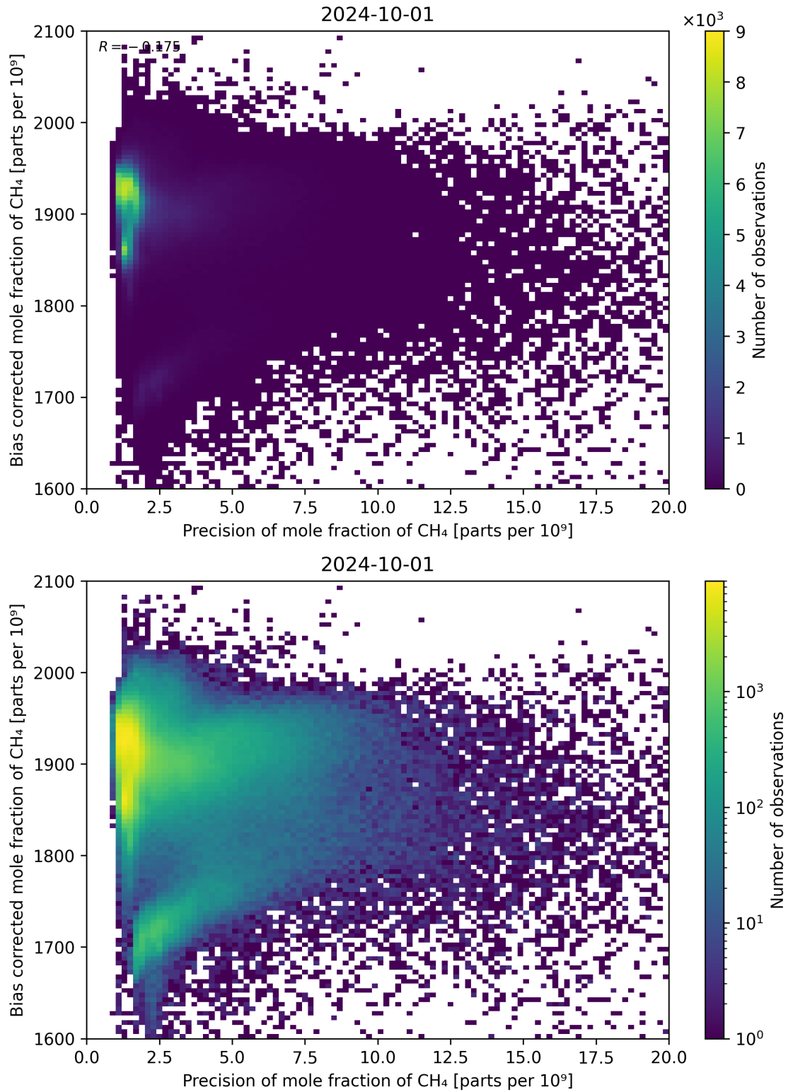
Figure 82: Scatter density plot of “Precision of mole fraction of CH 4 ” against “Bias corrected mole fraction of CH 4 ” for 2024-09-30 to 2024-10-02.
