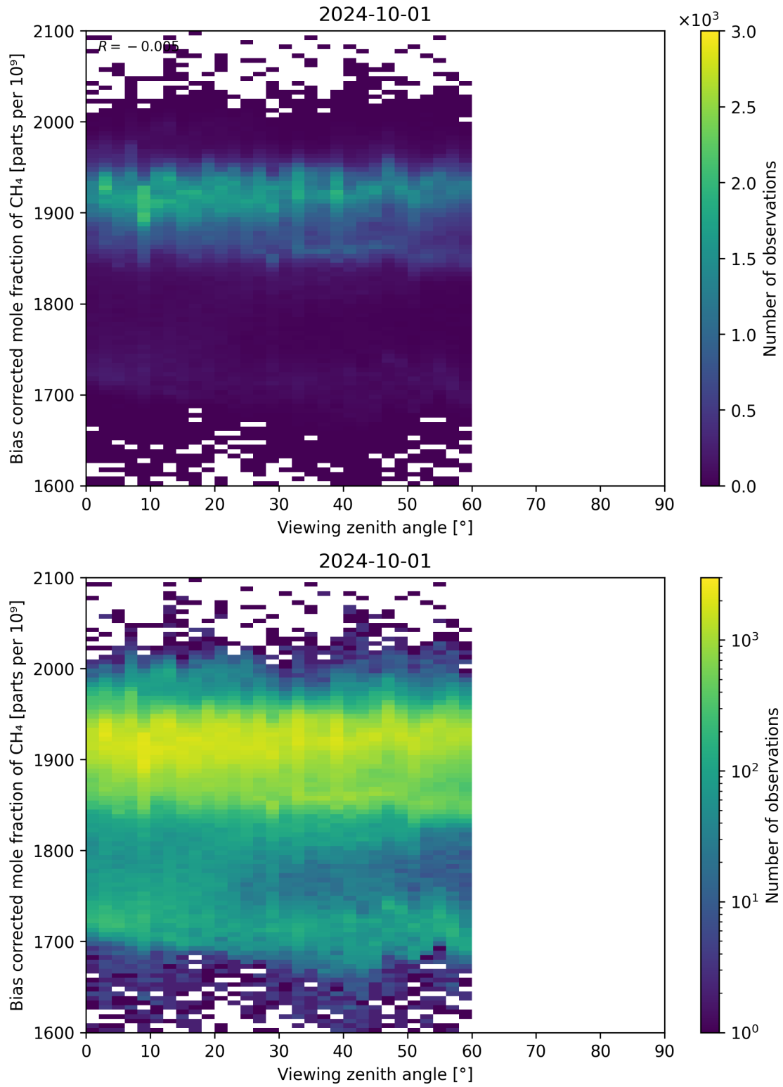
Figure 111: Scatter density plot of “Viewing zenith angle” against “Bias corrected mole fraction of CH 4 ” for 2024-09-30 to 2024-10-02.
