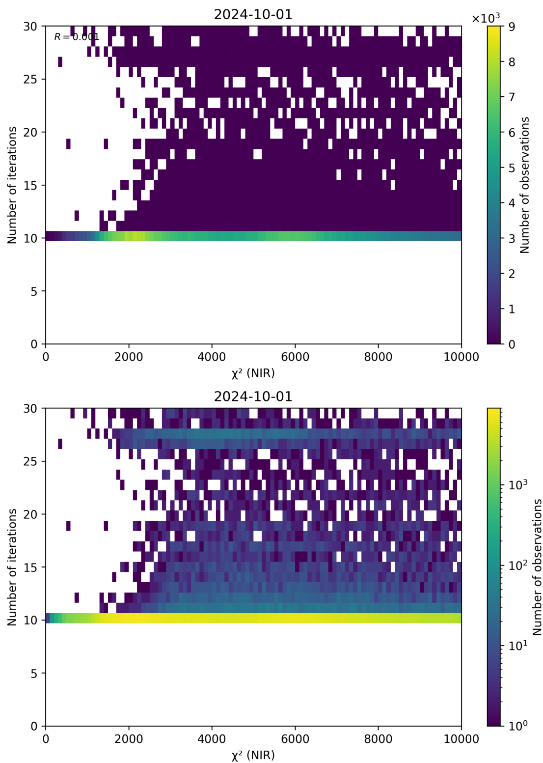
Figure 46: Scatter density plot of " \chi^2 (NIR)" against "Number of iterations" for 2024-09-30 to 2024-10-02.
