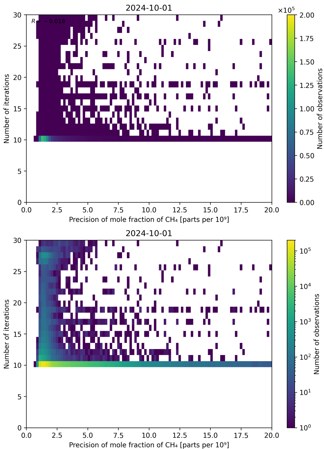
Figure 83: Scatter density plot of “Precision of mole fraction of CH 4 ” against “Number of iterations” for 2024-09-30 to 2024-10-02.
