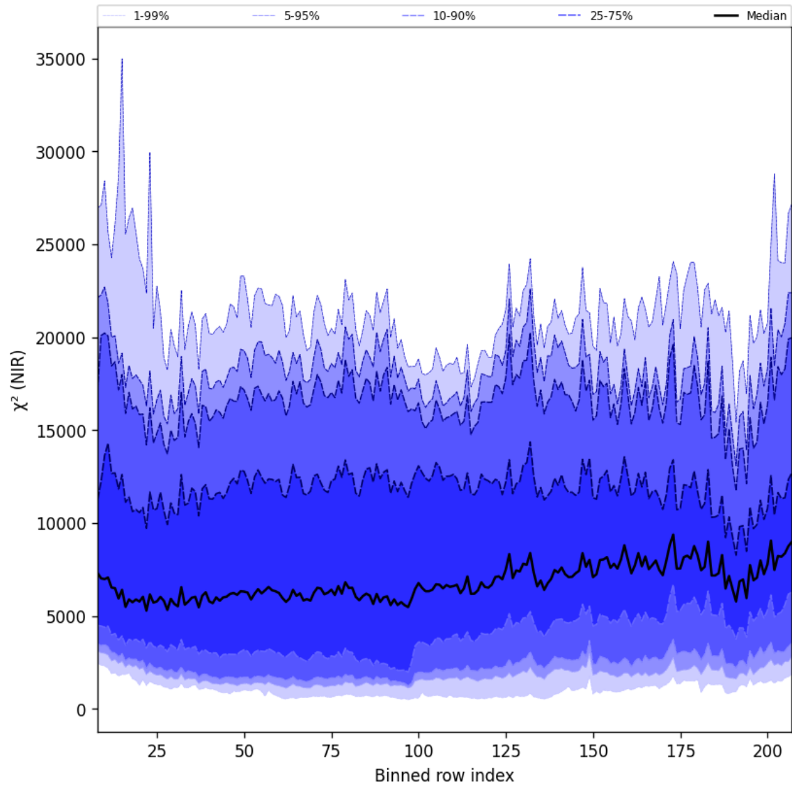
Figure 40: Along track statistics of “ \chi^2 (NIR)” for 2024-09-30 to 2024-10-02
