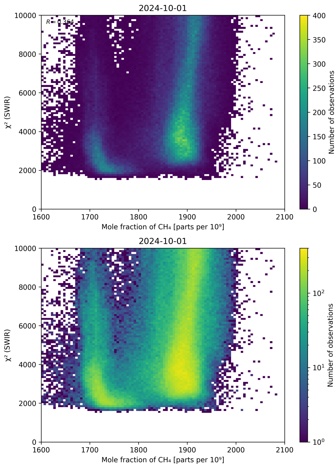
Figure 71: Scatter density plot of “Mole fraction of \text{CH}_4 ” against “ \chi^2 (SWIR)” for 2024-09-30 to 2024-10-02.
