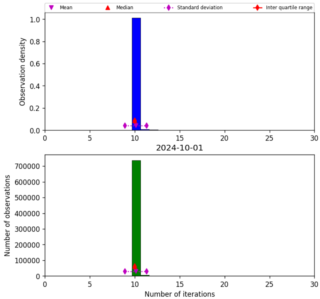
Figure 31: Histogram of “Number of iterations” for 2024-09-30 to 2024-10-02
