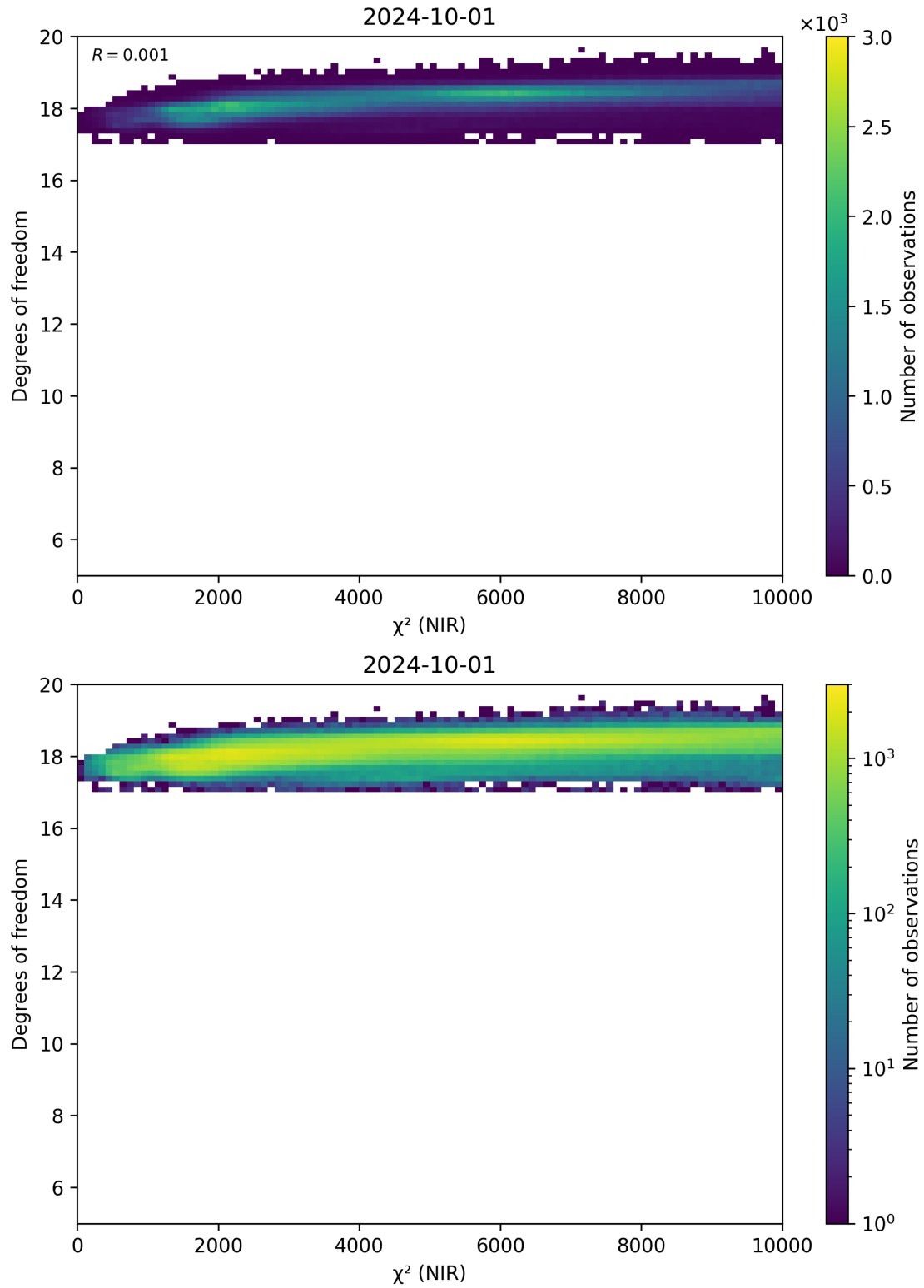
Figure 44: Scatter density plot of “ \chi^2 (NIR)” against “Degrees of freedom” for 2024-09-30 to 2024-10-02.
