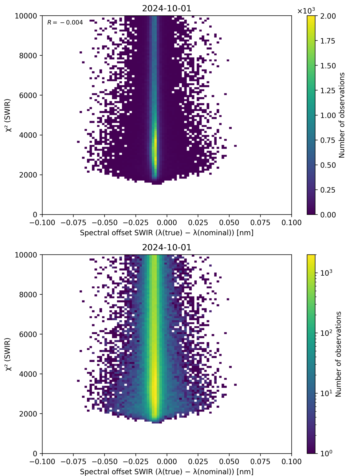
Figure 118: Scatter density plot of “Spectral offset SWIR ( \lambda_{\text{true}} - \lambda_{\text{nominal}} )” against “ \chi^2 (SWIR)” for 2024-09-30 to 2024-10-02.
