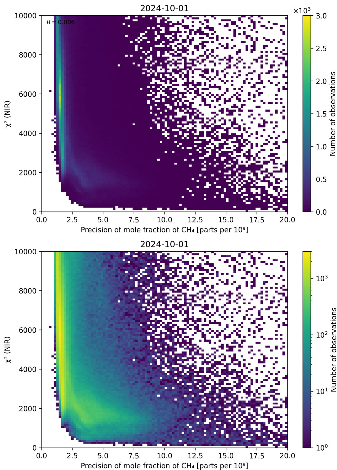
Figure 78: Scatter density plot of “Precision of mole fraction of CH 4 ” against “ \chi^2 (NIR)” for 2024-09-30 to 2024-10-02.
