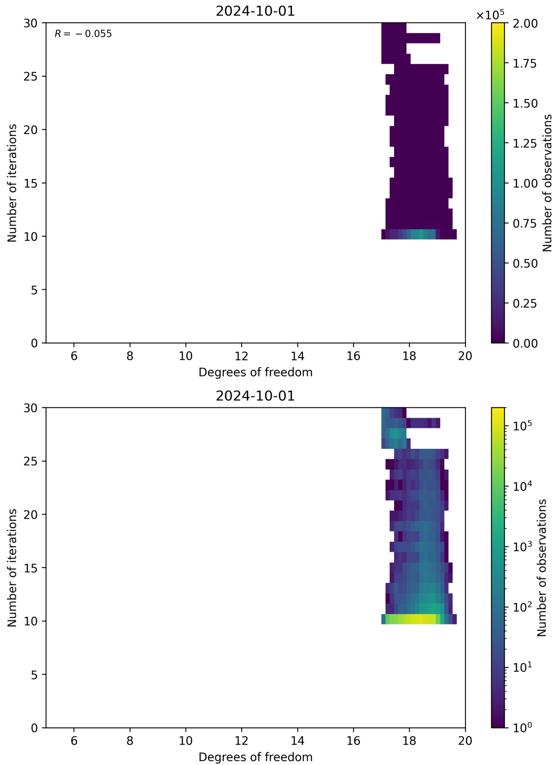
Figure 52: Scatter density plot of “Degrees of freedom” against “Number of iterations” for 2024-09-30 to 2024-10-02.
