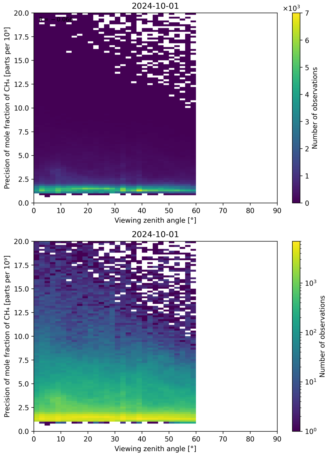
Figure 112: Scatter density plot of “Viewing zenith angle” against “Precision of mole fraction of CH 4 ” for 2024-09-30 to 2024-10-02.
