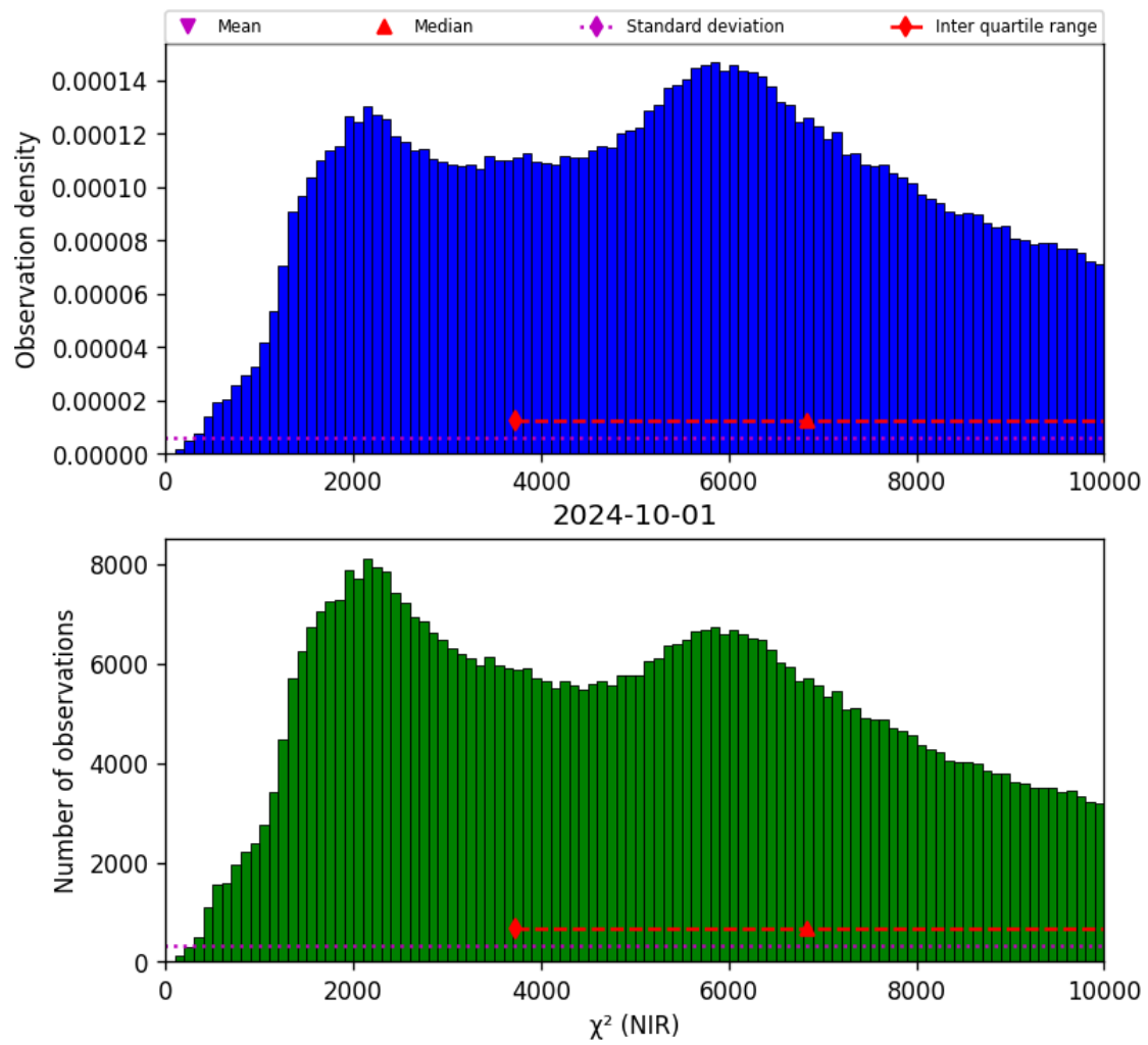
Figure 29: Histogram of “ \chi^2 (NIR)” for 2024-09-30 to 2024-10-02
