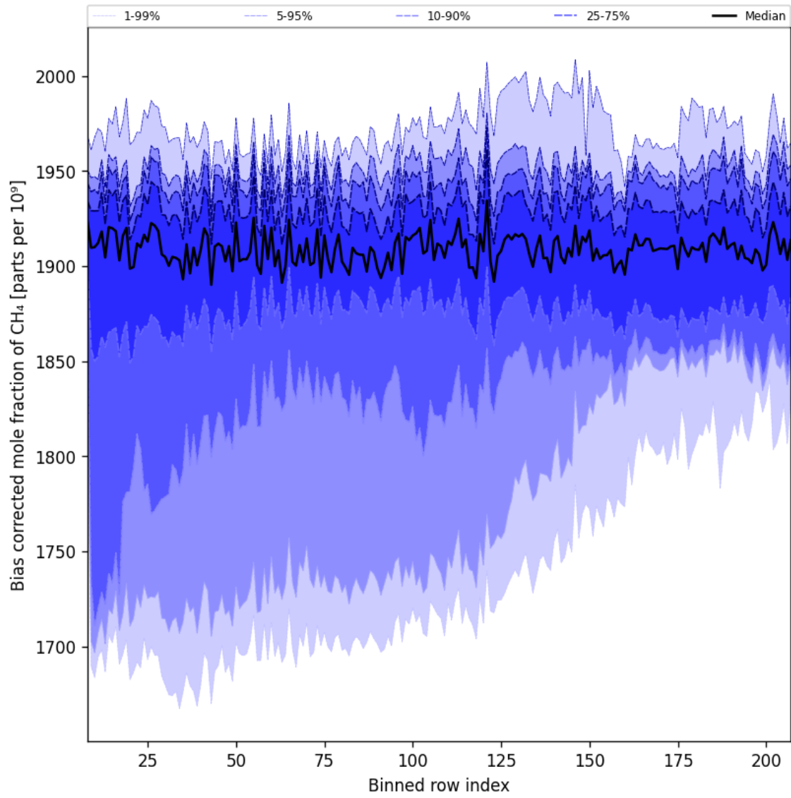
Figure 36: Along track statistics of “Bias corrected mole fraction of CH 4 ” for 2024-09-30 to 2024-10-02
