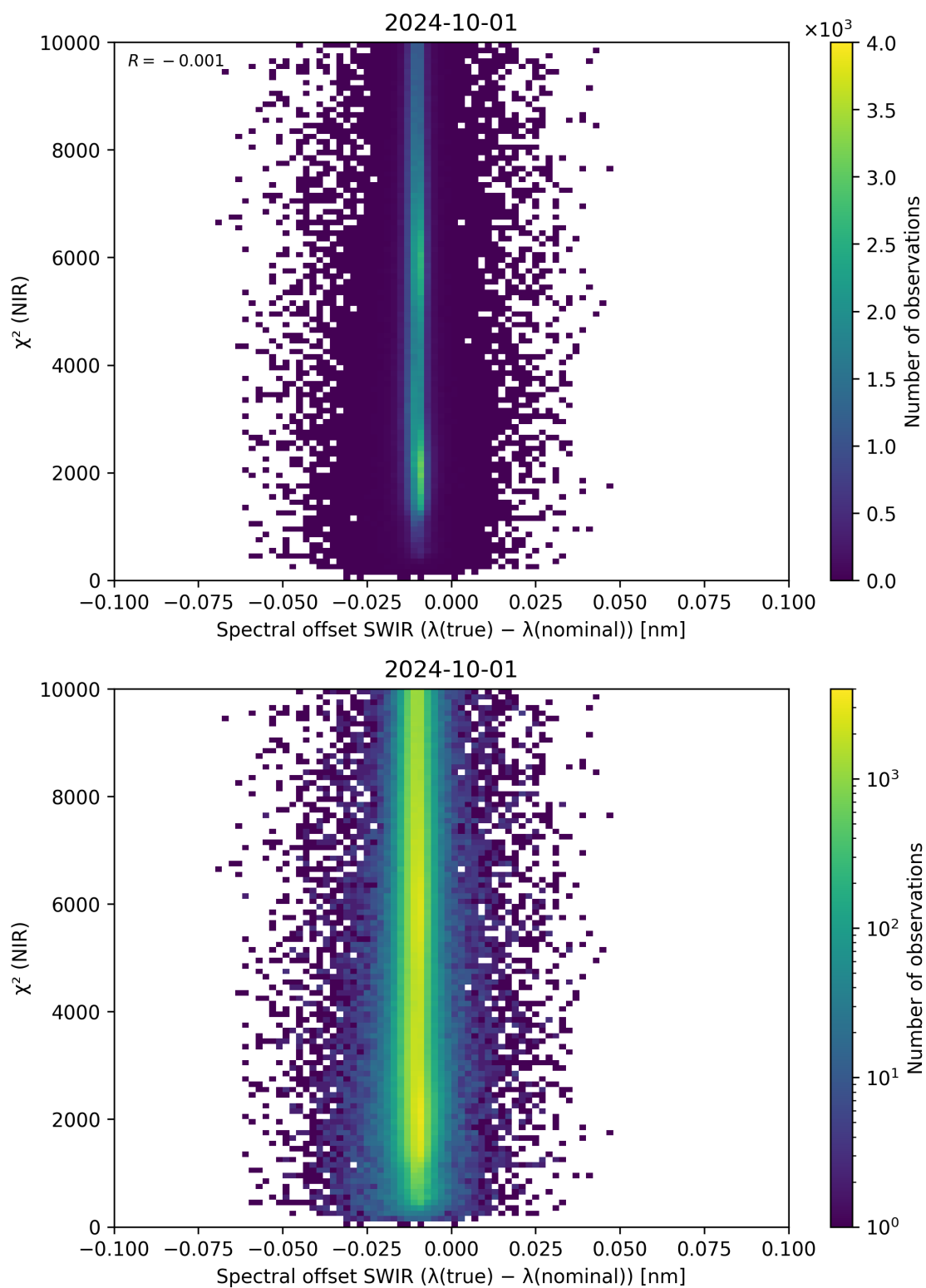
Figure 117: Scatter density plot of “Spectral offset SWIR ( \lambda_{\text{true}} - \lambda_{\text{nominal}} )” against “ \chi^2 (NIR)” for 2024-09-30 to 2024-10-02.
