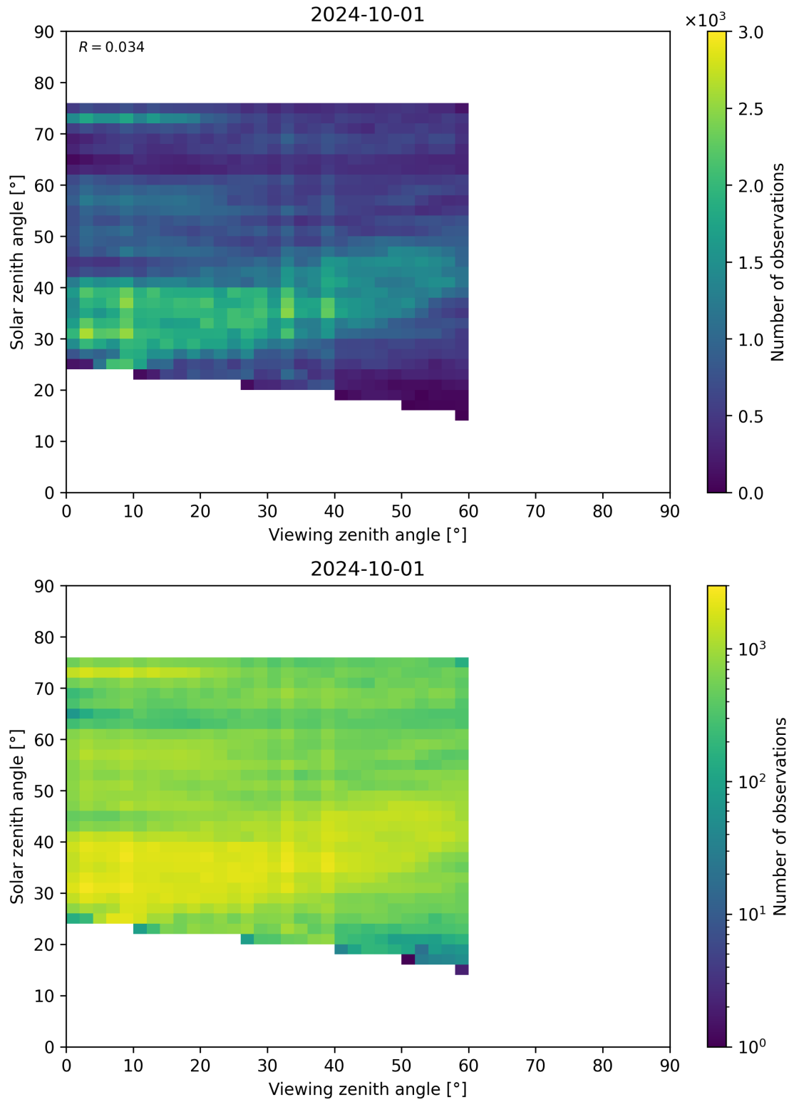
Figure 115: Scatter density plot of “Viewing zenith angle” against “Solar zenith angle” for 2024-09-30 to 2024-10-02.
