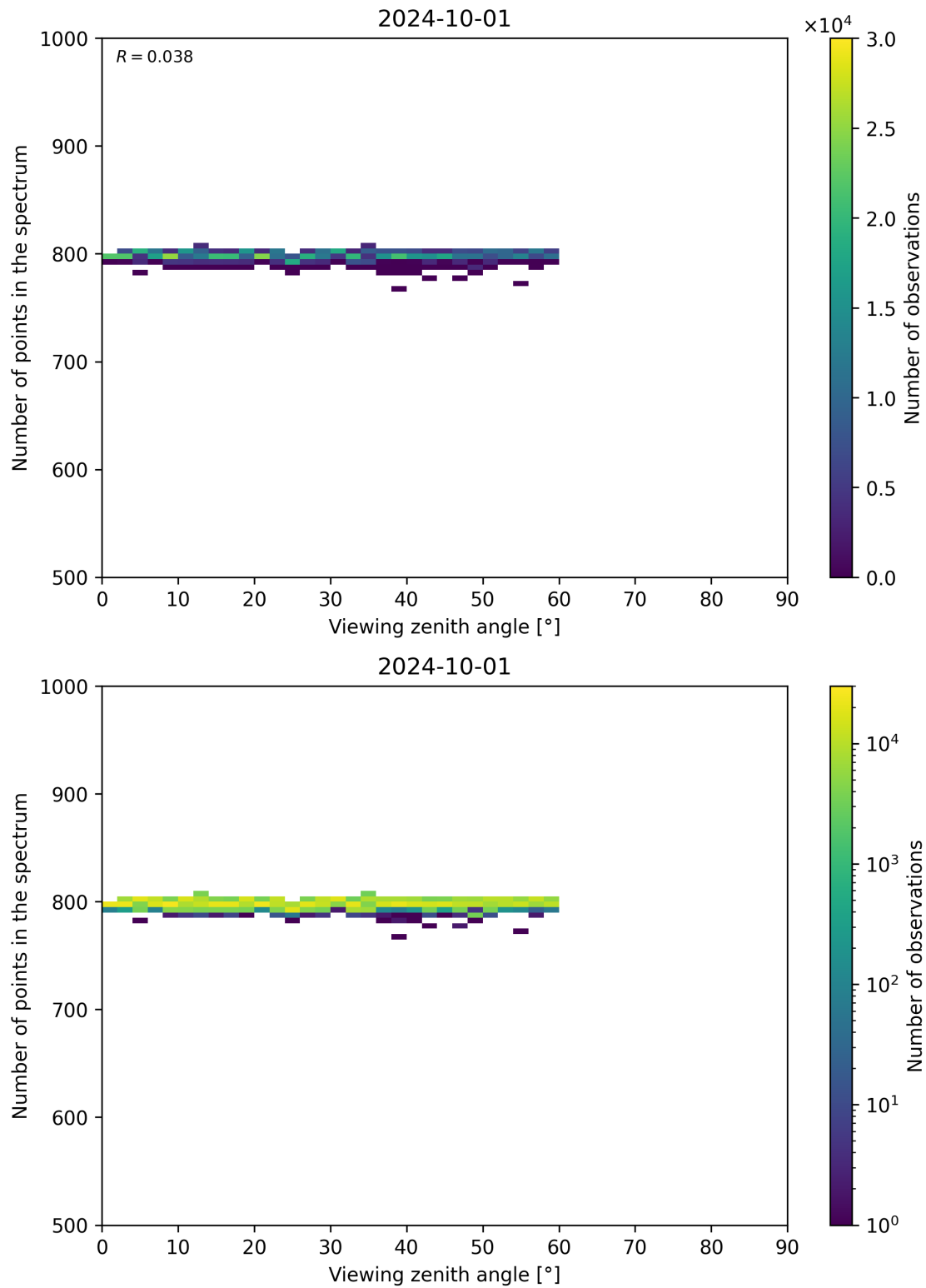
Figure 114: Scatter density plot of “Viewing zenith angle” against “Number of points in the spectrum” for 2024-09-30 to 2024-10-02.
