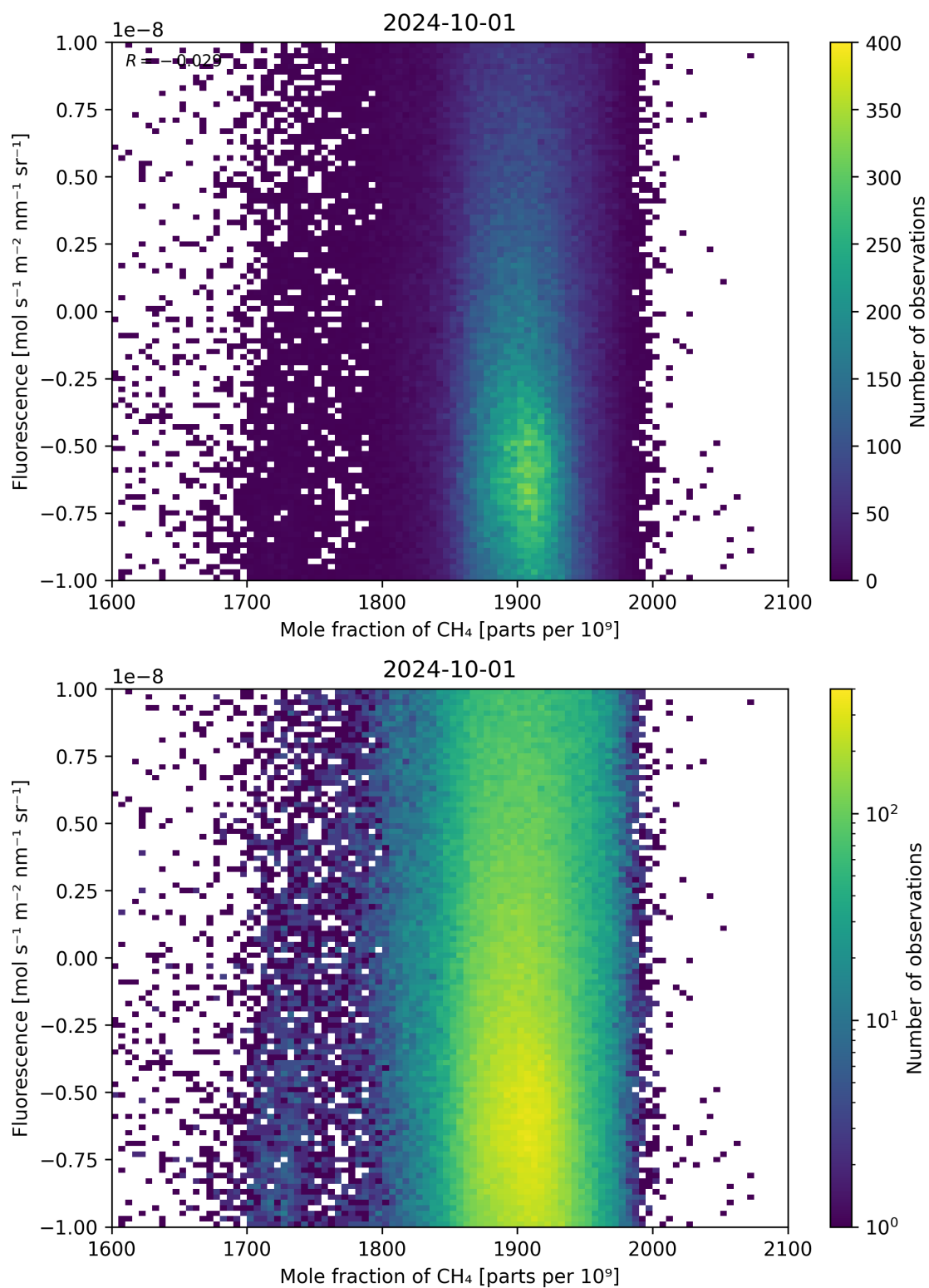
Figure 73: Scatter density plot of “Mole fraction of CH 4 ” against “Fluorescence” for 2024-09-30 to 2024-10-02.
