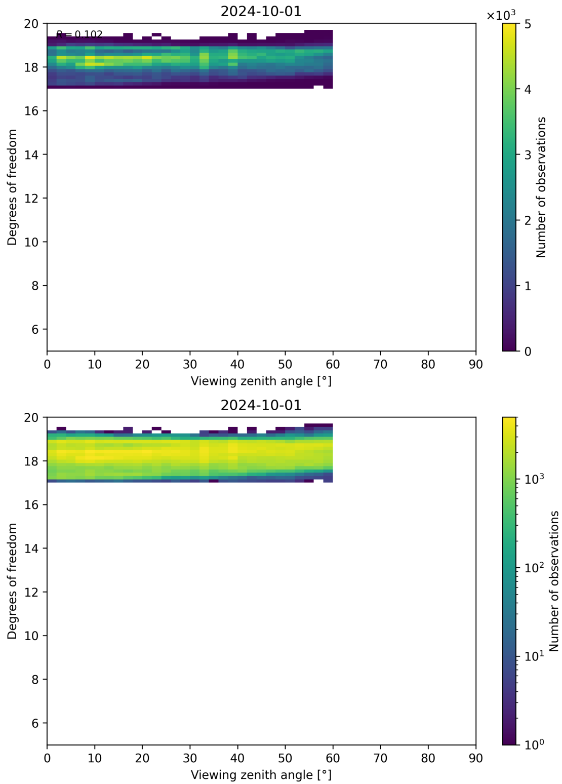
Figure 107: Scatter density plot of “Viewing zenith angle” against “Degrees of freedom” for 2024-09-30 to 2024-10-02.
