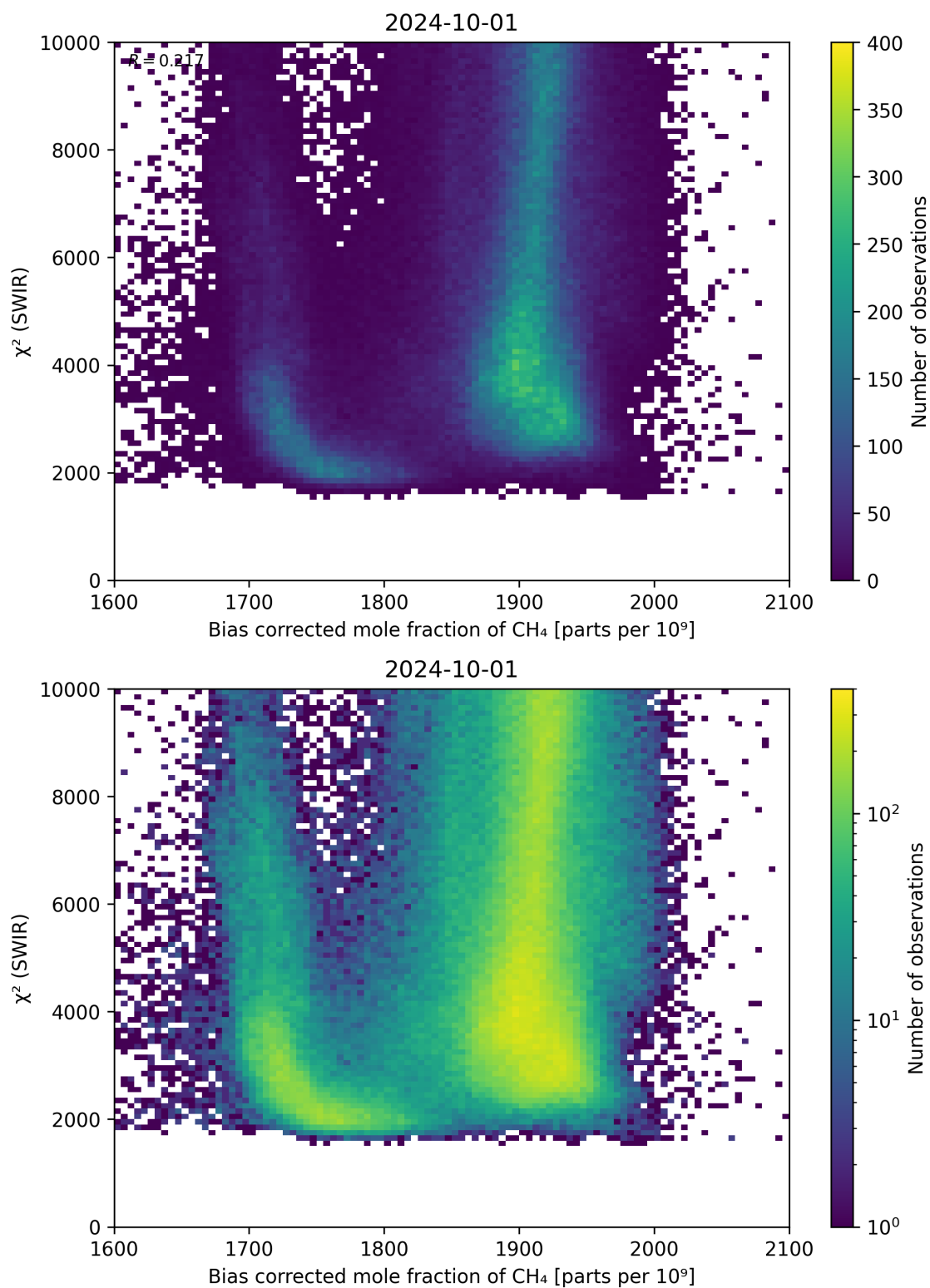
Figure 64: Scatter density plot of “Bias corrected mole fraction of \text{CH}_4 ” against “ \chi^2 (SWIR)” for 2024-09-30 to 2024-10-02.
