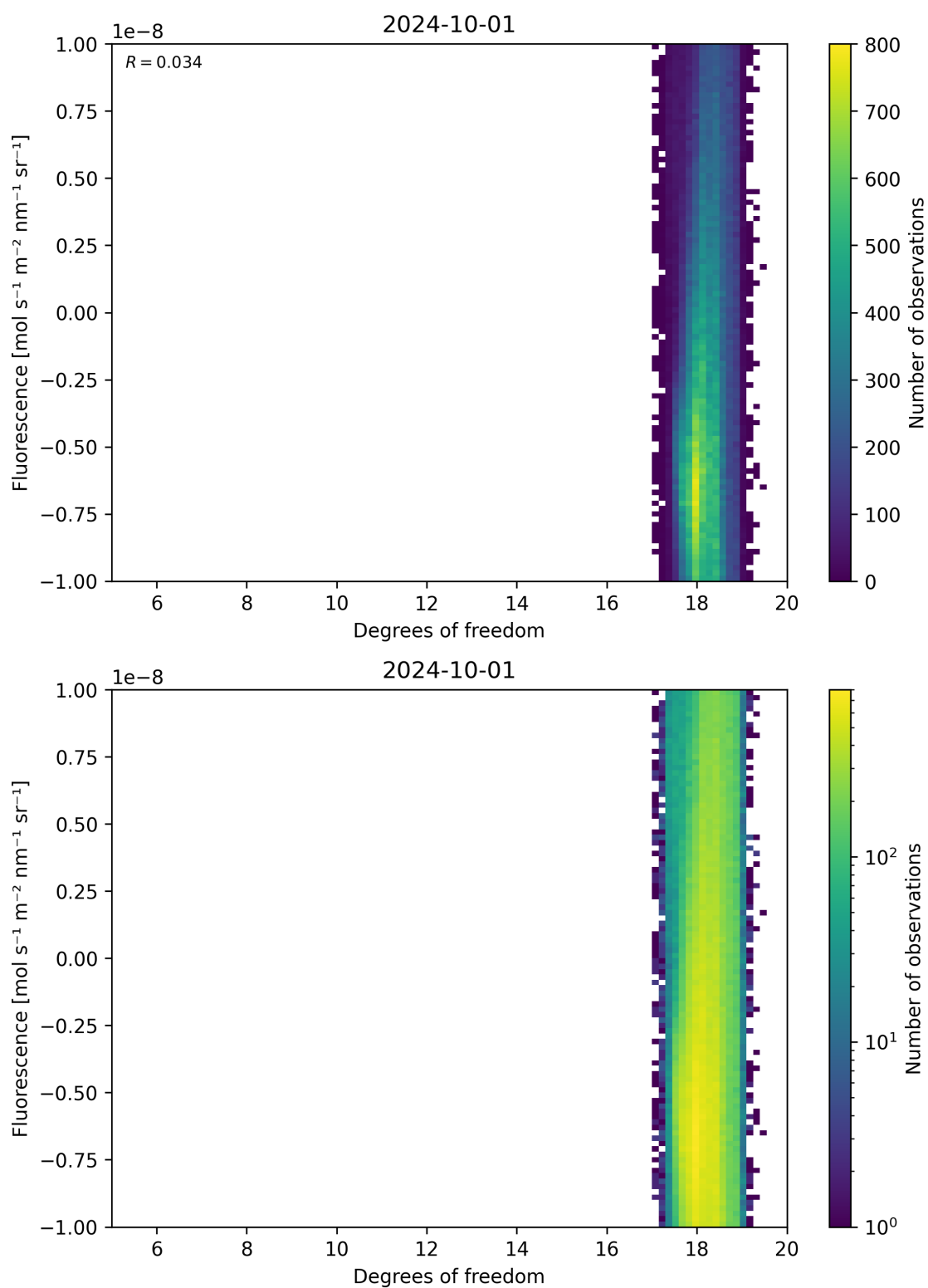
Figure 51: Scatter density plot of “Degrees of freedom” against “Fluorescence” for 2024-09-30 to 2024-10-02.
