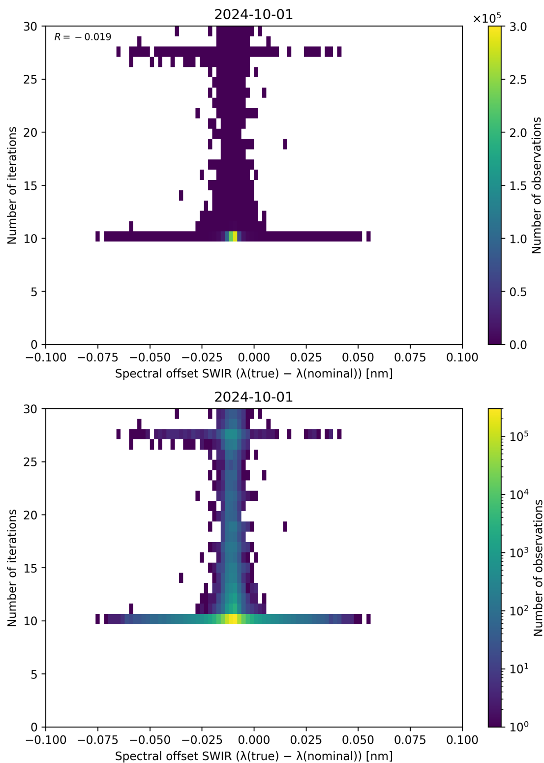
Figure 121: Scatter density plot of “Spectral offset SWIR ( \lambda_{\text{true}} - \lambda_{\text{nominal}} )” against “Number of iterations” for 2024-09-30 to 2024-10-02.
