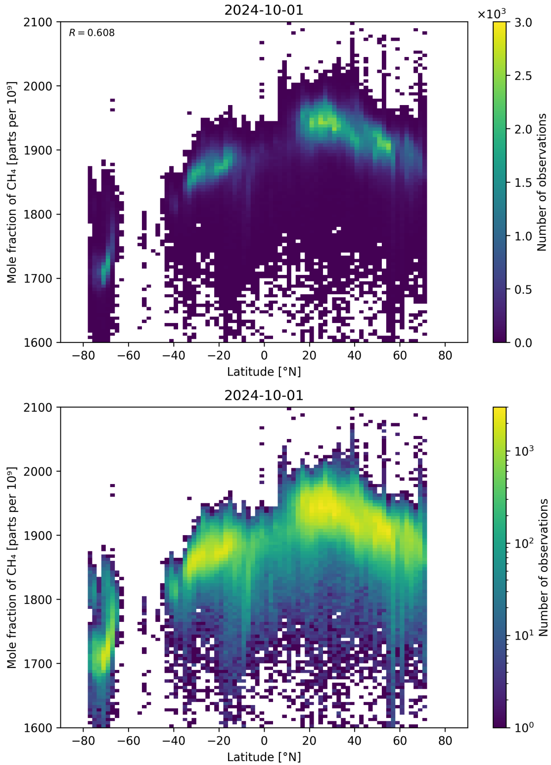
Figure 57: Scatter density plot of “Latitude” against “Mole fraction of \text{CH}_4 ” for 2024-09-30 to 2024-10-02.
