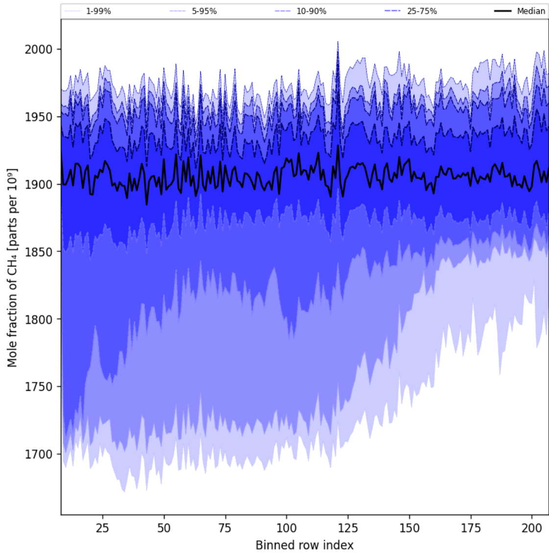
Figure 34: Along track statistics of “Mole fraction of CH 4 ” for 2024-09-30 to 2024-10-02
