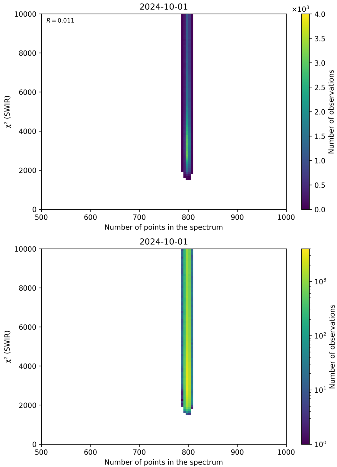
Figure 89: Scatter density plot of “Number of points in the spectrum” against “ \chi^2 (SWIR)” for 2024-09-30 to 2024-10-02.
