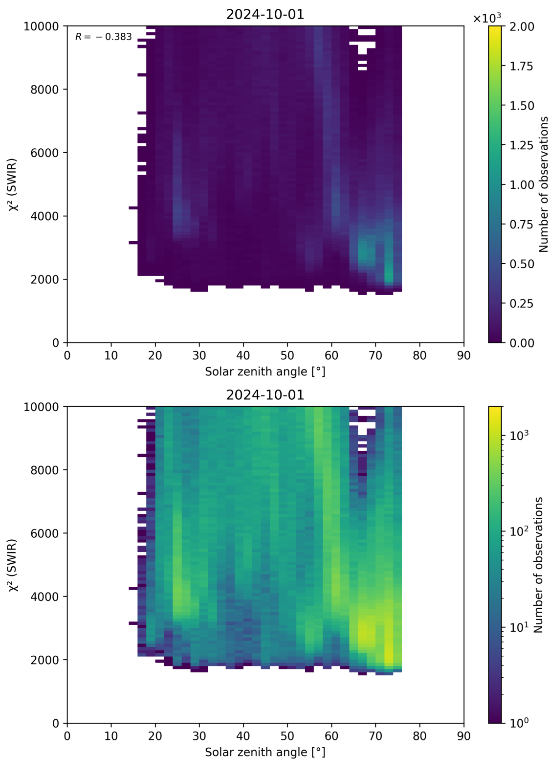
Figure 95: Scatter density plot of “Solar zenith angle” against “ \chi^2 (SWIR)” for 2024-09-30 to 2024-10-02.
