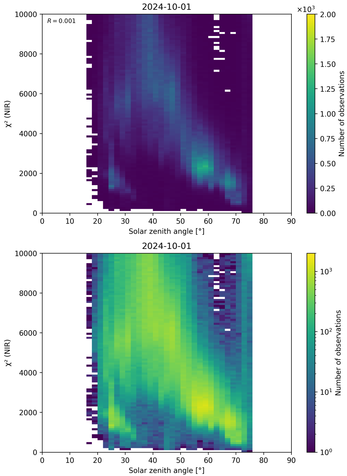
Figure 94: Scatter density plot of “Solar zenith angle” against “ \chi^2 (NIR)” for 2024-09-30 to 2024-10-02.
