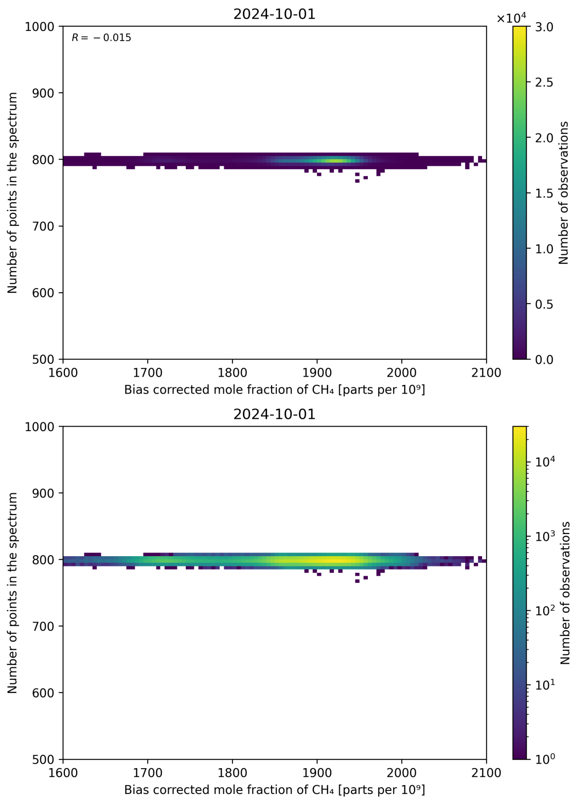
Figure 68: Scatter density plot of “Bias corrected mole fraction of CH 4 ” against “Number of points in the spectrum” for 2024-09-30 to 2024-10-02.
