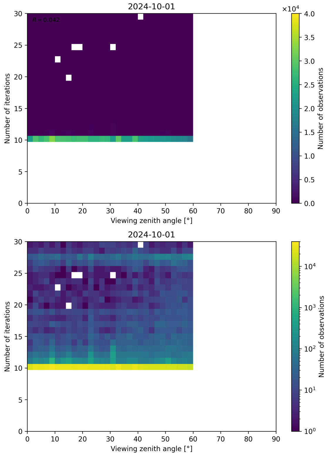
Figure 113: Scatter density plot of “Viewing zenith angle” against “Number of iterations” for 2024-09-30 to 2024-10-02.
