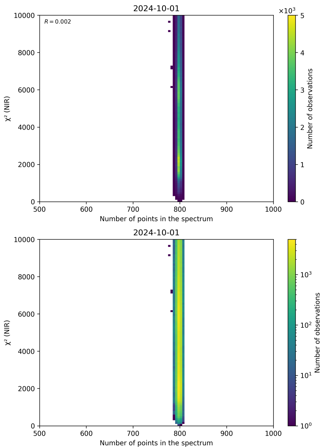
Figure 88: Scatter density plot of “Number of points in the spectrum” against “ \chi^2 (NIR)” for 2024-09-30 to 2024-10-02.
