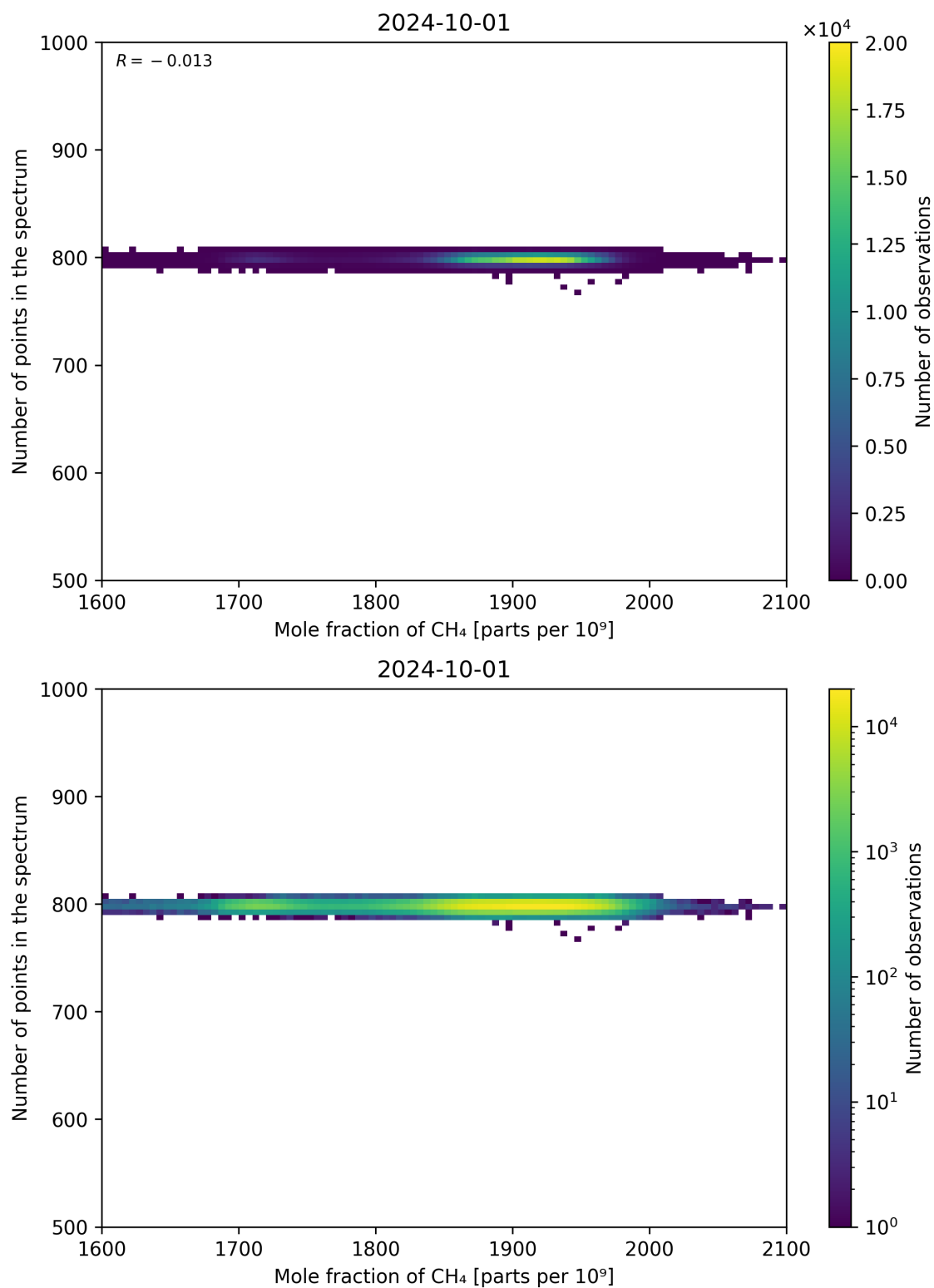
Figure 77: Scatter density plot of “Mole fraction of CH 4 ” against “Number of points in the spectrum” for 2024-09-30 to 2024-10-02.
