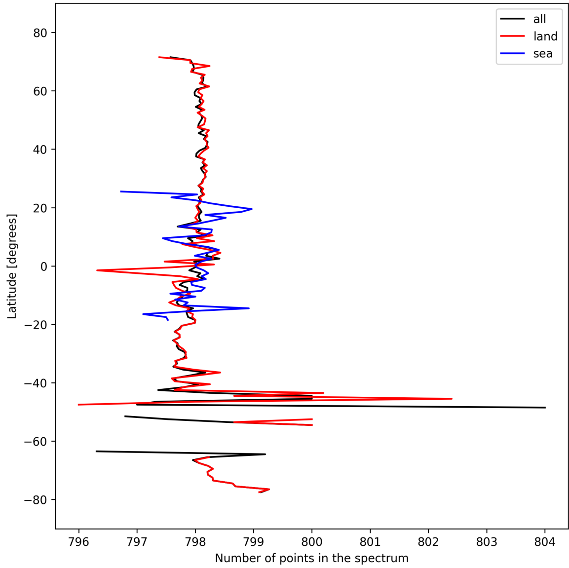
Figure 15: Zonal average of “Number of points in the spectrum” for 2024-09-30 to 2024-10-02.
