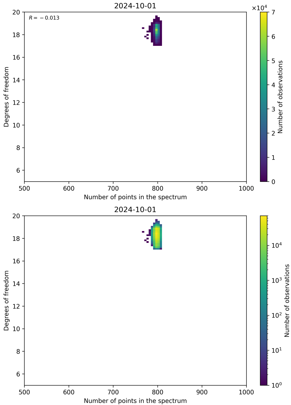
Figure 90: Scatter density plot of “Number of points in the spectrum” against “Degrees of freedom” for 2024-09-30 to 2024-10-02.
