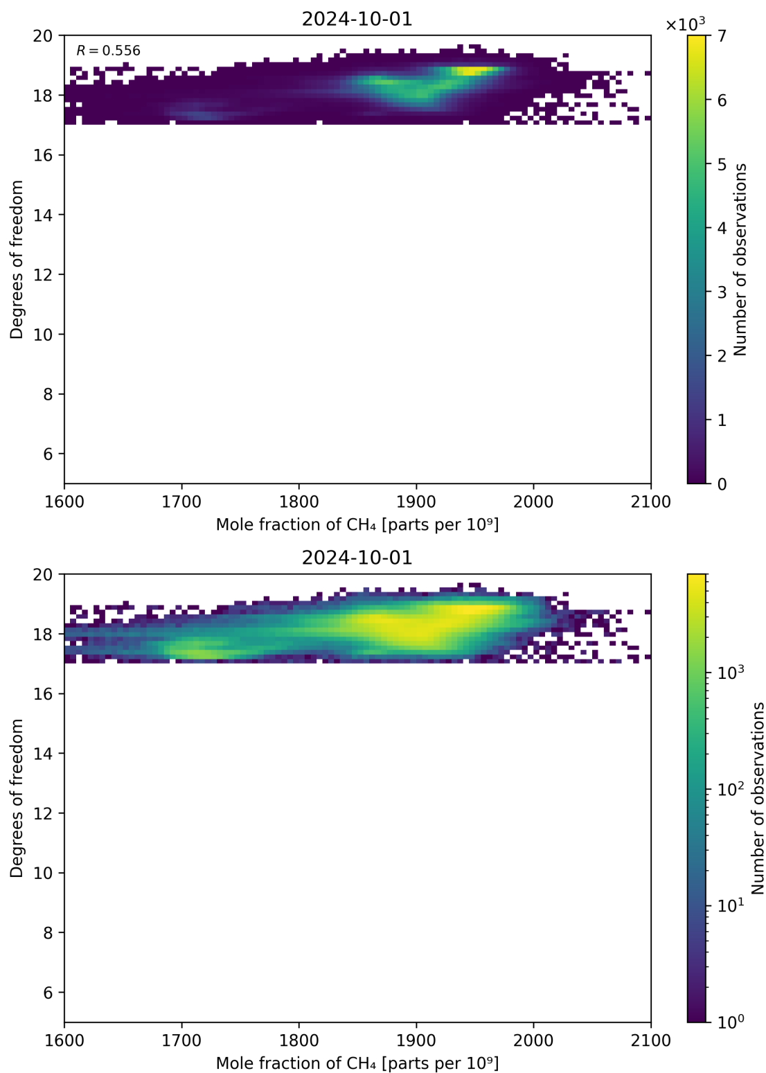
Figure 72: Scatter density plot of “Mole fraction of CH 4 ” against “Degrees of freedom” for 2024-09-30 to 2024-10-02.
