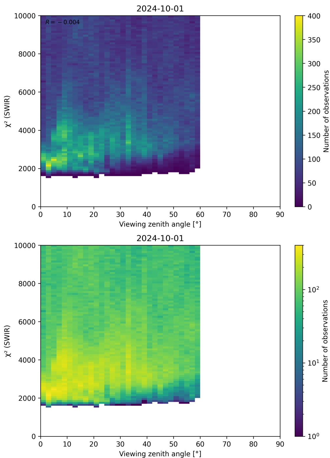
Figure 106: Scatter density plot of “Viewing zenith angle” against “ \chi^2 (SWIR)” for 2024-09-30 to 2024-10-02.
