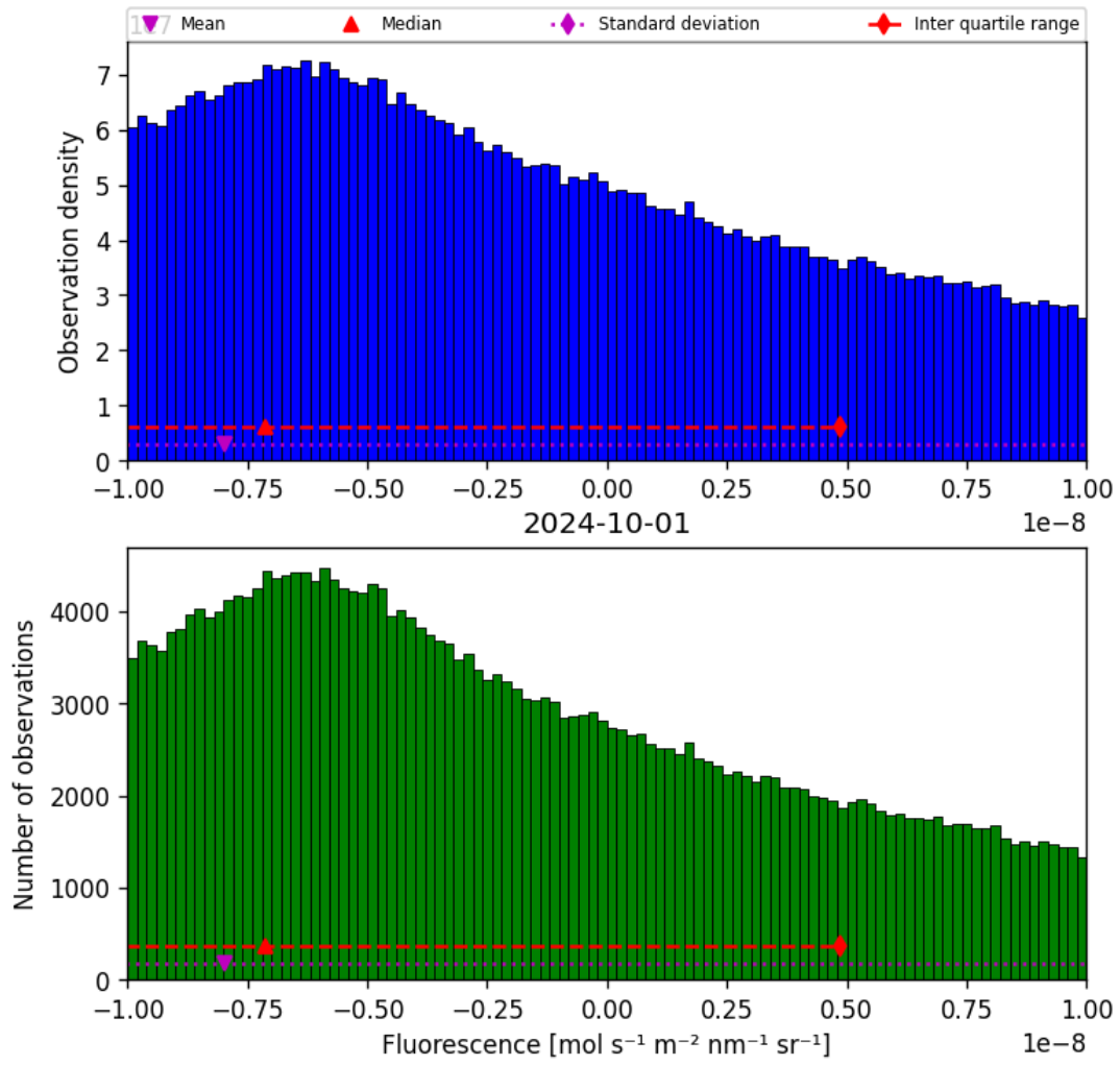
Figure 32: Histogram of “Fluorescence” for 2024-09-30 to 2024-10-02
