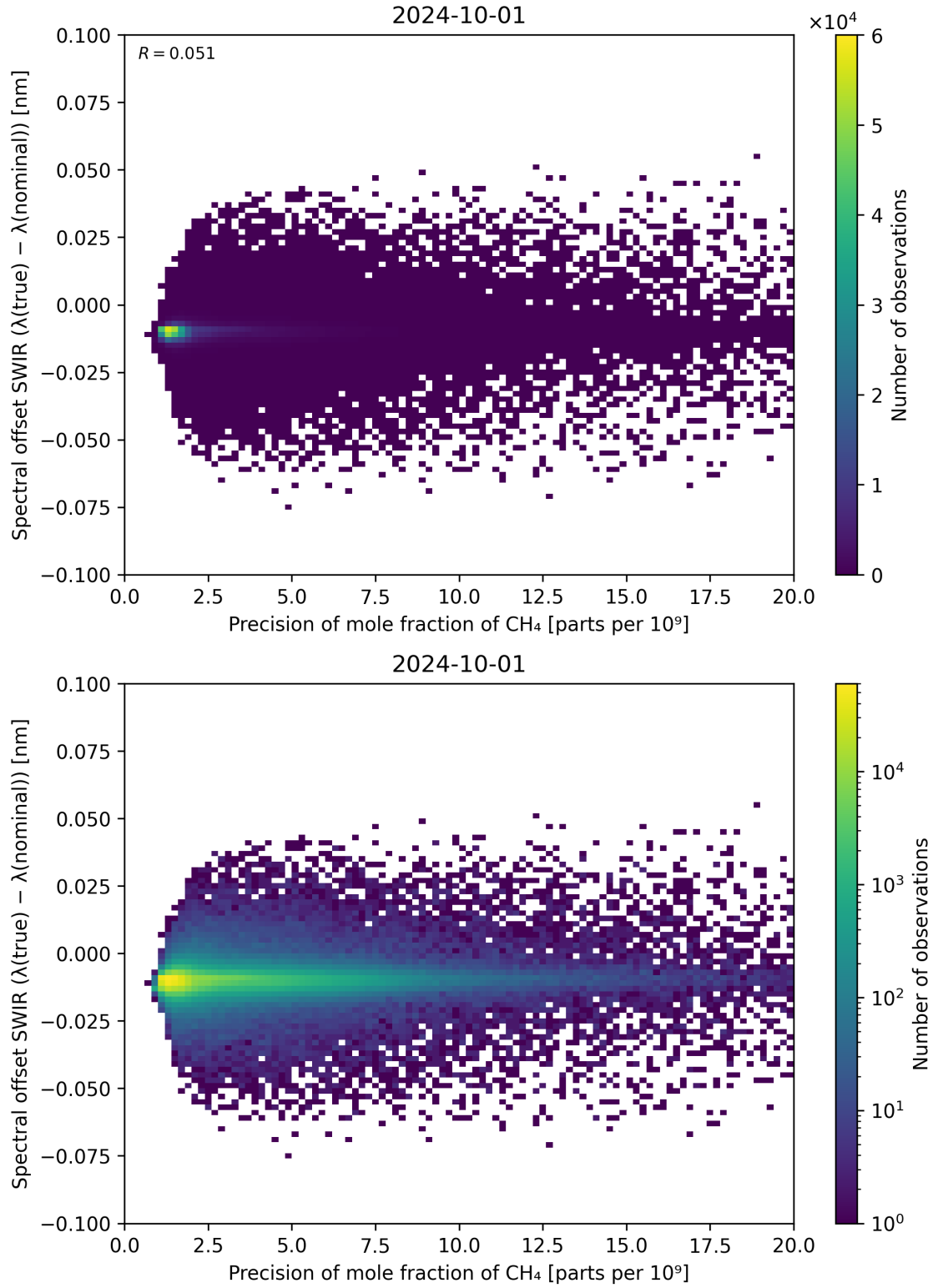
Figure 85: Scatter density plot of “Precision of mole fraction of CH 4 ” against “Spectral offset SWIR ( \lambda_{\text{true}} - \lambda_{\text{nominal}} )” for 2024-09-30 to 2024-10-02.
