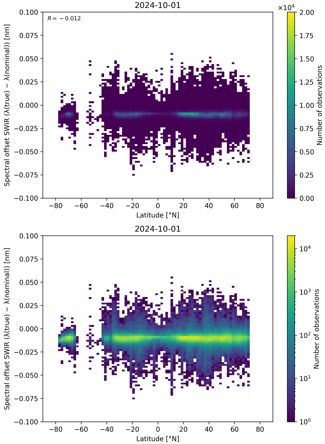
Figure 62: Scatter density plot of “Latitude” against “Spectral offset SWIR ( \lambda_{\text{true}} - \lambda_{\text{nominal}} )” for 2024-09-30 to 2024-10-02.
