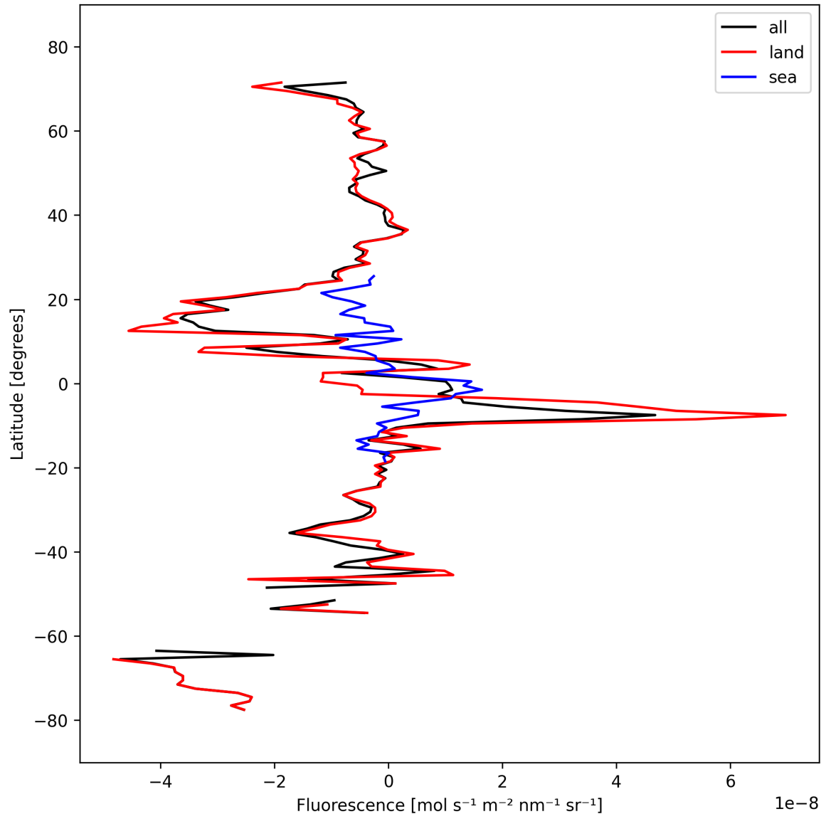
Figure 21: Zonal average of “Fluorescence” for 2024-09-30 to 2024-10-02.
