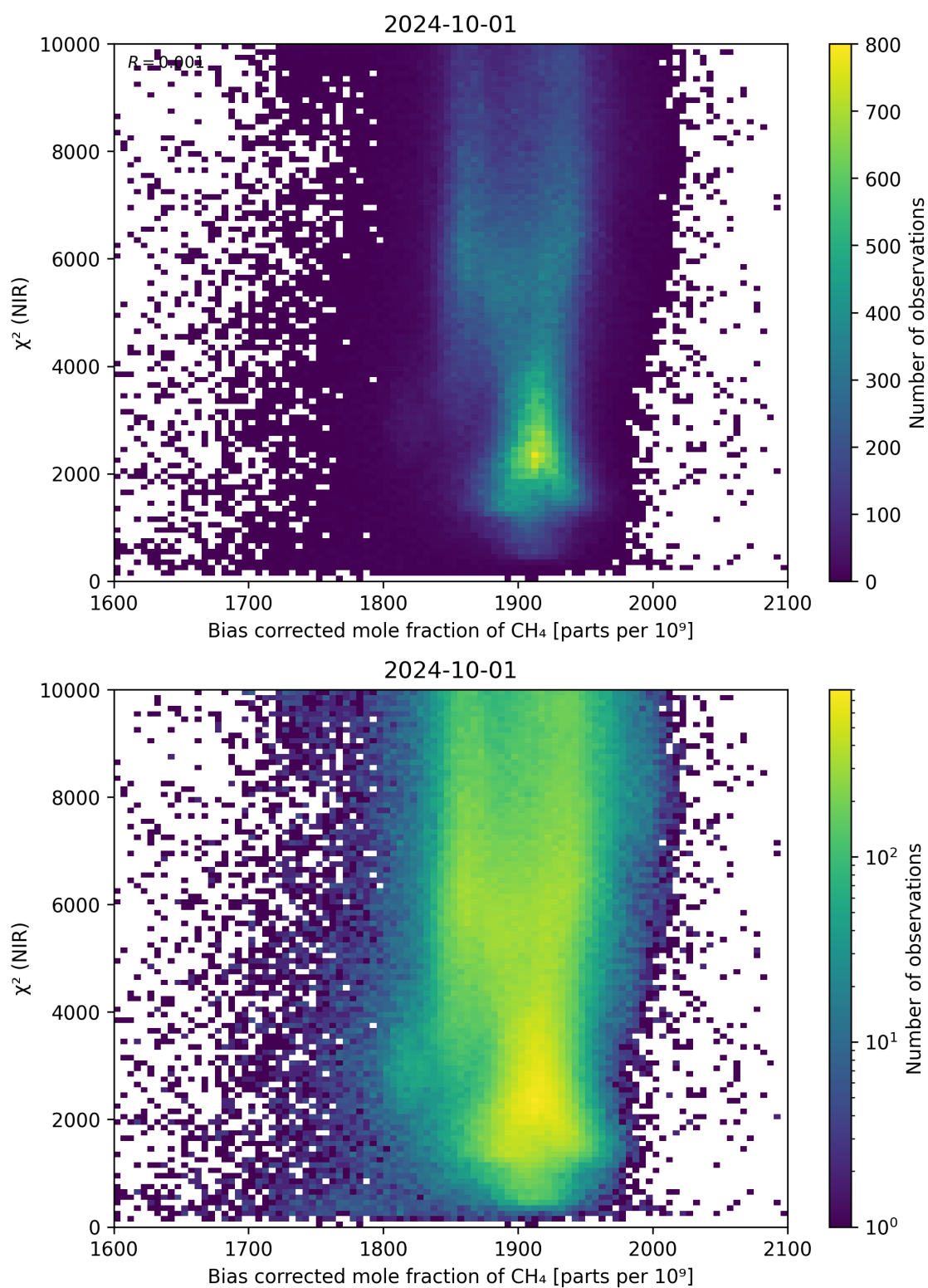
Figure 63: Scatter density plot of “Bias corrected mole fraction of \text{CH}_4 ” against “ \chi^2 (NIR)” for 2024-09-30 to 2024-10-02.
