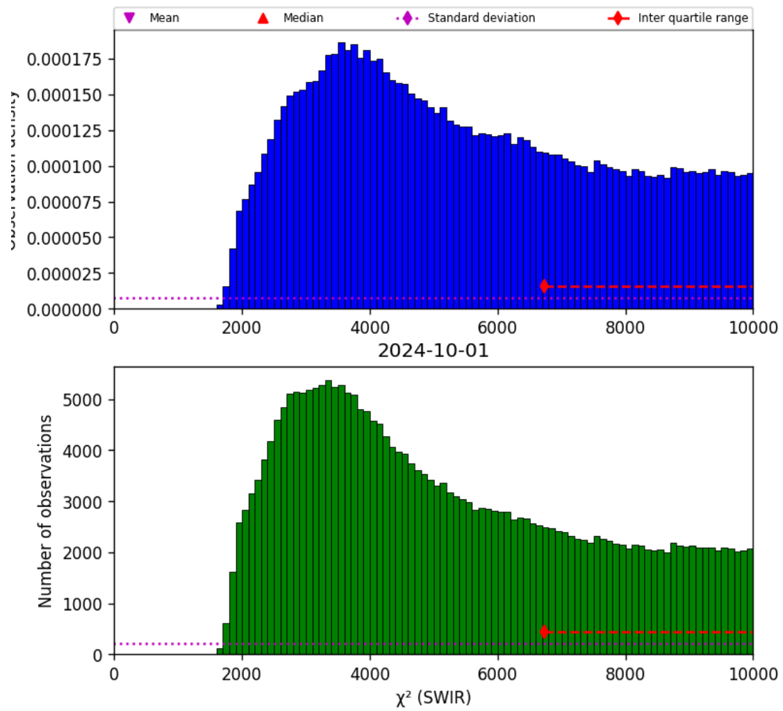
Figure 28: Histogram of “ \chi^2 (SWIR)” for 2024-09-30 to 2024-10-02
