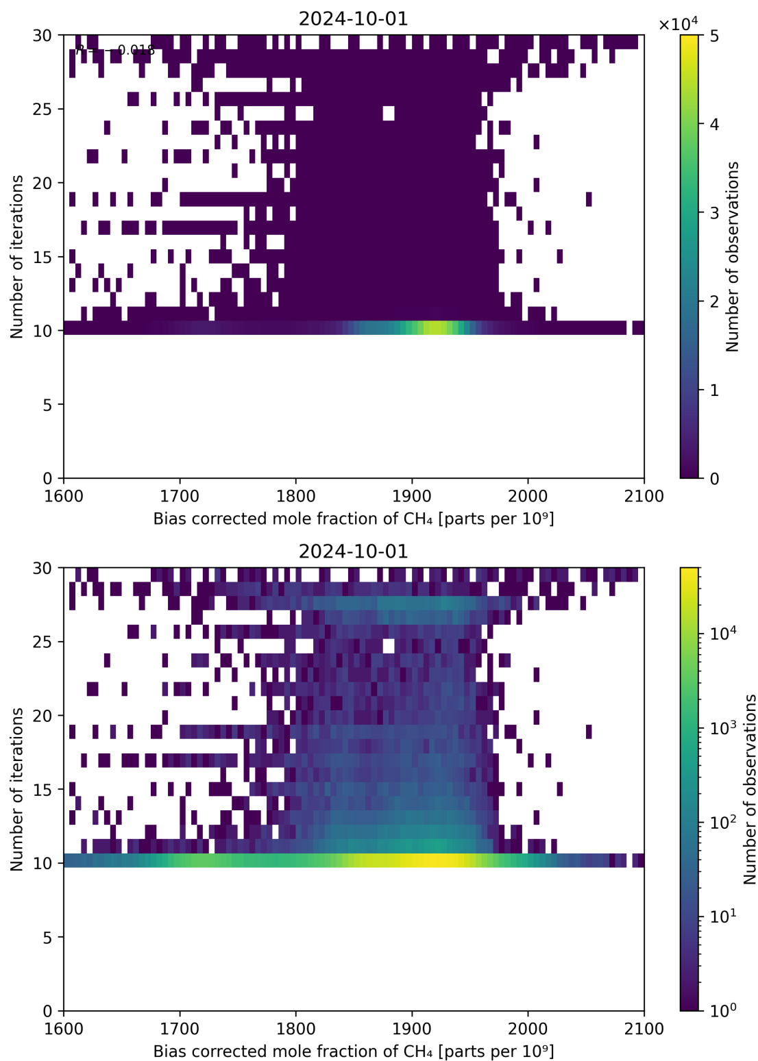
Figure 67: Scatter density plot of “Bias corrected mole fraction of CH 4 ” against “Number of iterations” for 2024-09-30 to 2024-10-02.
