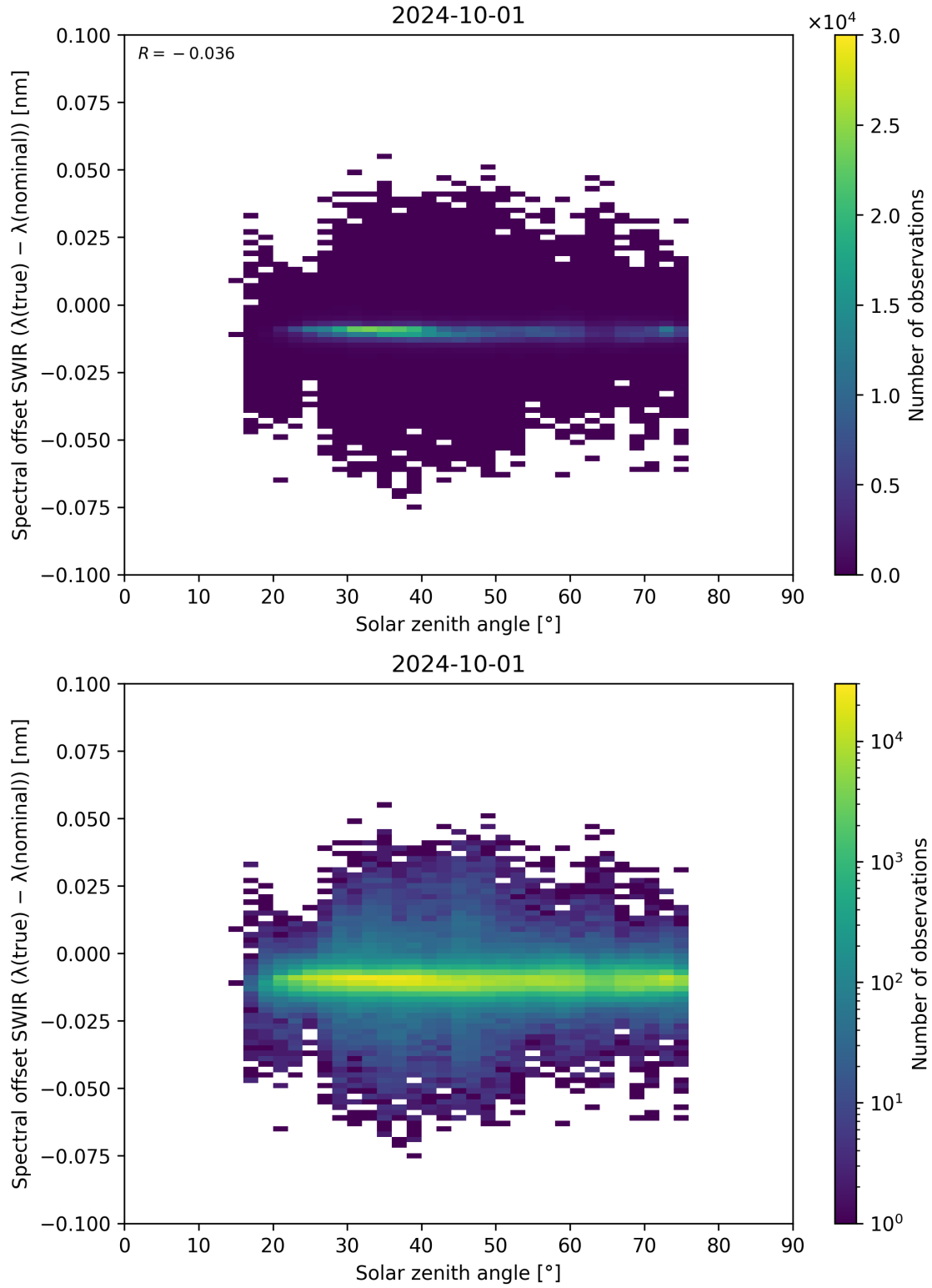
Figure 104: Scatter density plot of “Solar zenith angle” against “Spectral offset SWIR ( \lambda_{\text{true}} - \lambda_{\text{nominal}} )” for 2024-09-30 to 2024-10-02.
