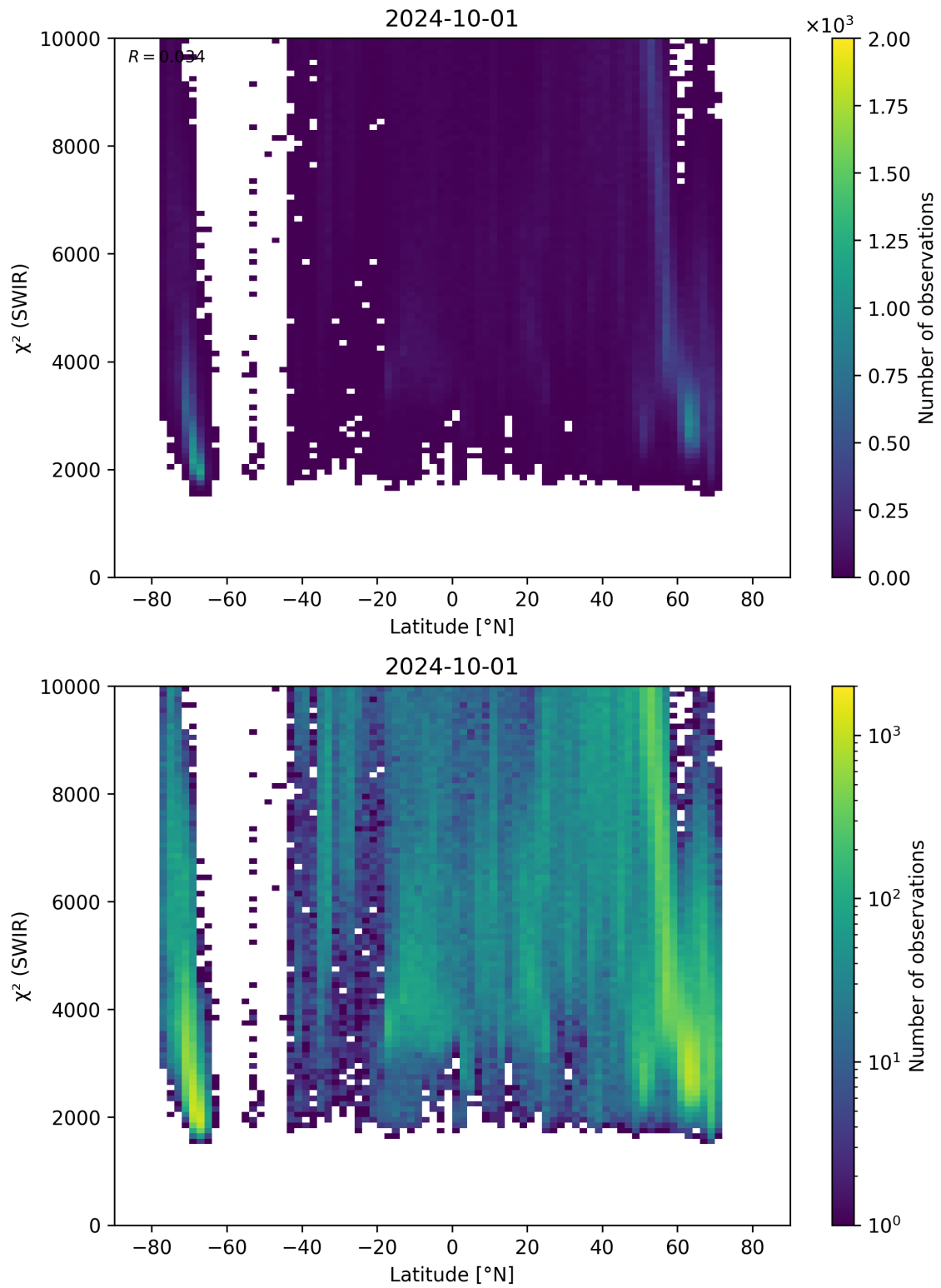
Figure 54: Scatter density plot of “Latitude” against “ \chi^2 (SWIR)” for 2024-09-30 to 2024-10-02.
