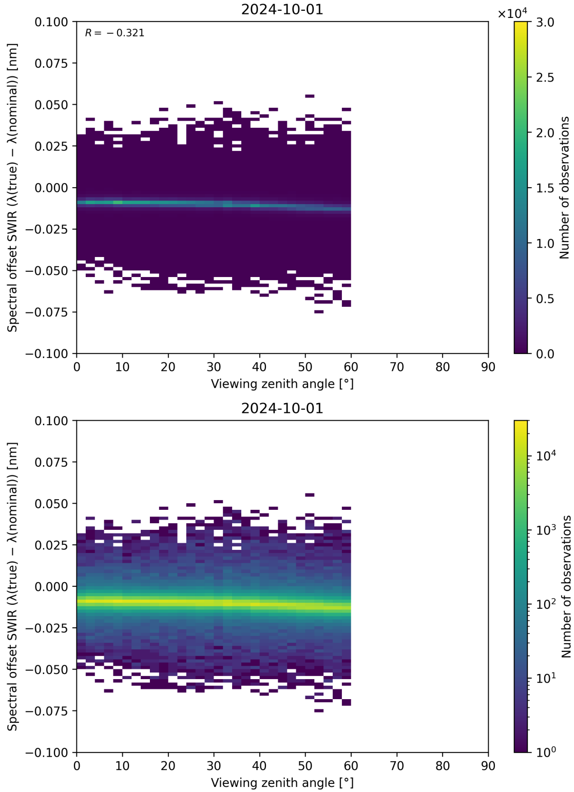
Figure 116: Scatter density plot of “Viewing zenith angle” against “Spectral offset SWIR ( \lambda_{\text{true}} - \lambda_{\text{nominal}} )” for 2024-09-30 to 2024-10-02.
