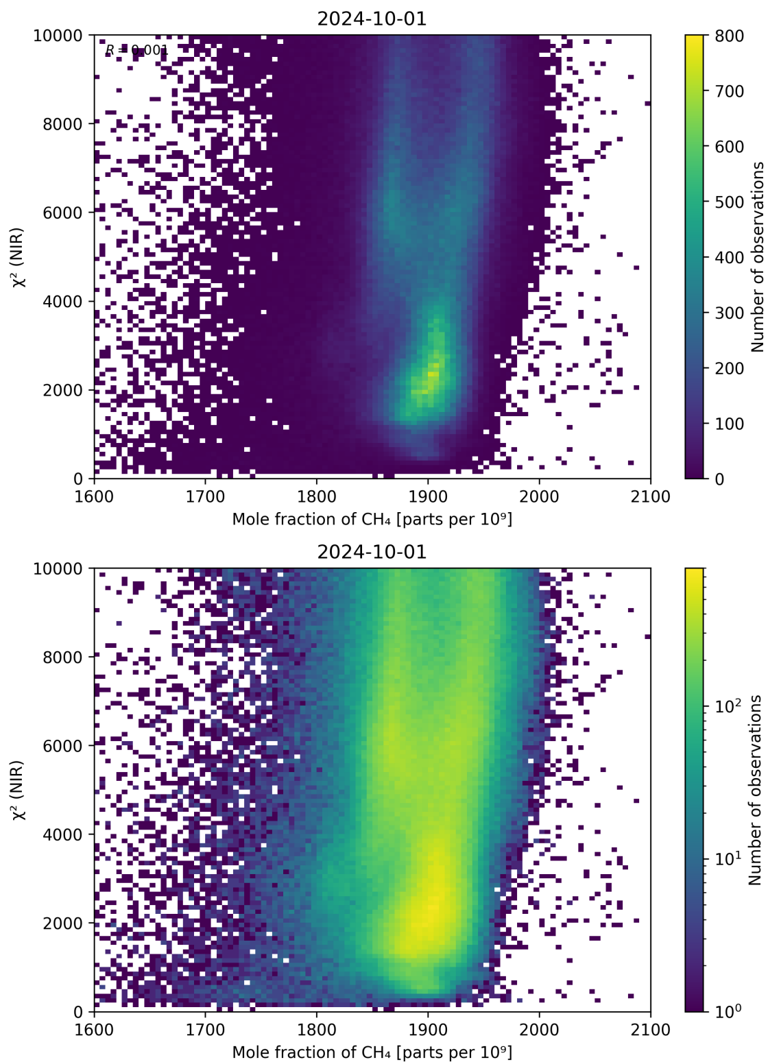
Figure 70: Scatter density plot of “Mole fraction of \text{CH}_4 ” against “ \chi^2 (NIR)” for 2024-09-30 to 2024-10-02.
