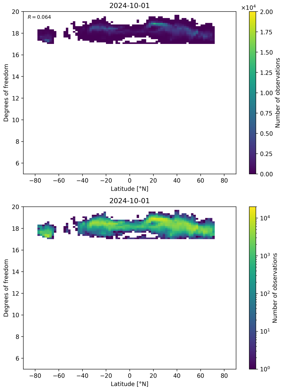
Figure 55: Scatter density plot of “Latitude” against “Degrees of freedom” for 2024-09-30 to 2024-10-02.
