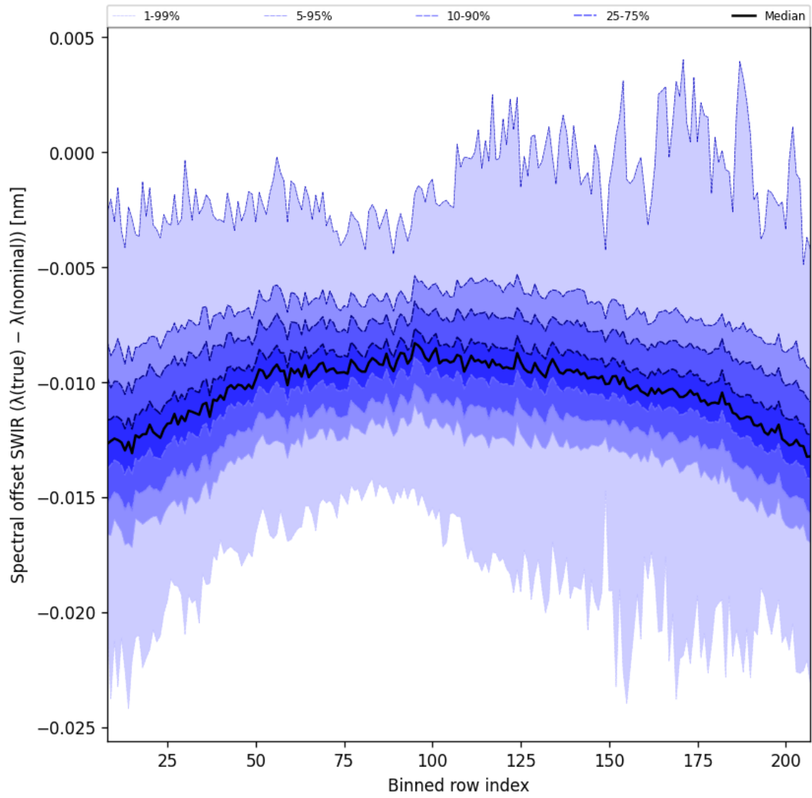
Figure 38: Along track statistics of “Spectral offset SWIR ( \lambda_{\text{true}} - \lambda_{\text{nominal}} )” for 2024-09-30 to 2024-10-02
