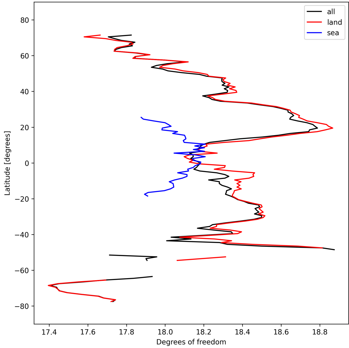
Figure 19: Zonal average of “Degrees of freedom” for 2024-09-30 to 2024-10-02.
