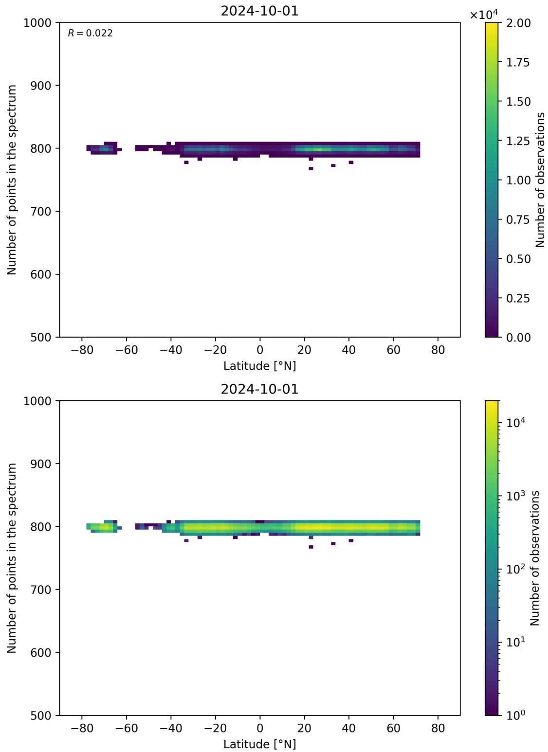
Figure 61: Scatter density plot of “Latitude” against “Number of points in the spectrum” for 2024-09-30 to 2024-10-02.
