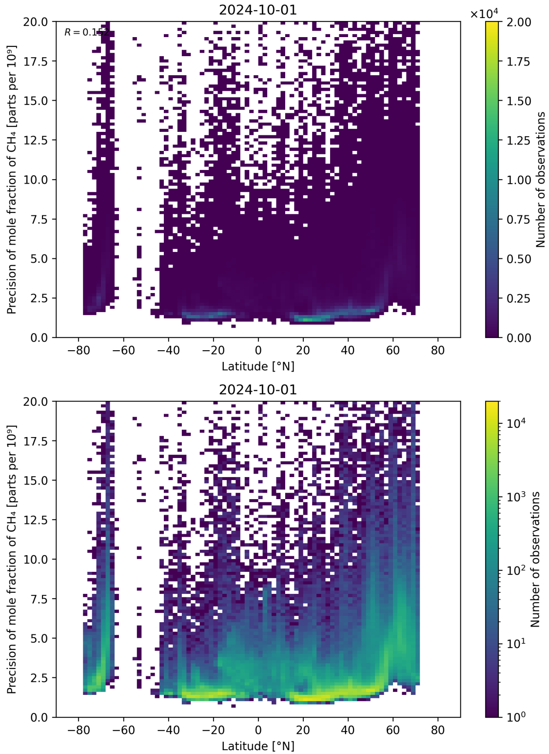
Figure 59: Scatter density plot of “Latitude” against “Precision of mole fraction of CH 4 ” for 2024-09-30 to 2024-10-02.
