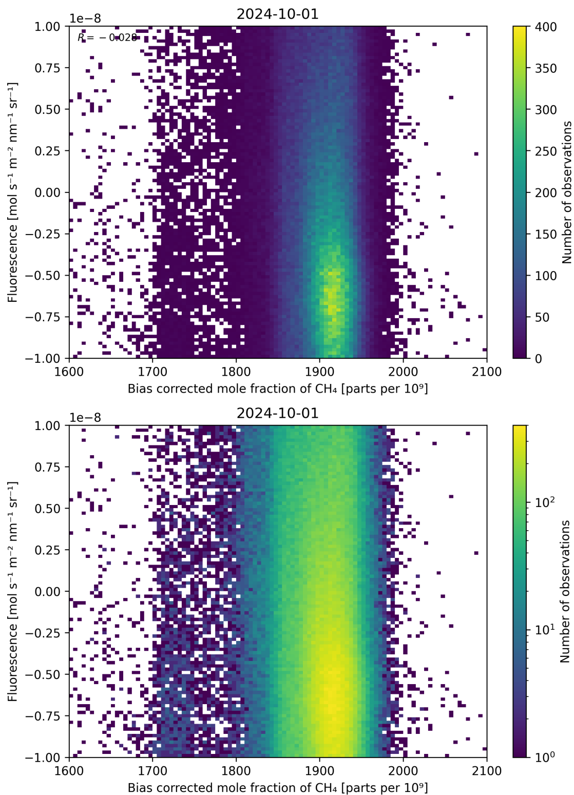
Figure 66: Scatter density plot of “Bias corrected mole fraction of CH 4 ” against “Fluorescence” for 2024-09-30 to 2024-10-02.
