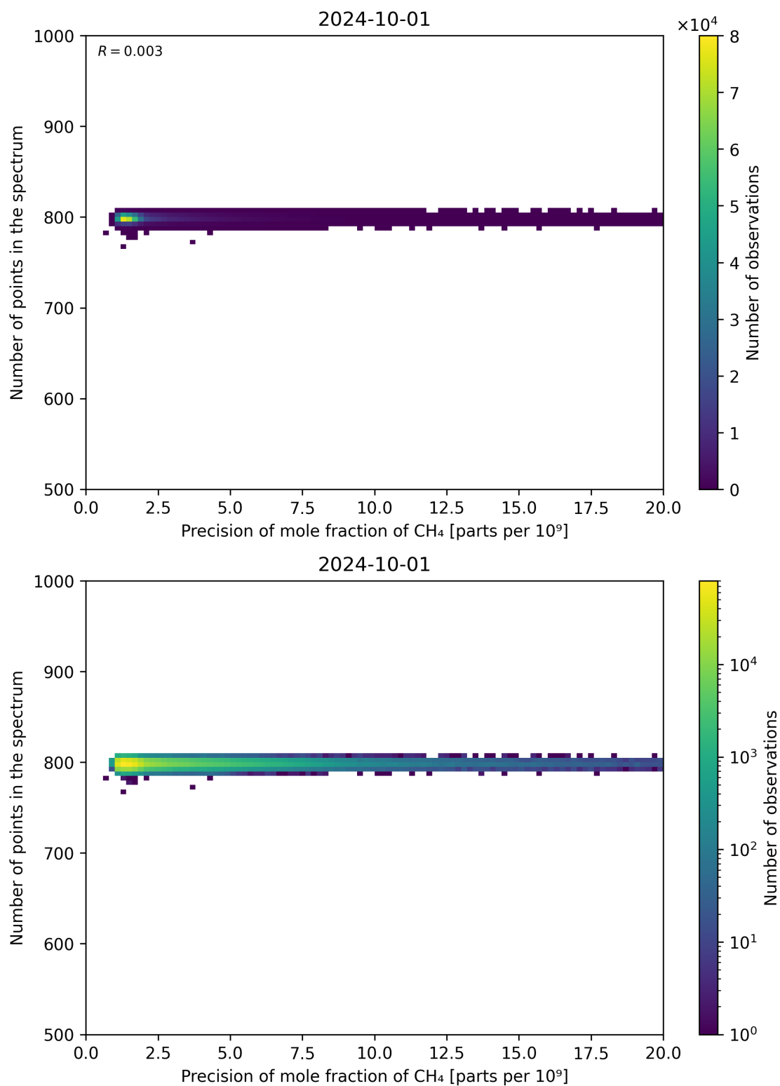
Figure 84: Scatter density plot of “Precision of mole fraction of CH 4 ” against “Number of points in the spectrum” for 2024-09-30 to 2024-10-02.
