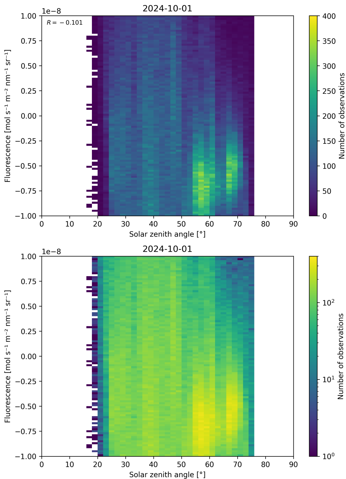
Figure 97: Scatter density plot of “Solar zenith angle” against “Fluorescence” for 2024-09-30 to 2024-10-02.
