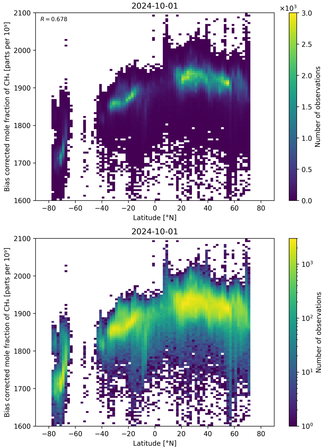
Figure 58: Scatter density plot of “Latitude” against “Bias corrected mole fraction of CH 4 ” for 2024-09-30 to 2024-10-02.
