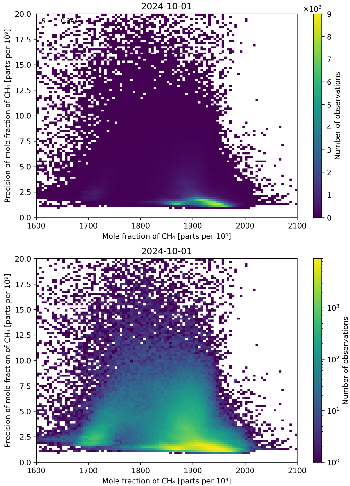
Figure 75: Scatter density plot of “Mole fraction of CH 4 ” against “Precision of mole fraction of CH 4 ” for 2024-09-30 to 2024-10-02.
