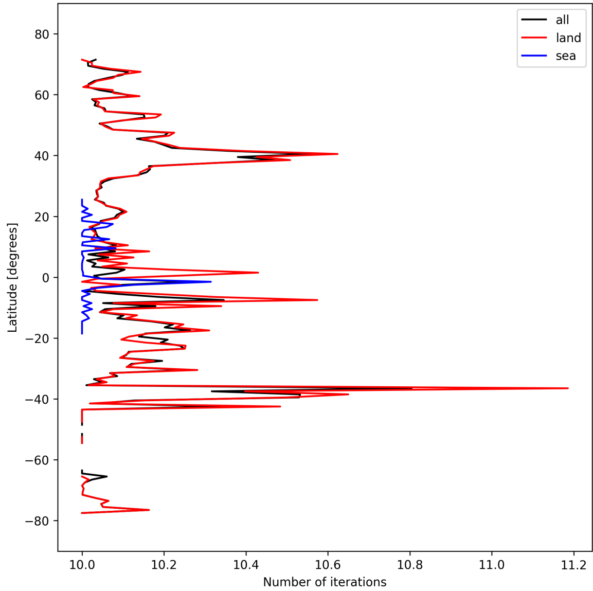
Figure 20: Zonal average of “Number of iterations” for 2024-09-30 to 2024-10-02.
