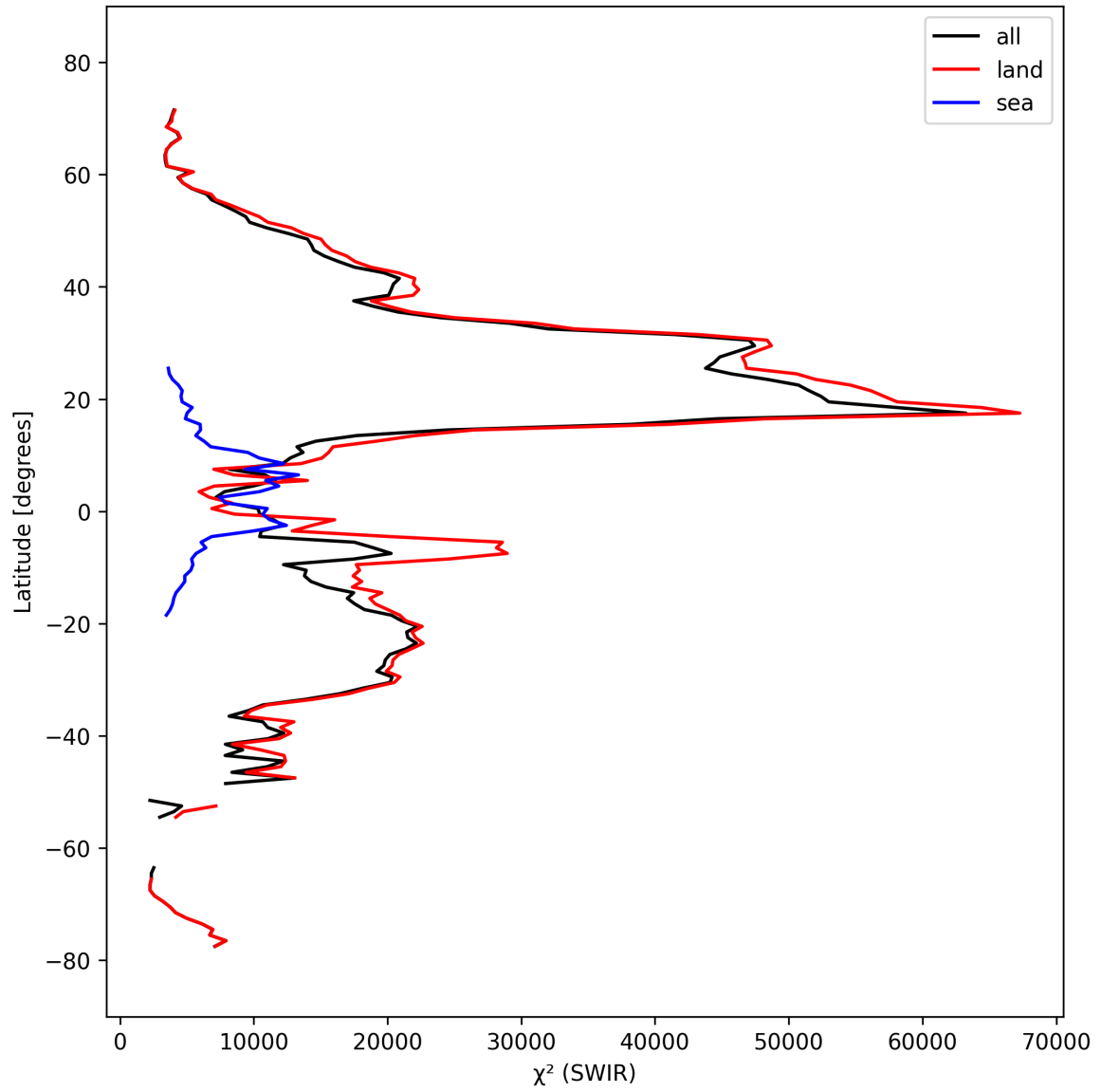
Figure 17: Zonal average of “ \chi^2 (SWIR)” for 2024-09-30 to 2024-10-02.
