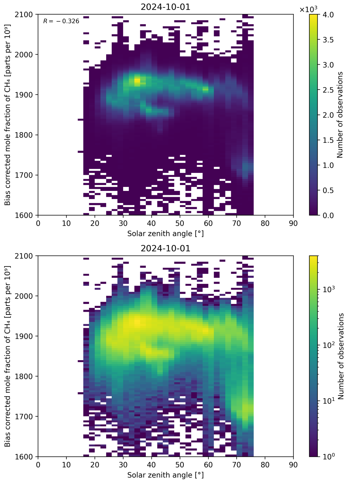
Figure 100: Scatter density plot of “Solar zenith angle” against “Bias corrected mole fraction of CH 4 ” for 2024-09-30 to 2024-10-02.
