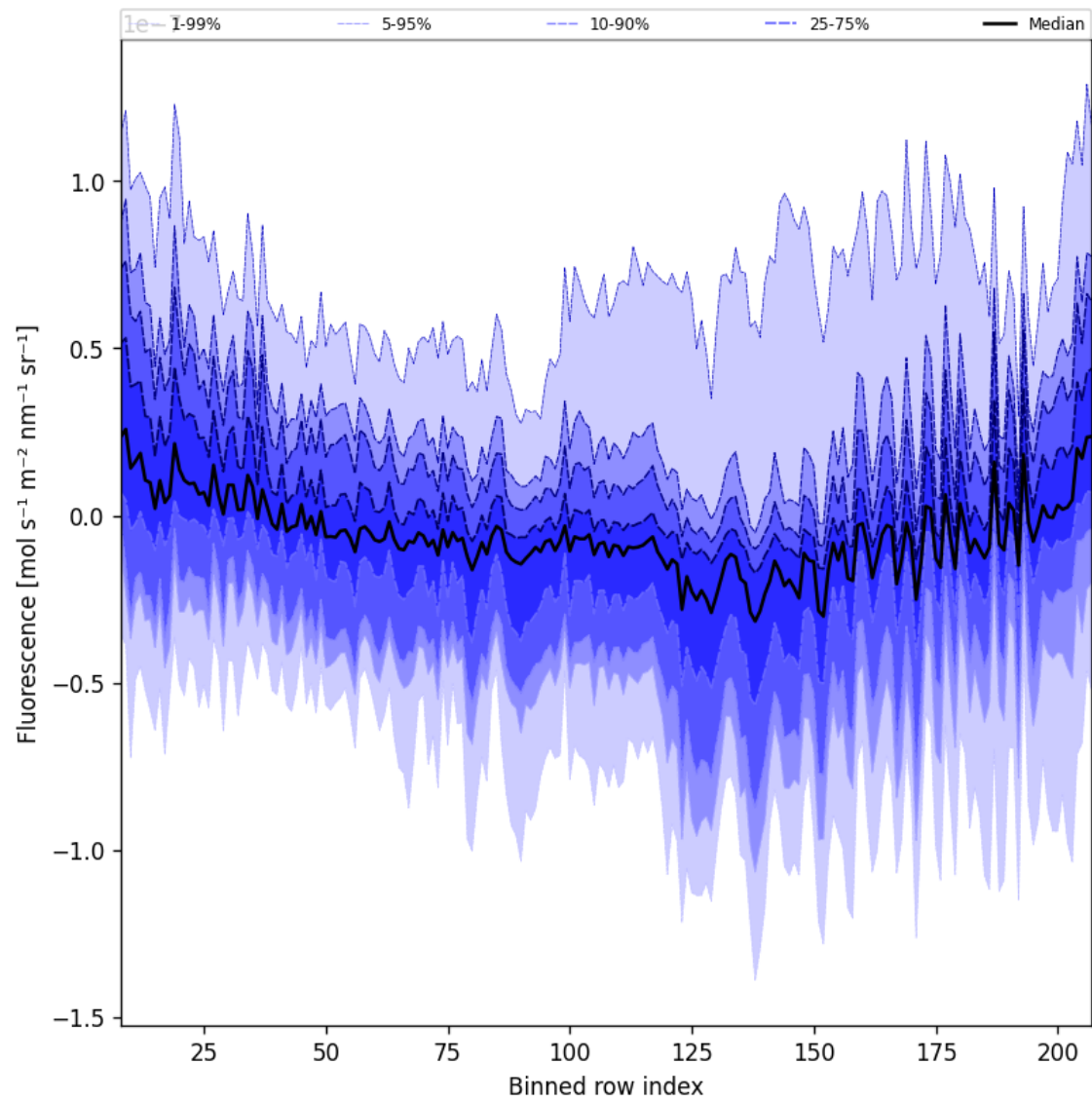
Figure 43: Along track statistics of “Fluorescence” for 2024-09-30 to 2024-10-02
