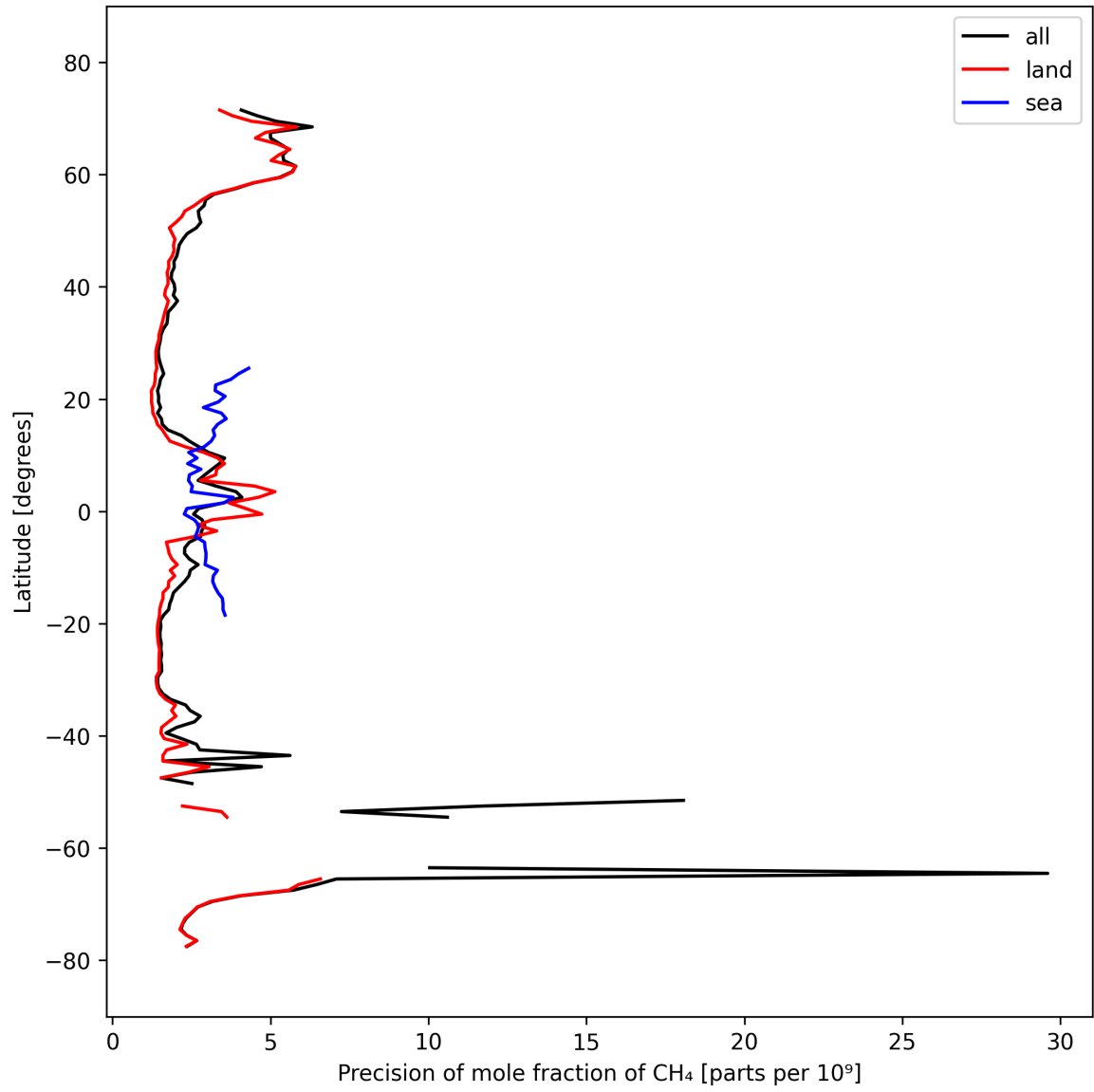
Figure 13: Zonal average of “Precision of mole fraction of CH 4 ” for 2024-09-30 to 2024-10-02.
