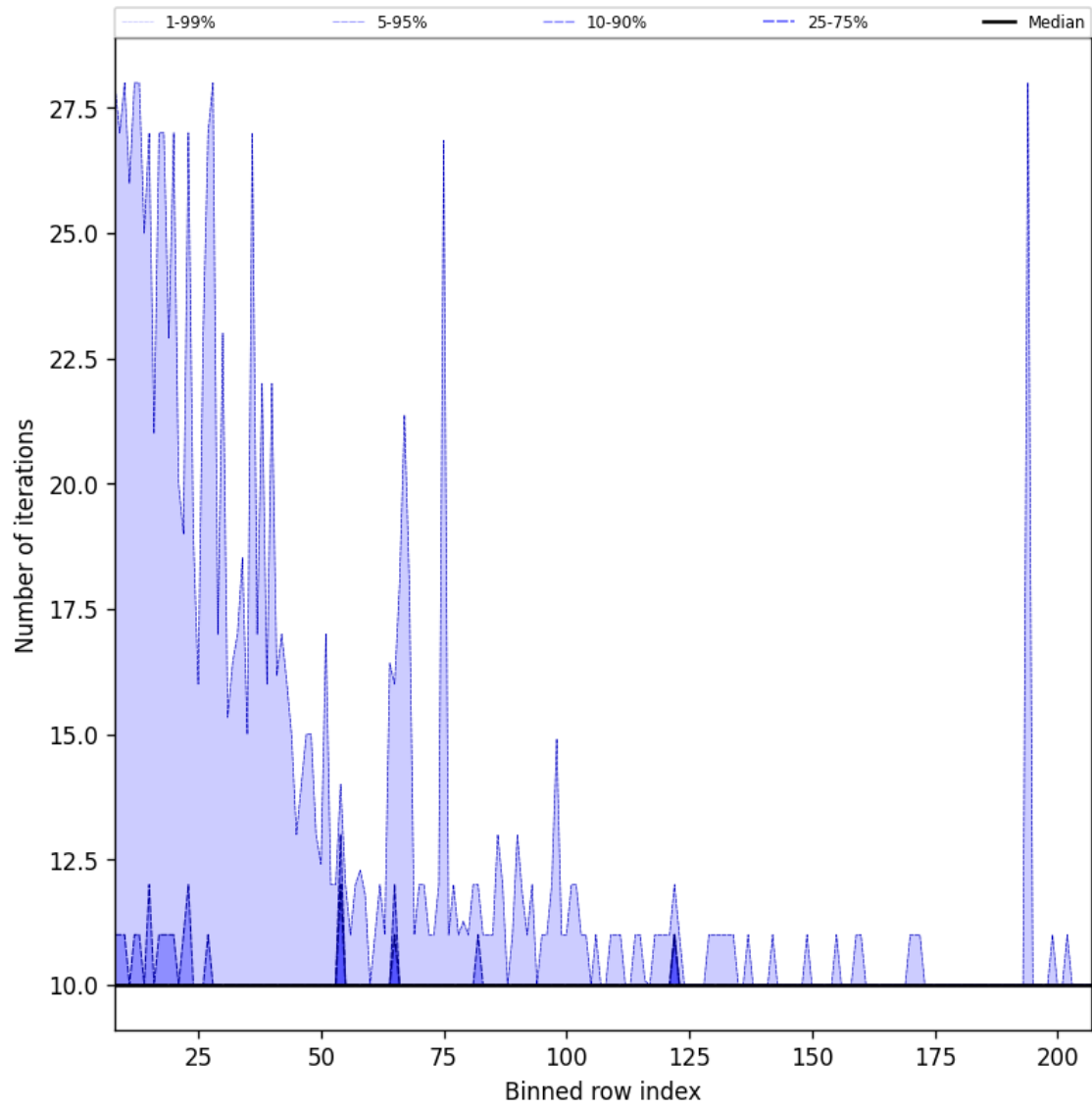
Figure 42: Along track statistics of “Number of iterations” for 2024-09-30 to 2024-10-02
