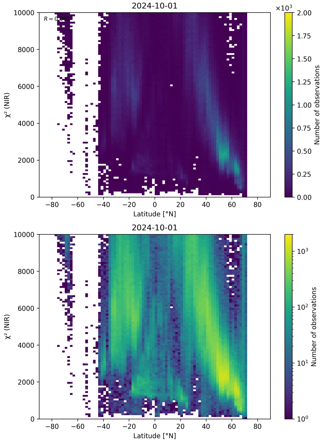
Figure 53: Scatter density plot of “Latitude” against “ \chi^2 (NIR)” for 2024-09-30 to 2024-10-02.
