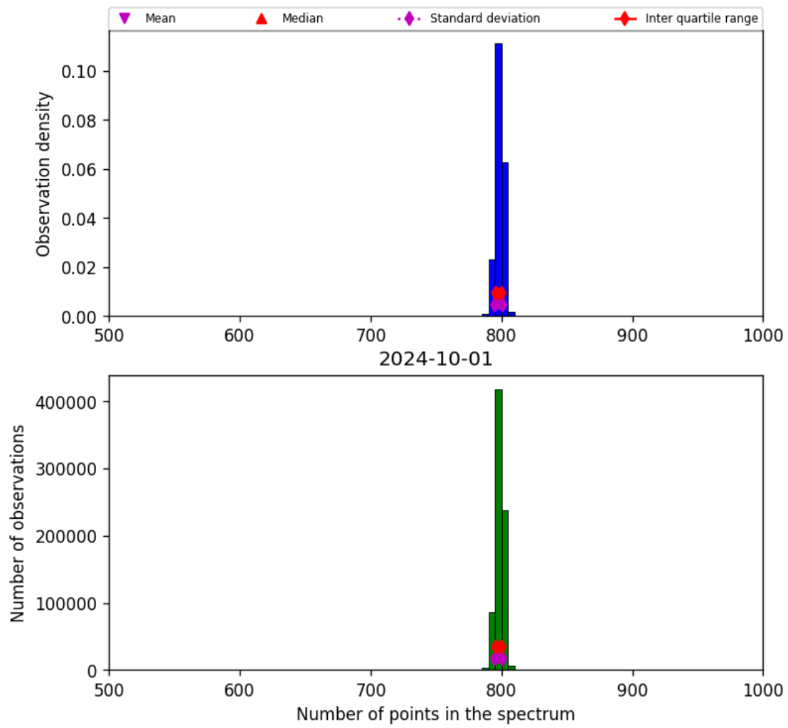
Figure 26: Histogram of “Number of points in the spectrum” for 2024-09-30 to 2024-10-02
