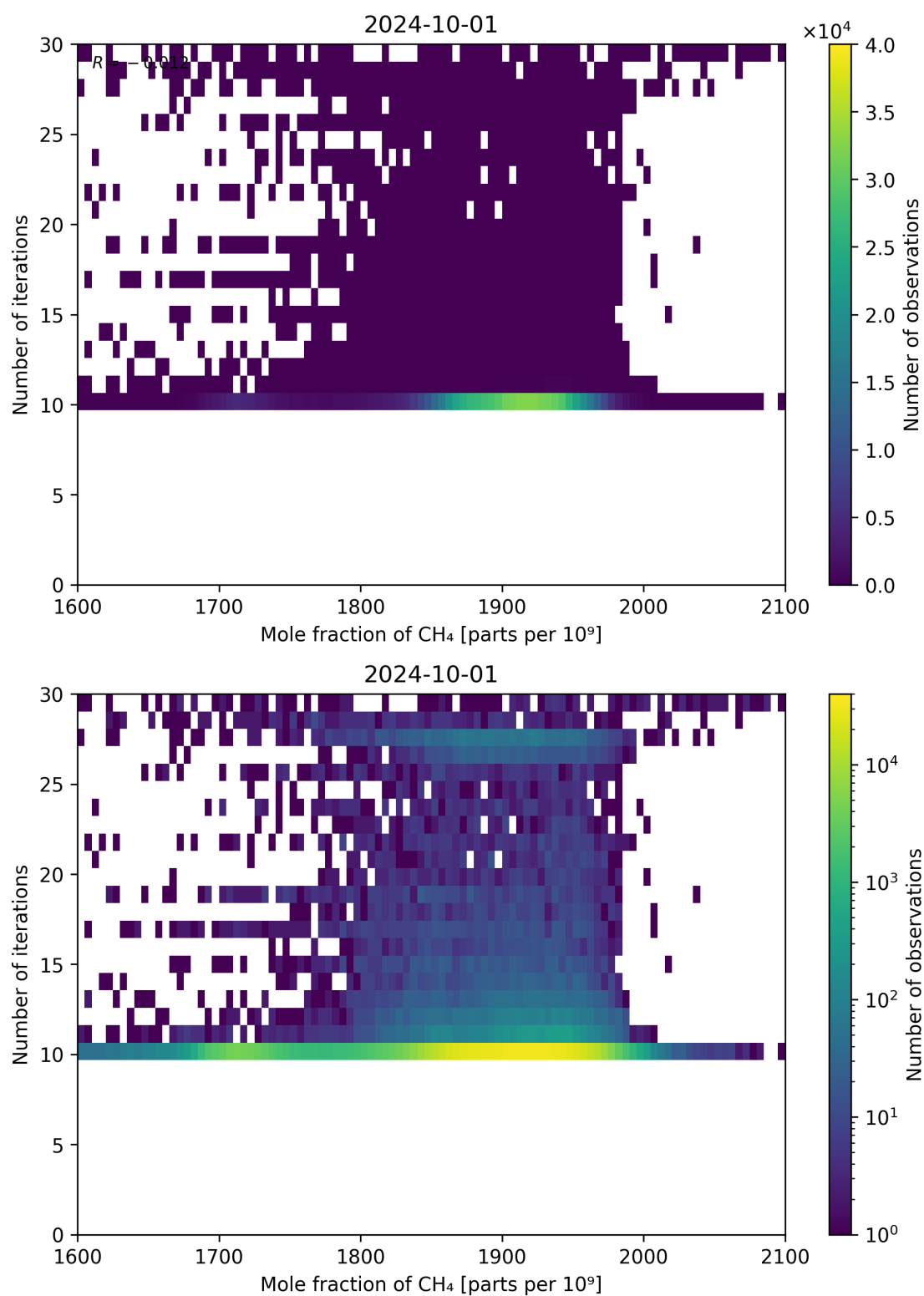
Figure 76: Scatter density plot of “Mole fraction of CH 4 ” against “Number of iterations” for 2024-09-30 to 2024-10-02.
