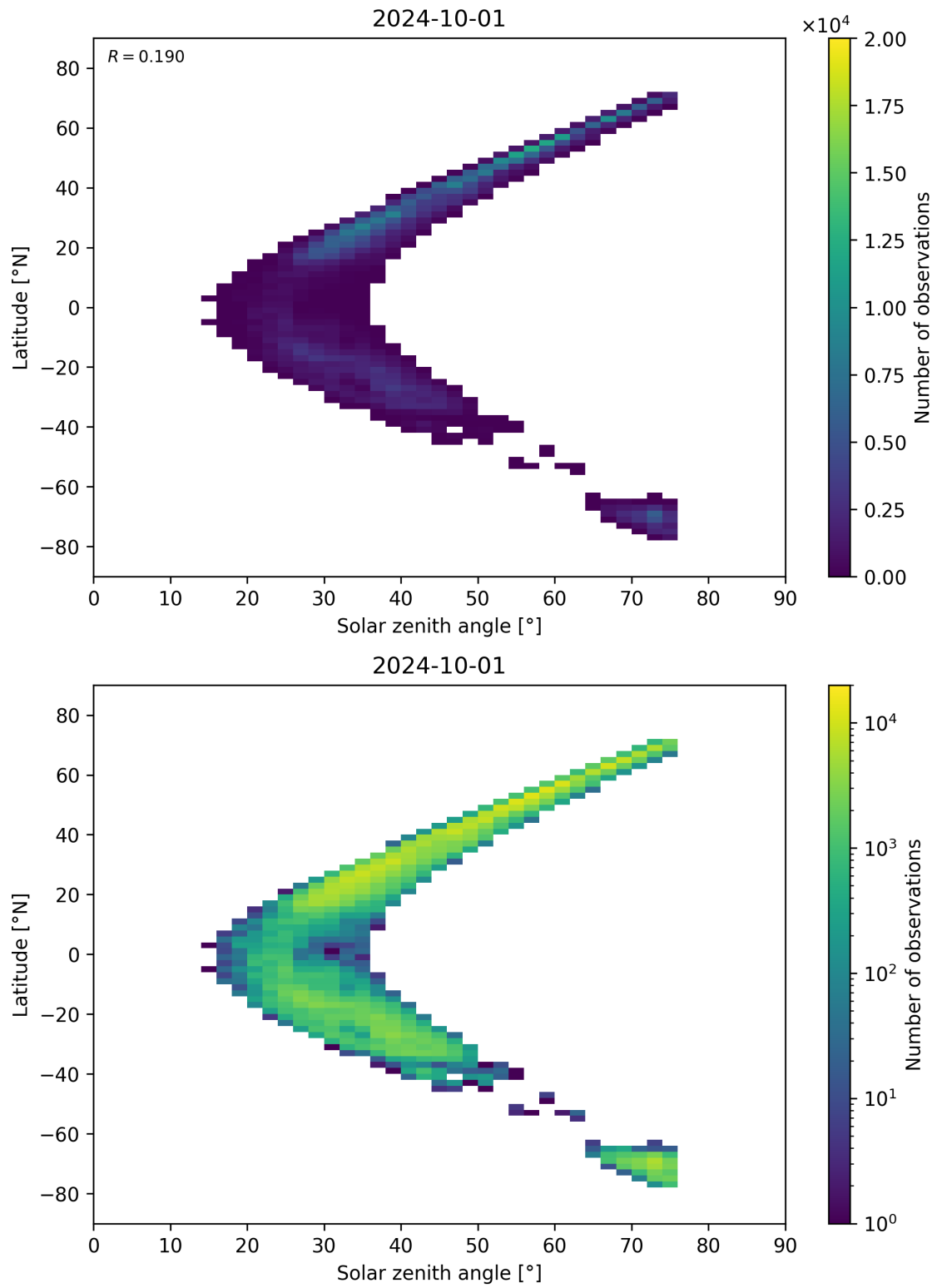
Figure 98: Scatter density plot of “Solar zenith angle” against “Latitude” for 2024-09-30 to 2024-10-02.
