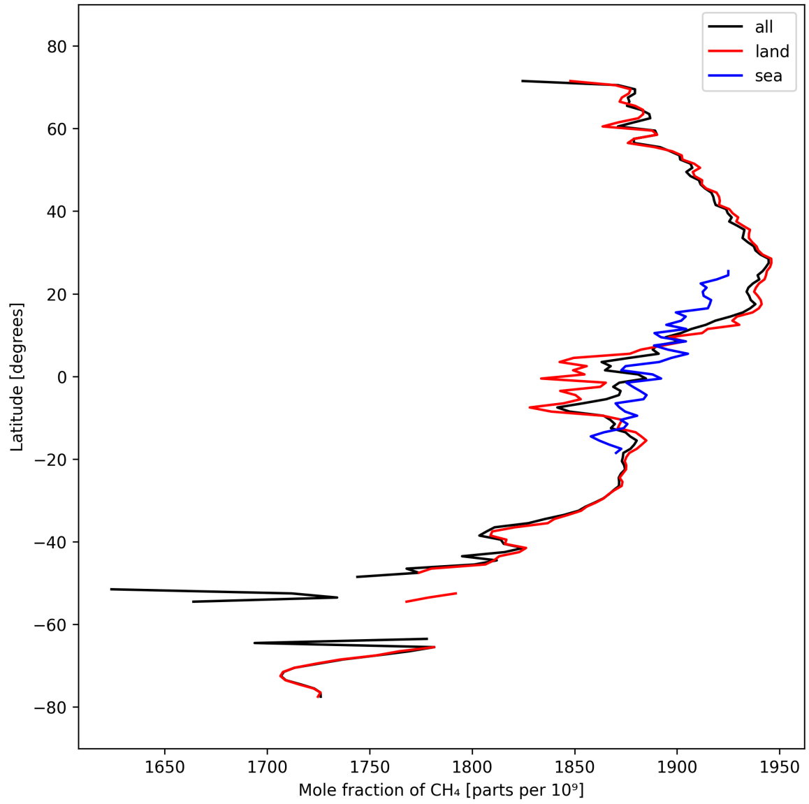
Figure 12: Zonal average of “Mole fraction of \text{CH}_4 ” for 2024-09-30 to 2024-10-02.
