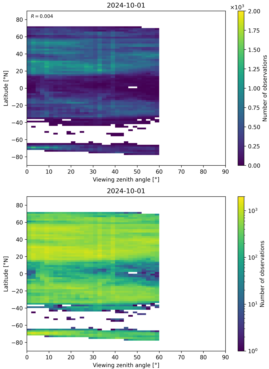
Figure 109: Scatter density plot of “Viewing zenith angle” against “Latitude” for 2024-09-30 to 2024-10-02.
