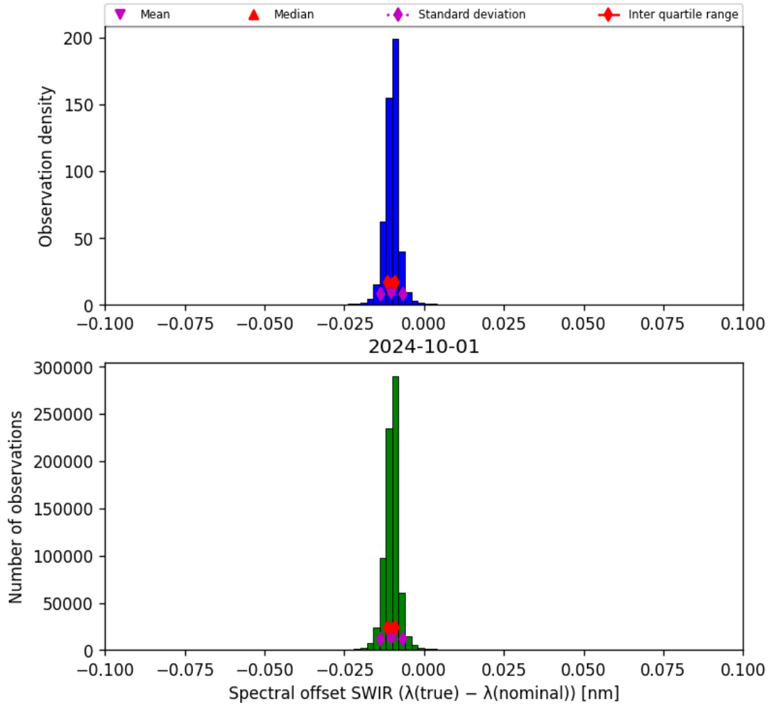
Figure 27: Histogram of “Spectral offset SWIR ( \lambda_{\text{true}} - \lambda_{\text{nominal}} )” for 2024-09-30 to 2024-10-02
