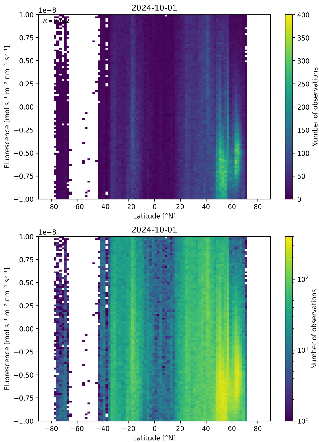
Figure 56: Scatter density plot of “Latitude” against “Fluorescence” for 2024-09-30 to 2024-10-02.
