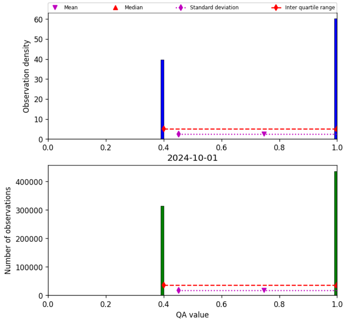
Figure 22: Histogram of “QA value” for 2024-09-30 to 2024-10-02
