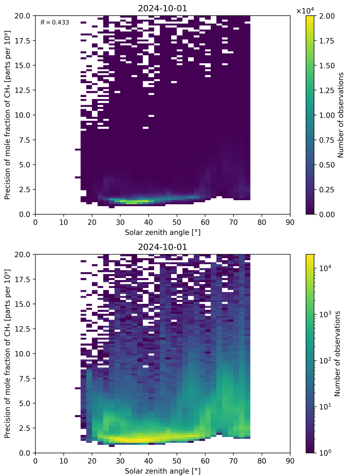
Figure 101: Scatter density plot of “Solar zenith angle” against “Precision of mole fraction of CH 4 ” for 2024-09-30 to 2024-10-02.
