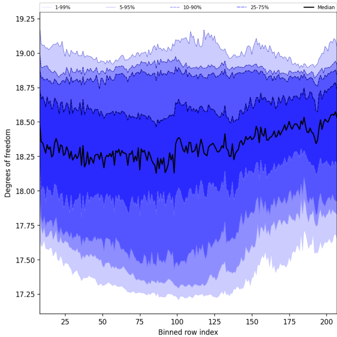
Figure 41: Along track statistics of “Degrees of freedom” for 2024-09-30 to 2024-10-02
