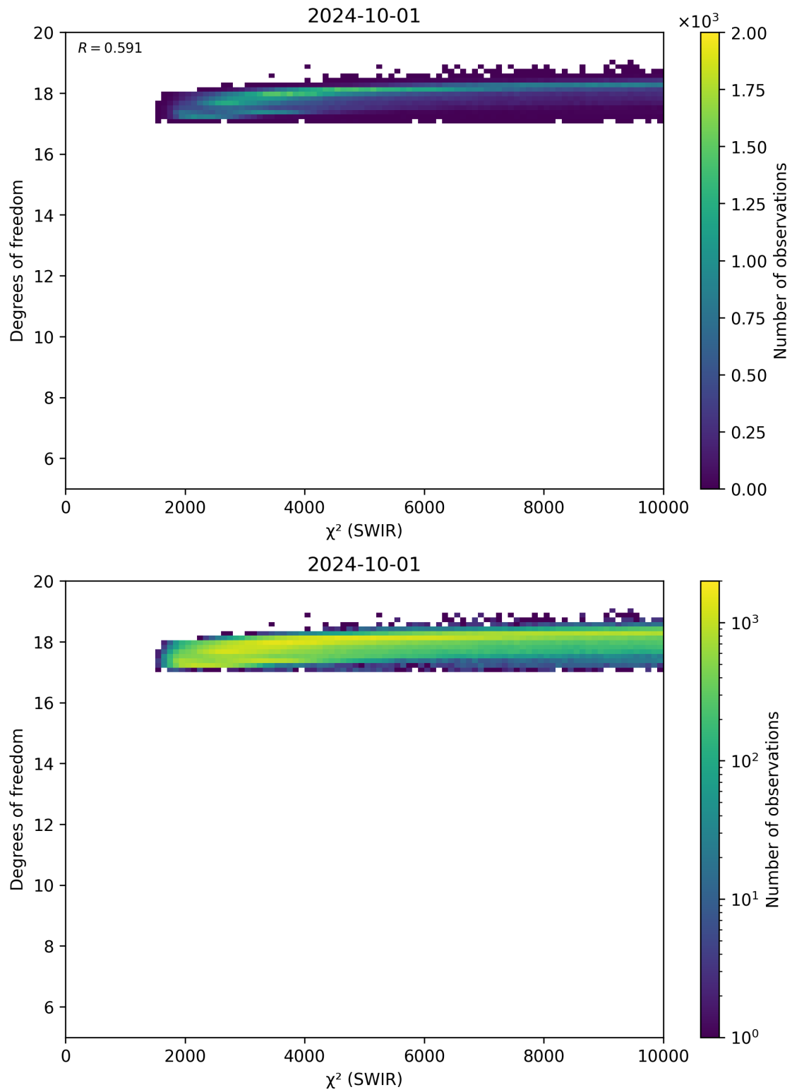
Figure 48: Scatter density plot of “ \chi^2 (SWIR)” against “Degrees of freedom” for 2024-09-30 to 2024-10-02.
