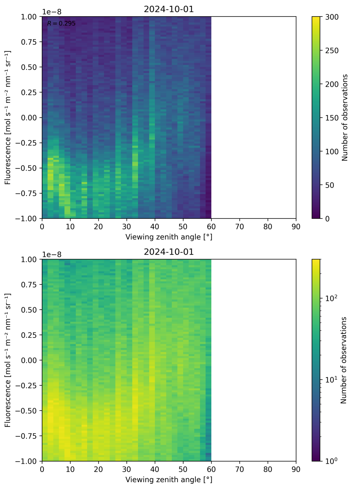
Figure 108: Scatter density plot of “Viewing zenith angle” against “Fluorescence” for 2024-09-30 to 2024-10-02.
