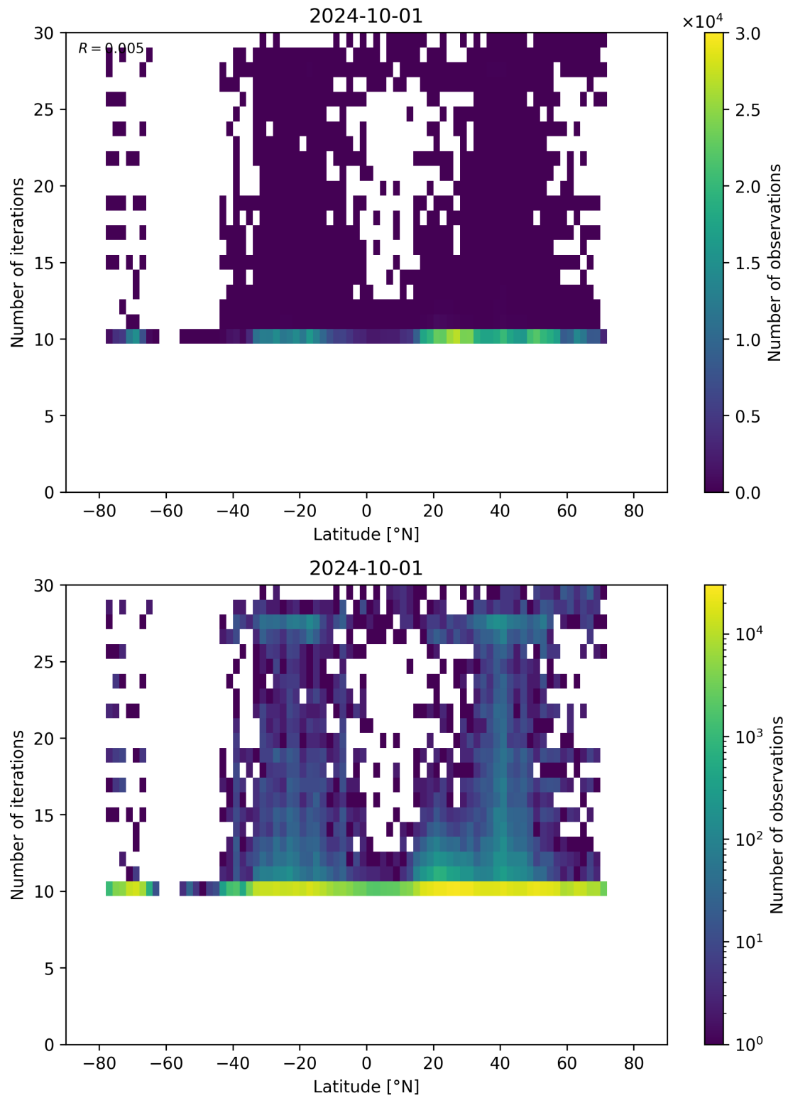
Figure 60: Scatter density plot of “Latitude” against “Number of iterations” for 2024-09-30 to 2024-10-02.
