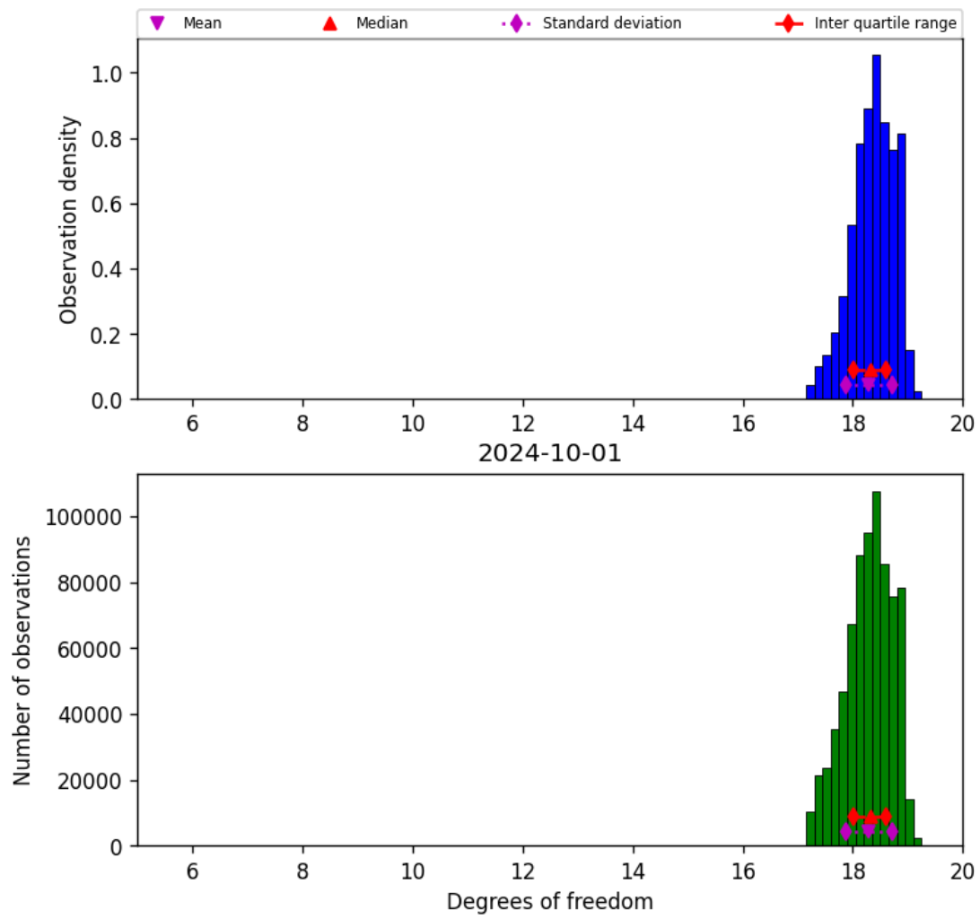
Figure 30: Histogram of “Degrees of freedom” for 2024-09-30 to 2024-10-02
