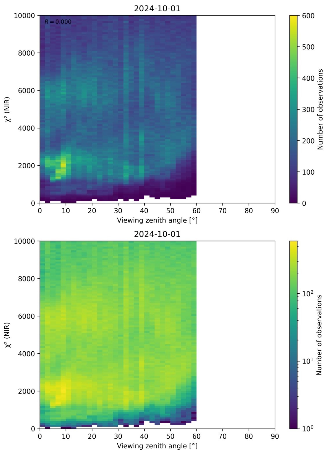
Figure 105: Scatter density plot of “Viewing zenith angle” against “ \chi^2 (NIR)” for 2024-09-30 to 2024-10-02.
