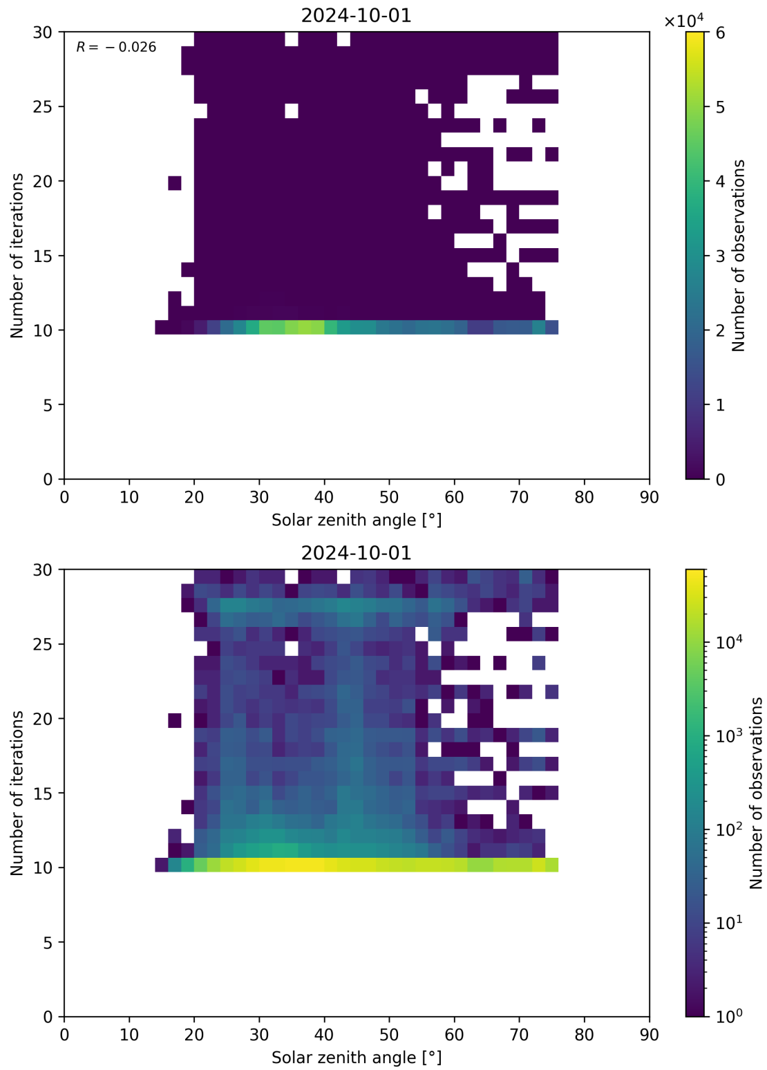
Figure 102: Scatter density plot of “Solar zenith angle” against “Number of iterations” for 2024-09-30 to 2024-10-02.
