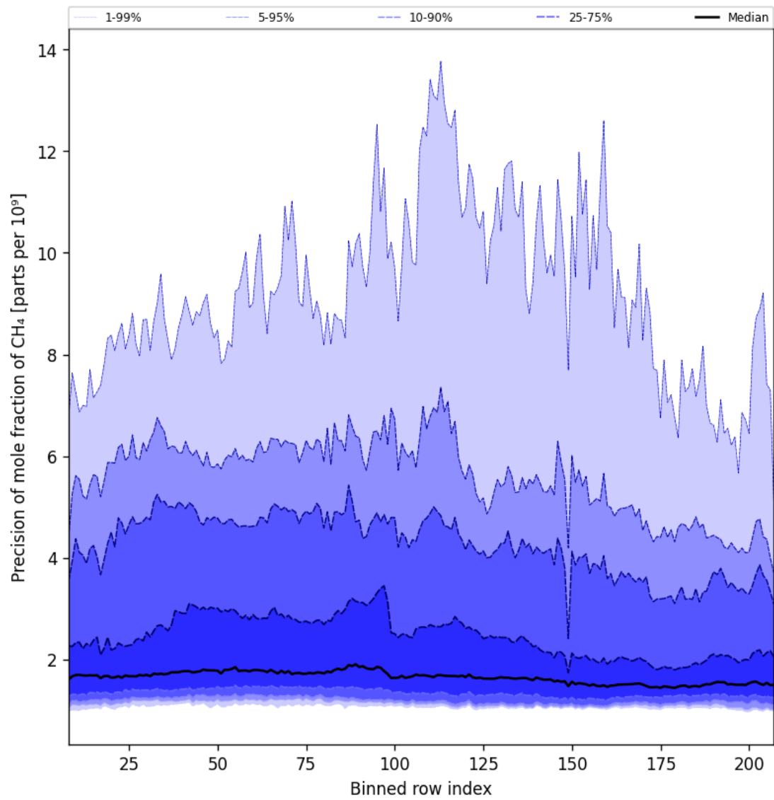
Figure 35: Along track statistics of “Precision of mole fraction of CH 4 ” for 2024-09-30 to 2024-10-02
