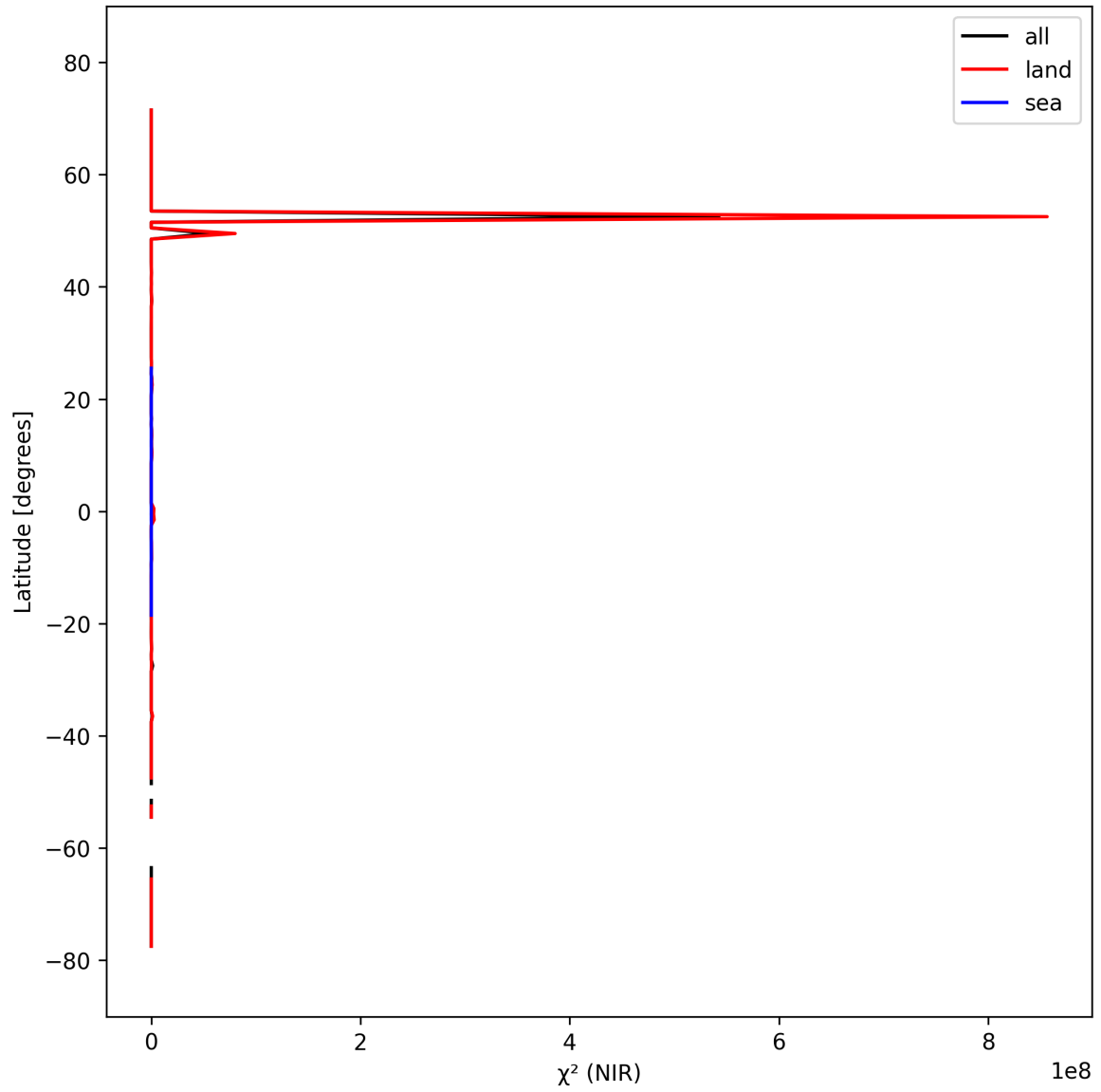
Figure 18: Zonal average of “ \chi^2 (NIR)” for 2024-09-30 to 2024-10-02.
