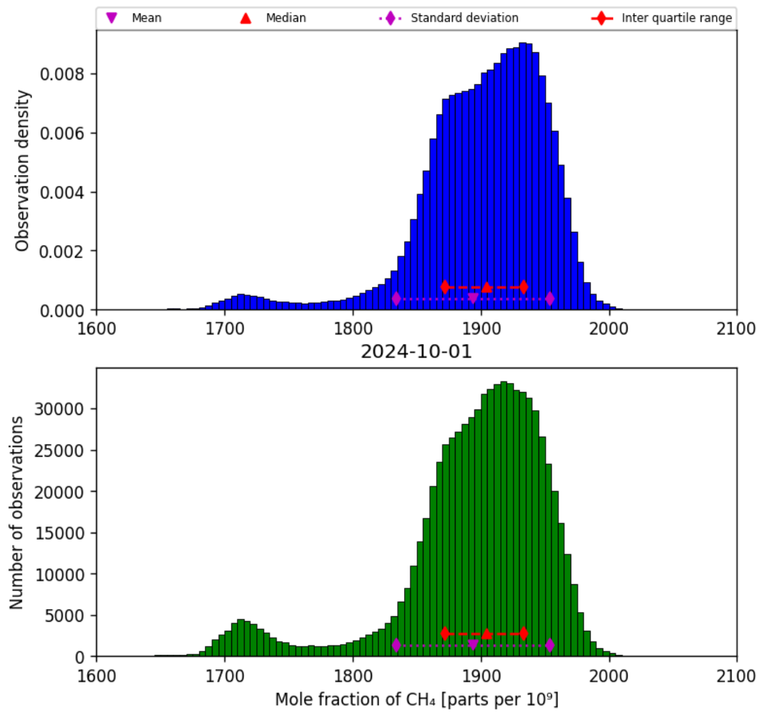
Figure 23: Histogram of “Mole fraction of CH 4 ” for 2024-09-30 to 2024-10-02
